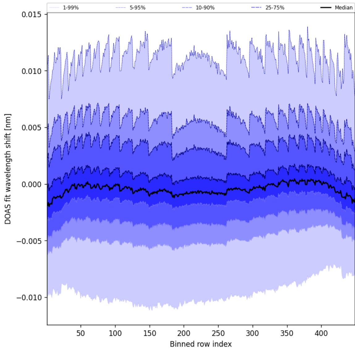
Figure 47: Along track statistics of “DOAS fit wavelength shift” for 2025-06-02 to 2025-06-03
