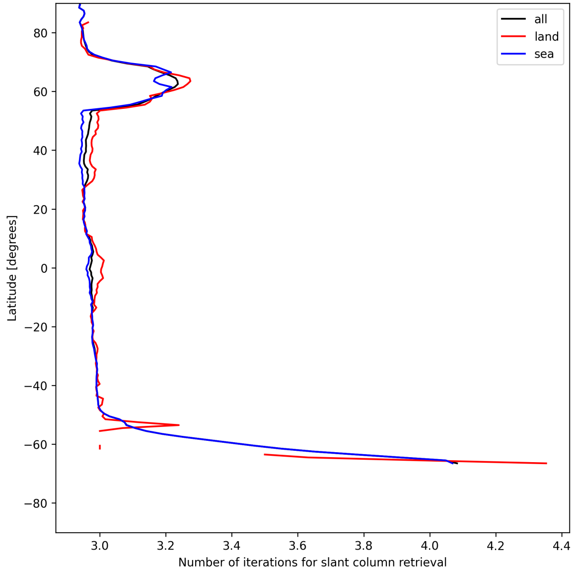
Figure 21: Zonal average of “Number of iterations for slant column retrieval” for 2025-06-02 to 2025-06-03.
