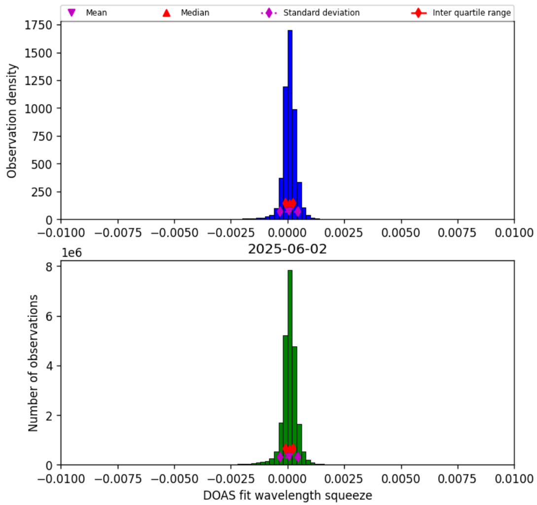
Figure 36: Histogram of “DOAS fit wavelength squeeze” for 2025-06-02 to 2025-06-03
