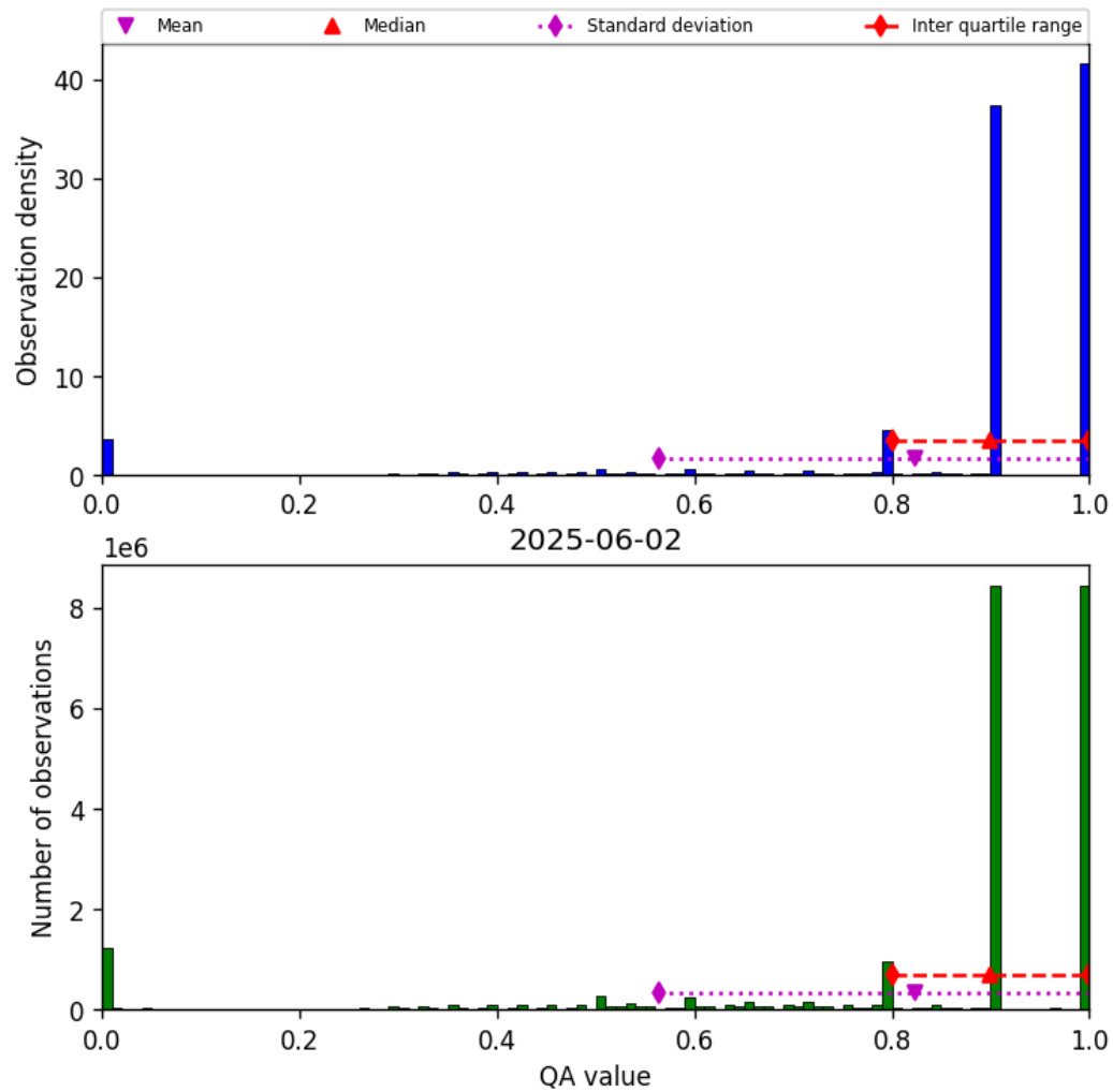
Figure 28: Histogram of “QA value” for 2025-06-02 to 2025-06-03
