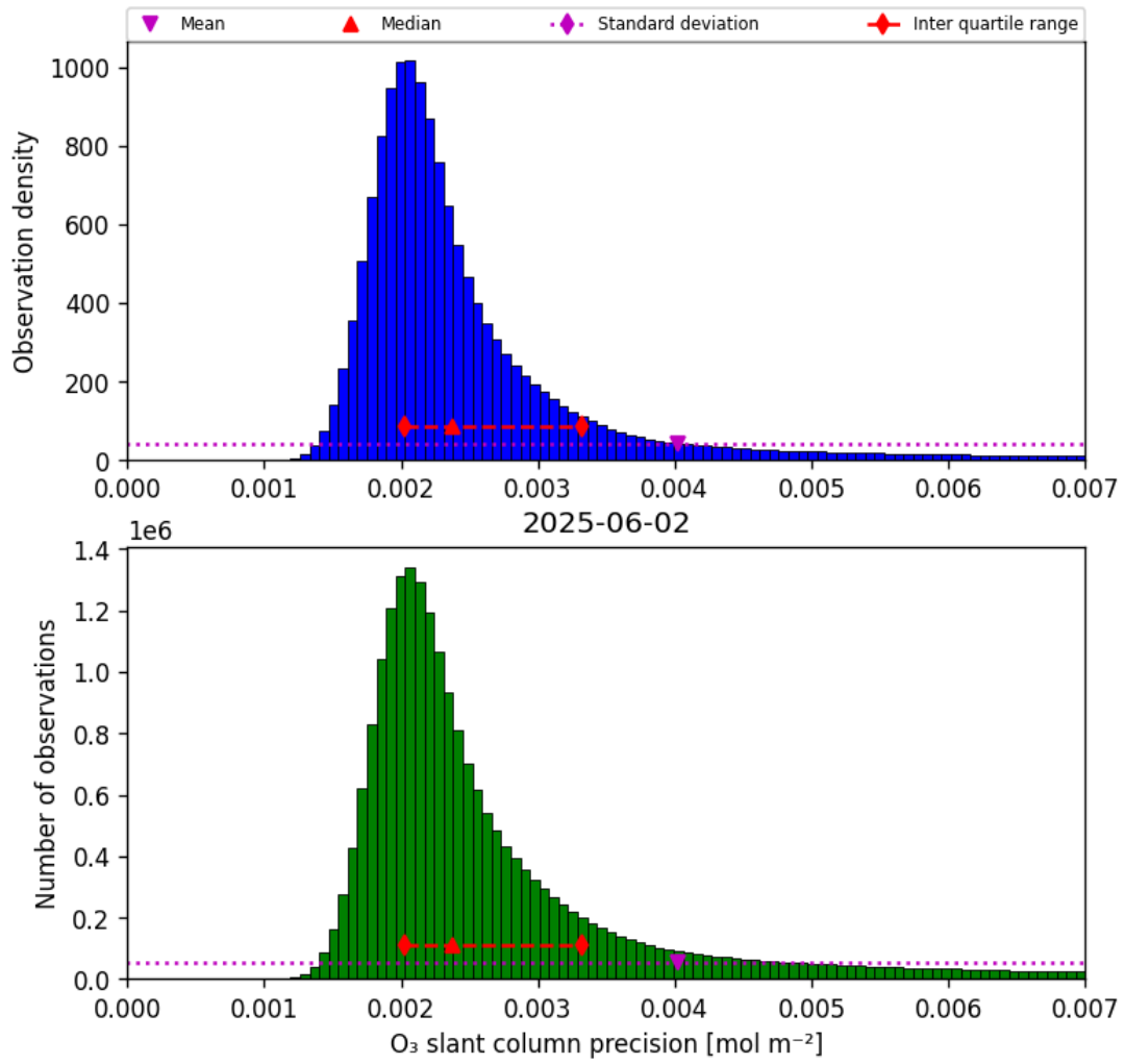
Figure 32: Histogram of “O 3 slant column precision” for 2025-06-02 to 2025-06-03
