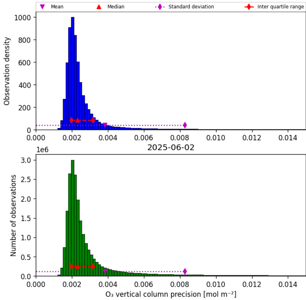
Figure 30: Histogram of "O 3 vertical column precision" for 2025-06-02 to 2025-06-03
