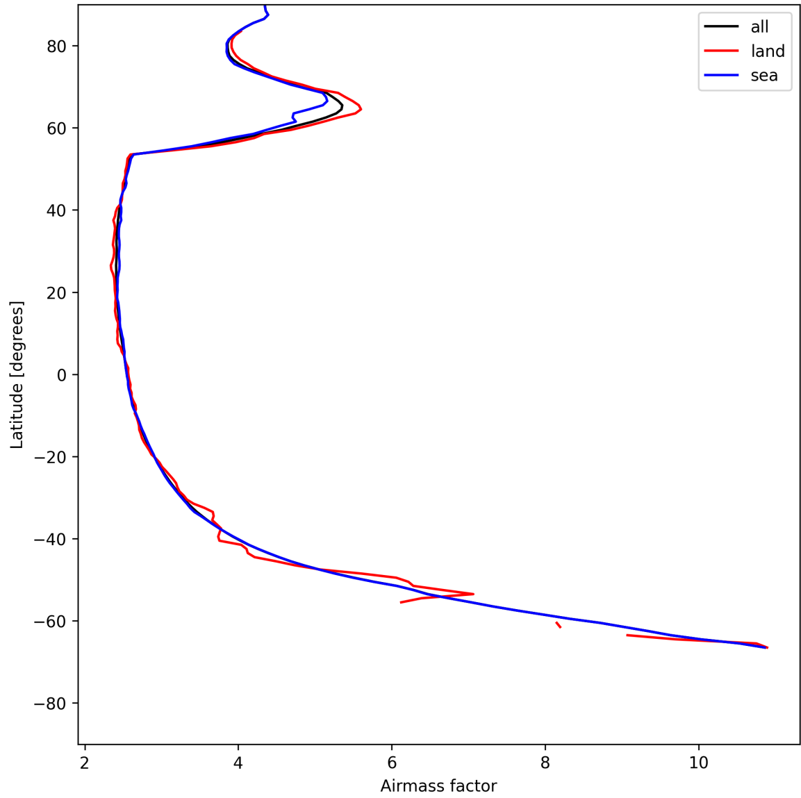
Figure 25: Zonal average of “Airmass factor” for 2025-06-02 to 2025-06-03.
