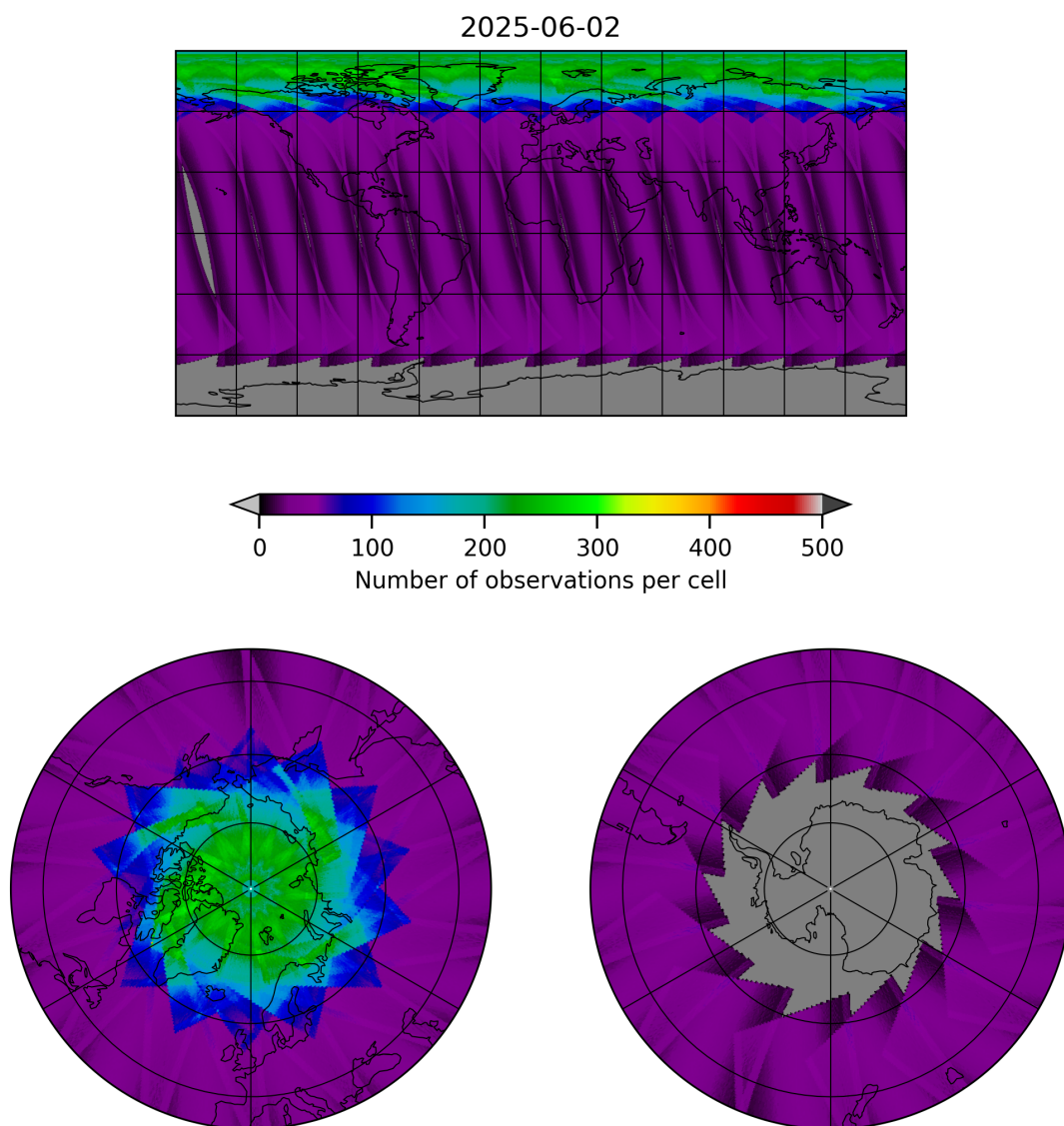
Figure 15: Map of the number of observations for 2025-06-02 to 2025-06-03
