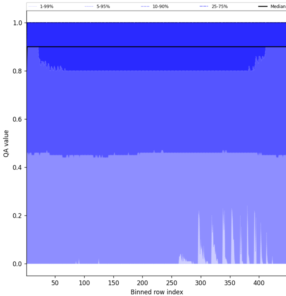
Figure 40: Along track statistics of “QA value” for 2025-06-02 to 2025-06-03
