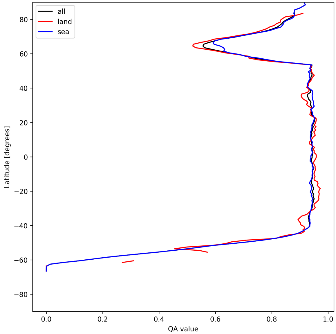
Figure 16: Zonal average of “QA value” for 2025-06-02 to 2025-06-03.
