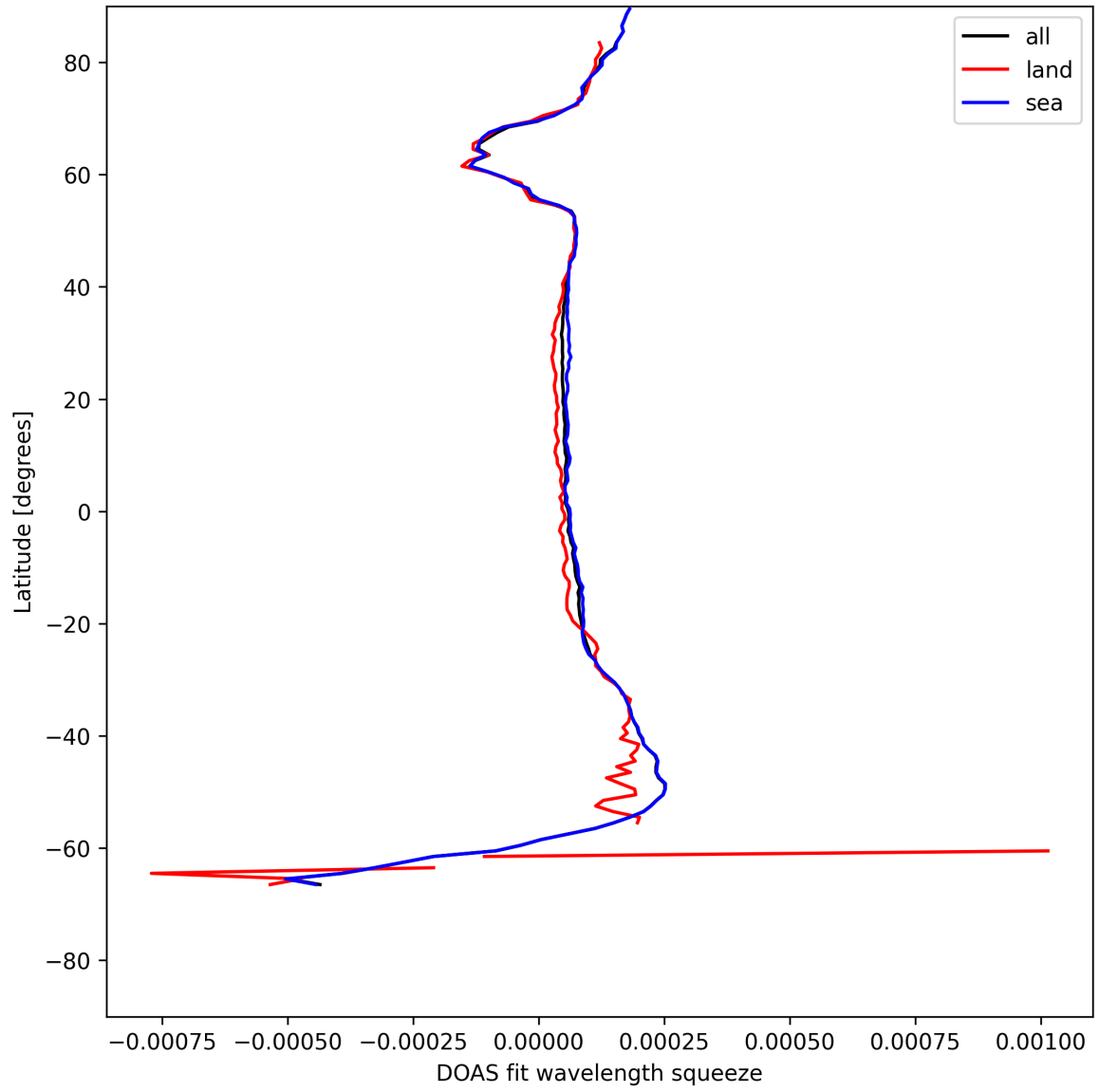
Figure 24: Zonal average of “DOAS fit wavelength squeeze” for 2025-06-02 to 2025-06-03.
