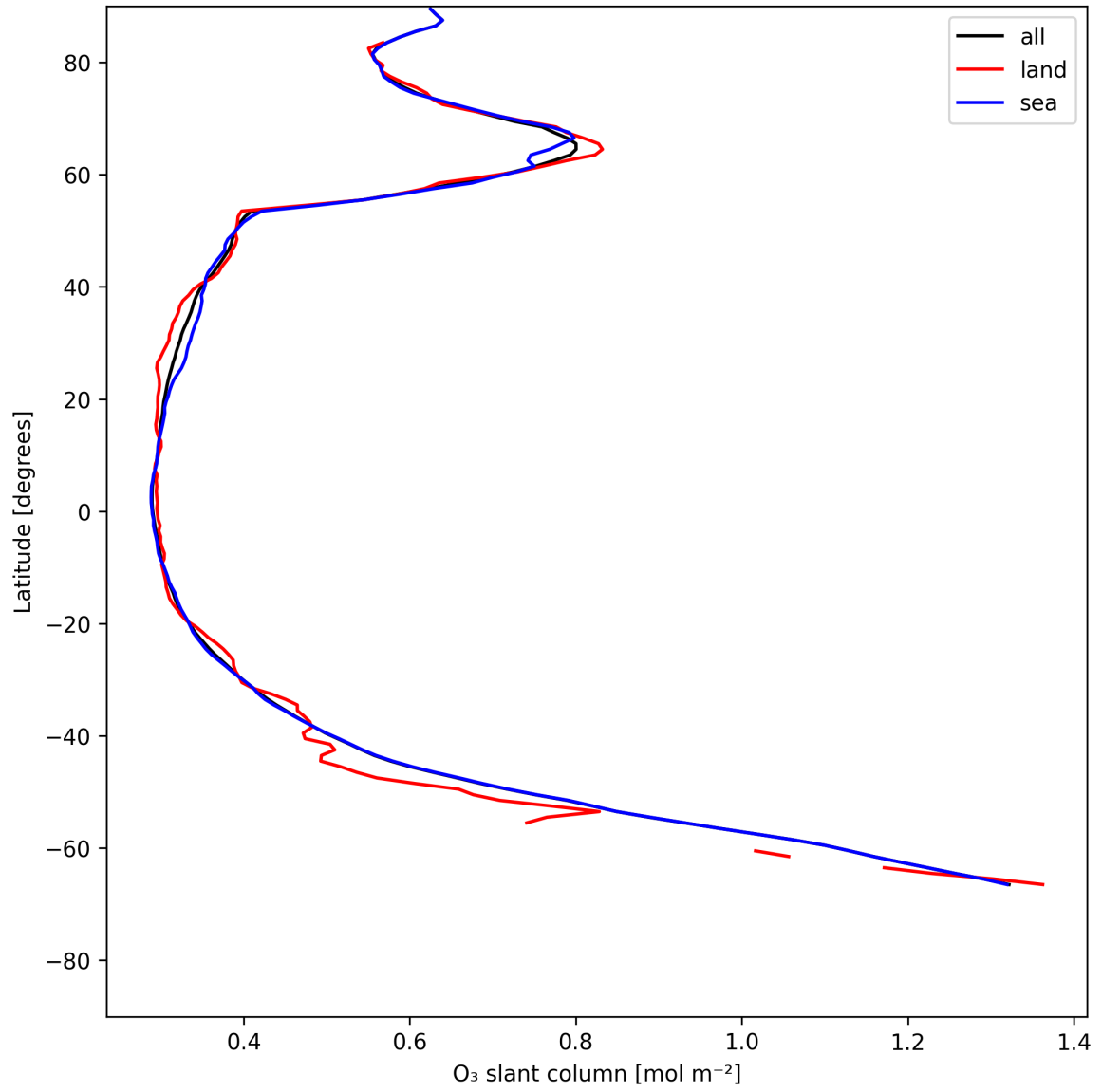
Figure 19: Zonal average of “O 3 slant column” for 2025-06-02 to 2025-06-03.
