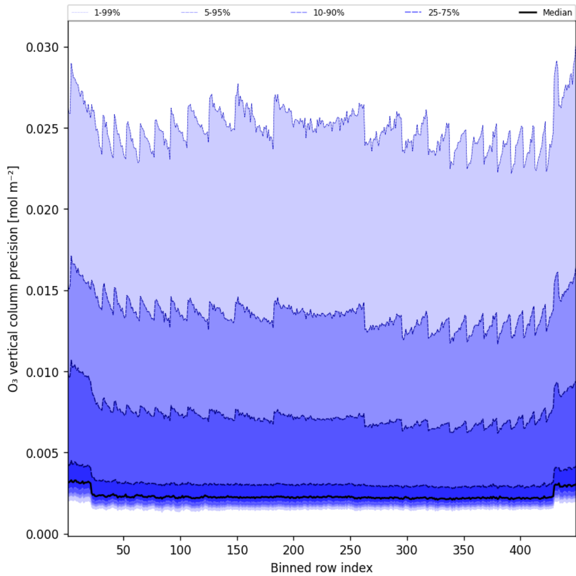
Figure 42: Along track statistics of “O 3 vertical column precision” for 2025-06-02 to 2025-06-03
