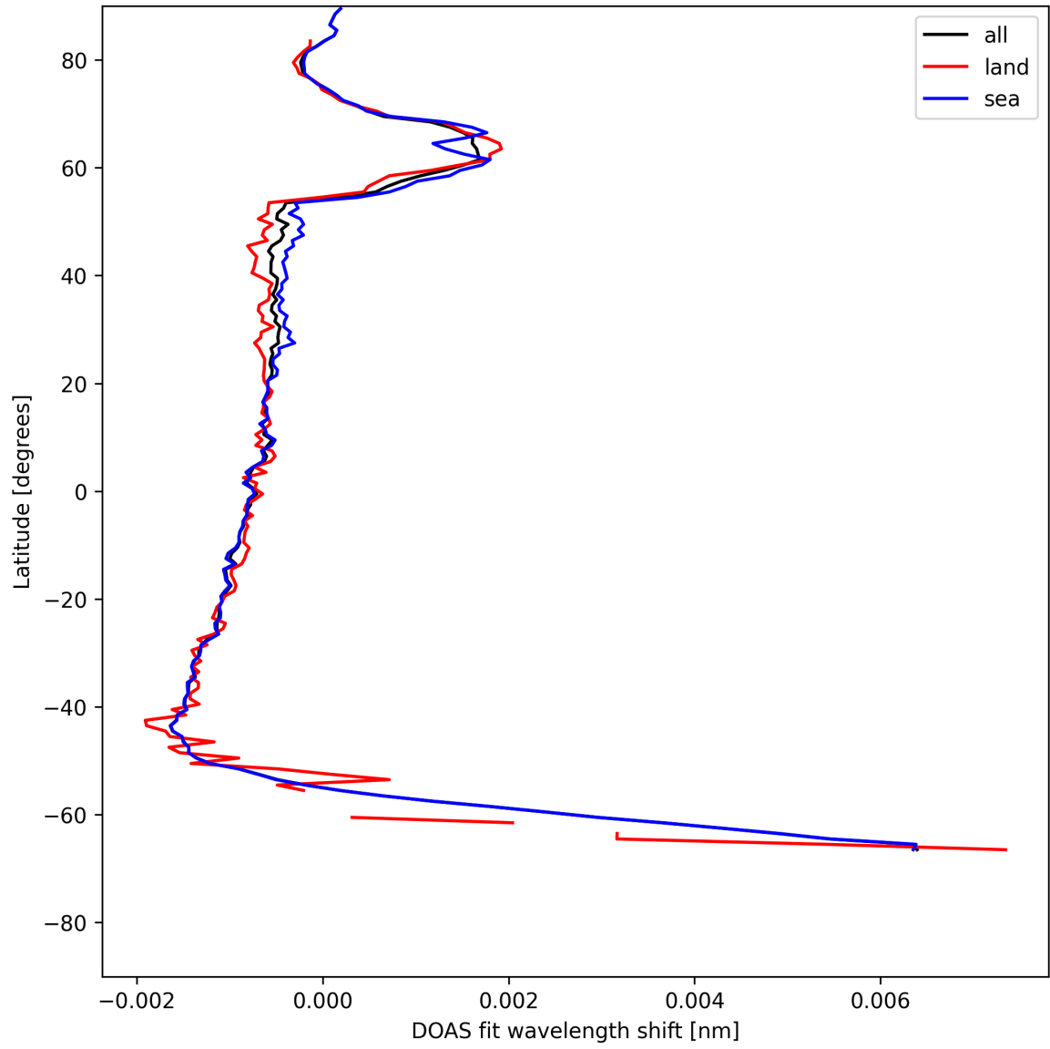
Figure 23: Zonal average of “DOAS fit wavelength shift” for 2025-06-02 to 2025-06-03.
