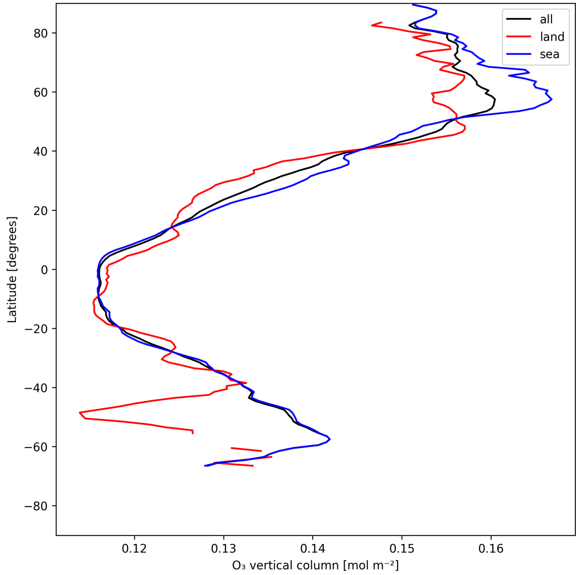
Figure 17: Zonal average of “O 3 vertical column” for 2025-06-02 to 2025-06-03.
