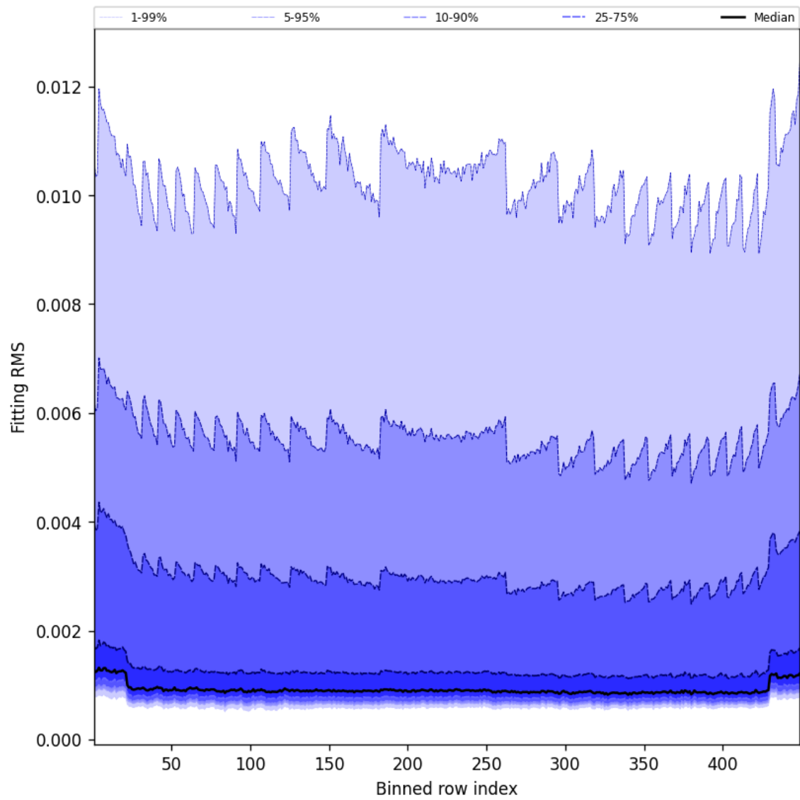
Figure 46: Along track statistics of “Fitting RMS” for 2025-06-02 to 2025-06-03
