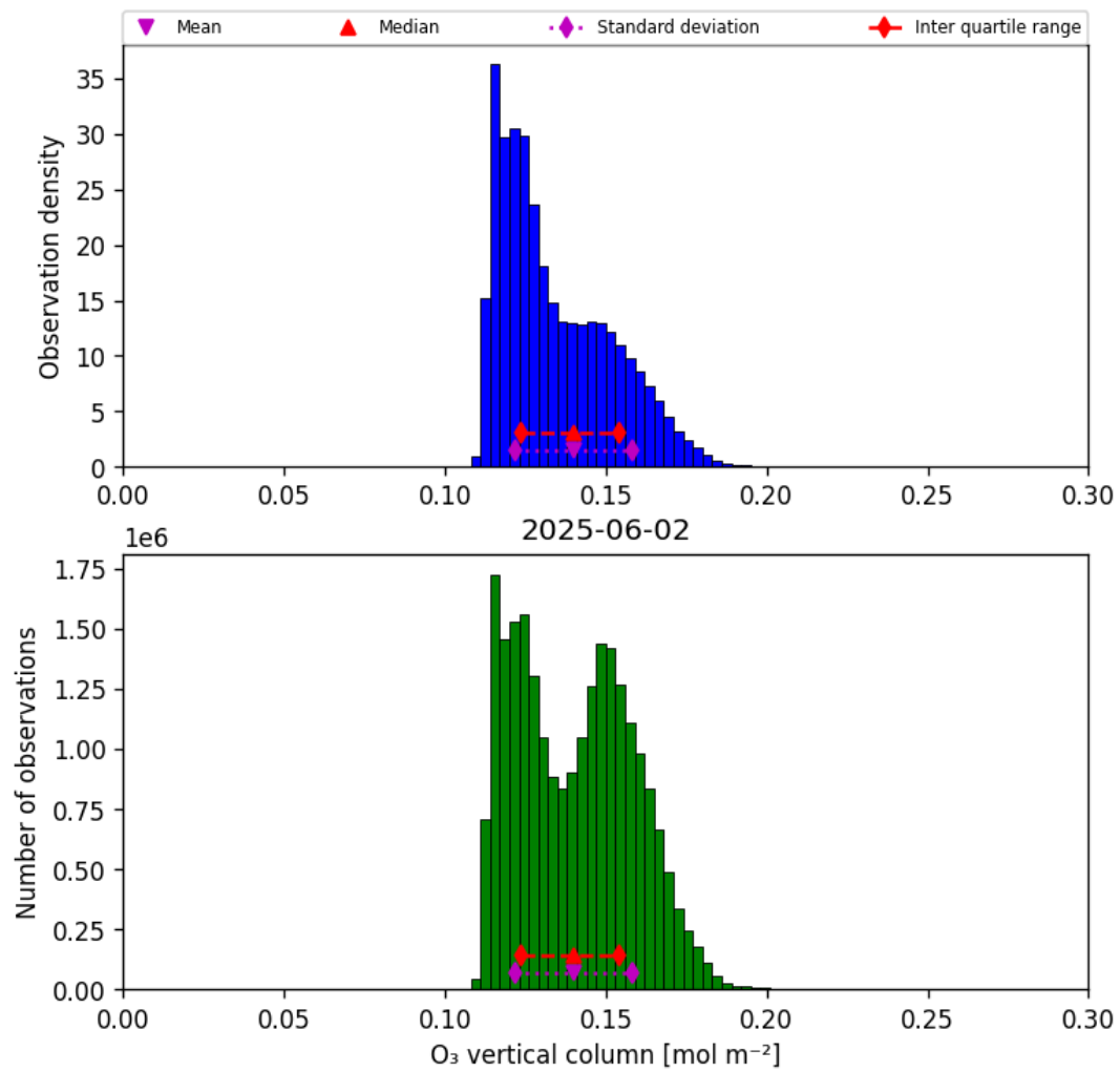
Figure 29: Histogram of “O 3 vertical column” for 2025-06-02 to 2025-06-03
