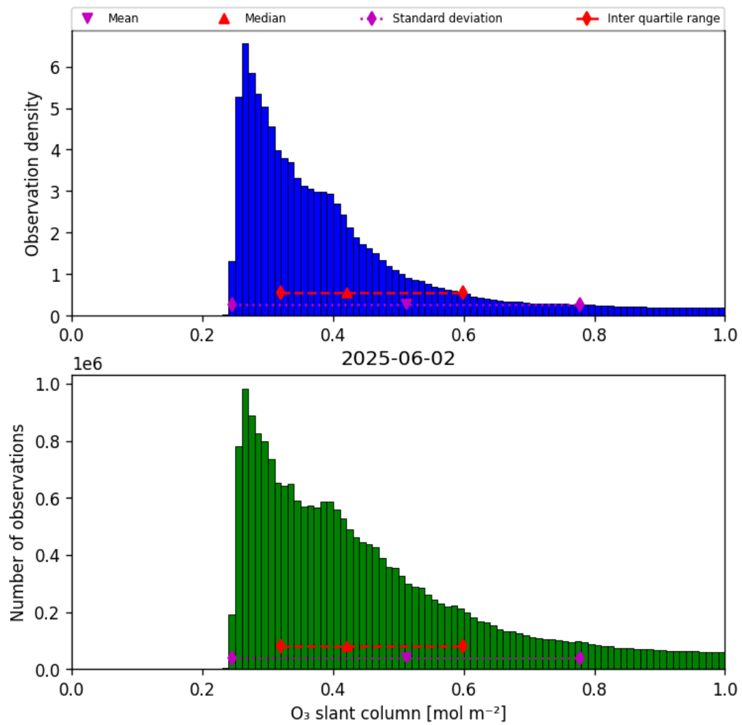
Figure 31: Histogram of “O 3 slant column” for 2025-06-02 to 2025-06-03
