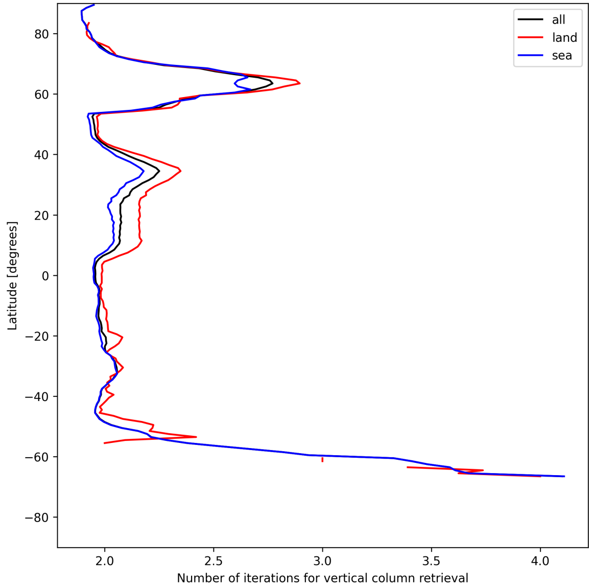
Figure 27: Zonal average of “Number of iterations for vertical column retrieval” for 2025-06-02 to 2025-06-03.
