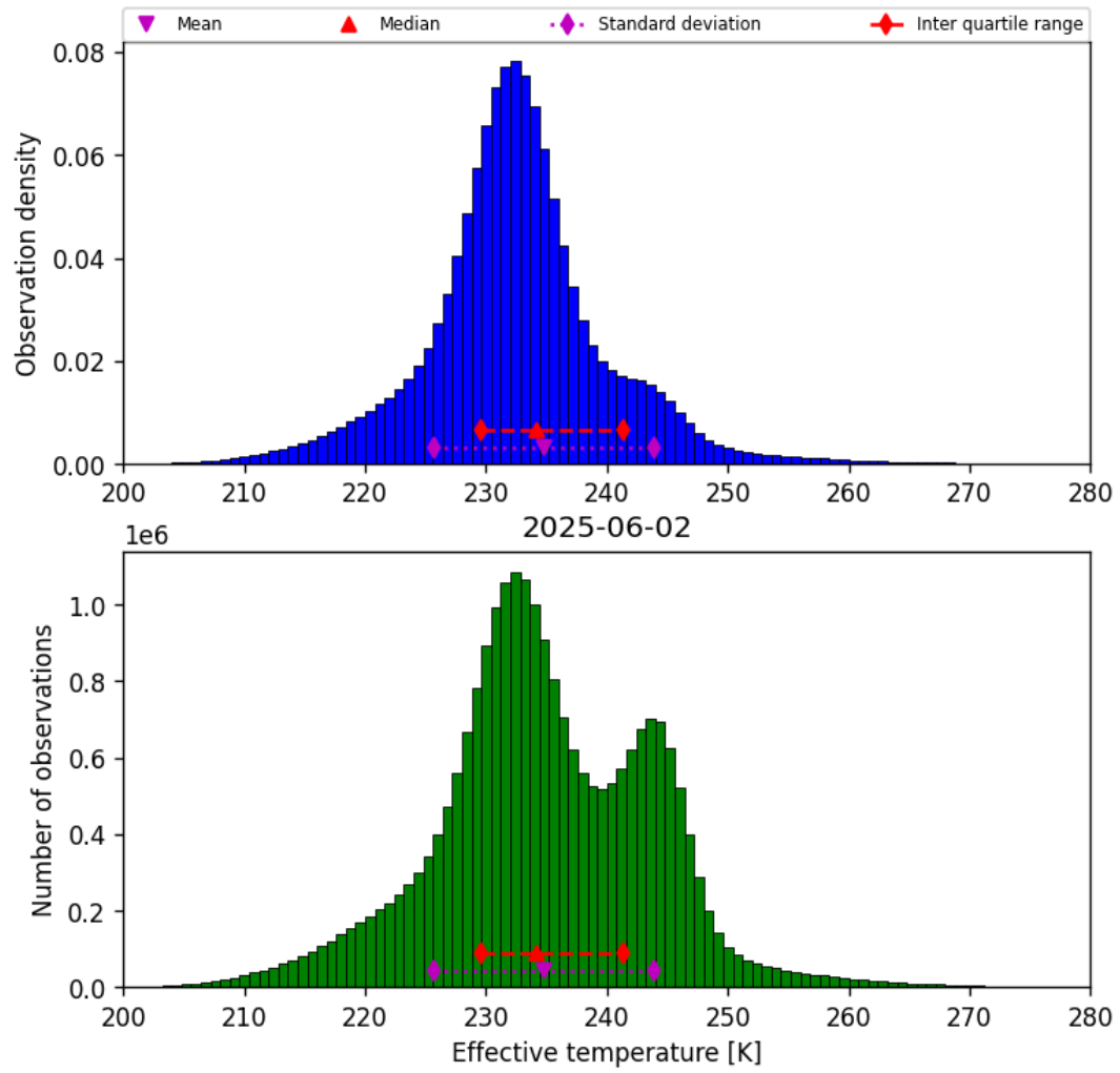
Figure 38: Histogram of “Effective temperature” for 2025-06-02 to 2025-06-03
