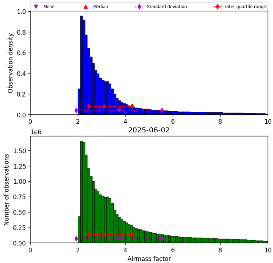
Figure 37: Histogram of “Airmass factor” for 2025-06-02 to 2025-06-03
