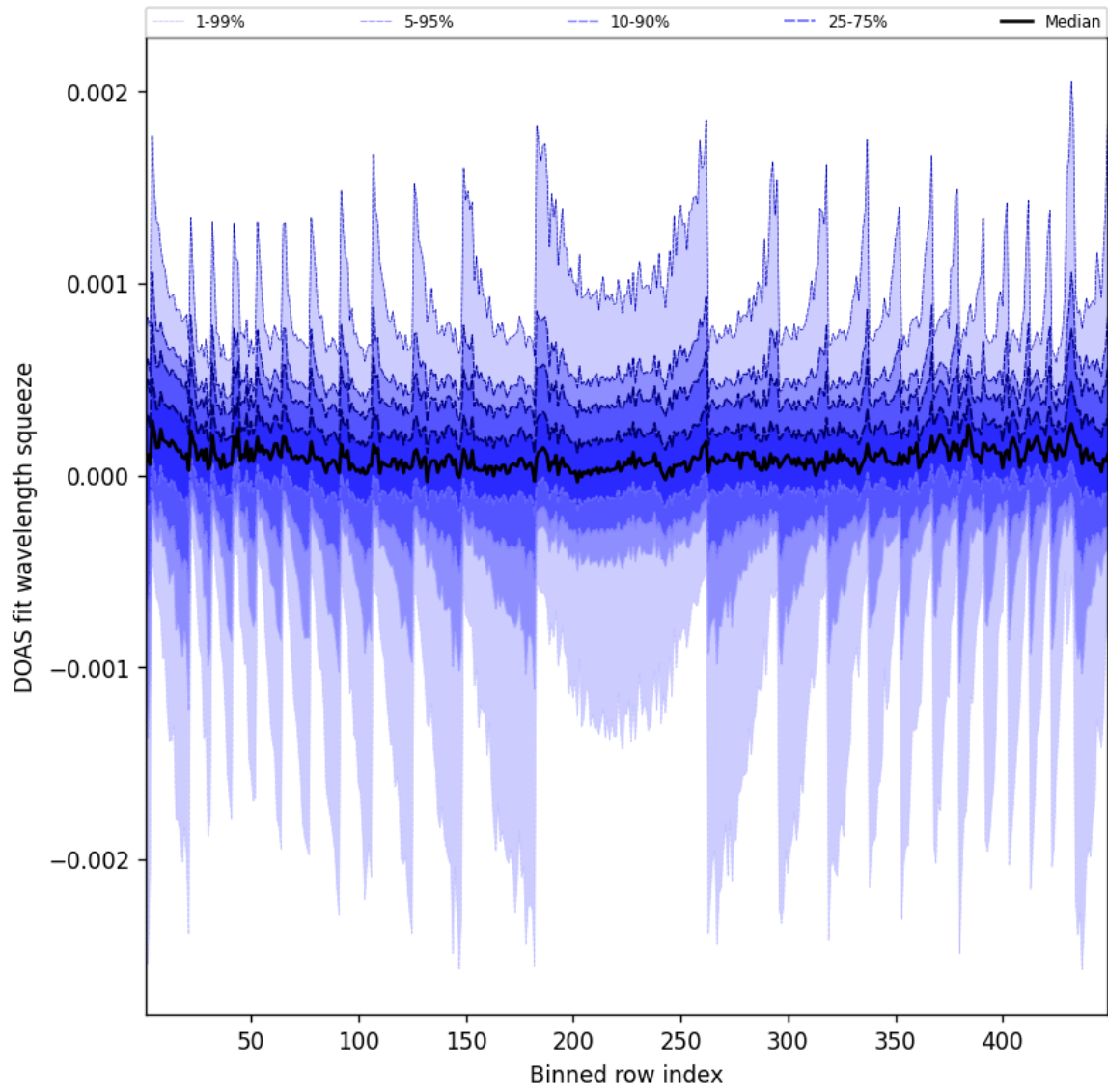
Figure 48: Along track statistics of “DOAS fit wavelength squeeze” for 2025-06-02 to 2025-06-03
