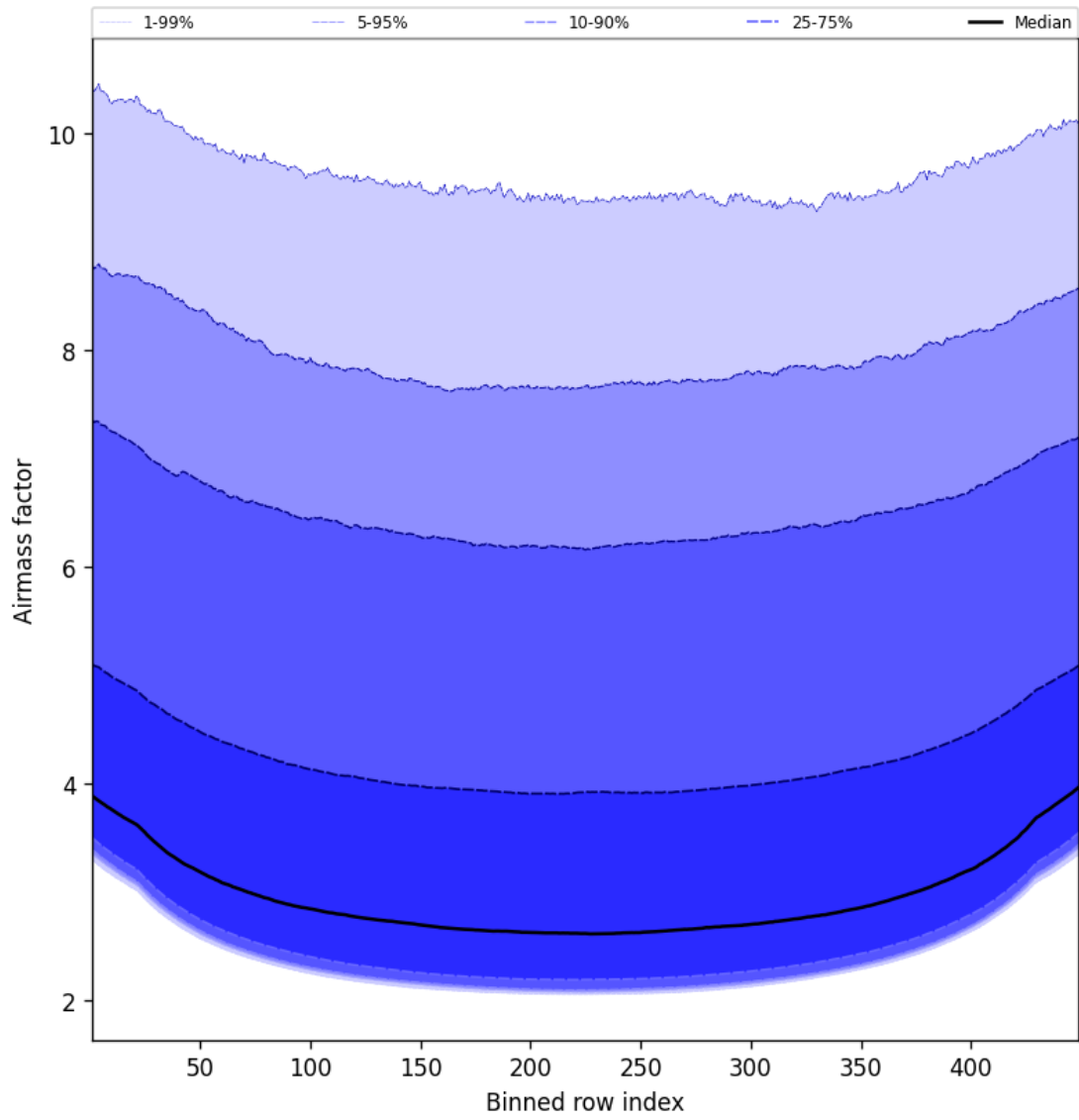
Figure 49: Along track statistics of “Airmass factor” for 2025-06-02 to 2025-06-03
