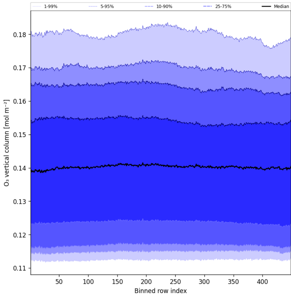
Figure 41: Along track statistics of “O 3 vertical column” for 2025-06-02 to 2025-06-03
