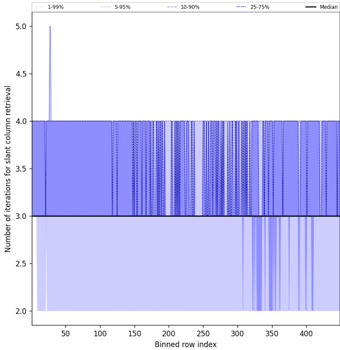
Figure 45: Along track statistics of “Number of iterations for slant column retrieval” for 2025-06-02 to 2025-06-03
