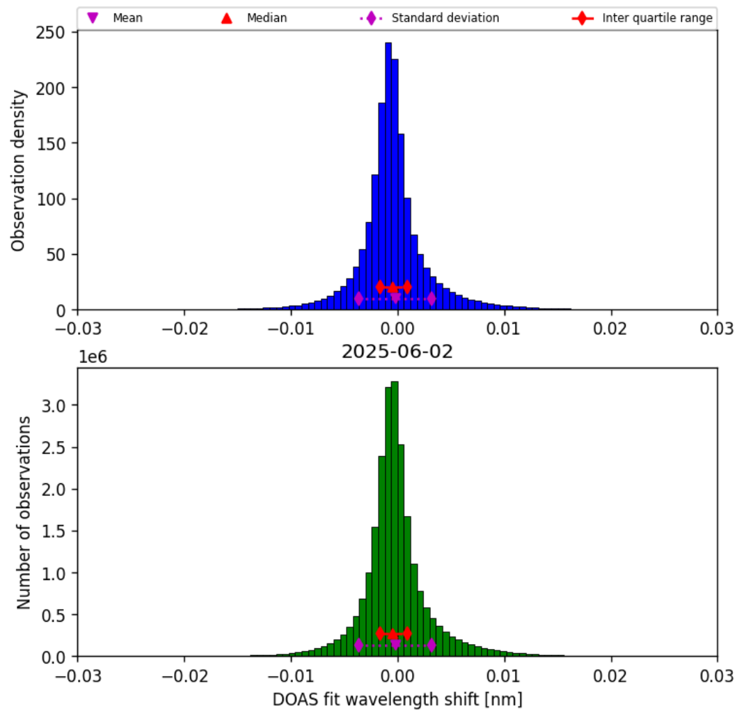
Figure 35: Histogram of “DOAS fit wavelength shift” for 2025-06-02 to 2025-06-03
