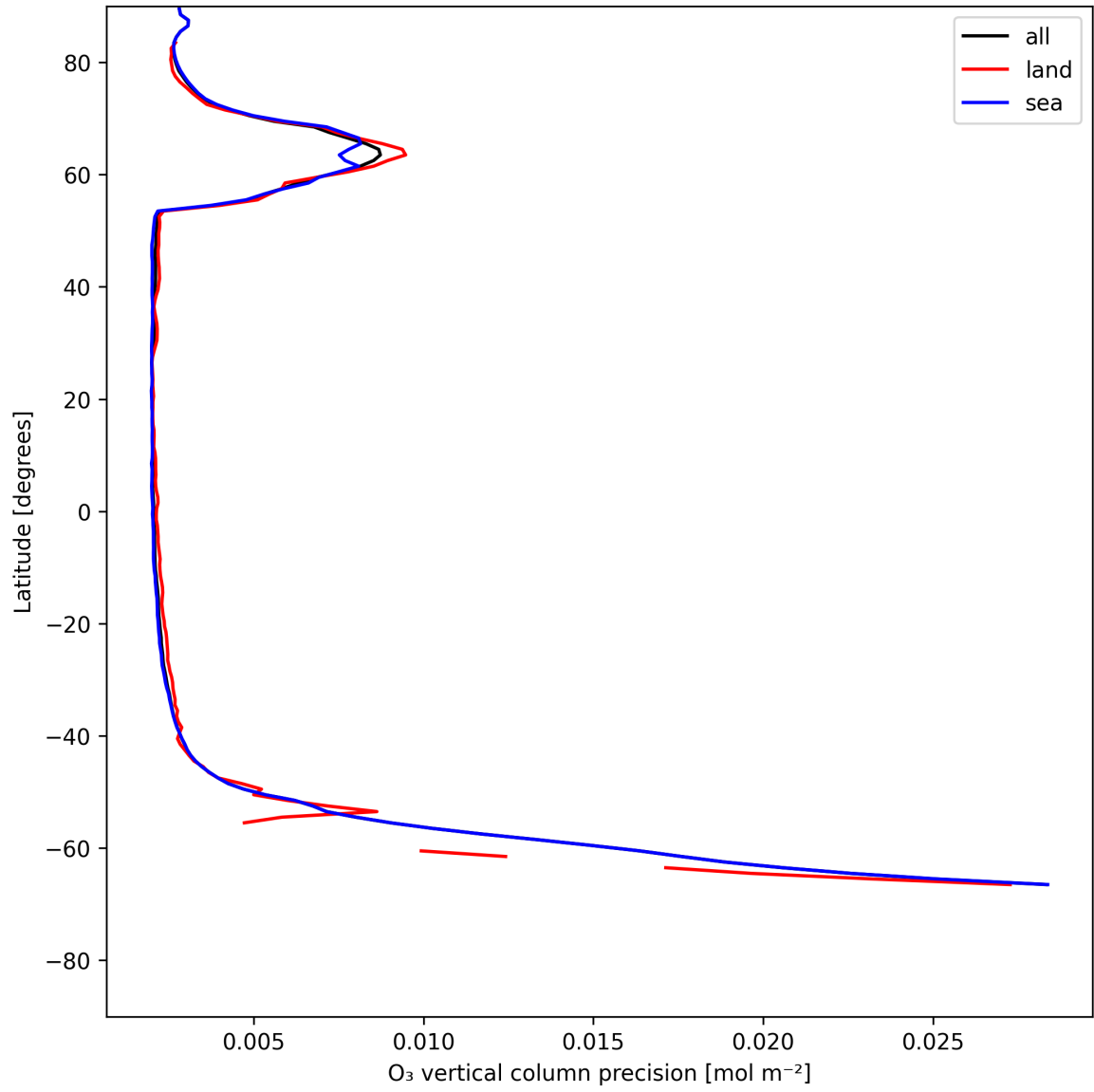
Figure 18: Zonal average of “O 3 vertical column precision” for 2025-06-02 to 2025-06-03.
