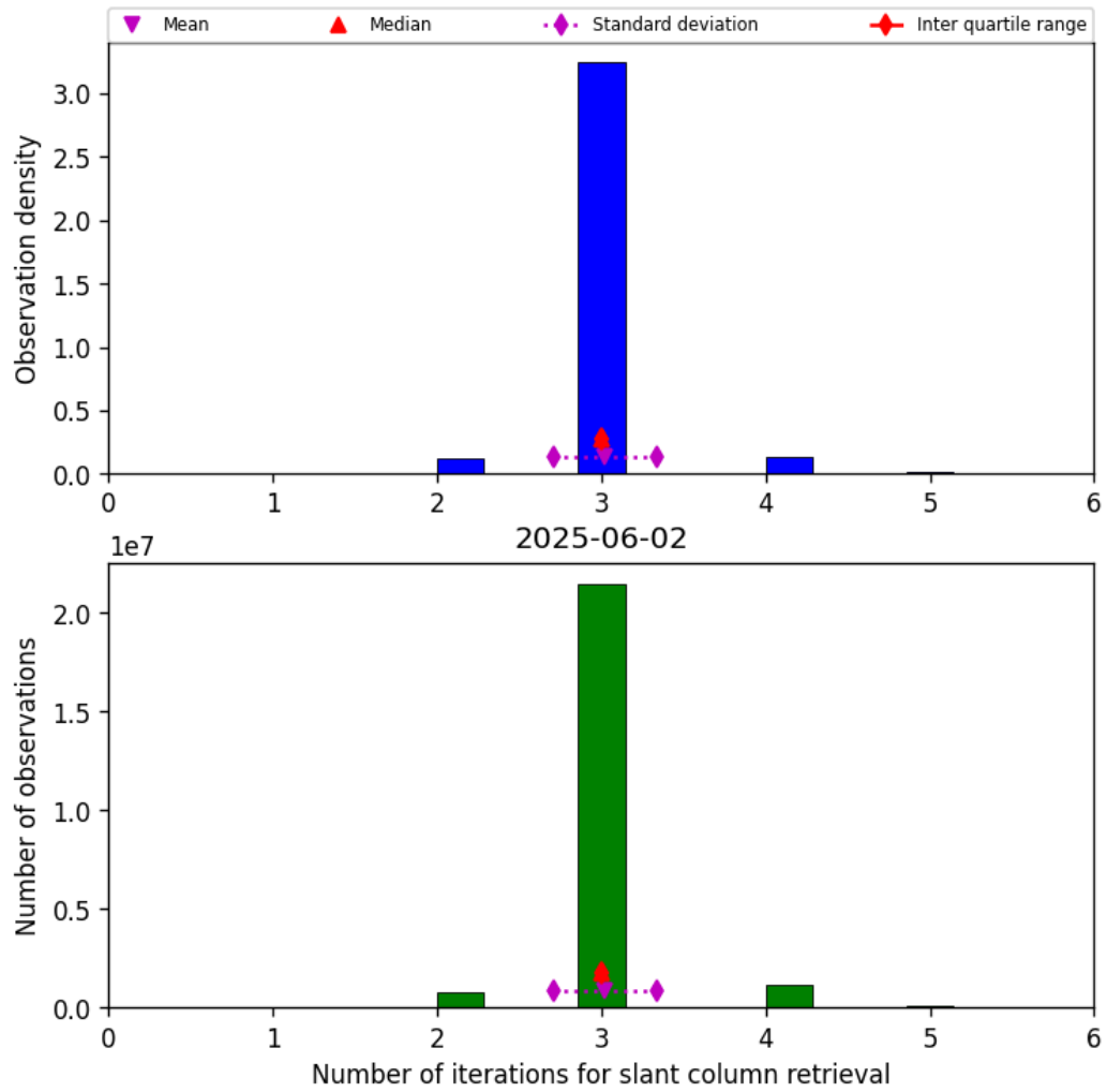
Figure 33: Histogram of “Number of iterations for slant column retrieval” for 2025-06-02 to 2025-06-03
