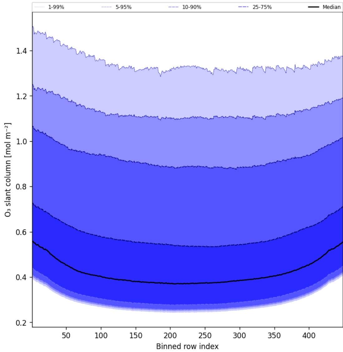
Figure 43: Along track statistics of “O 3 slant column” for 2025-06-02 to 2025-06-03
