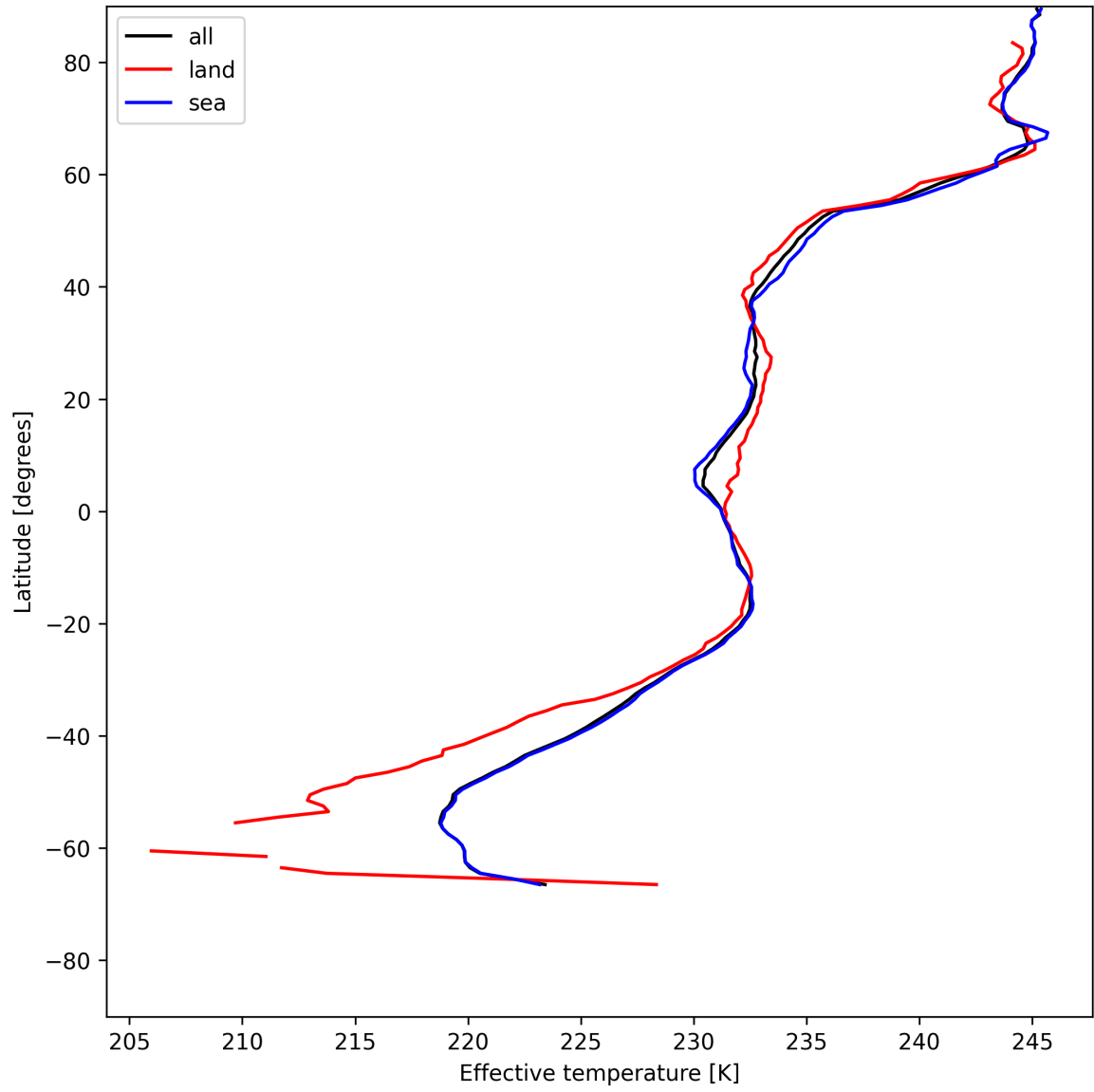
Figure 26: Zonal average of “Effective temperature” for 2025-06-02 to 2025-06-03.
