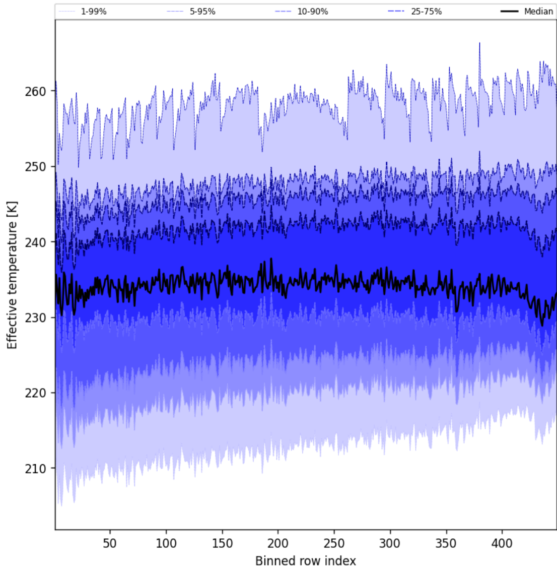
Figure 50: Along track statistics of “Effective temperature” for 2025-06-02 to 2025-06-03
