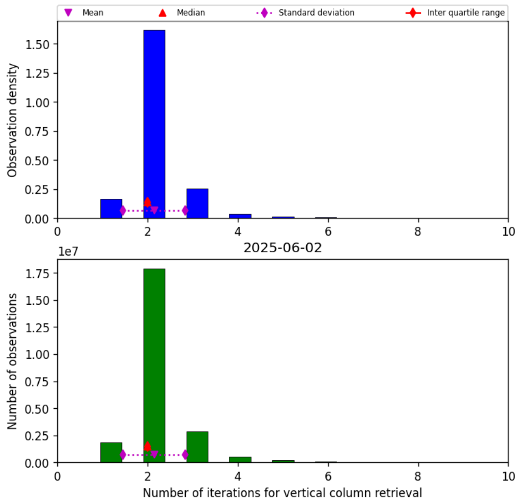
Figure 39: Histogram of “Number of iterations for vertical column retrieval” for 2025-06-02 to 2025-06-03
