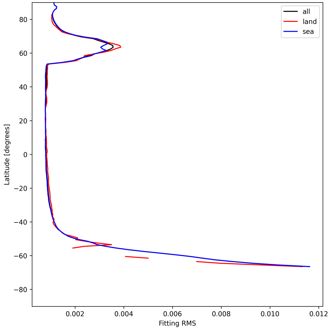
Figure 22: Zonal average of “Fitting RMS” for 2025-06-02 to 2025-06-03.
