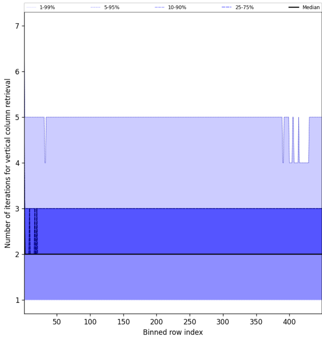
Figure 51: Along track statistics of “Number of iterations for vertical column retrieval” for 2025-06-02 to 2025-06-03
