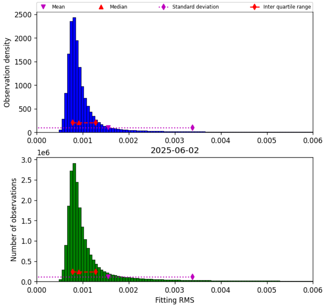
Figure 34: Histogram of “Fitting RMS” for 2025-06-02 to 2025-06-03
