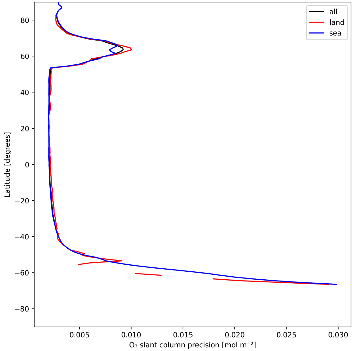
Figure 20: Zonal average of “O 3 slant column precision” for 2025-06-02 to 2025-06-03.
