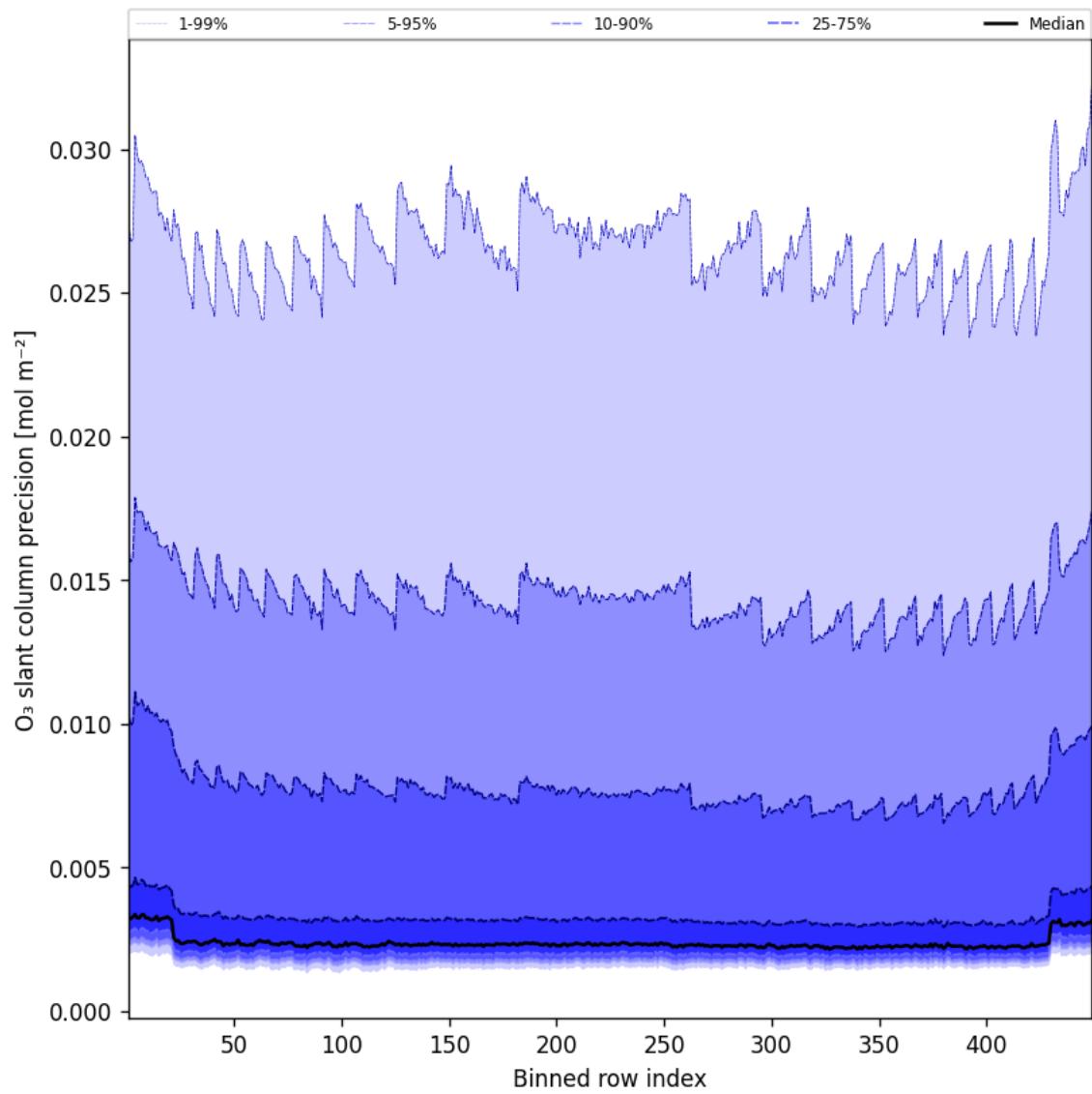
Figure 44: Along track statistics of “O 3 slant column precision” for 2025-06-02 to 2025-06-03
