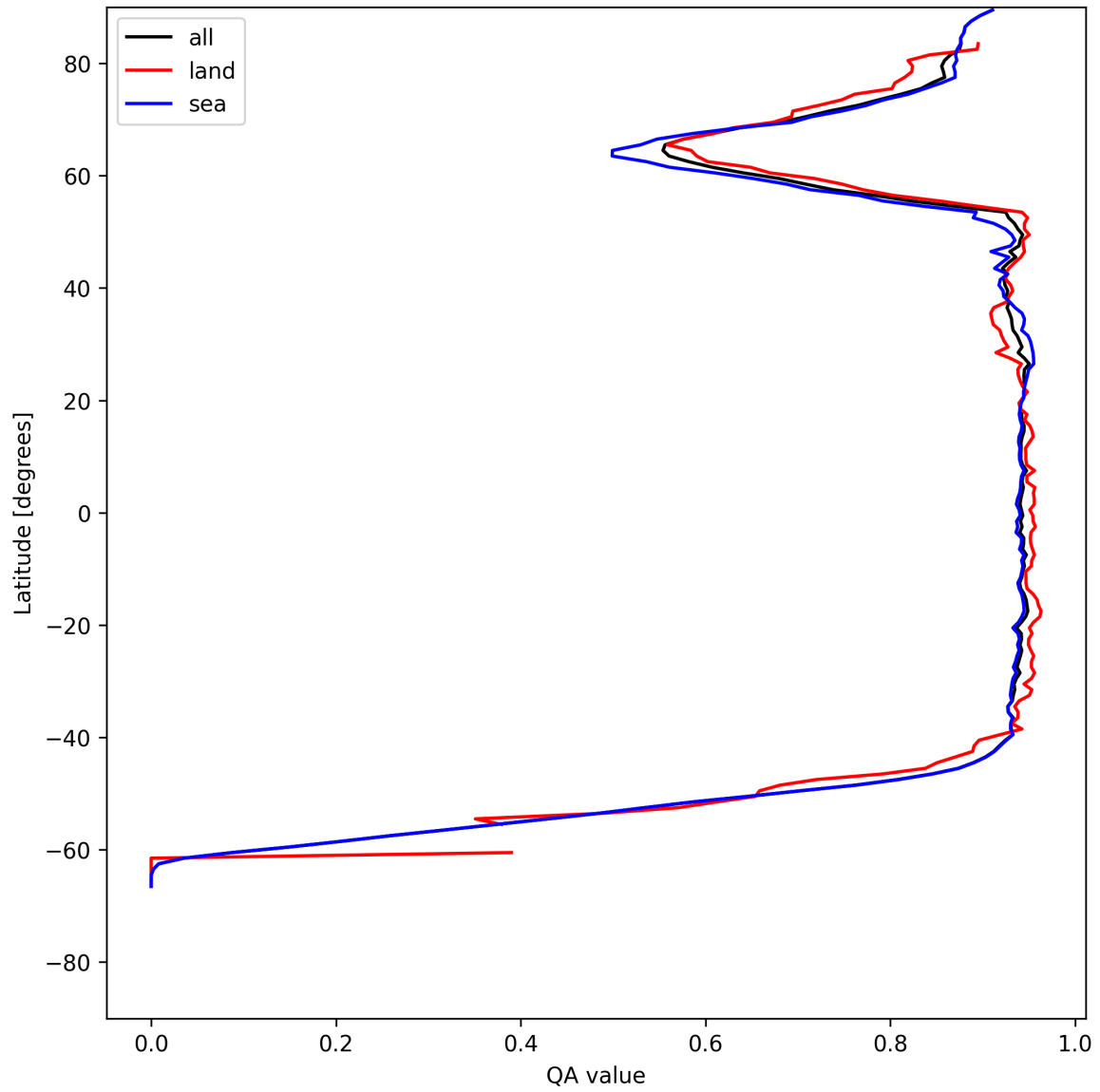
Figure 16: Zonal average of “QA value” for 2025-06-04 to 2025-06-04.
