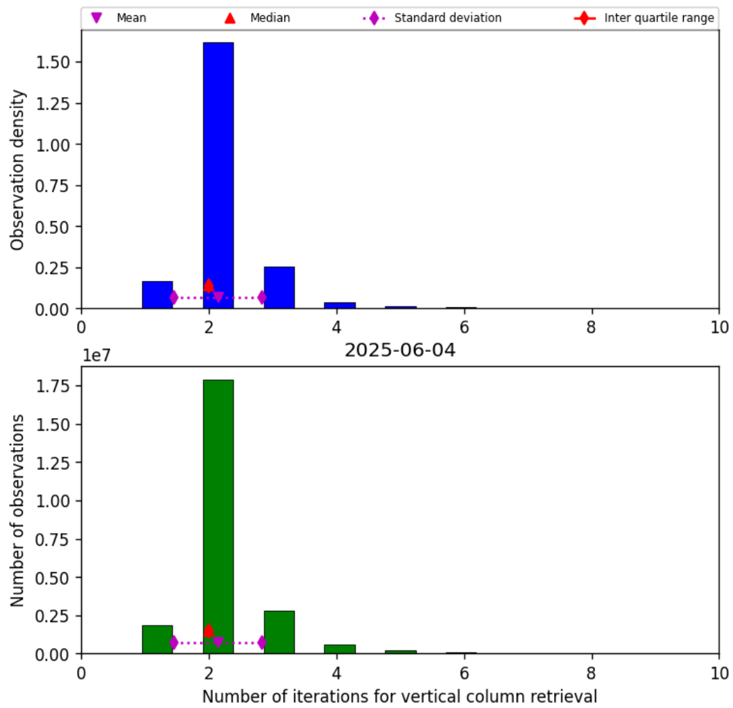
Figure 39: Histogram of “Number of iterations for vertical column retrieval” for 2025-06-04 to 2025-06-04
