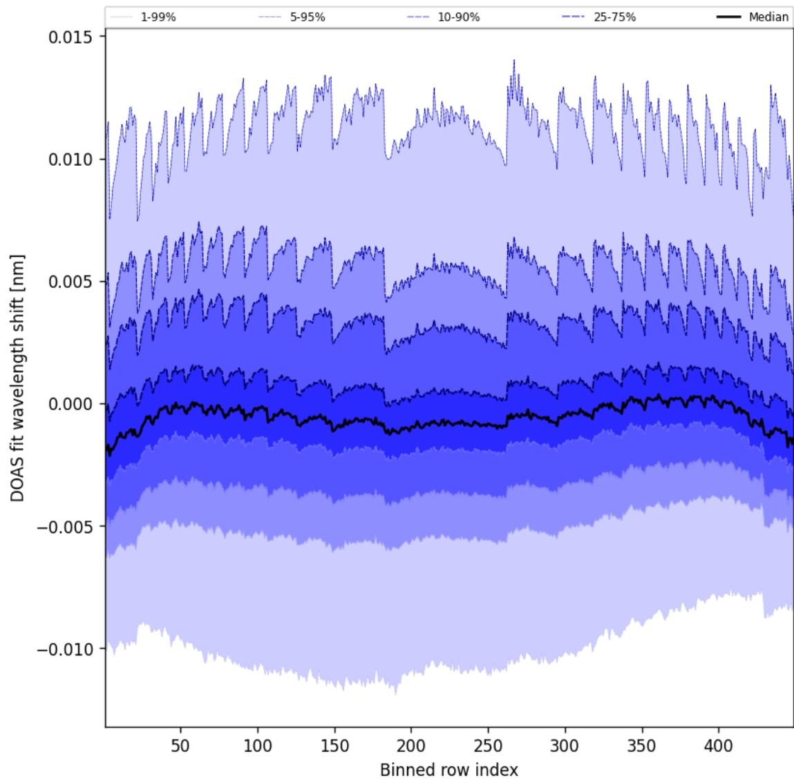
Figure 47: Along track statistics of "DOAS fit wavelength shift" for 2025-06-04 to 2025-06-04
