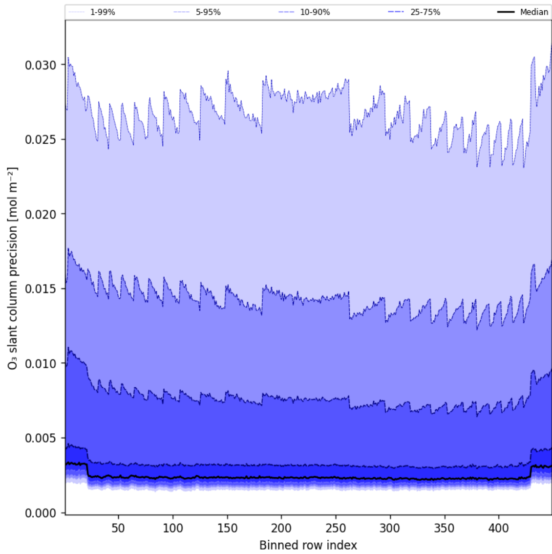
Figure 44: Along track statistics of “O 3 slant column precision” for 2025-06-04 to 2025-06-04
