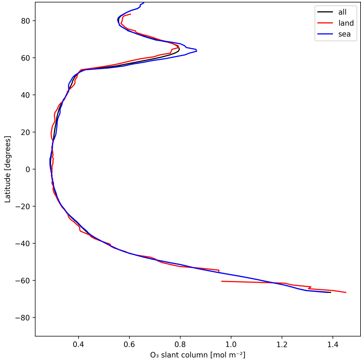
Figure 19: Zonal average of “O 3 slant column” for 2025-06-04 to 2025-06-04.
