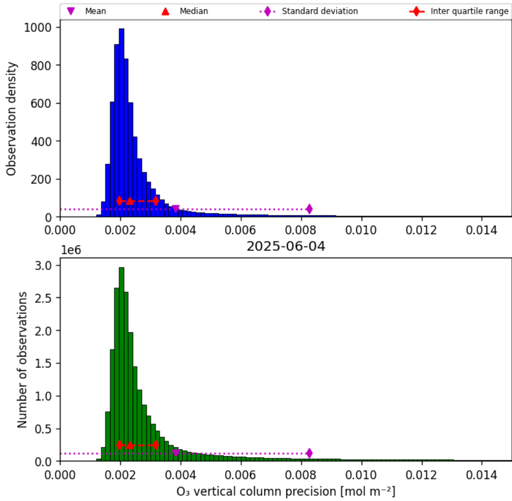
Figure 30: Histogram of “O 3 vertical column precision” for 2025-06-04 to 2025-06-04
