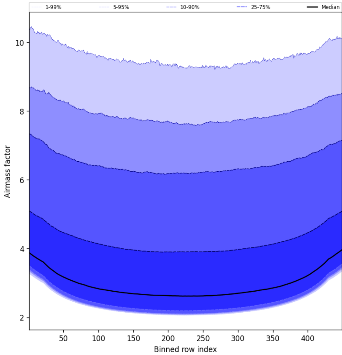
Figure 49: Along track statistics of “Airmass factor” for 2025-06-04 to 2025-06-04
