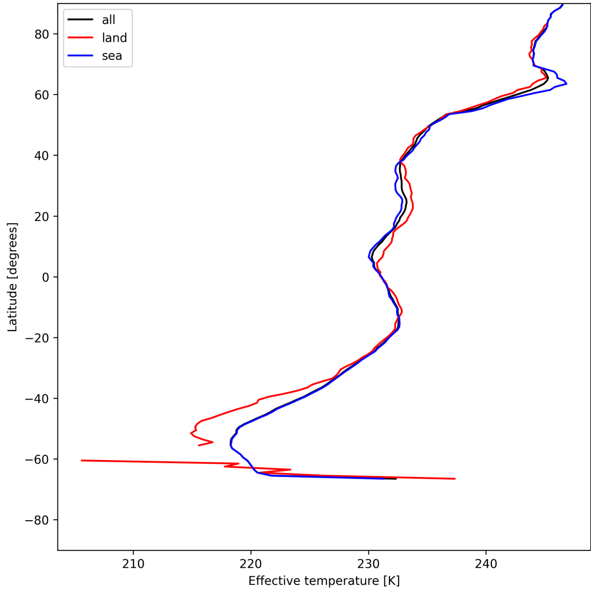
Figure 26: Zonal average of "Effective temperature" for 2025-06-04 to 2025-06-04.
