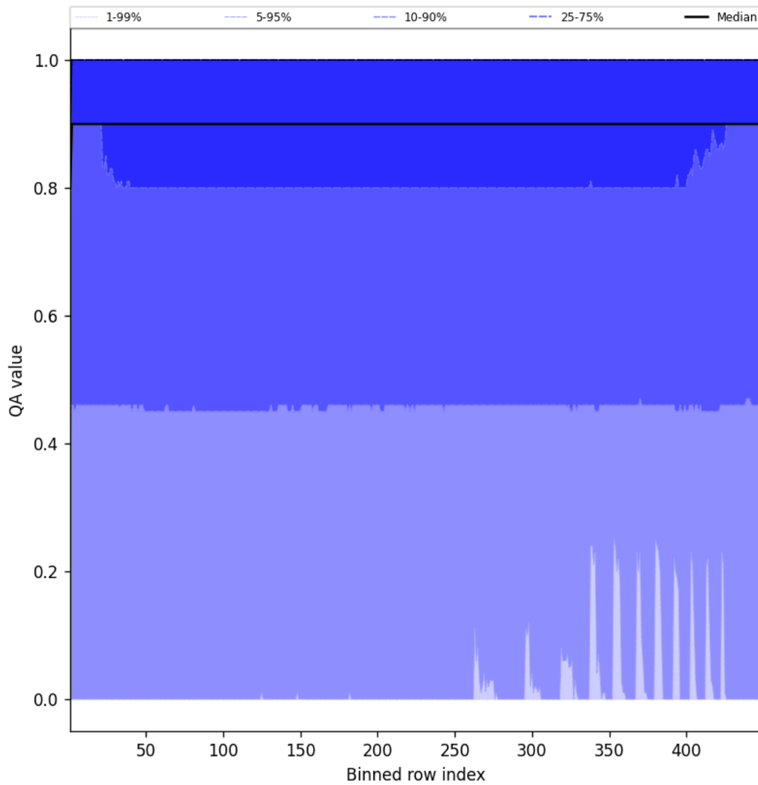
Figure 40: Along track statistics of “QA value” for 2025-06-04 to 2025-06-04
