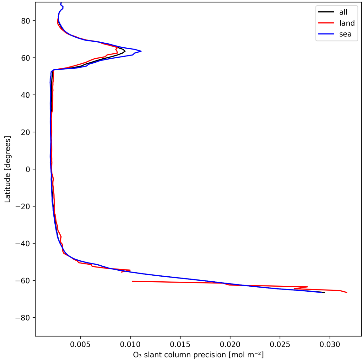
Figure 20: Zonal average of “O 3 slant column precision” for 2025-06-04 to 2025-06-04.
