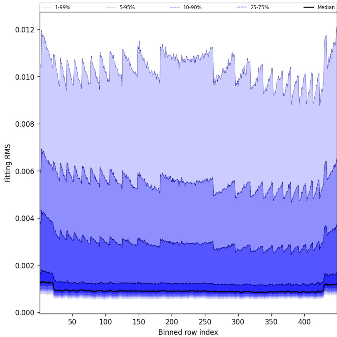
Figure 46: Along track statistics of “Fitting RMS” for 2025-06-04 to 2025-06-04
