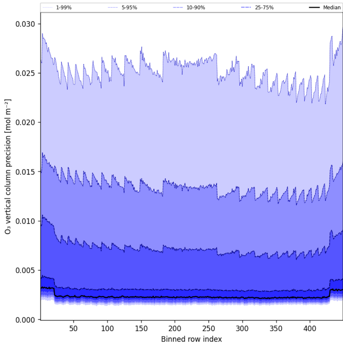
Figure 42: Along track statistics of “O 3 vertical column precision” for 2025-06-04 to 2025-06-04
