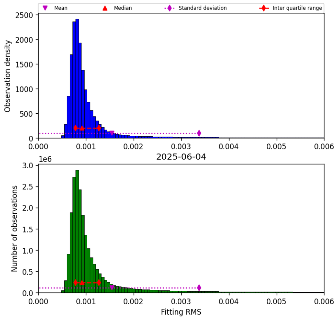
Figure 34: Histogram of “Fitting RMS” for 2025-06-04 to 2025-06-04
