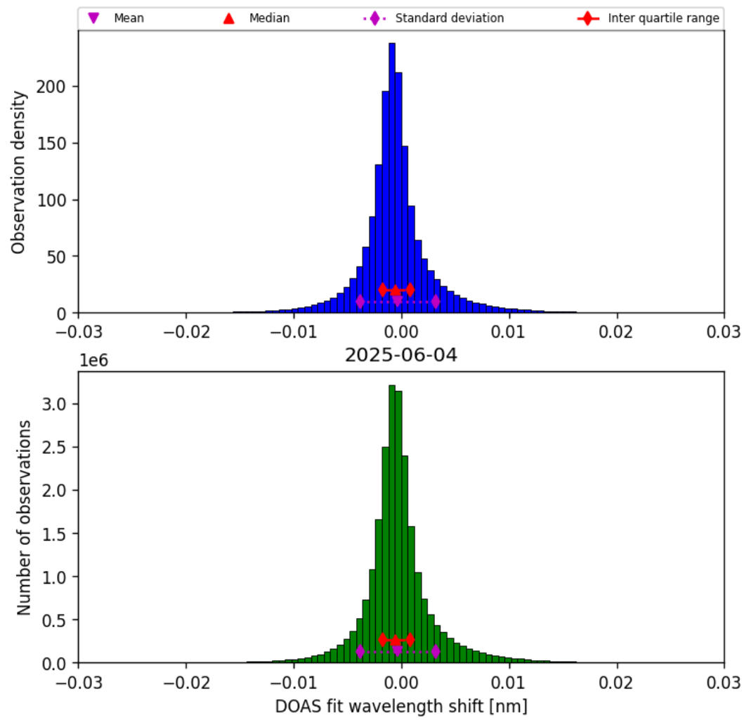
Figure 35: Histogram of “DOAS fit wavelength shift” for 2025-06-04 to 2025-06-04
