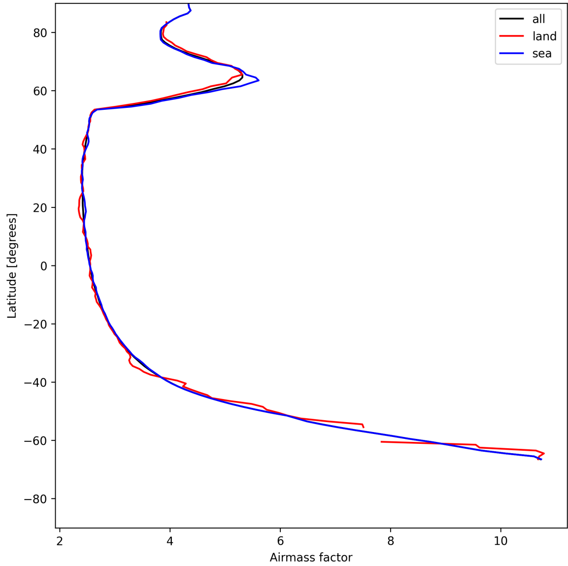
Figure 25: Zonal average of “Airmass factor” for 2025-06-04 to 2025-06-04.
