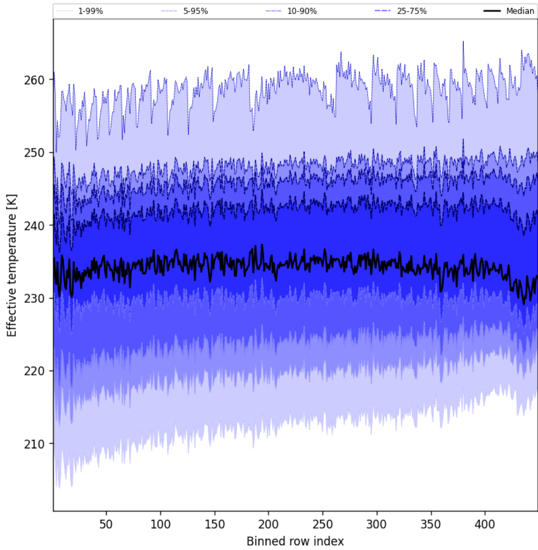
Figure 50: Along track statistics of “Effective temperature” for 2025-06-04 to 2025-06-04
