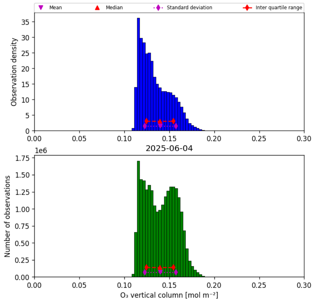
Figure 29: Histogram of “O 3 vertical column” for 2025-06-04 to 2025-06-04
