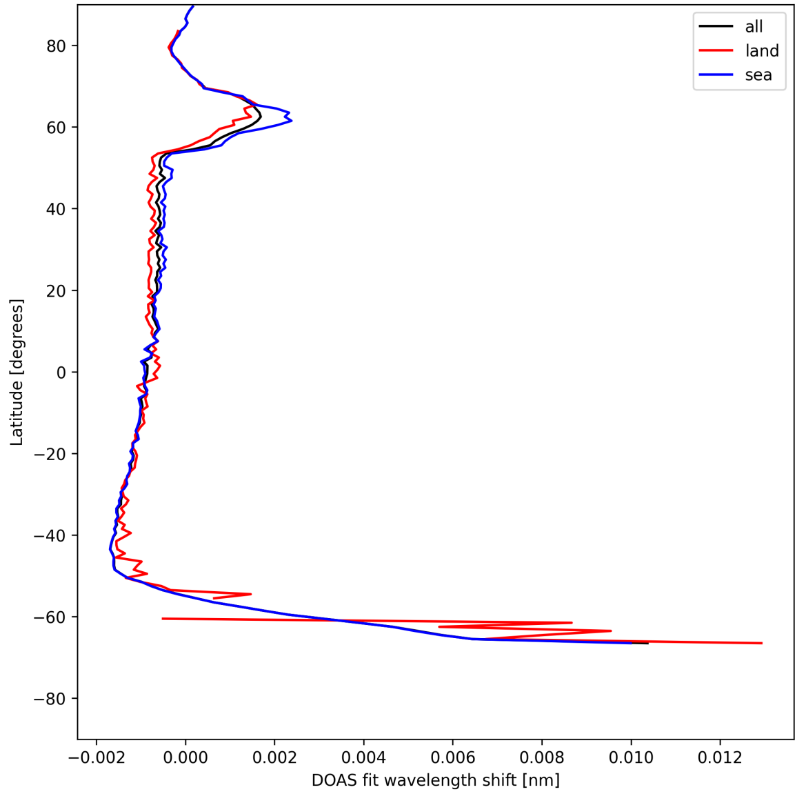
Figure 23: Zonal average of “DOAS fit wavelength shift” for 2025-06-04 to 2025-06-04.
