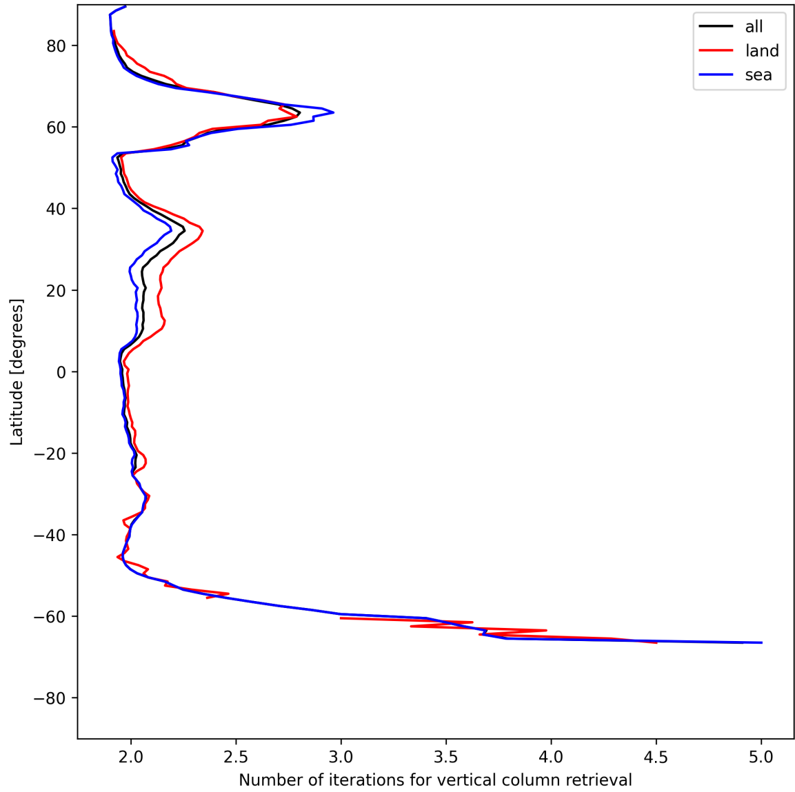
Figure 27: Zonal average of “Number of iterations for vertical column retrieval” for 2025-06-04 to 2025-06-04.
