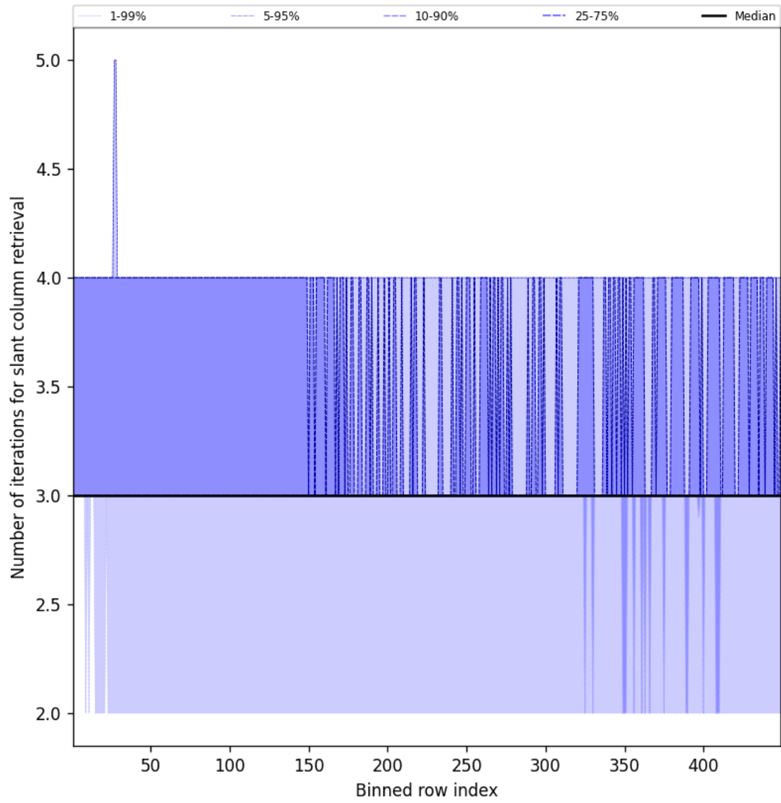
Figure 45: Along track statistics of “Number of iterations for slant column retrieval” for 2025-06-04 to 2025-06-04
