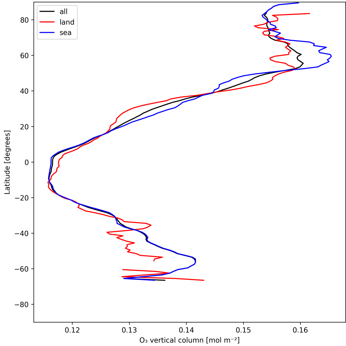
Figure 17: Zonal average of “O 3 vertical column” for 2025-06-04 to 2025-06-04.
