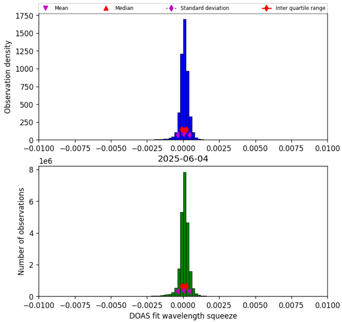
Figure 36: Histogram of “DOAS fit wavelength squeeze” for 2025-06-04 to 2025-06-04
