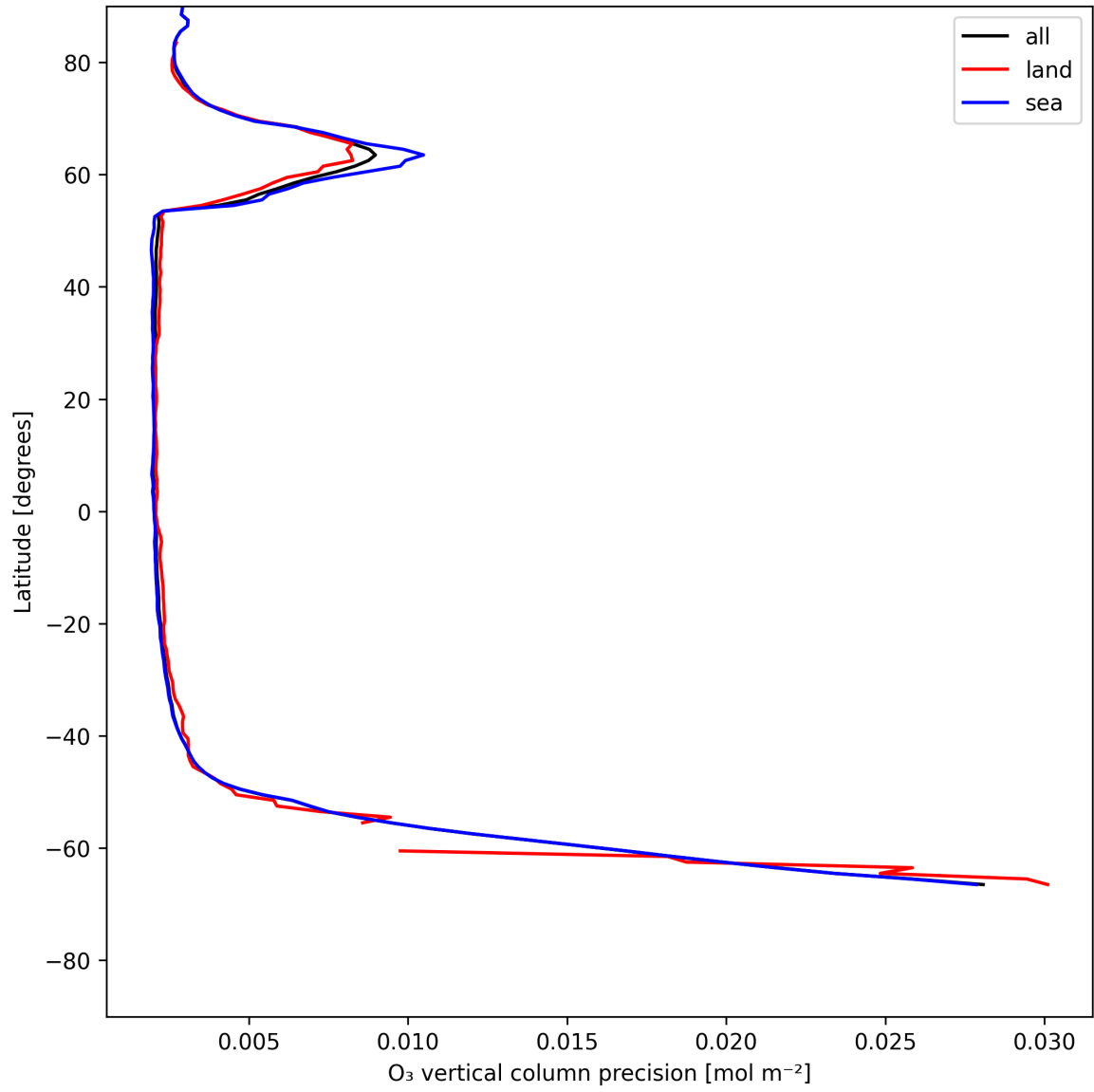
Figure 18: Zonal average of “O 3 vertical column precision” for 2025-06-04 to 2025-06-04.
