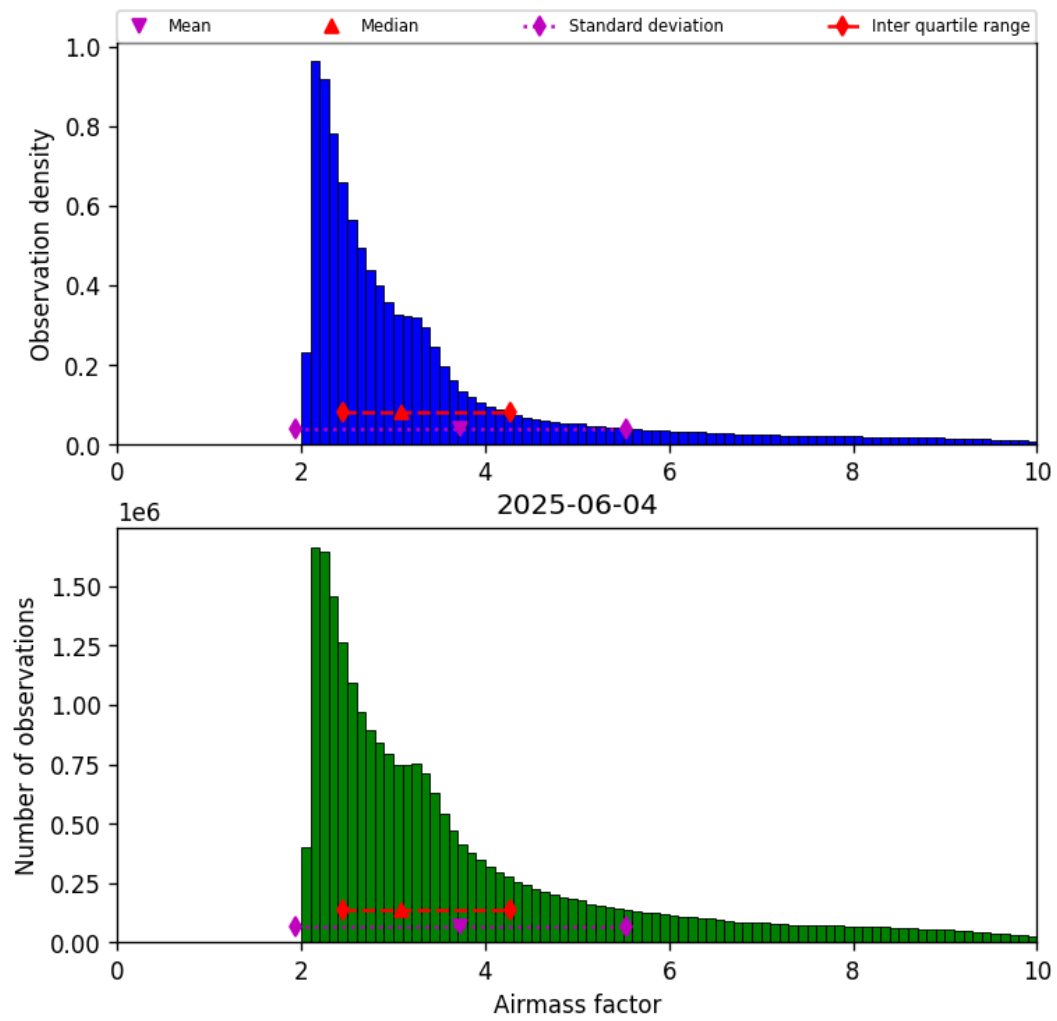
Figure 37: Histogram of “Airmass factor” for 2025-06-04 to 2025-06-04
