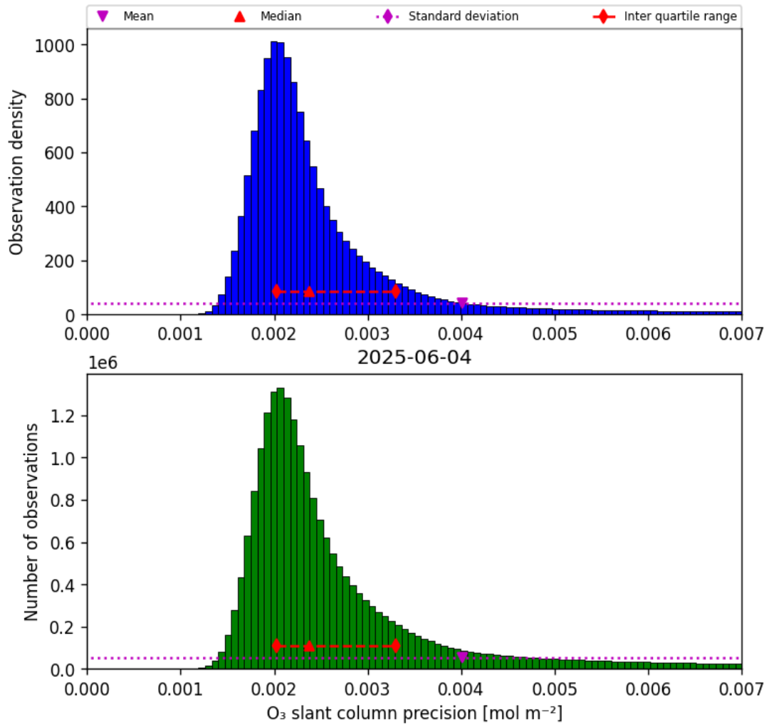
Figure 32: Histogram of “O 3 slant column precision” for 2025-06-04 to 2025-06-04
