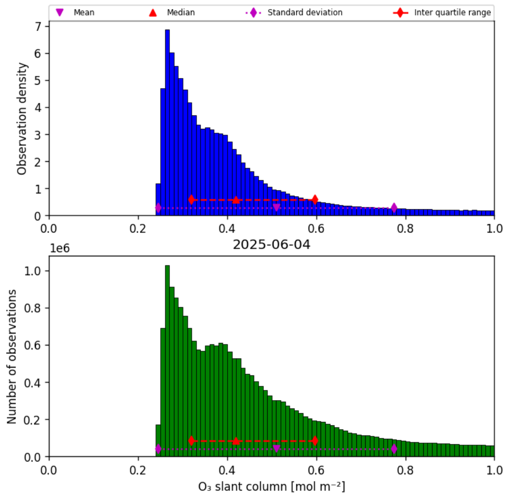
Figure 31: Histogram of “O 3 slant column” for 2025-06-04 to 2025-06-04
