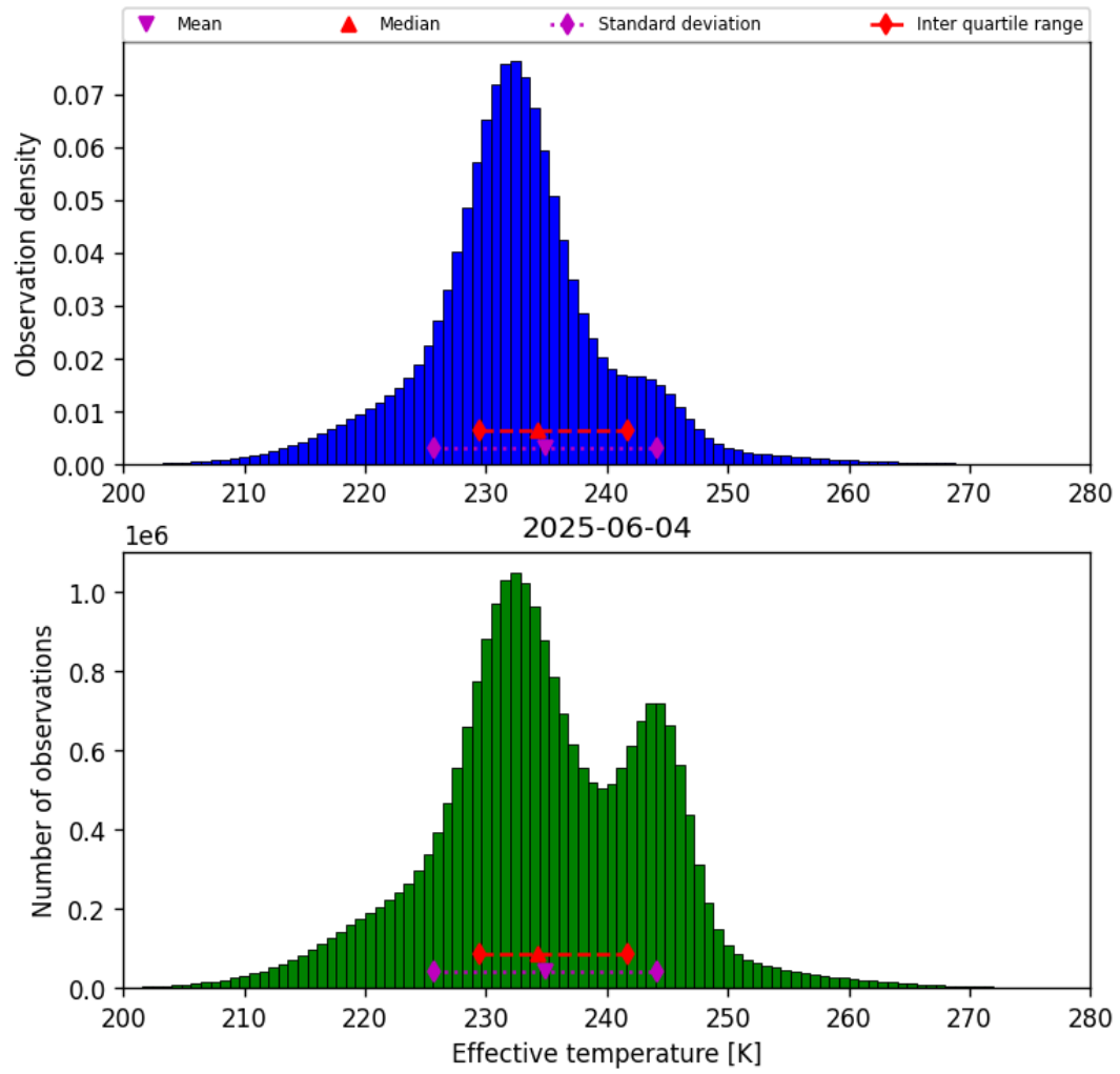
Figure 38: Histogram of “Effective temperature” for 2025-06-04 to 2025-06-04
