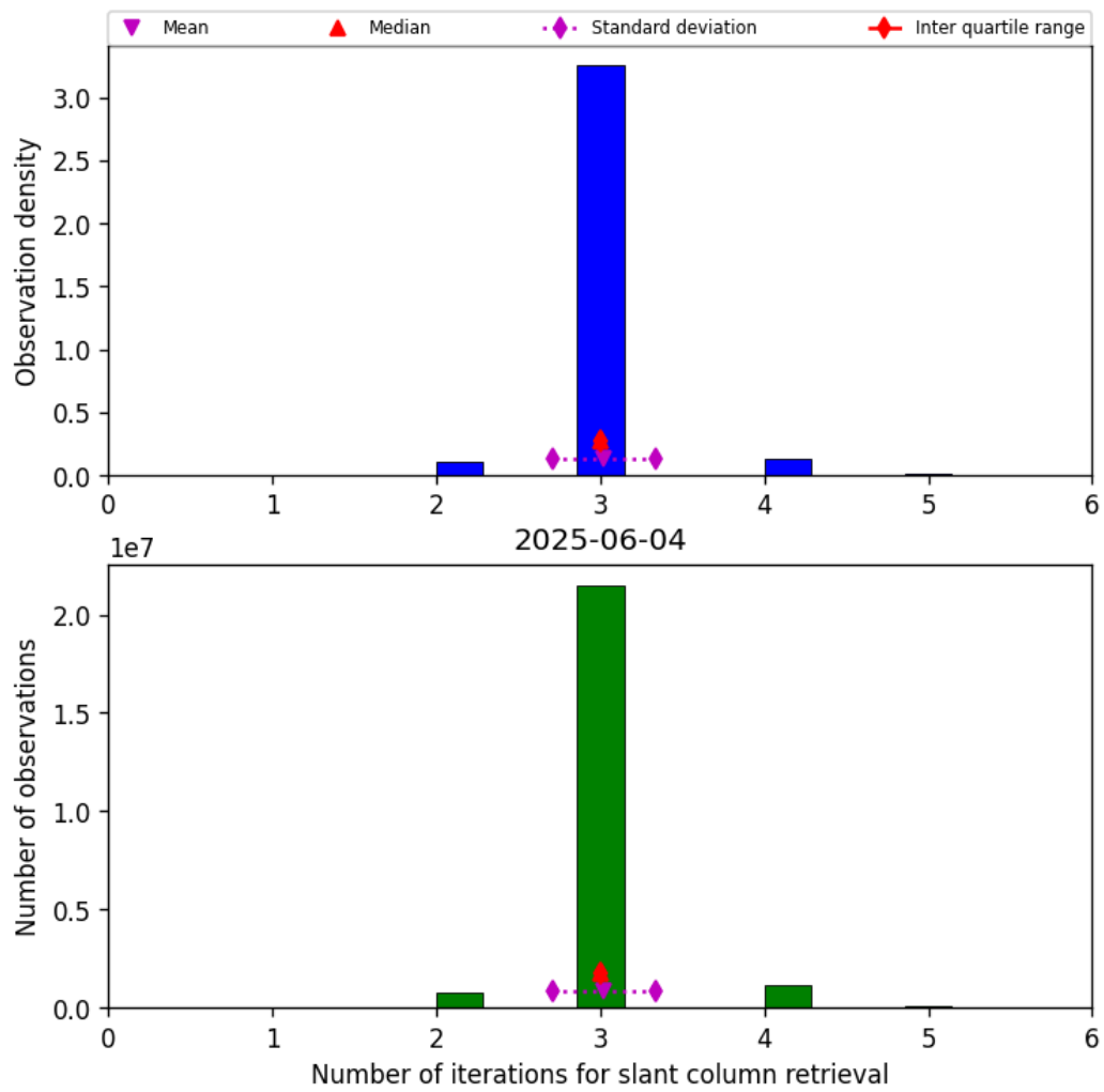
Figure 33: Histogram of “Number of iterations for slant column retrieval” for 2025-06-04 to 2025-06-04
