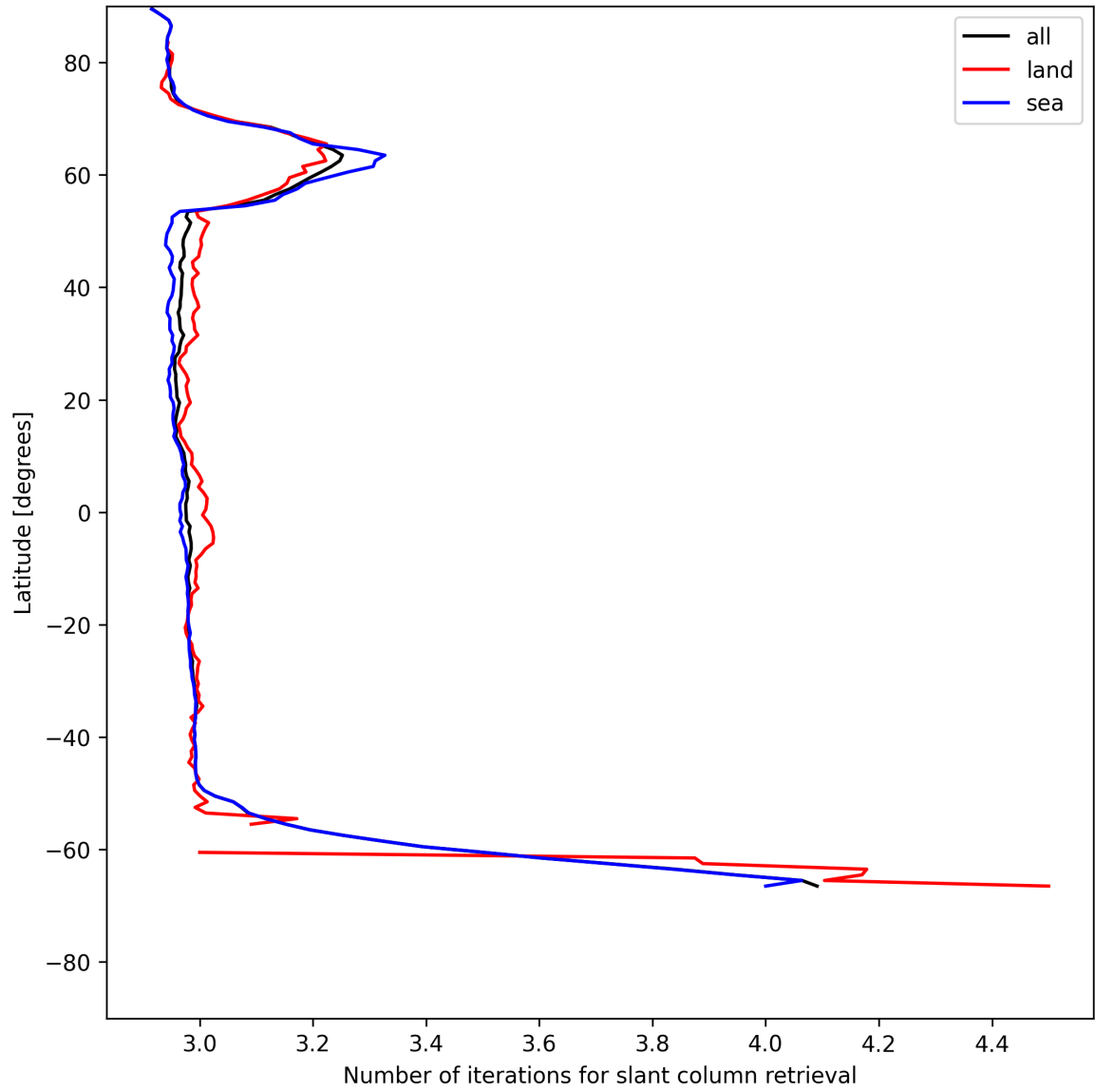
Figure 21: Zonal average of “Number of iterations for slant column retrieval” for 2025-06-04 to 2025-06-04.
