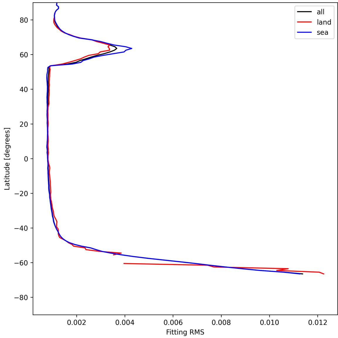
Figure 22: Zonal average of “Fitting RMS” for 2025-06-04 to 2025-06-04.
