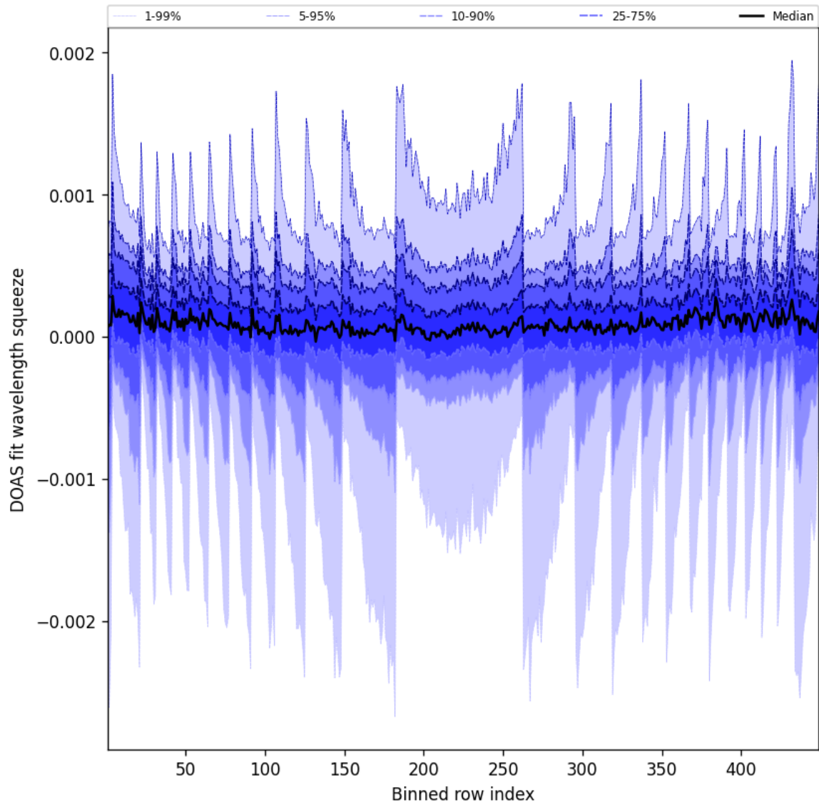
Figure 48: Along track statistics of “DOAS fit wavelength squeeze” for 2025-06-04 to 2025-06-04
