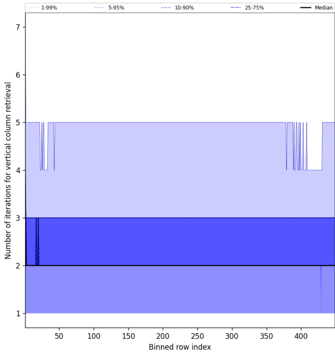
Figure 51: Along track statistics of “Number of iterations for vertical column retrieval” for 2025-06-04 to 2025-06-04
