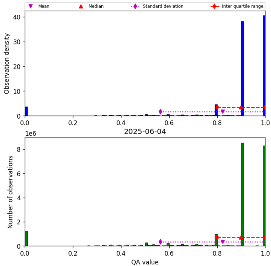
Figure 28: Histogram of “QA value” for 2025-06-04 to 2025-06-04
