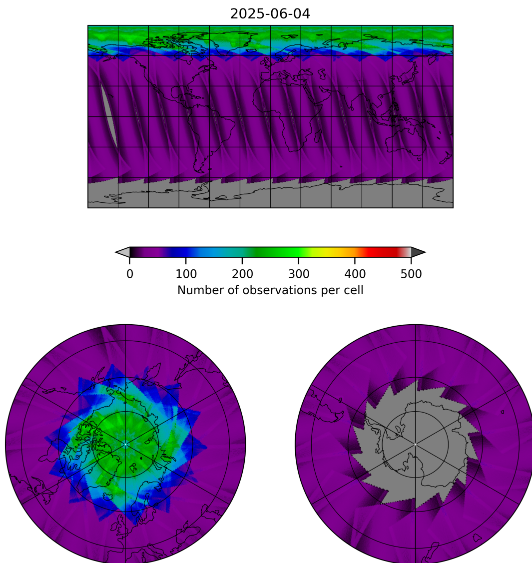
Figure 15: Map of the number of observations for 2025-06-04 to 2025-06-04
