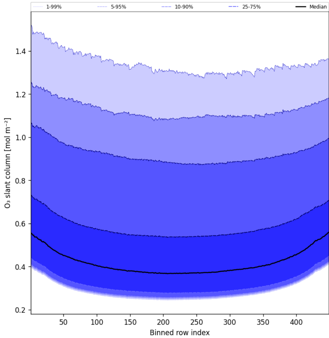
Figure 43: Along track statistics of “O 3 slant column” for 2025-06-04 to 2025-06-04
