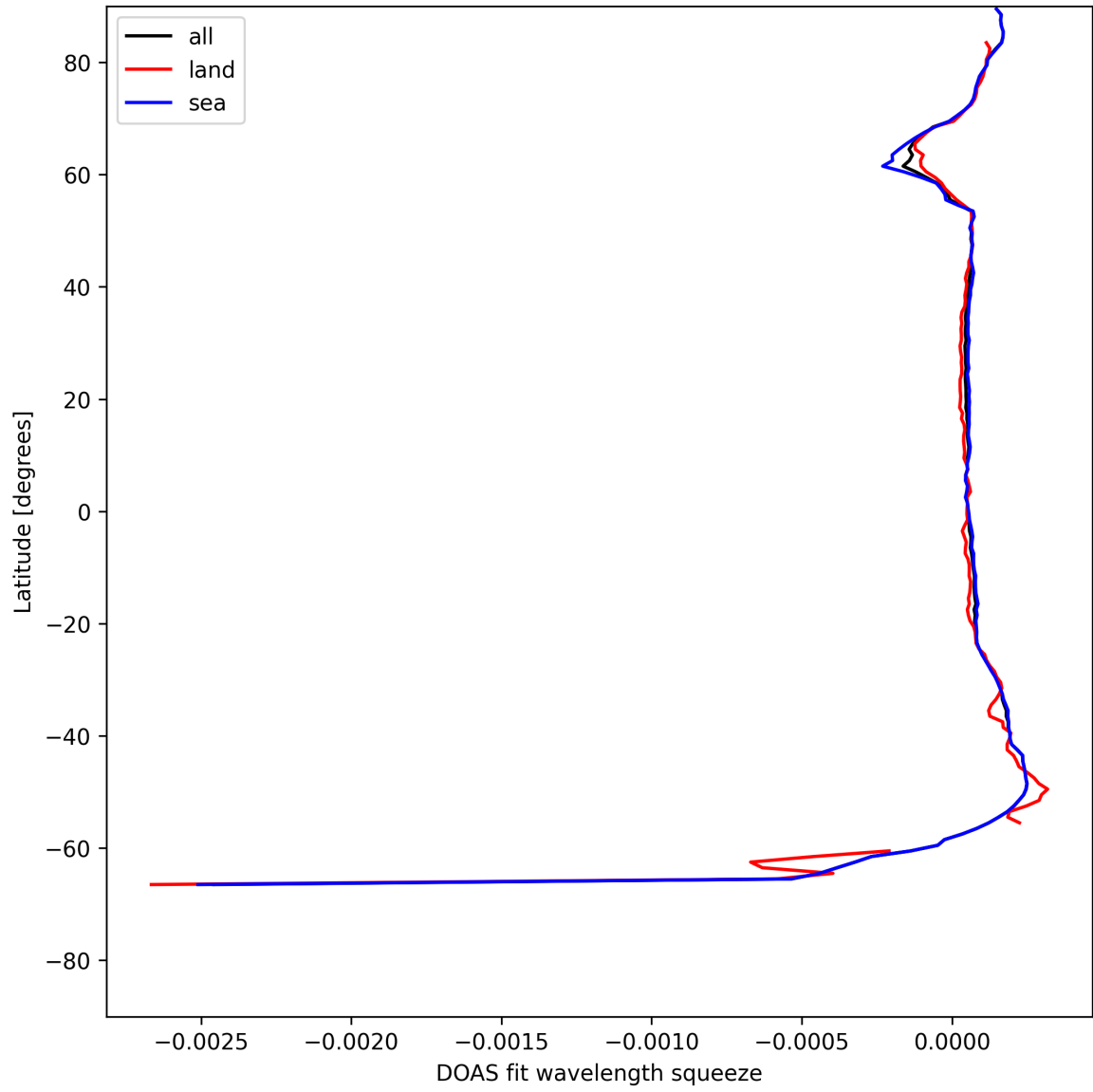
Figure 24: Zonal average of “DOAS fit wavelength squeeze” for 2025-06-04 to 2025-06-04.
