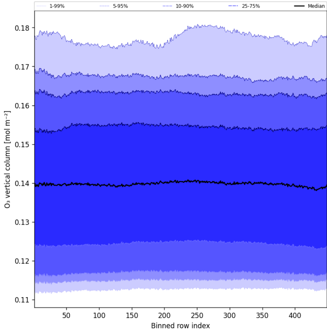
Figure 41: Along track statistics of “O 3 vertical column” for 2025-06-04 to 2025-06-04
