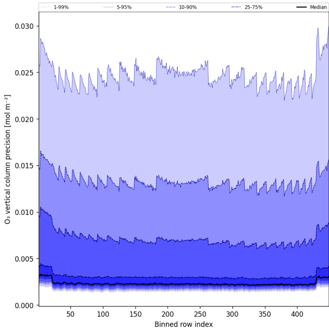
Figure 42: Along track statistics of “O 3 vertical column precision” for 2025-06-05 to 2025-06-06
