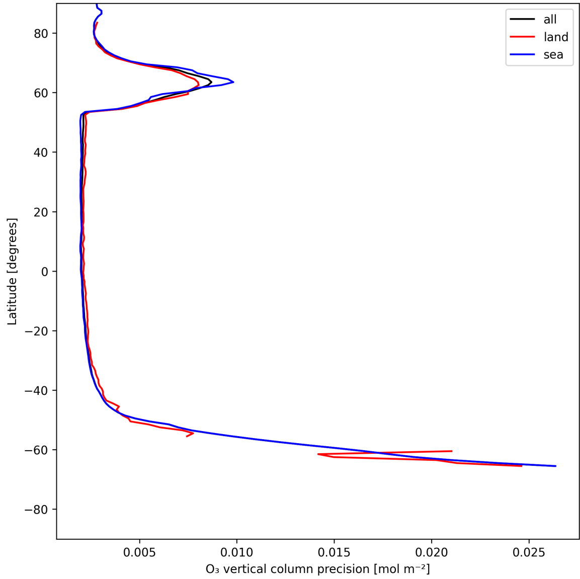
Figure 18: Zonal average of “O 3 vertical column precision” for 2025-06-05 to 2025-06-06.
