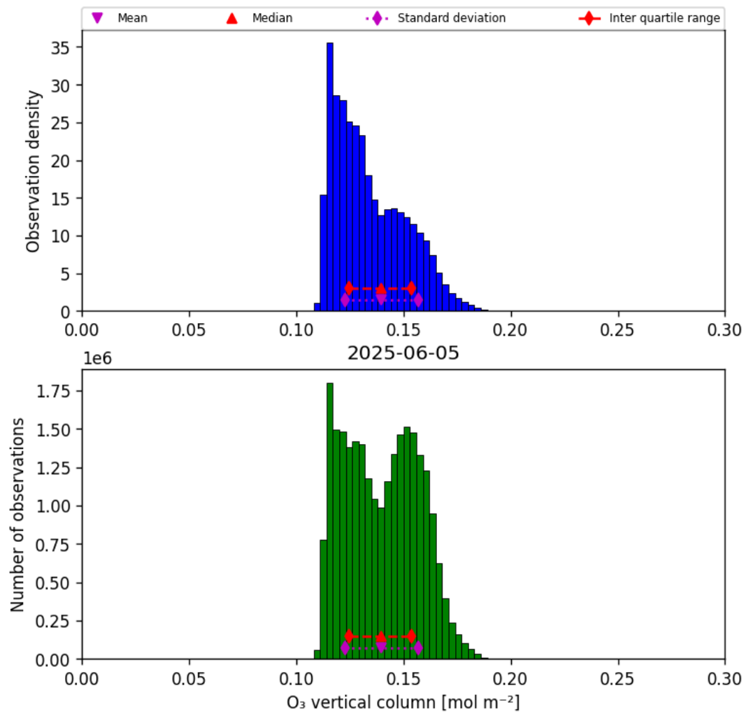
Figure 29: Histogram of “O 3 vertical column” for 2025-06-05 to 2025-06-06
