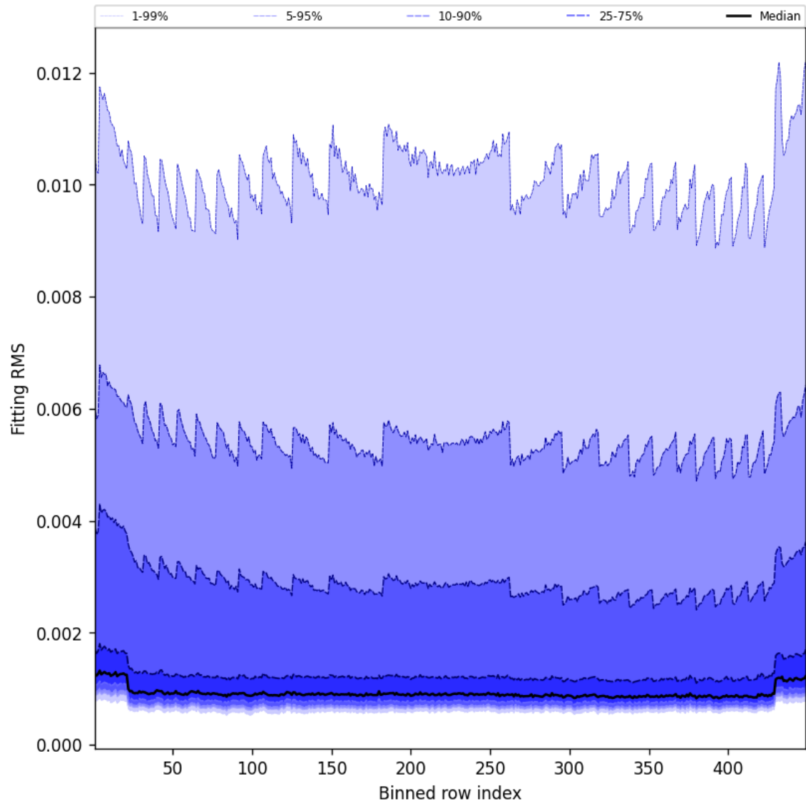
Figure 46: Along track statistics of “Fitting RMS” for 2025-06-05 to 2025-06-06
