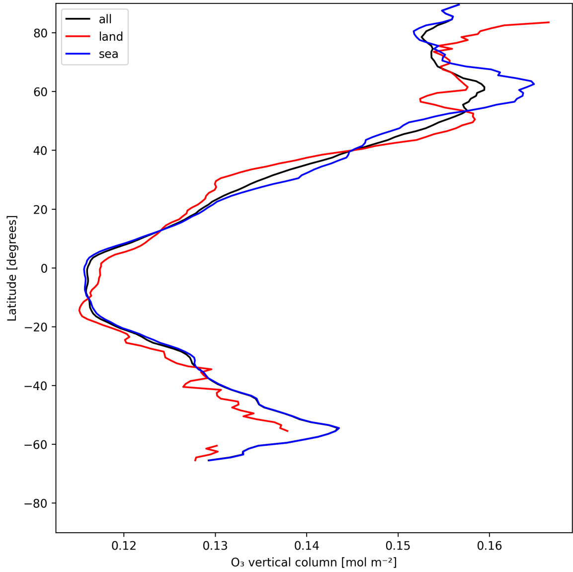
Figure 17: Zonal average of “O 3 vertical column” for 2025-06-05 to 2025-06-06.
