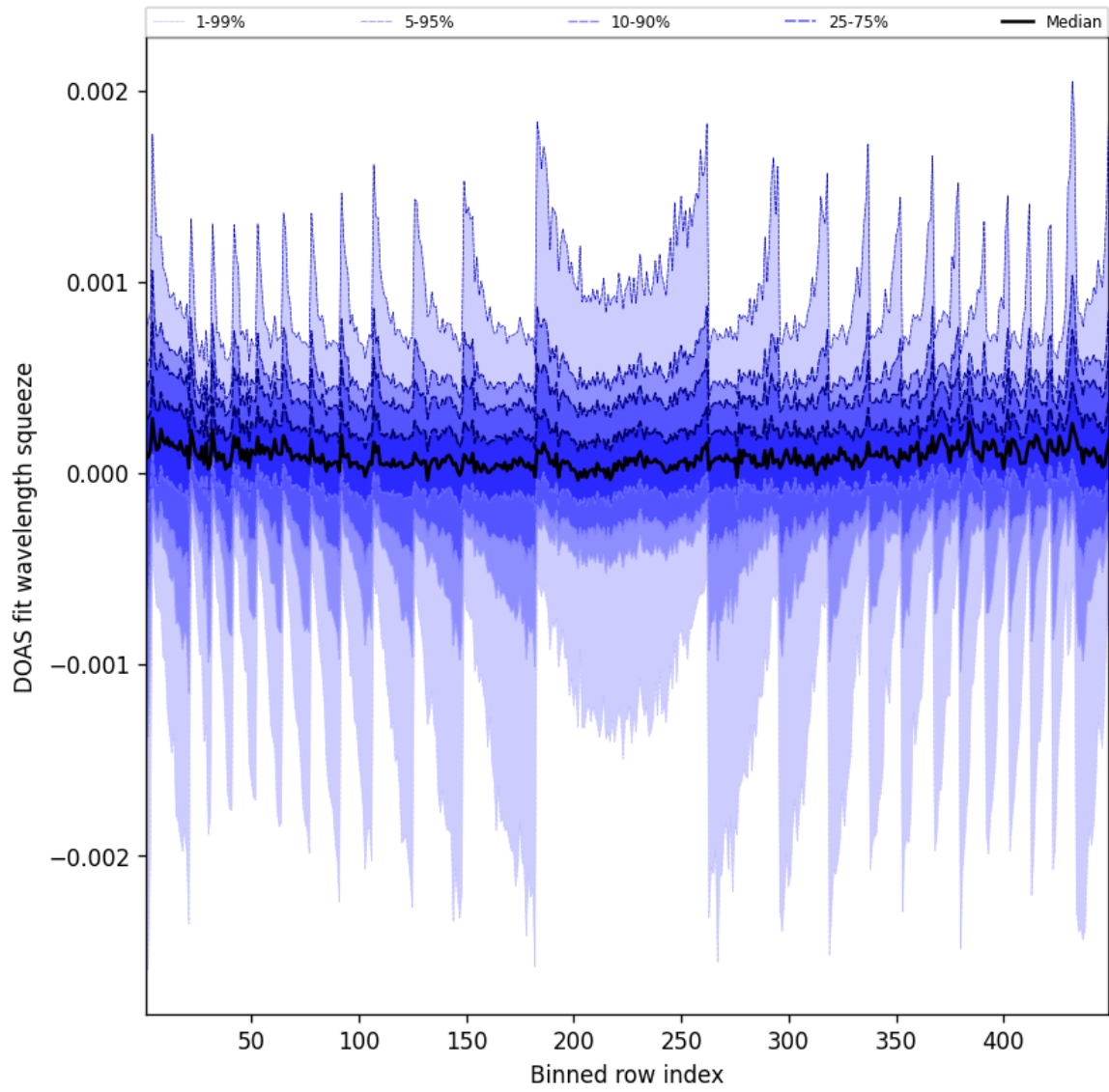
Figure 48: Along track statistics of “DOAS fit wavelength squeeze” for 2025-06-05 to 2025-06-06
