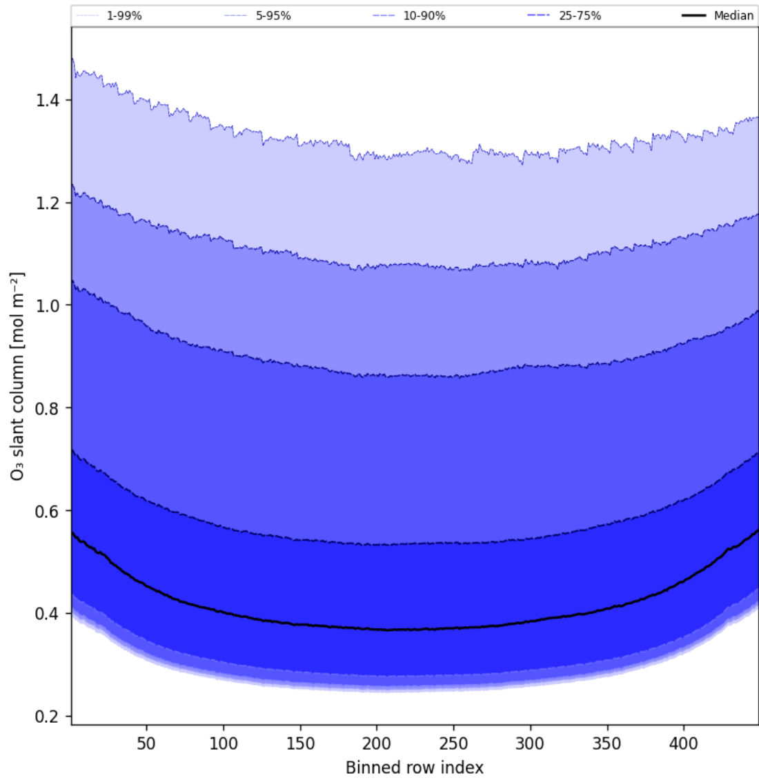
Figure 43: Along track statistics of “O 3 slant column” for 2025-06-05 to 2025-06-06
