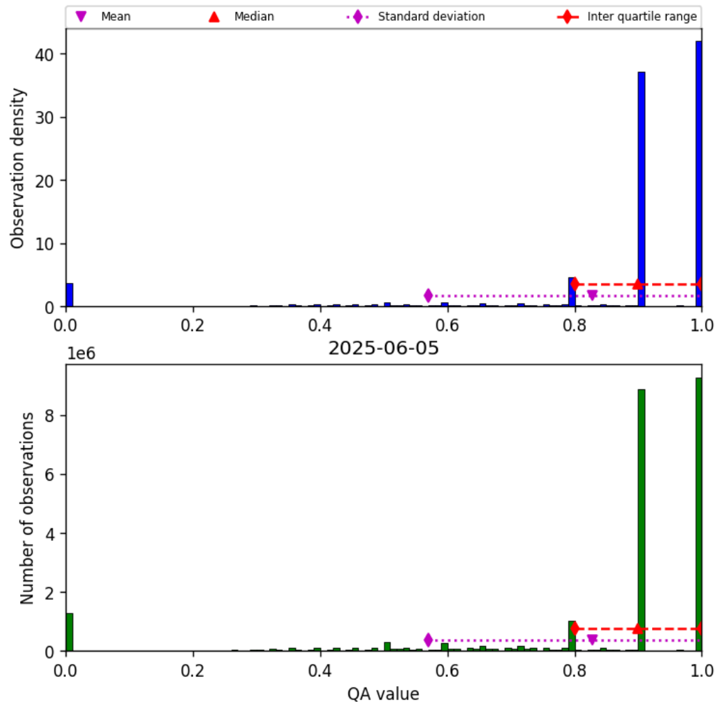
Figure 28: Histogram of “QA value” for 2025-06-05 to 2025-06-06
