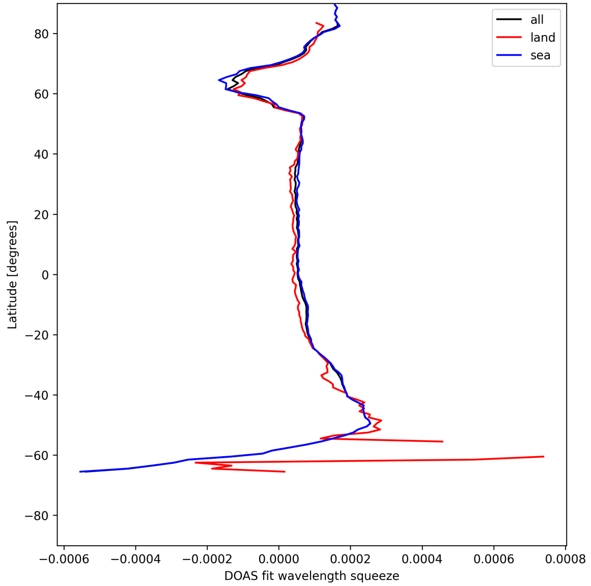
Figure 24: Zonal average of “DOAS fit wavelength squeeze” for 2025-06-05 to 2025-06-06.
