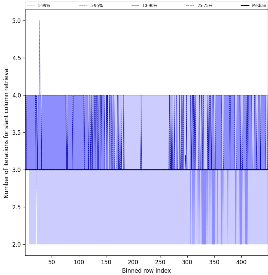
Figure 45: Along track statistics of “Number of iterations for slant column retrieval” for 2025-06-05 to 2025-06-06
