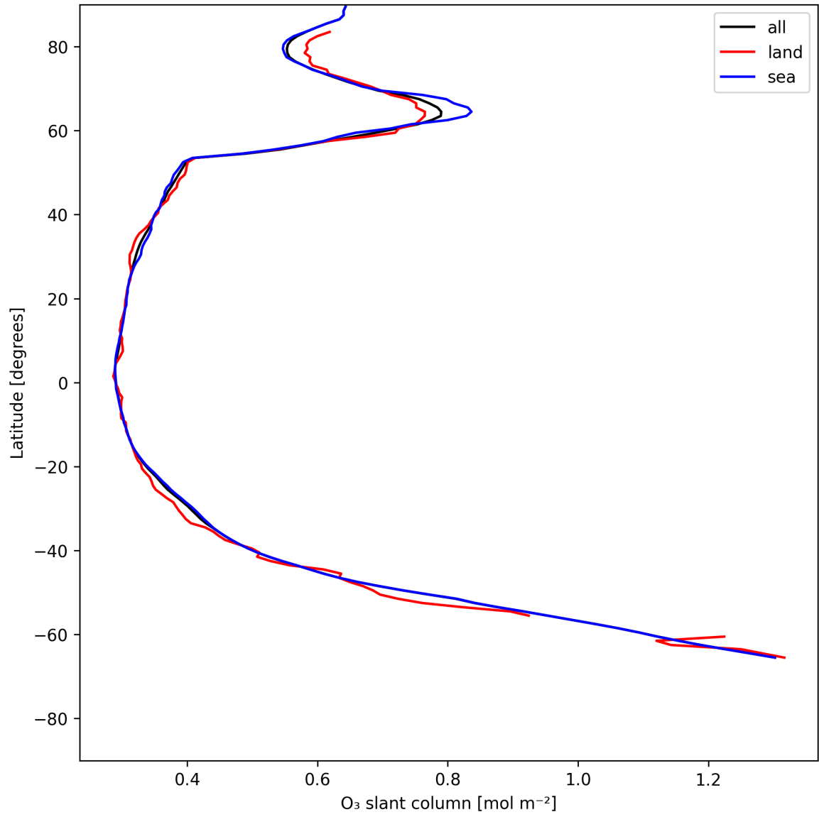
Figure 19: Zonal average of “O 3 slant column” for 2025-06-05 to 2025-06-06.
