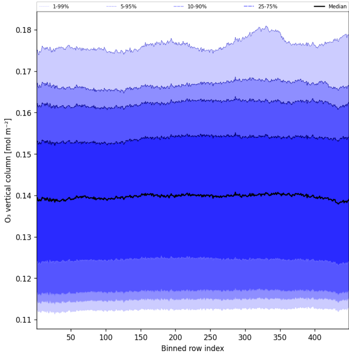
Figure 41: Along track statistics of “O 3 vertical column” for 2025-06-05 to 2025-06-06
