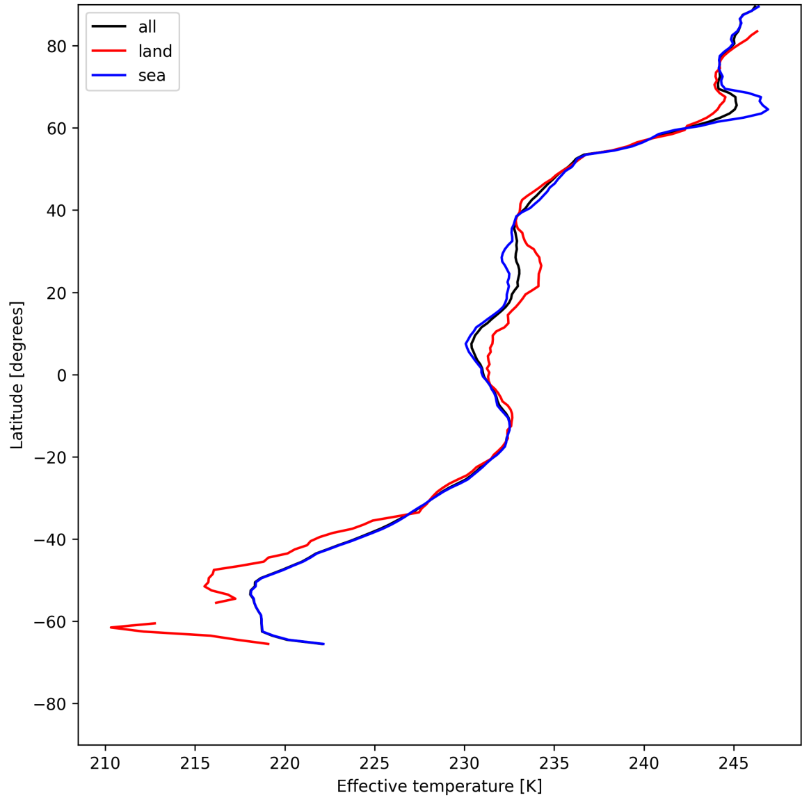
Figure 26: Zonal average of "Effective temperature" for 2025-06-05 to 2025-06-06.
