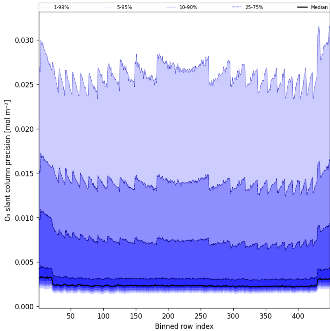
Figure 44: Along track statistics of “O 3 slant column precision” for 2025-06-05 to 2025-06-06
