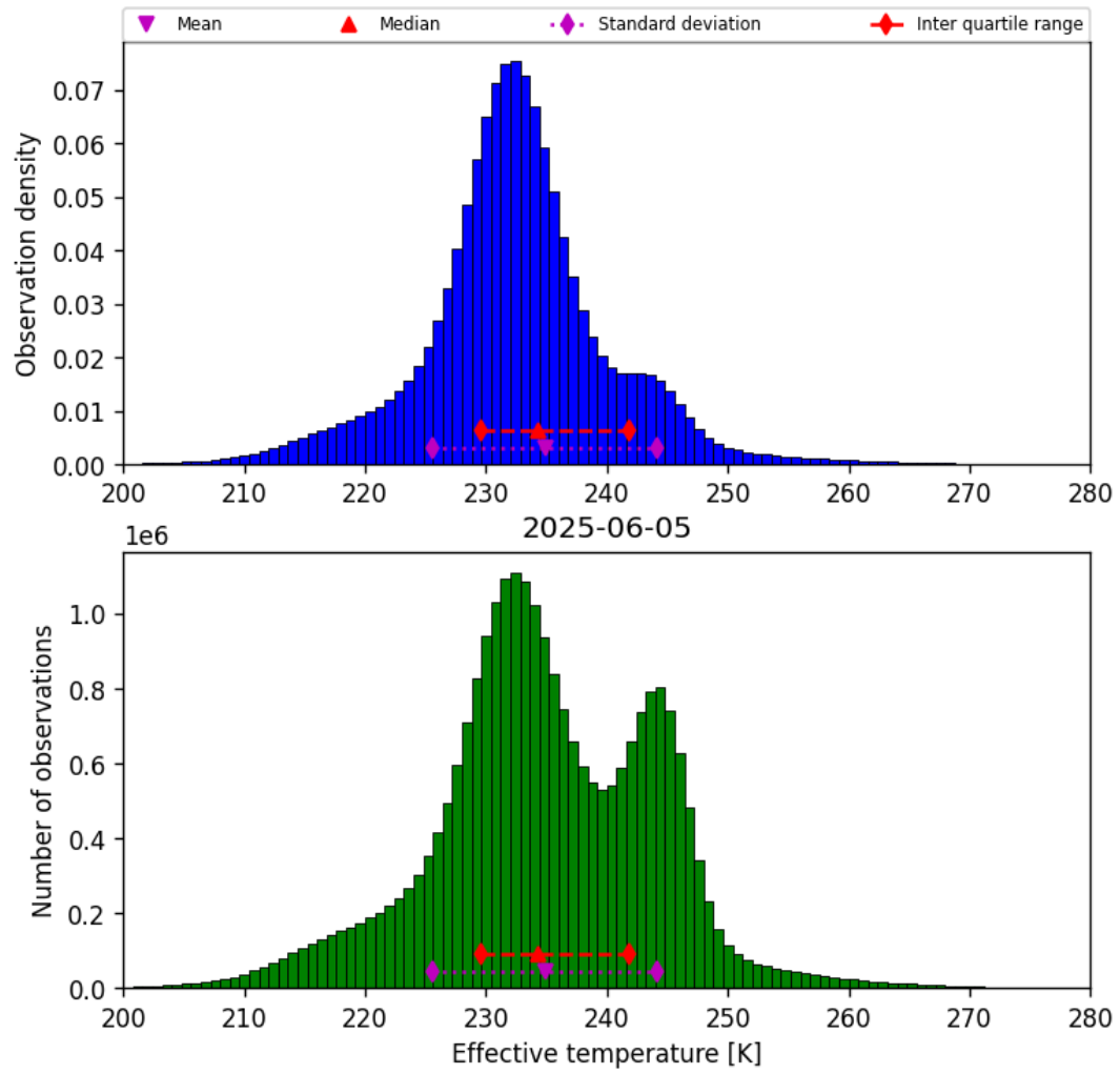
Figure 38: Histogram of “Effective temperature” for 2025-06-05 to 2025-06-06
