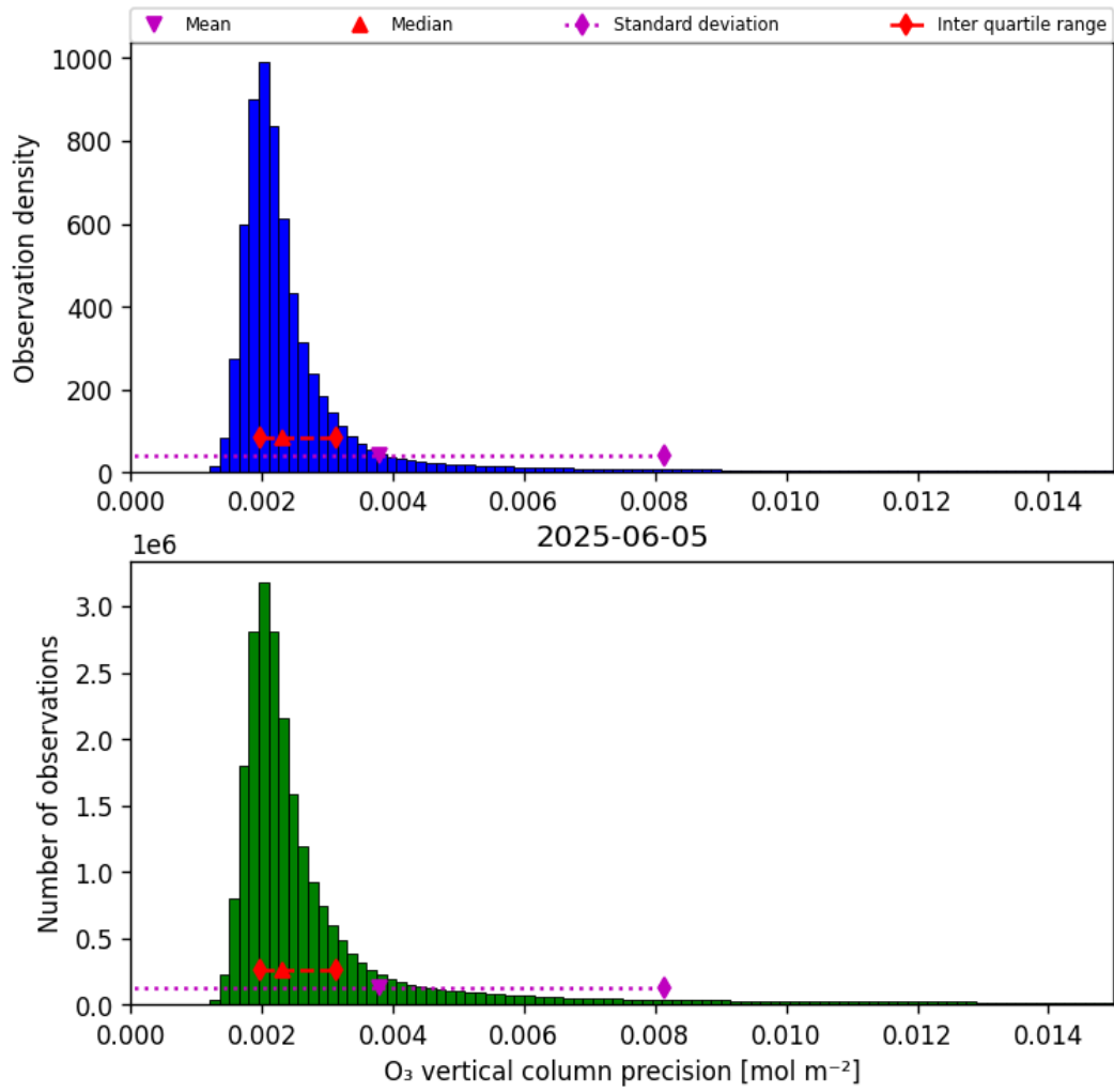
Figure 30: Histogram of “O 3 vertical column precision” for 2025-06-05 to 2025-06-06
