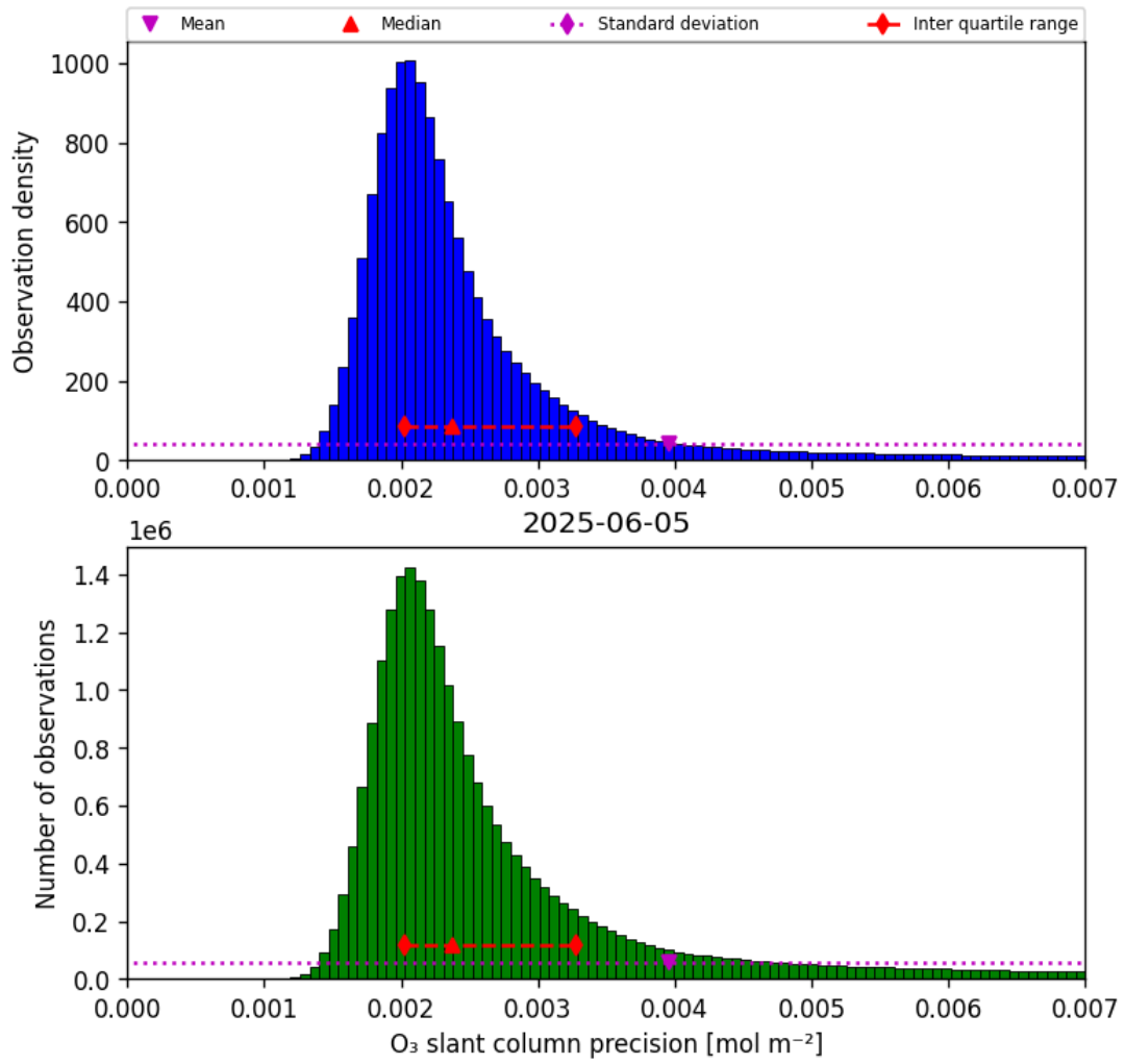
Figure 32: Histogram of “O 3 slant column precision” for 2025-06-05 to 2025-06-06
