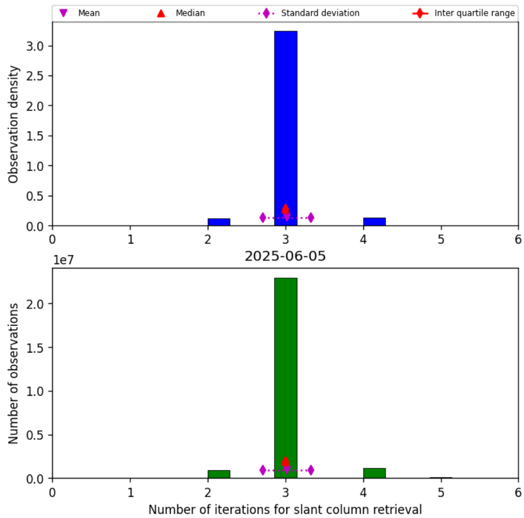
Figure 33: Histogram of “Number of iterations for slant column retrieval” for 2025-06-05 to 2025-06-06
