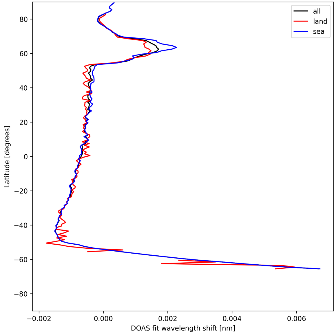
Figure 23: Zonal average of “DOAS fit wavelength shift” for 2025-06-05 to 2025-06-06.
