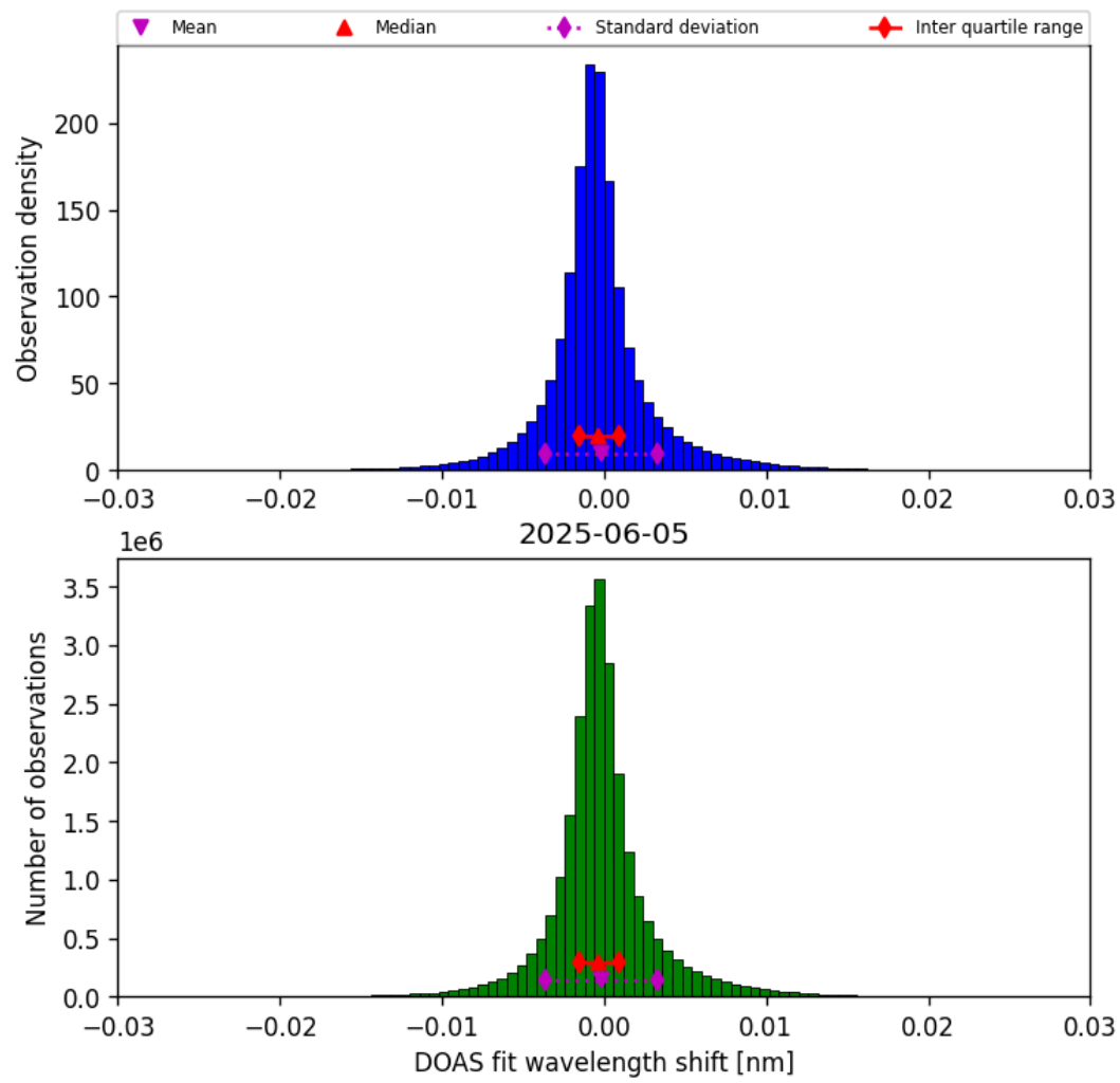
Figure 35: Histogram of “DOAS fit wavelength shift” for 2025-06-05 to 2025-06-06
