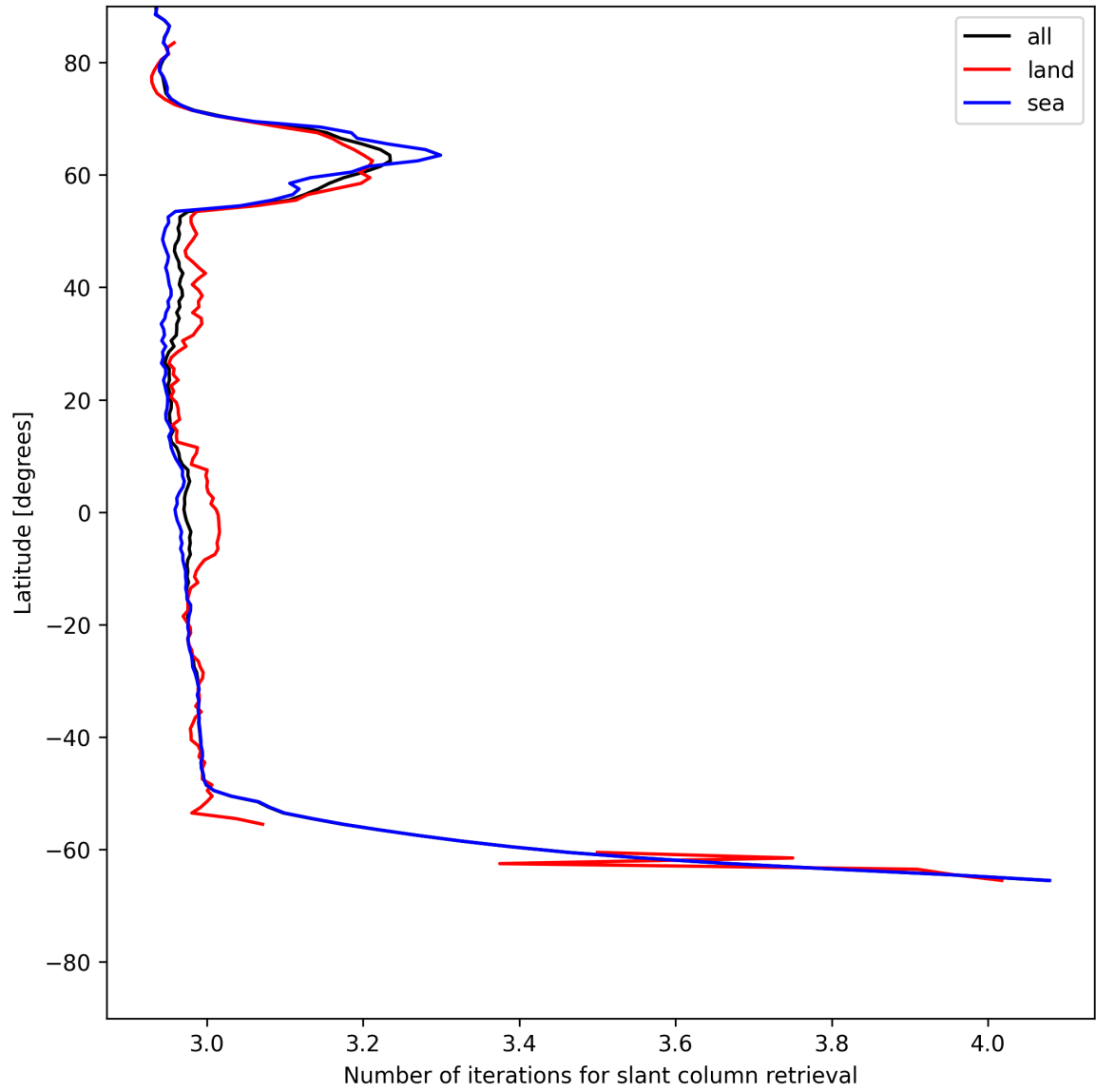
Figure 21: Zonal average of “Number of iterations for slant column retrieval” for 2025-06-05 to 2025-06-06.
