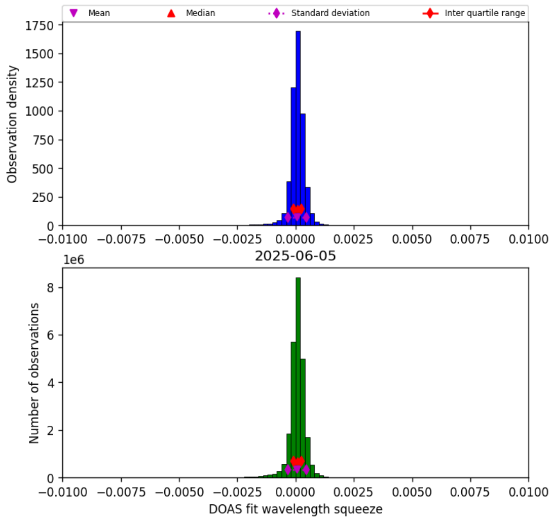
Figure 36: Histogram of “DOAS fit wavelength squeeze” for 2025-06-05 to 2025-06-06
