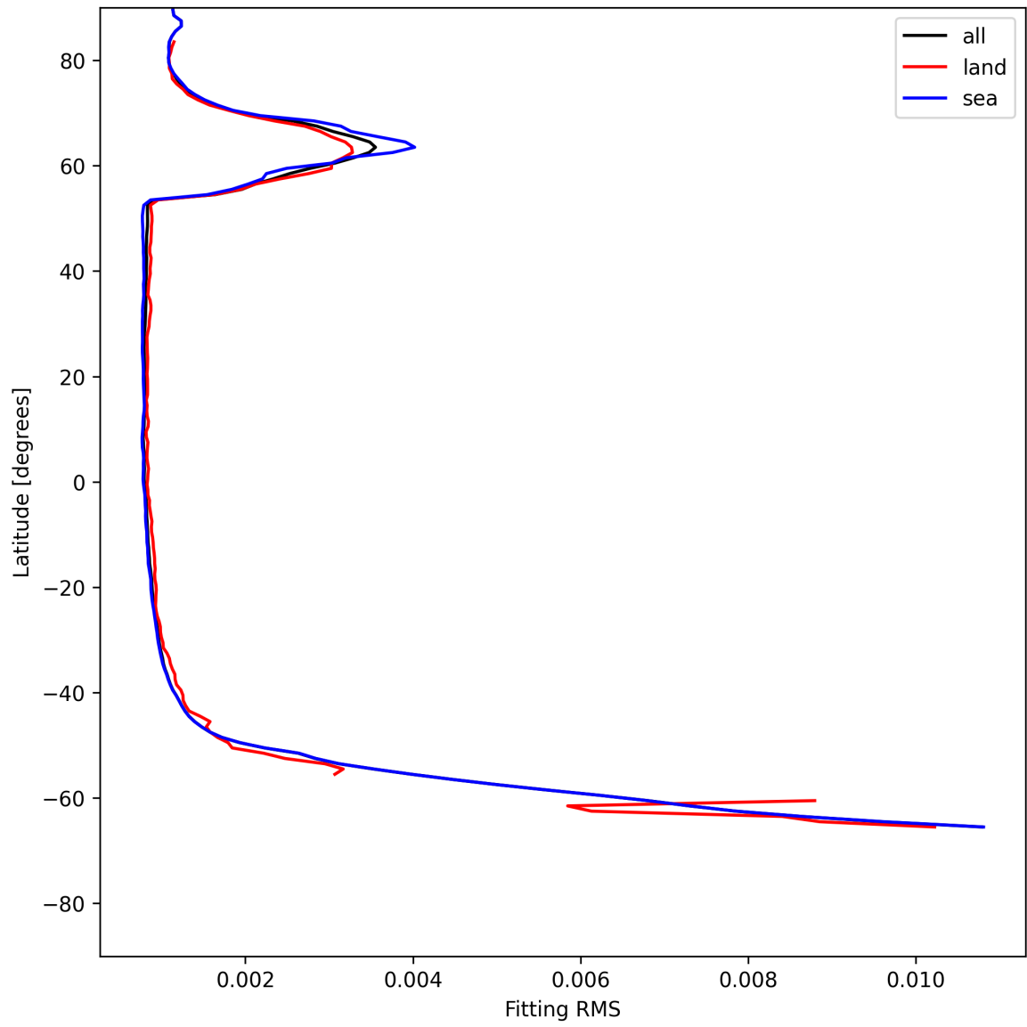
Figure 22: Zonal average of “Fitting RMS” for 2025-06-05 to 2025-06-06.
