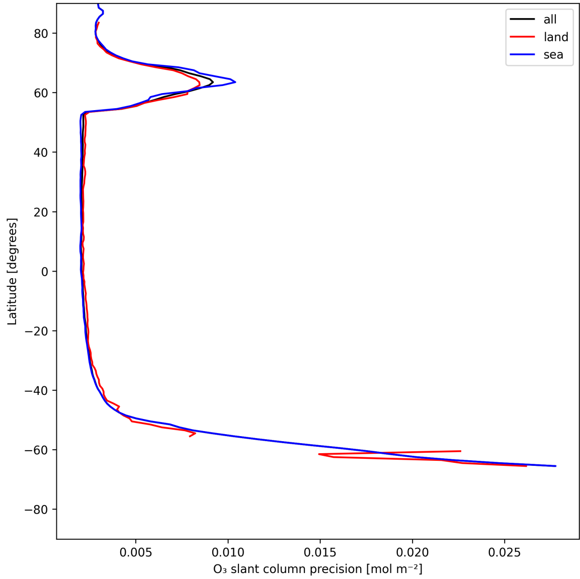
Figure 20: Zonal average of “O 3 slant column precision” for 2025-06-05 to 2025-06-06.
