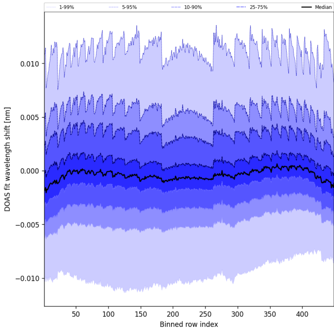
Figure 47: Along track statistics of “DOAS fit wavelength shift” for 2025-06-05 to 2025-06-06
