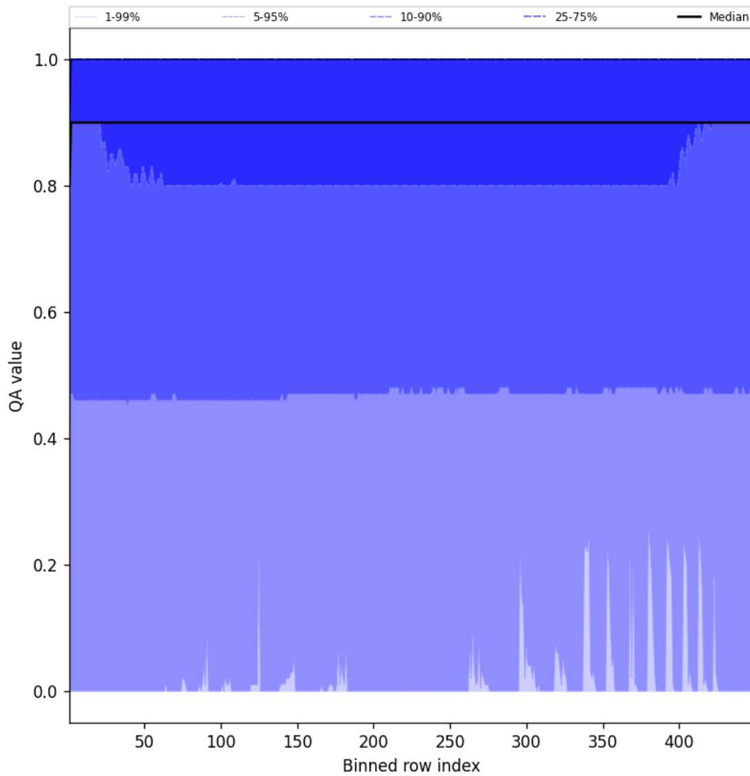
Figure 40: Along track statistics of “QA value” for 2025-06-05 to 2025-06-06
