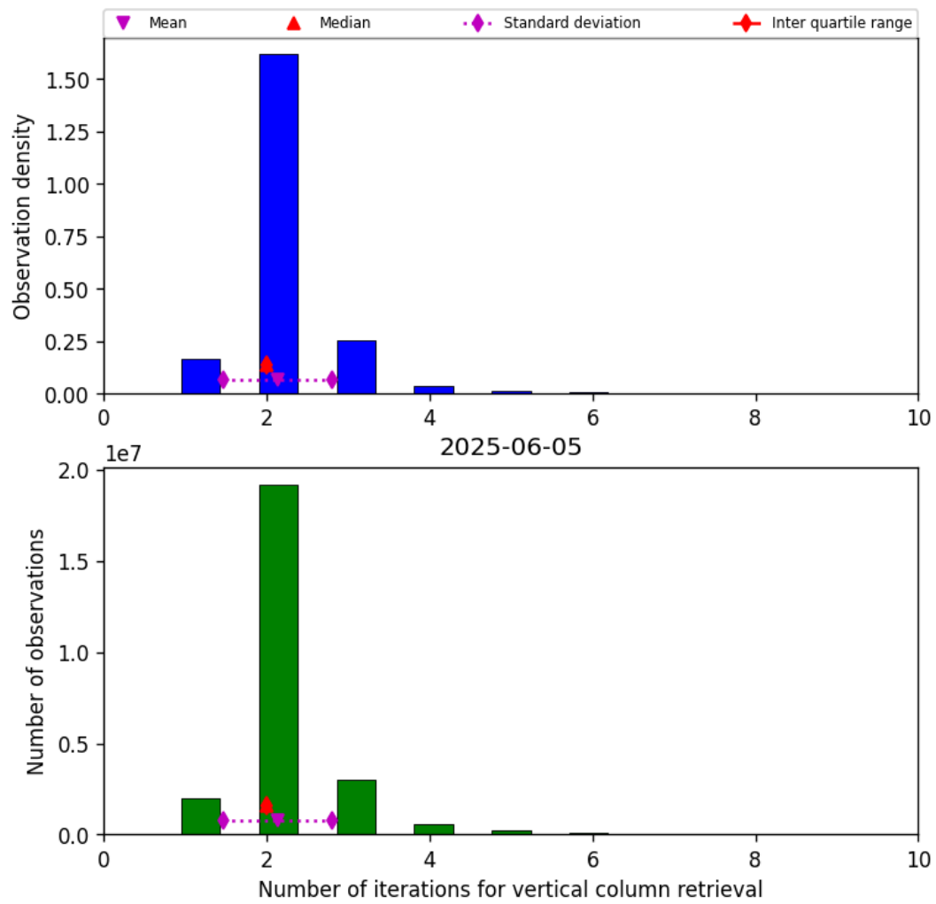
Figure 39: Histogram of “Number of iterations for vertical column retrieval” for 2025-06-05 to 2025-06-06
