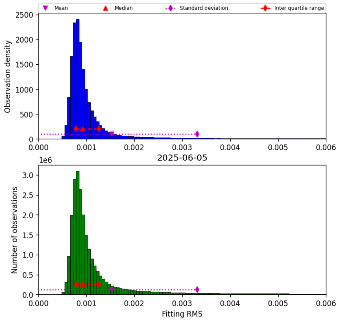
Figure 34: Histogram of “Fitting RMS” for 2025-06-05 to 2025-06-06
