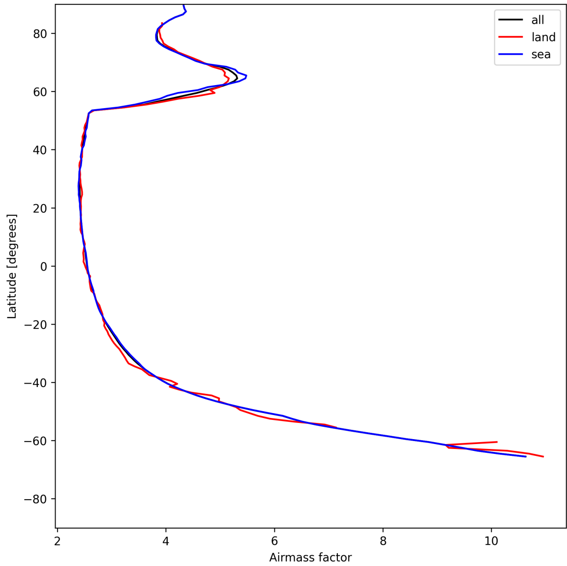
Figure 25: Zonal average of “Airmass factor” for 2025-06-05 to 2025-06-06.
