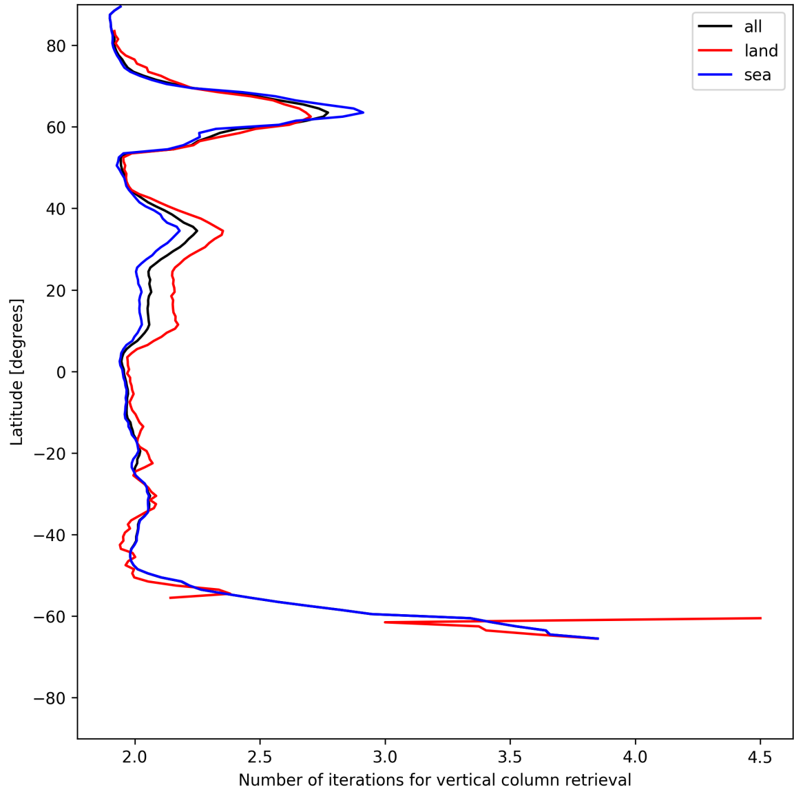
Figure 27: Zonal average of “Number of iterations for vertical column retrieval” for 2025-06-05 to 2025-06-06.
