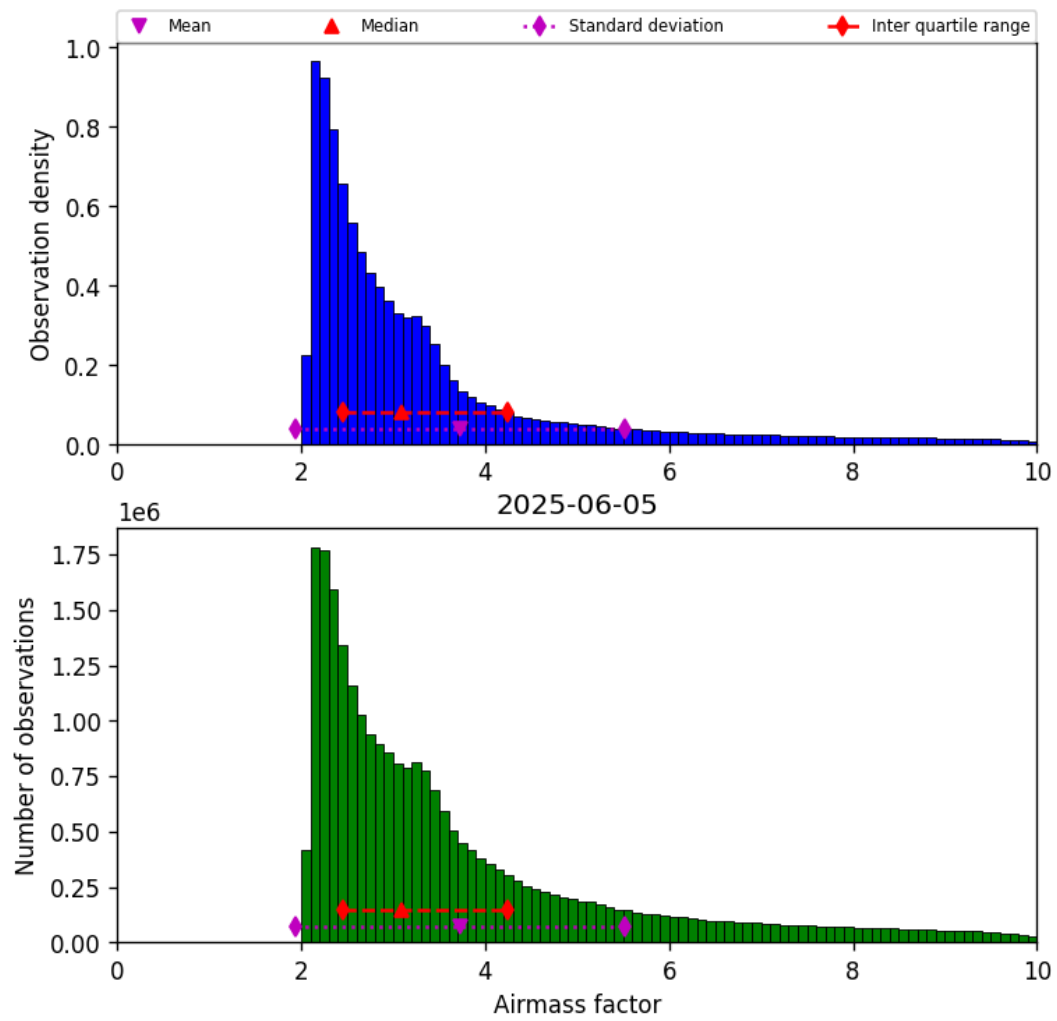
Figure 37: Histogram of “Airmass factor” for 2025-06-05 to 2025-06-06
