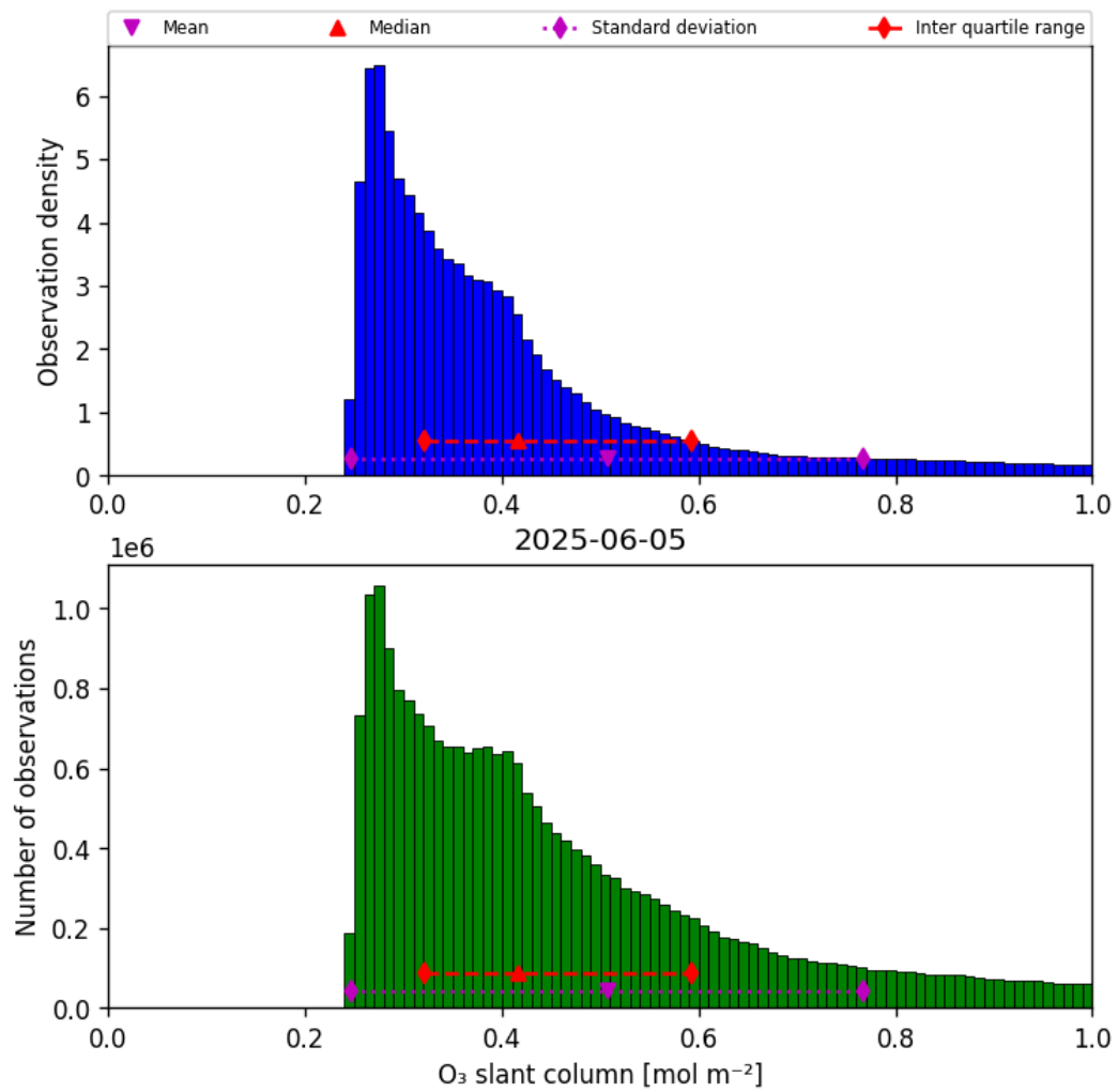
Figure 31: Histogram of “O 3 slant column” for 2025-06-05 to 2025-06-06
