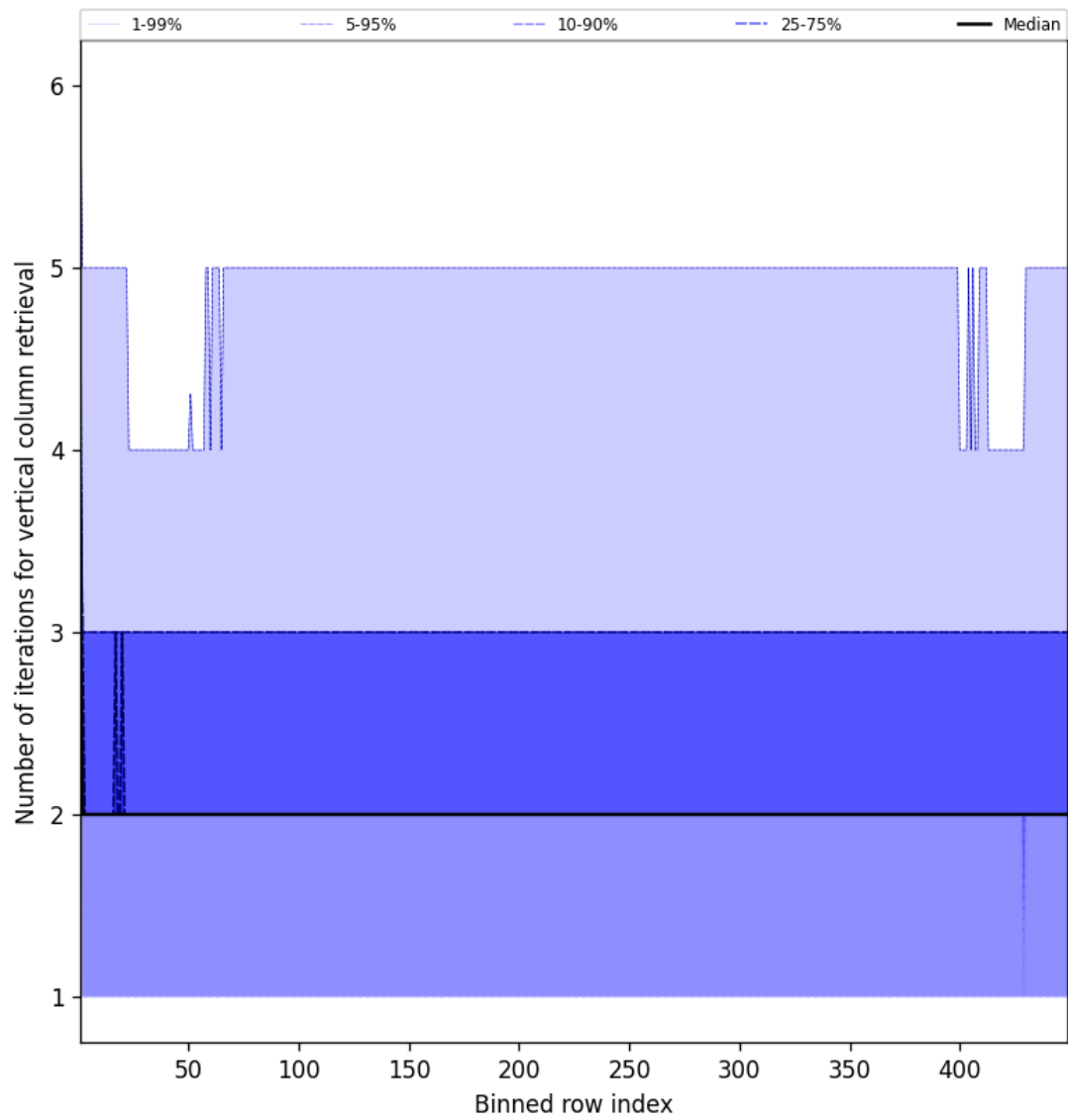
Figure 51: Along track statistics of “Number of iterations for vertical column retrieval” for 2025-06-05 to 2025-06-06
