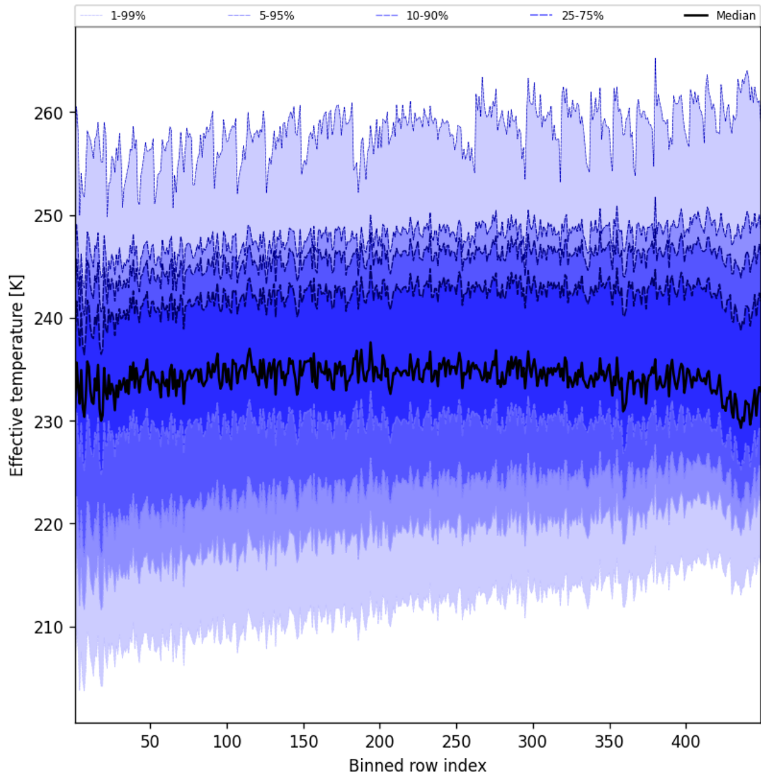
Figure 50: Along track statistics of “Effective temperature” for 2025-06-05 to 2025-06-06
