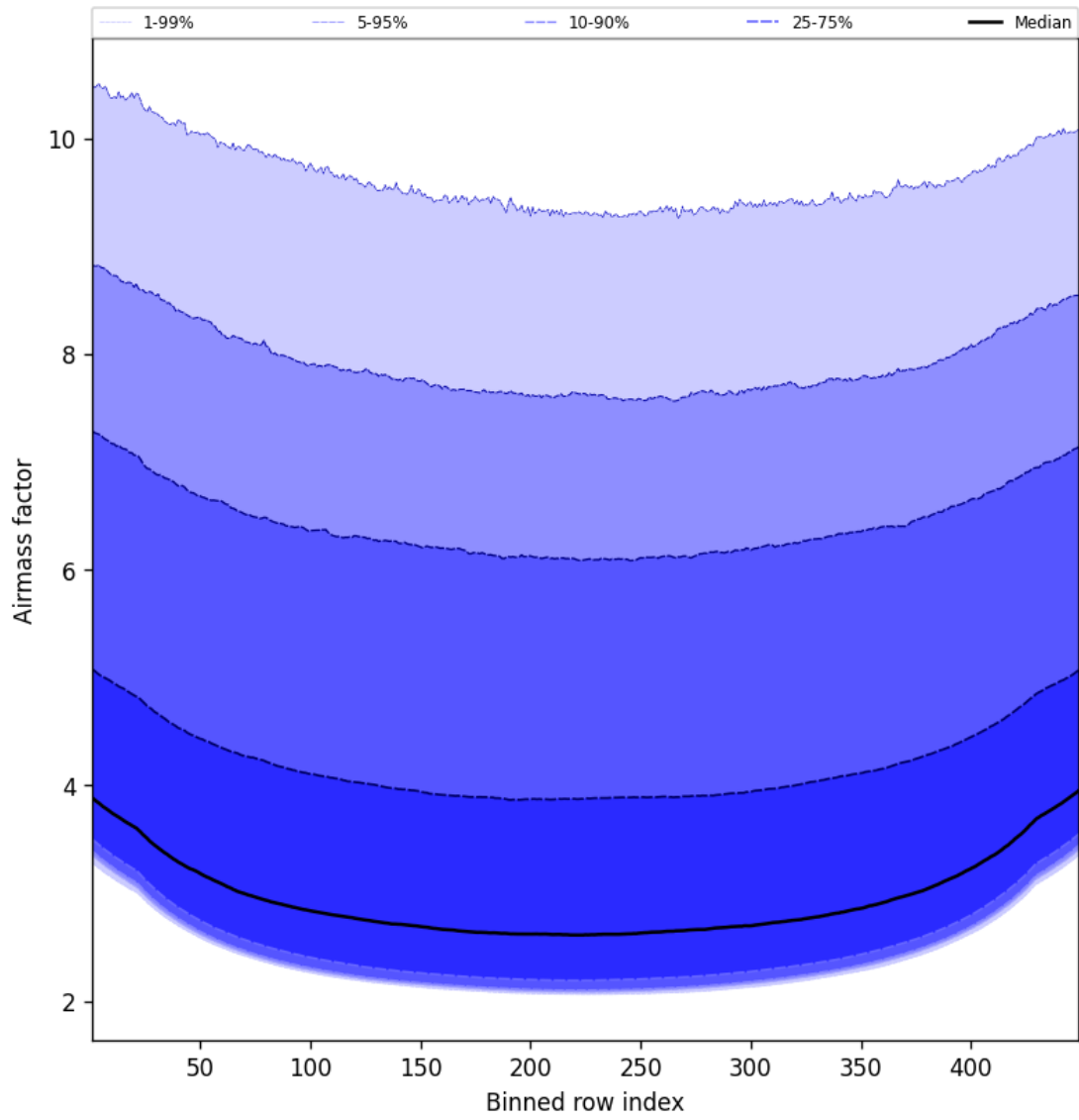
Figure 49: Along track statistics of “Airmass factor” for 2025-06-05 to 2025-06-06
