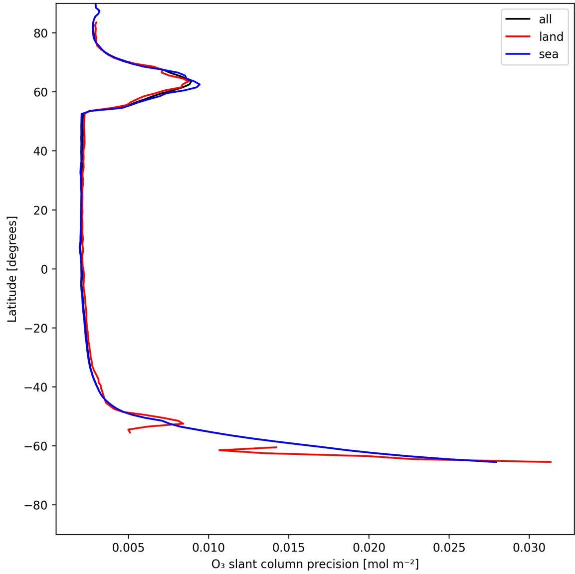
Figure 20: Zonal average of “O 3 slant column precision” for 2025-06-07 to 2025-06-08.
