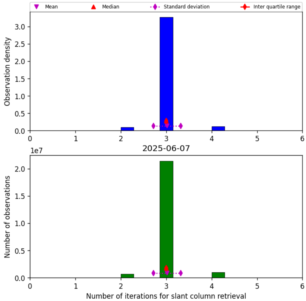
Figure 33: Histogram of “Number of iterations for slant column retrieval” for 2025-06-07 to 2025-06-08
