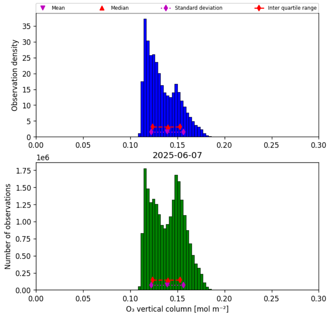
Figure 29: Histogram of “O 3 vertical column” for 2025-06-07 to 2025-06-08
