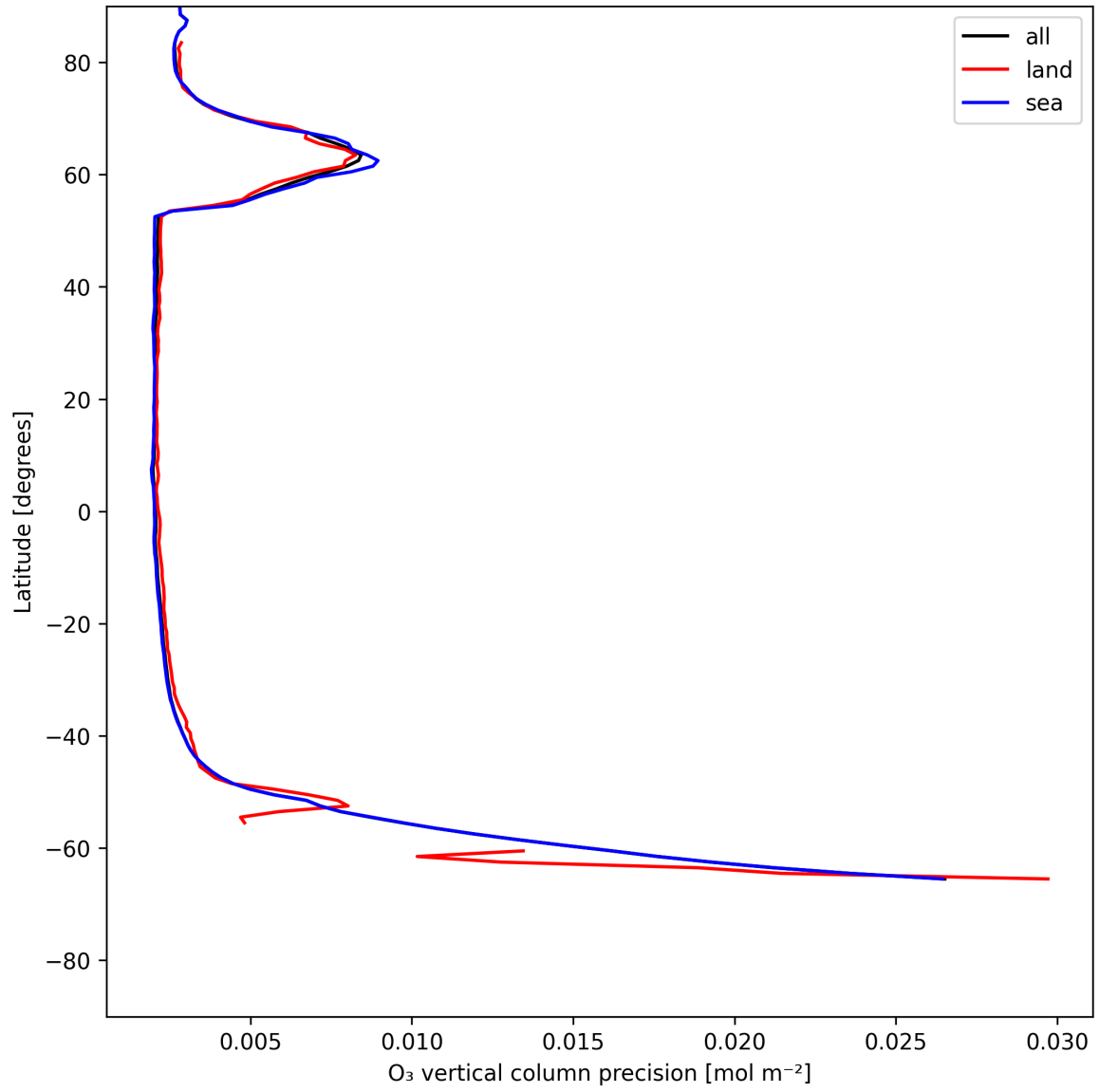
Figure 18: Zonal average of “O 3 vertical column precision” for 2025-06-07 to 2025-06-08.
