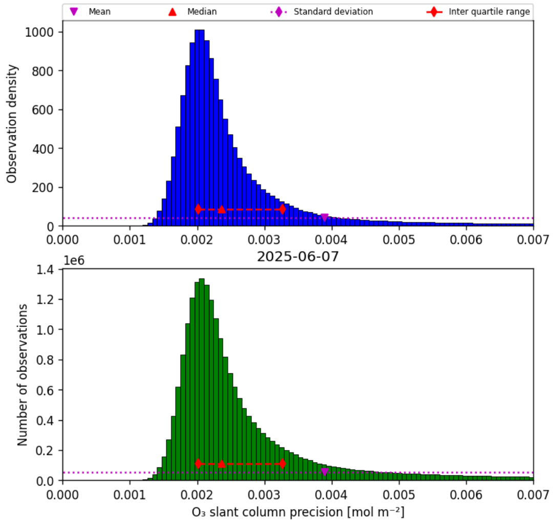
Figure 32: Histogram of “O 3 slant column precision” for 2025-06-07 to 2025-06-08
