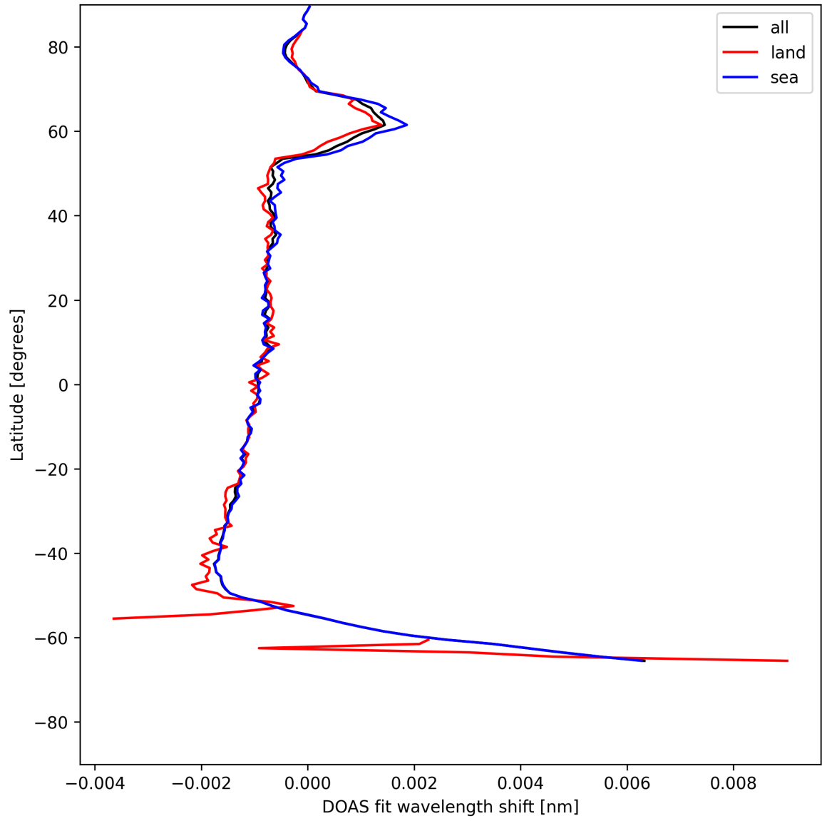
Figure 23: Zonal average of “DOAS fit wavelength shift” for 2025-06-07 to 2025-06-08.
