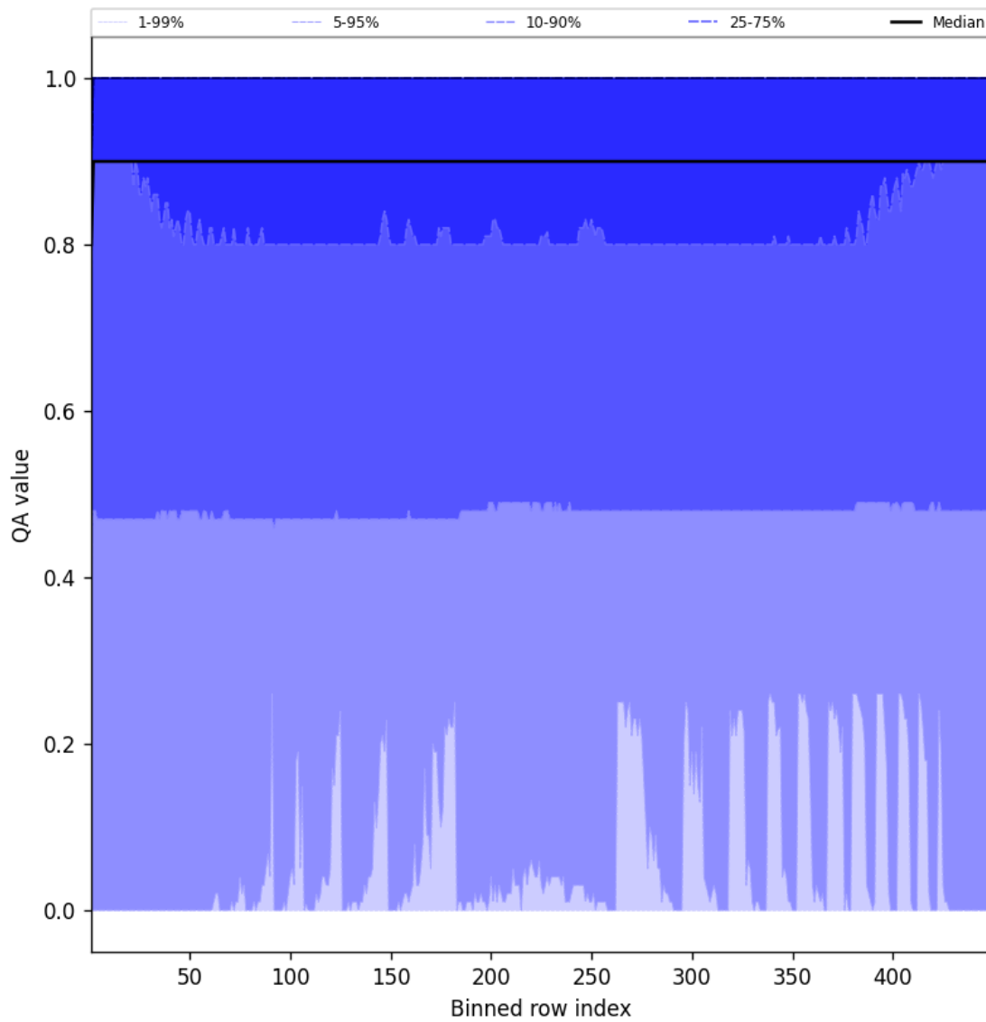
Figure 40: Along track statistics of “QA value” for 2025-06-07 to 2025-06-08
