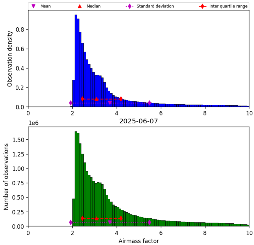
Figure 37: Histogram of “Airmass factor” for 2025-06-07 to 2025-06-08
