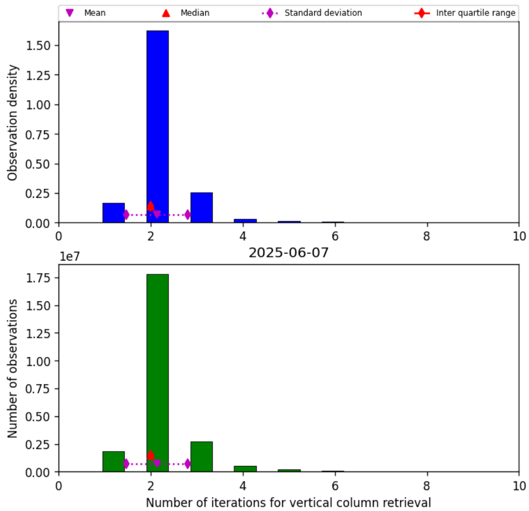
Figure 39: Histogram of “Number of iterations for vertical column retrieval” for 2025-06-07 to 2025-06-08
