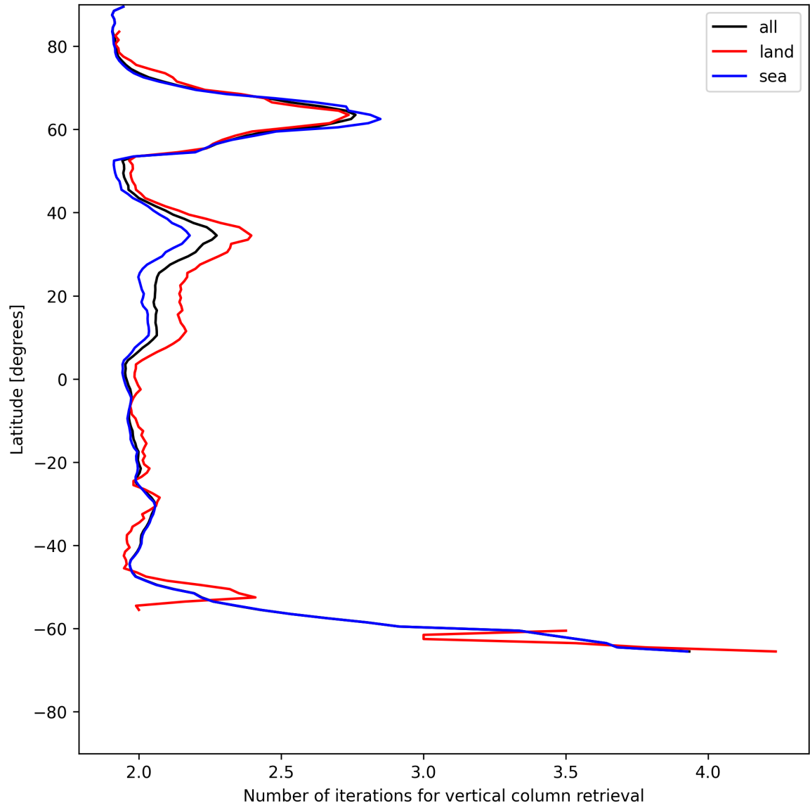
Figure 27: Zonal average of “Number of iterations for vertical column retrieval” for 2025-06-07 to 2025-06-08.
