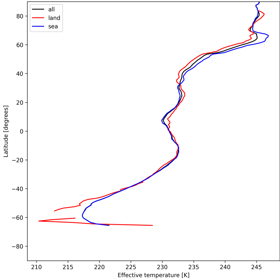
Figure 26: Zonal average of "Effective temperature" for 2025-06-07 to 2025-06-08.
