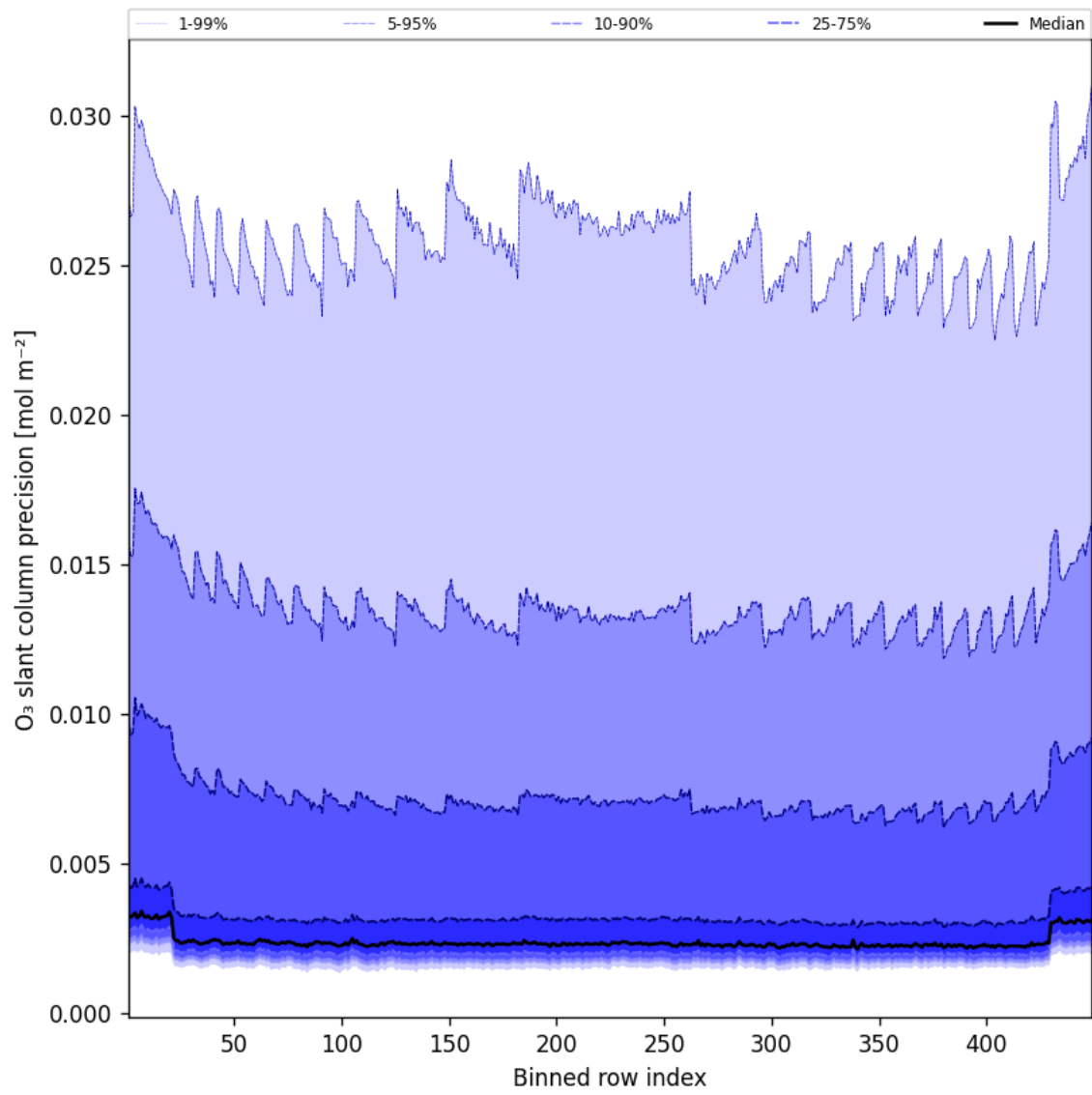
Figure 44: Along track statistics of “O 3 slant column precision” for 2025-06-07 to 2025-06-08
