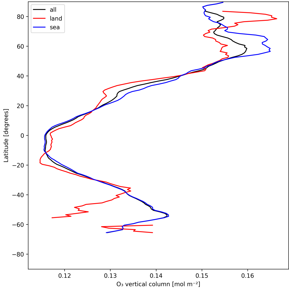
Figure 17: Zonal average of “O 3 vertical column” for 2025-06-07 to 2025-06-08.
