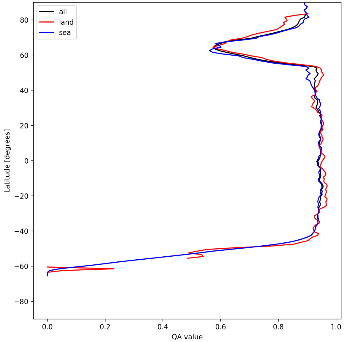
Figure 16: Zonal average of “QA value” for 2025-06-07 to 2025-06-08.
