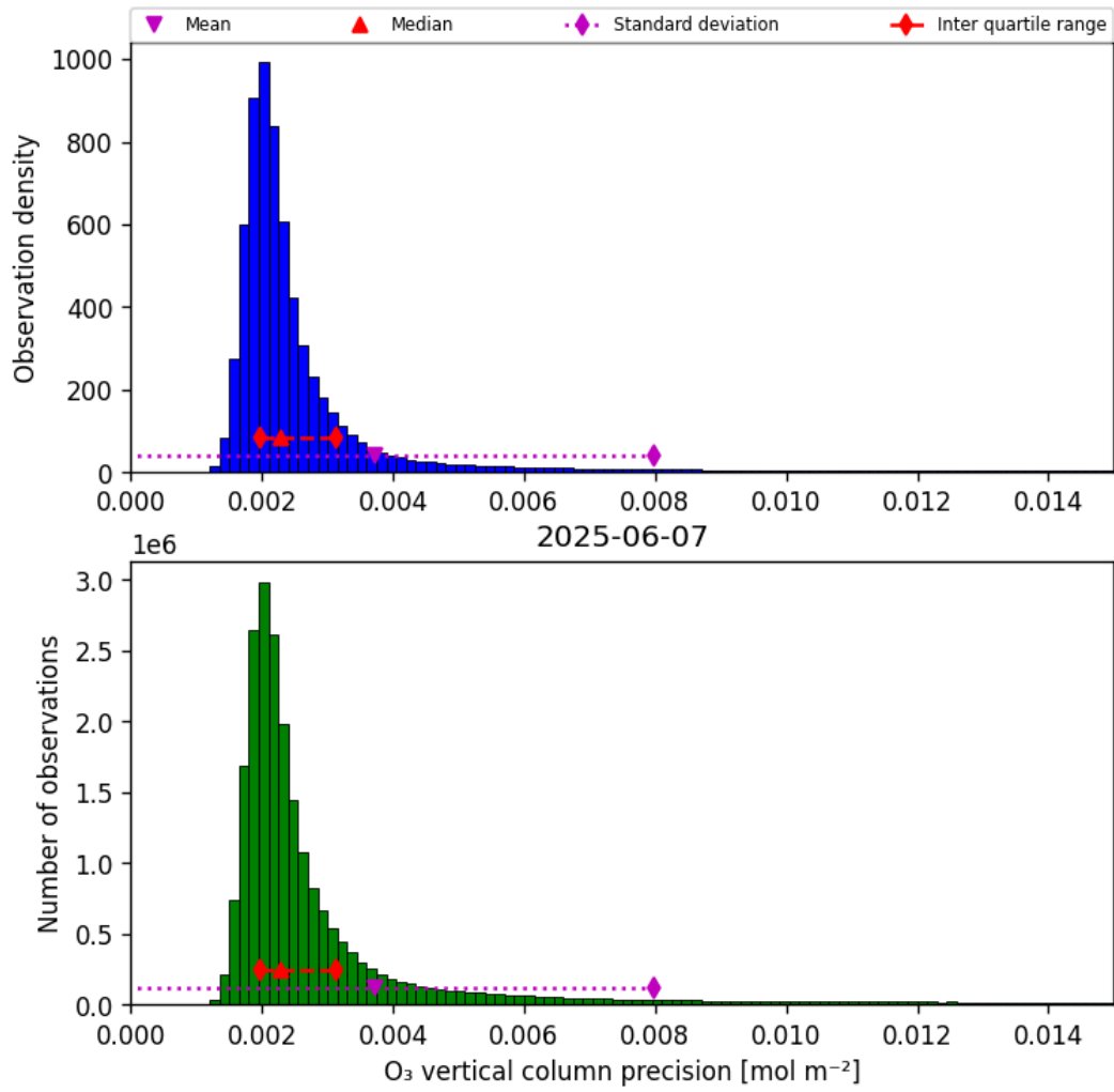
Figure 30: Histogram of “O 3 vertical column precision” for 2025-06-07 to 2025-06-08
