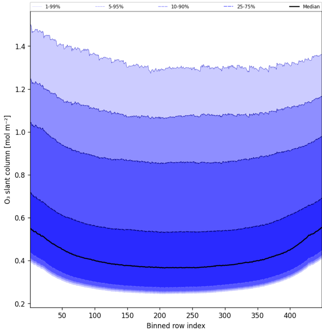
Figure 43: Along track statistics of “O 3 slant column” for 2025-06-07 to 2025-06-08
