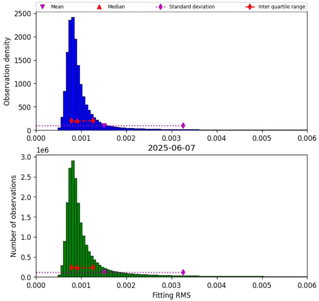
Figure 34: Histogram of “Fitting RMS” for 2025-06-07 to 2025-06-08
