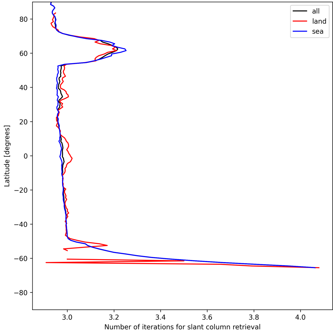
Figure 21: Zonal average of “Number of iterations for slant column retrieval” for 2025-06-07 to 2025-06-08.
