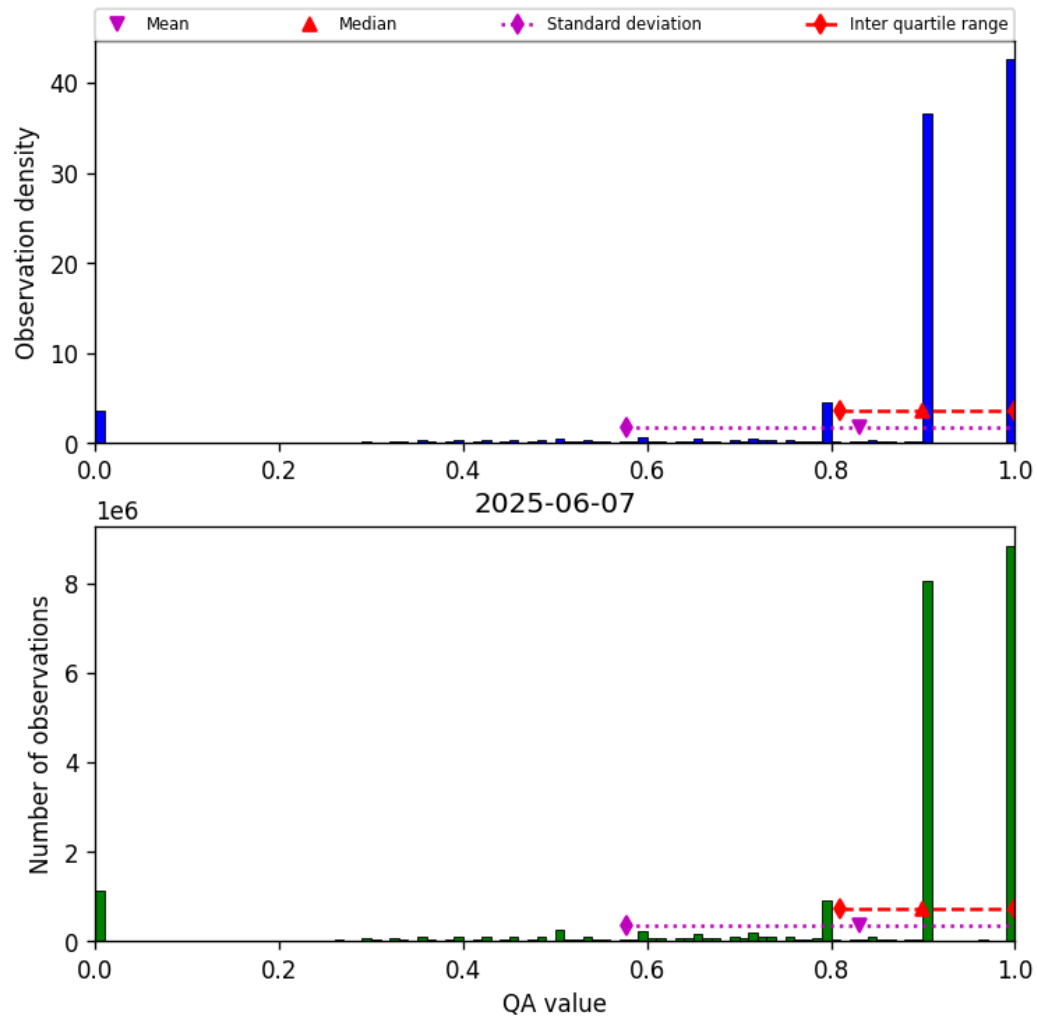
Figure 28: Histogram of “QA value” for 2025-06-07 to 2025-06-08
