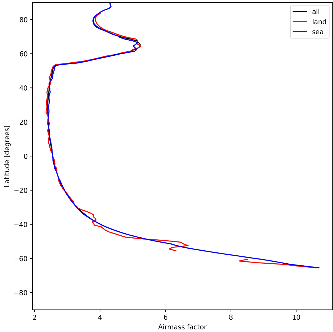
Figure 25: Zonal average of “Airmass factor” for 2025-06-07 to 2025-06-08.
