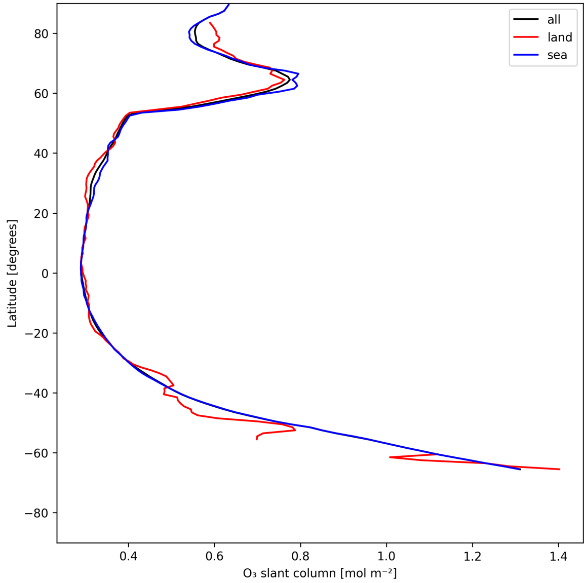
Figure 19: Zonal average of “O 3 slant column” for 2025-06-07 to 2025-06-08.
