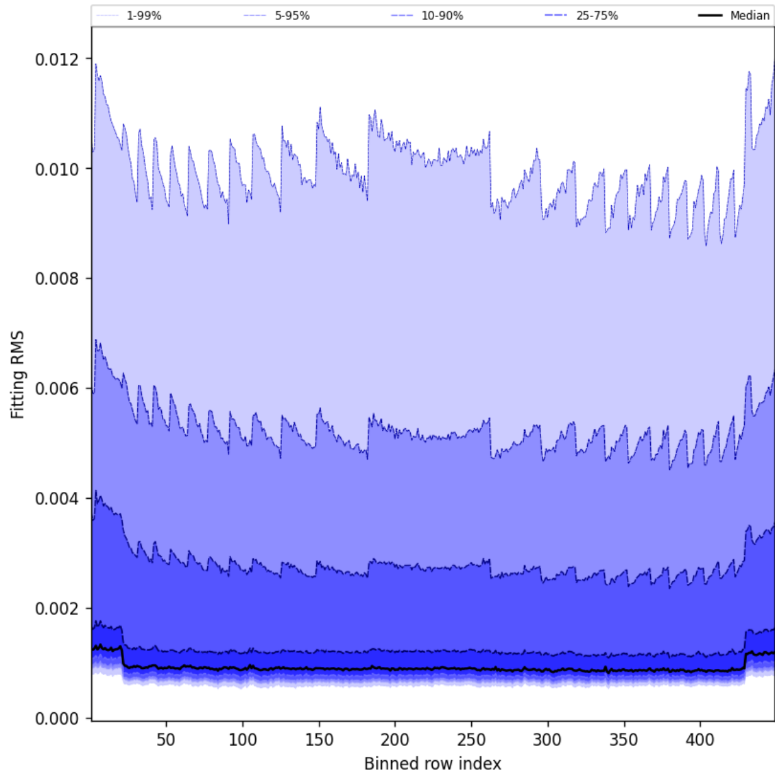
Figure 46: Along track statistics of “Fitting RMS” for 2025-06-07 to 2025-06-08
