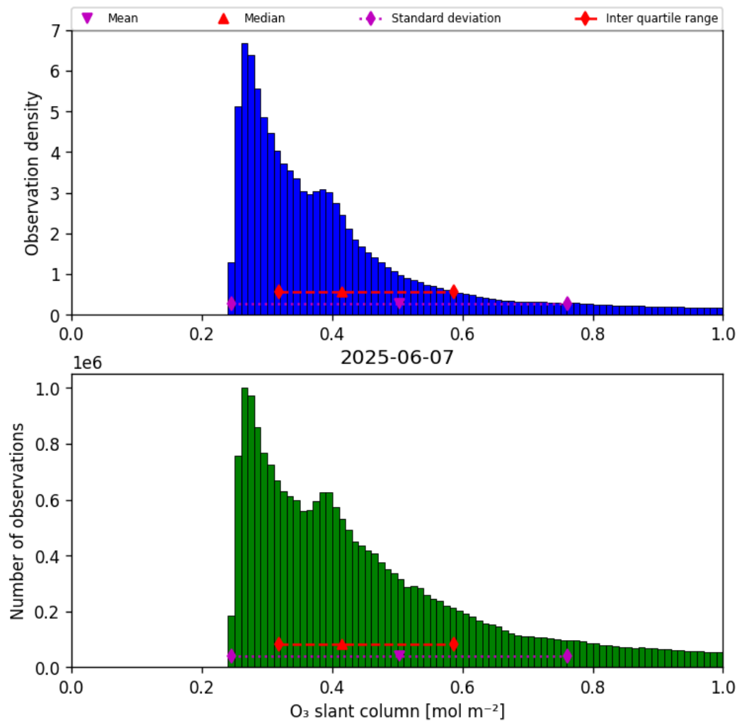
Figure 31: Histogram of “O 3 slant column” for 2025-06-07 to 2025-06-08
