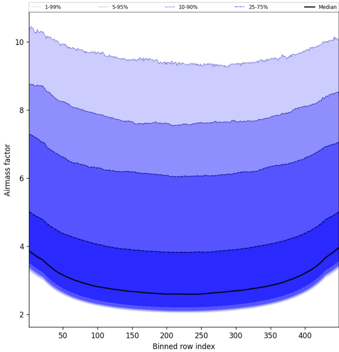
Figure 49: Along track statistics of “Airmass factor” for 2025-06-07 to 2025-06-08
