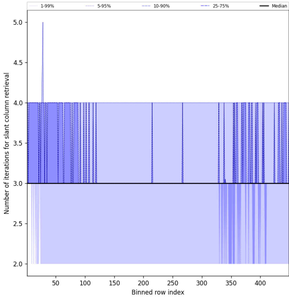
Figure 45: Along track statistics of “Number of iterations for slant column retrieval” for 2025-06-07 to 2025-06-08
