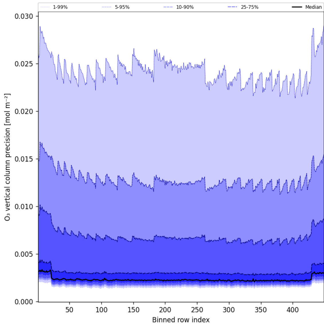
Figure 42: Along track statistics of “O 3 vertical column precision” for 2025-06-07 to 2025-06-08
