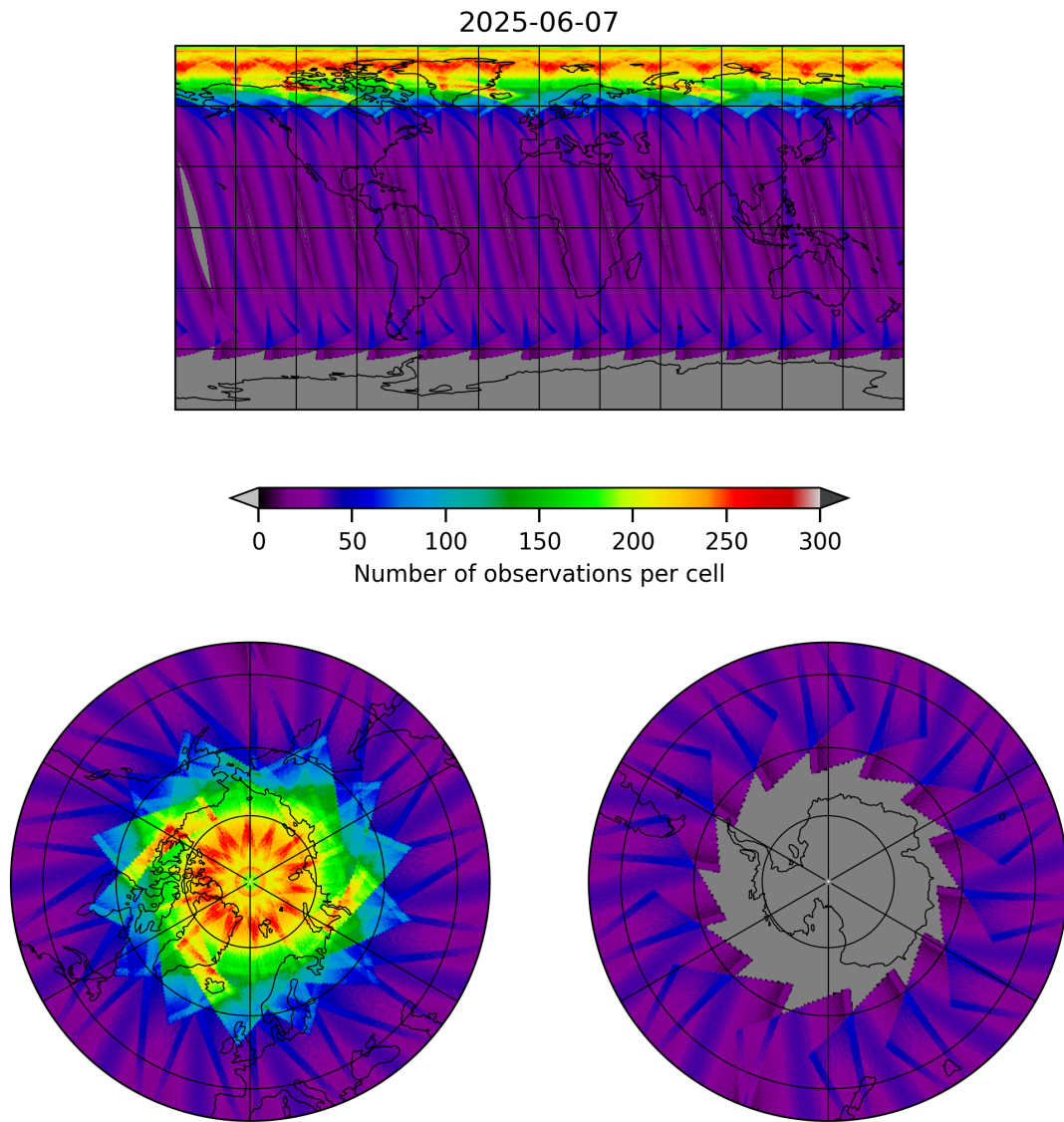
Figure 15: Map of the number of observations for 2025-06-07 to 2025-06-08
