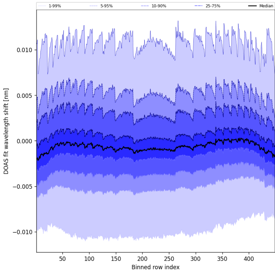
Figure 47: Along track statistics of "DOAS fit wavelength shift" for 2025-06-07 to 2025-06-08
