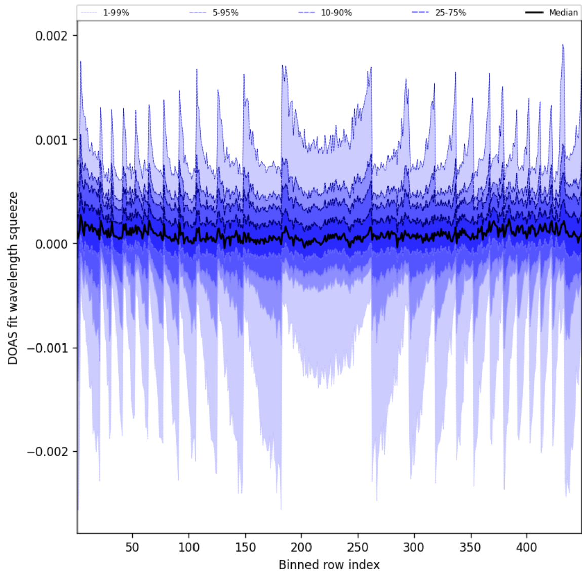
Figure 48: Along track statistics of “DOAS fit wavelength squeeze” for 2025-06-07 to 2025-06-08
