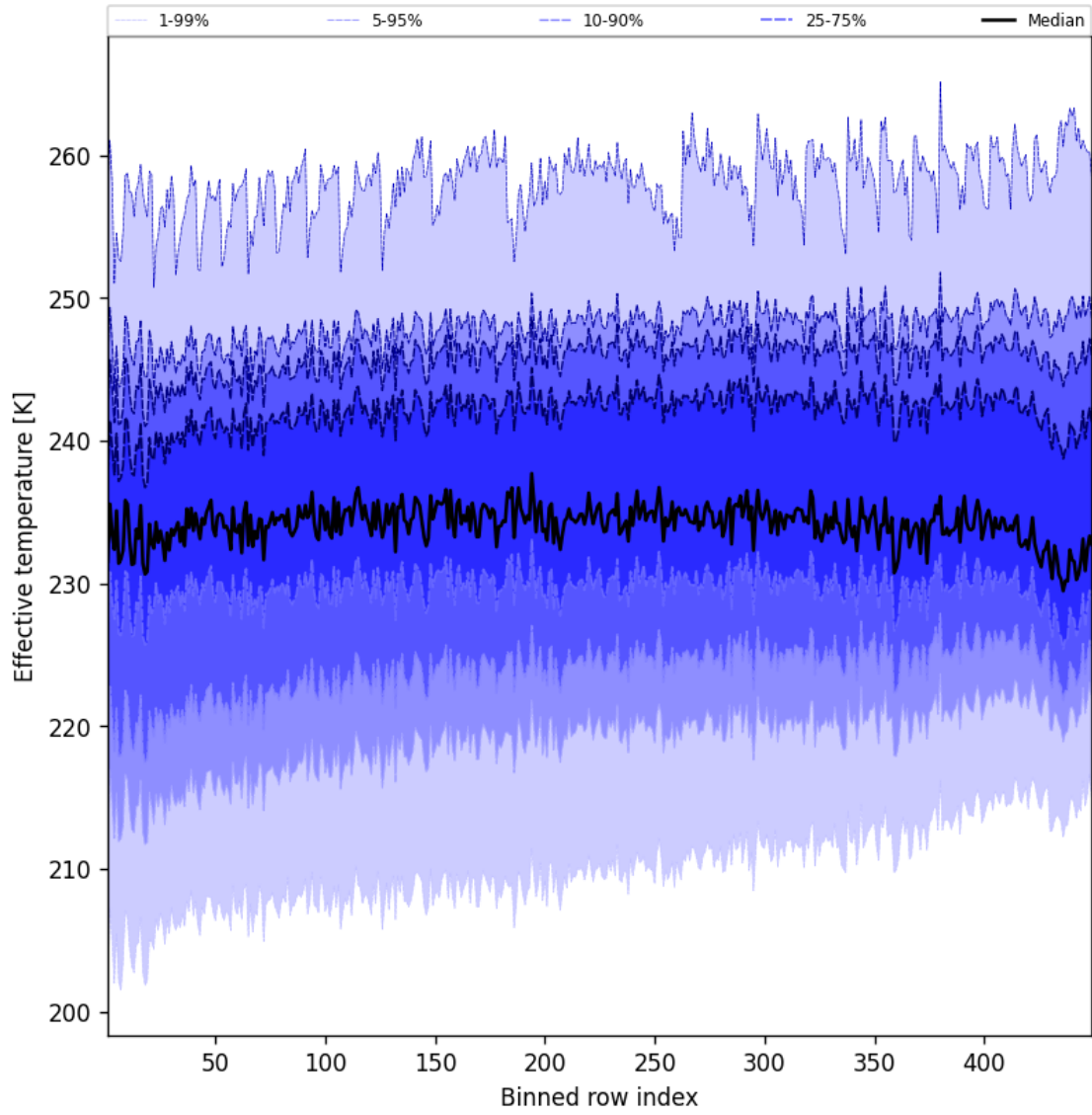
Figure 50: Along track statistics of “Effective temperature” for 2025-06-07 to 2025-06-08
