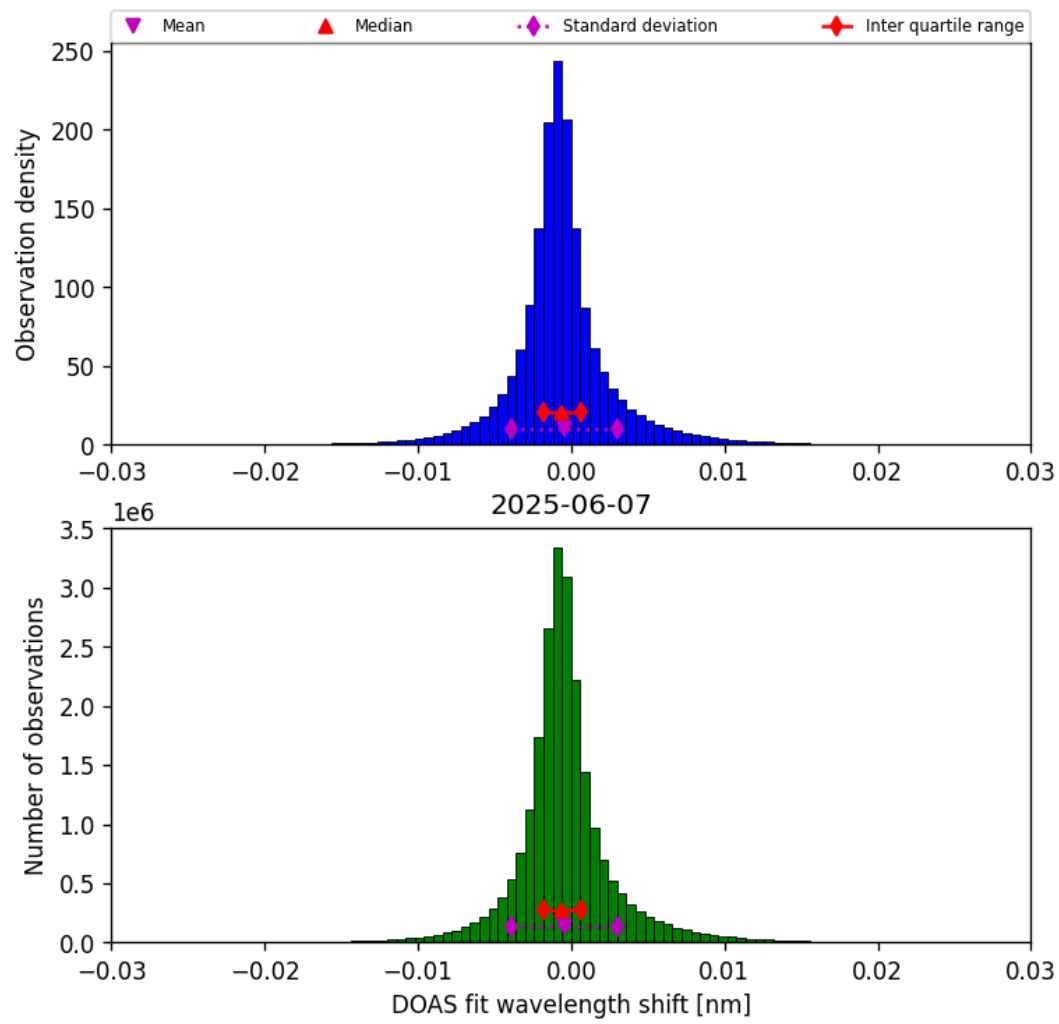
Figure 35: Histogram of “DOAS fit wavelength shift” for 2025-06-07 to 2025-06-08
