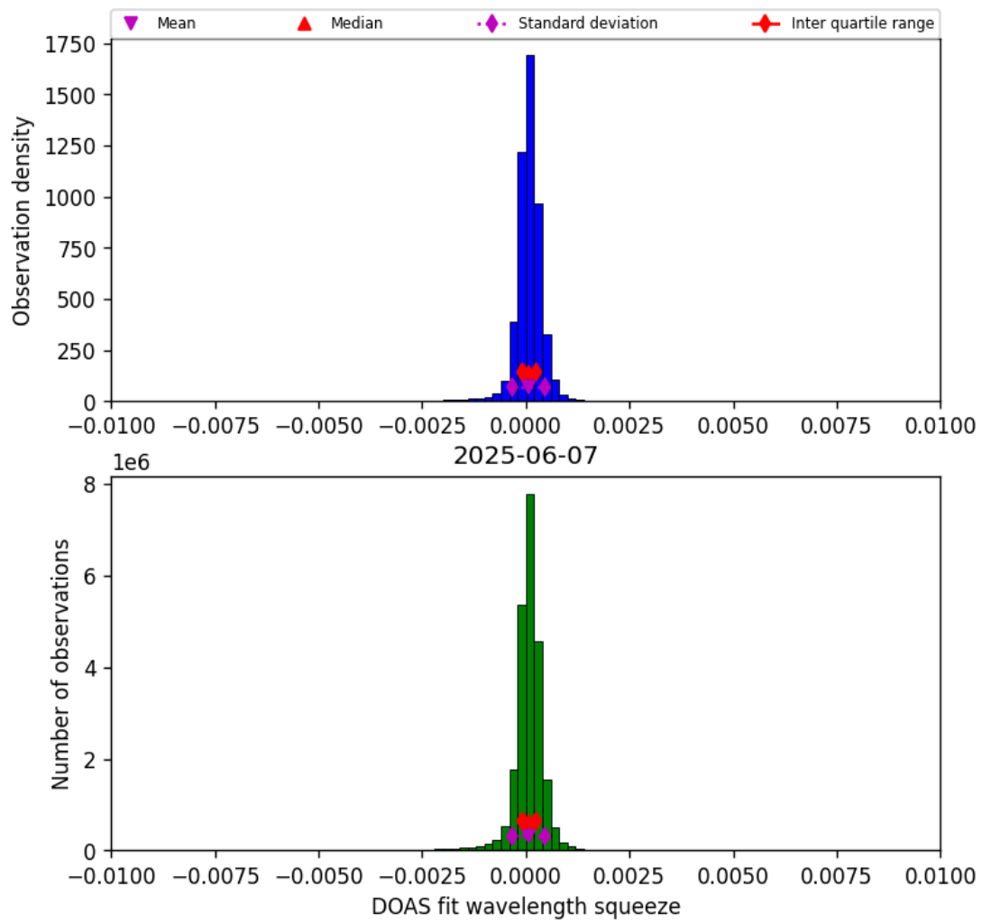
Figure 36: Histogram of “DOAS fit wavelength squeeze” for 2025-06-07 to 2025-06-08
