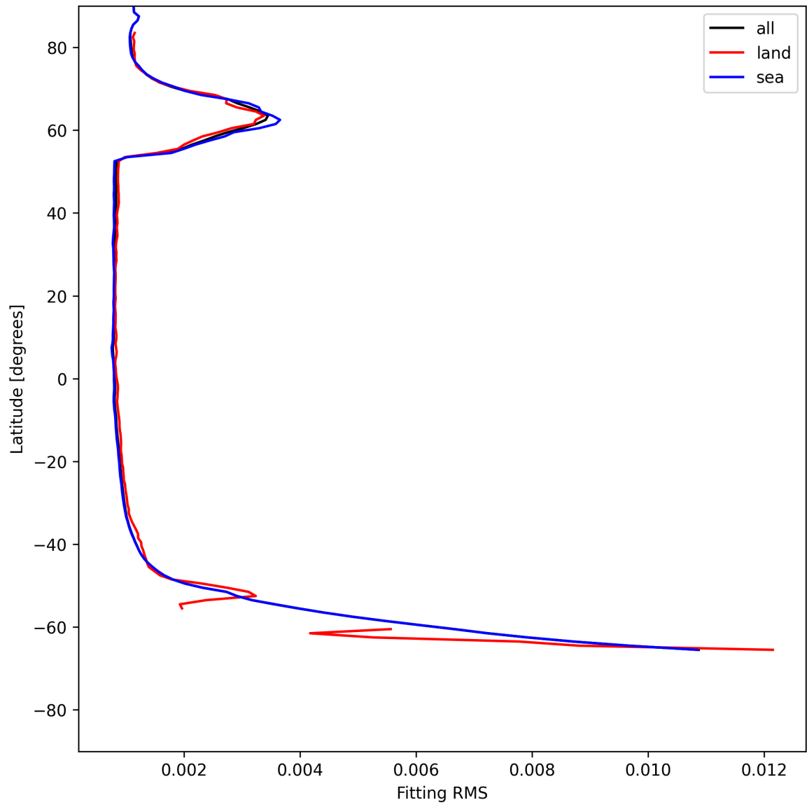
Figure 22: Zonal average of “Fitting RMS” for 2025-06-07 to 2025-06-08.
