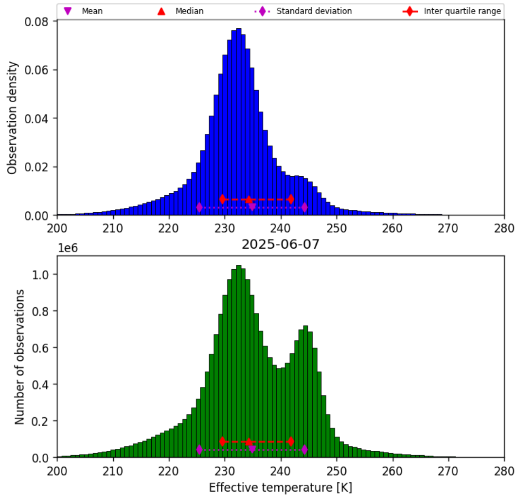
Figure 38: Histogram of “Effective temperature” for 2025-06-07 to 2025-06-08
