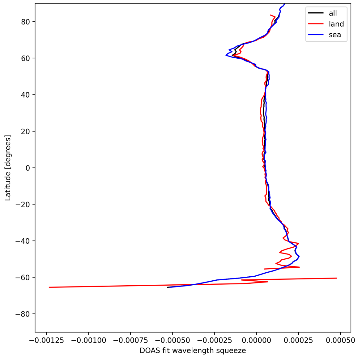
Figure 24: Zonal average of “DOAS fit wavelength squeeze” for 2025-06-07 to 2025-06-08.
