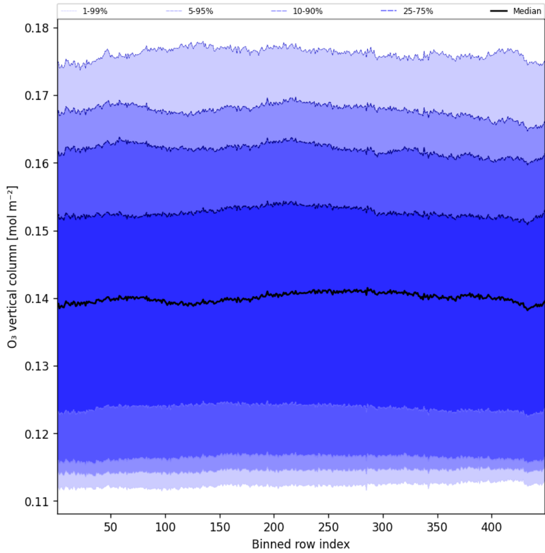
Figure 41: Along track statistics of “O 3 vertical column” for 2025-06-07 to 2025-06-08
