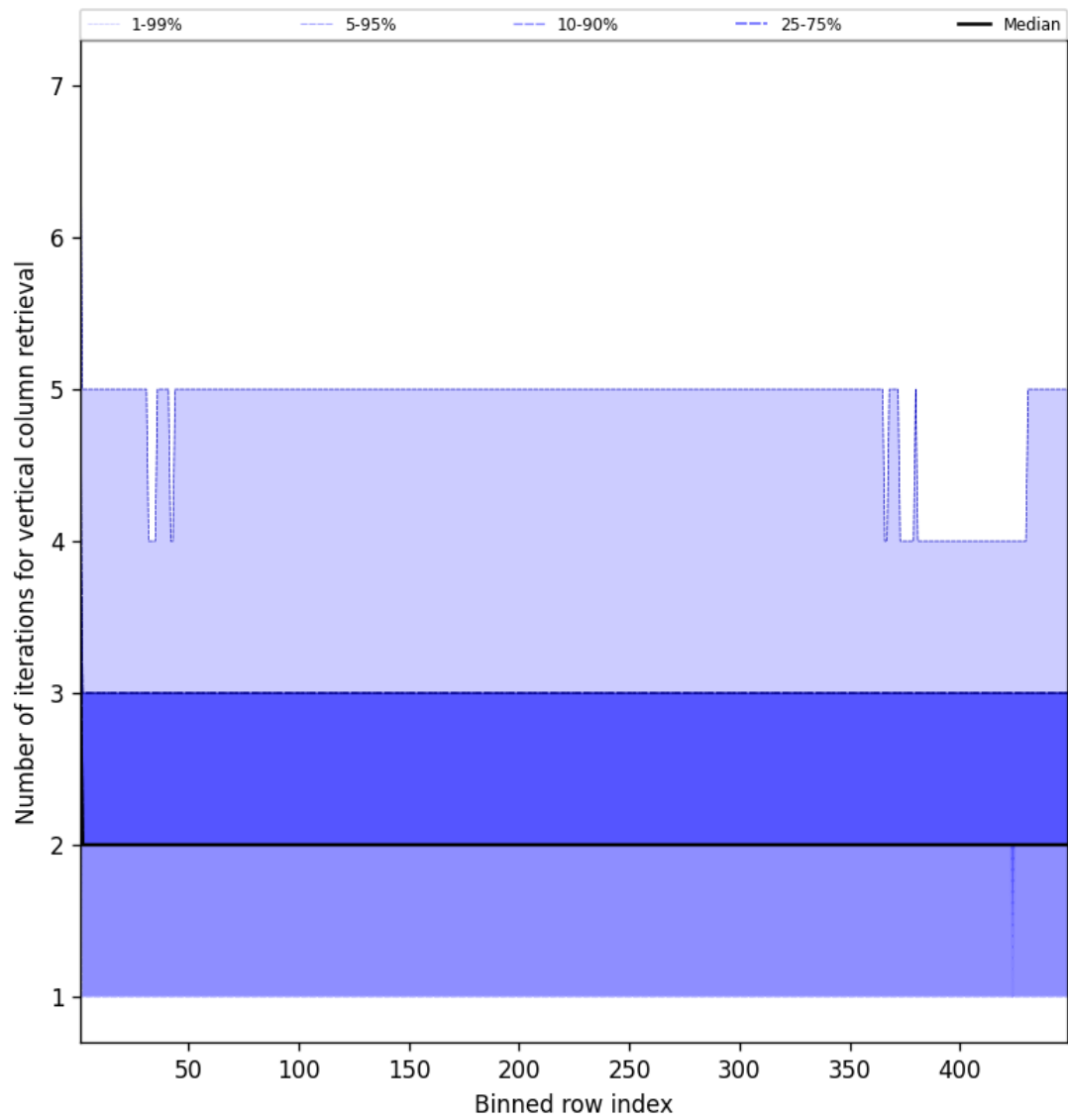
Figure 51: Along track statistics of “Number of iterations for vertical column retrieval” for 2025-06-07 to 2025-06-08
