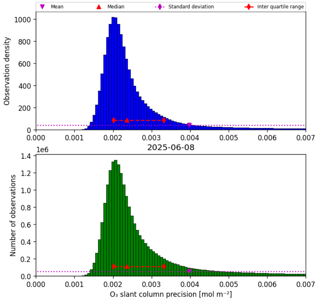
Figure 32: Histogram of “O 3 slant column precision” for 2025-06-08 to 2025-06-09
