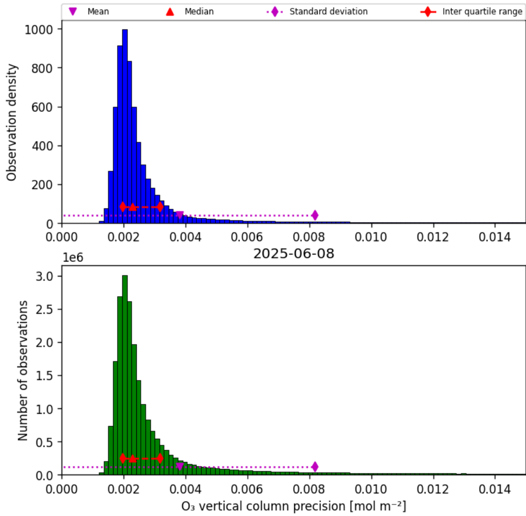
Figure 30: Histogram of “O 3 vertical column precision” for 2025-06-08 to 2025-06-09
