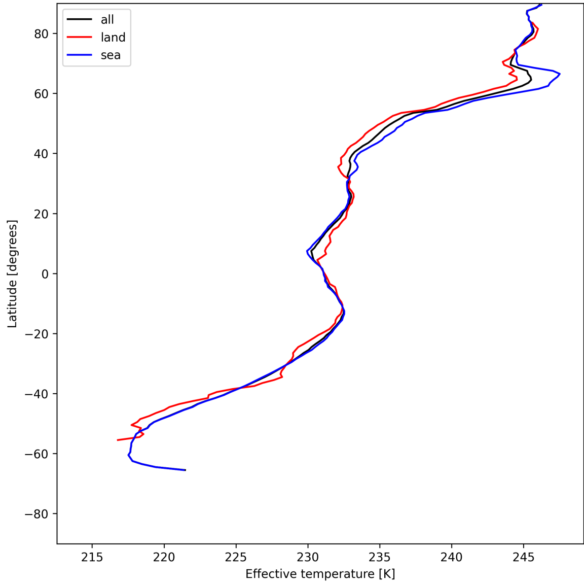
Figure 26: Zonal average of "Effective temperature" for 2025-06-08 to 2025-06-09.
