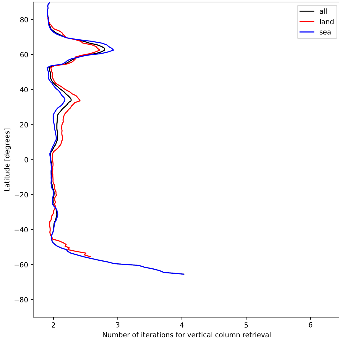
Figure 27: Zonal average of “Number of iterations for vertical column retrieval” for 2025-06-08 to 2025-06-09.
