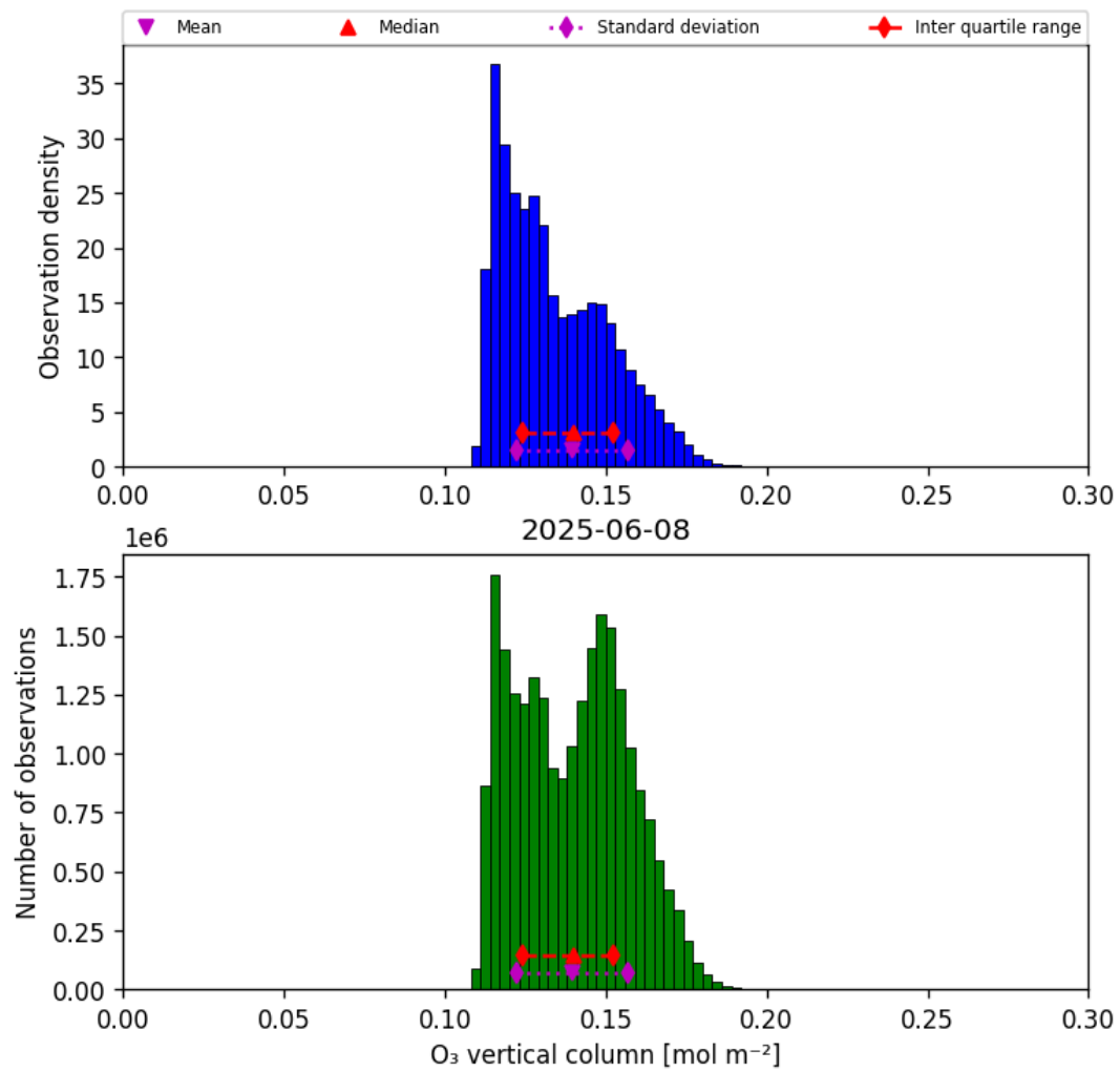
Figure 29: Histogram of “O 3 vertical column” for 2025-06-08 to 2025-06-09
