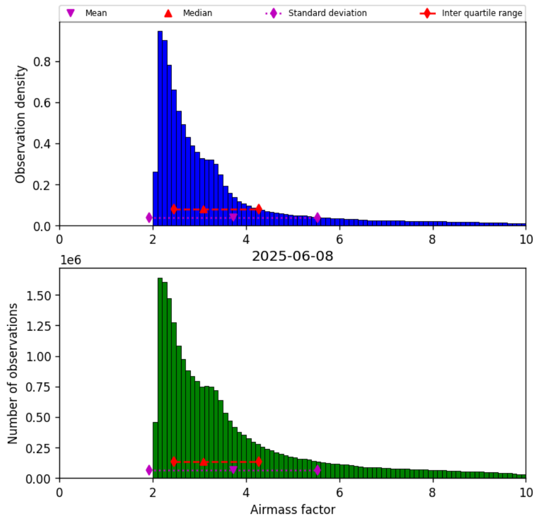
Figure 37: Histogram of “Airmass factor” for 2025-06-08 to 2025-06-09
