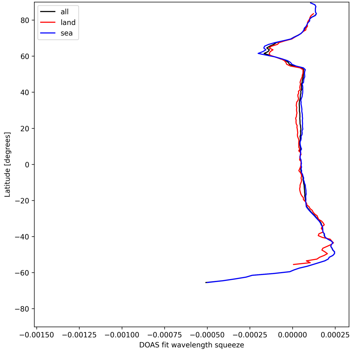
Figure 24: Zonal average of “DOAS fit wavelength squeeze” for 2025-06-08 to 2025-06-09.
