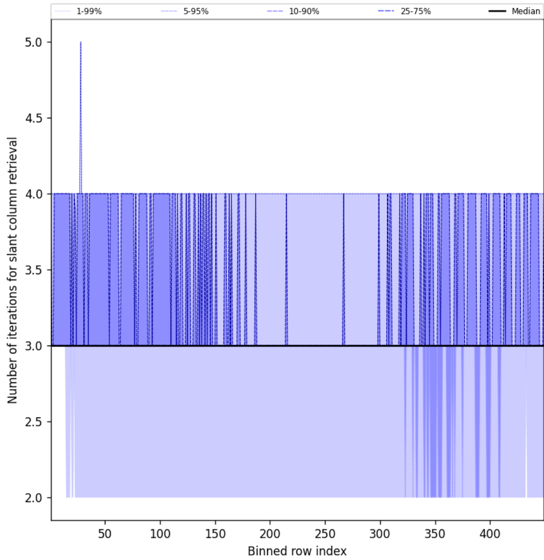
Figure 45: Along track statistics of “Number of iterations for slant column retrieval” for 2025-06-08 to 2025-06-09
