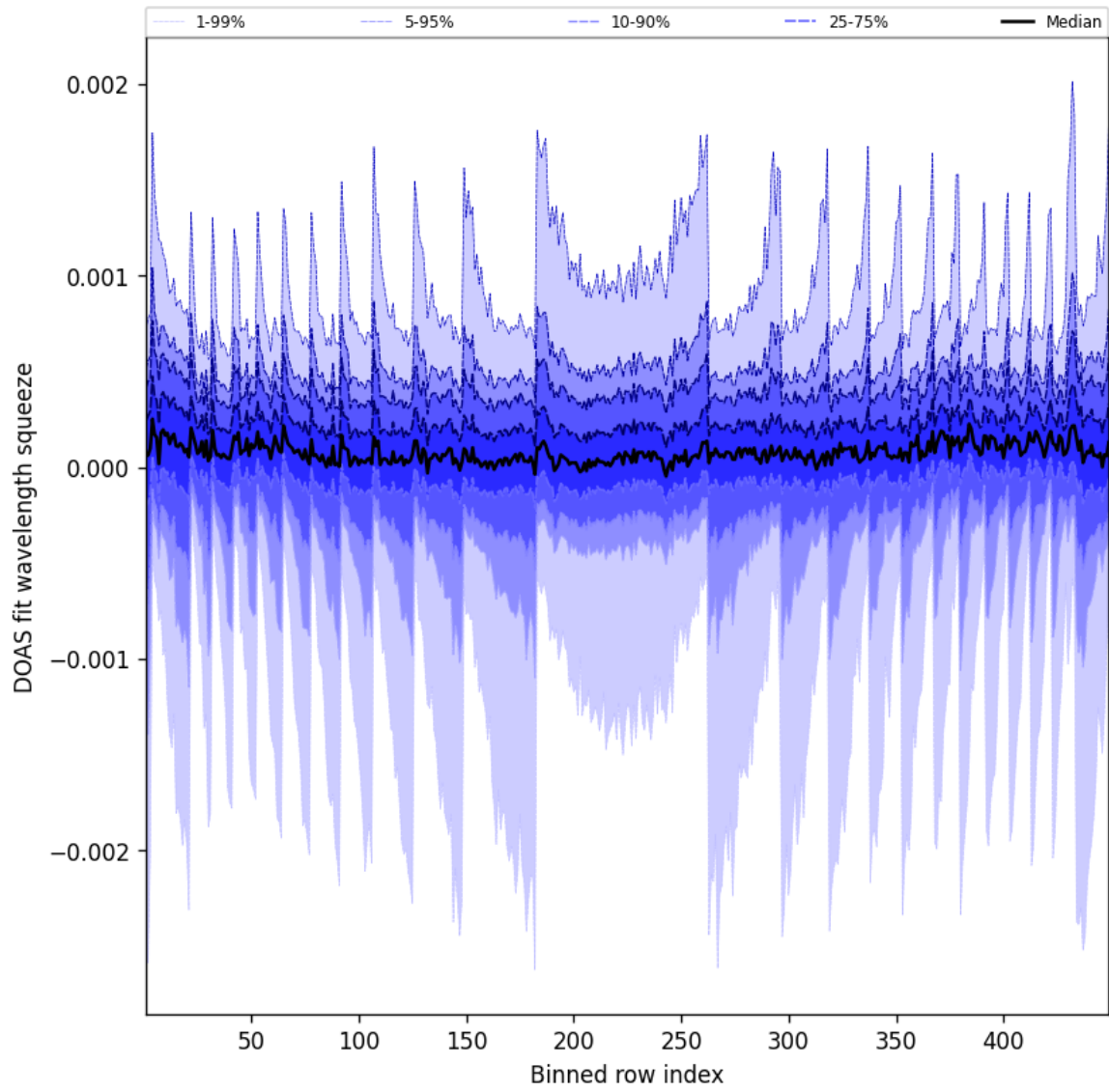
Figure 48: Along track statistics of “DOAS fit wavelength squeeze” for 2025-06-08 to 2025-06-09
