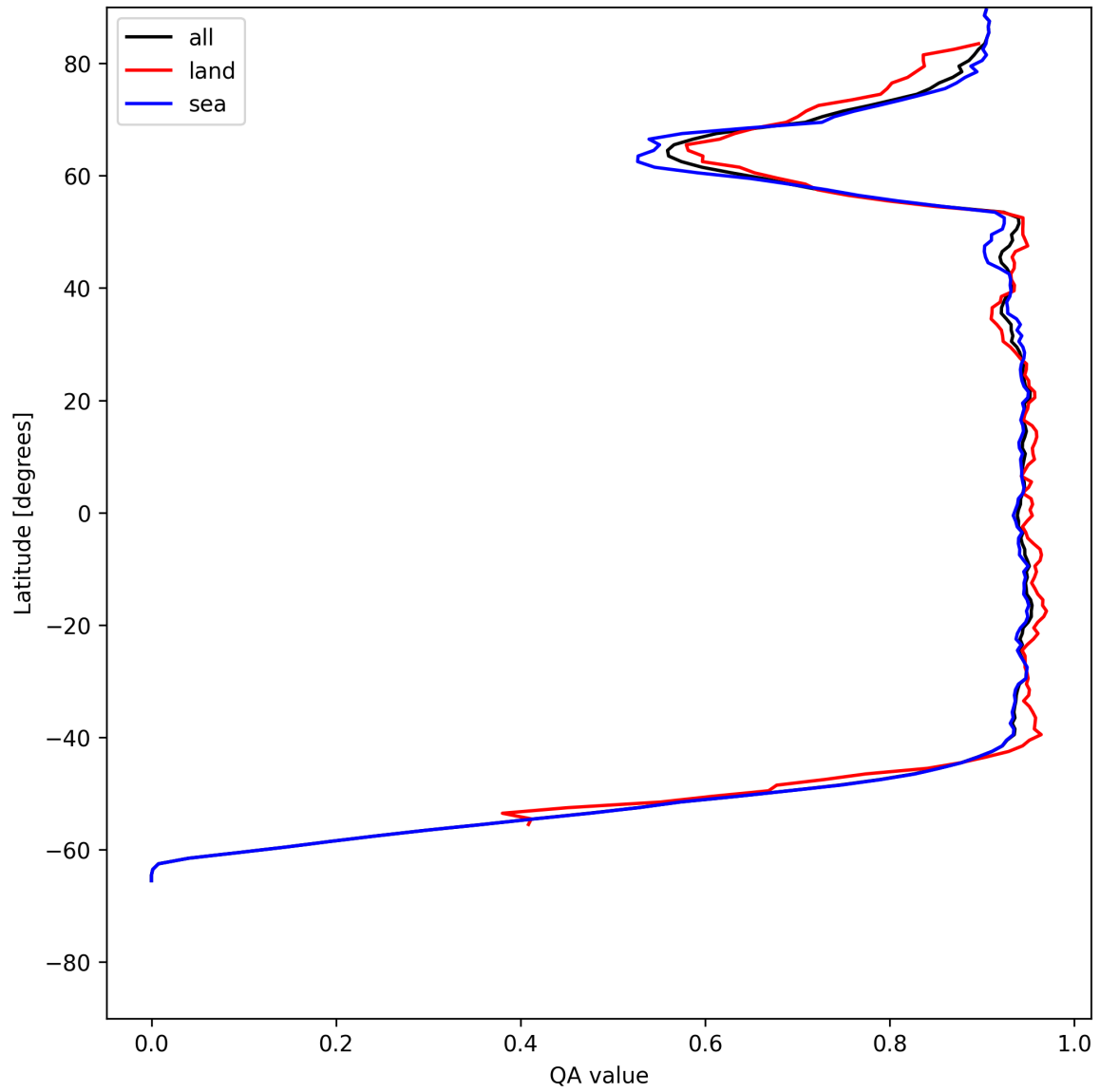
Figure 16: Zonal average of “QA value” for 2025-06-08 to 2025-06-09.
