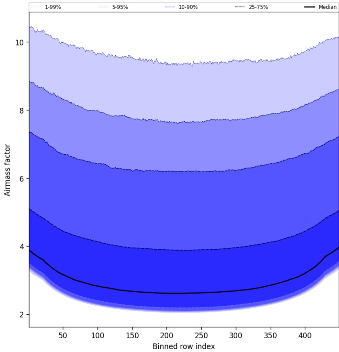
Figure 49: Along track statistics of “Airmass factor” for 2025-06-08 to 2025-06-09
