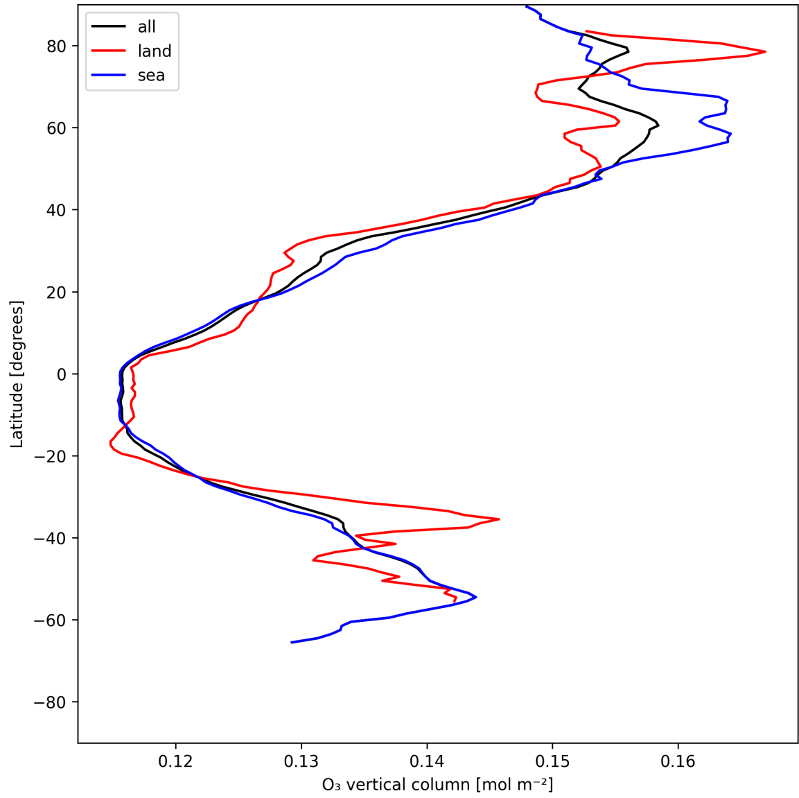
Figure 17: Zonal average of “O 3 vertical column” for 2025-06-08 to 2025-06-09.
