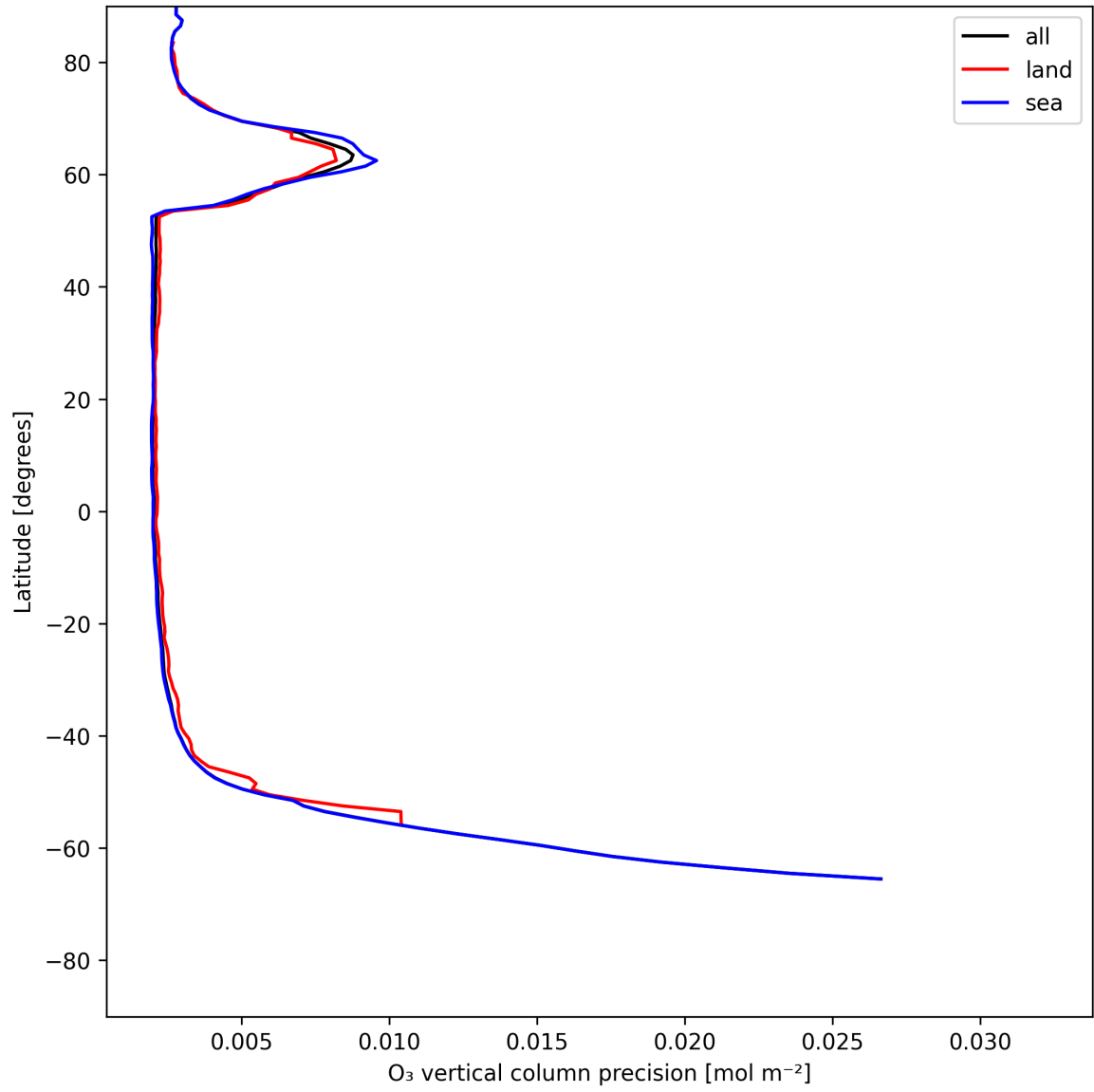
Figure 18: Zonal average of “O 3 vertical column precision” for 2025-06-08 to 2025-06-09.
