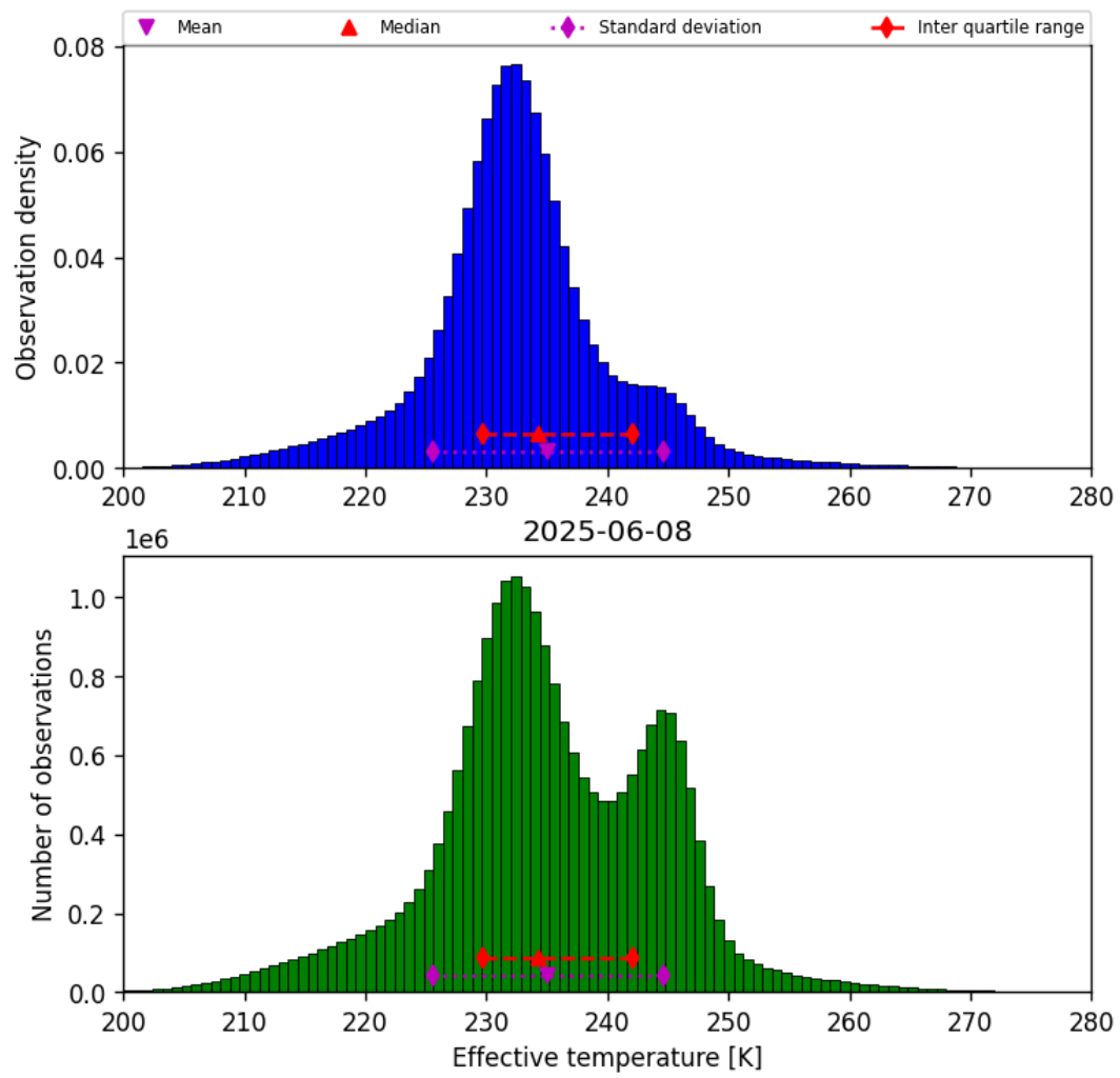
Figure 38: Histogram of “Effective temperature” for 2025-06-08 to 2025-06-09
