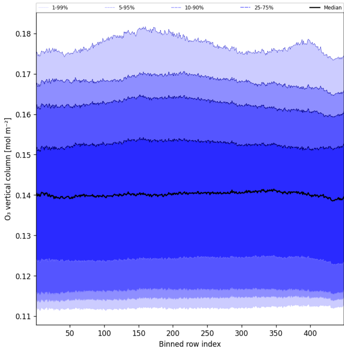
Figure 41: Along track statistics of “O 3 vertical column” for 2025-06-08 to 2025-06-09
