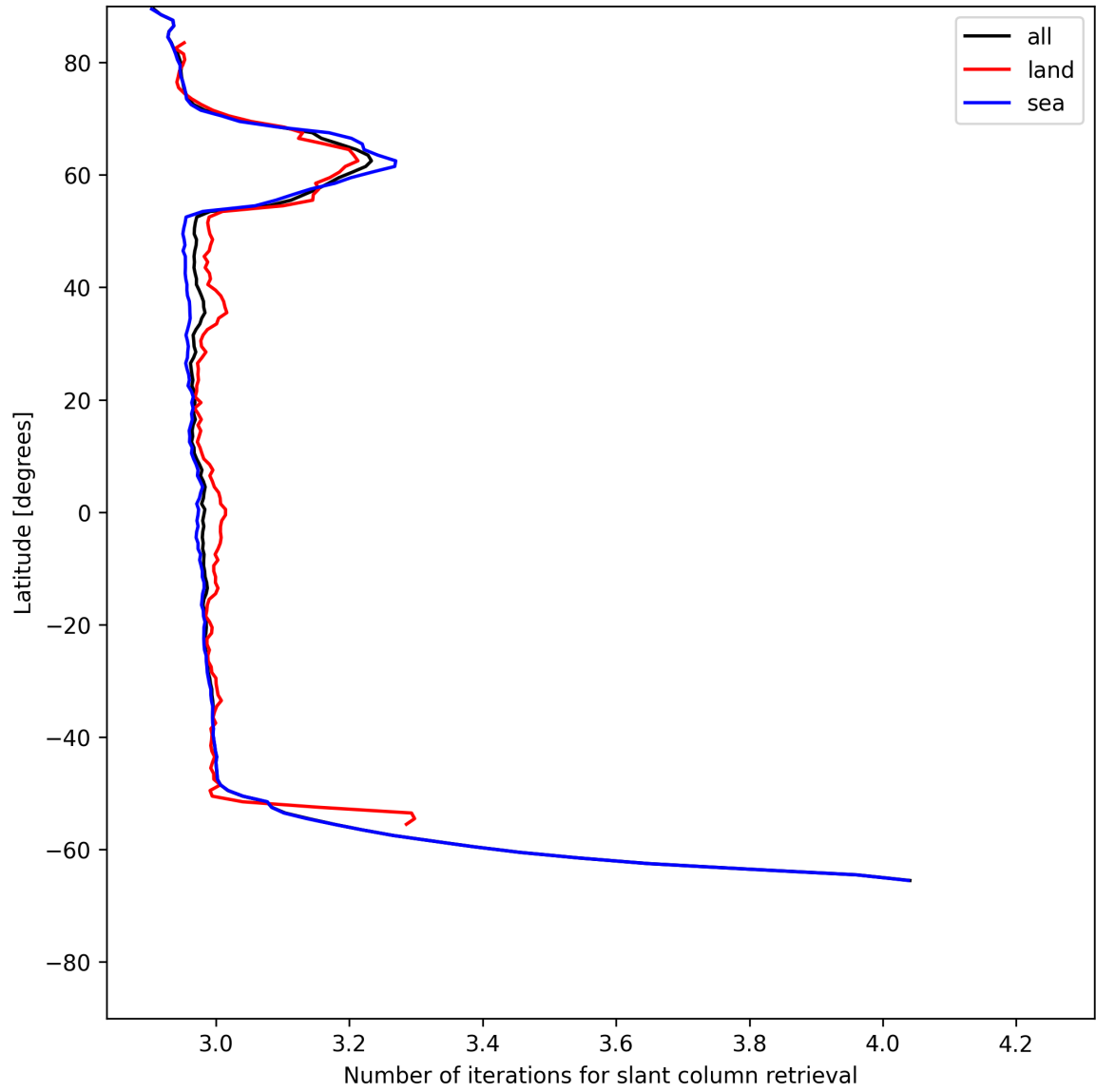
Figure 21: Zonal average of “Number of iterations for slant column retrieval” for 2025-06-08 to 2025-06-09.
