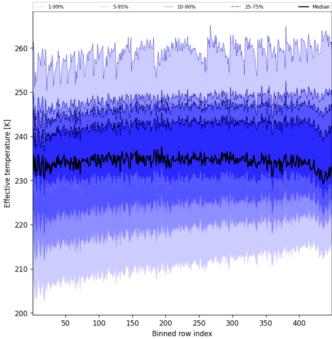
Figure 50: Along track statistics of “Effective temperature” for 2025-06-08 to 2025-06-09
