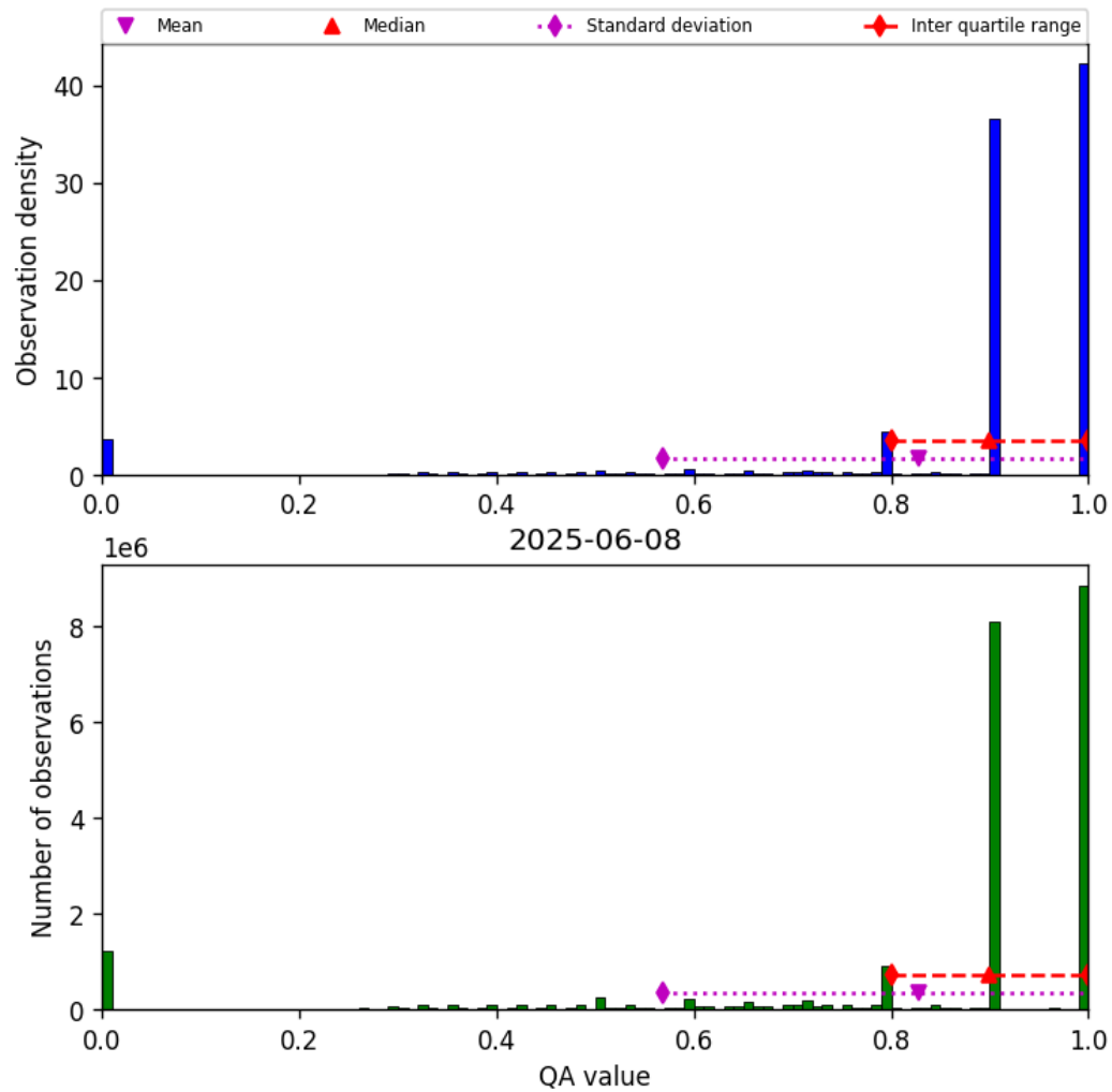
Figure 28: Histogram of “QA value” for 2025-06-08 to 2025-06-09
