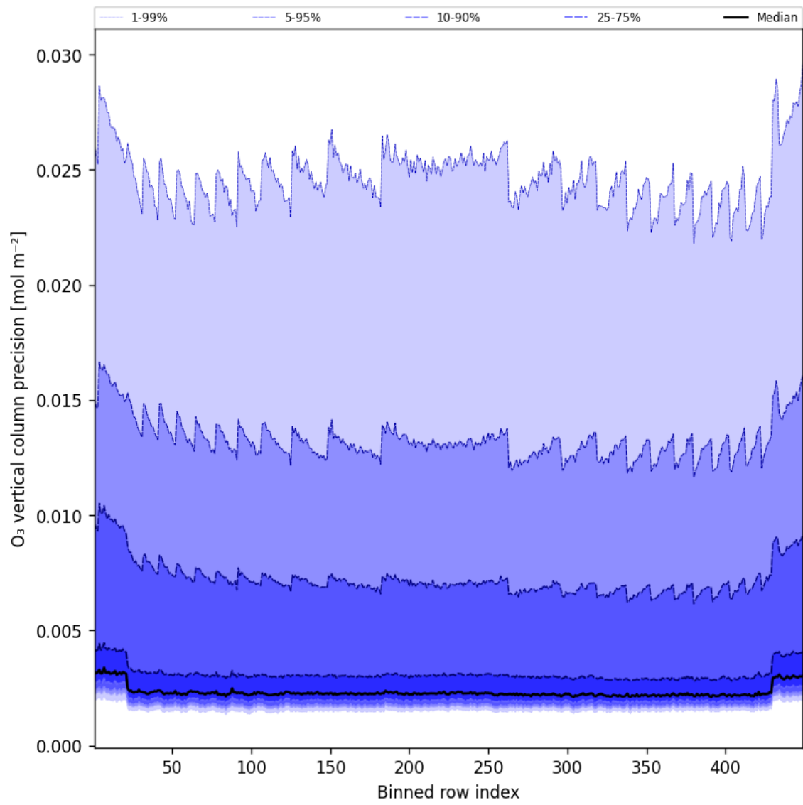
Figure 42: Along track statistics of “O 3 vertical column precision” for 2025-06-08 to 2025-06-09
