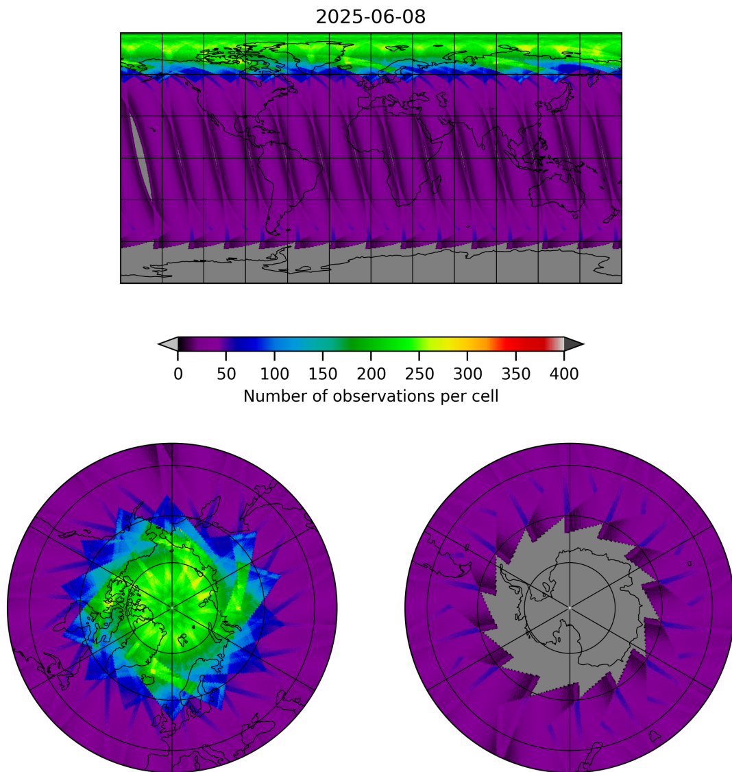
Figure 15: Map of the number of observations for 2025-06-08 to 2025-06-09
