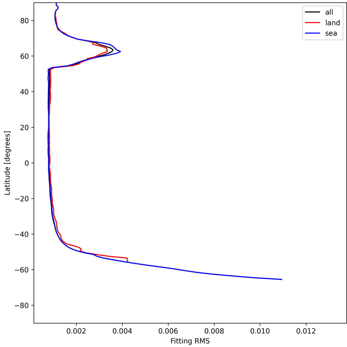
Figure 22: Zonal average of “Fitting RMS” for 2025-06-08 to 2025-06-09.
