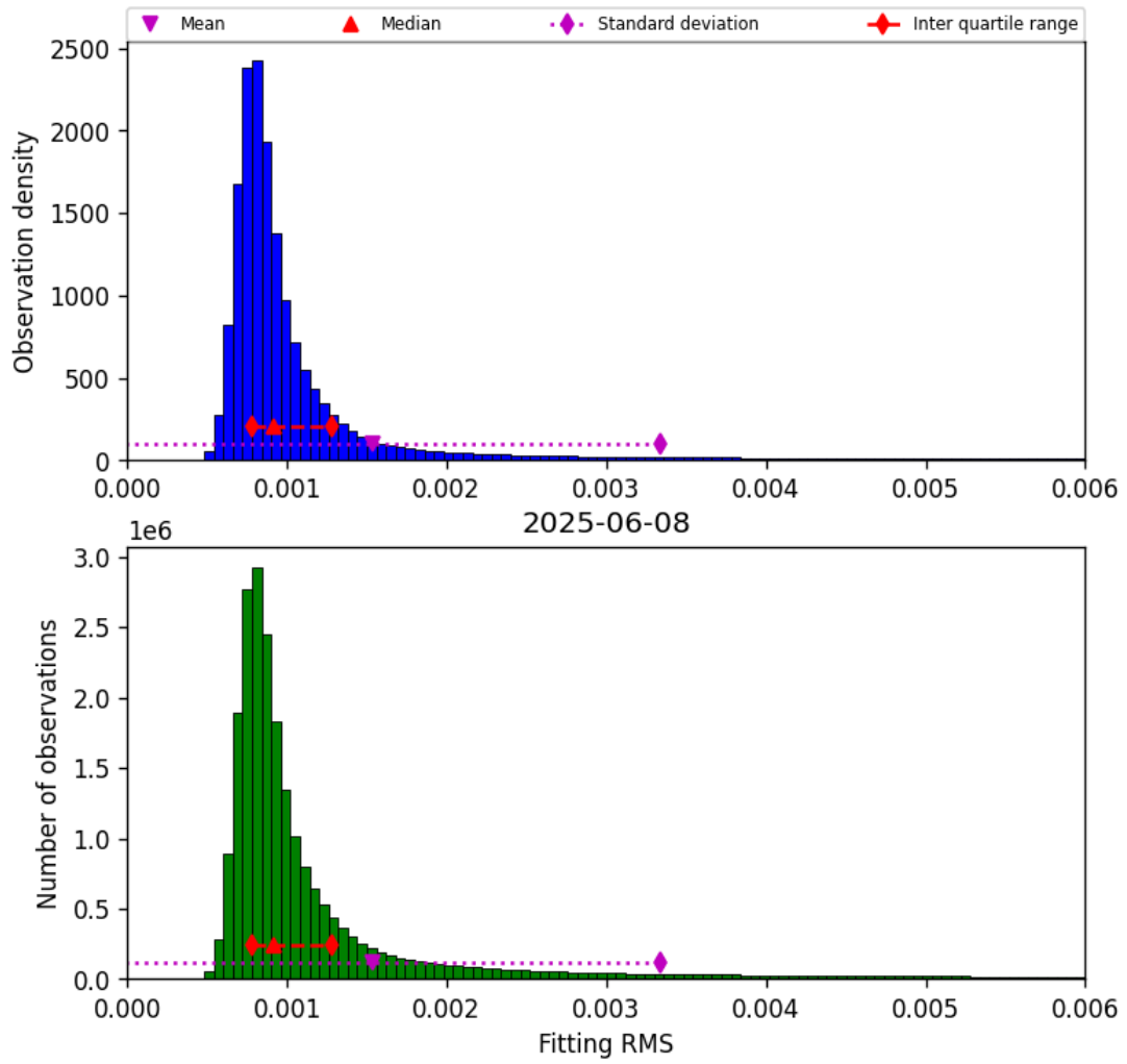
Figure 34: Histogram of “Fitting RMS” for 2025-06-08 to 2025-06-09
