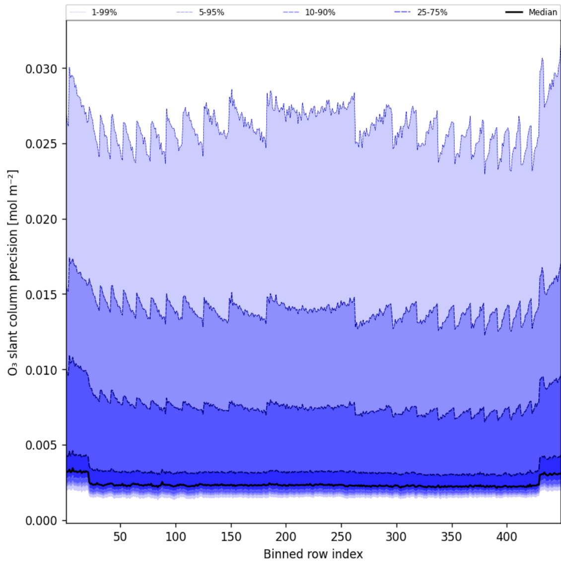
Figure 44: Along track statistics of “O 3 slant column precision” for 2025-06-08 to 2025-06-09
