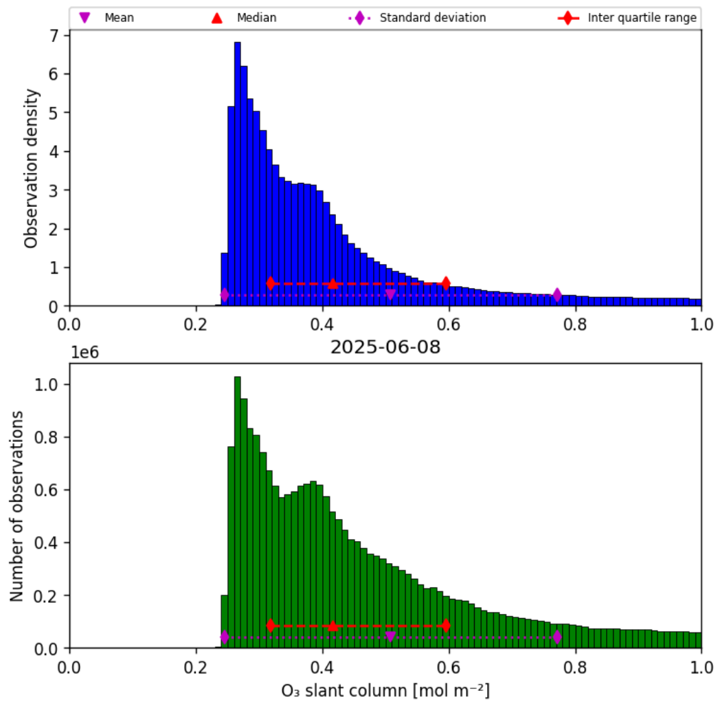
Figure 31: Histogram of “O 3 slant column” for 2025-06-08 to 2025-06-09
