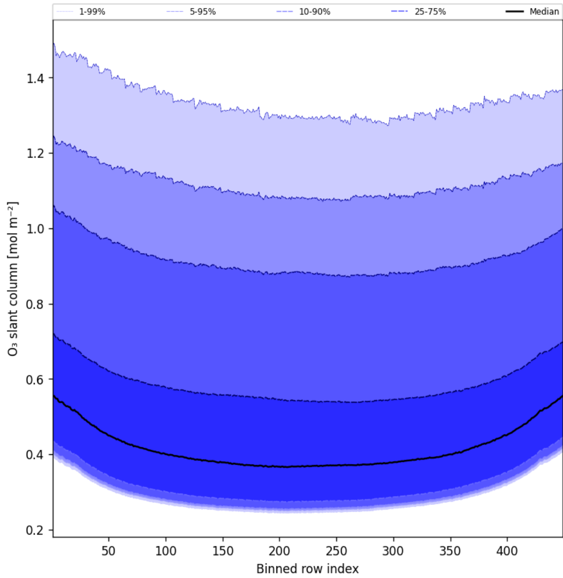
Figure 43: Along track statistics of “O 3 slant column” for 2025-06-08 to 2025-06-09
