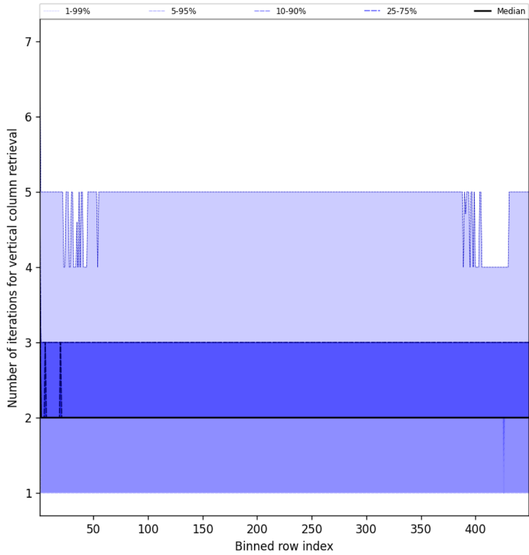
Figure 51: Along track statistics of “Number of iterations for vertical column retrieval” for 2025-06-08 to 2025-06-09
