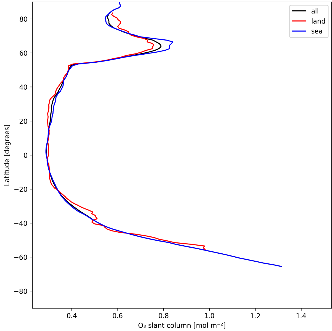
Figure 19: Zonal average of “O 3 slant column” for 2025-06-08 to 2025-06-09.
