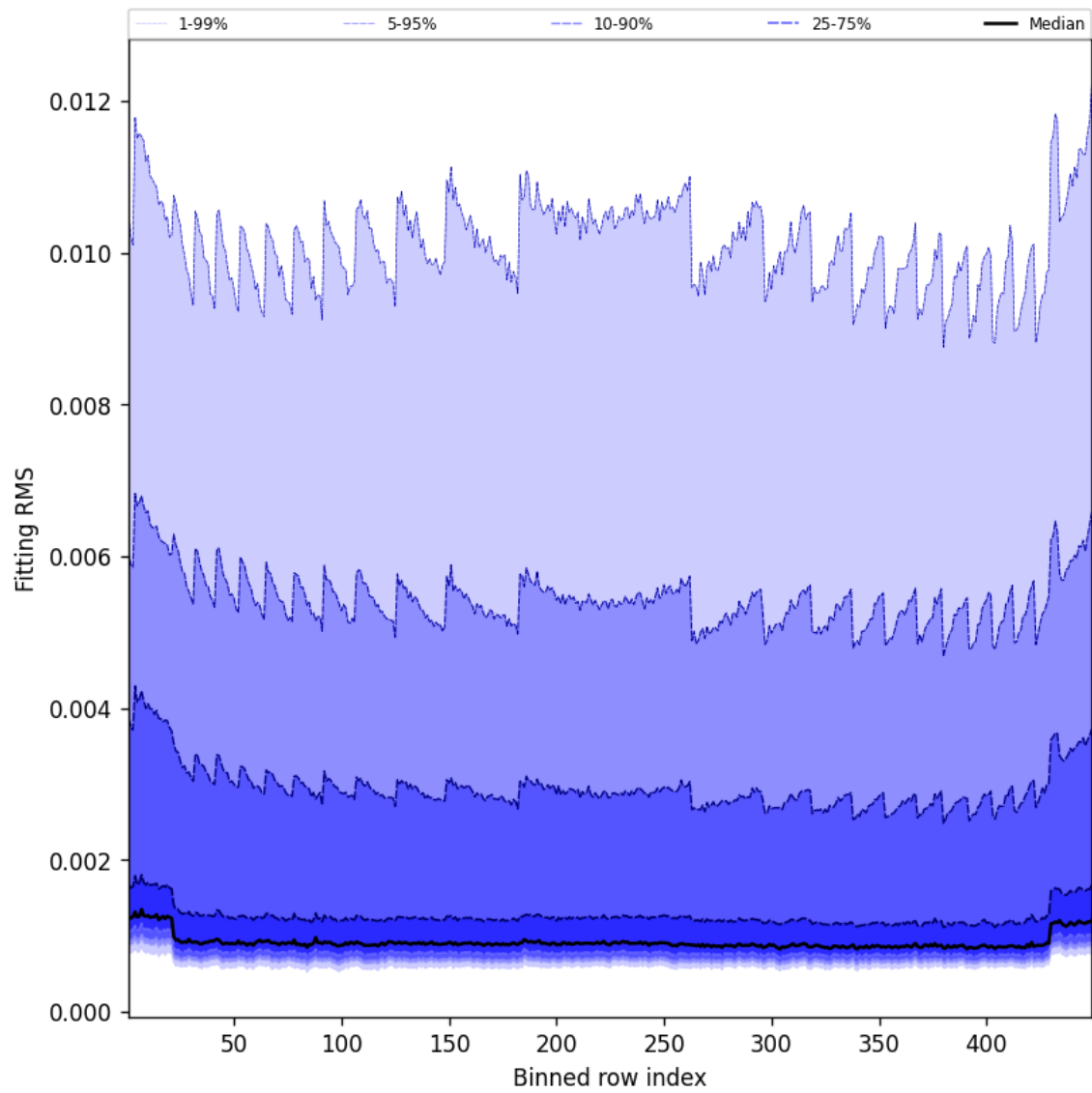
Figure 46: Along track statistics of “Fitting RMS” for 2025-06-08 to 2025-06-09
