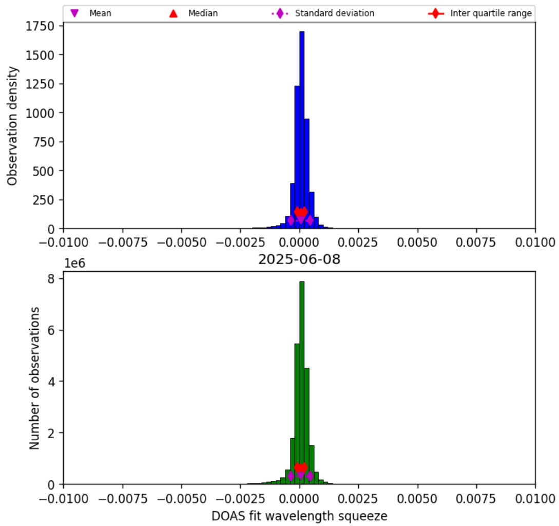
Figure 36: Histogram of “DOAS fit wavelength squeeze” for 2025-06-08 to 2025-06-09
