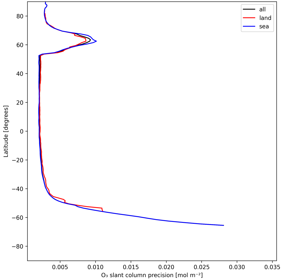
Figure 20: Zonal average of “O 3 slant column precision” for 2025-06-08 to 2025-06-09.
