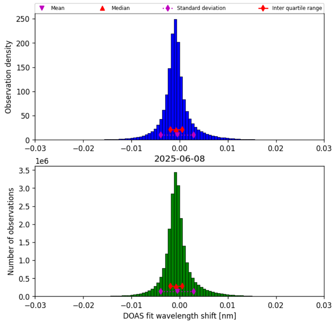
Figure 35: Histogram of “DOAS fit wavelength shift” for 2025-06-08 to 2025-06-09
