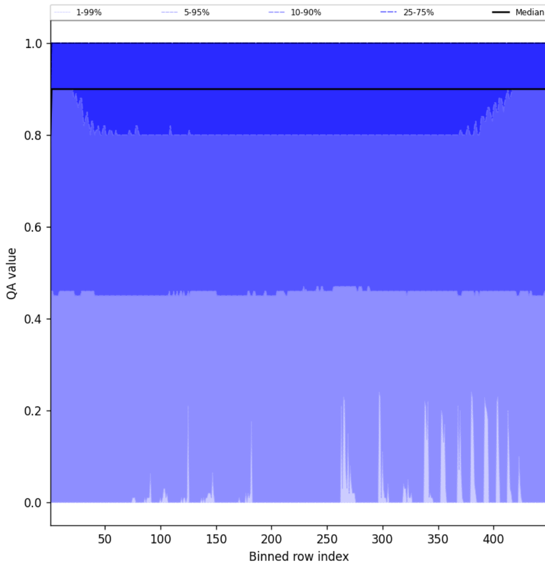
Figure 40: Along track statistics of “QA value” for 2025-06-08 to 2025-06-09
