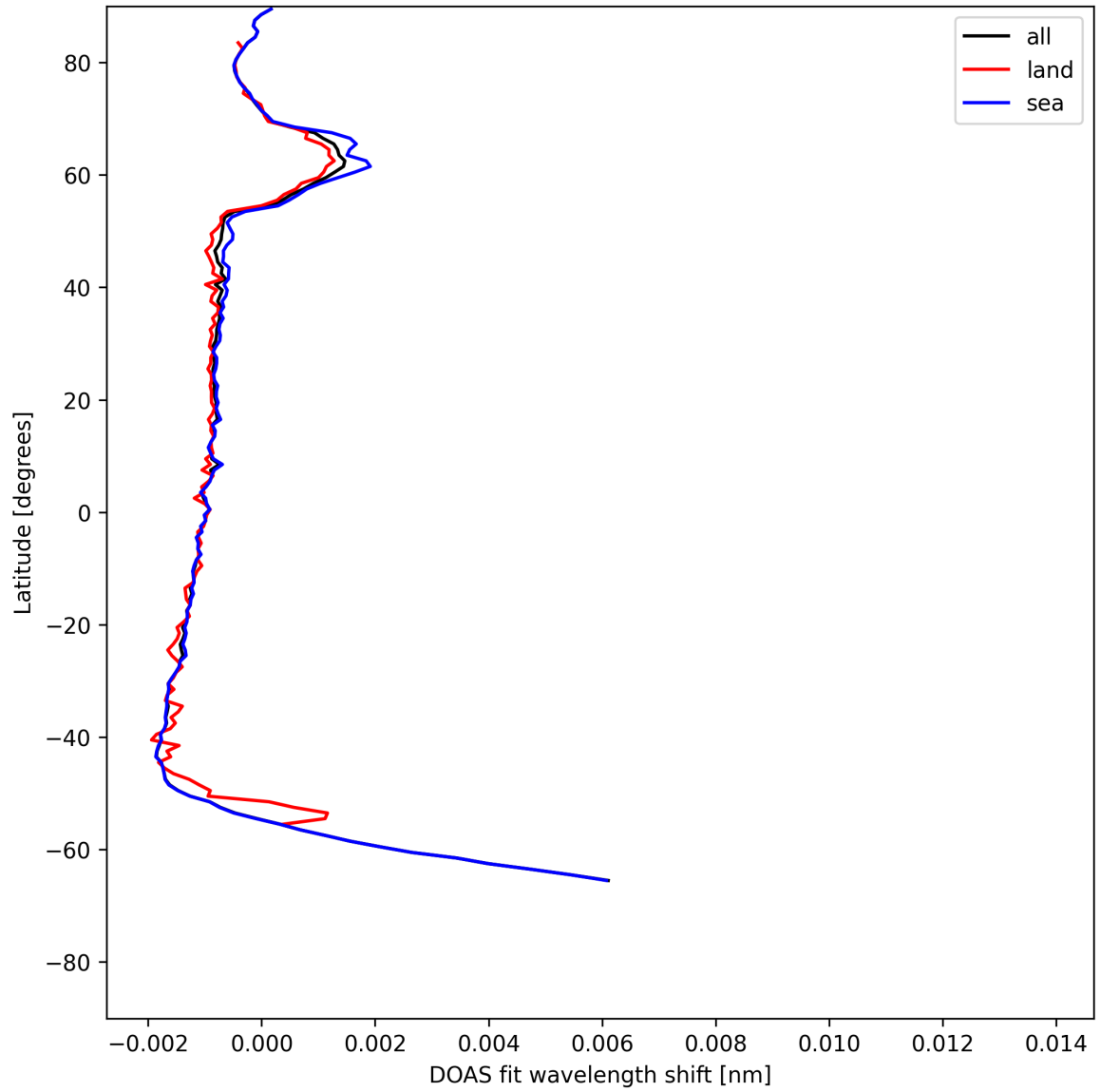
Figure 23: Zonal average of “DOAS fit wavelength shift” for 2025-06-08 to 2025-06-09.
