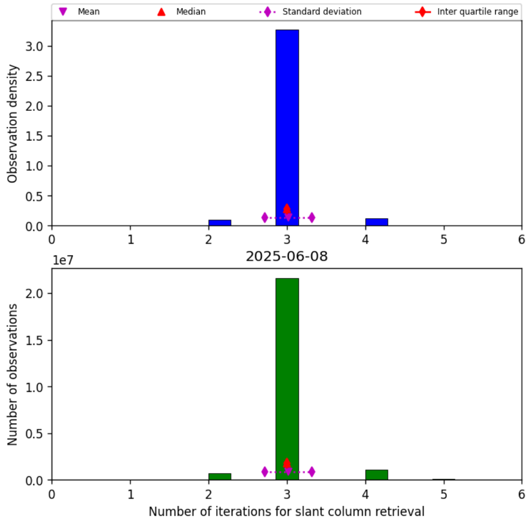
Figure 33: Histogram of “Number of iterations for slant column retrieval” for 2025-06-08 to 2025-06-09
