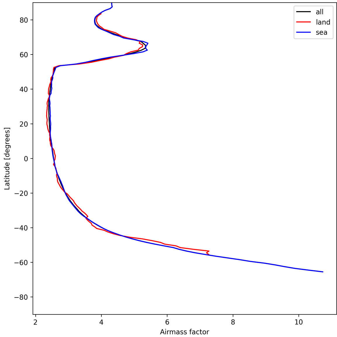
Figure 25: Zonal average of “Airmass factor” for 2025-06-08 to 2025-06-09.
