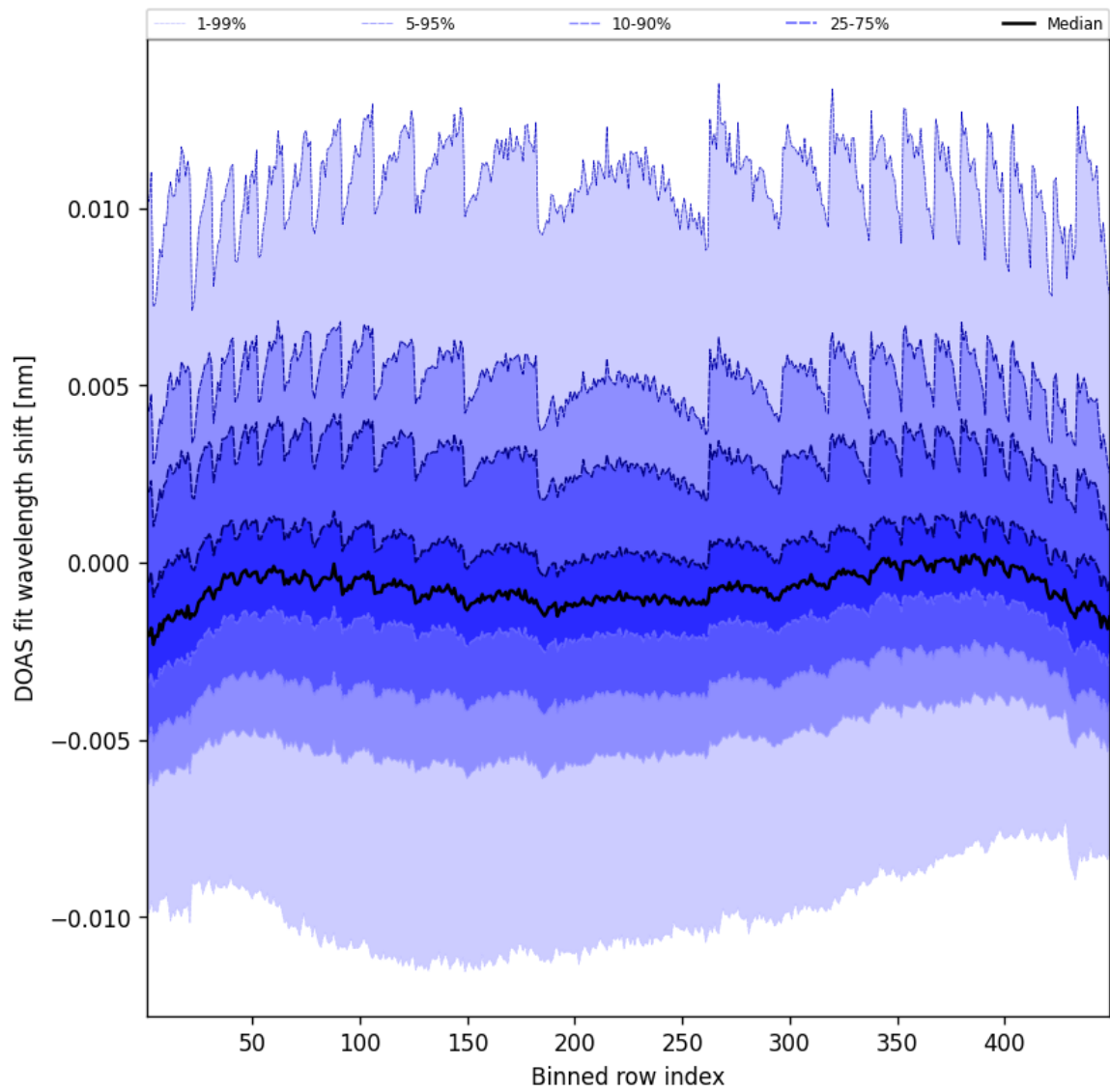
Figure 47: Along track statistics of “DOAS fit wavelength shift” for 2025-06-08 to 2025-06-09
