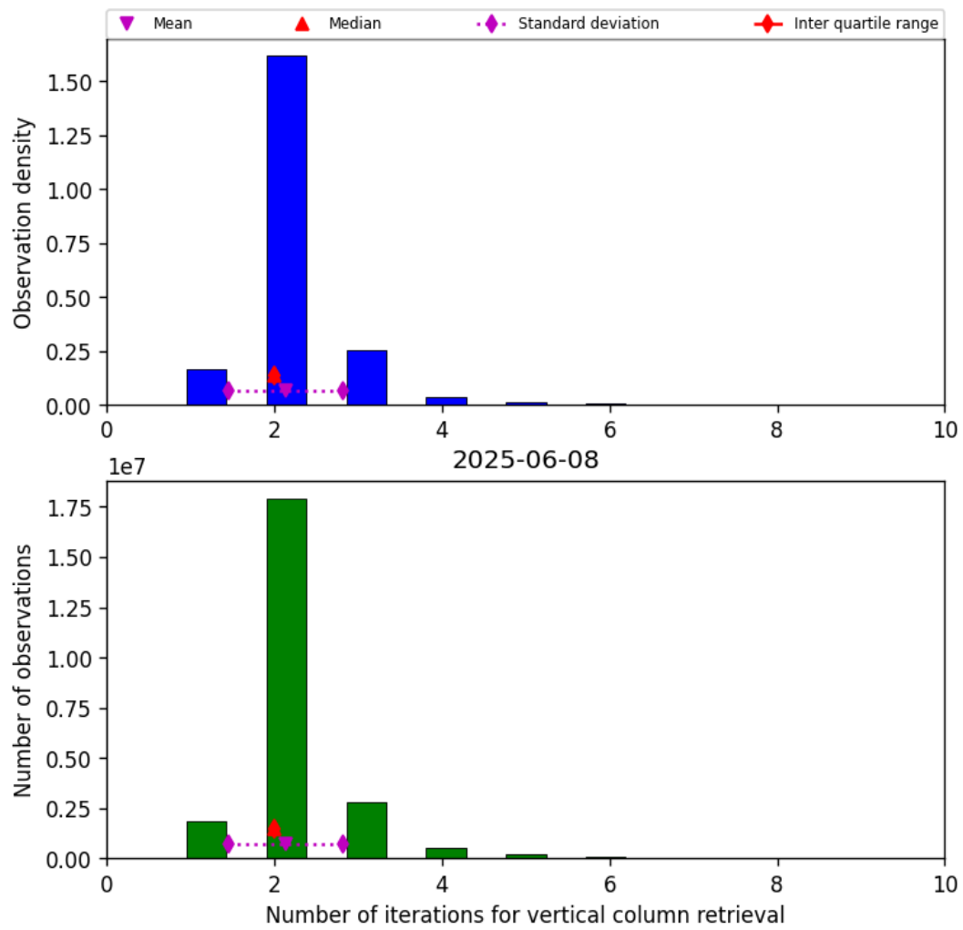
Figure 39: Histogram of “Number of iterations for vertical column retrieval” for 2025-06-08 to 2025-06-09
