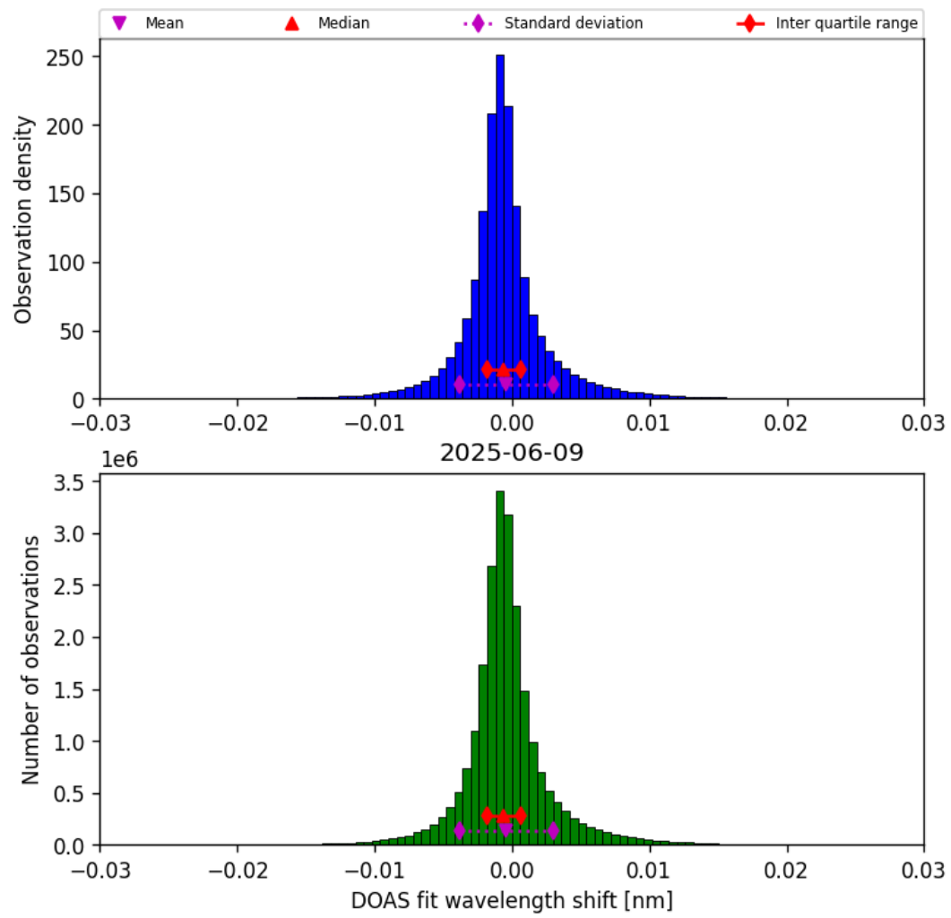
Figure 35: Histogram of “DOAS fit wavelength shift” for 2025-06-09 to 2025-06-09
