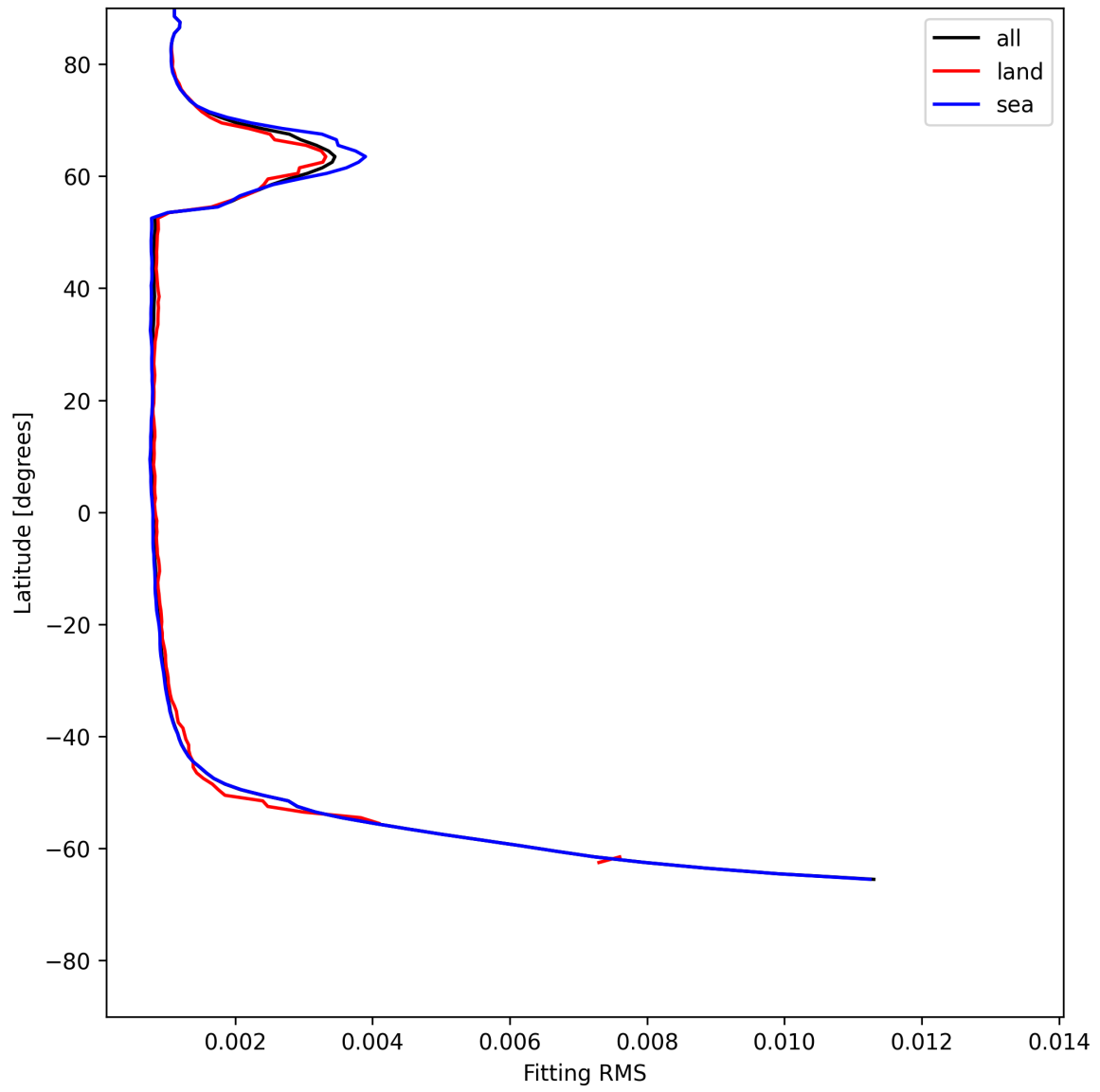
Figure 22: Zonal average of “Fitting RMS” for 2025-06-09 to 2025-06-09.
