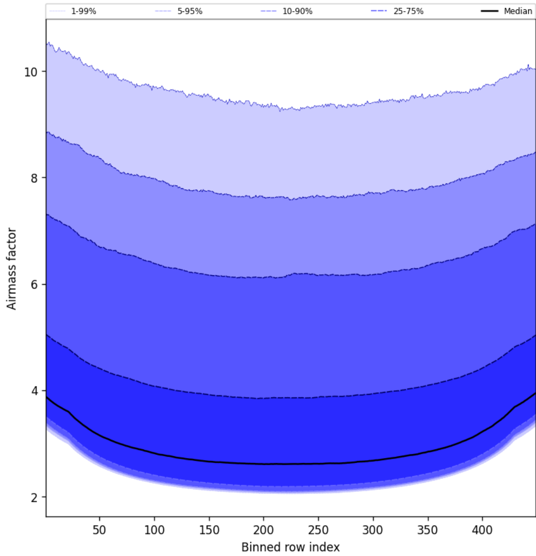
Figure 49: Along track statistics of “Airmass factor” for 2025-06-09 to 2025-06-09
