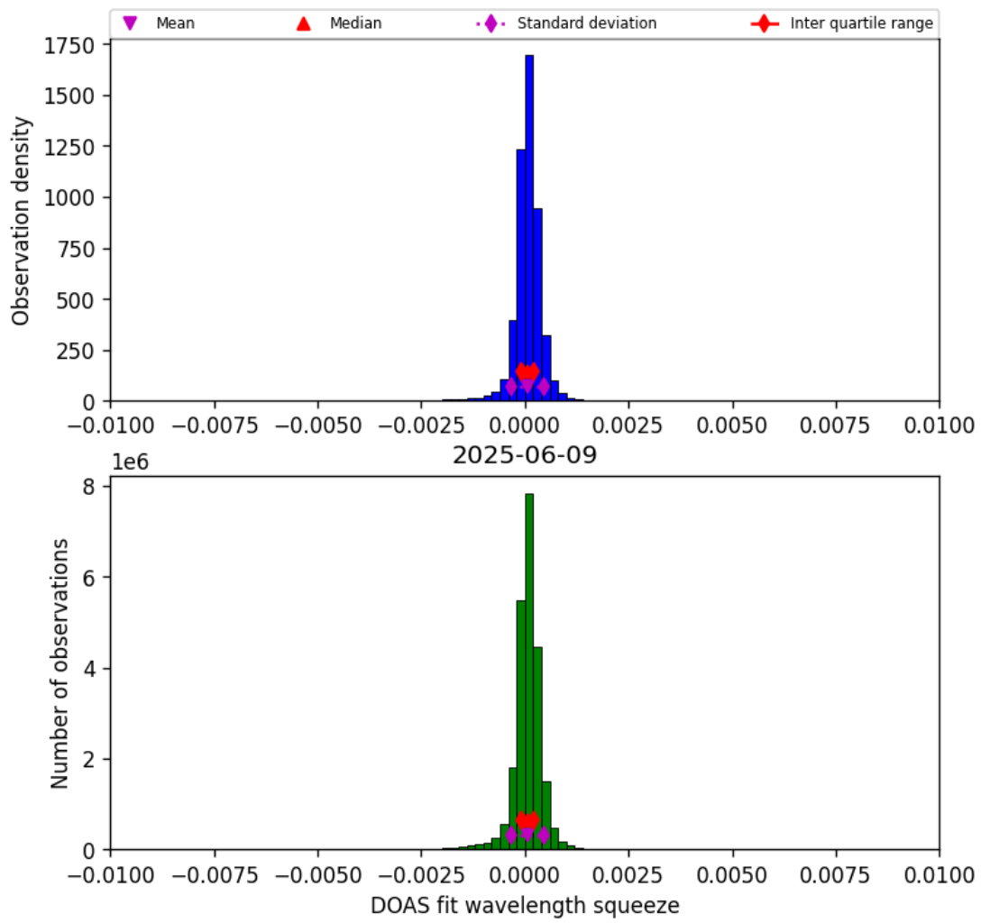
Figure 36: Histogram of “DOAS fit wavelength squeeze” for 2025-06-09 to 2025-06-09
