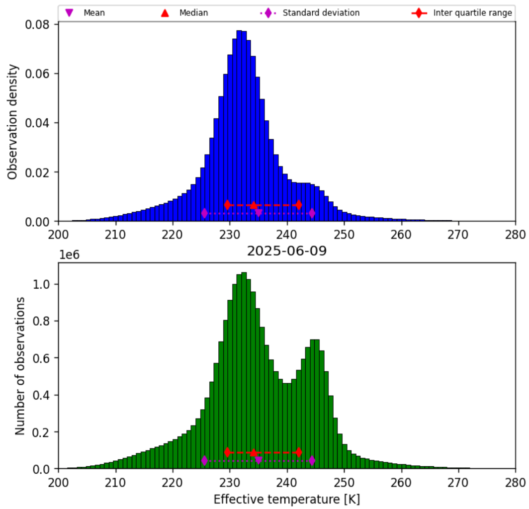
Figure 38: Histogram of “Effective temperature” for 2025-06-09 to 2025-06-09
