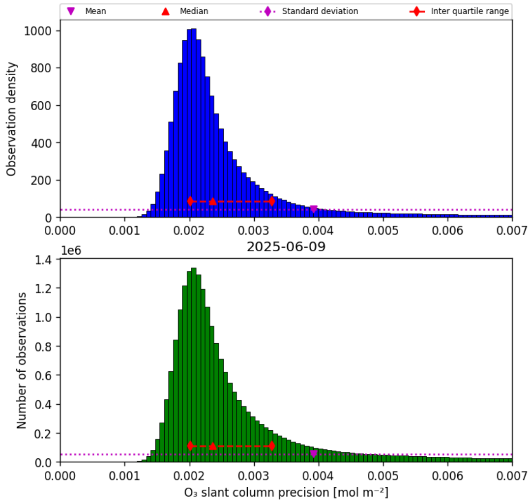
Figure 32: Histogram of “O 3 slant column precision” for 2025-06-09 to 2025-06-09
