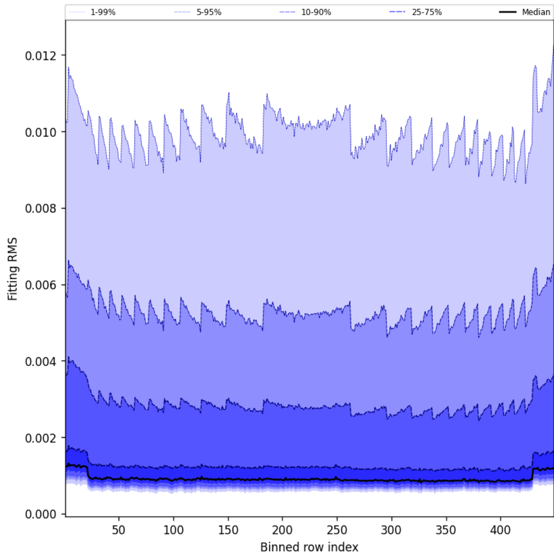
Figure 46: Along track statistics of “Fitting RMS” for 2025-06-09 to 2025-06-09
