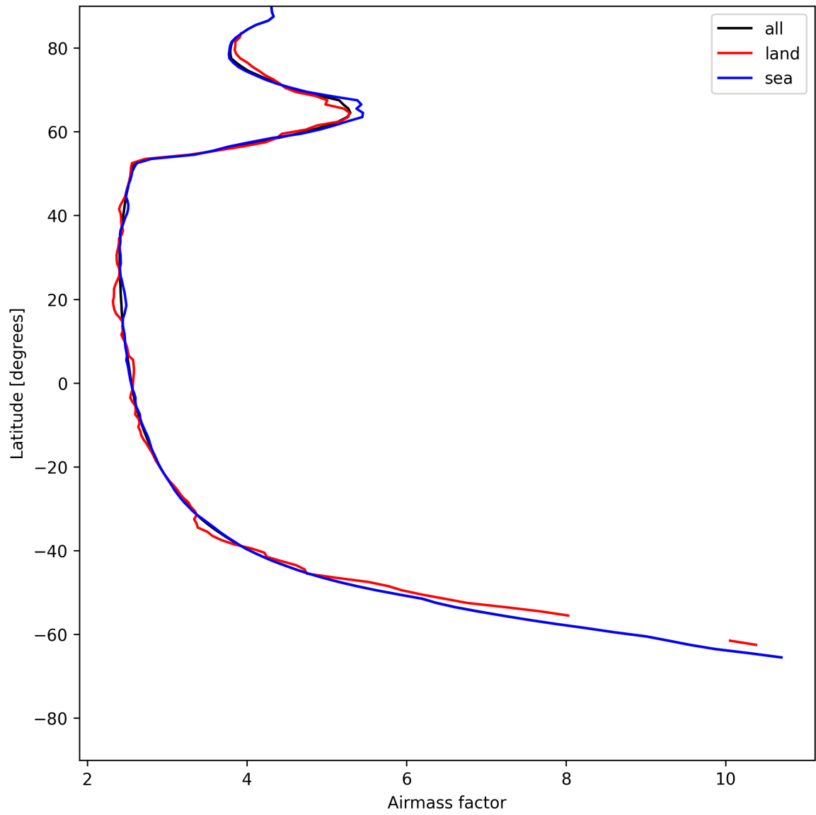
Figure 25: Zonal average of “Airmass factor” for 2025-06-09 to 2025-06-09.
