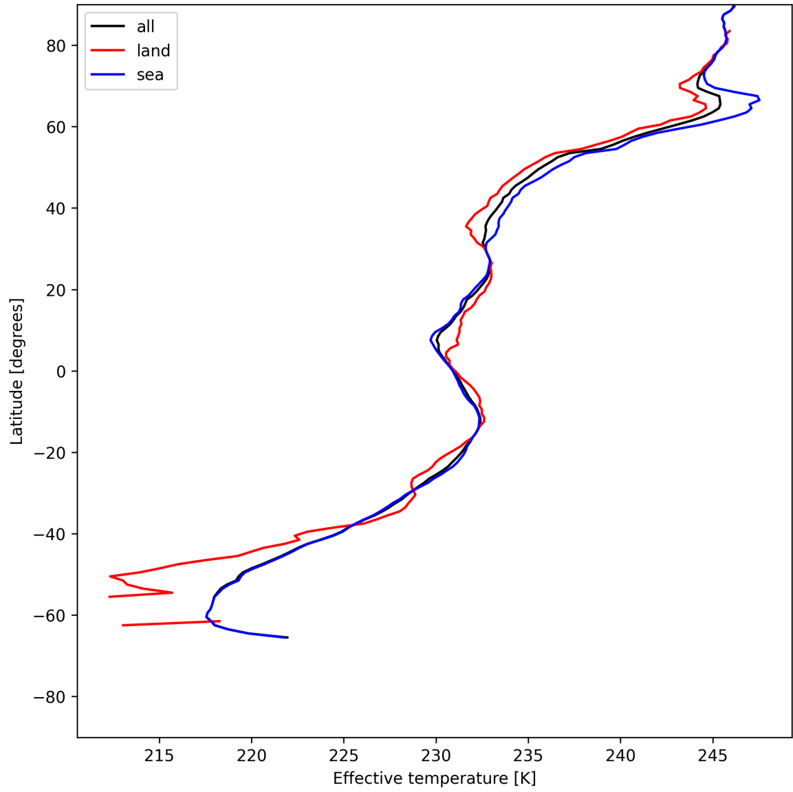
Figure 26: Zonal average of "Effective temperature" for 2025-06-09 to 2025-06-09.
