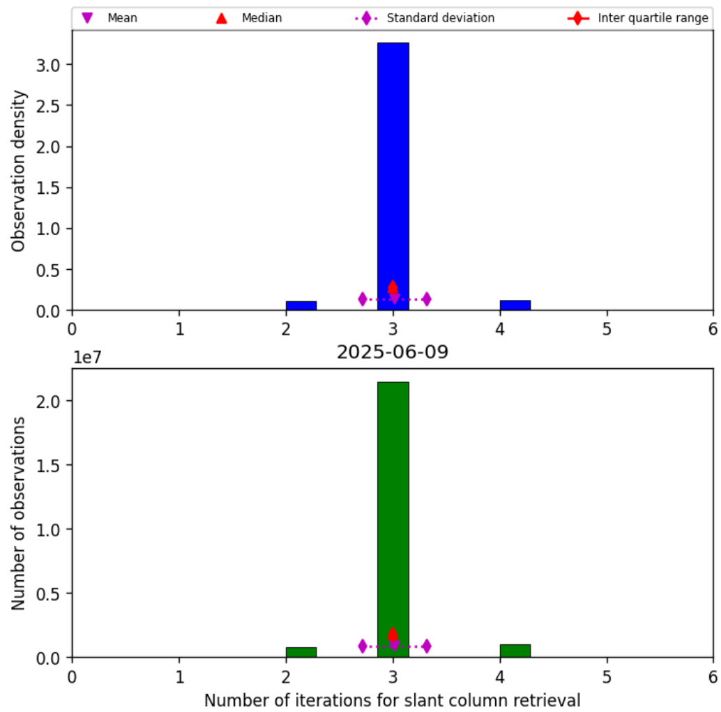
Figure 33: Histogram of “Number of iterations for slant column retrieval” for 2025-06-09 to 2025-06-09
