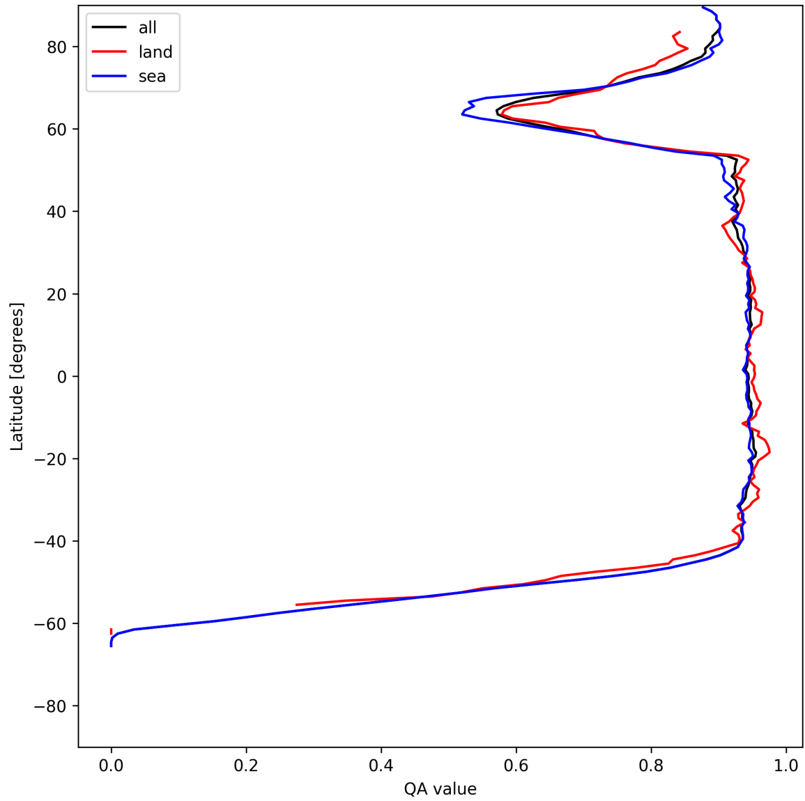
Figure 16: Zonal average of “QA value” for 2025-06-09 to 2025-06-09.
