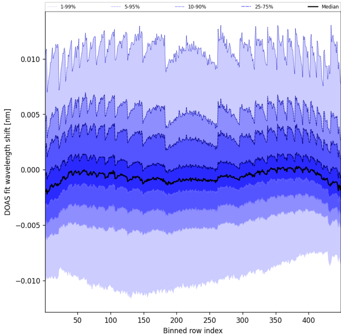
Figure 47: Along track statistics of "DOAS fit wavelength shift" for 2025-06-09 to 2025-06-09
