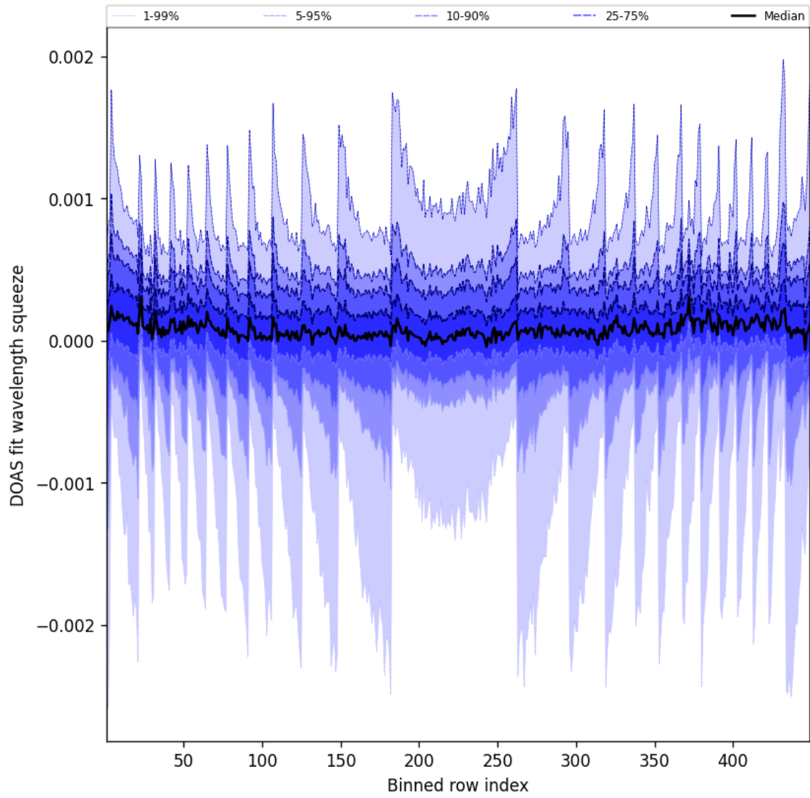
Figure 48: Along track statistics of “DOAS fit wavelength squeeze” for 2025-06-09 to 2025-06-09
