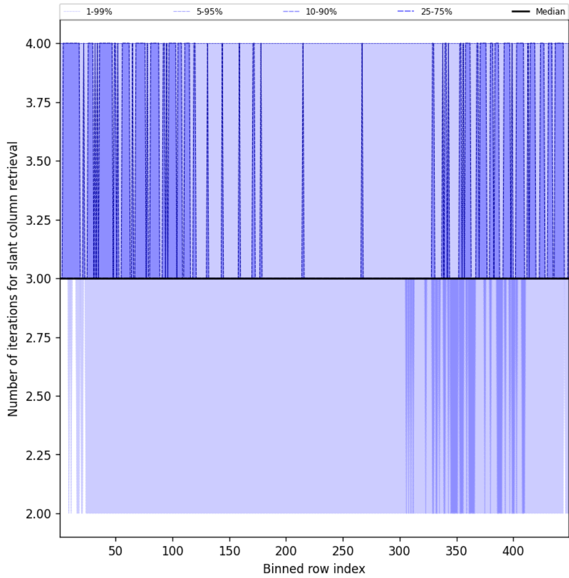
Figure 45: Along track statistics of “Number of iterations for slant column retrieval” for 2025-06-09 to 2025-06-09
