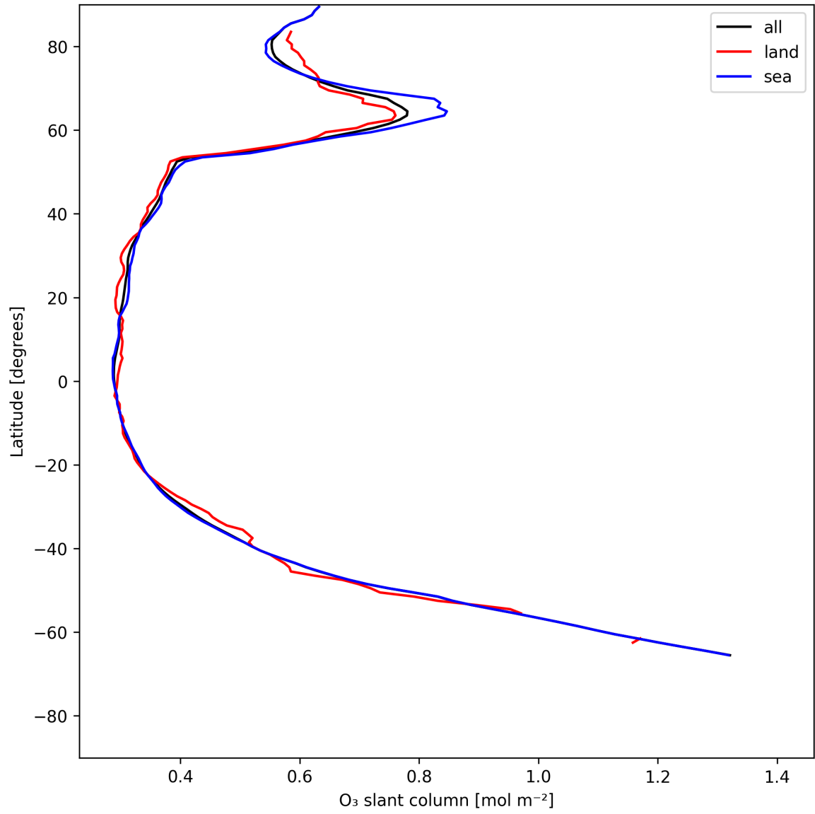
Figure 19: Zonal average of “O 3 slant column” for 2025-06-09 to 2025-06-09.
