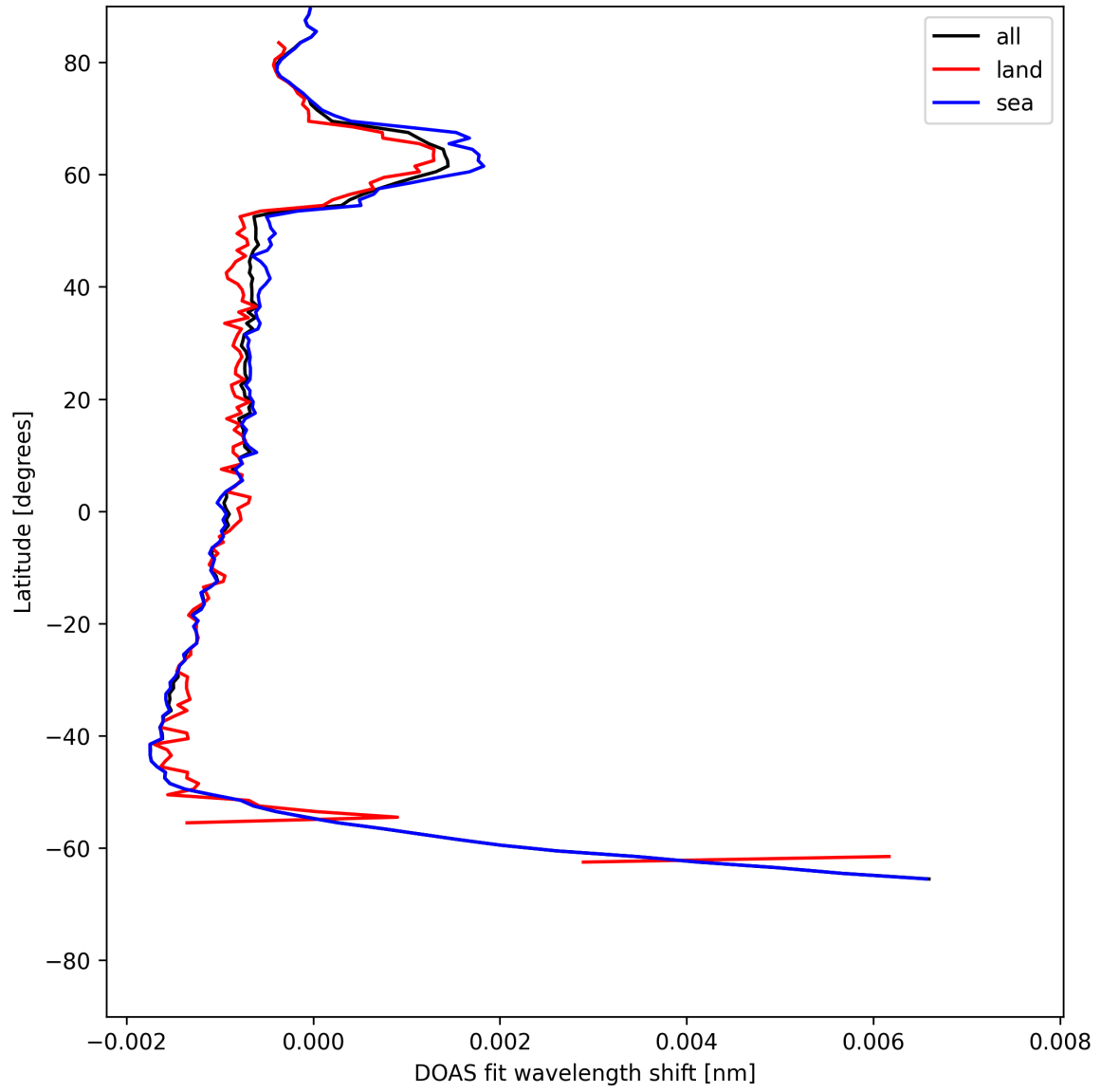
Figure 23: Zonal average of “DOAS fit wavelength shift” for 2025-06-09 to 2025-06-09.
