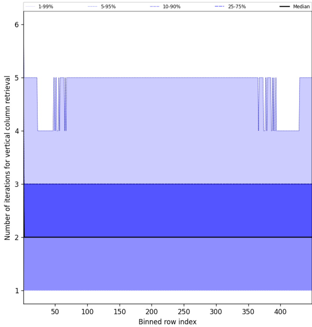
Figure 51: Along track statistics of “Number of iterations for vertical column retrieval” for 2025-06-09 to 2025-06-09
