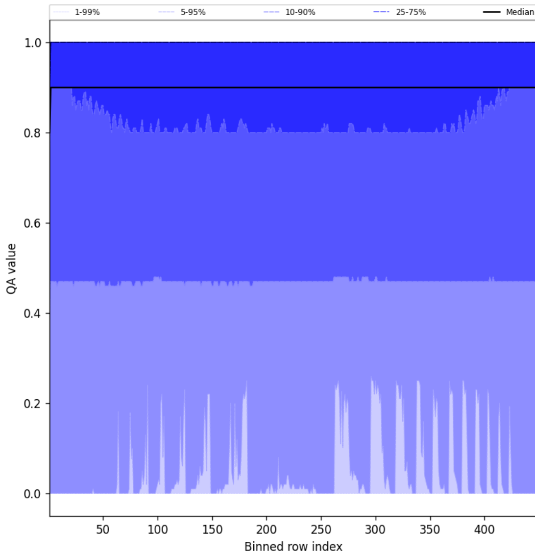
Figure 40: Along track statistics of “QA value” for 2025-06-09 to 2025-06-09
