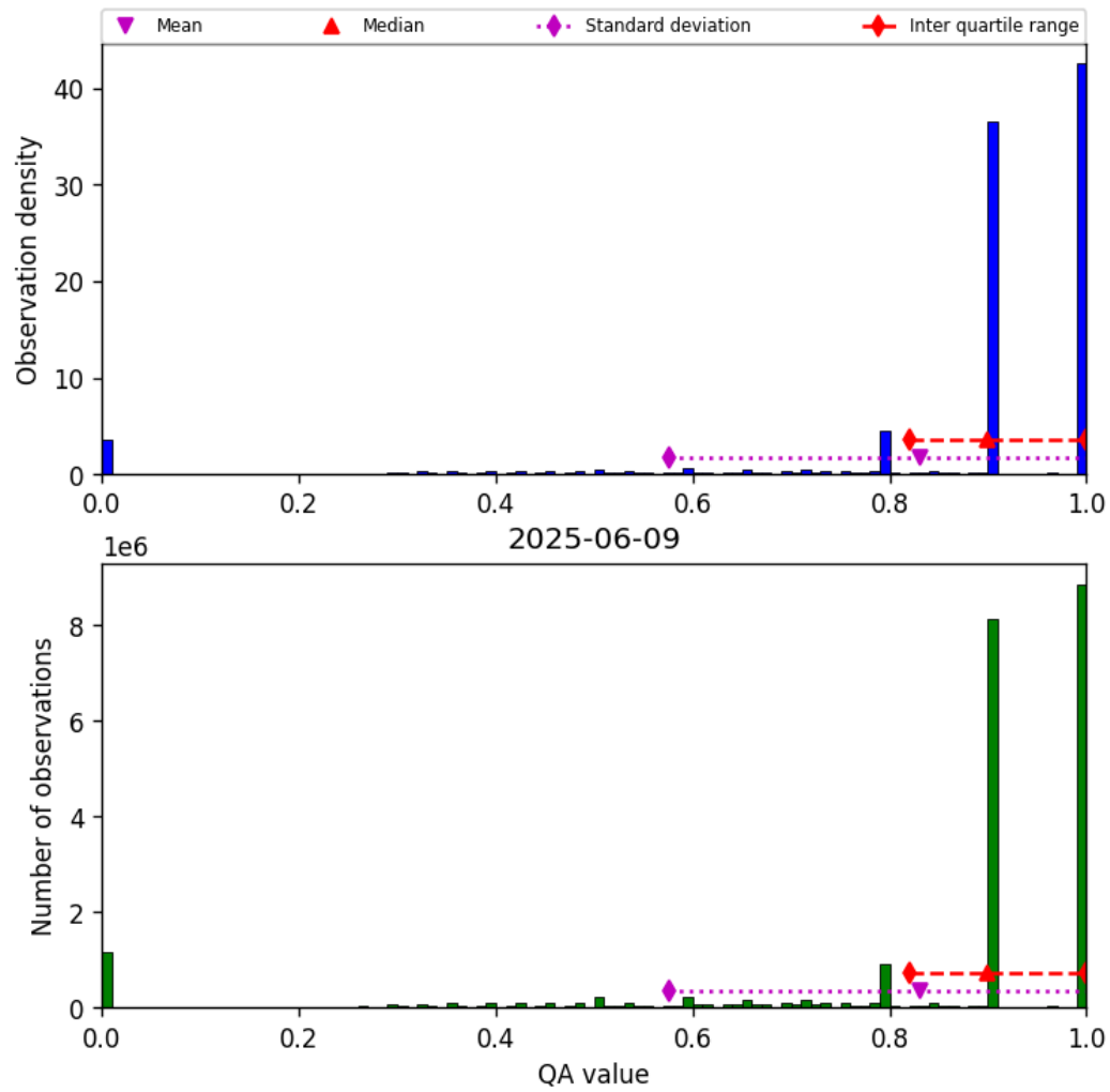
Figure 28: Histogram of “QA value” for 2025-06-09 to 2025-06-09
