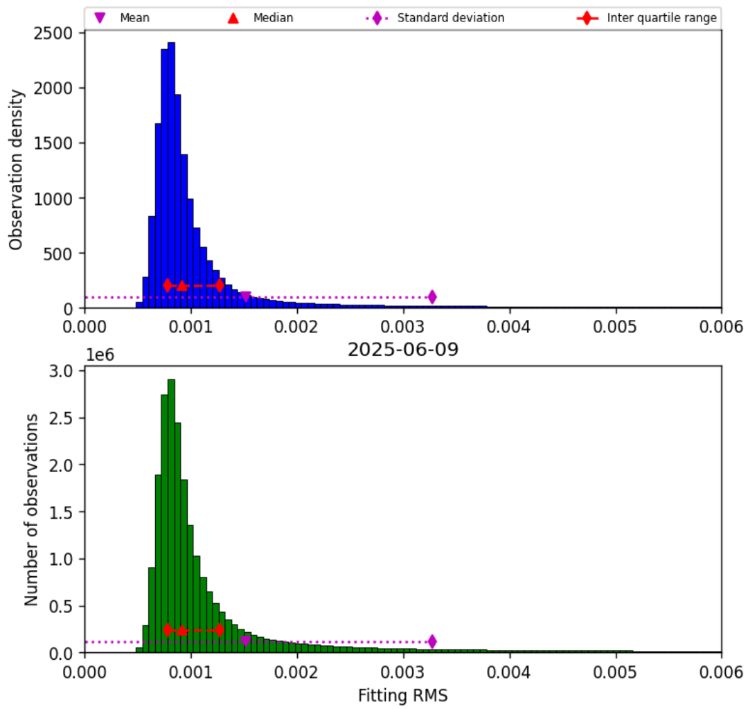
Figure 34: Histogram of “Fitting RMS” for 2025-06-09 to 2025-06-09
