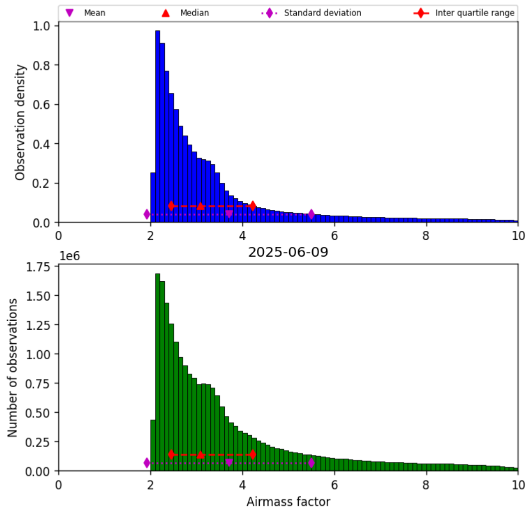
Figure 37: Histogram of “Airmass factor” for 2025-06-09 to 2025-06-09
