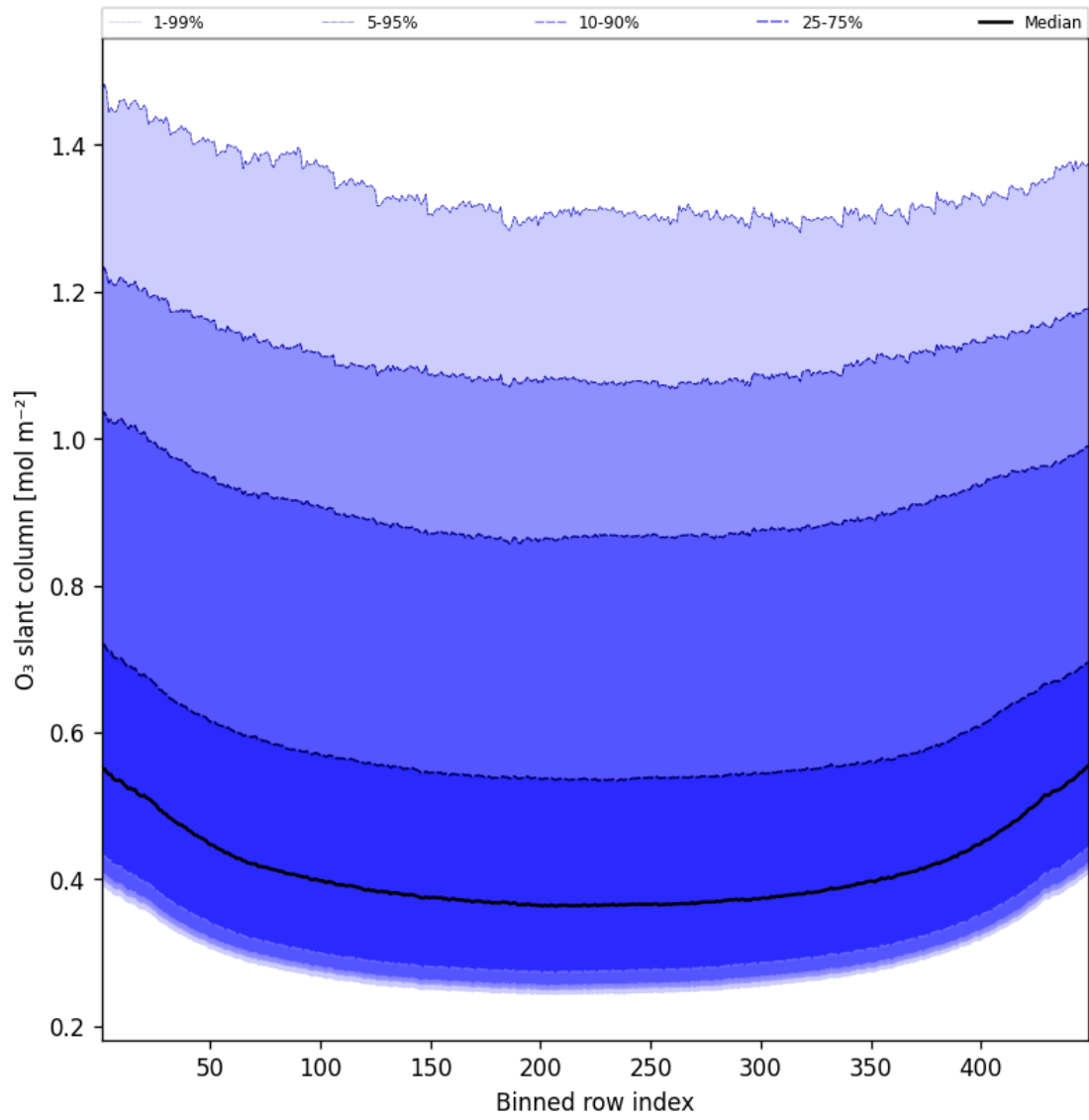
Figure 43: Along track statistics of “O 3 slant column” for 2025-06-09 to 2025-06-09
