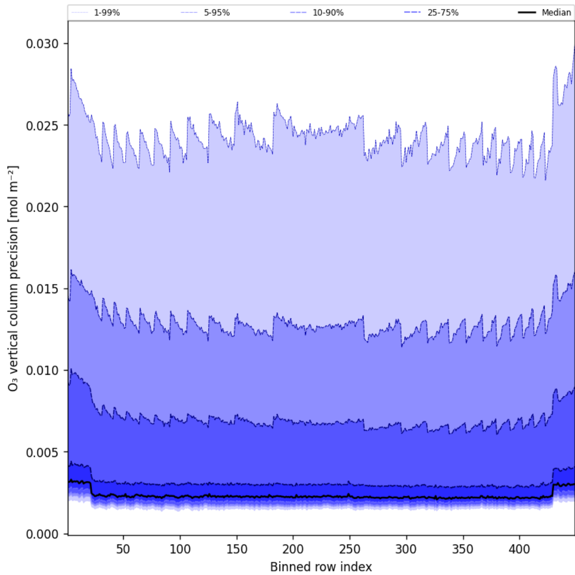
Figure 42: Along track statistics of “O 3 vertical column precision” for 2025-06-09 to 2025-06-09
