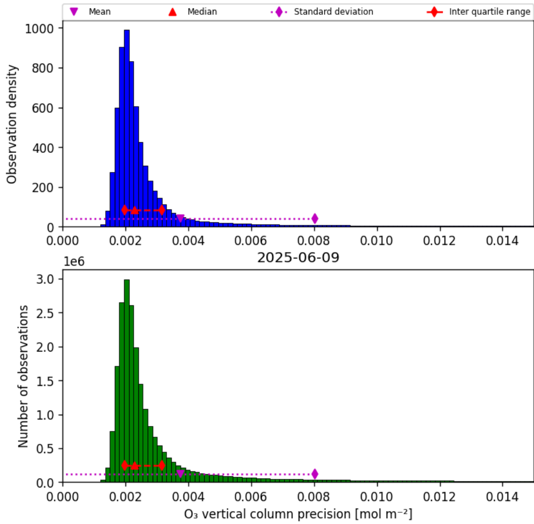
Figure 30: Histogram of “O 3 vertical column precision” for 2025-06-09 to 2025-06-09
