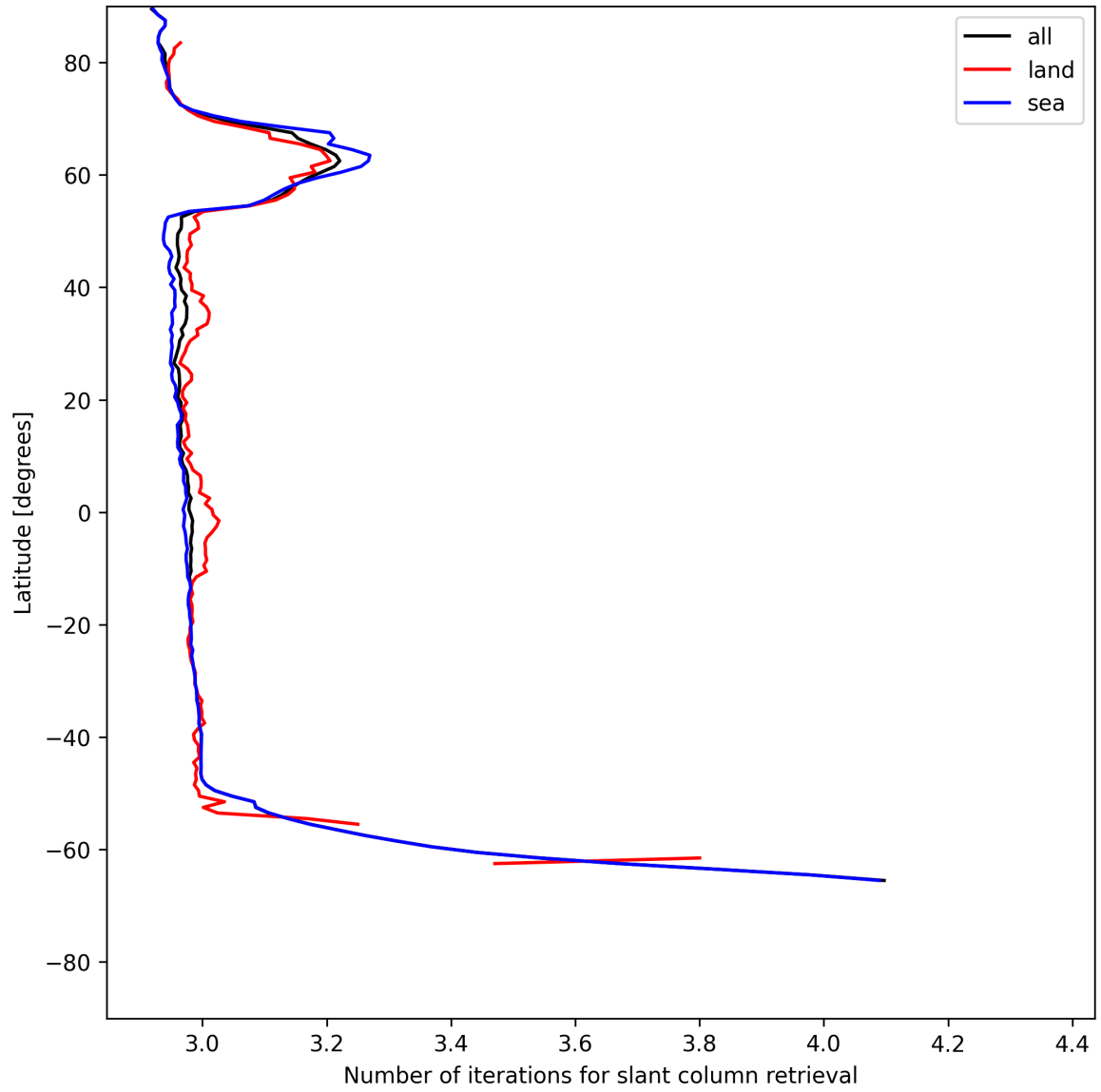
Figure 21: Zonal average of “Number of iterations for slant column retrieval” for 2025-06-09 to 2025-06-09.
