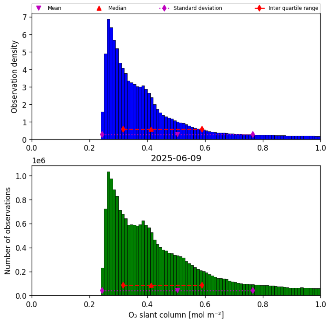
Figure 31: Histogram of “O 3 slant column” for 2025-06-09 to 2025-06-09
