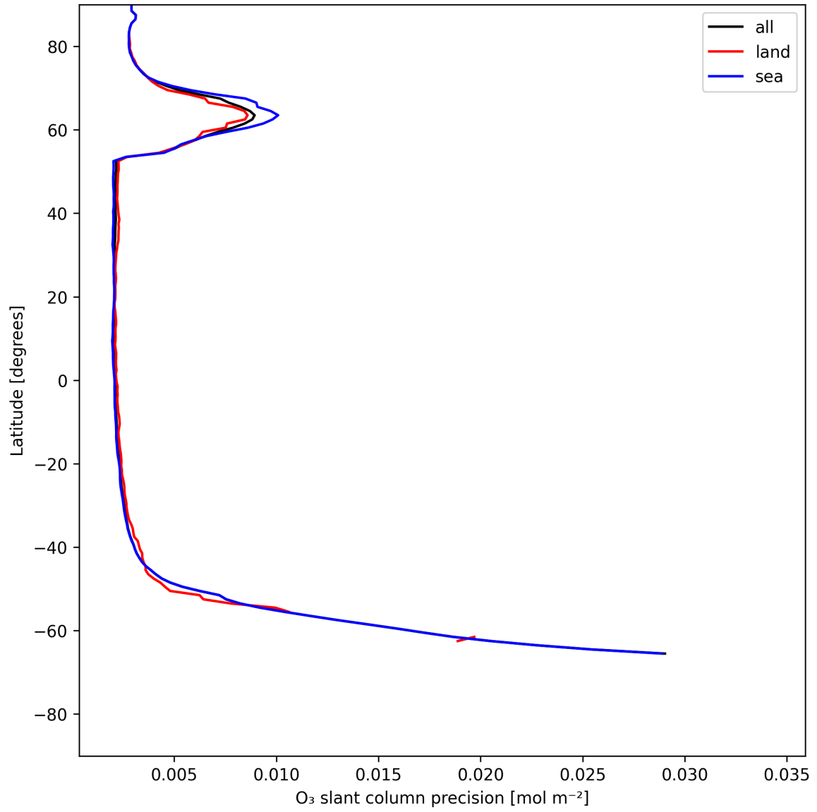
Figure 20: Zonal average of “O 3 slant column precision” for 2025-06-09 to 2025-06-09.
