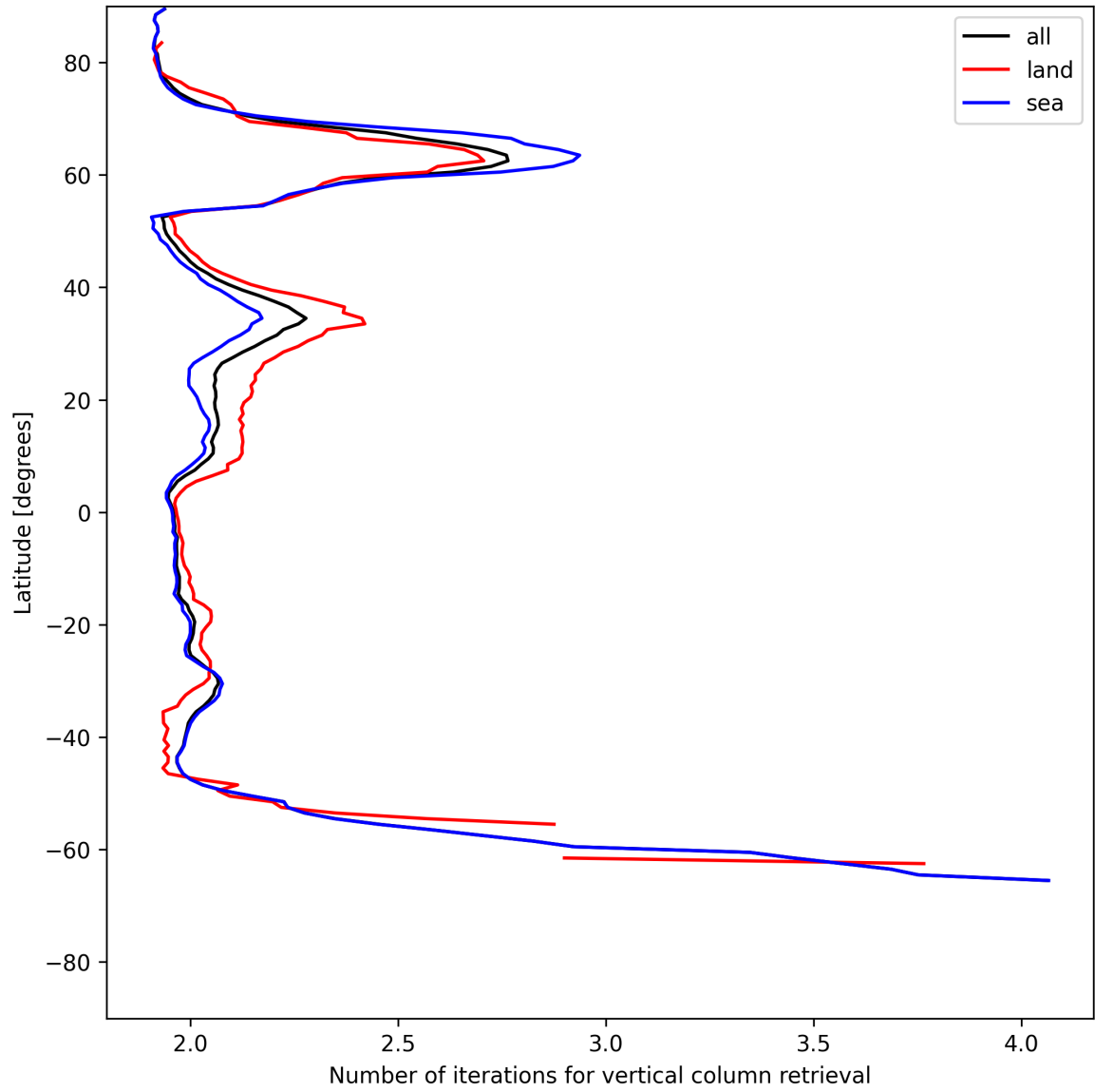
Figure 27: Zonal average of “Number of iterations for vertical column retrieval” for 2025-06-09 to 2025-06-09.
