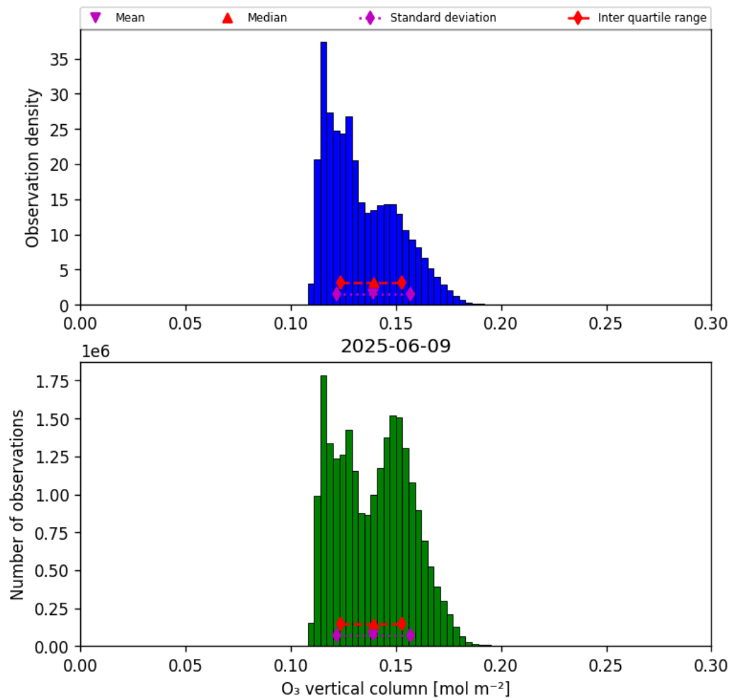
Figure 29: Histogram of “O 3 vertical column” for 2025-06-09 to 2025-06-09
