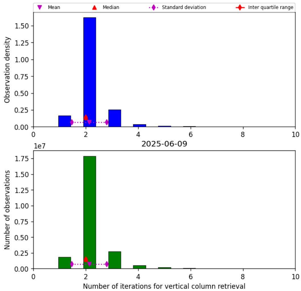
Figure 39: Histogram of “Number of iterations for vertical column retrieval” for 2025-06-09 to 2025-06-09
