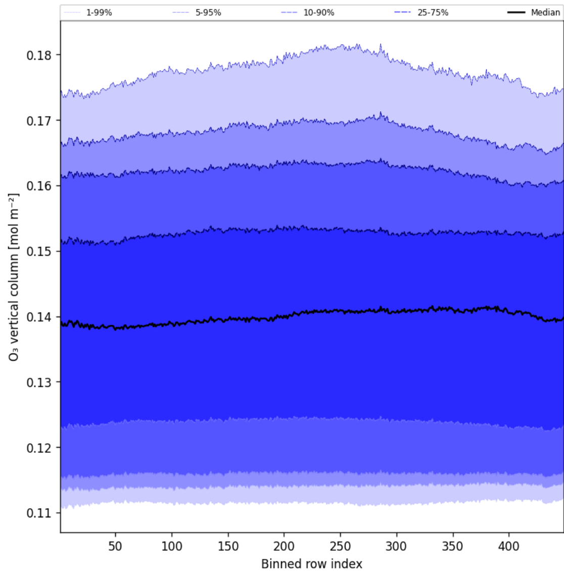
Figure 41: Along track statistics of “O 3 vertical column” for 2025-06-09 to 2025-06-09
