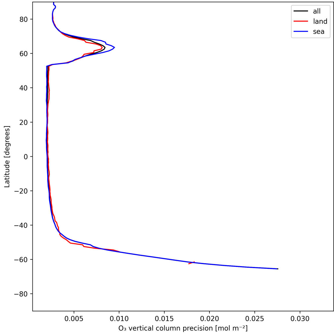
Figure 18: Zonal average of “O 3 vertical column precision” for 2025-06-09 to 2025-06-09.
