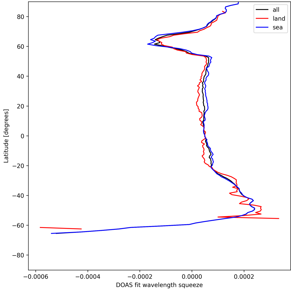
Figure 24: Zonal average of “DOAS fit wavelength squeeze” for 2025-06-09 to 2025-06-09.
