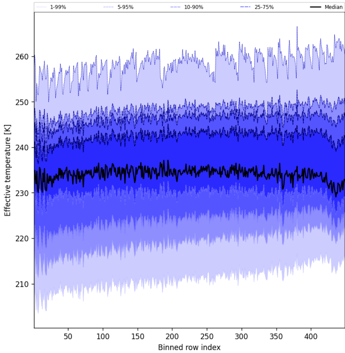
Figure 50: Along track statistics of “Effective temperature” for 2025-06-09 to 2025-06-09
