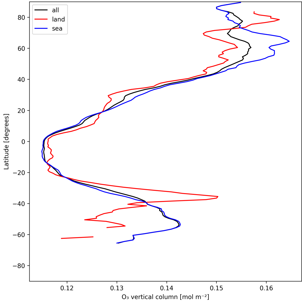
Figure 17: Zonal average of “O 3 vertical column” for 2025-06-09 to 2025-06-09.
