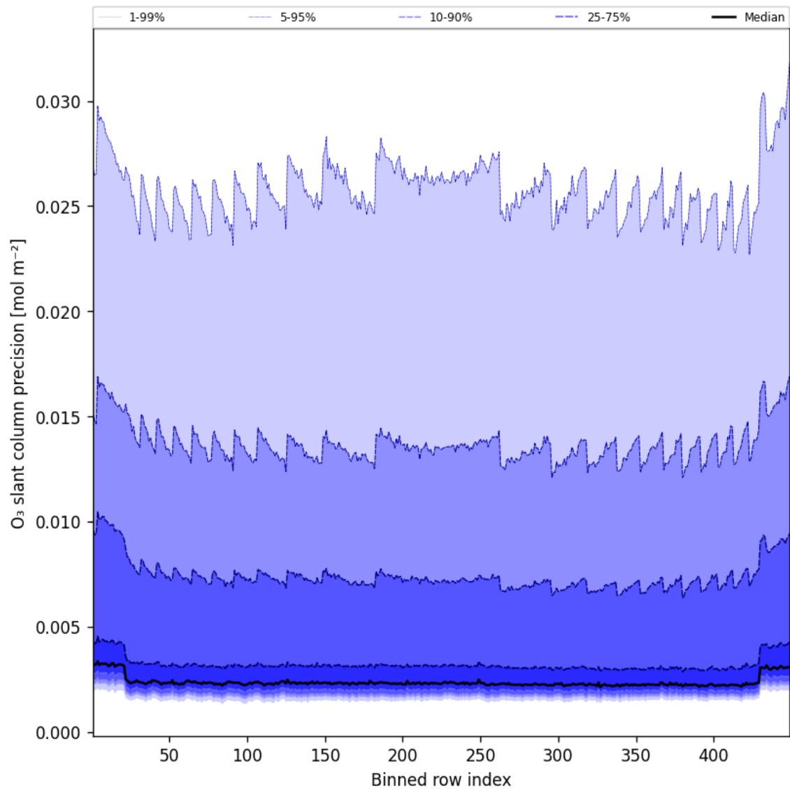
Figure 44: Along track statistics of “O 3 slant column precision” for 2025-06-09 to 2025-06-09
