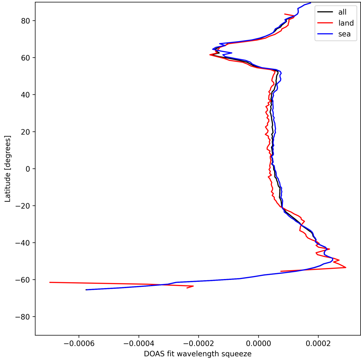
Figure 24: Zonal average of “DOAS fit wavelength squeeze” for 2025-06-10 to 2025-06-11.
