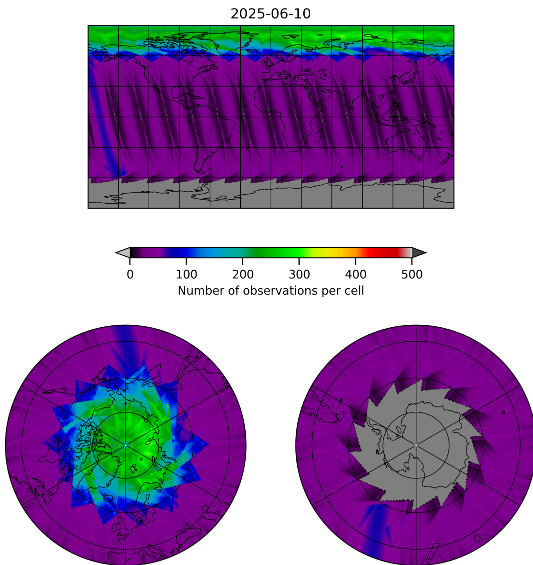
Figure 15: Map of the number of observations for 2025-06-10 to 2025-06-11
