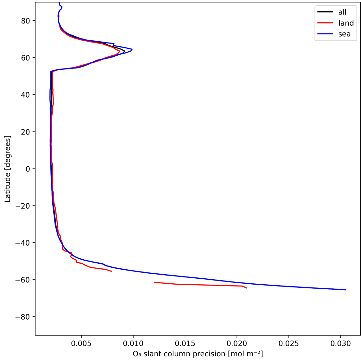
Figure 20: Zonal average of “O 3 slant column precision” for 2025-06-10 to 2025-06-11.
