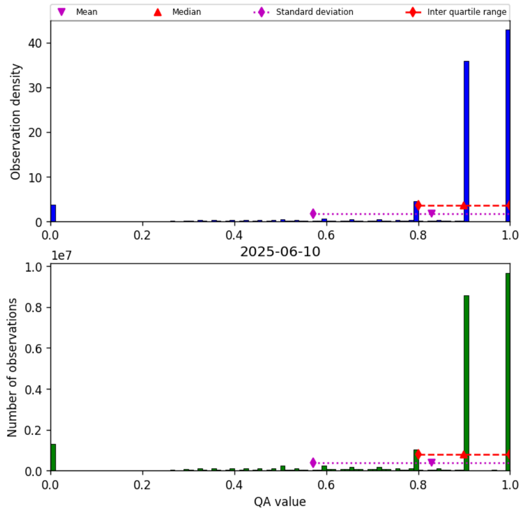
Figure 28: Histogram of “QA value” for 2025-06-10 to 2025-06-11
