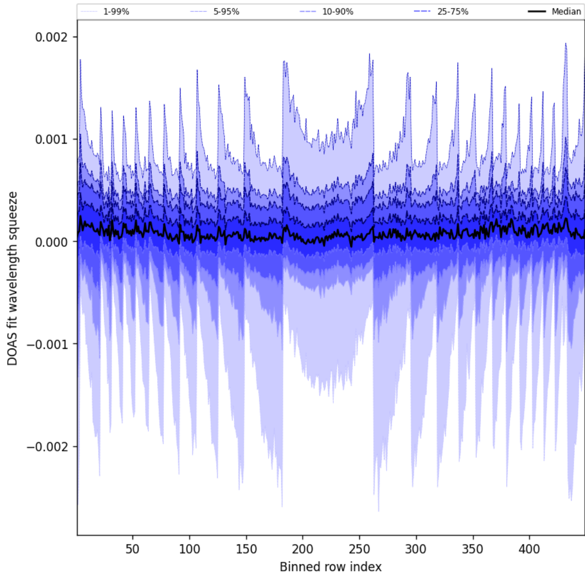
Figure 48: Along track statistics of “DOAS fit wavelength squeeze” for 2025-06-10 to 2025-06-11
