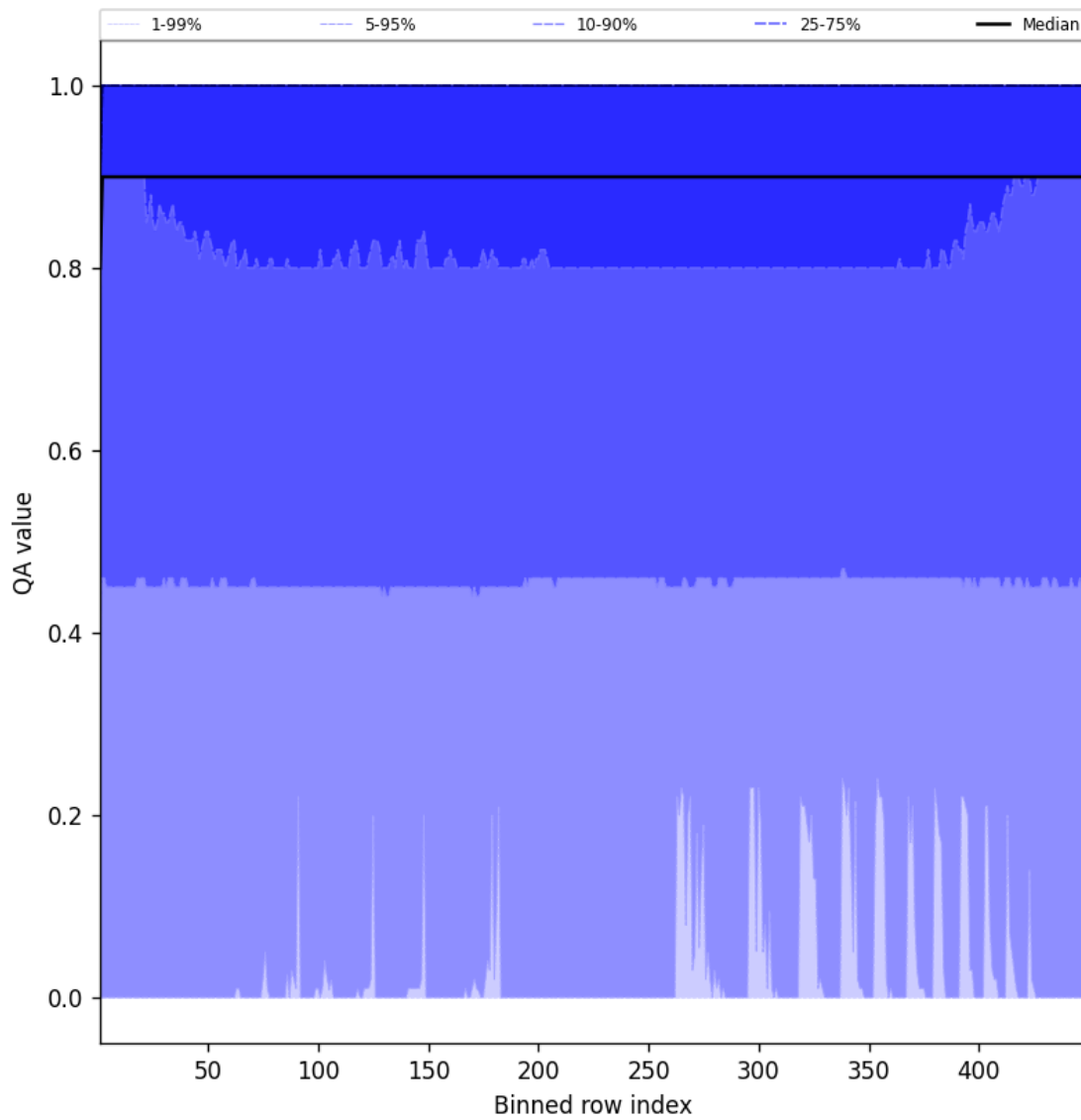
Figure 40: Along track statistics of “QA value” for 2025-06-10 to 2025-06-11
