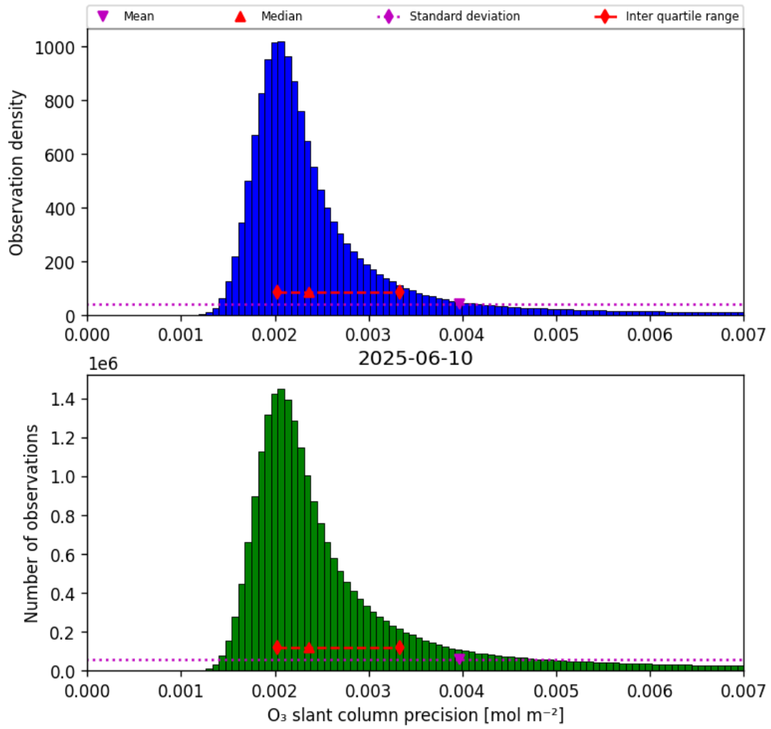
Figure 32: Histogram of “O 3 slant column precision” for 2025-06-10 to 2025-06-11
