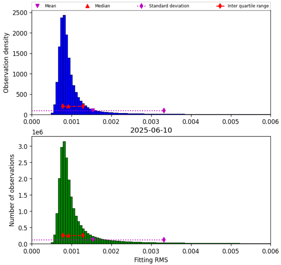
Figure 34: Histogram of “Fitting RMS” for 2025-06-10 to 2025-06-11
