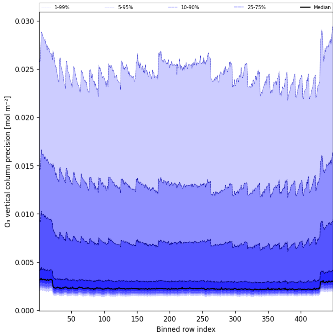
Figure 42: Along track statistics of “O 3 vertical column precision” for 2025-06-10 to 2025-06-11
