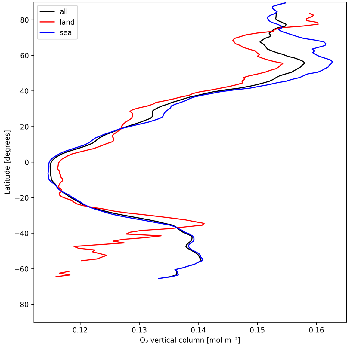
Figure 17: Zonal average of “O 3 vertical column” for 2025-06-10 to 2025-06-11.
