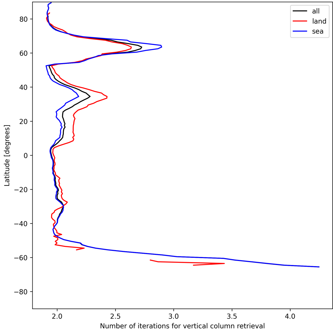
Figure 27: Zonal average of “Number of iterations for vertical column retrieval” for 2025-06-10 to 2025-06-11.
