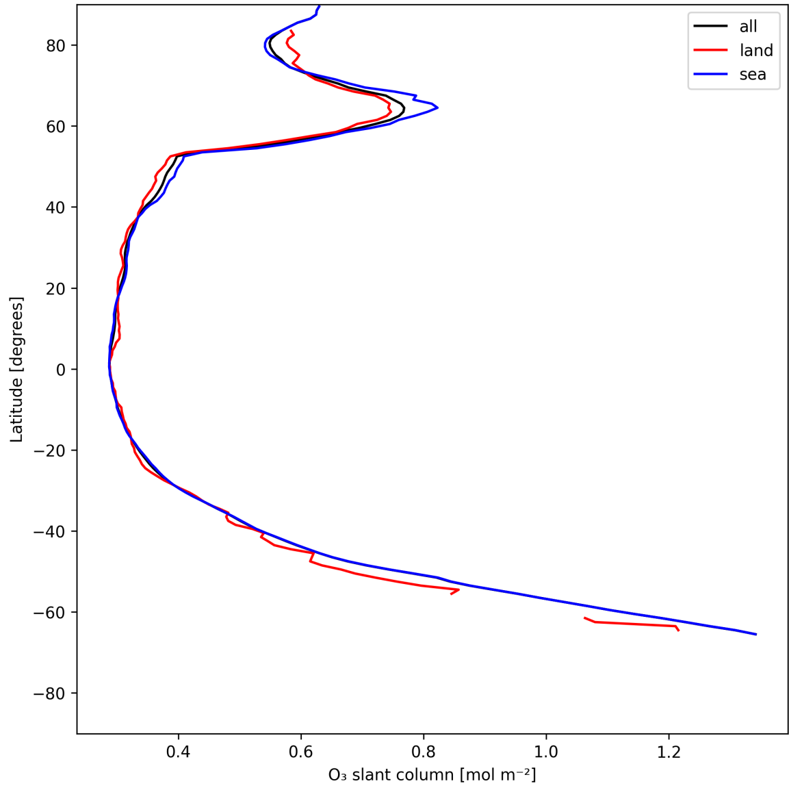
Figure 19: Zonal average of “O 3 slant column” for 2025-06-10 to 2025-06-11.
