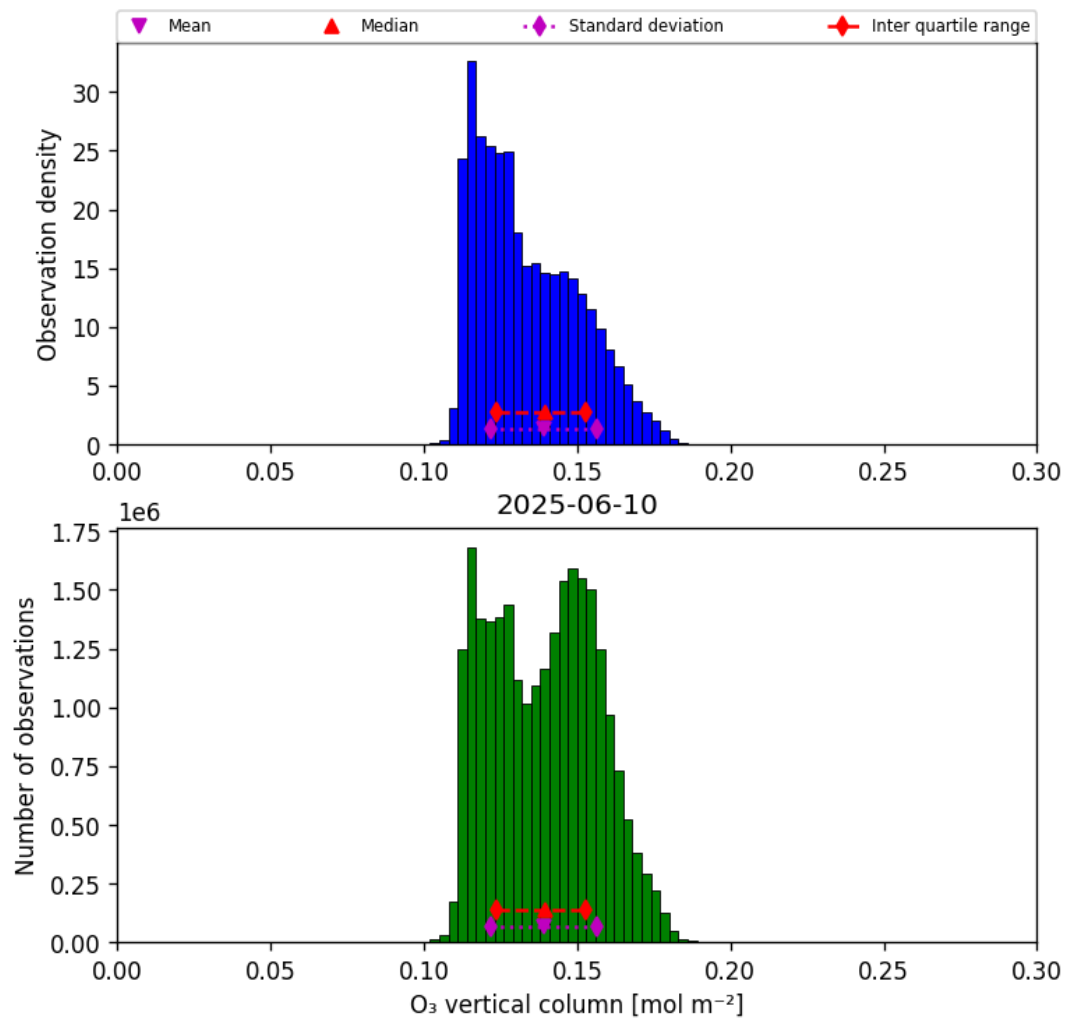
Figure 29: Histogram of “O 3 vertical column” for 2025-06-10 to 2025-06-11
