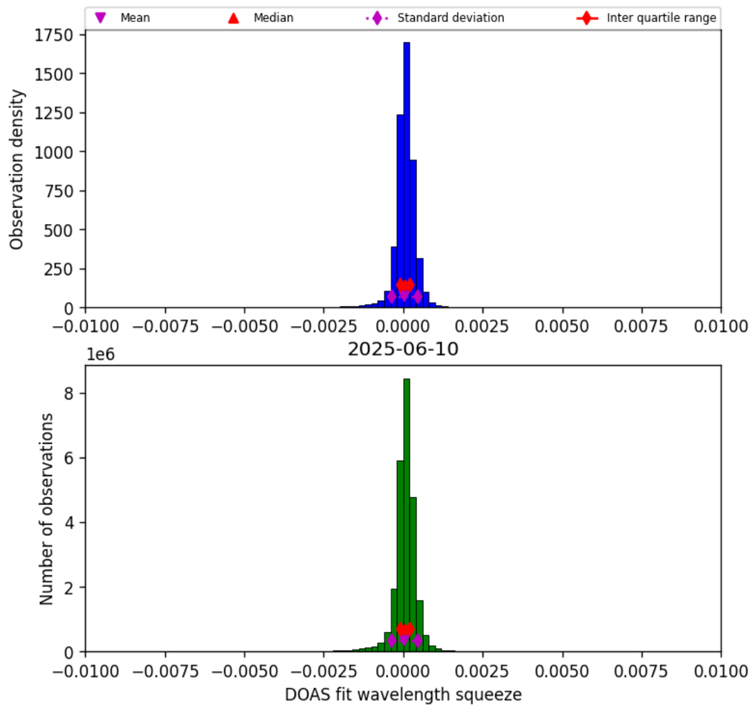
Figure 36: Histogram of “DOAS fit wavelength squeeze” for 2025-06-10 to 2025-06-11
