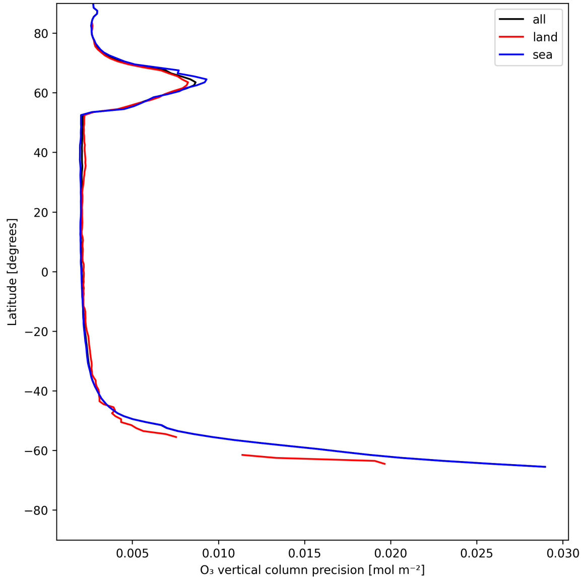
Figure 18: Zonal average of “O 3 vertical column precision” for 2025-06-10 to 2025-06-11.
