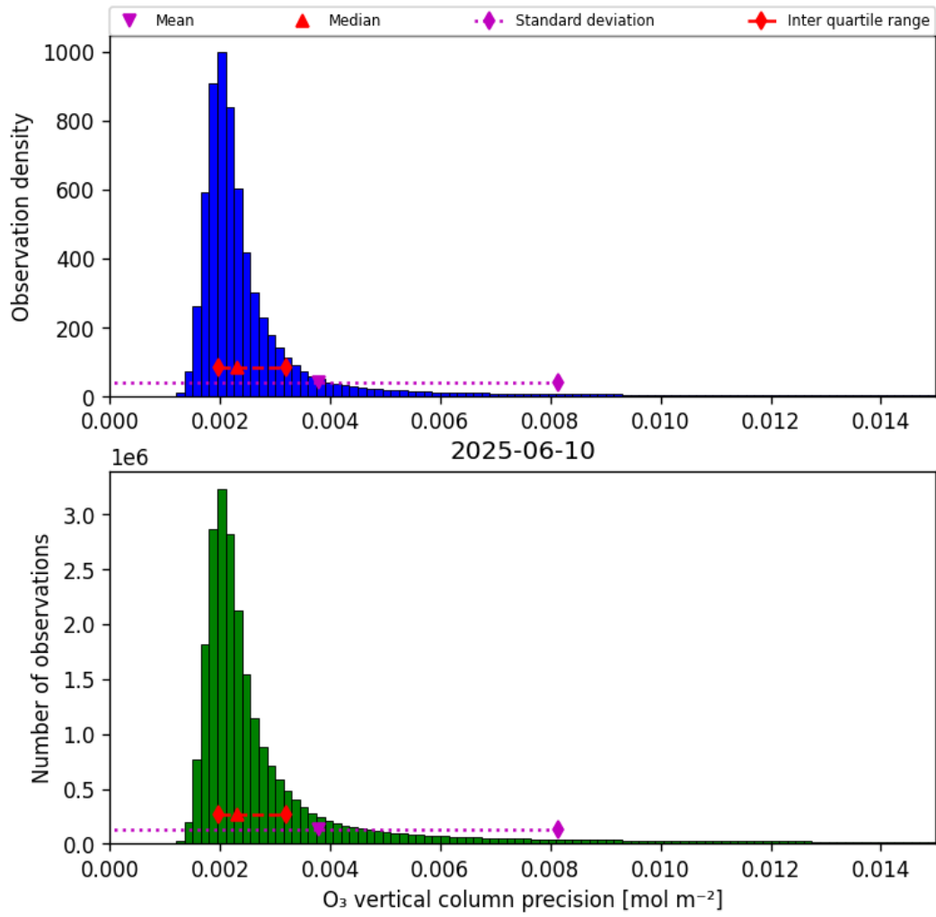
Figure 30: Histogram of “O 3 vertical column precision” for 2025-06-10 to 2025-06-11
