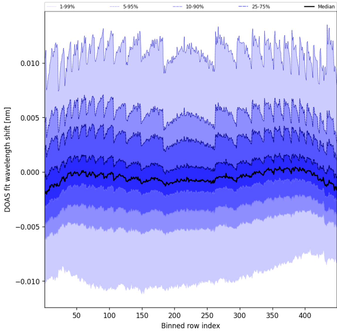
Figure 47: Along track statistics of “DOAS fit wavelength shift” for 2025-06-10 to 2025-06-11
