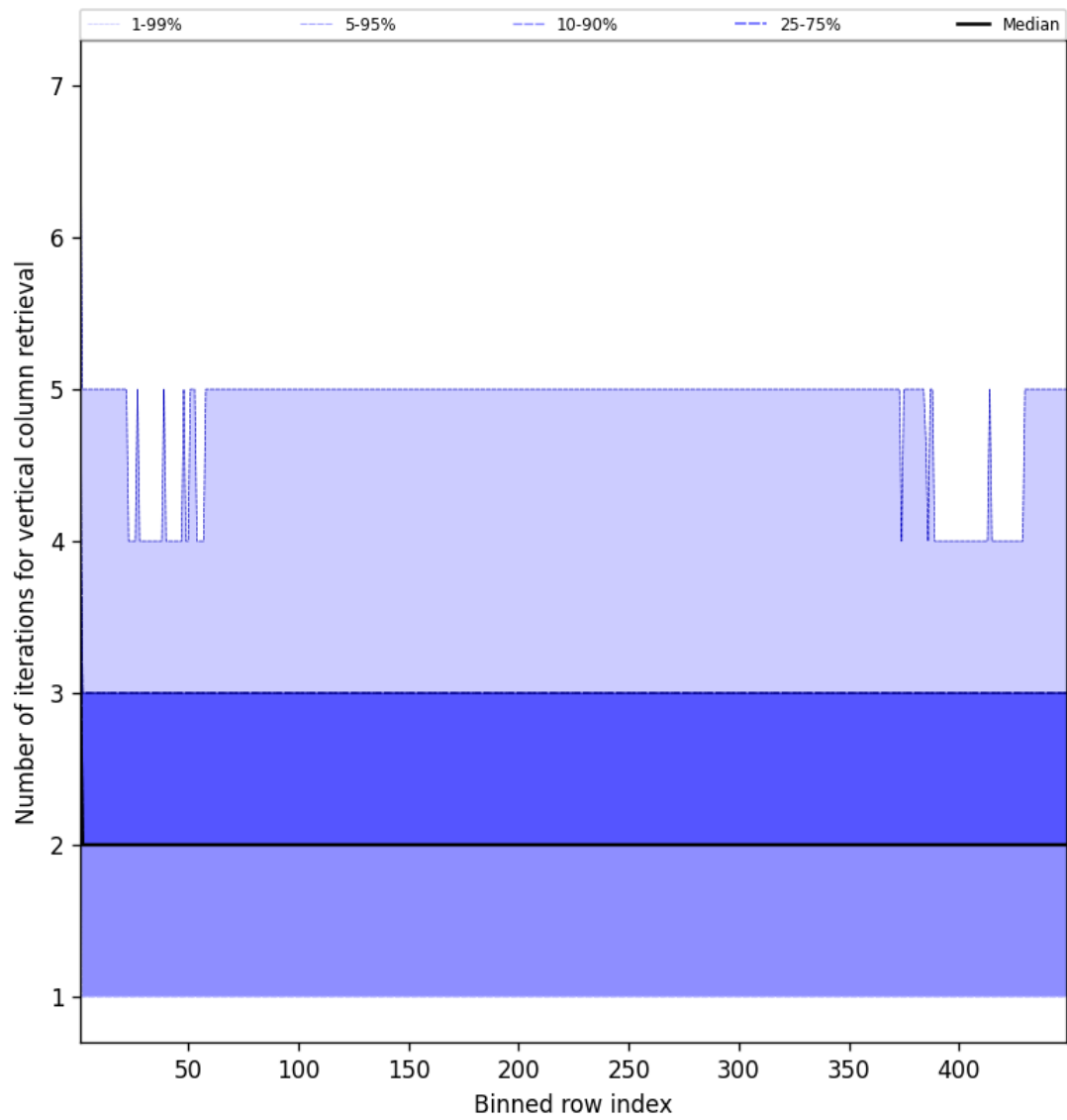
Figure 51: Along track statistics of “Number of iterations for vertical column retrieval” for 2025-06-10 to 2025-06-11
