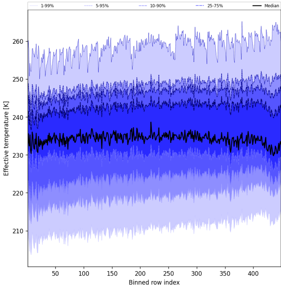
Figure 50: Along track statistics of “Effective temperature” for 2025-06-10 to 2025-06-11
