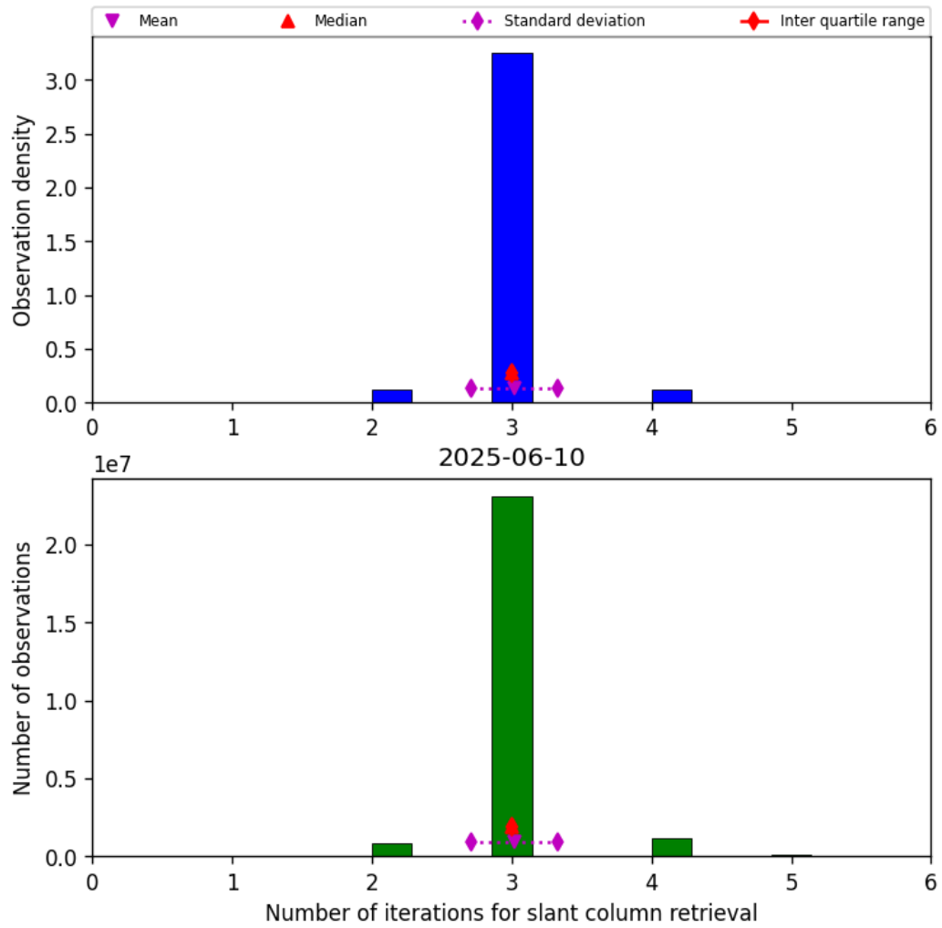
Figure 33: Histogram of “Number of iterations for slant column retrieval” for 2025-06-10 to 2025-06-11
