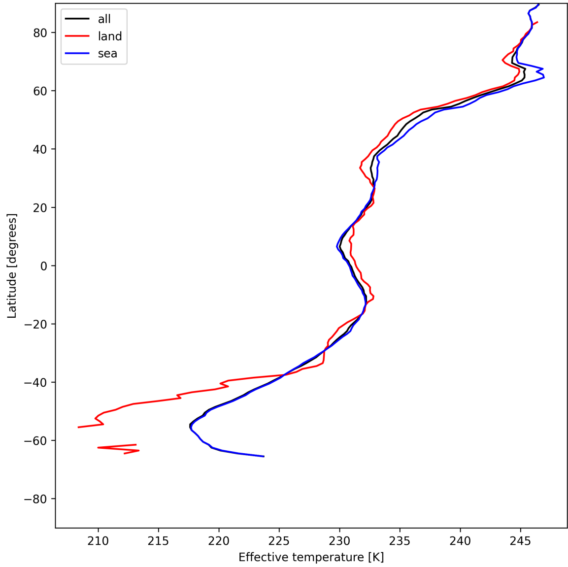
Figure 26: Zonal average of "Effective temperature" for 2025-06-10 to 2025-06-11.
