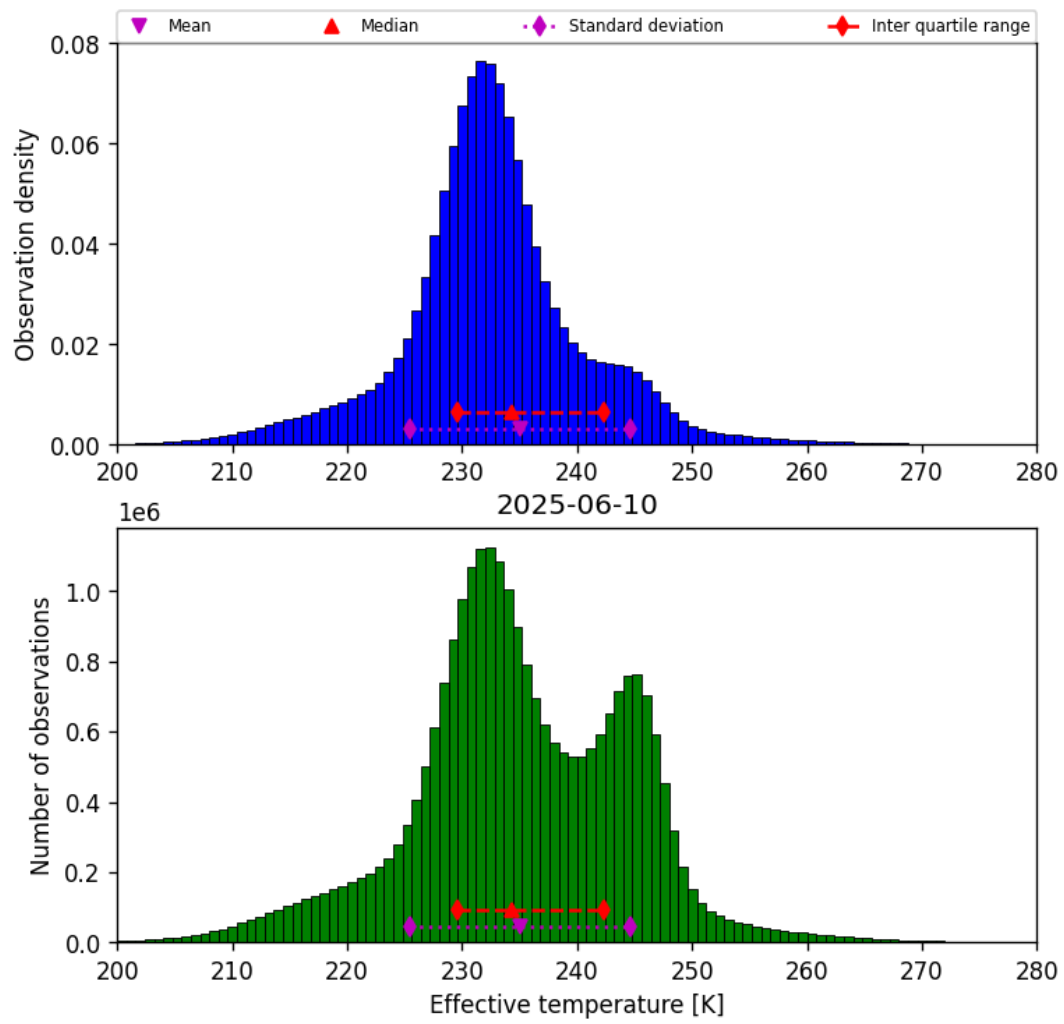
Figure 38: Histogram of “Effective temperature” for 2025-06-10 to 2025-06-11
