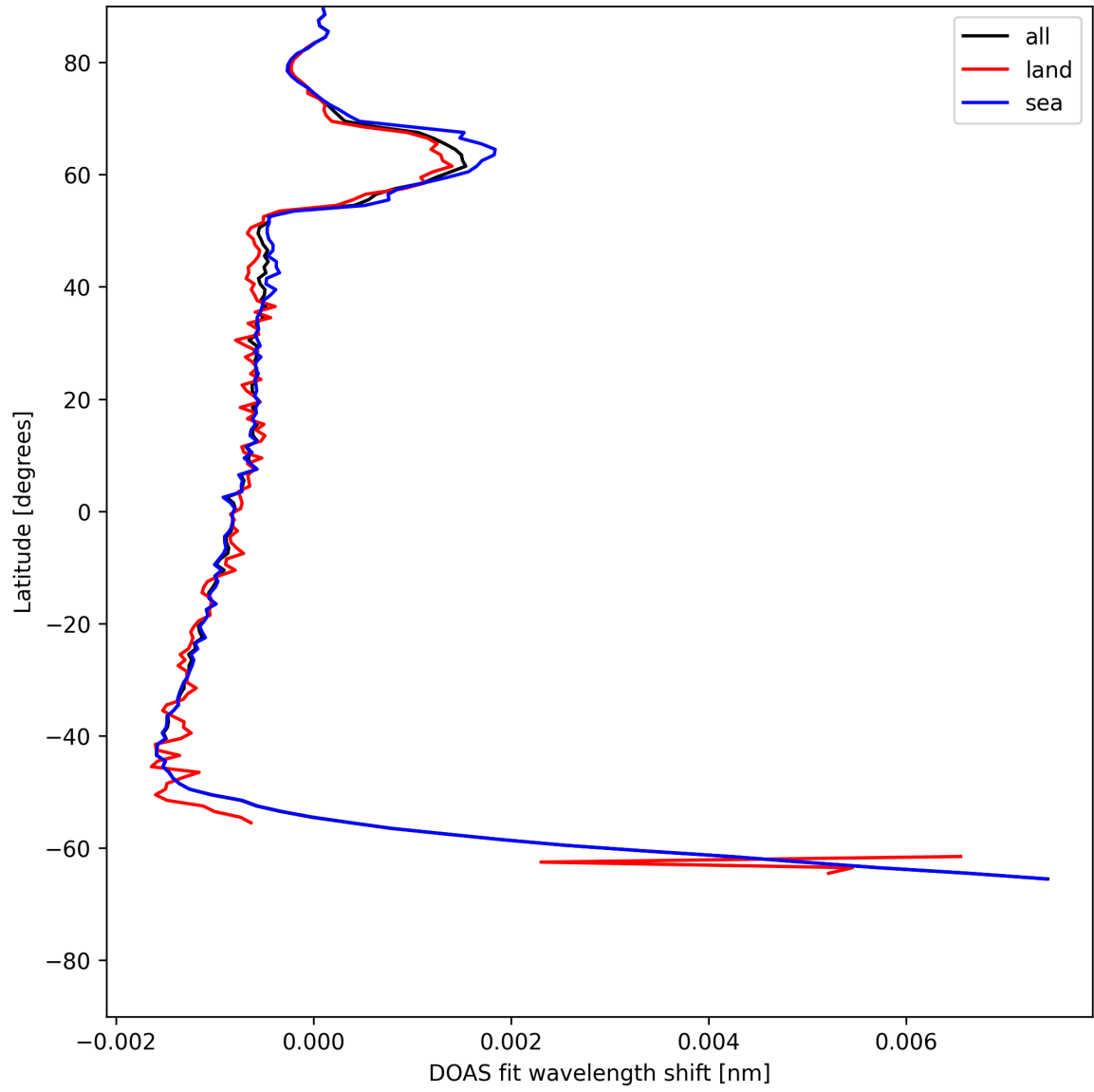
Figure 23: Zonal average of “DOAS fit wavelength shift” for 2025-06-10 to 2025-06-11.
