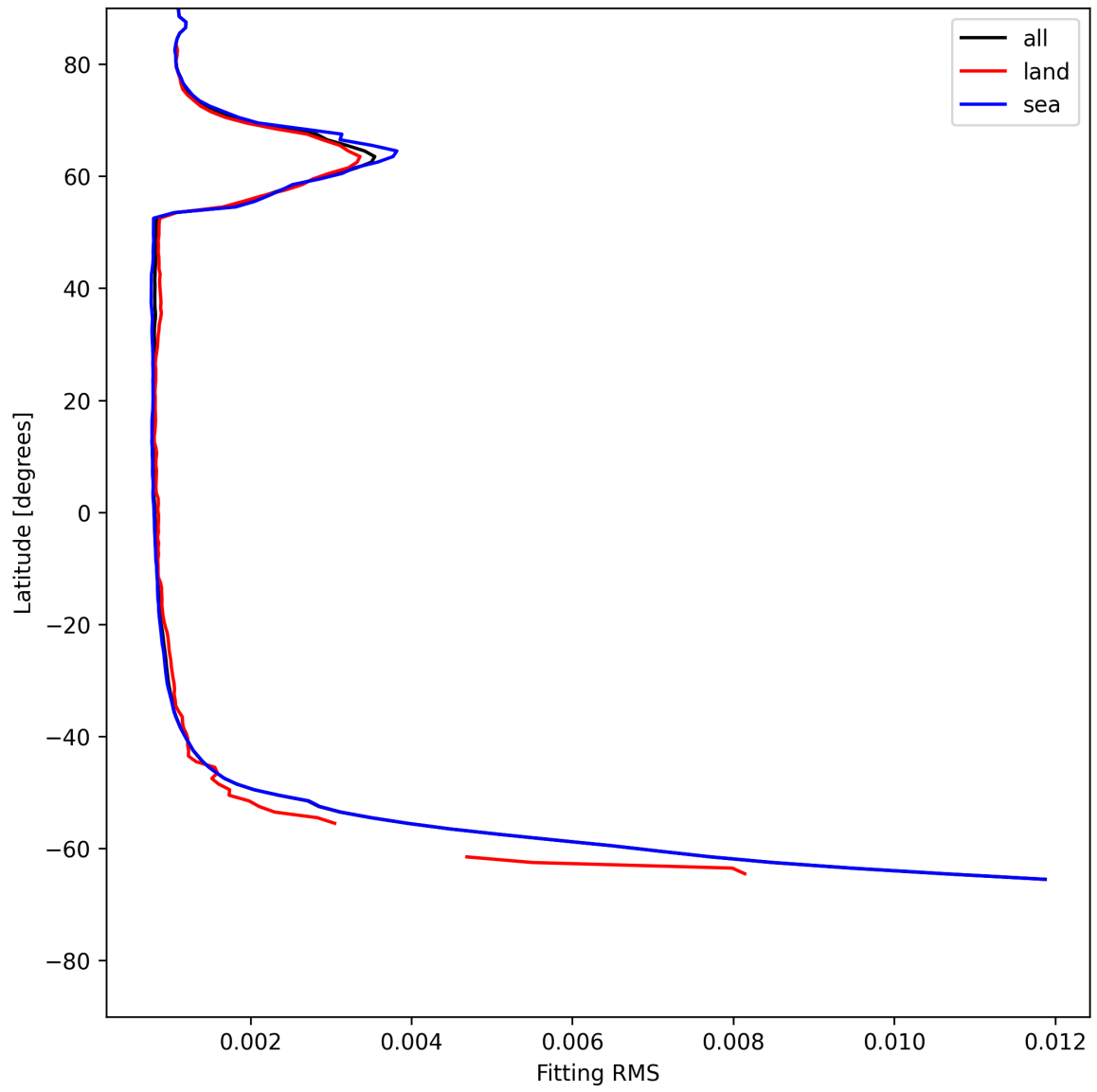
Figure 22: Zonal average of “Fitting RMS” for 2025-06-10 to 2025-06-11.
