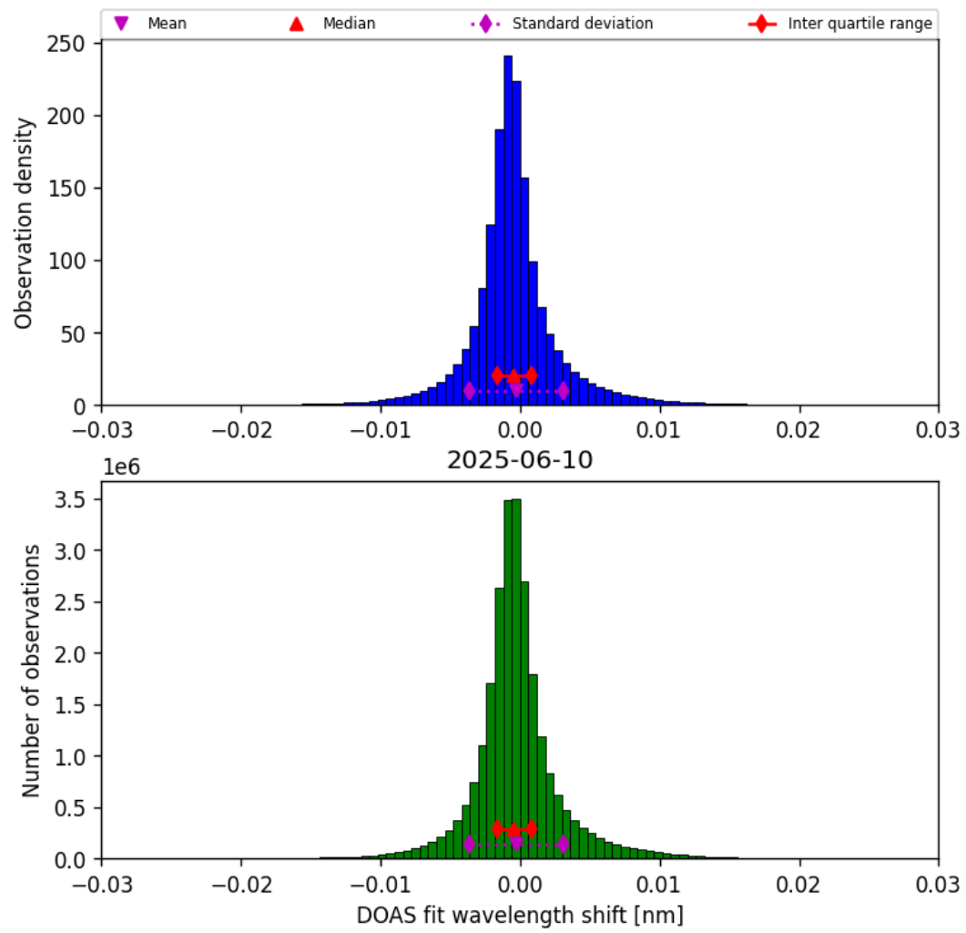
Figure 35: Histogram of “DOAS fit wavelength shift” for 2025-06-10 to 2025-06-11
