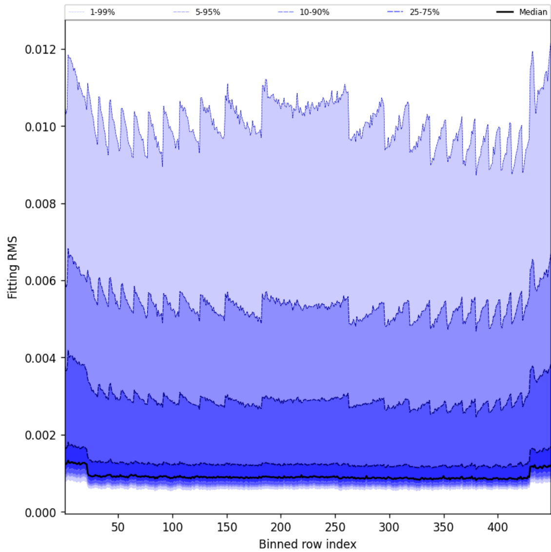
Figure 46: Along track statistics of “Fitting RMS” for 2025-06-10 to 2025-06-11
