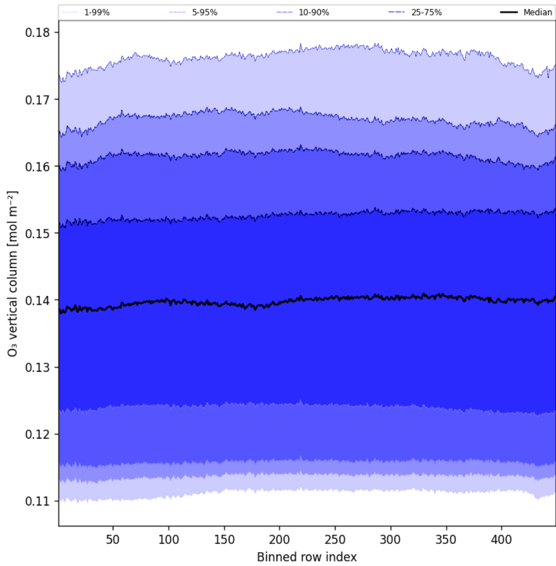
Figure 41: Along track statistics of “ O_3 vertical column” for 2025-06-10 to 2025-06-11
