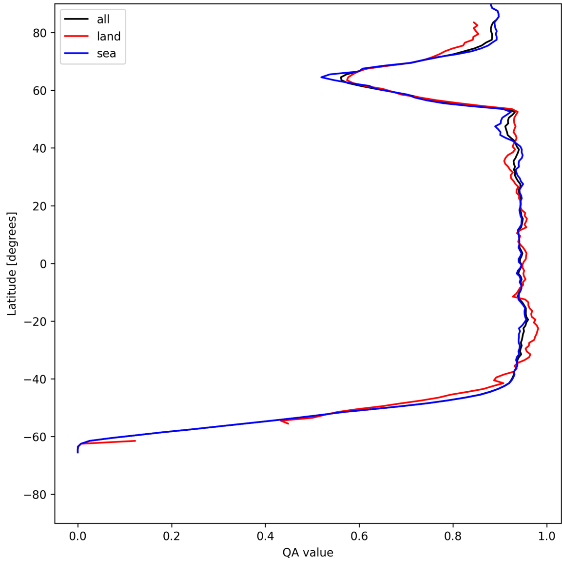
Figure 16: Zonal average of “QA value” for 2025-06-10 to 2025-06-11.
