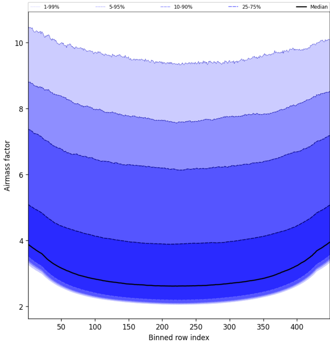
Figure 49: Along track statistics of “Airmass factor” for 2025-06-10 to 2025-06-11
