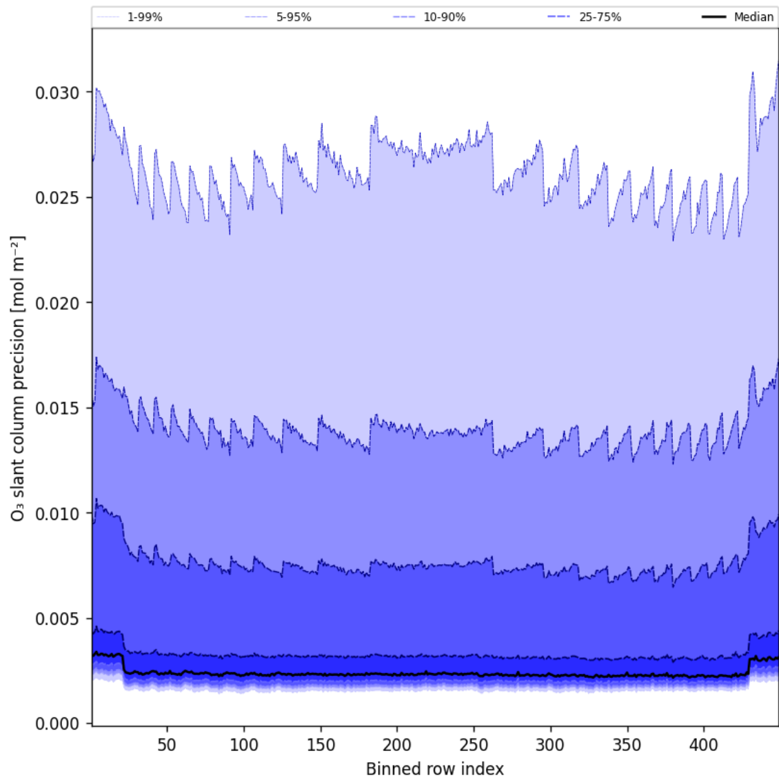
Figure 44: Along track statistics of “O 3 slant column precision” for 2025-06-10 to 2025-06-11
