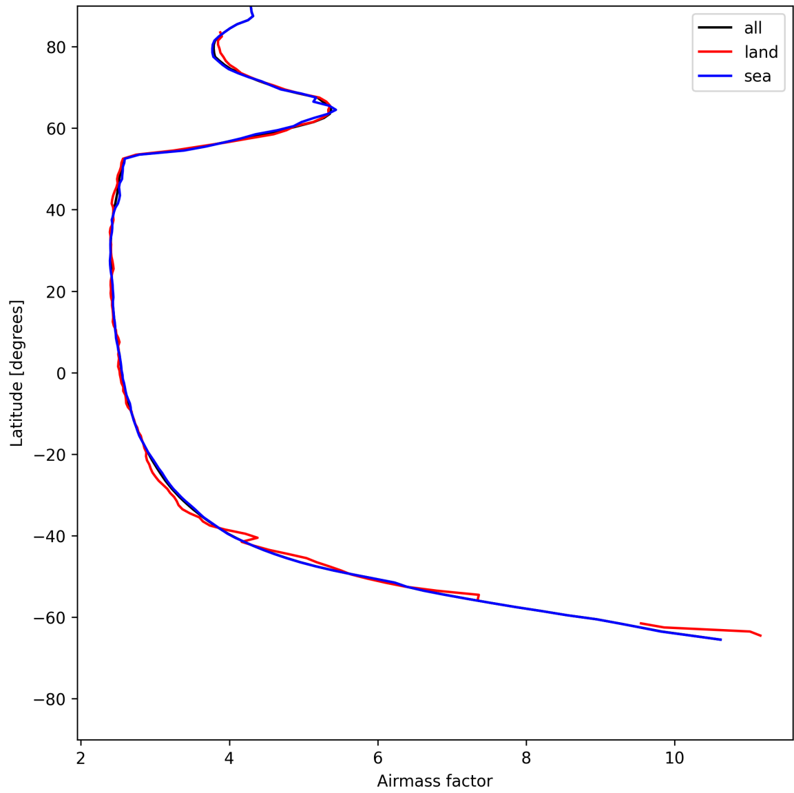
Figure 25: Zonal average of “Airmass factor” for 2025-06-10 to 2025-06-11.
