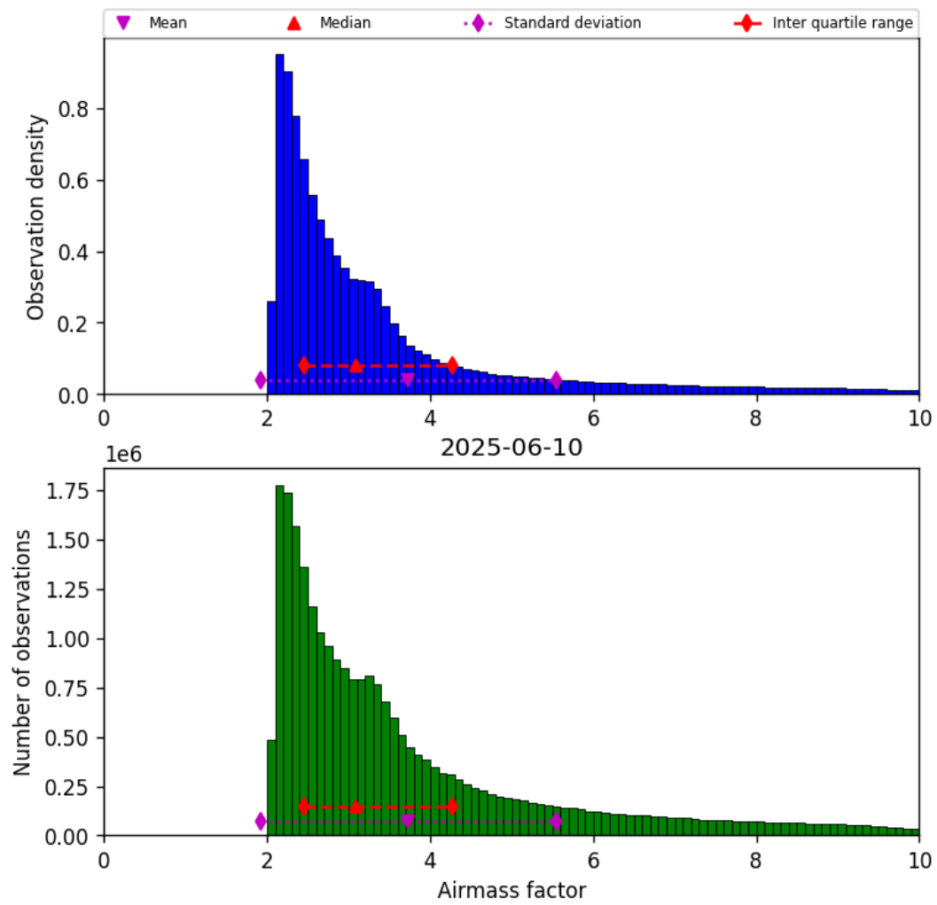
Figure 37: Histogram of “Airmass factor” for 2025-06-10 to 2025-06-11
