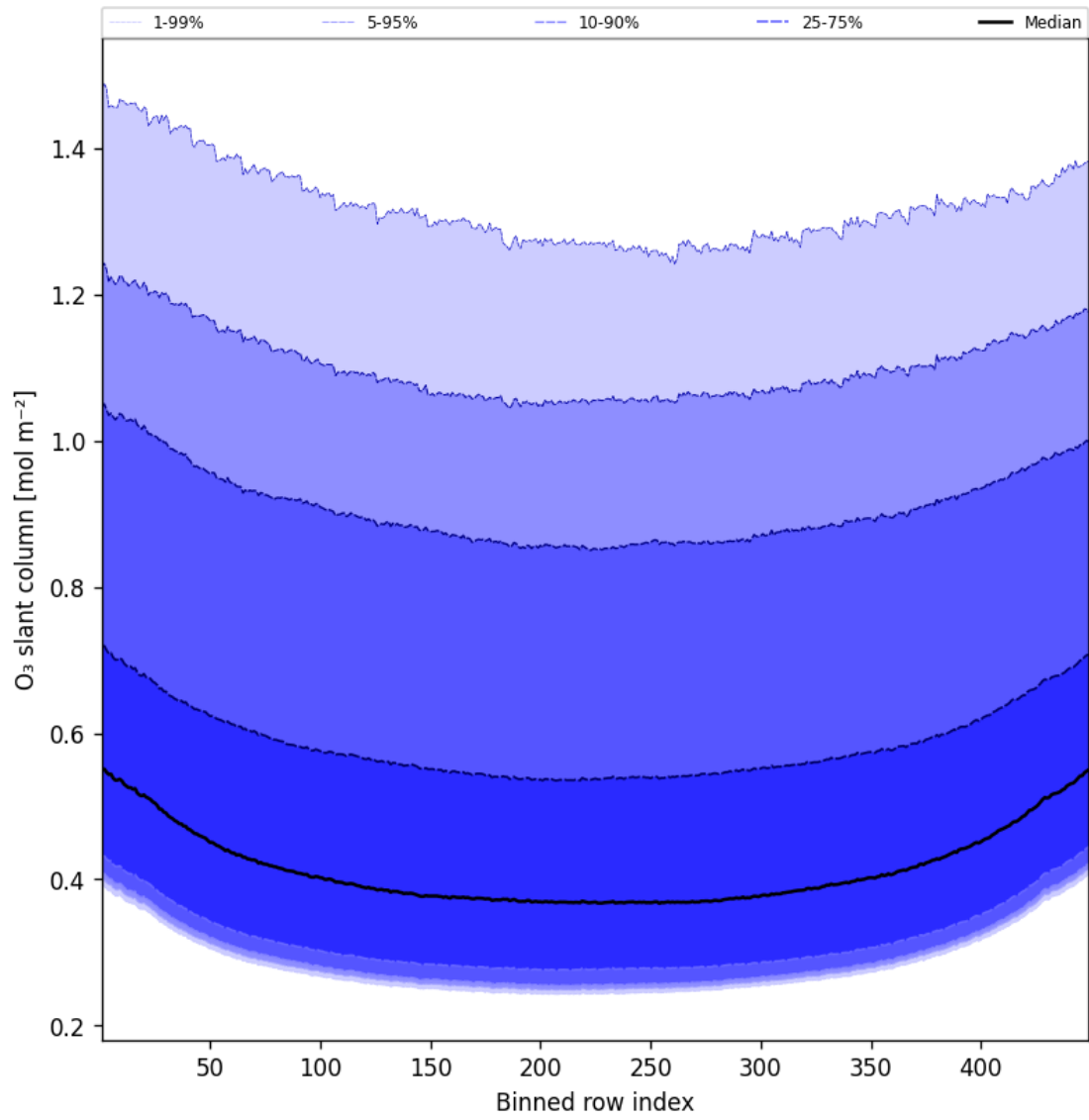
Figure 43: Along track statistics of “O 3 slant column” for 2025-06-10 to 2025-06-11
