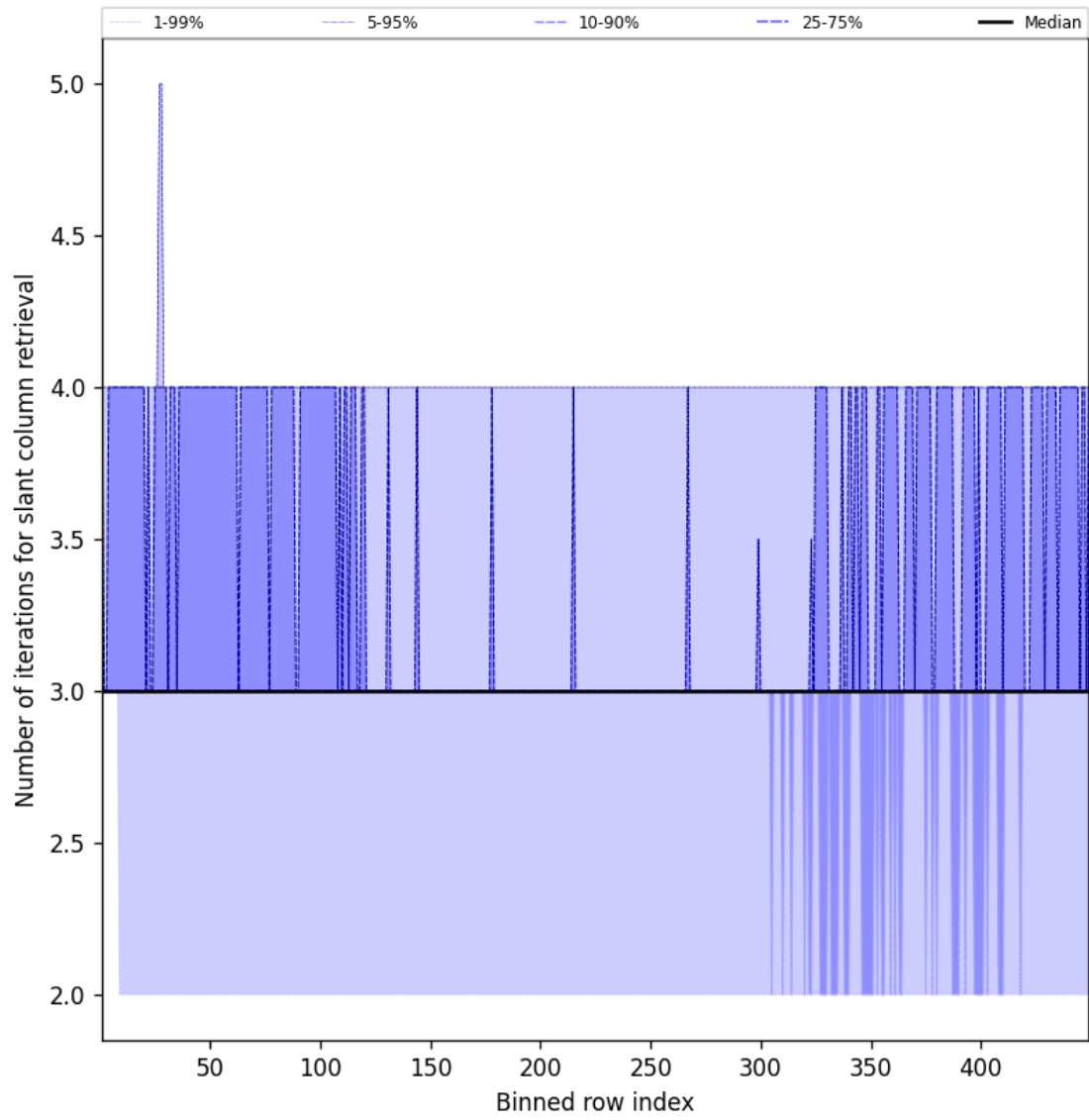
Figure 45: Along track statistics of “Number of iterations for slant column retrieval” for 2025-06-10 to 2025-06-11
