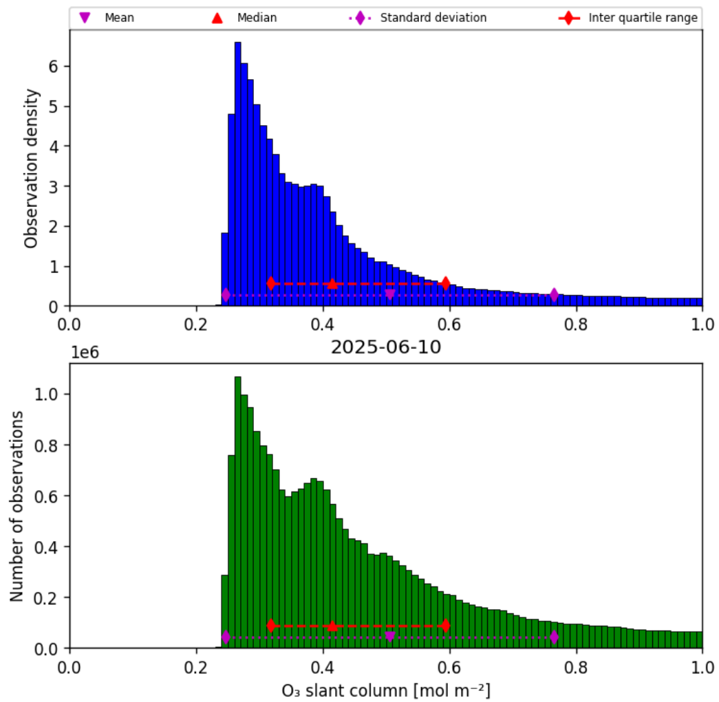
Figure 31: Histogram of “O 3 slant column” for 2025-06-10 to 2025-06-11
