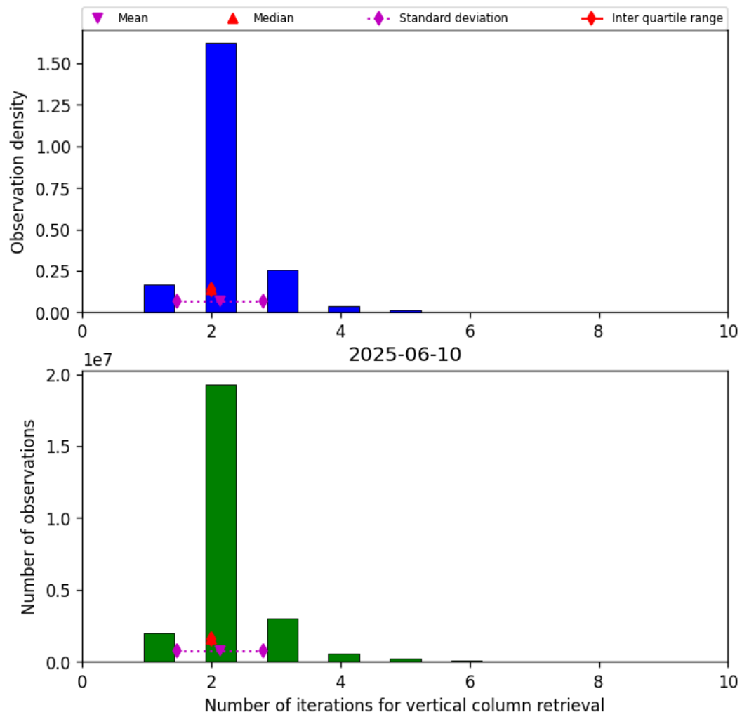
Figure 39: Histogram of “Number of iterations for vertical column retrieval” for 2025-06-10 to 2025-06-11
