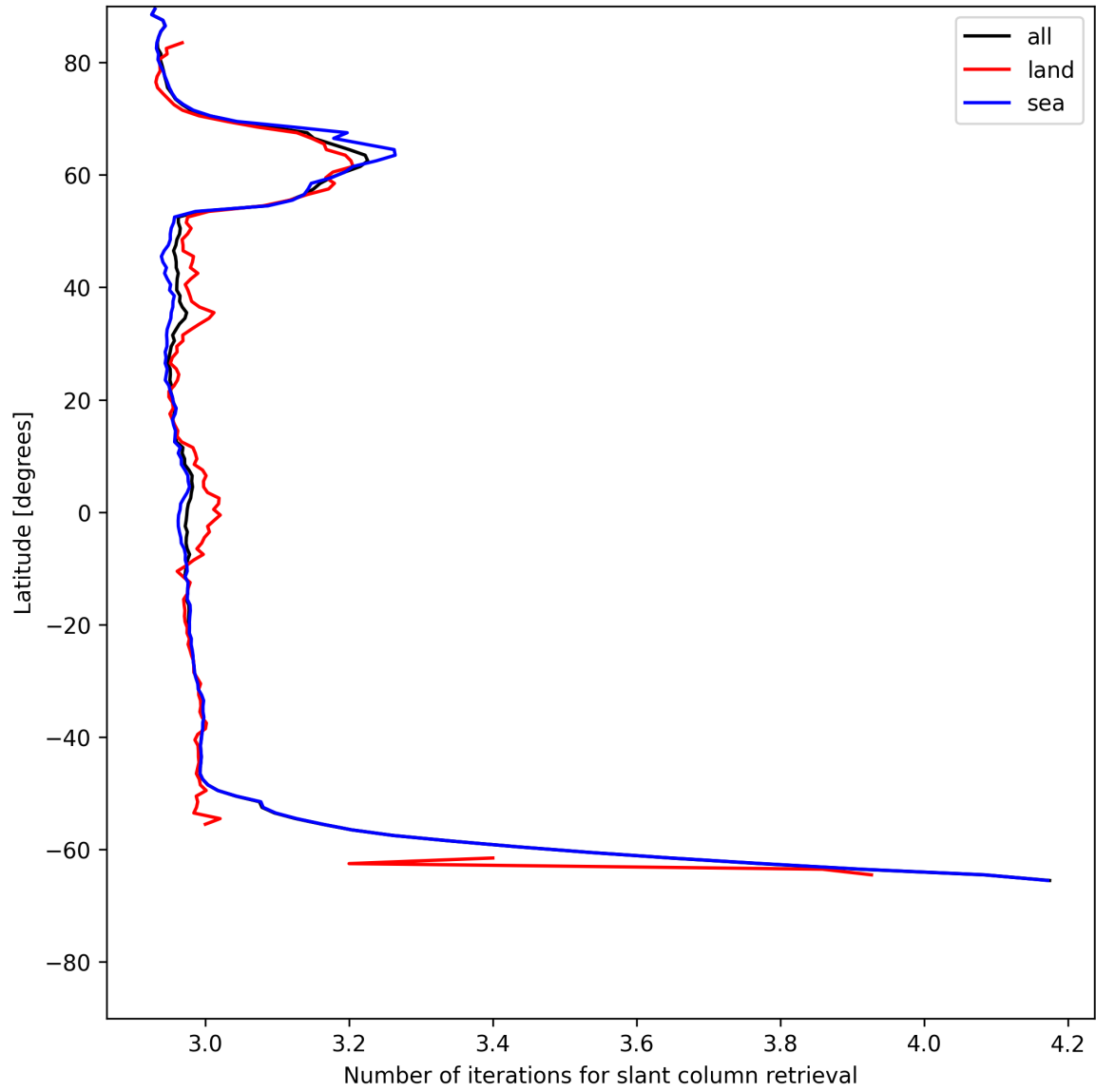
Figure 21: Zonal average of “Number of iterations for slant column retrieval” for 2025-06-10 to 2025-06-11.
