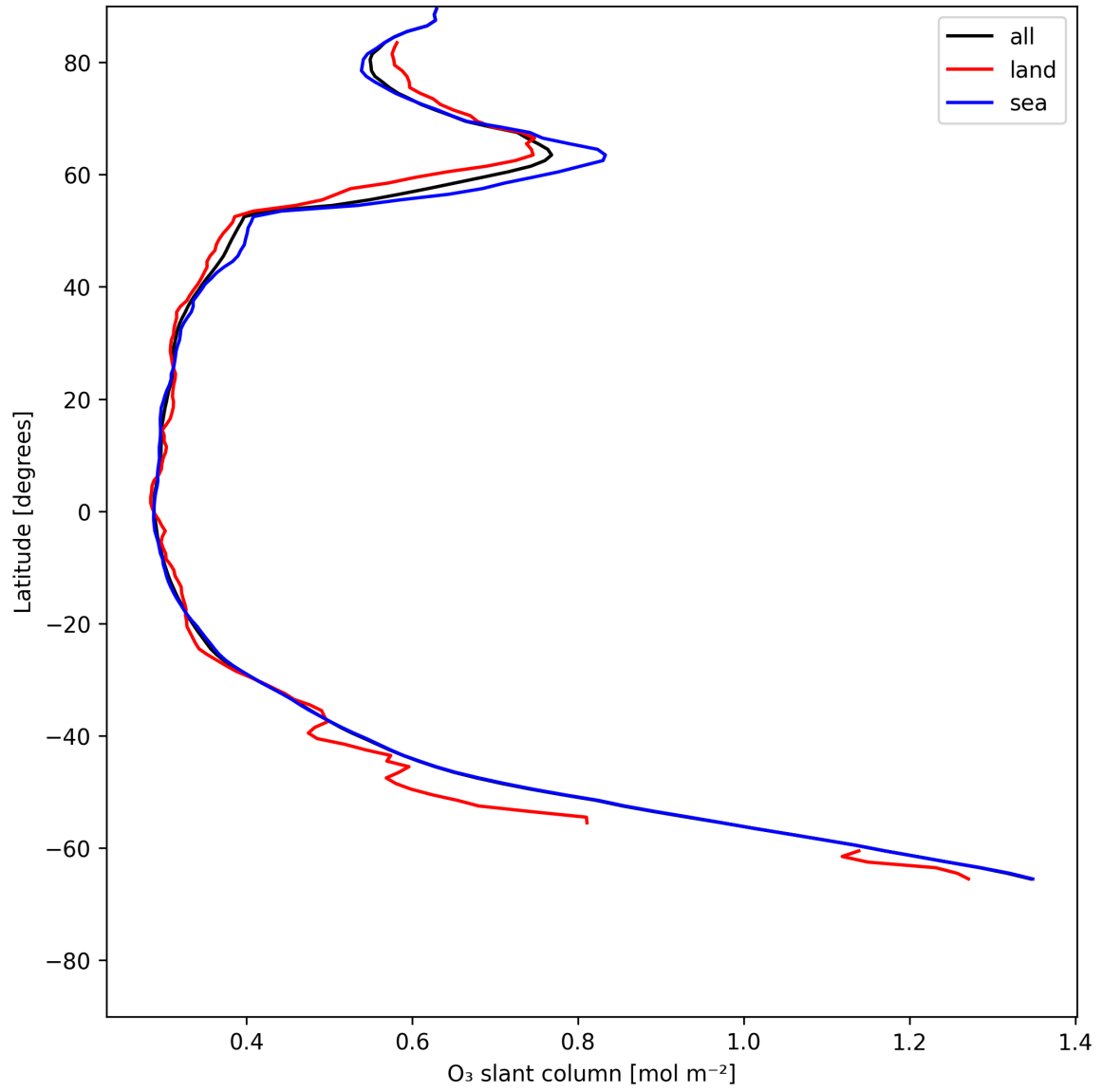
Figure 19: Zonal average of “O 3 slant column” for 2025-06-11 to 2025-06-12.
