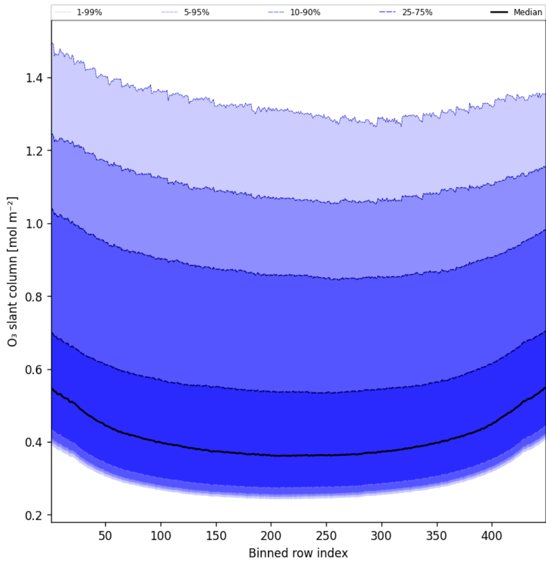
Figure 43: Along track statistics of “O 3 slant column” for 2025-06-11 to 2025-06-12
