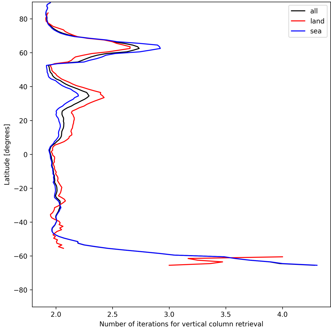
Figure 27: Zonal average of “Number of iterations for vertical column retrieval” for 2025-06-11 to 2025-06-12.
