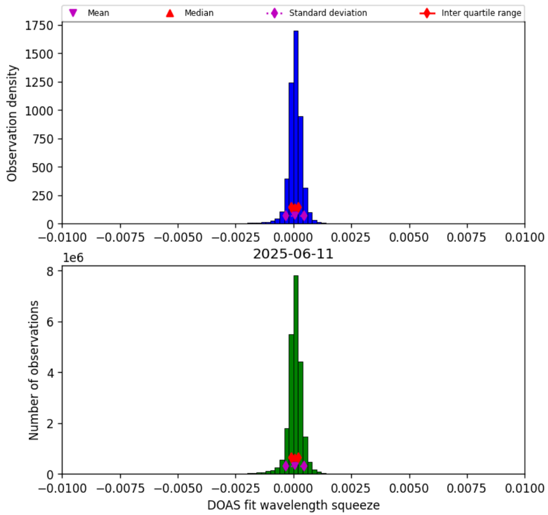
Figure 36: Histogram of “DOAS fit wavelength squeeze” for 2025-06-11 to 2025-06-12
