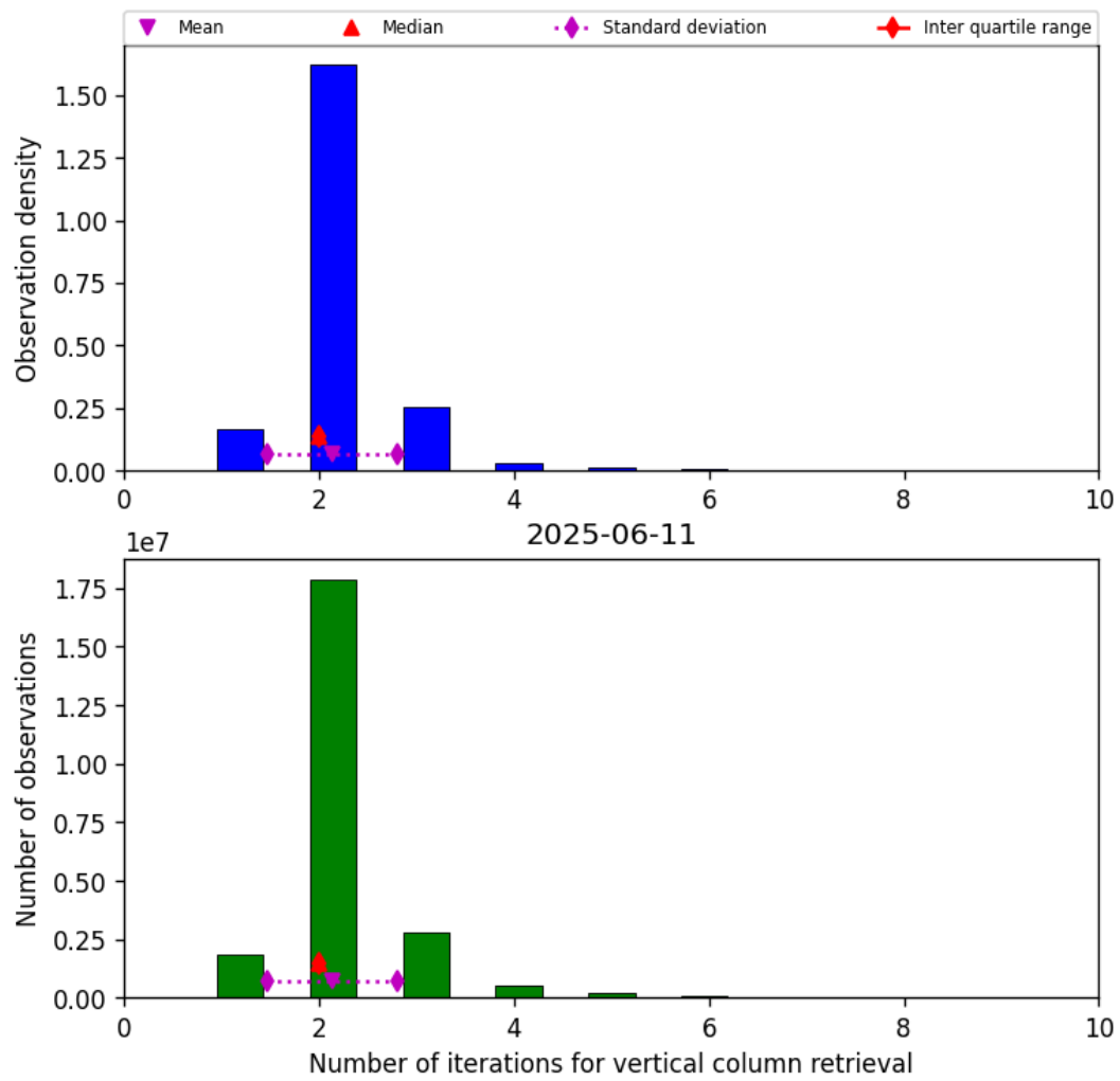
Figure 39: Histogram of “Number of iterations for vertical column retrieval” for 2025-06-11 to 2025-06-12
