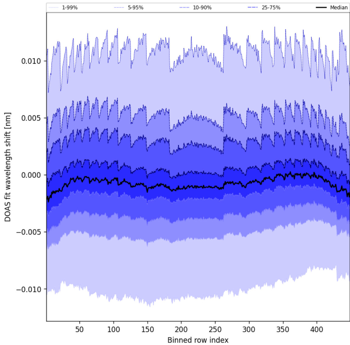
Figure 47: Along track statistics of “DOAS fit wavelength shift” for 2025-06-11 to 2025-06-12
