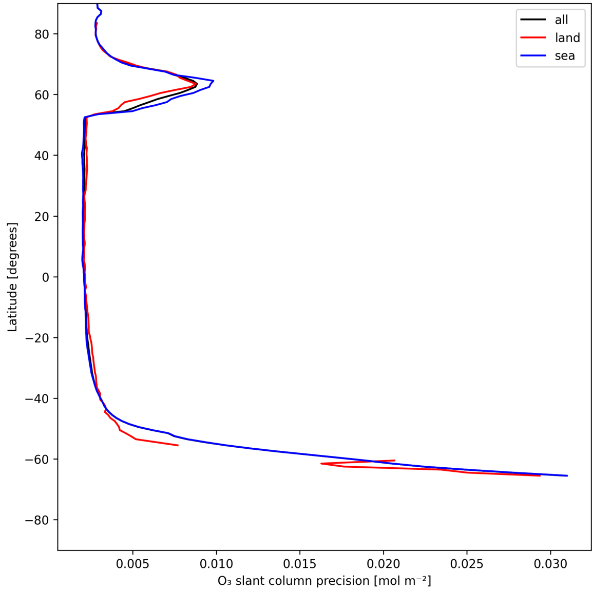
Figure 20: Zonal average of “O 3 slant column precision” for 2025-06-11 to 2025-06-12.
