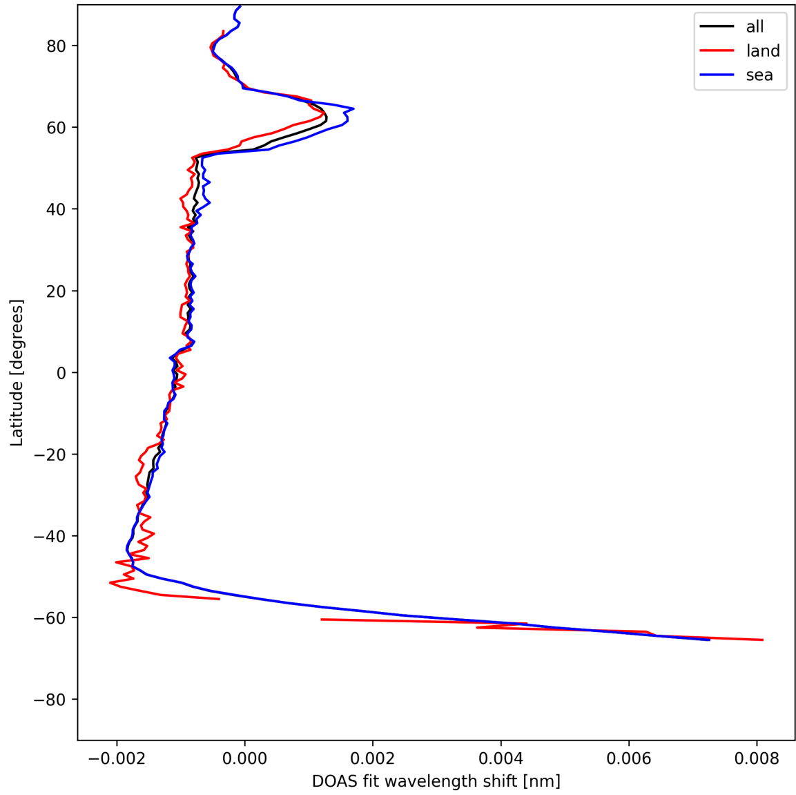
Figure 23: Zonal average of “DOAS fit wavelength shift” for 2025-06-11 to 2025-06-12.
