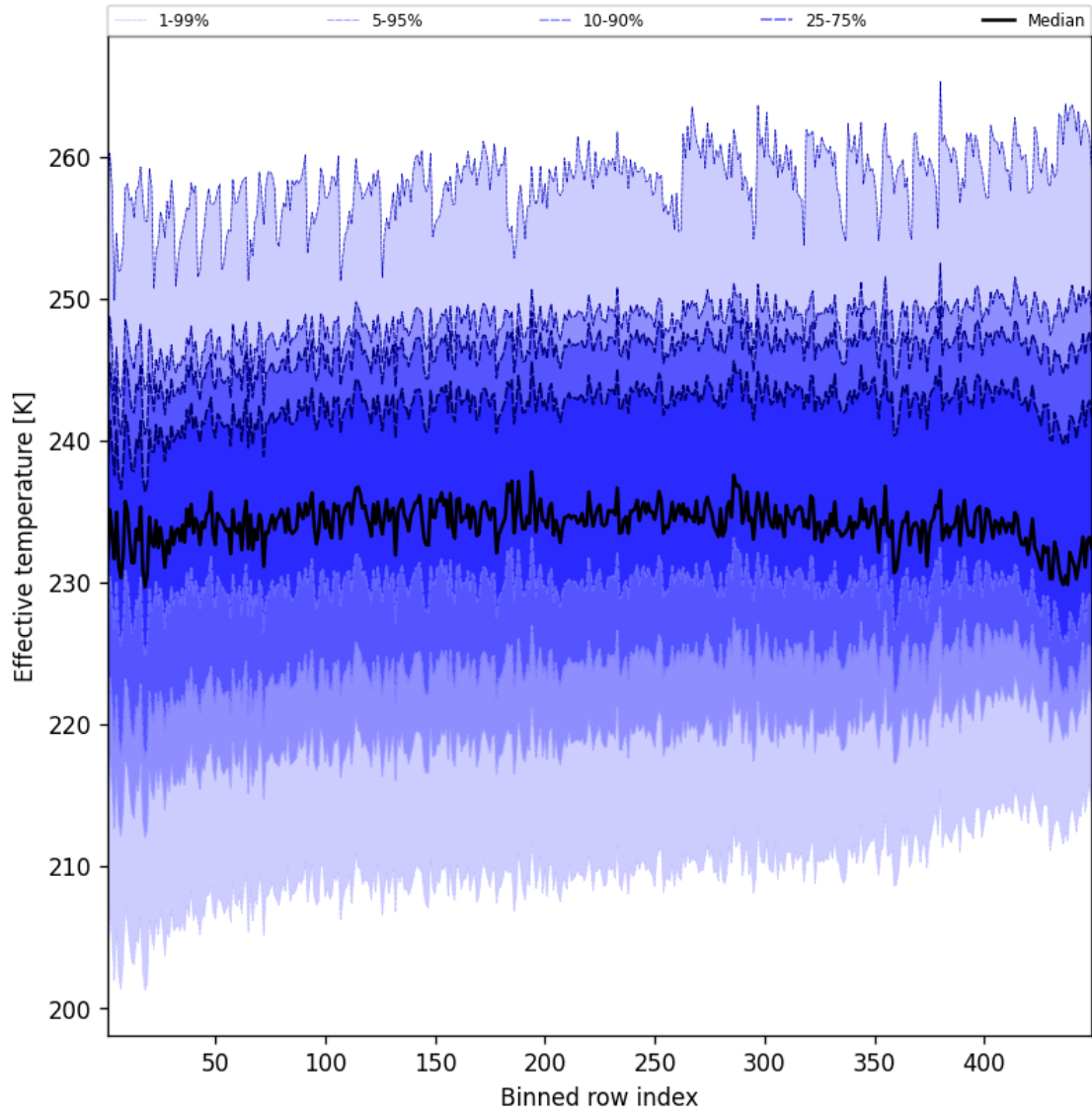
Figure 50: Along track statistics of “Effective temperature” for 2025-06-11 to 2025-06-12
