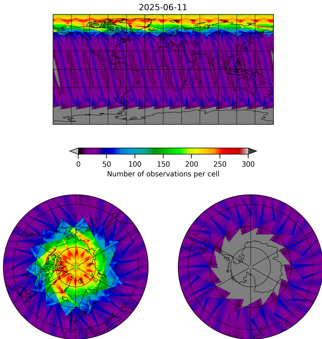
Figure 15: Map of the number of observations for 2025-06-11 to 2025-06-12
