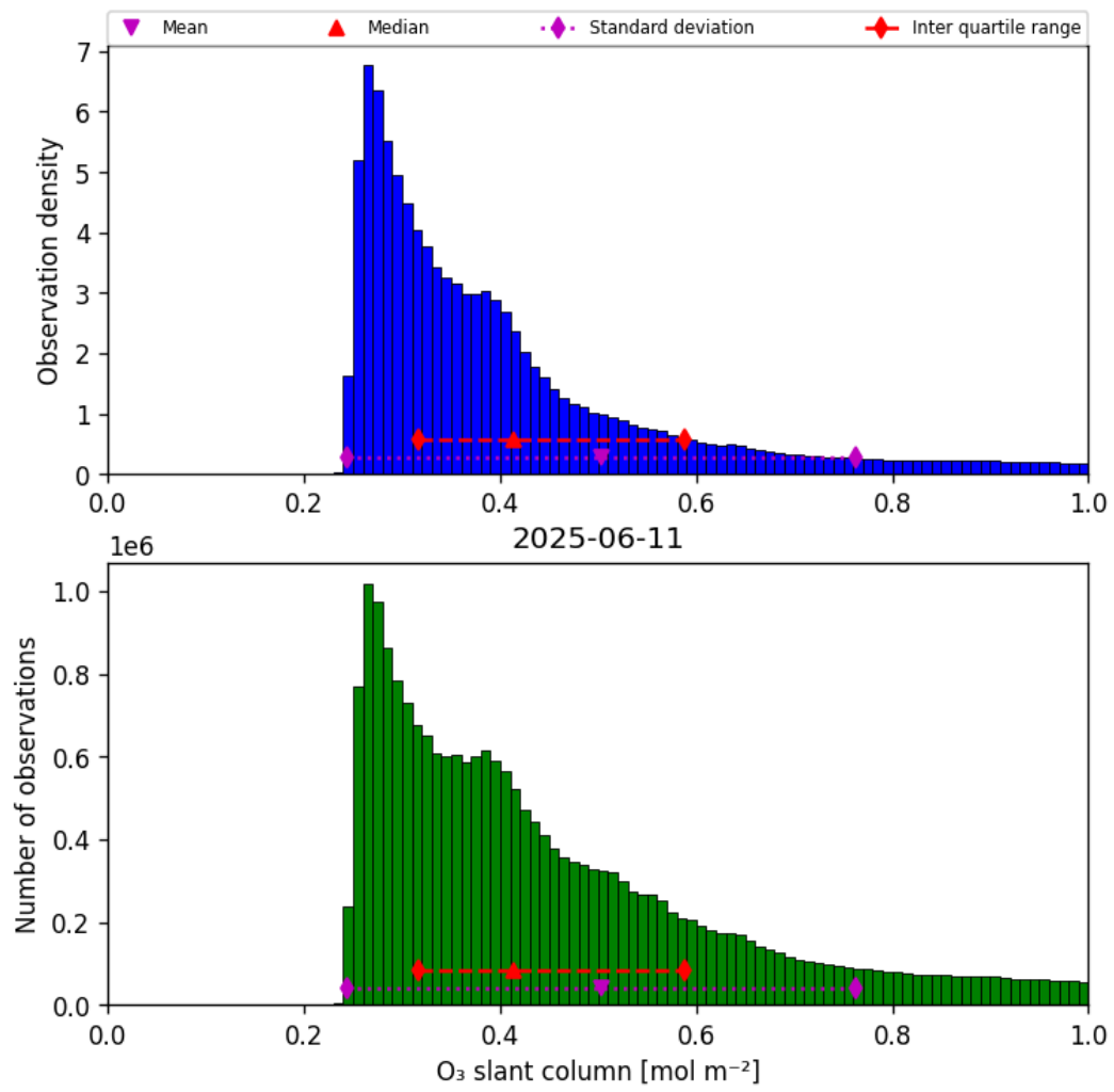
Figure 31: Histogram of “O 3 slant column” for 2025-06-11 to 2025-06-12
