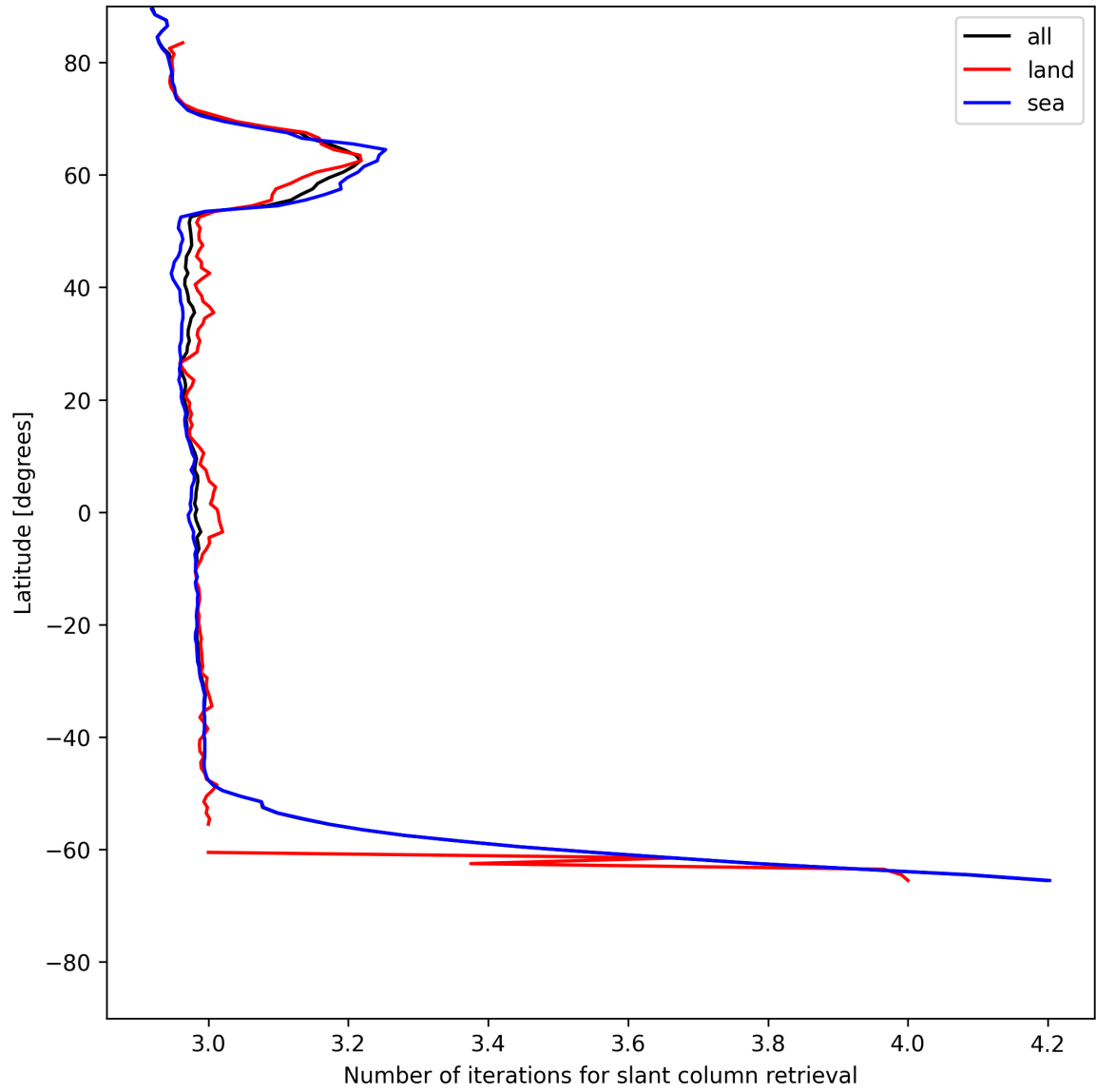
Figure 21: Zonal average of “Number of iterations for slant column retrieval” for 2025-06-11 to 2025-06-12.
