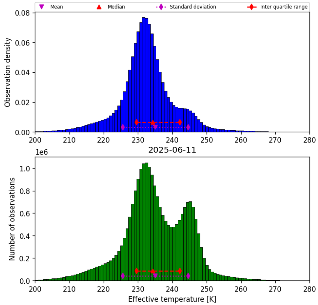
Figure 38: Histogram of “Effective temperature” for 2025-06-11 to 2025-06-12
