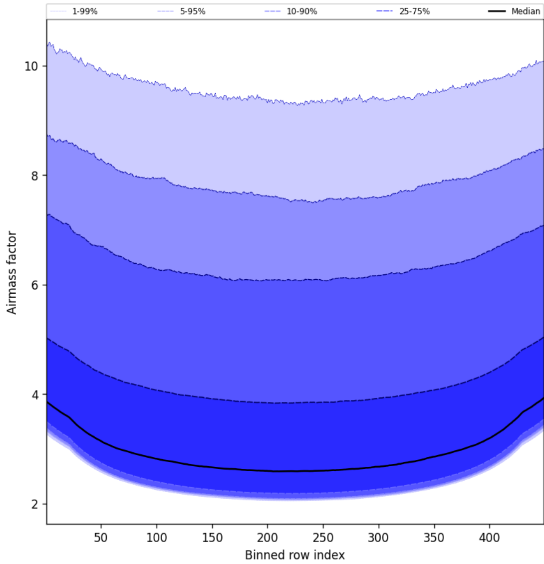
Figure 49: Along track statistics of “Airmass factor” for 2025-06-11 to 2025-06-12
