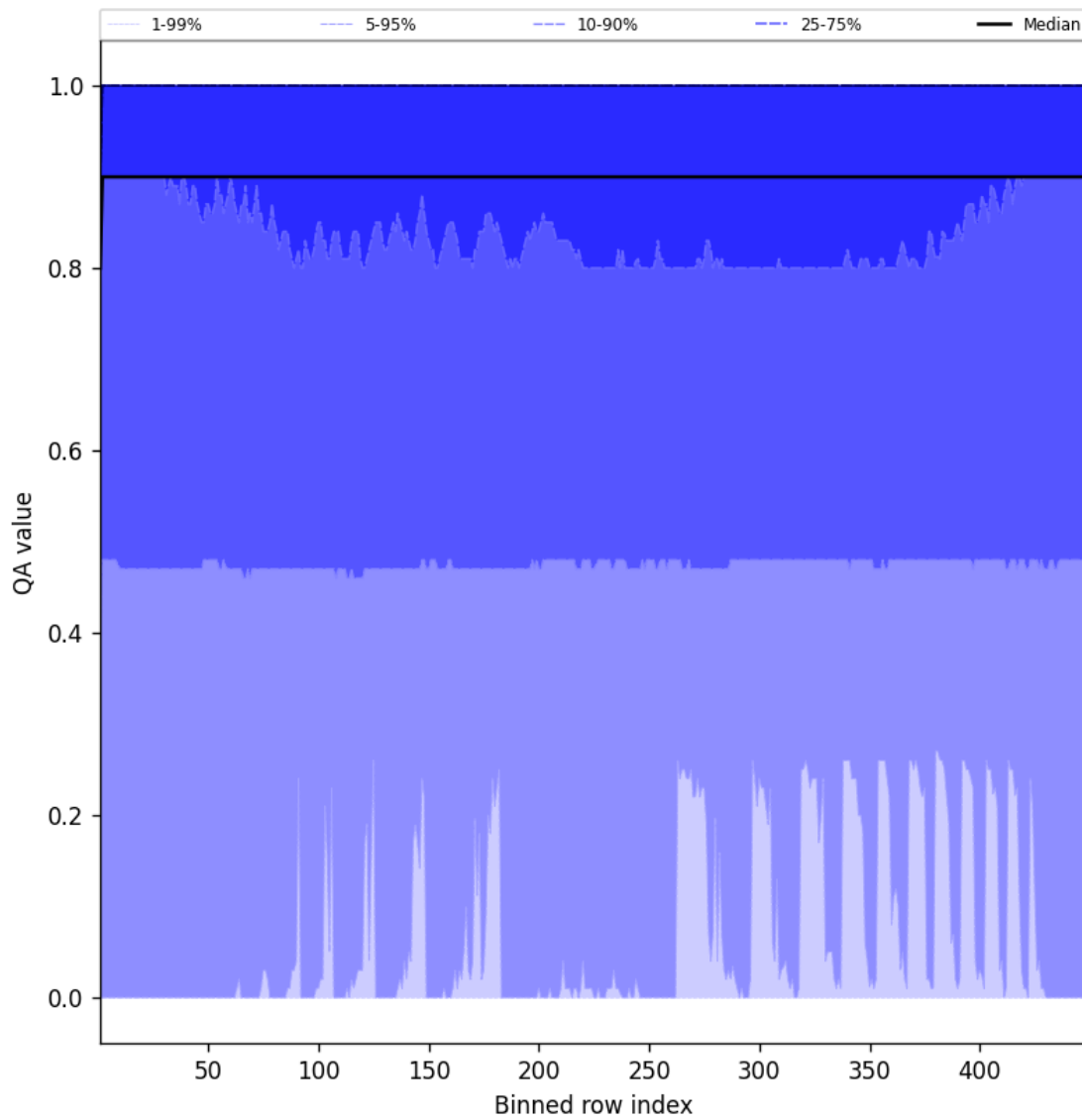
Figure 40: Along track statistics of “QA value” for 2025-06-11 to 2025-06-12
