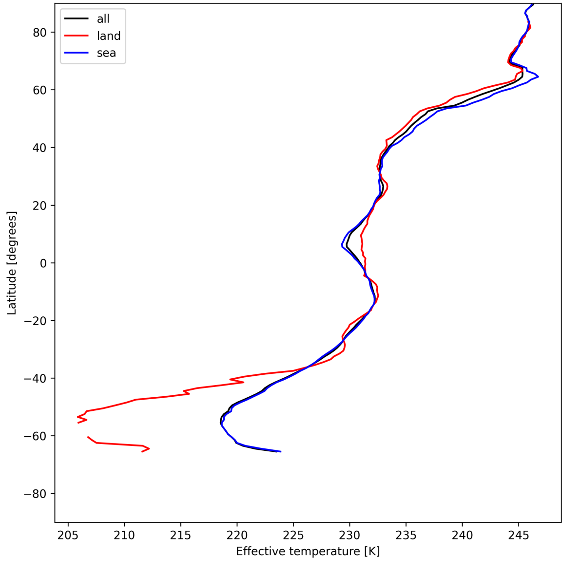
Figure 26: Zonal average of “Effective temperature” for 2025-06-11 to 2025-06-12.
