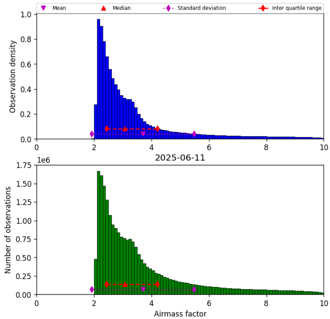
Figure 37: Histogram of “Airmass factor” for 2025-06-11 to 2025-06-12
