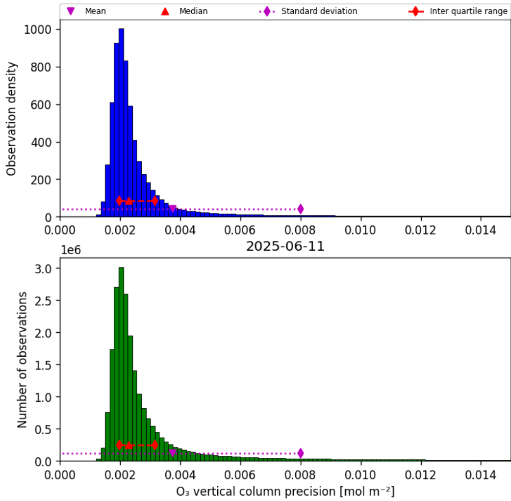
Figure 30: Histogram of “O 3 vertical column precision” for 2025-06-11 to 2025-06-12
