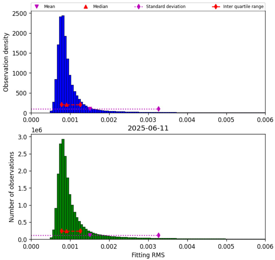
Figure 34: Histogram of “Fitting RMS” for 2025-06-11 to 2025-06-12
