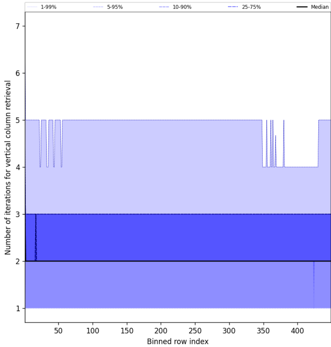
Figure 51: Along track statistics of “Number of iterations for vertical column retrieval” for 2025-06-11 to 2025-06-12
