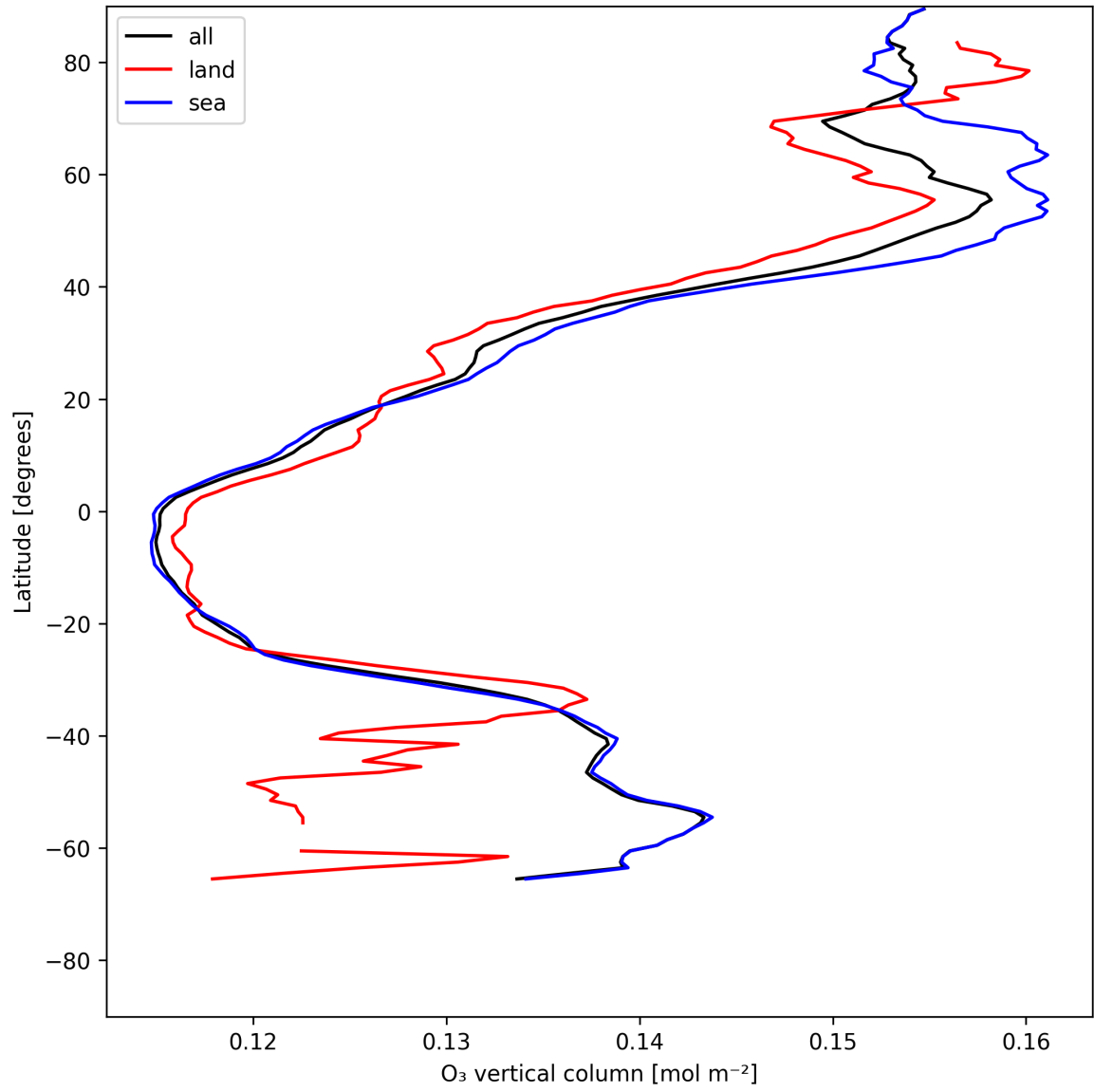
Figure 17: Zonal average of “O 3 vertical column” for 2025-06-11 to 2025-06-12.
