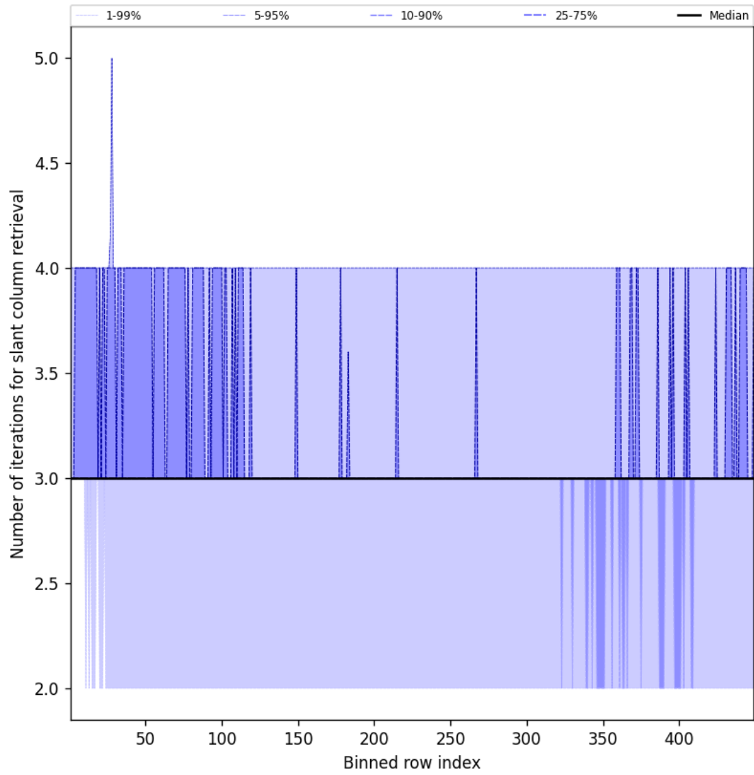
Figure 45: Along track statistics of “Number of iterations for slant column retrieval” for 2025-06-11 to 2025-06-12
