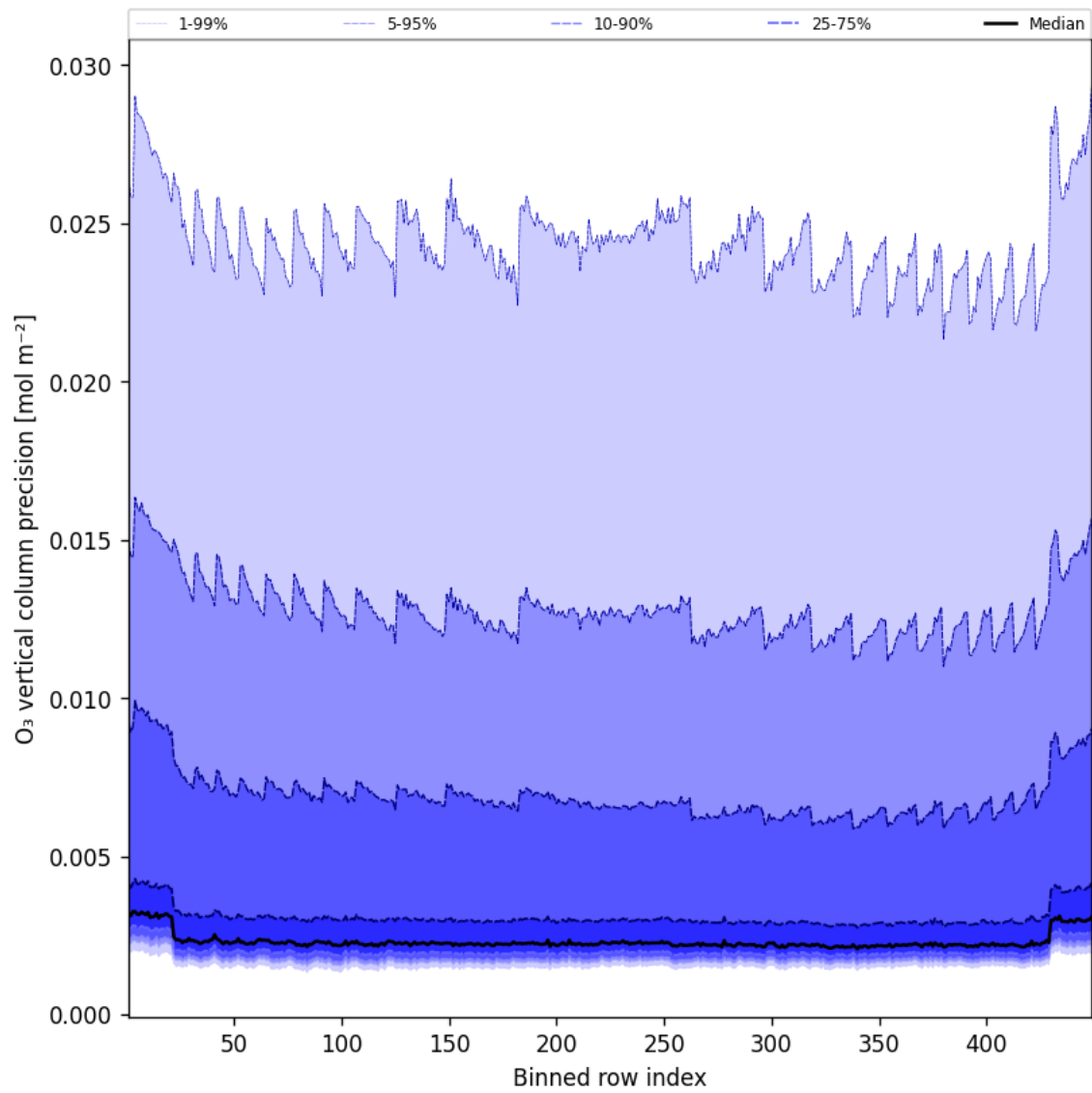
Figure 42: Along track statistics of “O 3 vertical column precision” for 2025-06-11 to 2025-06-12
