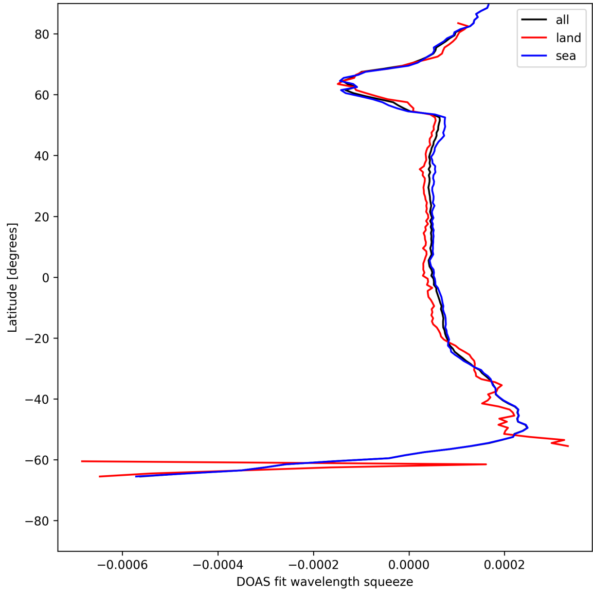
Figure 24: Zonal average of “DOAS fit wavelength squeeze” for 2025-06-11 to 2025-06-12.
