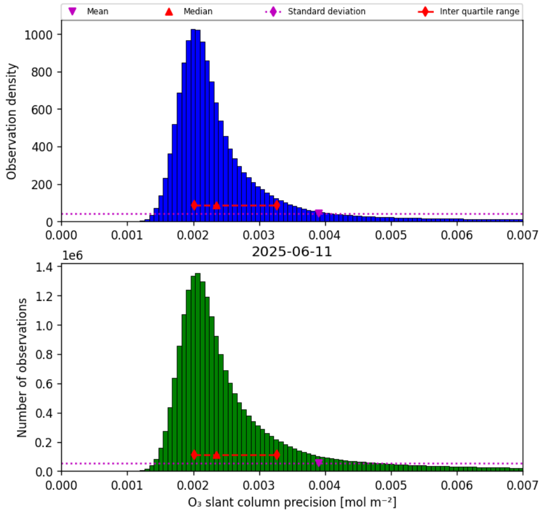
Figure 32: Histogram of “O 3 slant column precision” for 2025-06-11 to 2025-06-12
