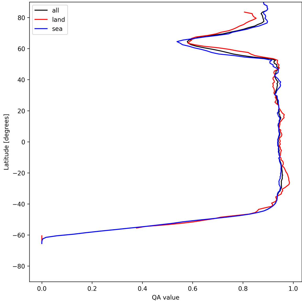
Figure 16: Zonal average of “QA value” for 2025-06-11 to 2025-06-12.
