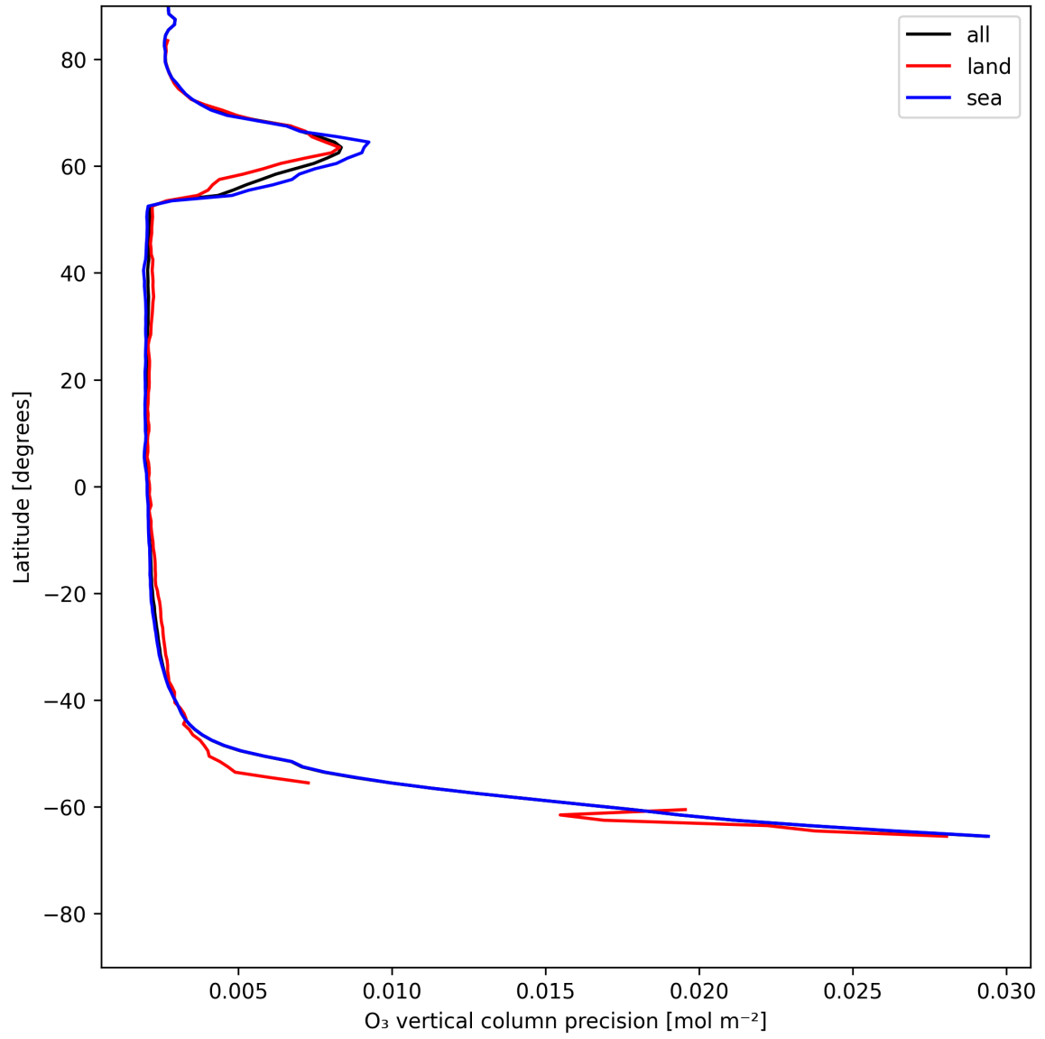
Figure 18: Zonal average of “O 3 vertical column precision” for 2025-06-11 to 2025-06-12.
