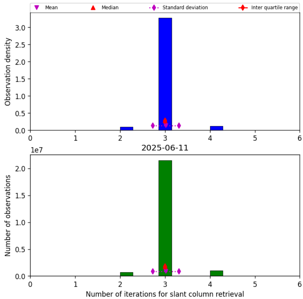
Figure 33: Histogram of “Number of iterations for slant column retrieval” for 2025-06-11 to 2025-06-12
