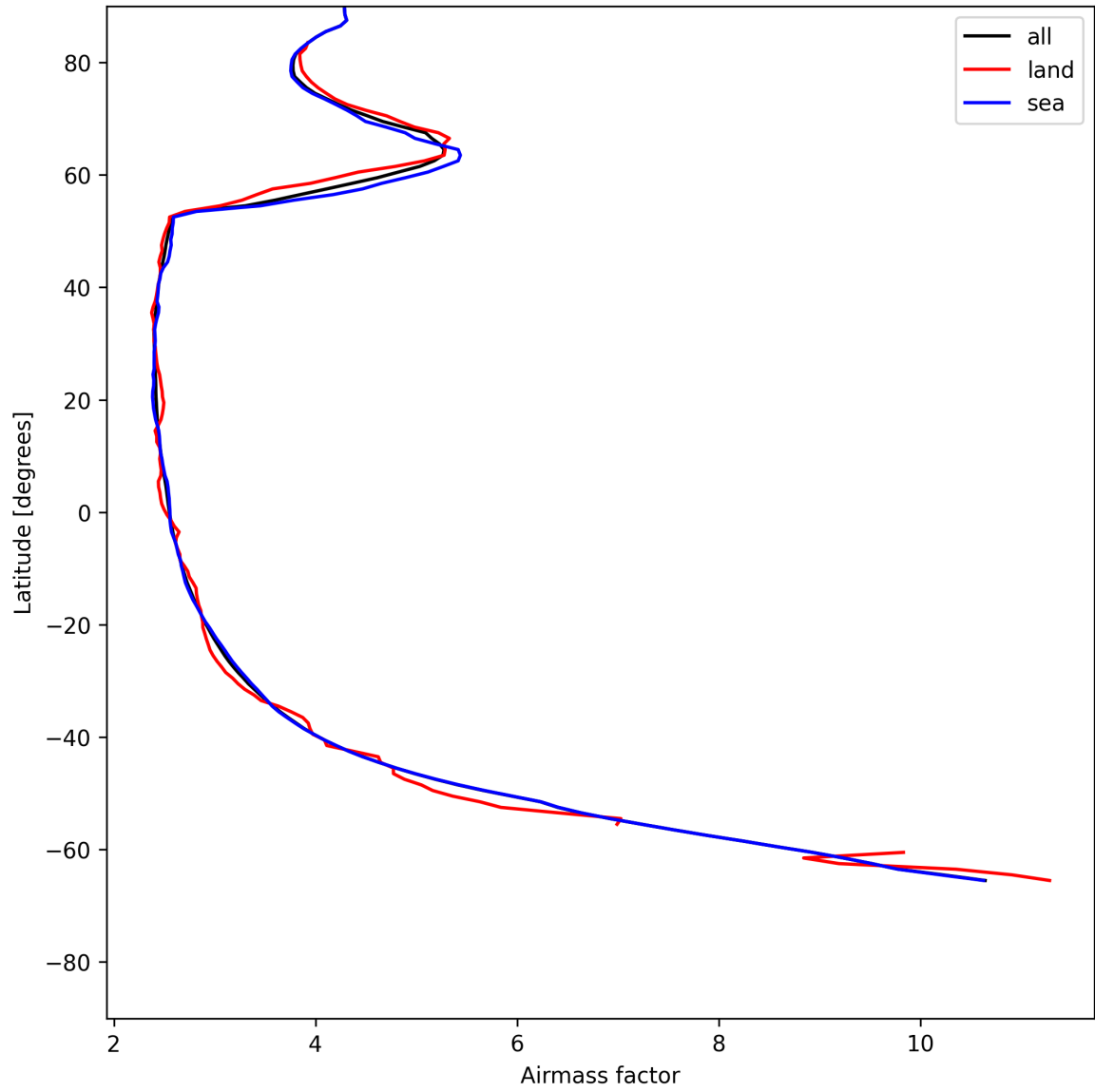
Figure 25: Zonal average of “Airmass factor” for 2025-06-11 to 2025-06-12.
