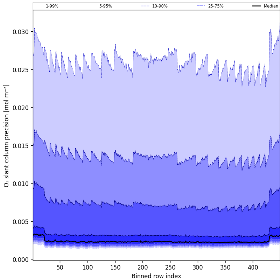
Figure 44: Along track statistics of “O 3 slant column precision” for 2025-06-11 to 2025-06-12
