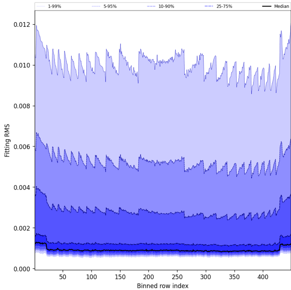
Figure 46: Along track statistics of “Fitting RMS” for 2025-06-11 to 2025-06-12
