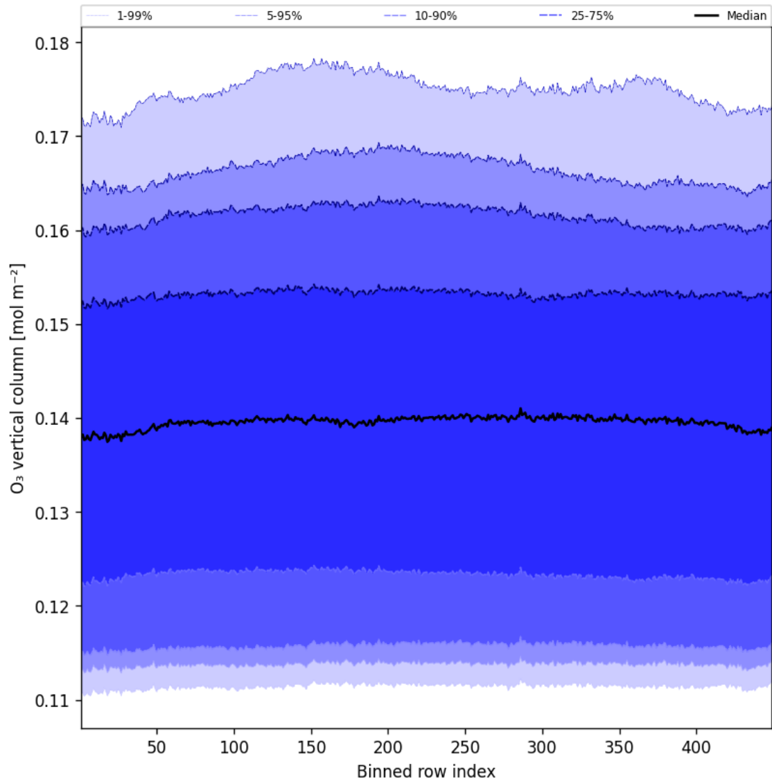
Figure 41: Along track statistics of “O 3 vertical column” for 2025-06-11 to 2025-06-12
