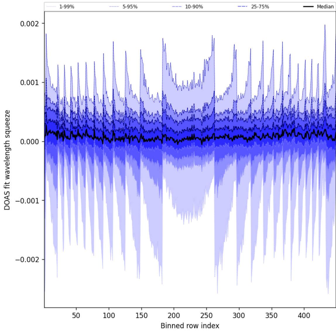
Figure 48: Along track statistics of “DOAS fit wavelength squeeze” for 2025-06-11 to 2025-06-12
