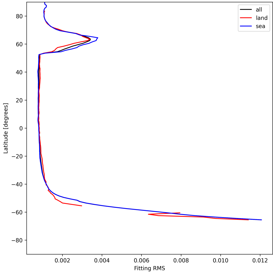
Figure 22: Zonal average of “Fitting RMS” for 2025-06-11 to 2025-06-12.
