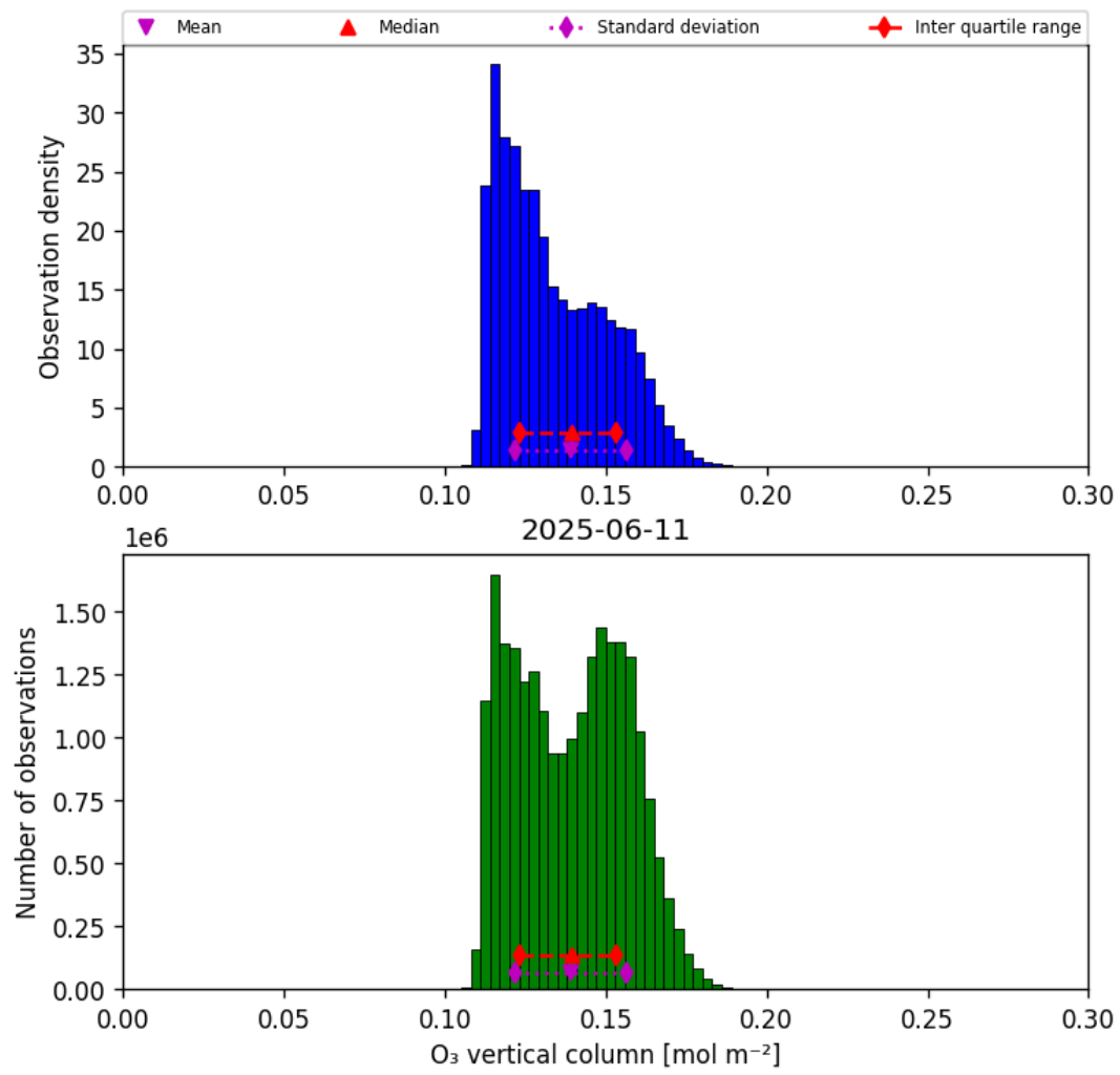
Figure 29: Histogram of “O 3 vertical column” for 2025-06-11 to 2025-06-12
