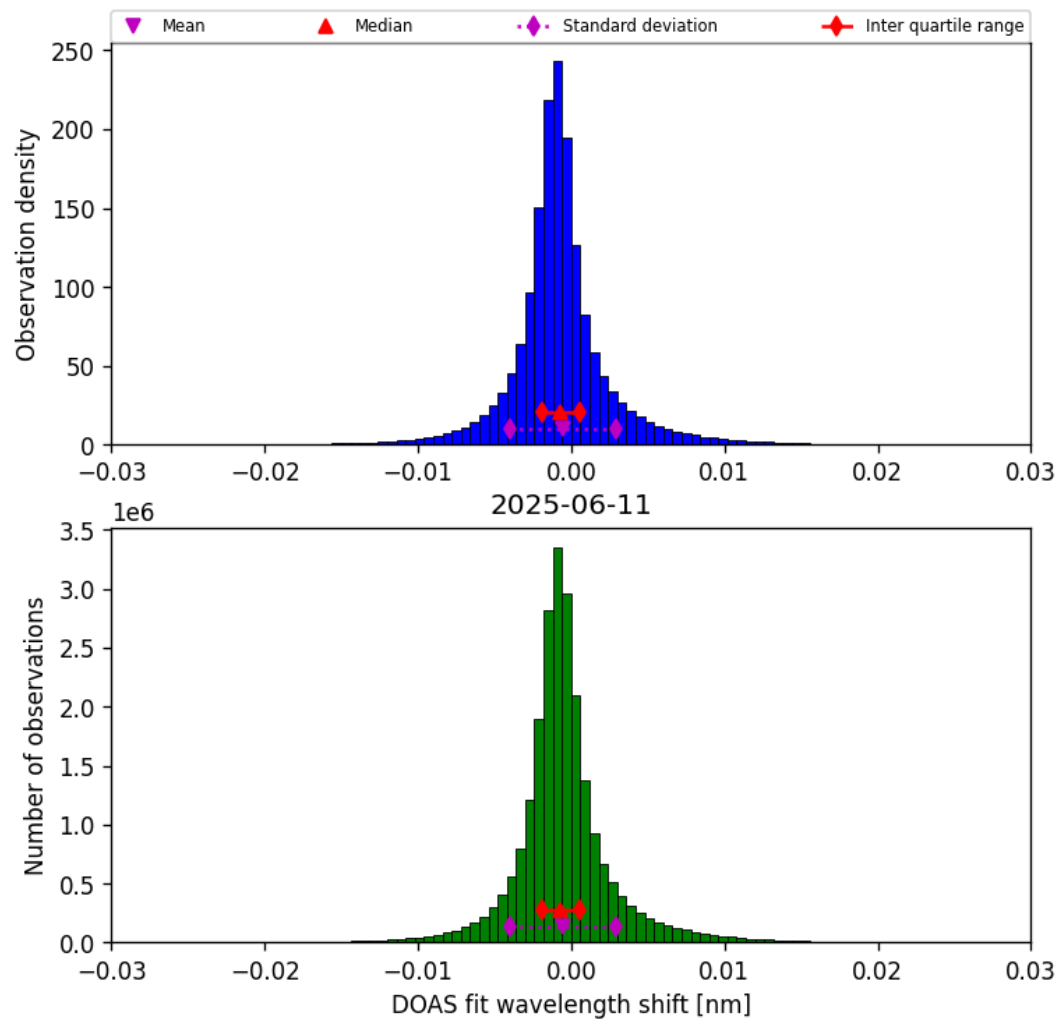
Figure 35: Histogram of “DOAS fit wavelength shift” for 2025-06-11 to 2025-06-12
