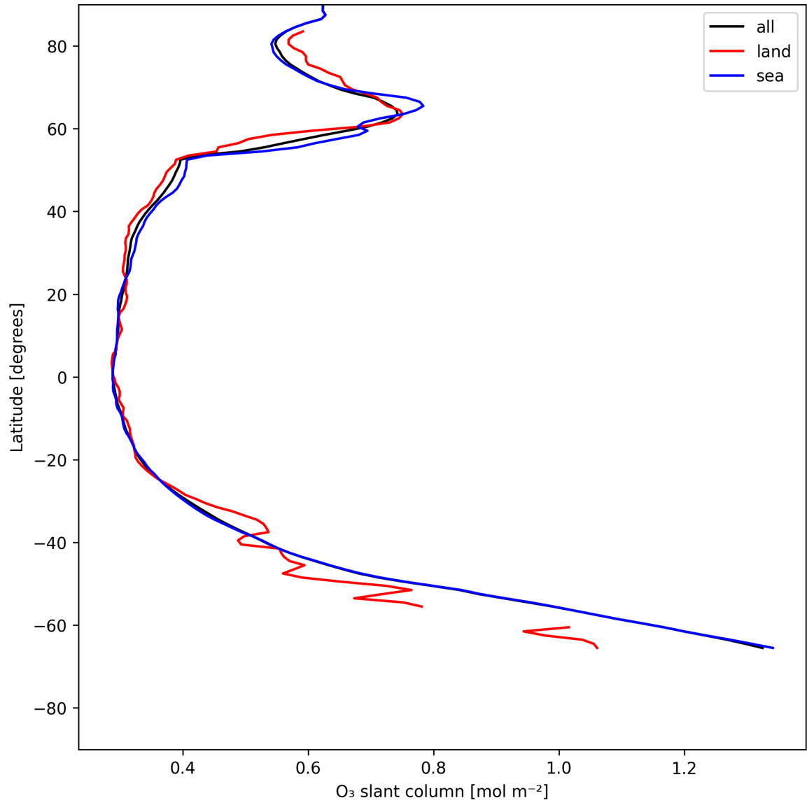
Figure 19: Zonal average of “O 3 slant column” for 2025-06-12 to 2025-06-13.
