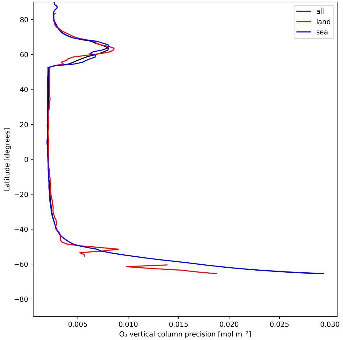
Figure 18: Zonal average of "O 3 vertical column precision" for 2025-06-12 to 2025-06-13.
