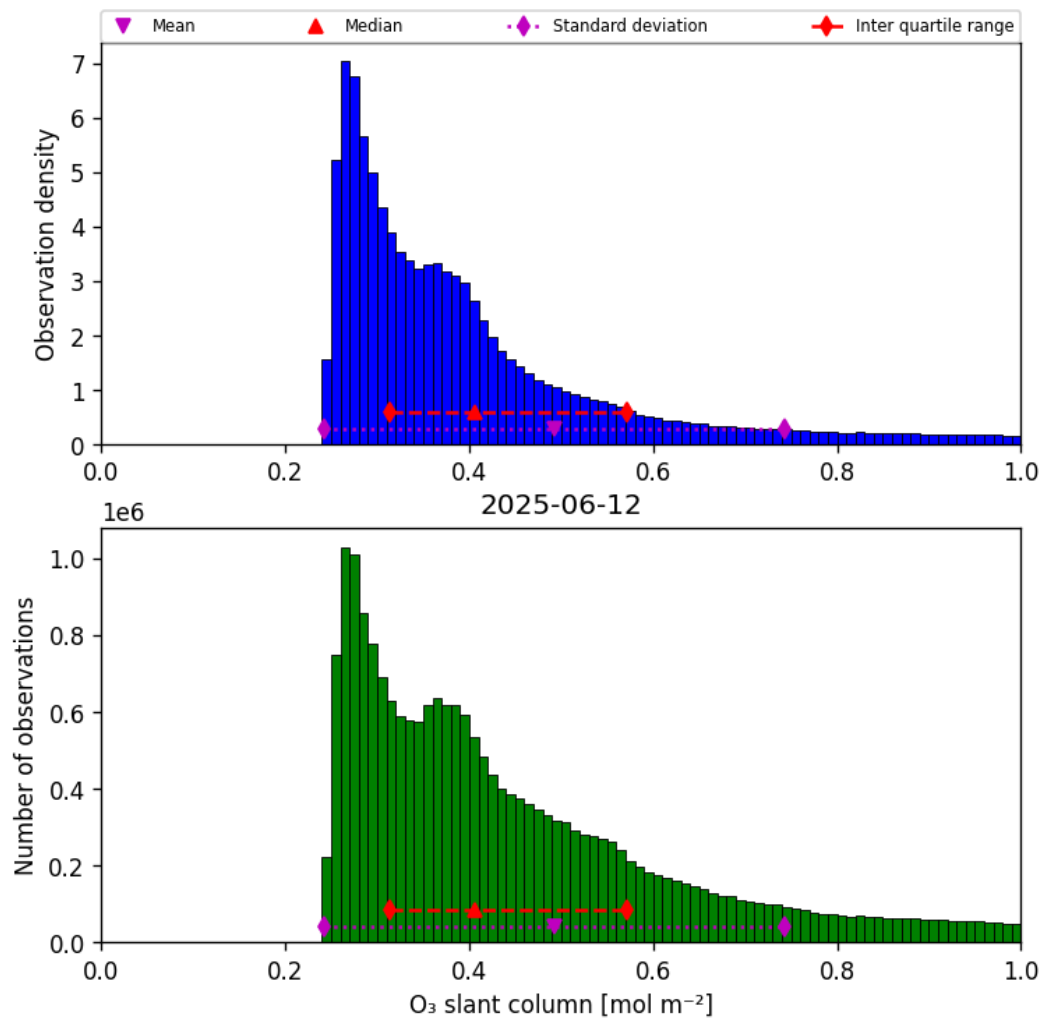
Figure 31: Histogram of “O 3 slant column” for 2025-06-12 to 2025-06-13
