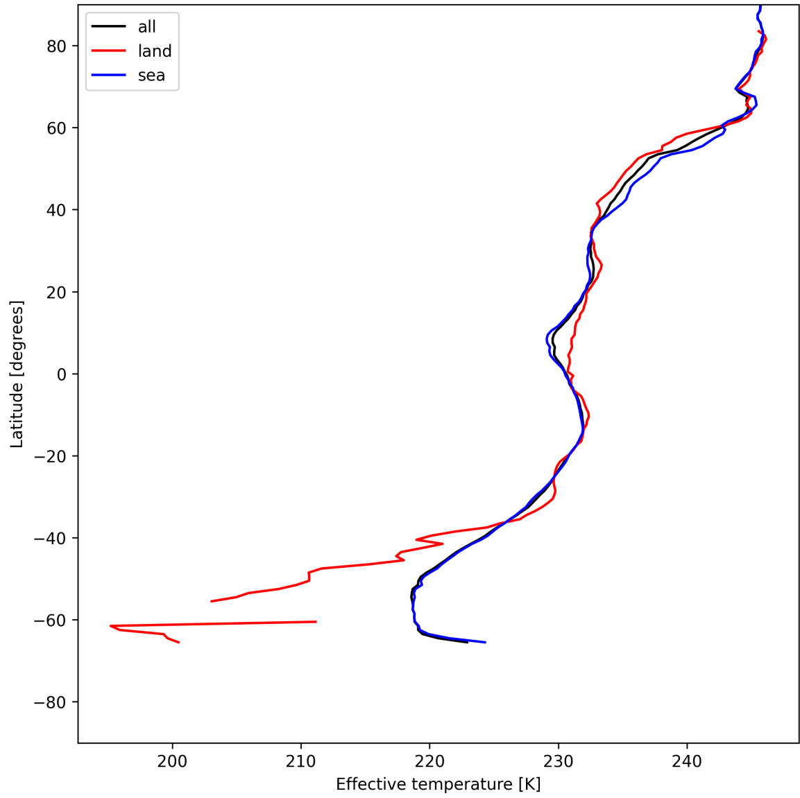
Figure 26: Zonal average of “Effective temperature” for 2025-06-12 to 2025-06-13.
