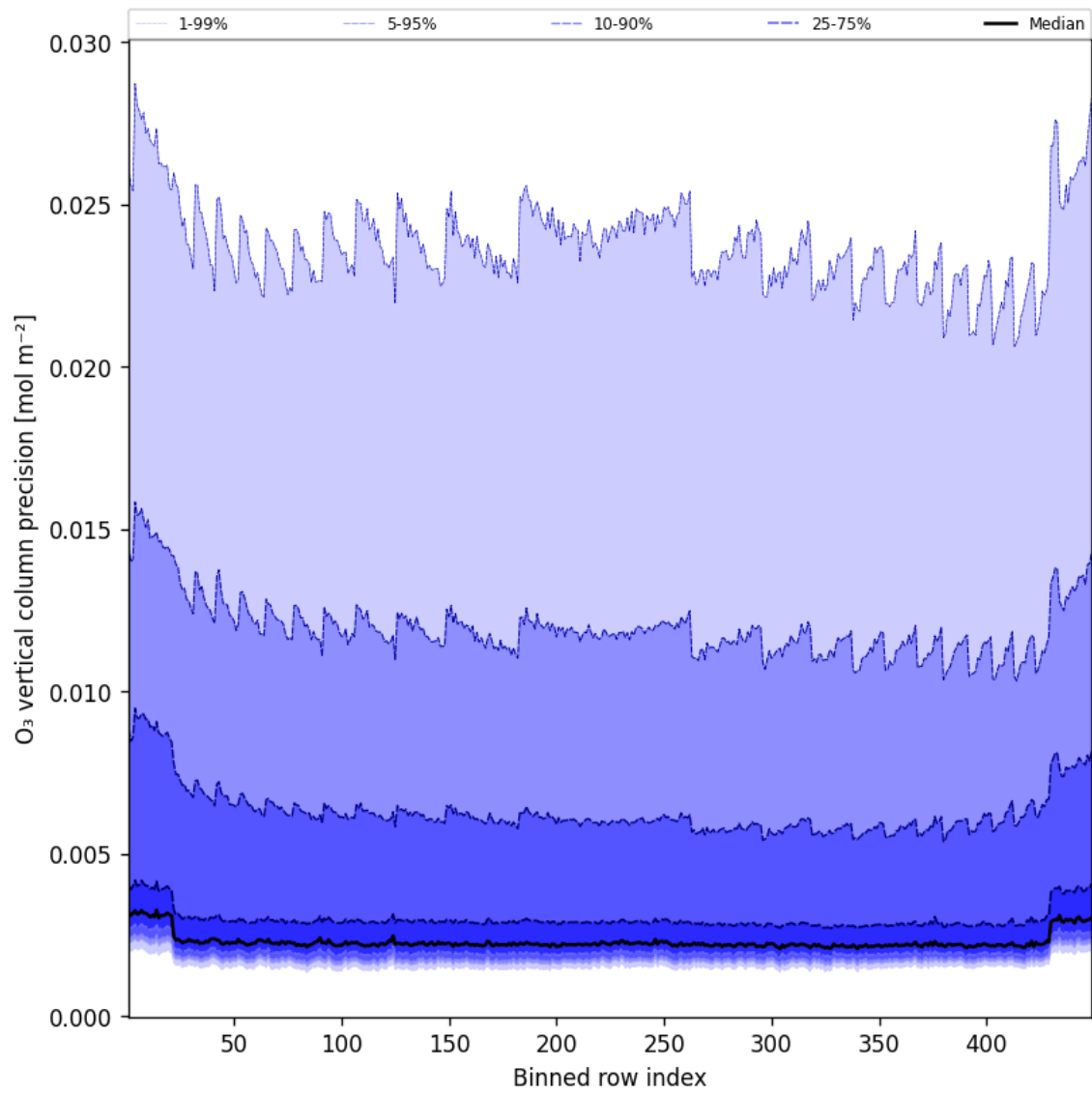
Figure 42: Along track statistics of “O 3 vertical column precision” for 2025-06-12 to 2025-06-13
