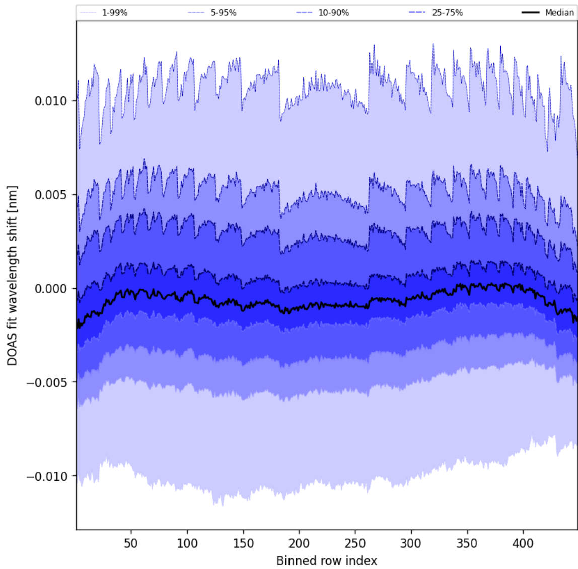
Figure 47: Along track statistics of “DOAS fit wavelength shift” for 2025-06-12 to 2025-06-13
