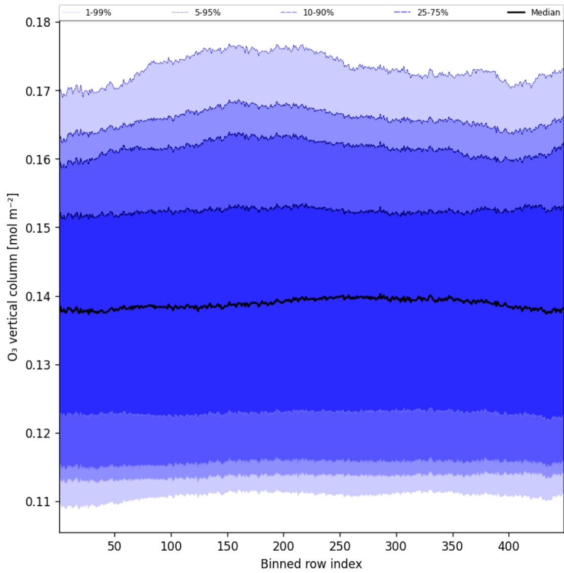
Figure 41: Along track statistics of “O 3 vertical column” for 2025-06-12 to 2025-06-13
