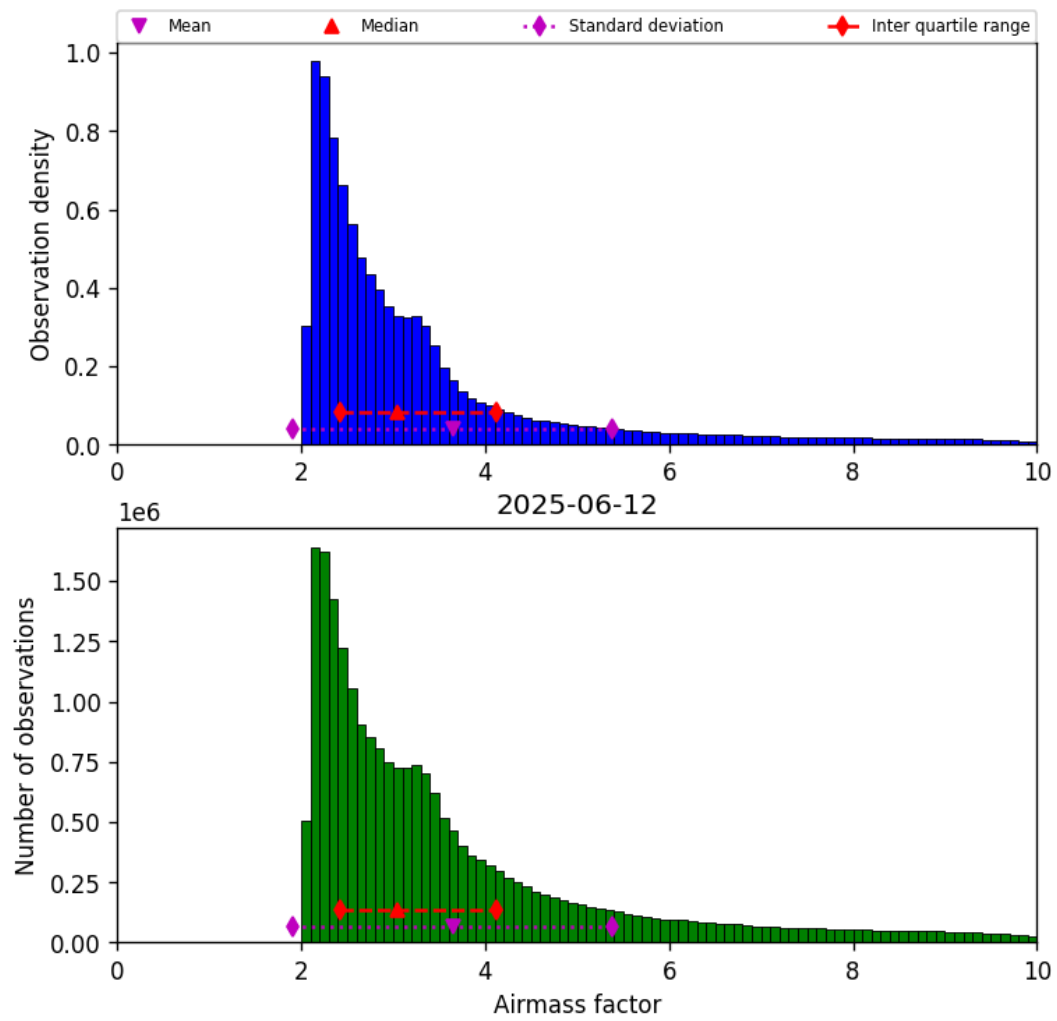
Figure 37: Histogram of “Airmass factor” for 2025-06-12 to 2025-06-13
