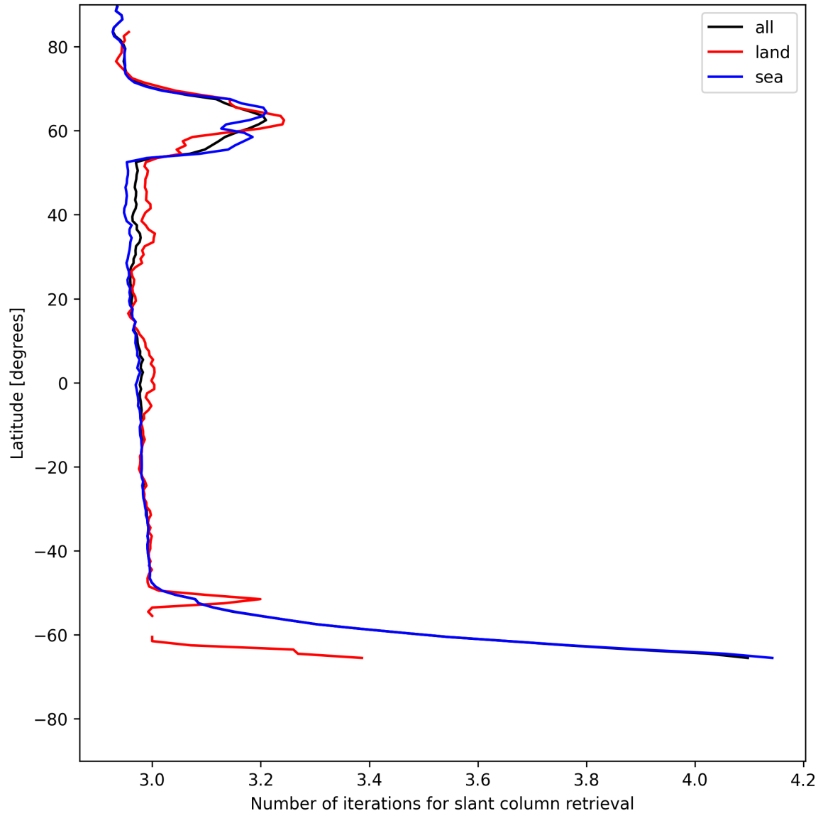
Figure 21: Zonal average of “Number of iterations for slant column retrieval” for 2025-06-12 to 2025-06-13.
