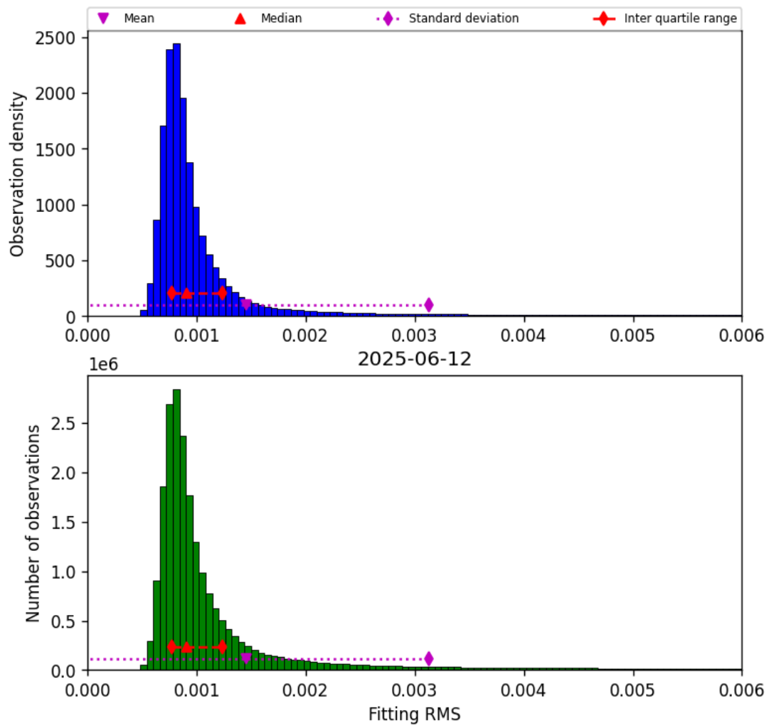
Figure 34: Histogram of “Fitting RMS” for 2025-06-12 to 2025-06-13
