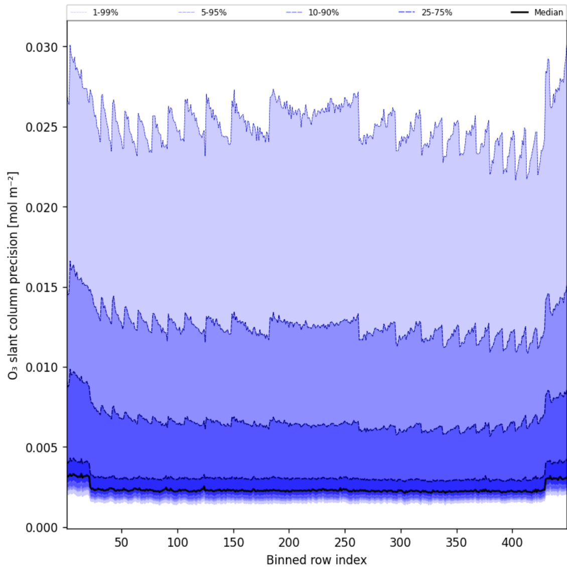
Figure 44: Along track statistics of “O 3 slant column precision” for 2025-06-12 to 2025-06-13
