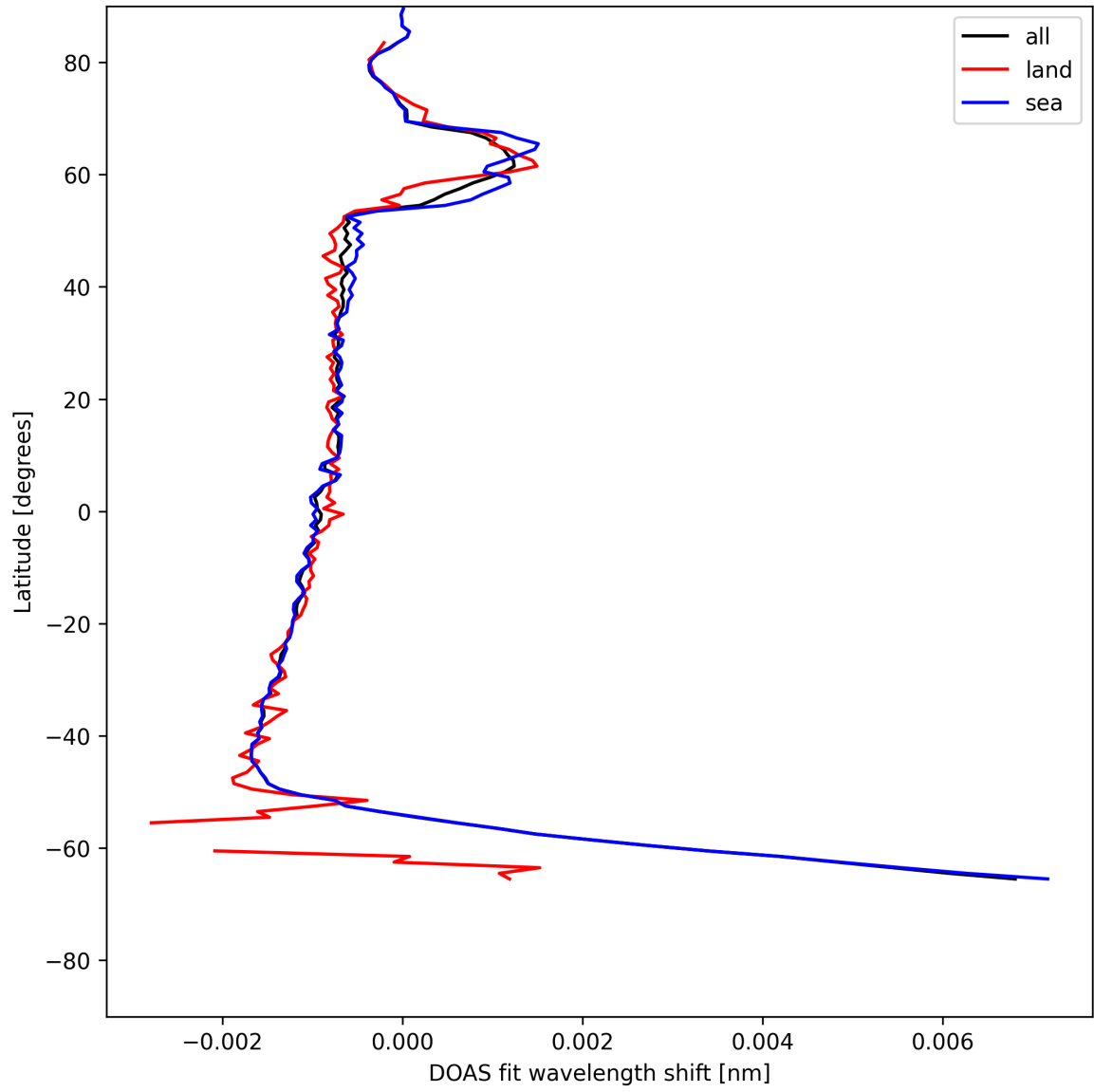
Figure 23: Zonal average of "DOAS fit wavelength shift" for 2025-06-12 to 2025-06-13.
