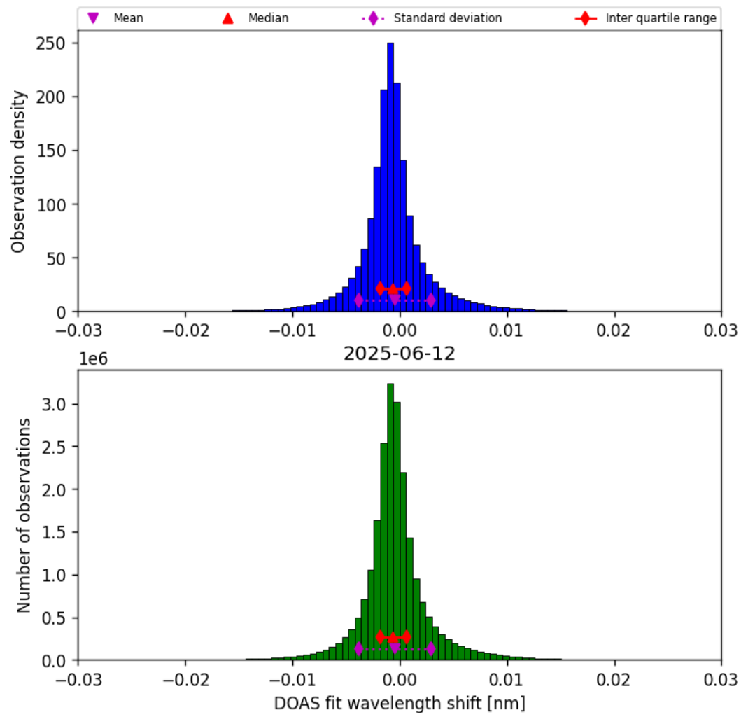
Figure 35: Histogram of “DOAS fit wavelength shift” for 2025-06-12 to 2025-06-13
