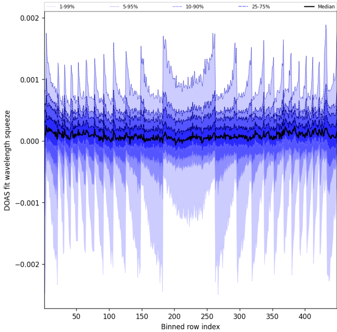
Figure 48: Along track statistics of “DOAS fit wavelength squeeze” for 2025-06-12 to 2025-06-13
