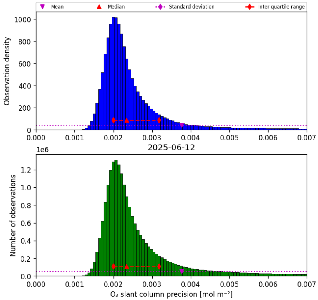
Figure 32: Histogram of “O 3 slant column precision” for 2025-06-12 to 2025-06-13
