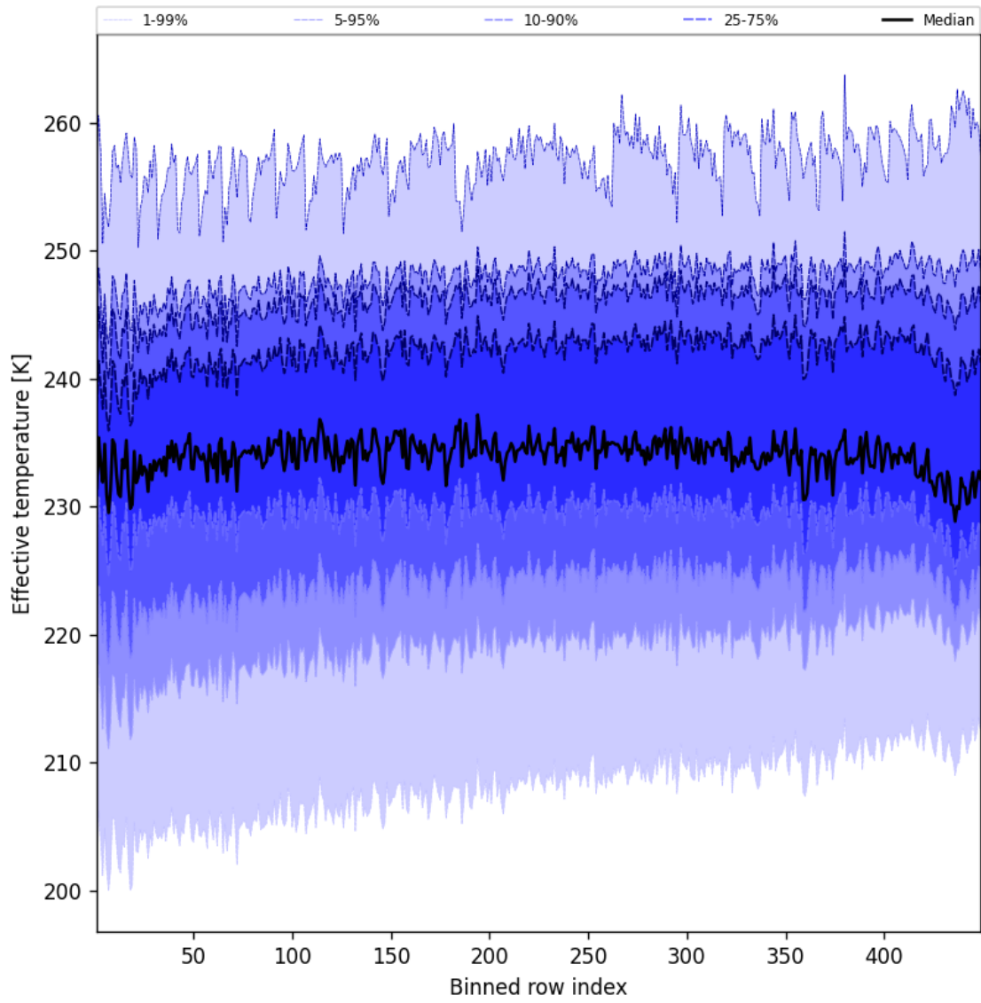
Figure 50: Along track statistics of “Effective temperature” for 2025-06-12 to 2025-06-13
