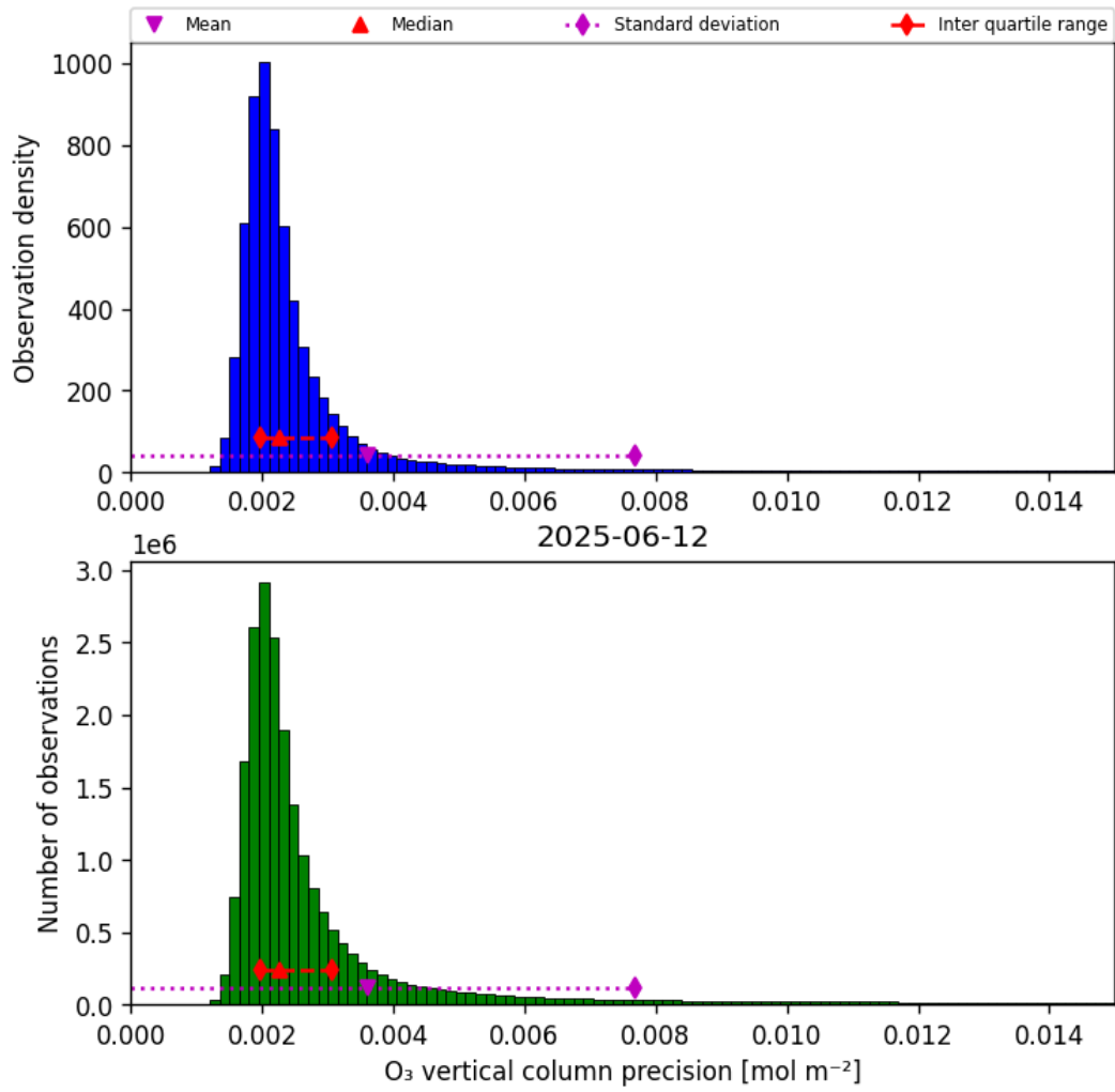
Figure 30: Histogram of “O 3 vertical column precision” for 2025-06-12 to 2025-06-13
