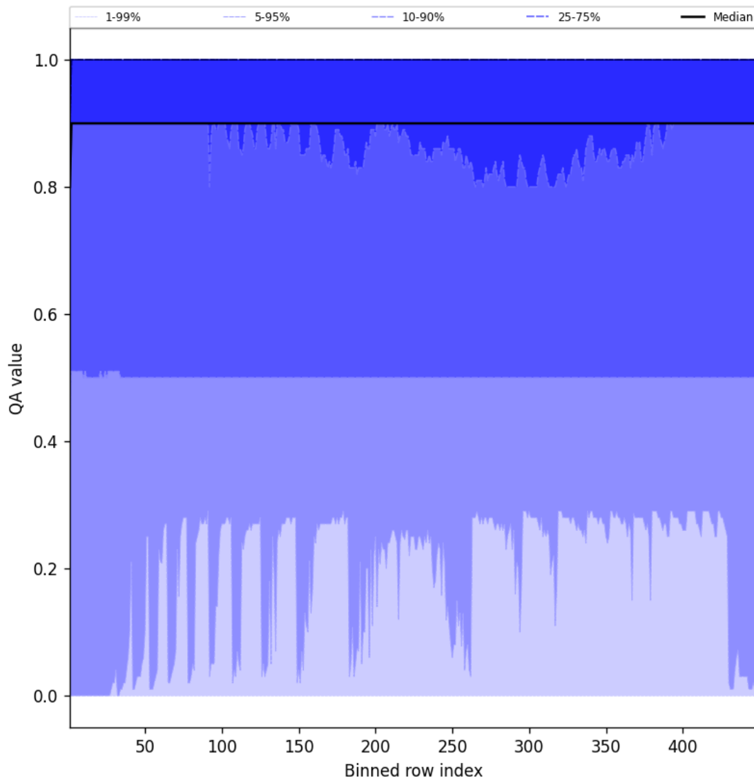
Figure 40: Along track statistics of “QA value” for 2025-06-12 to 2025-06-13
