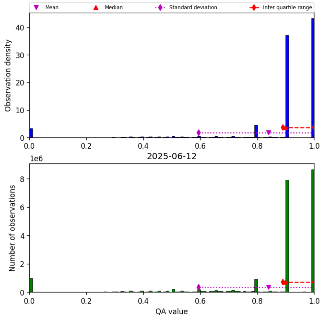
Figure 28: Histogram of “QA value” for 2025-06-12 to 2025-06-13
