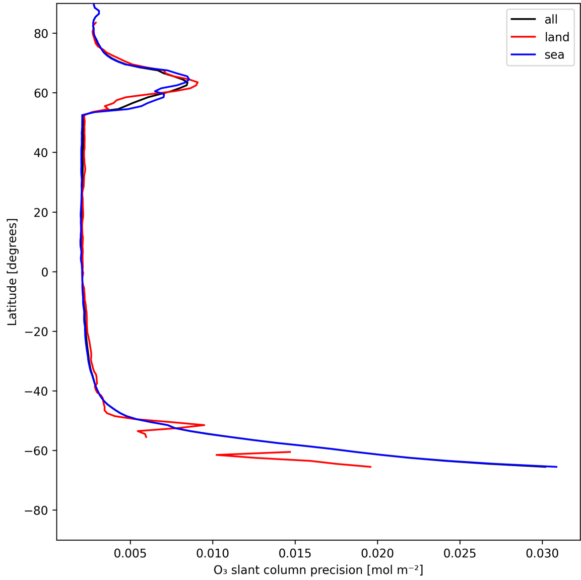
Figure 20: Zonal average of "O 3 slant column precision" for 2025-06-12 to 2025-06-13.
