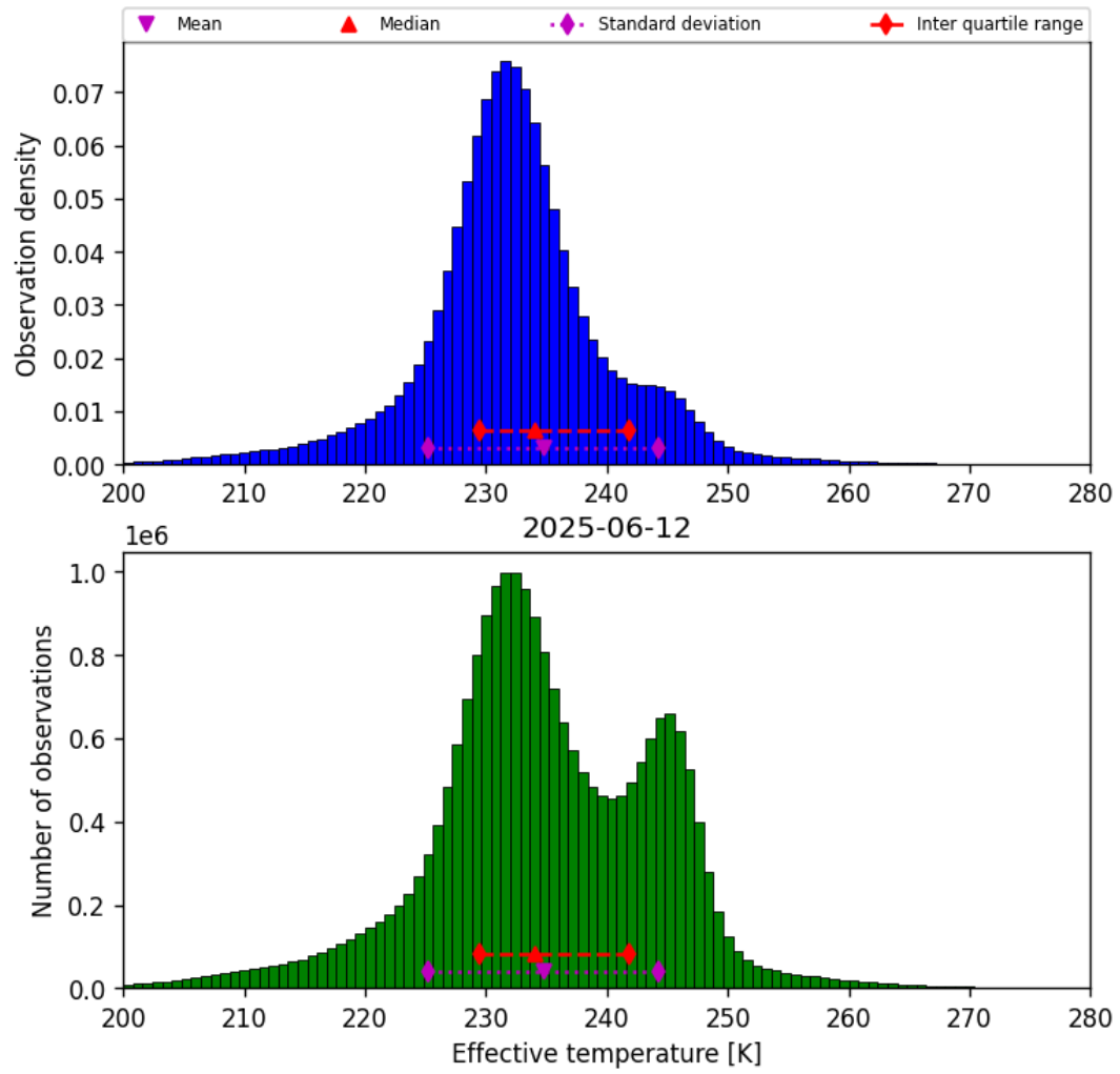
Figure 38: Histogram of “Effective temperature” for 2025-06-12 to 2025-06-13
