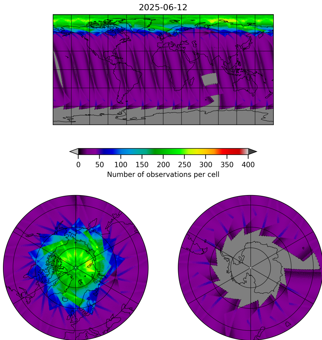
Figure 15: Map of the number of observations for 2025-06-12 to 2025-06-13
