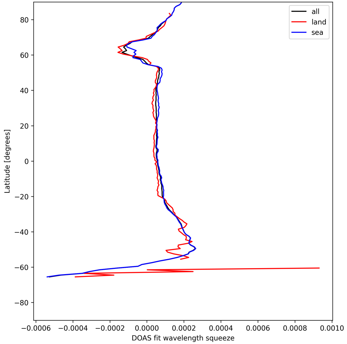
Figure 24: Zonal average of “DOAS fit wavelength squeeze” for 2025-06-12 to 2025-06-13.
