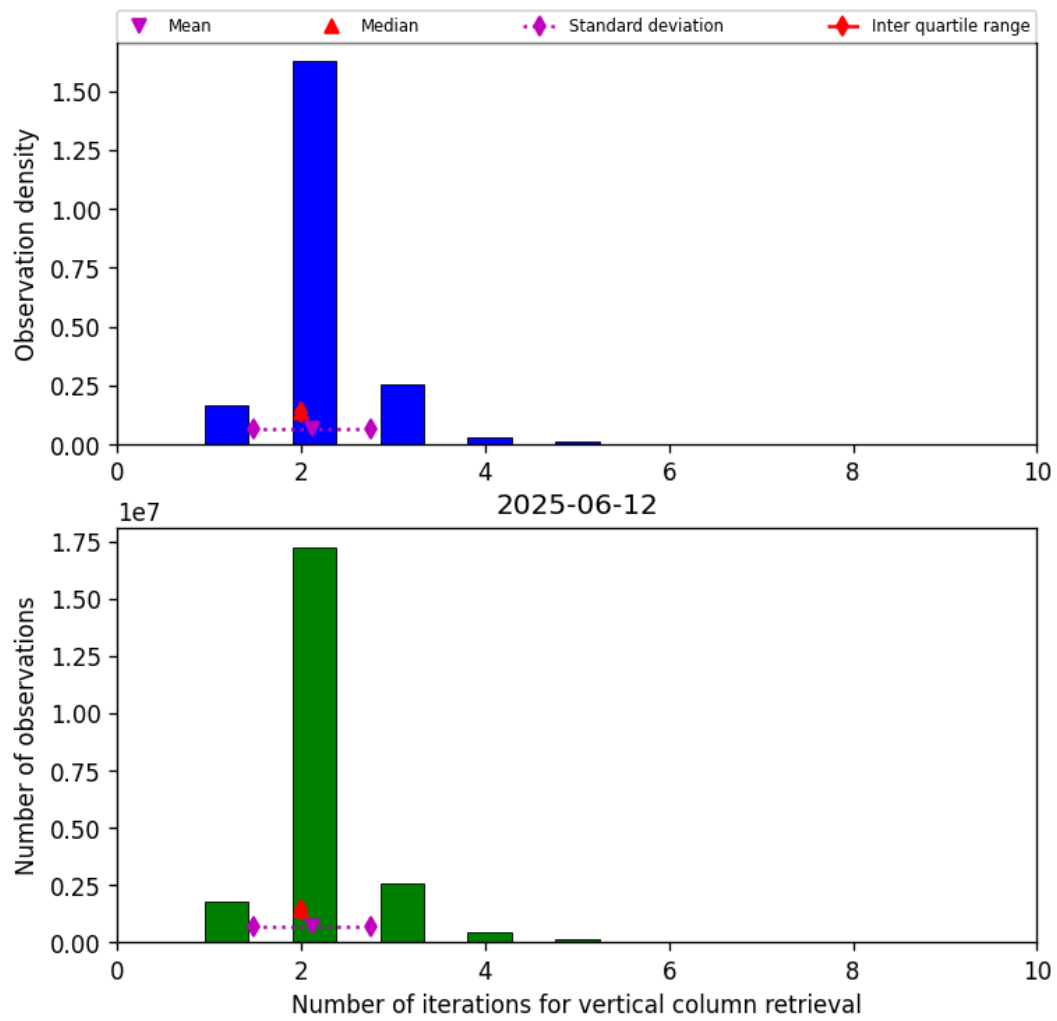
Figure 39: Histogram of “Number of iterations for vertical column retrieval” for 2025-06-12 to 2025-06-13
