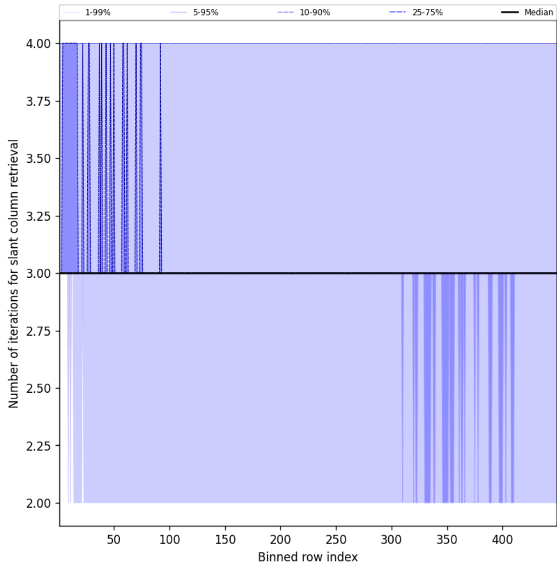
Figure 45: Along track statistics of “Number of iterations for slant column retrieval” for 2025-06-12 to 2025-06-13
