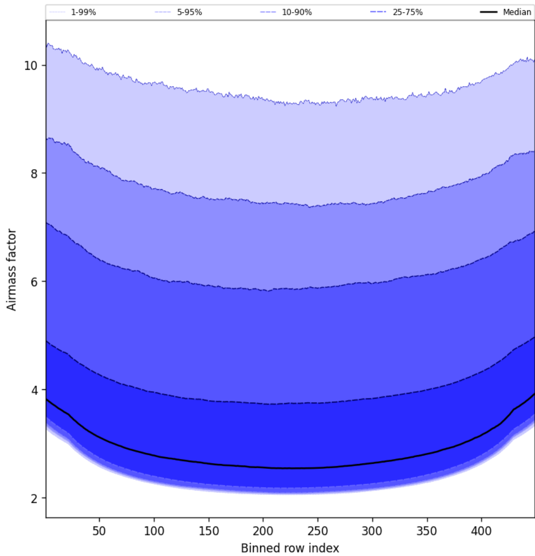
Figure 49: Along track statistics of “Airmass factor” for 2025-06-12 to 2025-06-13
