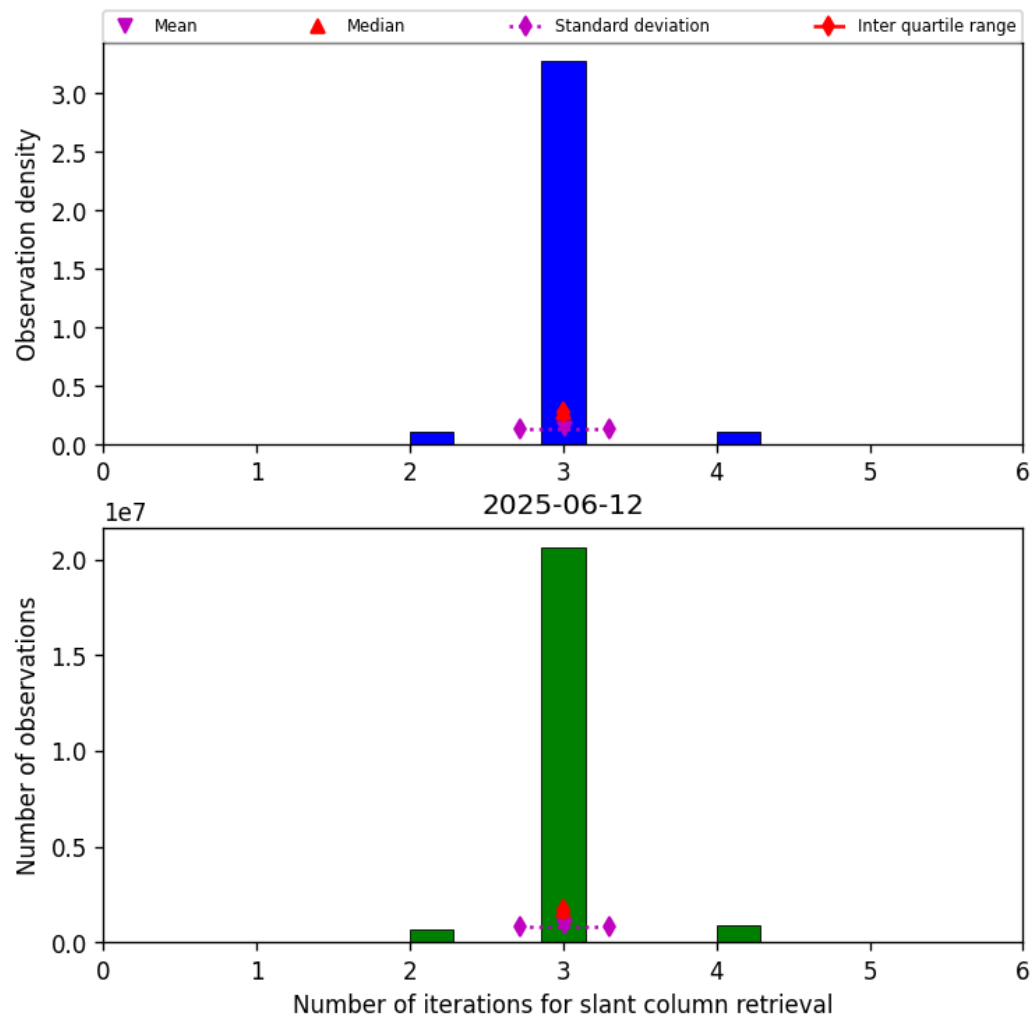
Figure 33: Histogram of “Number of iterations for slant column retrieval” for 2025-06-12 to 2025-06-13
