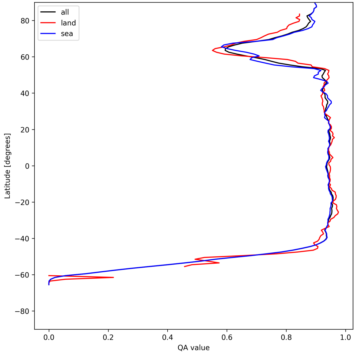
Figure 16: Zonal average of “QA value” for 2025-06-12 to 2025-06-13.
