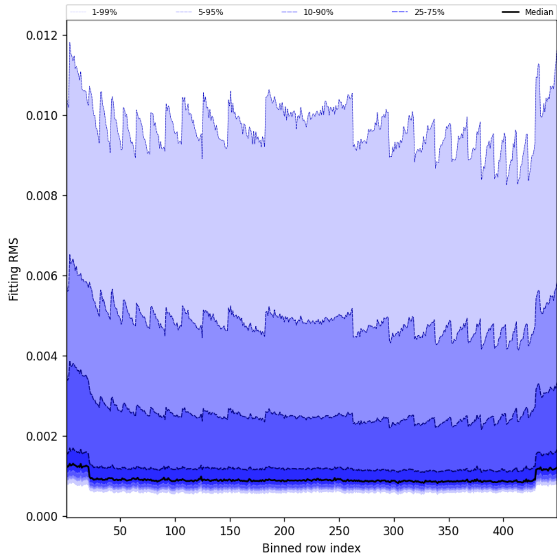
Figure 46: Along track statistics of “Fitting RMS” for 2025-06-12 to 2025-06-13
