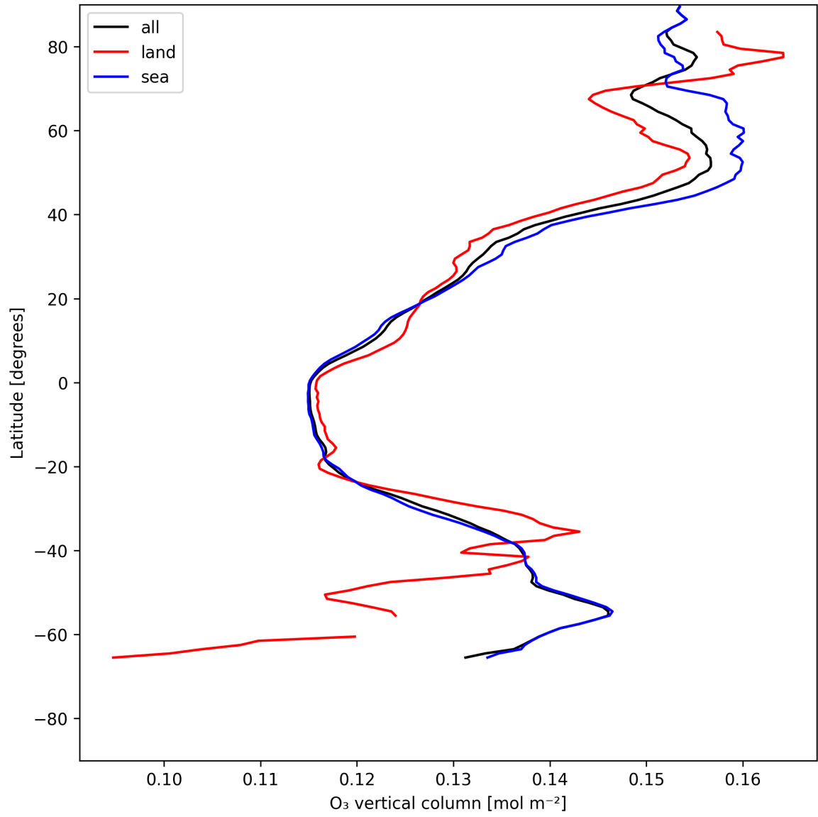
Figure 17: Zonal average of “O 3 vertical column” for 2025-06-12 to 2025-06-13.
