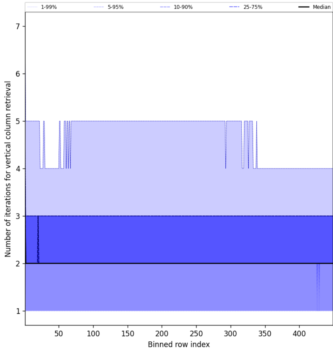
Figure 51: Along track statistics of “Number of iterations for vertical column retrieval” for 2025-06-12 to 2025-06-13
