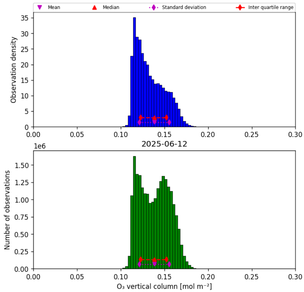
Figure 29: Histogram of “O 3 vertical column” for 2025-06-12 to 2025-06-13
