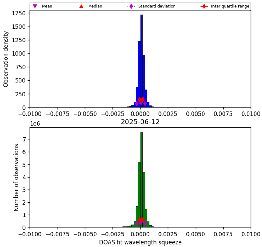
Figure 36: Histogram of “DOAS fit wavelength squeeze” for 2025-06-12 to 2025-06-13
