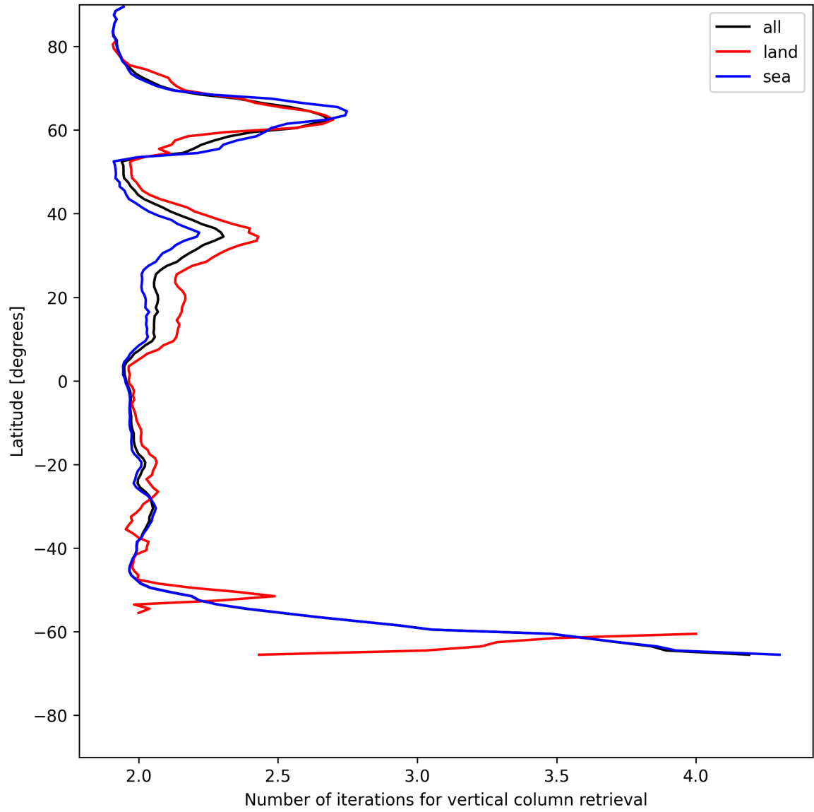
Figure 27: Zonal average of “Number of iterations for vertical column retrieval” for 2025-06-12 to 2025-06-13.
