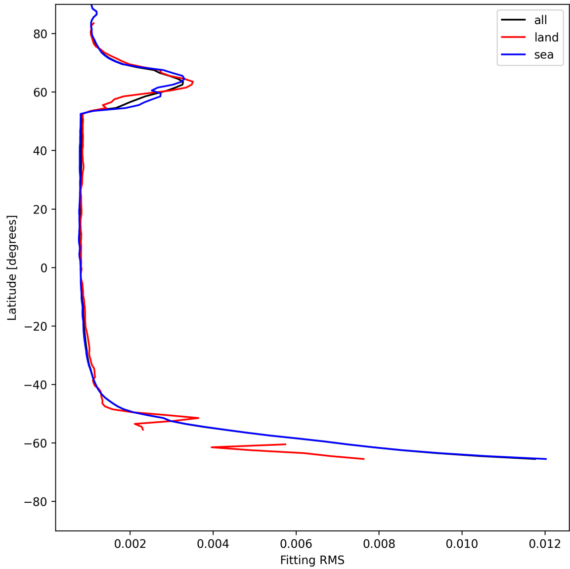
Figure 22: Zonal average of “Fitting RMS” for 2025-06-12 to 2025-06-13.
