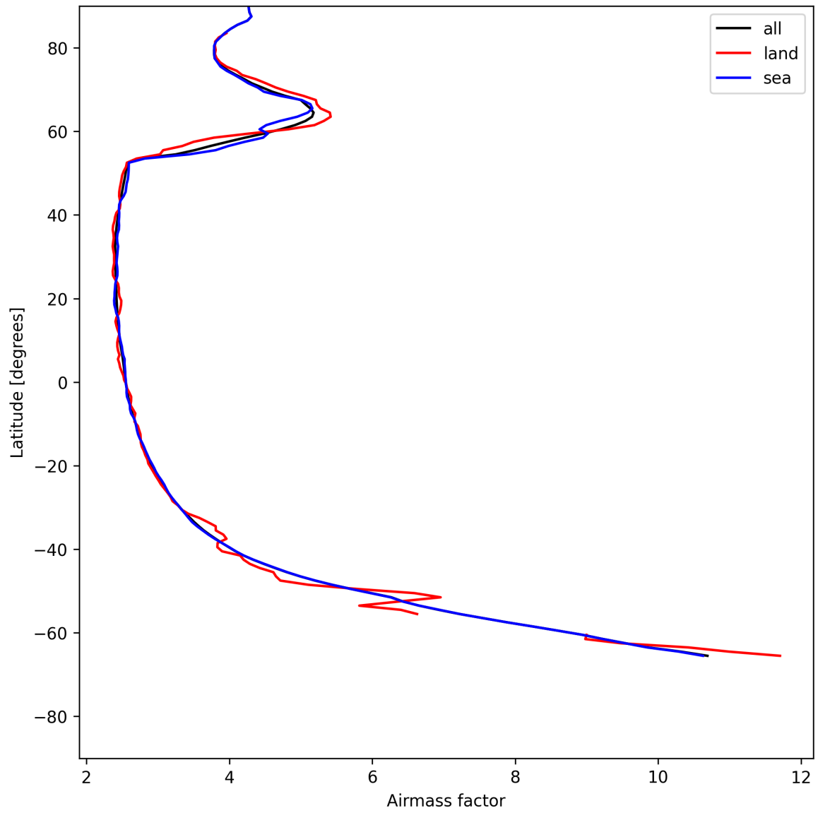
Figure 25: Zonal average of “Airmass factor” for 2025-06-12 to 2025-06-13.
