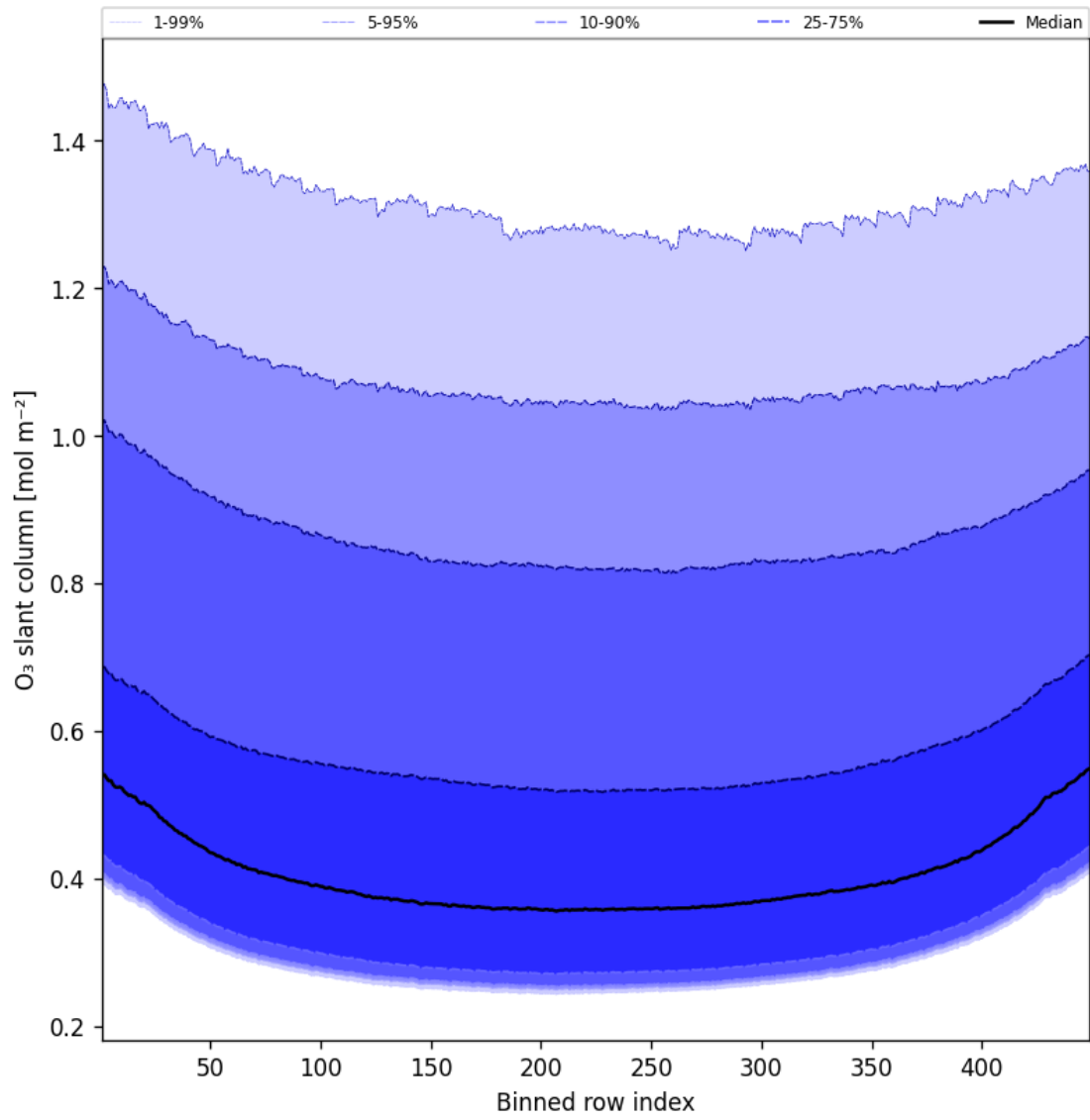
Figure 43: Along track statistics of “O 3 slant column” for 2025-06-12 to 2025-06-13
