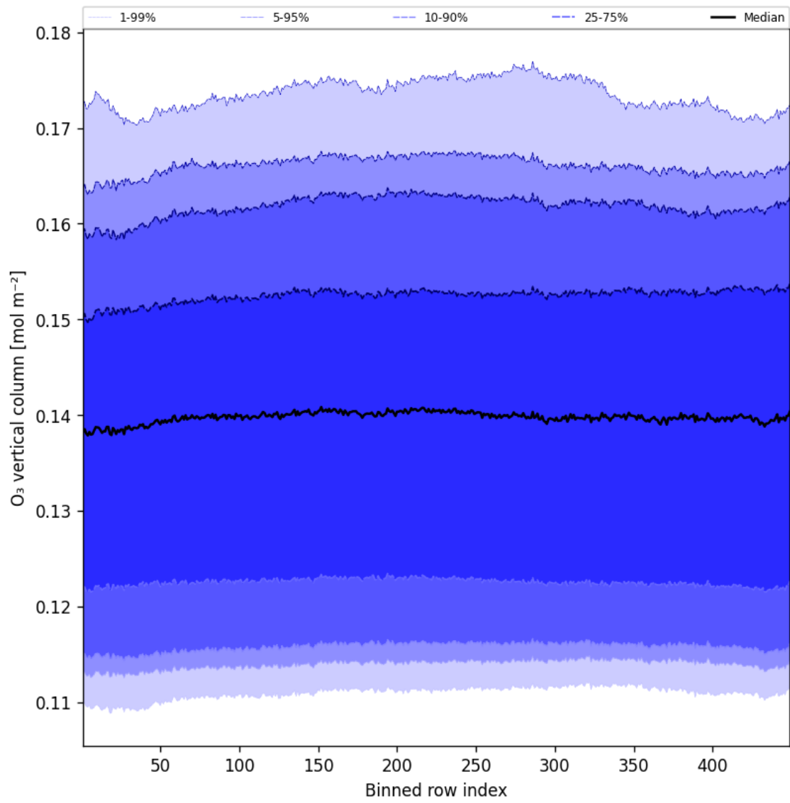
Figure 41: Along track statistics of “O 3 vertical column” for 2025-06-13 to 2025-06-14
