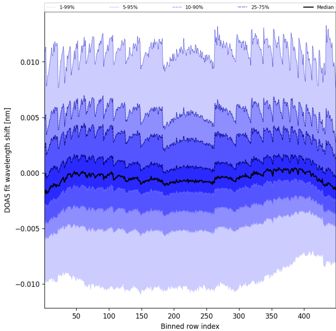
Figure 47: Along track statistics of “DOAS fit wavelength shift” for 2025-06-13 to 2025-06-14
