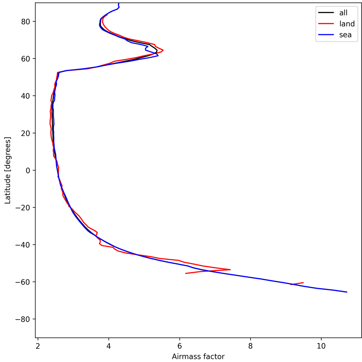
Figure 25: Zonal average of “Airmass factor” for 2025-06-13 to 2025-06-14.
