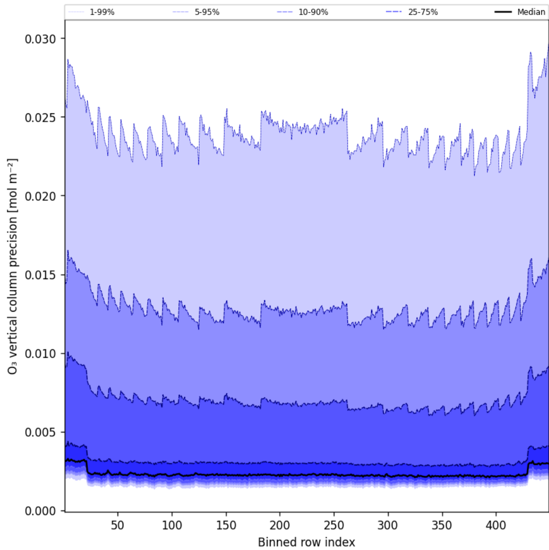
Figure 42: Along track statistics of “O 3 vertical column precision” for 2025-06-13 to 2025-06-14
