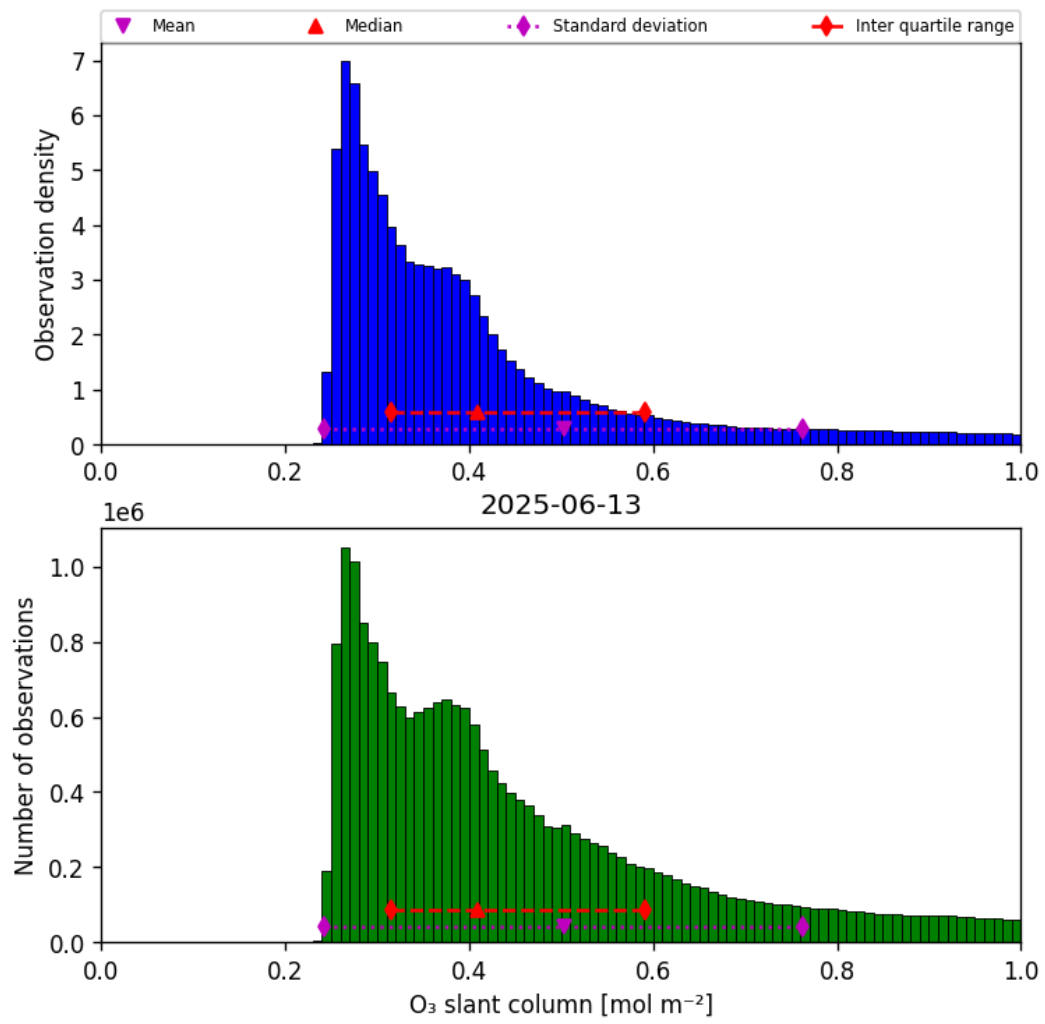
Figure 31: Histogram of “O 3 slant column” for 2025-06-13 to 2025-06-14
