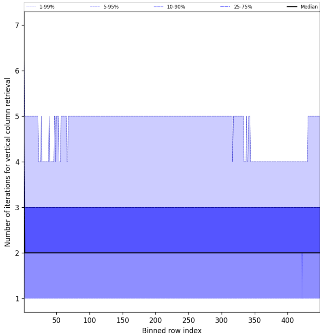
Figure 51: Along track statistics of “Number of iterations for vertical column retrieval” for 2025-06-13 to 2025-06-14
