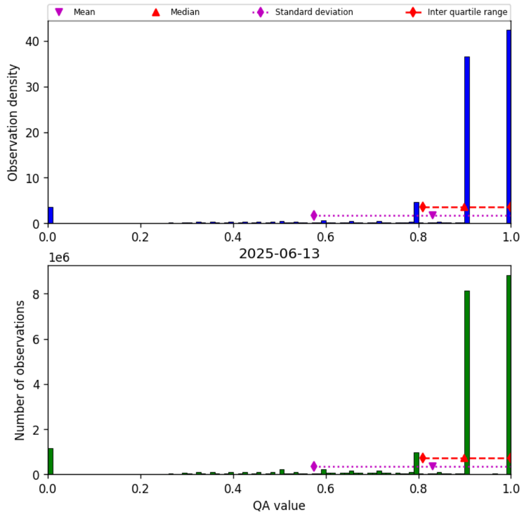
Figure 28: Histogram of “QA value” for 2025-06-13 to 2025-06-14
