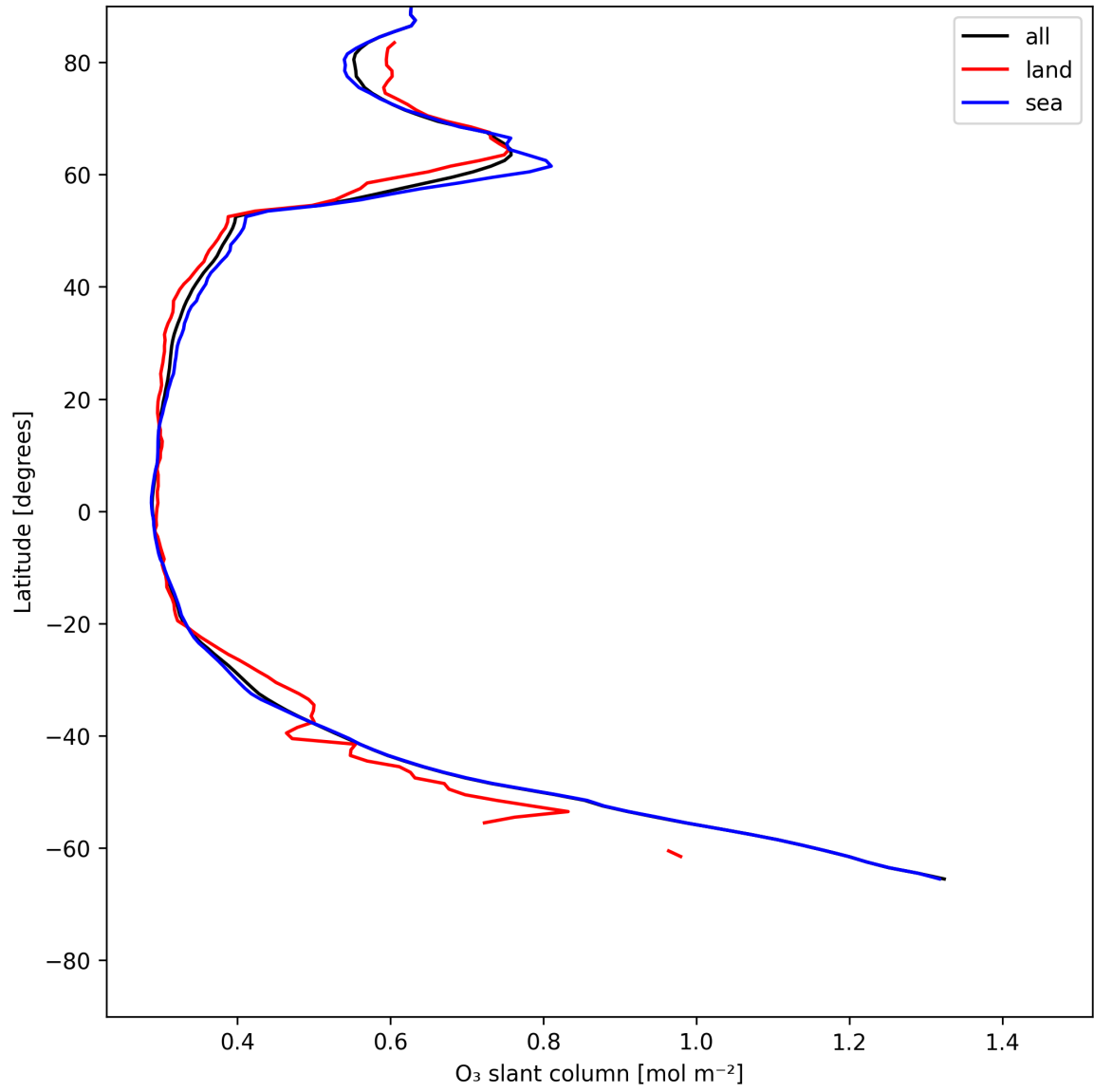
Figure 19: Zonal average of “O 3 slant column” for 2025-06-13 to 2025-06-14.
