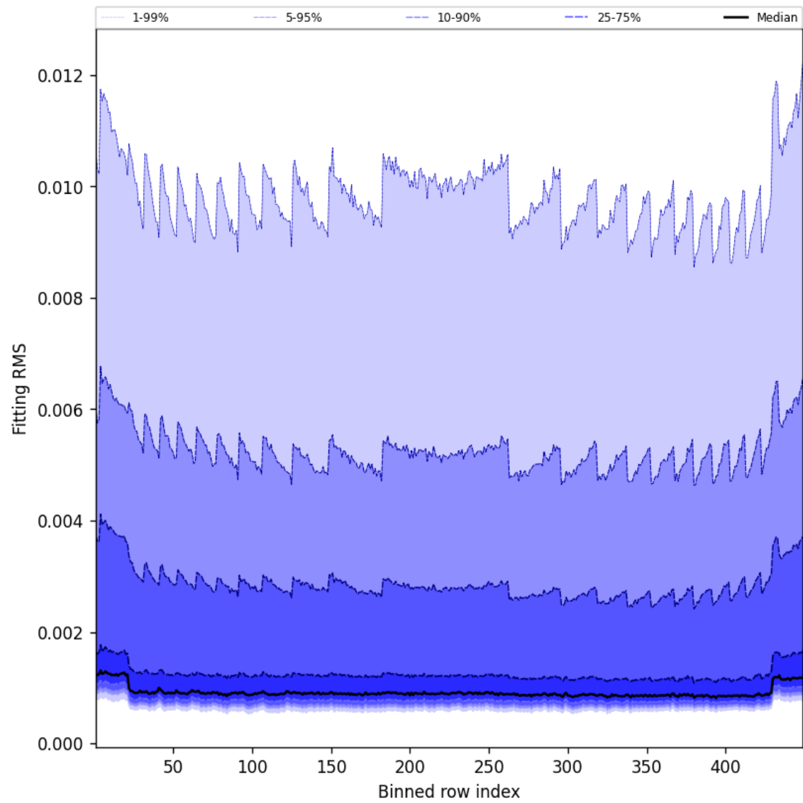
Figure 46: Along track statistics of “Fitting RMS” for 2025-06-13 to 2025-06-14
