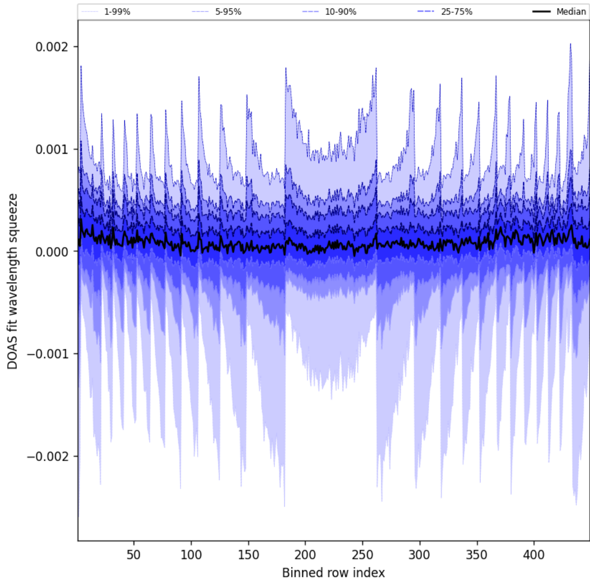
Figure 48: Along track statistics of “DOAS fit wavelength squeeze” for 2025-06-13 to 2025-06-14
