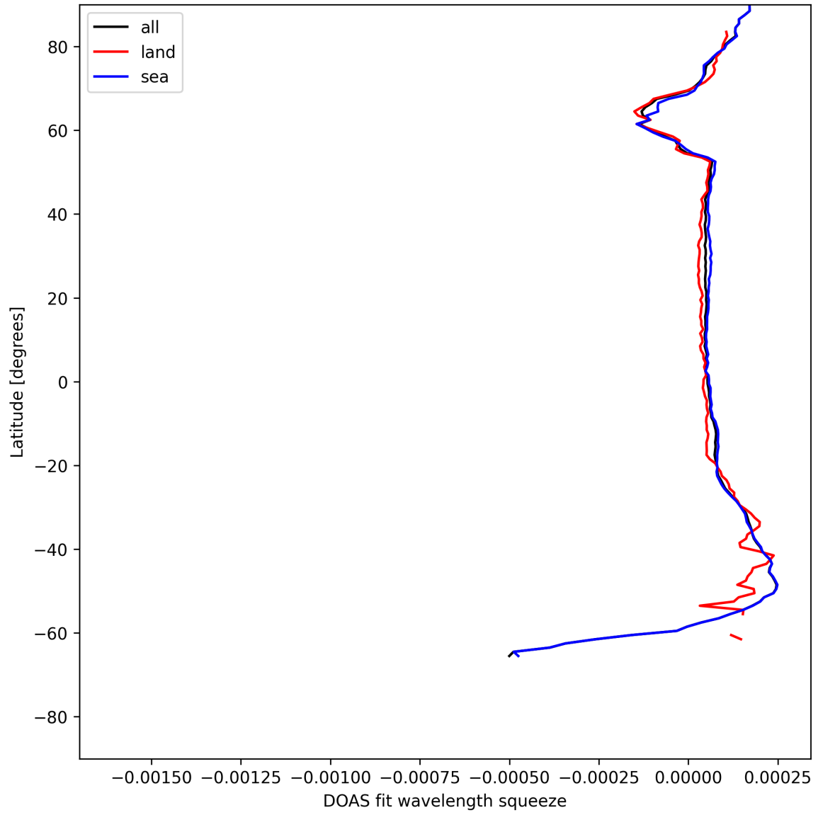
Figure 24: Zonal average of “DOAS fit wavelength squeeze” for 2025-06-13 to 2025-06-14.
