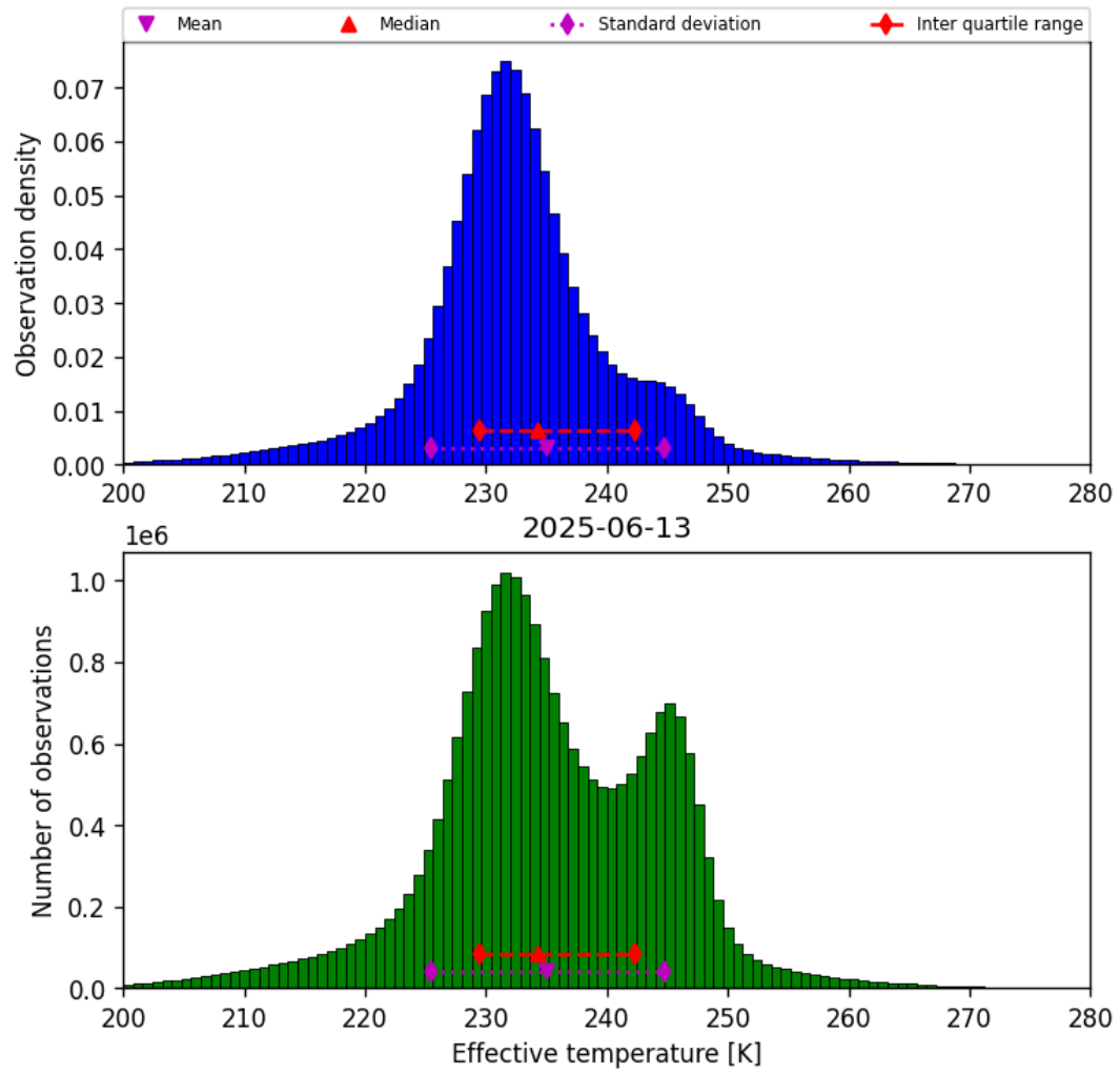
Figure 38: Histogram of “Effective temperature” for 2025-06-13 to 2025-06-14
