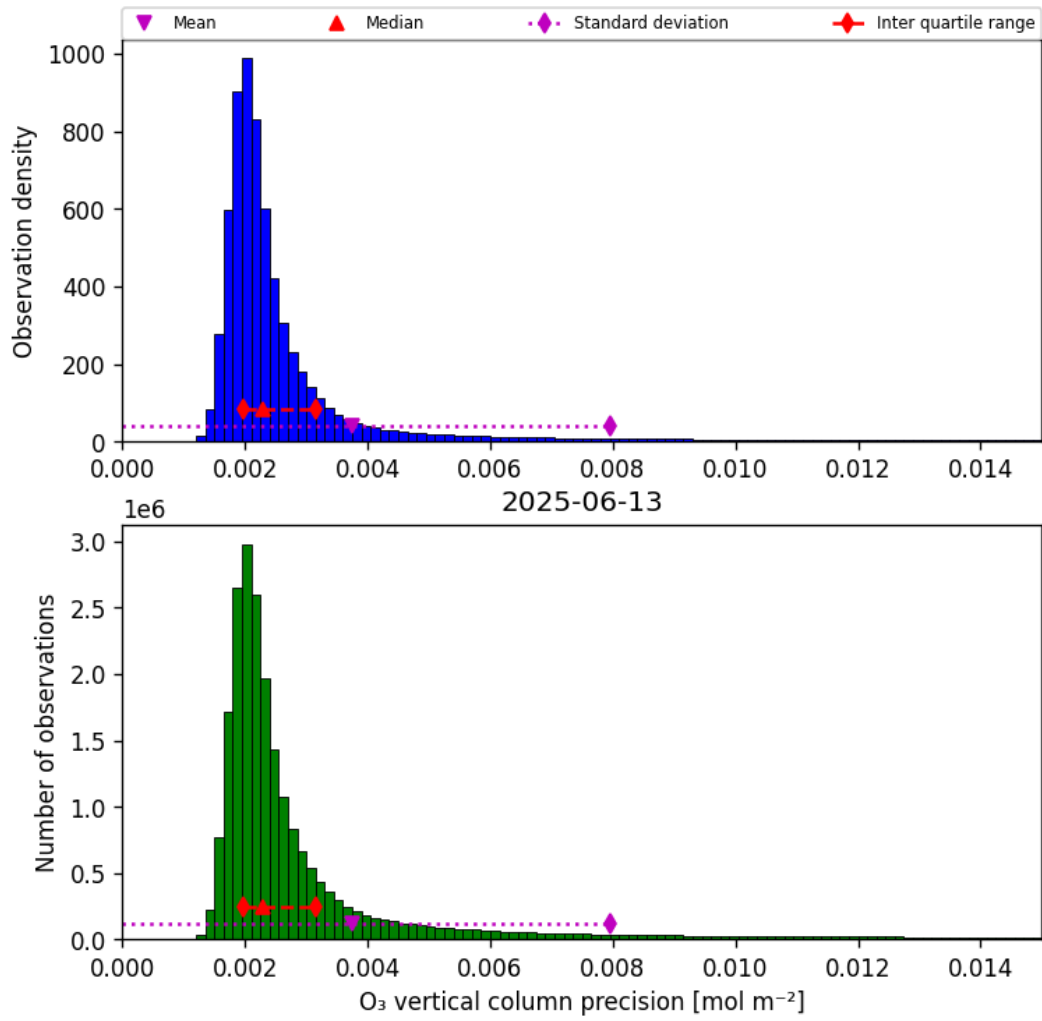
Figure 30: Histogram of “O 3 vertical column precision” for 2025-06-13 to 2025-06-14
