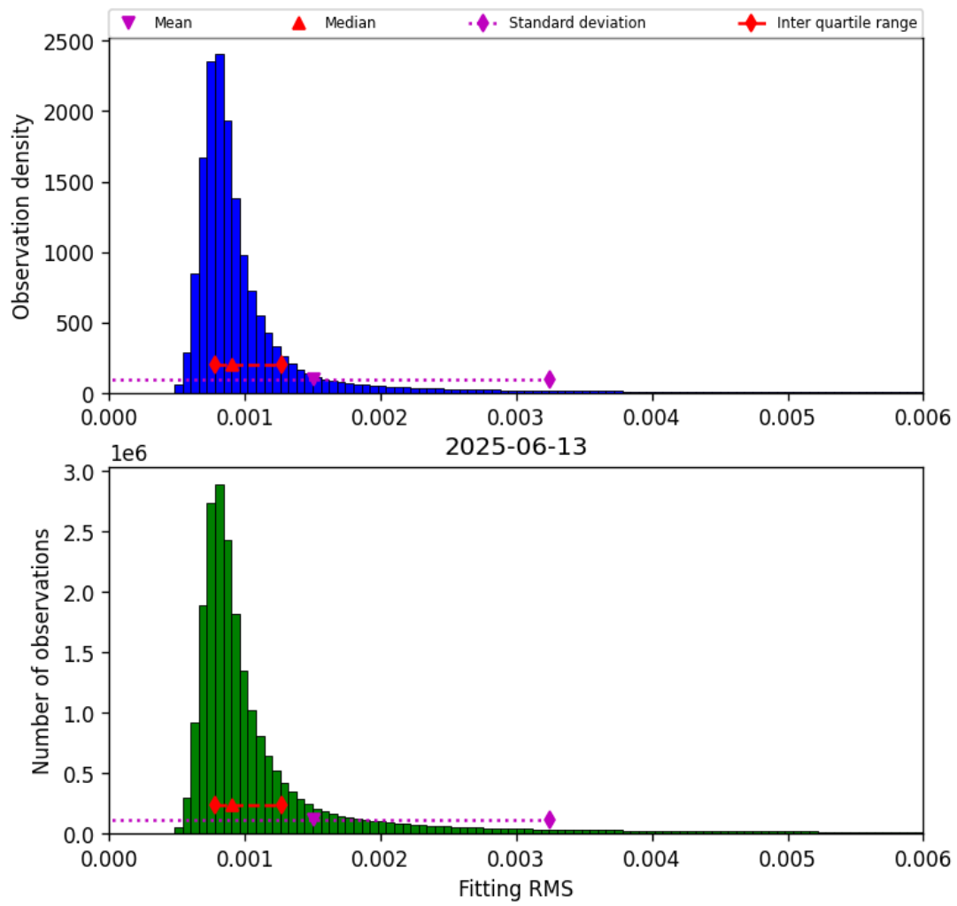
Figure 34: Histogram of “Fitting RMS” for 2025-06-13 to 2025-06-14
