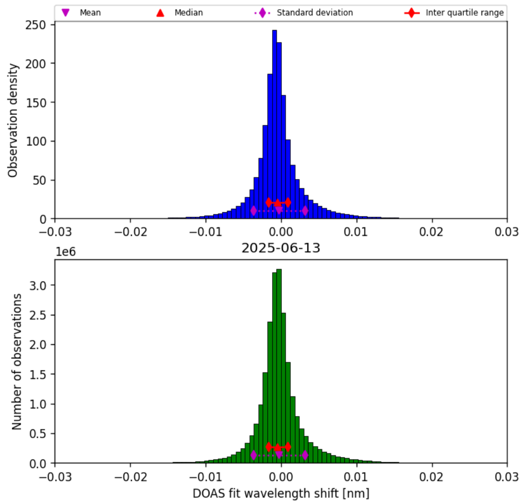
Figure 35: Histogram of “DOAS fit wavelength shift” for 2025-06-13 to 2025-06-14
