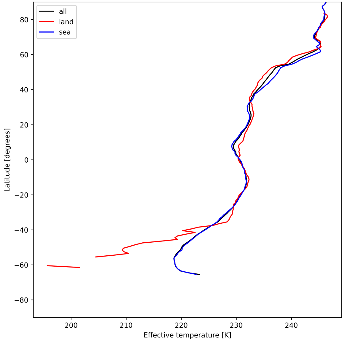
Figure 26: Zonal average of "Effective temperature" for 2025-06-13 to 2025-06-14.
