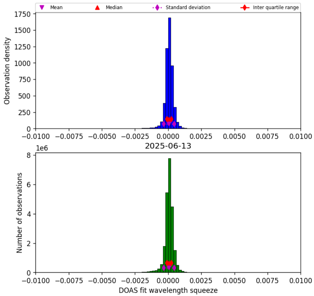
Figure 36: Histogram of “DOAS fit wavelength squeeze” for 2025-06-13 to 2025-06-14
