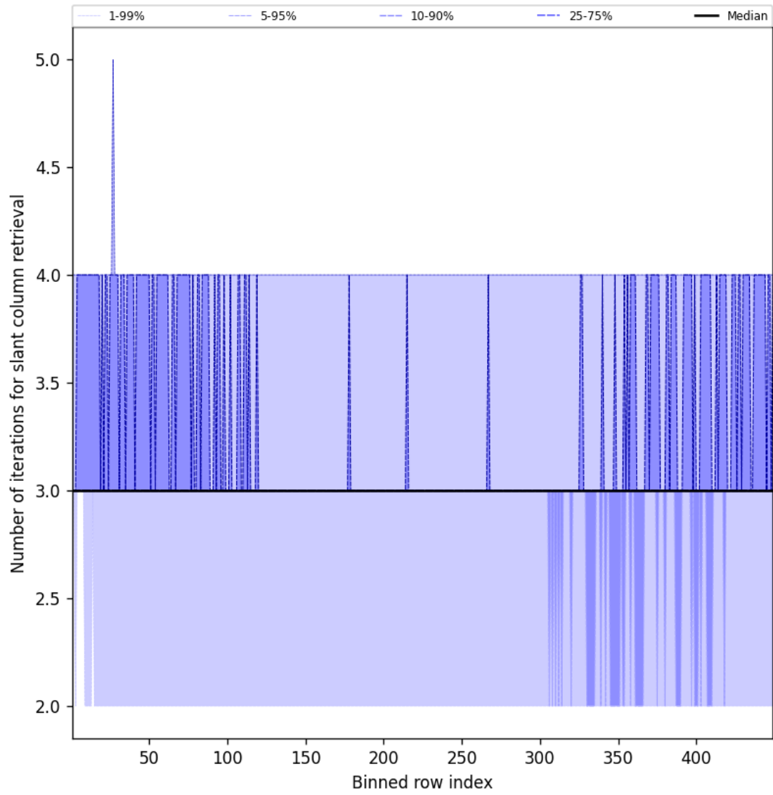
Figure 45: Along track statistics of “Number of iterations for slant column retrieval” for 2025-06-13 to 2025-06-14
