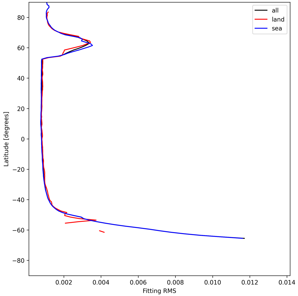
Figure 22: Zonal average of “Fitting RMS” for 2025-06-13 to 2025-06-14.
