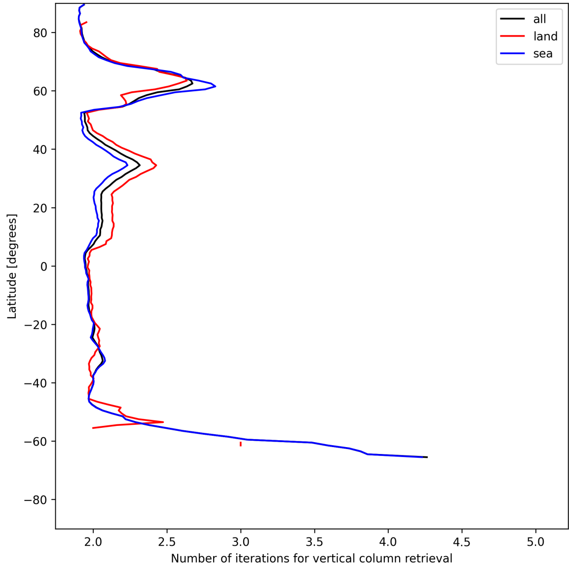
Figure 27: Zonal average of “Number of iterations for vertical column retrieval” for 2025-06-13 to 2025-06-14.
