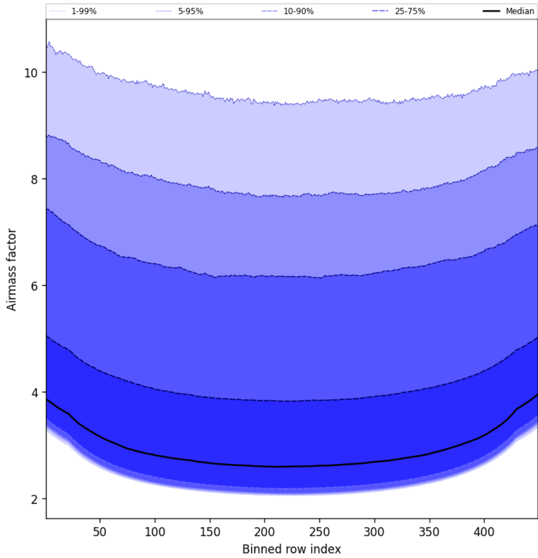
Figure 49: Along track statistics of “Airmass factor” for 2025-06-13 to 2025-06-14
