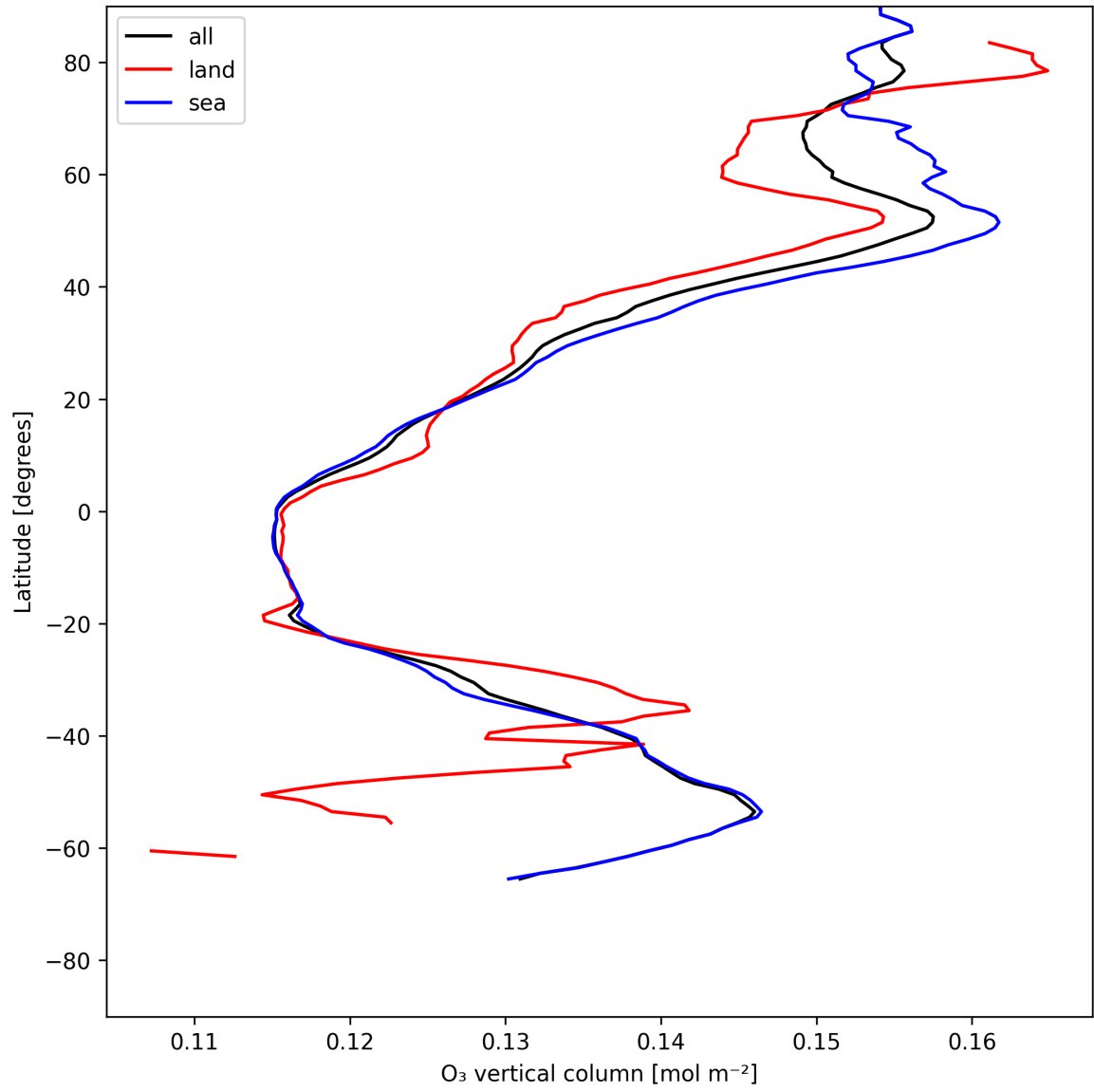
Figure 17: Zonal average of “O 3 vertical column” for 2025-06-13 to 2025-06-14.
