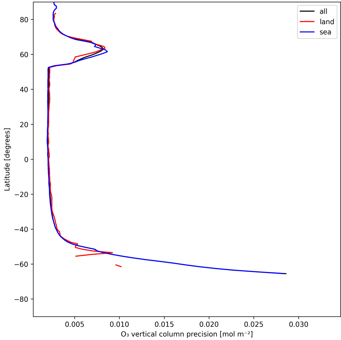
Figure 18: Zonal average of “O 3 vertical column precision” for 2025-06-13 to 2025-06-14.
