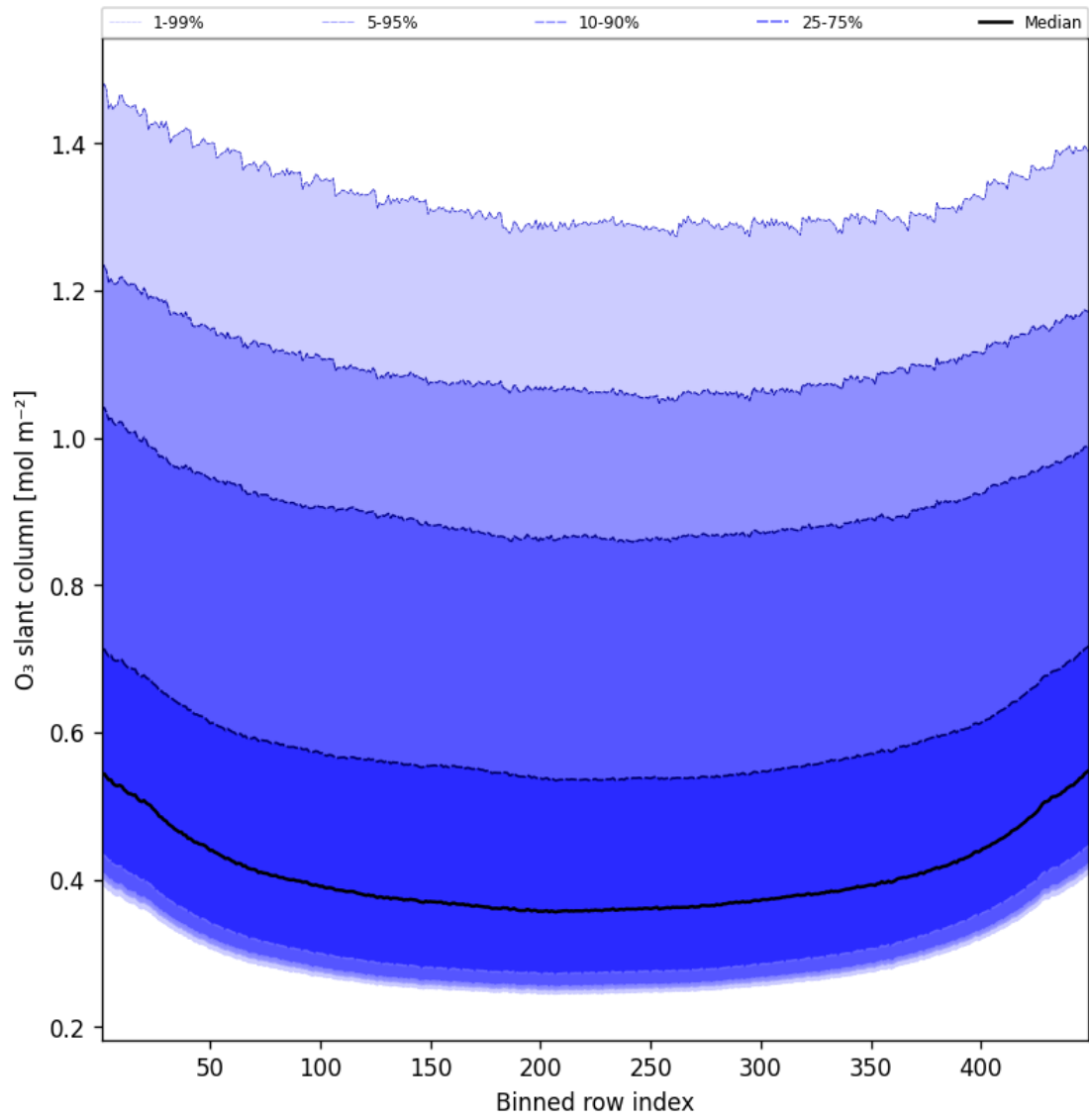
Figure 43: Along track statistics of “O 3 slant column” for 2025-06-13 to 2025-06-14
