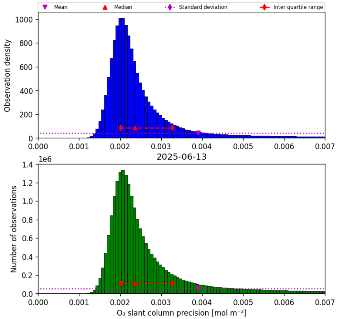
Figure 32: Histogram of “O 3 slant column precision” for 2025-06-13 to 2025-06-14
