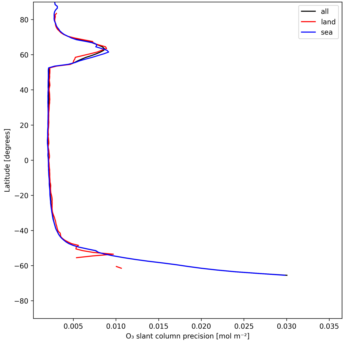
Figure 20: Zonal average of “O 3 slant column precision” for 2025-06-13 to 2025-06-14.
