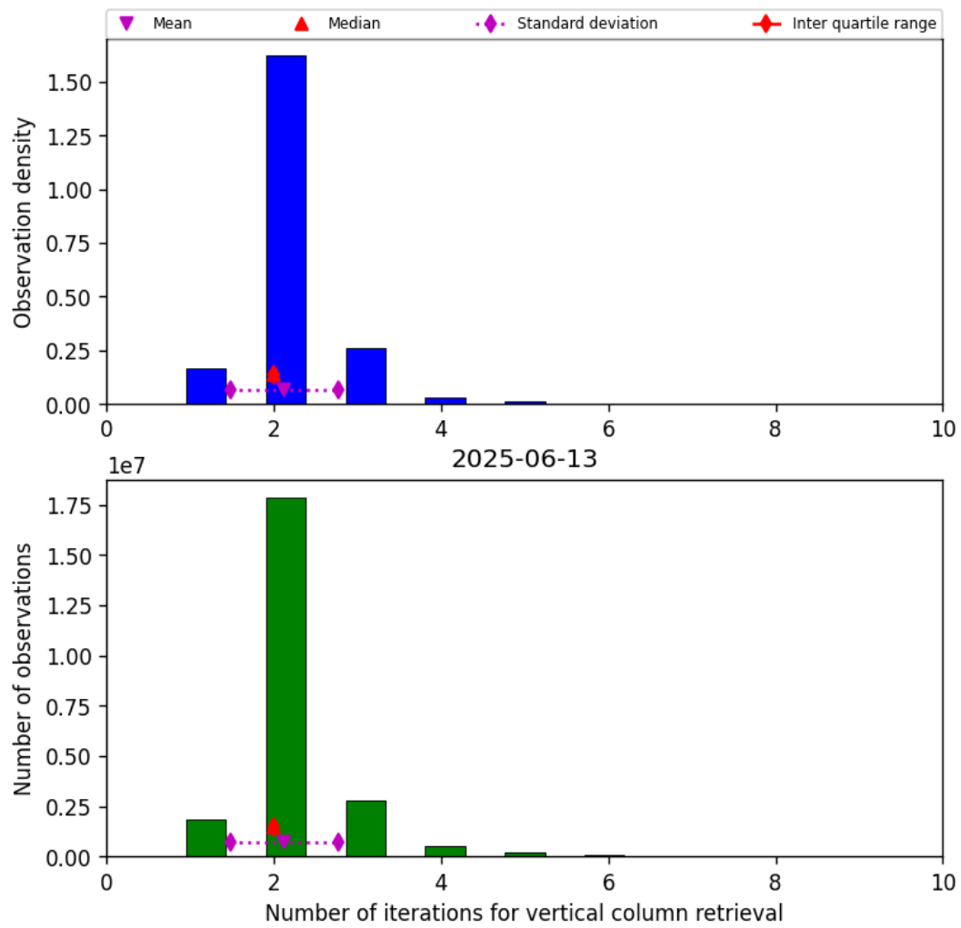
Figure 39: Histogram of “Number of iterations for vertical column retrieval” for 2025-06-13 to 2025-06-14
