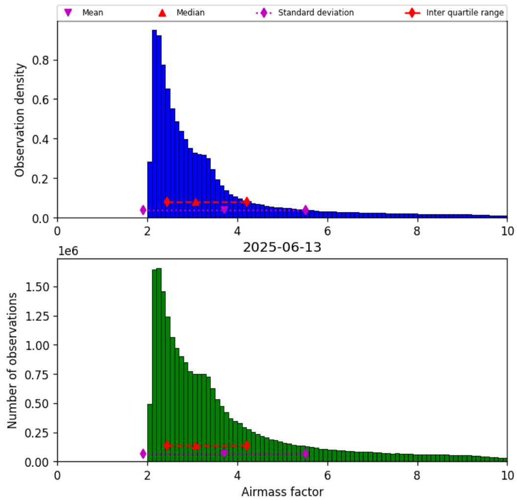
Figure 37: Histogram of “Airmass factor” for 2025-06-13 to 2025-06-14
