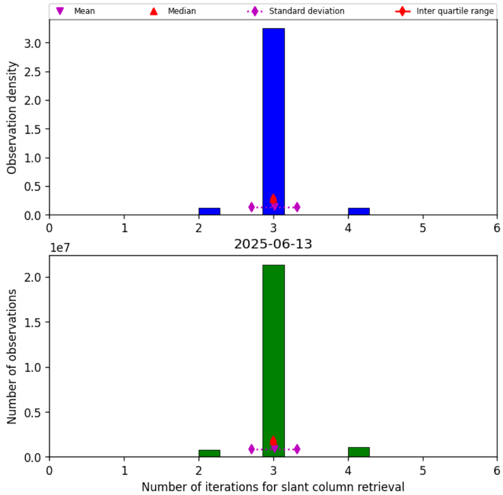
Figure 33: Histogram of “Number of iterations for slant column retrieval” for 2025-06-13 to 2025-06-14
