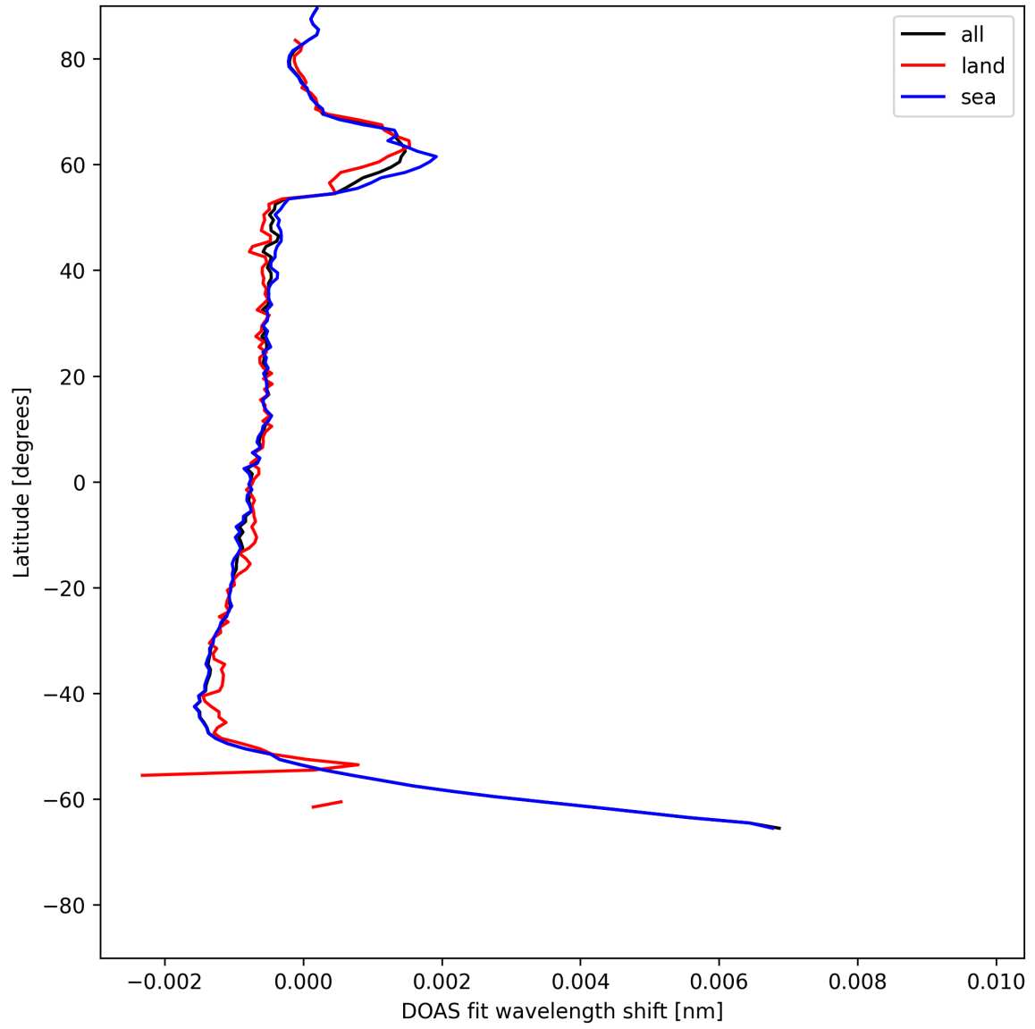
Figure 23: Zonal average of “DOAS fit wavelength shift” for 2025-06-13 to 2025-06-14.
