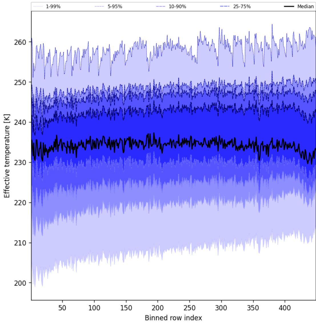
Figure 50: Along track statistics of “Effective temperature” for 2025-06-13 to 2025-06-14
