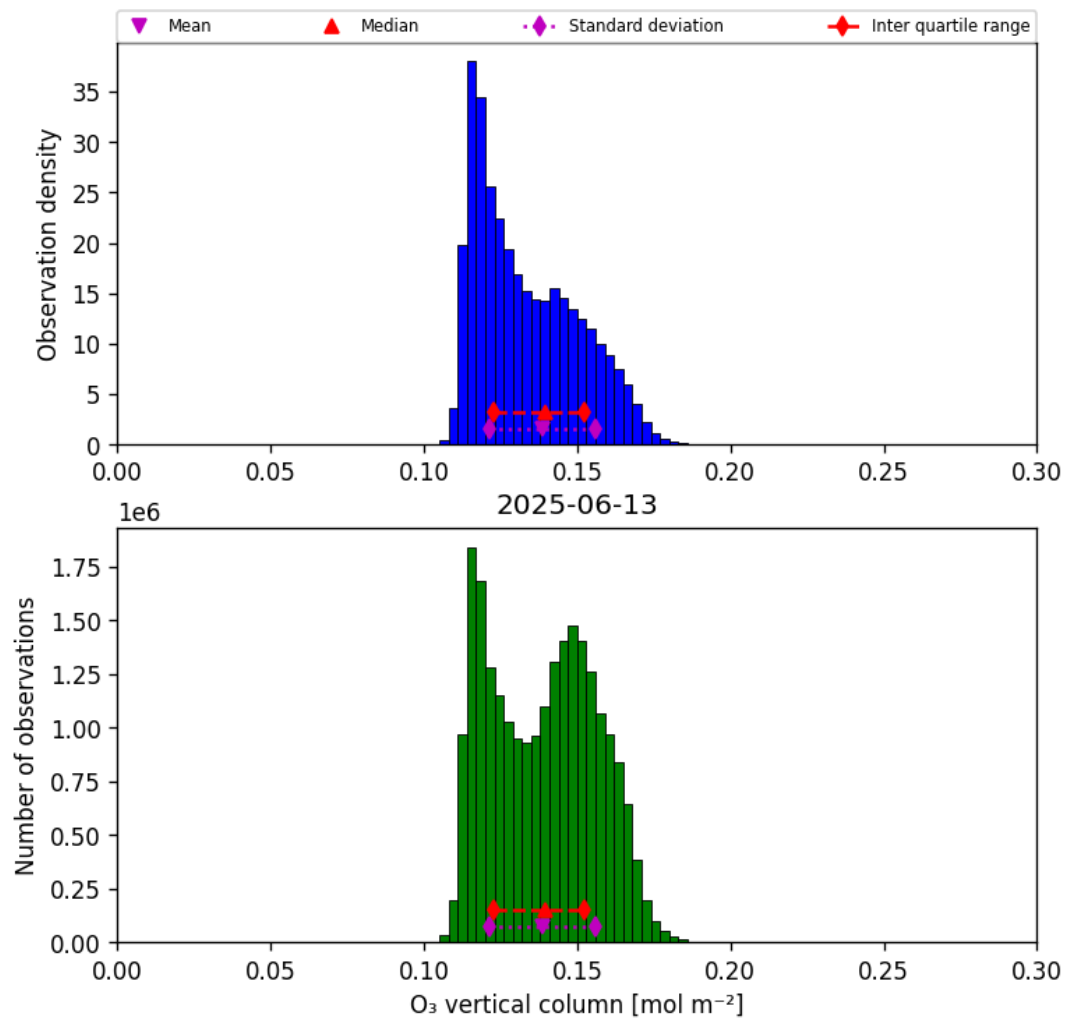
Figure 29: Histogram of “O 3 vertical column” for 2025-06-13 to 2025-06-14
