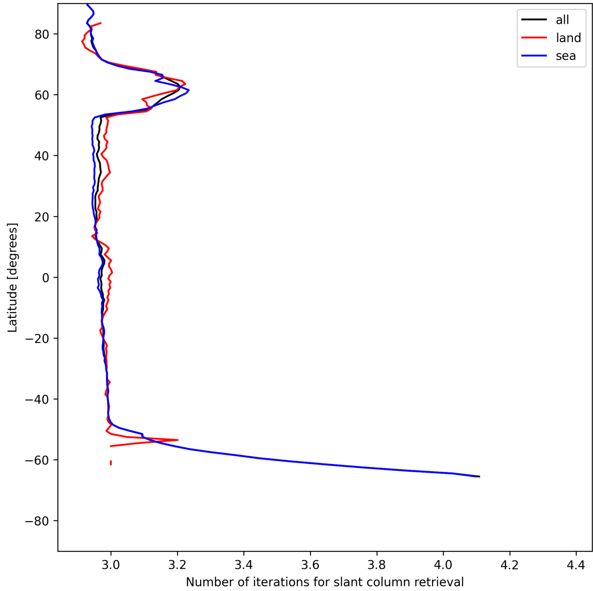
Figure 21: Zonal average of “Number of iterations for slant column retrieval” for 2025-06-13 to 2025-06-14.
