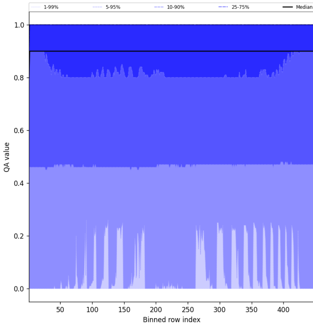
Figure 40: Along track statistics of “QA value” for 2025-06-13 to 2025-06-14
