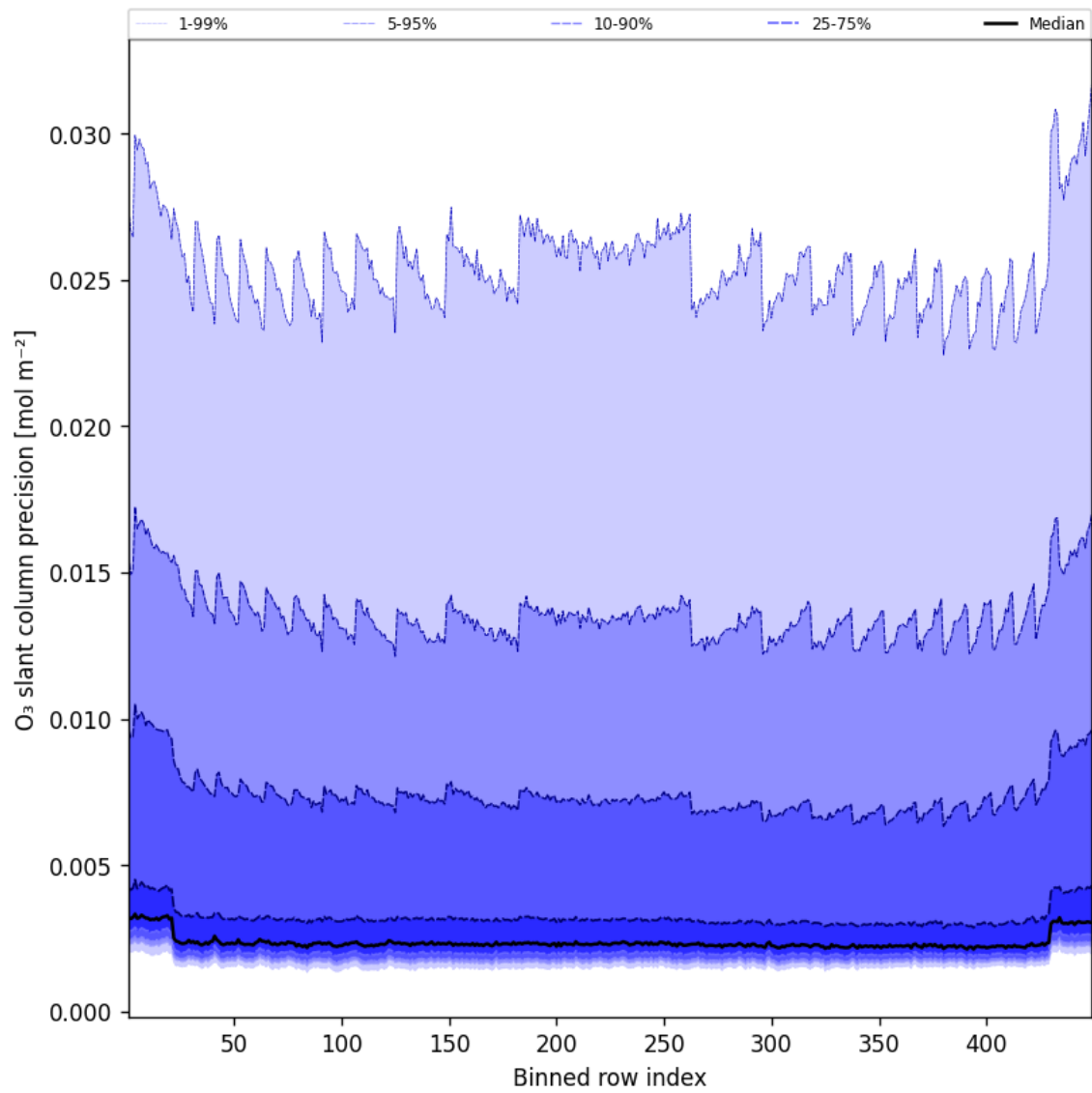
Figure 44: Along track statistics of “O 3 slant column precision” for 2025-06-13 to 2025-06-14
