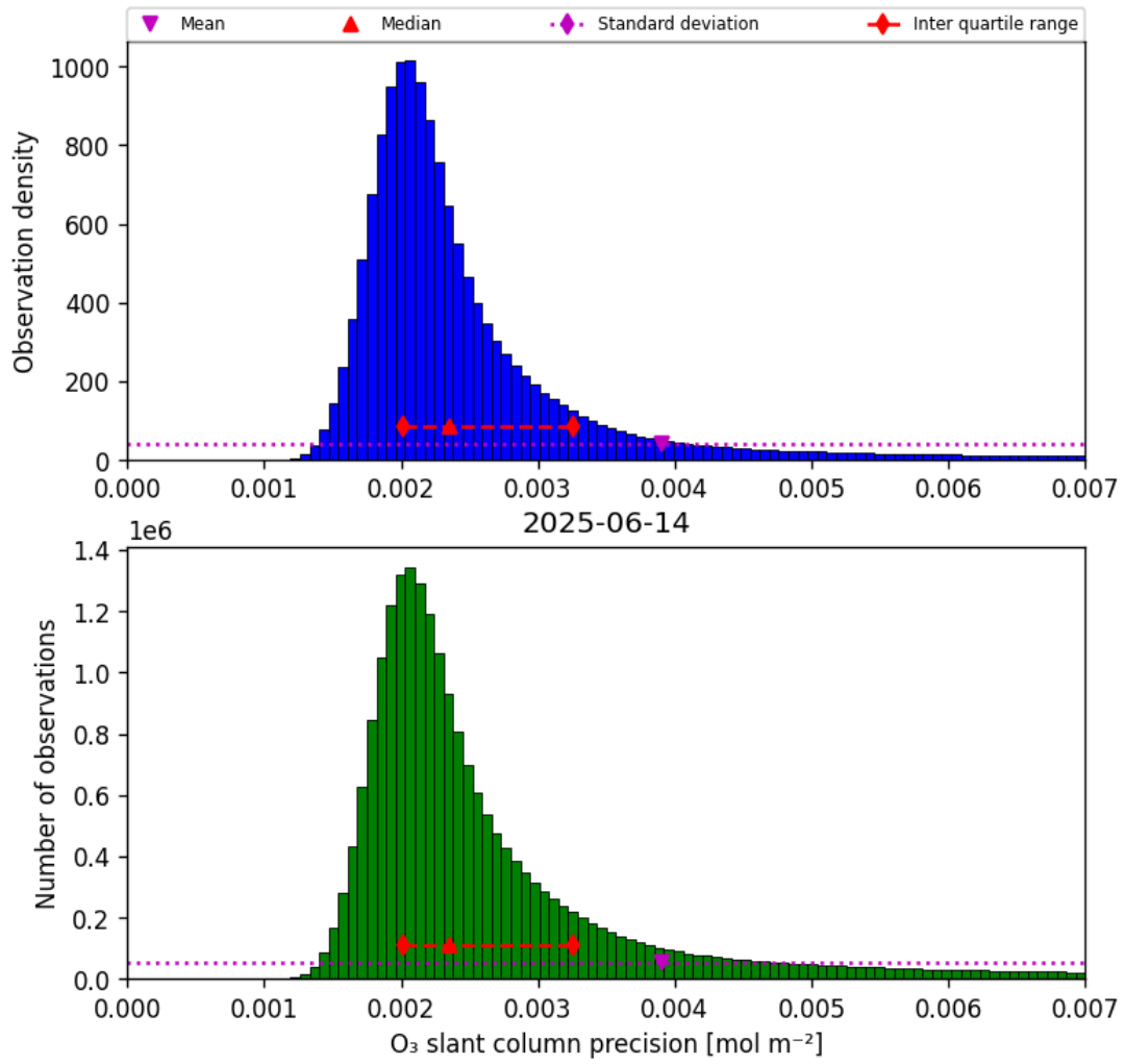
Figure 32: Histogram of "O 3 slant column precision" for 2025-06-14 to 2025-06-14
