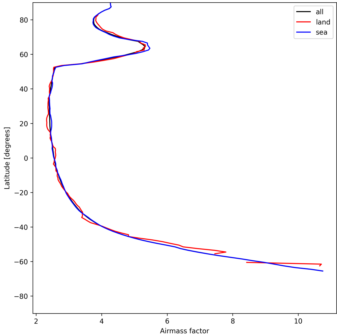
Figure 25: Zonal average of “Airmass factor” for 2025-06-14 to 2025-06-14.
