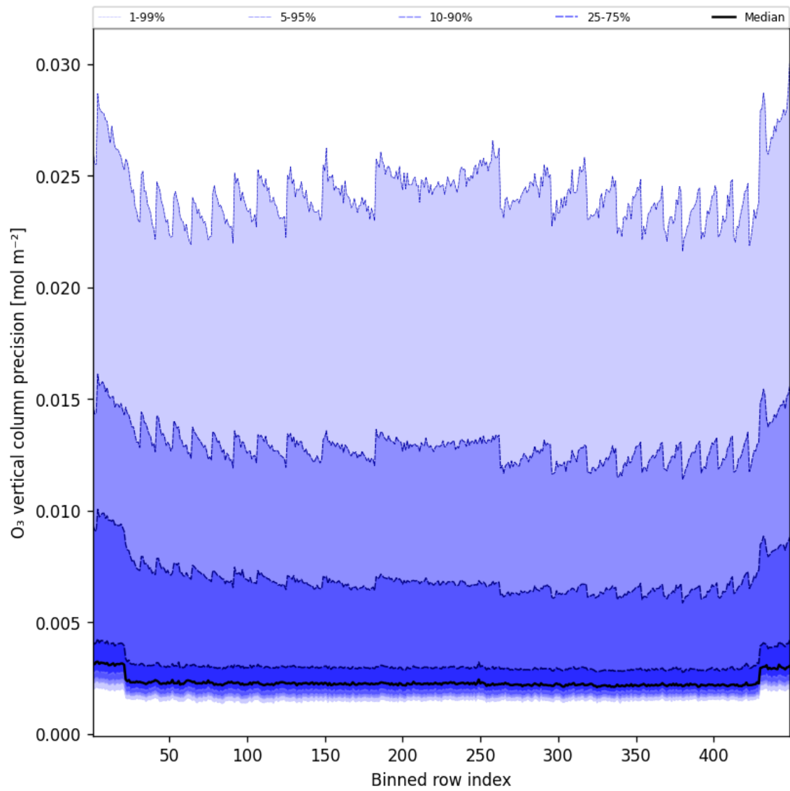
Figure 42: Along track statistics of “O 3 vertical column precision” for 2025-06-14 to 2025-06-14
