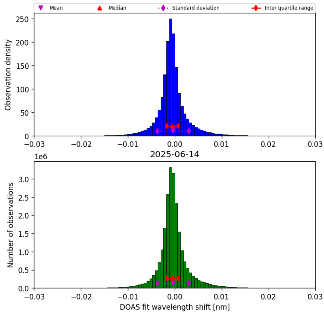
Figure 35: Histogram of “DOAS fit wavelength shift” for 2025-06-14 to 2025-06-14
