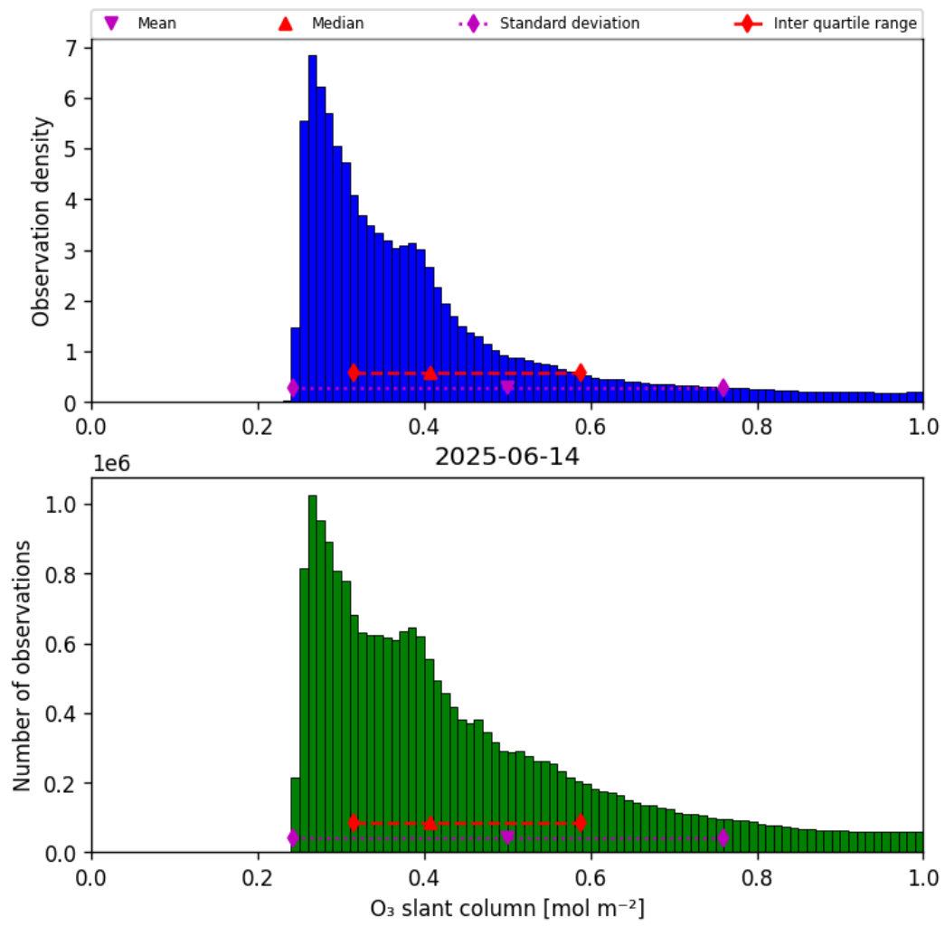
Figure 31: Histogram of “O 3 slant column” for 2025-06-14 to 2025-06-14
