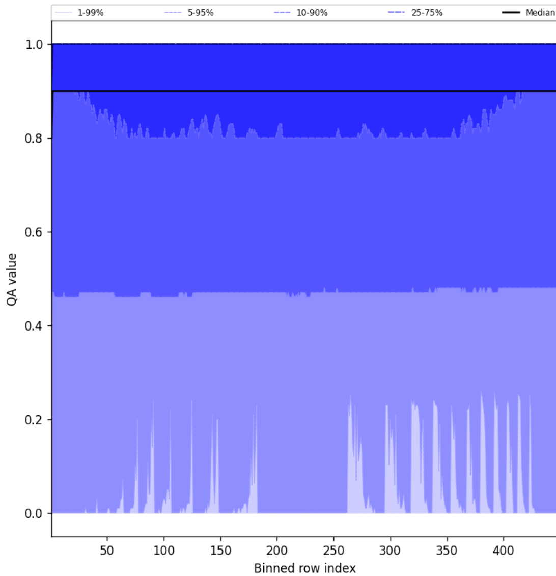
Figure 40: Along track statistics of “QA value” for 2025-06-14 to 2025-06-14
