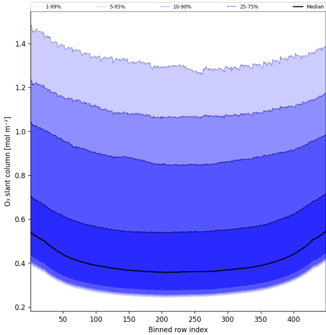
Figure 43: Along track statistics of “O 3 slant column” for 2025-06-14 to 2025-06-14
