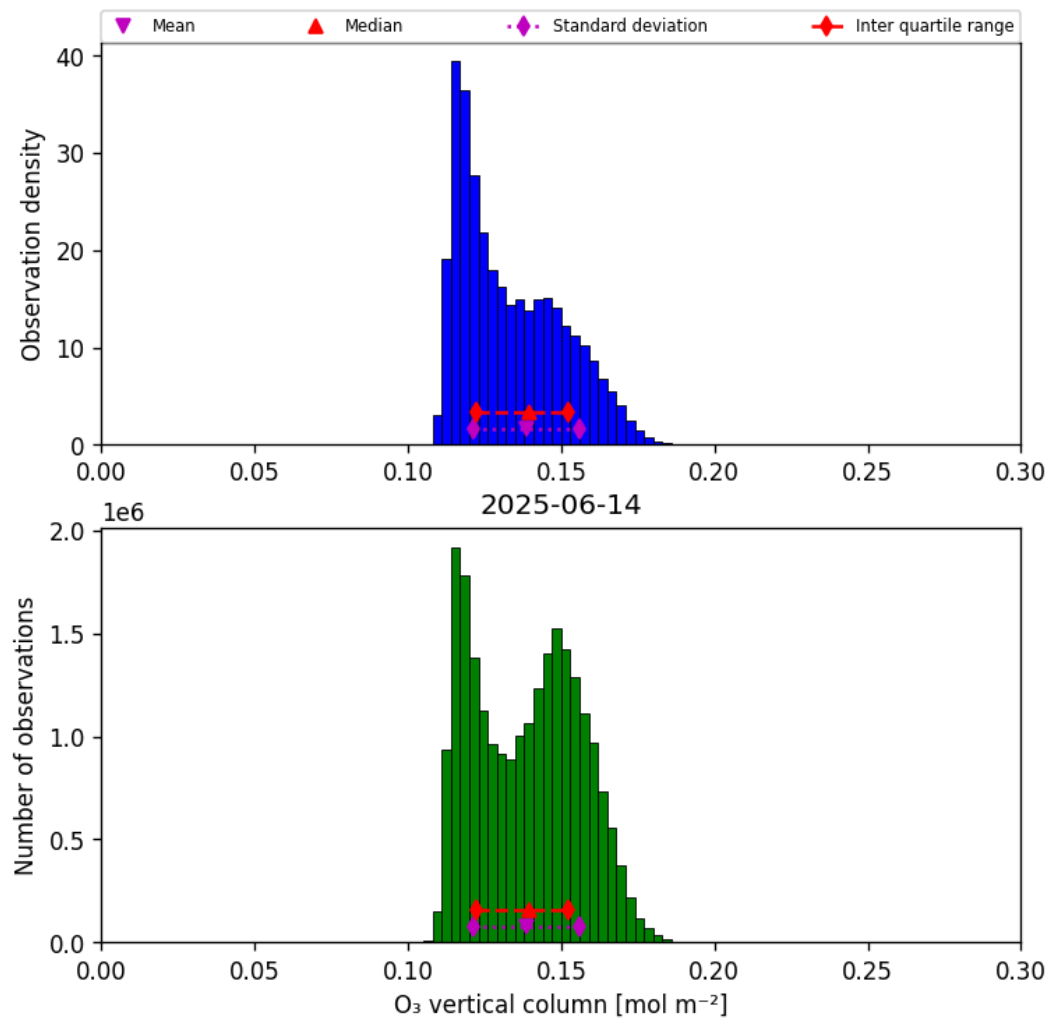
Figure 29: Histogram of “O 3 vertical column” for 2025-06-14 to 2025-06-14
