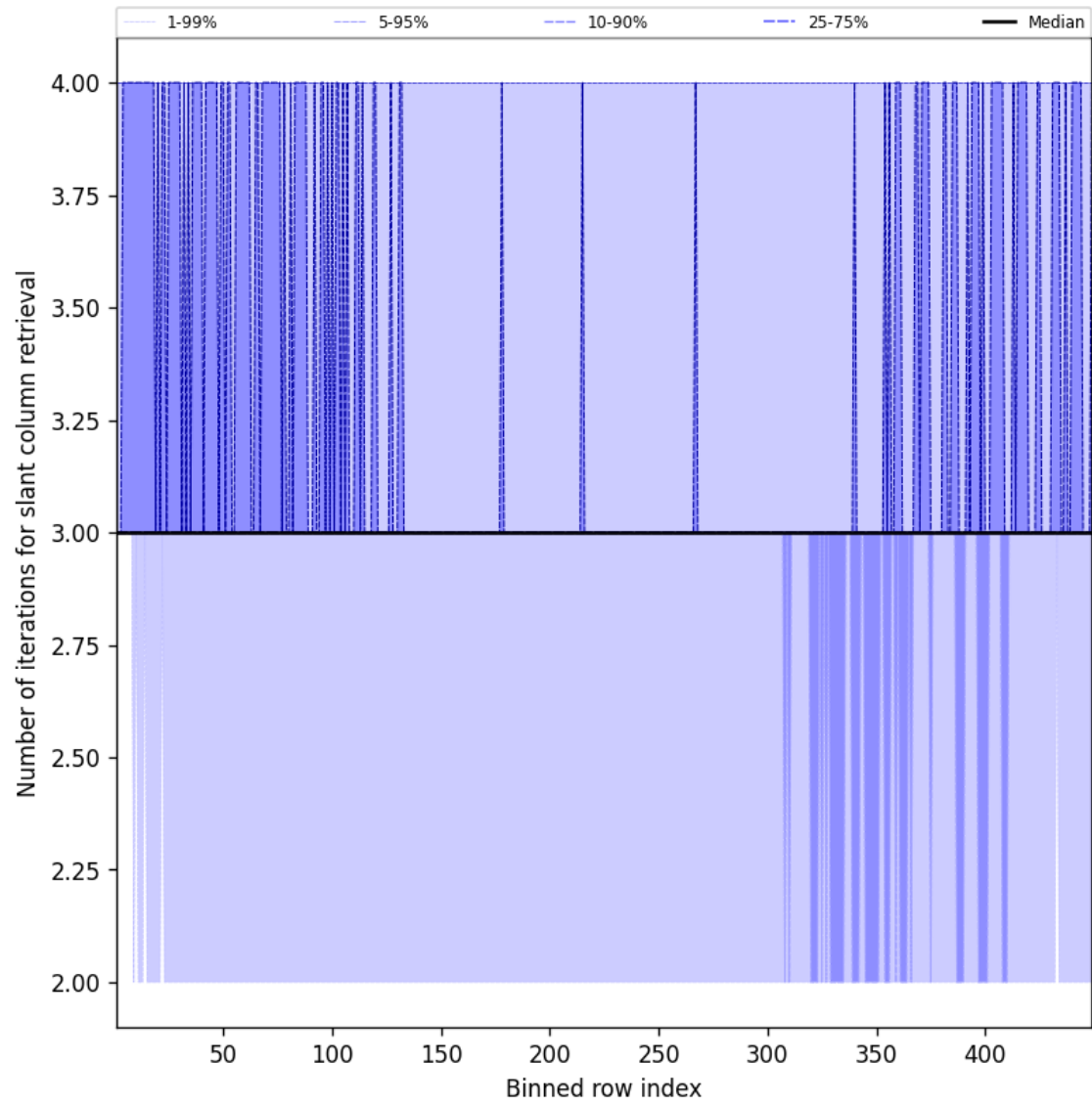
Figure 45: Along track statistics of “Number of iterations for slant column retrieval” for 2025-06-14 to 2025-06-14
