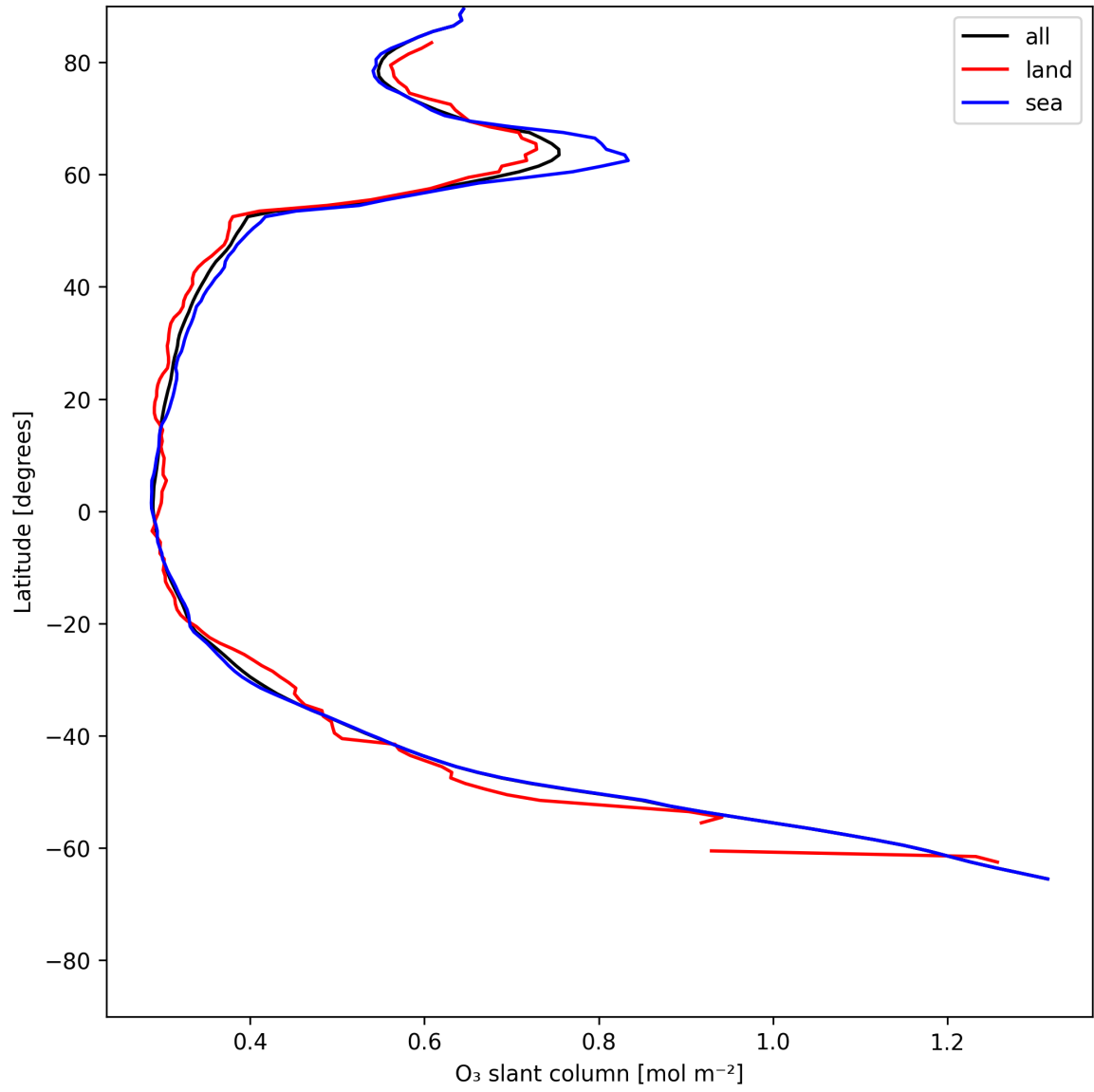
Figure 19: Zonal average of “O 3 slant column” for 2025-06-14 to 2025-06-14.
