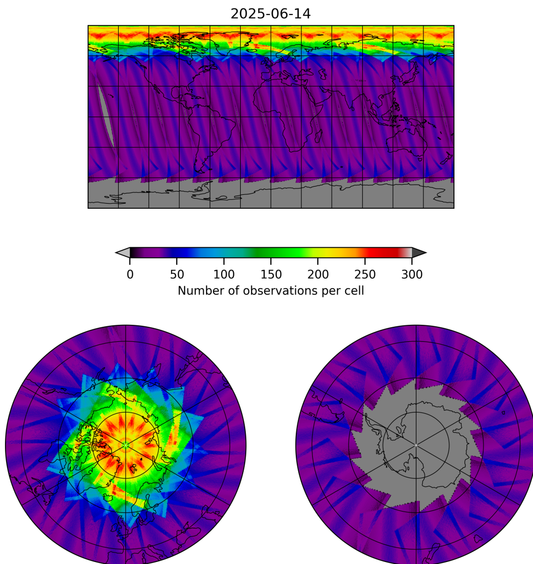
Figure 15: Map of the number of observations for 2025-06-14 to 2025-06-14
