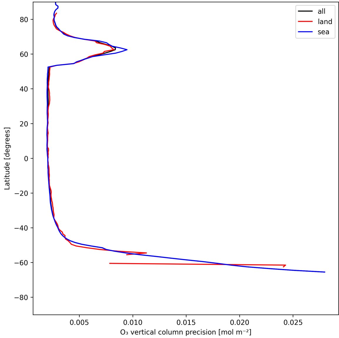
Figure 18: Zonal average of “O 3 vertical column precision” for 2025-06-14 to 2025-06-14.
