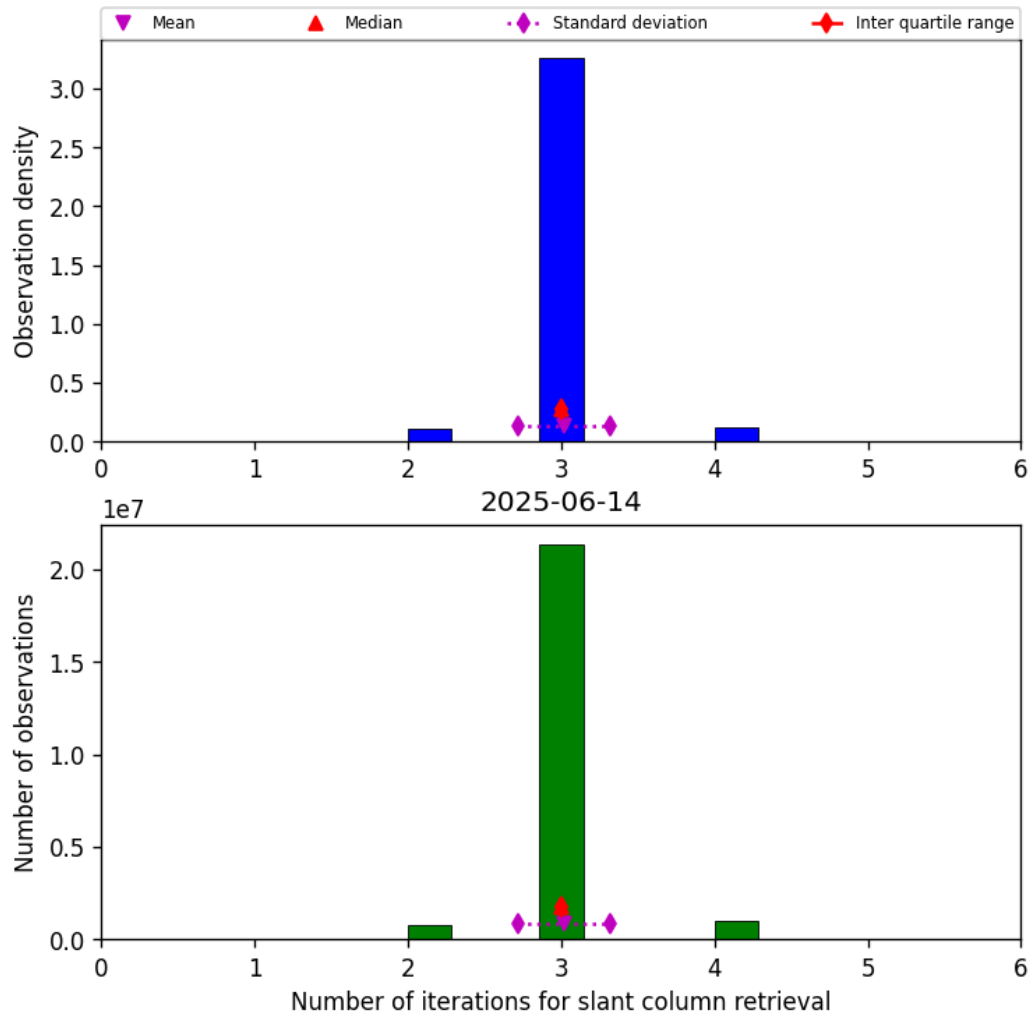
Figure 33: Histogram of “Number of iterations for slant column retrieval” for 2025-06-14 to 2025-06-14
