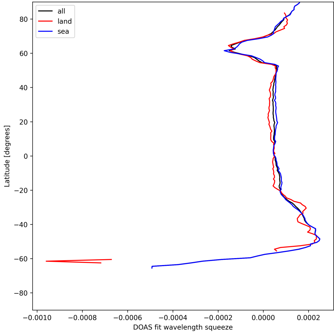
Figure 24: Zonal average of “DOAS fit wavelength squeeze” for 2025-06-14 to 2025-06-14.
