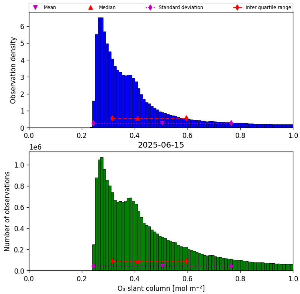
Figure 31: Histogram of “O 3 slant column” for 2025-06-15 to 2025-06-16
