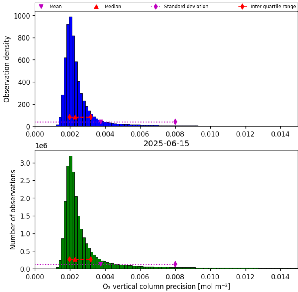
Figure 30: Histogram of “O 3 vertical column precision” for 2025-06-15 to 2025-06-16
