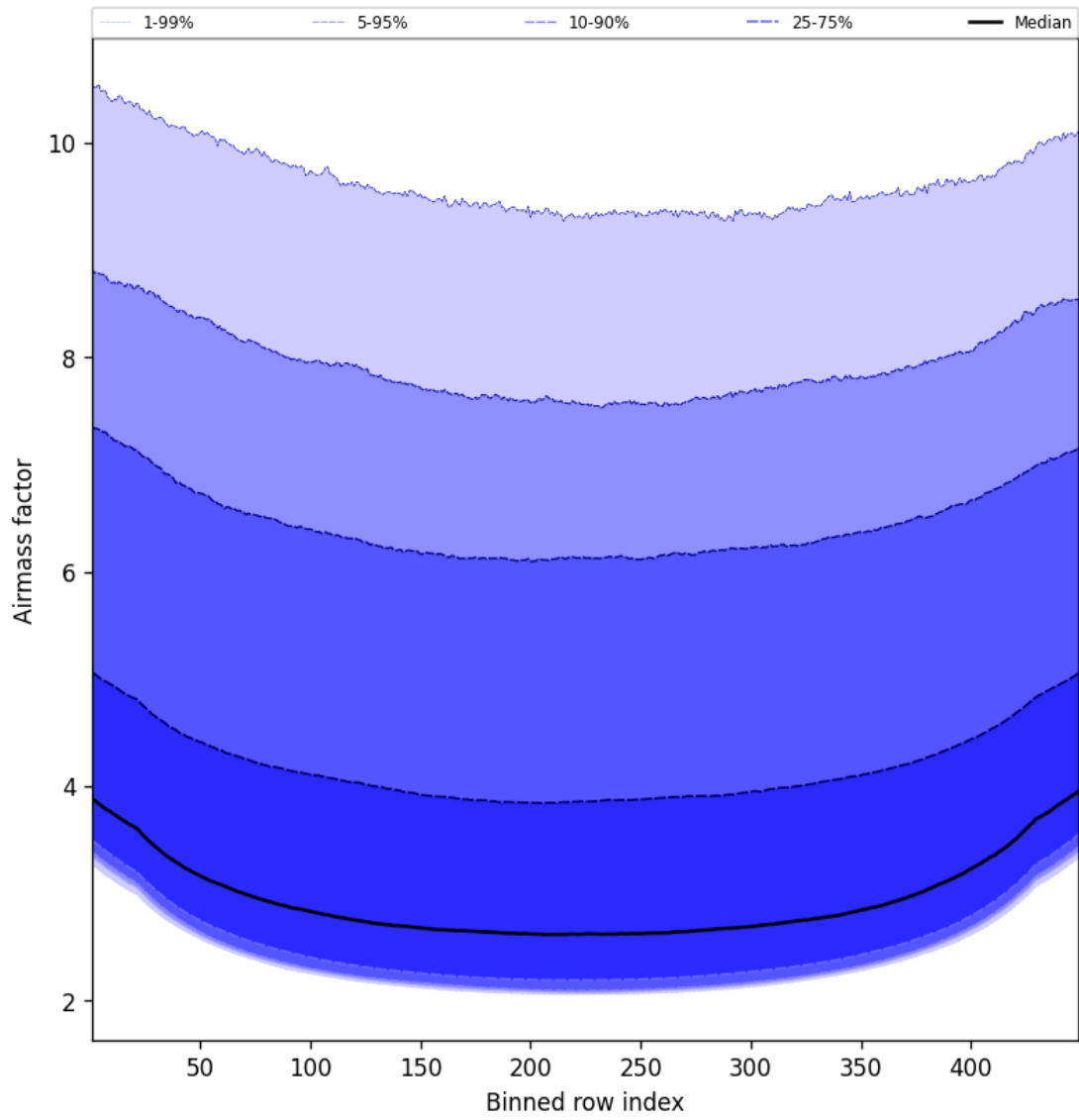
Figure 49: Along track statistics of “Airmass factor” for 2025-06-15 to 2025-06-16
