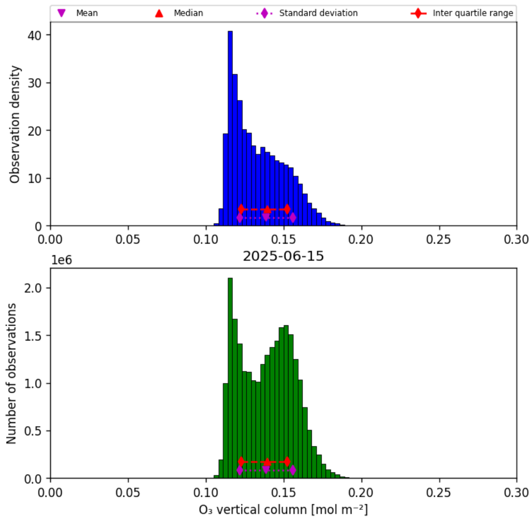
Figure 29: Histogram of “O 3 vertical column” for 2025-06-15 to 2025-06-16
