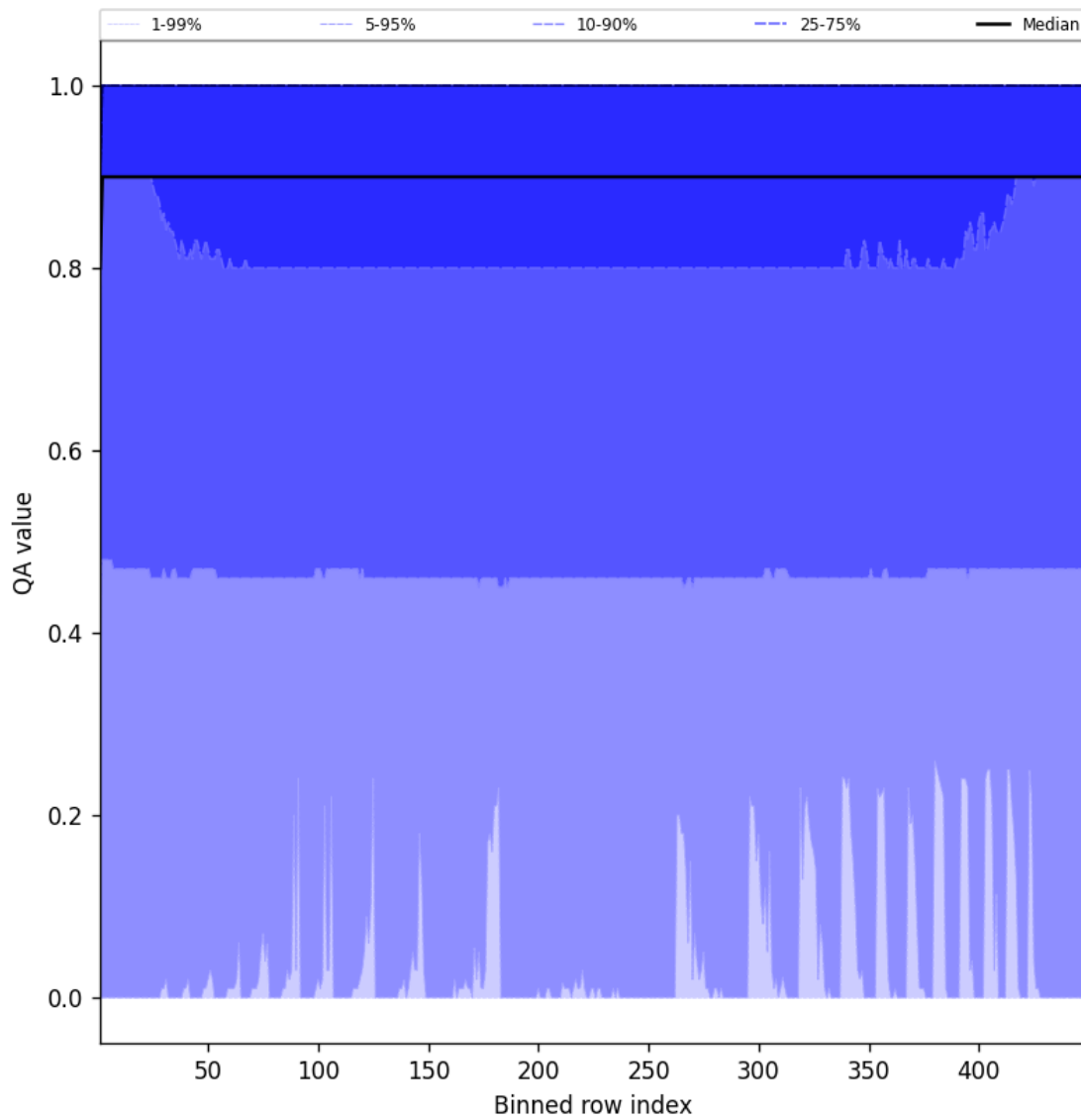
Figure 40: Along track statistics of “QA value” for 2025-06-15 to 2025-06-16
