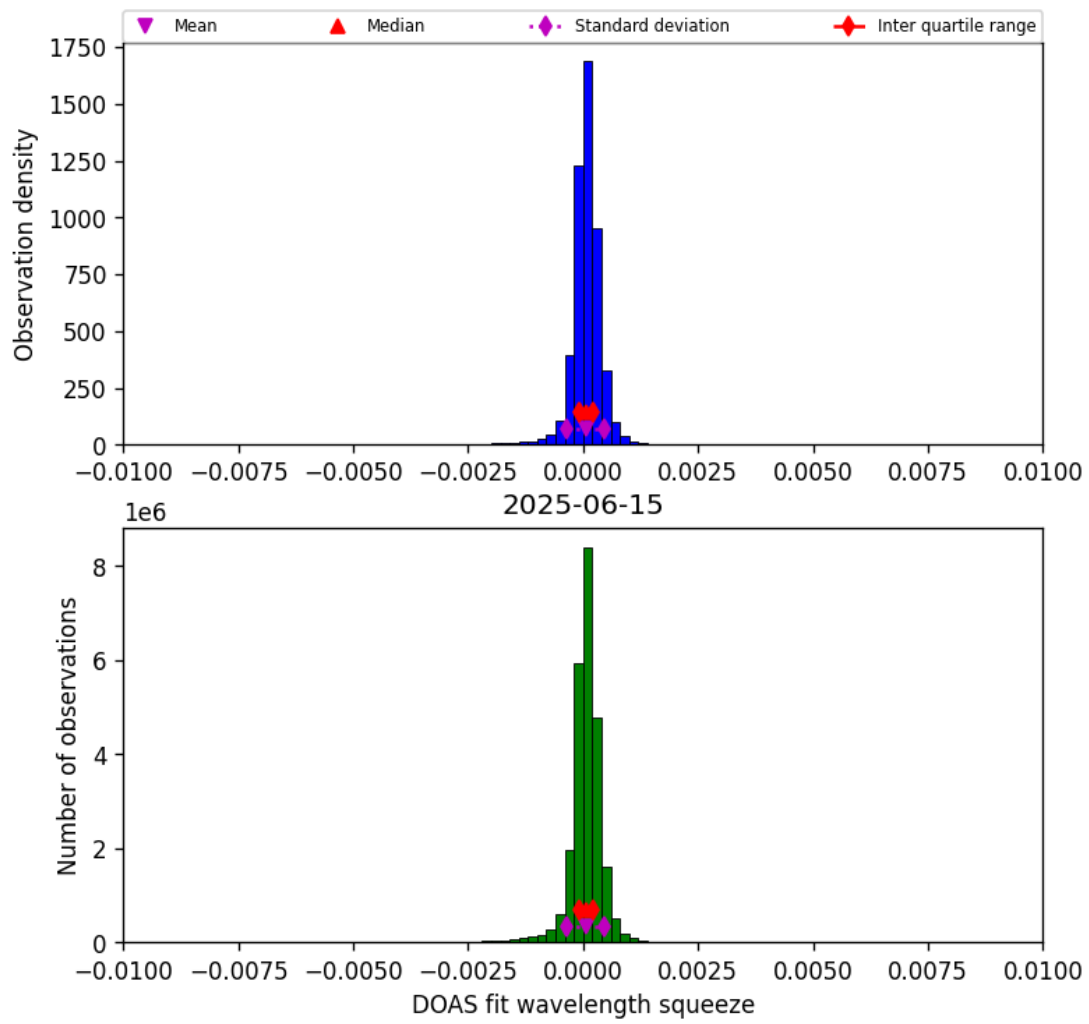
Figure 36: Histogram of “DOAS fit wavelength squeeze” for 2025-06-15 to 2025-06-16
