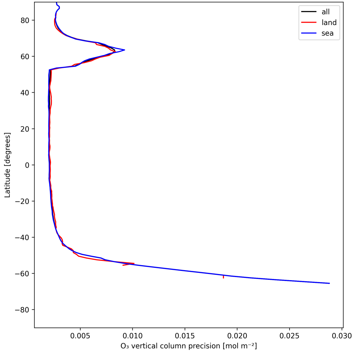
Figure 18: Zonal average of "O 3 vertical column precision" for 2025-06-15 to 2025-06-16.
