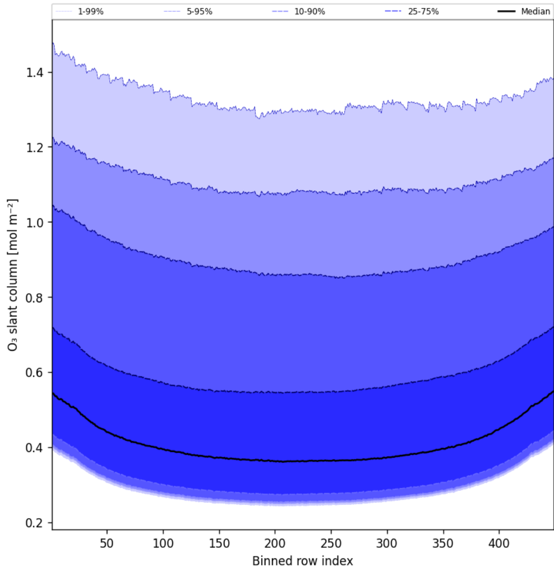
Figure 43: Along track statistics of “O 3 slant column” for 2025-06-15 to 2025-06-16
