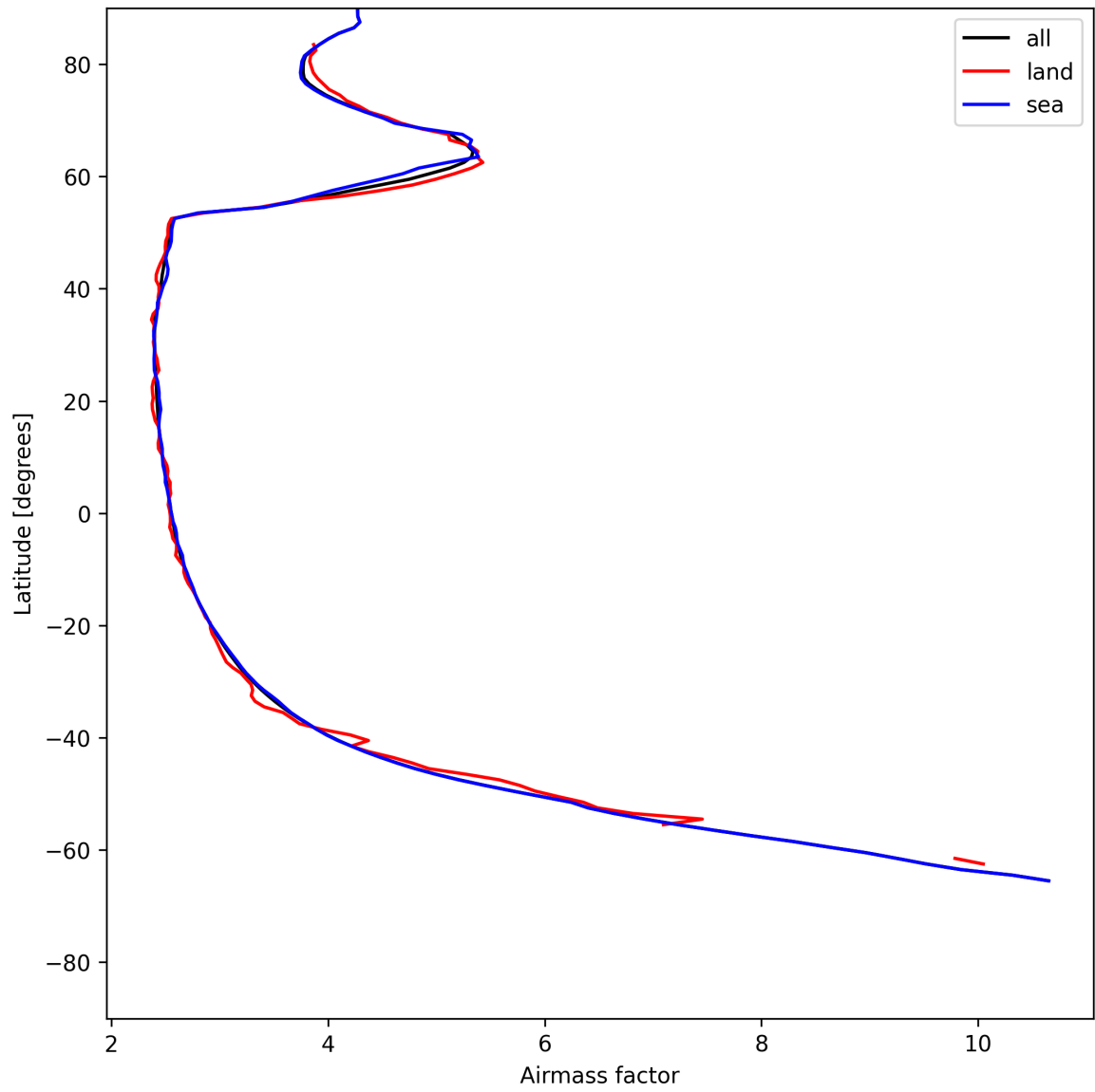
Figure 25: Zonal average of “Airmass factor” for 2025-06-15 to 2025-06-16.
