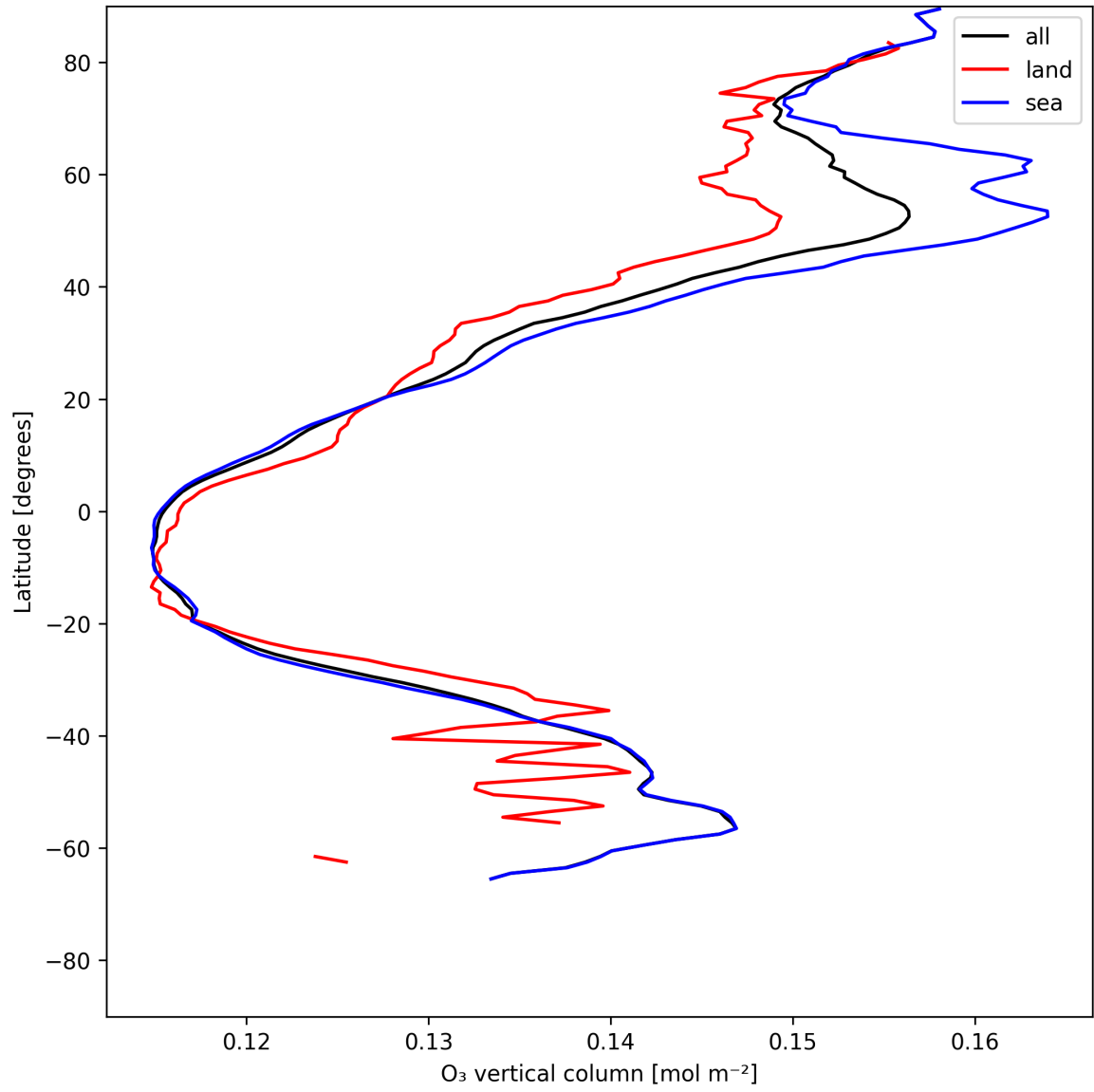
Figure 17: Zonal average of “O 3 vertical column” for 2025-06-15 to 2025-06-16.
