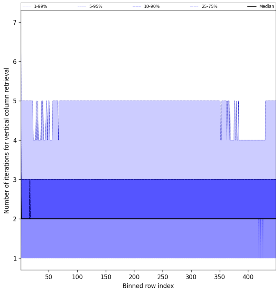
Figure 51: Along track statistics of “Number of iterations for vertical column retrieval” for 2025-06-15 to 2025-06-16
