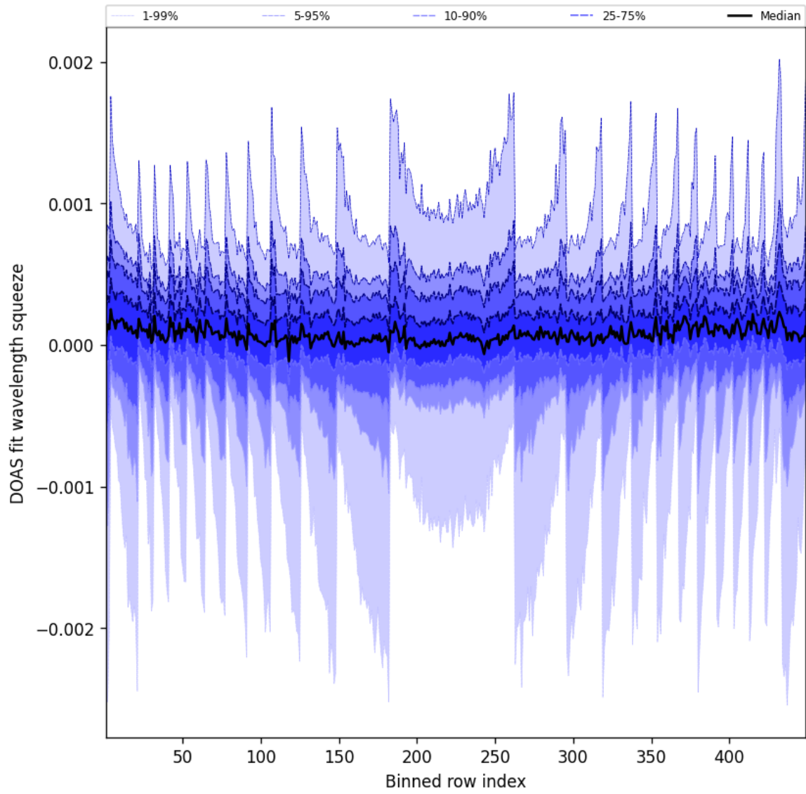
Figure 48: Along track statistics of “DOAS fit wavelength squeeze” for 2025-06-15 to 2025-06-16
