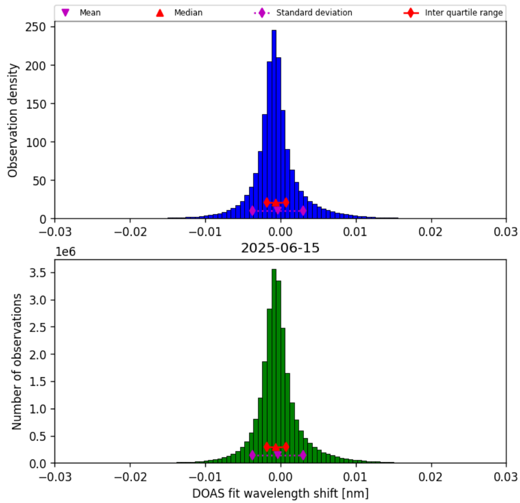
Figure 35: Histogram of “DOAS fit wavelength shift” for 2025-06-15 to 2025-06-16
