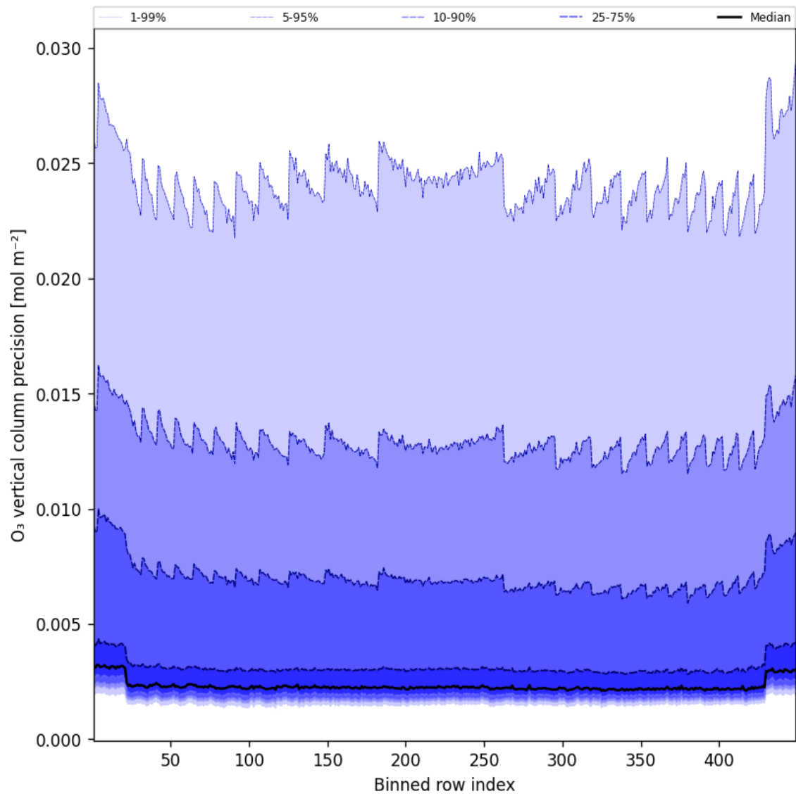
Figure 42: Along track statistics of “O 3 vertical column precision” for 2025-06-15 to 2025-06-16
