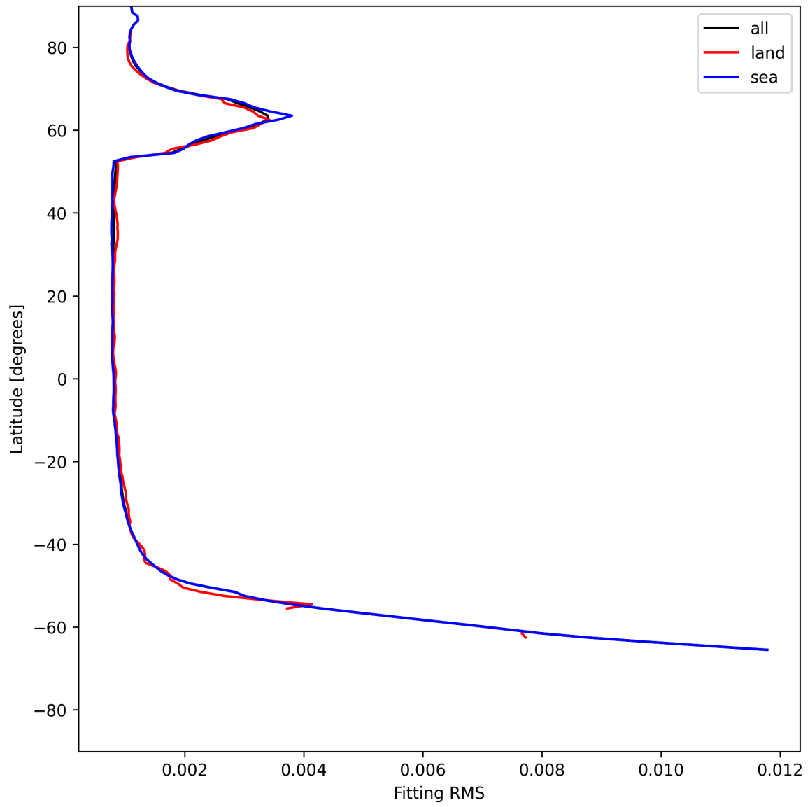
Figure 22: Zonal average of “Fitting RMS” for 2025-06-15 to 2025-06-16.
