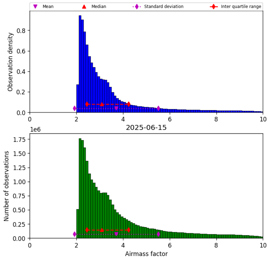
Figure 37: Histogram of “Airmass factor” for 2025-06-15 to 2025-06-16
