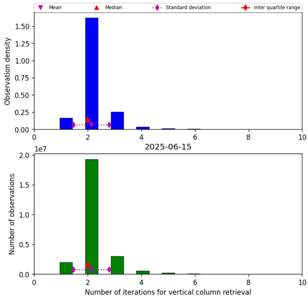
Figure 39: Histogram of “Number of iterations for vertical column retrieval” for 2025-06-15 to 2025-06-16
