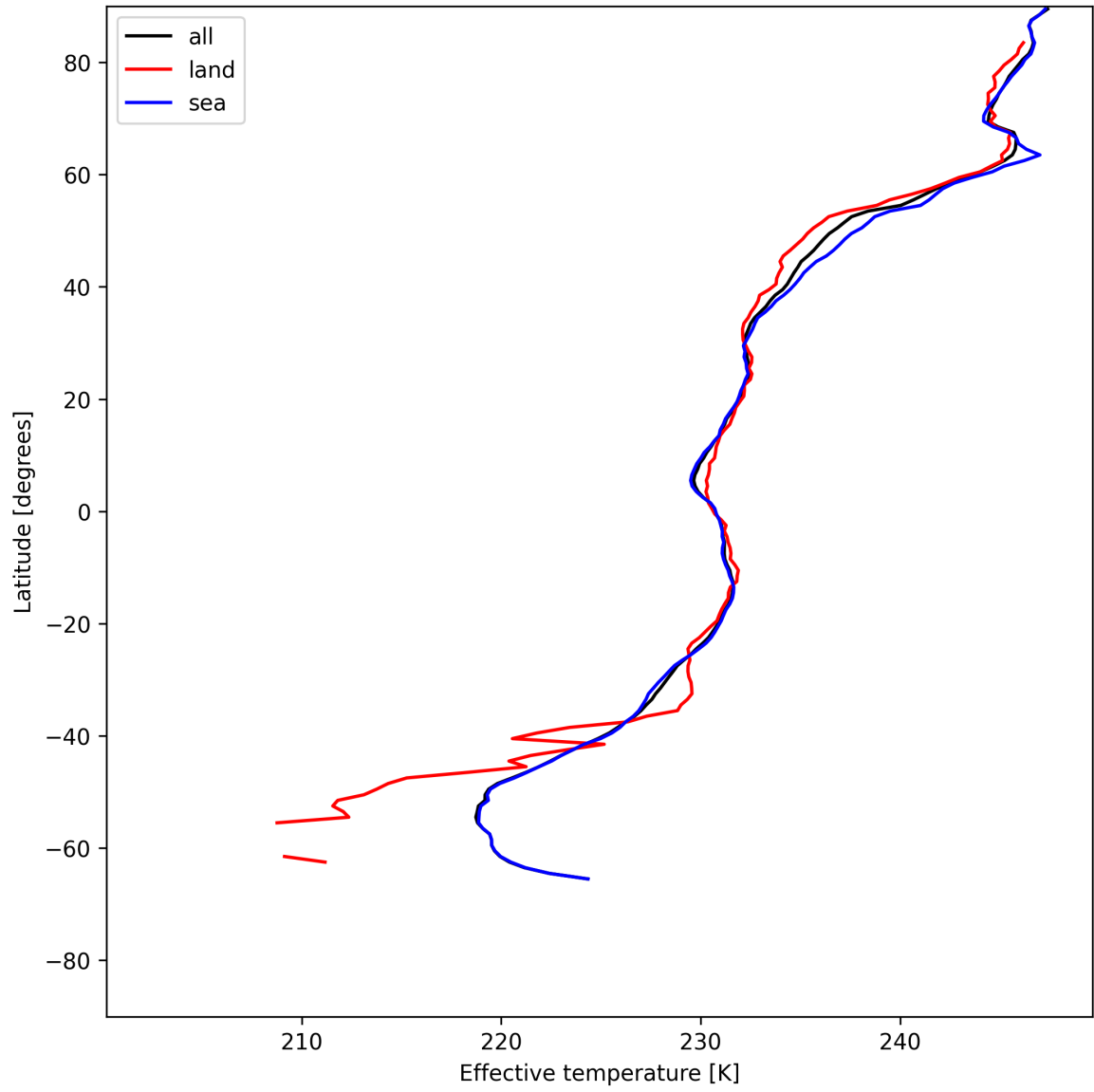
Figure 26: Zonal average of “Effective temperature” for 2025-06-15 to 2025-06-16.
