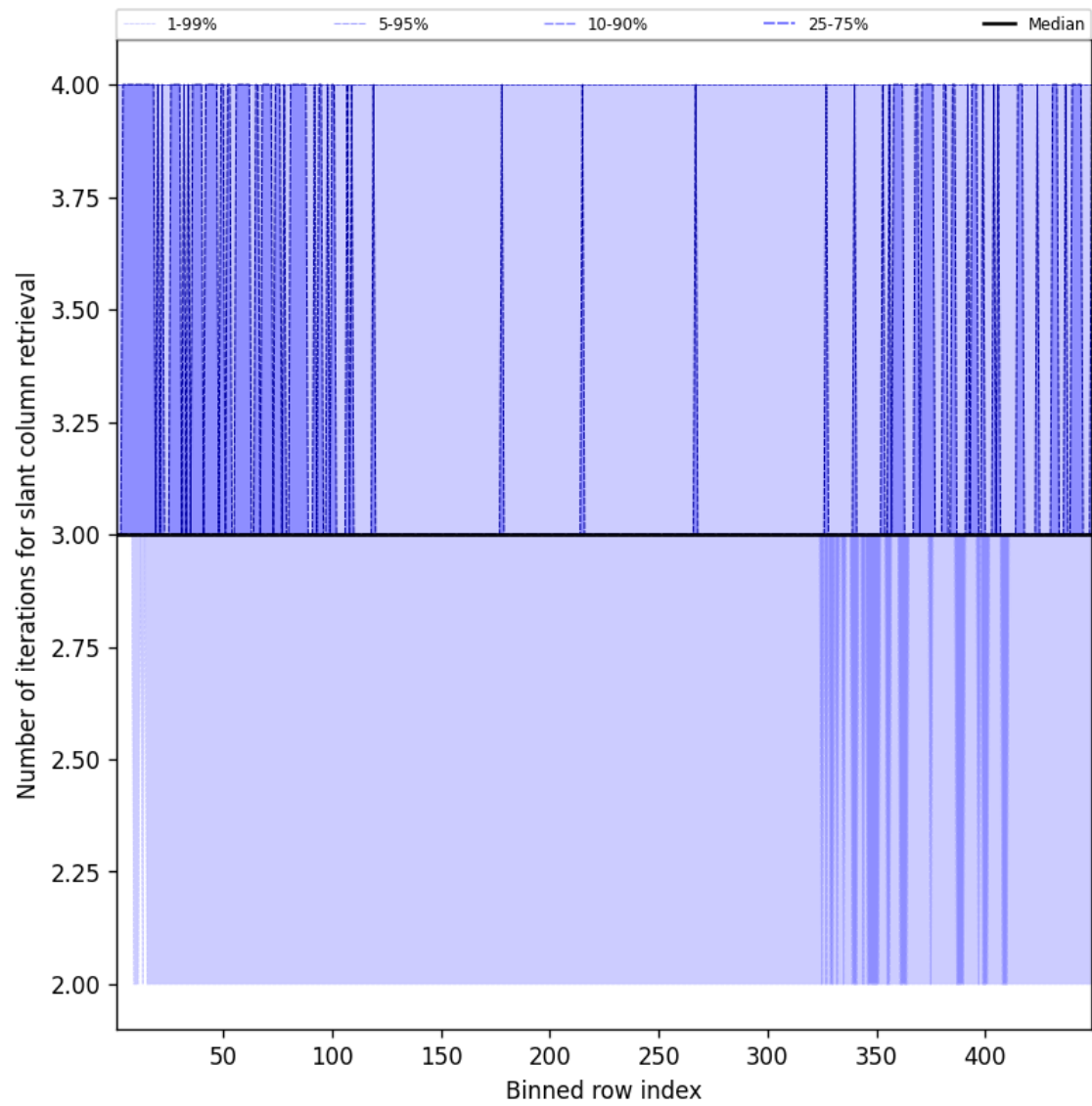
Figure 45: Along track statistics of “Number of iterations for slant column retrieval” for 2025-06-15 to 2025-06-16
