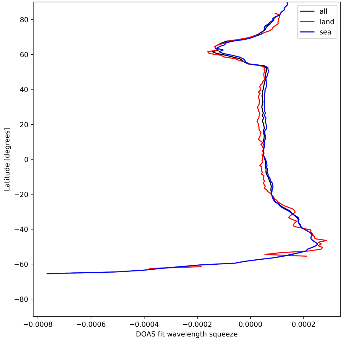
Figure 24: Zonal average of “DOAS fit wavelength squeeze” for 2025-06-15 to 2025-06-16.
