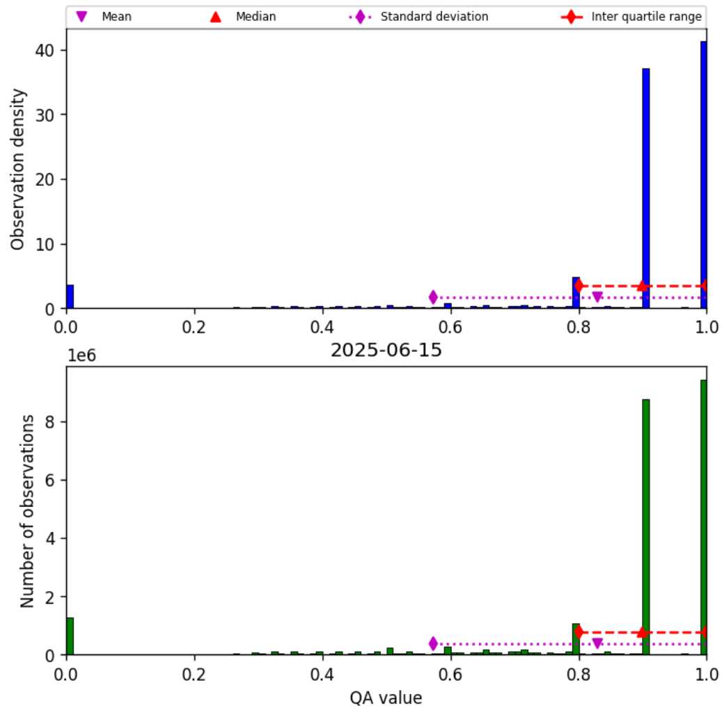
Figure 28: Histogram of “QA value” for 2025-06-15 to 2025-06-16
