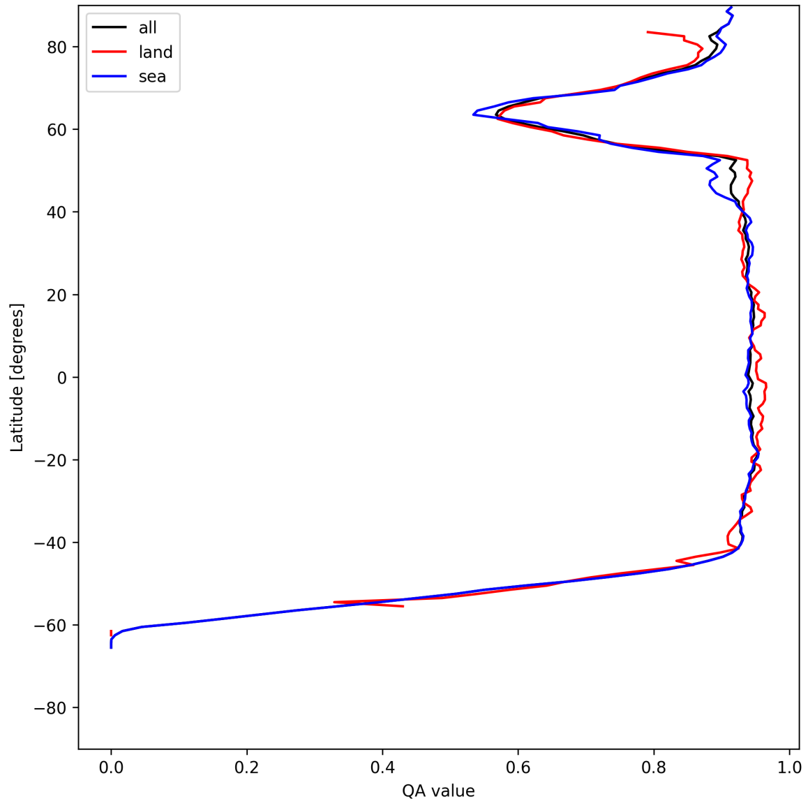
Figure 16: Zonal average of “QA value” for 2025-06-15 to 2025-06-16.
