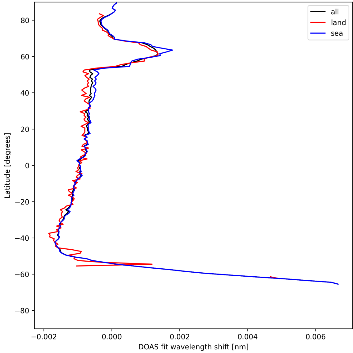
Figure 23: Zonal average of “DOAS fit wavelength shift” for 2025-06-15 to 2025-06-16.
