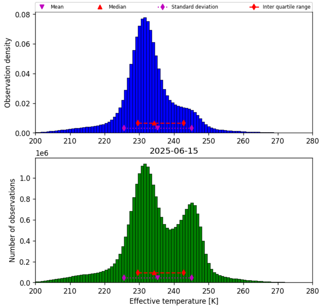
Figure 38: Histogram of “Effective temperature” for 2025-06-15 to 2025-06-16
