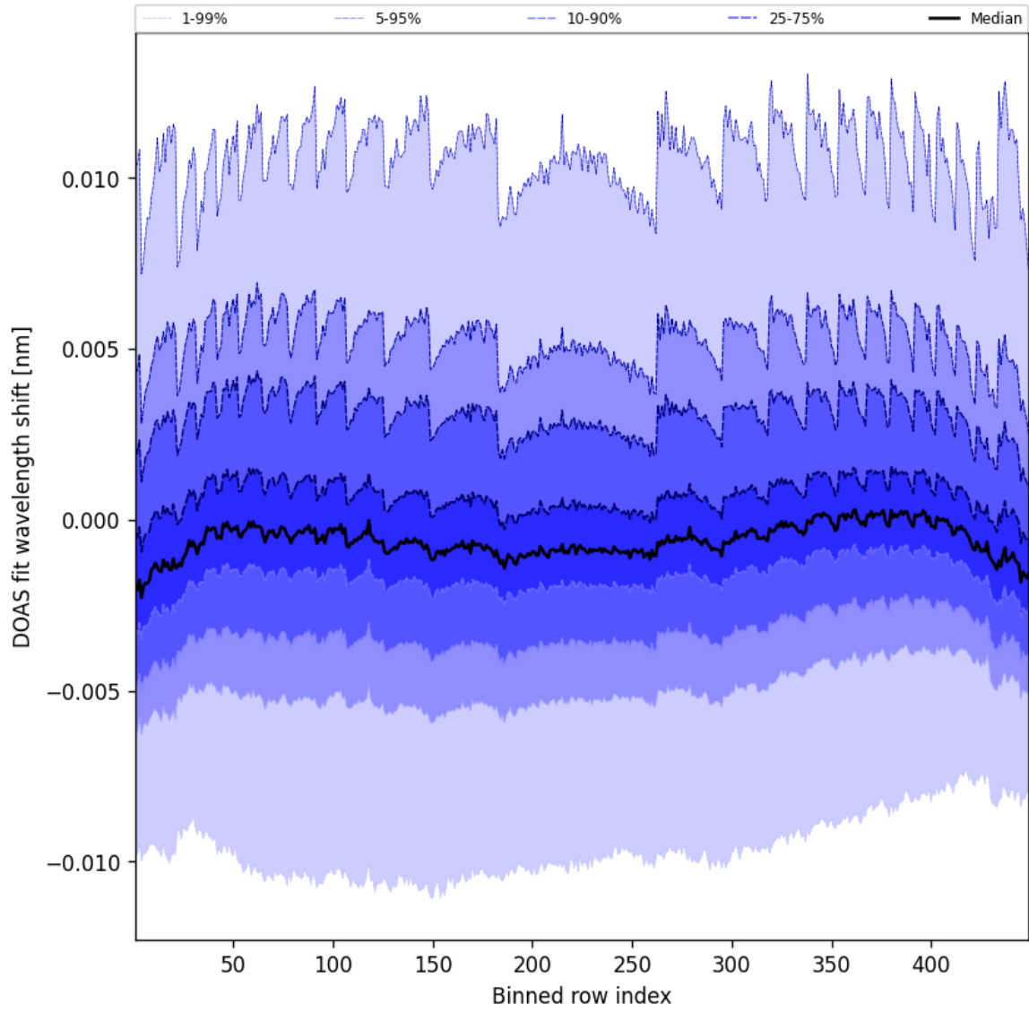
Figure 47: Along track statistics of “DOAS fit wavelength shift” for 2025-06-15 to 2025-06-16
