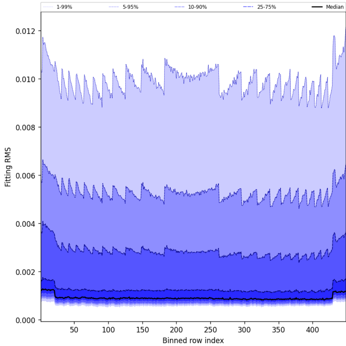
Figure 46: Along track statistics of “Fitting RMS” for 2025-06-15 to 2025-06-16
