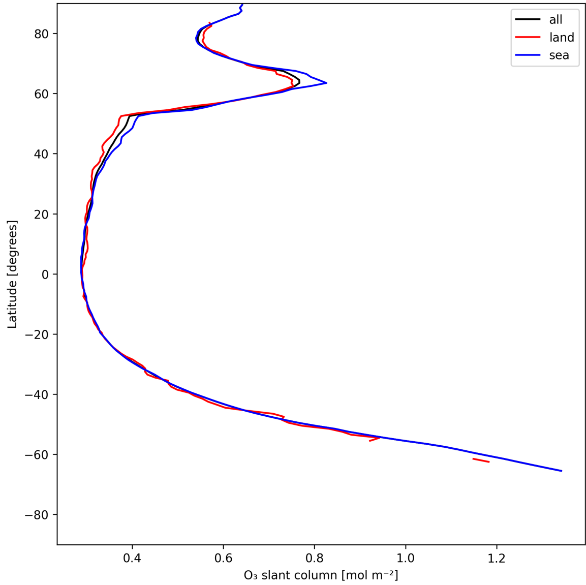
Figure 19: Zonal average of “O 3 slant column” for 2025-06-15 to 2025-06-16.
