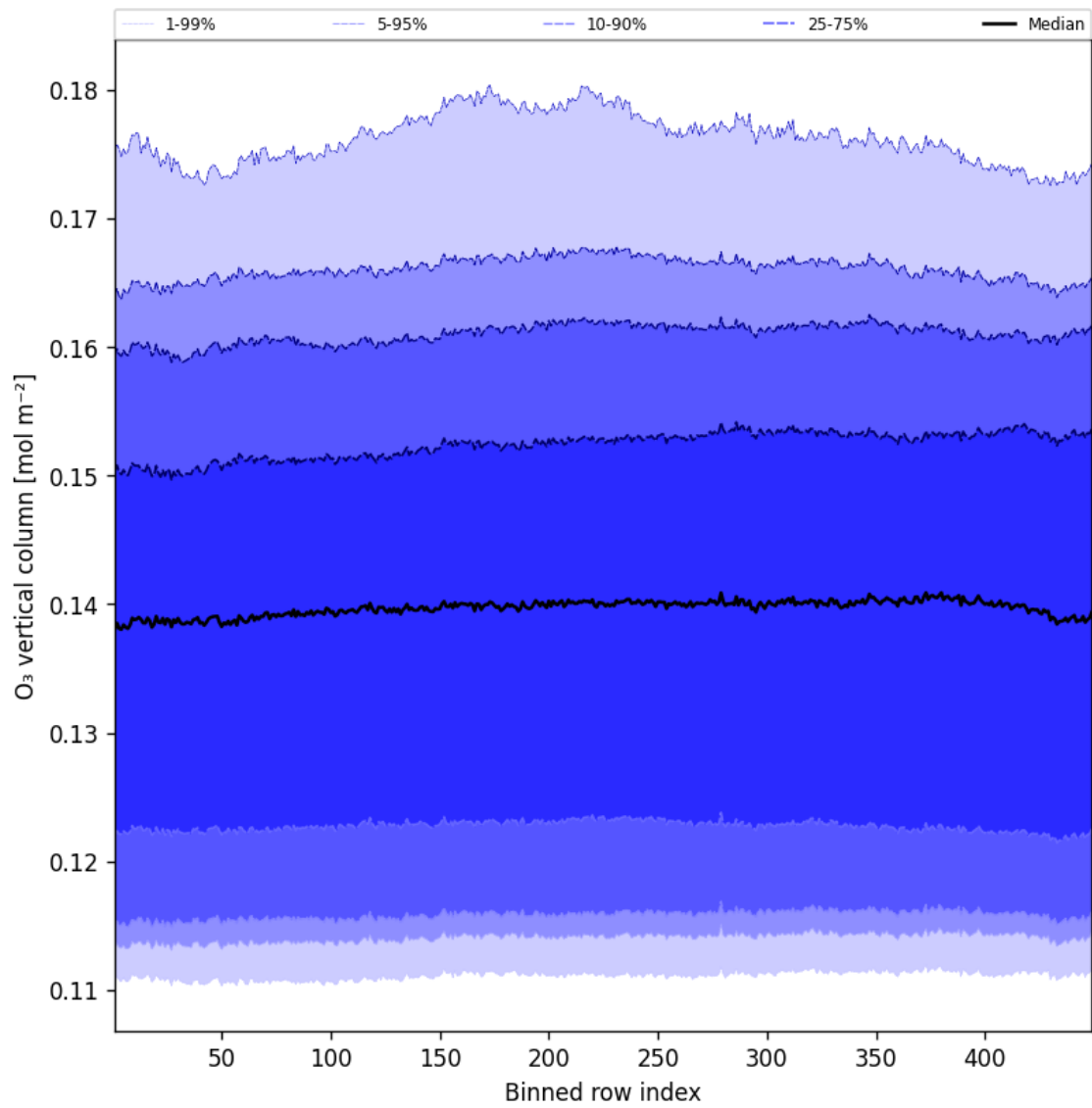
Figure 41: Along track statistics of “O 3 vertical column” for 2025-06-15 to 2025-06-16
