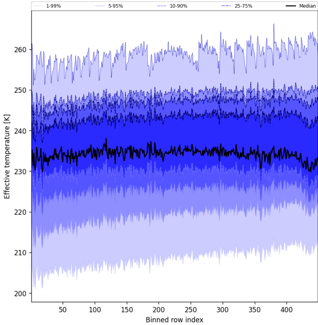
Figure 50: Along track statistics of “Effective temperature” for 2025-06-15 to 2025-06-16
