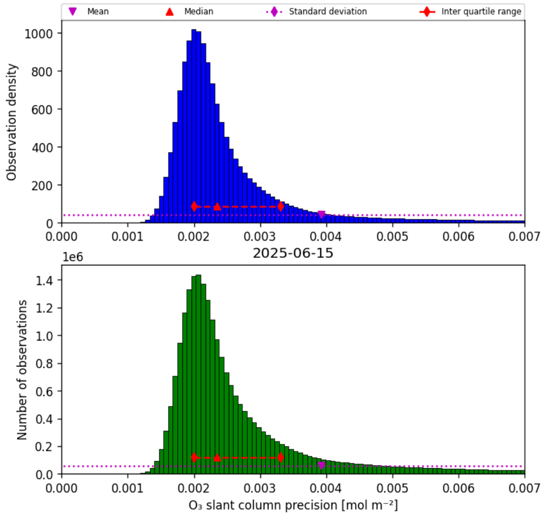
Figure 32: Histogram of “O 3 slant column precision” for 2025-06-15 to 2025-06-16
