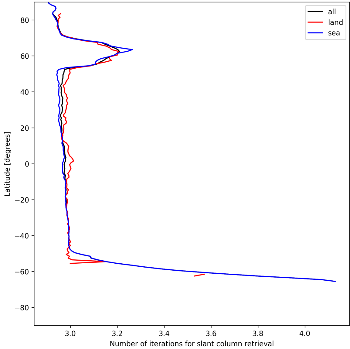
Figure 21: Zonal average of “Number of iterations for slant column retrieval” for 2025-06-15 to 2025-06-16.
