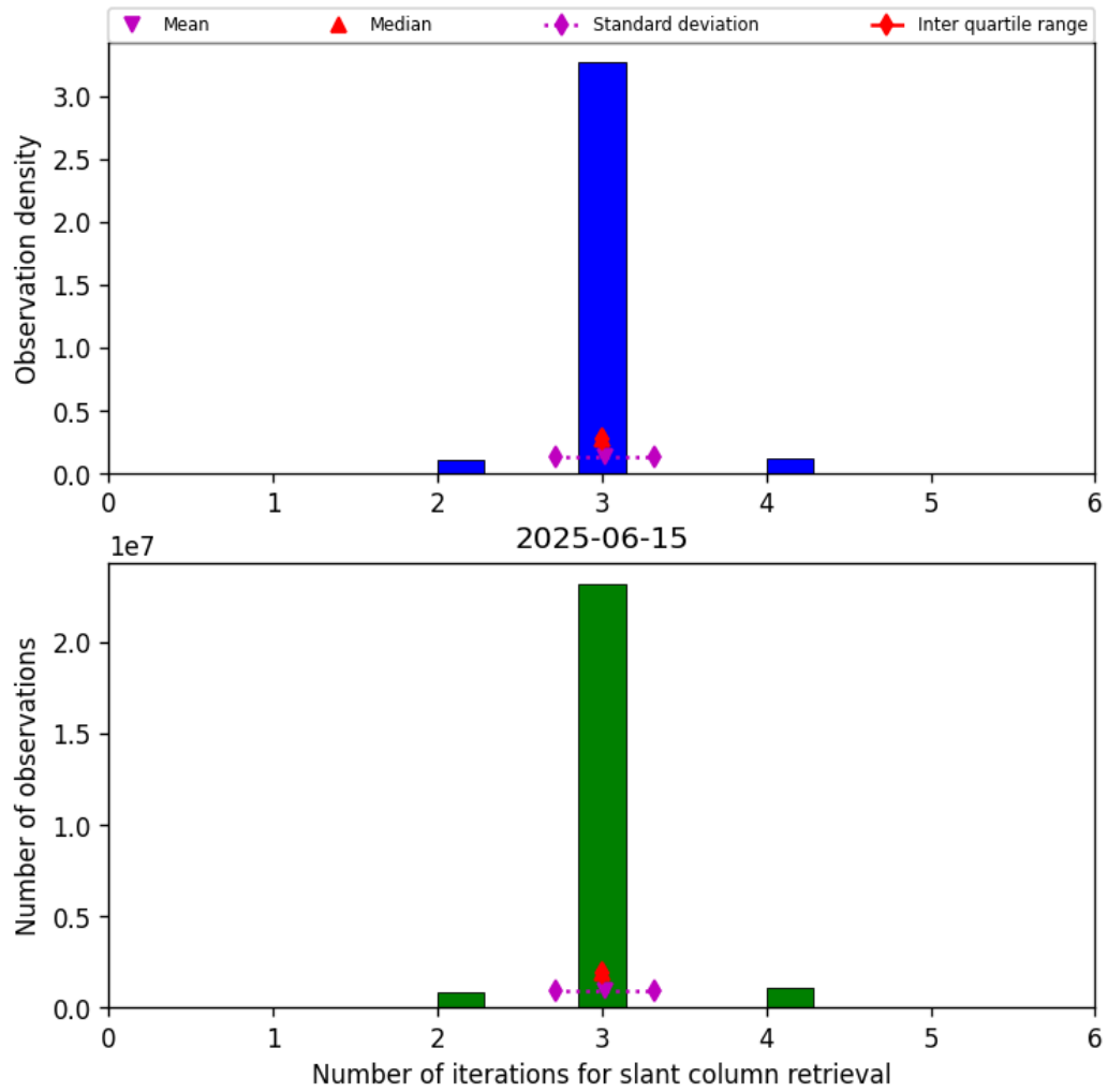
Figure 33: Histogram of “Number of iterations for slant column retrieval” for 2025-06-15 to 2025-06-16
