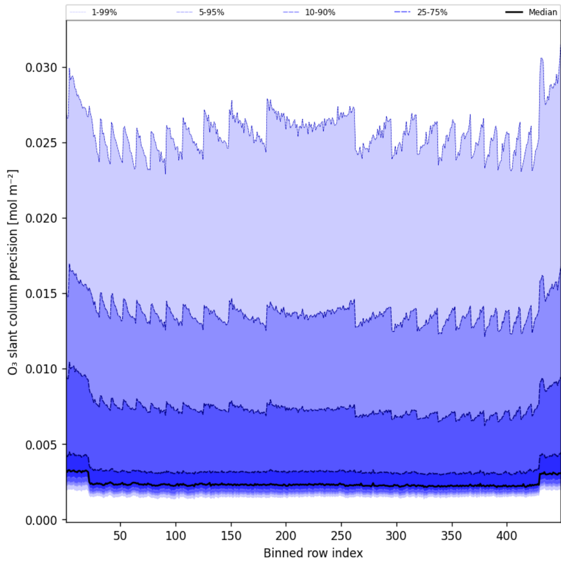
Figure 44: Along track statistics of “O 3 slant column precision” for 2025-06-15 to 2025-06-16
