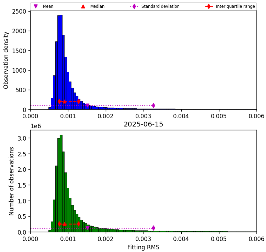
Figure 34: Histogram of “Fitting RMS” for 2025-06-15 to 2025-06-16
