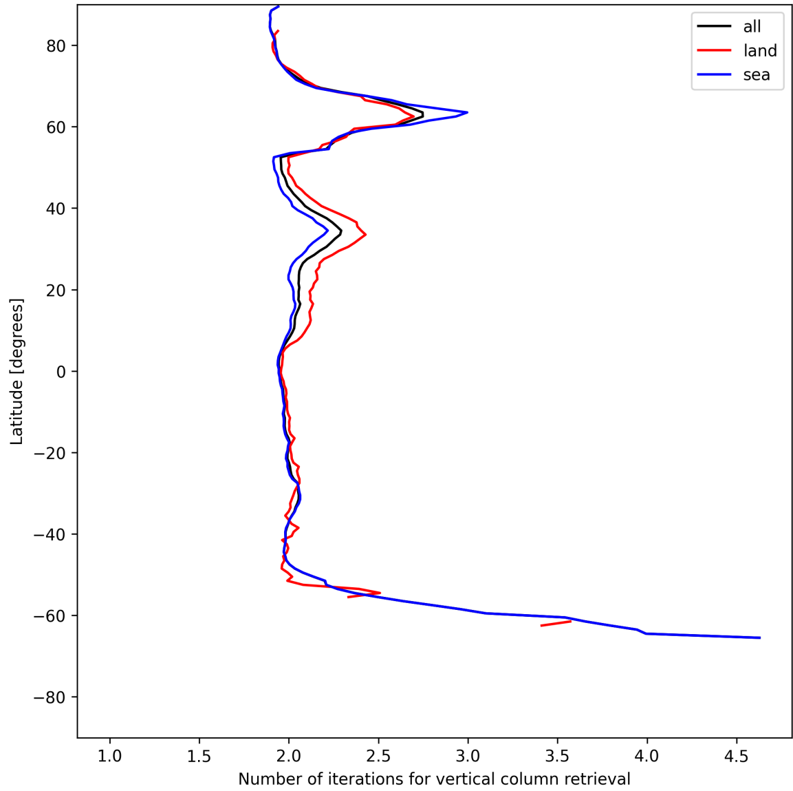
Figure 27: Zonal average of “Number of iterations for vertical column retrieval” for 2025-06-15 to 2025-06-16.
