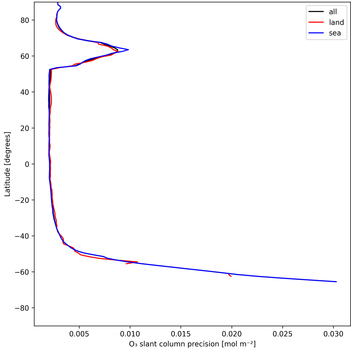
Figure 20: Zonal average of “O 3 slant column precision” for 2025-06-15 to 2025-06-16.
