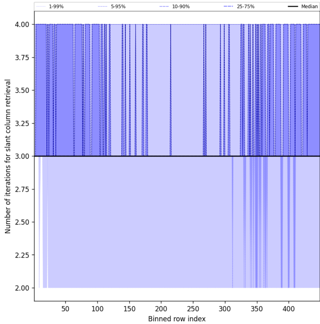
Figure 45: Along track statistics of “Number of iterations for slant column retrieval” for 2025-06-16 to 2025-06-17
