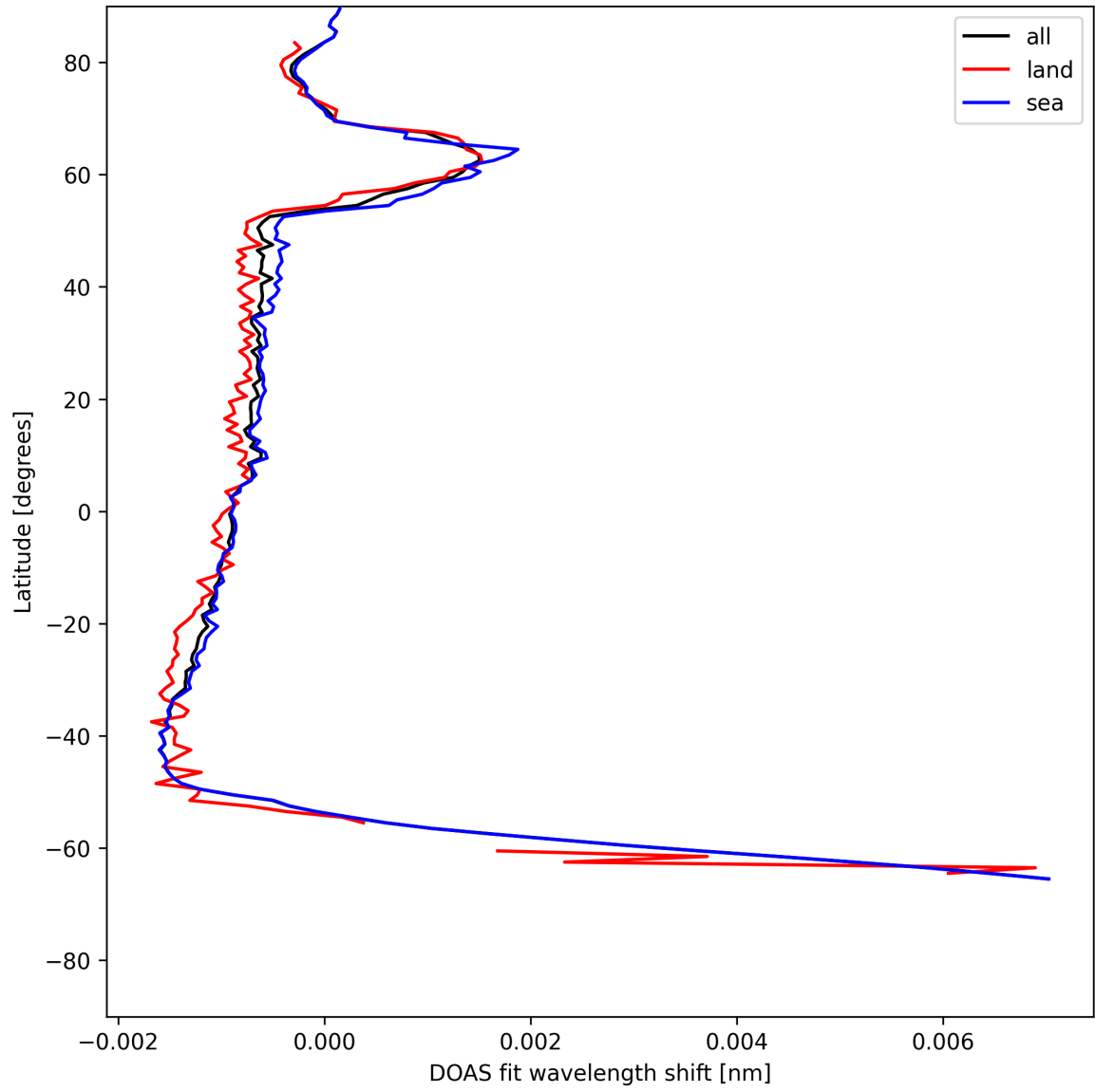
Figure 23: Zonal average of “DOAS fit wavelength shift” for 2025-06-16 to 2025-06-17.
