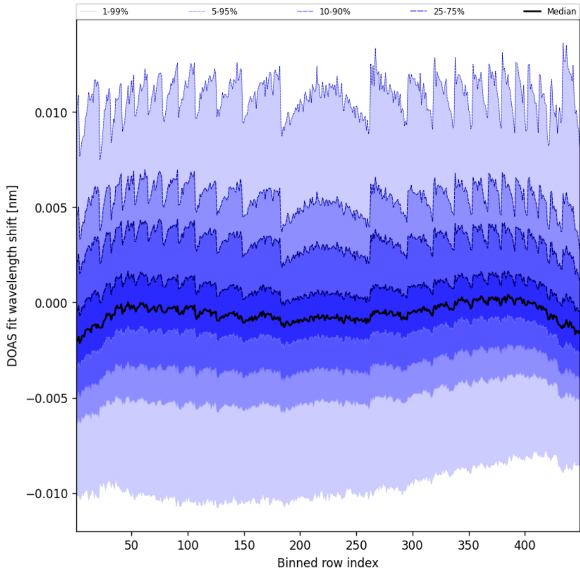
Figure 47: Along track statistics of "DOAS fit wavelength shift" for 2025-06-16 to 2025-06-17
