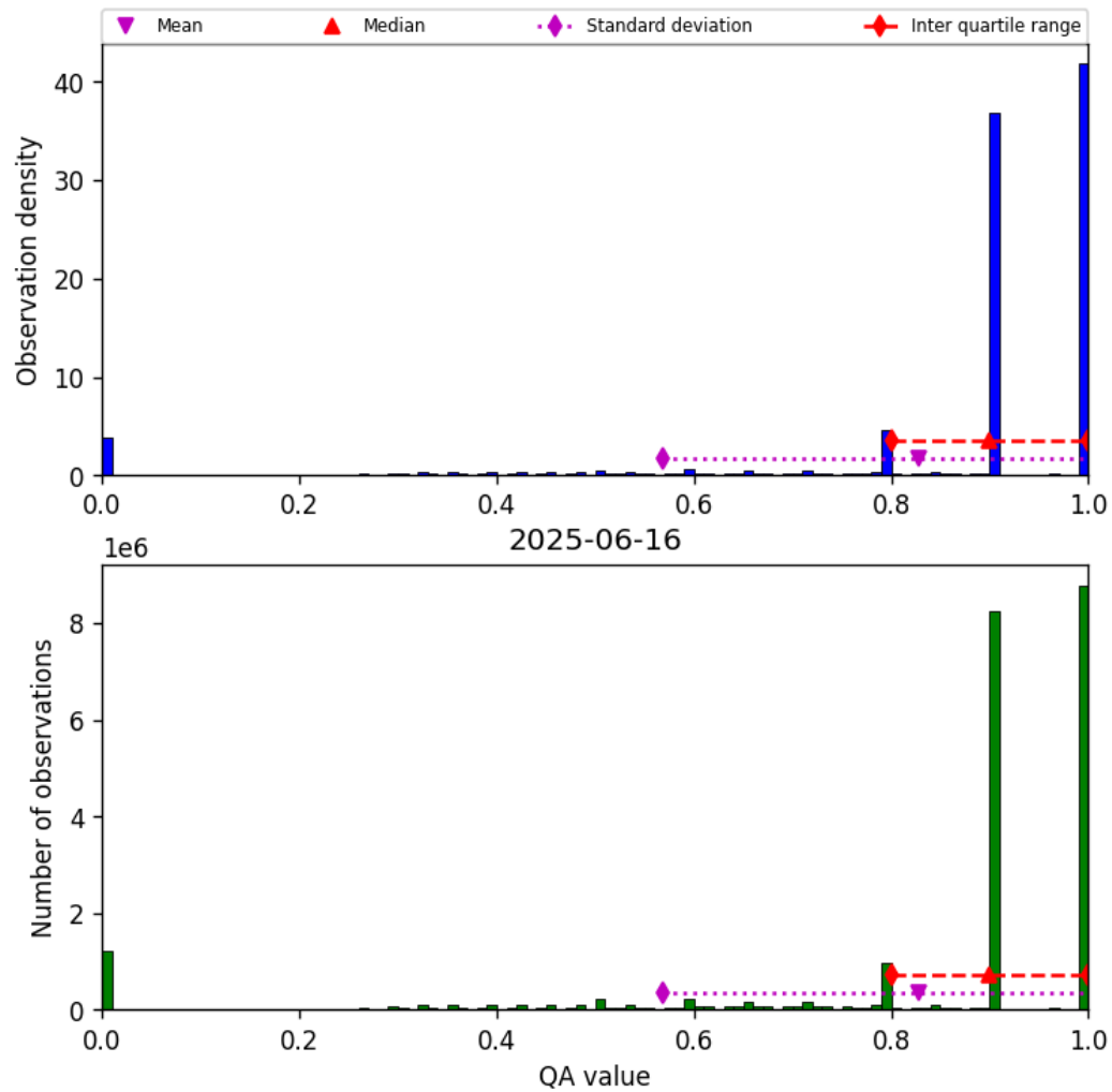
Figure 28: Histogram of “QA value” for 2025-06-16 to 2025-06-17
