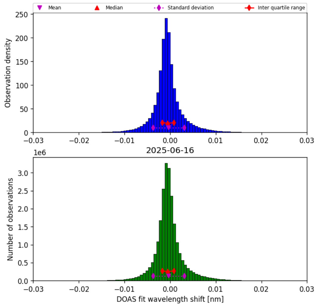
Figure 35: Histogram of “DOAS fit wavelength shift” for 2025-06-16 to 2025-06-17
