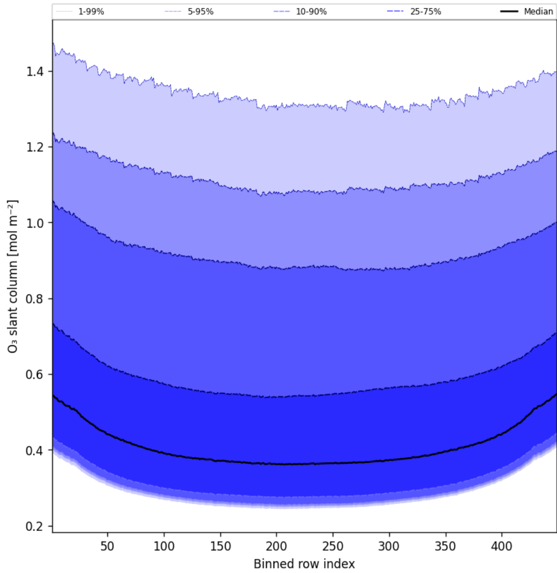
Figure 43: Along track statistics of “O 3 slant column” for 2025-06-16 to 2025-06-17
