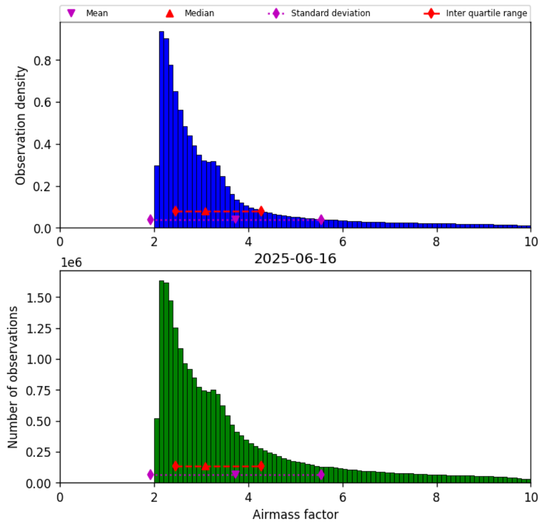
Figure 37: Histogram of “Airmass factor” for 2025-06-16 to 2025-06-17
