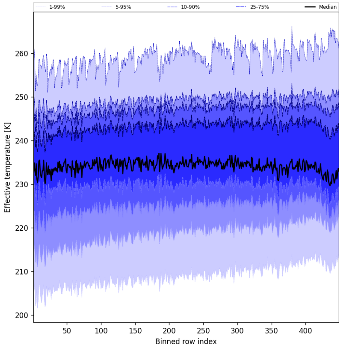
Figure 50: Along track statistics of “Effective temperature” for 2025-06-16 to 2025-06-17
