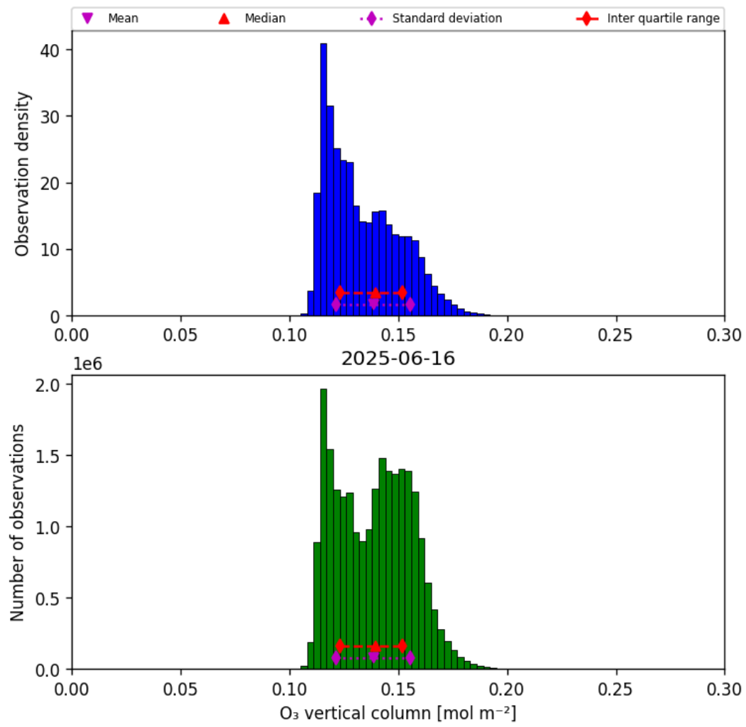
Figure 29: Histogram of “O 3 vertical column” for 2025-06-16 to 2025-06-17
