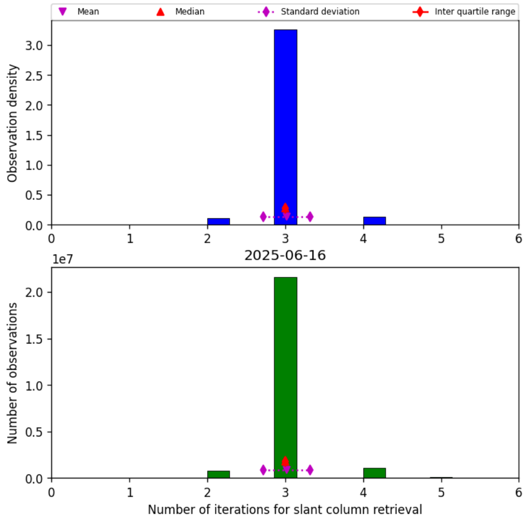
Figure 33: Histogram of “Number of iterations for slant column retrieval” for 2025-06-16 to 2025-06-17
