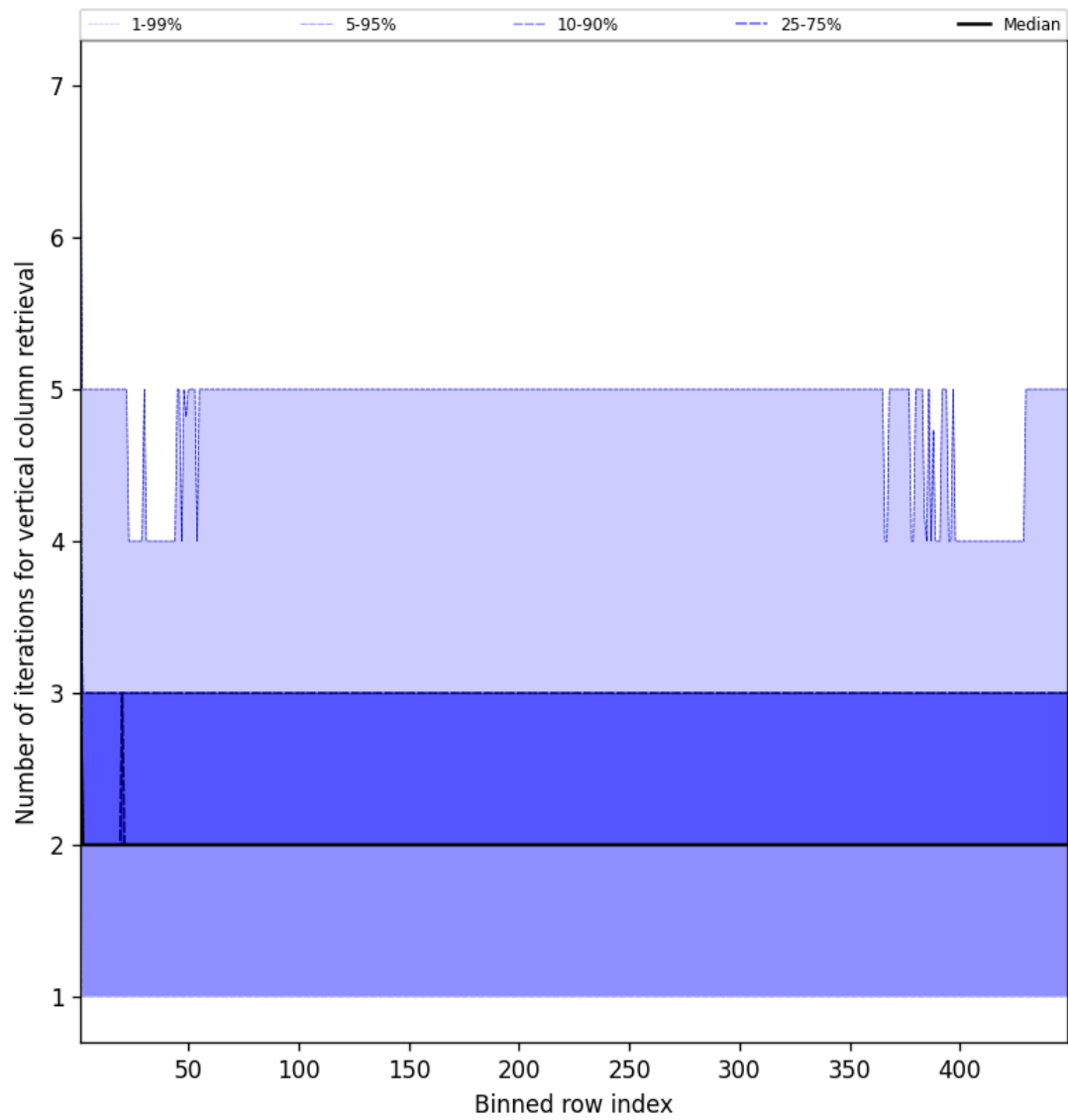
Figure 51: Along track statistics of “Number of iterations for vertical column retrieval” for 2025-06-16 to 2025-06-17
