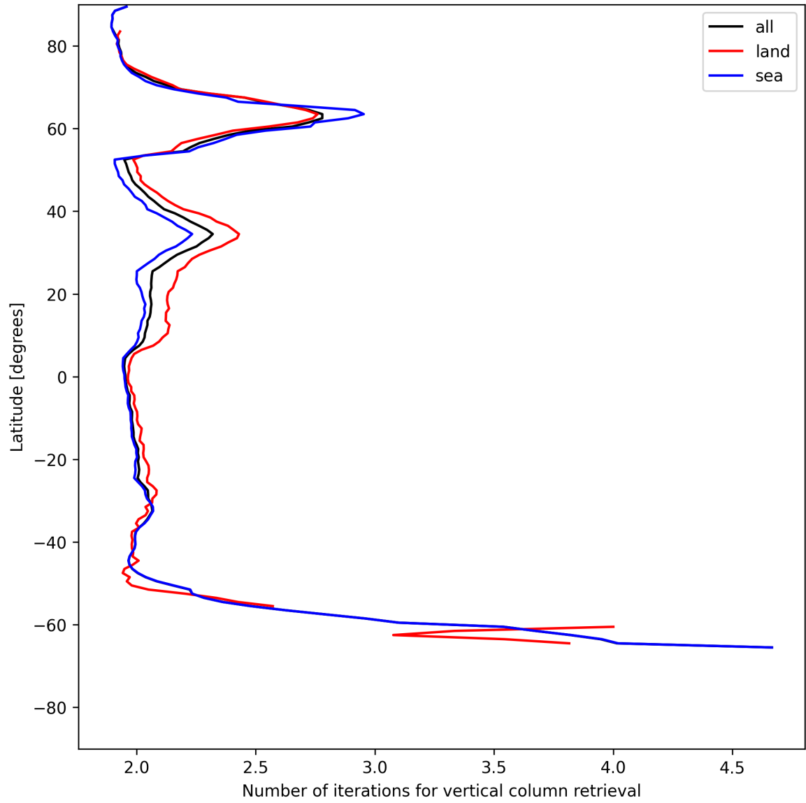
Figure 27: Zonal average of “Number of iterations for vertical column retrieval” for 2025-06-16 to 2025-06-17.
