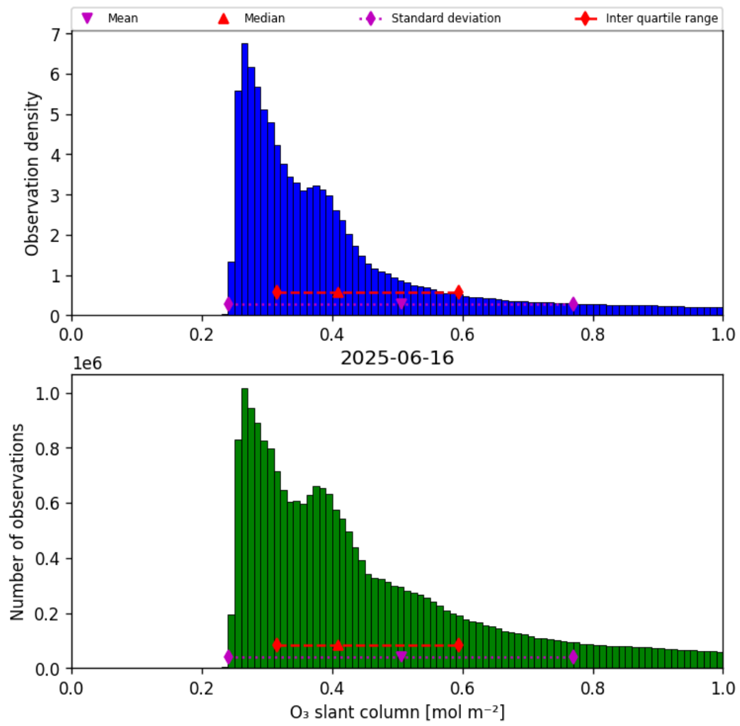
Figure 31: Histogram of “O 3 slant column” for 2025-06-16 to 2025-06-17
