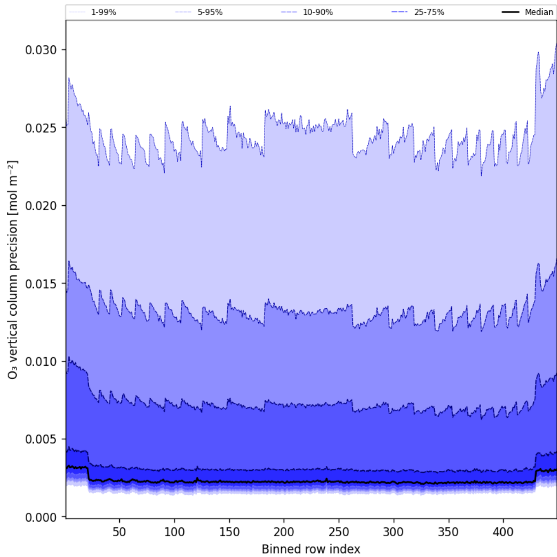
Figure 42: Along track statistics of “O 3 vertical column precision” for 2025-06-16 to 2025-06-17
