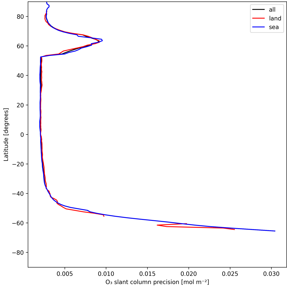
Figure 20: Zonal average of “O 3 slant column precision” for 2025-06-16 to 2025-06-17.
