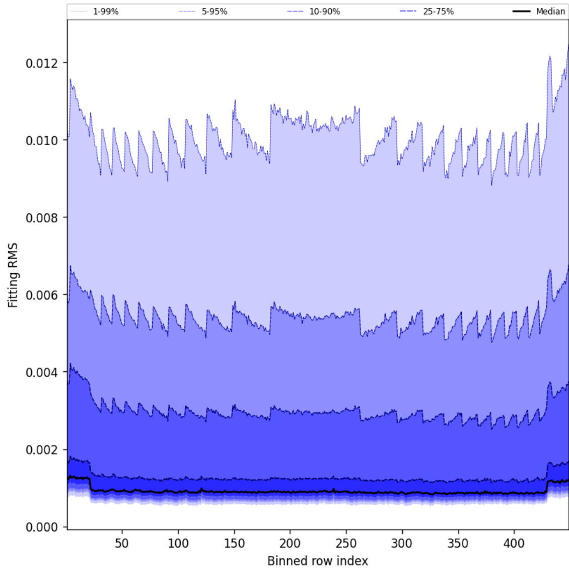
Figure 46: Along track statistics of “Fitting RMS” for 2025-06-16 to 2025-06-17
