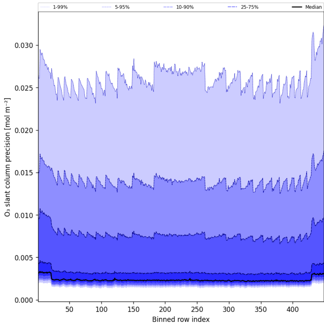
Figure 44: Along track statistics of “O 3 slant column precision” for 2025-06-16 to 2025-06-17
