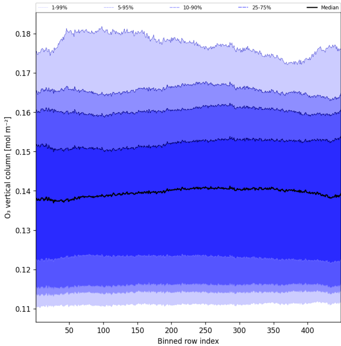
Figure 41: Along track statistics of “O 3 vertical column” for 2025-06-16 to 2025-06-17
