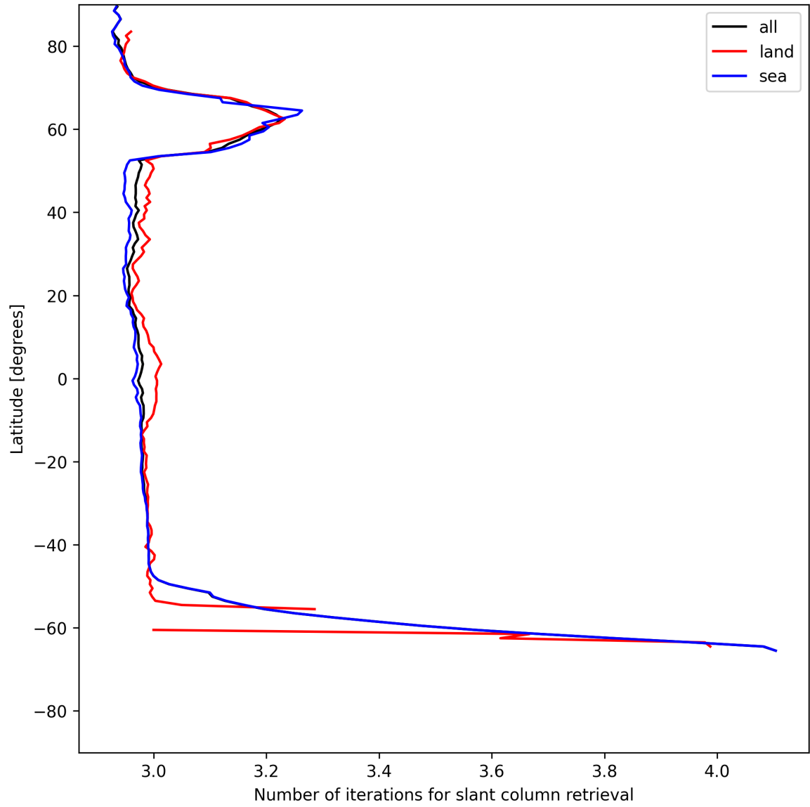
Figure 21: Zonal average of “Number of iterations for slant column retrieval” for 2025-06-16 to 2025-06-17.
