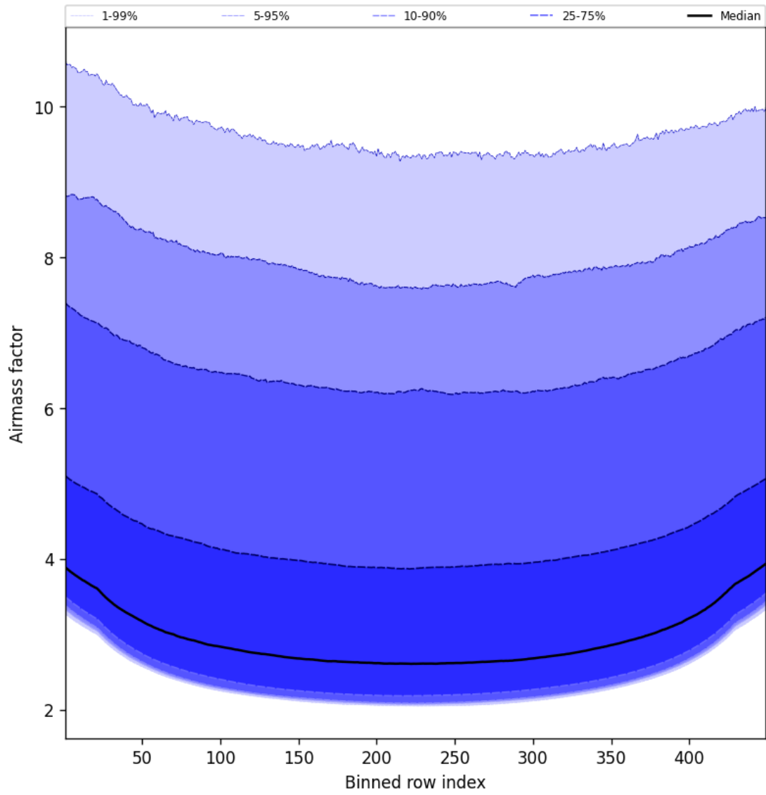
Figure 49: Along track statistics of “Airmass factor” for 2025-06-16 to 2025-06-17
