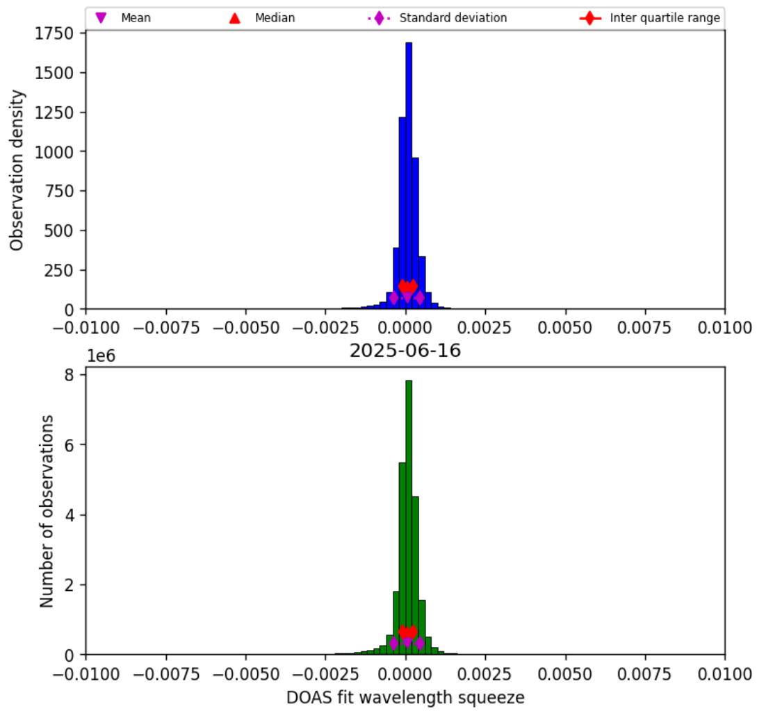
Figure 36: Histogram of “DOAS fit wavelength squeeze” for 2025-06-16 to 2025-06-17
