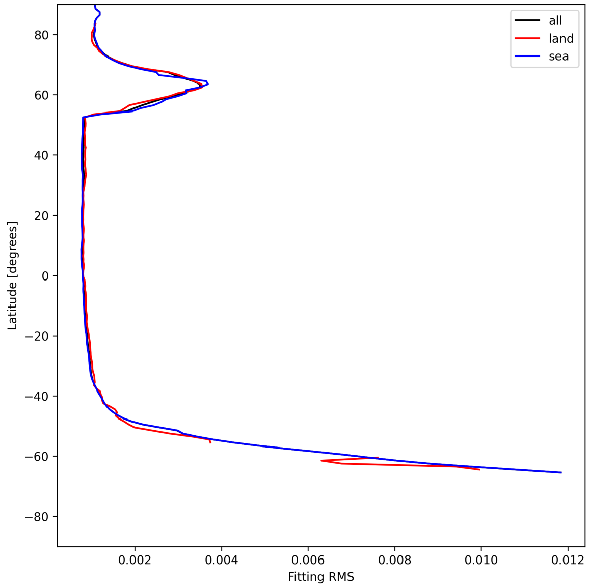
Figure 22: Zonal average of “Fitting RMS” for 2025-06-16 to 2025-06-17.
