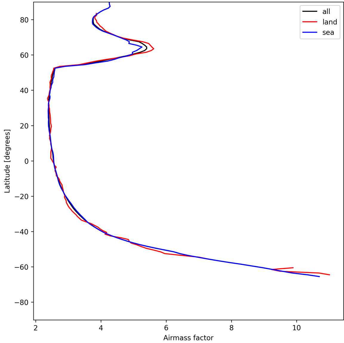
Figure 25: Zonal average of “Airmass factor” for 2025-06-16 to 2025-06-17.
