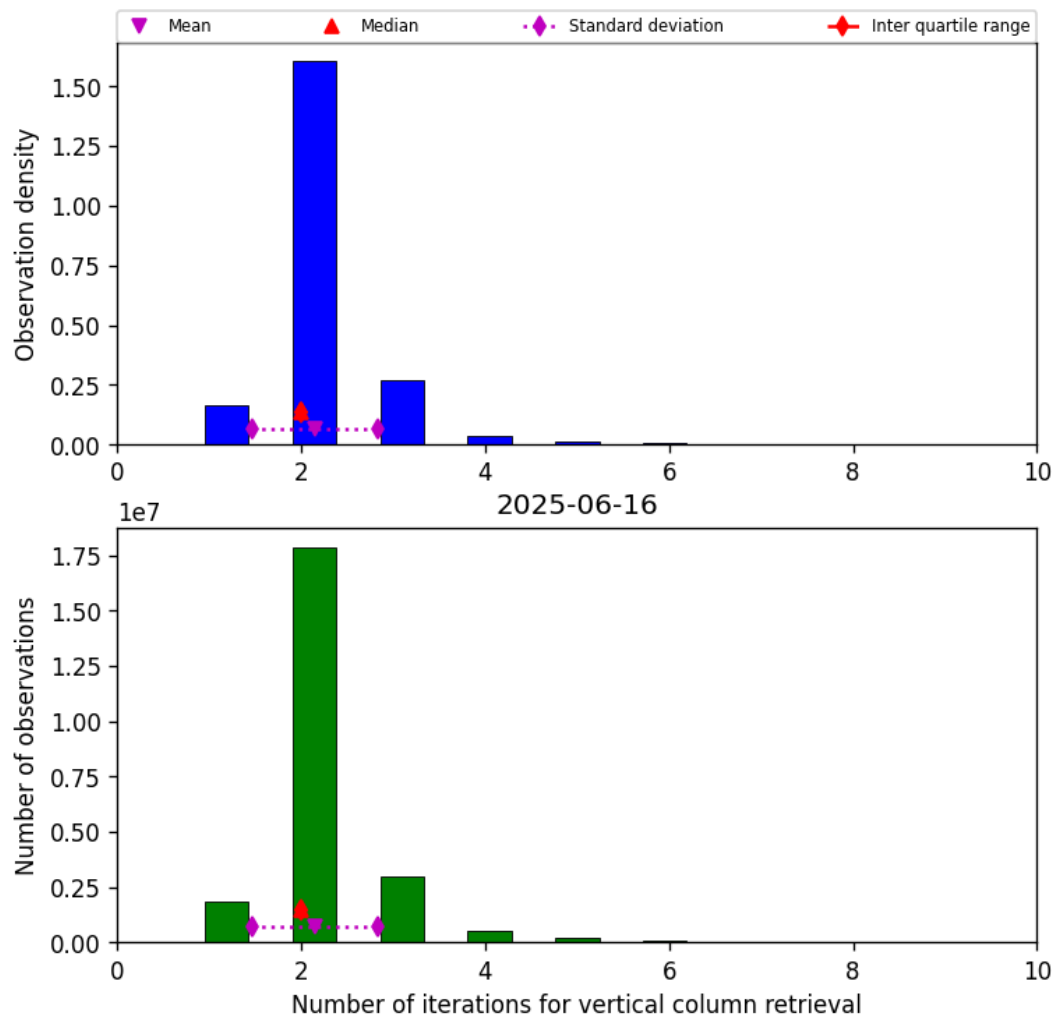
Figure 39: Histogram of “Number of iterations for vertical column retrieval” for 2025-06-16 to 2025-06-17
