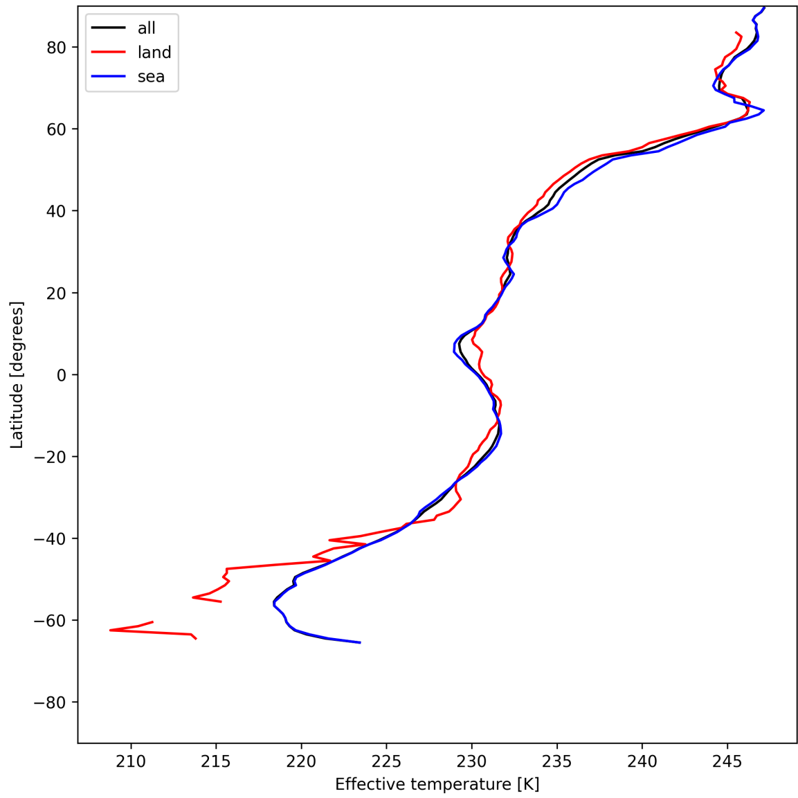
Figure 26: Zonal average of “Effective temperature” for 2025-06-16 to 2025-06-17.
