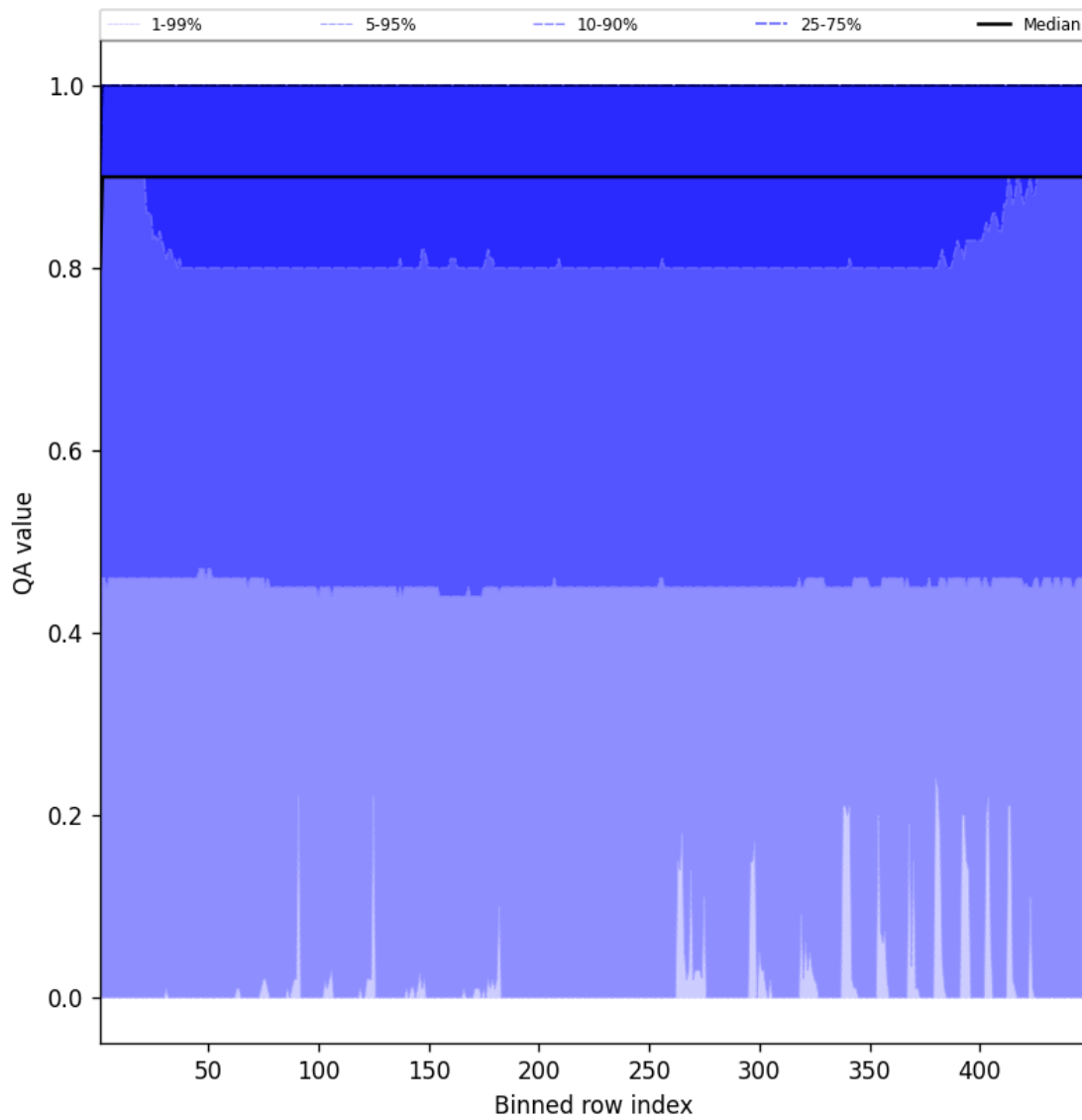
Figure 40: Along track statistics of “QA value” for 2025-06-16 to 2025-06-17
