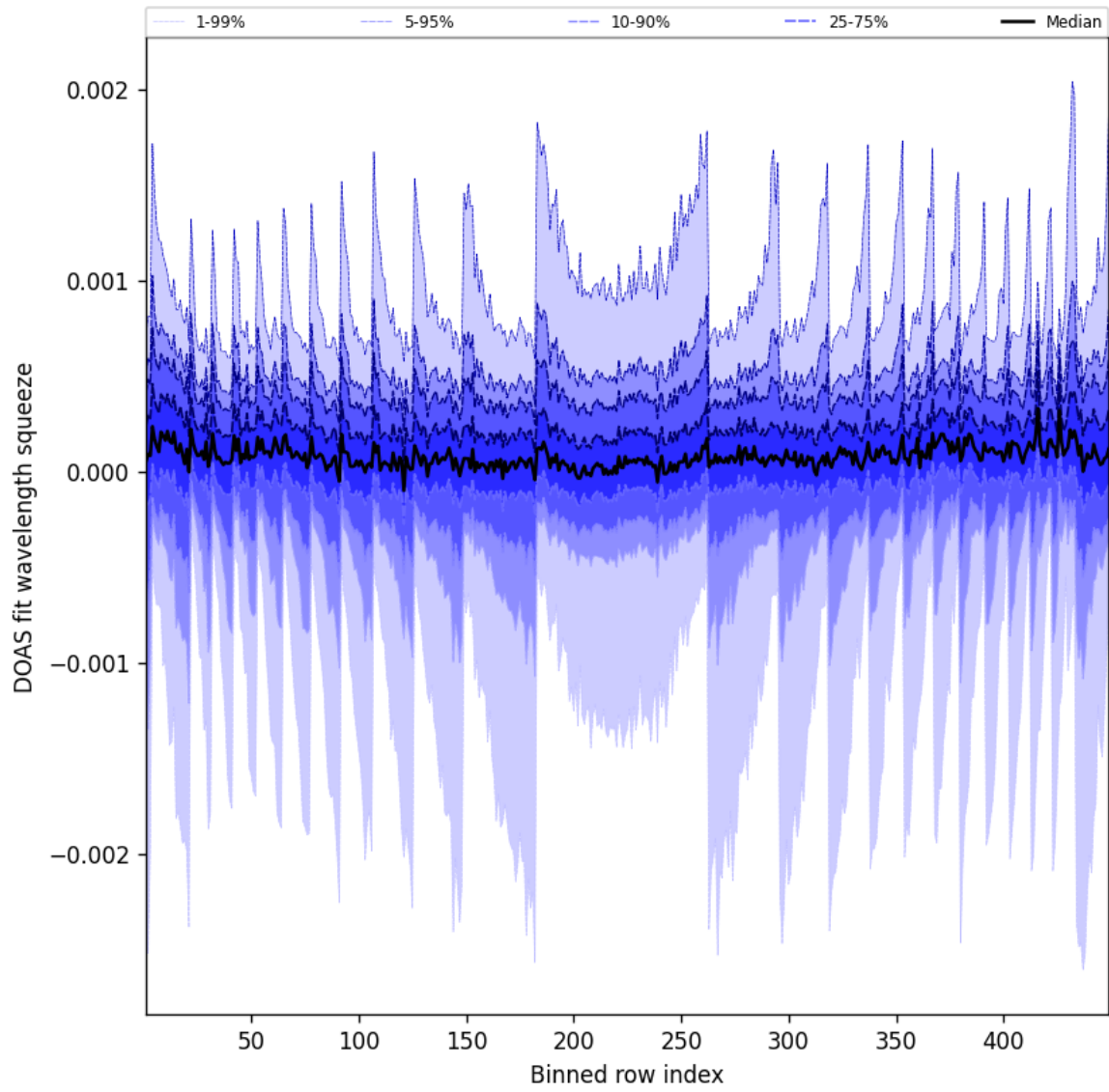
Figure 48: Along track statistics of “DOAS fit wavelength squeeze” for 2025-06-16 to 2025-06-17
