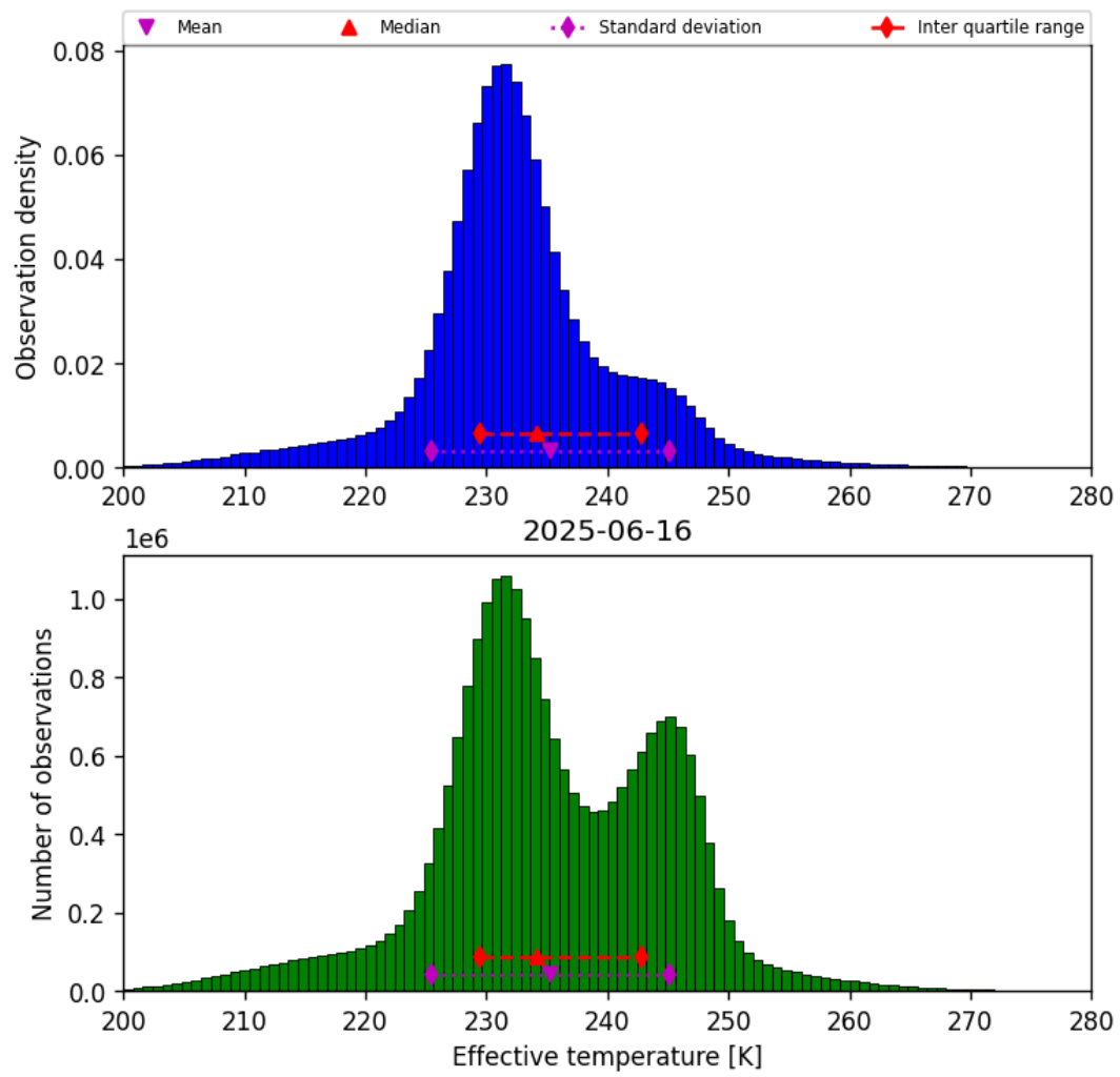
Figure 38: Histogram of “Effective temperature” for 2025-06-16 to 2025-06-17
