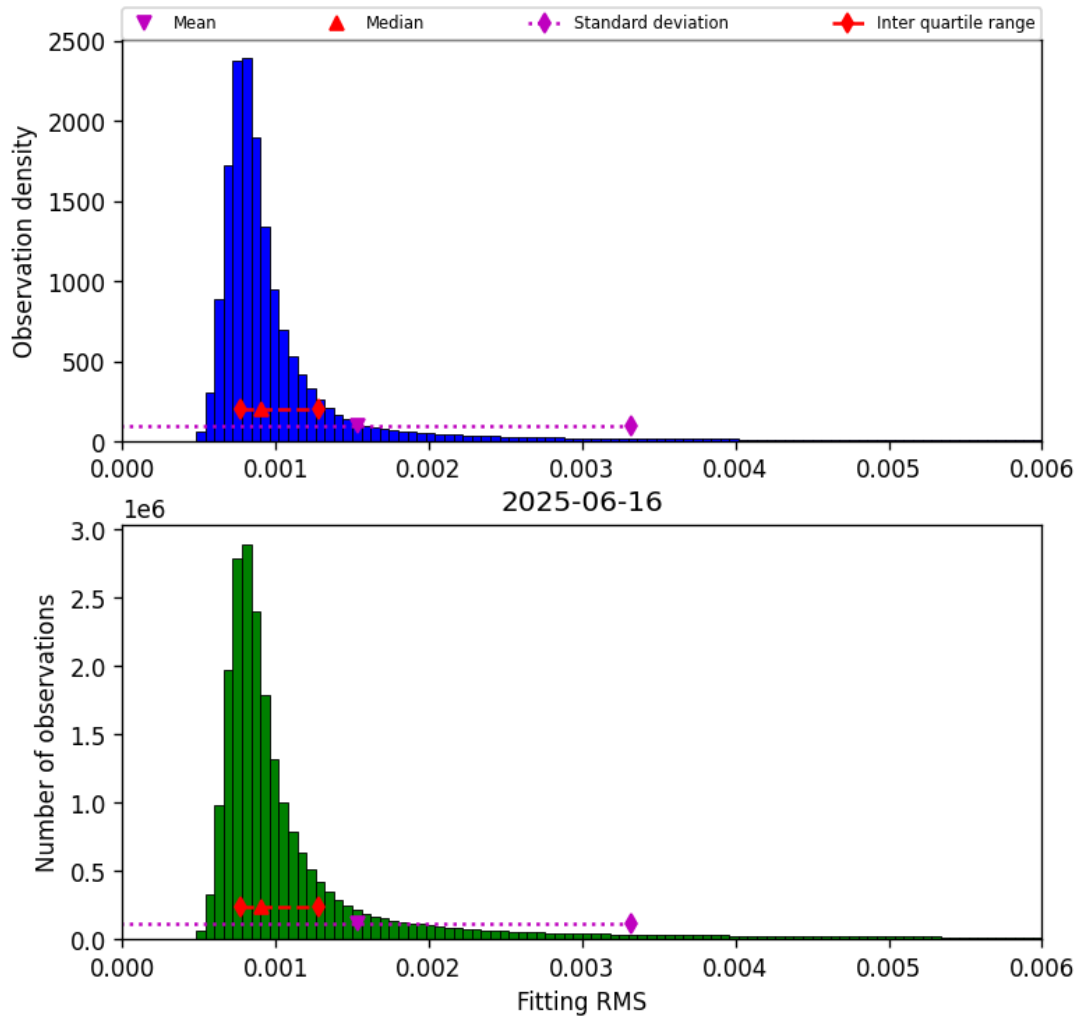
Figure 34: Histogram of “Fitting RMS” for 2025-06-16 to 2025-06-17
