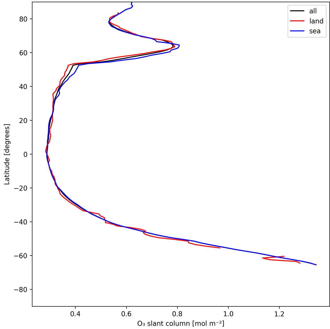
Figure 19: Zonal average of “O 3 slant column” for 2025-06-16 to 2025-06-17.
