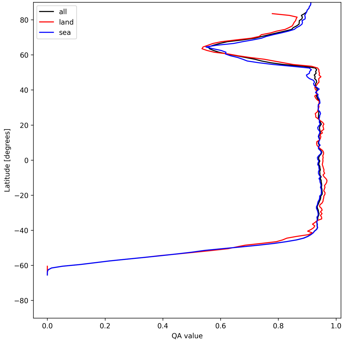
Figure 16: Zonal average of “QA value” for 2025-06-16 to 2025-06-17.
