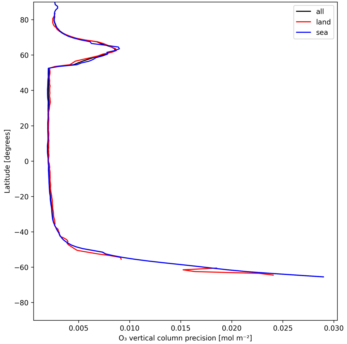
Figure 18: Zonal average of “O 3 vertical column precision” for 2025-06-16 to 2025-06-17.
