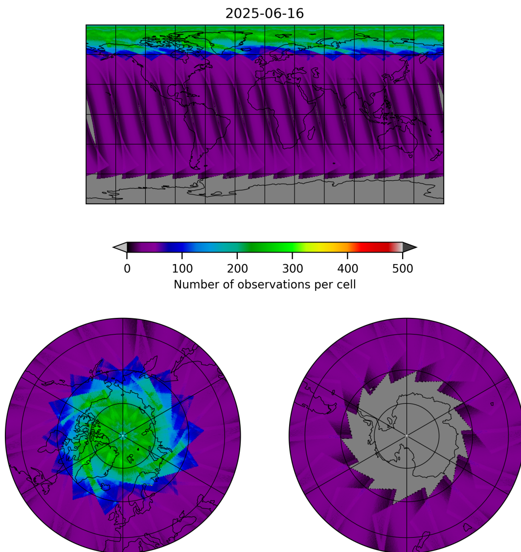
Figure 15: Map of the number of observations for 2025-06-16 to 2025-06-17
