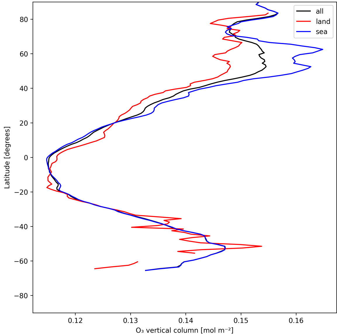
Figure 17: Zonal average of “O 3 vertical column” for 2025-06-16 to 2025-06-17.
