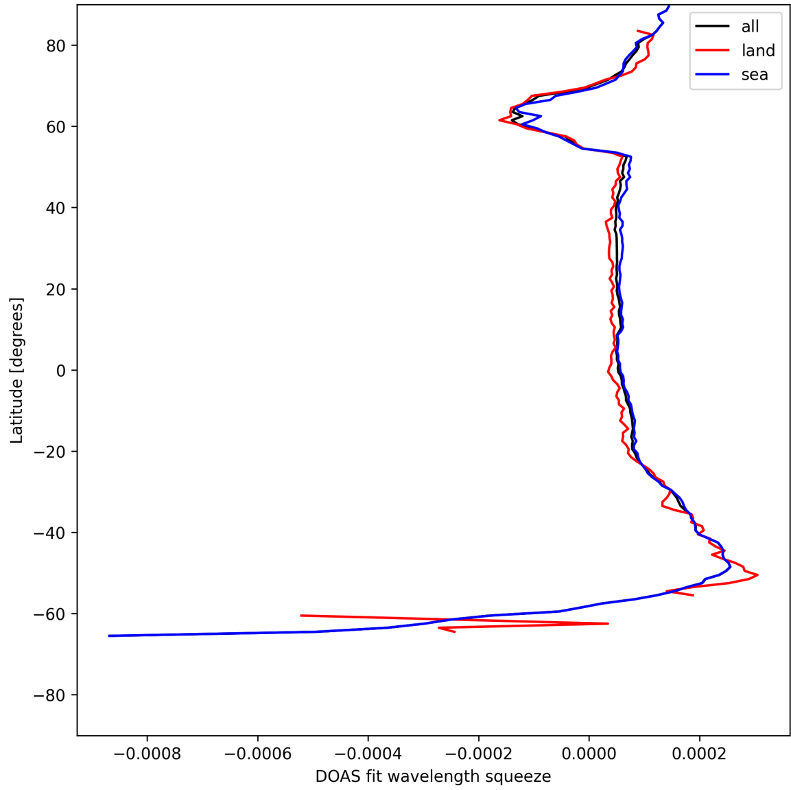
Figure 24: Zonal average of “DOAS fit wavelength squeeze” for 2025-06-16 to 2025-06-17.
