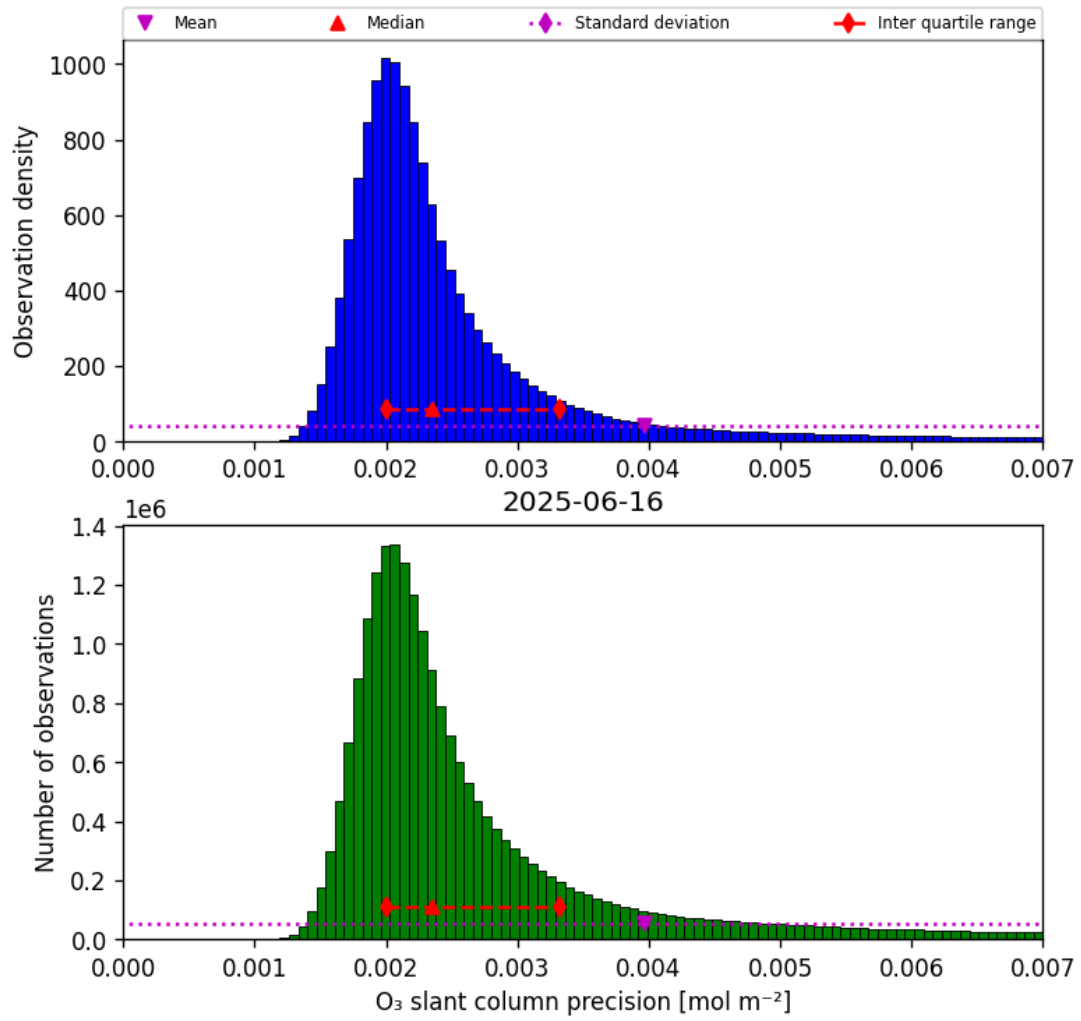
Figure 32: Histogram of “O 3 slant column precision” for 2025-06-16 to 2025-06-17
