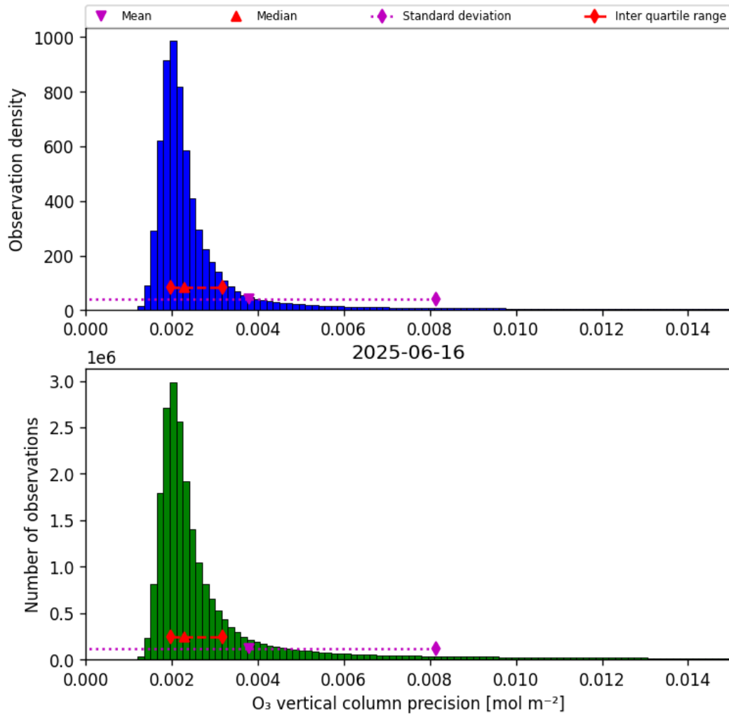
Figure 30: Histogram of “O 3 vertical column precision” for 2025-06-16 to 2025-06-17
