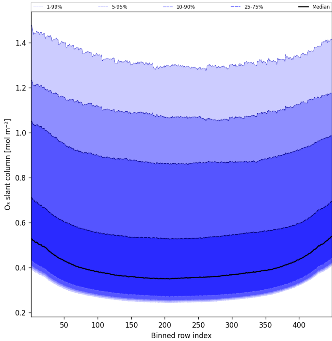
Figure 43: Along track statistics of “O 3 slant column” for 2025-06-17 to 2025-06-17
