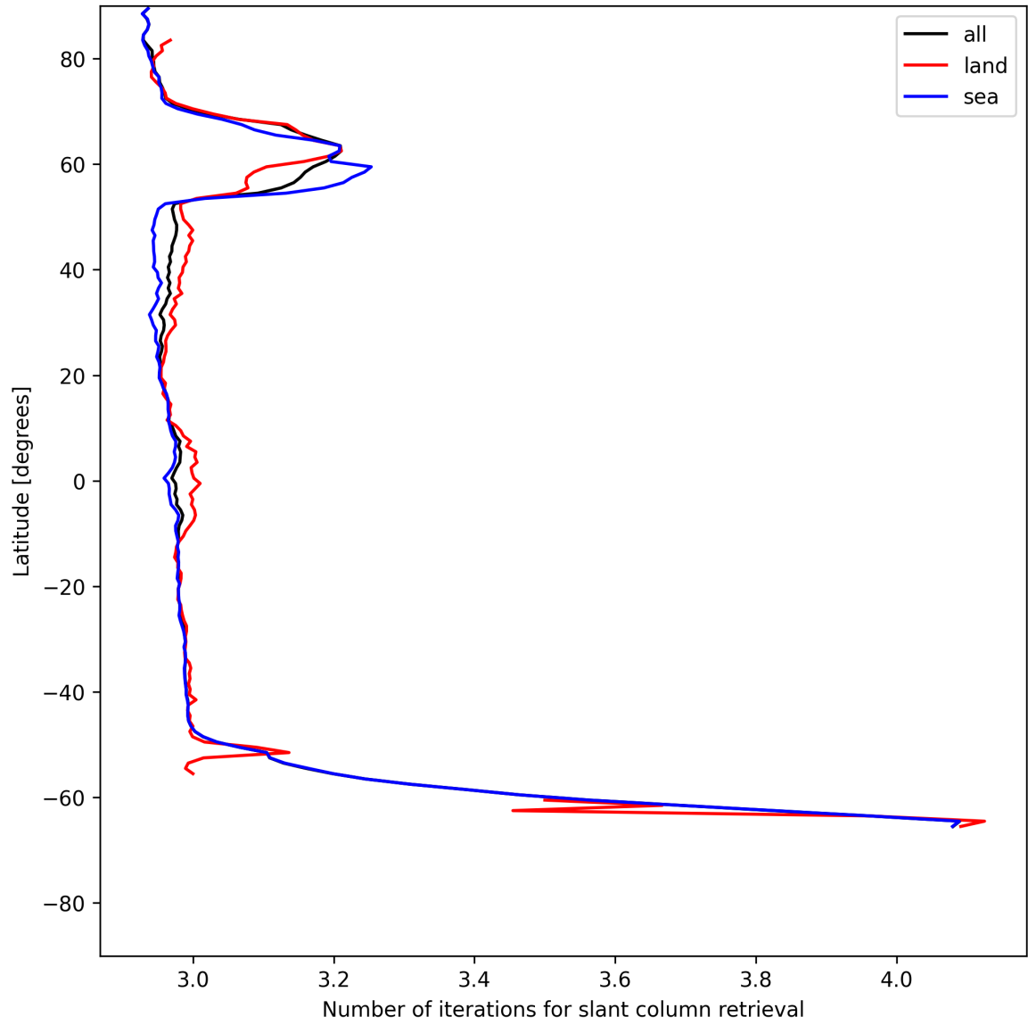
Figure 21: Zonal average of “Number of iterations for slant column retrieval” for 2025-06-17 to 2025-06-17.
