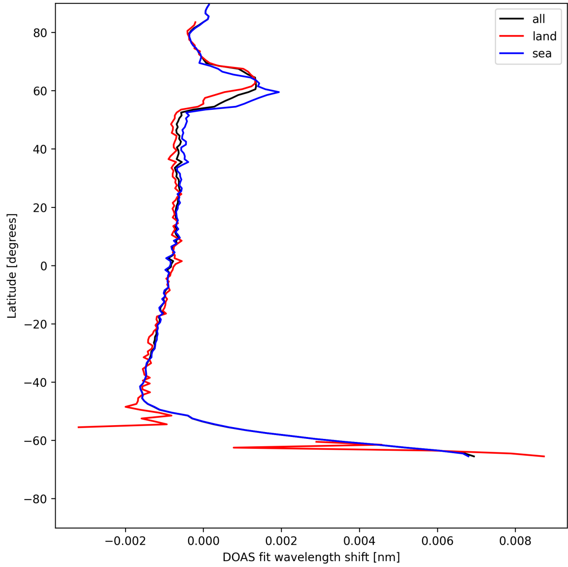
Figure 23: Zonal average of "DOAS fit wavelength shift" for 2025-06-17 to 2025-06-17.
