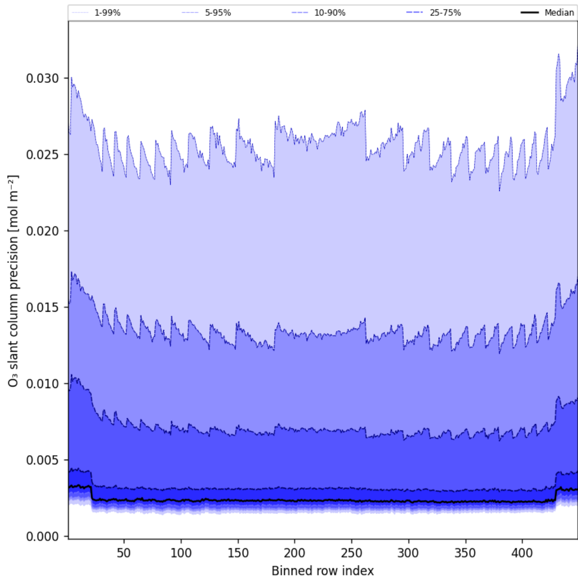
Figure 44: Along track statistics of “O 3 slant column precision” for 2025-06-17 to 2025-06-17
