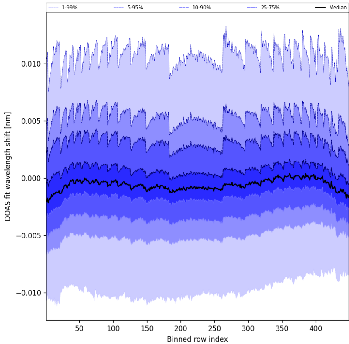
Figure 47: Along track statistics of "DOAS fit wavelength shift" for 2025-06-17 to 2025-06-17
