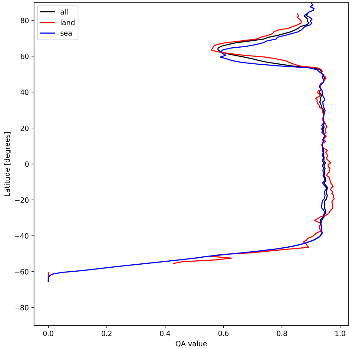
Figure 16: Zonal average of “QA value” for 2025-06-17 to 2025-06-17.
