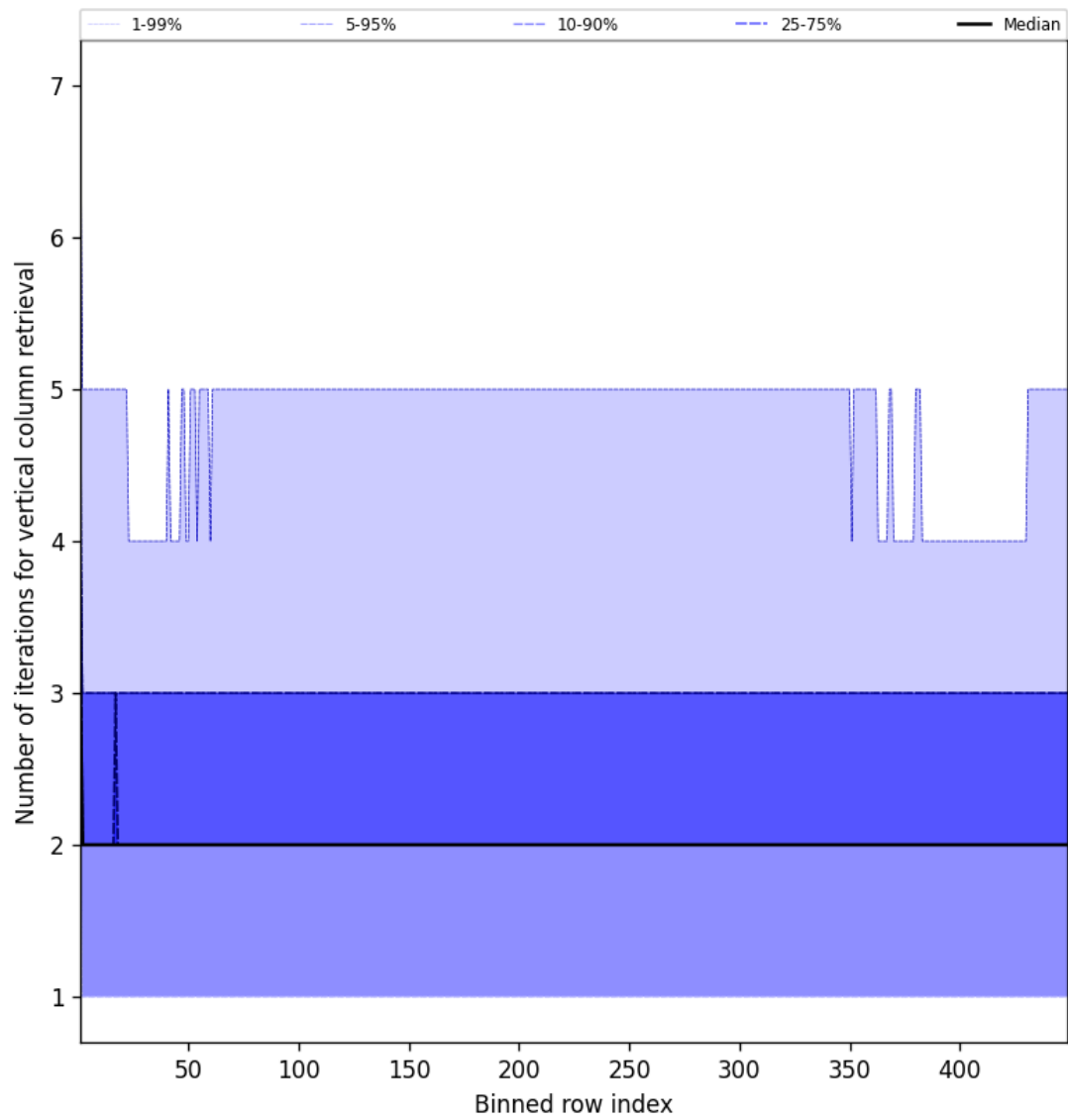
Figure 51: Along track statistics of “Number of iterations for vertical column retrieval” for 2025-06-17 to 2025-06-17
