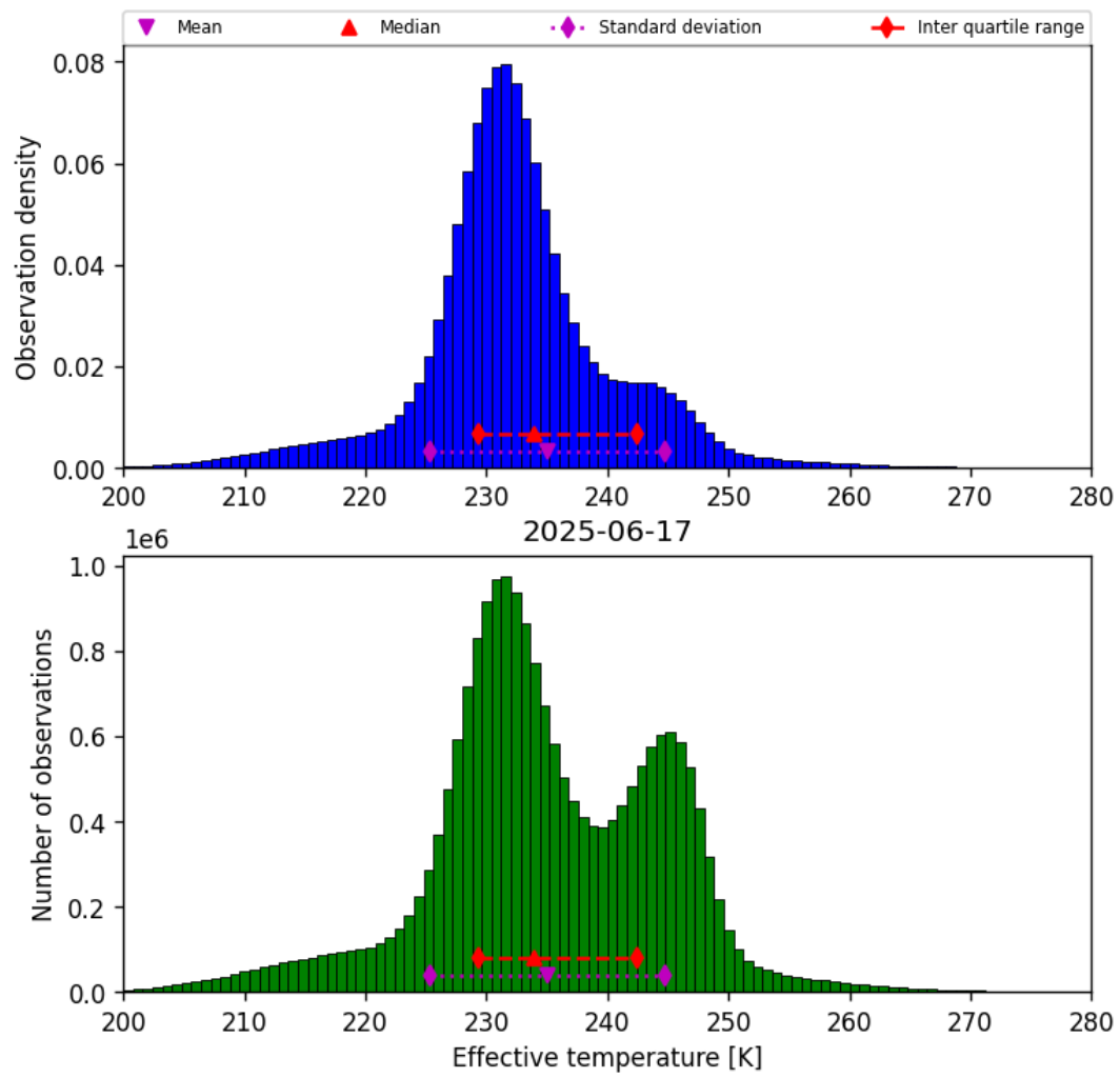
Figure 38: Histogram of “Effective temperature” for 2025-06-17 to 2025-06-17
