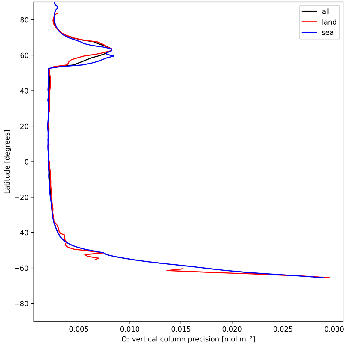
Figure 18: Zonal average of “O 3 vertical column precision” for 2025-06-17 to 2025-06-17.
