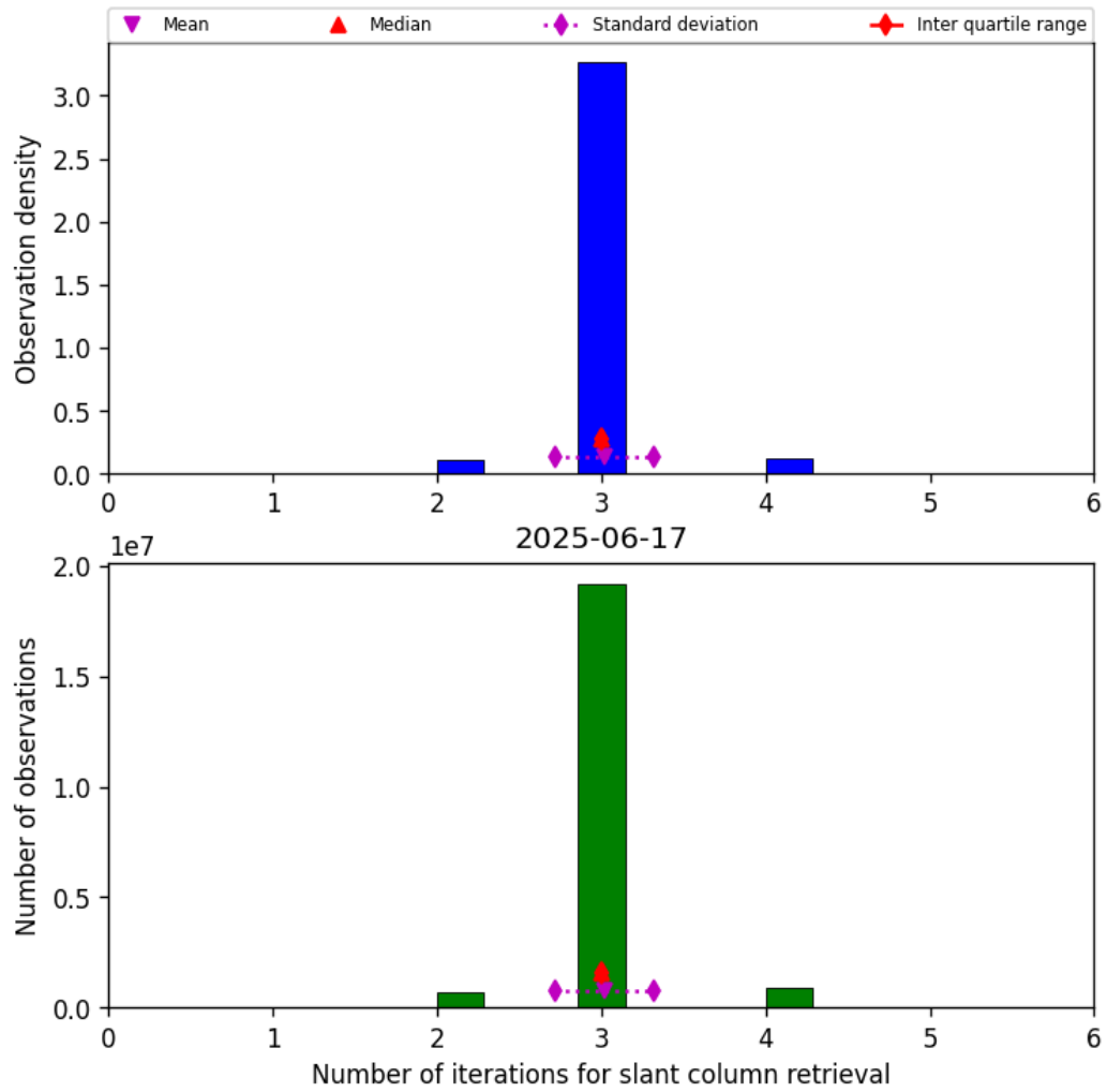
Figure 33: Histogram of “Number of iterations for slant column retrieval” for 2025-06-17 to 2025-06-17
