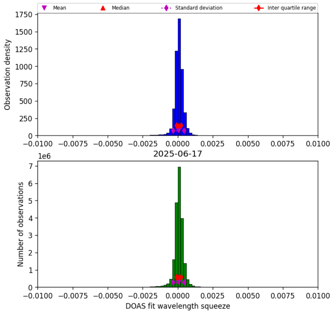
Figure 36: Histogram of “DOAS fit wavelength squeeze” for 2025-06-17 to 2025-06-17
