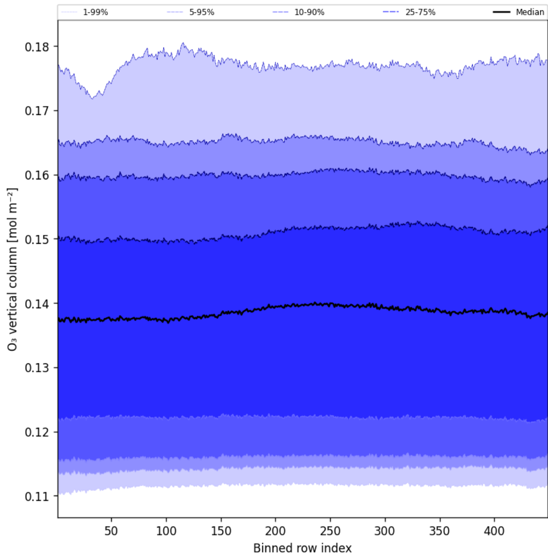
Figure 41: Along track statistics of “O 3 vertical column” for 2025-06-17 to 2025-06-17
