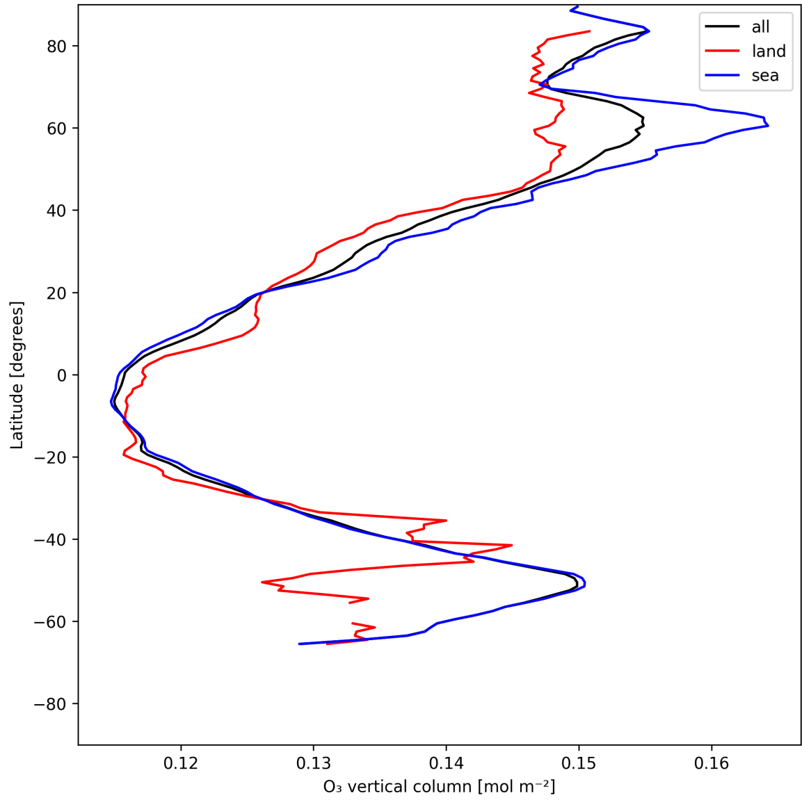
Figure 17: Zonal average of “O 3 vertical column” for 2025-06-17 to 2025-06-17.
