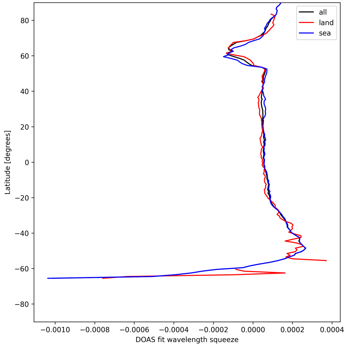
Figure 24: Zonal average of “DOAS fit wavelength squeeze” for 2025-06-17 to 2025-06-17.
