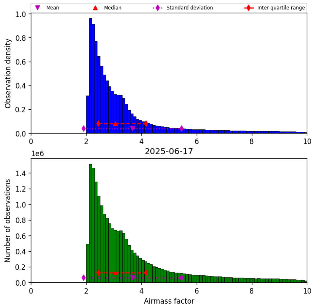
Figure 37: Histogram of “Airmass factor” for 2025-06-17 to 2025-06-17
