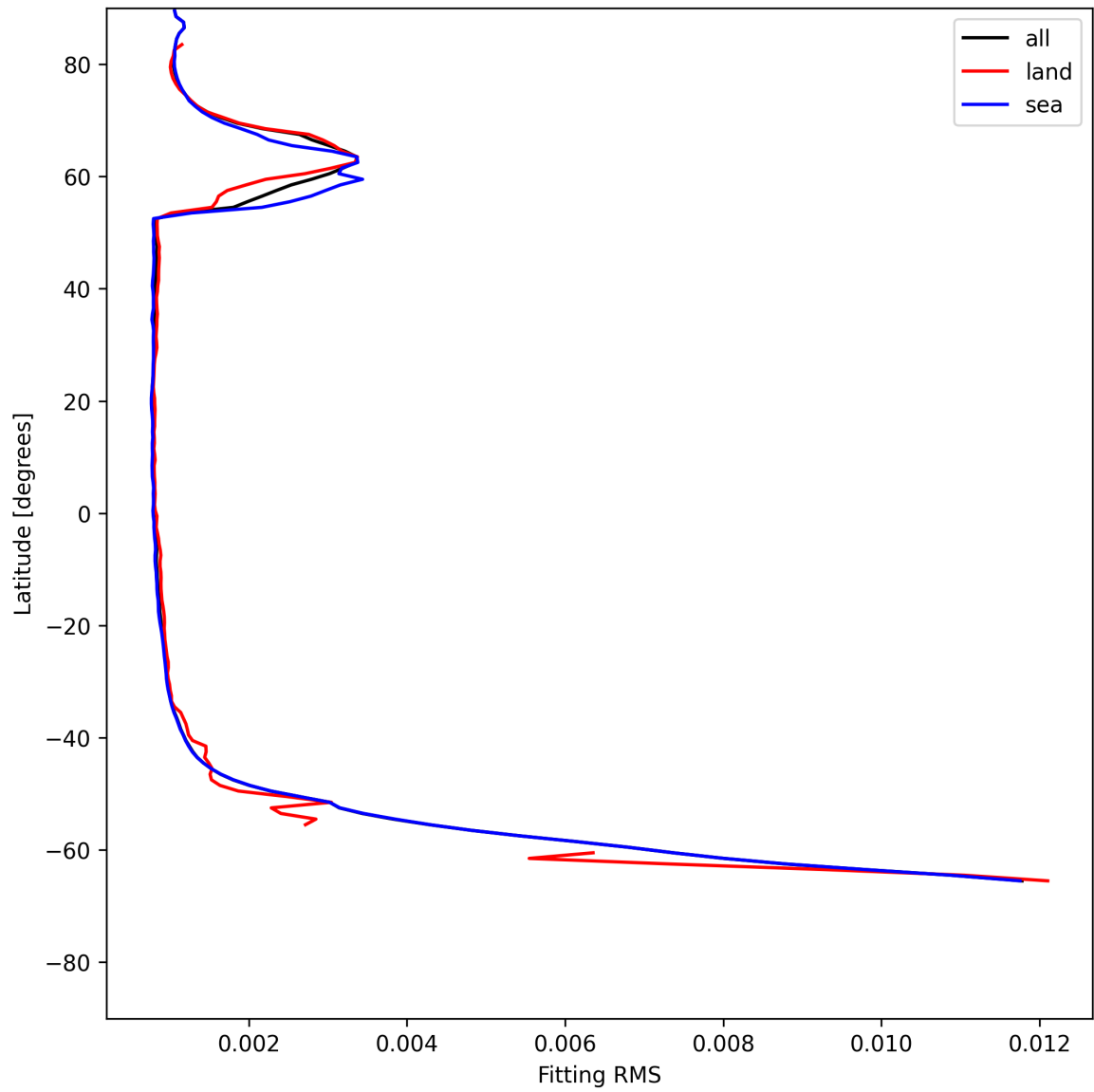
Figure 22: Zonal average of “Fitting RMS” for 2025-06-17 to 2025-06-17.
