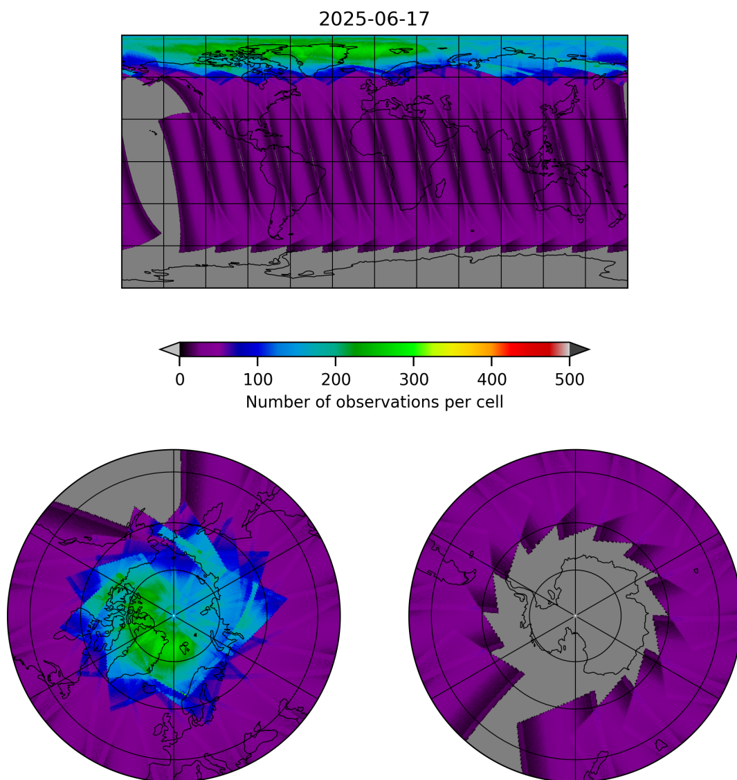
Figure 15: Map of the number of observations for 2025-06-17 to 2025-06-17
