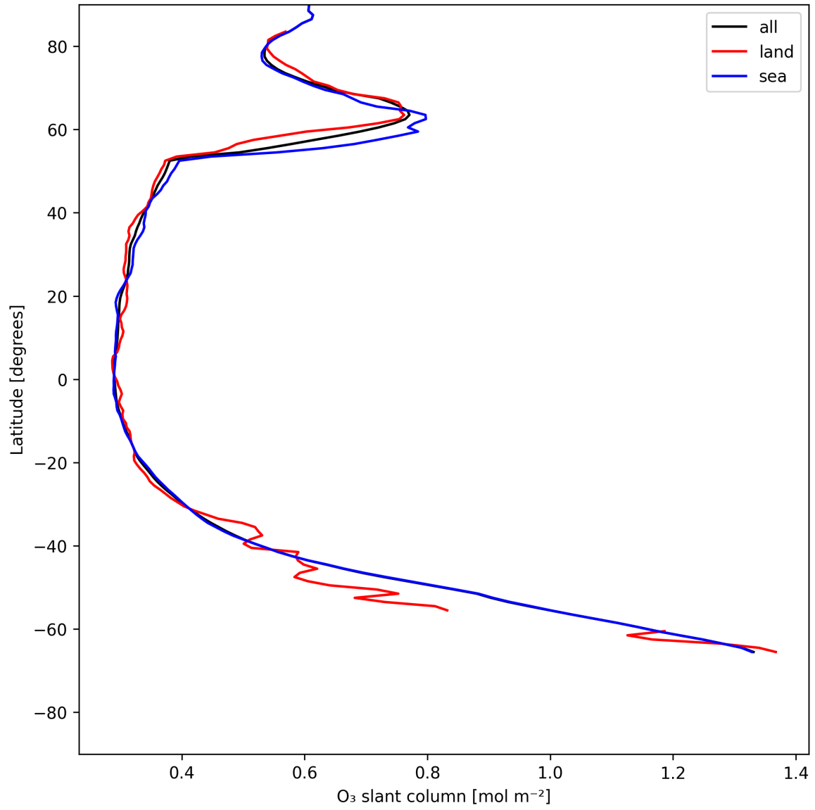
Figure 19: Zonal average of “O 3 slant column” for 2025-06-17 to 2025-06-17.
