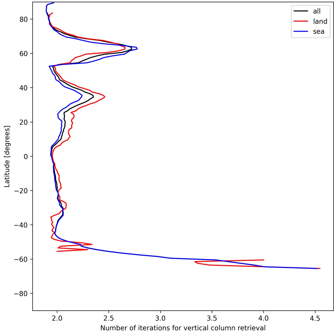
Figure 27: Zonal average of “Number of iterations for vertical column retrieval” for 2025-06-17 to 2025-06-17.
