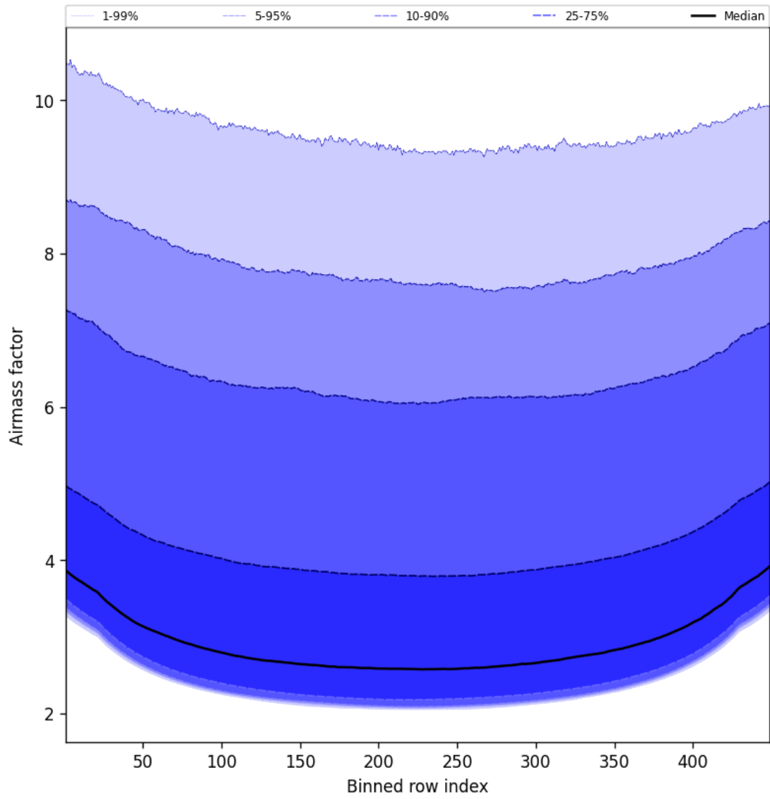
Figure 49: Along track statistics of “Airmass factor” for 2025-06-17 to 2025-06-17
