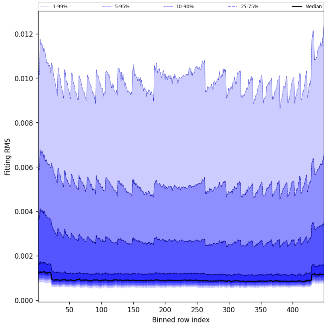
Figure 46: Along track statistics of “Fitting RMS” for 2025-06-17 to 2025-06-17
