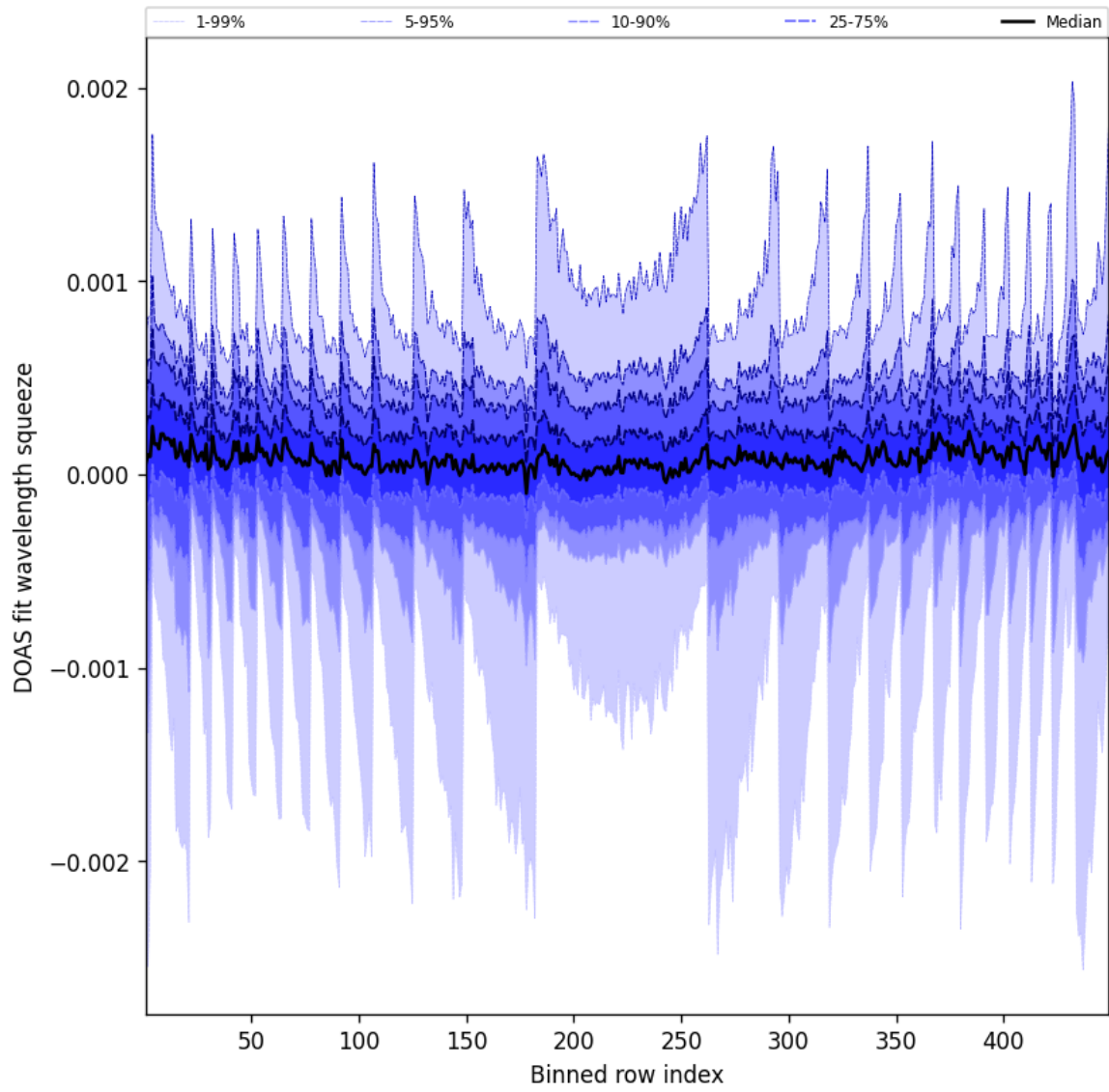
Figure 48: Along track statistics of “DOAS fit wavelength squeeze” for 2025-06-17 to 2025-06-17
