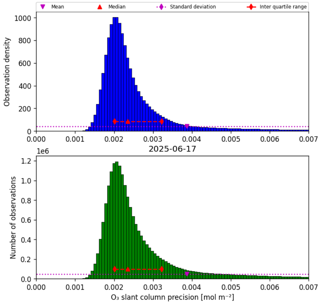
Figure 32: Histogram of “O 3 slant column precision” for 2025-06-17 to 2025-06-17
