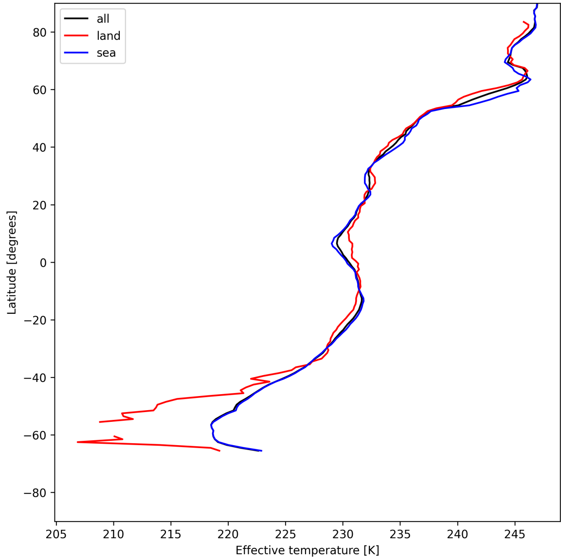
Figure 26: Zonal average of "Effective temperature" for 2025-06-17 to 2025-06-17.
