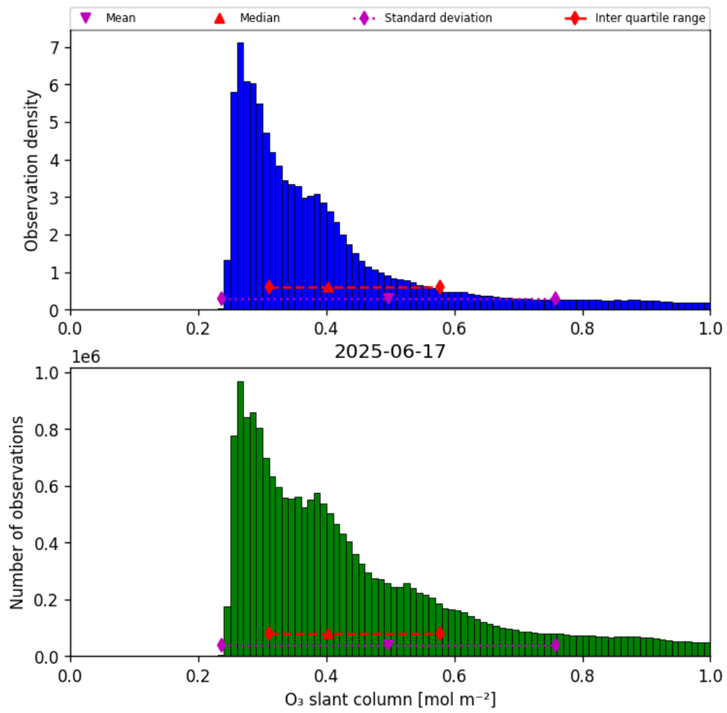
Figure 31: Histogram of “O 3 slant column” for 2025-06-17 to 2025-06-17
