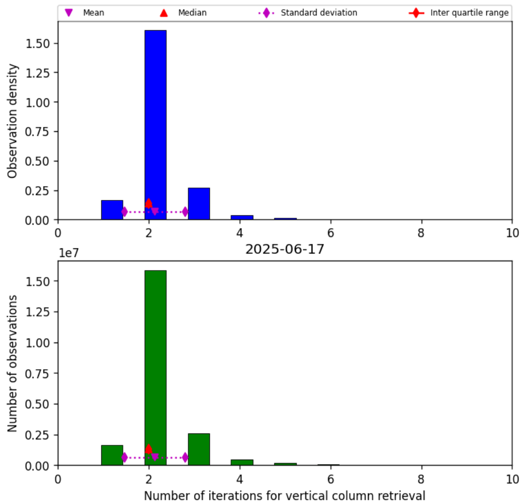
Figure 39: Histogram of “Number of iterations for vertical column retrieval” for 2025-06-17 to 2025-06-17
