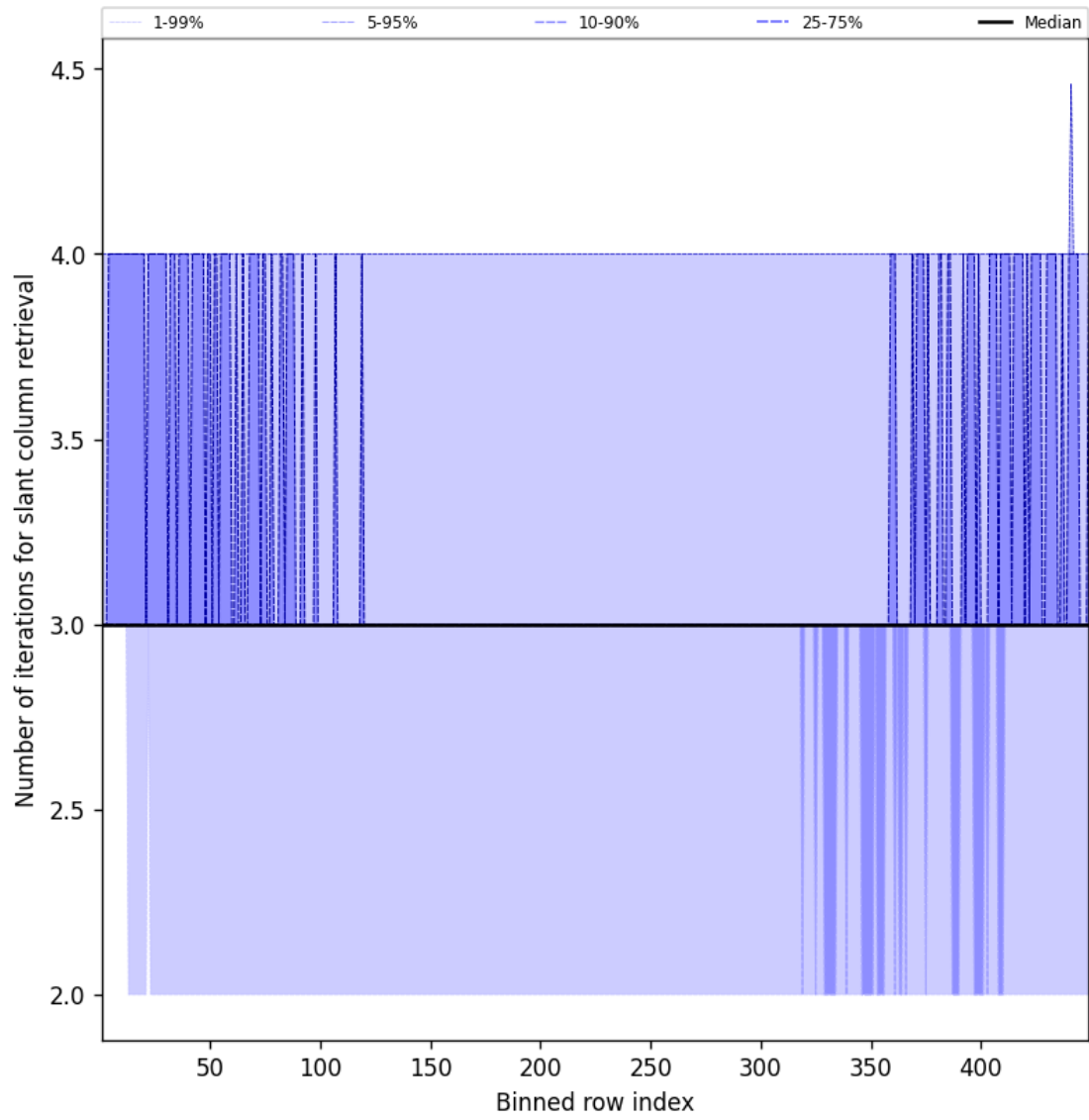
Figure 45: Along track statistics of “Number of iterations for slant column retrieval” for 2025-06-17 to 2025-06-17
