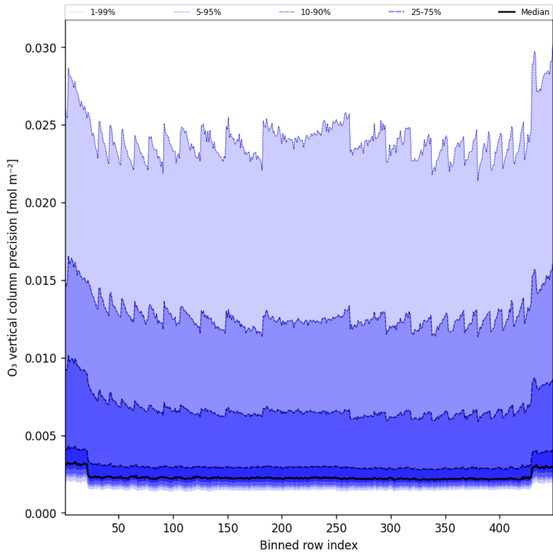
Figure 42: Along track statistics of “O 3 vertical column precision” for 2025-06-17 to 2025-06-17
