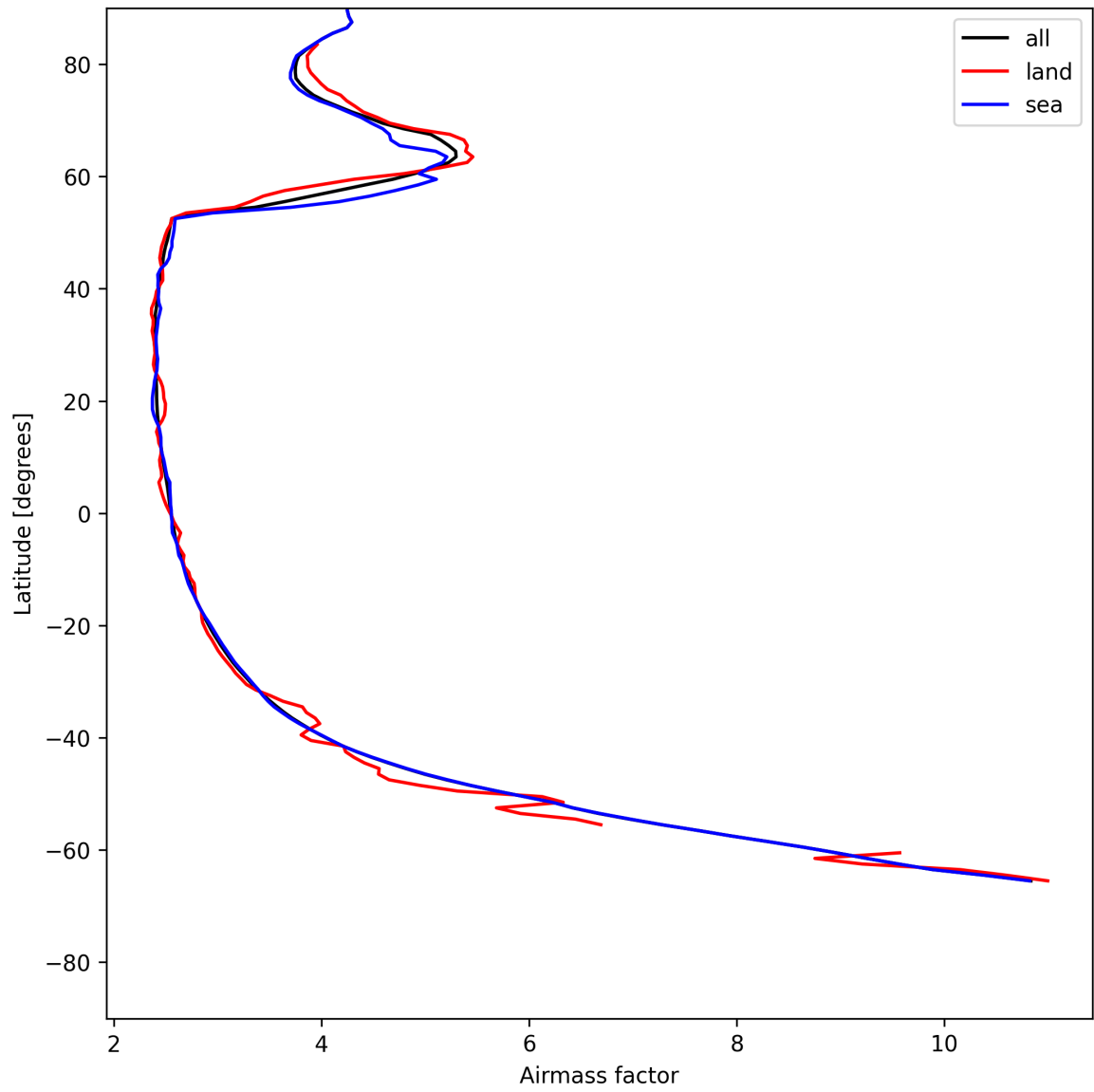
Figure 25: Zonal average of “Airmass factor” for 2025-06-17 to 2025-06-17.
