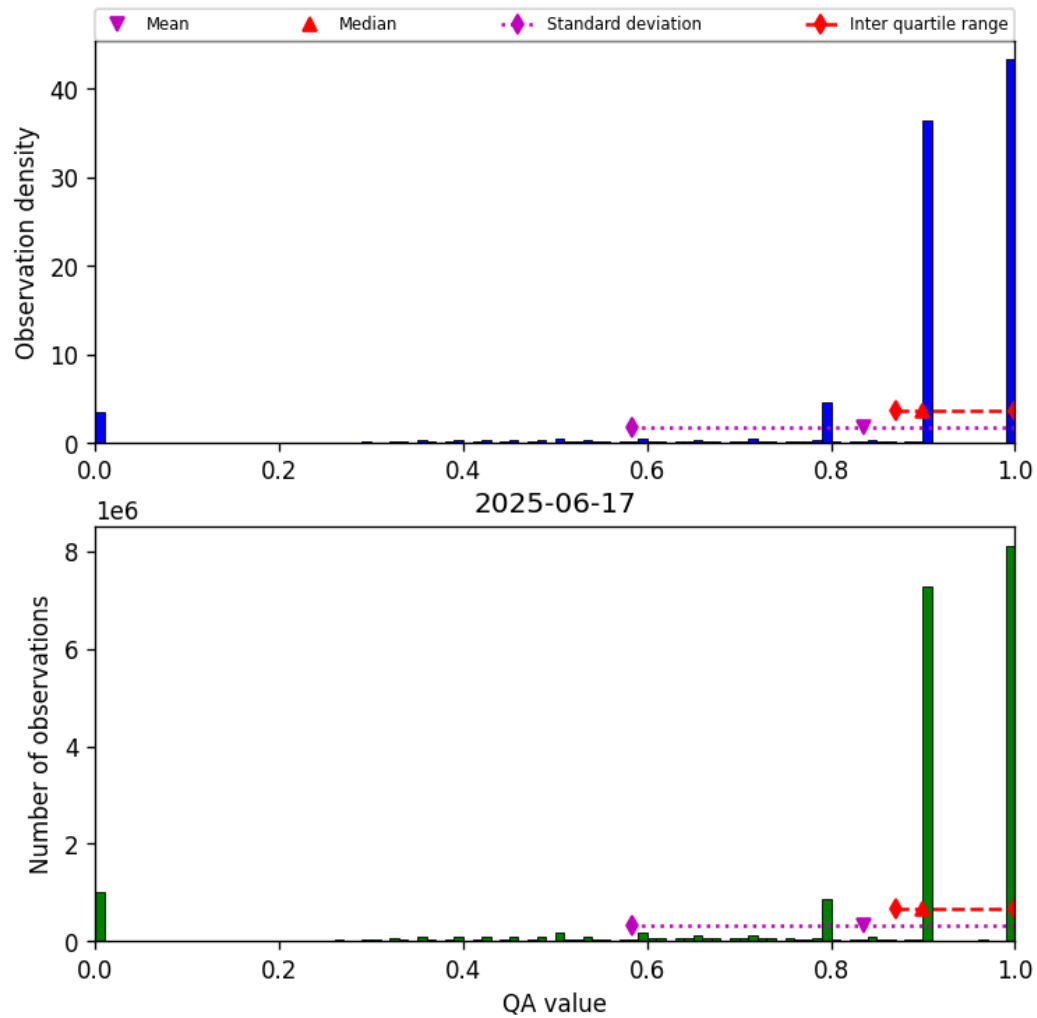
Figure 28: Histogram of “QA value” for 2025-06-17 to 2025-06-17
