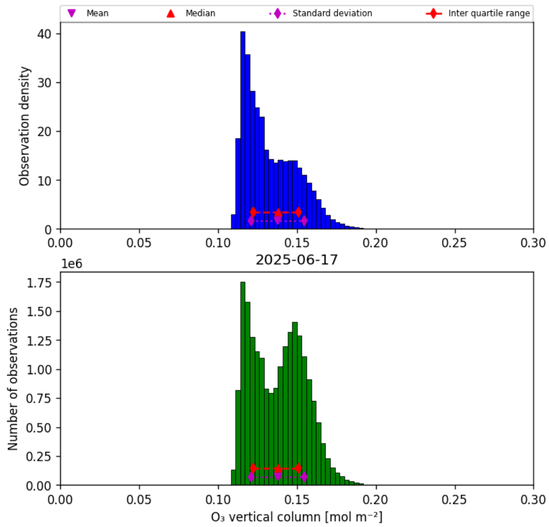
Figure 29: Histogram of “O 3 vertical column” for 2025-06-17 to 2025-06-17
