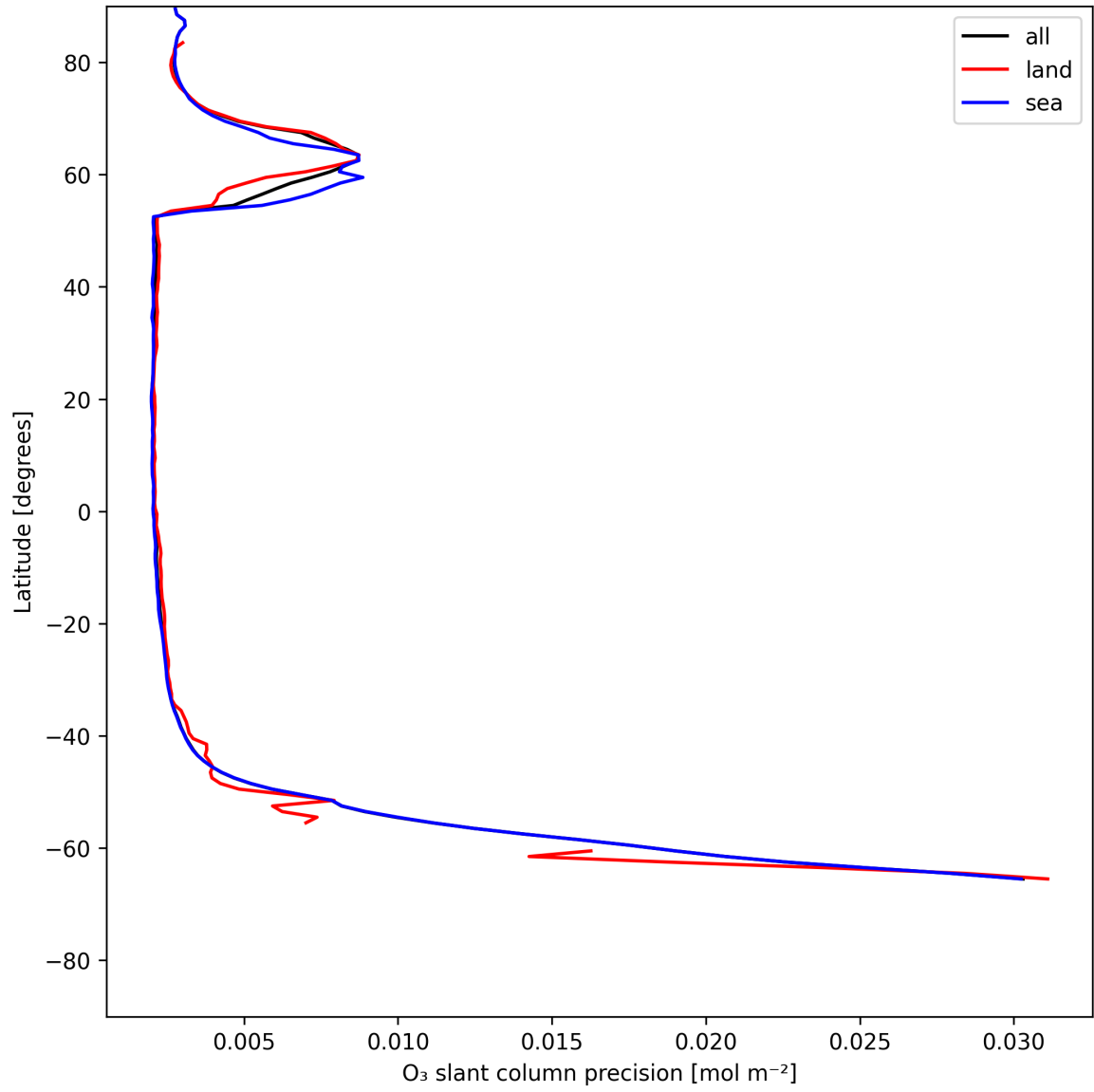
Figure 20: Zonal average of “O 3 slant column precision” for 2025-06-17 to 2025-06-17.
