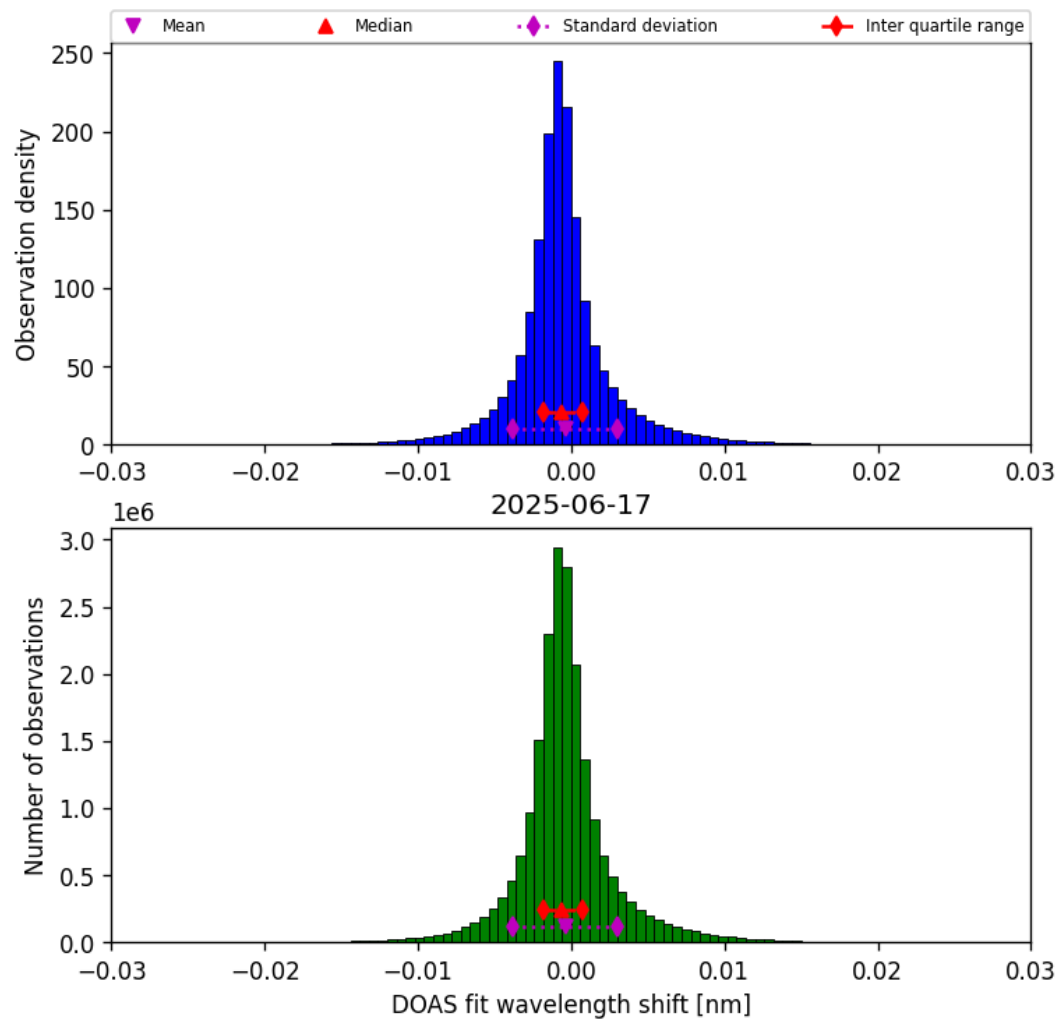
Figure 35: Histogram of “DOAS fit wavelength shift” for 2025-06-17 to 2025-06-17
