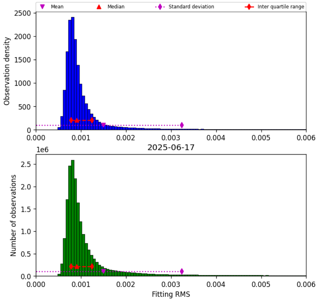
Figure 34: Histogram of “Fitting RMS” for 2025-06-17 to 2025-06-17
