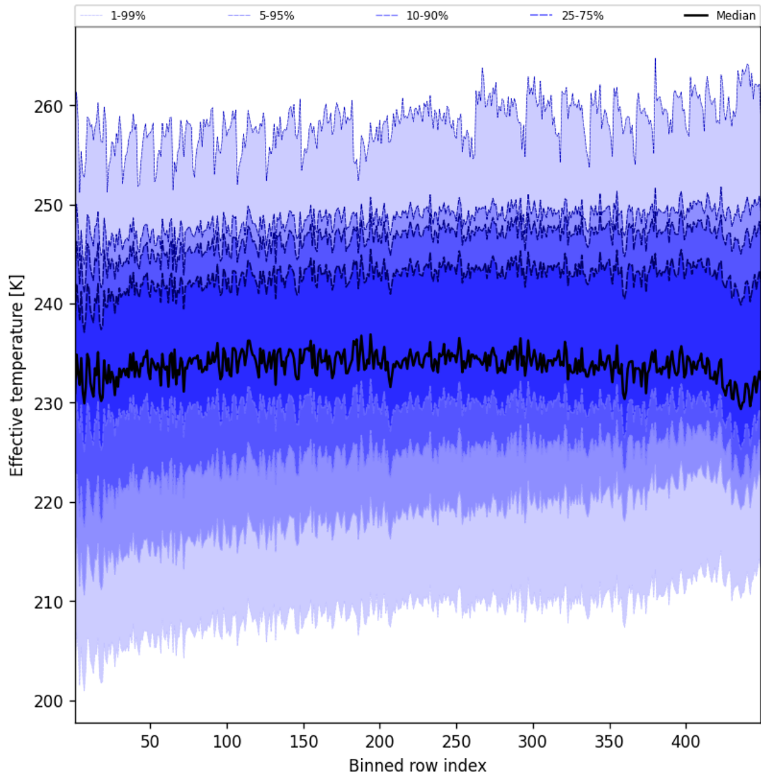
Figure 50: Along track statistics of “Effective temperature” for 2025-06-17 to 2025-06-17
