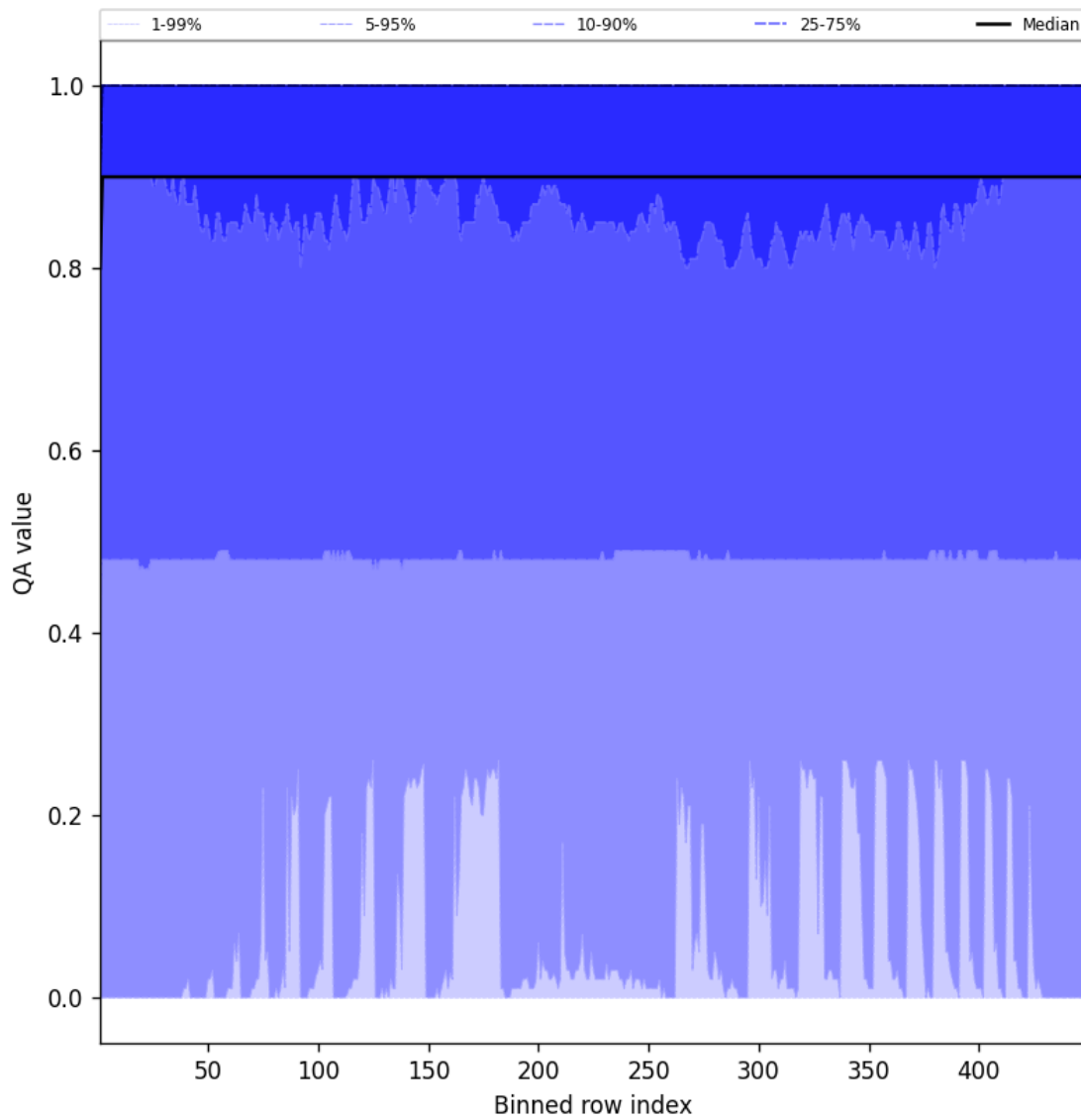
Figure 40: Along track statistics of “QA value” for 2025-06-17 to 2025-06-17
