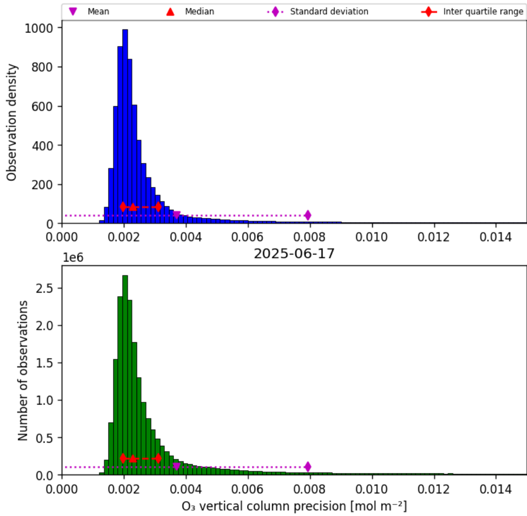
Figure 30: Histogram of “O 3 vertical column precision” for 2025-06-17 to 2025-06-17
