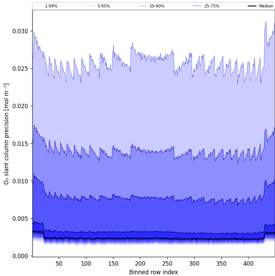
Figure 44: Along track statistics of “O 3 slant column precision” for 2025-06-18 to 2025-06-19
