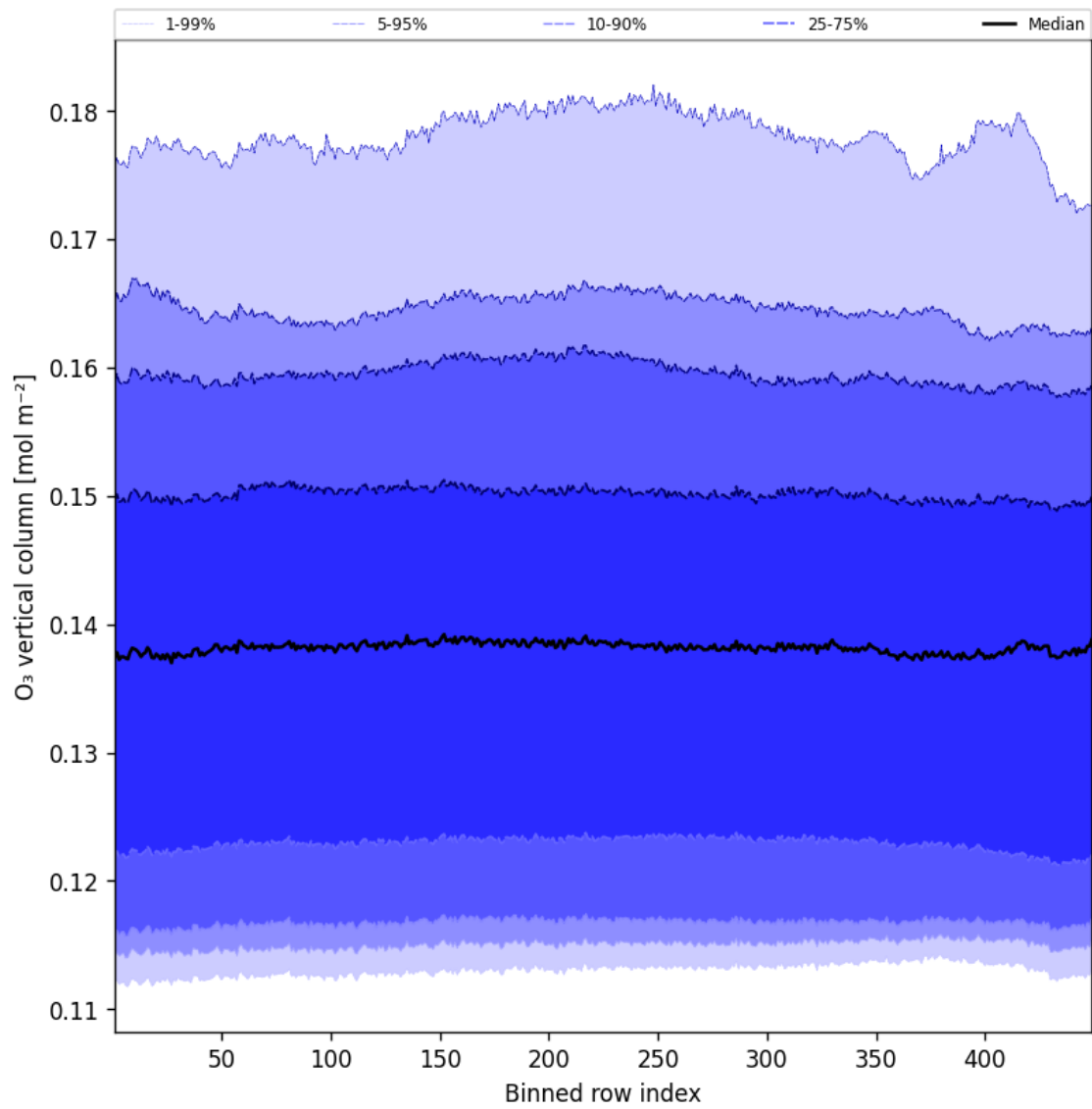
Figure 41: Along track statistics of “O 3 vertical column” for 2025-06-18 to 2025-06-19
