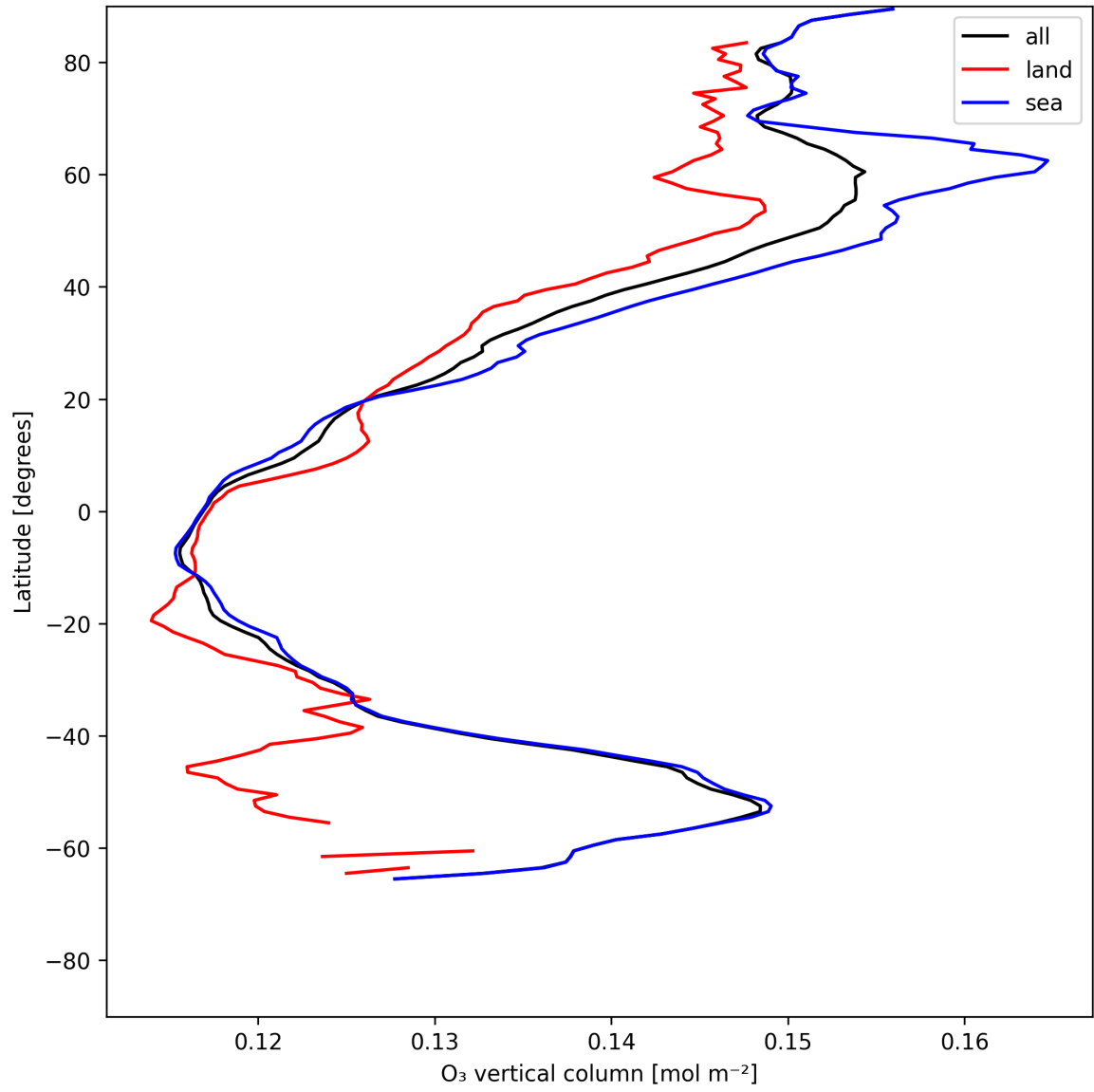
Figure 17: Zonal average of “O 3 vertical column” for 2025-06-18 to 2025-06-19.
