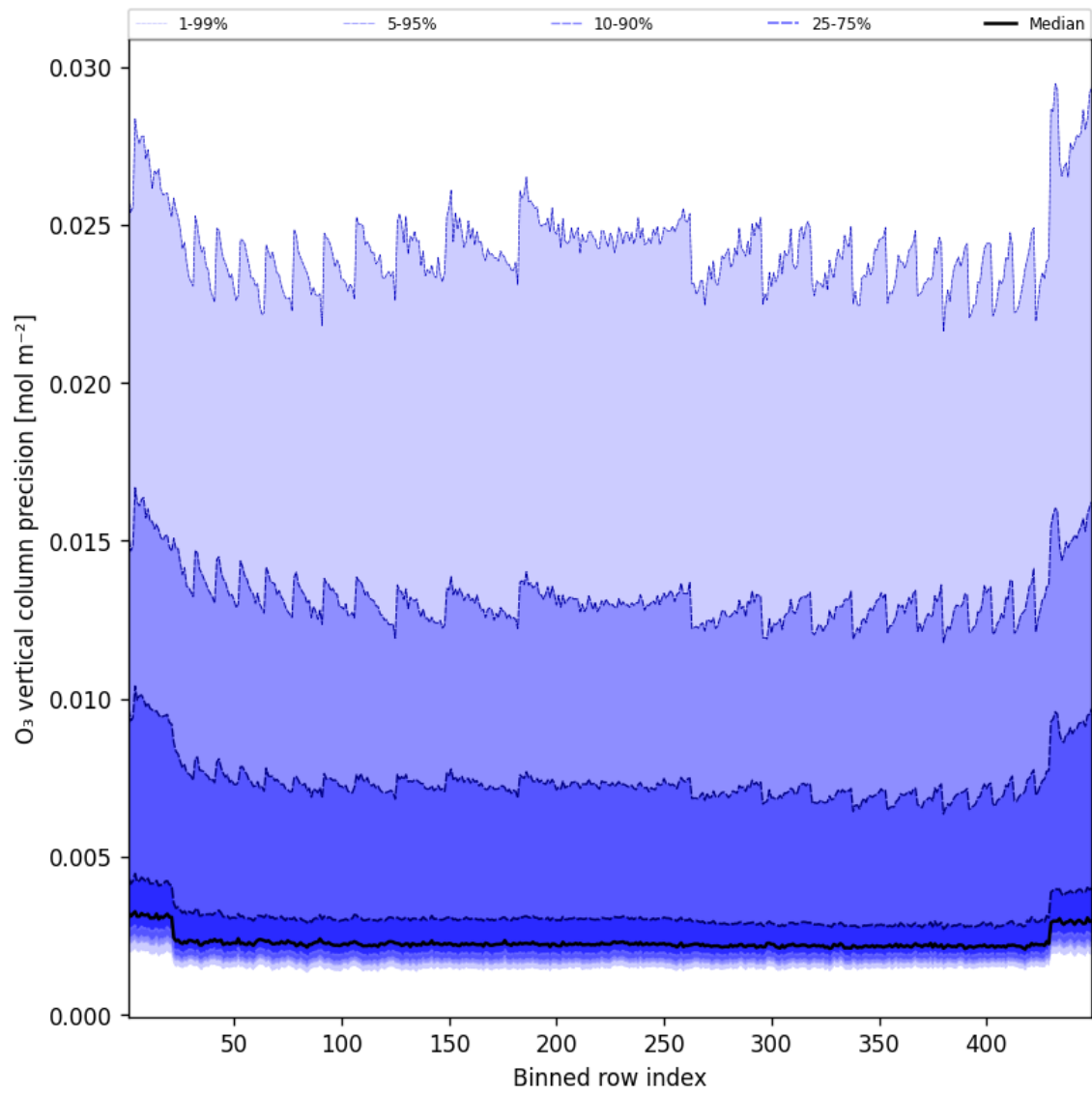
Figure 42: Along track statistics of “O 3 vertical column precision” for 2025-06-18 to 2025-06-19
