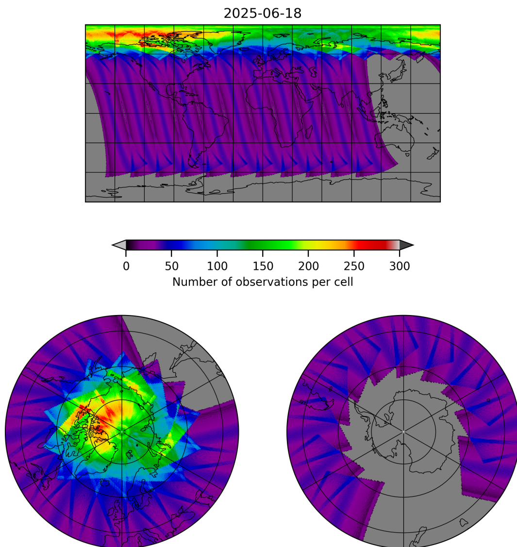
Figure 15: Map of the number of observations for 2025-06-18 to 2025-06-19
