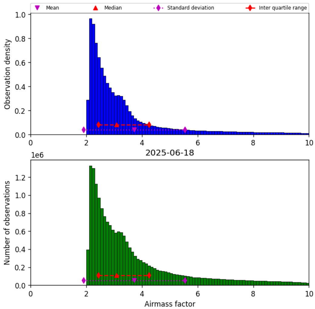
Figure 37: Histogram of “Airmass factor” for 2025-06-18 to 2025-06-19
