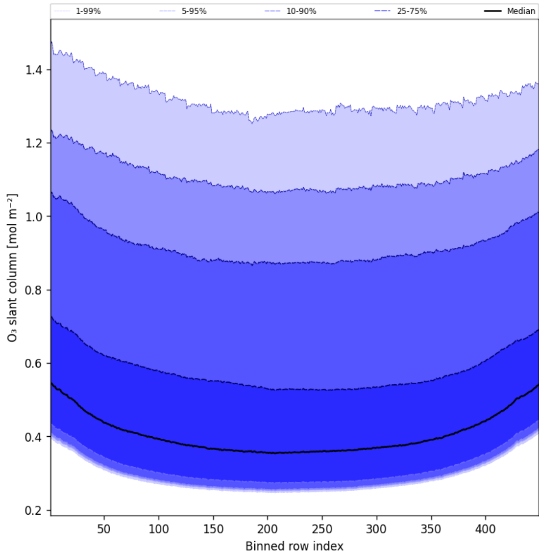
Figure 43: Along track statistics of “O 3 slant column” for 2025-06-18 to 2025-06-19
