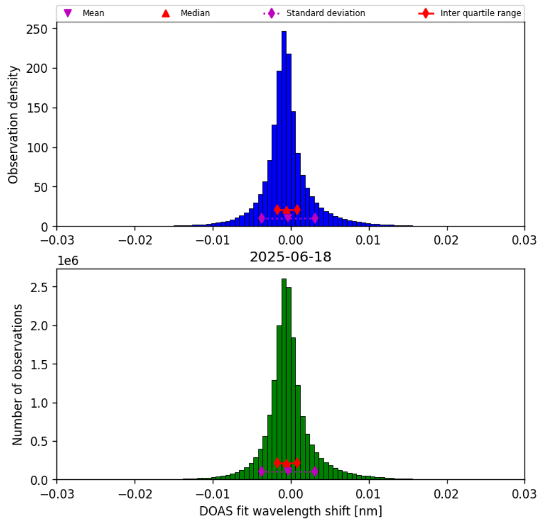
Figure 35: Histogram of “DOAS fit wavelength shift” for 2025-06-18 to 2025-06-19
