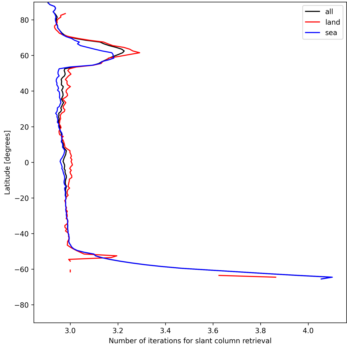
Figure 21: Zonal average of “Number of iterations for slant column retrieval” for 2025-06-18 to 2025-06-19.
