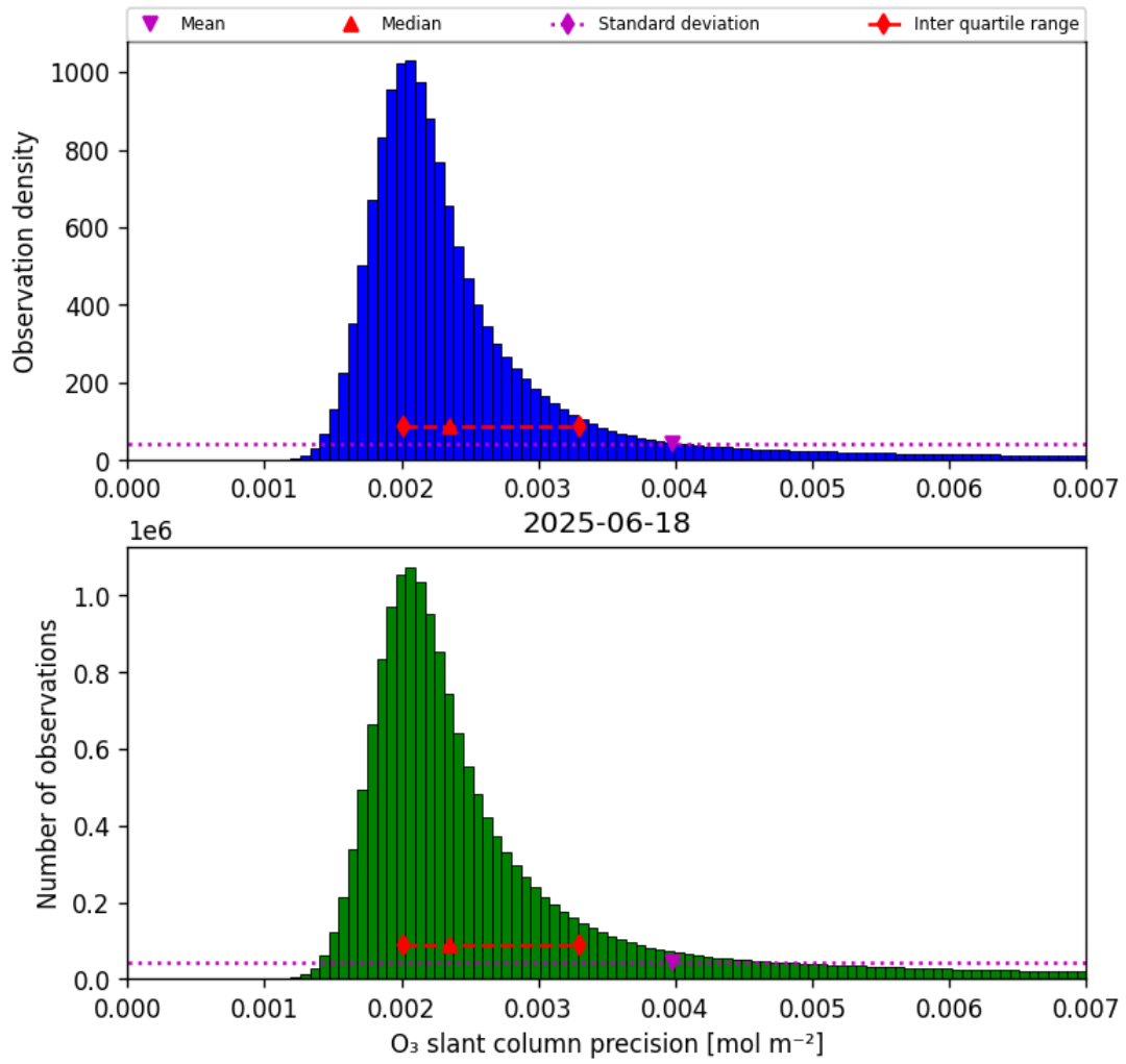
Figure 32: Histogram of “O 3 slant column precision” for 2025-06-18 to 2025-06-19
