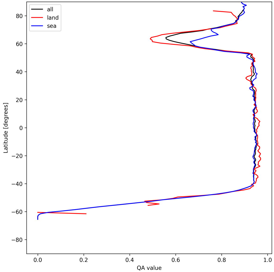
Figure 16: Zonal average of “QA value” for 2025-06-18 to 2025-06-19.
