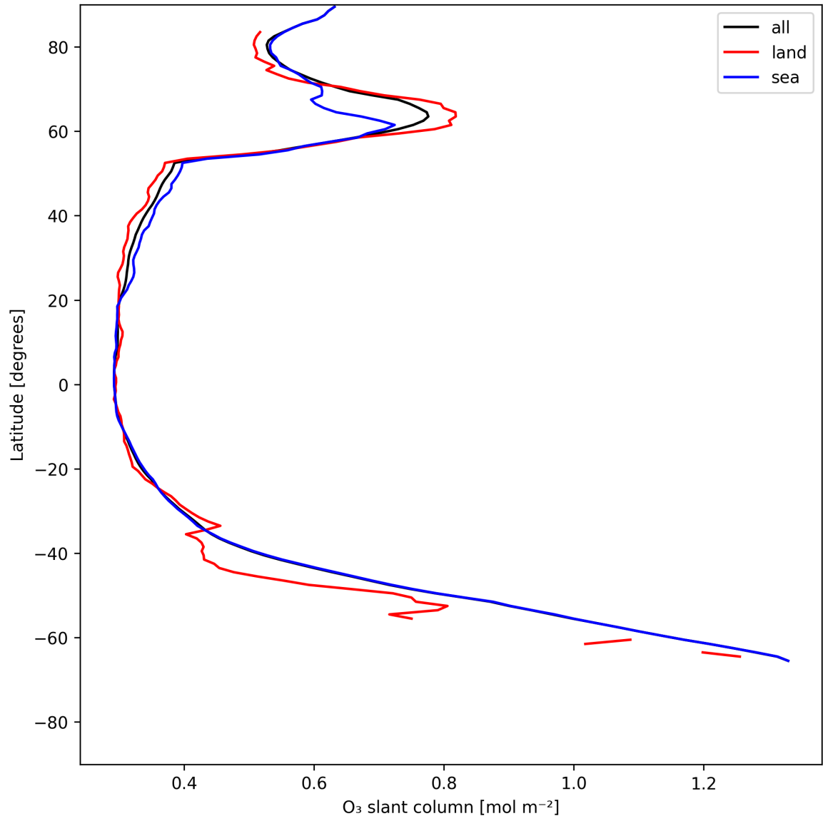
Figure 19: Zonal average of “O 3 slant column” for 2025-06-18 to 2025-06-19.
