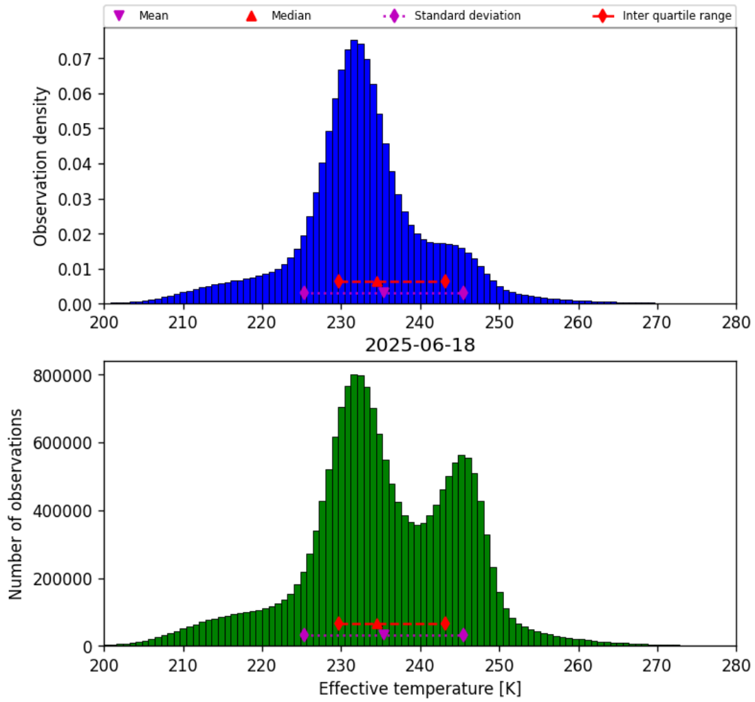
Figure 38: Histogram of “Effective temperature” for 2025-06-18 to 2025-06-19
