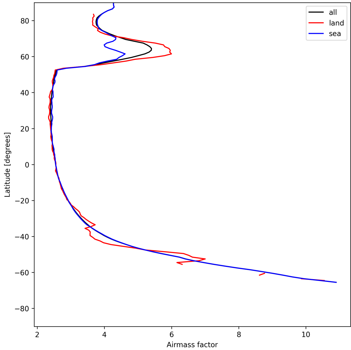
Figure 25: Zonal average of “Airmass factor” for 2025-06-18 to 2025-06-19.
