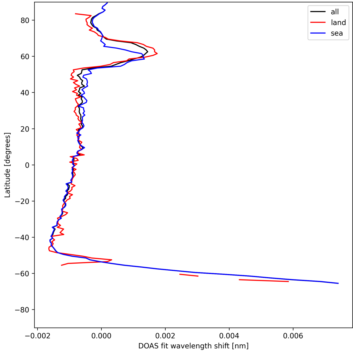
Figure 23: Zonal average of “DOAS fit wavelength shift” for 2025-06-18 to 2025-06-19.
