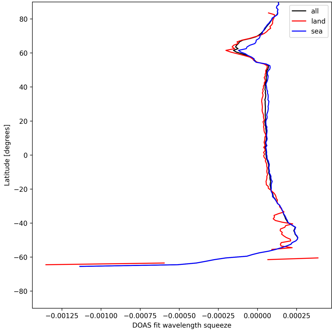
Figure 24: Zonal average of “DOAS fit wavelength squeeze” for 2025-06-18 to 2025-06-19.
