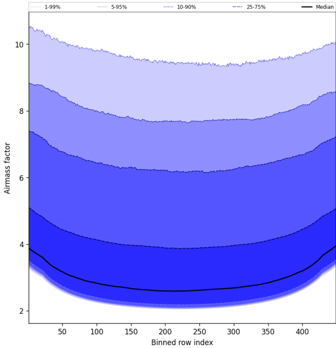
Figure 49: Along track statistics of “Airmass factor” for 2025-06-18 to 2025-06-19
