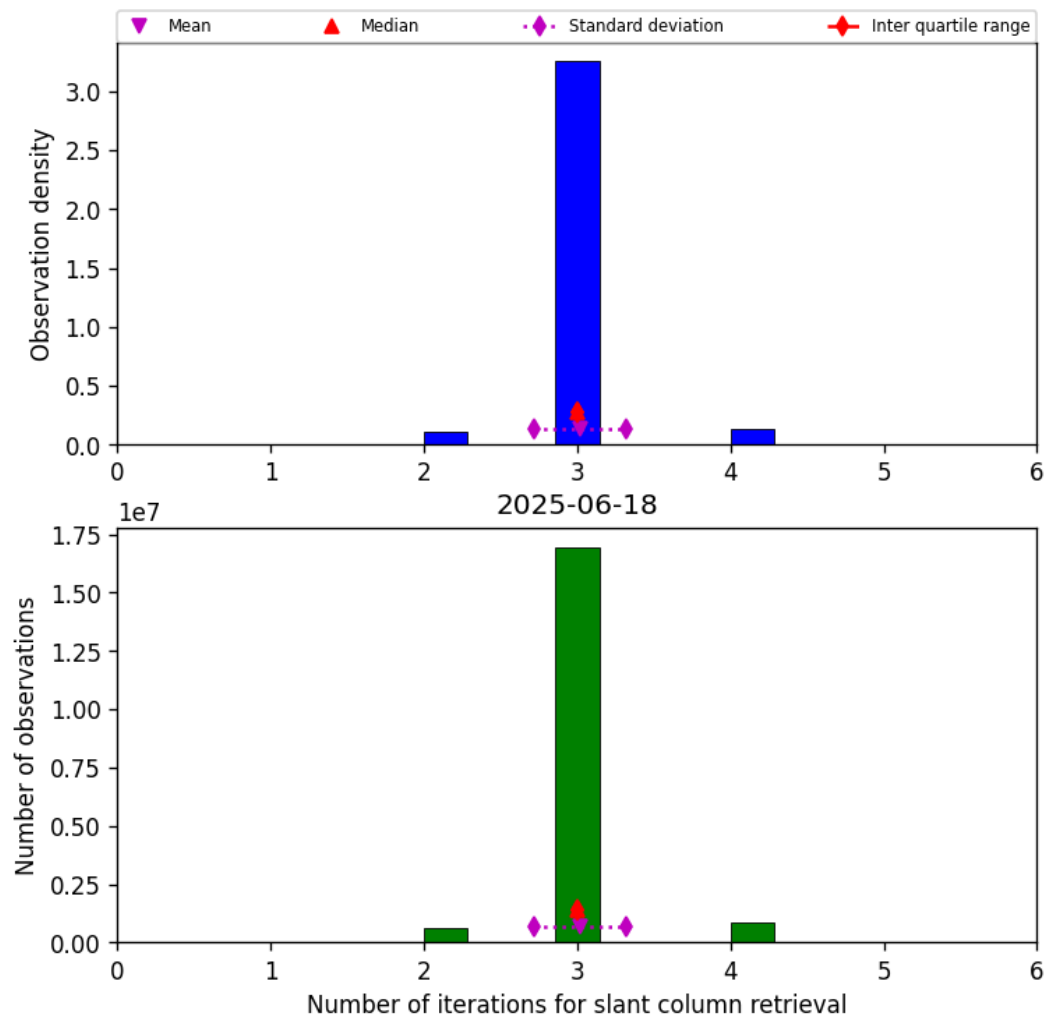
Figure 33: Histogram of “Number of iterations for slant column retrieval” for 2025-06-18 to 2025-06-19
