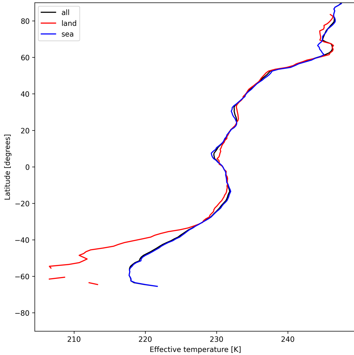
Figure 26: Zonal average of “Effective temperature” for 2025-06-18 to 2025-06-19.
