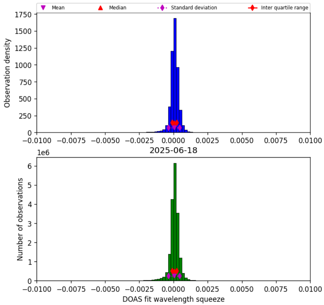
Figure 36: Histogram of “DOAS fit wavelength squeeze” for 2025-06-18 to 2025-06-19
