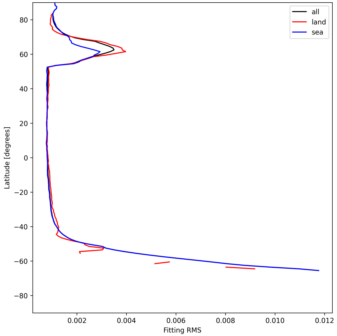
Figure 22: Zonal average of “Fitting RMS” for 2025-06-18 to 2025-06-19.
