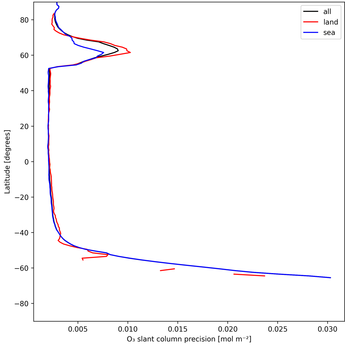
Figure 20: Zonal average of "O 3 slant column precision" for 2025-06-18 to 2025-06-19.
