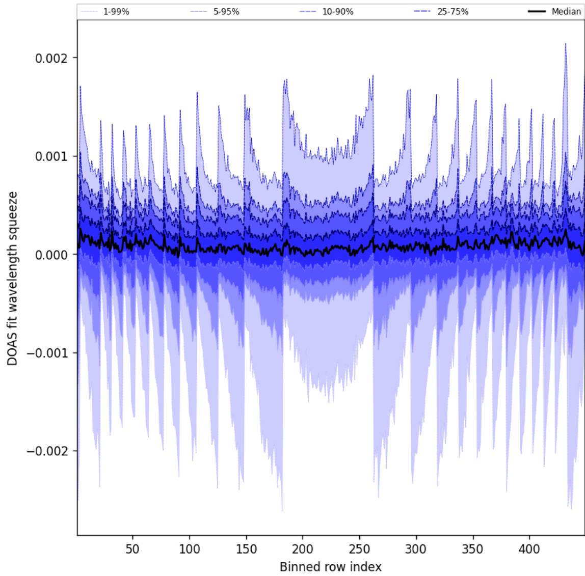
Figure 48: Along track statistics of “DOAS fit wavelength squeeze” for 2025-06-18 to 2025-06-19
