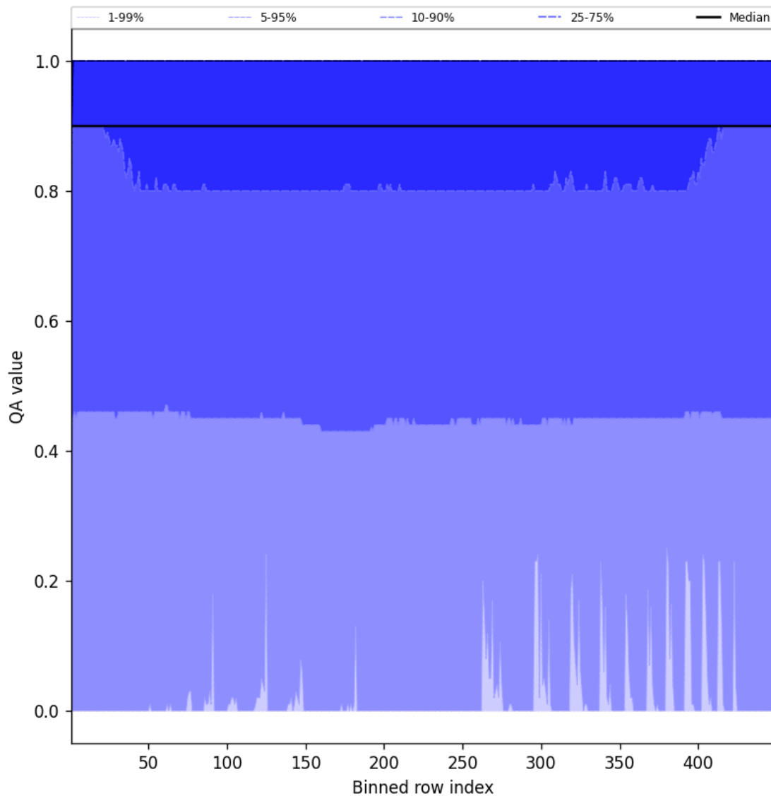
Figure 40: Along track statistics of “QA value” for 2025-06-18 to 2025-06-19
