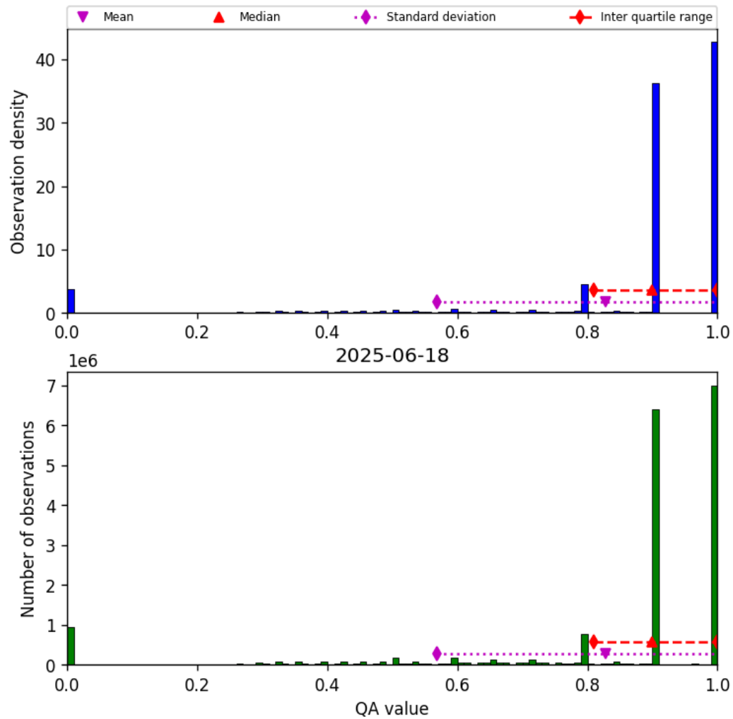
Figure 28: Histogram of “QA value” for 2025-06-18 to 2025-06-19
