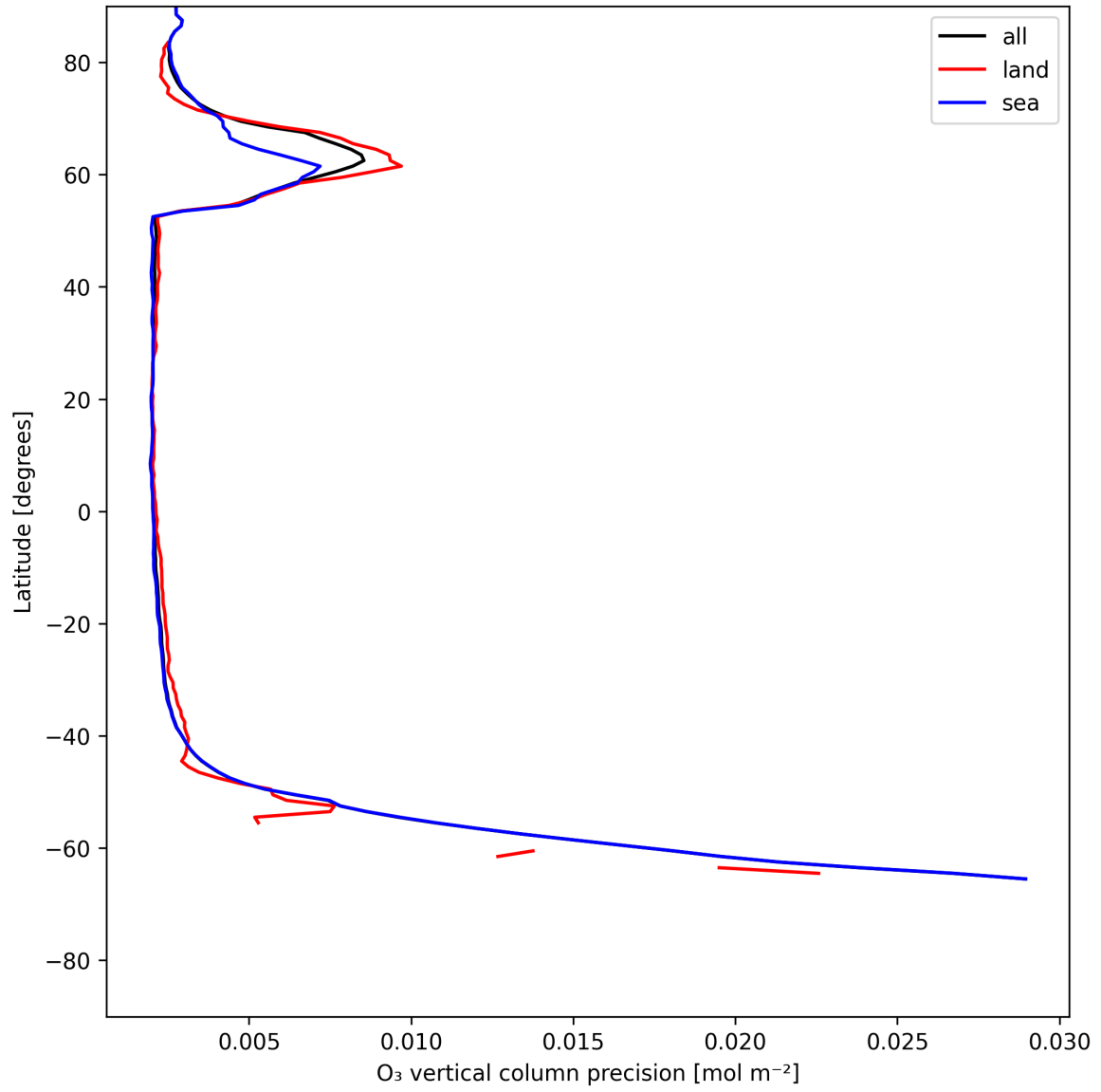
Figure 18: Zonal average of "O 3 vertical column precision" for 2025-06-18 to 2025-06-19.
