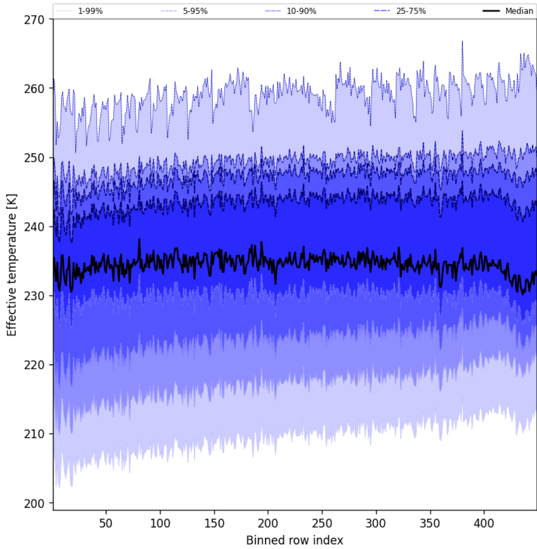
Figure 50: Along track statistics of “Effective temperature” for 2025-06-18 to 2025-06-19
