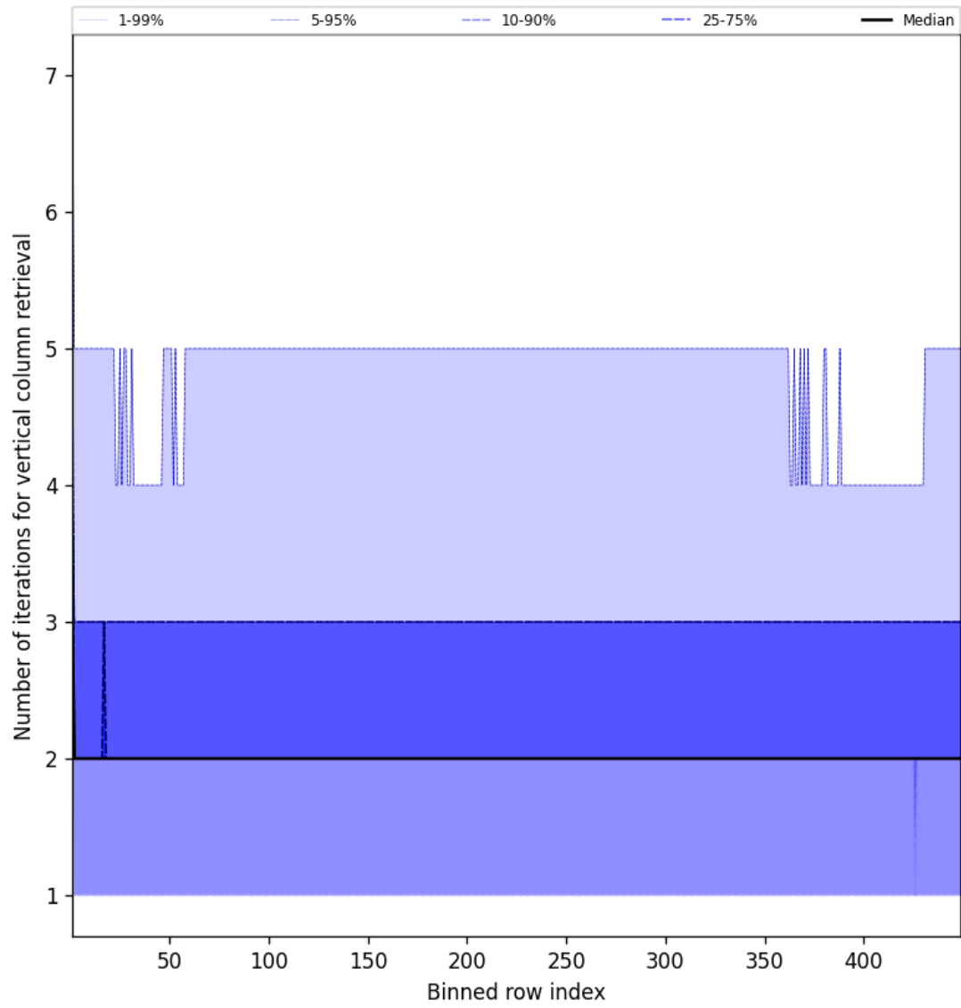
Figure 51: Along track statistics of “Number of iterations for vertical column retrieval” for 2025-06-18 to 2025-06-19
