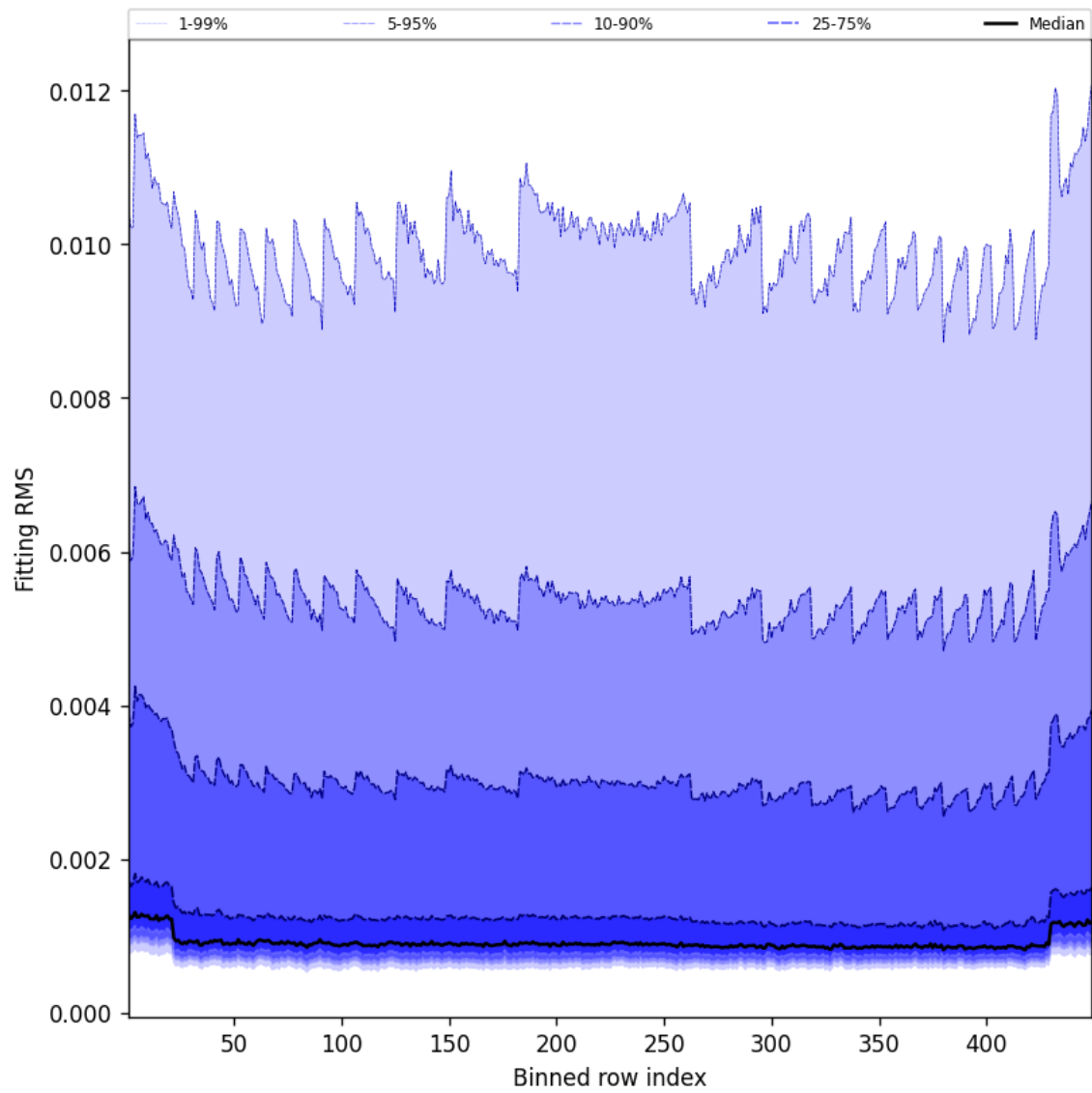
Figure 46: Along track statistics of “Fitting RMS” for 2025-06-18 to 2025-06-19
