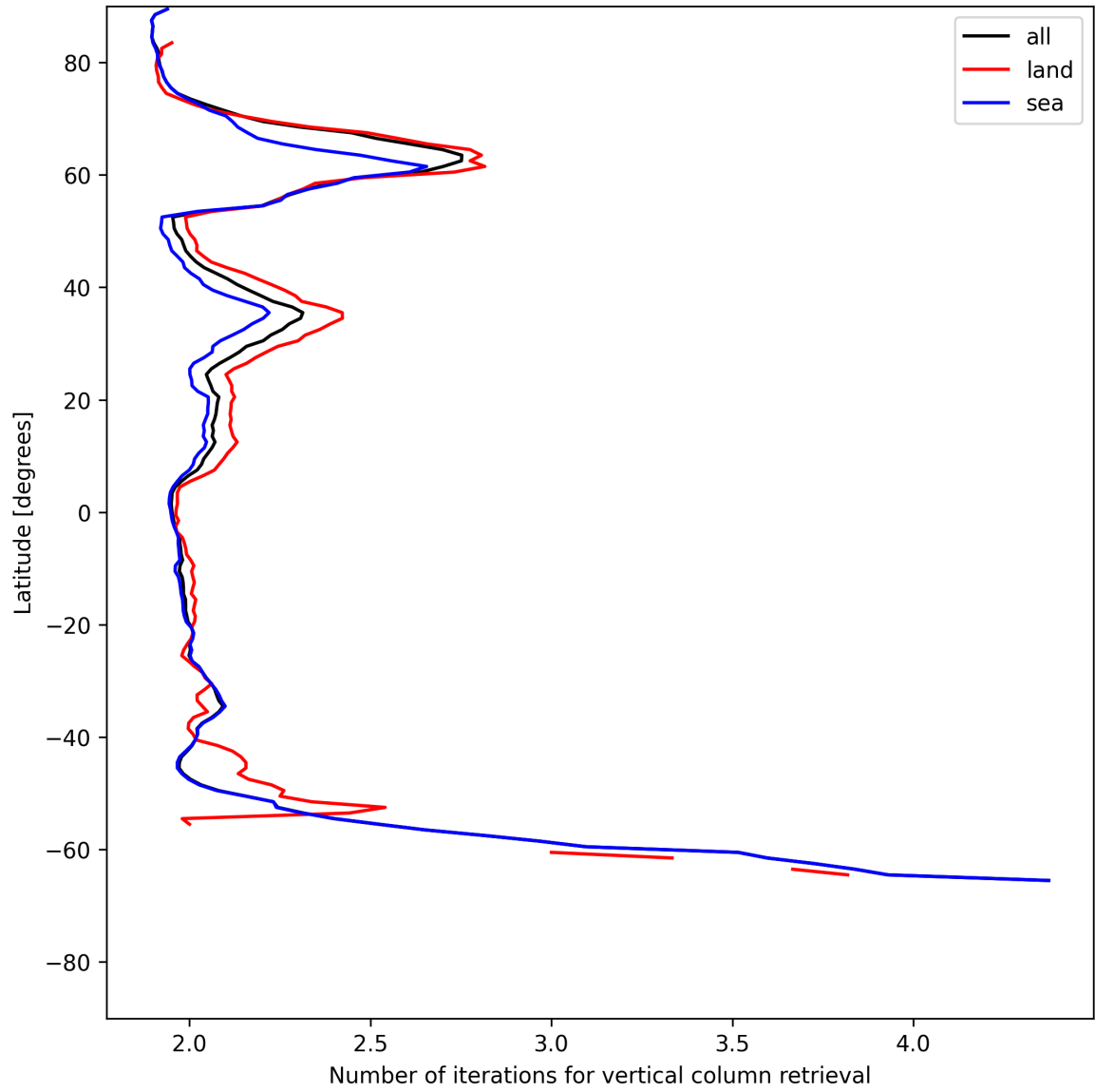
Figure 27: Zonal average of “Number of iterations for vertical column retrieval” for 2025-06-18 to 2025-06-19.
