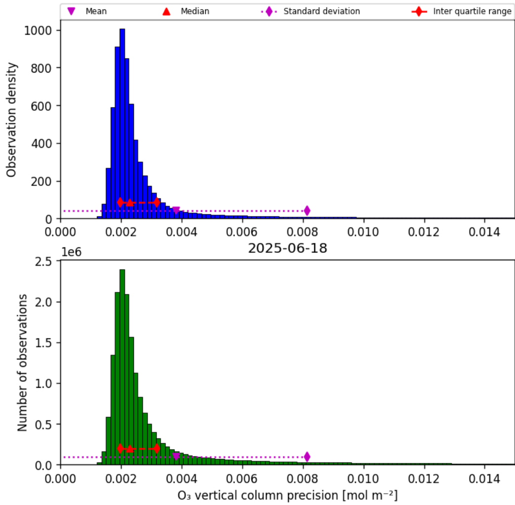
Figure 30: Histogram of “O 3 vertical column precision” for 2025-06-18 to 2025-06-19
