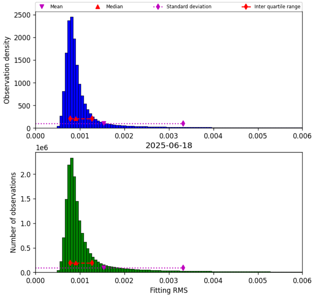
Figure 34: Histogram of “Fitting RMS” for 2025-06-18 to 2025-06-19
