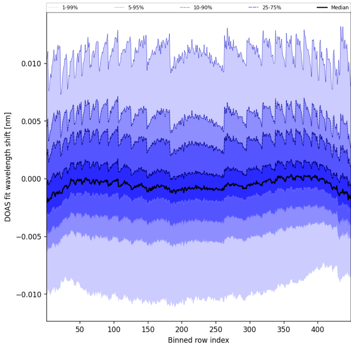
Figure 47: Along track statistics of “DOAS fit wavelength shift” for 2025-06-18 to 2025-06-19
