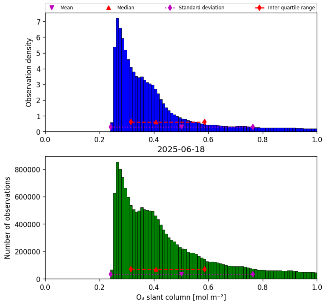
Figure 31: Histogram of “O 3 slant column” for 2025-06-18 to 2025-06-19
