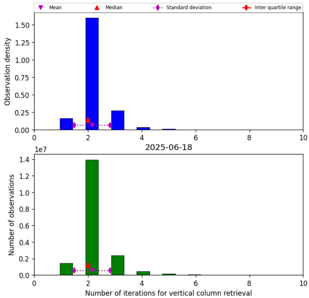
Figure 39: Histogram of “Number of iterations for vertical column retrieval” for 2025-06-18 to 2025-06-19
