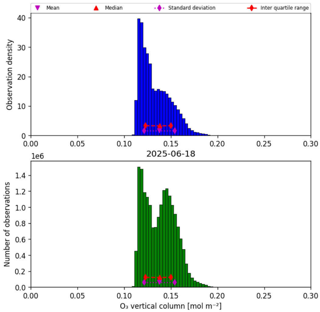
Figure 29: Histogram of “O 3 vertical column” for 2025-06-18 to 2025-06-19
