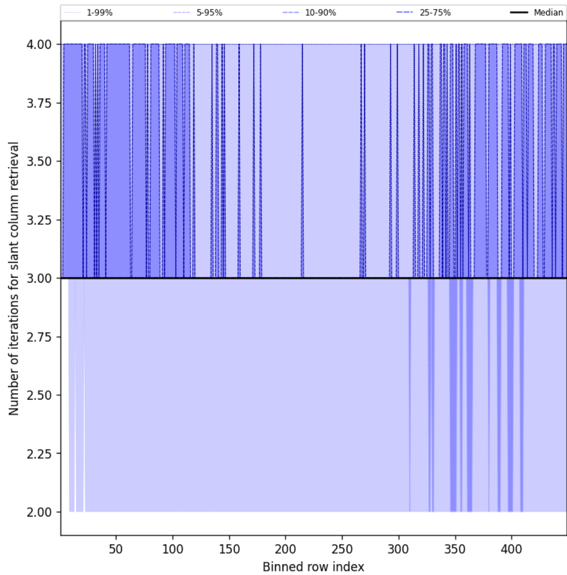
Figure 45: Along track statistics of “Number of iterations for slant column retrieval” for 2025-06-18 to 2025-06-19
