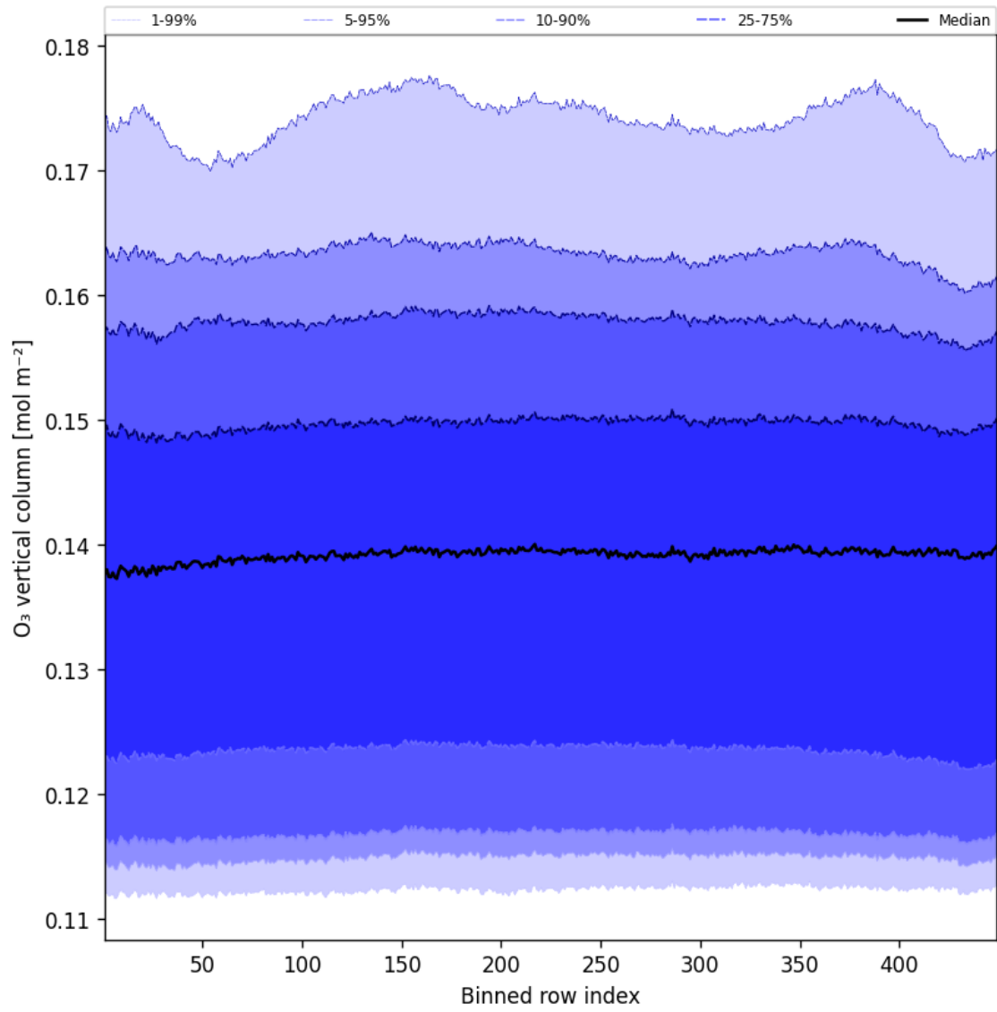
Figure 41: Along track statistics of “O 3 vertical column” for 2025-06-19 to 2025-06-20
