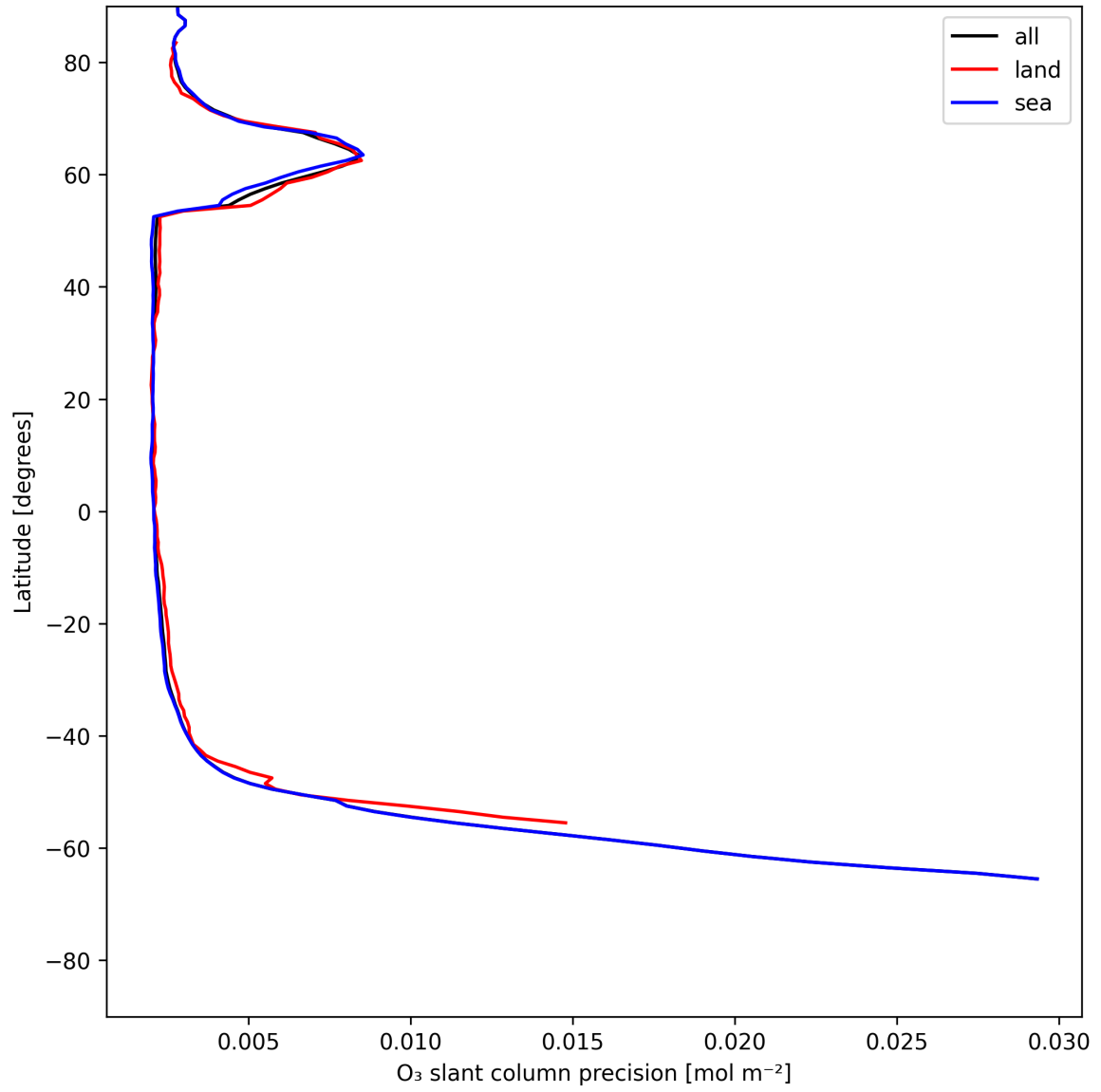
Figure 20: Zonal average of “O 3 slant column precision” for 2025-06-19 to 2025-06-20.
