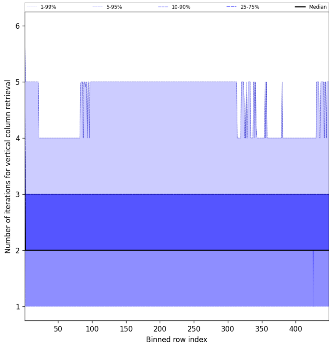
Figure 51: Along track statistics of “Number of iterations for vertical column retrieval” for 2025-06-19 to 2025-06-20
