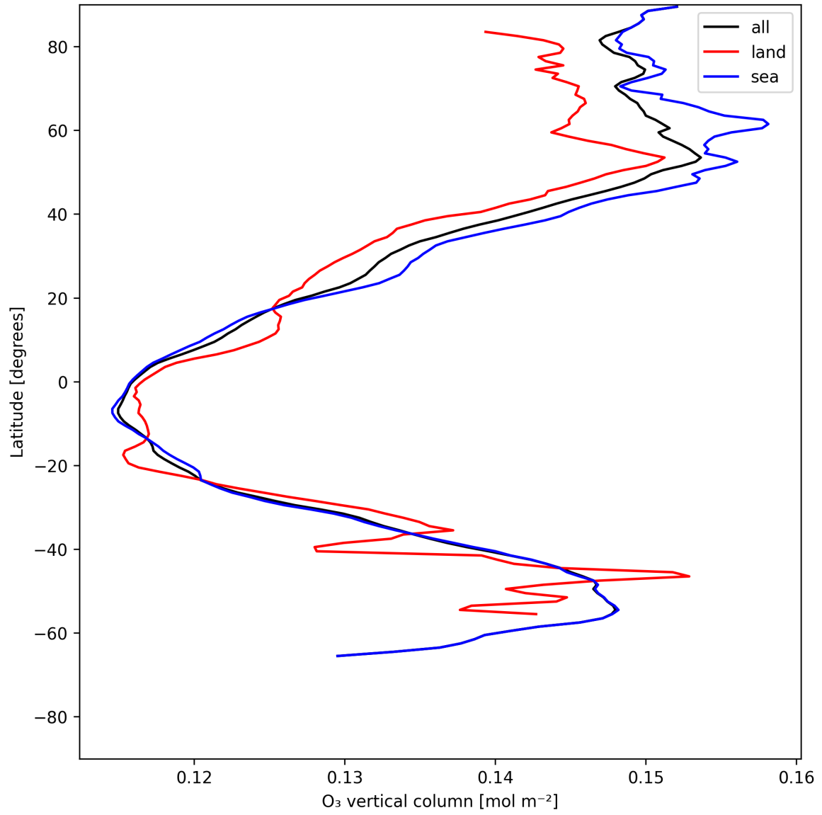
Figure 17: Zonal average of “O 3 vertical column” for 2025-06-19 to 2025-06-20.
