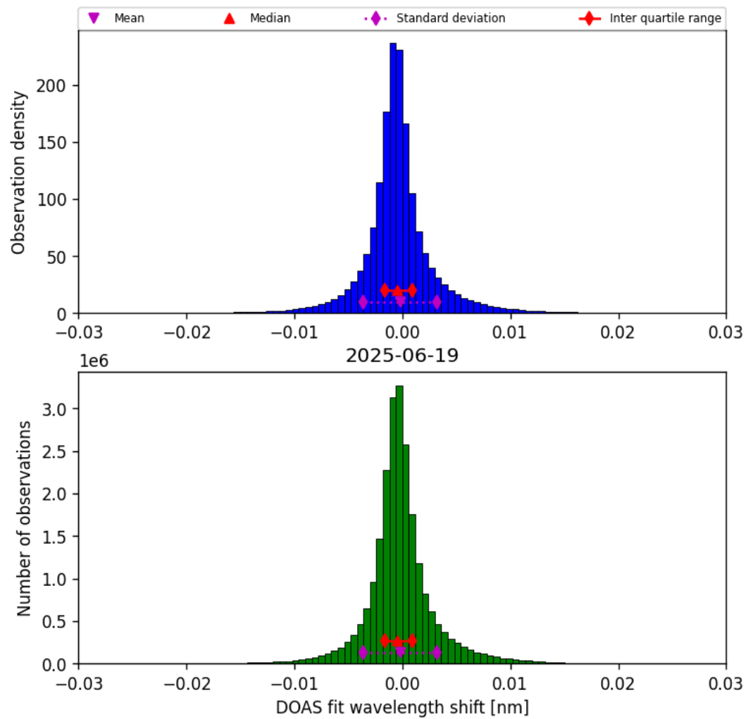
Figure 35: Histogram of “DOAS fit wavelength shift” for 2025-06-19 to 2025-06-20
