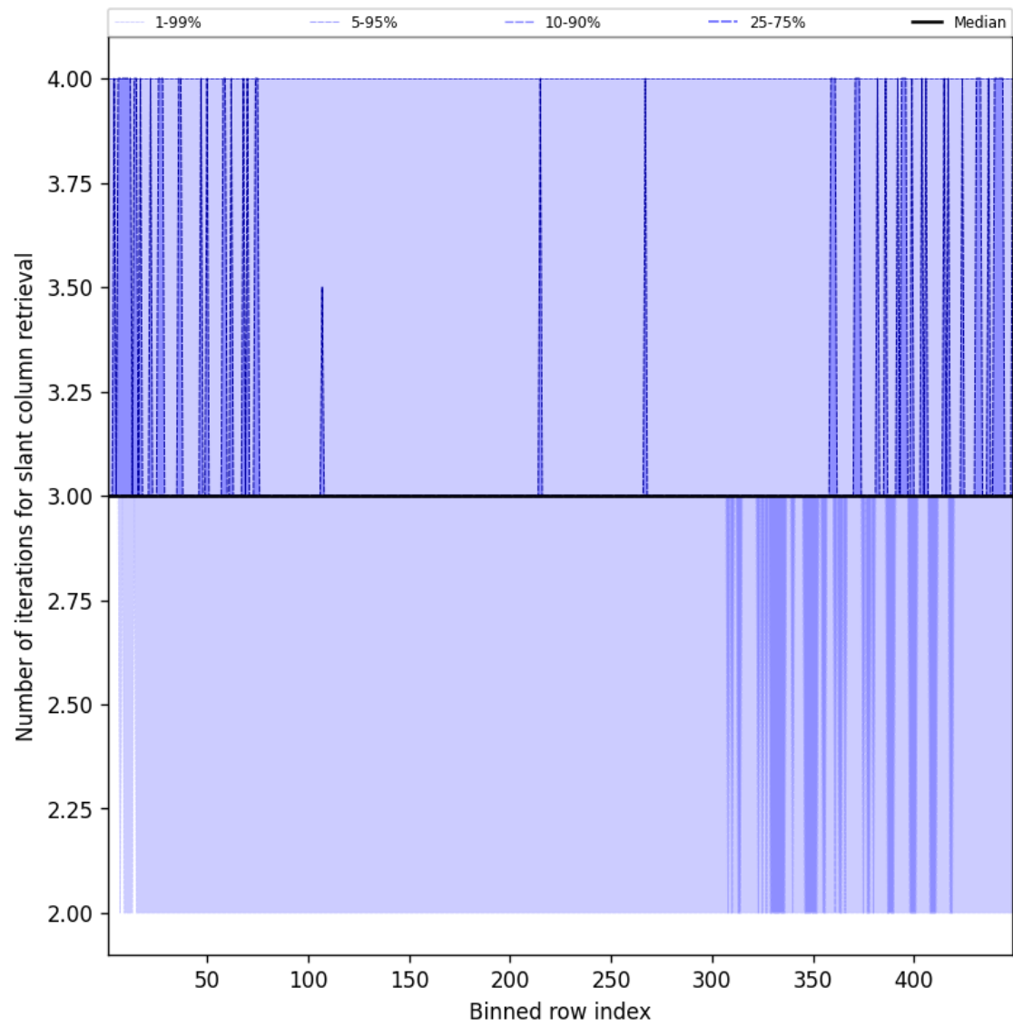
Figure 45: Along track statistics of “Number of iterations for slant column retrieval” for 2025-06-19 to 2025-06-20
