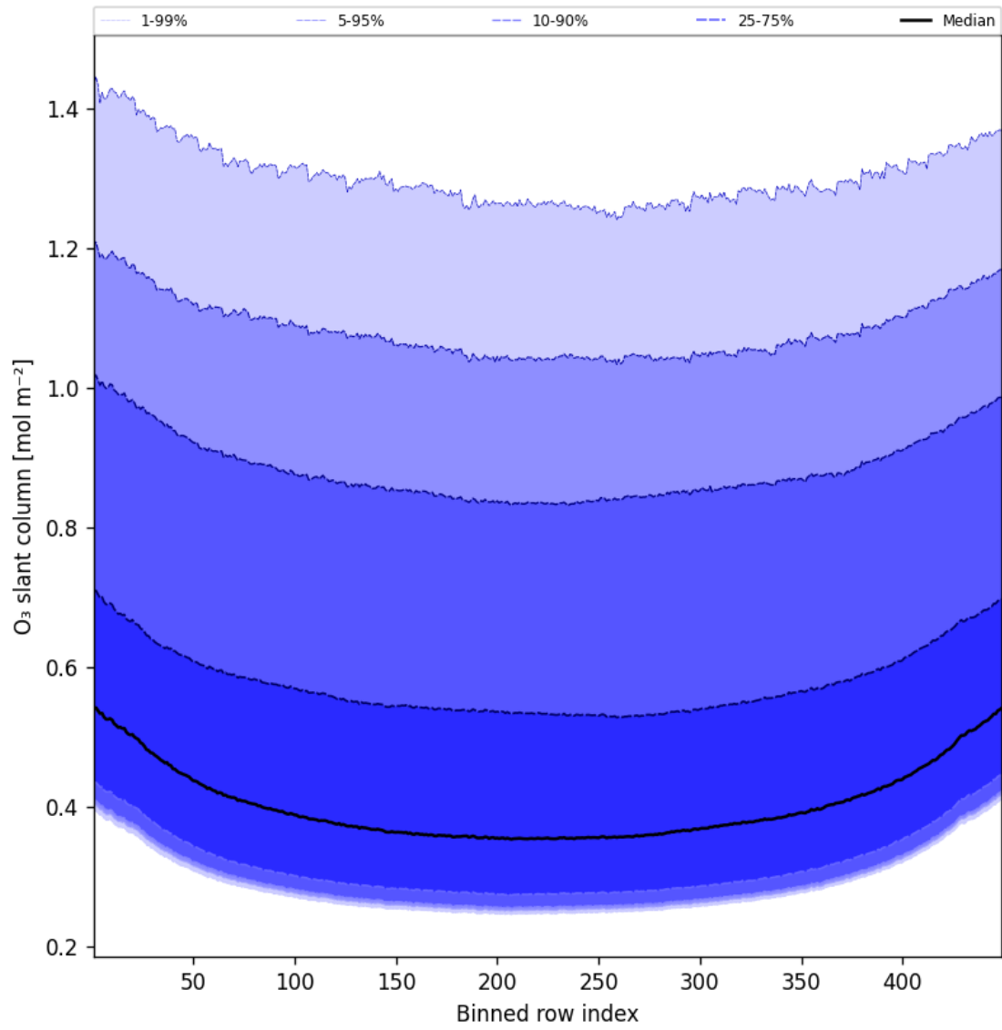
Figure 43: Along track statistics of “O 3 slant column” for 2025-06-19 to 2025-06-20
