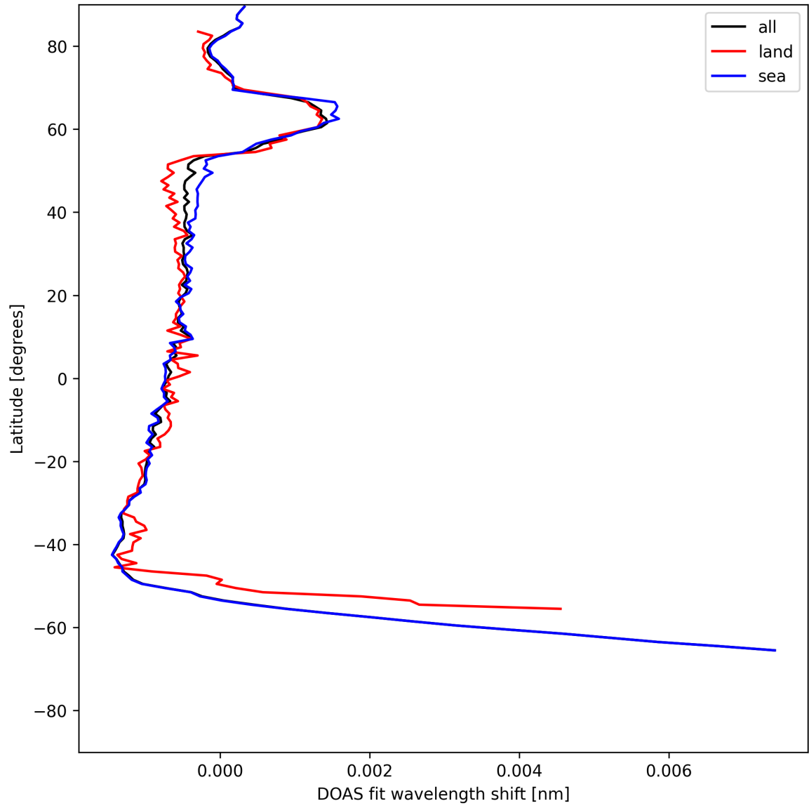
Figure 23: Zonal average of “DOAS fit wavelength shift” for 2025-06-19 to 2025-06-20.
