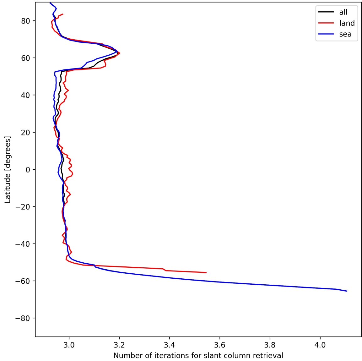
Figure 21: Zonal average of “Number of iterations for slant column retrieval” for 2025-06-19 to 2025-06-20.
