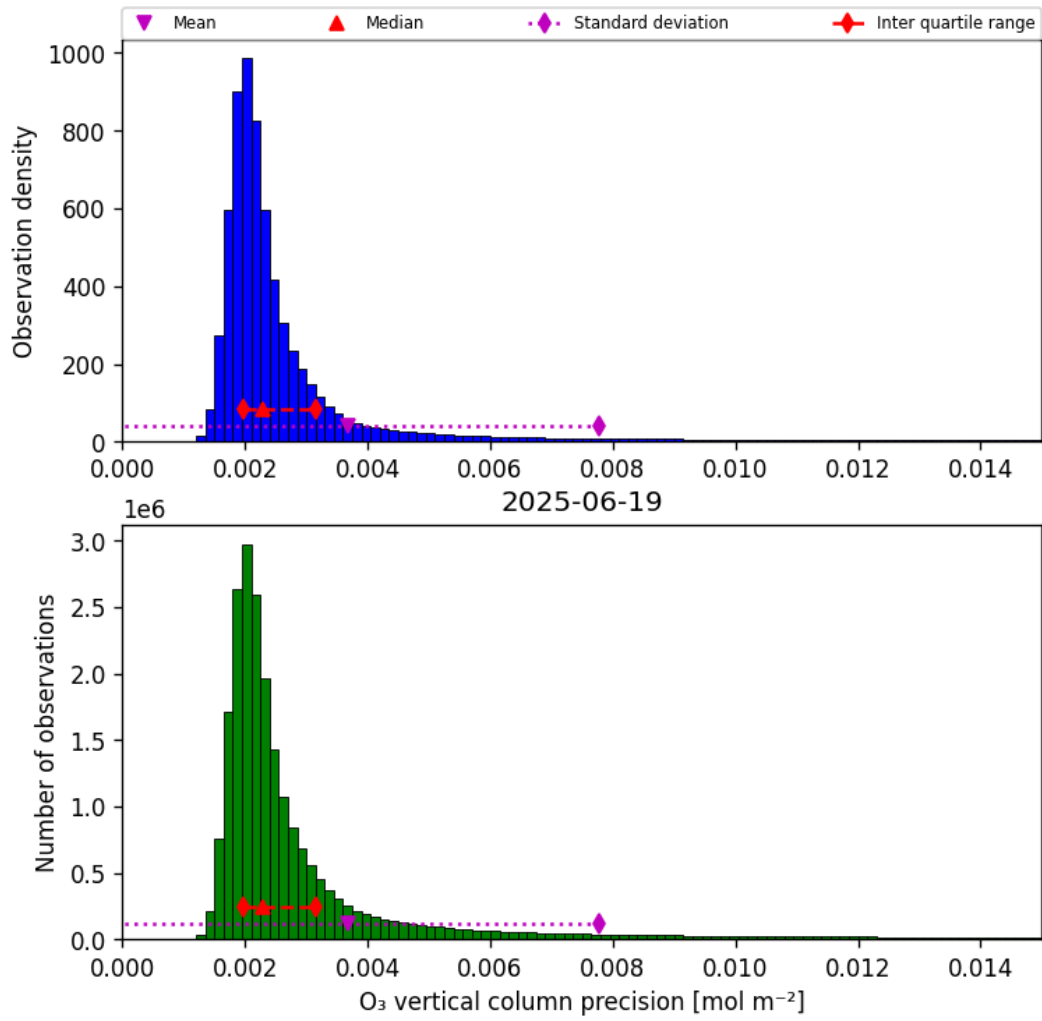
Figure 30: Histogram of “O 3 vertical column precision” for 2025-06-19 to 2025-06-20
