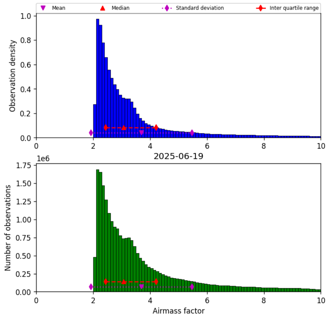
Figure 37: Histogram of “Airmass factor” for 2025-06-19 to 2025-06-20
