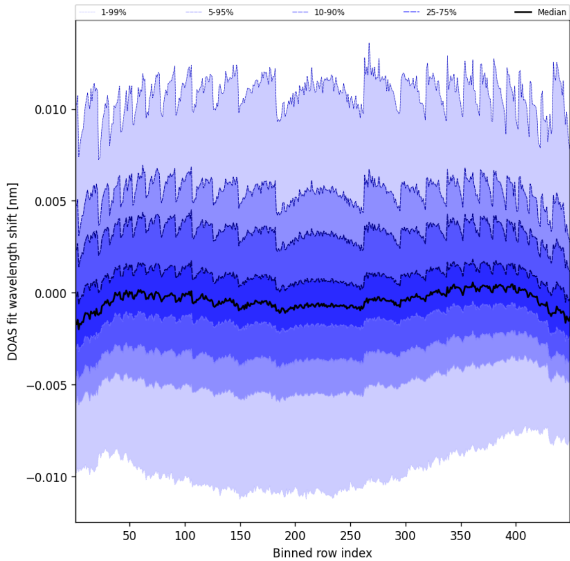
Figure 47: Along track statistics of “DOAS fit wavelength shift” for 2025-06-19 to 2025-06-20
