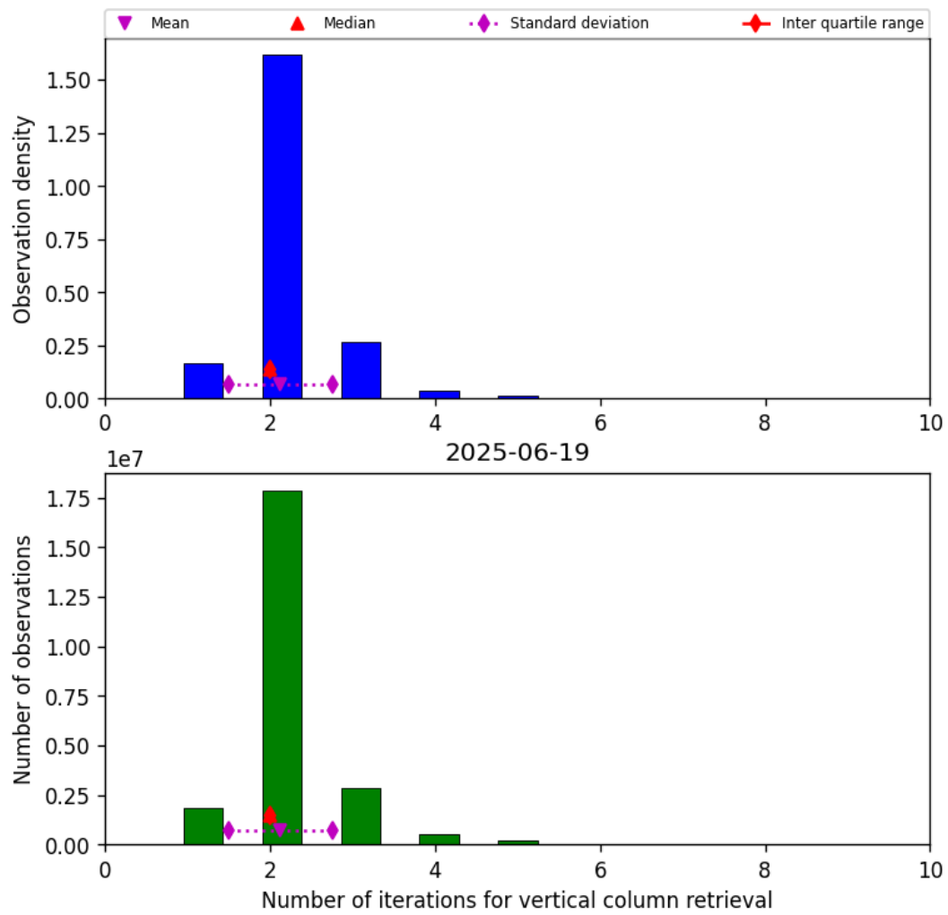
Figure 39: Histogram of “Number of iterations for vertical column retrieval” for 2025-06-19 to 2025-06-20
