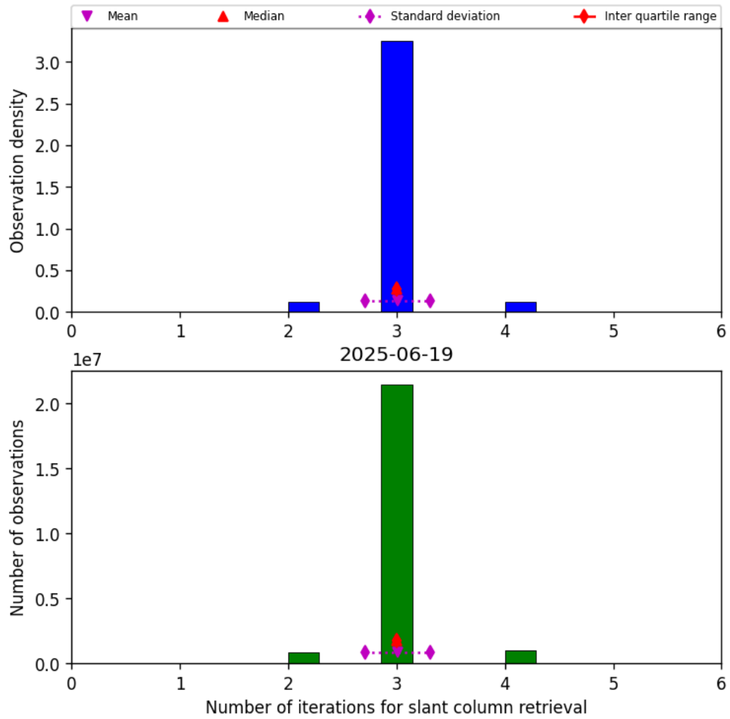
Figure 33: Histogram of "Number of iterations for slant column retrieval" for 2025-06-19 to 2025-06-20
