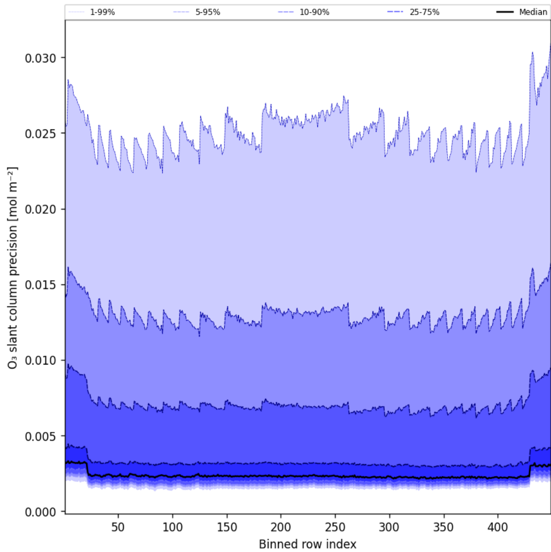
Figure 44: Along track statistics of “O 3 slant column precision” for 2025-06-19 to 2025-06-20
