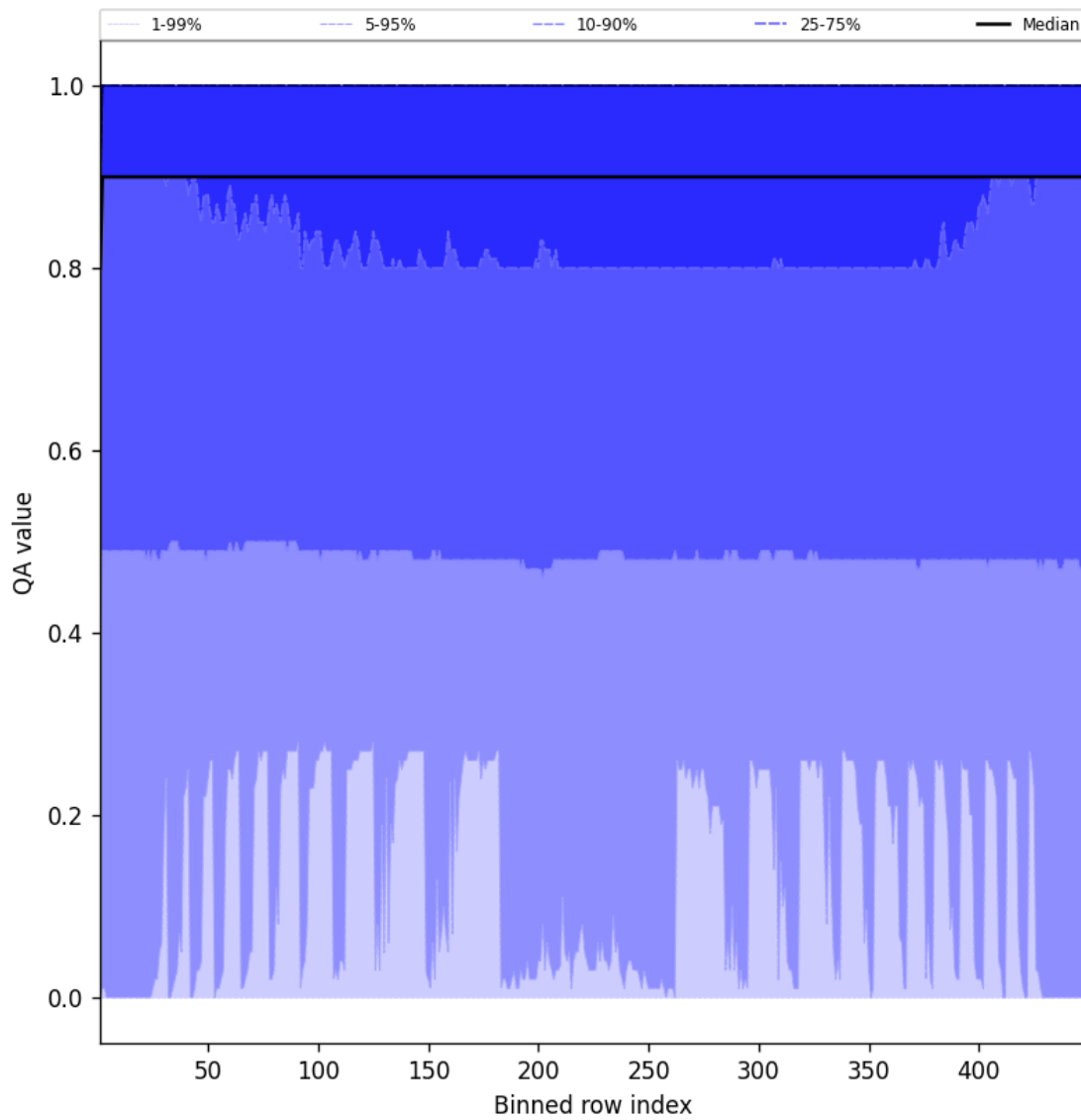
Figure 40: Along track statistics of “QA value” for 2025-06-19 to 2025-06-20
