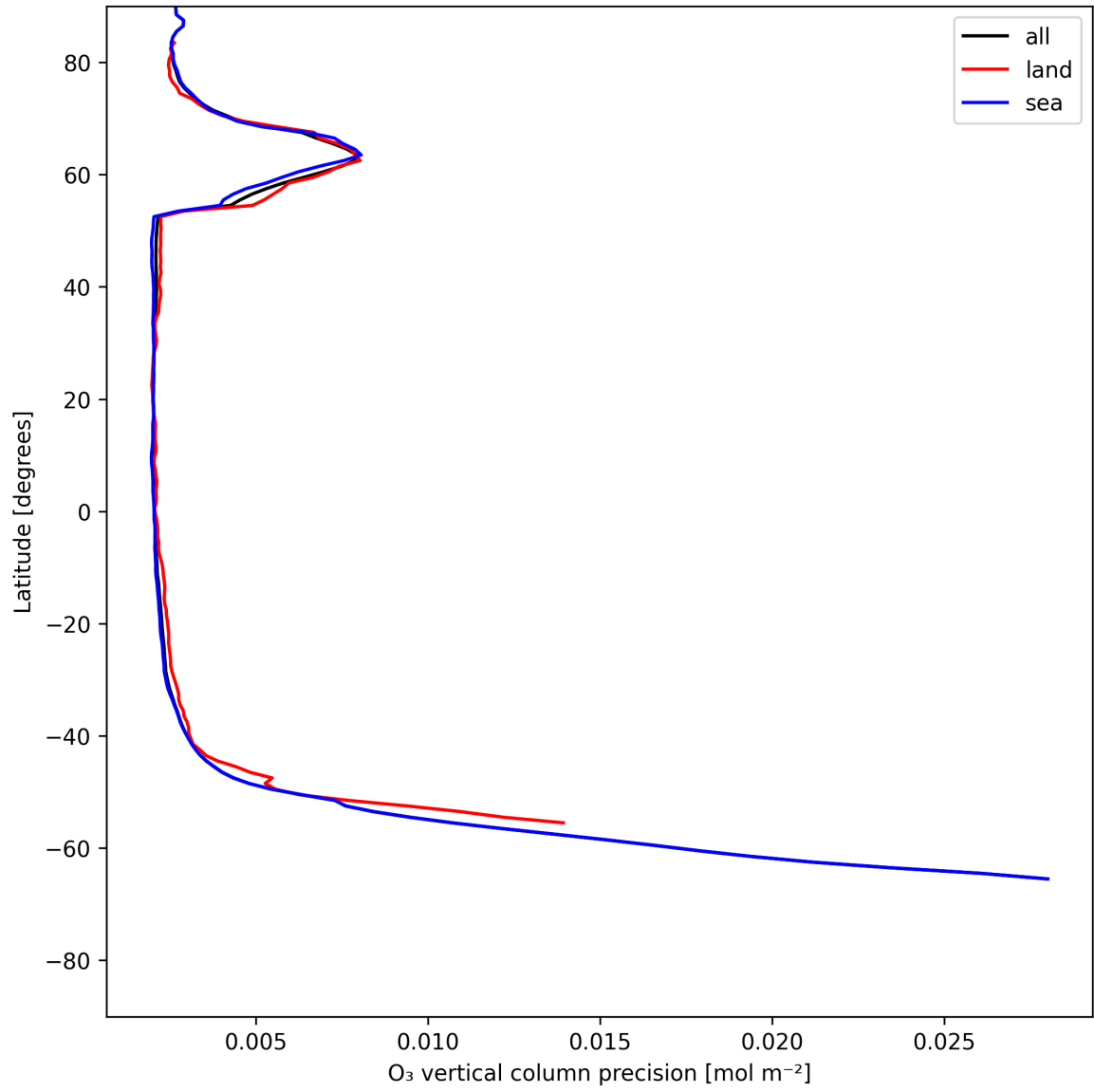
Figure 18: Zonal average of “O 3 vertical column precision” for 2025-06-19 to 2025-06-20.
