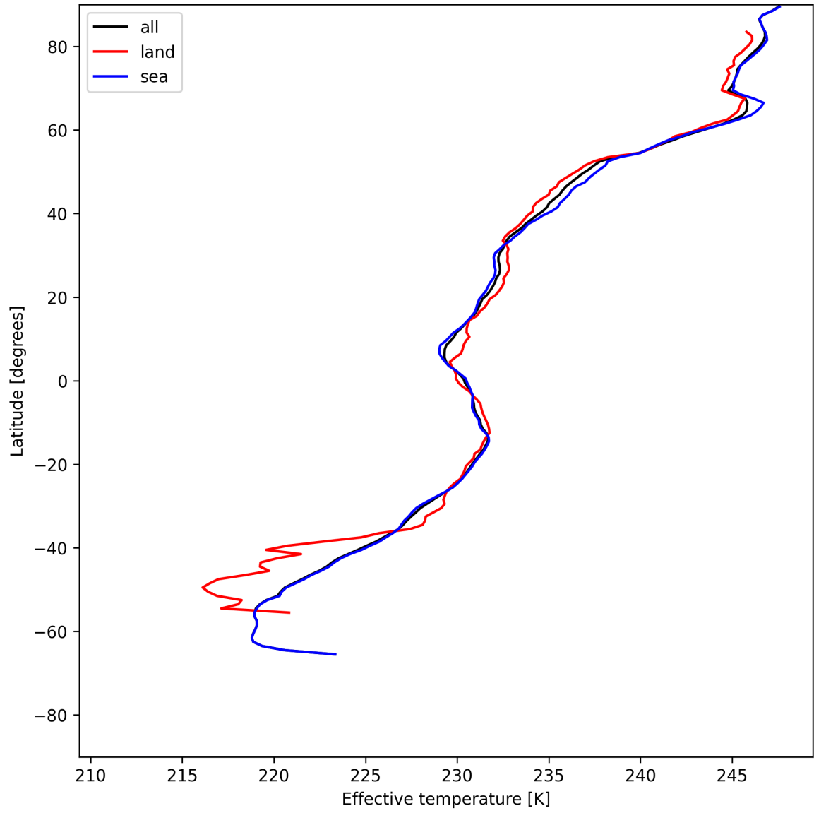
Figure 26: Zonal average of "Effective temperature" for 2025-06-19 to 2025-06-20.
