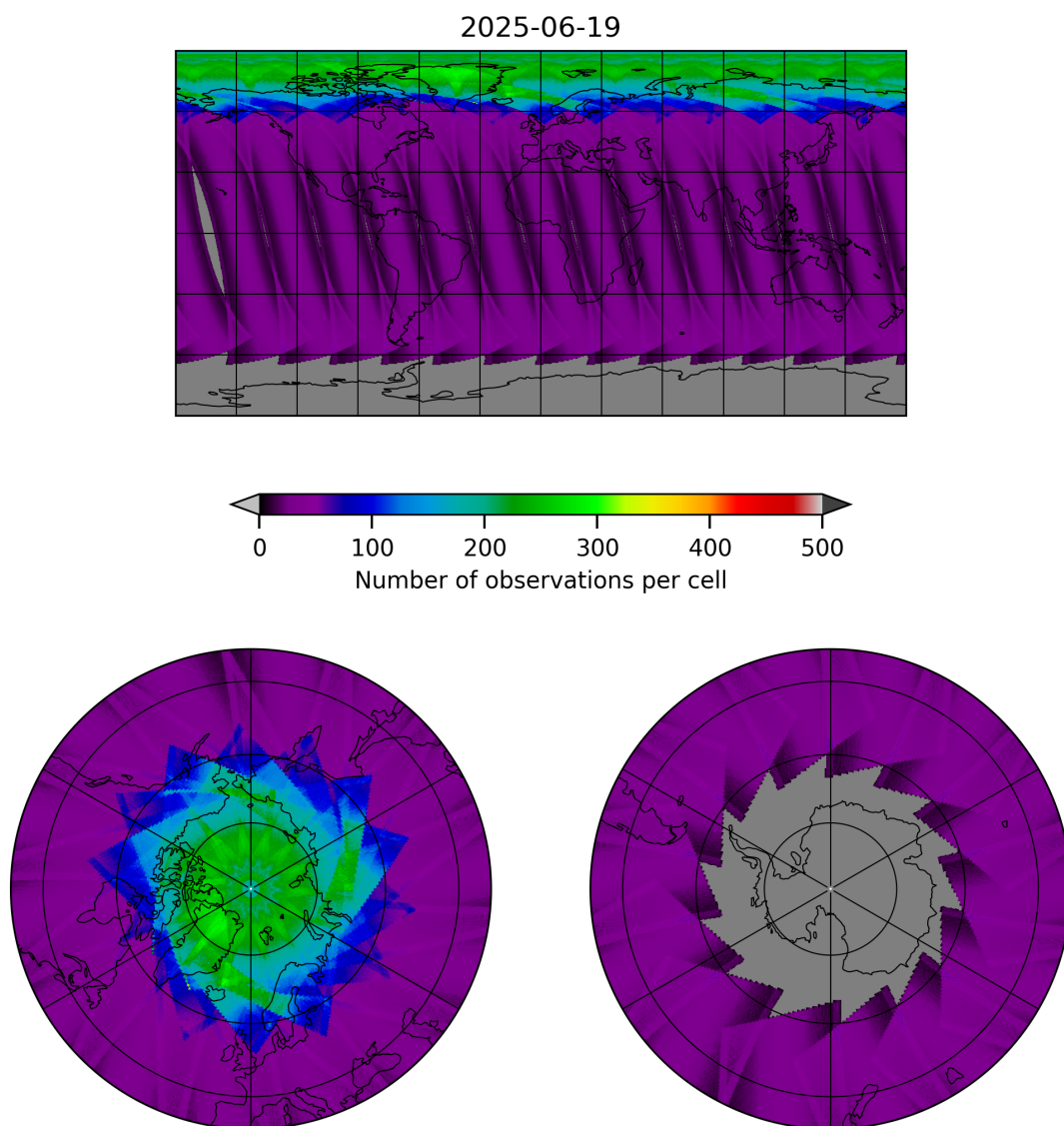
Figure 15: Map of the number of observations for 2025-06-19 to 2025-06-20
