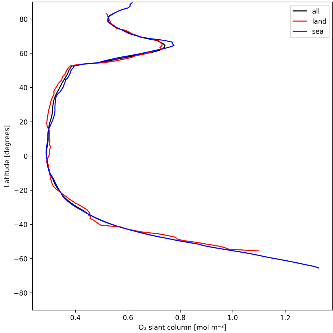
Figure 19: Zonal average of “O 3 slant column” for 2025-06-19 to 2025-06-20.
