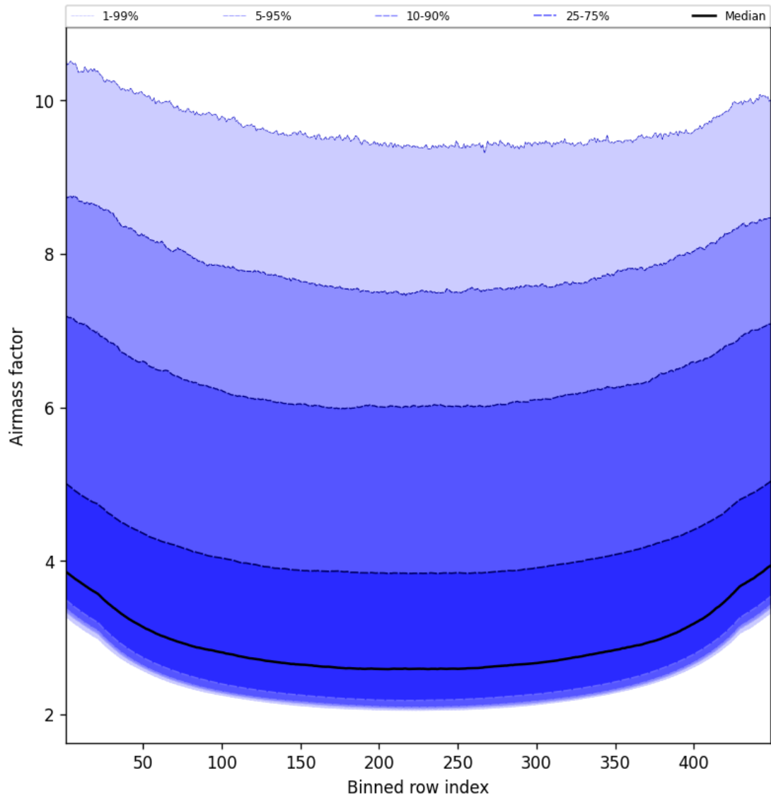
Figure 49: Along track statistics of “Airmass factor” for 2025-06-19 to 2025-06-20
