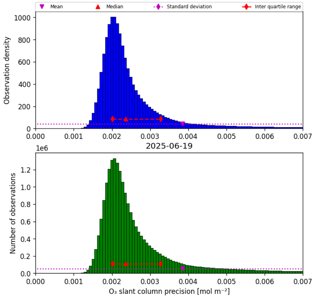
Figure 32: Histogram of “O 3 slant column precision” for 2025-06-19 to 2025-06-20
