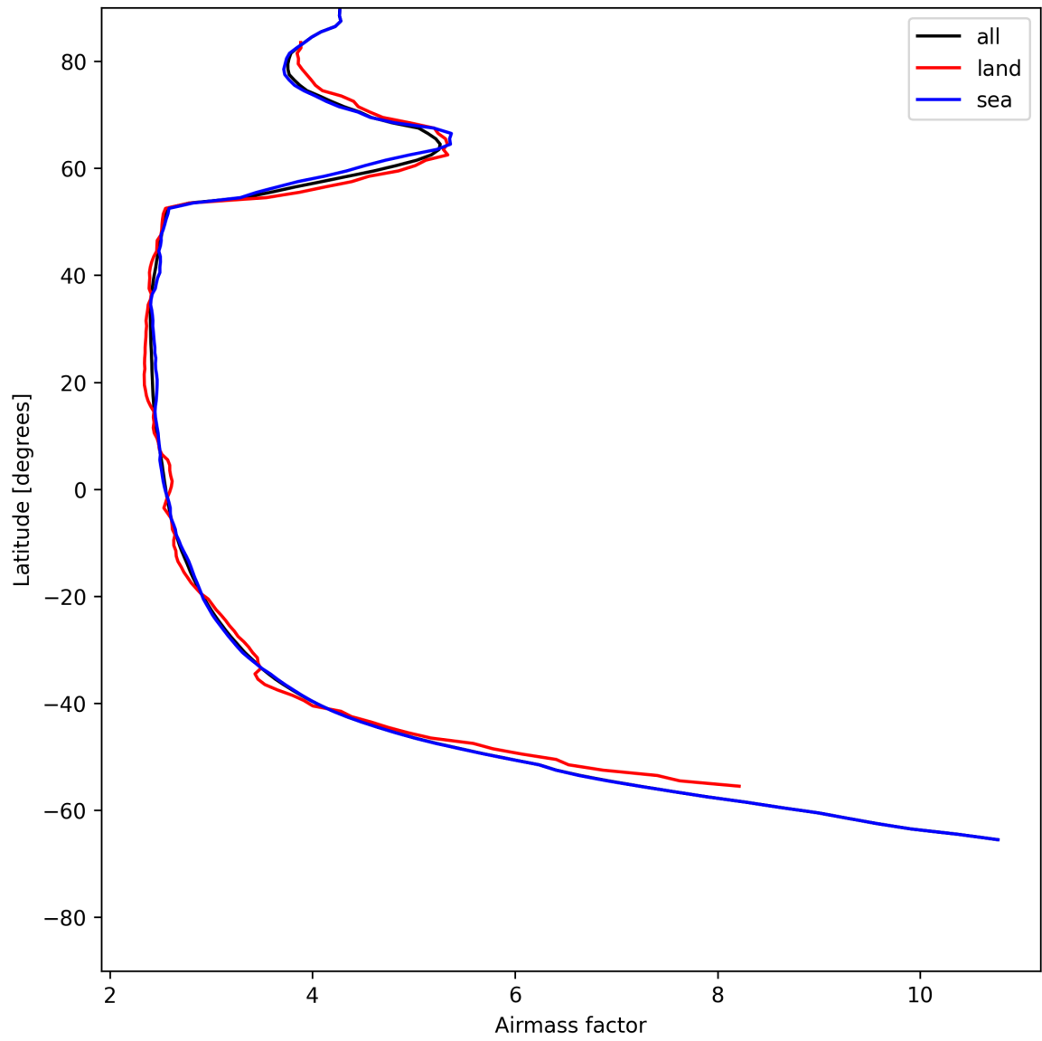
Figure 25: Zonal average of “Airmass factor” for 2025-06-19 to 2025-06-20.
