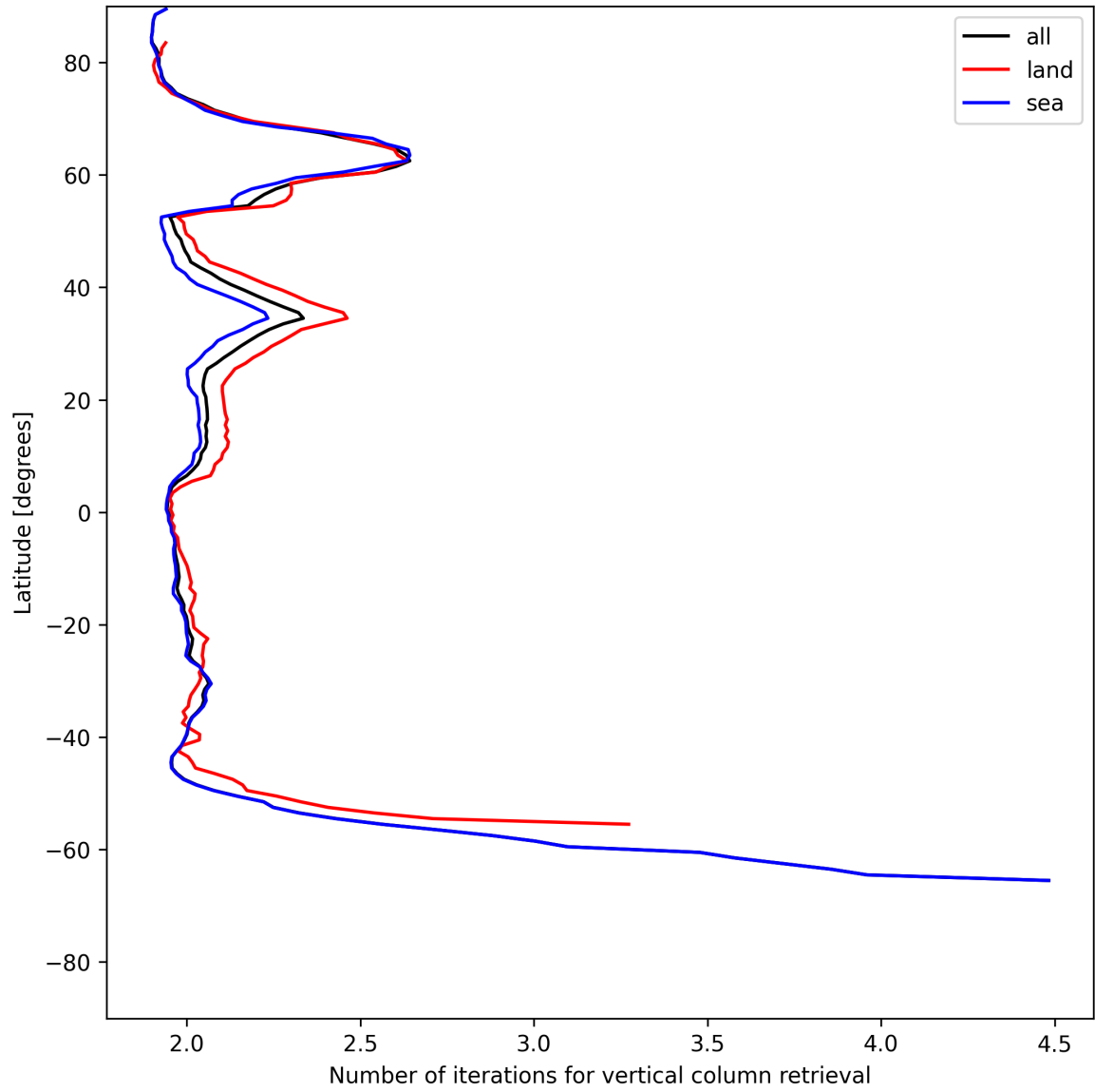
Figure 27: Zonal average of “Number of iterations for vertical column retrieval” for 2025-06-19 to 2025-06-20.
