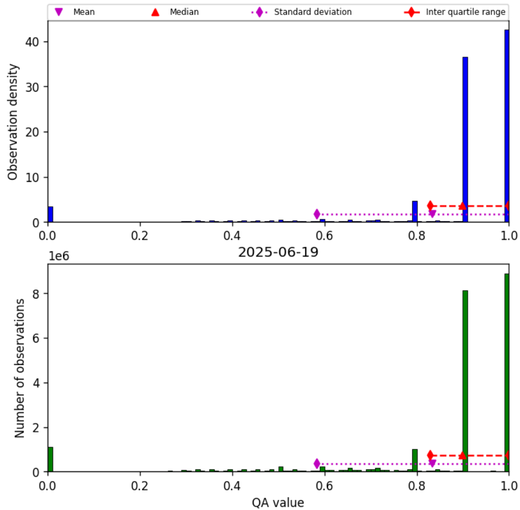
Figure 28: Histogram of “QA value” for 2025-06-19 to 2025-06-20
