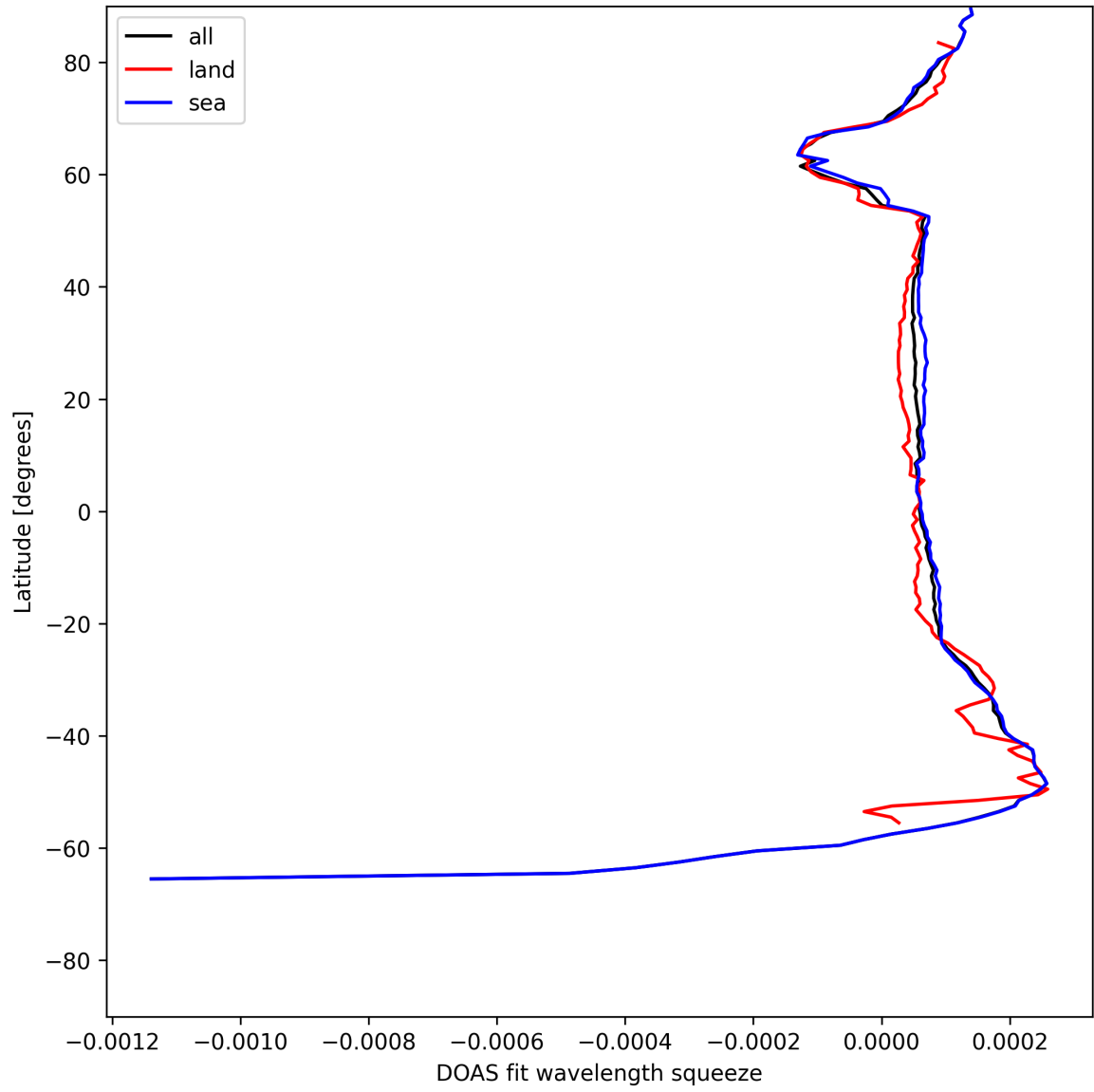
Figure 24: Zonal average of “DOAS fit wavelength squeeze” for 2025-06-19 to 2025-06-20.
