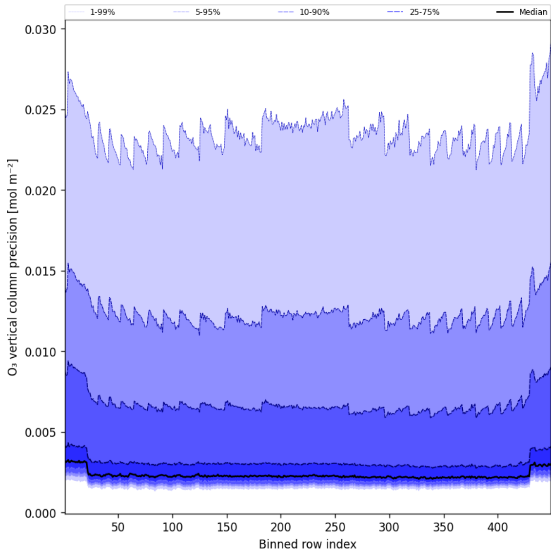
Figure 42: Along track statistics of “O 3 vertical column precision” for 2025-06-19 to 2025-06-20
