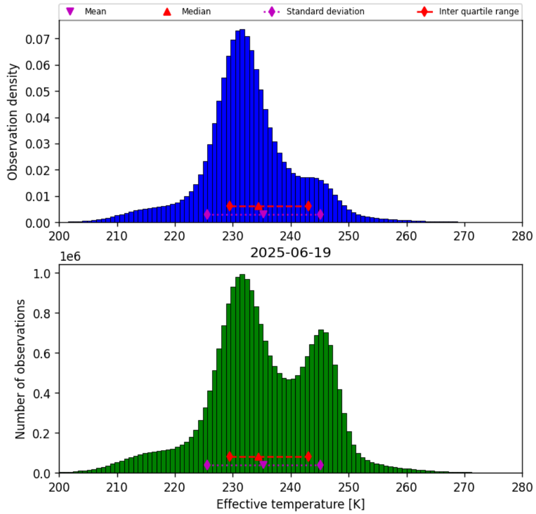
Figure 38: Histogram of “Effective temperature” for 2025-06-19 to 2025-06-20
