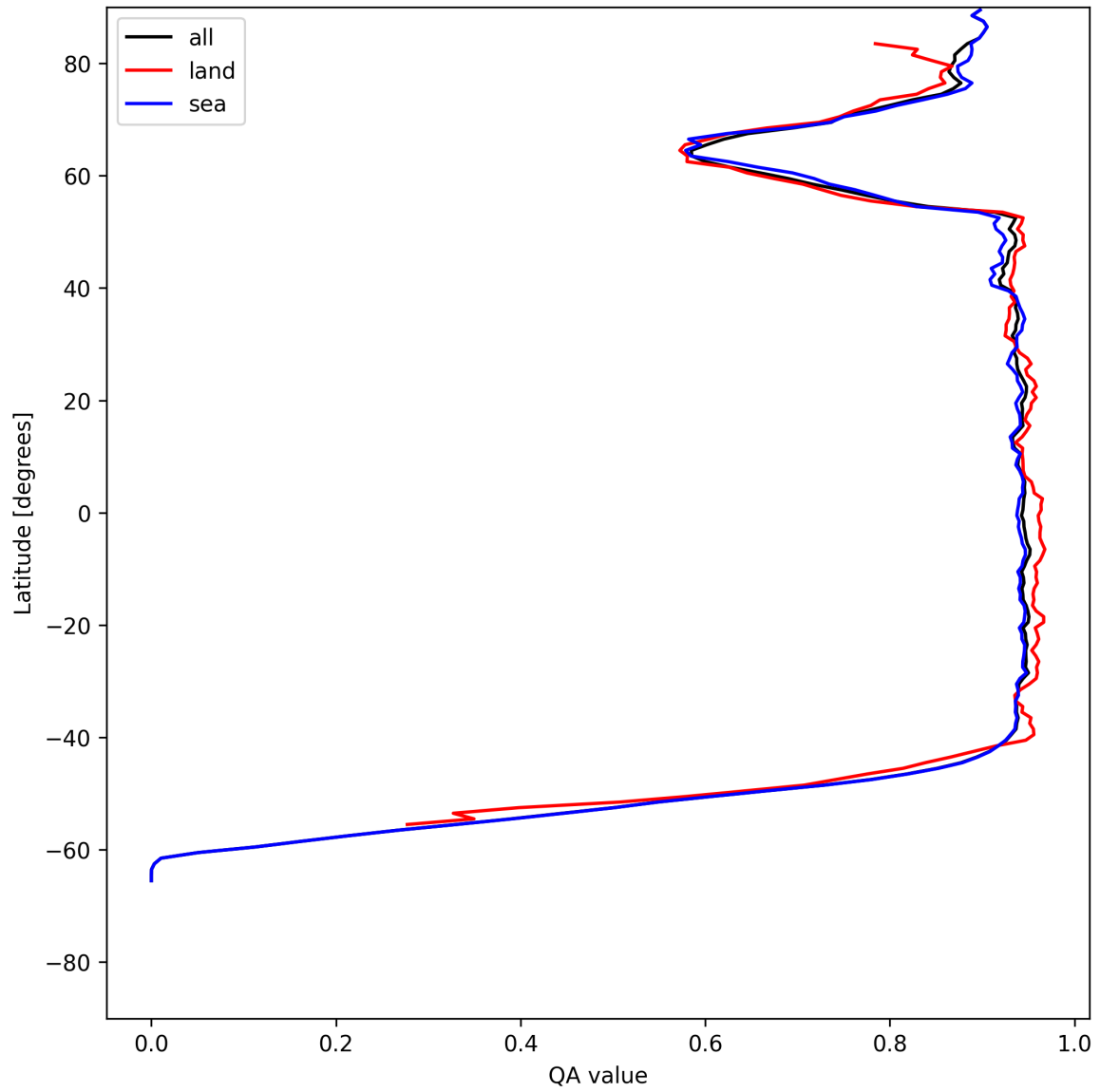
Figure 16: Zonal average of “QA value” for 2025-06-19 to 2025-06-20.
