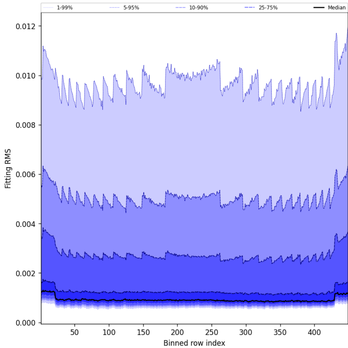
Figure 46: Along track statistics of “Fitting RMS” for 2025-06-19 to 2025-06-20
