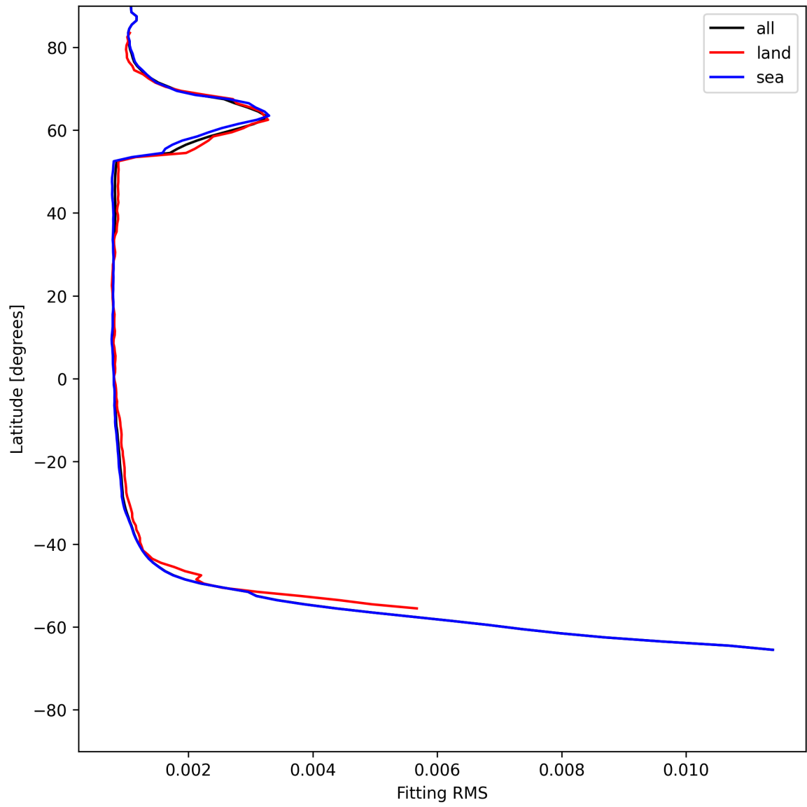
Figure 22: Zonal average of “Fitting RMS” for 2025-06-19 to 2025-06-20.
