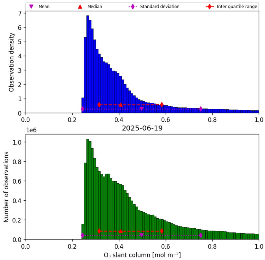
Figure 31: Histogram of “O 3 slant column” for 2025-06-19 to 2025-06-20
