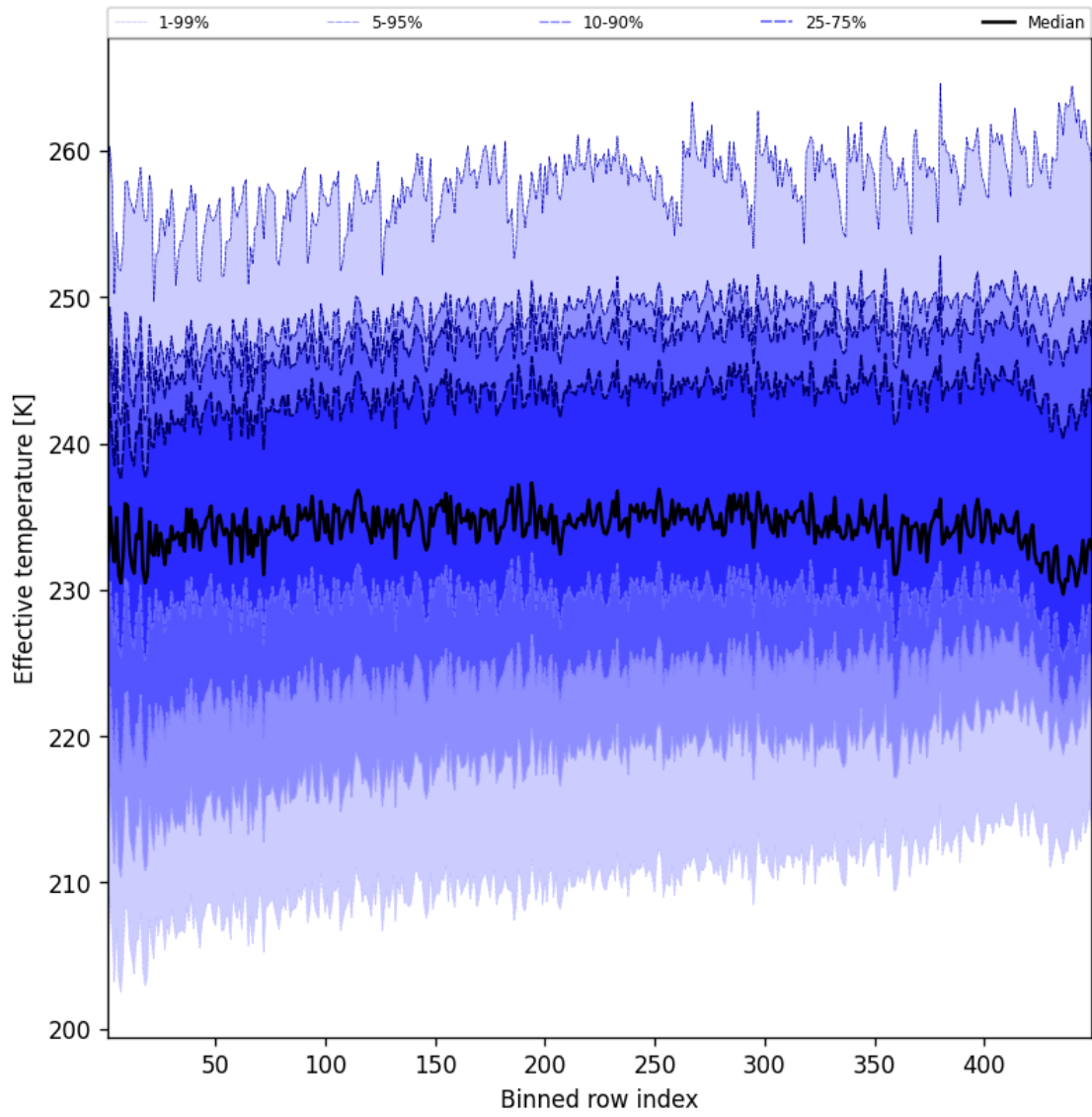
Figure 50: Along track statistics of “Effective temperature” for 2025-06-19 to 2025-06-20
