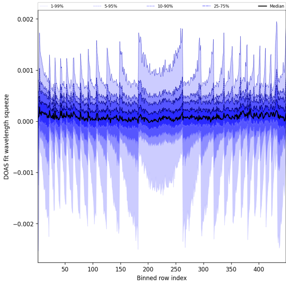
Figure 48: Along track statistics of “DOAS fit wavelength squeeze” for 2025-06-19 to 2025-06-20
