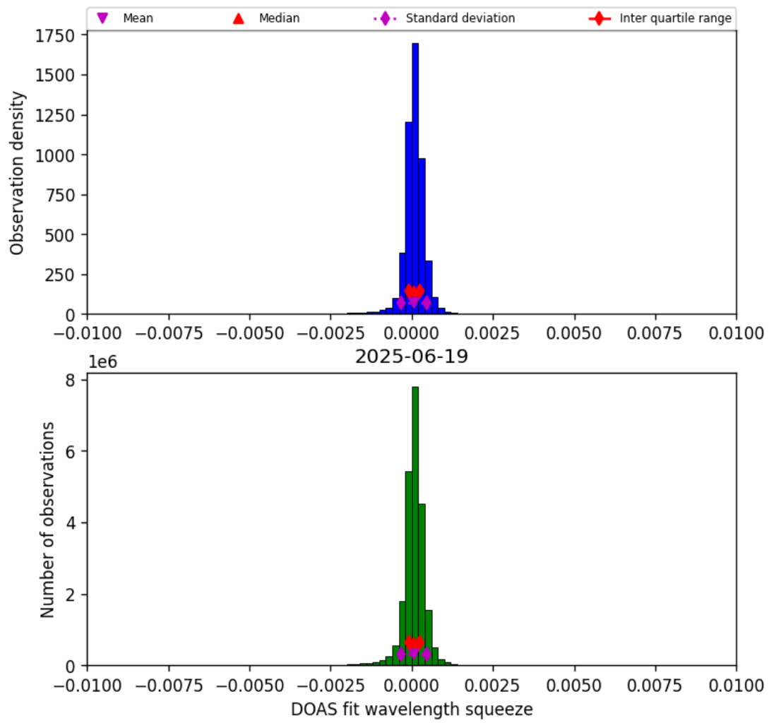
Figure 36: Histogram of “DOAS fit wavelength squeeze” for 2025-06-19 to 2025-06-20
