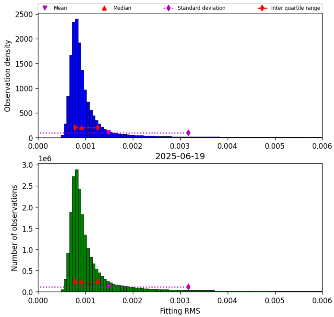
Figure 34: Histogram of “Fitting RMS” for 2025-06-19 to 2025-06-20
