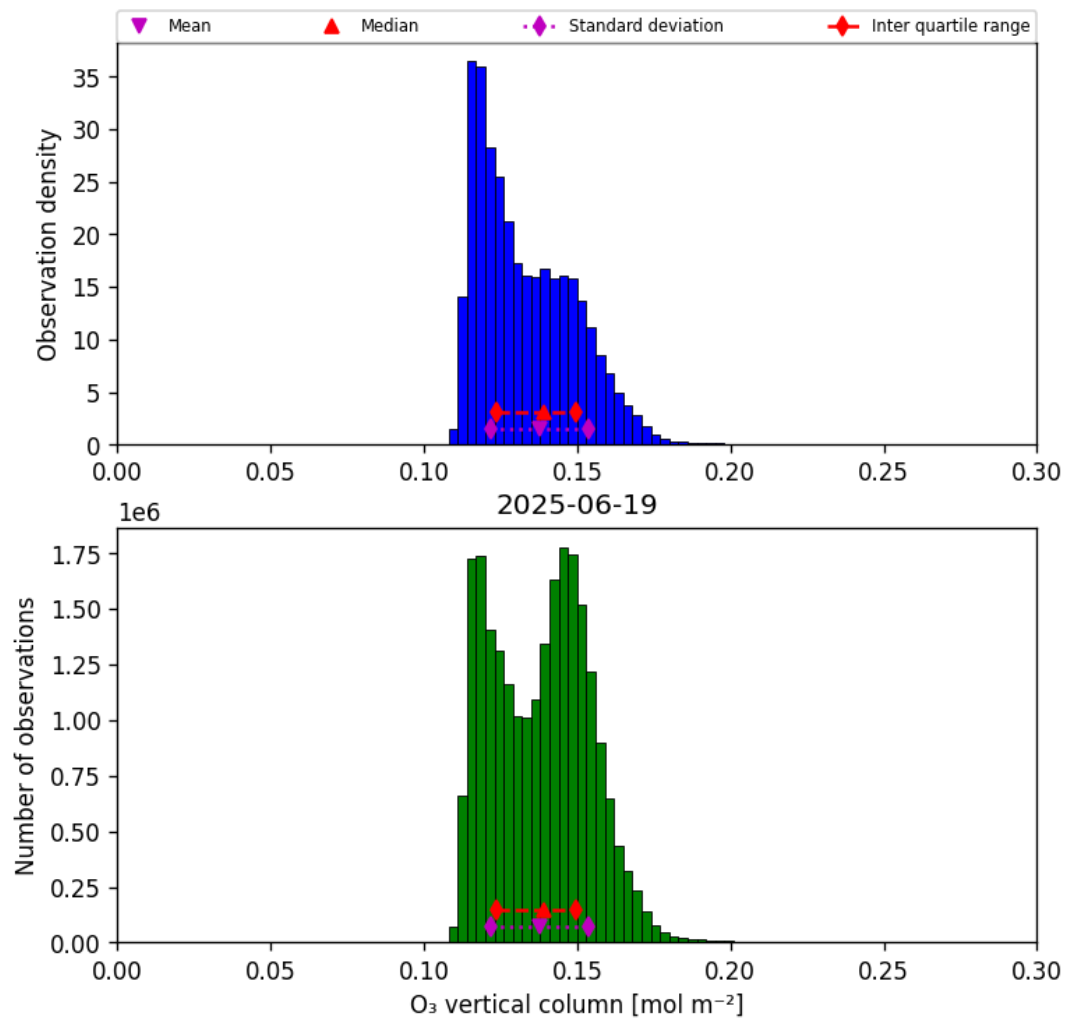
Figure 29: Histogram of “O 3 vertical column” for 2025-06-19 to 2025-06-20
