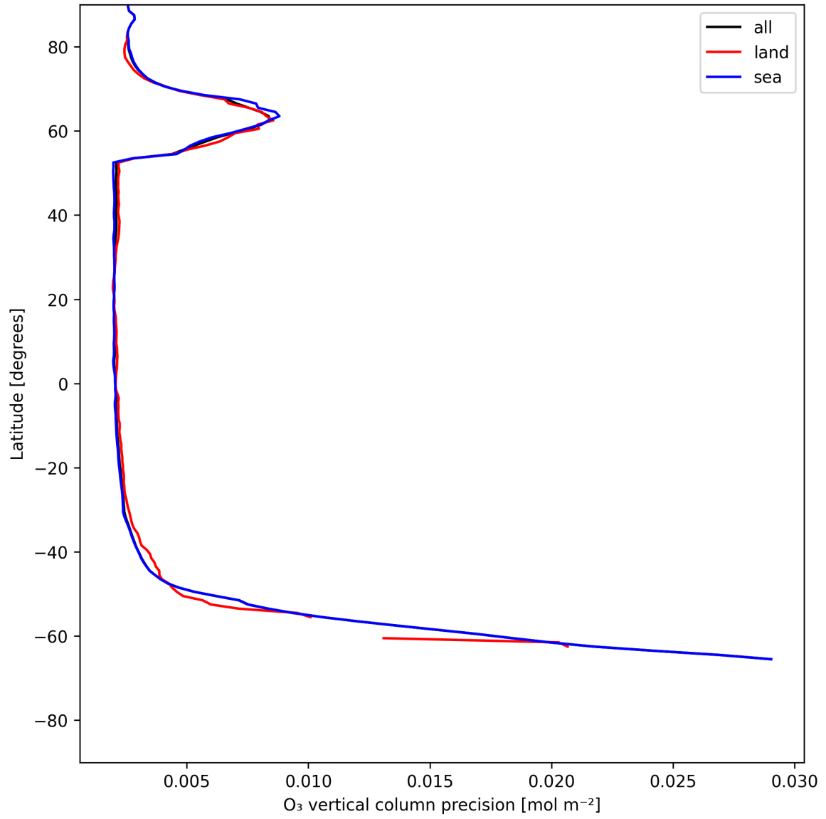
Figure 18: Zonal average of “O 3 vertical column precision” for 2025-06-20 to 2025-06-20.
