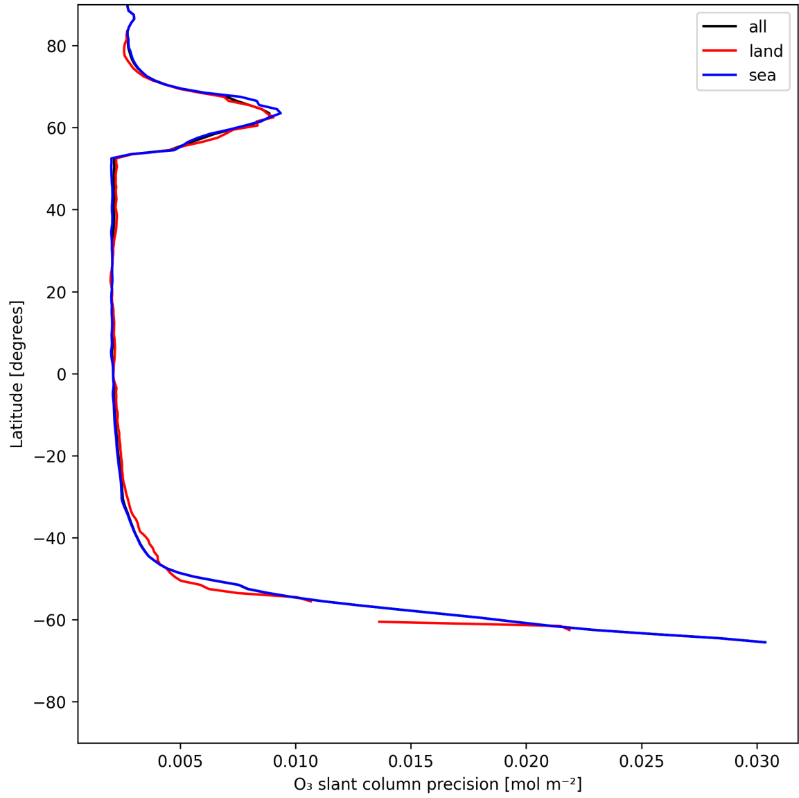
Figure 20: Zonal average of “O 3 slant column precision” for 2025-06-20 to 2025-06-20.
