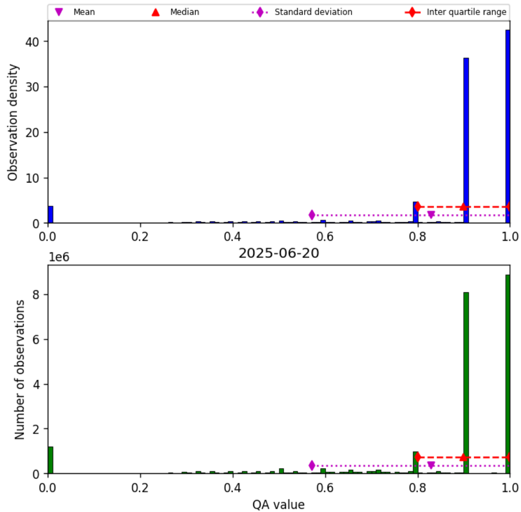
Figure 28: Histogram of “QA value” for 2025-06-20 to 2025-06-20
