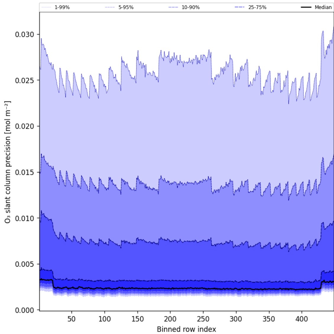
Figure 44: Along track statistics of “O 3 slant column precision” for 2025-06-20 to 2025-06-20
