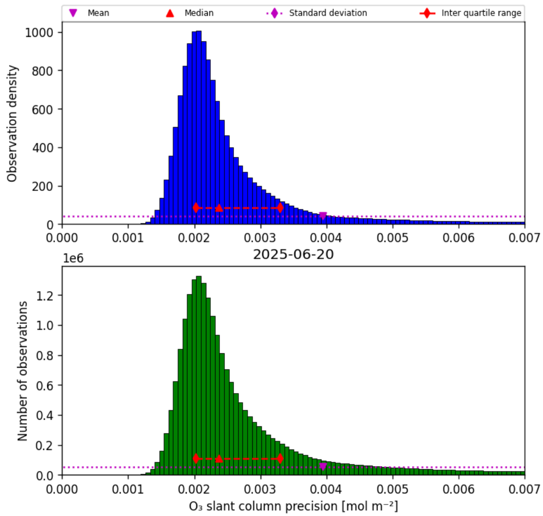
Figure 32: Histogram of “O 3 slant column precision” for 2025-06-20 to 2025-06-20
