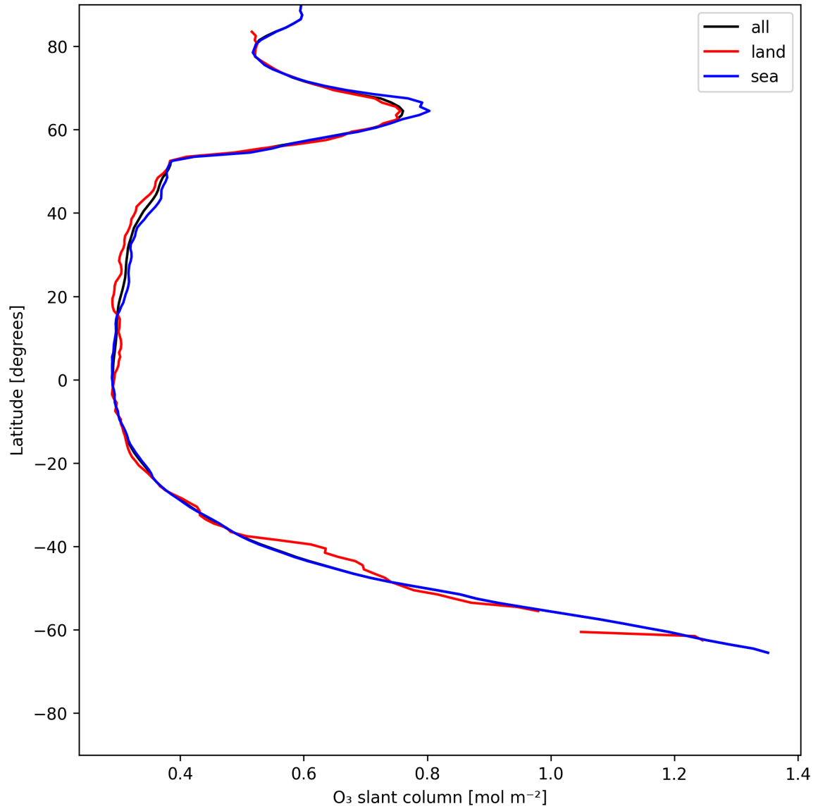
Figure 19: Zonal average of “O 3 slant column” for 2025-06-20 to 2025-06-20.
