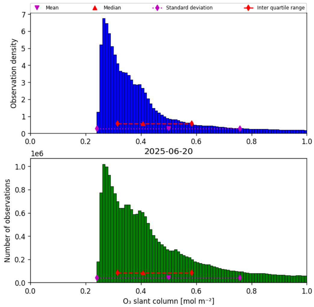
Figure 31: Histogram of “O 3 slant column” for 2025-06-20 to 2025-06-20
