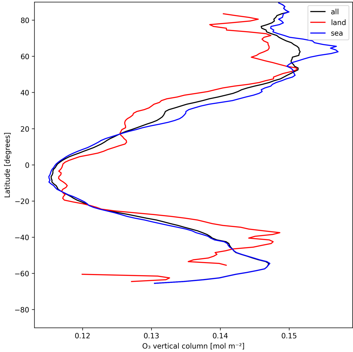
Figure 17: Zonal average of “O 3 vertical column” for 2025-06-21 to 2025-06-22.
