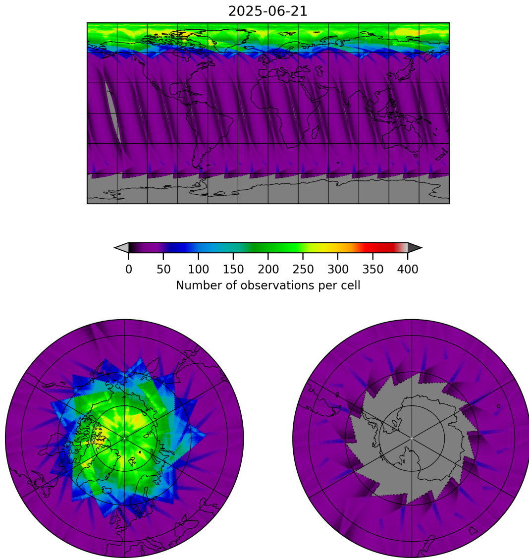
Figure 15: Map of the number of observations for 2025-06-21 to 2025-06-22
