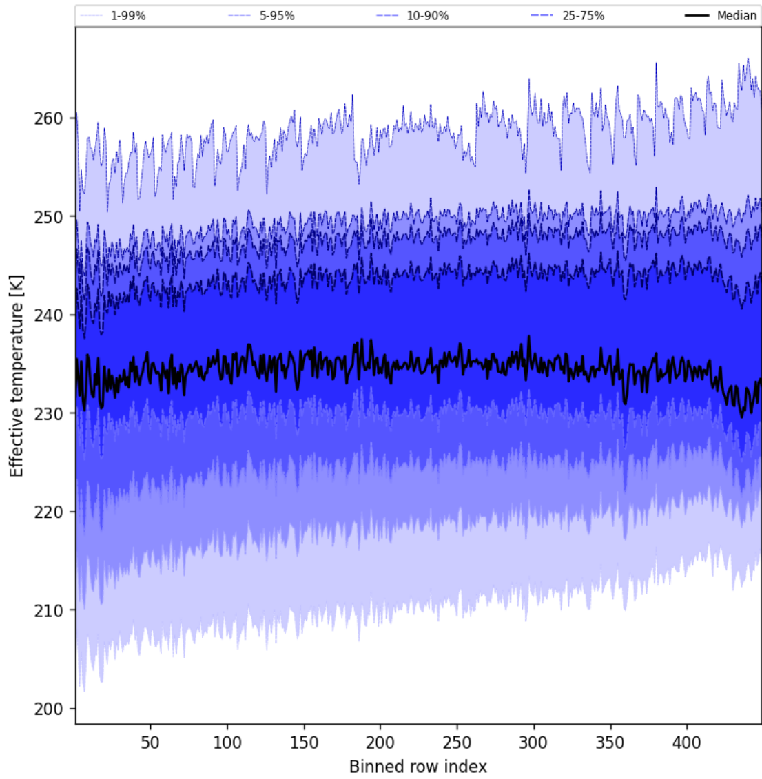
Figure 50: Along track statistics of “Effective temperature” for 2025-06-21 to 2025-06-22
