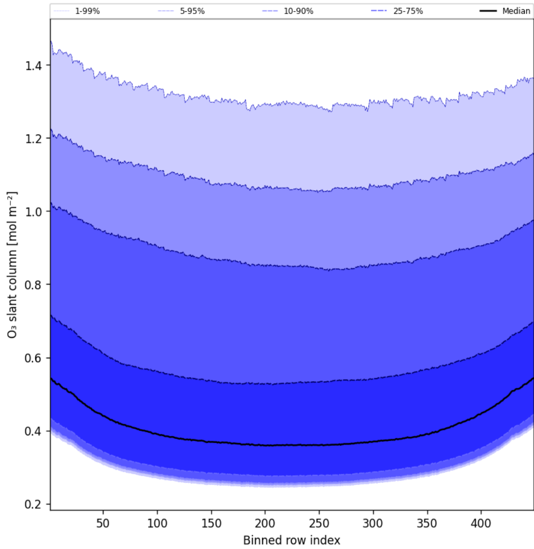
Figure 43: Along track statistics of “O 3 slant column” for 2025-06-21 to 2025-06-22
