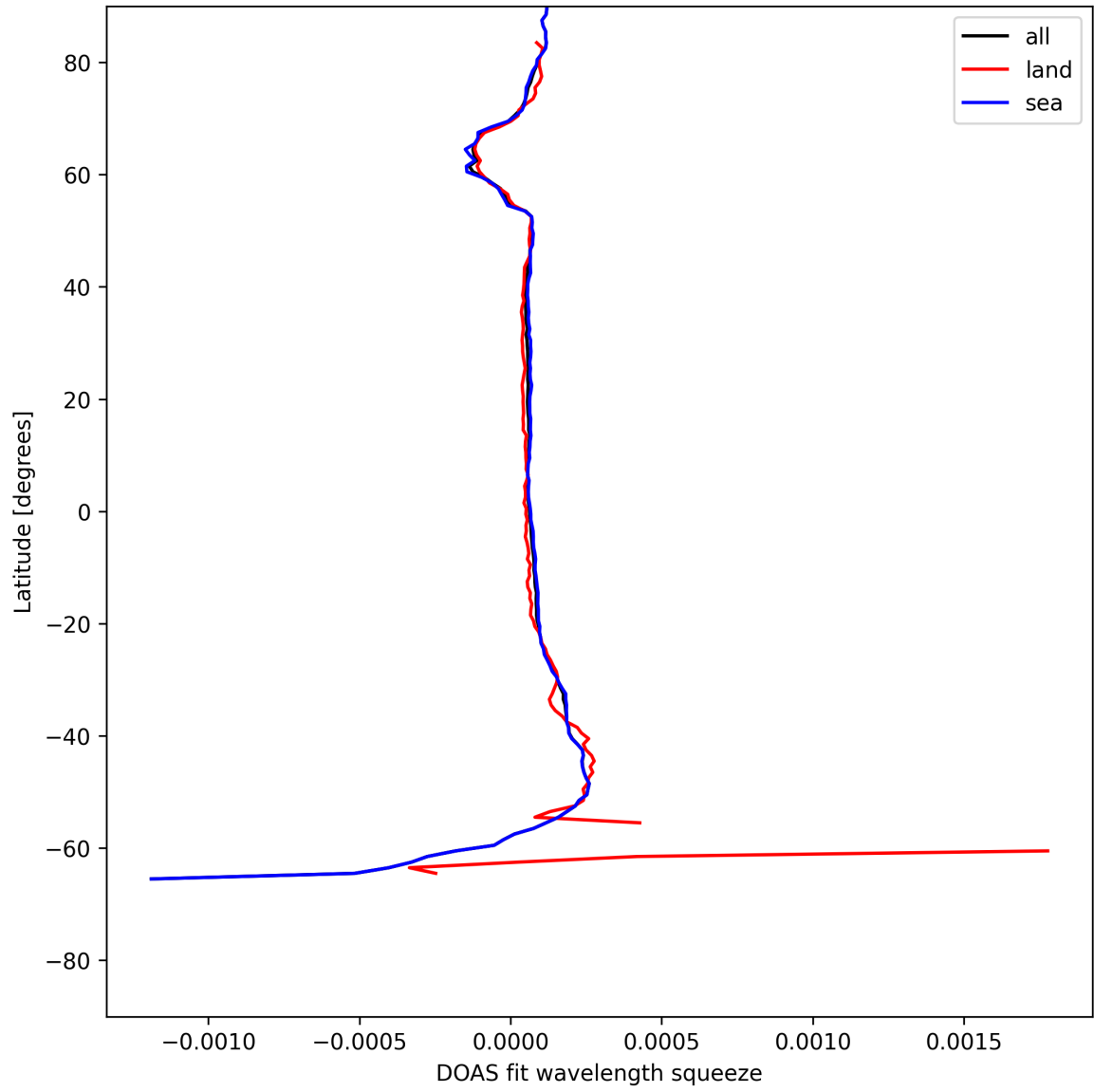
Figure 24: Zonal average of “DOAS fit wavelength squeeze” for 2025-06-21 to 2025-06-22.
