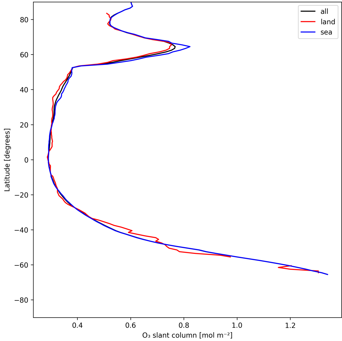
Figure 19: Zonal average of “O 3 slant column” for 2025-06-21 to 2025-06-22.
