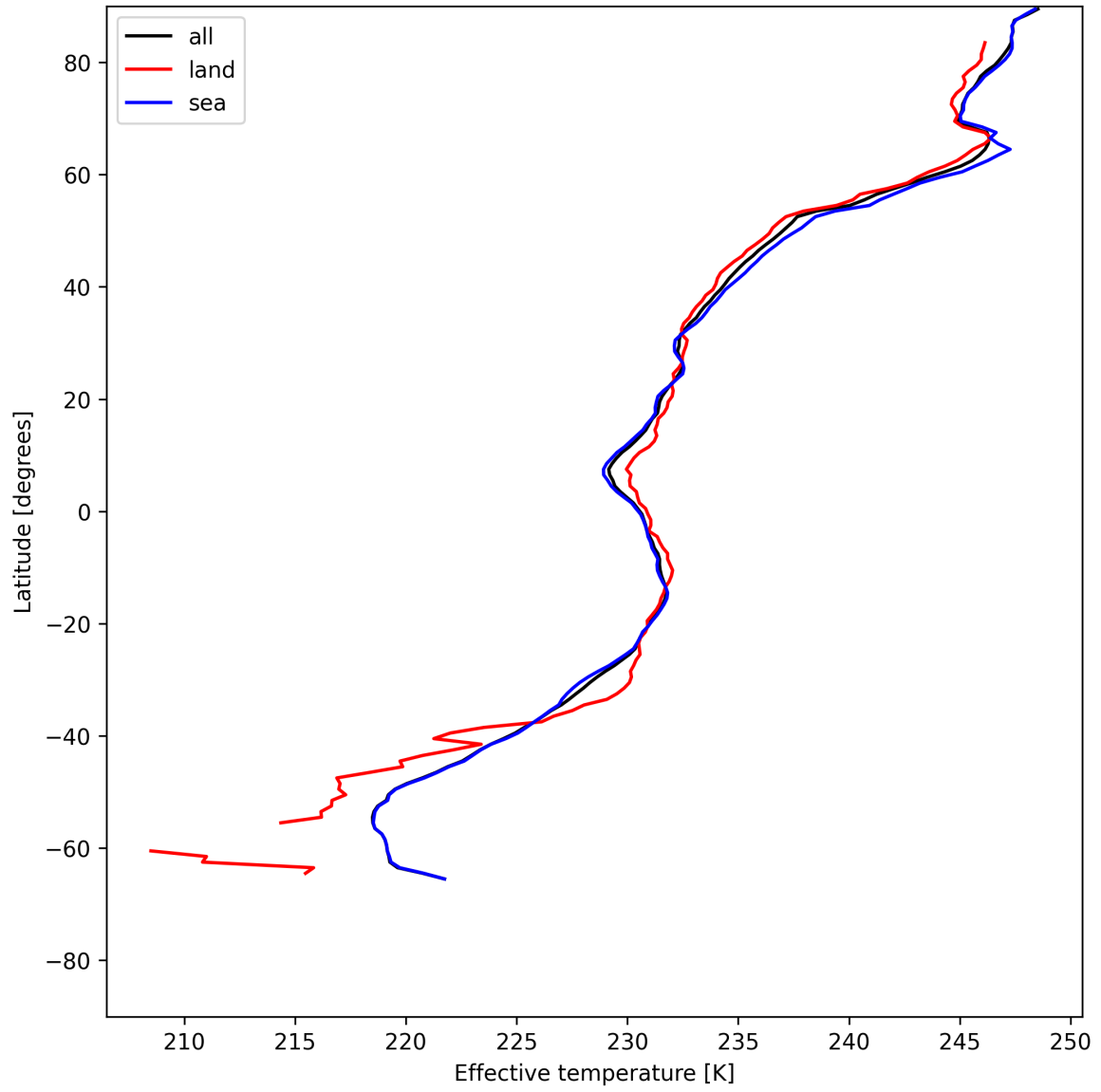
Figure 26: Zonal average of “Effective temperature” for 2025-06-21 to 2025-06-22.
