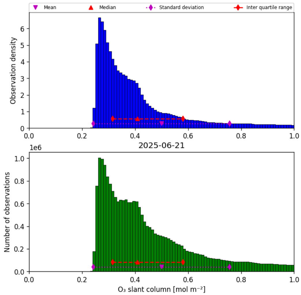
Figure 31: Histogram of “O 3 slant column” for 2025-06-21 to 2025-06-22
