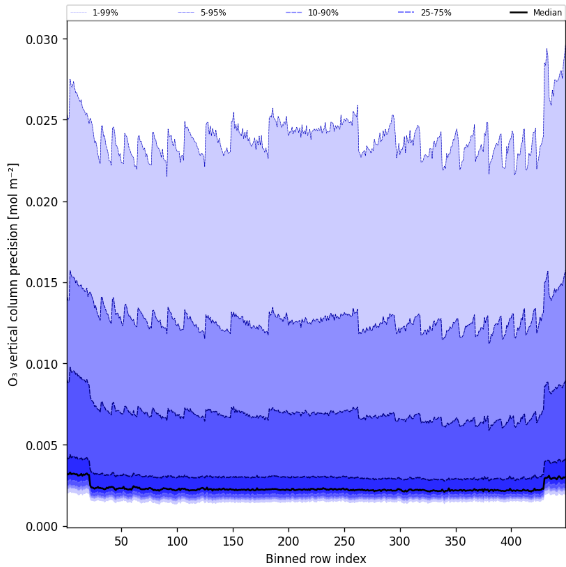
Figure 42: Along track statistics of “O 3 vertical column precision” for 2025-06-21 to 2025-06-22
