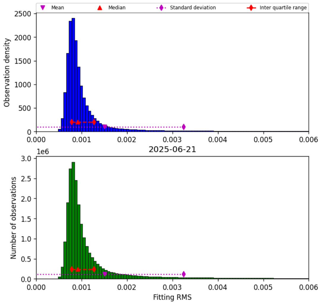
Figure 34: Histogram of “Fitting RMS” for 2025-06-21 to 2025-06-22
