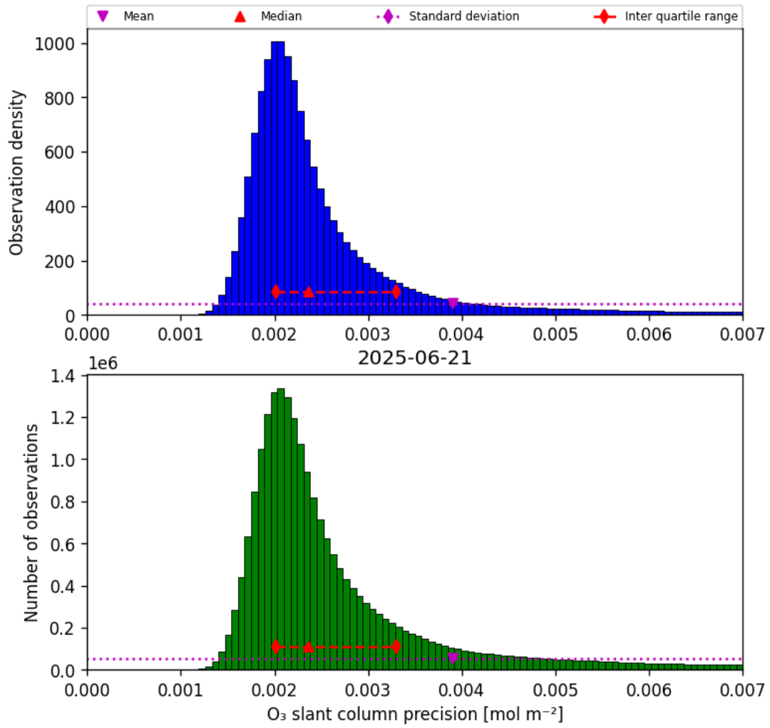
Figure 32: Histogram of “O 3 slant column precision” for 2025-06-21 to 2025-06-22
