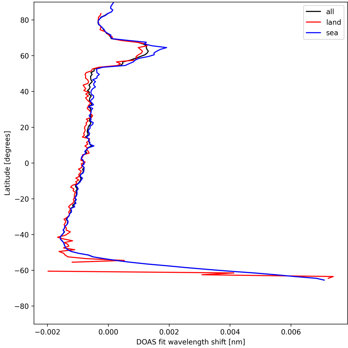
Figure 23: Zonal average of “DOAS fit wavelength shift” for 2025-06-21 to 2025-06-22.
