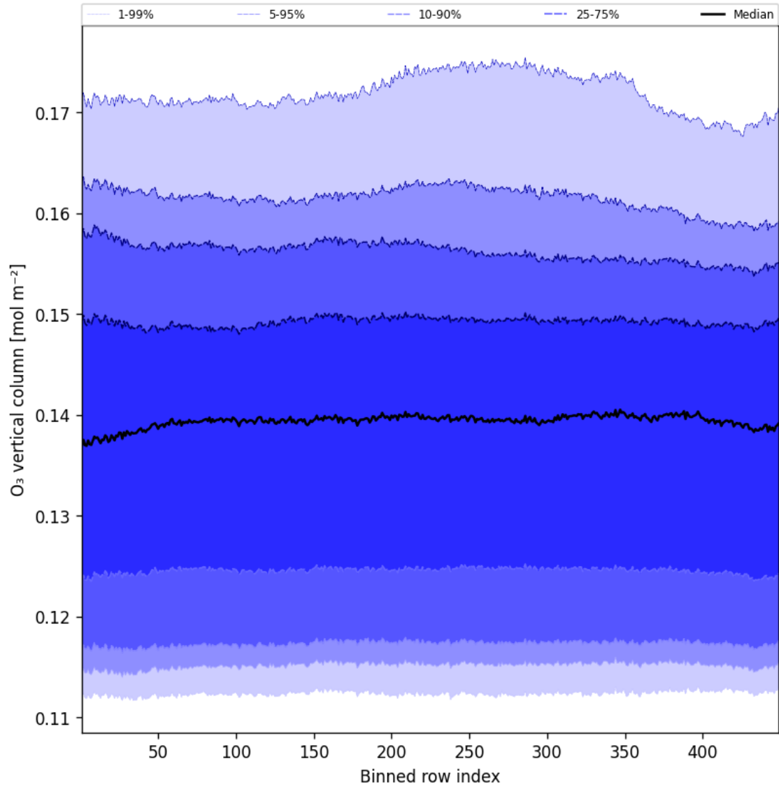
Figure 41: Along track statistics of “O 3 vertical column” for 2025-06-21 to 2025-06-22
