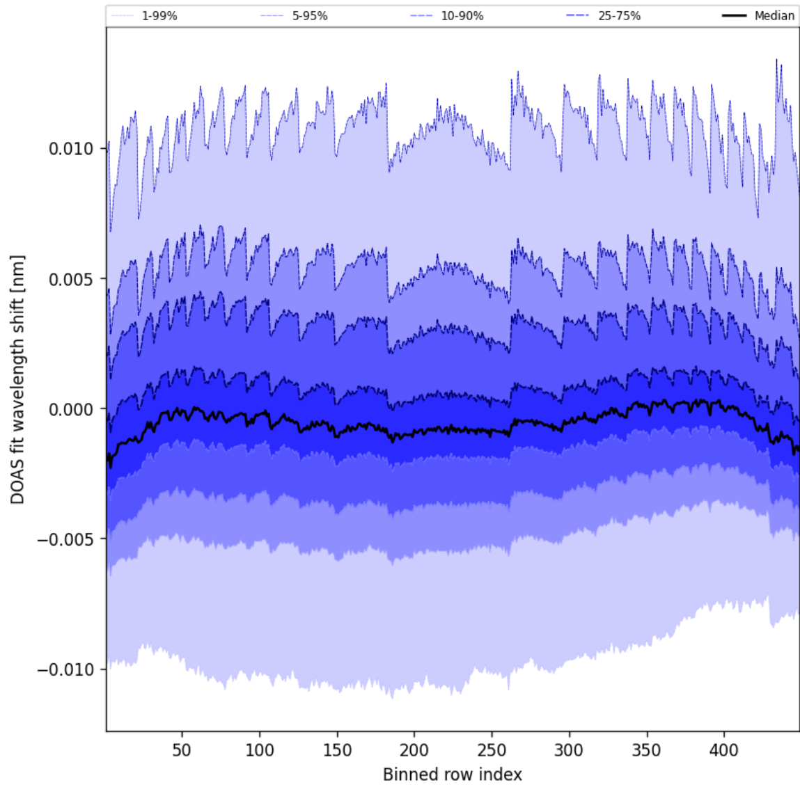
Figure 47: Along track statistics of “DOAS fit wavelength shift” for 2025-06-21 to 2025-06-22
