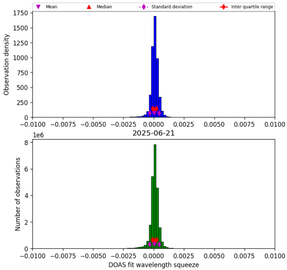
Figure 36: Histogram of “DOAS fit wavelength squeeze” for 2025-06-21 to 2025-06-22
