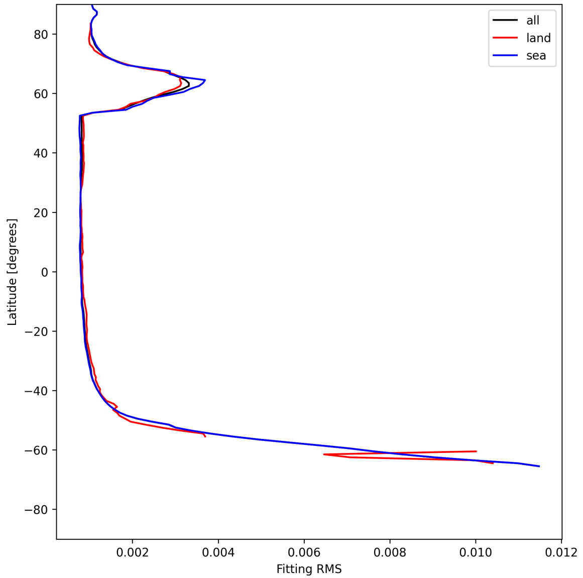
Figure 22: Zonal average of “Fitting RMS” for 2025-06-21 to 2025-06-22.
