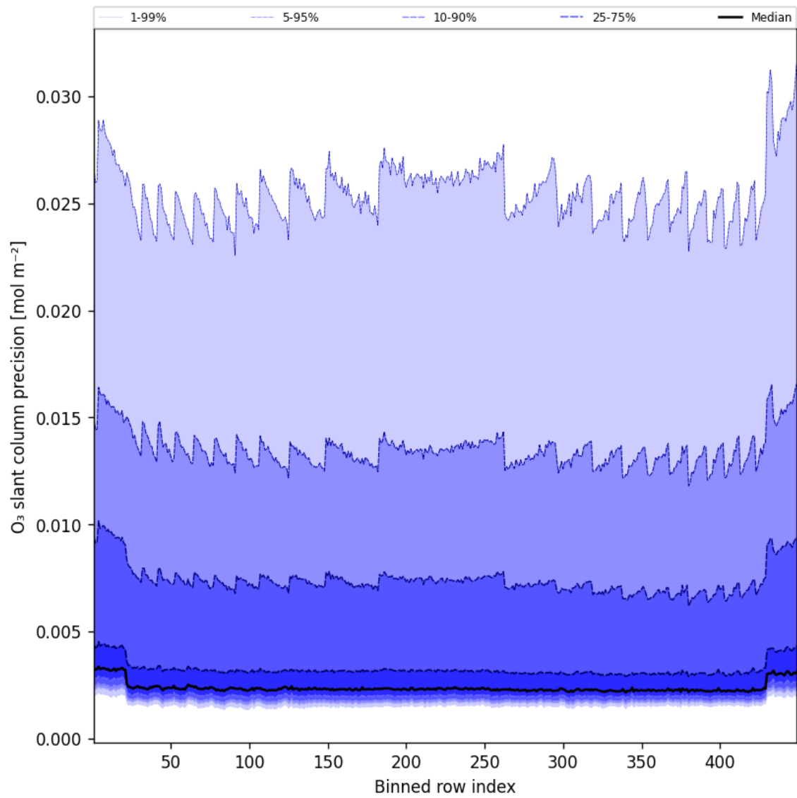
Figure 44: Along track statistics of “O 3 slant column precision” for 2025-06-21 to 2025-06-22
