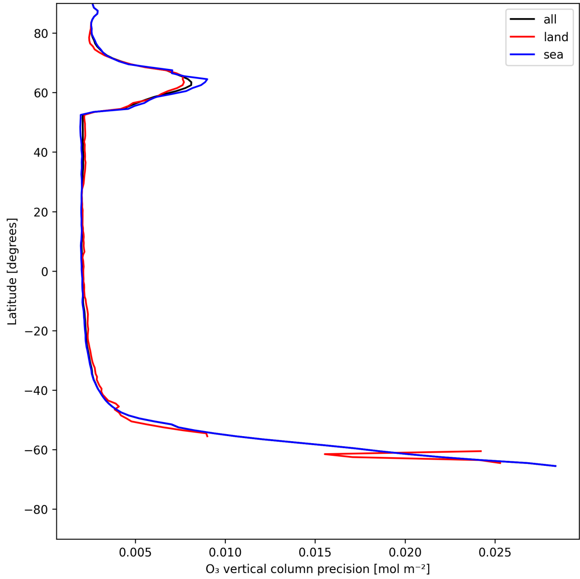
Figure 18: Zonal average of “O 3 vertical column precision” for 2025-06-21 to 2025-06-22.
