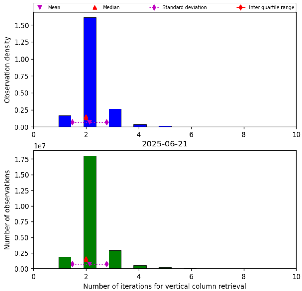
Figure 39: Histogram of “Number of iterations for vertical column retrieval” for 2025-06-21 to 2025-06-22
