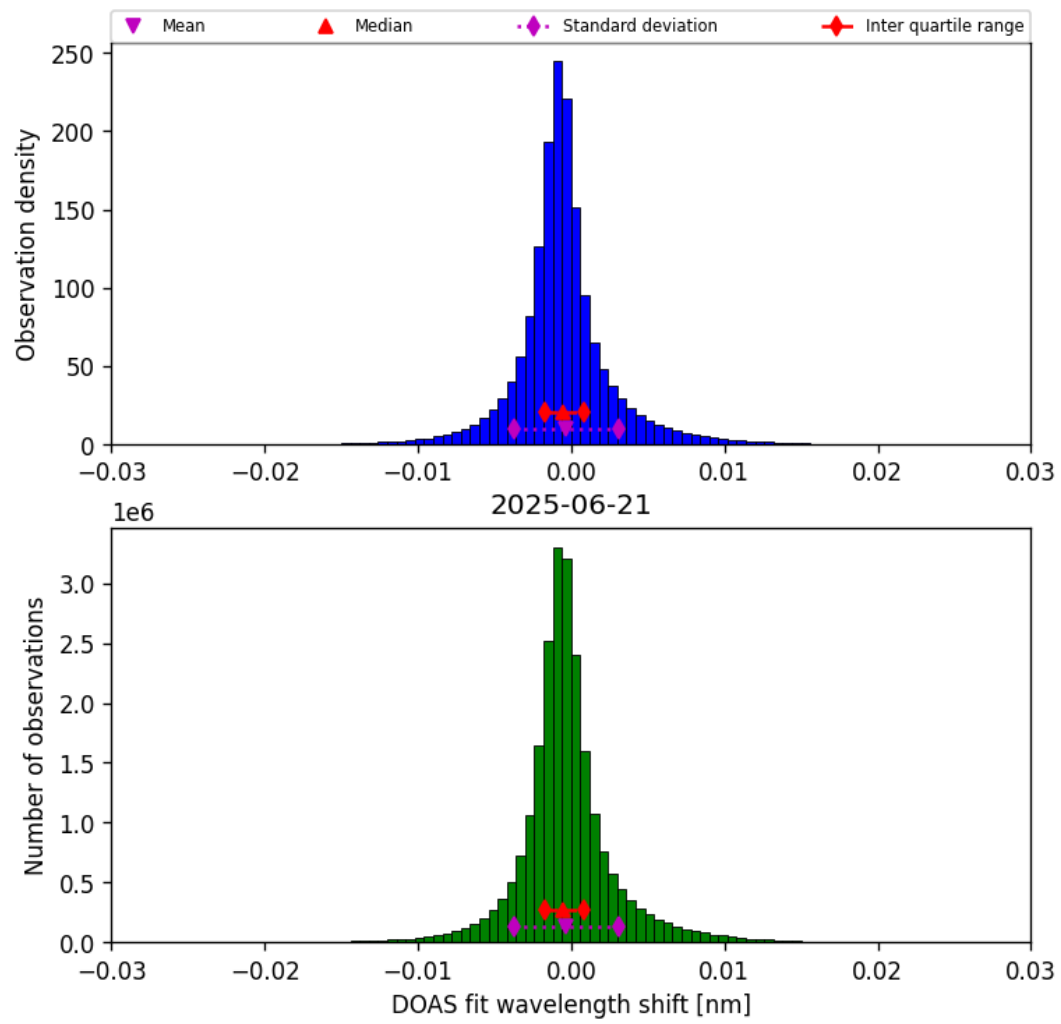
Figure 35: Histogram of “DOAS fit wavelength shift” for 2025-06-21 to 2025-06-22
