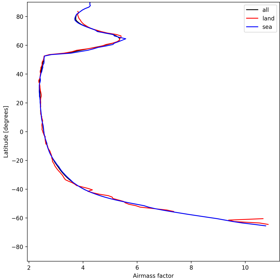
Figure 25: Zonal average of “Airmass factor” for 2025-06-21 to 2025-06-22.
