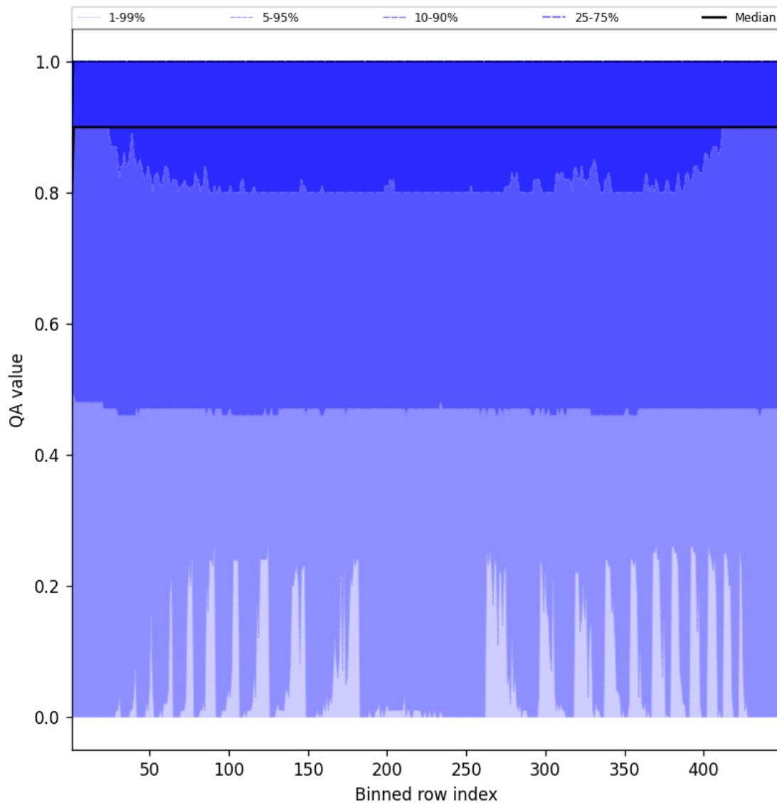
Figure 40: Along track statistics of “QA value” for 2025-06-21 to 2025-06-22
