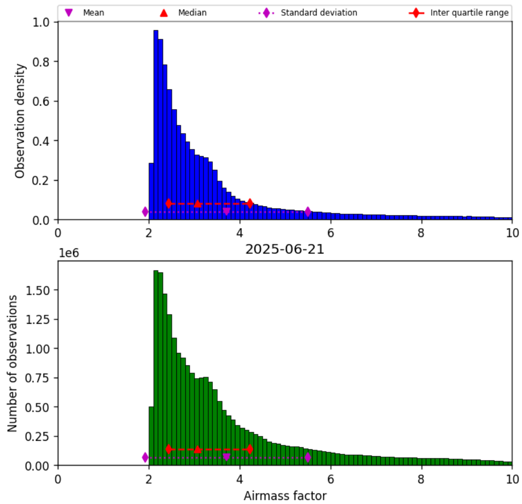
Figure 37: Histogram of “Airmass factor” for 2025-06-21 to 2025-06-22
