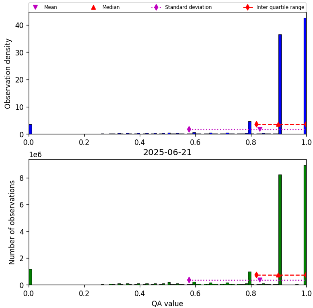
Figure 28: Histogram of “QA value” for 2025-06-21 to 2025-06-22
