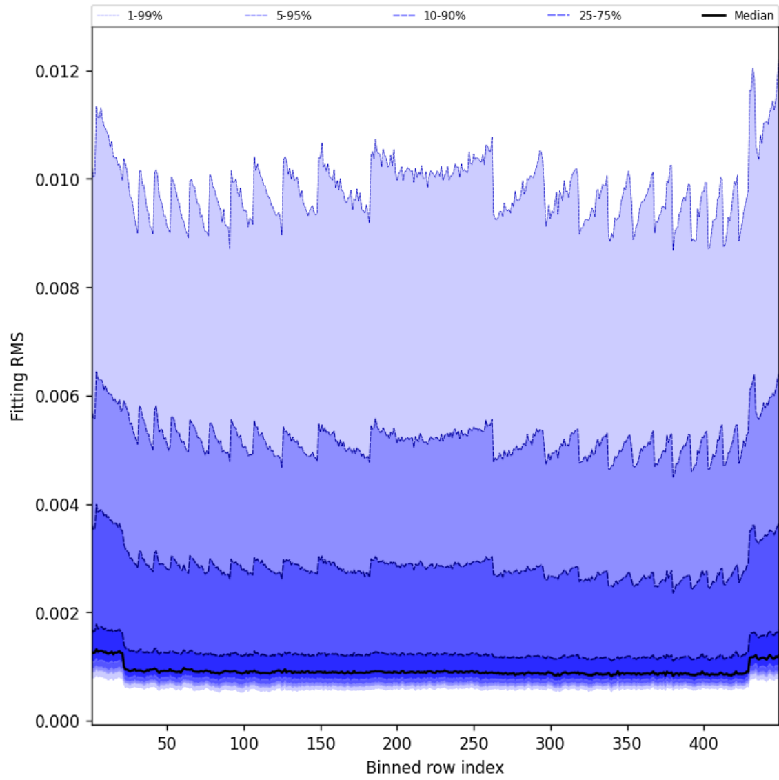
Figure 46: Along track statistics of “Fitting RMS” for 2025-06-21 to 2025-06-22
