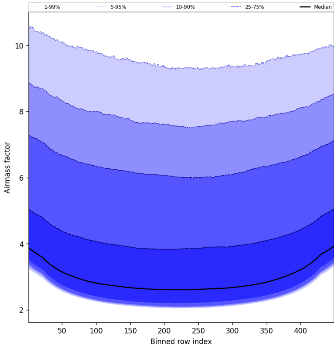
Figure 49: Along track statistics of “Airmass factor” for 2025-06-21 to 2025-06-22
