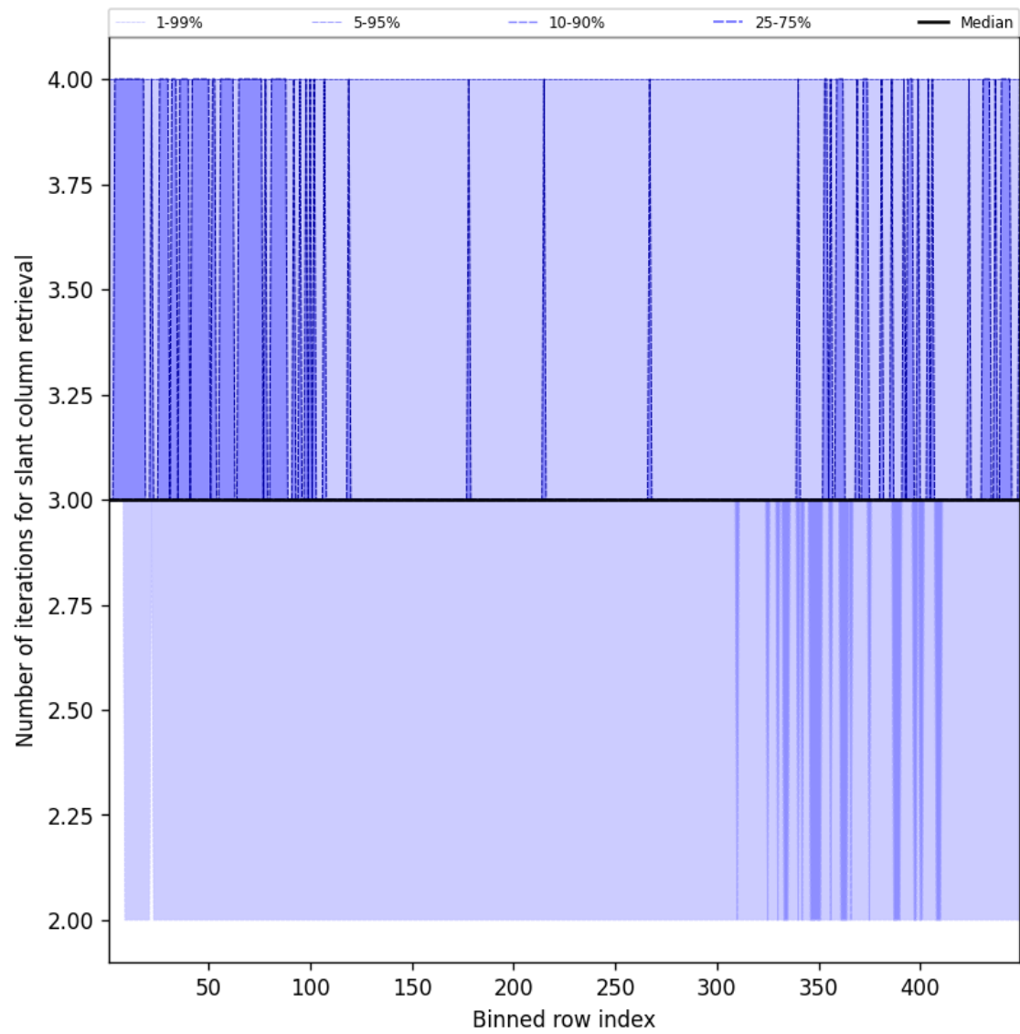
Figure 45: Along track statistics of “Number of iterations for slant column retrieval” for 2025-06-21 to 2025-06-22
