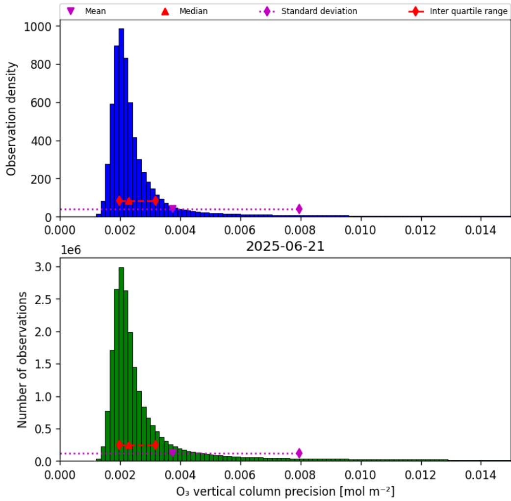
Figure 30: Histogram of “O 3 vertical column precision” for 2025-06-21 to 2025-06-22
