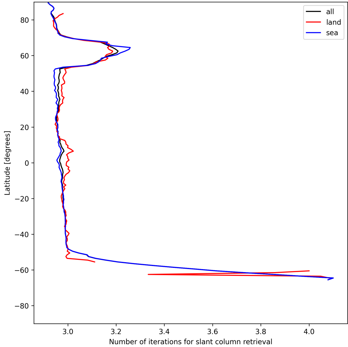
Figure 21: Zonal average of “Number of iterations for slant column retrieval” for 2025-06-21 to 2025-06-22.
