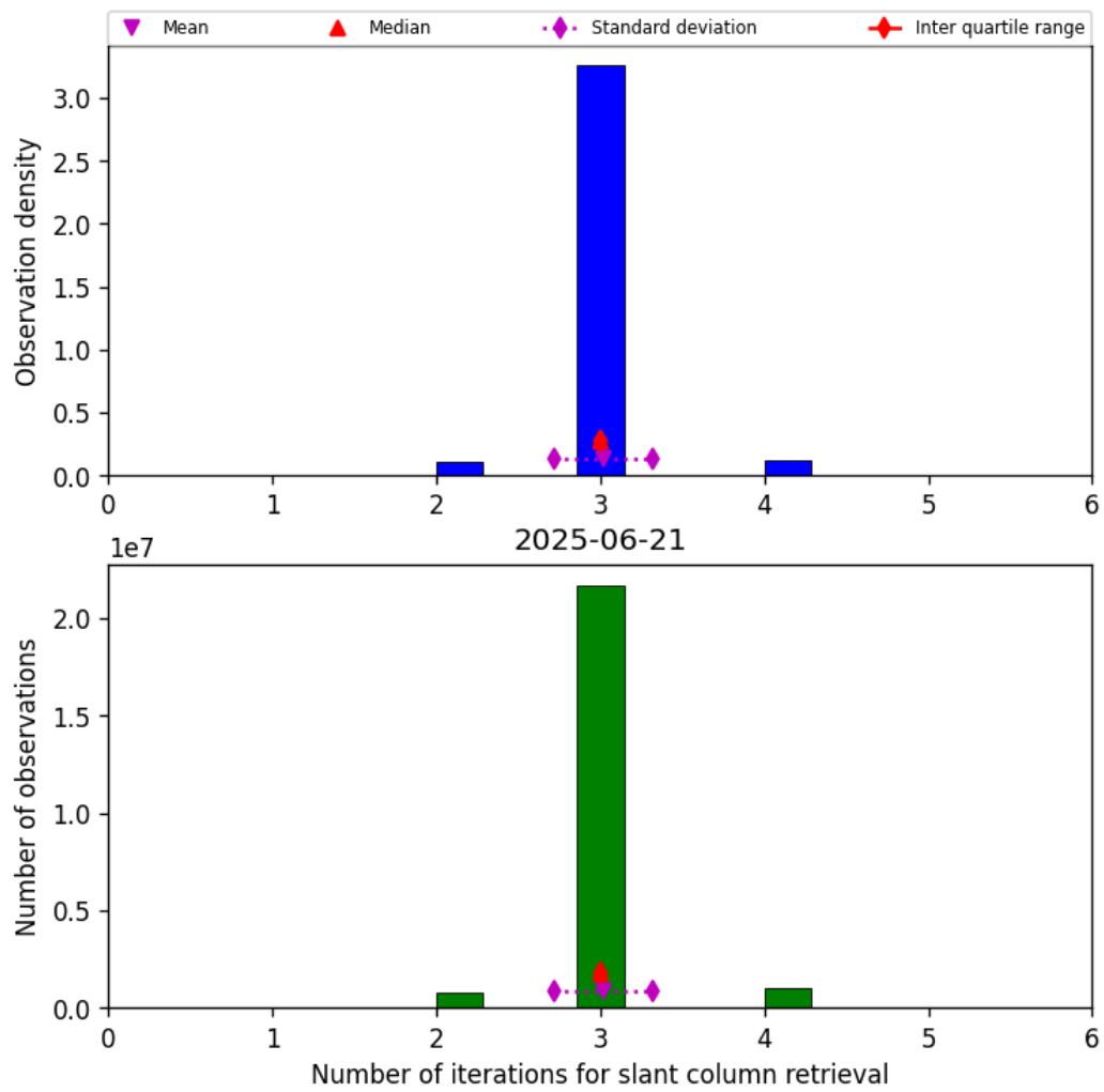
Figure 33: Histogram of “Number of iterations for slant column retrieval” for 2025-06-21 to 2025-06-22
