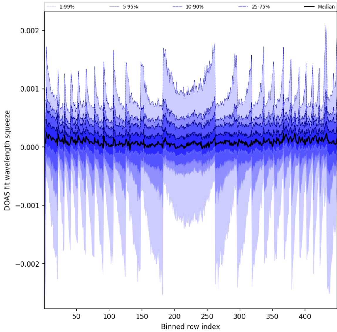
Figure 48: Along track statistics of “DOAS fit wavelength squeeze” for 2025-06-21 to 2025-06-22
