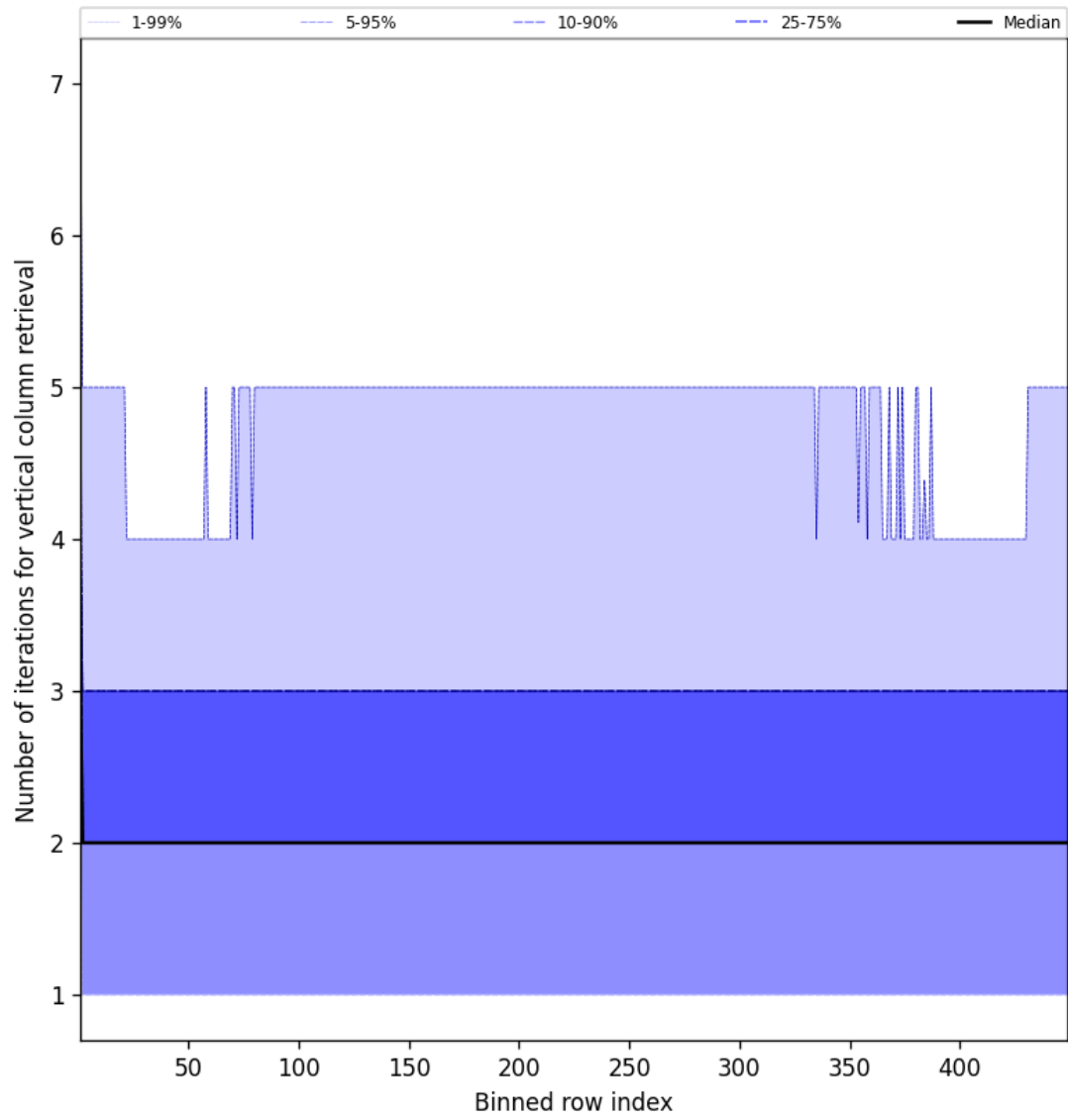
Figure 51: Along track statistics of “Number of iterations for vertical column retrieval” for 2025-06-21 to 2025-06-22
