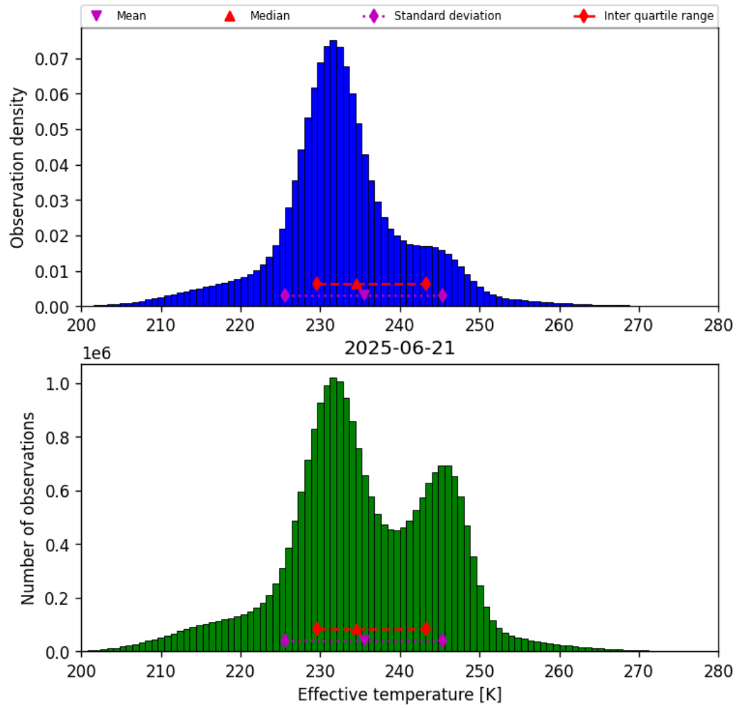
Figure 38: Histogram of “Effective temperature” for 2025-06-21 to 2025-06-22
