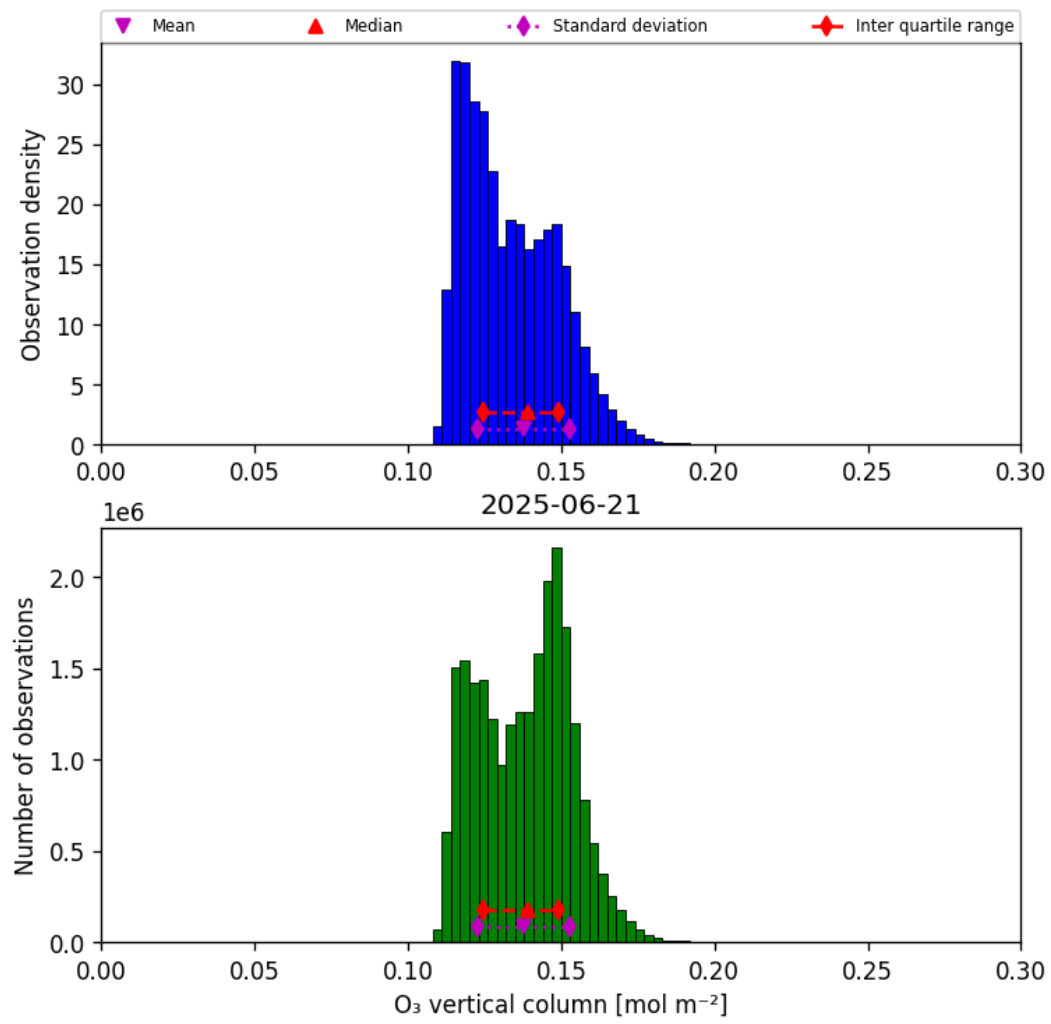
Figure 29: Histogram of “O 3 vertical column” for 2025-06-21 to 2025-06-22
