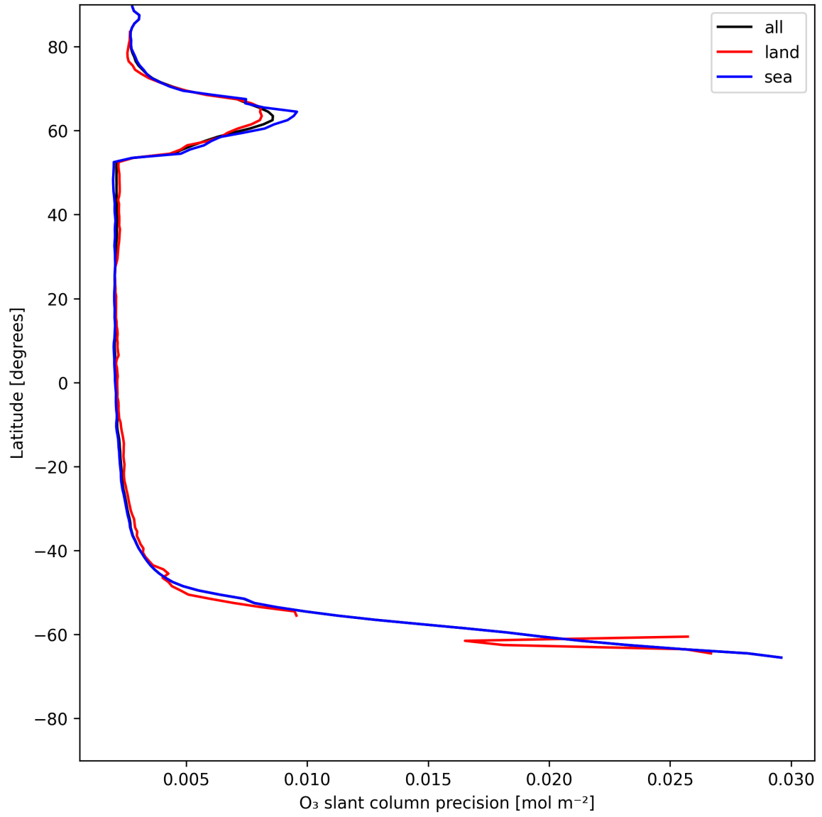
Figure 20: Zonal average of “O 3 slant column precision” for 2025-06-21 to 2025-06-22.
