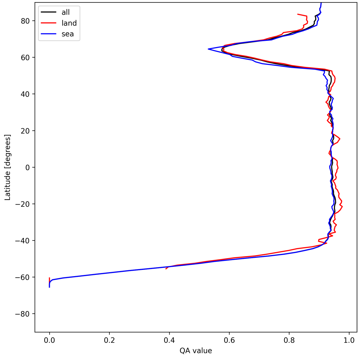
Figure 16: Zonal average of “QA value” for 2025-06-21 to 2025-06-22.
