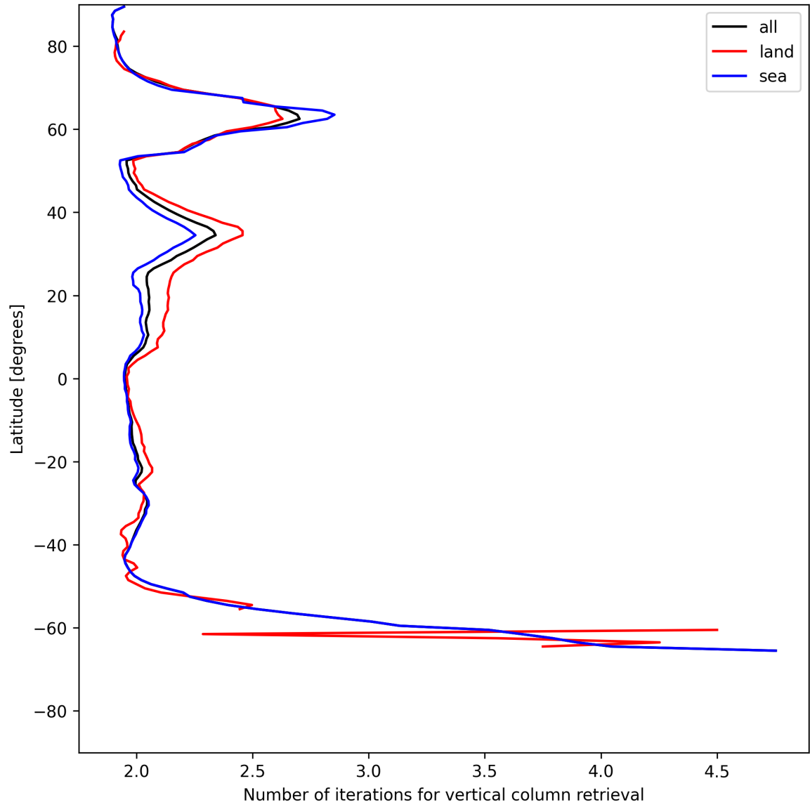
Figure 27: Zonal average of “Number of iterations for vertical column retrieval” for 2025-06-21 to 2025-06-22.
