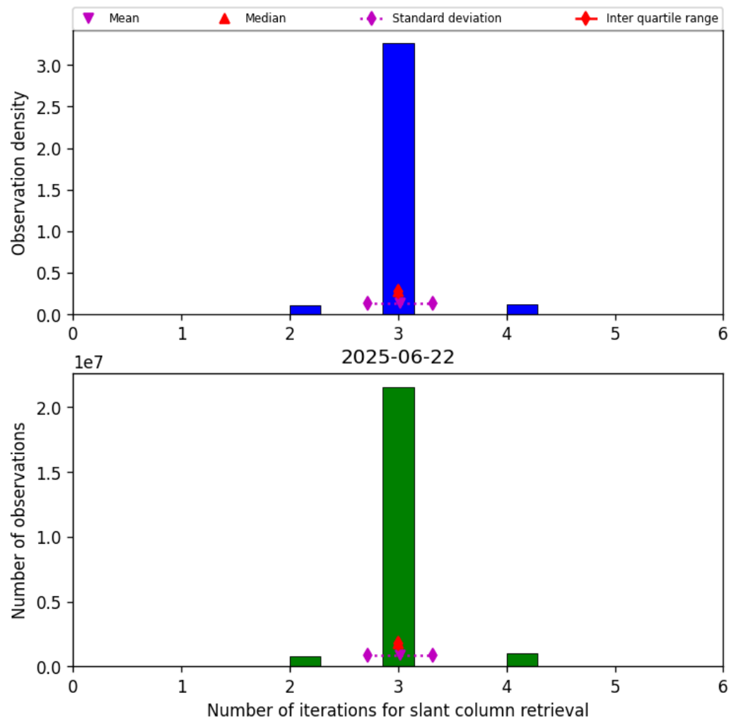
Figure 33: Histogram of "Number of iterations for slant column retrieval" for 2025-06-22 to 2025-06-23
