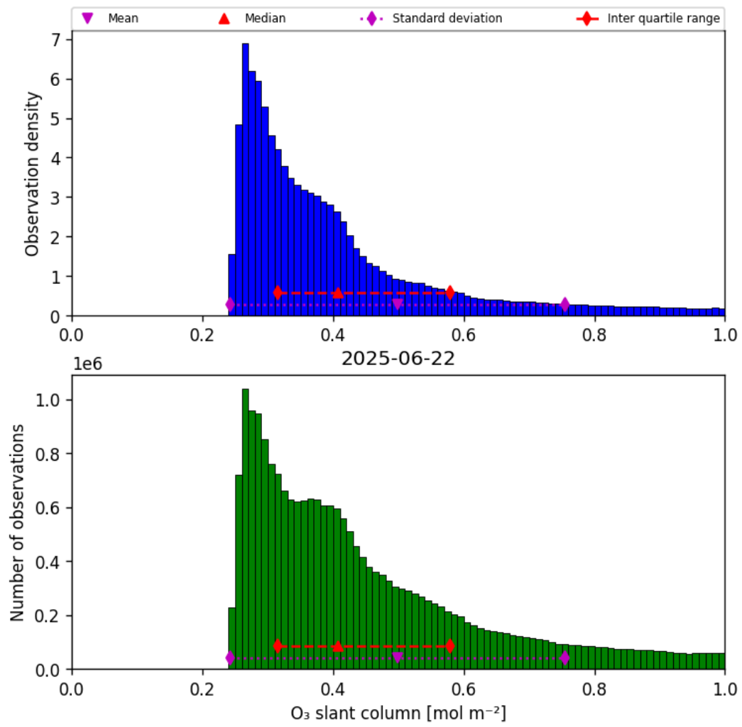
Figure 31: Histogram of “O 3 slant column” for 2025-06-22 to 2025-06-23
