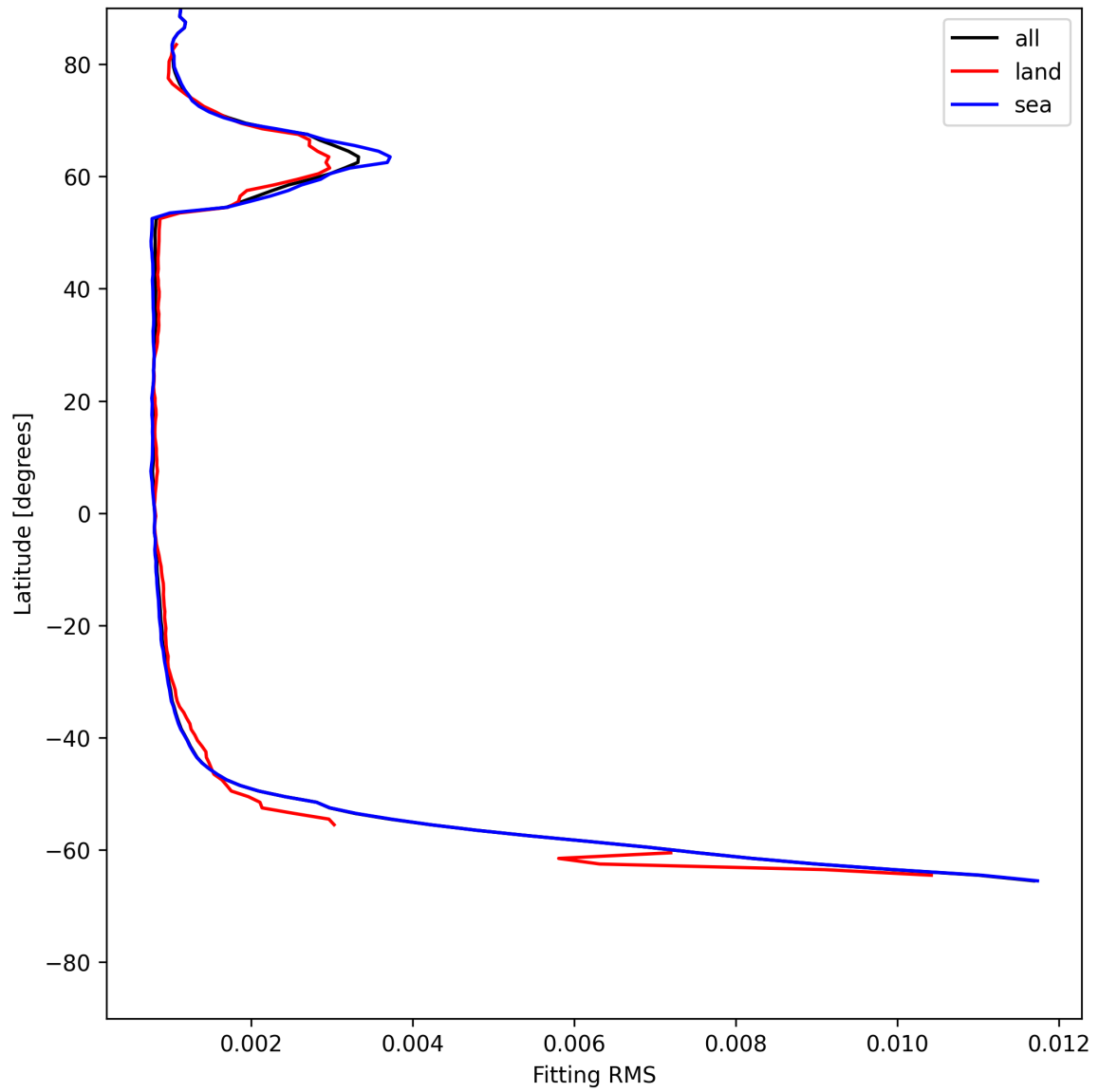
Figure 22: Zonal average of “Fitting RMS” for 2025-06-22 to 2025-06-23.
