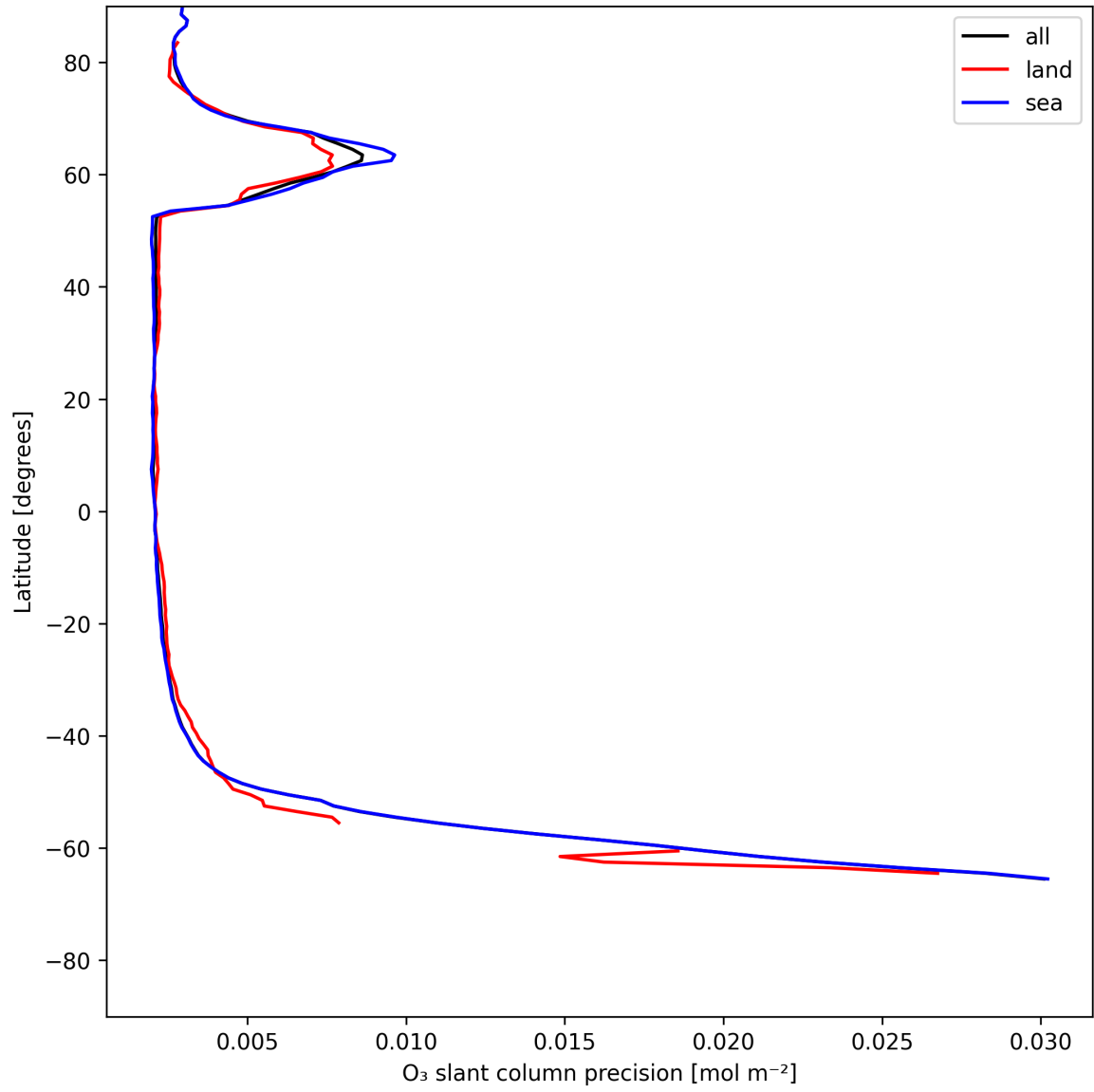
Figure 20: Zonal average of "O 3 slant column precision" for 2025-06-22 to 2025-06-23.
