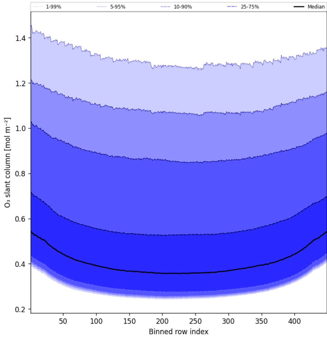
Figure 43: Along track statistics of “O 3 slant column” for 2025-06-22 to 2025-06-23
