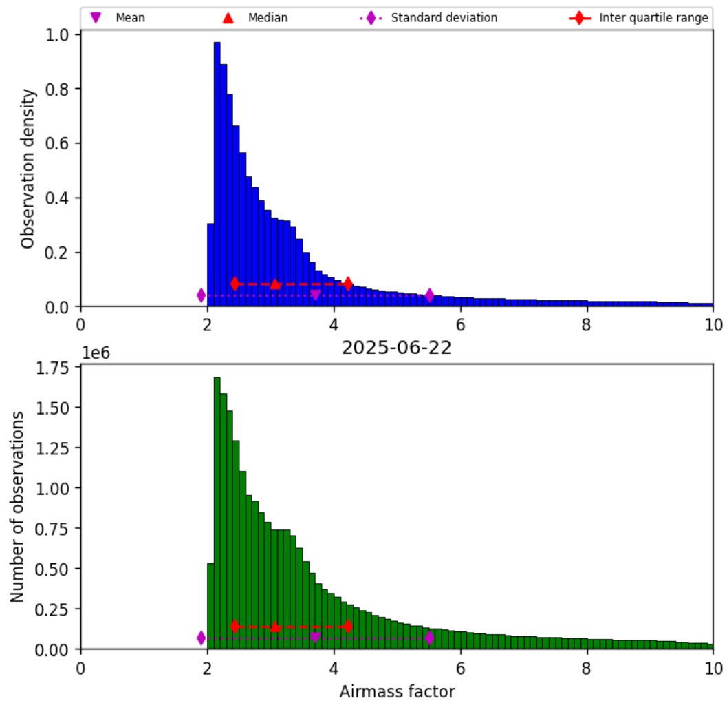
Figure 37: Histogram of “Airmass factor” for 2025-06-22 to 2025-06-23
