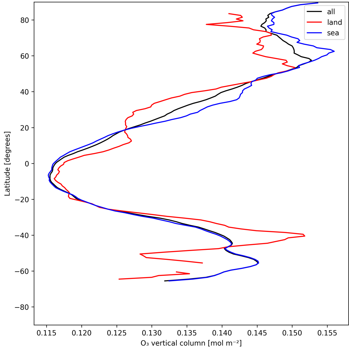
Figure 17: Zonal average of “O 3 vertical column” for 2025-06-22 to 2025-06-23.
