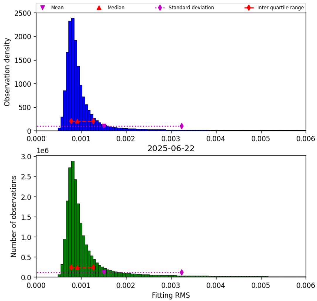
Figure 34: Histogram of “Fitting RMS” for 2025-06-22 to 2025-06-23
