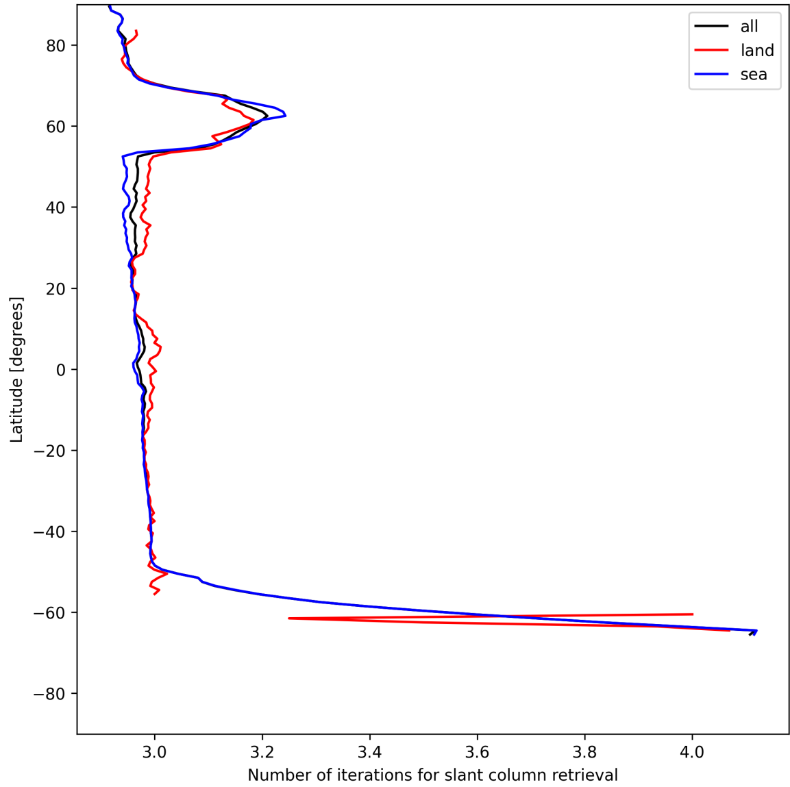
Figure 21: Zonal average of “Number of iterations for slant column retrieval” for 2025-06-22 to 2025-06-23.
