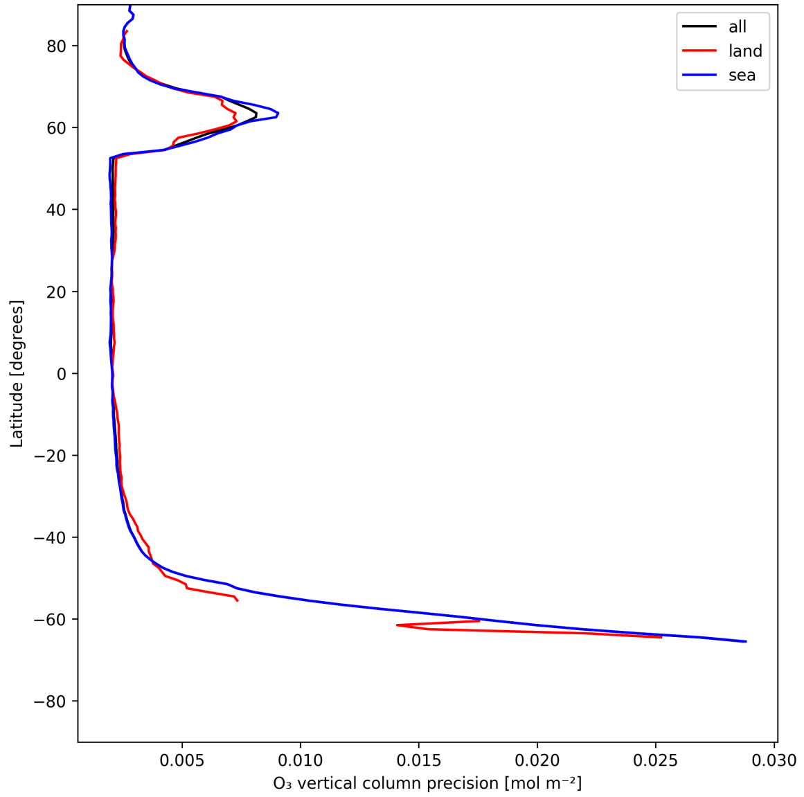
Figure 18: Zonal average of “O 3 vertical column precision” for 2025-06-22 to 2025-06-23.
