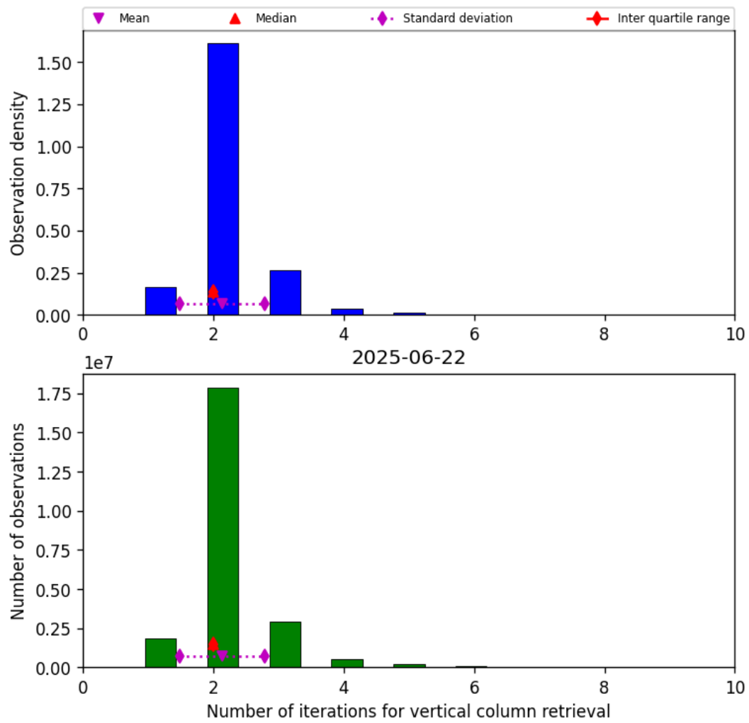
Figure 39: Histogram of “Number of iterations for vertical column retrieval” for 2025-06-22 to 2025-06-23
