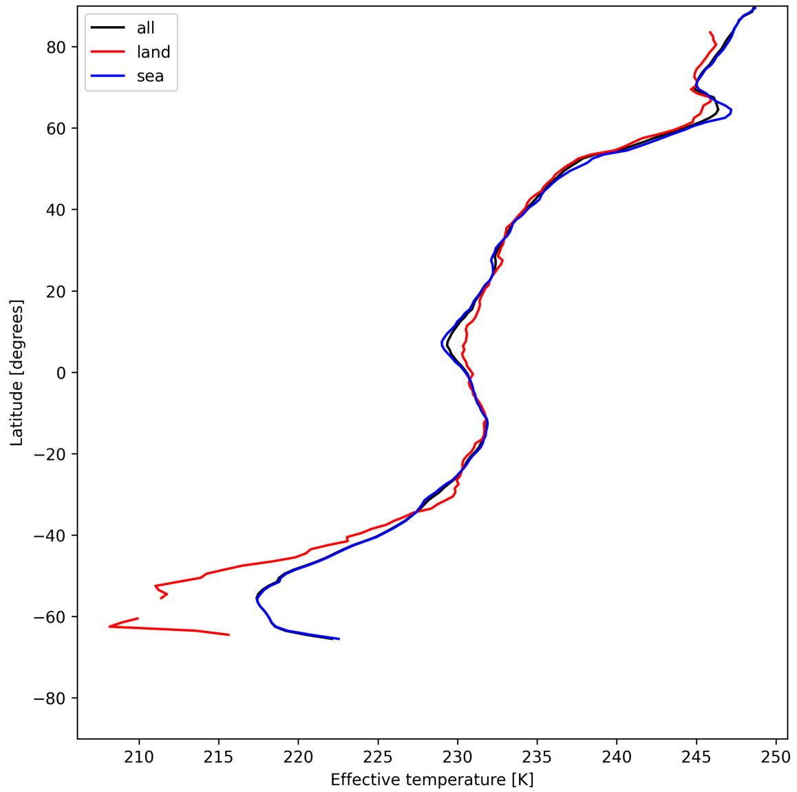
Figure 26: Zonal average of "Effective temperature" for 2025-06-22 to 2025-06-23.
