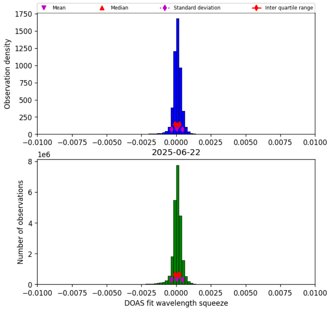
Figure 36: Histogram of “DOAS fit wavelength squeeze” for 2025-06-22 to 2025-06-23
