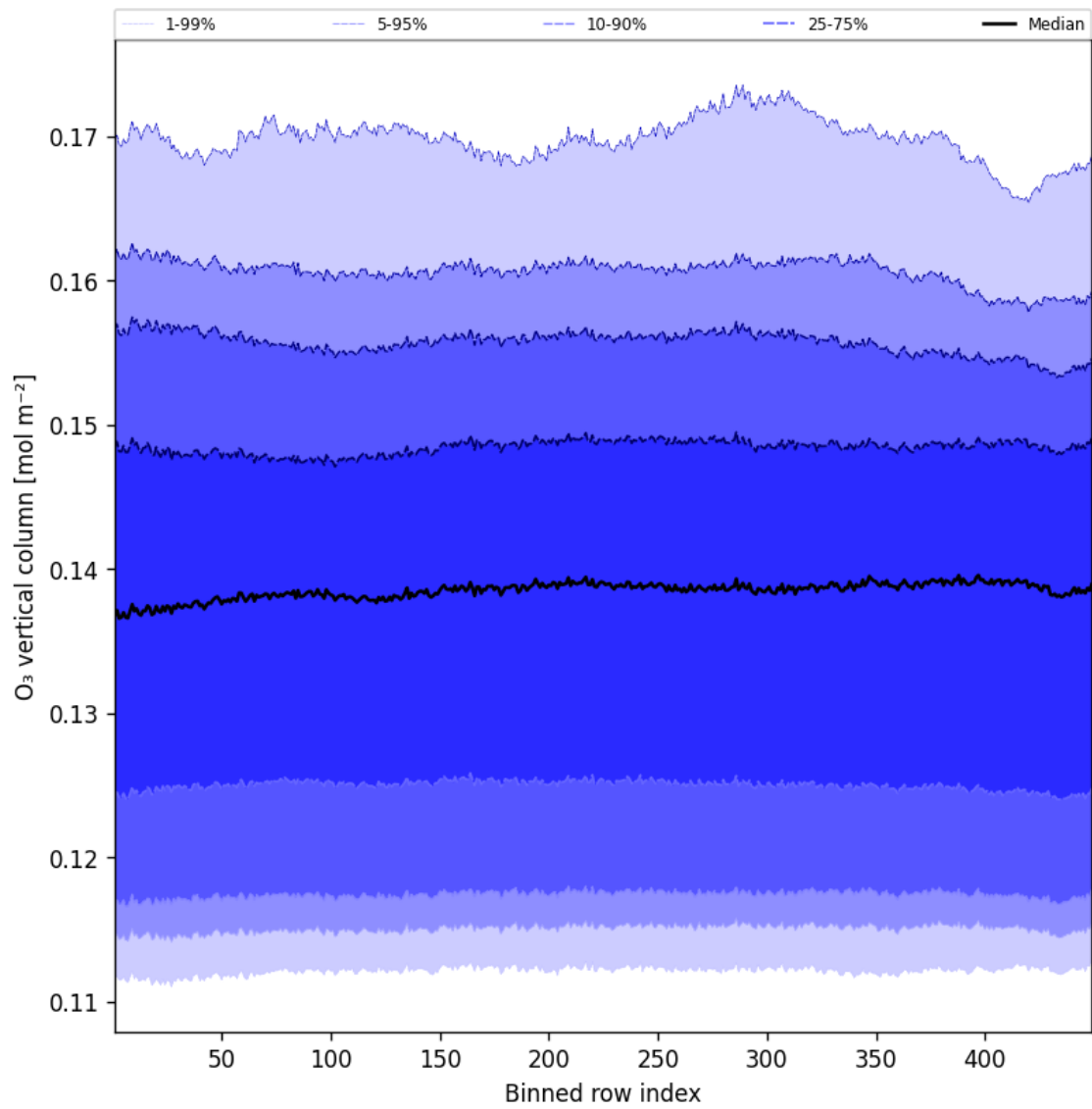
Figure 41: Along track statistics of “O 3 vertical column” for 2025-06-22 to 2025-06-23
