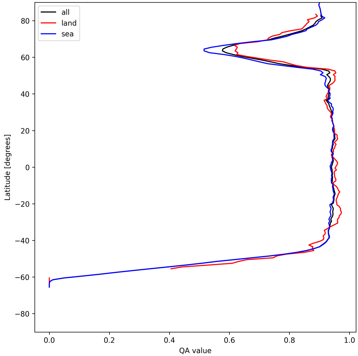
Figure 16: Zonal average of “QA value” for 2025-06-22 to 2025-06-23.
