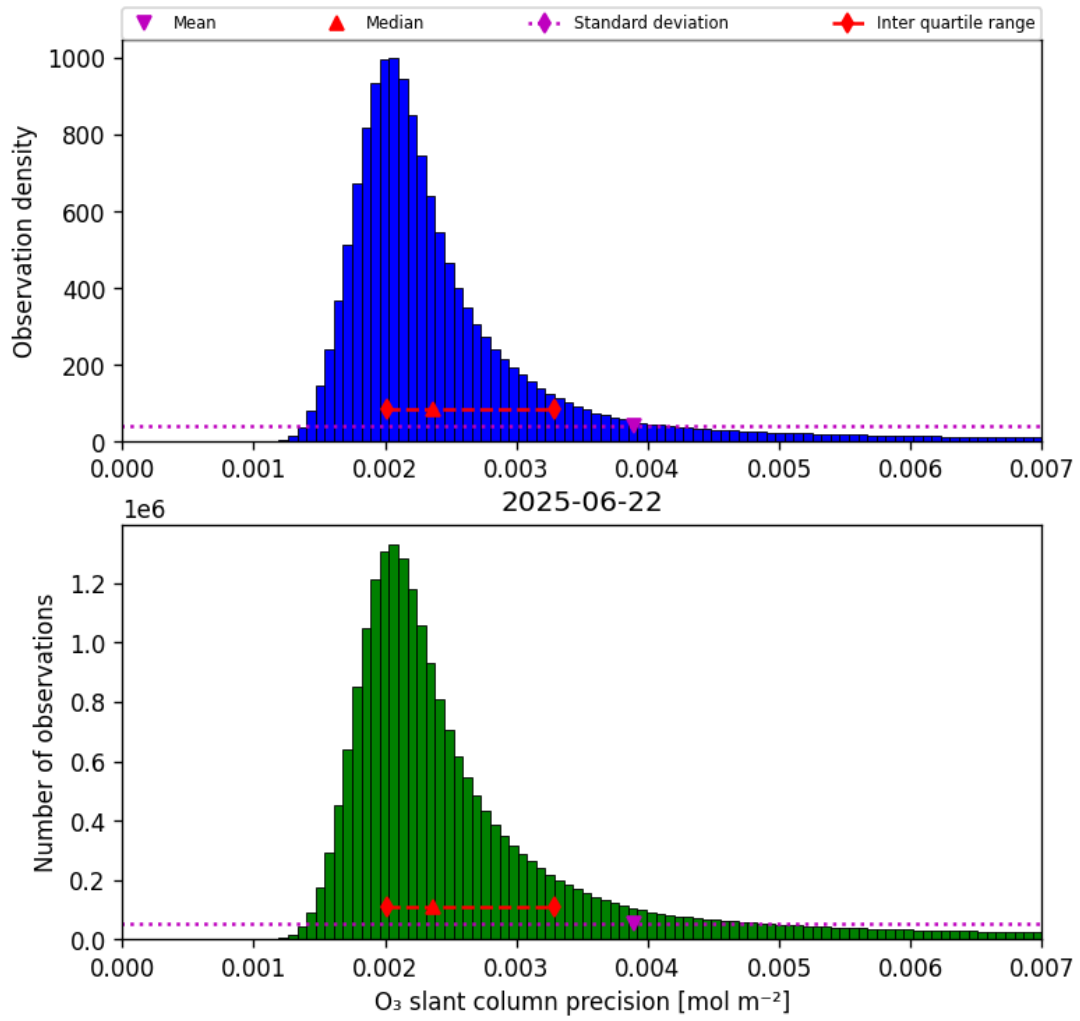
Figure 32: Histogram of “O 3 slant column precision” for 2025-06-22 to 2025-06-23
