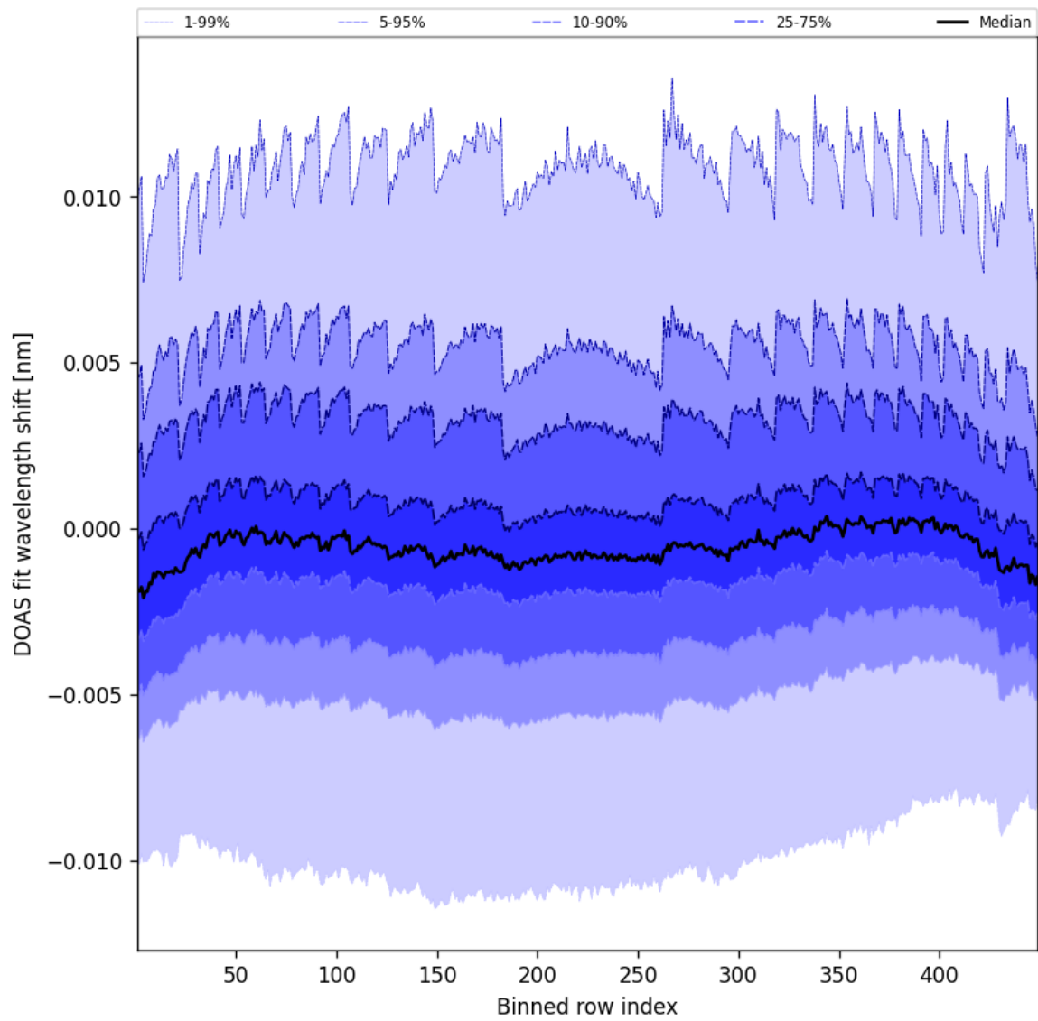
Figure 47: Along track statistics of “DOAS fit wavelength shift” for 2025-06-22 to 2025-06-23
