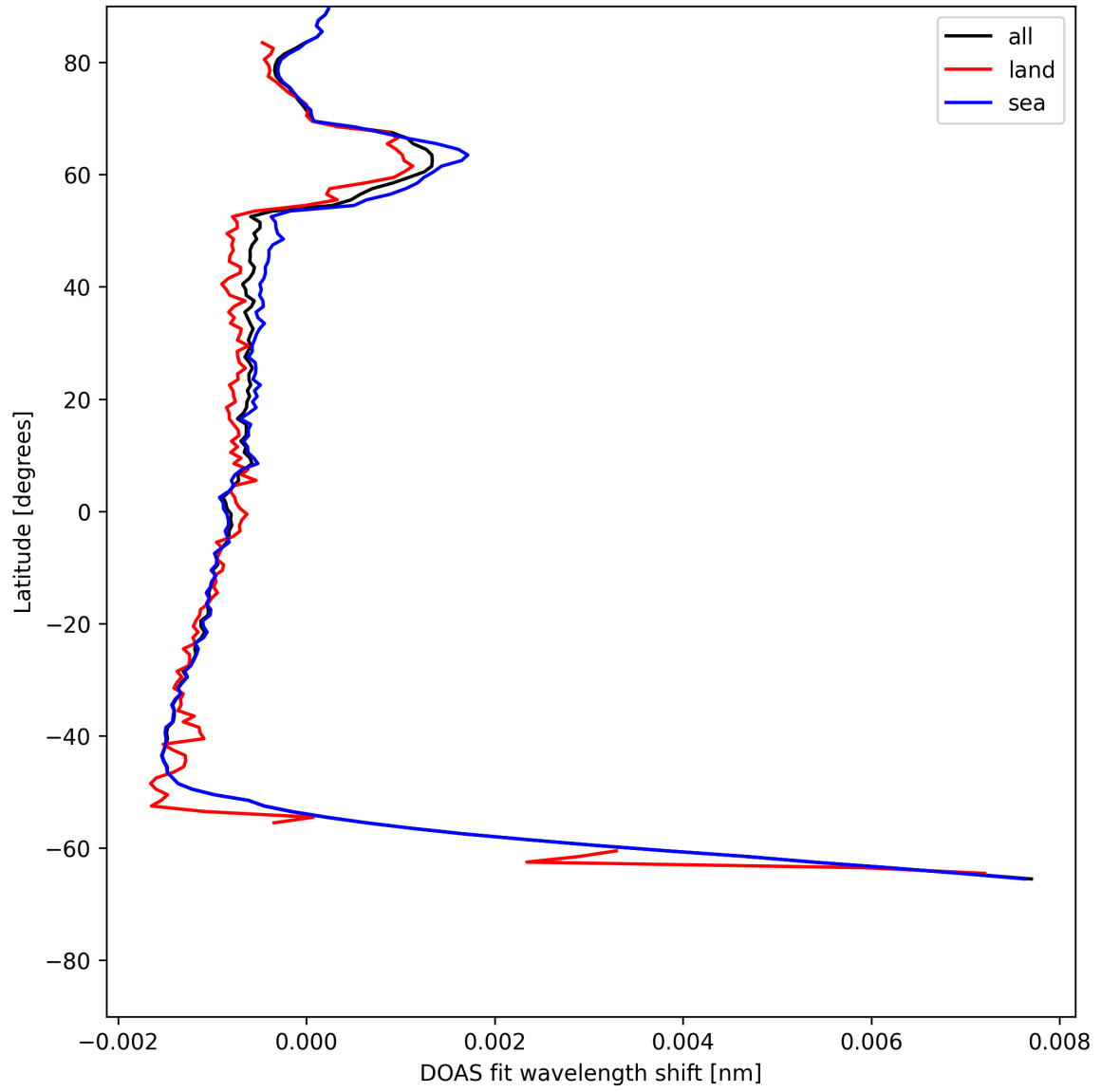
Figure 23: Zonal average of “DOAS fit wavelength shift” for 2025-06-22 to 2025-06-23.
