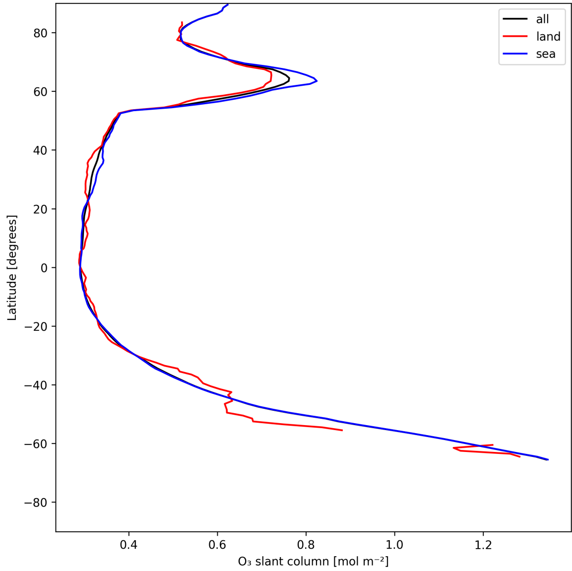
Figure 19: Zonal average of “O 3 slant column” for 2025-06-22 to 2025-06-23.
