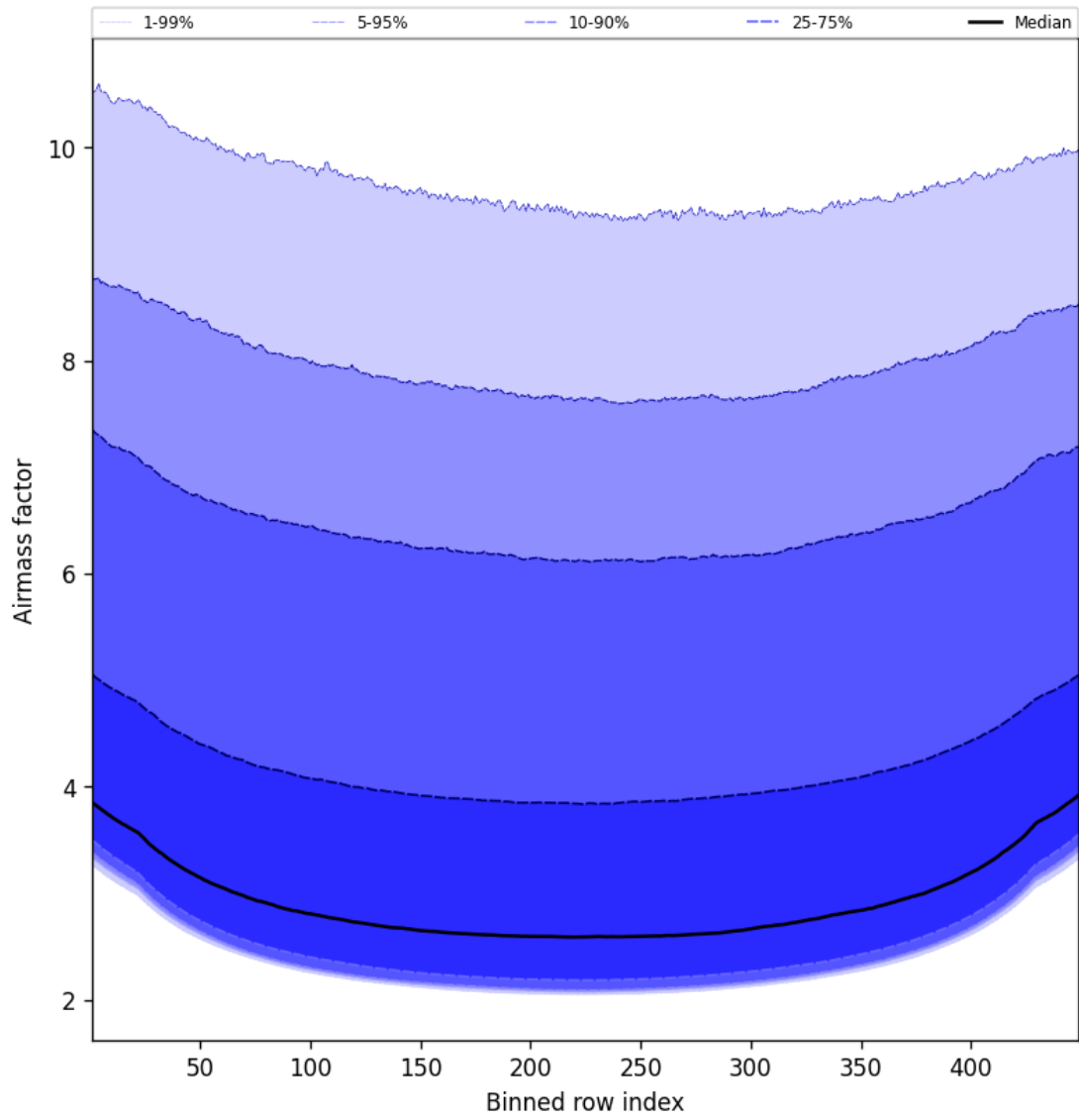
Figure 49: Along track statistics of “Airmass factor” for 2025-06-22 to 2025-06-23
