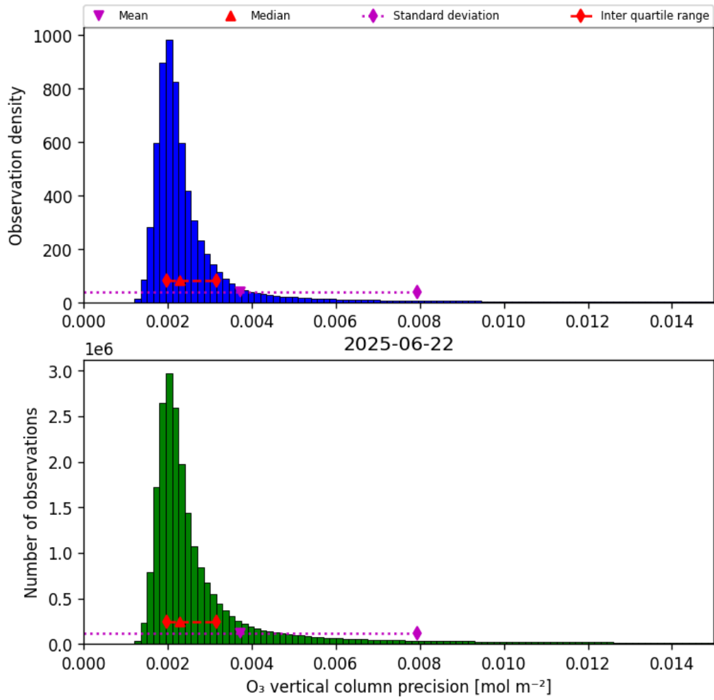
Figure 30: Histogram of "O 3 vertical column precision" for 2025-06-22 to 2025-06-23
