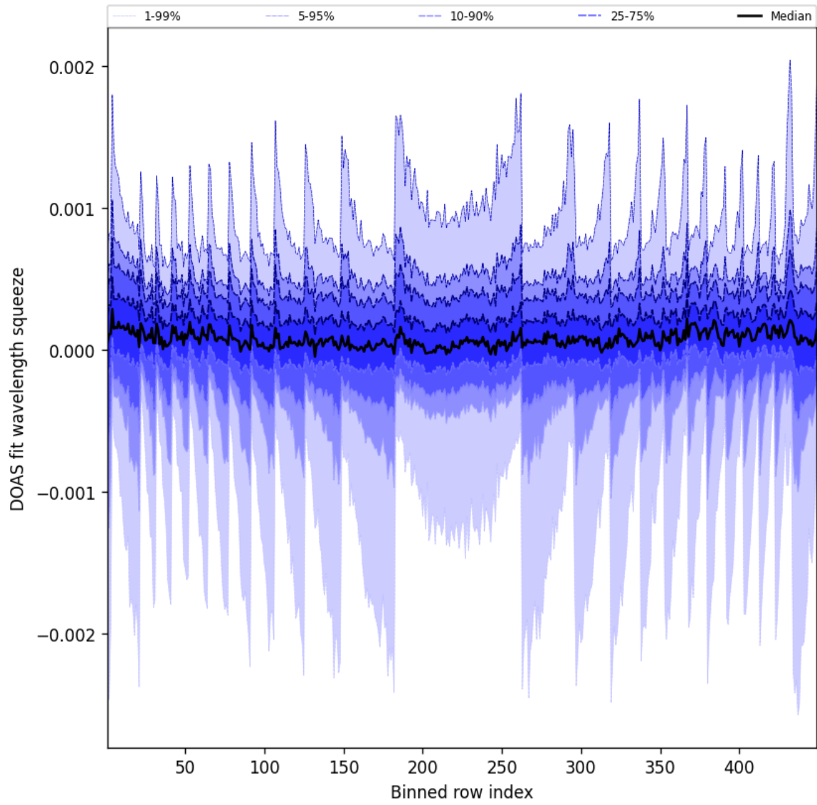
Figure 48: Along track statistics of “DOAS fit wavelength squeeze” for 2025-06-22 to 2025-06-23
