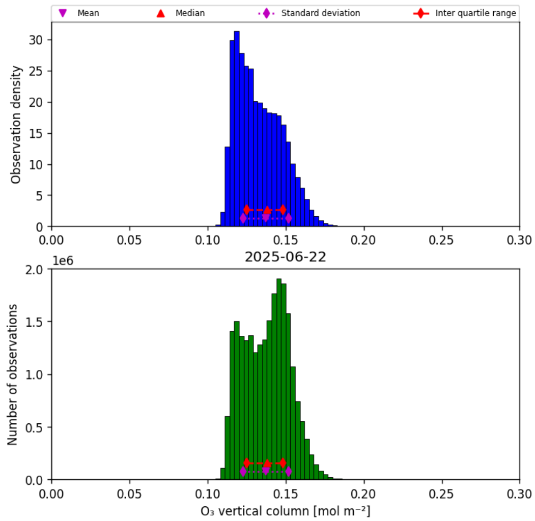
Figure 29: Histogram of “O 3 vertical column” for 2025-06-22 to 2025-06-23
