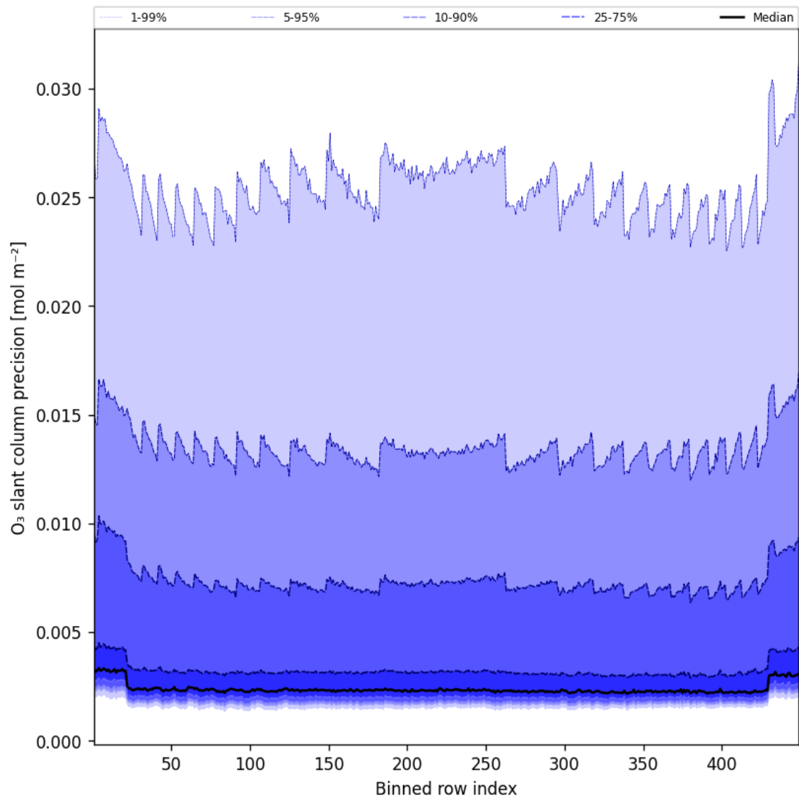
Figure 44: Along track statistics of “O 3 slant column precision” for 2025-06-22 to 2025-06-23
