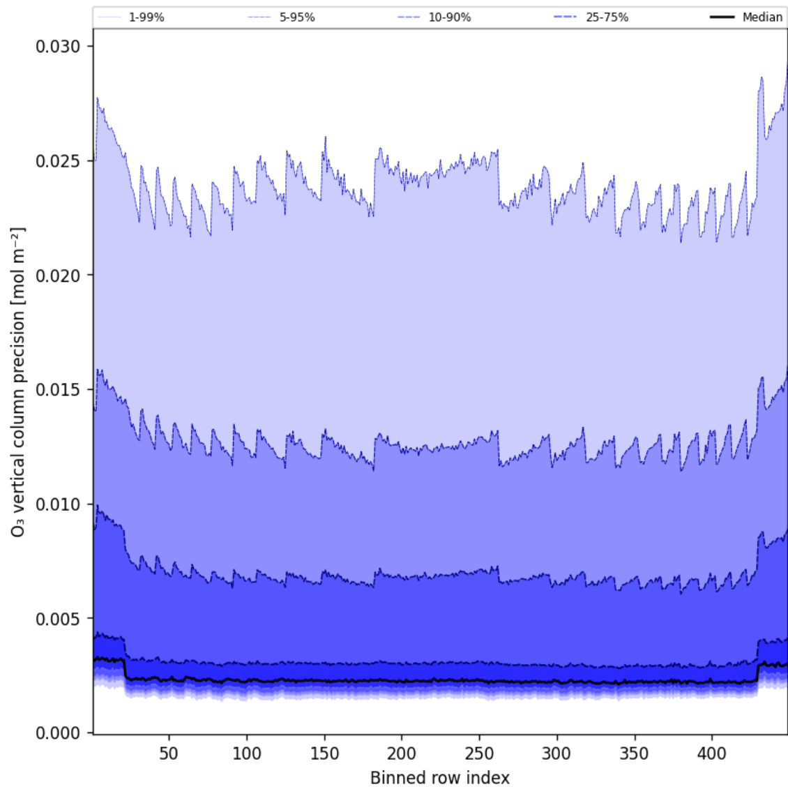
Figure 42: Along track statistics of “O 3 vertical column precision” for 2025-06-22 to 2025-06-23
