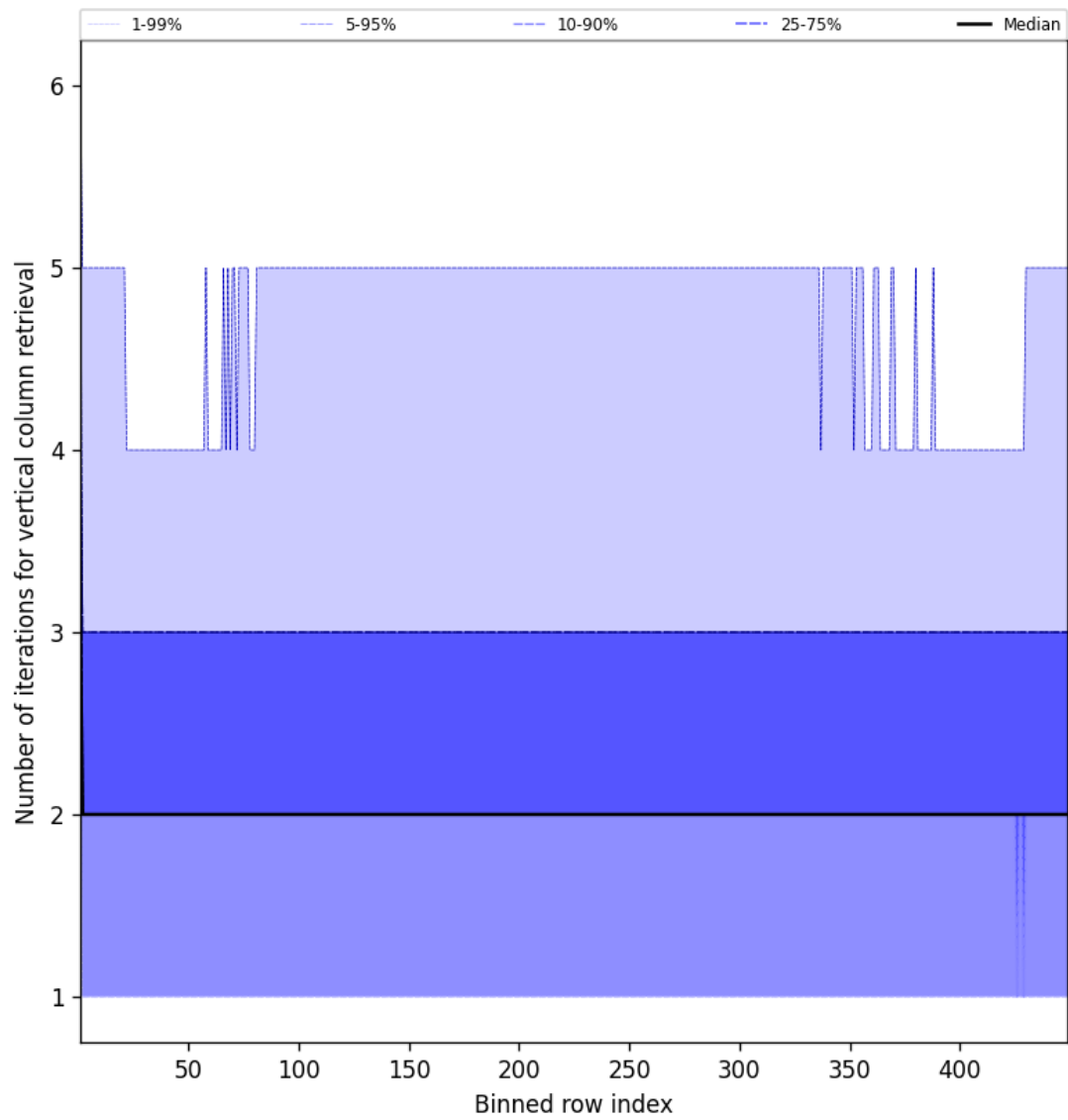
Figure 51: Along track statistics of “Number of iterations for vertical column retrieval” for 2025-06-22 to 2025-06-23
