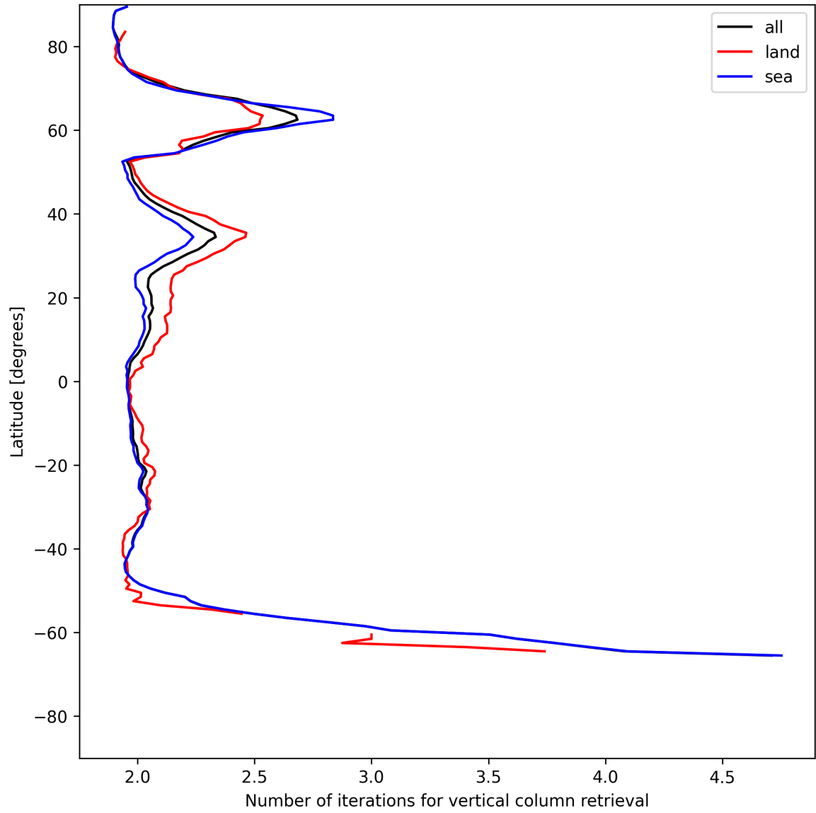
Figure 27: Zonal average of “Number of iterations for vertical column retrieval” for 2025-06-22 to 2025-06-23.
