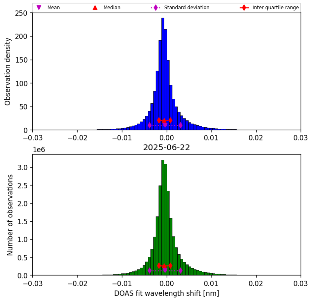
Figure 35: Histogram of “DOAS fit wavelength shift” for 2025-06-22 to 2025-06-23
