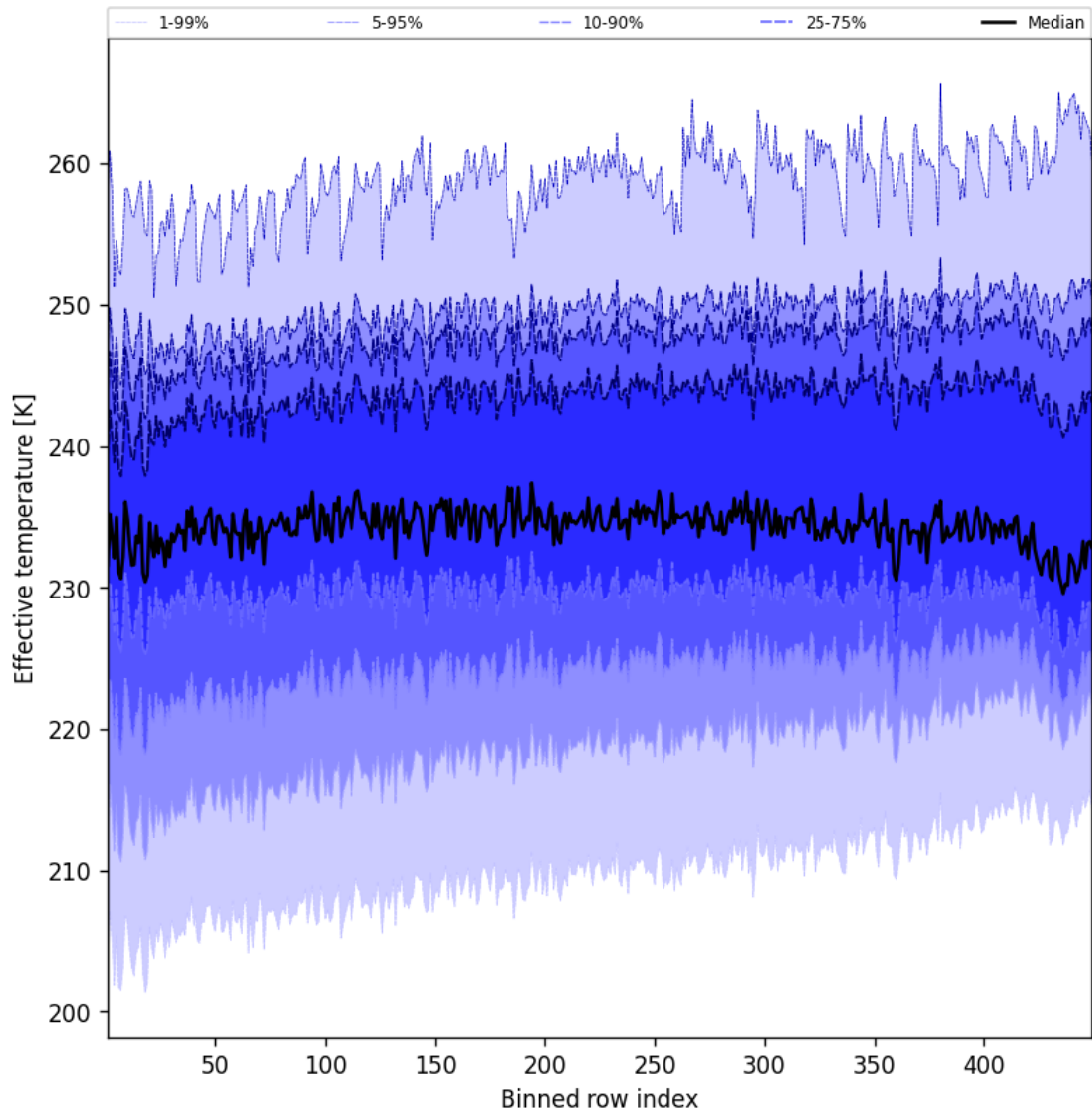
Figure 50: Along track statistics of “Effective temperature” for 2025-06-22 to 2025-06-23
