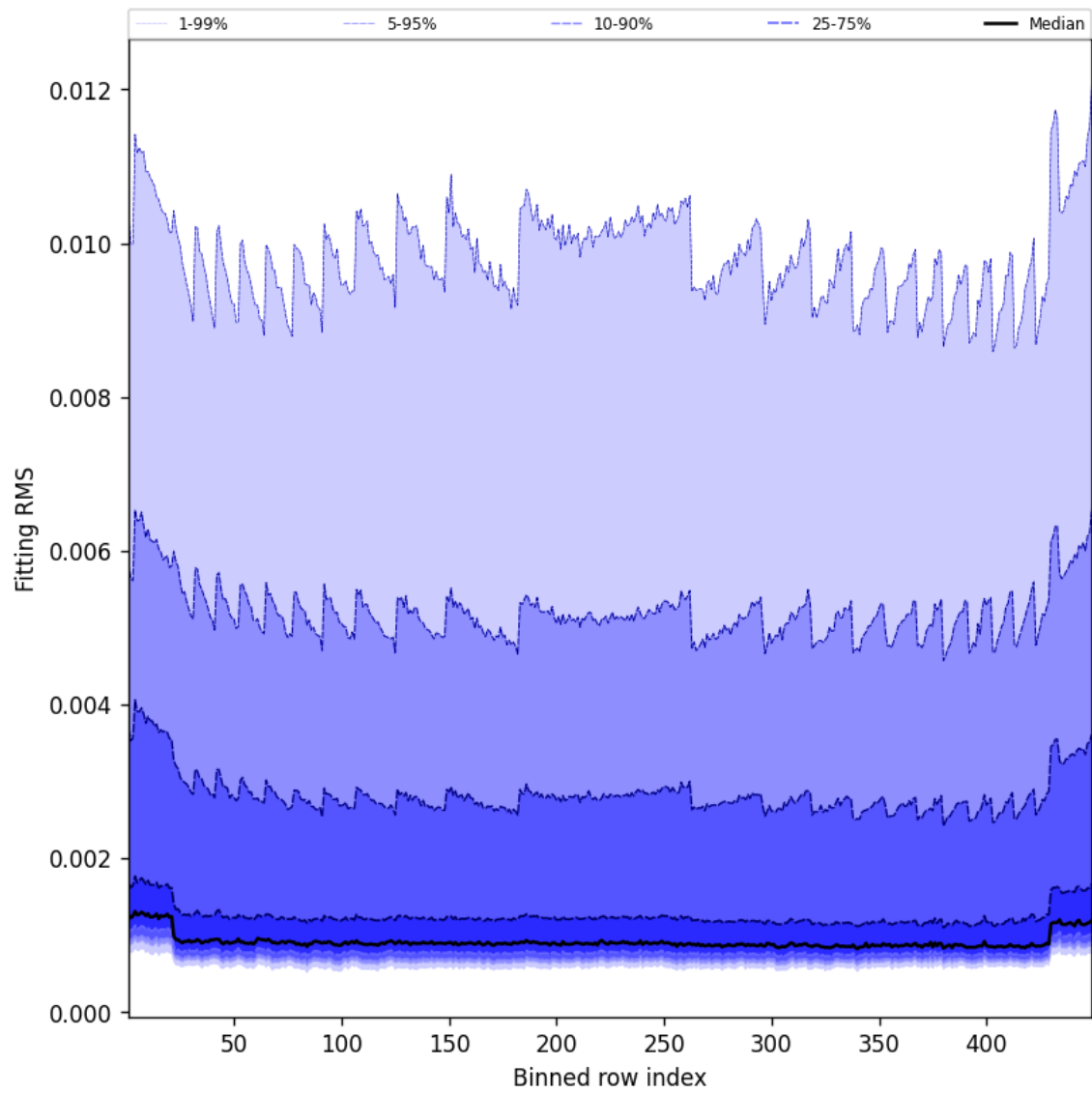
Figure 46: Along track statistics of “Fitting RMS” for 2025-06-22 to 2025-06-23
