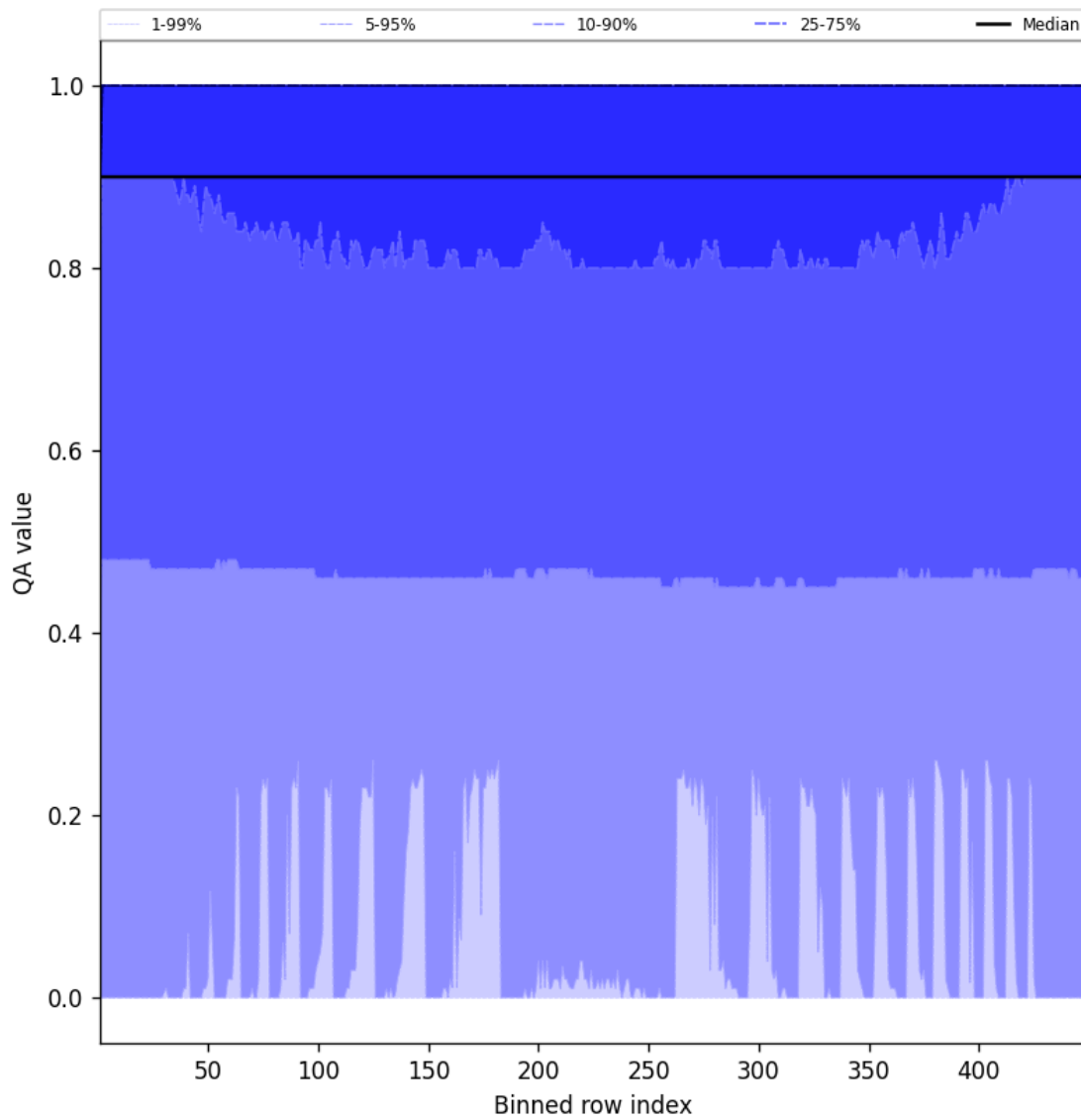
Figure 40: Along track statistics of “QA value” for 2025-06-22 to 2025-06-23
