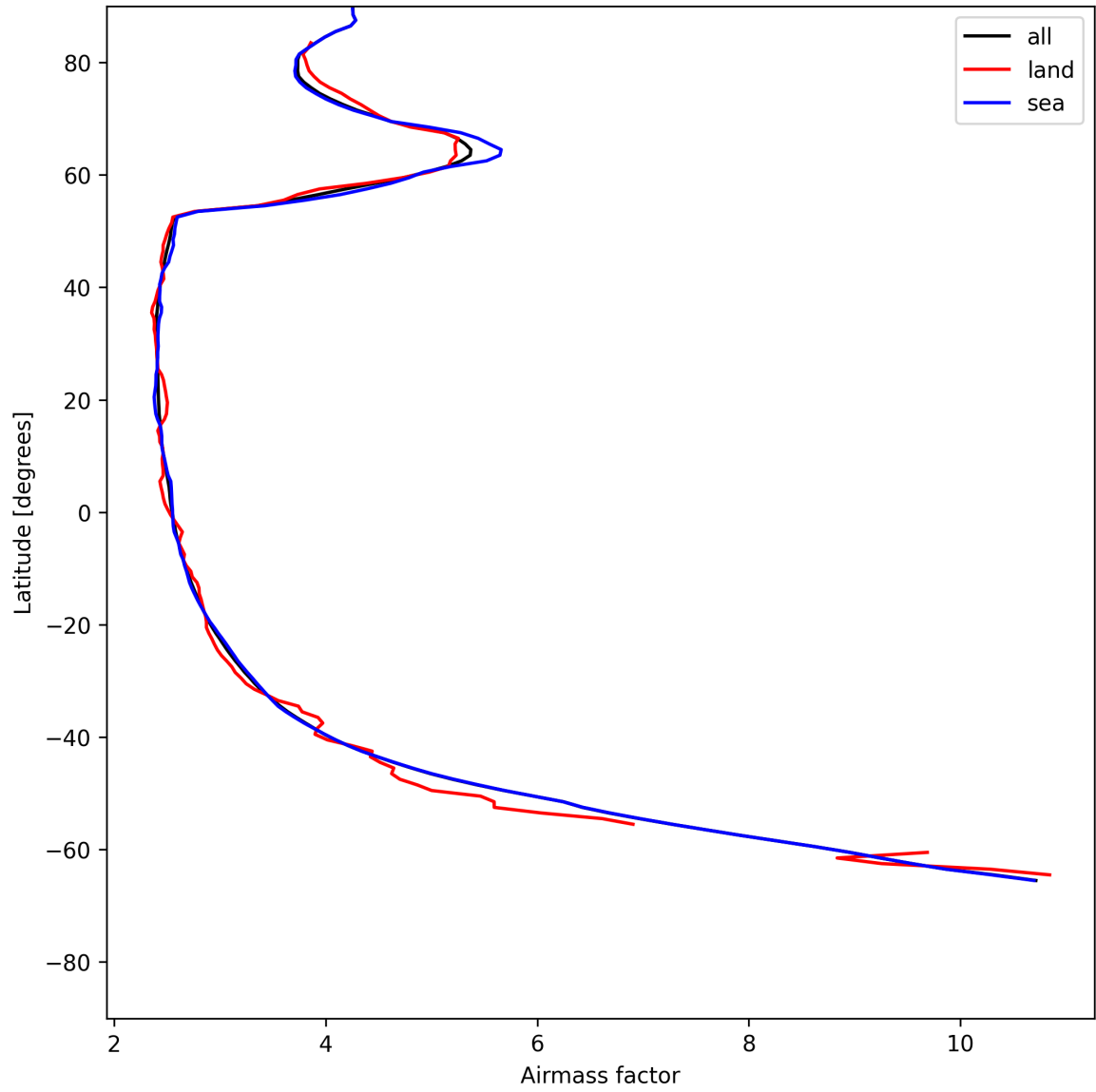
Figure 25: Zonal average of “Airmass factor” for 2025-06-22 to 2025-06-23.
