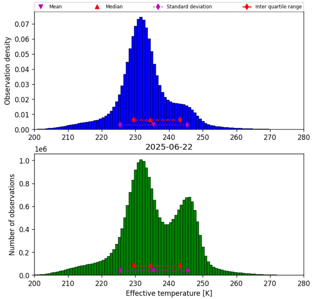
Figure 38: Histogram of “Effective temperature” for 2025-06-22 to 2025-06-23
