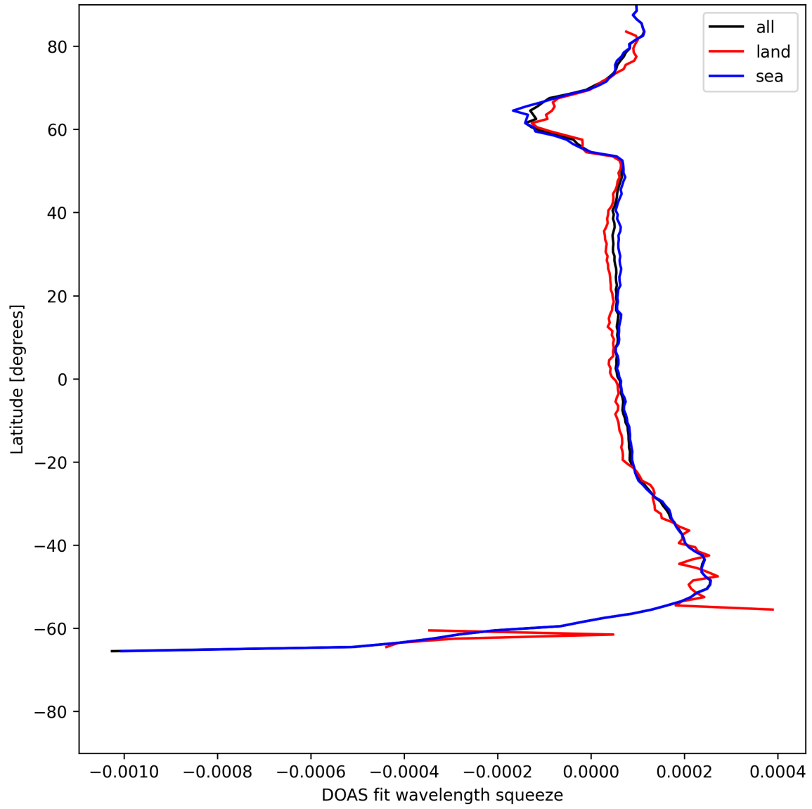
Figure 24: Zonal average of “DOAS fit wavelength squeeze” for 2025-06-22 to 2025-06-23.
