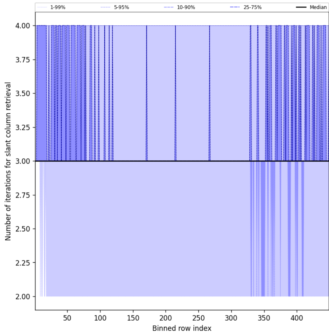
Figure 45: Along track statistics of “Number of iterations for slant column retrieval” for 2025-06-22 to 2025-06-23
