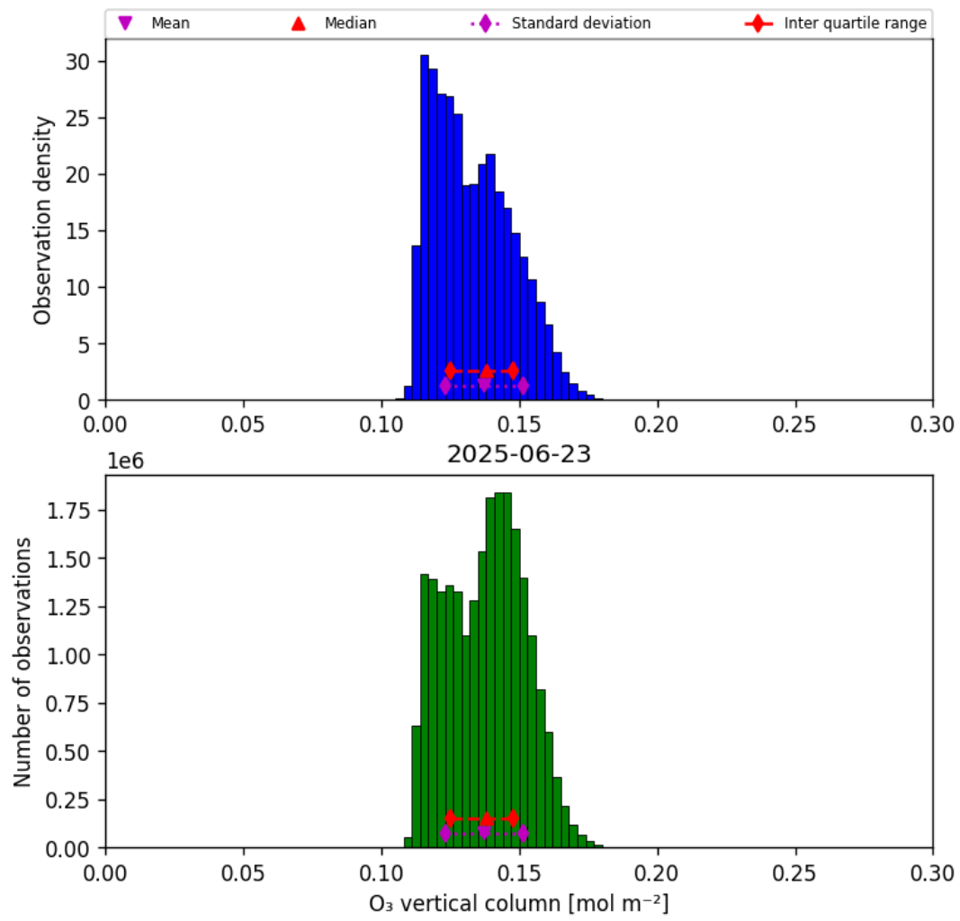
Figure 29: Histogram of “O 3 vertical column” for 2025-06-23 to 2025-06-24
