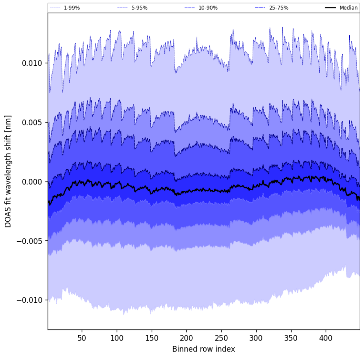
Figure 47: Along track statistics of “DOAS fit wavelength shift” for 2025-06-23 to 2025-06-24
