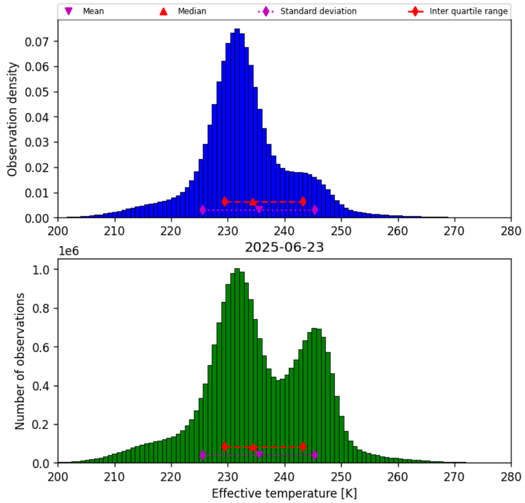
Figure 38: Histogram of “Effective temperature” for 2025-06-23 to 2025-06-24
