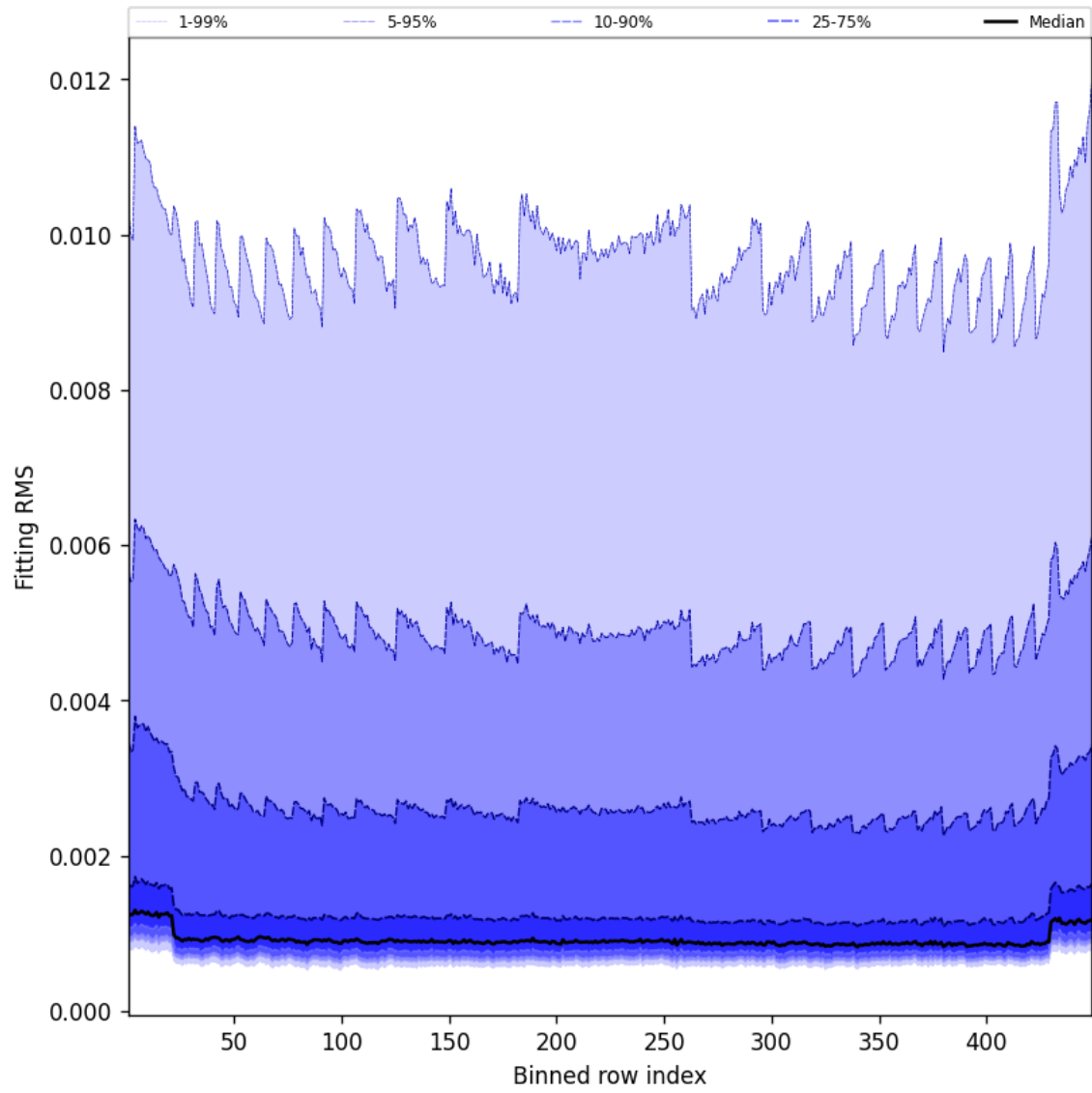
Figure 46: Along track statistics of “Fitting RMS” for 2025-06-23 to 2025-06-24
