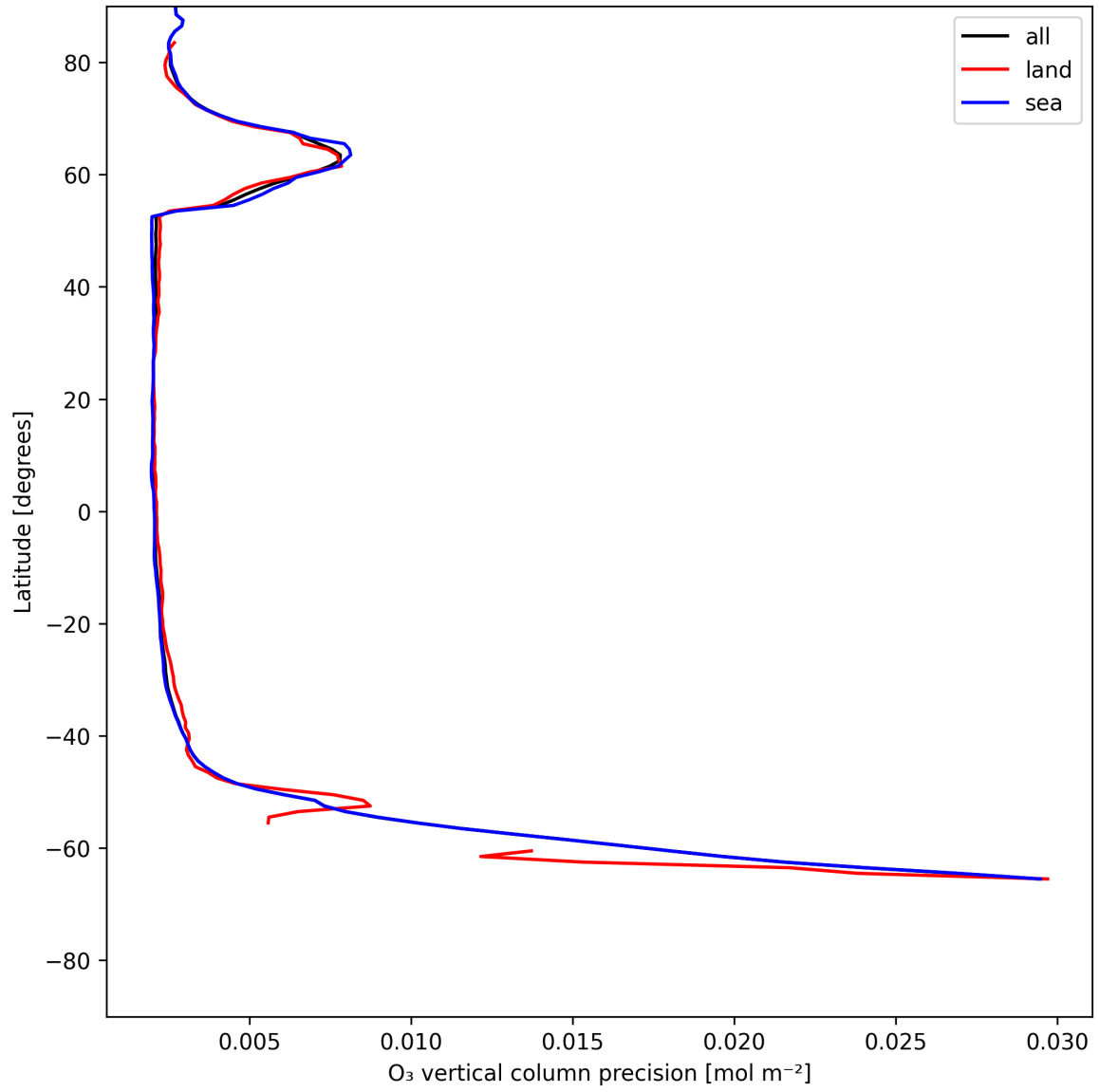
Figure 18: Zonal average of "O 3 vertical column precision" for 2025-06-23 to 2025-06-24.
