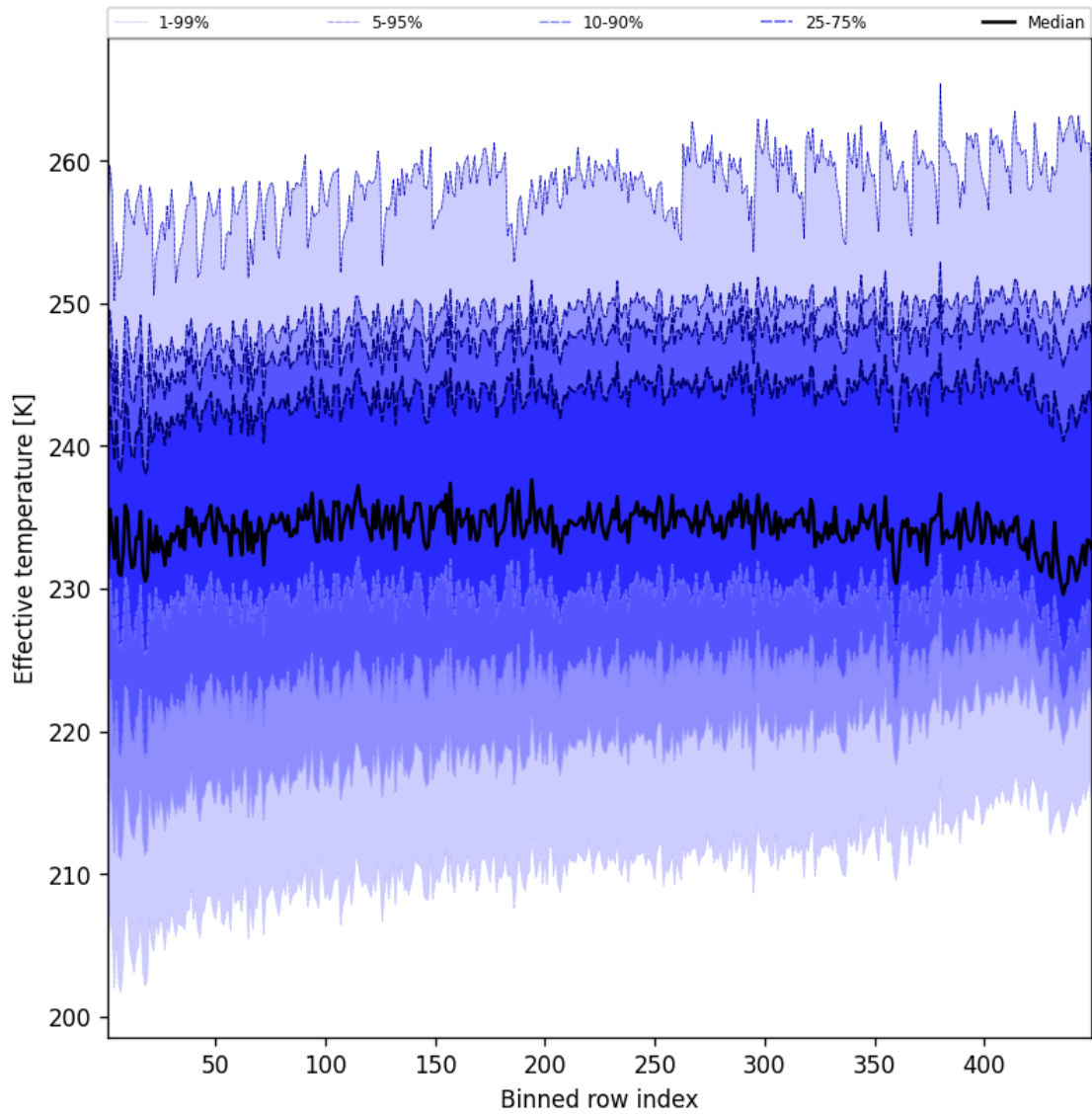
Figure 50: Along track statistics of “Effective temperature” for 2025-06-23 to 2025-06-24
