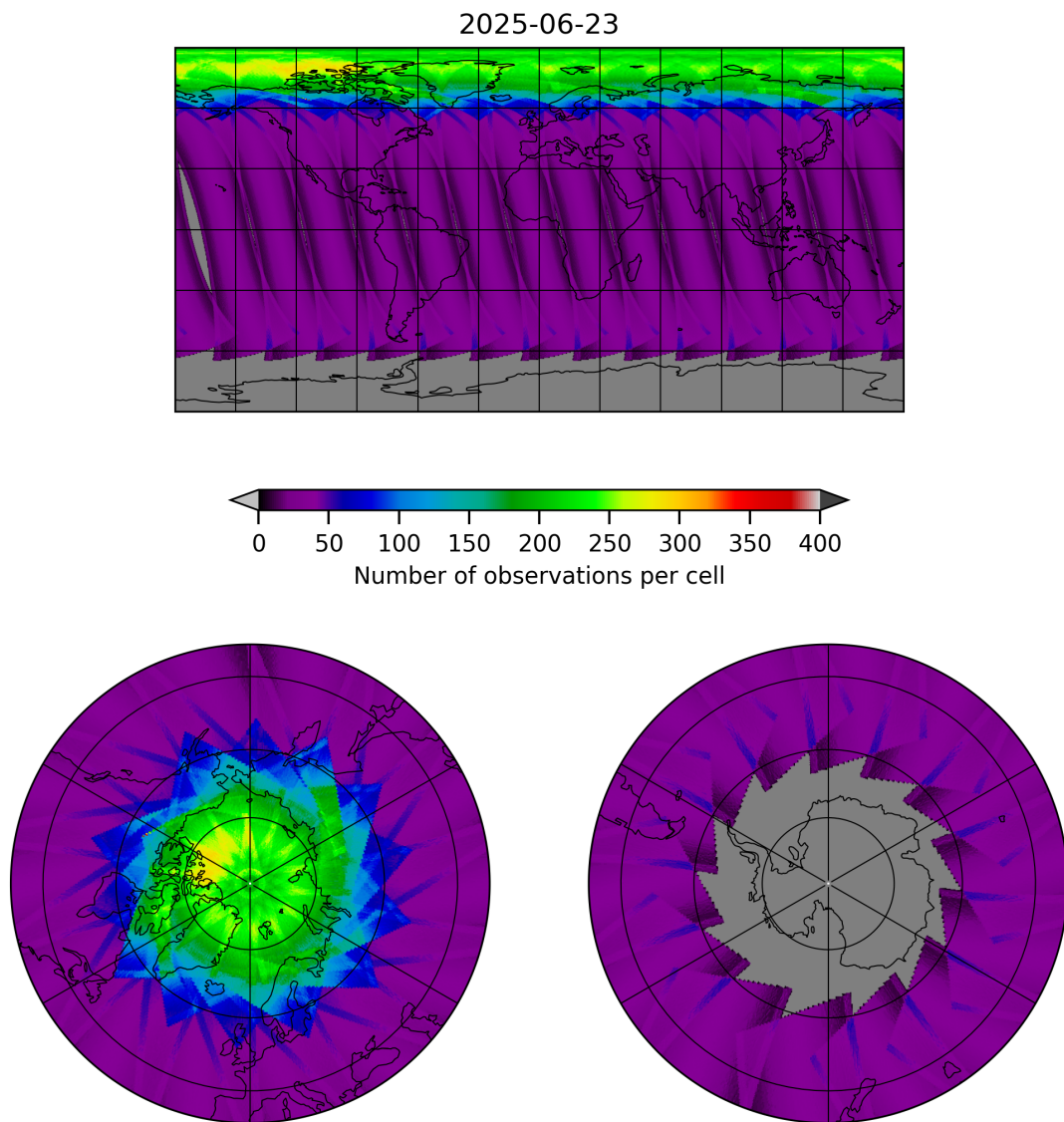
Figure 15: Map of the number of observations for 2025-06-23 to 2025-06-24
