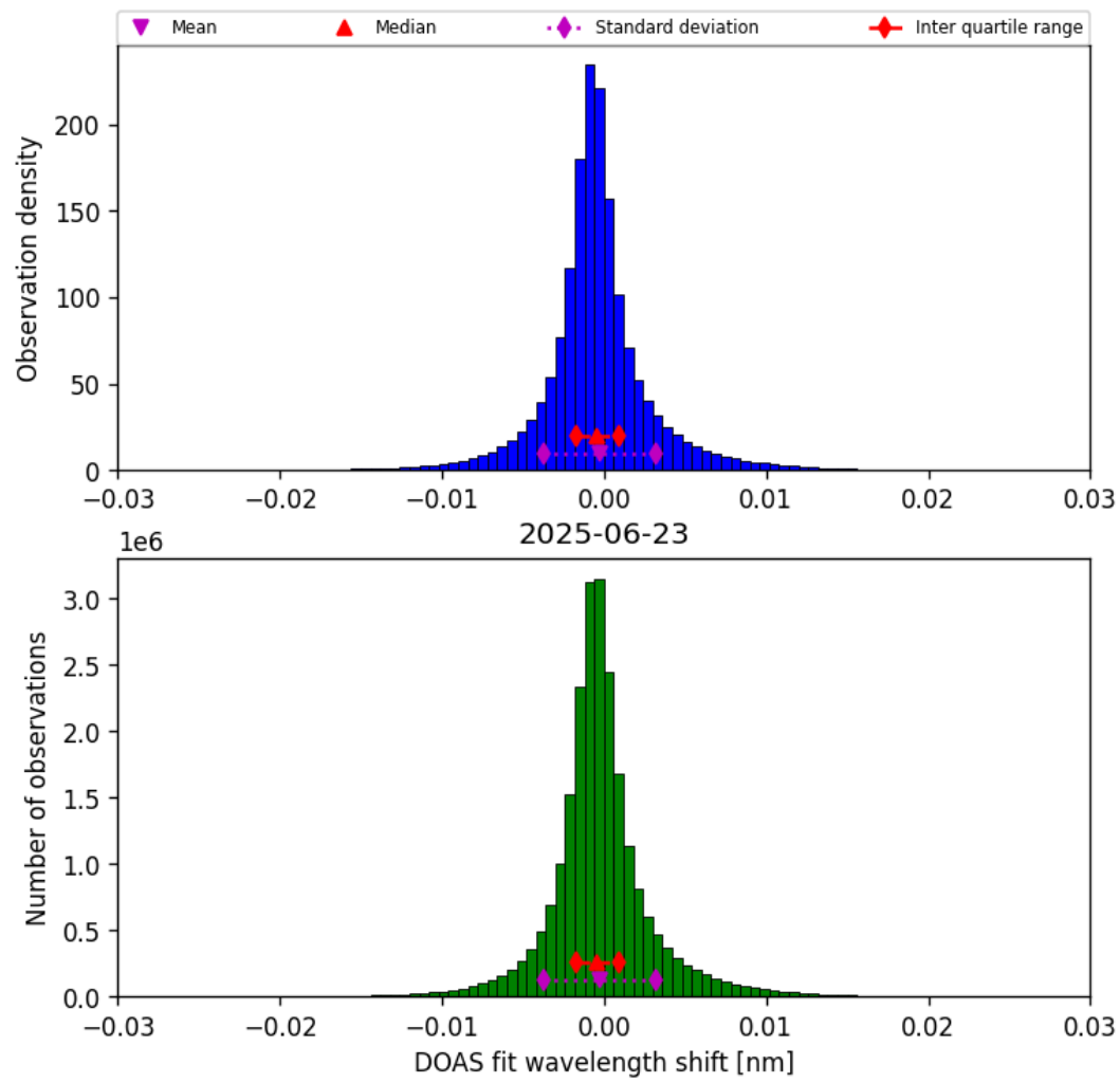
Figure 35: Histogram of “DOAS fit wavelength shift” for 2025-06-23 to 2025-06-24
