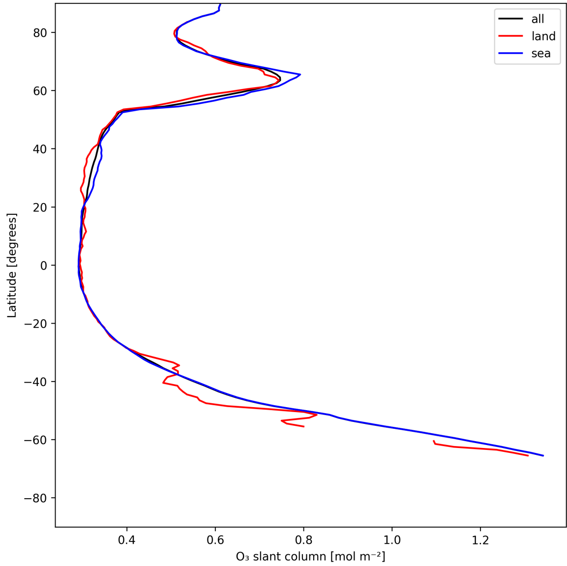
Figure 19: Zonal average of “O 3 slant column” for 2025-06-23 to 2025-06-24.
