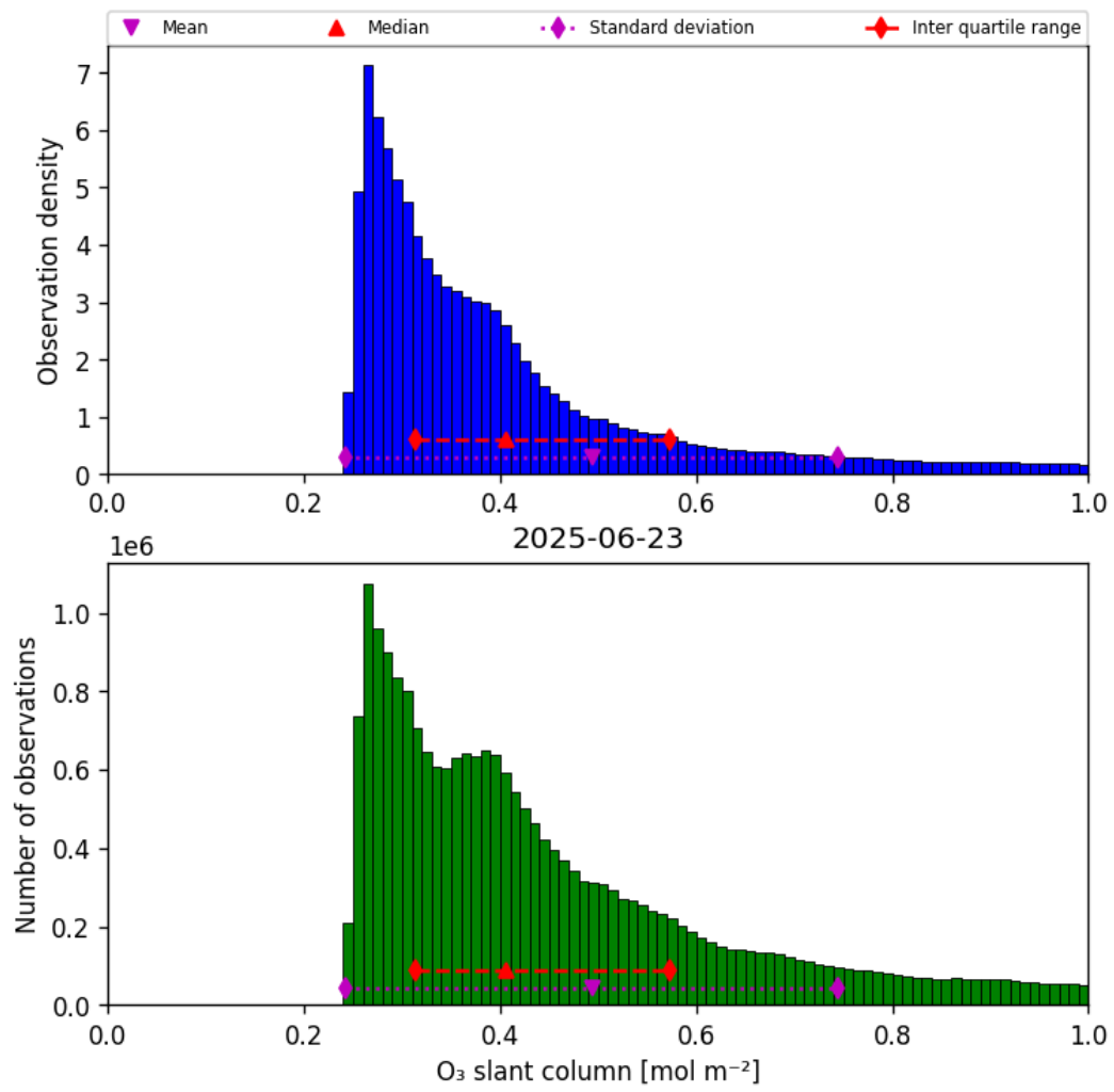
Figure 31: Histogram of “O 3 slant column” for 2025-06-23 to 2025-06-24
