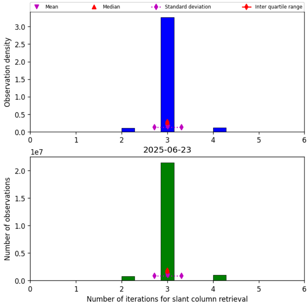
Figure 33: Histogram of “Number of iterations for slant column retrieval” for 2025-06-23 to 2025-06-24
