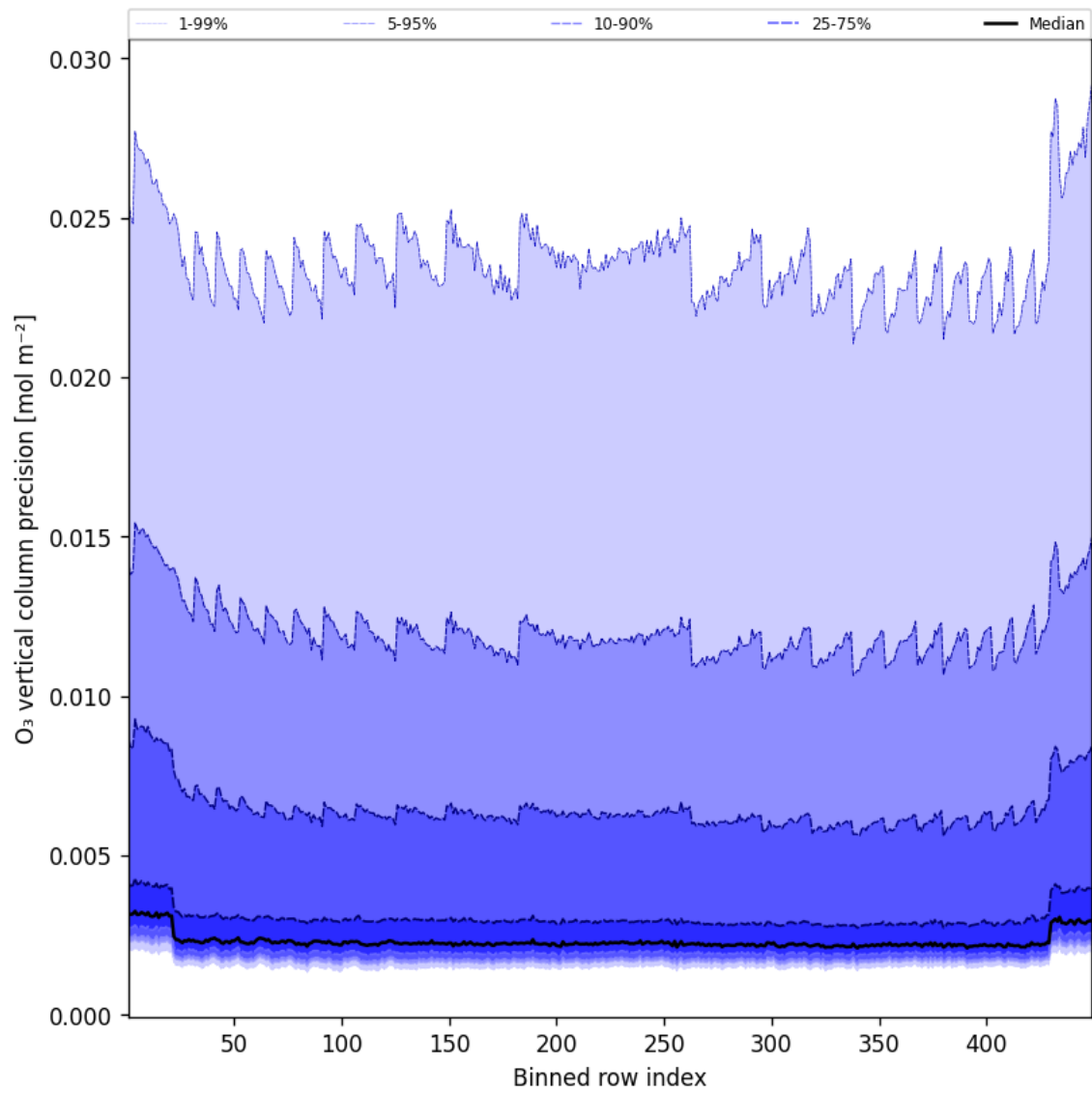
Figure 42: Along track statistics of “O 3 vertical column precision” for 2025-06-23 to 2025-06-24
