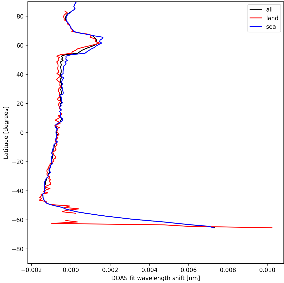
Figure 23: Zonal average of “DOAS fit wavelength shift” for 2025-06-23 to 2025-06-24.
