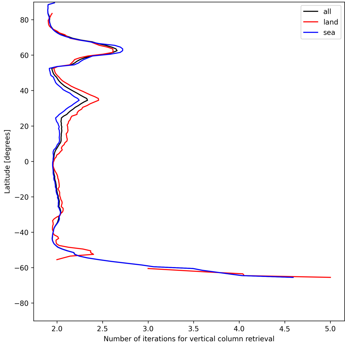
Figure 27: Zonal average of “Number of iterations for vertical column retrieval” for 2025-06-23 to 2025-06-24.
