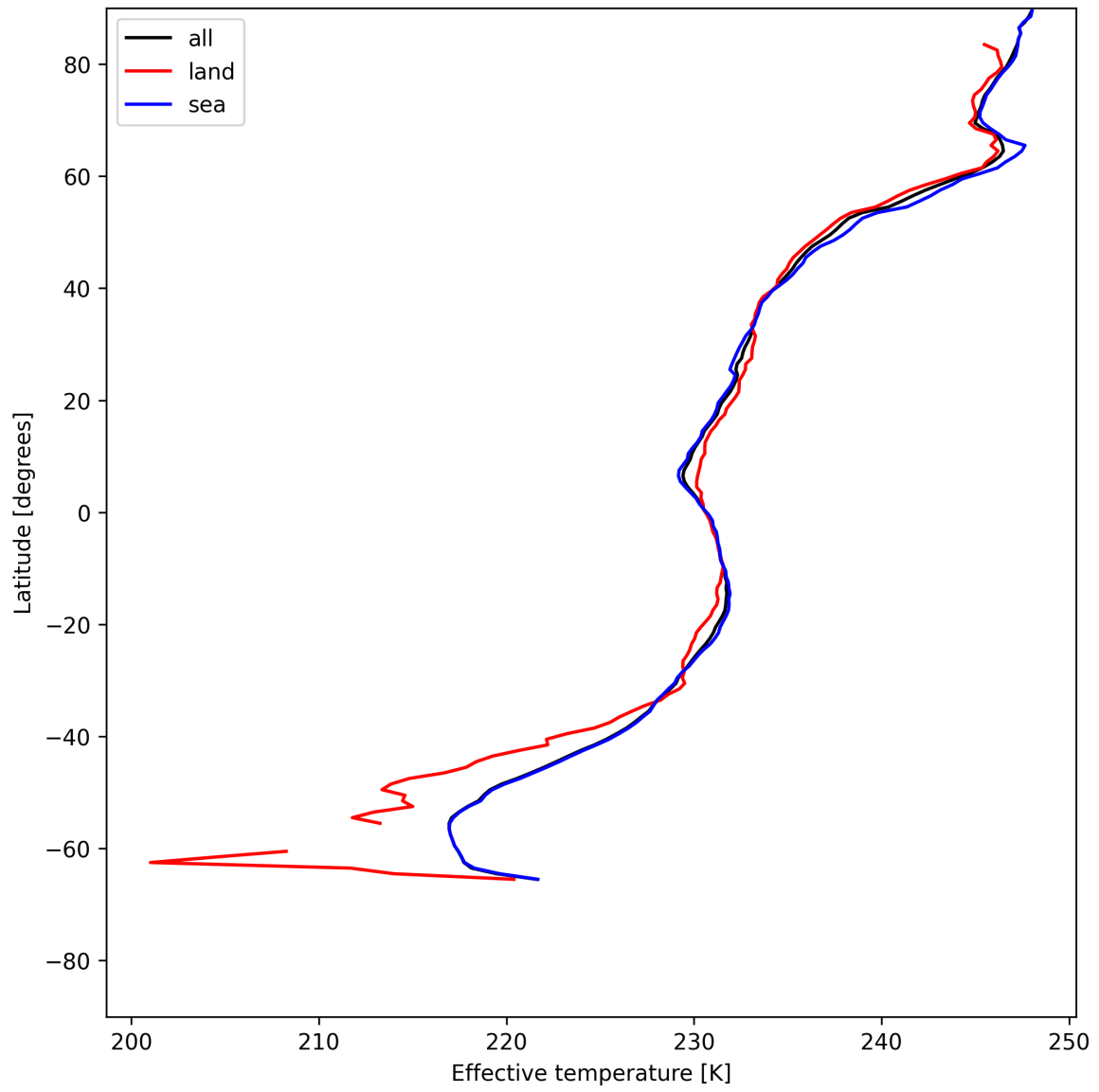
Figure 26: Zonal average of "Effective temperature" for 2025-06-23 to 2025-06-24.
