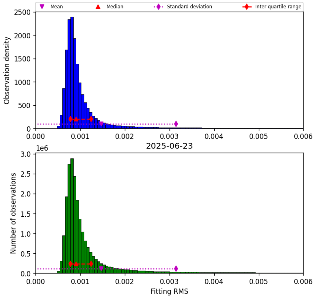
Figure 34: Histogram of “Fitting RMS” for 2025-06-23 to 2025-06-24
