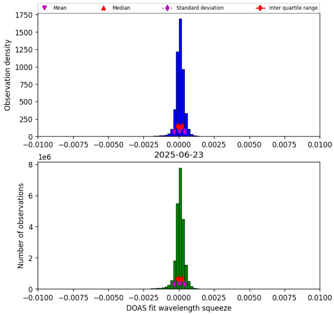
Figure 36: Histogram of “DOAS fit wavelength squeeze” for 2025-06-23 to 2025-06-24
