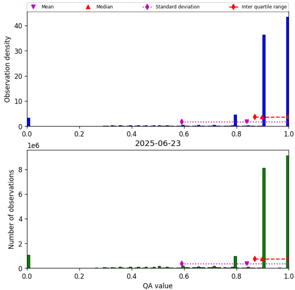
Figure 28: Histogram of “QA value” for 2025-06-23 to 2025-06-24
