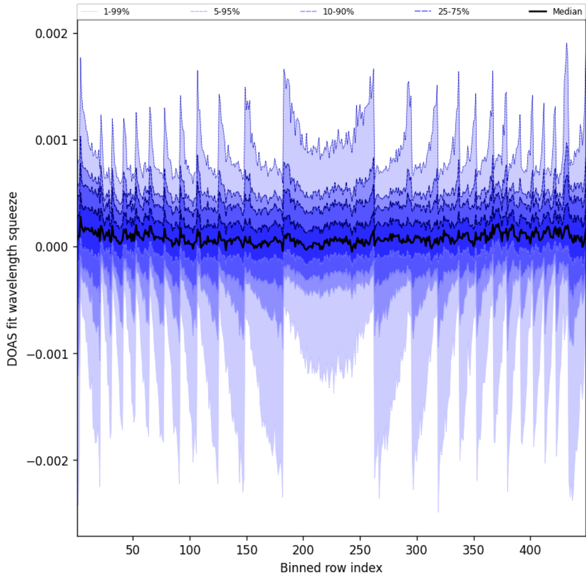
Figure 48: Along track statistics of “DOAS fit wavelength squeeze” for 2025-06-23 to 2025-06-24
