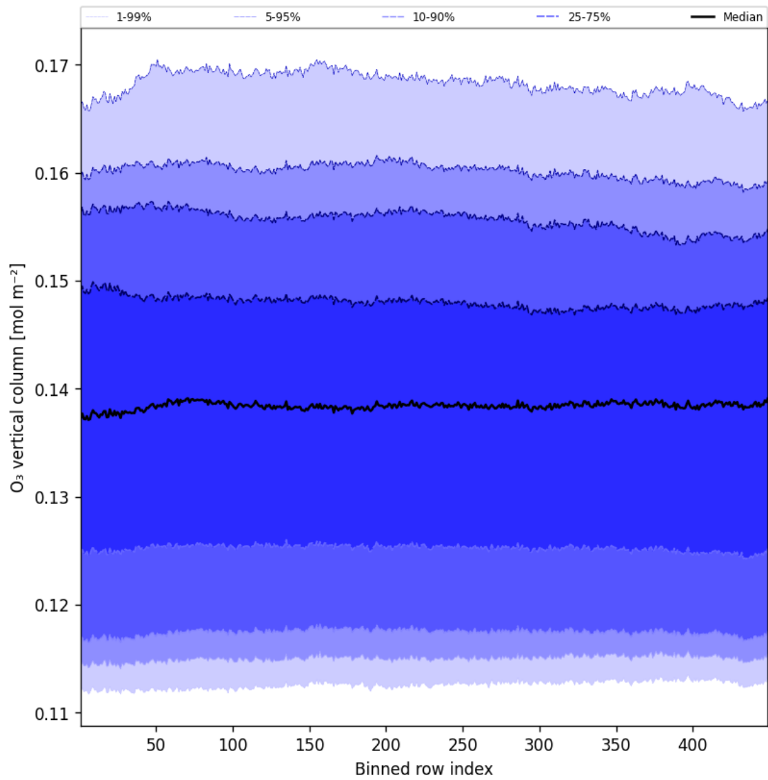
Figure 41: Along track statistics of “ O_3 vertical column” for 2025-06-23 to 2025-06-24
