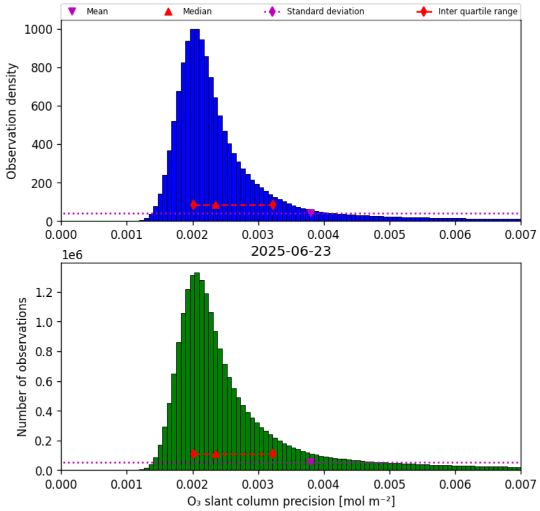
Figure 32: Histogram of "O 3 slant column precision" for 2025-06-23 to 2025-06-24
