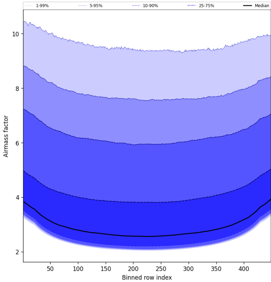
Figure 49: Along track statistics of “Airmass factor” for 2025-06-23 to 2025-06-24
