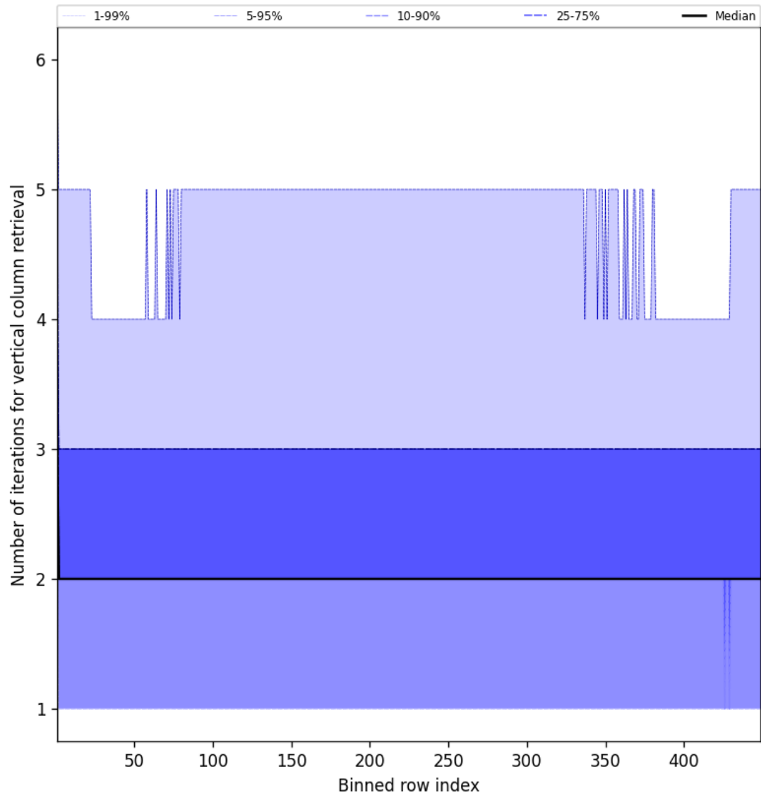
Figure 51: Along track statistics of “Number of iterations for vertical column retrieval” for 2025-06-23 to 2025-06-24
