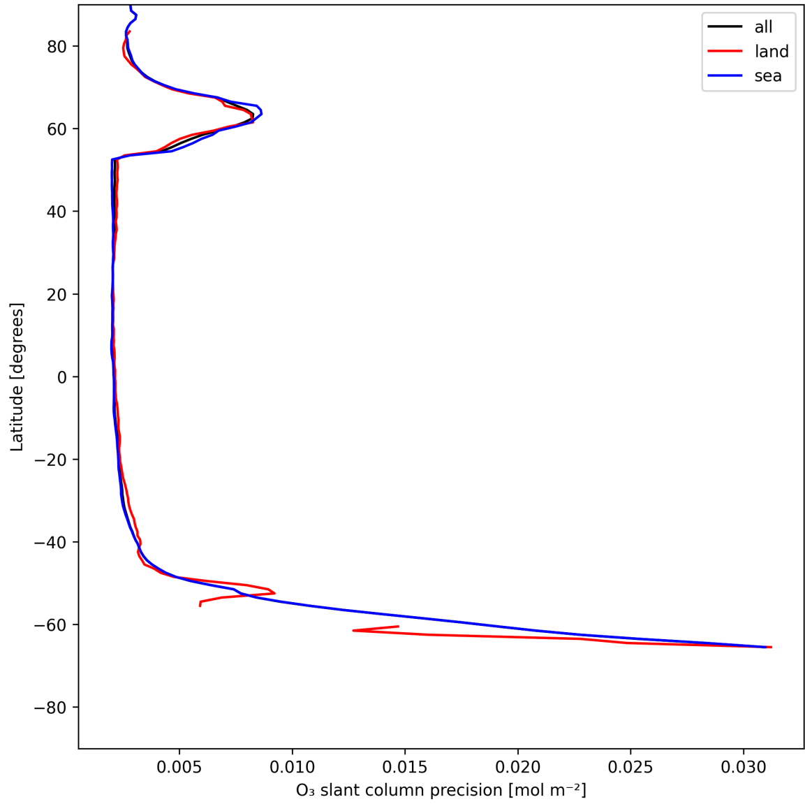
Figure 20: Zonal average of “O 3 slant column precision” for 2025-06-23 to 2025-06-24.
