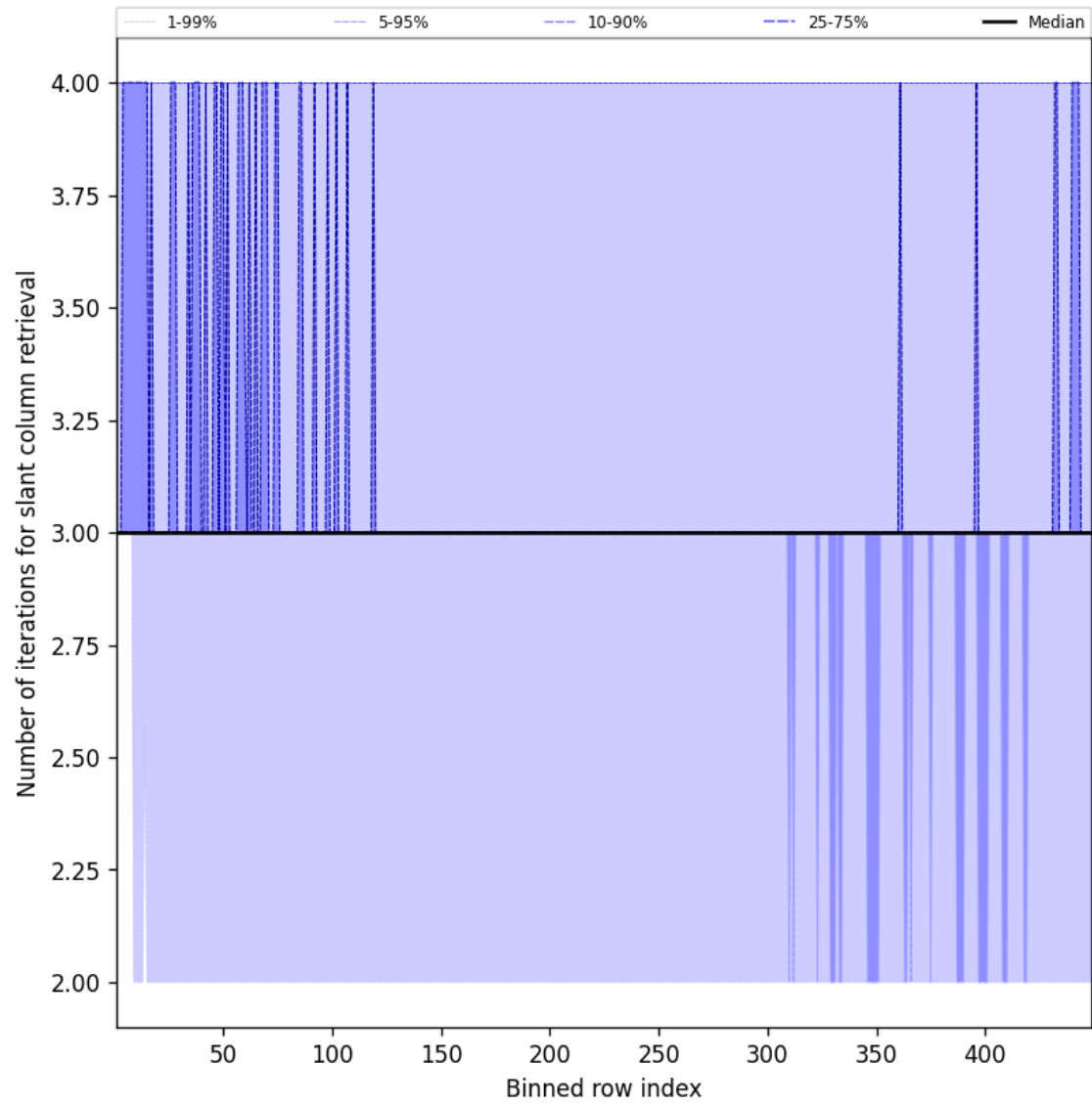
Figure 45: Along track statistics of “Number of iterations for slant column retrieval” for 2025-06-23 to 2025-06-24
