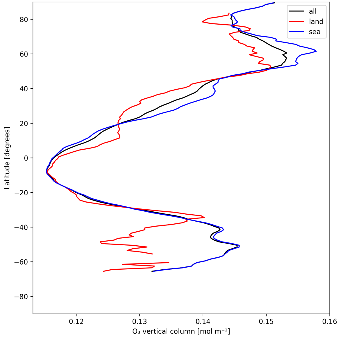
Figure 17: Zonal average of “O 3 vertical column” for 2025-06-23 to 2025-06-24.
