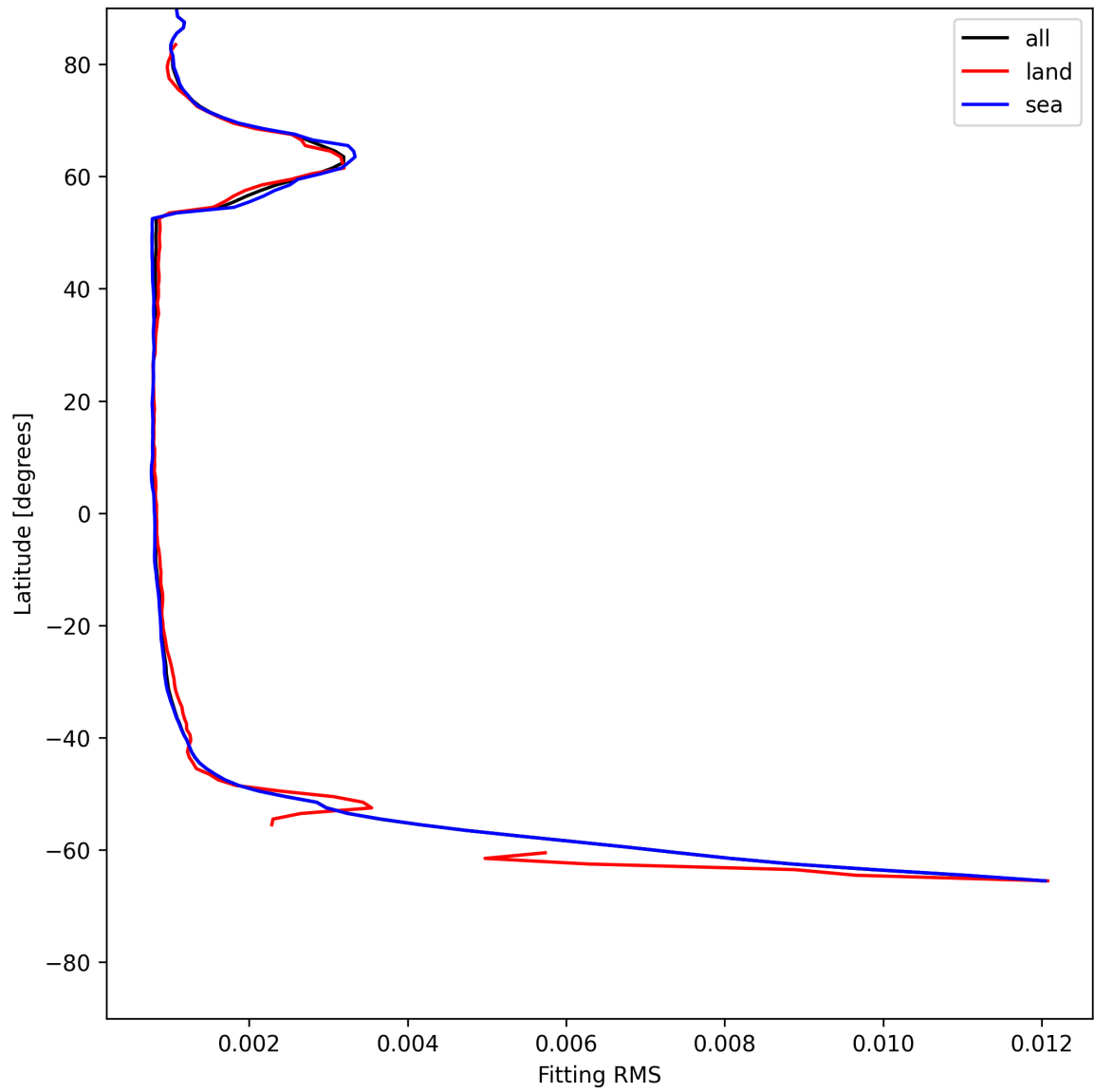
Figure 22: Zonal average of “Fitting RMS” for 2025-06-23 to 2025-06-24.
