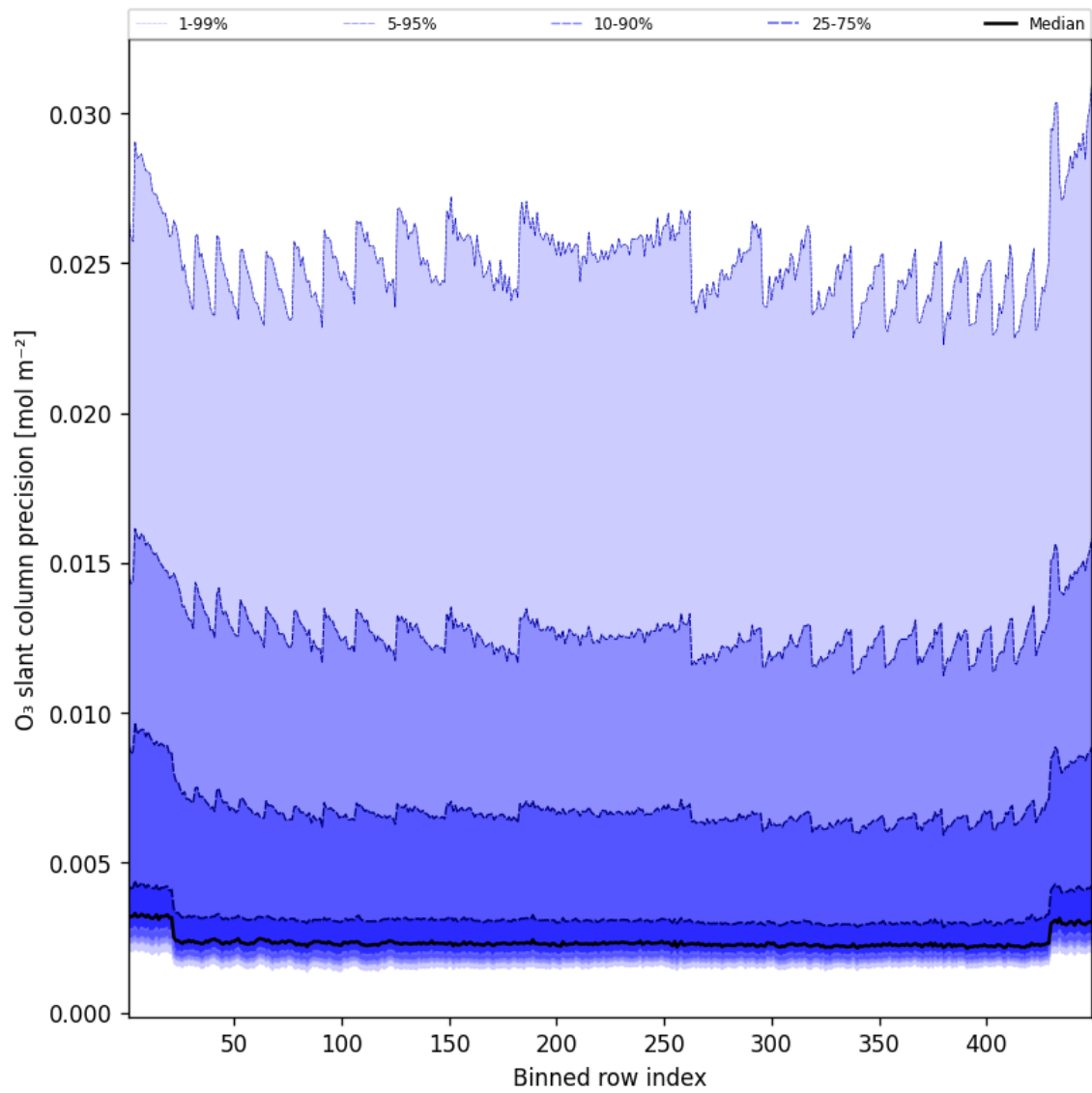
Figure 44: Along track statistics of “O 3 slant column precision” for 2025-06-23 to 2025-06-24
