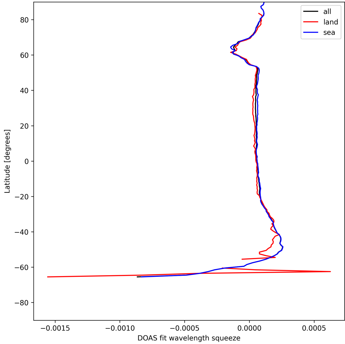
Figure 24: Zonal average of “DOAS fit wavelength squeeze” for 2025-06-23 to 2025-06-24.
