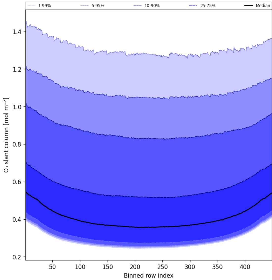
Figure 43: Along track statistics of “O 3 slant column” for 2025-06-23 to 2025-06-24
