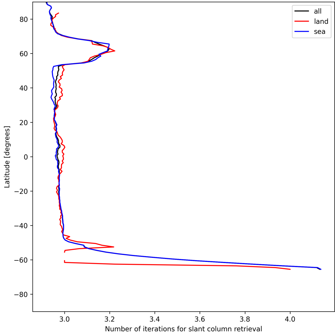
Figure 21: Zonal average of “Number of iterations for slant column retrieval” for 2025-06-23 to 2025-06-24.
