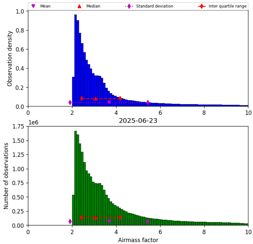
Figure 37: Histogram of “Airmass factor” for 2025-06-23 to 2025-06-24
