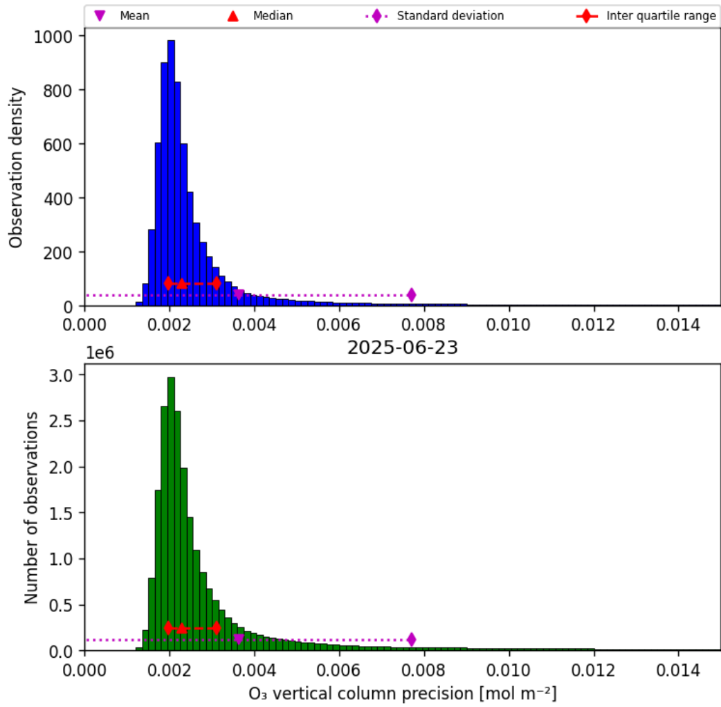
Figure 30: Histogram of “O 3 vertical column precision” for 2025-06-23 to 2025-06-24
