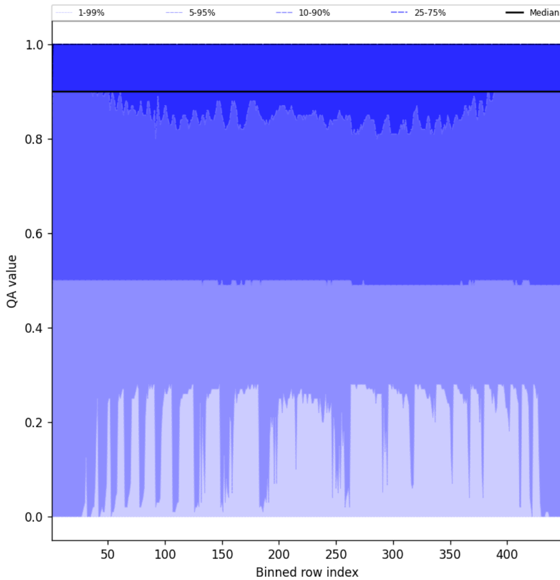
Figure 40: Along track statistics of “QA value” for 2025-06-23 to 2025-06-24
