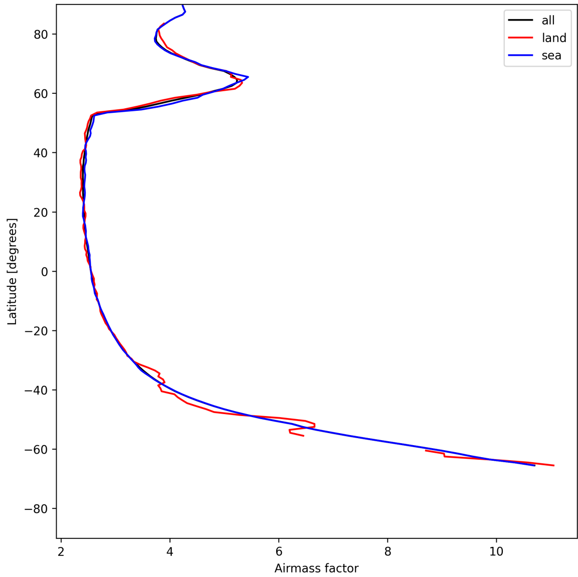
Figure 25: Zonal average of “Airmass factor” for 2025-06-23 to 2025-06-24.
