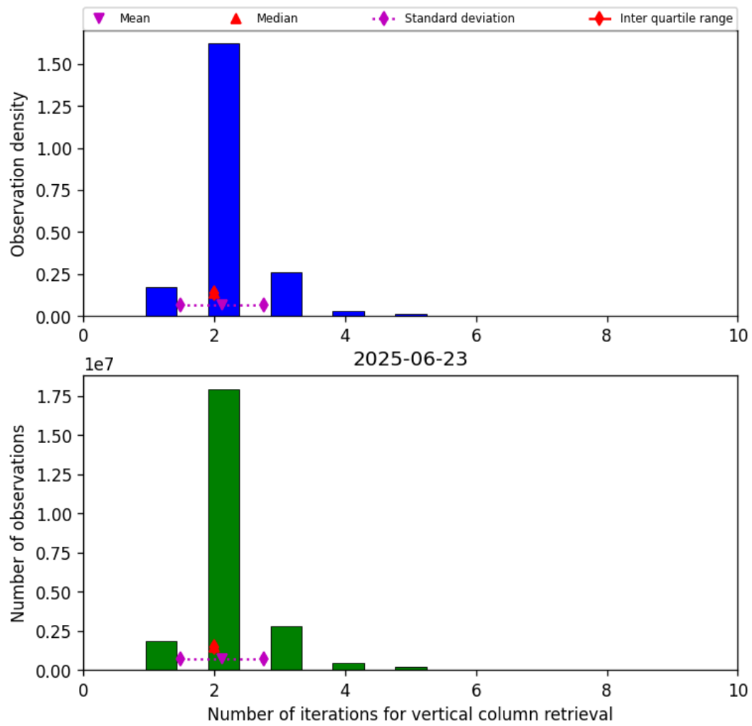
Figure 39: Histogram of “Number of iterations for vertical column retrieval” for 2025-06-23 to 2025-06-24
