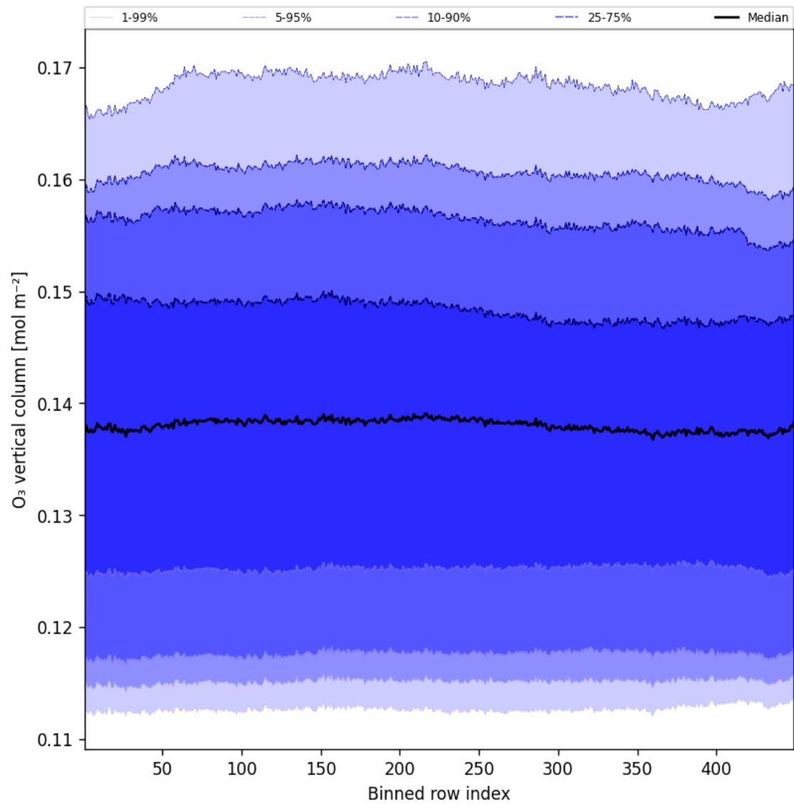
Figure 41: Along track statistics of “ O_3 vertical column” for 2025-06-24 to 2025-06-25
