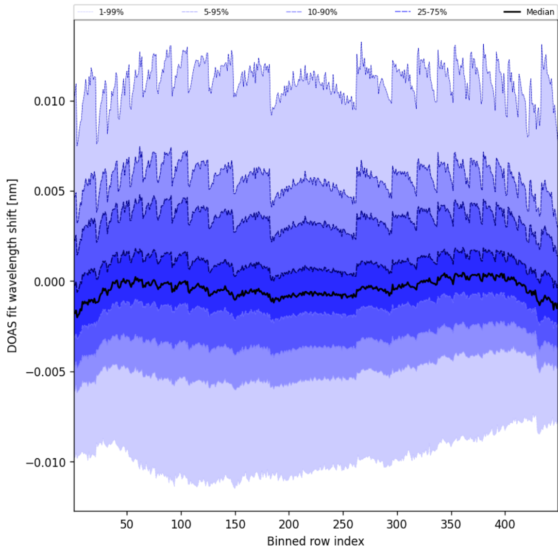
Figure 47: Along track statistics of “DOAS fit wavelength shift” for 2025-06-24 to 2025-06-25
