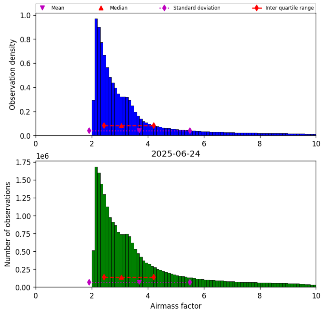
Figure 37: Histogram of “Airmass factor” for 2025-06-24 to 2025-06-25
