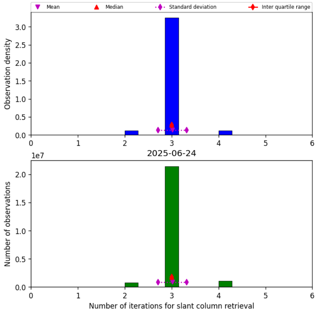
Figure 33: Histogram of “Number of iterations for slant column retrieval” for 2025-06-24 to 2025-06-25
