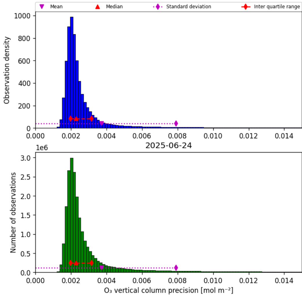
Figure 30: Histogram of “O 3 vertical column precision” for 2025-06-24 to 2025-06-25
