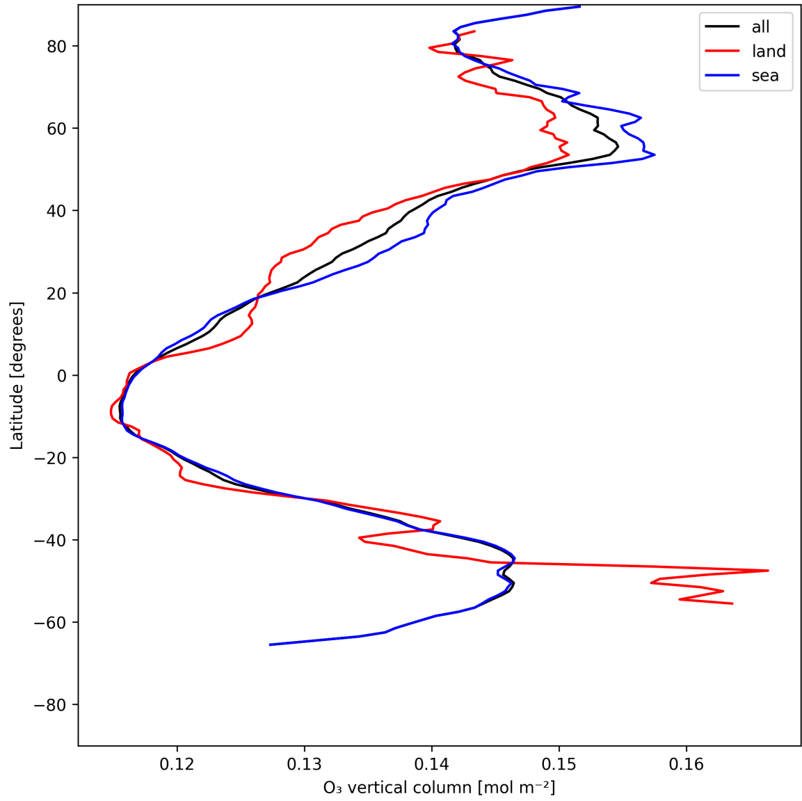
Figure 17: Zonal average of “O 3 vertical column” for 2025-06-24 to 2025-06-25.
