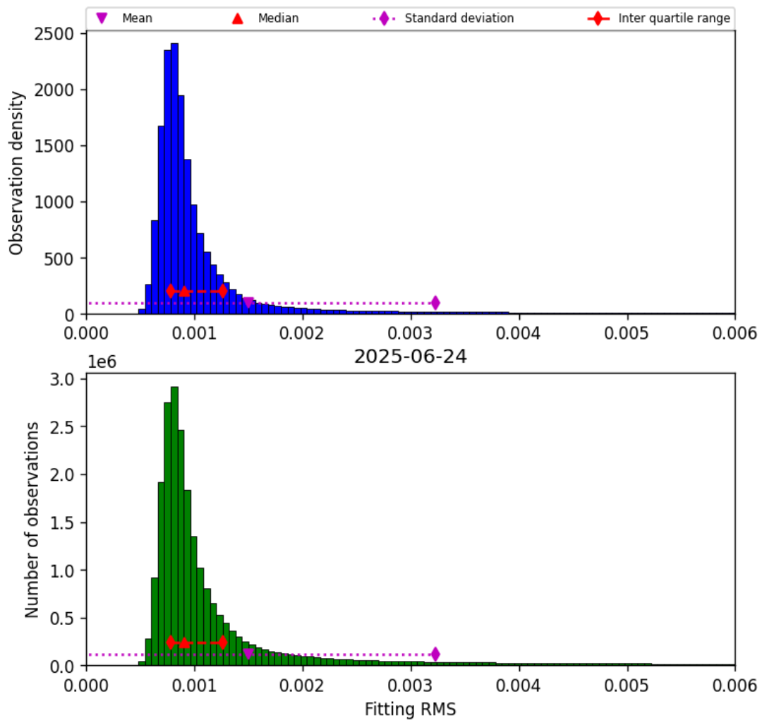
Figure 34: Histogram of “Fitting RMS” for 2025-06-24 to 2025-06-25
