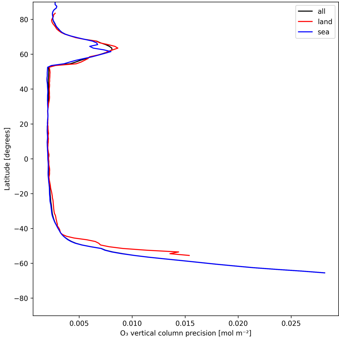
Figure 18: Zonal average of “O 3 vertical column precision” for 2025-06-24 to 2025-06-25.
