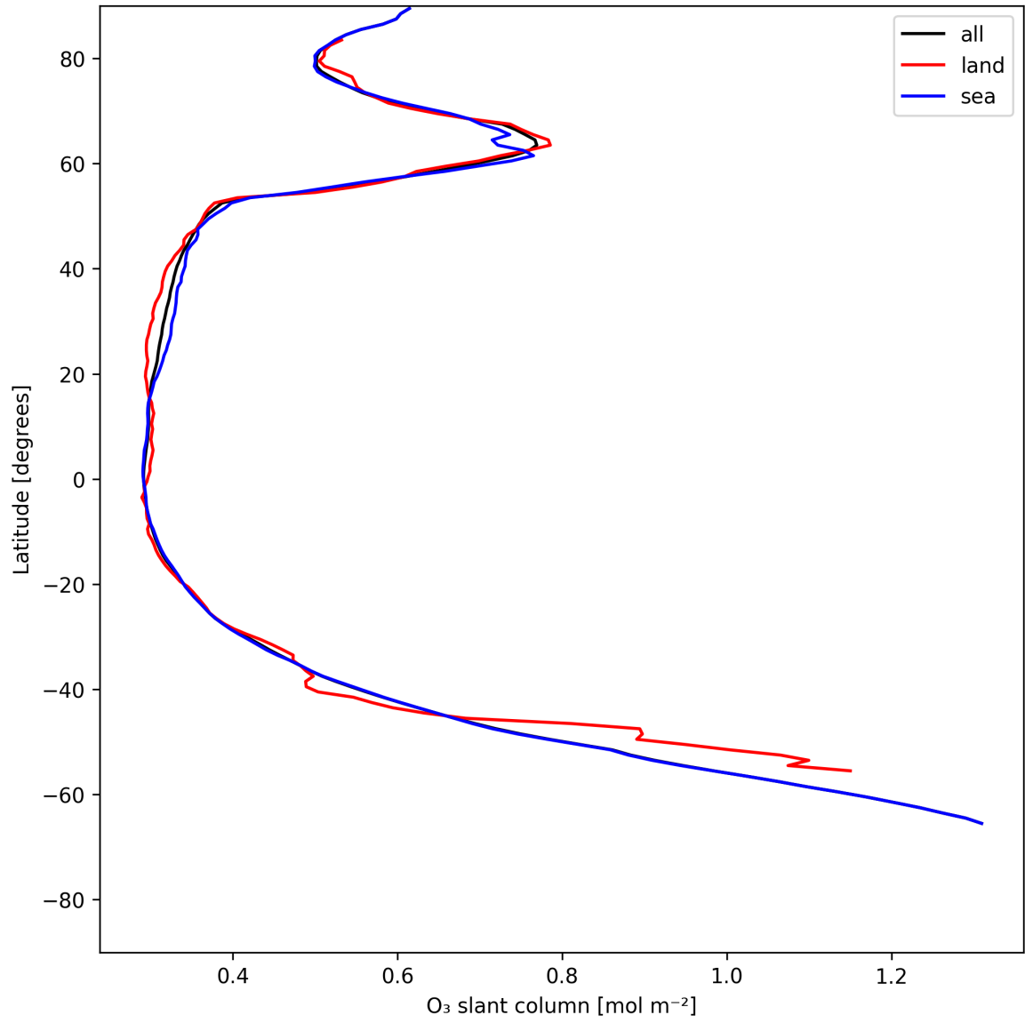
Figure 19: Zonal average of “O 3 slant column” for 2025-06-24 to 2025-06-25.
