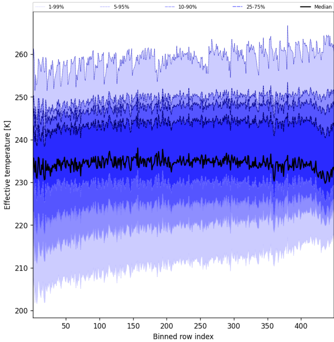
Figure 50: Along track statistics of “Effective temperature” for 2025-06-24 to 2025-06-25
