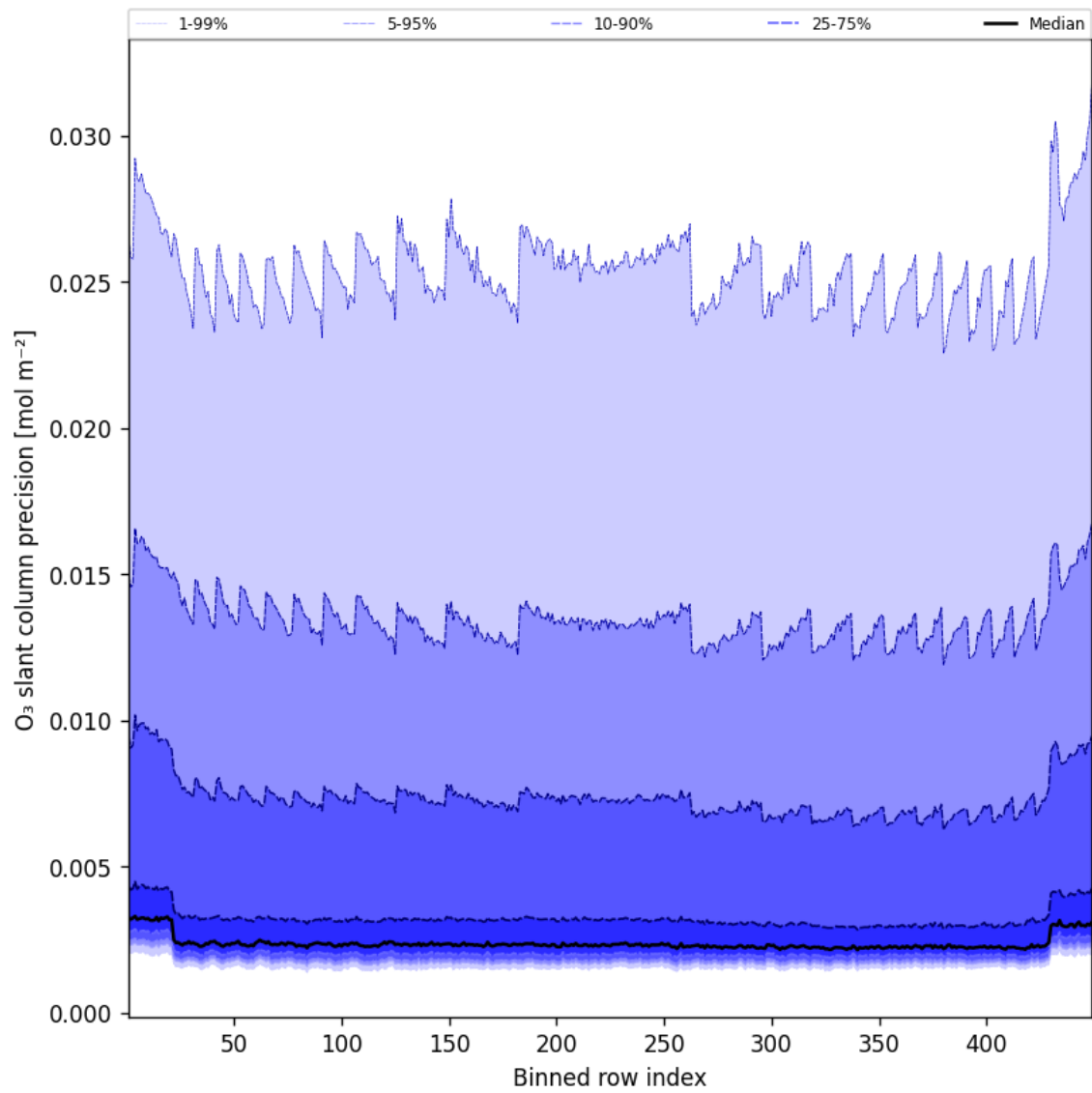
Figure 44: Along track statistics of “O 3 slant column precision” for 2025-06-24 to 2025-06-25
