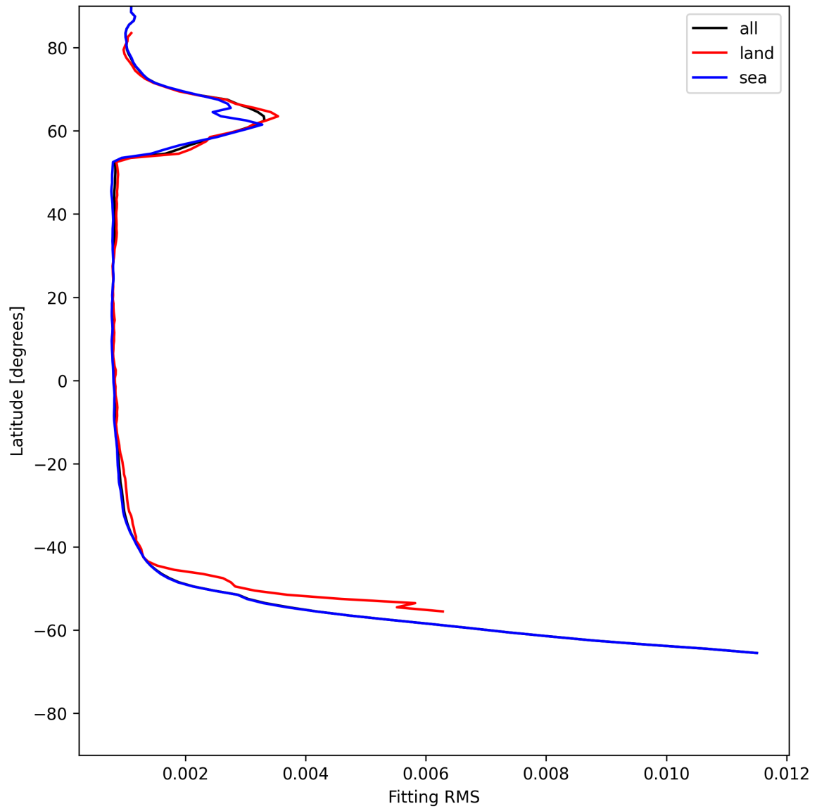
Figure 22: Zonal average of “Fitting RMS” for 2025-06-24 to 2025-06-25.
