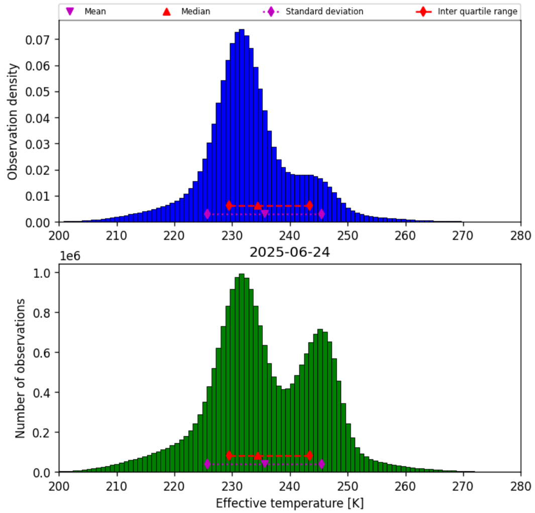
Figure 38: Histogram of “Effective temperature” for 2025-06-24 to 2025-06-25
