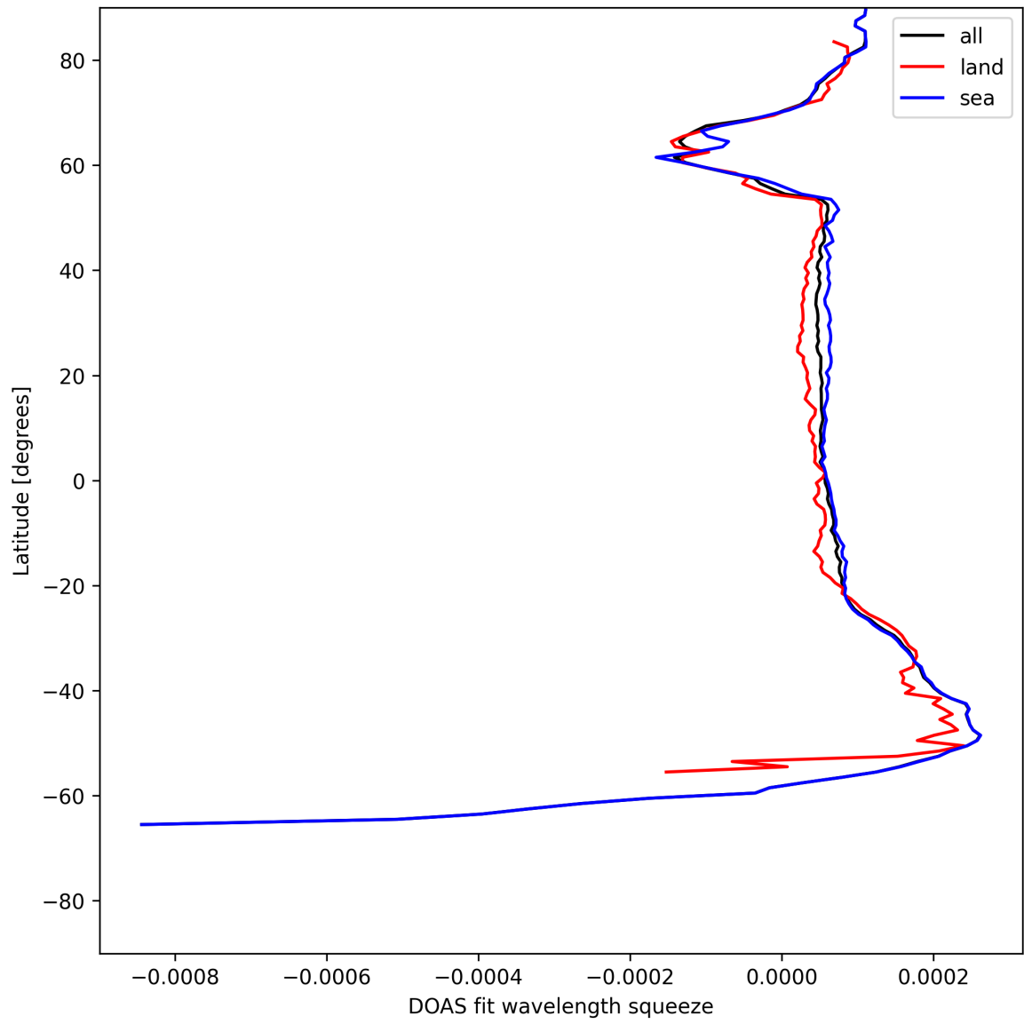
Figure 24: Zonal average of “DOAS fit wavelength squeeze” for 2025-06-24 to 2025-06-25.
