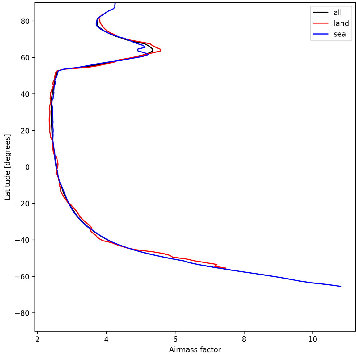
Figure 25: Zonal average of “Airmass factor” for 2025-06-24 to 2025-06-25.
