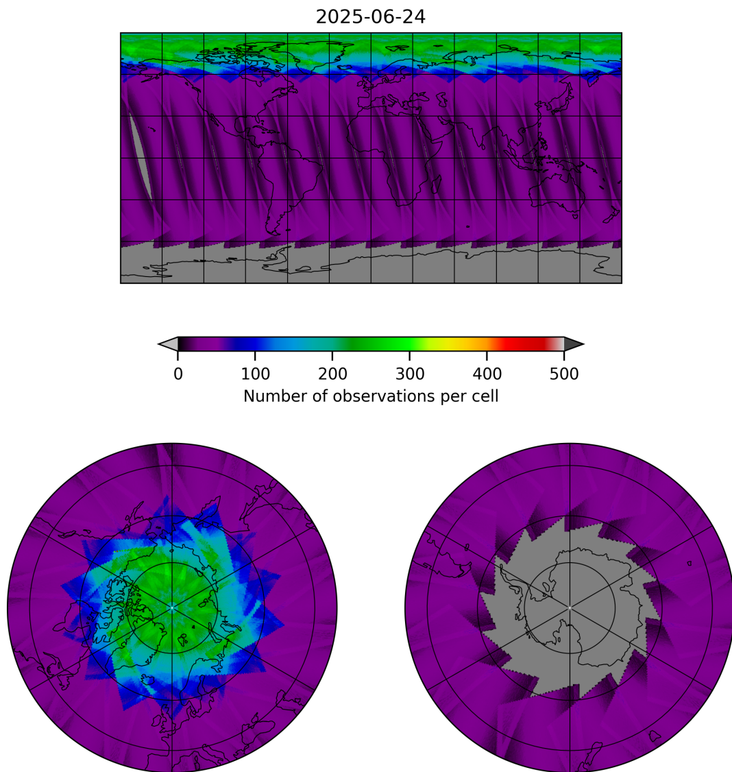
Figure 15: Map of the number of observations for 2025-06-24 to 2025-06-25
