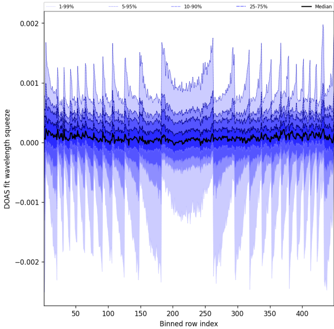
Figure 48: Along track statistics of “DOAS fit wavelength squeeze” for 2025-06-24 to 2025-06-25
