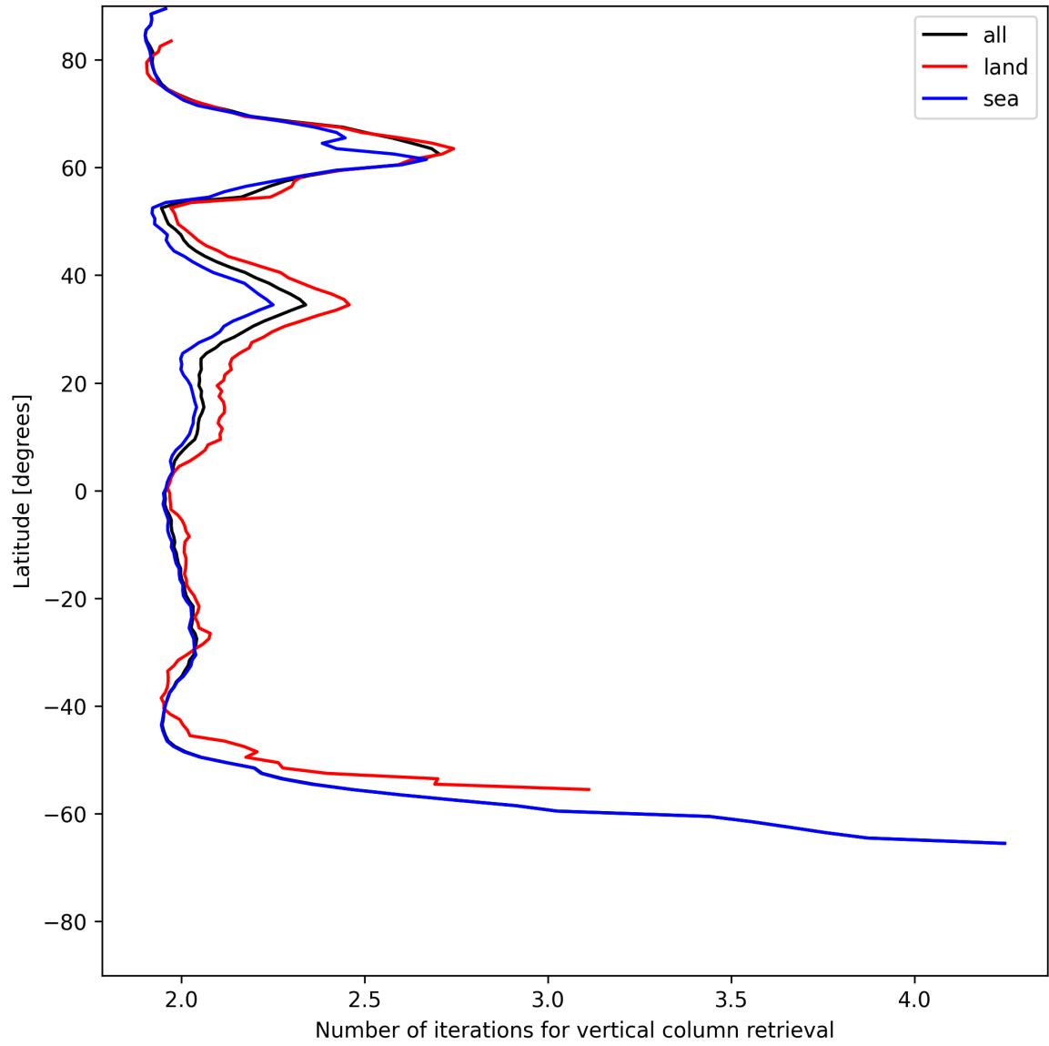
Figure 27: Zonal average of “Number of iterations for vertical column retrieval” for 2025-06-24 to 2025-06-25.
