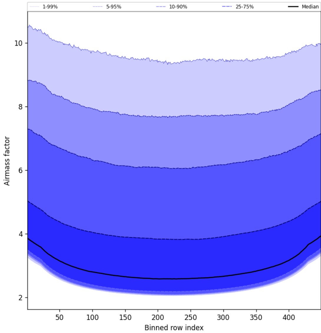
Figure 49: Along track statistics of “Airmass factor” for 2025-06-24 to 2025-06-25
