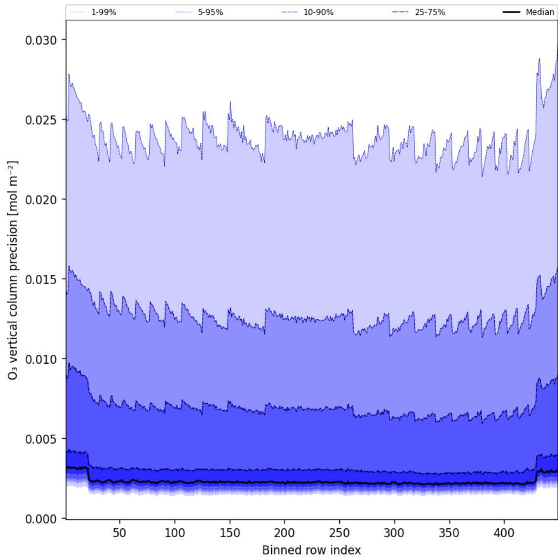
Figure 42: Along track statistics of “O 3 vertical column precision” for 2025-06-24 to 2025-06-25
