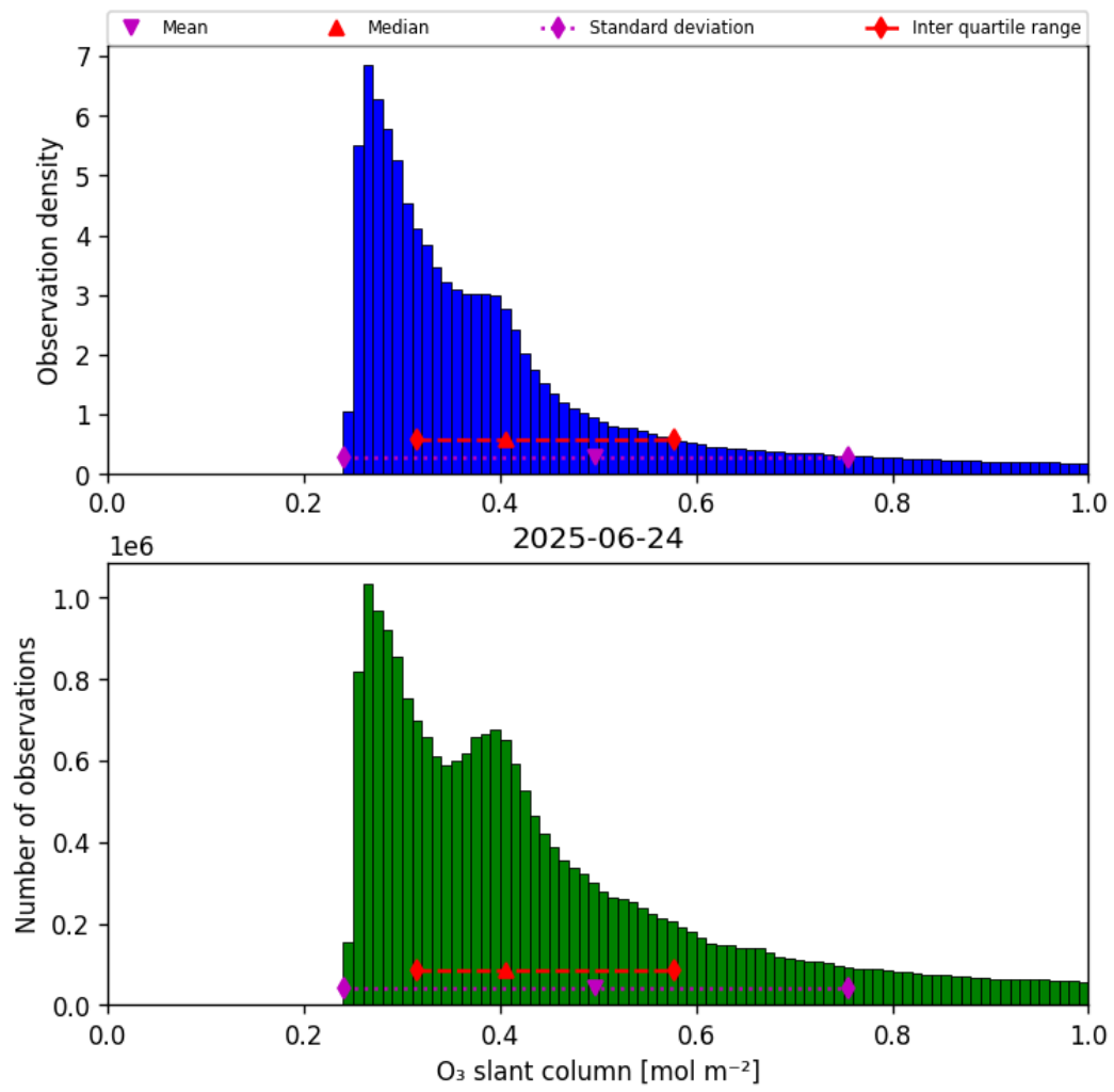
Figure 31: Histogram of “O 3 slant column” for 2025-06-24 to 2025-06-25
