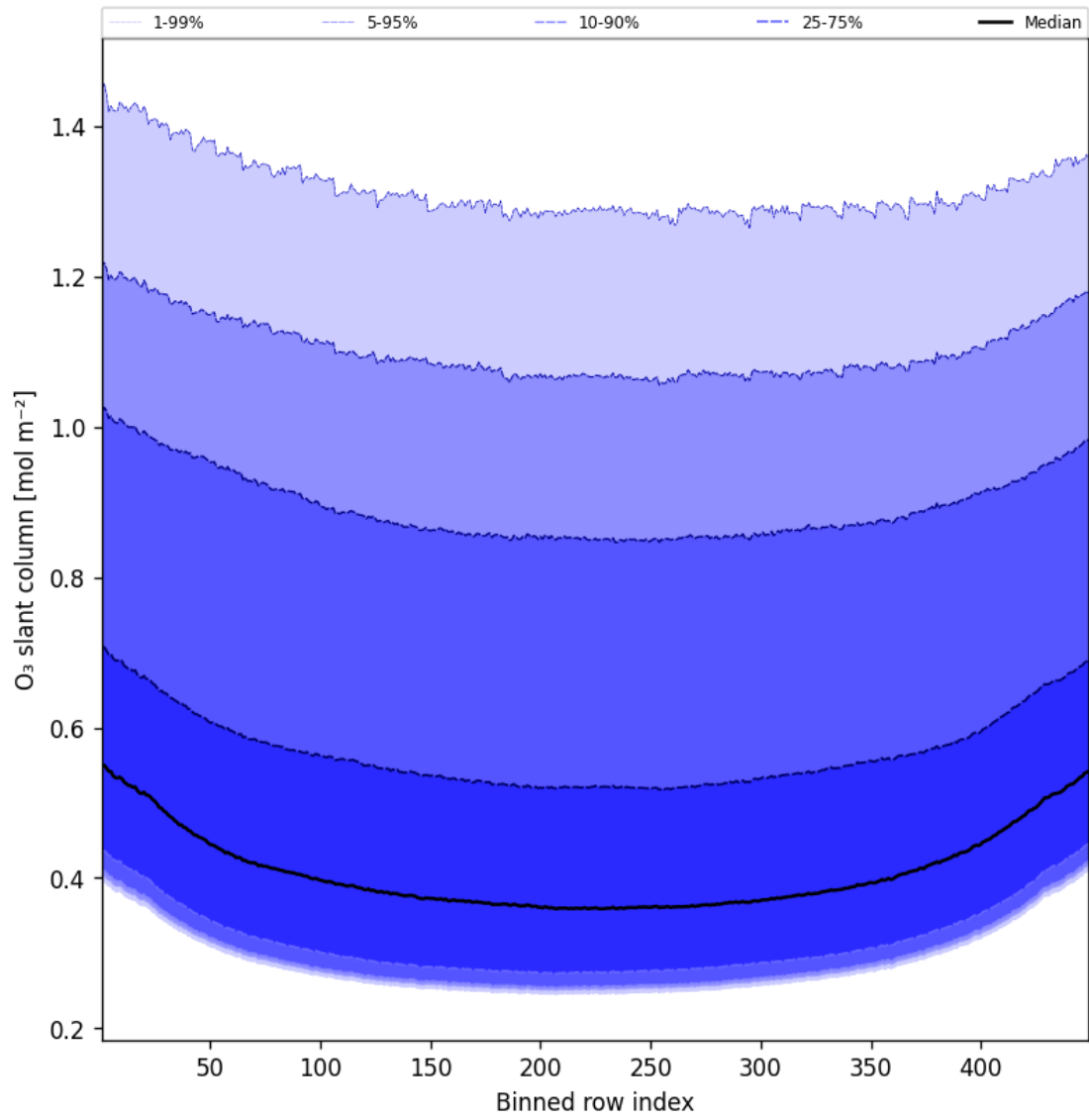
Figure 43: Along track statistics of “O 3 slant column” for 2025-06-24 to 2025-06-25
