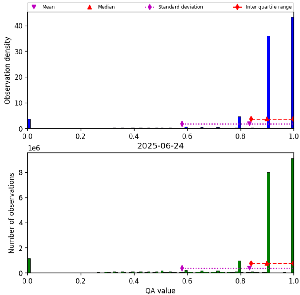
Figure 28: Histogram of “QA value” for 2025-06-24 to 2025-06-25
