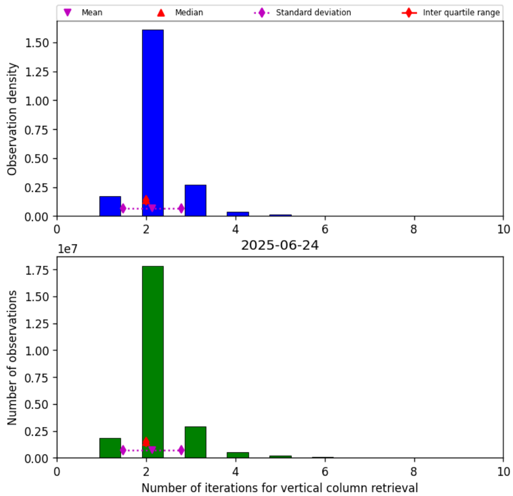
Figure 39: Histogram of “Number of iterations for vertical column retrieval” for 2025-06-24 to 2025-06-25
