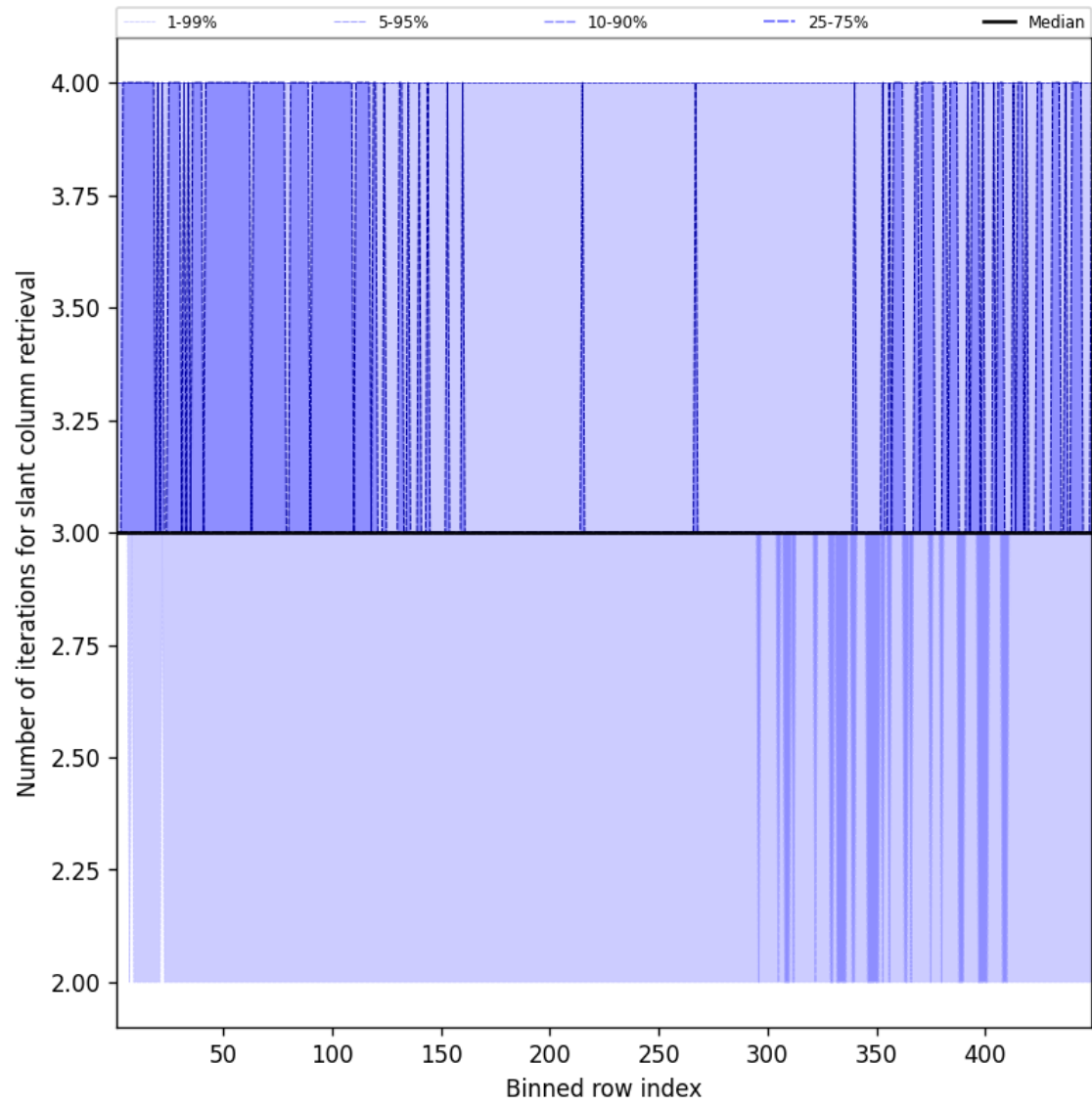
Figure 45: Along track statistics of “Number of iterations for slant column retrieval” for 2025-06-24 to 2025-06-25
