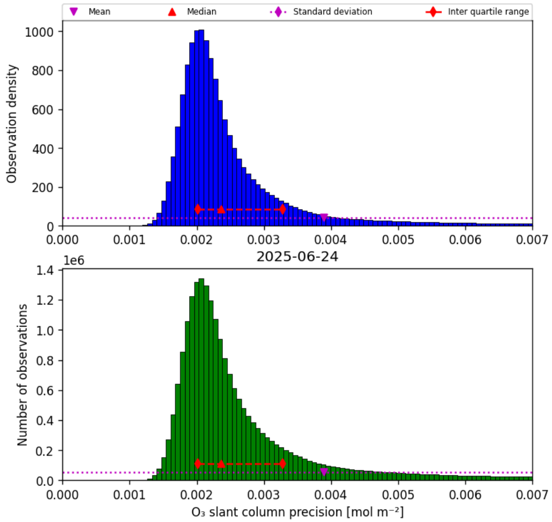
Figure 32: Histogram of “O 3 slant column precision” for 2025-06-24 to 2025-06-25
