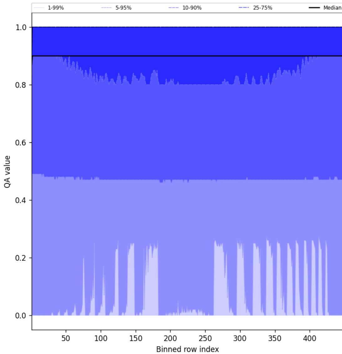
Figure 40: Along track statistics of “QA value” for 2025-06-24 to 2025-06-25
