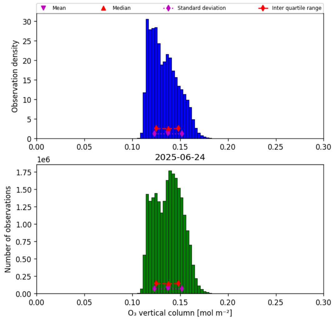
Figure 29: Histogram of “O 3 vertical column” for 2025-06-24 to 2025-06-25
