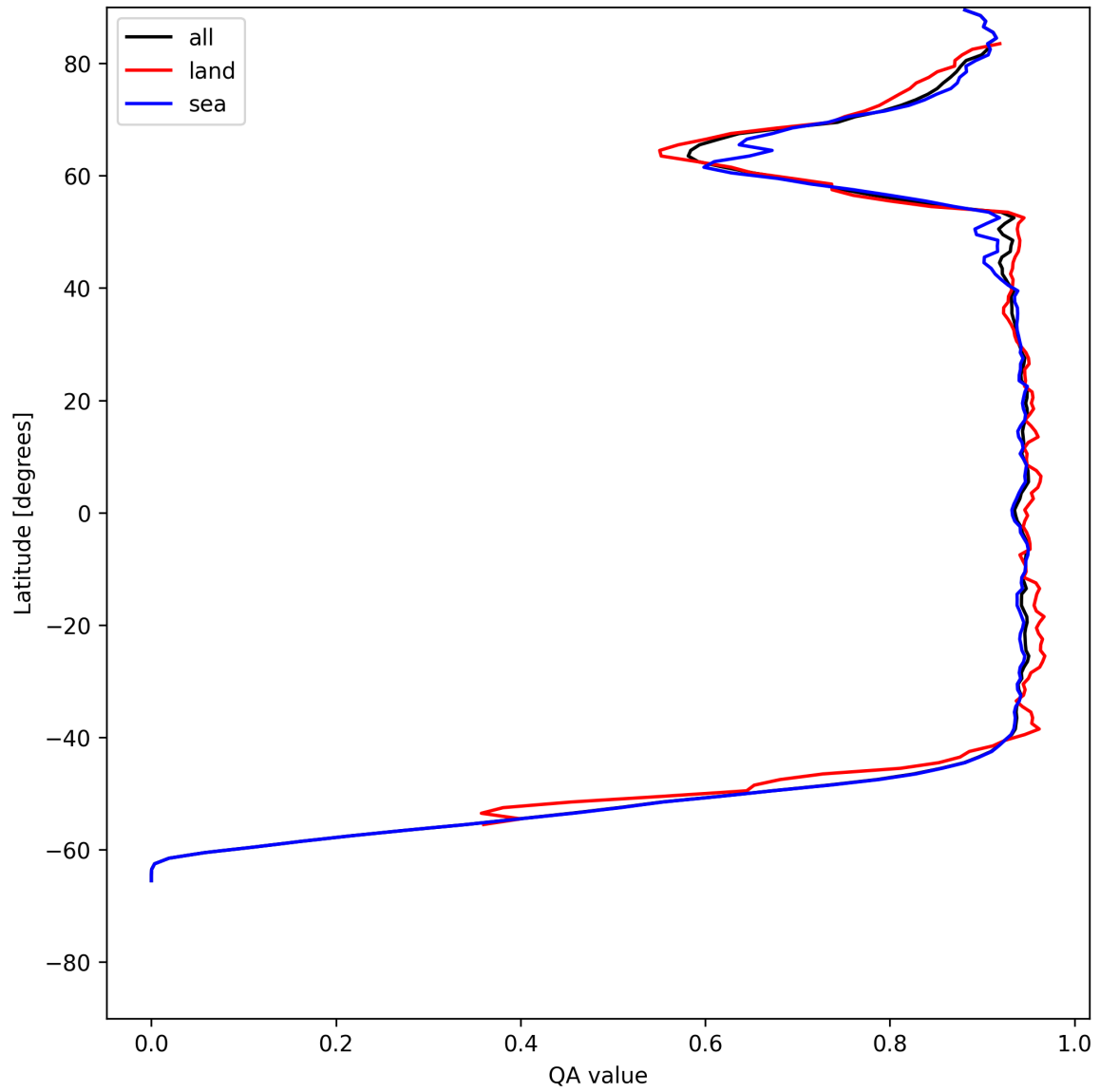
Figure 16: Zonal average of “QA value” for 2025-06-24 to 2025-06-25.
