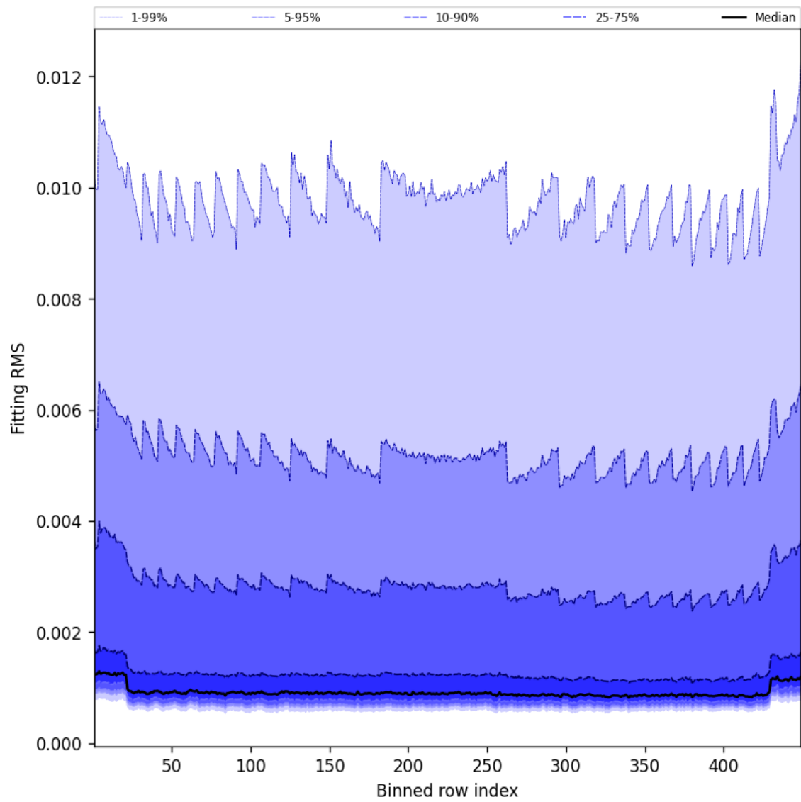
Figure 46: Along track statistics of “Fitting RMS” for 2025-06-24 to 2025-06-25
