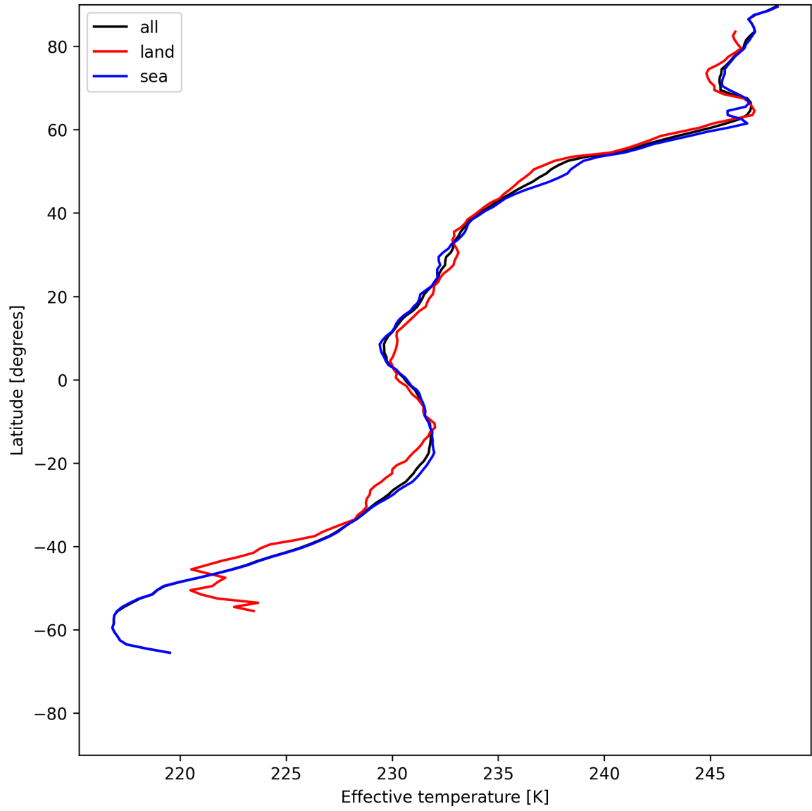
Figure 26: Zonal average of "Effective temperature" for 2025-06-24 to 2025-06-25.
