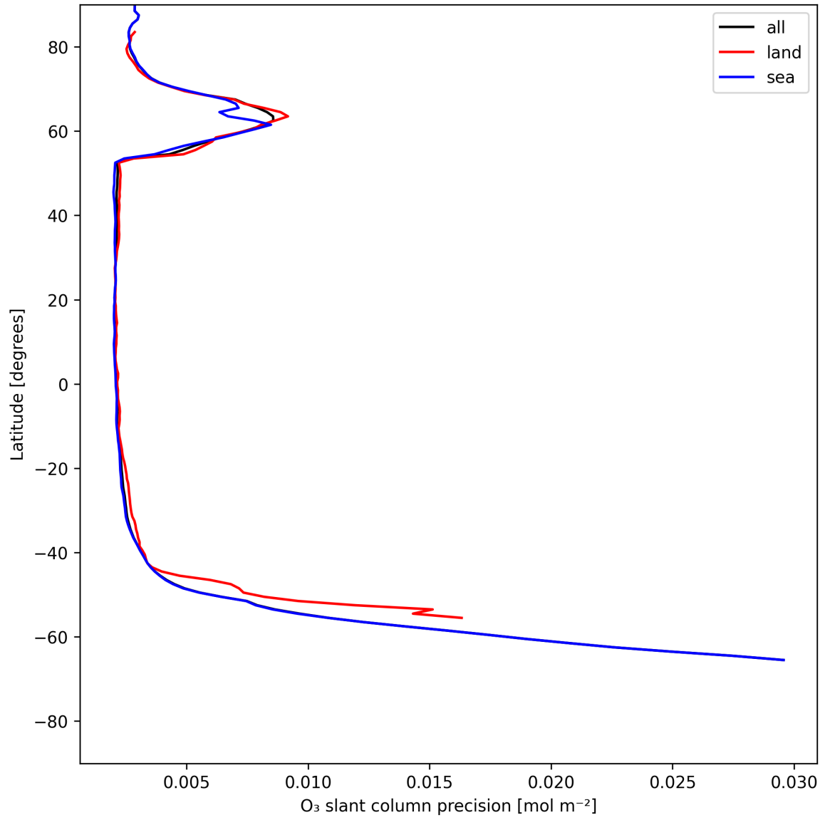
Figure 20: Zonal average of "O 3 slant column precision" for 2025-06-24 to 2025-06-25.
