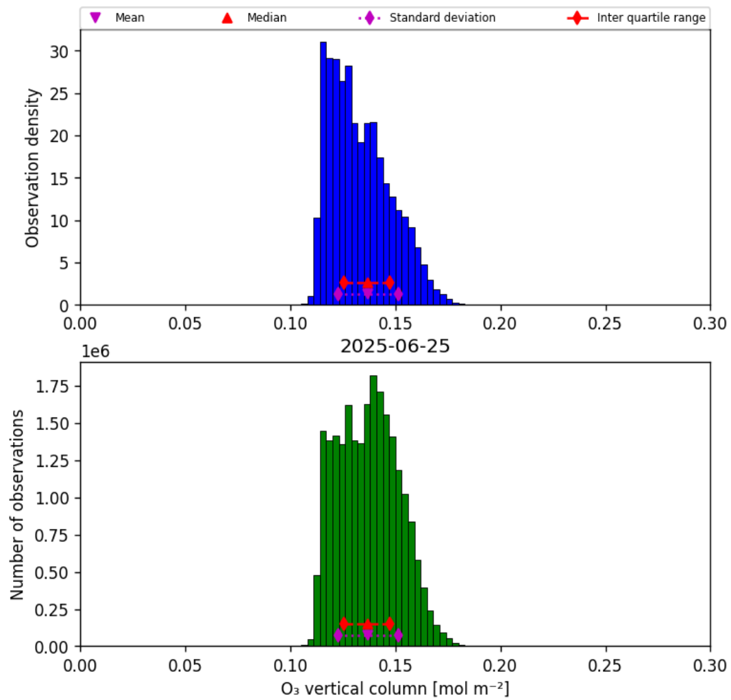
Figure 29: Histogram of “O 3 vertical column” for 2025-06-25 to 2025-06-25
