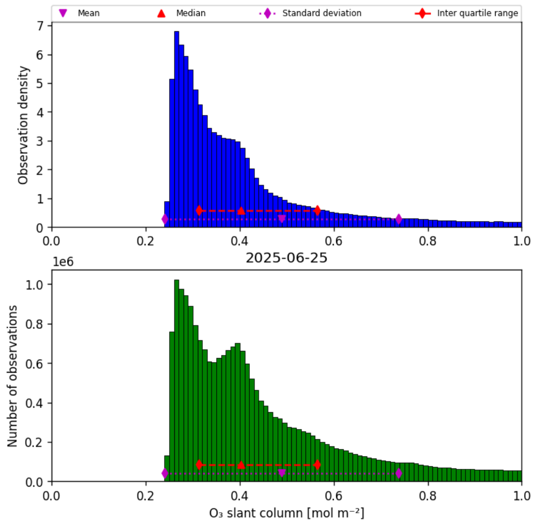
Figure 31: Histogram of “O 3 slant column” for 2025-06-25 to 2025-06-25
