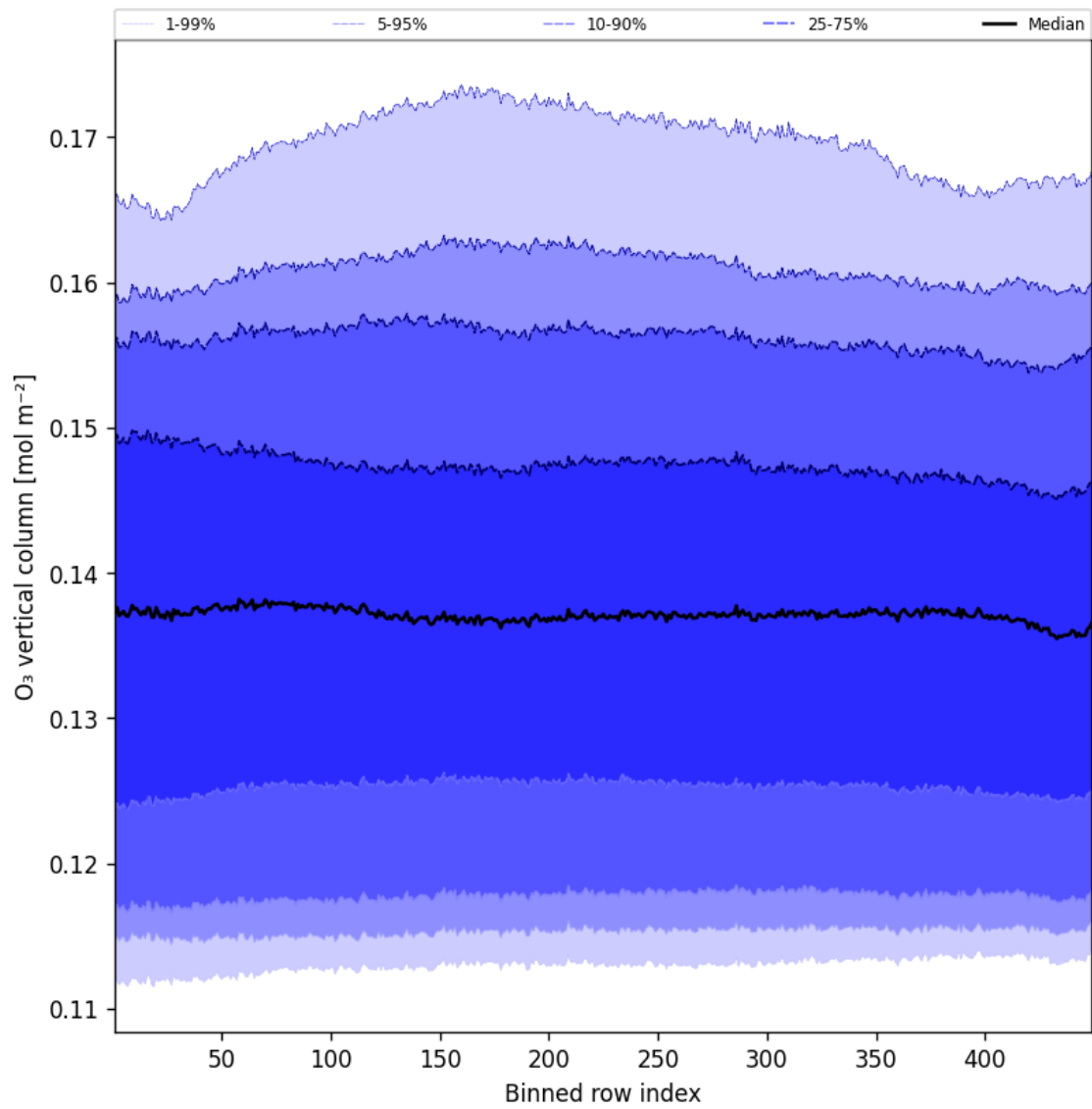
Figure 41: Along track statistics of “O 3 vertical column” for 2025-06-25 to 2025-06-25
