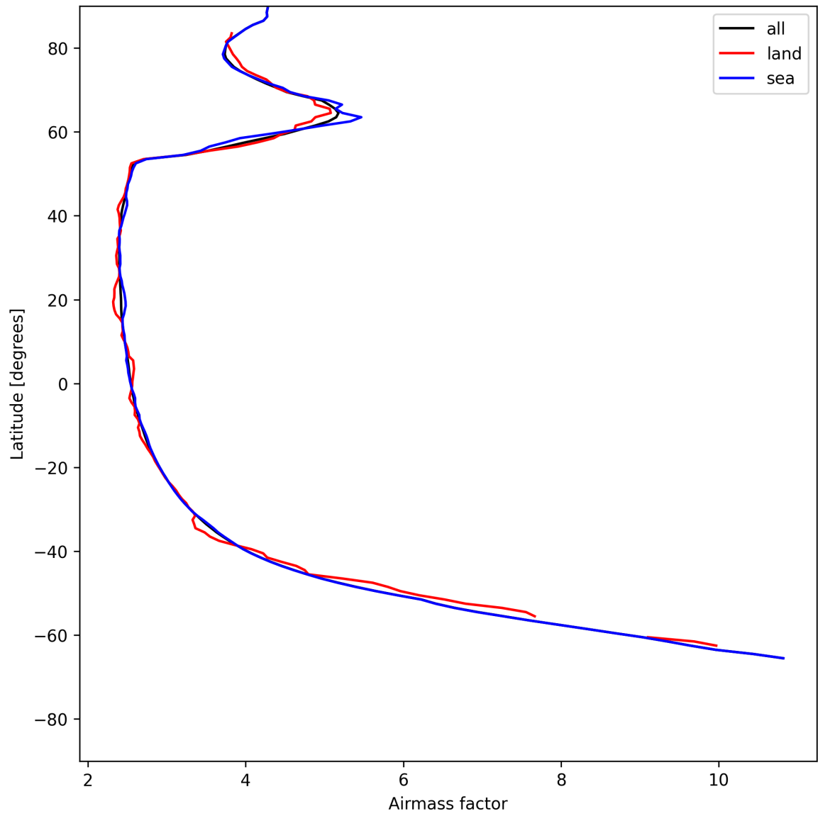
Figure 25: Zonal average of “Airmass factor” for 2025-06-25 to 2025-06-25.
