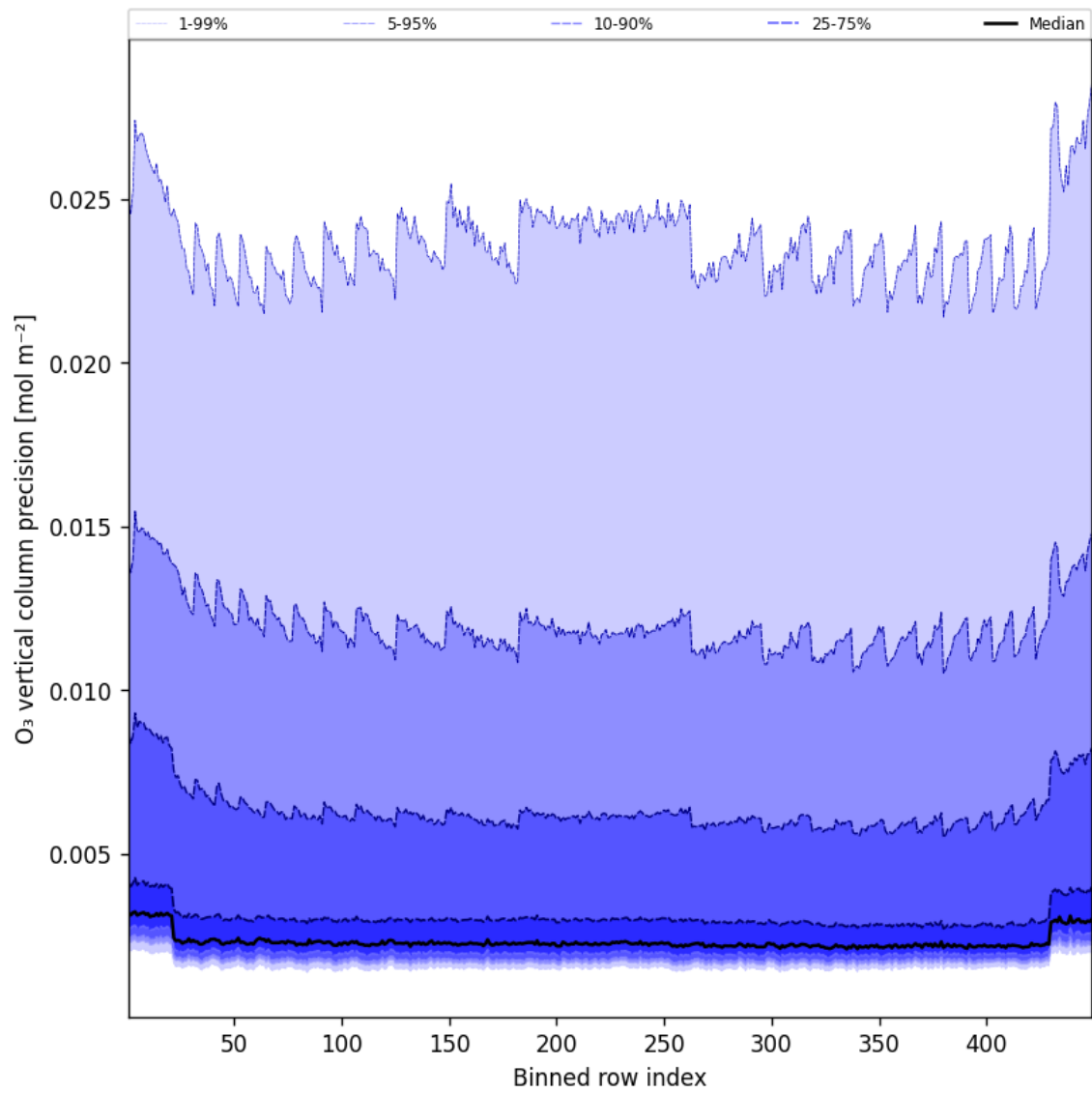
Figure 42: Along track statistics of “O 3 vertical column precision” for 2025-06-25 to 2025-06-25
