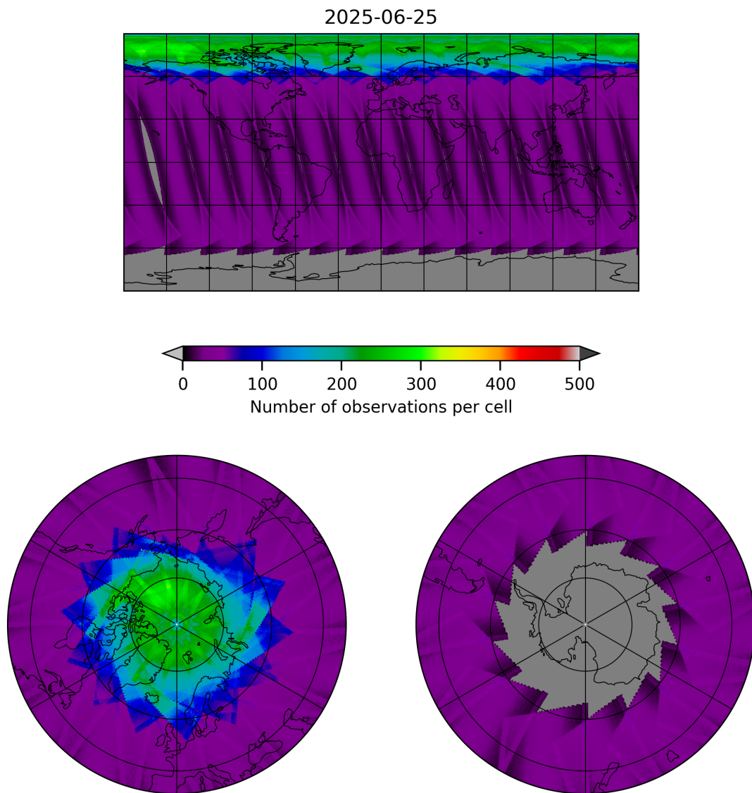
Figure 15: Map of the number of observations for 2025-06-25 to 2025-06-25
