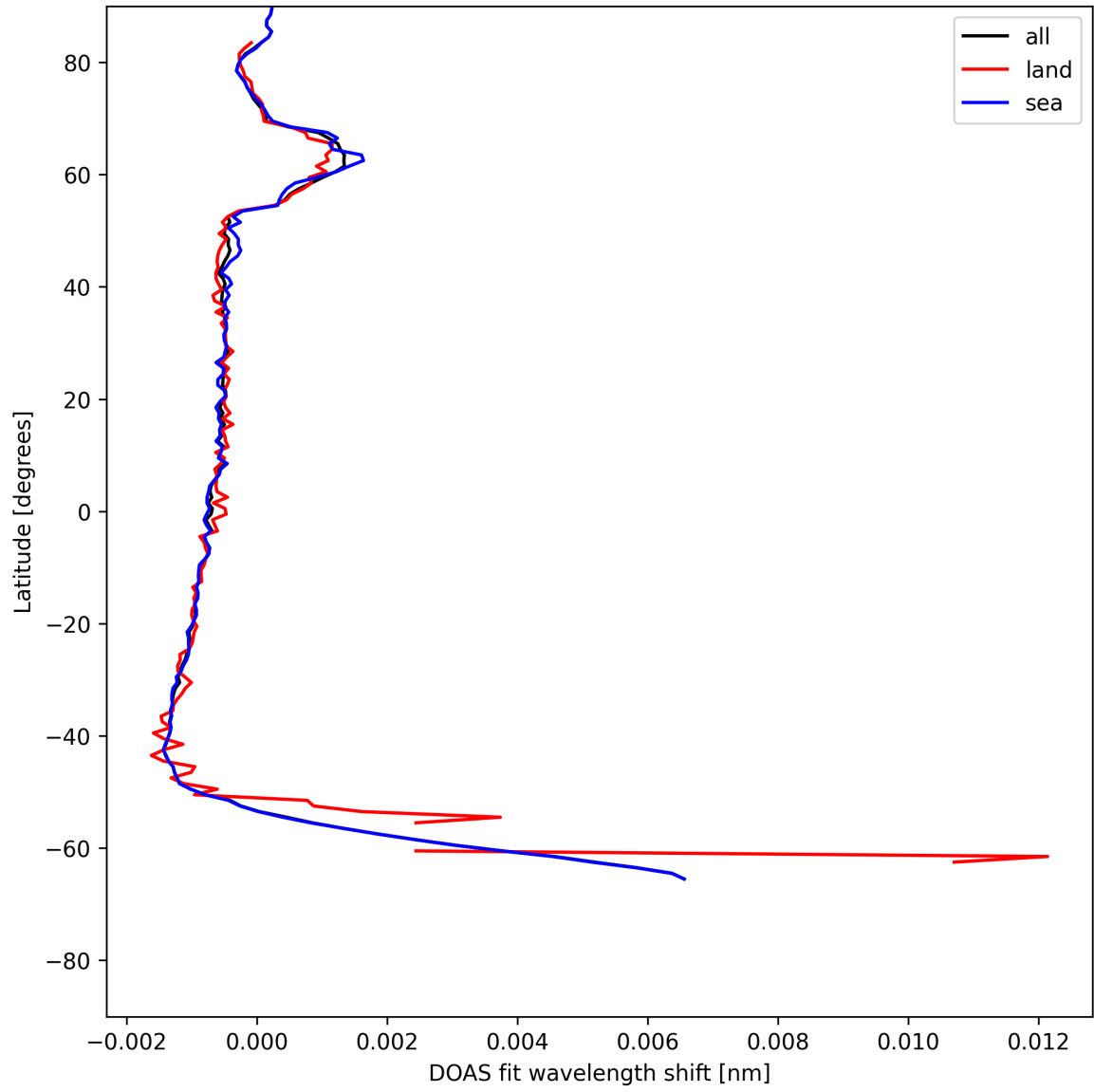
Figure 23: Zonal average of “DOAS fit wavelength shift” for 2025-06-25 to 2025-06-25.
