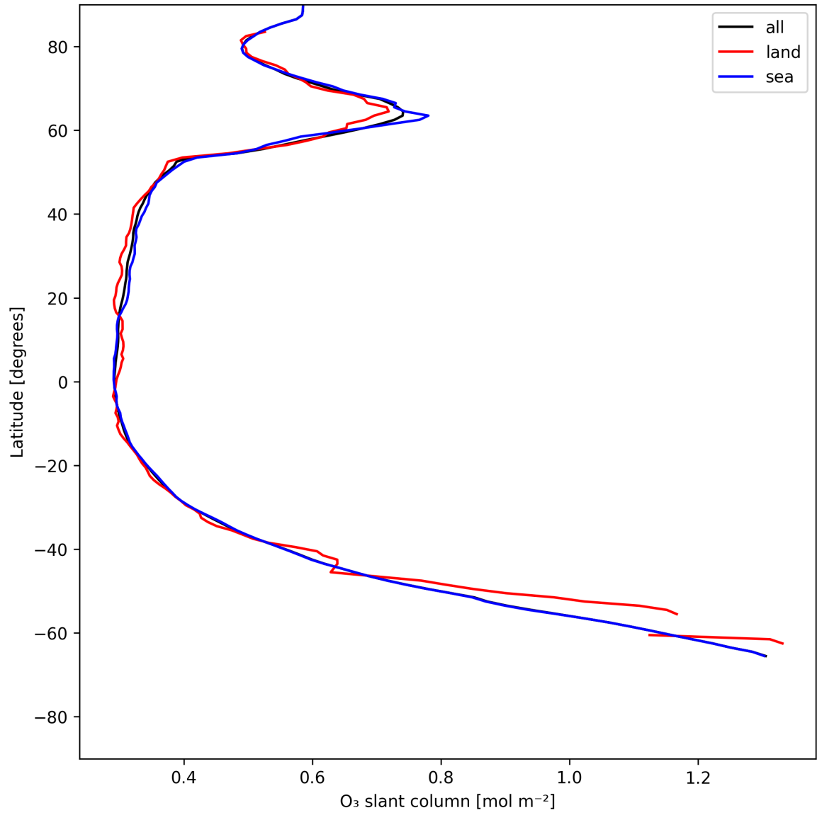
Figure 19: Zonal average of “O 3 slant column” for 2025-06-25 to 2025-06-25.
