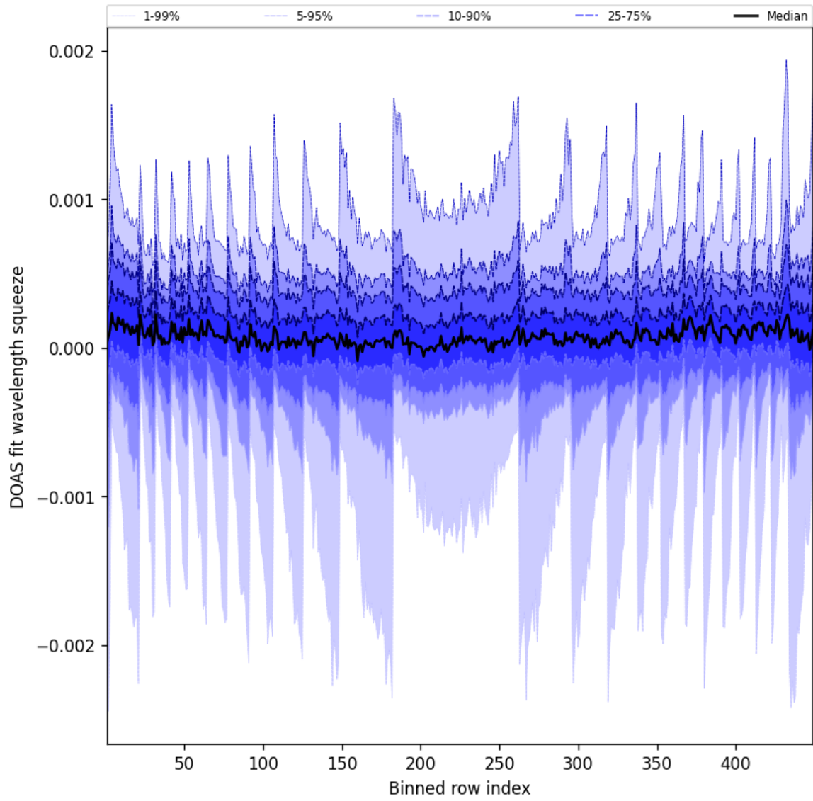
Figure 48: Along track statistics of “DOAS fit wavelength squeeze” for 2025-06-25 to 2025-06-25
