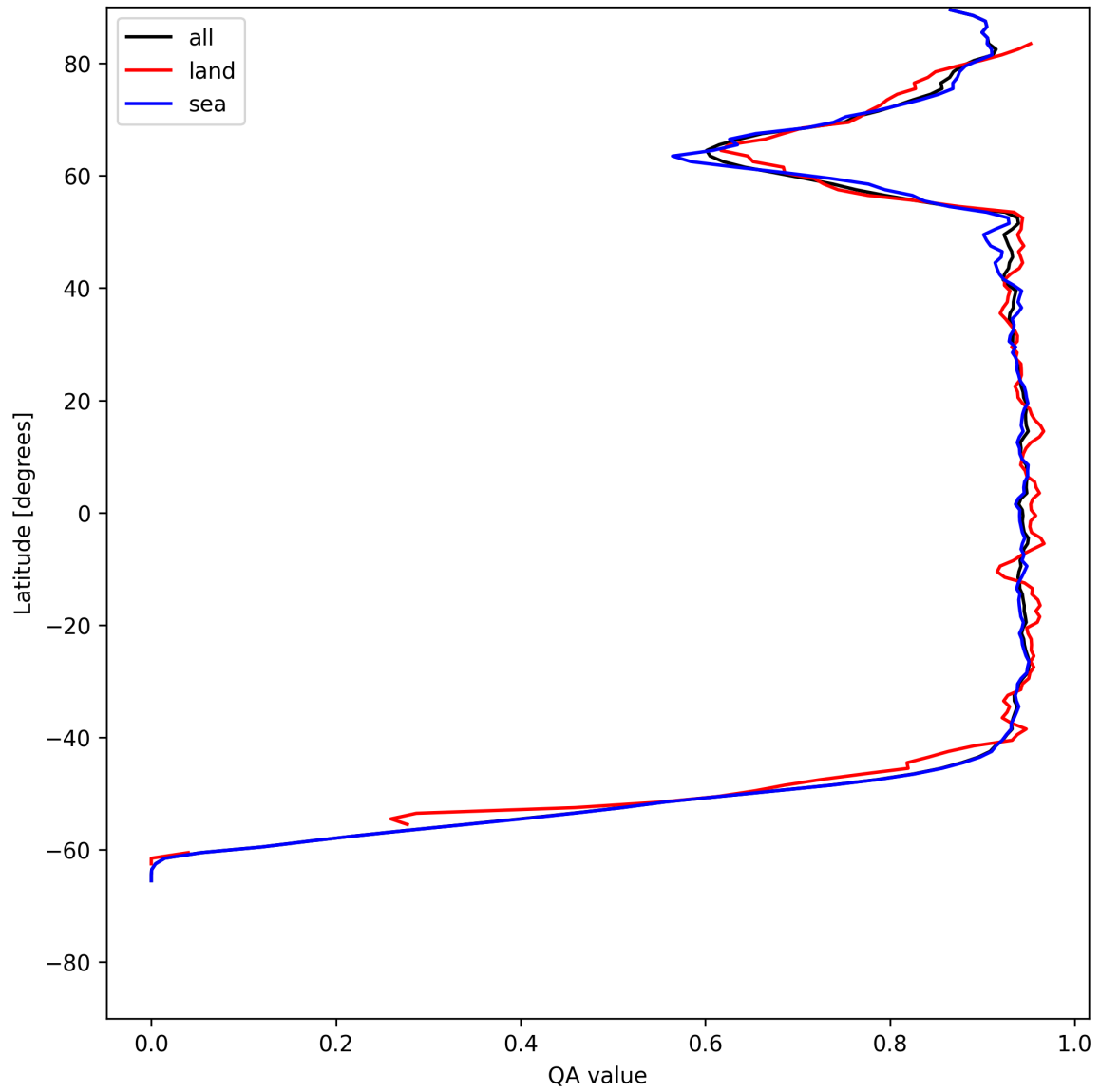
Figure 16: Zonal average of “QA value” for 2025-06-25 to 2025-06-25.
