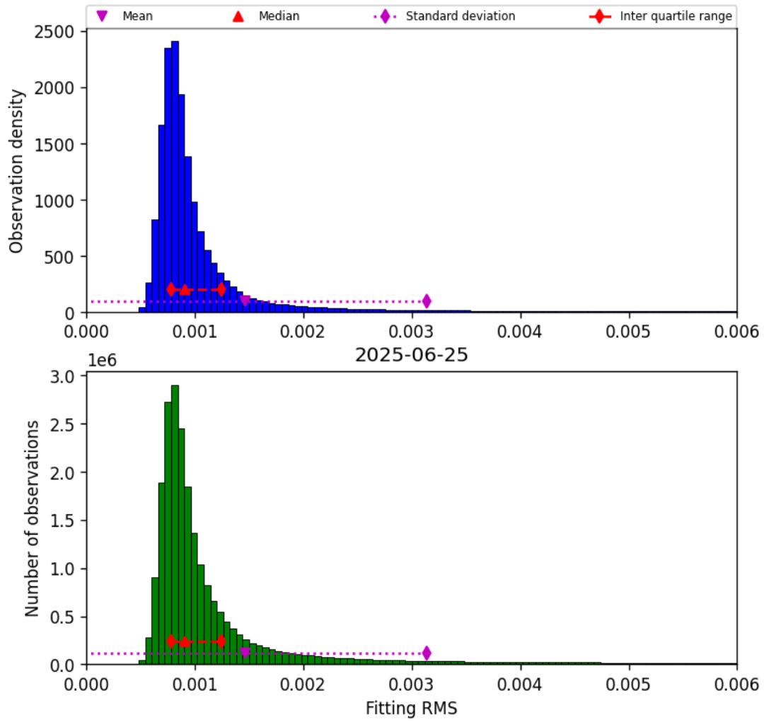
Figure 34: Histogram of “Fitting RMS” for 2025-06-25 to 2025-06-25
