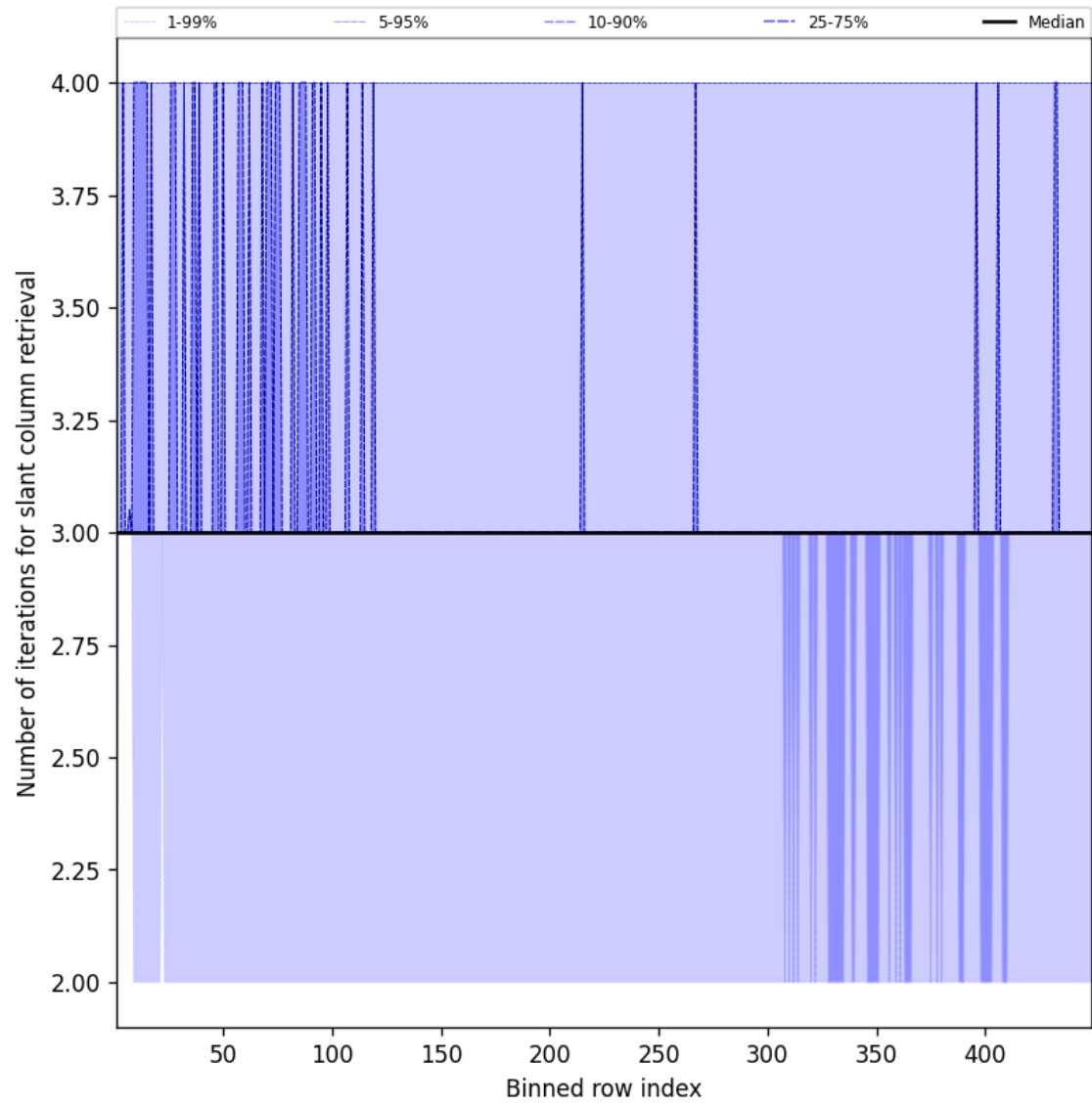
Figure 45: Along track statistics of “Number of iterations for slant column retrieval” for 2025-06-25 to 2025-06-25
