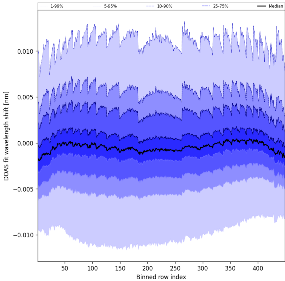
Figure 47: Along track statistics of “DOAS fit wavelength shift” for 2025-06-25 to 2025-06-25
