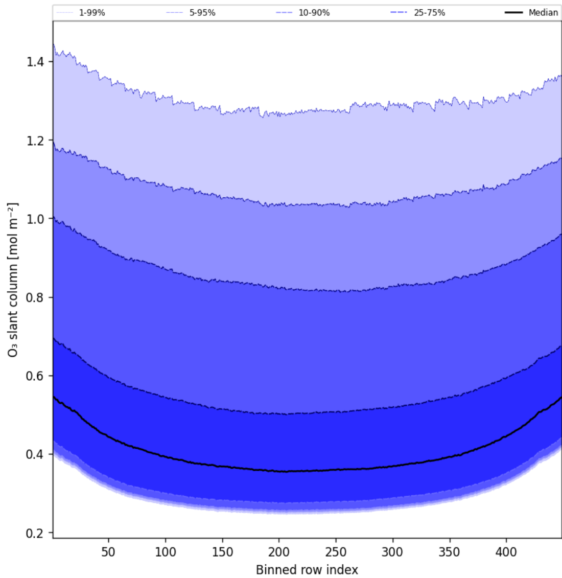
Figure 43: Along track statistics of “O 3 slant column” for 2025-06-25 to 2025-06-25
