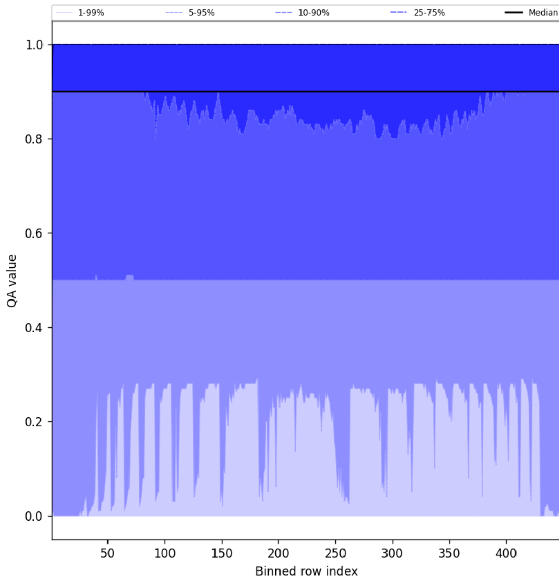
Figure 40: Along track statistics of “QA value” for 2025-06-25 to 2025-06-25
