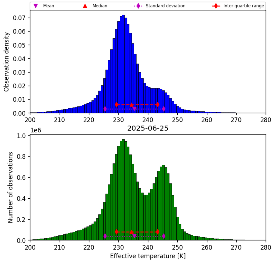
Figure 38: Histogram of “Effective temperature” for 2025-06-25 to 2025-06-25
