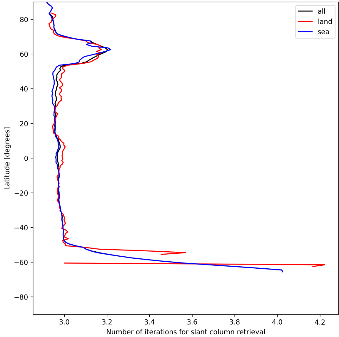
Figure 21: Zonal average of “Number of iterations for slant column retrieval” for 2025-06-25 to 2025-06-25.
