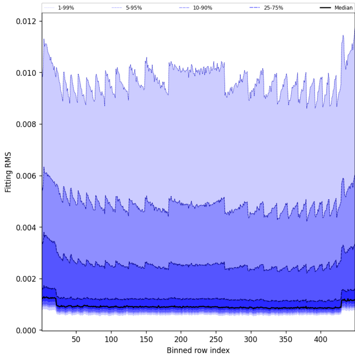
Figure 46: Along track statistics of “Fitting RMS” for 2025-06-25 to 2025-06-25
