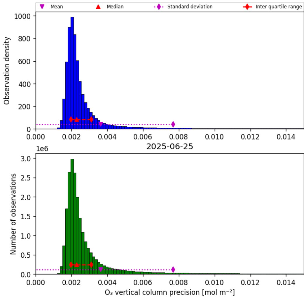
Figure 30: Histogram of “O 3 vertical column precision” for 2025-06-25 to 2025-06-25
