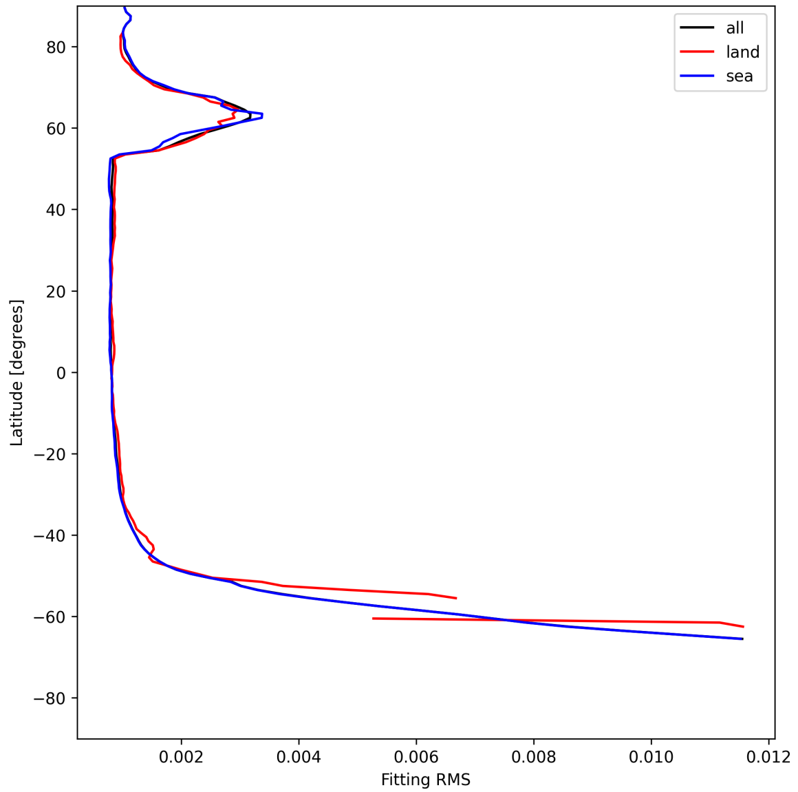
Figure 22: Zonal average of “Fitting RMS” for 2025-06-25 to 2025-06-25.
