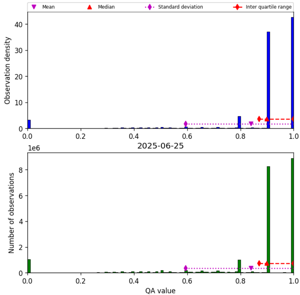
Figure 28: Histogram of “QA value” for 2025-06-25 to 2025-06-25
