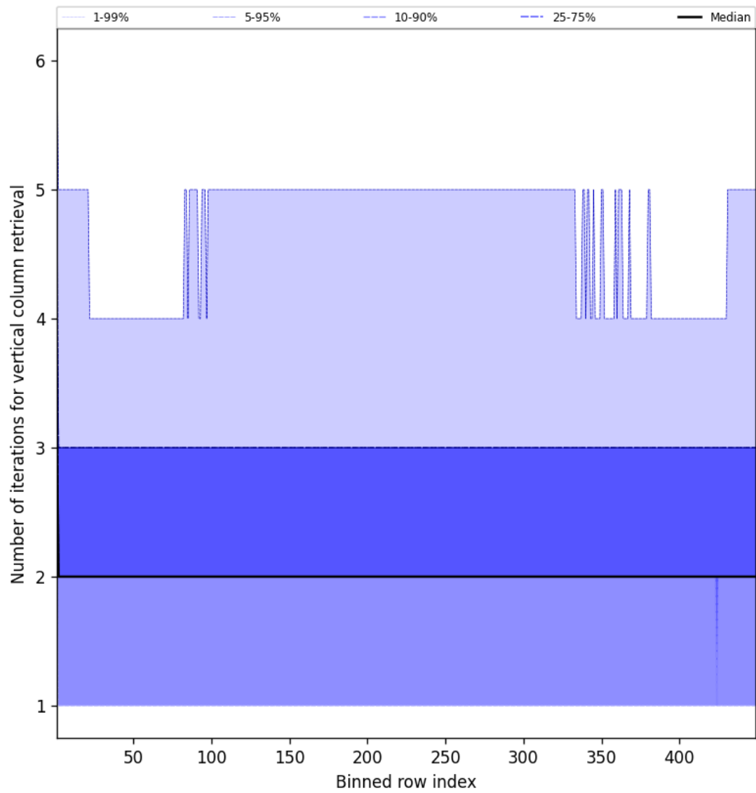
Figure 51: Along track statistics of “Number of iterations for vertical column retrieval” for 2025-06-25 to 2025-06-25
