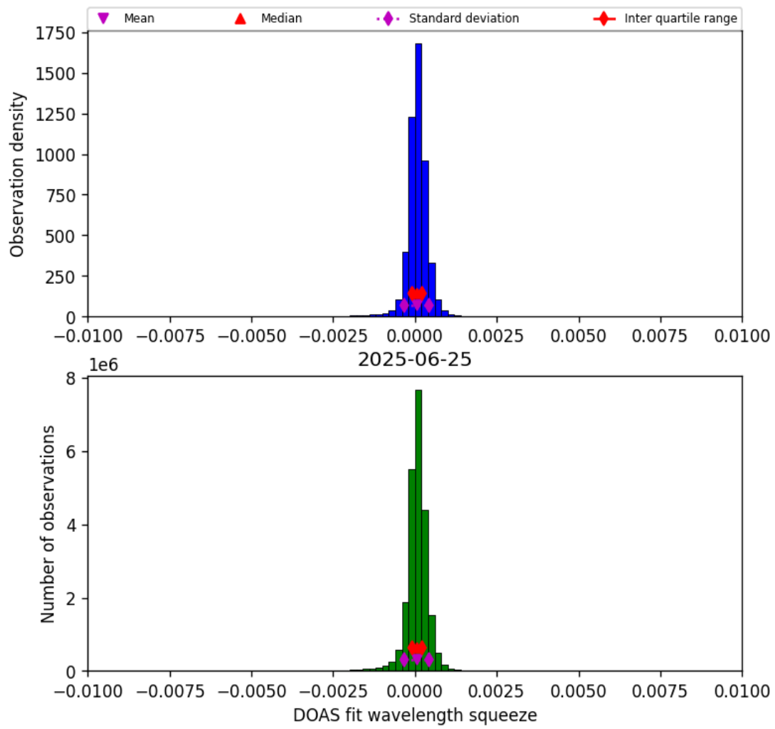
Figure 36: Histogram of “DOAS fit wavelength squeeze” for 2025-06-25 to 2025-06-25
