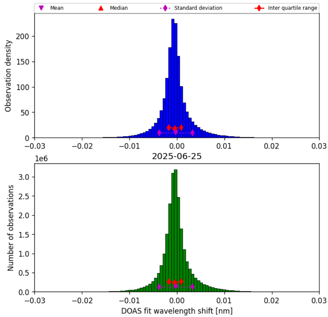
Figure 35: Histogram of “DOAS fit wavelength shift” for 2025-06-25 to 2025-06-25
