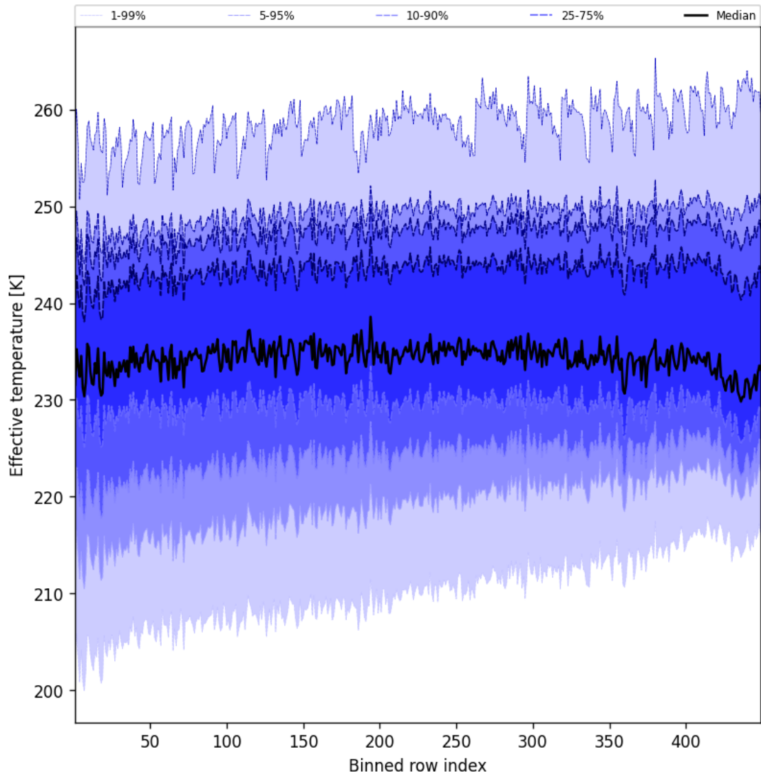
Figure 50: Along track statistics of “Effective temperature” for 2025-06-25 to 2025-06-25
