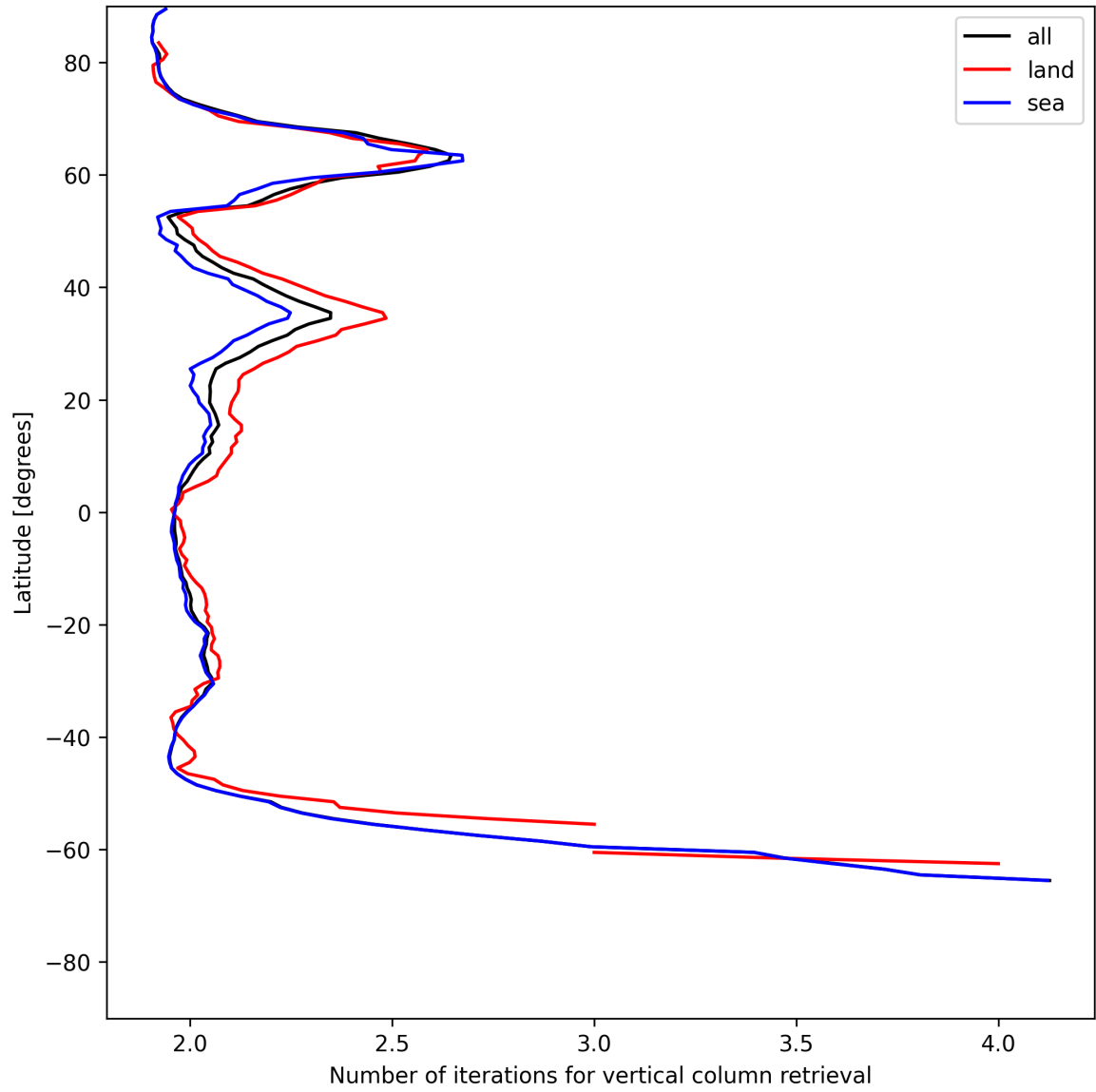
Figure 27: Zonal average of “Number of iterations for vertical column retrieval” for 2025-06-25 to 2025-06-25.
