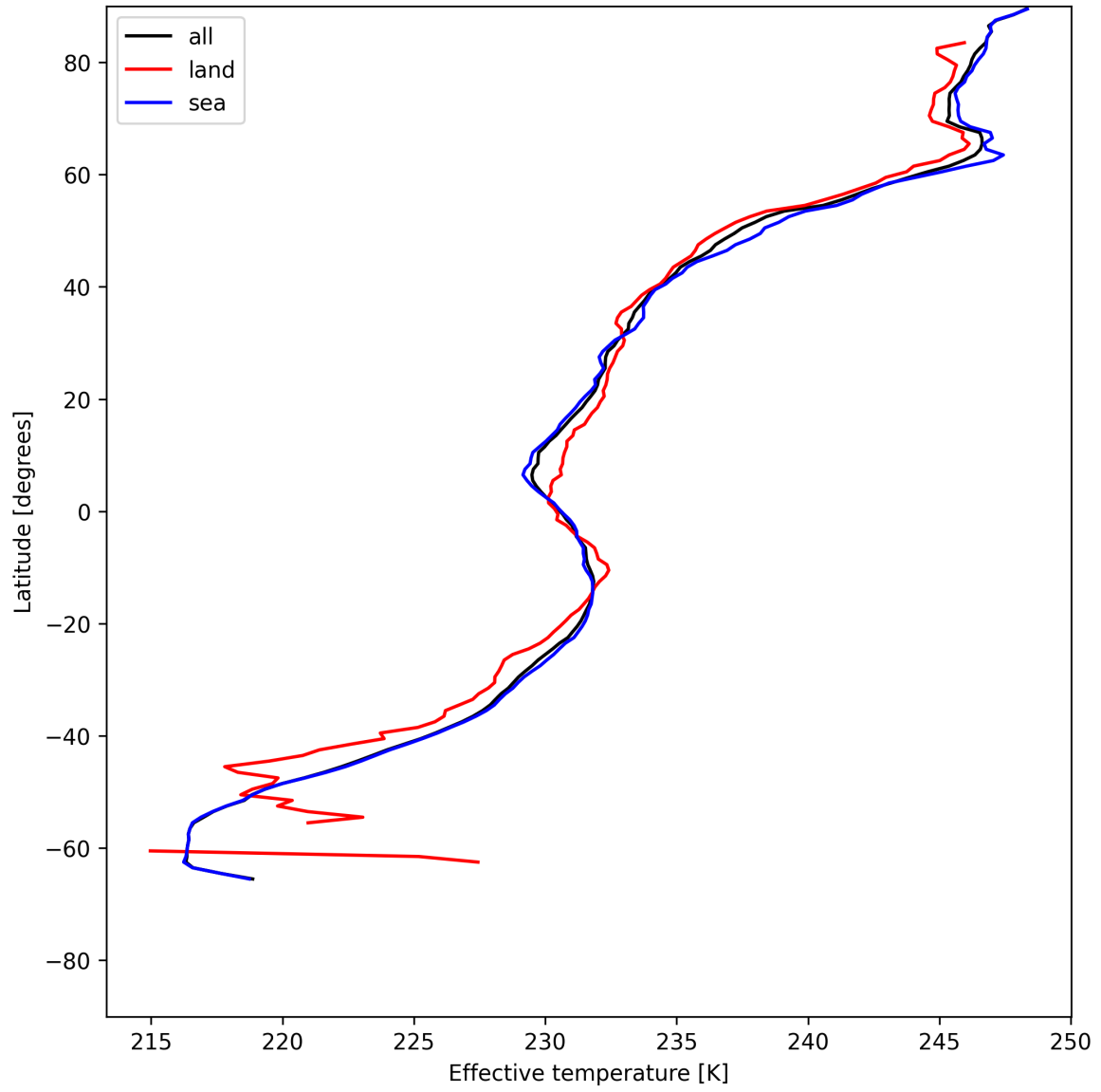
Figure 26: Zonal average of "Effective temperature" for 2025-06-25 to 2025-06-25.
