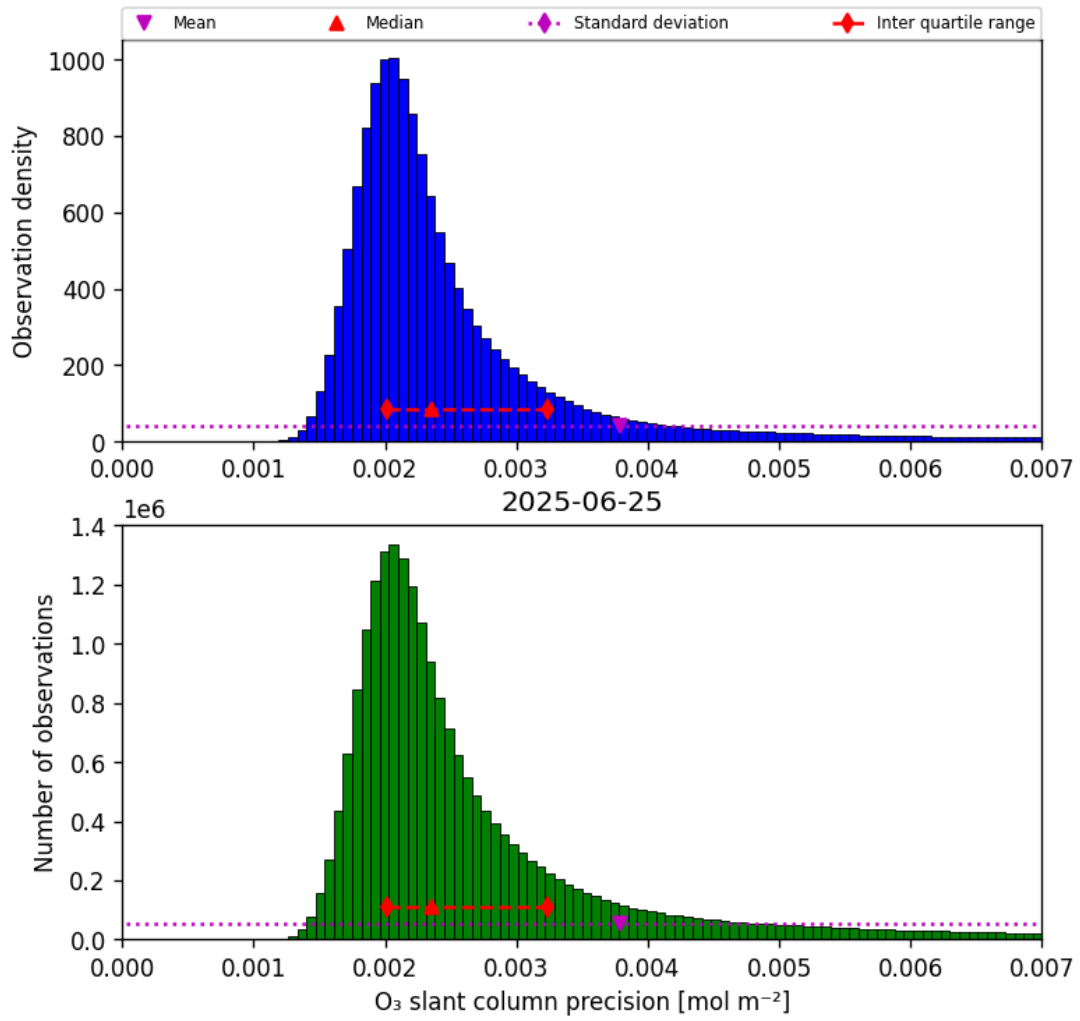
Figure 32: Histogram of “O 3 slant column precision” for 2025-06-25 to 2025-06-25
