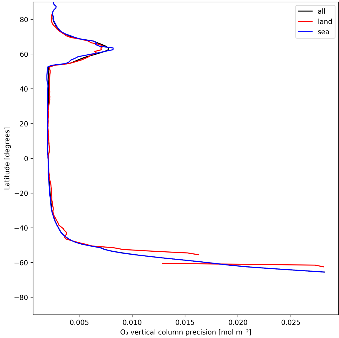
Figure 18: Zonal average of “O 3 vertical column precision” for 2025-06-25 to 2025-06-25.
