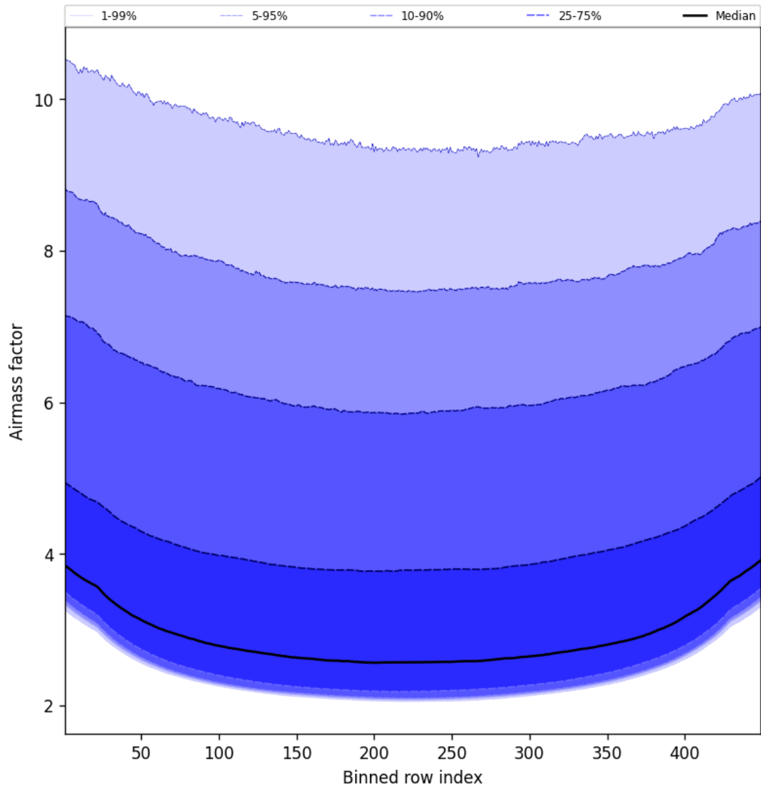
Figure 49: Along track statistics of “Airmass factor” for 2025-06-25 to 2025-06-25
