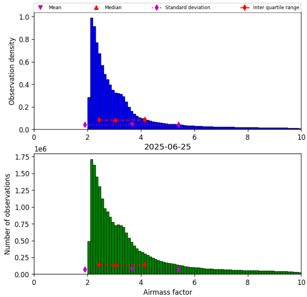
Figure 37: Histogram of “Airmass factor” for 2025-06-25 to 2025-06-25
