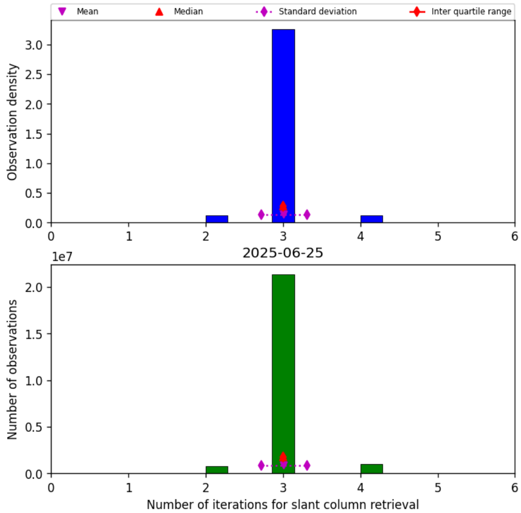
Figure 33: Histogram of "Number of iterations for slant column retrieval" for 2025-06-25 to 2025-06-25
