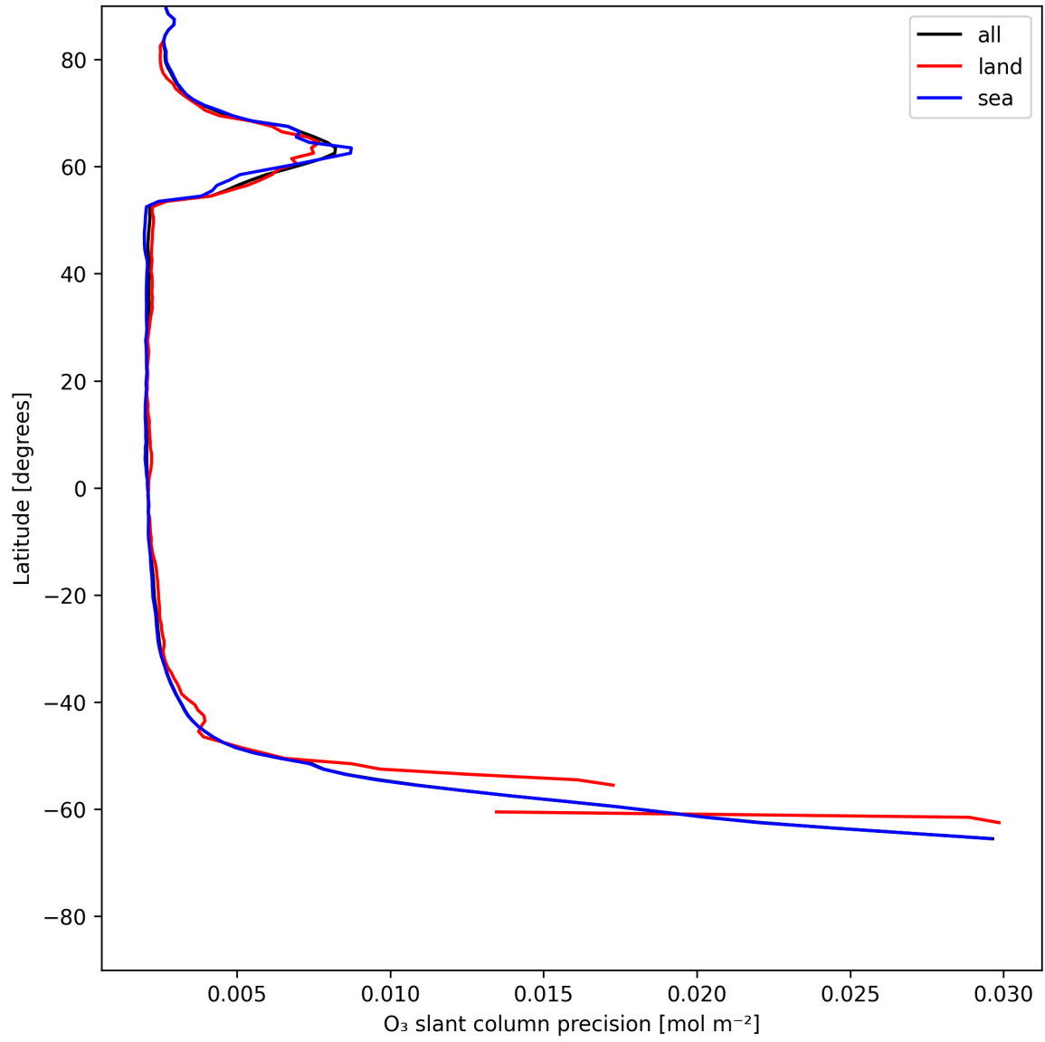
Figure 20: Zonal average of “O 3 slant column precision” for 2025-06-25 to 2025-06-25.
