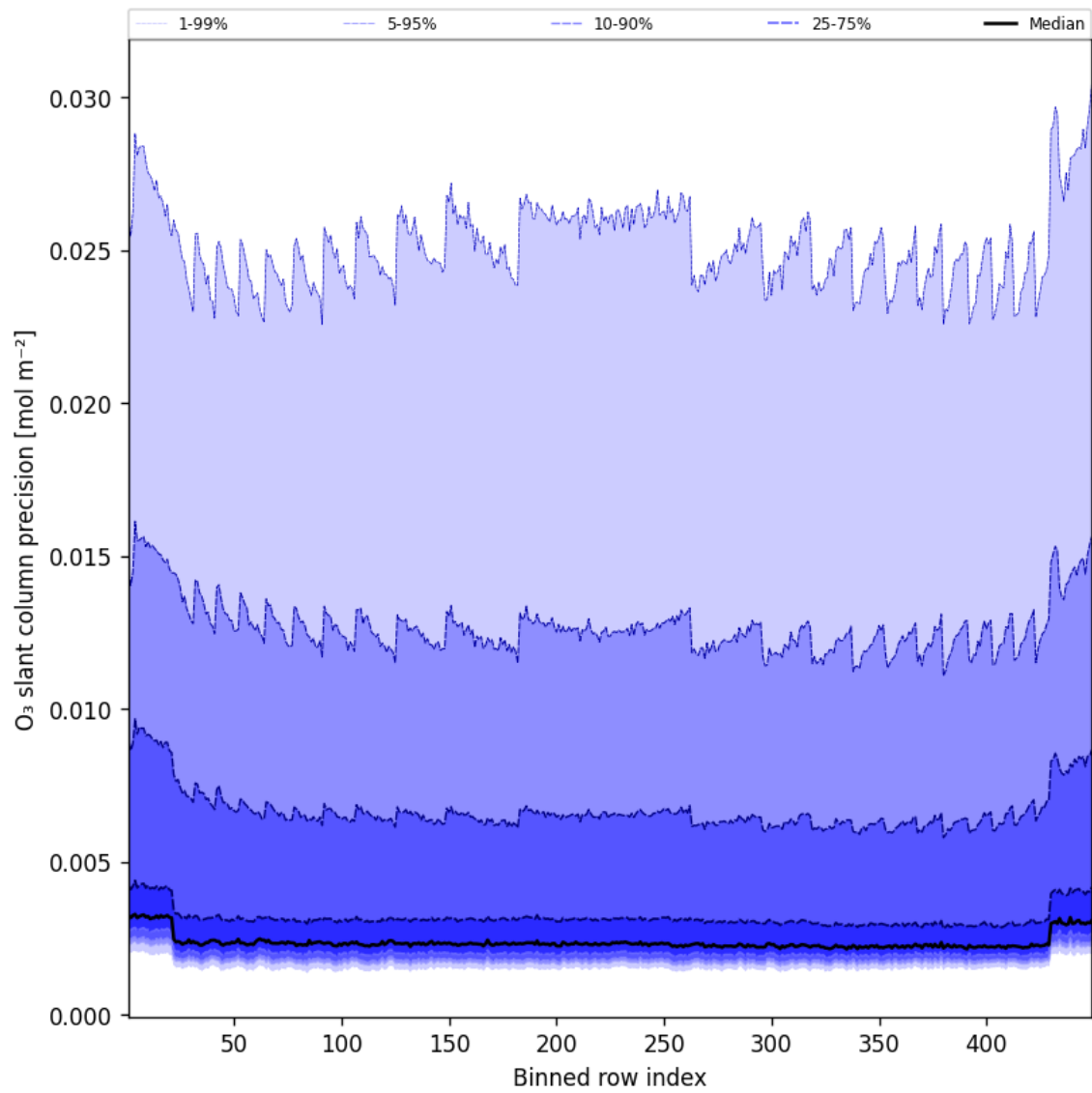
Figure 44: Along track statistics of “O 3 slant column precision” for 2025-06-25 to 2025-06-25
