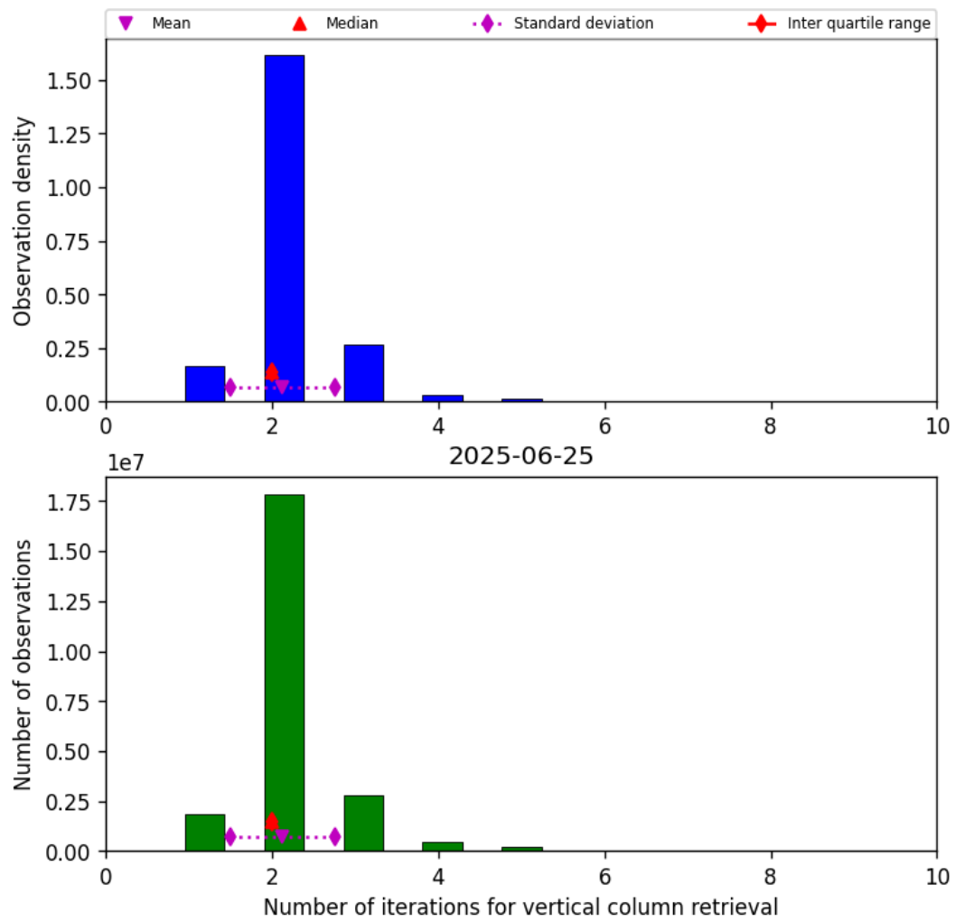
Figure 39: Histogram of “Number of iterations for vertical column retrieval” for 2025-06-25 to 2025-06-25
