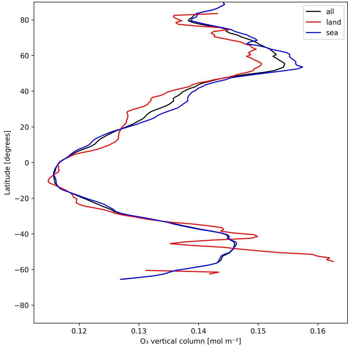
Figure 17: Zonal average of “O 3 vertical column” for 2025-06-25 to 2025-06-25.
