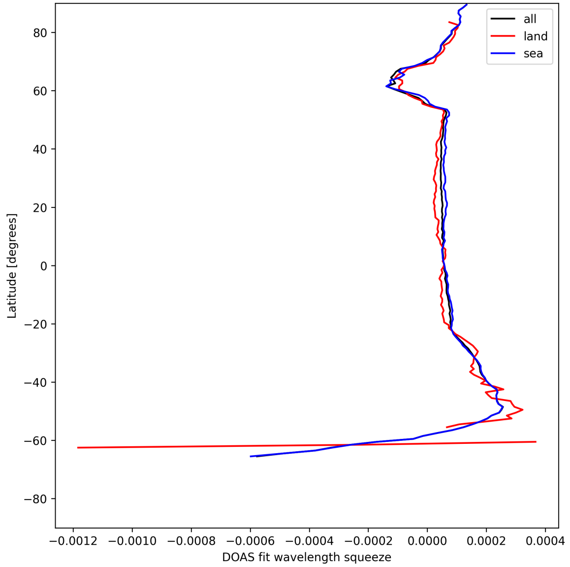
Figure 24: Zonal average of “DOAS fit wavelength squeeze” for 2025-06-25 to 2025-06-25.
