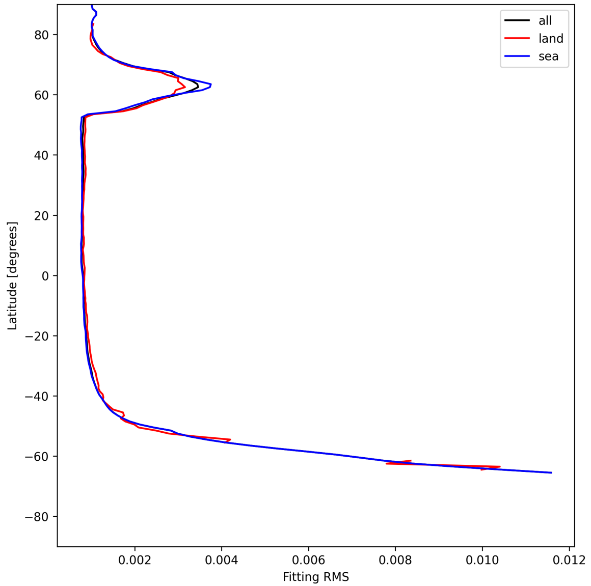
Figure 22: Zonal average of “Fitting RMS” for 2025-06-26 to 2025-06-27.
