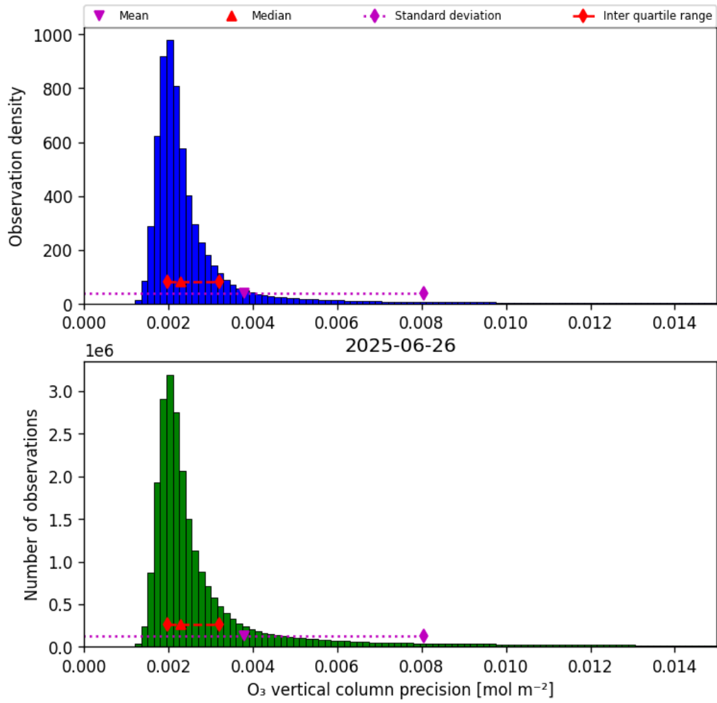
Figure 30: Histogram of “O 3 vertical column precision” for 2025-06-26 to 2025-06-27
