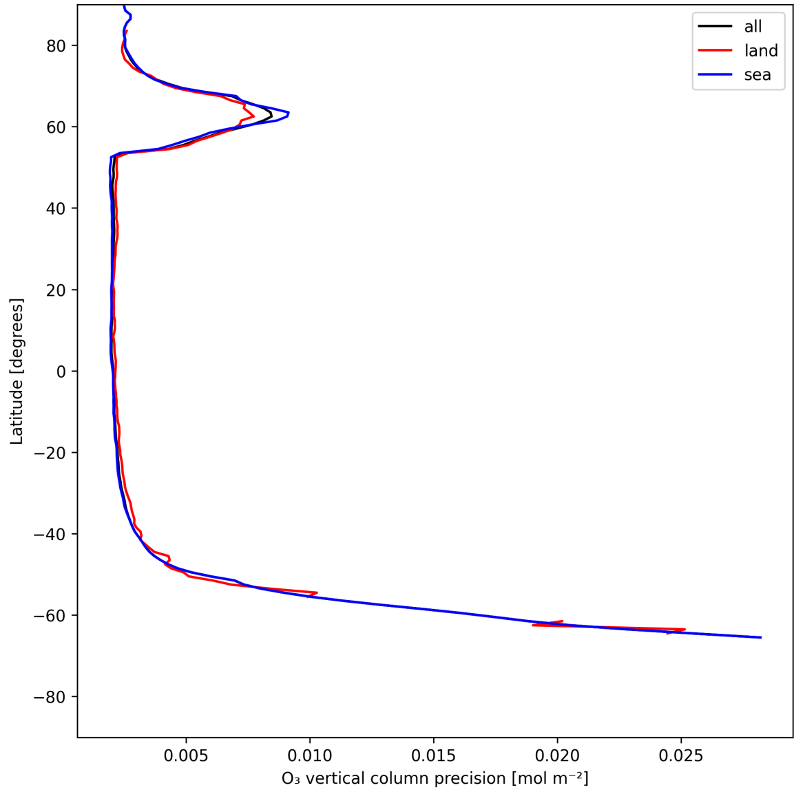
Figure 18: Zonal average of “O 3 vertical column precision” for 2025-06-26 to 2025-06-27.
