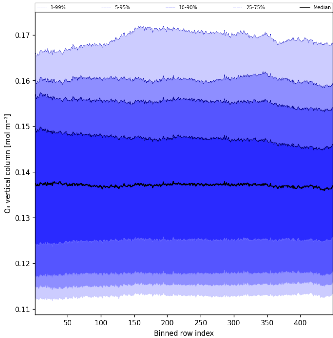
Figure 41: Along track statistics of “ \text{O}_3 vertical column” for 2025-06-26 to 2025-06-27
