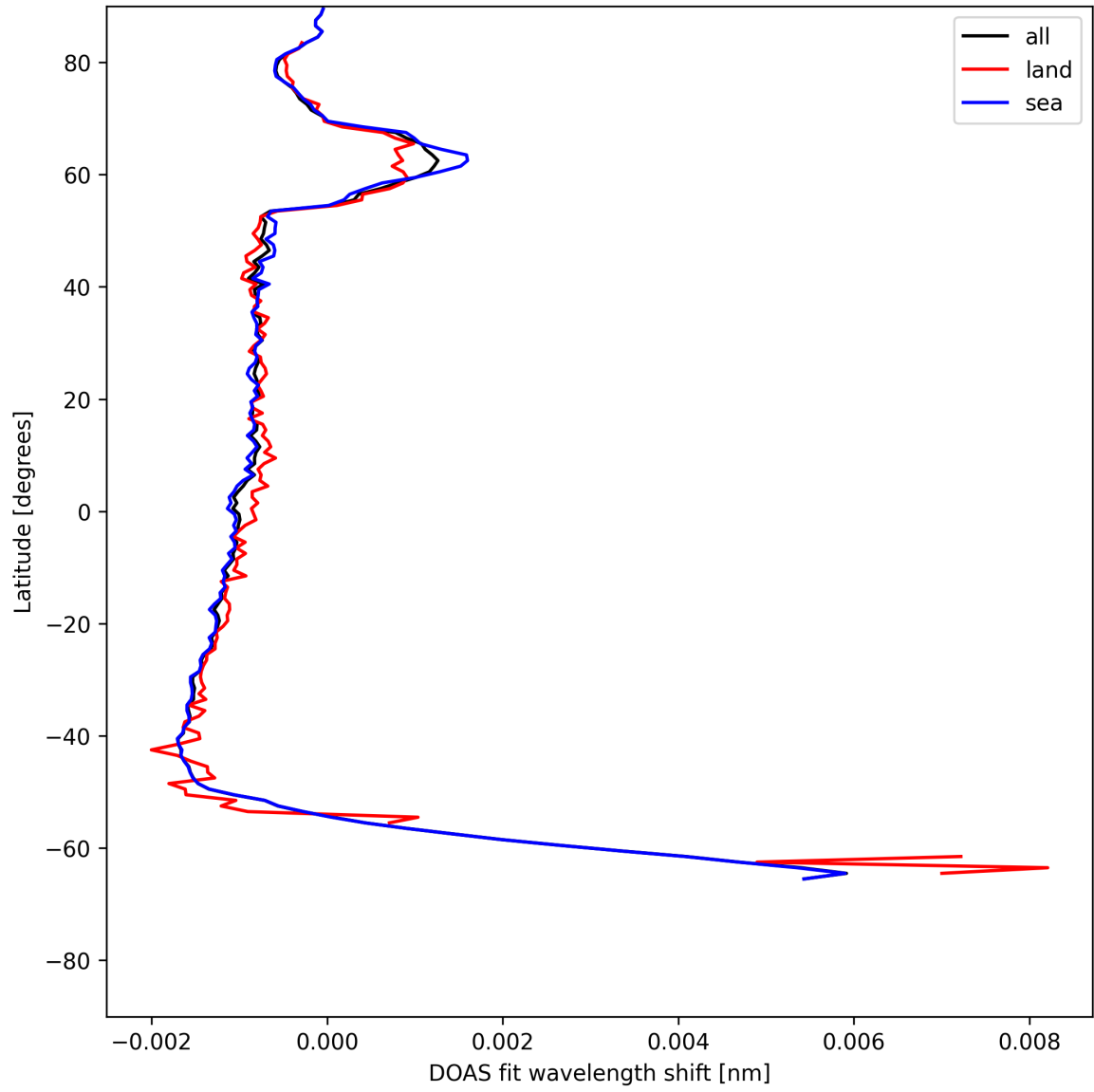
Figure 23: Zonal average of “DOAS fit wavelength shift” for 2025-06-26 to 2025-06-27.
