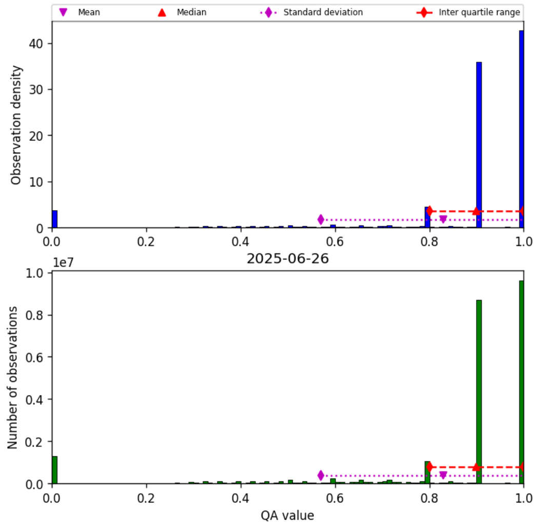
Figure 28: Histogram of “QA value” for 2025-06-26 to 2025-06-27
