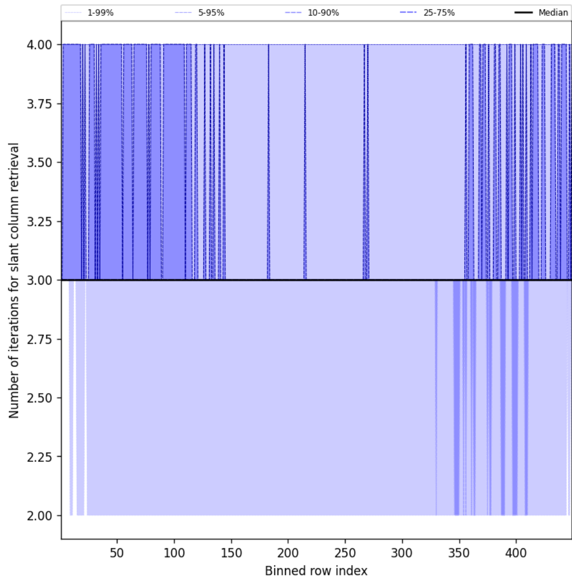
Figure 45: Along track statistics of “Number of iterations for slant column retrieval” for 2025-06-26 to 2025-06-27
