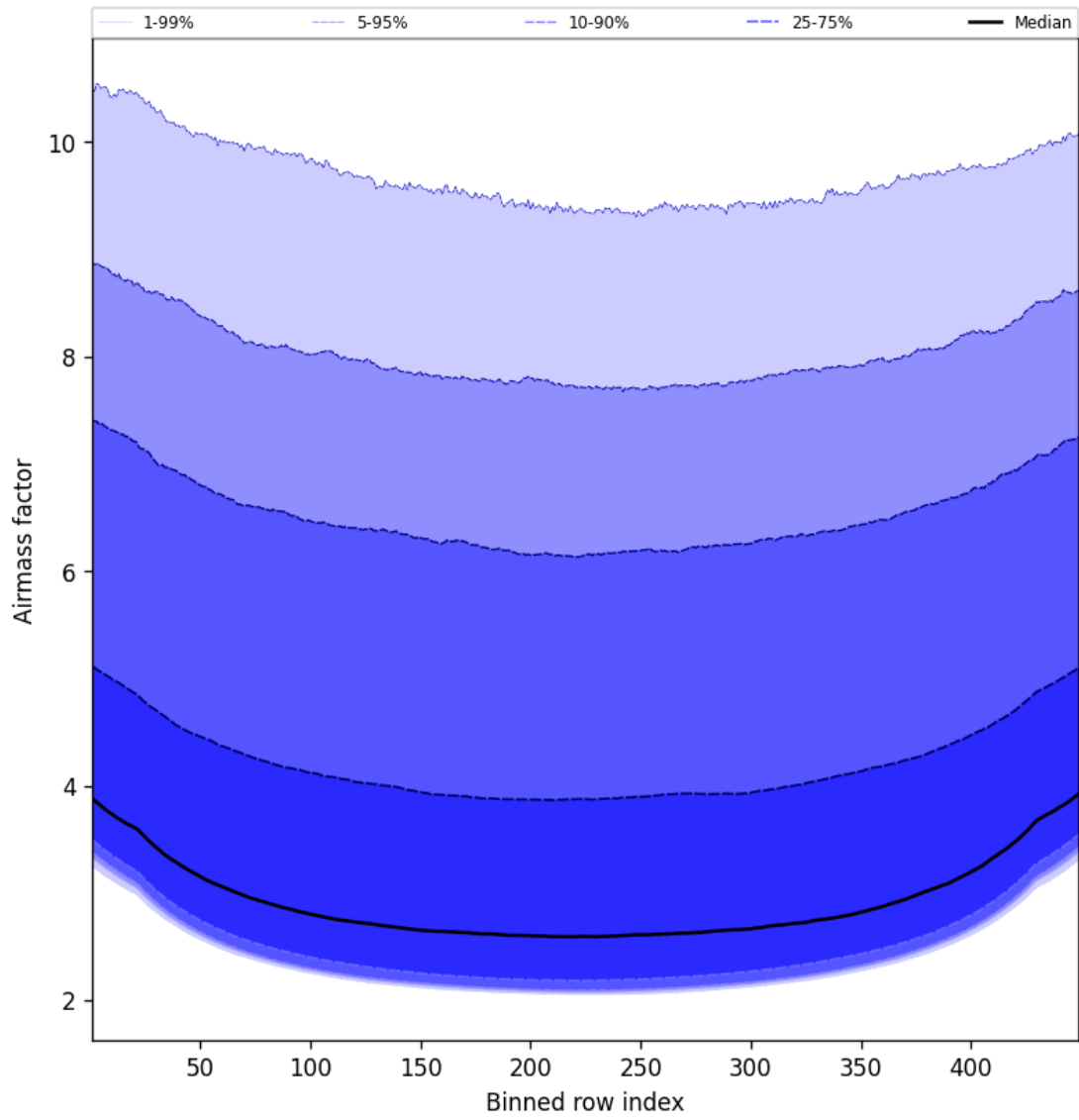
Figure 49: Along track statistics of “Airmass factor” for 2025-06-26 to 2025-06-27
