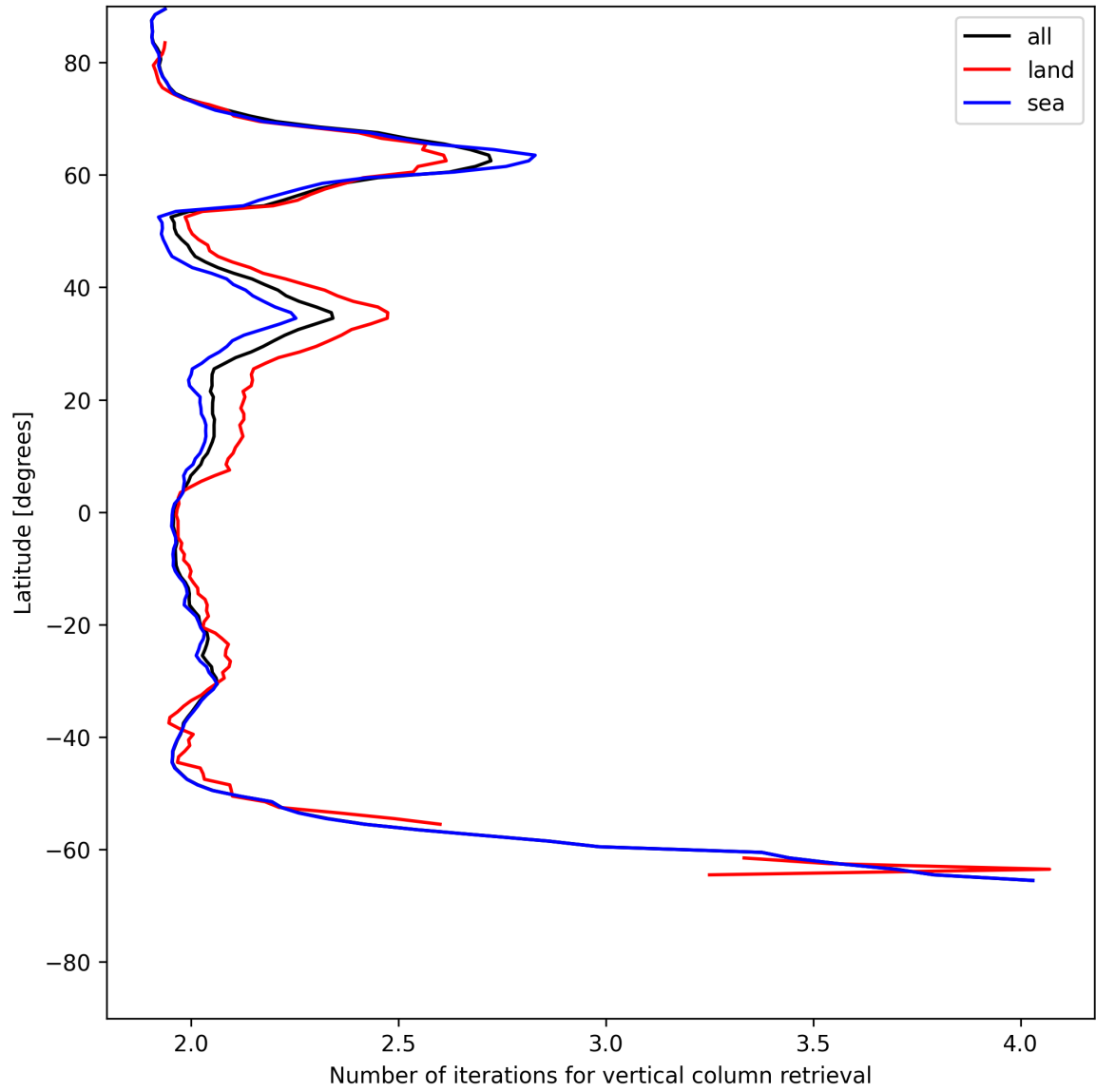
Figure 27: Zonal average of “Number of iterations for vertical column retrieval” for 2025-06-26 to 2025-06-27.
