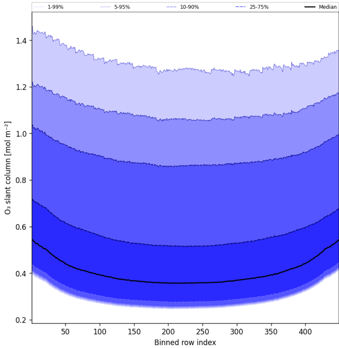
Figure 43: Along track statistics of “O 3 slant column” for 2025-06-26 to 2025-06-27
