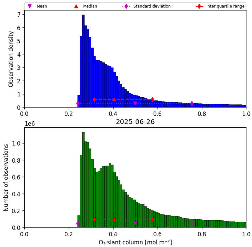
Figure 31: Histogram of “O 3 slant column” for 2025-06-26 to 2025-06-27
