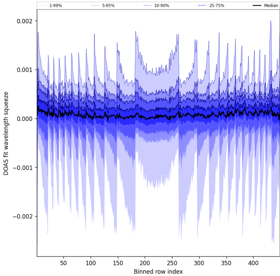
Figure 48: Along track statistics of “DOAS fit wavelength squeeze” for 2025-06-26 to 2025-06-27
