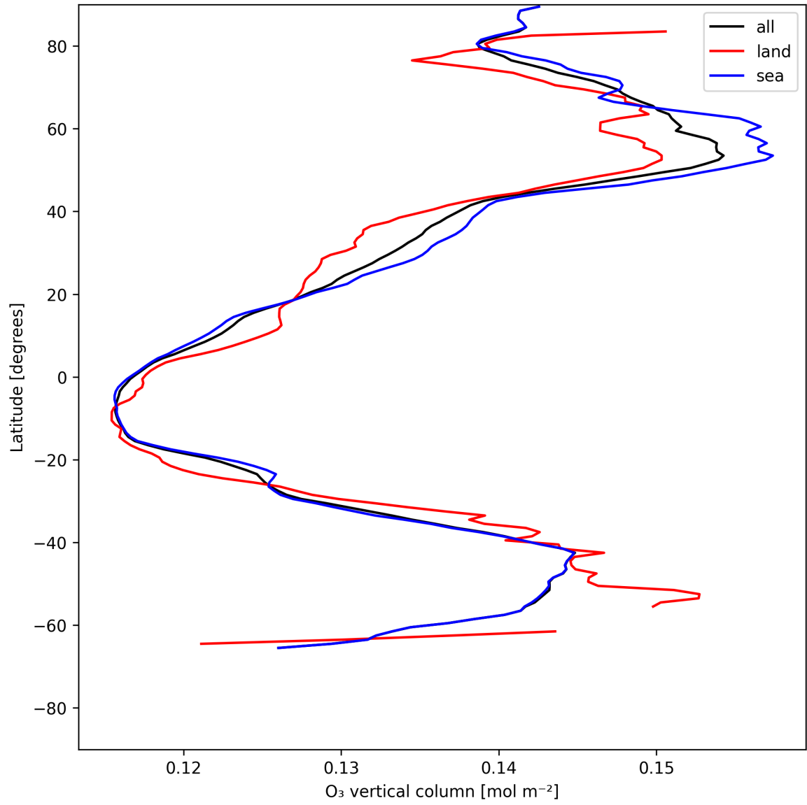
Figure 17: Zonal average of “O 3 vertical column” for 2025-06-26 to 2025-06-27.
