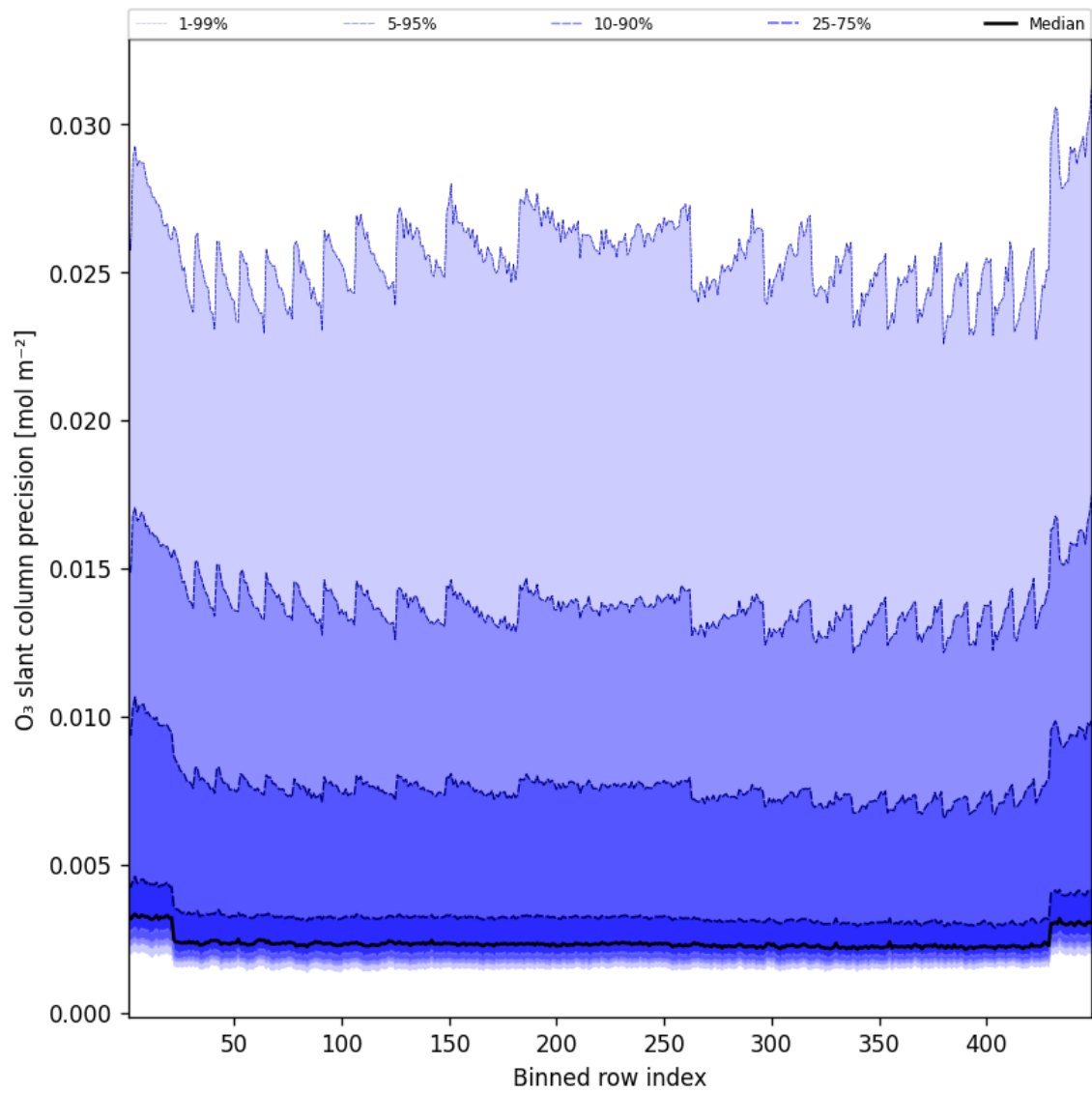
Figure 44: Along track statistics of “O 3 slant column precision” for 2025-06-26 to 2025-06-27
