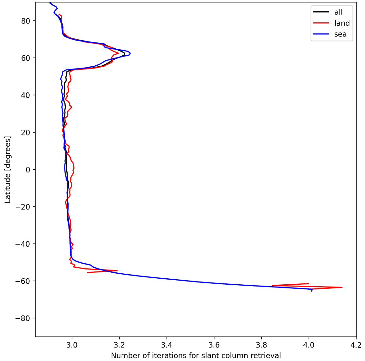
Figure 21: Zonal average of “Number of iterations for slant column retrieval” for 2025-06-26 to 2025-06-27.
