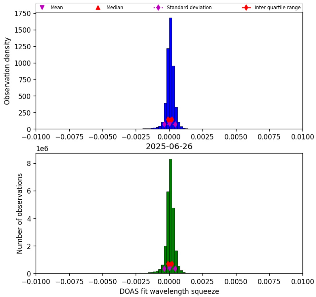
Figure 36: Histogram of “DOAS fit wavelength squeeze” for 2025-06-26 to 2025-06-27
