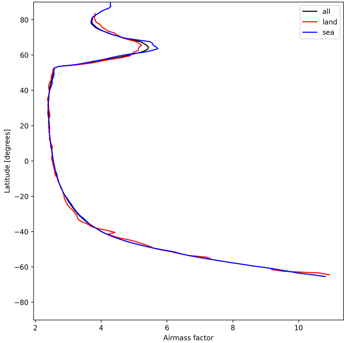
Figure 25: Zonal average of “Airmass factor” for 2025-06-26 to 2025-06-27.
