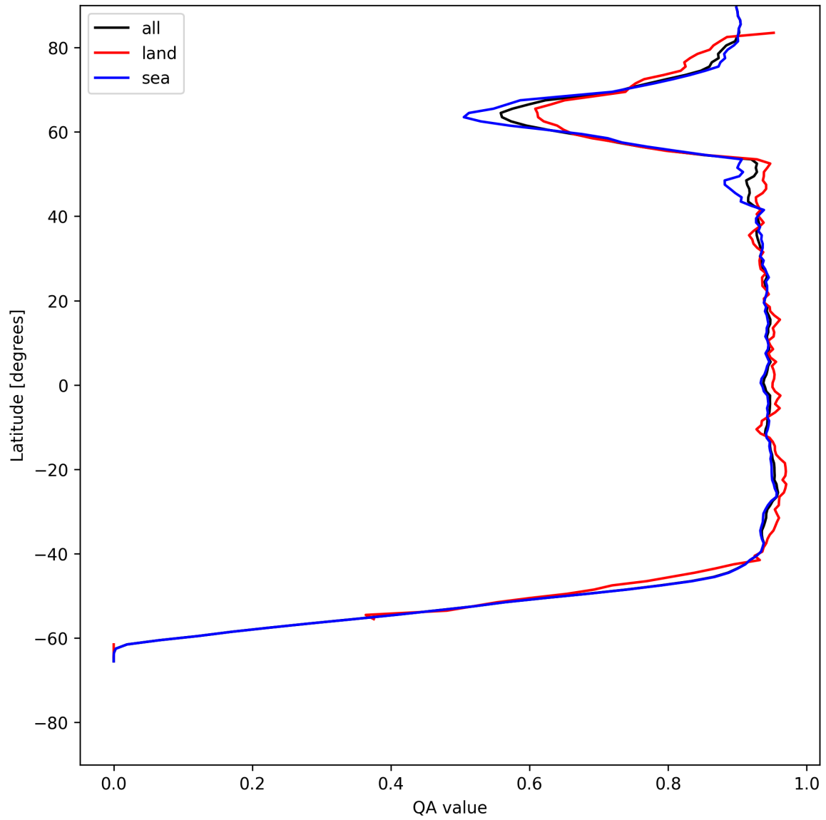
Figure 16: Zonal average of “QA value” for 2025-06-26 to 2025-06-27.
