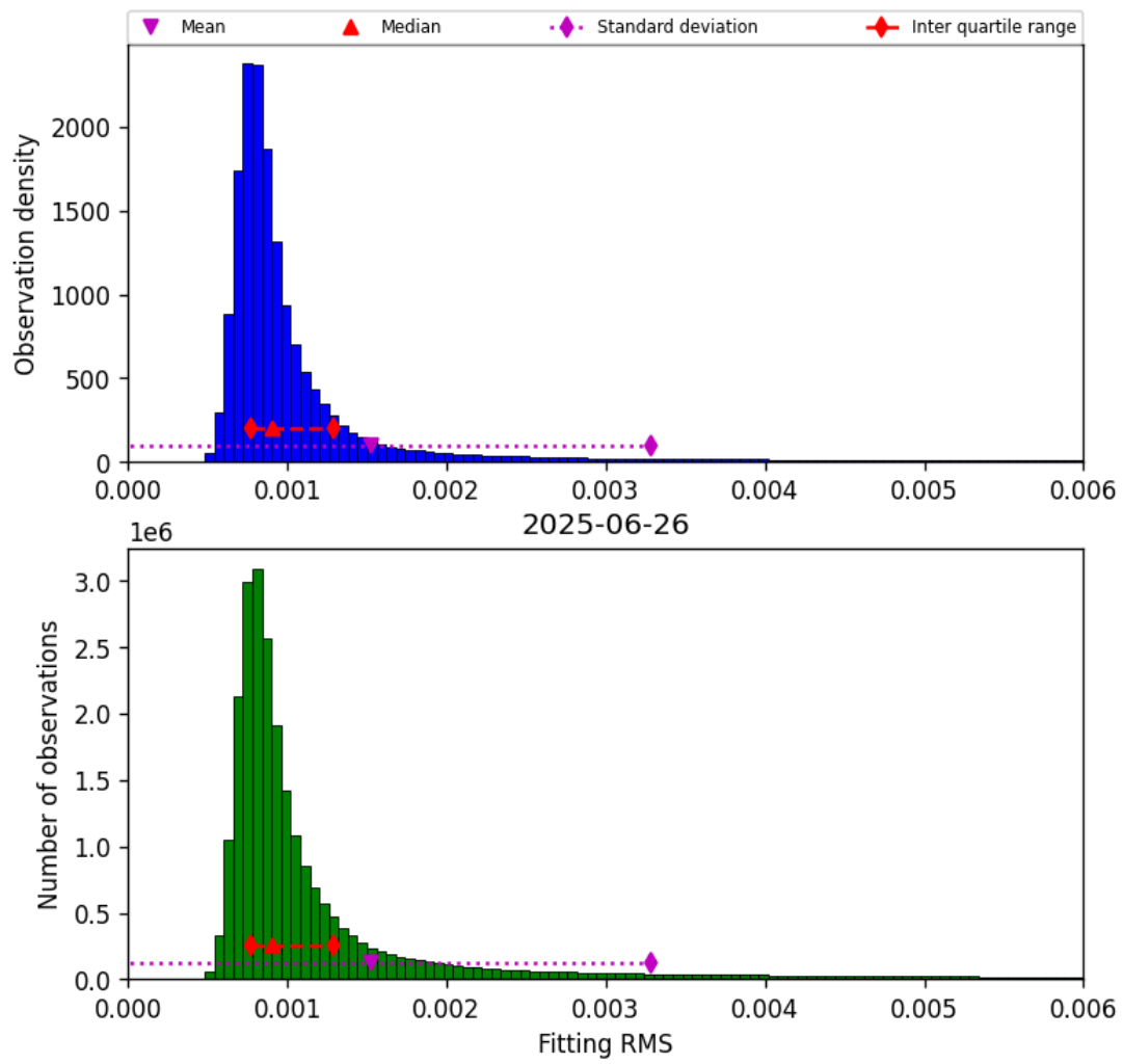
Figure 34: Histogram of “Fitting RMS” for 2025-06-26 to 2025-06-27
