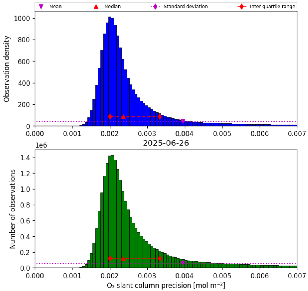
Figure 32: Histogram of “O 3 slant column precision” for 2025-06-26 to 2025-06-27
