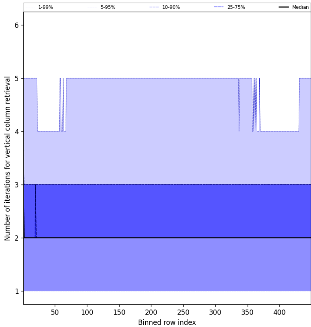
Figure 51: Along track statistics of “Number of iterations for vertical column retrieval” for 2025-06-26 to 2025-06-27
