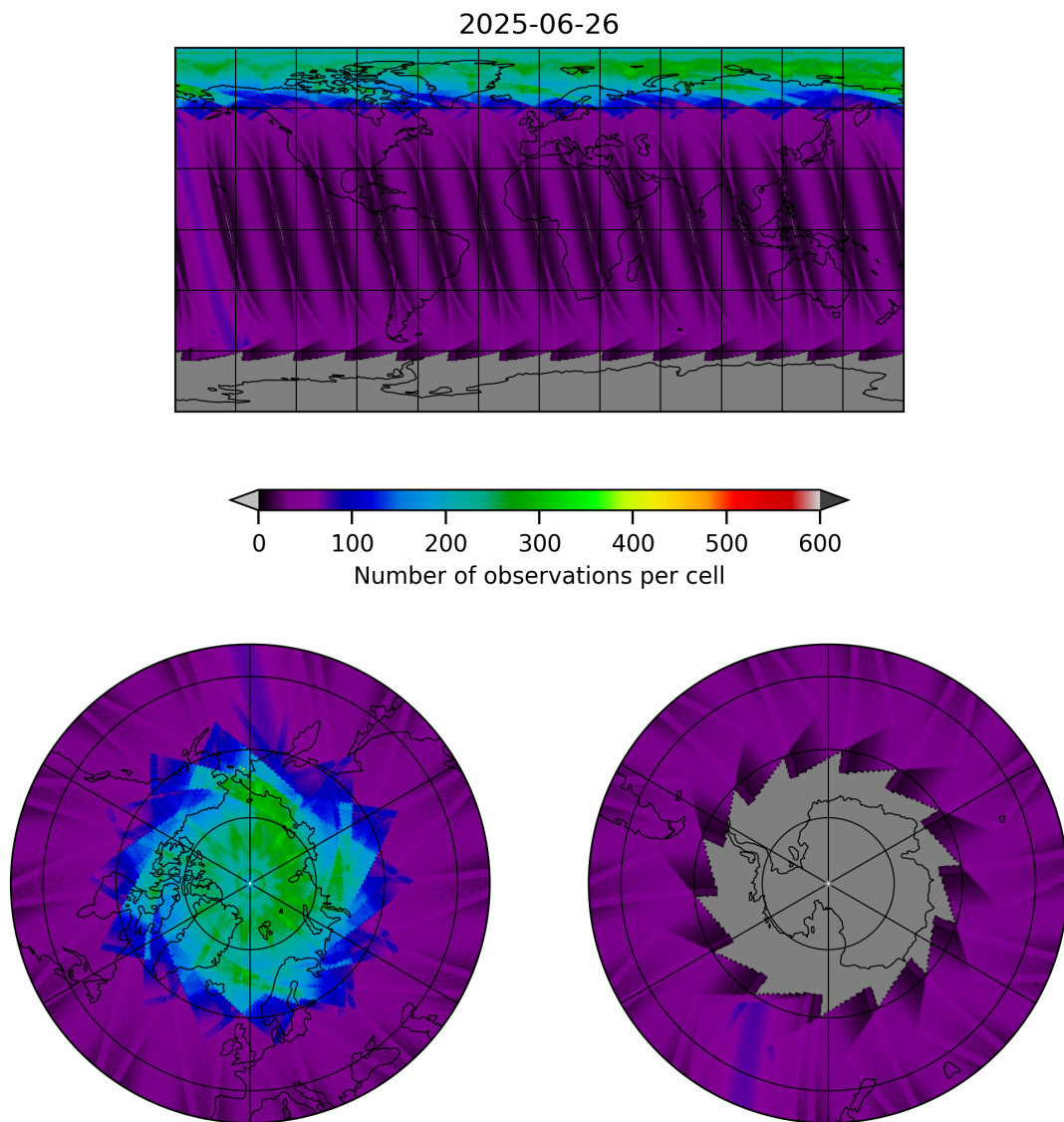
Figure 15: Map of the number of observations for 2025-06-26 to 2025-06-27
