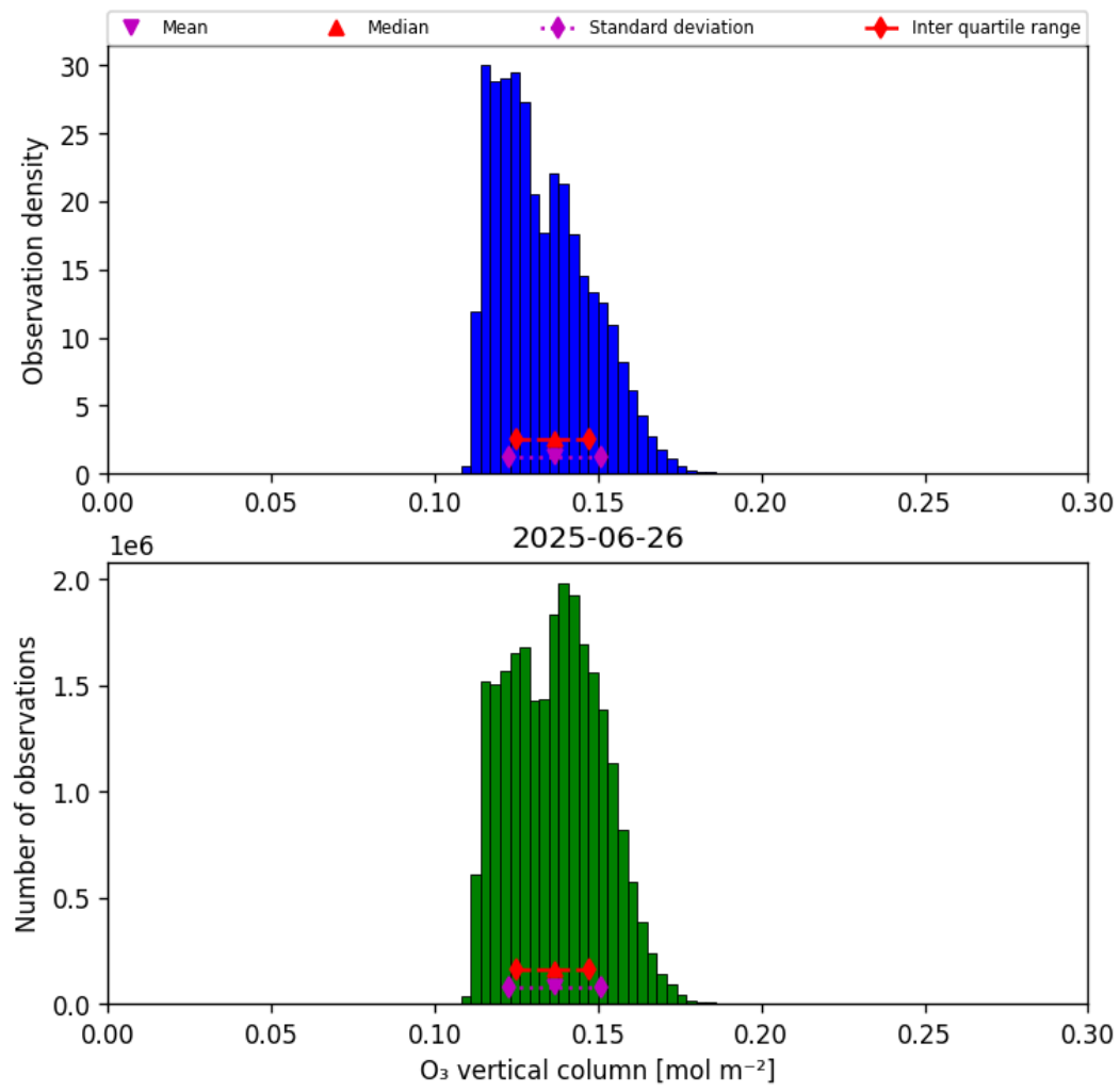
Figure 29: Histogram of “O 3 vertical column” for 2025-06-26 to 2025-06-27
