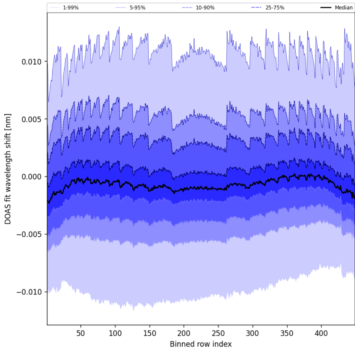
Figure 47: Along track statistics of “DOAS fit wavelength shift” for 2025-06-26 to 2025-06-27
