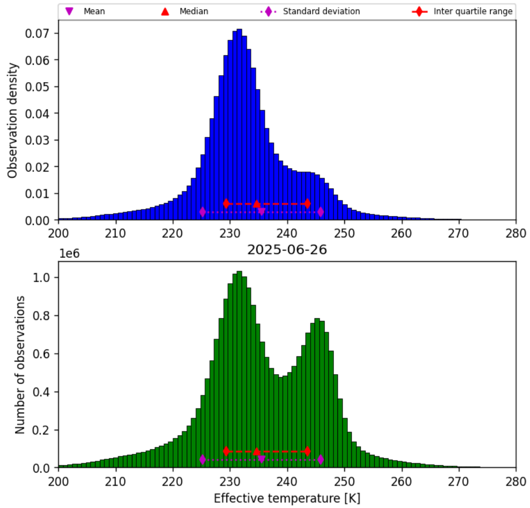
Figure 38: Histogram of “Effective temperature” for 2025-06-26 to 2025-06-27
