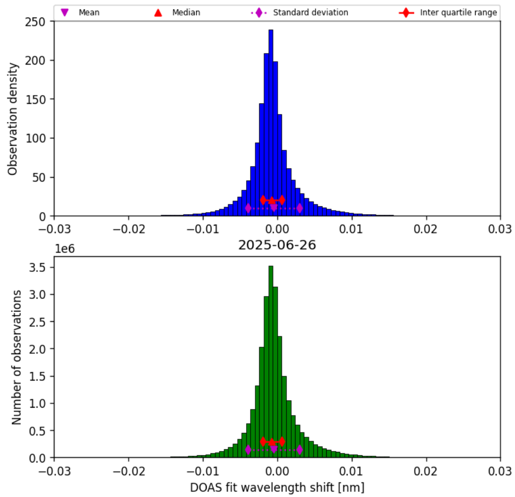
Figure 35: Histogram of “DOAS fit wavelength shift” for 2025-06-26 to 2025-06-27
