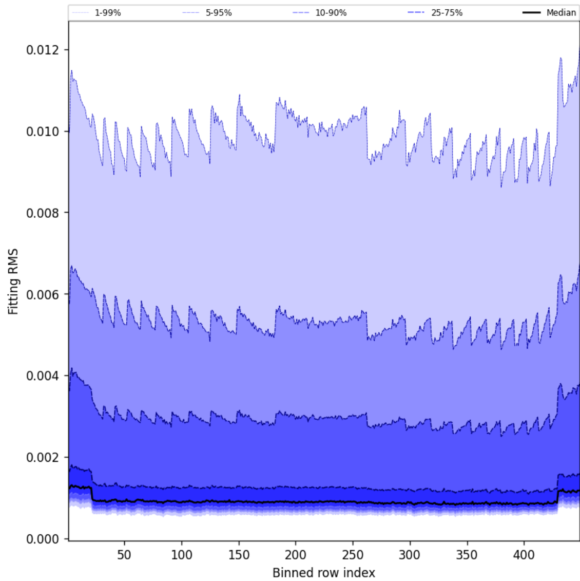
Figure 46: Along track statistics of “Fitting RMS” for 2025-06-26 to 2025-06-27
