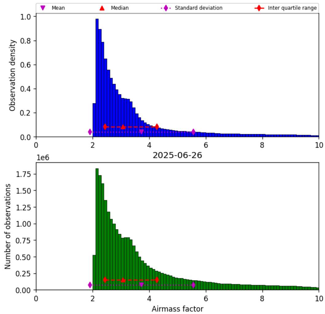
Figure 37: Histogram of “Airmass factor” for 2025-06-26 to 2025-06-27
