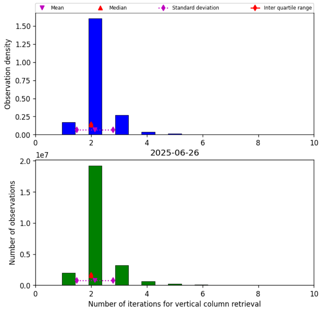
Figure 39: Histogram of “Number of iterations for vertical column retrieval” for 2025-06-26 to 2025-06-27
