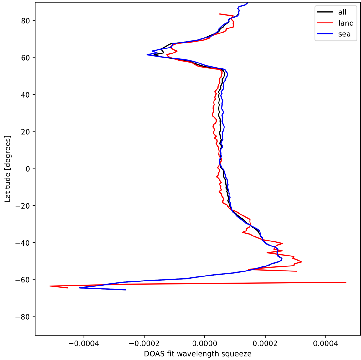
Figure 24: Zonal average of “DOAS fit wavelength squeeze” for 2025-06-26 to 2025-06-27.
