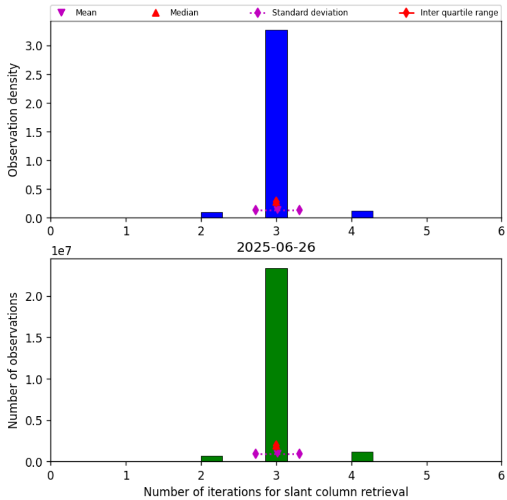
Figure 33: Histogram of “Number of iterations for slant column retrieval” for 2025-06-26 to 2025-06-27
