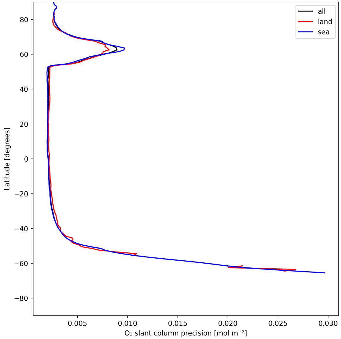
Figure 20: Zonal average of “O 3 slant column precision” for 2025-06-26 to 2025-06-27.
