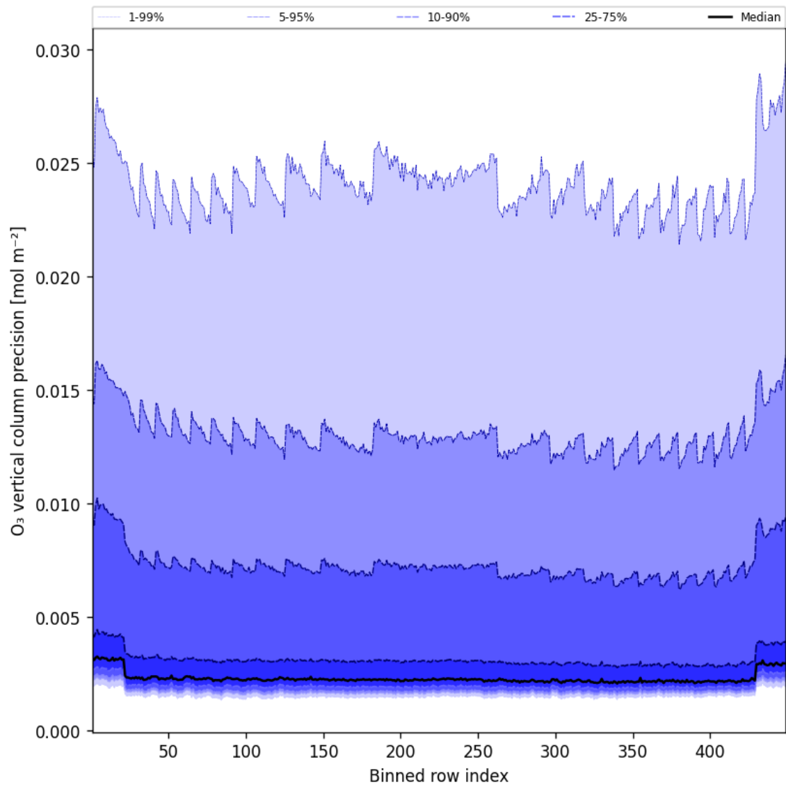
Figure 42: Along track statistics of “O 3 vertical column precision” for 2025-06-26 to 2025-06-27
