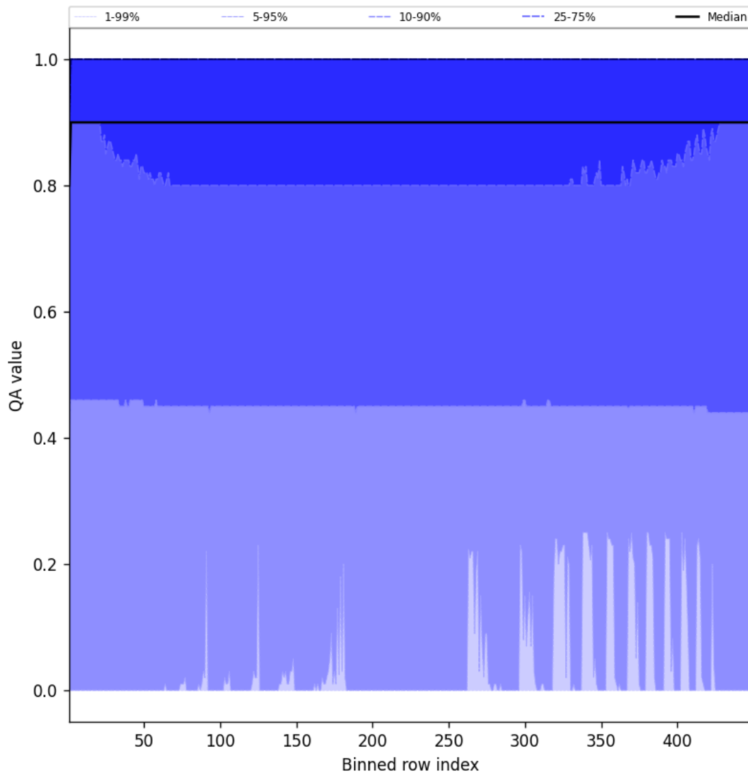
Figure 40: Along track statistics of “QA value” for 2025-06-26 to 2025-06-27
