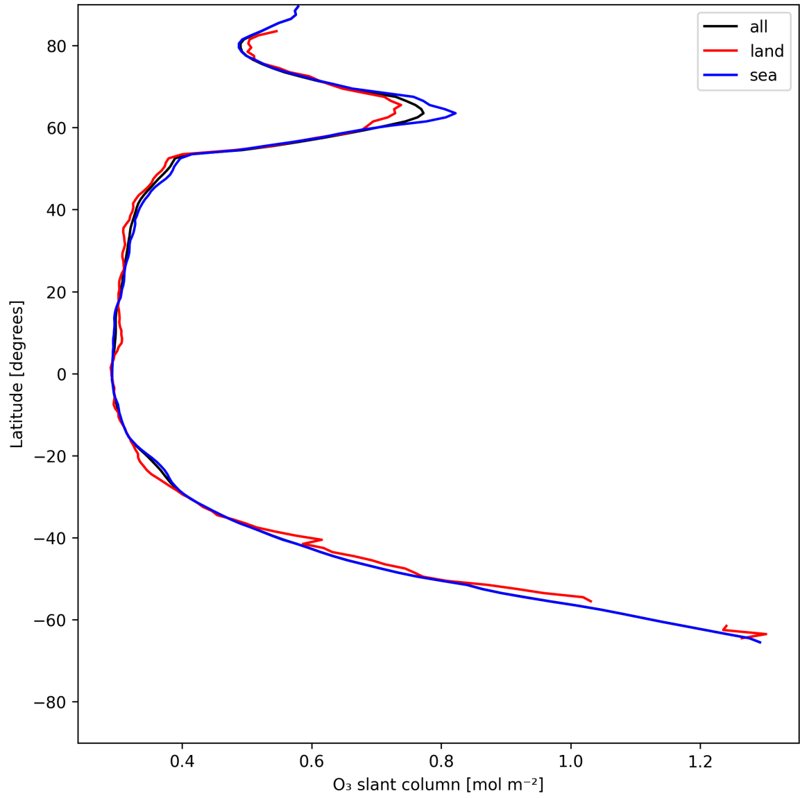
Figure 19: Zonal average of “O 3 slant column” for 2025-06-26 to 2025-06-27.
