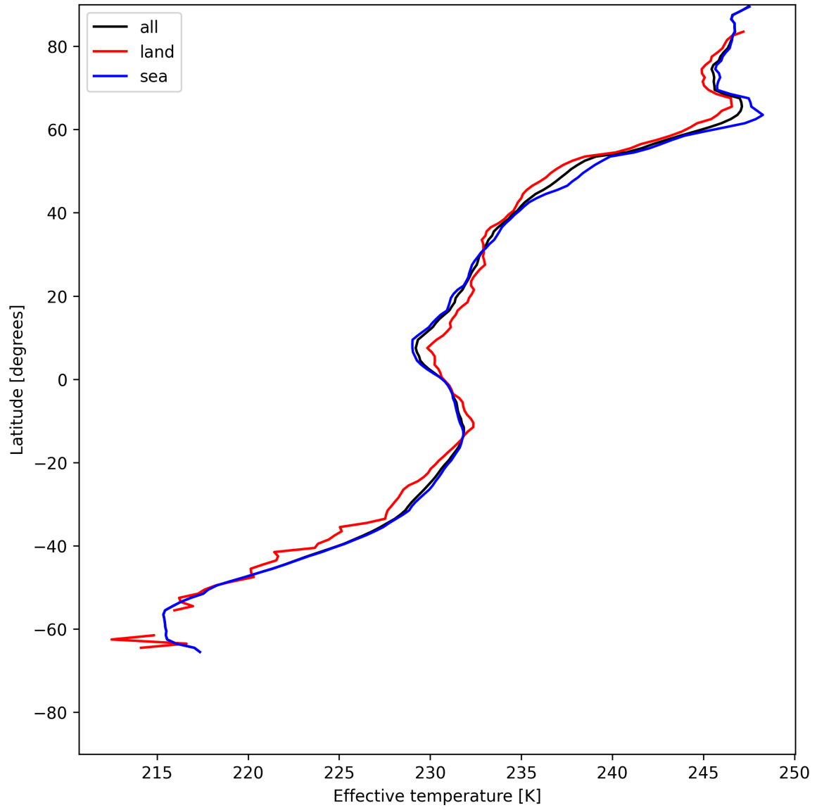
Figure 26: Zonal average of "Effective temperature" for 2025-06-26 to 2025-06-27.
