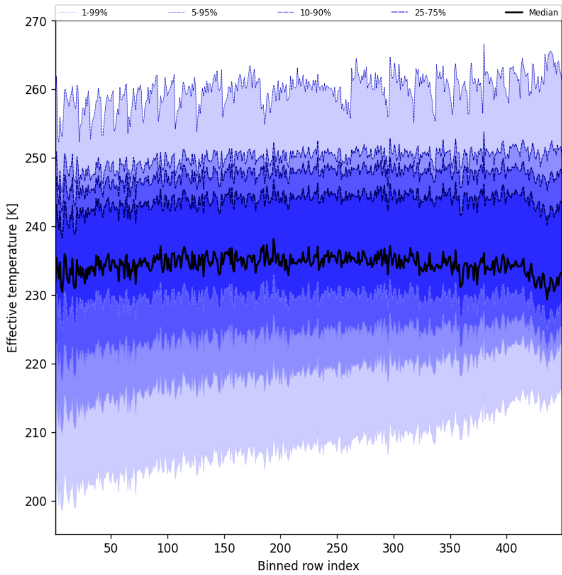
Figure 50: Along track statistics of “Effective temperature” for 2025-06-26 to 2025-06-27
