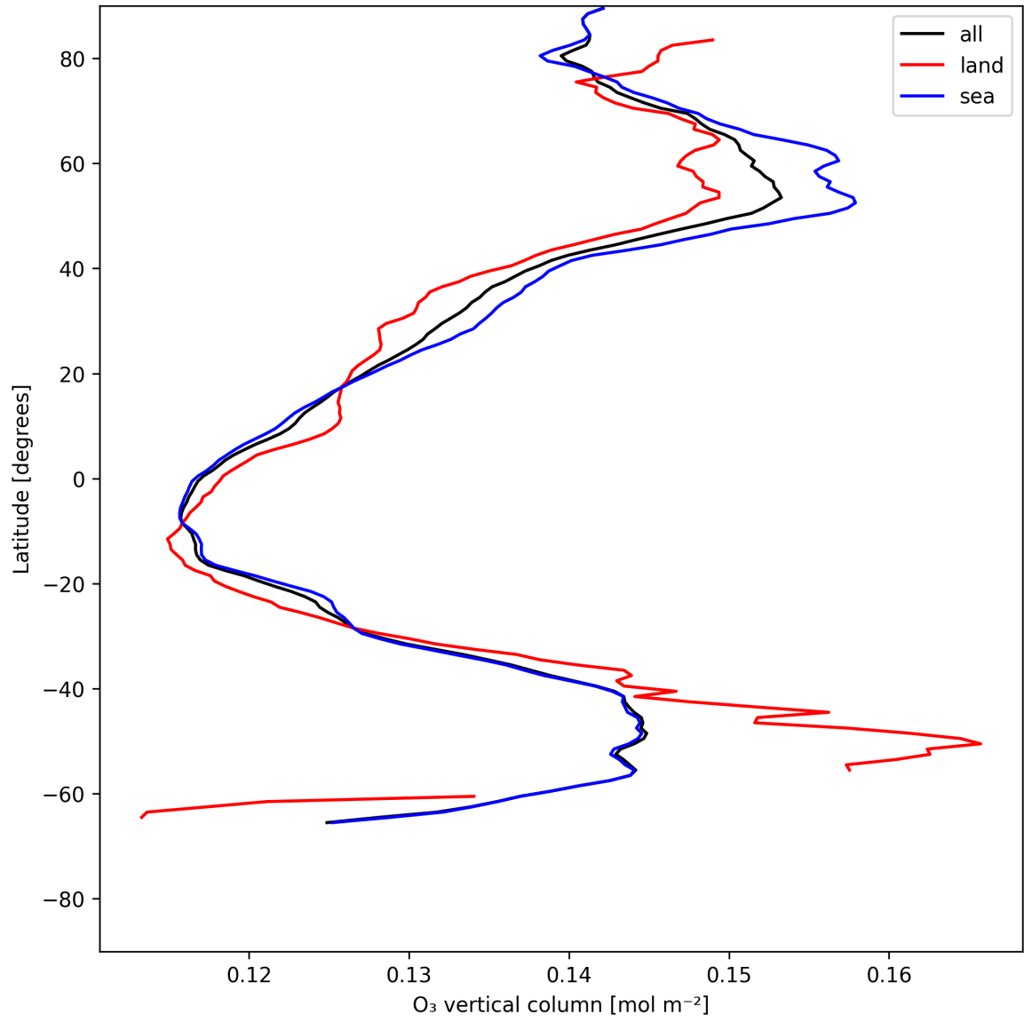
Figure 17: Zonal average of “O 3 vertical column” for 2025-06-27 to 2025-06-28.
