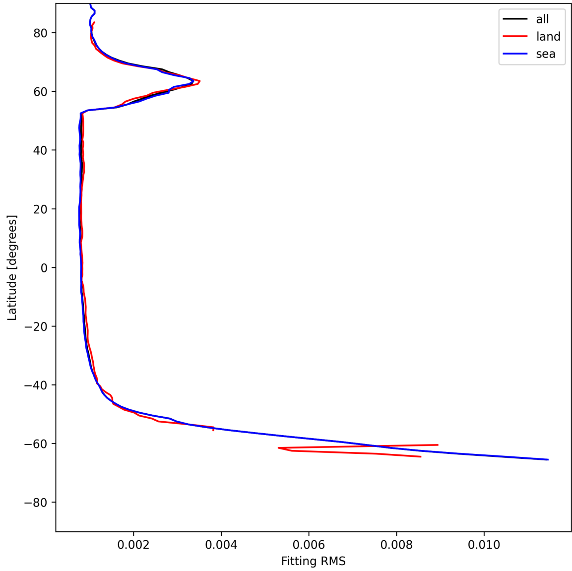
Figure 22: Zonal average of “Fitting RMS” for 2025-06-27 to 2025-06-28.
