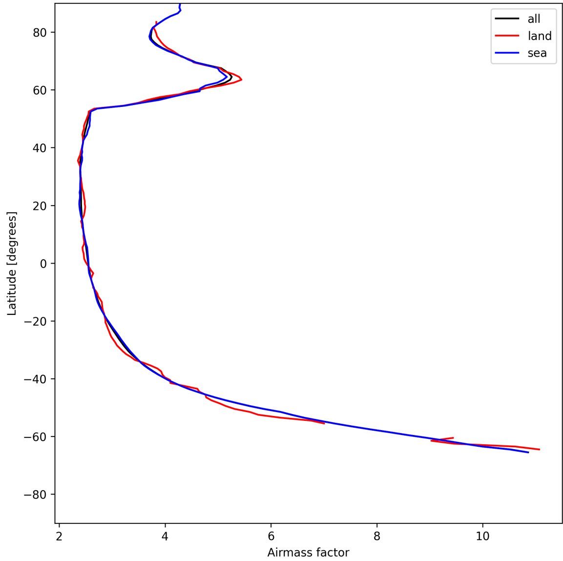
Figure 25: Zonal average of “Airmass factor” for 2025-06-27 to 2025-06-28.
