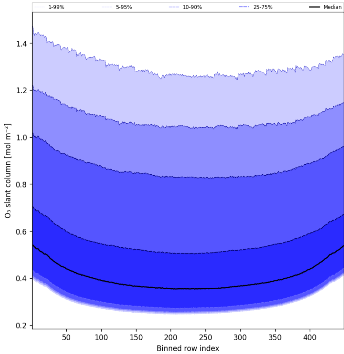
Figure 43: Along track statistics of “O 3 slant column” for 2025-06-27 to 2025-06-28
