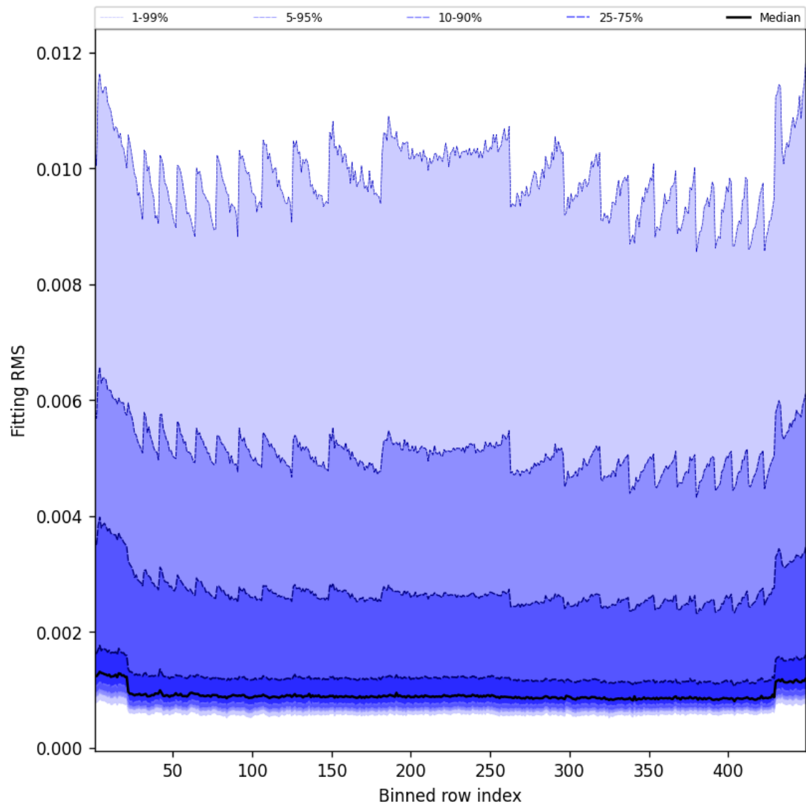
Figure 46: Along track statistics of “Fitting RMS” for 2025-06-27 to 2025-06-28
