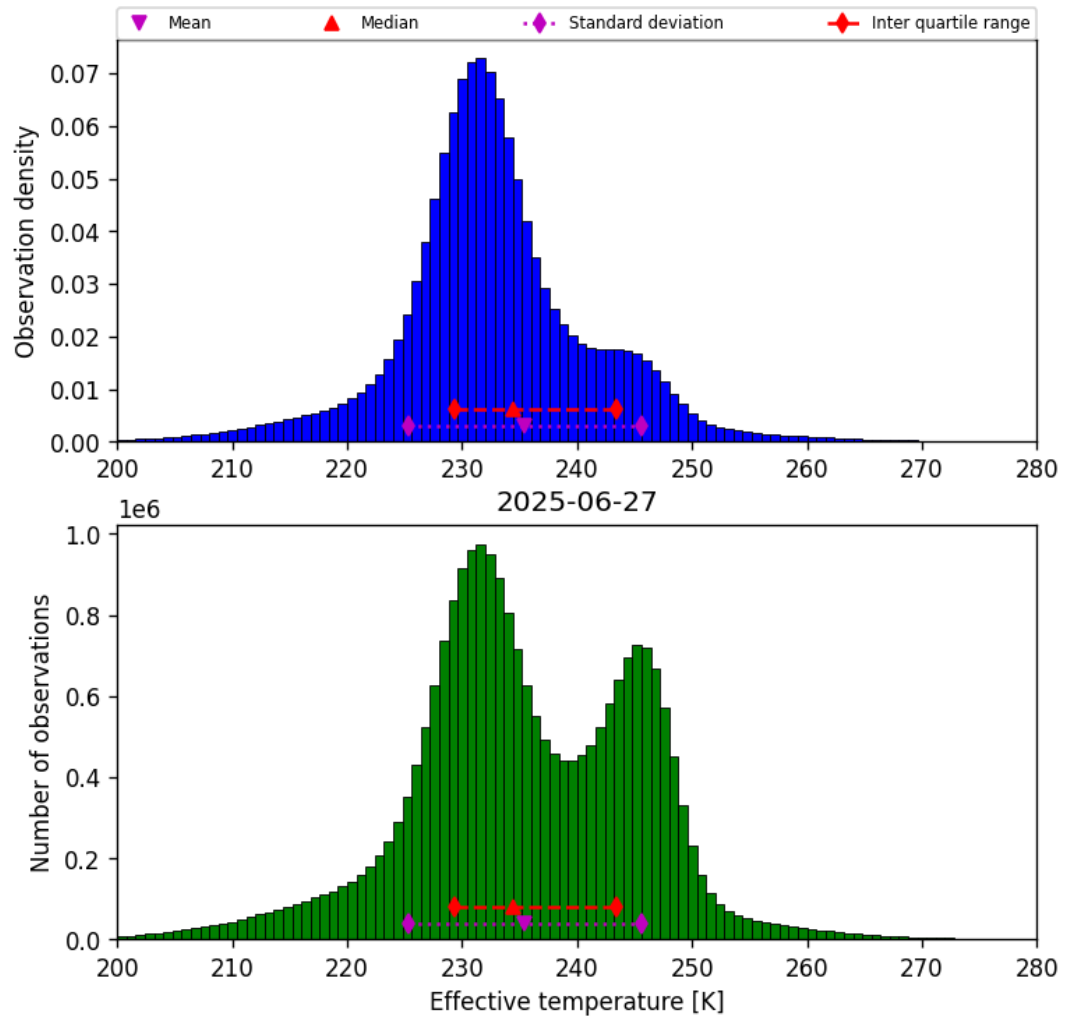
Figure 38: Histogram of “Effective temperature” for 2025-06-27 to 2025-06-28
