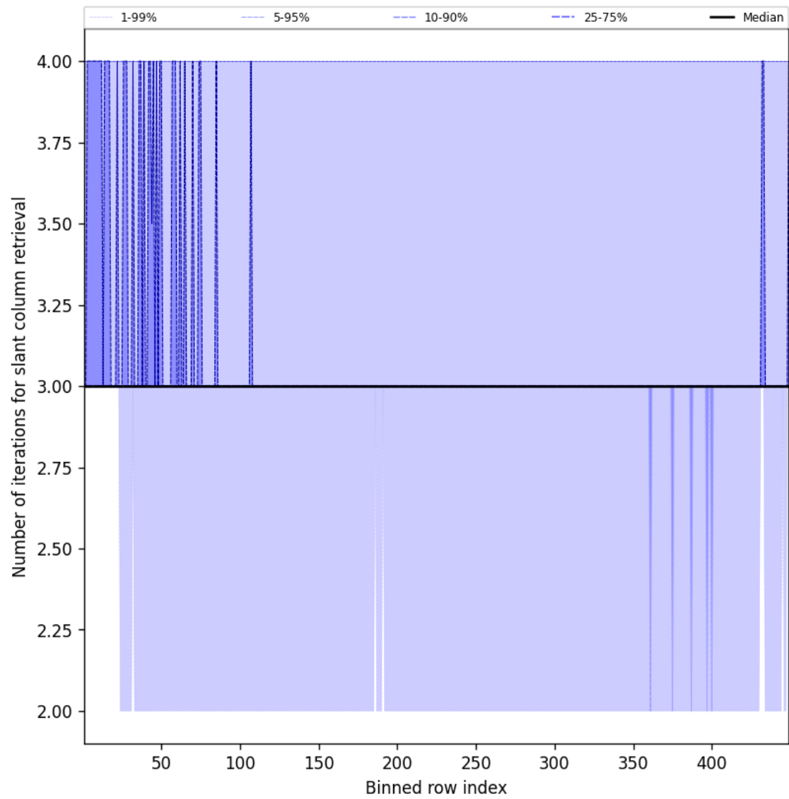
Figure 45: Along track statistics of “Number of iterations for slant column retrieval” for 2025-06-27 to 2025-06-28
