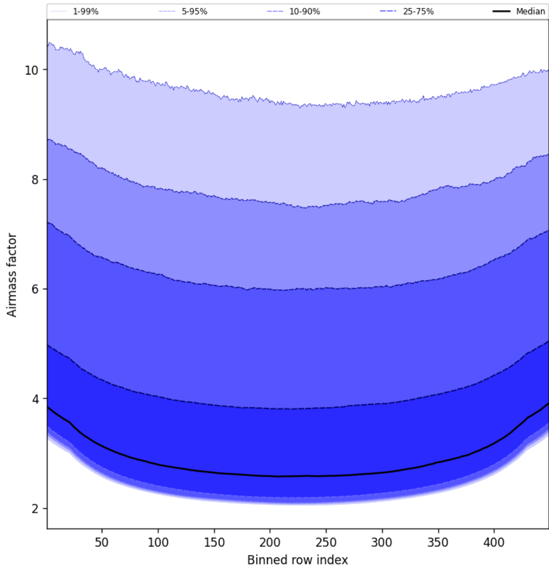
Figure 49: Along track statistics of “Airmass factor” for 2025-06-27 to 2025-06-28
