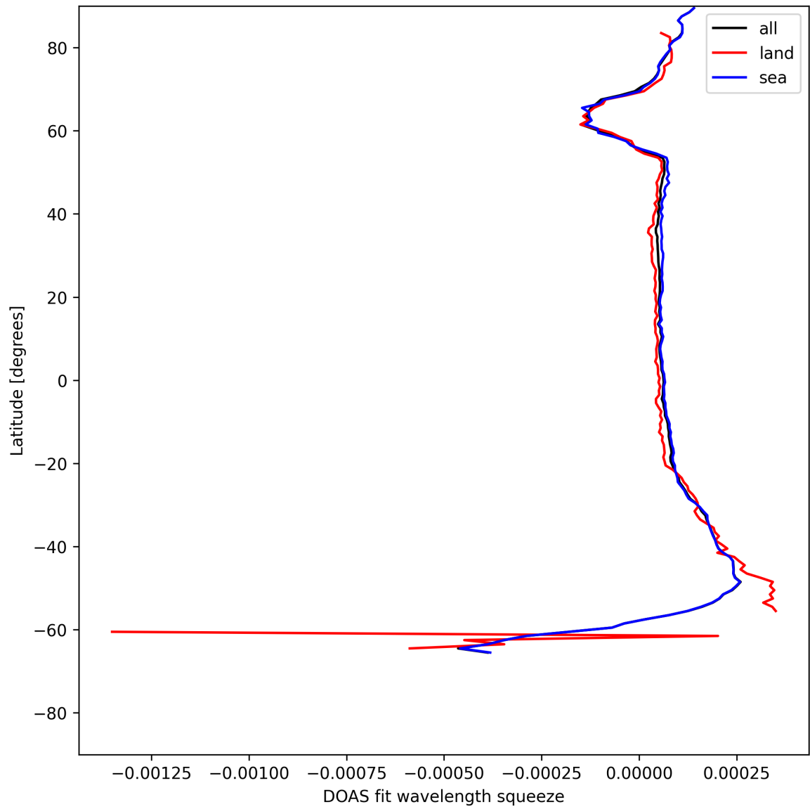
Figure 24: Zonal average of “DOAS fit wavelength squeeze” for 2025-06-27 to 2025-06-28.
