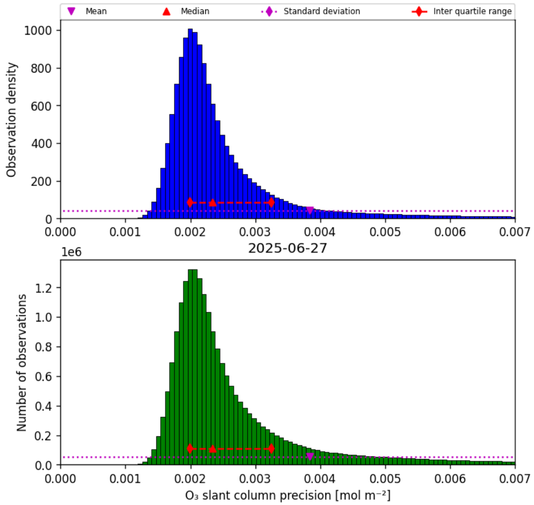
Figure 32: Histogram of “O 3 slant column precision” for 2025-06-27 to 2025-06-28
