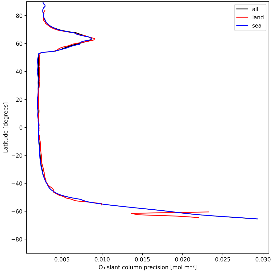
Figure 20: Zonal average of “O 3 slant column precision” for 2025-06-27 to 2025-06-28.
