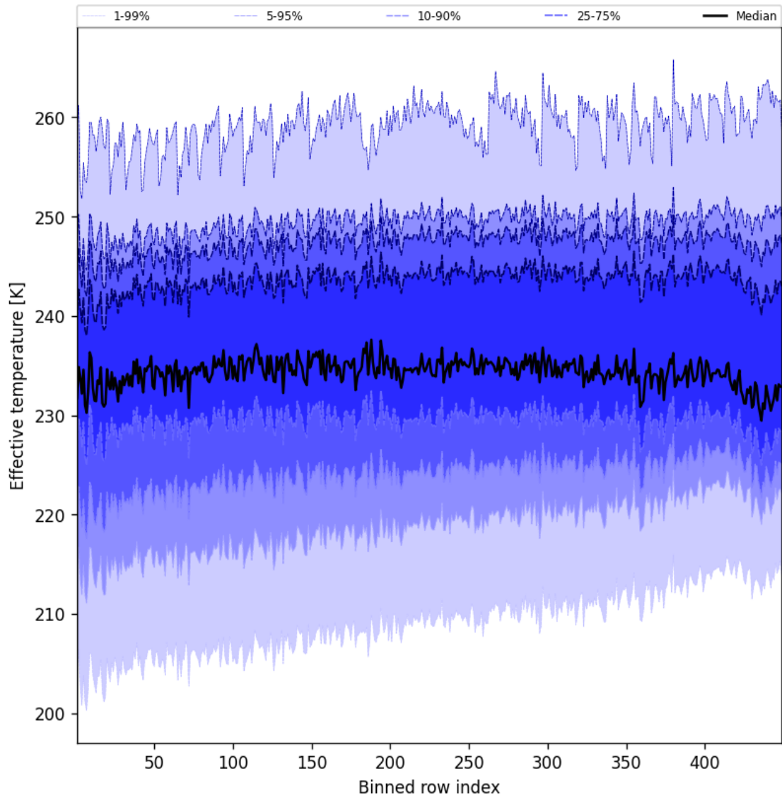
Figure 50: Along track statistics of “Effective temperature” for 2025-06-27 to 2025-06-28
