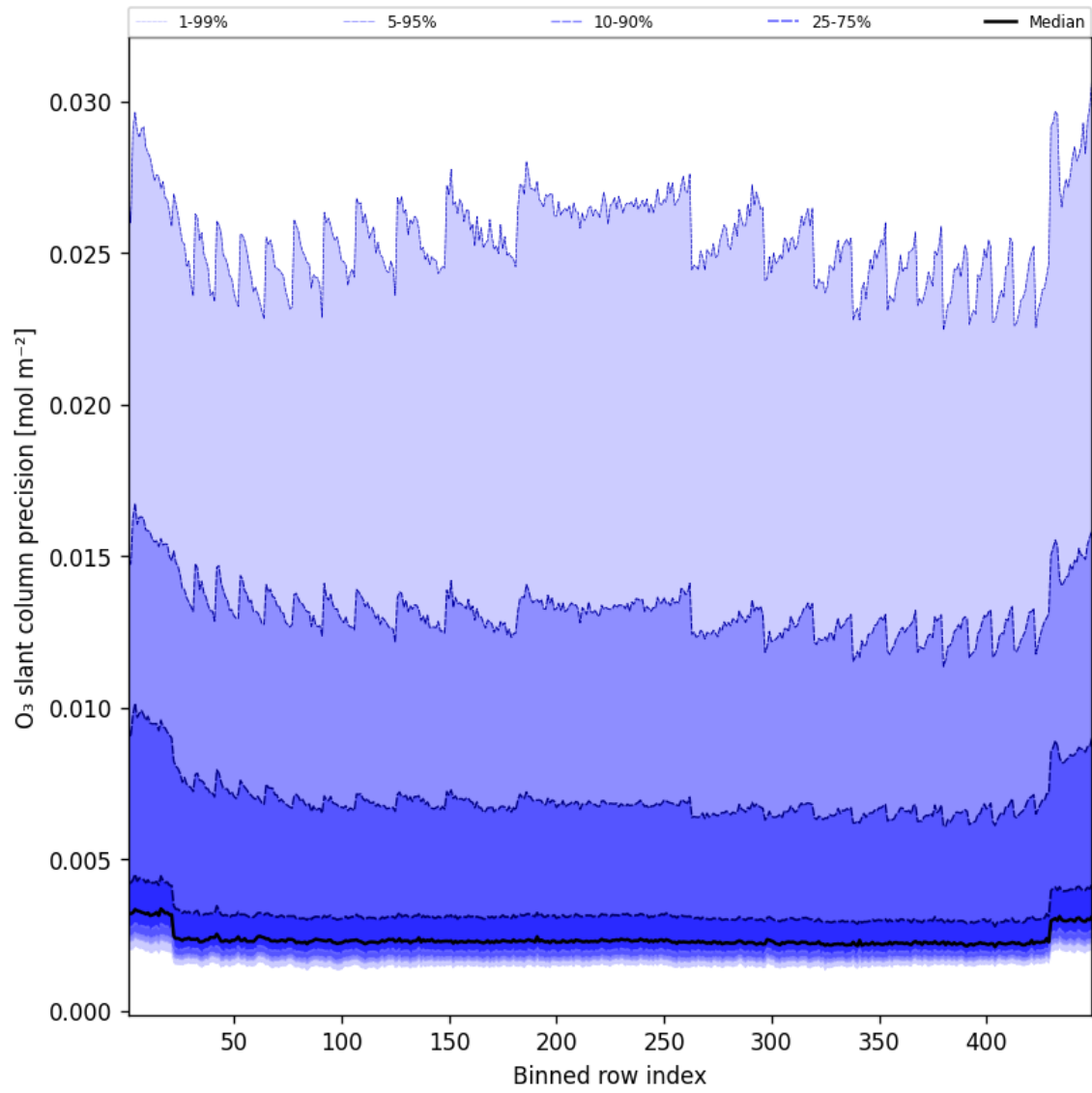
Figure 44: Along track statistics of “O 3 slant column precision” for 2025-06-27 to 2025-06-28
