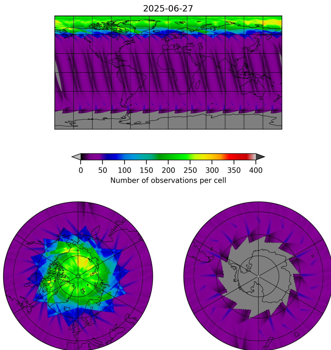
Figure 15: Map of the number of observations for 2025-06-27 to 2025-06-28
