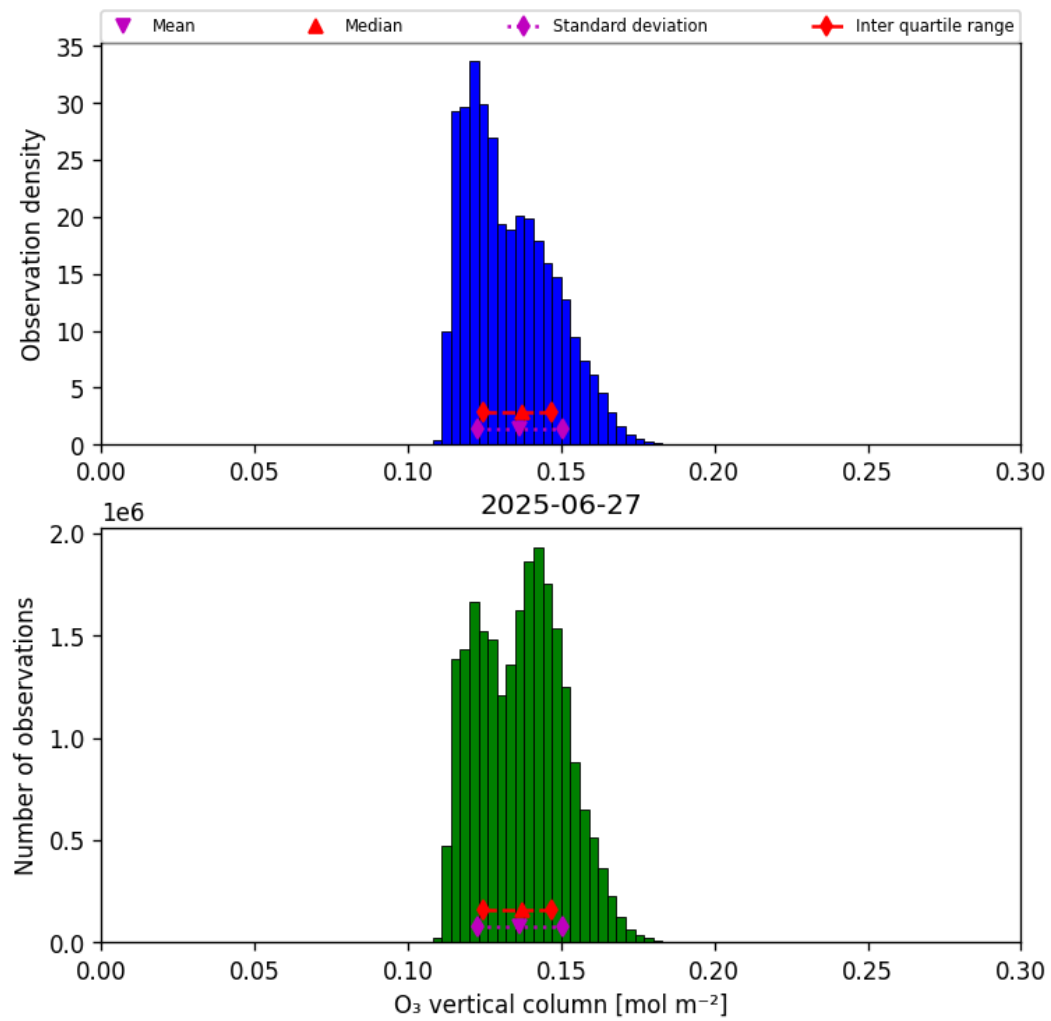
Figure 29: Histogram of “O 3 vertical column” for 2025-06-27 to 2025-06-28
