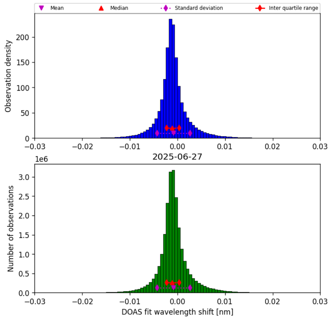
Figure 35: Histogram of “DOAS fit wavelength shift” for 2025-06-27 to 2025-06-28
