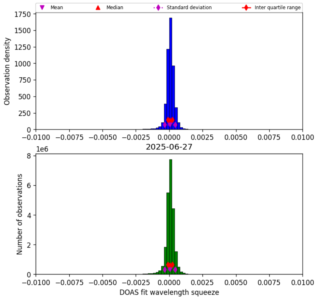
Figure 36: Histogram of “DOAS fit wavelength squeeze” for 2025-06-27 to 2025-06-28
