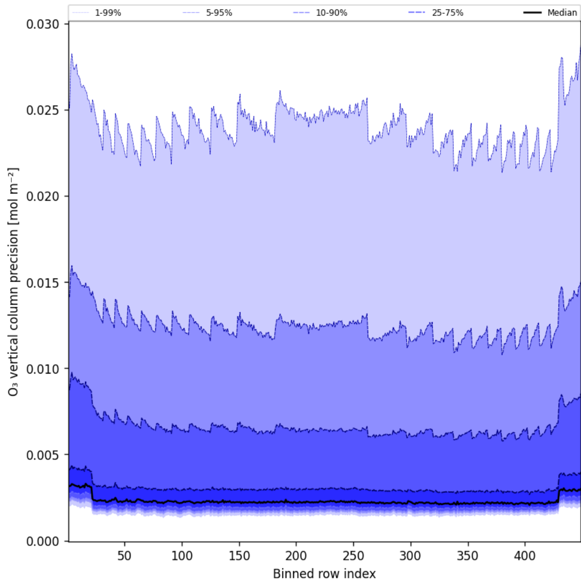
Figure 42: Along track statistics of “O 3 vertical column precision” for 2025-06-27 to 2025-06-28
