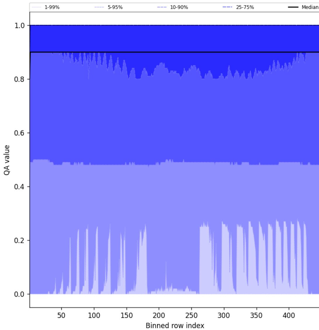
Figure 40: Along track statistics of “QA value” for 2025-06-27 to 2025-06-28
