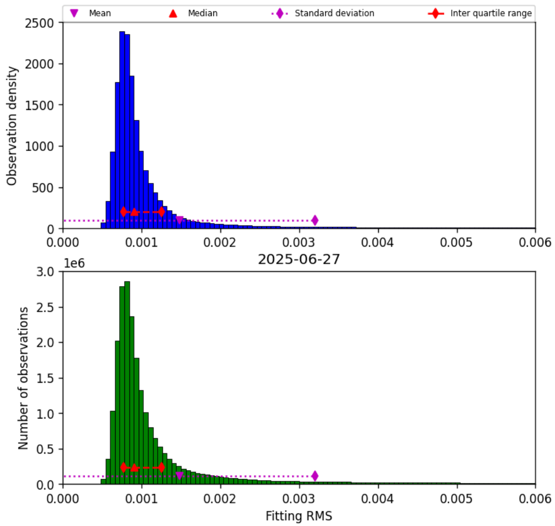
Figure 34: Histogram of “Fitting RMS” for 2025-06-27 to 2025-06-28
