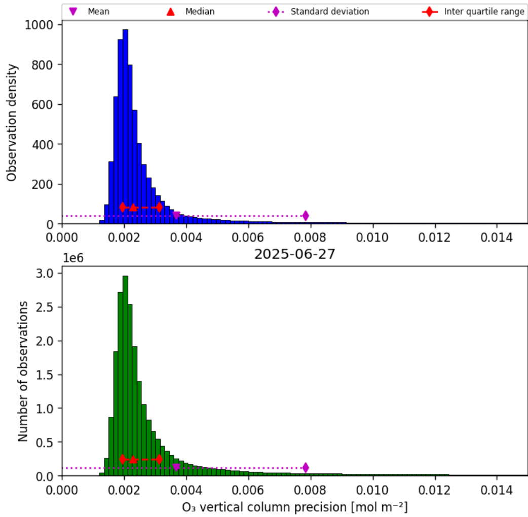
Figure 30: Histogram of “O 3 vertical column precision” for 2025-06-27 to 2025-06-28
