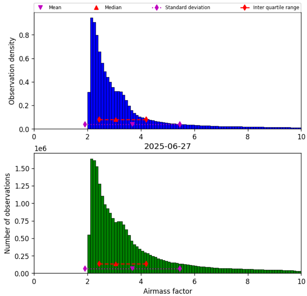
Figure 37: Histogram of “Airmass factor” for 2025-06-27 to 2025-06-28
