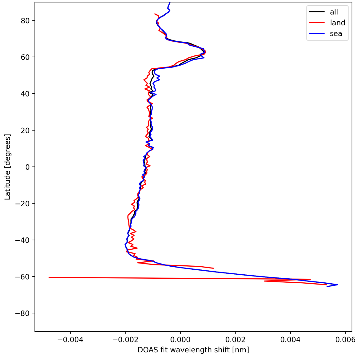
Figure 23: Zonal average of “DOAS fit wavelength shift” for 2025-06-27 to 2025-06-28.
