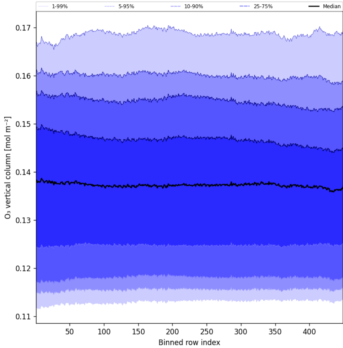
Figure 41: Along track statistics of “ O_3 vertical column” for 2025-06-27 to 2025-06-28
