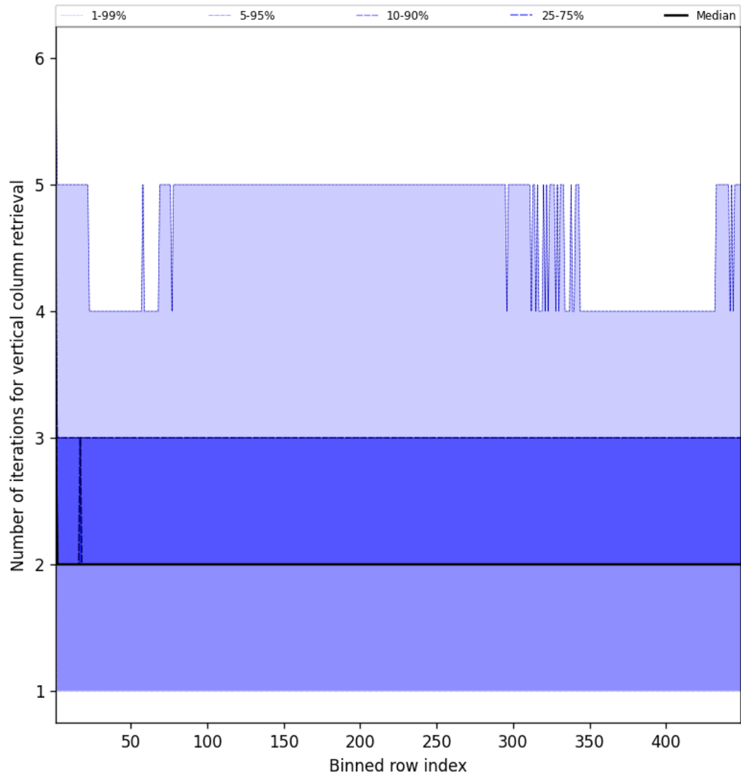
Figure 51: Along track statistics of “Number of iterations for vertical column retrieval” for 2025-06-27 to 2025-06-28
