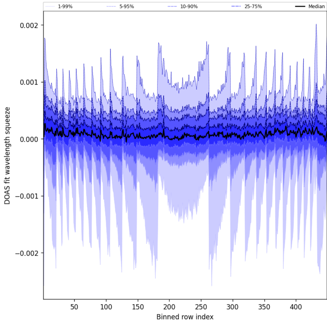
Figure 48: Along track statistics of “DOAS fit wavelength squeeze” for 2025-06-27 to 2025-06-28
