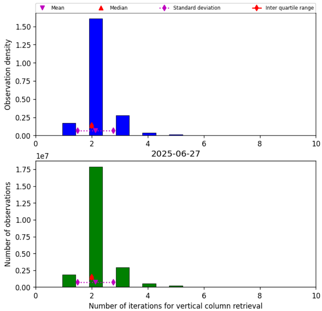
Figure 39: Histogram of “Number of iterations for vertical column retrieval” for 2025-06-27 to 2025-06-28
