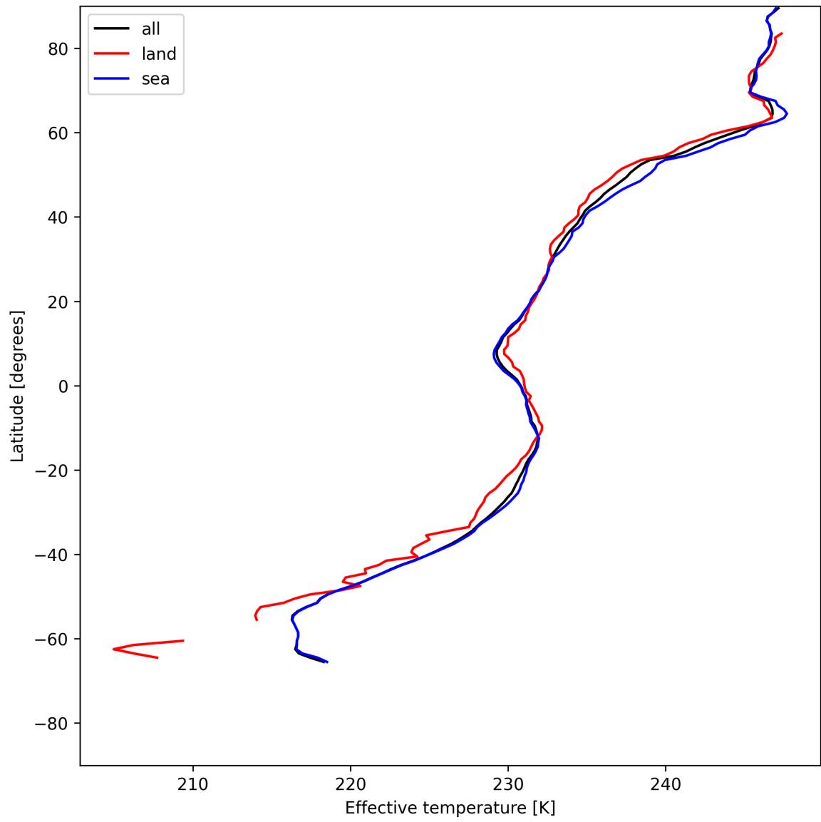
Figure 26: Zonal average of "Effective temperature" for 2025-06-27 to 2025-06-28.
