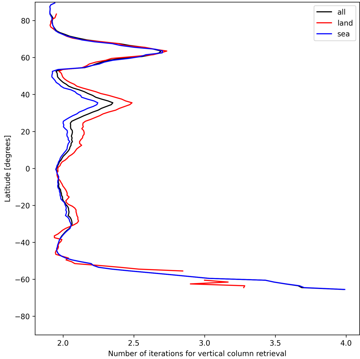
Figure 27: Zonal average of “Number of iterations for vertical column retrieval” for 2025-06-27 to 2025-06-28.
