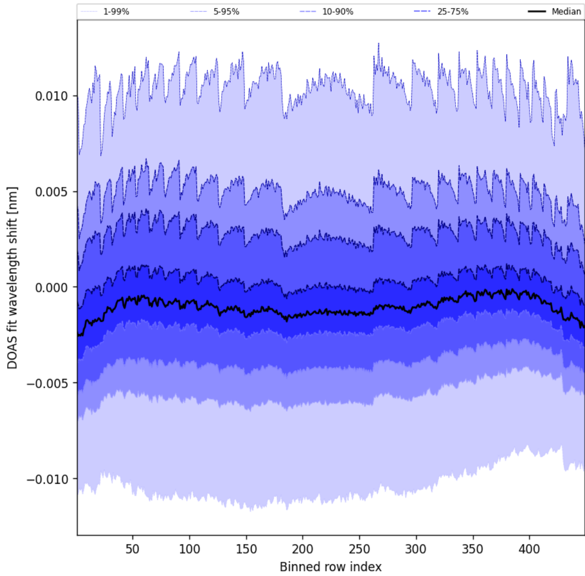
Figure 47: Along track statistics of “DOAS fit wavelength shift” for 2025-06-27 to 2025-06-28
