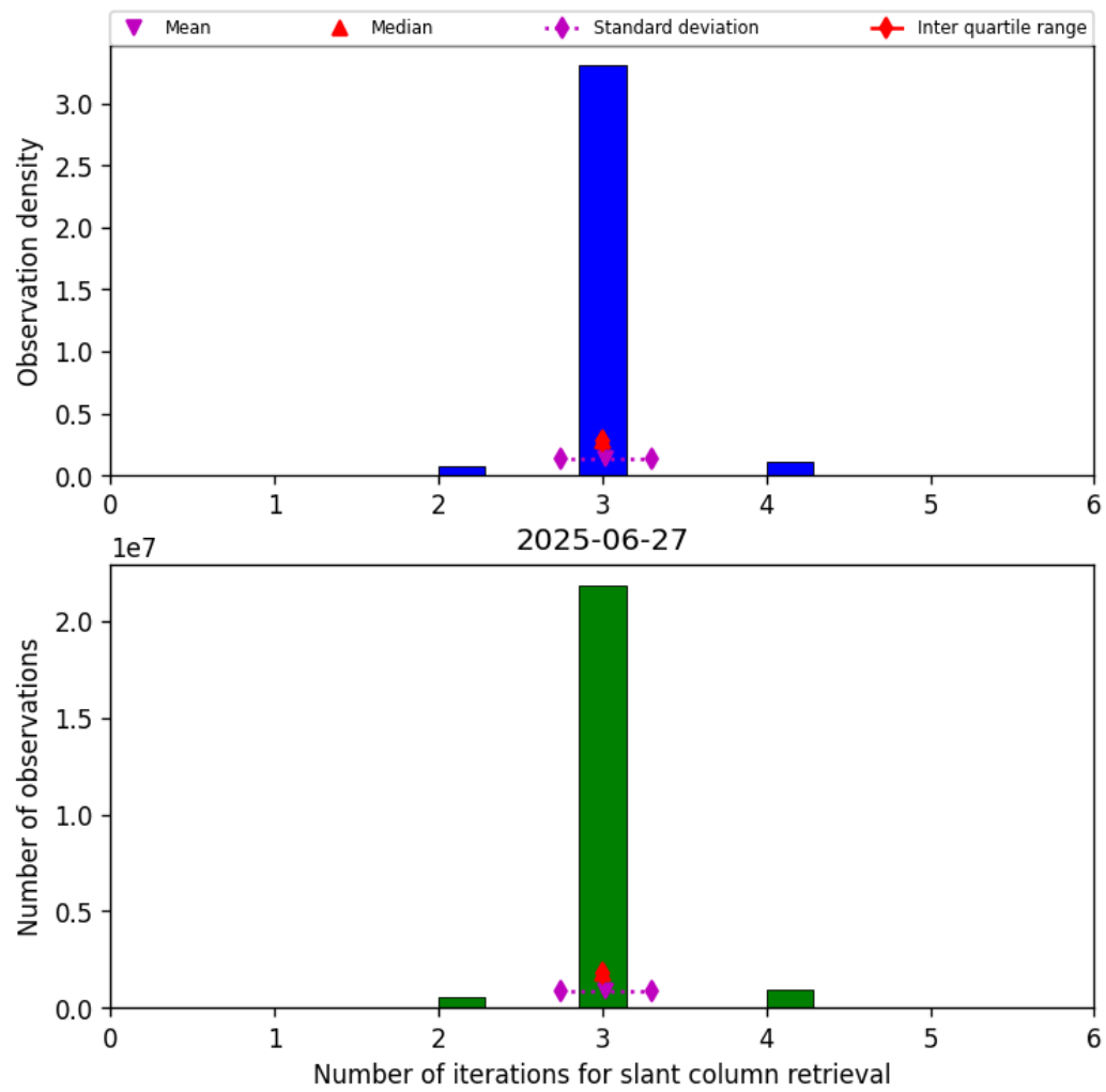
Figure 33: Histogram of “Number of iterations for slant column retrieval” for 2025-06-27 to 2025-06-28
