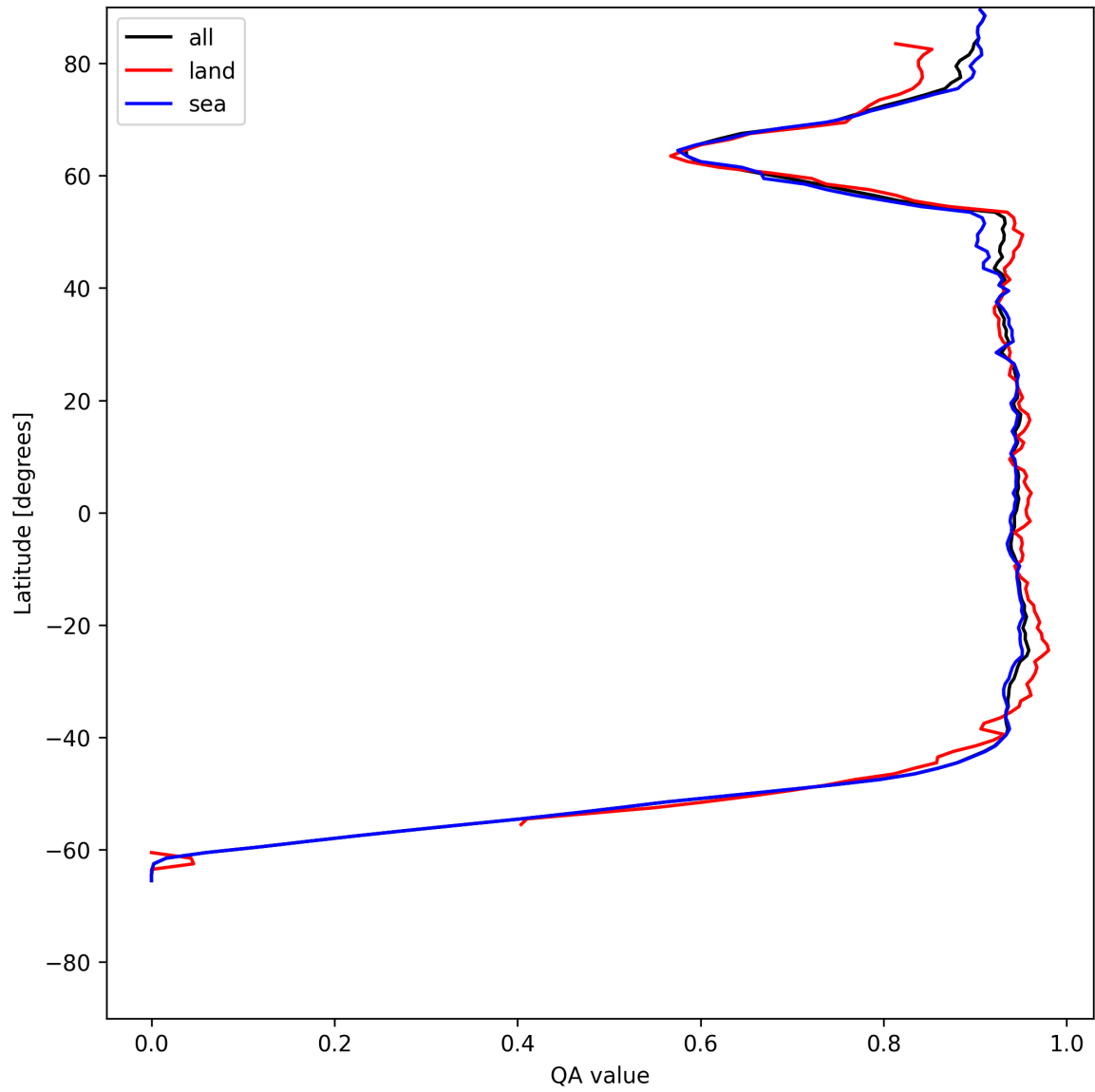
Figure 16: Zonal average of “QA value” for 2025-06-27 to 2025-06-28.
