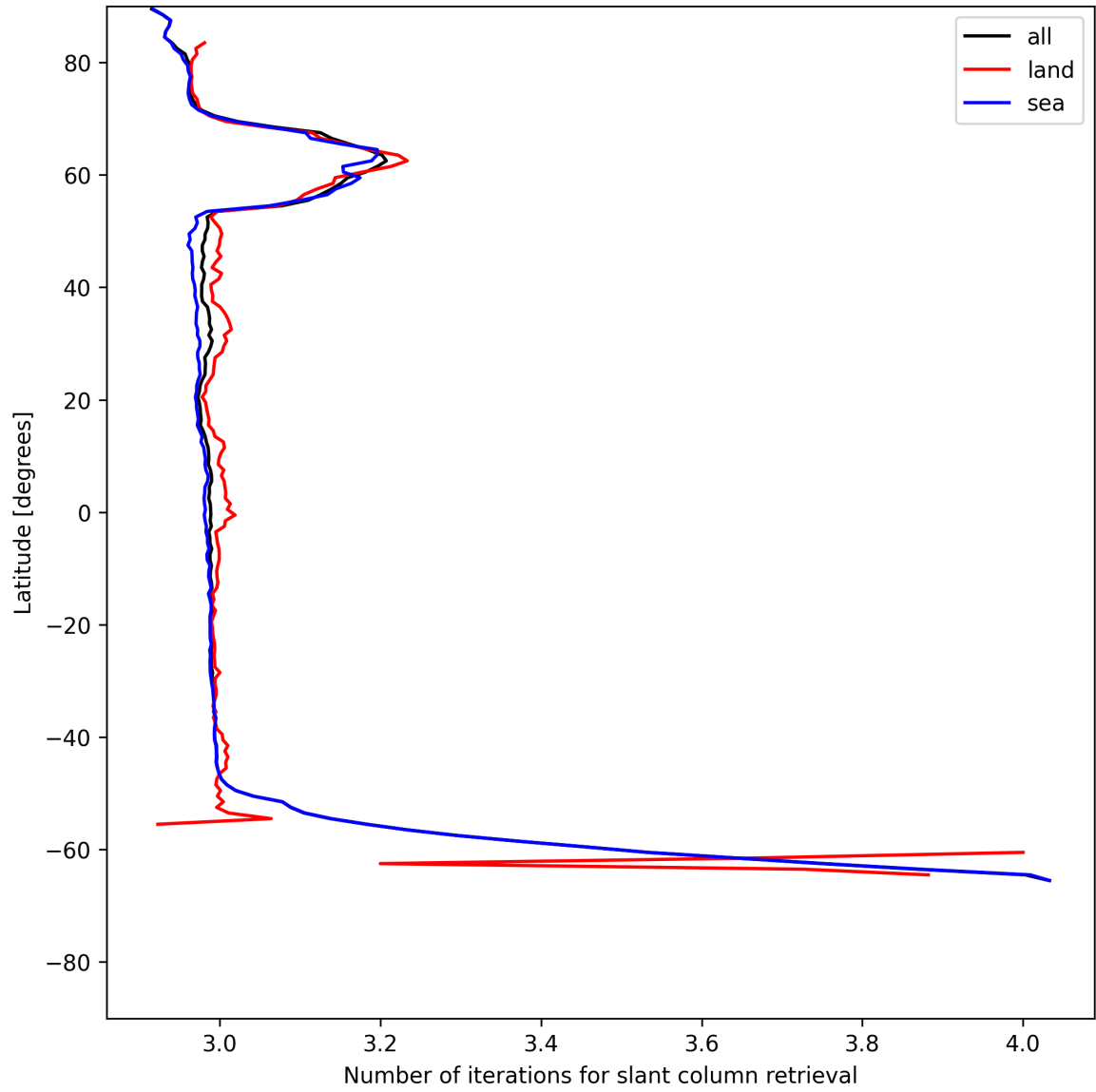
Figure 21: Zonal average of “Number of iterations for slant column retrieval” for 2025-06-27 to 2025-06-28.
