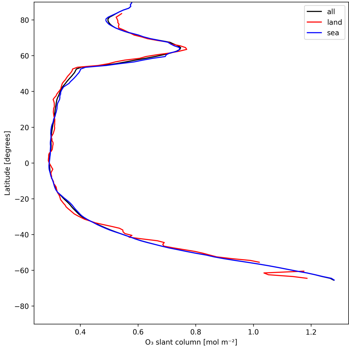
Figure 19: Zonal average of “O 3 slant column” for 2025-06-27 to 2025-06-28.
