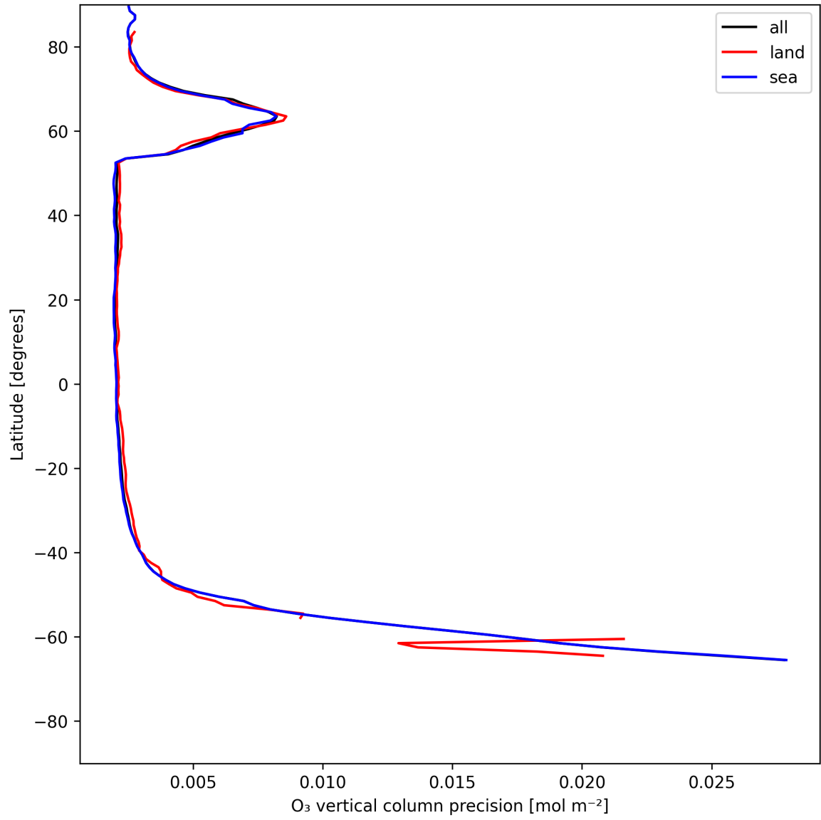
Figure 18: Zonal average of “O 3 vertical column precision” for 2025-06-27 to 2025-06-28.
