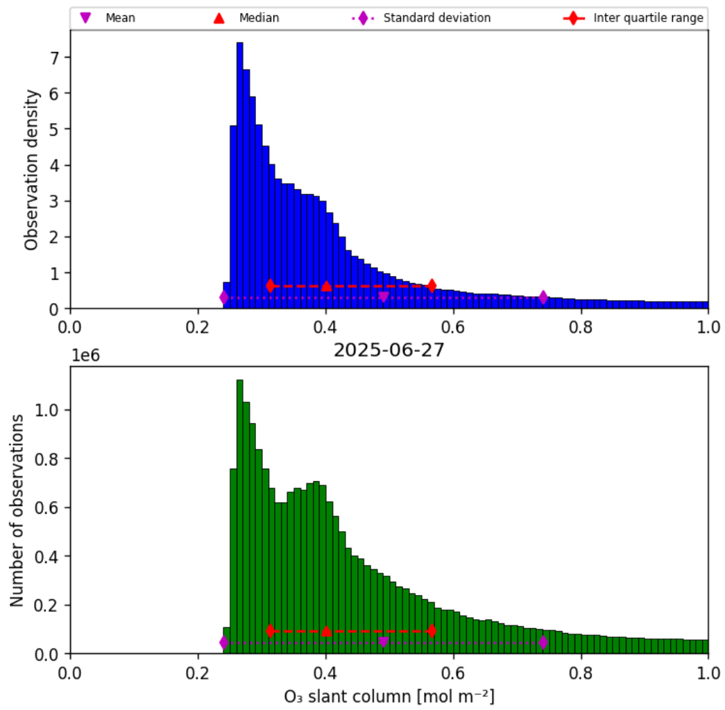
Figure 31: Histogram of “O 3 slant column” for 2025-06-27 to 2025-06-28
