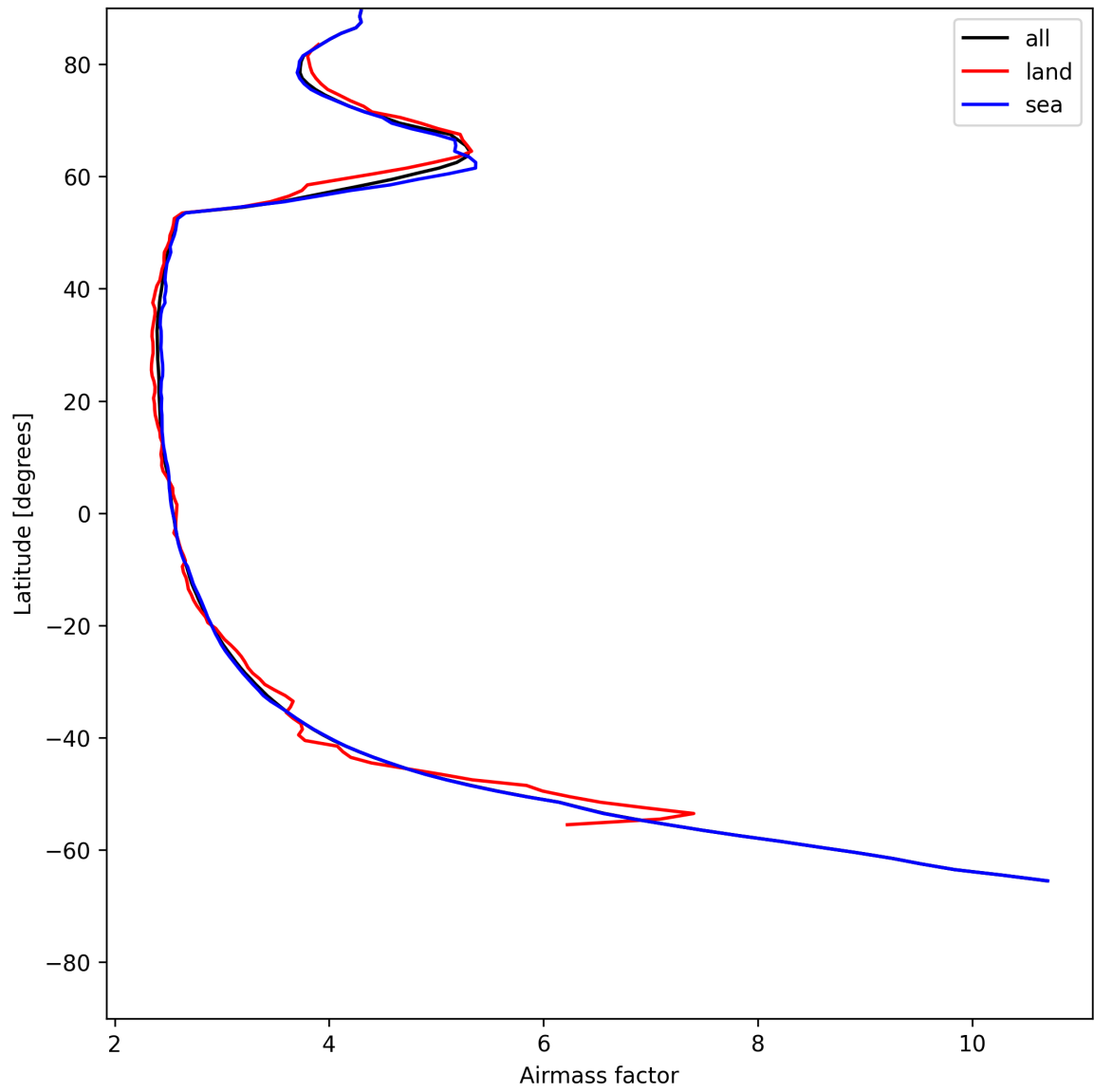
Figure 25: Zonal average of “Airmass factor” for 2025-06-29 to 2025-06-30.
