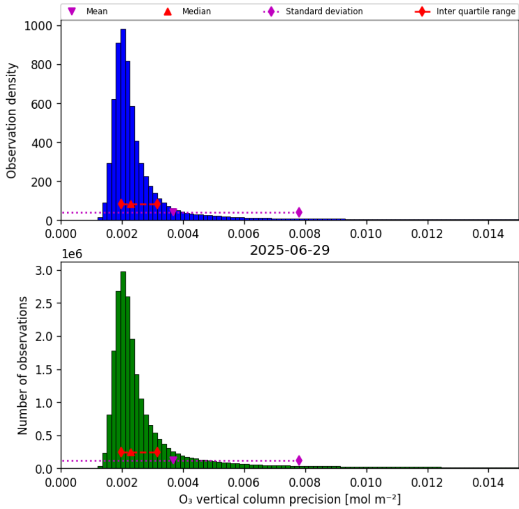
Figure 30: Histogram of “O 3 vertical column precision” for 2025-06-29 to 2025-06-30
