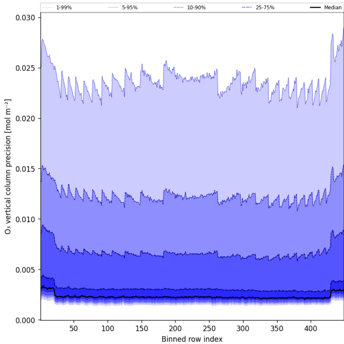
Figure 42: Along track statistics of “O 3 vertical column precision” for 2025-06-29 to 2025-06-30
