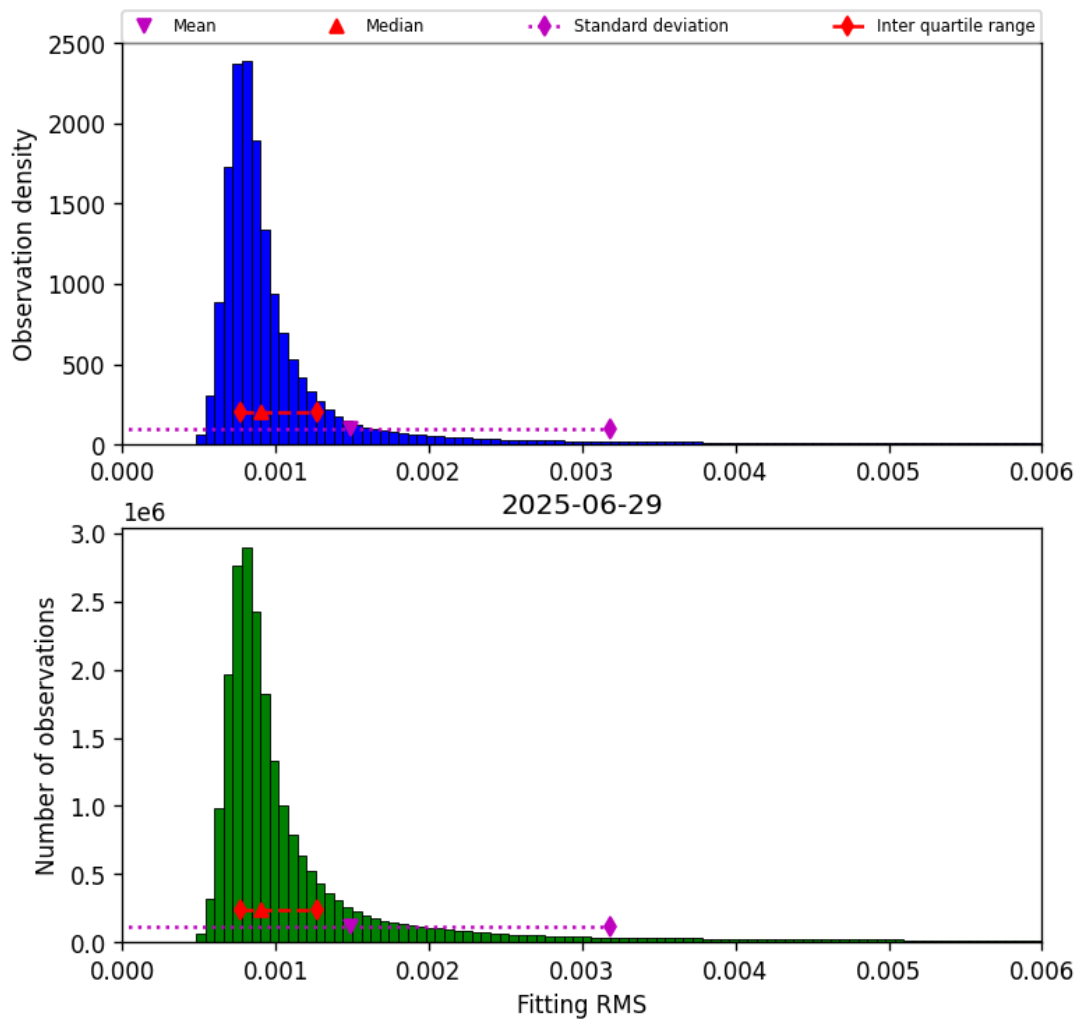
Figure 34: Histogram of “Fitting RMS” for 2025-06-29 to 2025-06-30
