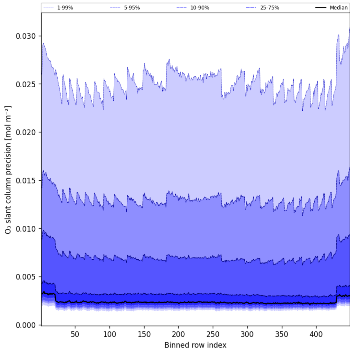
Figure 44: Along track statistics of “O 3 slant column precision” for 2025-06-29 to 2025-06-30
