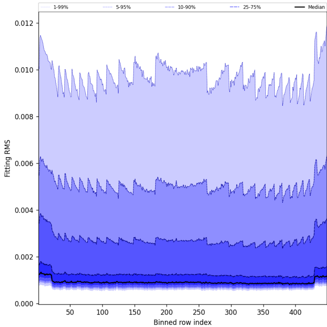
Figure 46: Along track statistics of “Fitting RMS” for 2025-06-29 to 2025-06-30
