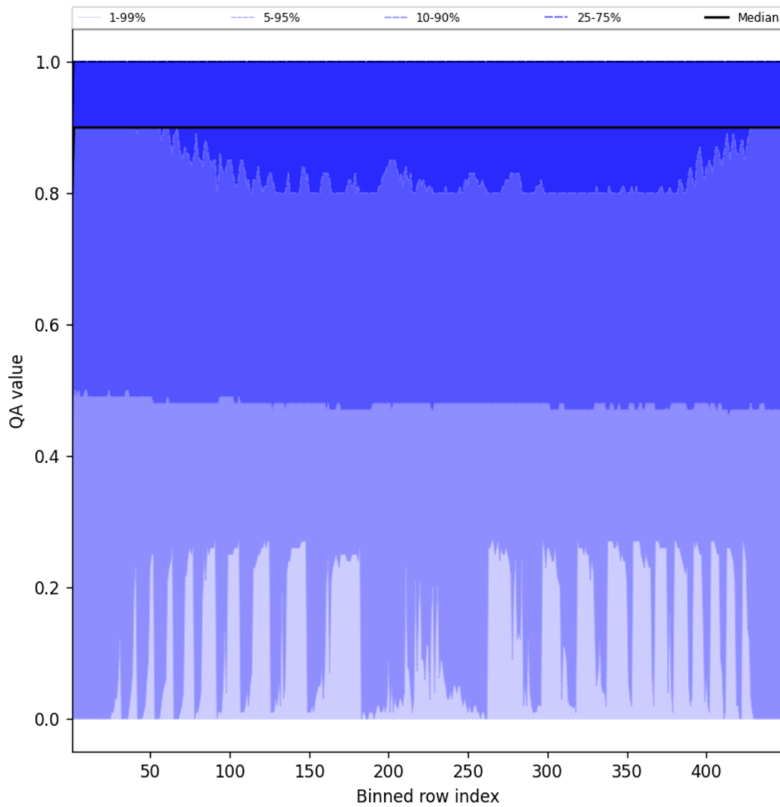
Figure 40: Along track statistics of “QA value” for 2025-06-29 to 2025-06-30
