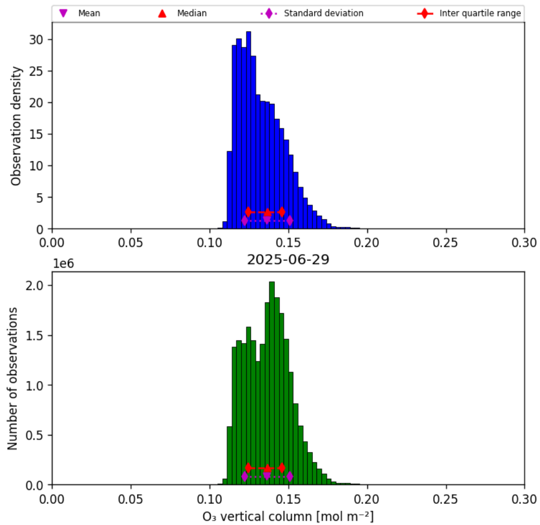
Figure 29: Histogram of “O 3 vertical column” for 2025-06-29 to 2025-06-30
