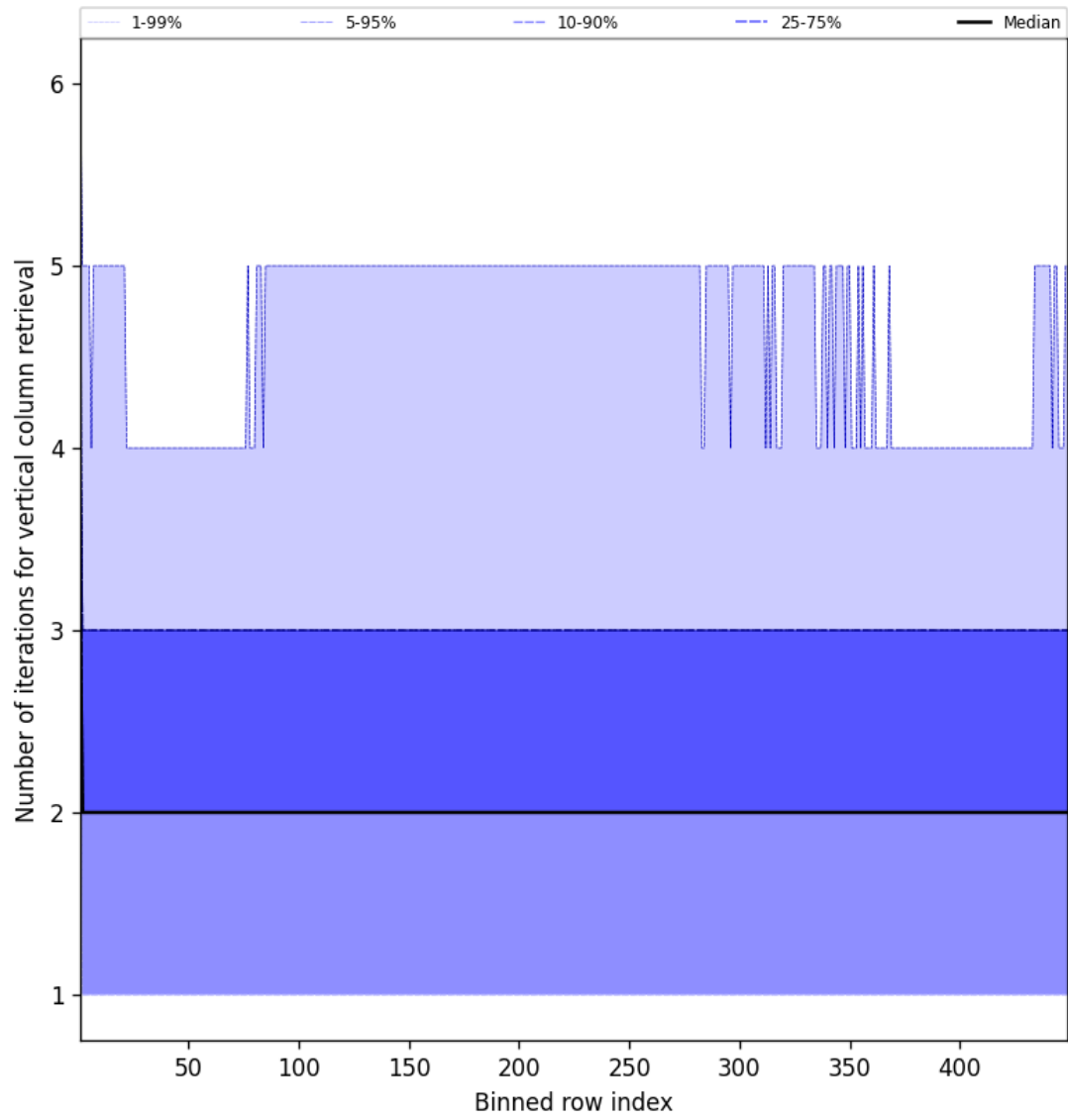
Figure 51: Along track statistics of “Number of iterations for vertical column retrieval” for 2025-06-29 to 2025-06-30
