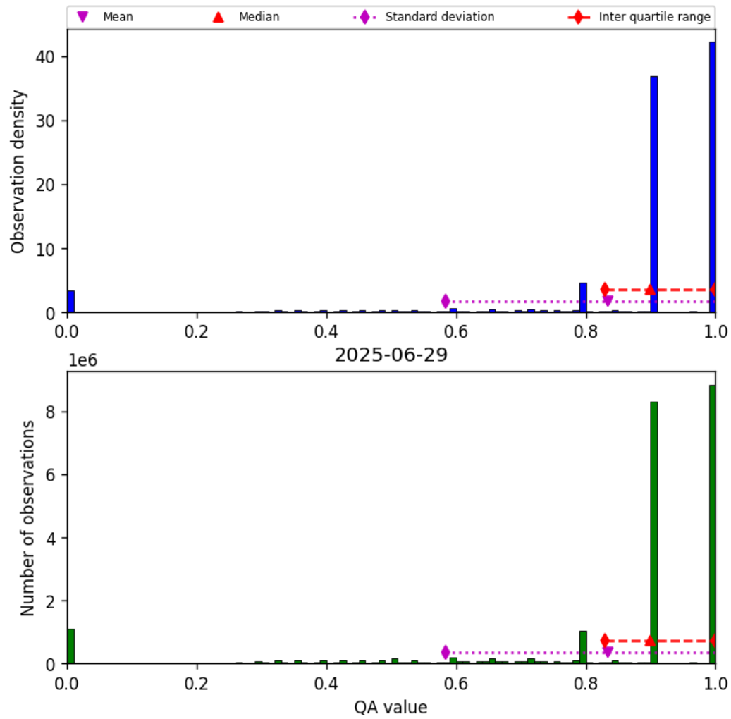
Figure 28: Histogram of “QA value” for 2025-06-29 to 2025-06-30
