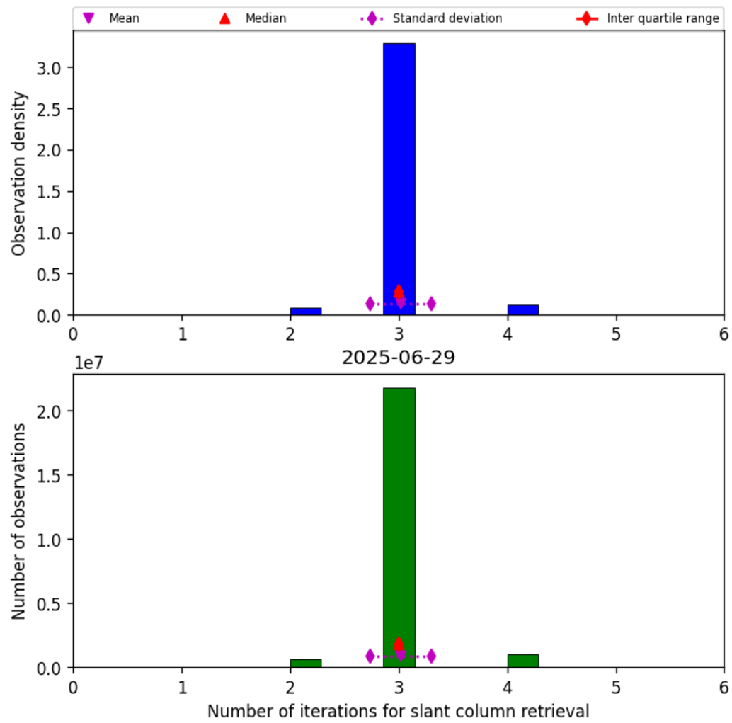
Figure 33: Histogram of "Number of iterations for slant column retrieval" for 2025-06-29 to 2025-06-30
