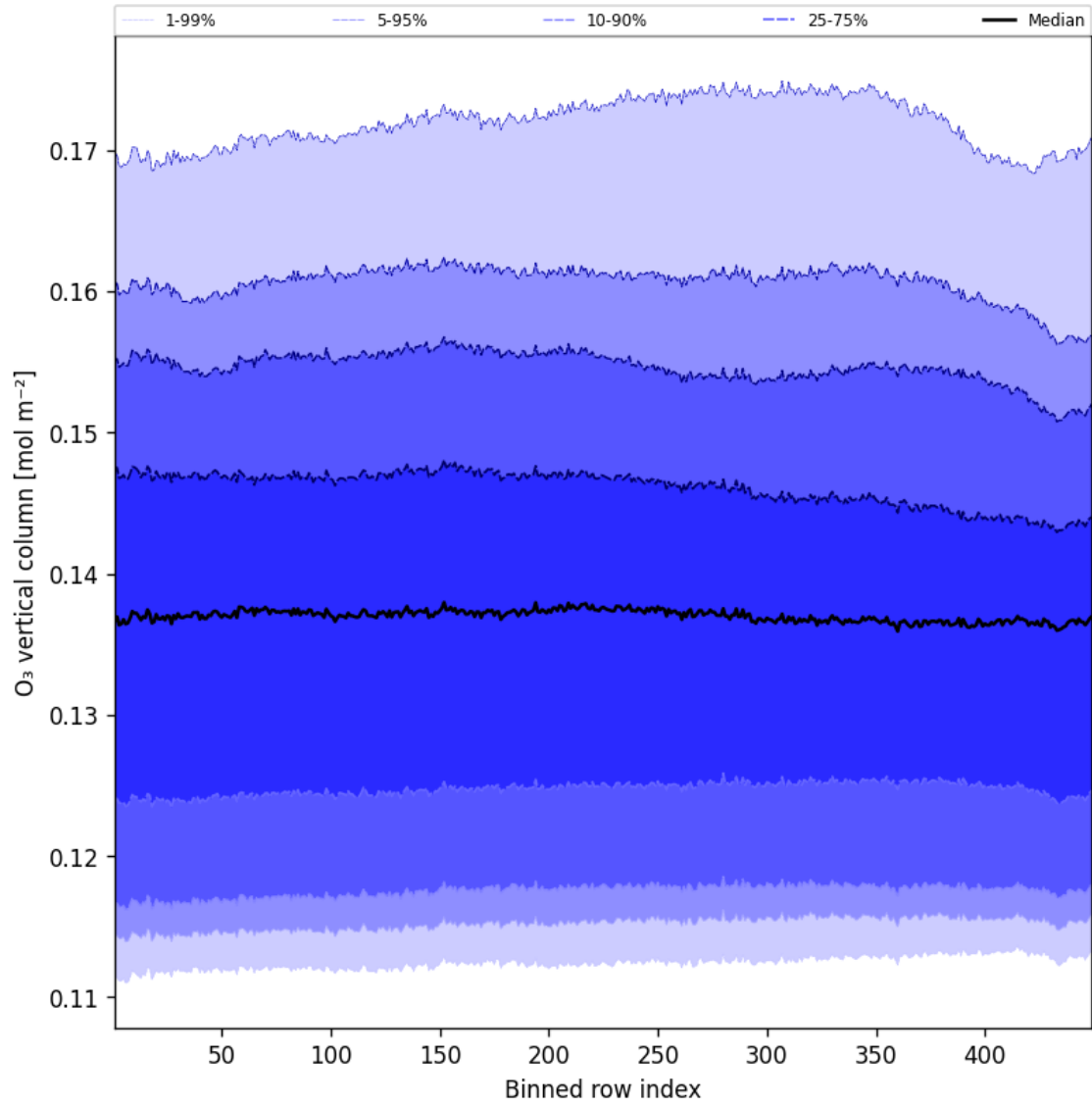
Figure 41: Along track statistics of “O 3 vertical column” for 2025-06-29 to 2025-06-30
