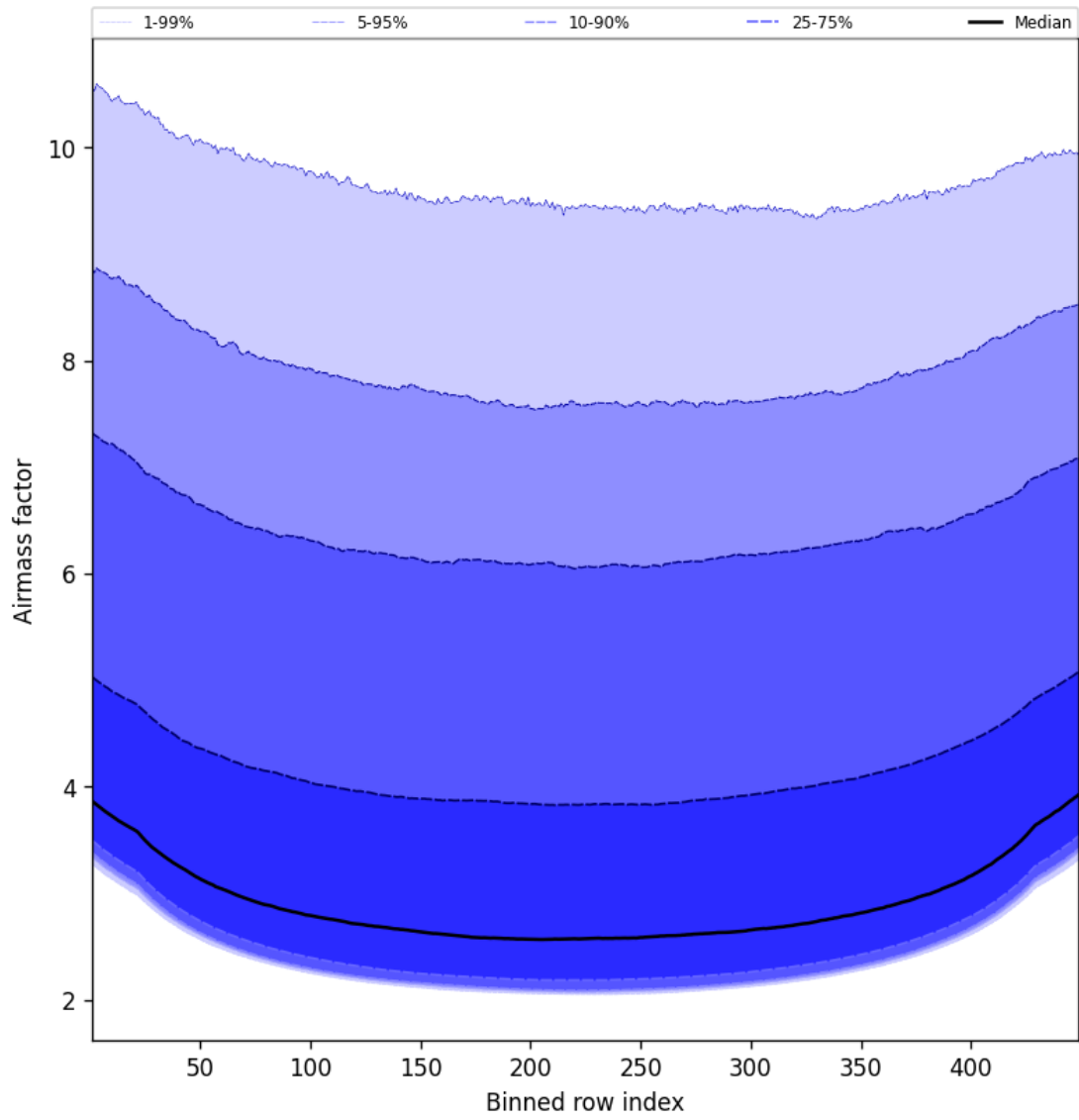
Figure 49: Along track statistics of “Airmass factor” for 2025-06-29 to 2025-06-30
