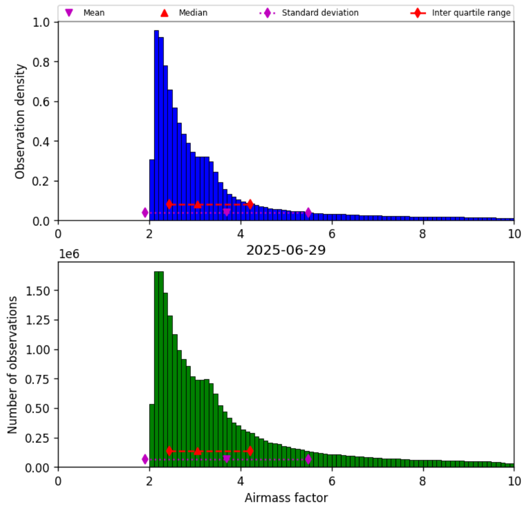
Figure 37: Histogram of “Airmass factor” for 2025-06-29 to 2025-06-30
