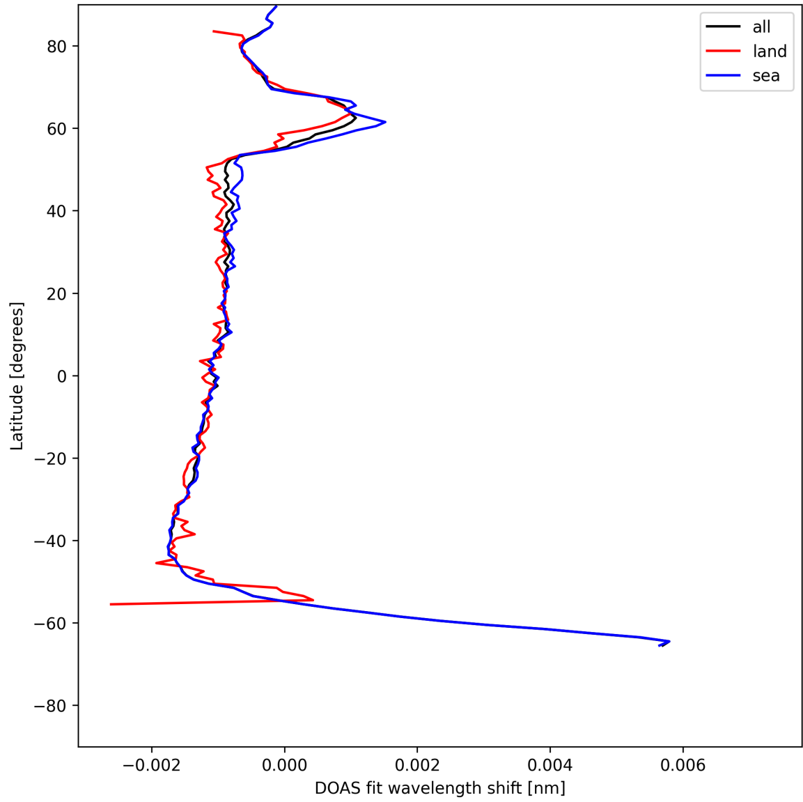
Figure 23: Zonal average of “DOAS fit wavelength shift” for 2025-06-29 to 2025-06-30.
