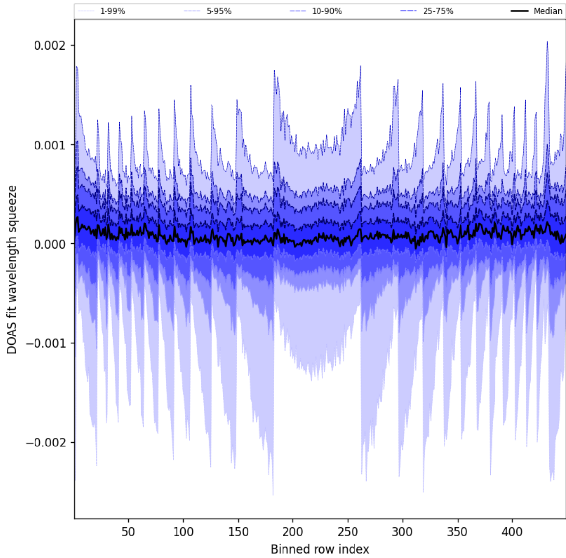
Figure 48: Along track statistics of “DOAS fit wavelength squeeze” for 2025-06-29 to 2025-06-30
