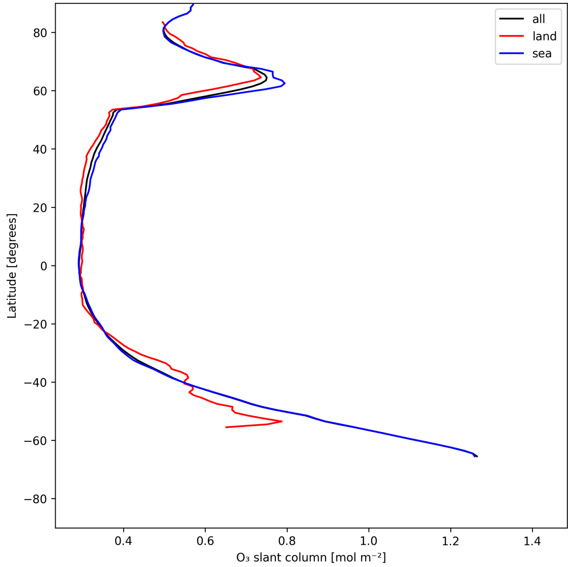
Figure 19: Zonal average of “O 3 slant column” for 2025-06-29 to 2025-06-30.
