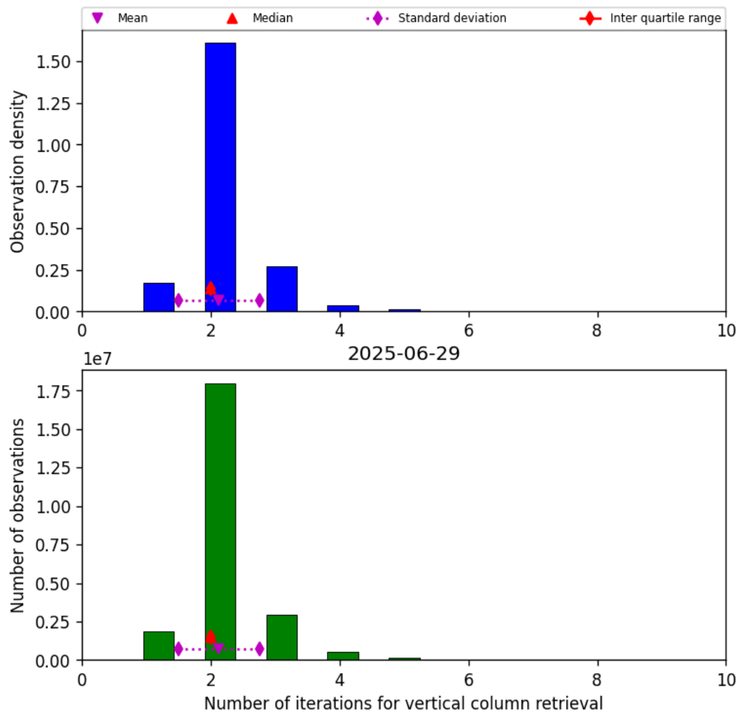
Figure 39: Histogram of “Number of iterations for vertical column retrieval” for 2025-06-29 to 2025-06-30
