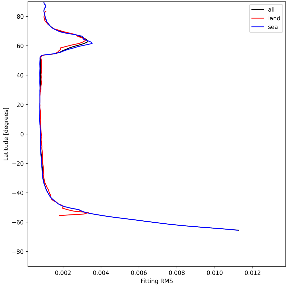
Figure 22: Zonal average of “Fitting RMS” for 2025-06-29 to 2025-06-30.
