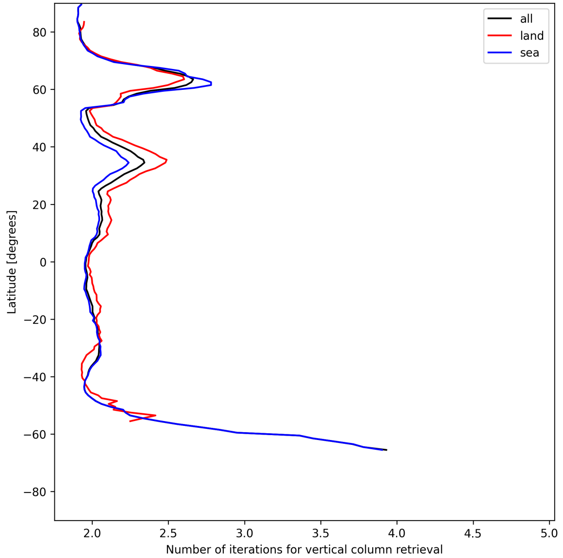
Figure 27: Zonal average of “Number of iterations for vertical column retrieval” for 2025-06-29 to 2025-06-30.
