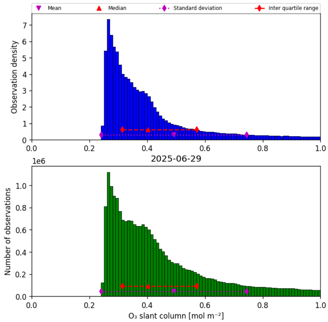
Figure 31: Histogram of “O 3 slant column” for 2025-06-29 to 2025-06-30
