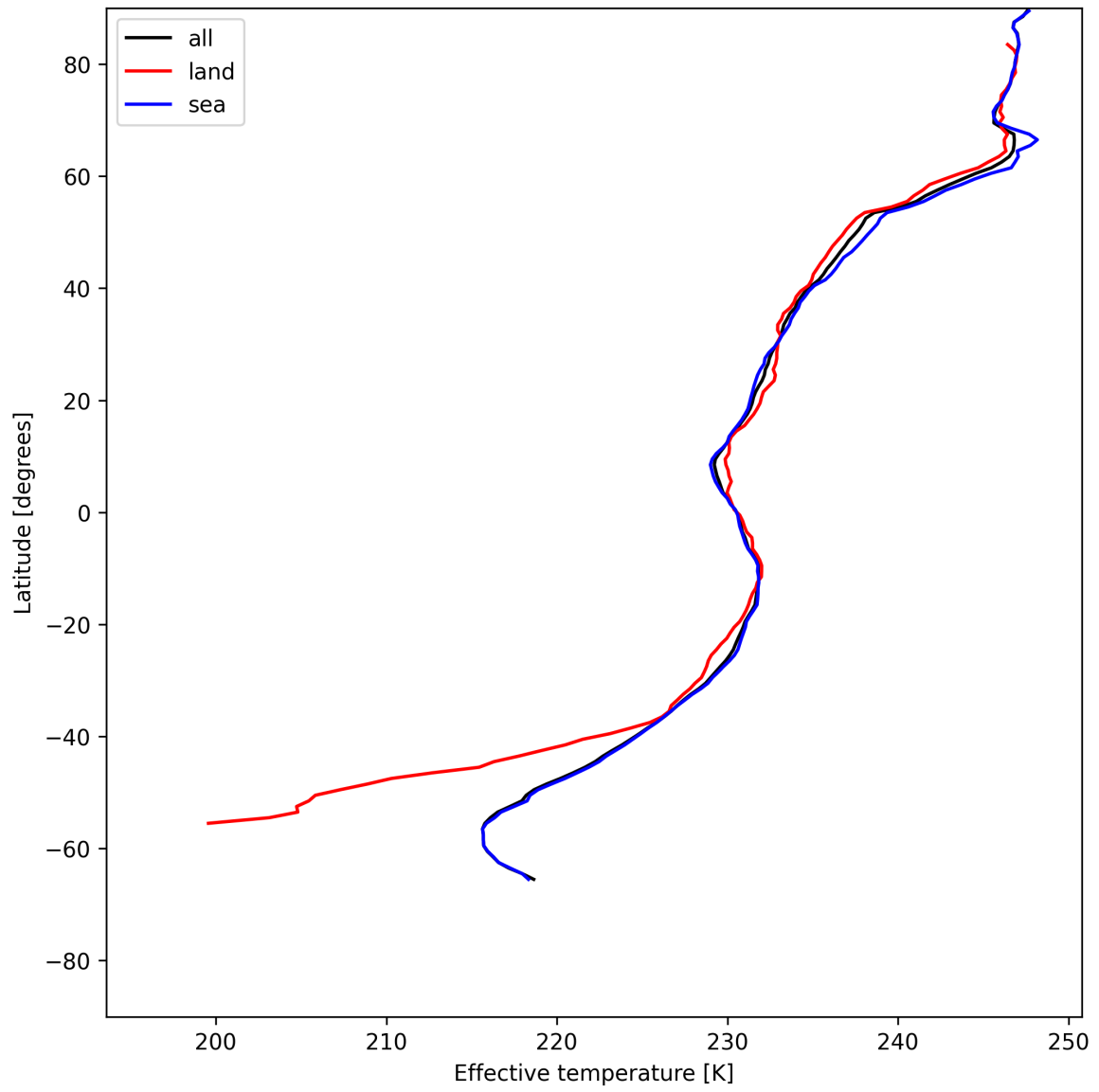
Figure 26: Zonal average of "Effective temperature" for 2025-06-29 to 2025-06-30.
