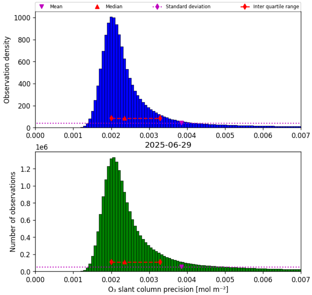
Figure 32: Histogram of “O 3 slant column precision” for 2025-06-29 to 2025-06-30
