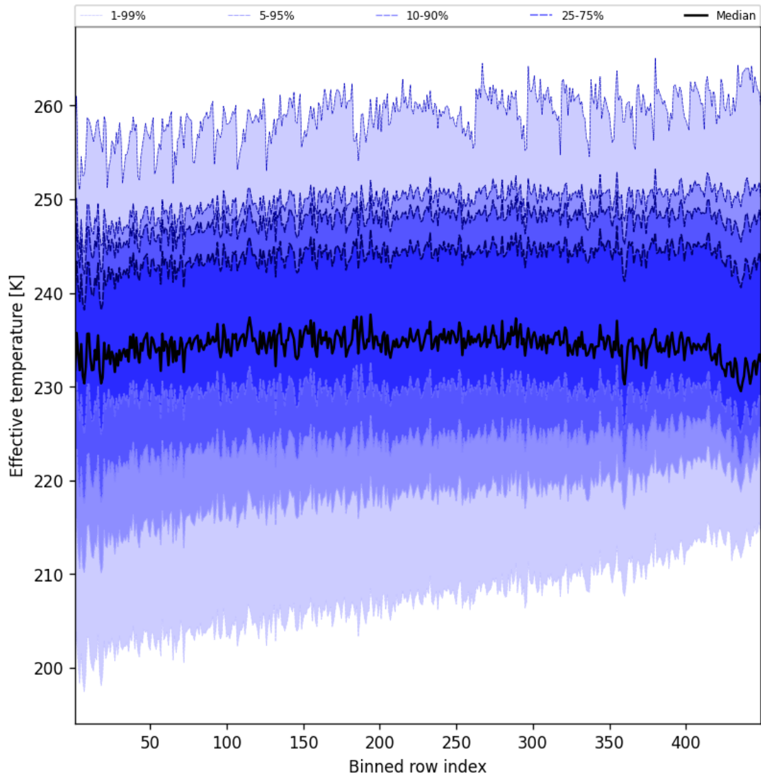
Figure 50: Along track statistics of “Effective temperature” for 2025-06-29 to 2025-06-30
