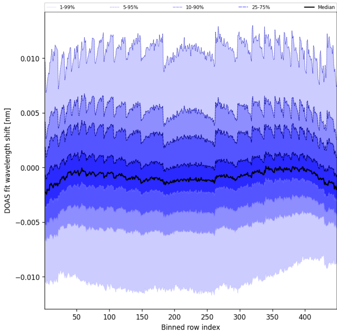
Figure 47: Along track statistics of “DOAS fit wavelength shift” for 2025-06-29 to 2025-06-30
