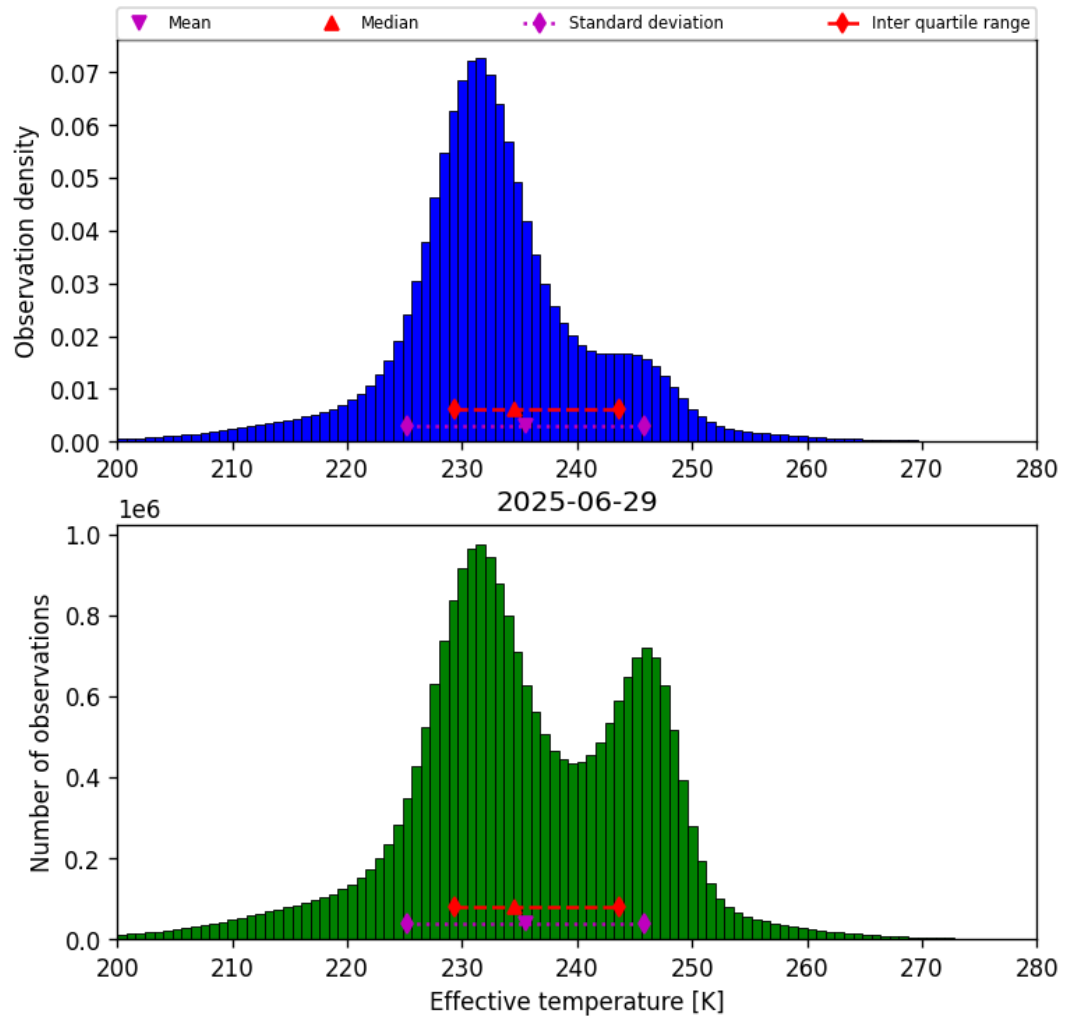
Figure 38: Histogram of “Effective temperature” for 2025-06-29 to 2025-06-30
