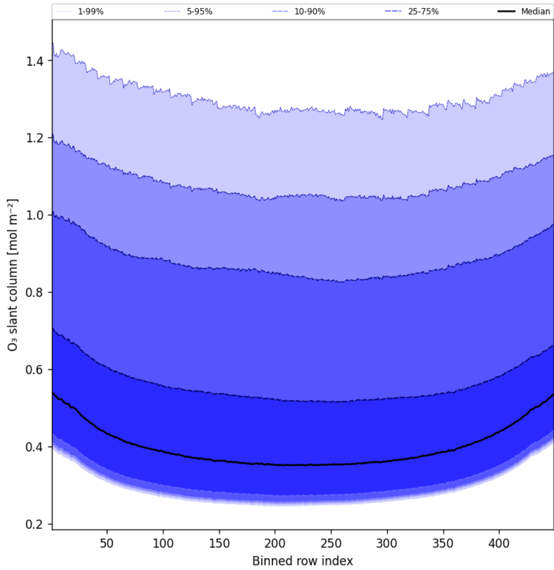
Figure 43: Along track statistics of “O 3 slant column” for 2025-06-29 to 2025-06-30
