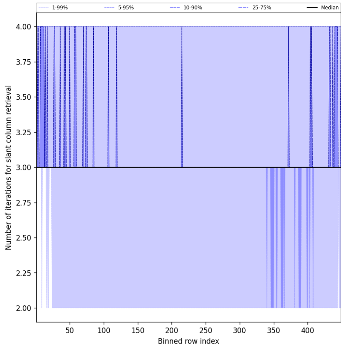
Figure 45: Along track statistics of “Number of iterations for slant column retrieval” for 2025-06-29 to 2025-06-30
