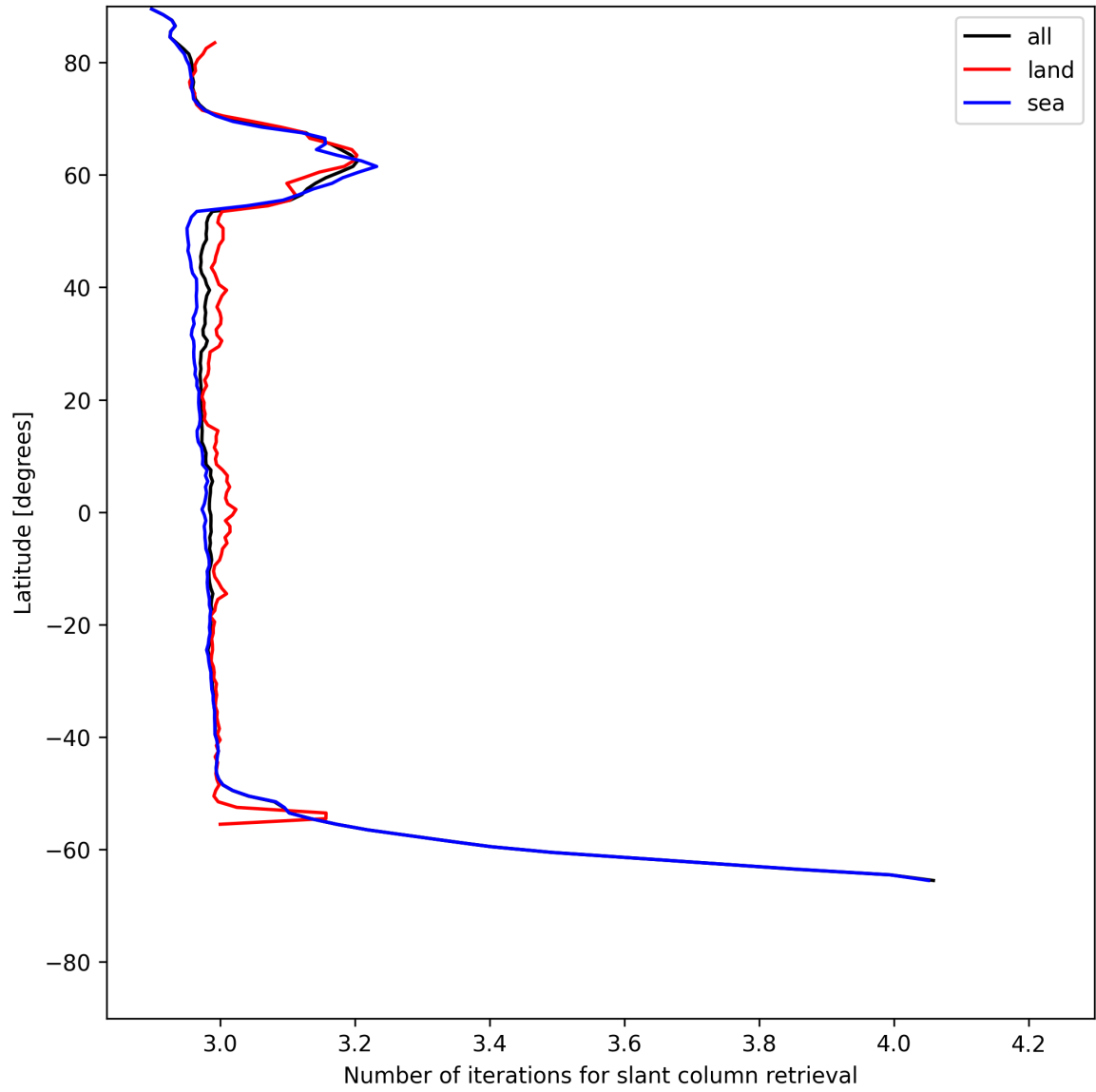
Figure 21: Zonal average of “Number of iterations for slant column retrieval” for 2025-06-29 to 2025-06-30.
