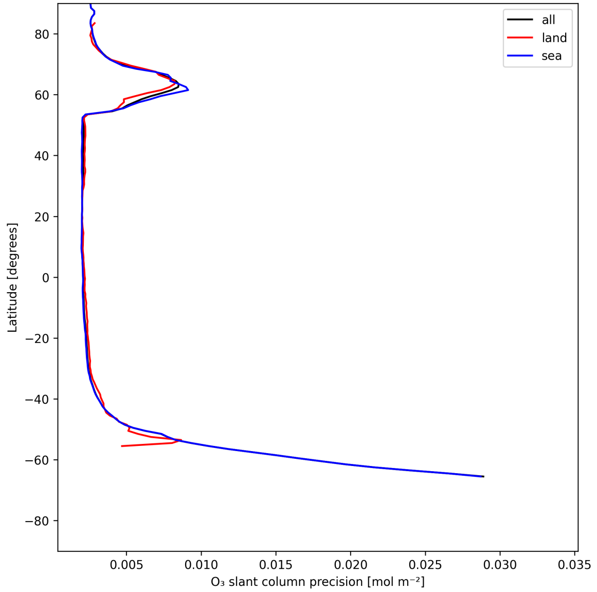
Figure 20: Zonal average of “O 3 slant column precision” for 2025-06-29 to 2025-06-30.
