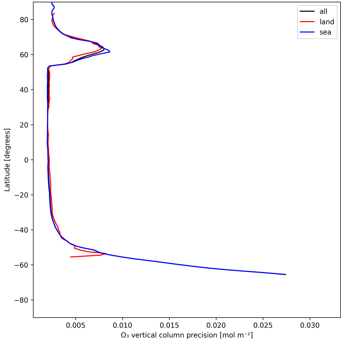
Figure 18: Zonal average of “O 3 vertical column precision” for 2025-06-29 to 2025-06-30.
