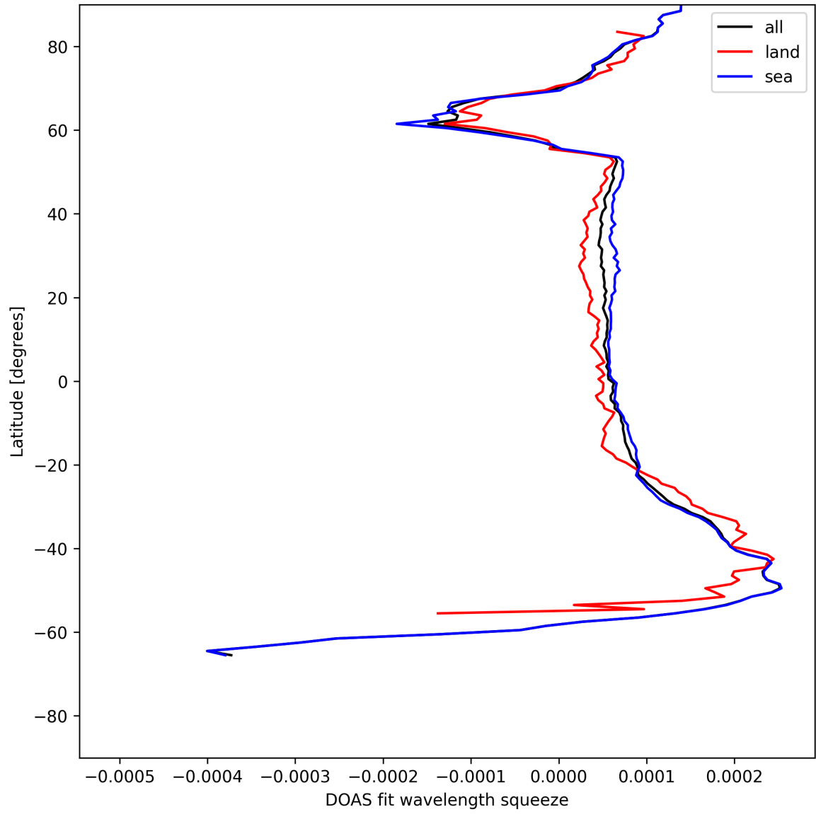
Figure 24: Zonal average of “DOAS fit wavelength squeeze” for 2025-06-29 to 2025-06-30.
