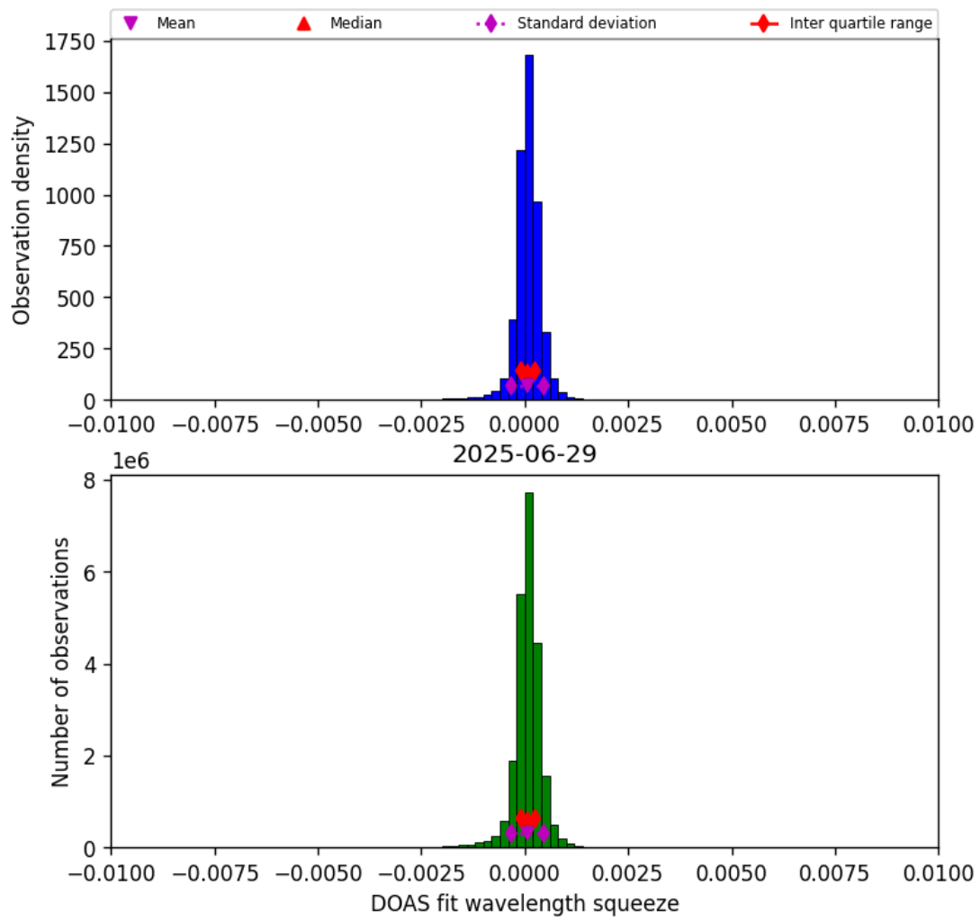
Figure 36: Histogram of “DOAS fit wavelength squeeze” for 2025-06-29 to 2025-06-30
