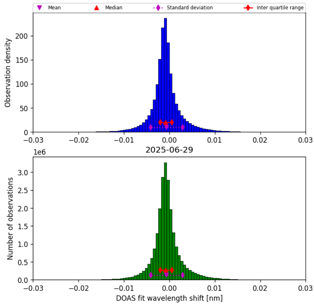
Figure 35: Histogram of “DOAS fit wavelength shift” for 2025-06-29 to 2025-06-30
