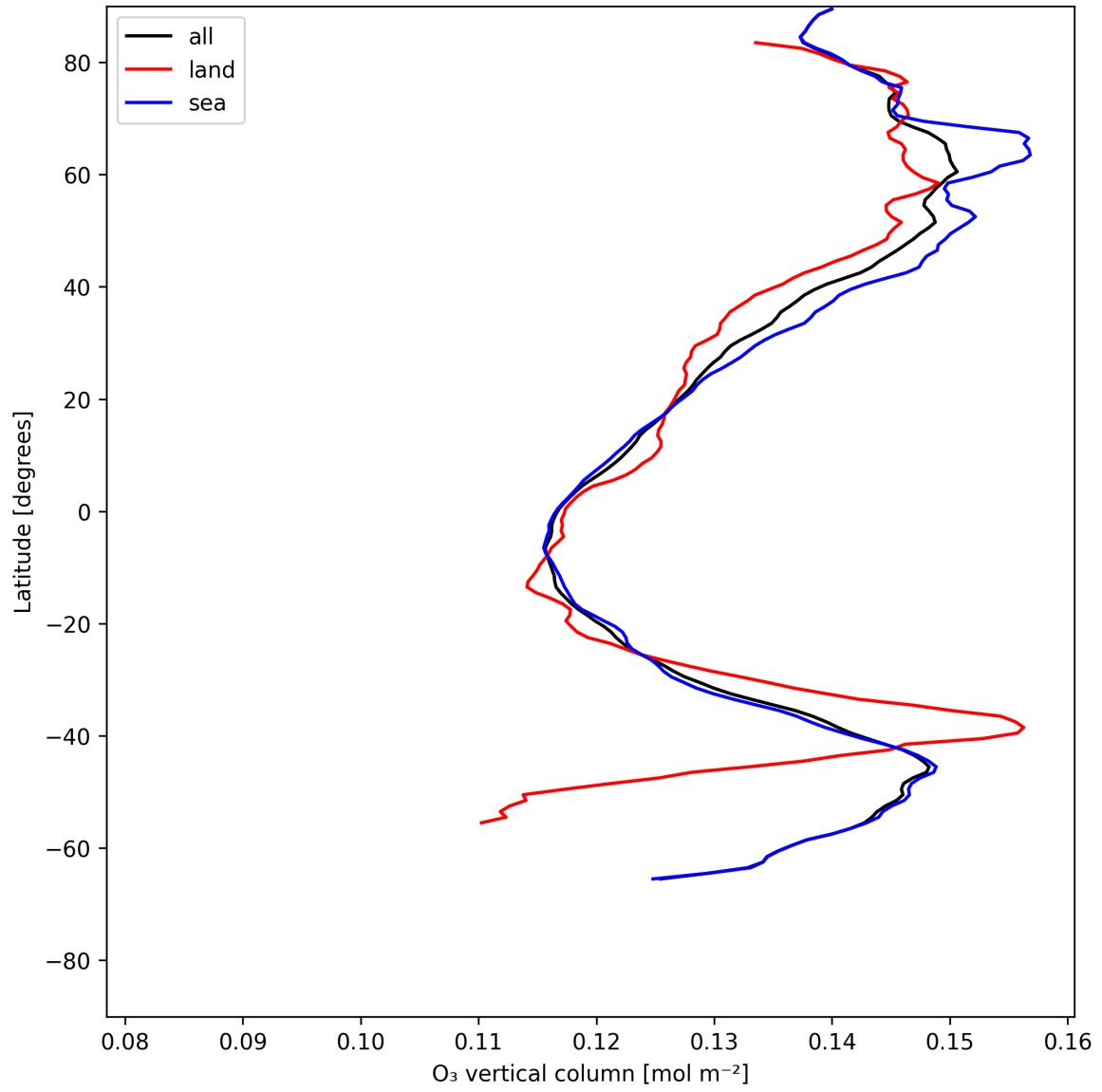
Figure 17: Zonal average of “O 3 vertical column” for 2025-06-29 to 2025-06-30.
