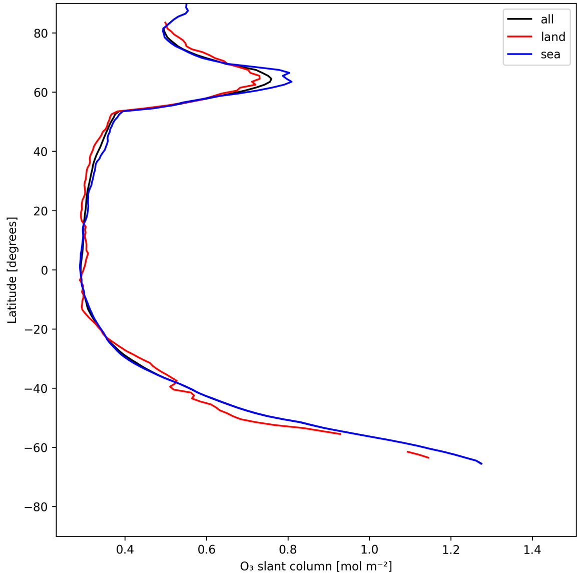
Figure 19: Zonal average of “O 3 slant column” for 2025-06-30 to 2025-06-30.
