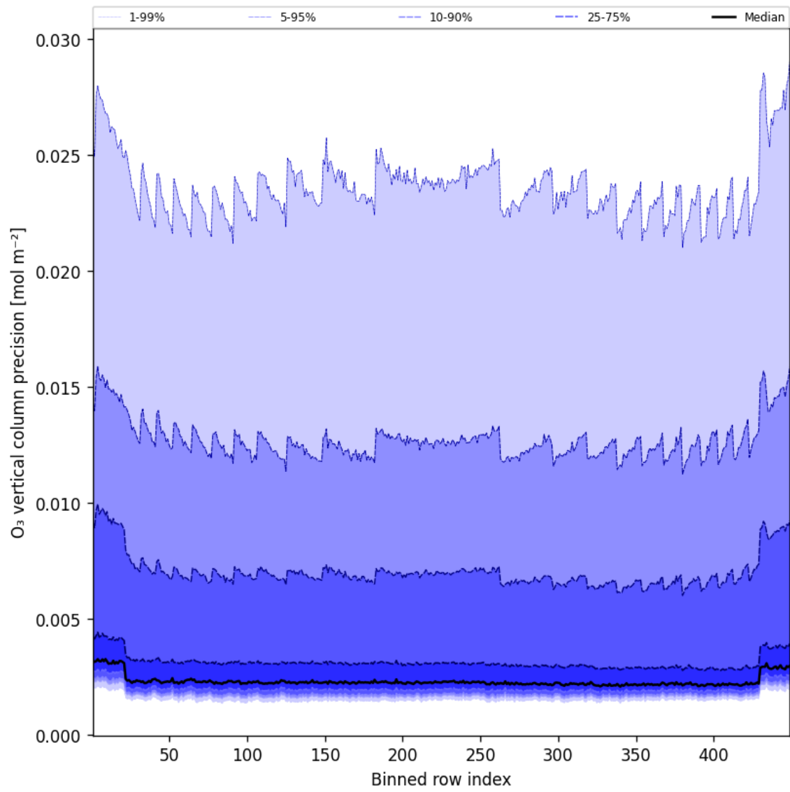
Figure 42: Along track statistics of “O 3 vertical column precision” for 2025-06-30 to 2025-06-30
