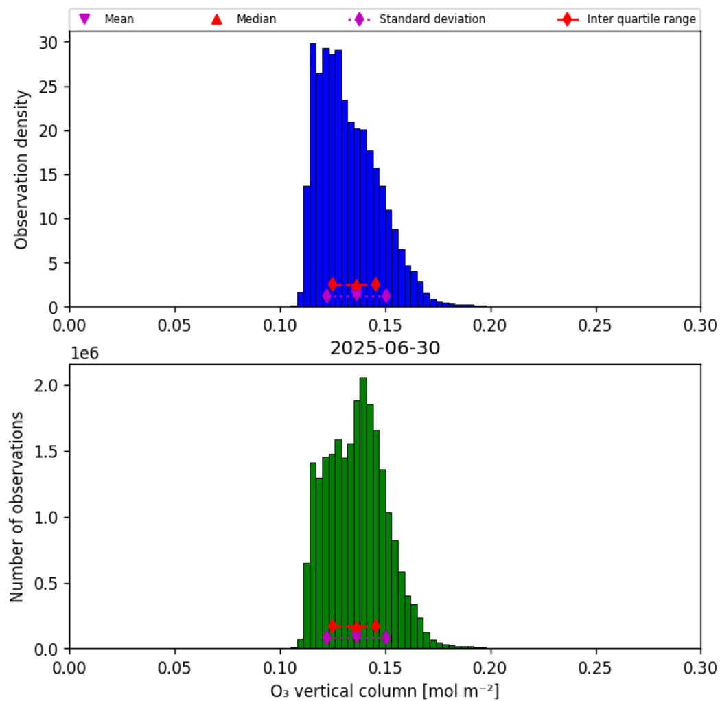
Figure 29: Histogram of “O 3 vertical column” for 2025-06-30 to 2025-06-30
