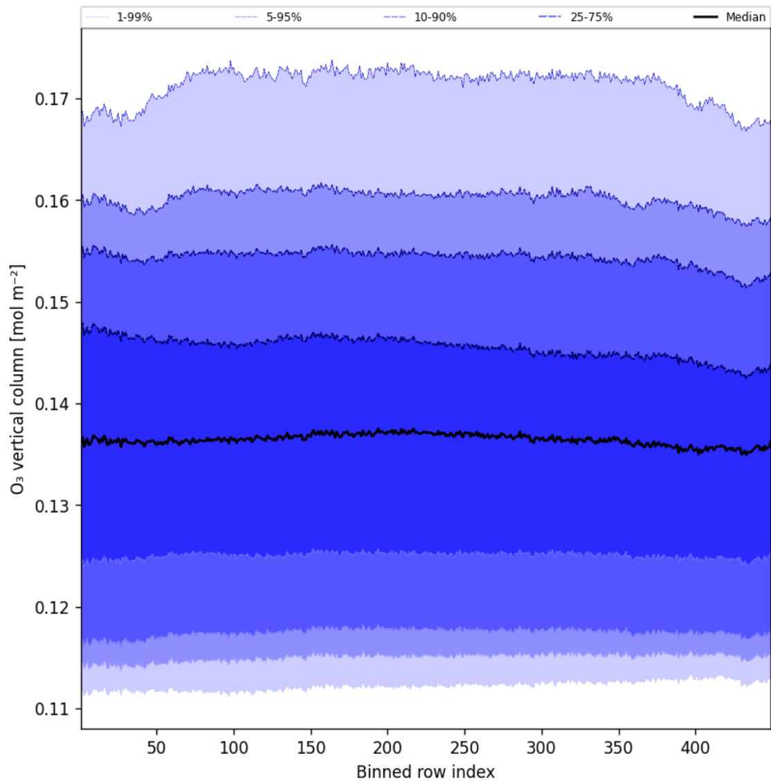
Figure 41: Along track statistics of “O 3 vertical column” for 2025-06-30 to 2025-06-30
