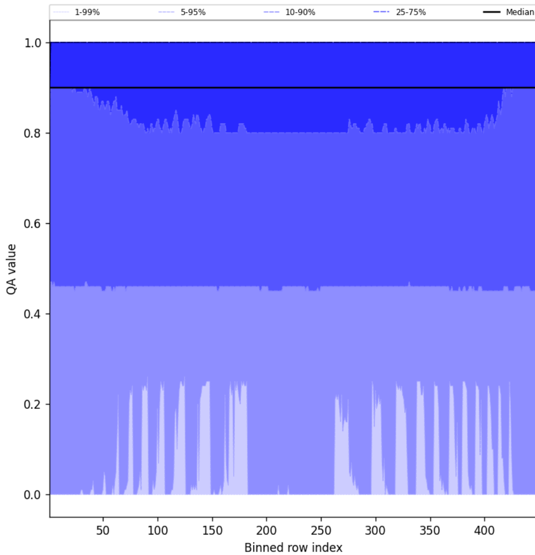
Figure 40: Along track statistics of “QA value” for 2025-06-30 to 2025-06-30
