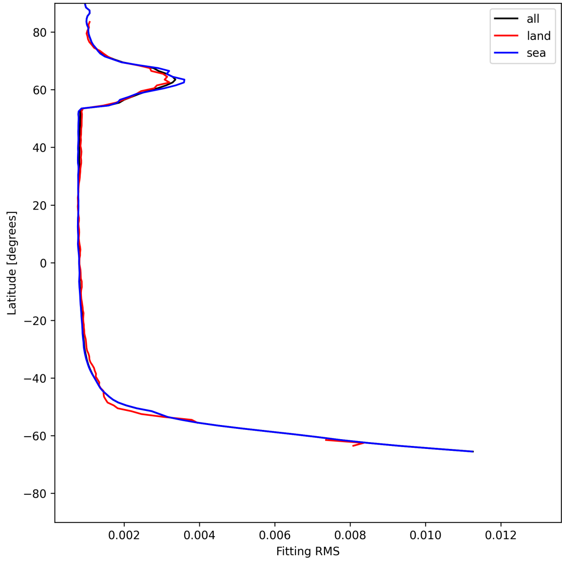
Figure 22: Zonal average of “Fitting RMS” for 2025-06-30 to 2025-06-30.
