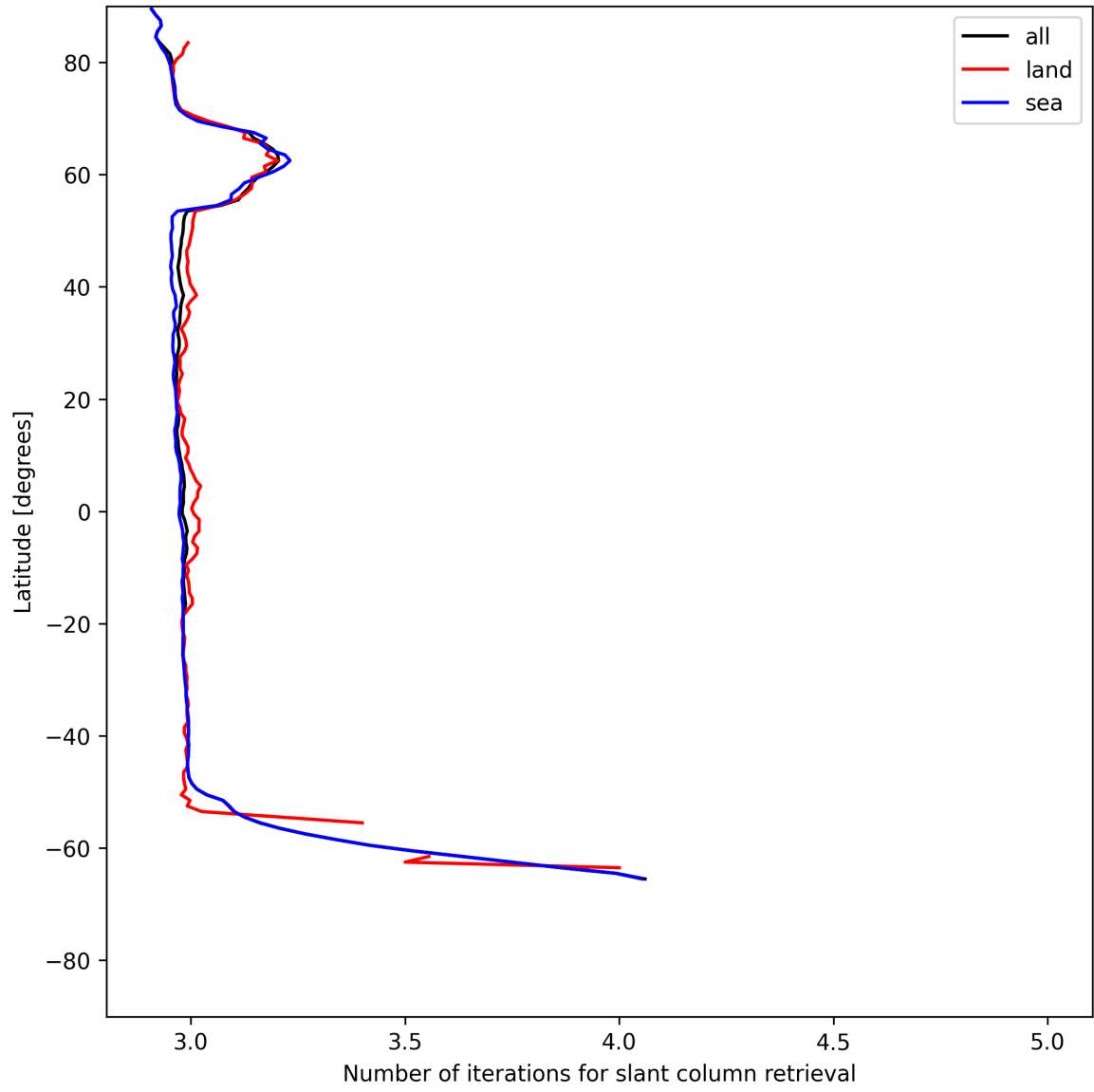
Figure 21: Zonal average of “Number of iterations for slant column retrieval” for 2025-06-30 to 2025-06-30.
