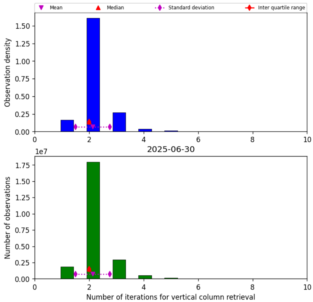
Figure 39: Histogram of “Number of iterations for vertical column retrieval” for 2025-06-30 to 2025-06-30
