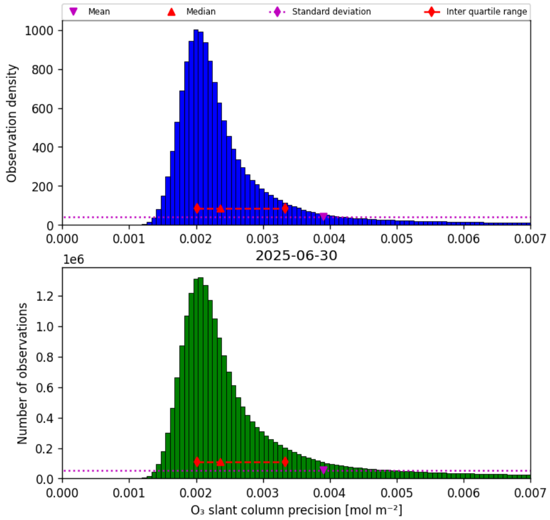
Figure 32: Histogram of “O 3 slant column precision” for 2025-06-30 to 2025-06-30
