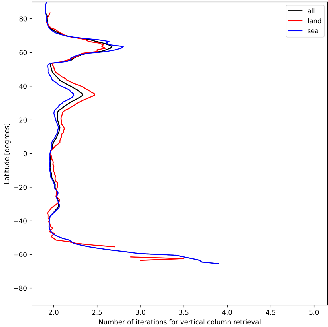
Figure 27: Zonal average of “Number of iterations for vertical column retrieval” for 2025-06-30 to 2025-06-30.
