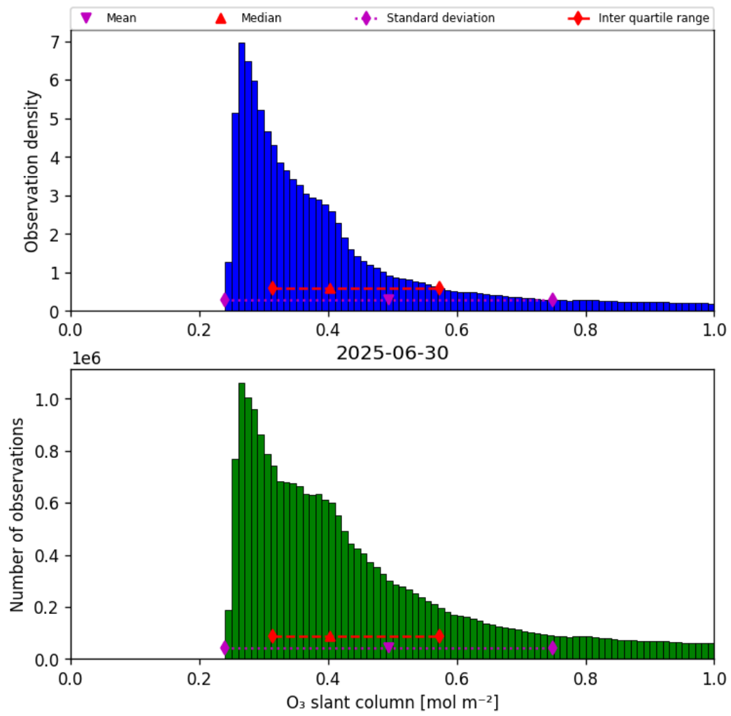
Figure 31: Histogram of “O 3 slant column” for 2025-06-30 to 2025-06-30
