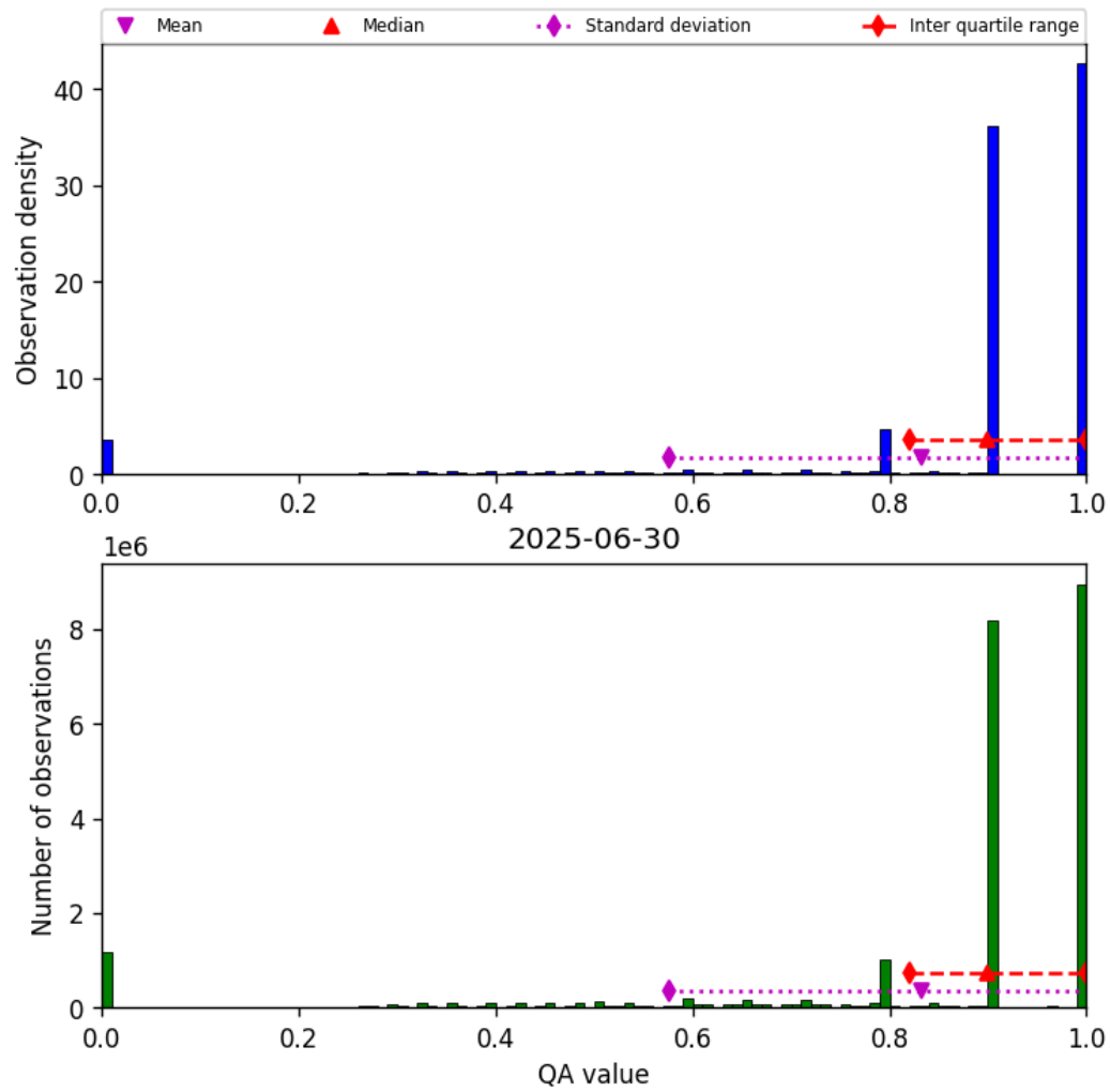
Figure 28: Histogram of “QA value” for 2025-06-30 to 2025-06-30
