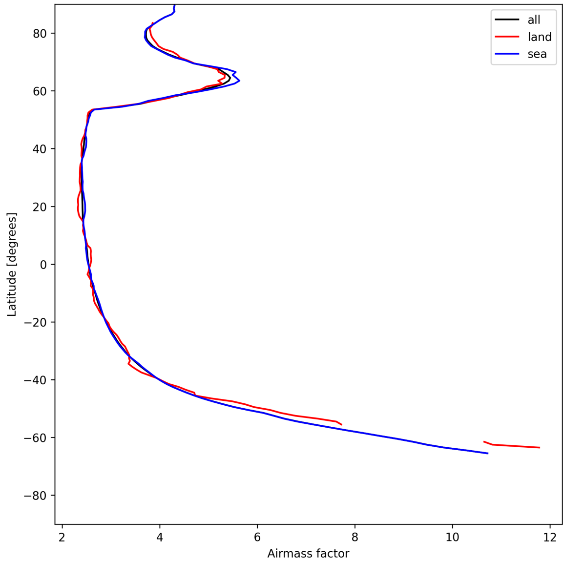
Figure 25: Zonal average of “Airmass factor” for 2025-06-30 to 2025-06-30.
