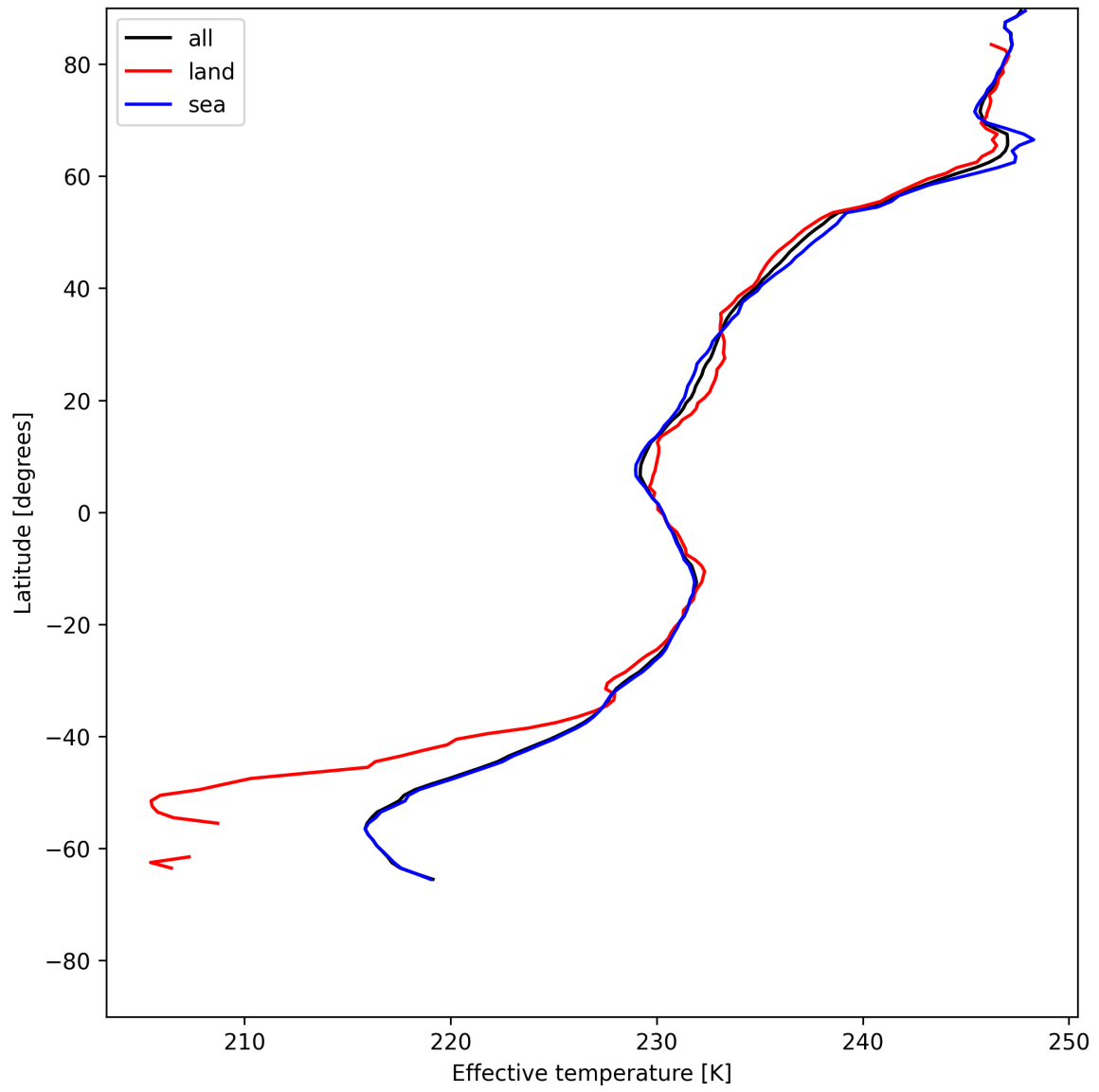
Figure 26: Zonal average of “Effective temperature” for 2025-06-30 to 2025-06-30.
