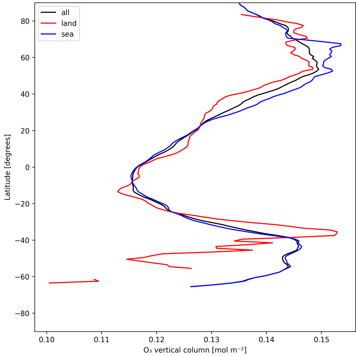
Figure 17: Zonal average of “O 3 vertical column” for 2025-06-30 to 2025-06-30.
