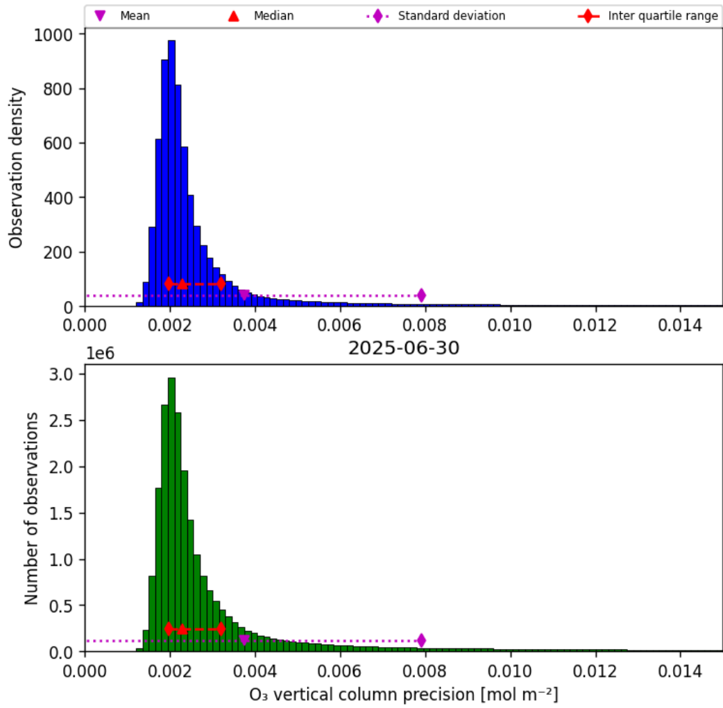
Figure 30: Histogram of "O 3 vertical column precision" for 2025-06-30 to 2025-06-30
