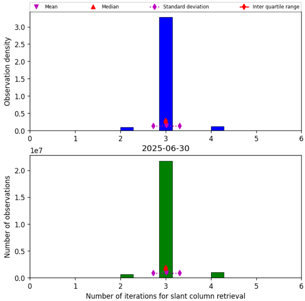
Figure 33: Histogram of “Number of iterations for slant column retrieval” for 2025-06-30 to 2025-06-30
