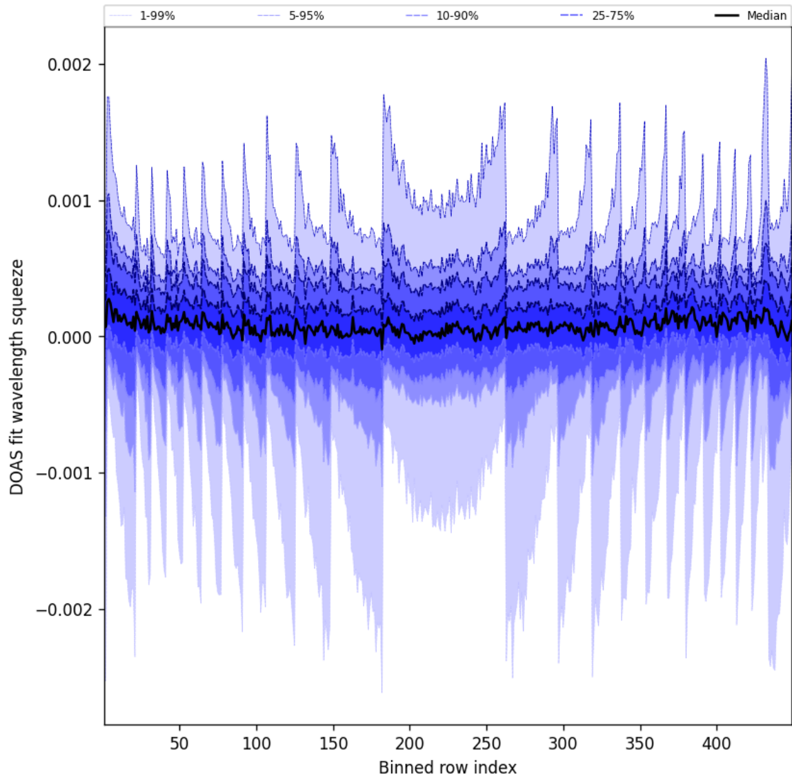
Figure 48: Along track statistics of “DOAS fit wavelength squeeze” for 2025-06-30 to 2025-06-30
