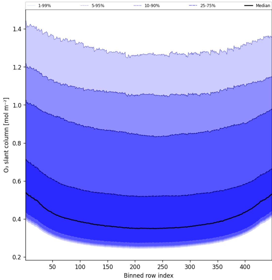
Figure 43: Along track statistics of “O 3 slant column” for 2025-06-30 to 2025-06-30
