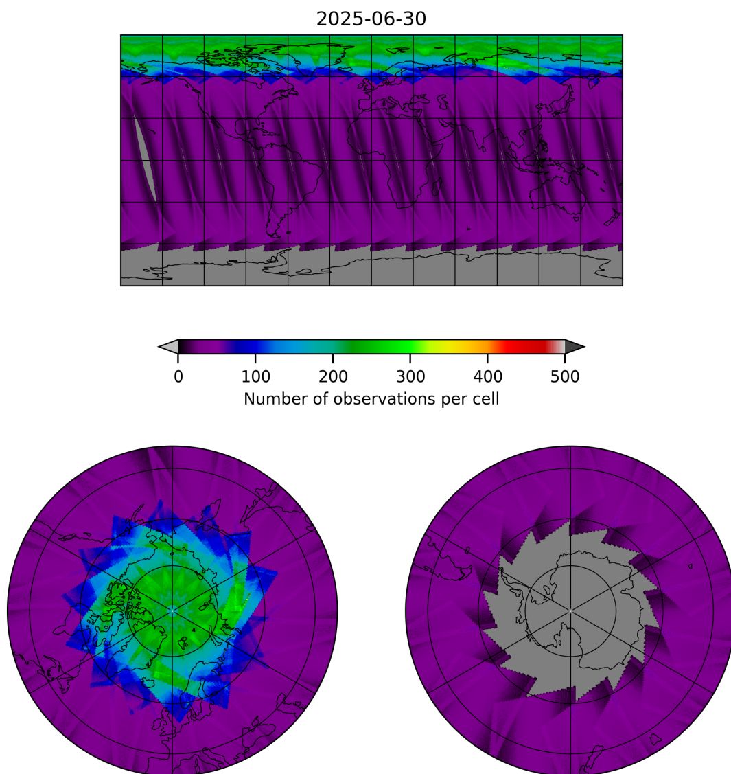
Figure 15: Map of the number of observations for 2025-06-30 to 2025-06-30
