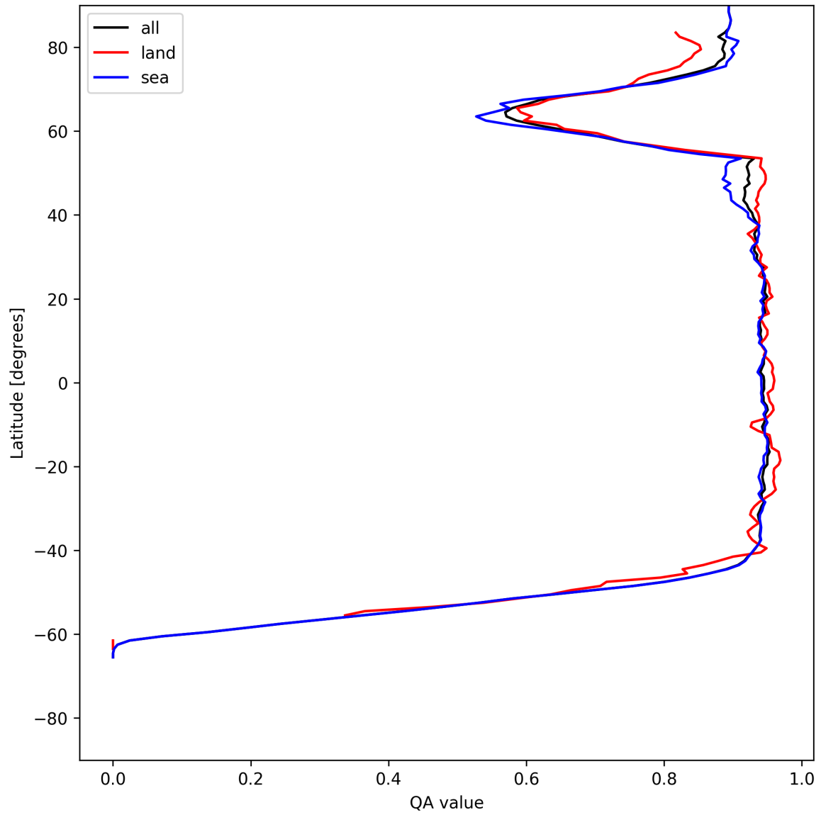
Figure 16: Zonal average of “QA value” for 2025-06-30 to 2025-06-30.
