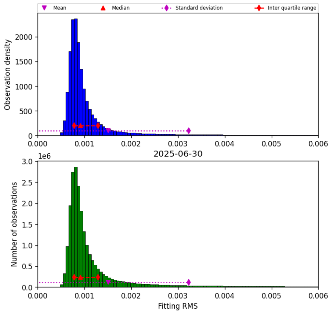
Figure 34: Histogram of “Fitting RMS” for 2025-06-30 to 2025-06-30
