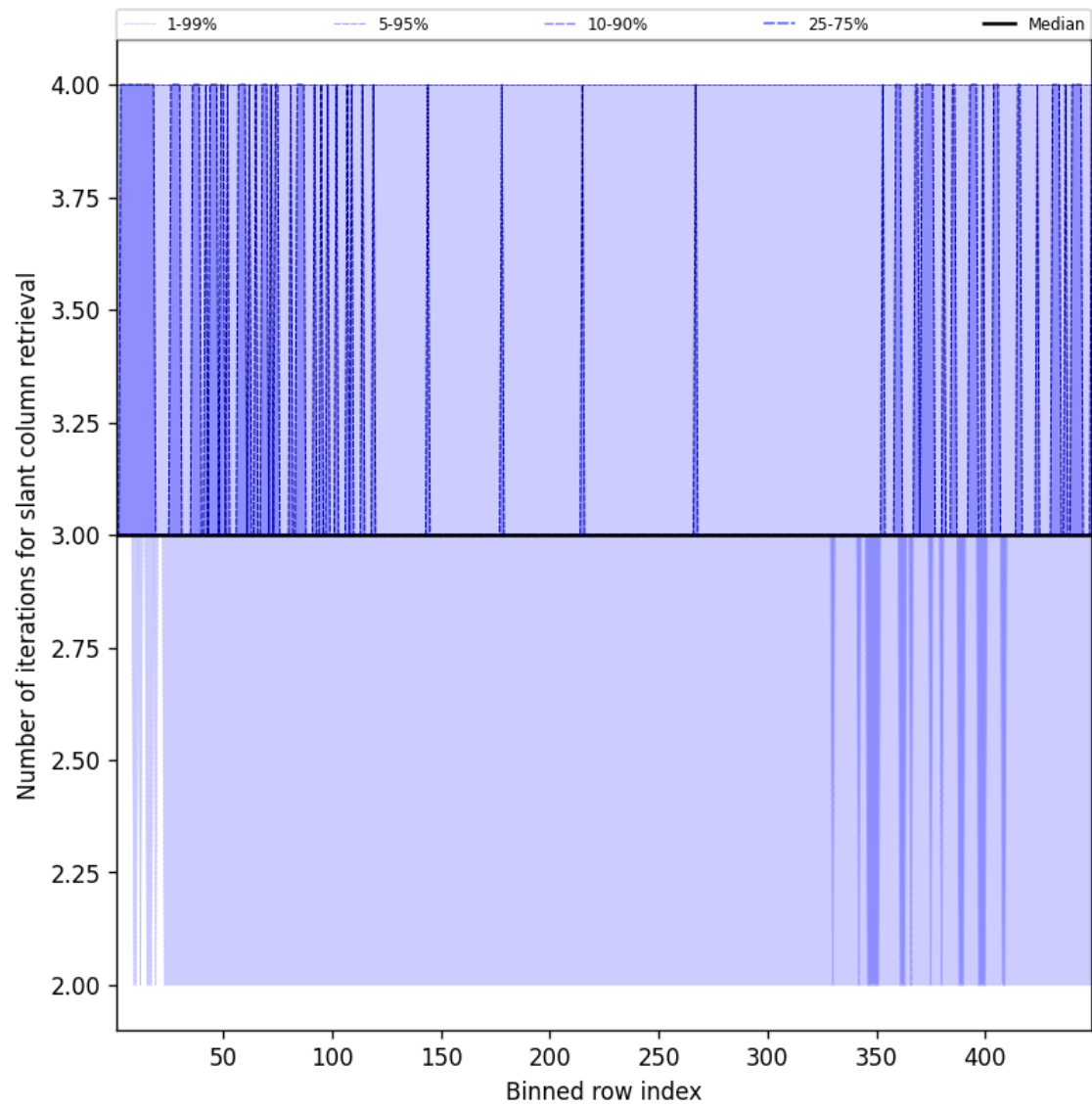
Figure 45: Along track statistics of “Number of iterations for slant column retrieval” for 2025-06-30 to 2025-06-30
