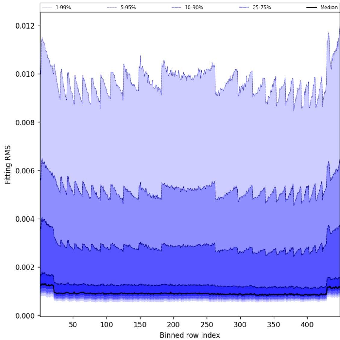
Figure 46: Along track statistics of “Fitting RMS” for 2025-06-30 to 2025-06-30
