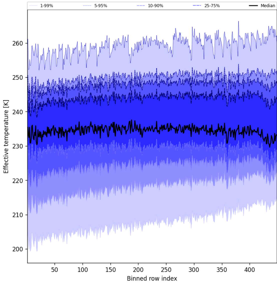
Figure 50: Along track statistics of “Effective temperature” for 2025-06-30 to 2025-06-30
