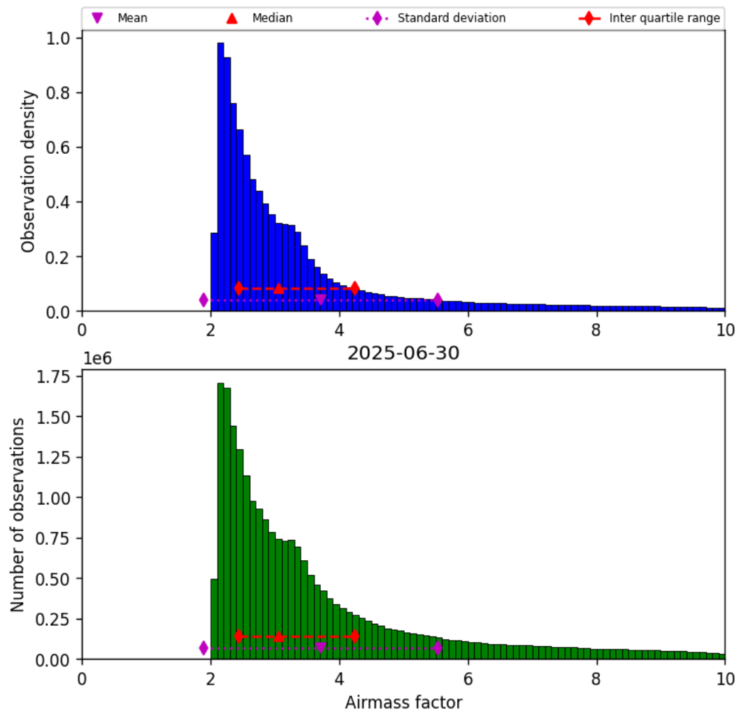
Figure 37: Histogram of “Airmass factor” for 2025-06-30 to 2025-06-30
