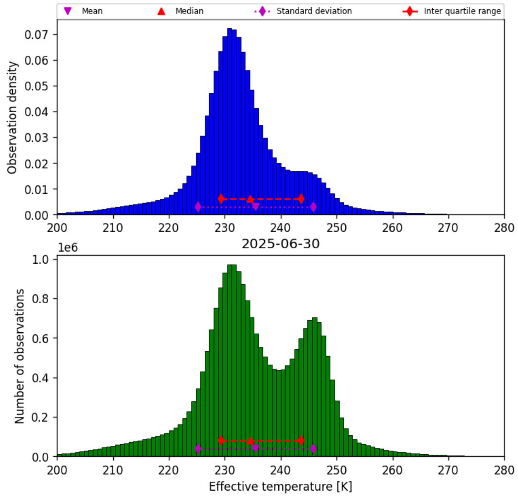
Figure 38: Histogram of “Effective temperature” for 2025-06-30 to 2025-06-30
