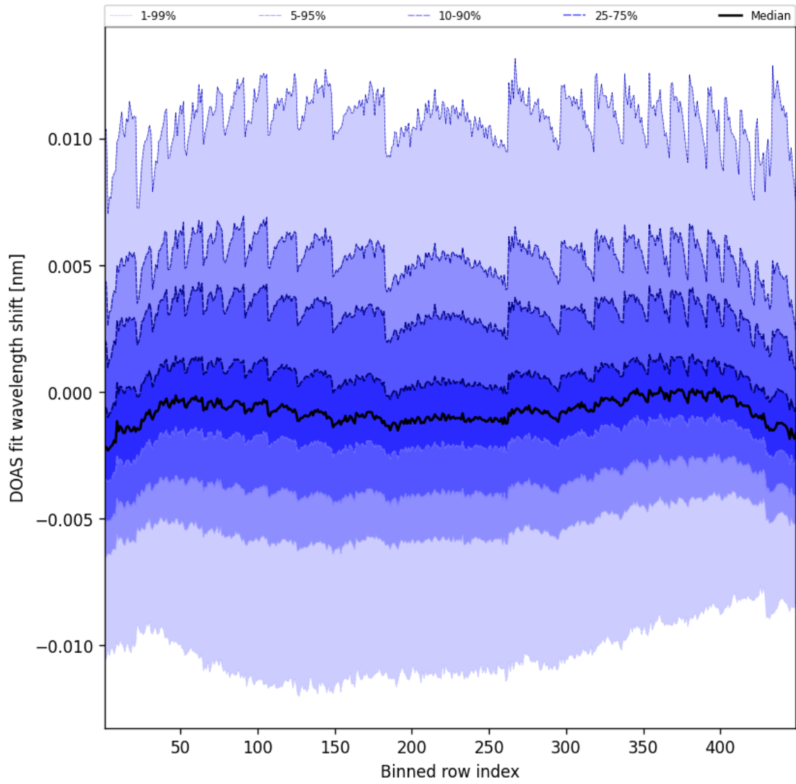
Figure 47: Along track statistics of “DOAS fit wavelength shift” for 2025-06-30 to 2025-06-30
