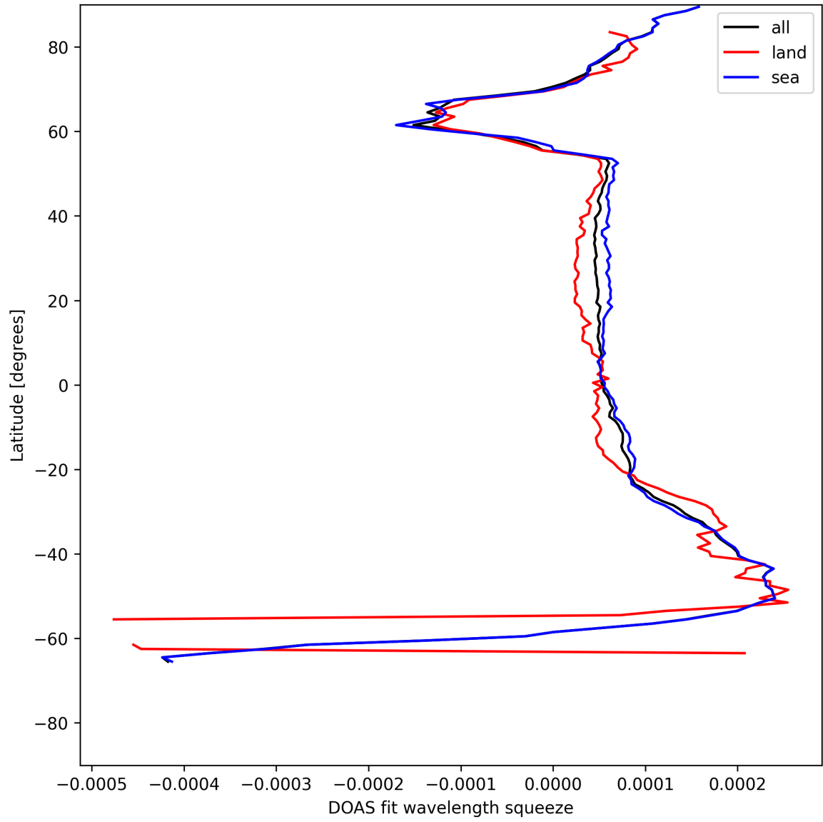
Figure 24: Zonal average of “DOAS fit wavelength squeeze” for 2025-06-30 to 2025-06-30.
