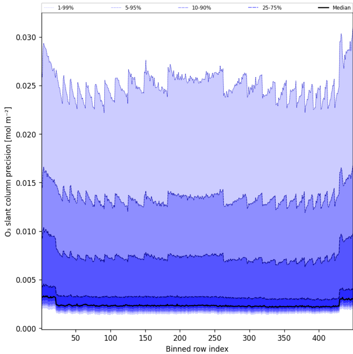
Figure 44: Along track statistics of “O 3 slant column precision” for 2025-06-30 to 2025-06-30
