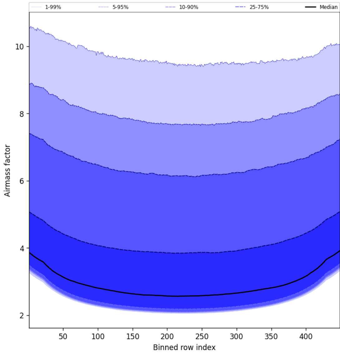
Figure 49: Along track statistics of “Airmass factor” for 2025-06-30 to 2025-06-30
