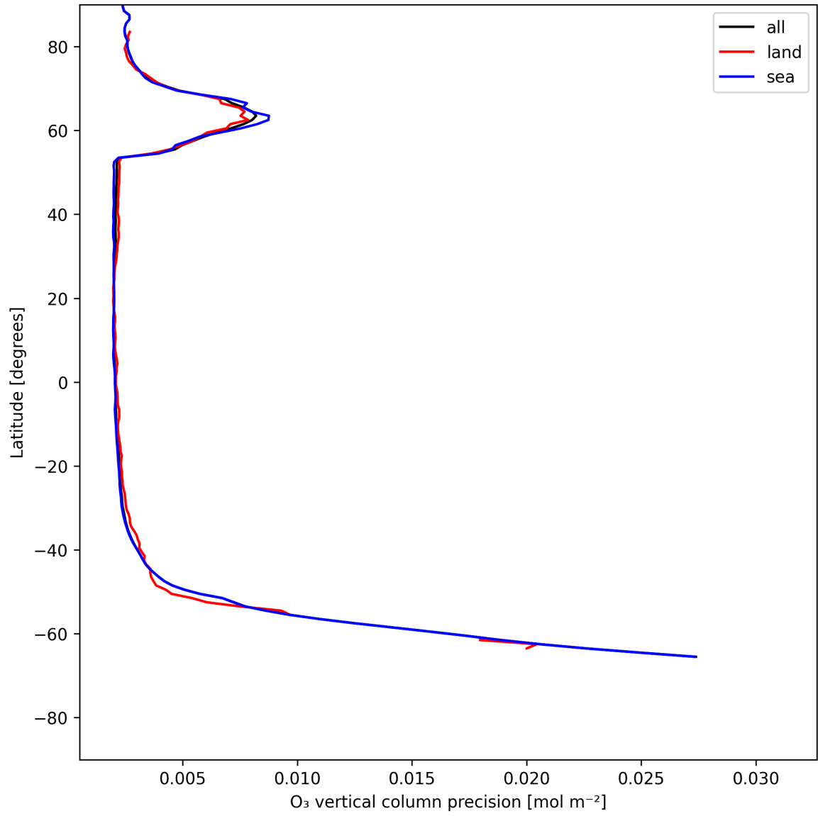
Figure 18: Zonal average of “O 3 vertical column precision” for 2025-06-30 to 2025-06-30.
