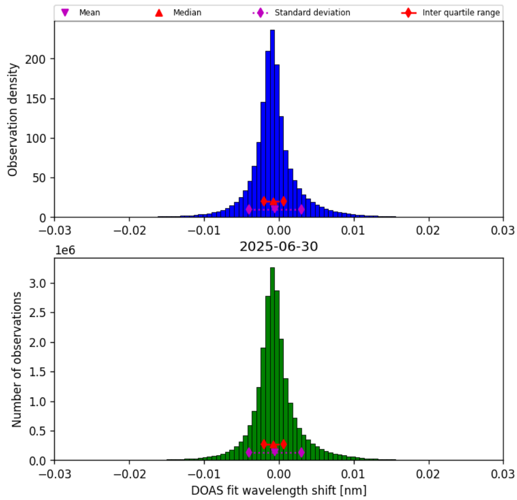
Figure 35: Histogram of “DOAS fit wavelength shift” for 2025-06-30 to 2025-06-30
