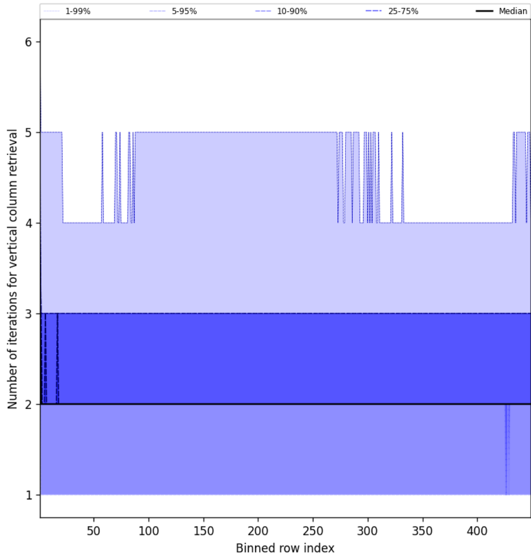
Figure 51: Along track statistics of “Number of iterations for vertical column retrieval” for 2025-06-30 to 2025-06-30
