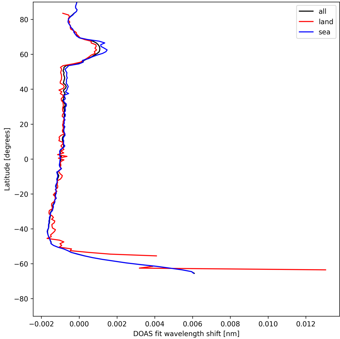
Figure 23: Zonal average of "DOAS fit wavelength shift" for 2025-06-30 to 2025-06-30.
