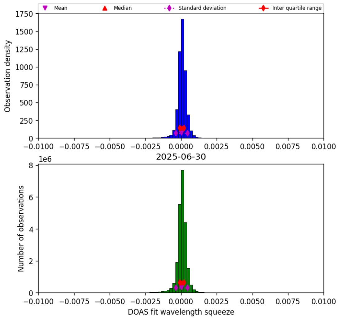
Figure 36: Histogram of “DOAS fit wavelength squeeze” for 2025-06-30 to 2025-06-30
