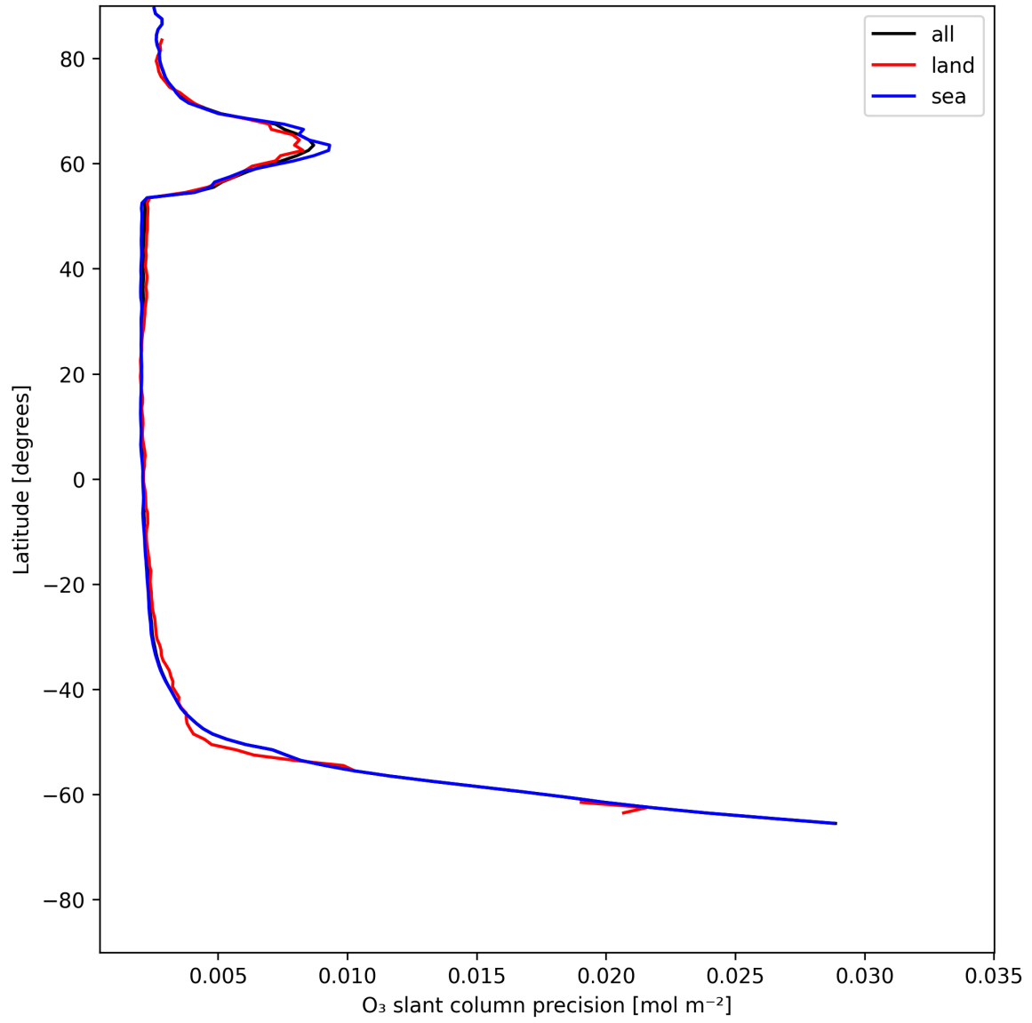
Figure 20: Zonal average of “O 3 slant column precision” for 2025-06-30 to 2025-06-30.
