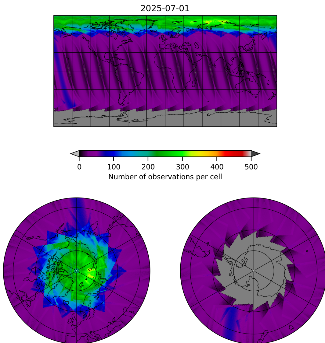
Figure 15: Map of the number of observations for 2025-07-01 to 2025-07-02
