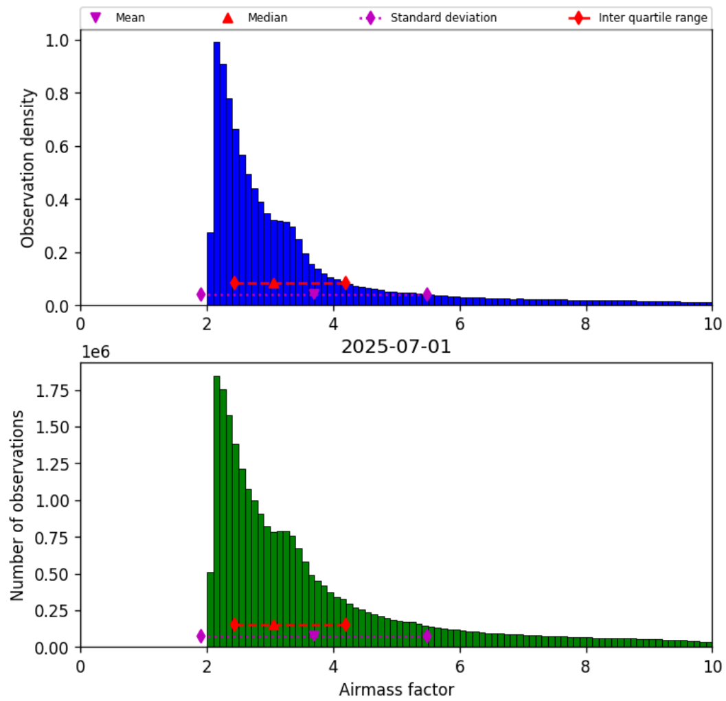
Figure 37: Histogram of “Airmass factor” for 2025-07-01 to 2025-07-02
