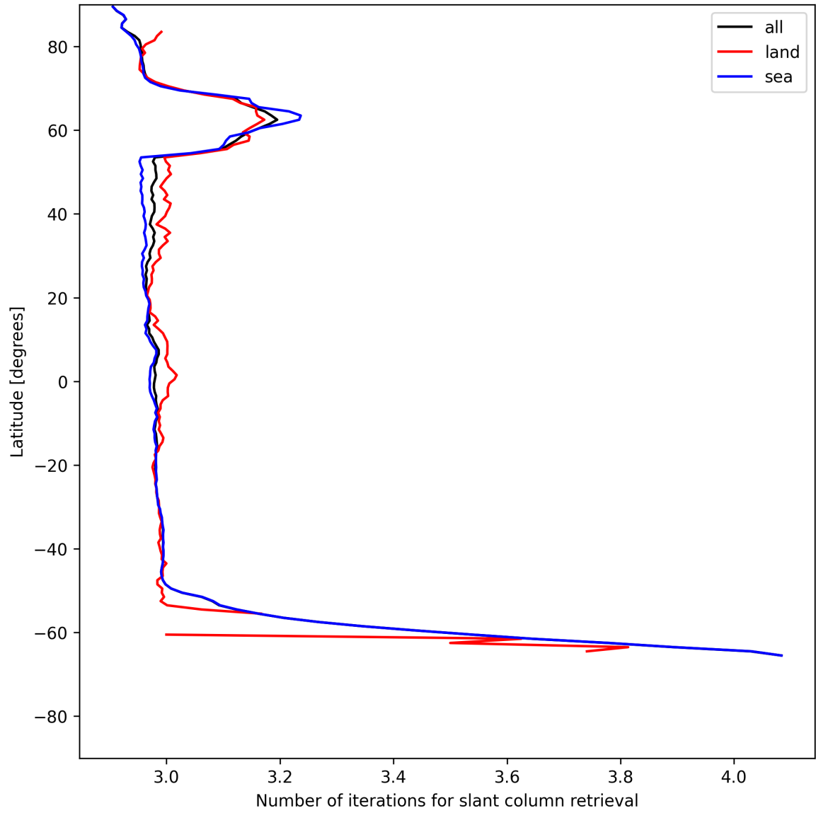
Figure 21: Zonal average of “Number of iterations for slant column retrieval” for 2025-07-01 to 2025-07-02.
