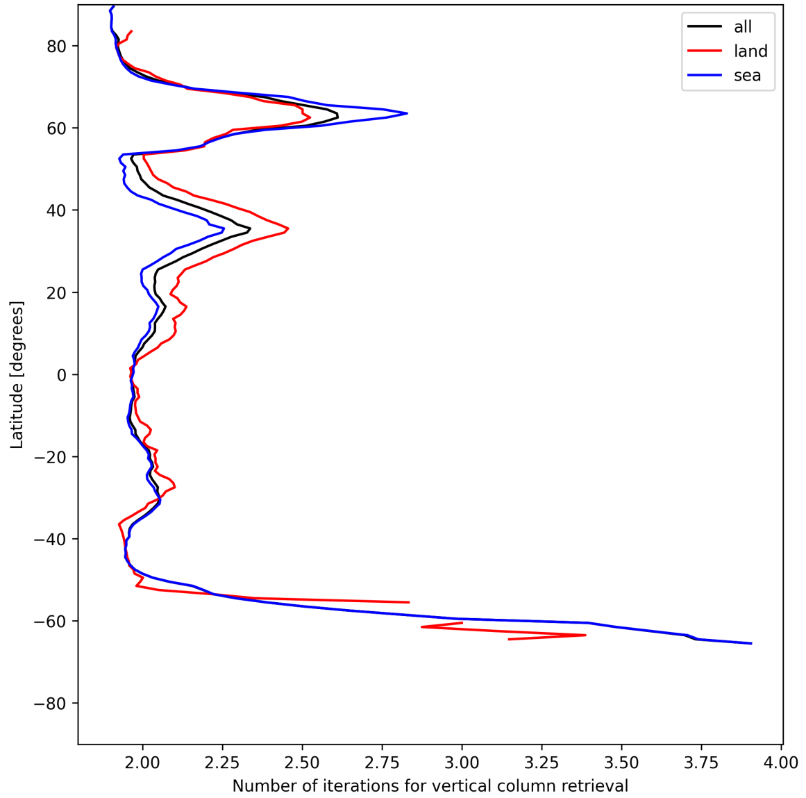
Figure 27: Zonal average of “Number of iterations for vertical column retrieval” for 2025-07-01 to 2025-07-02.
