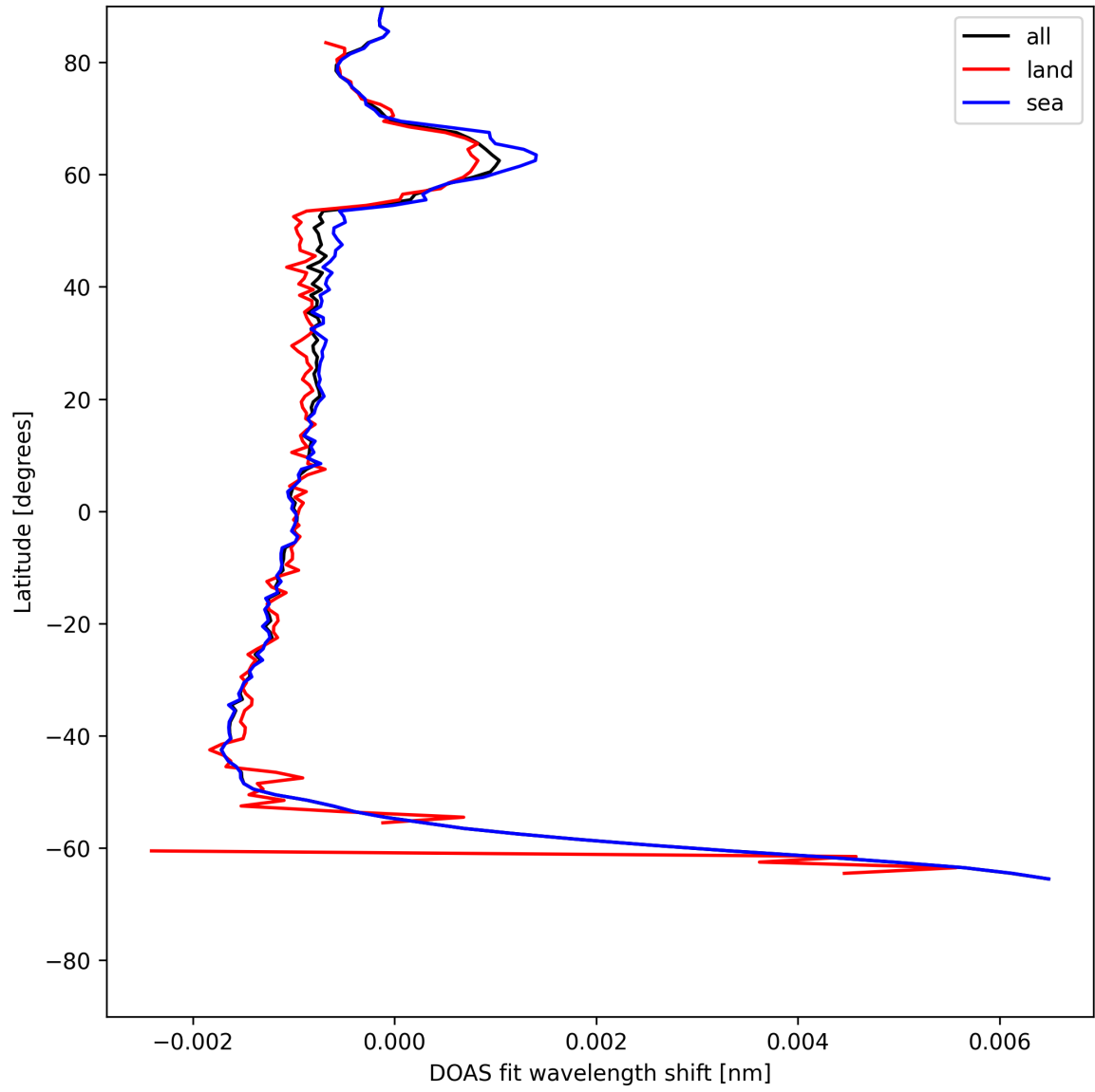
Figure 23: Zonal average of “DOAS fit wavelength shift” for 2025-07-01 to 2025-07-02.
