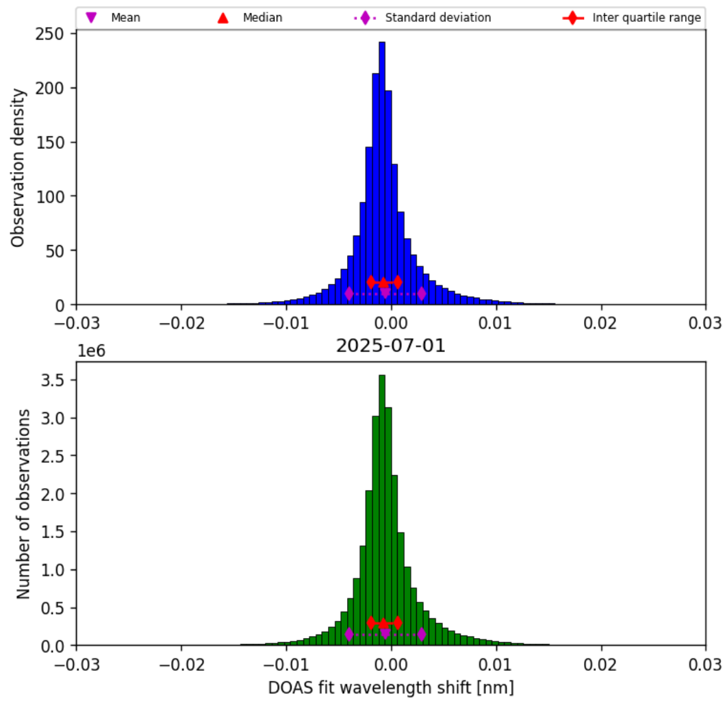
Figure 35: Histogram of “DOAS fit wavelength shift” for 2025-07-01 to 2025-07-02
