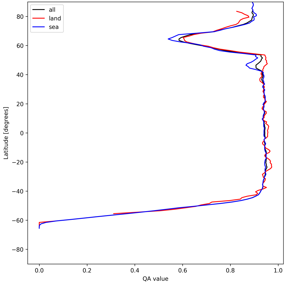
Figure 16: Zonal average of “QA value” for 2025-07-01 to 2025-07-02.
