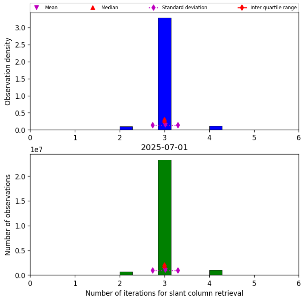
Figure 33: Histogram of “Number of iterations for slant column retrieval” for 2025-07-01 to 2025-07-02
