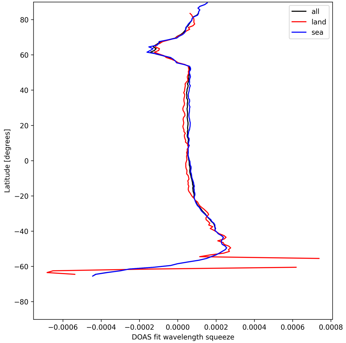
Figure 24: Zonal average of “DOAS fit wavelength squeeze” for 2025-07-01 to 2025-07-02.
