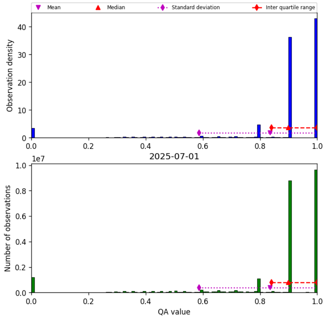
Figure 28: Histogram of “QA value” for 2025-07-01 to 2025-07-02
