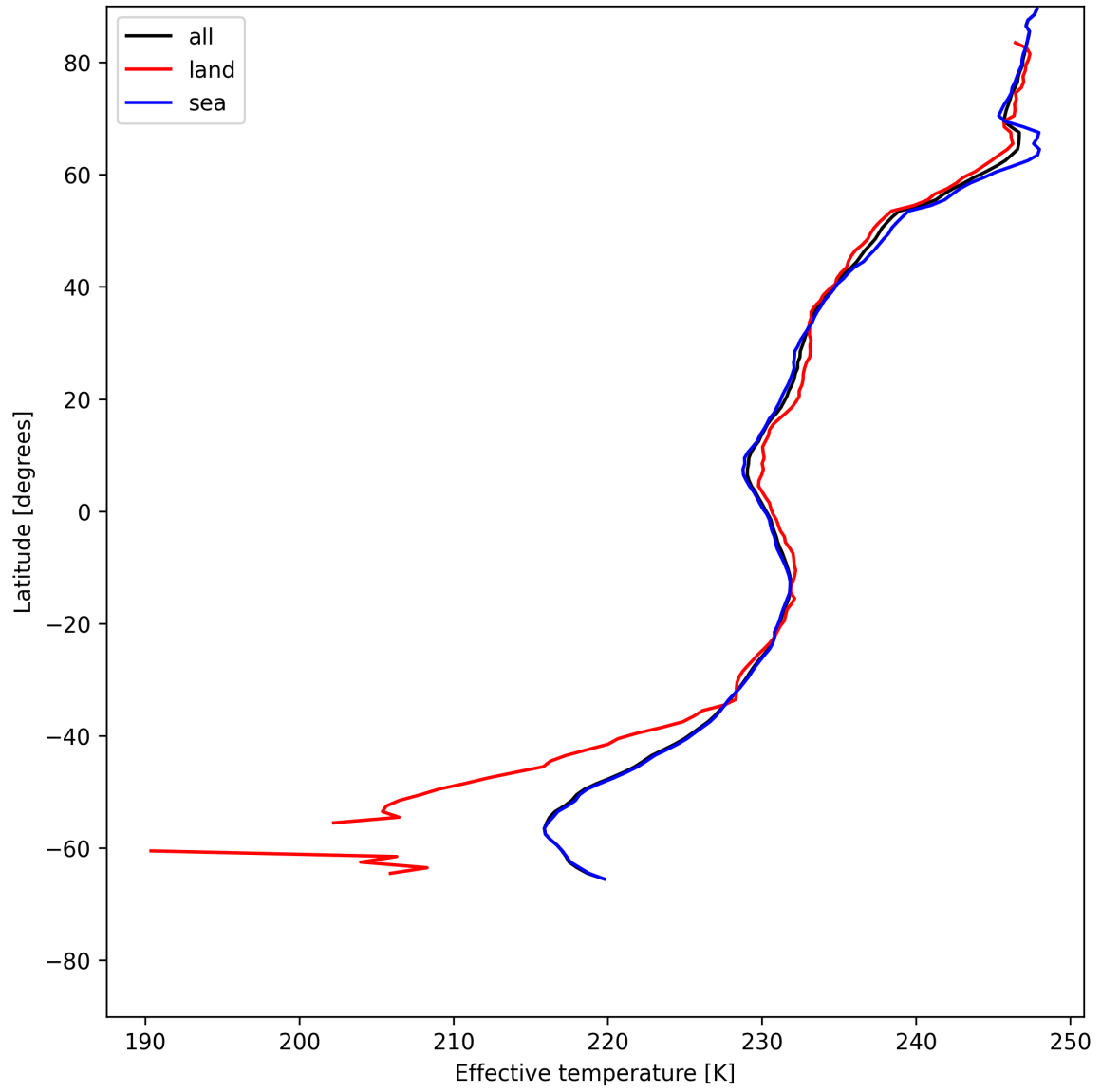
Figure 26: Zonal average of "Effective temperature" for 2025-07-01 to 2025-07-02.
