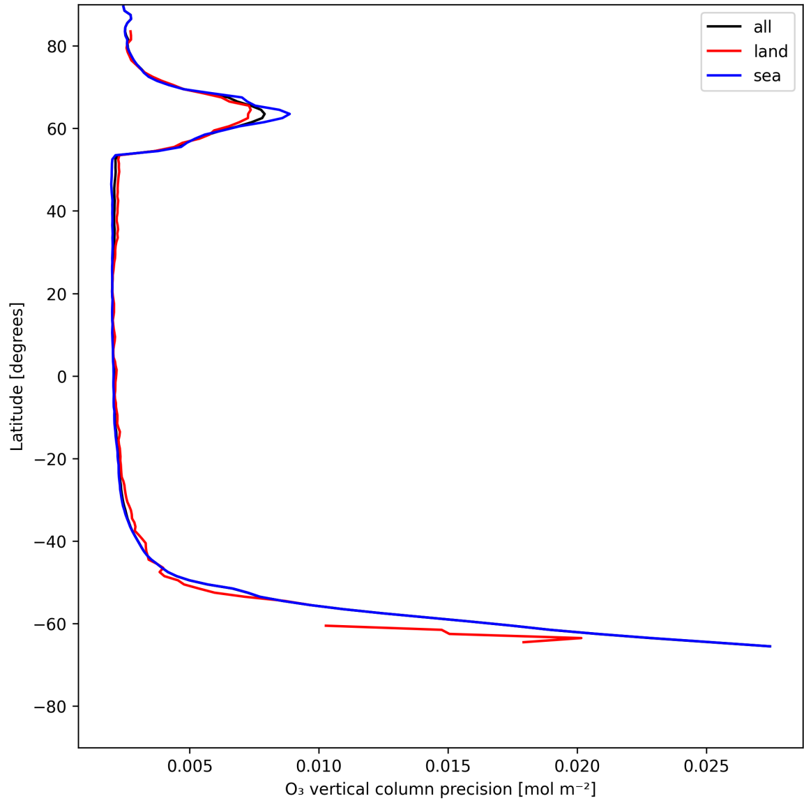
Figure 18: Zonal average of “O 3 vertical column precision” for 2025-07-01 to 2025-07-02.
