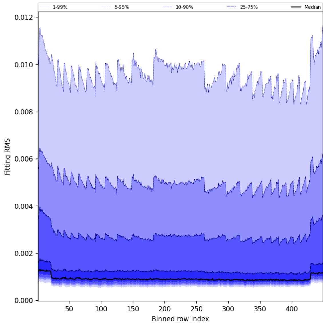
Figure 46: Along track statistics of “Fitting RMS” for 2025-07-01 to 2025-07-02
