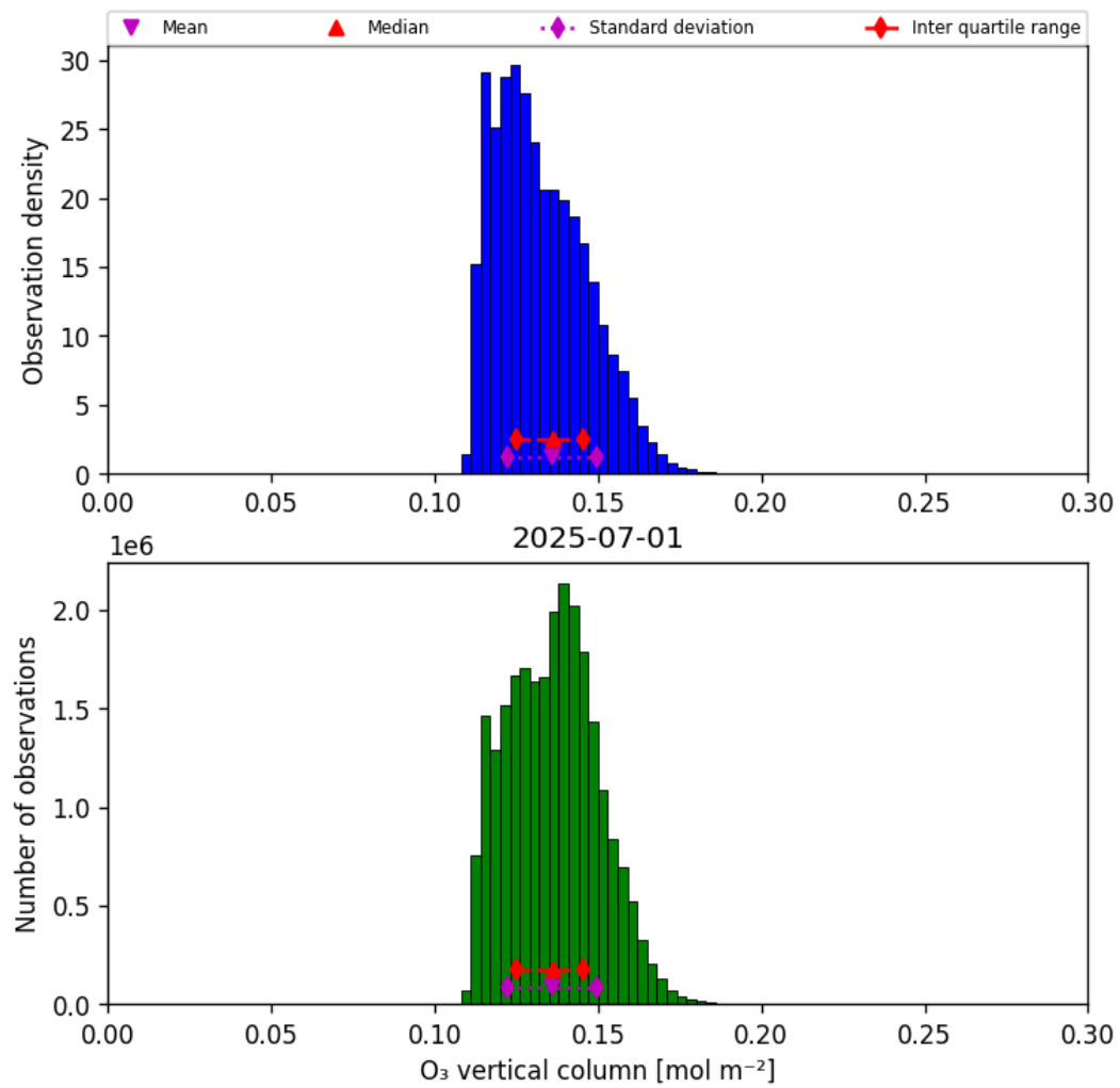
Figure 29: Histogram of “O 3 vertical column” for 2025-07-01 to 2025-07-02
