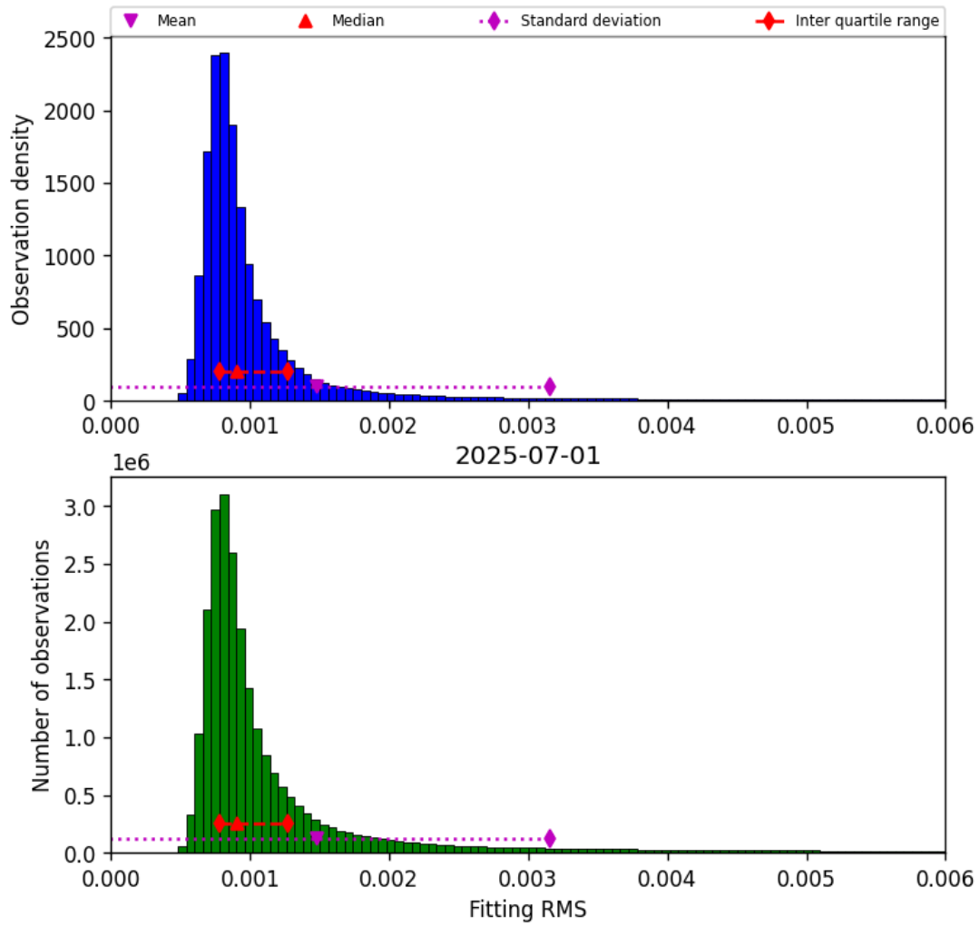
Figure 34: Histogram of “Fitting RMS” for 2025-07-01 to 2025-07-02
