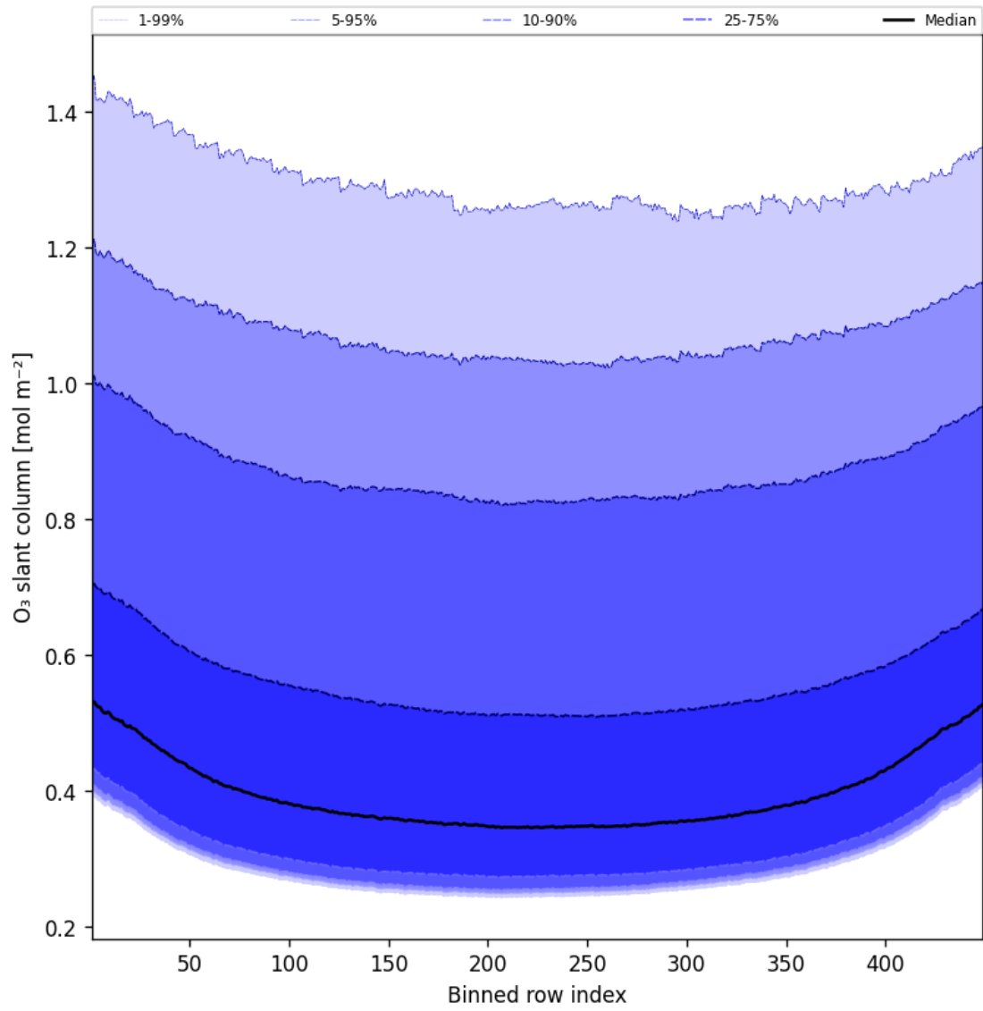
Figure 43: Along track statistics of “O 3 slant column” for 2025-07-01 to 2025-07-02
