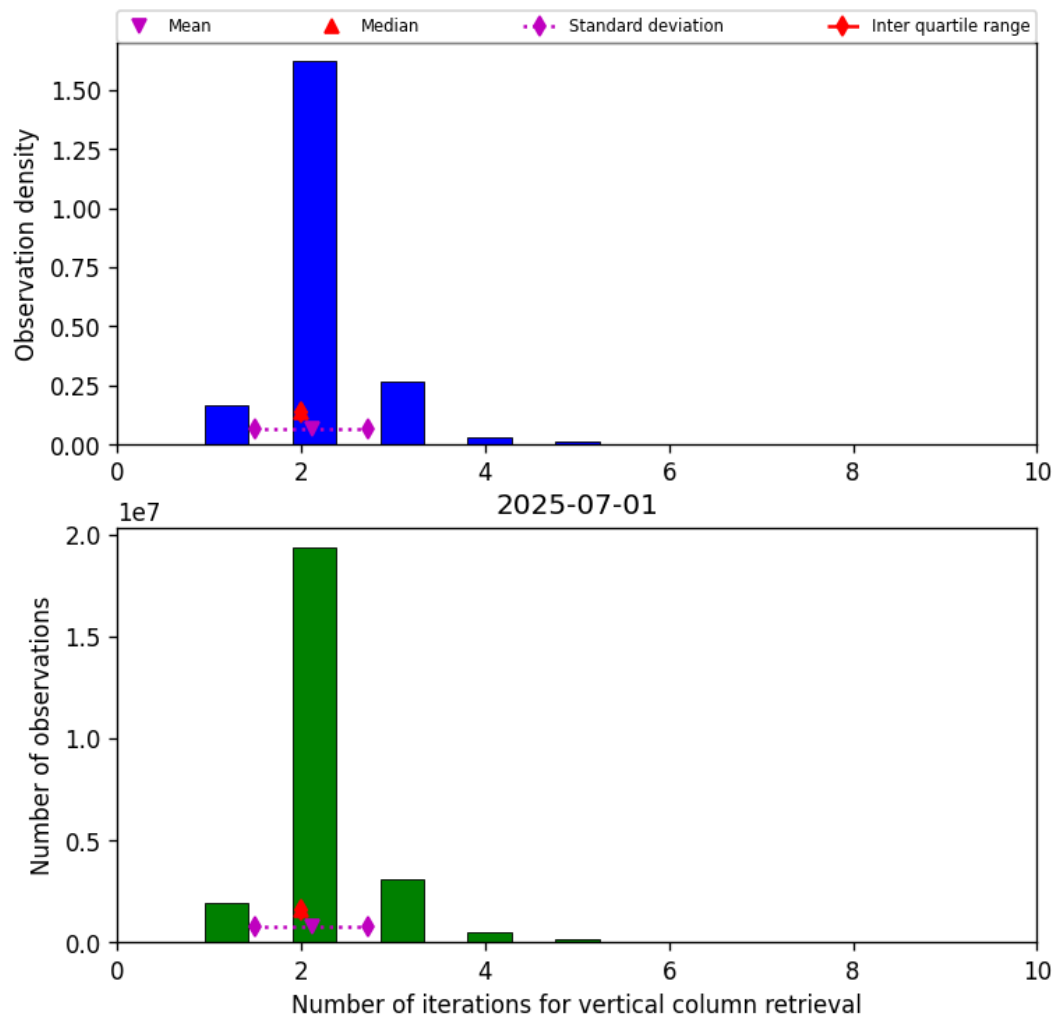
Figure 39: Histogram of “Number of iterations for vertical column retrieval” for 2025-07-01 to 2025-07-02
