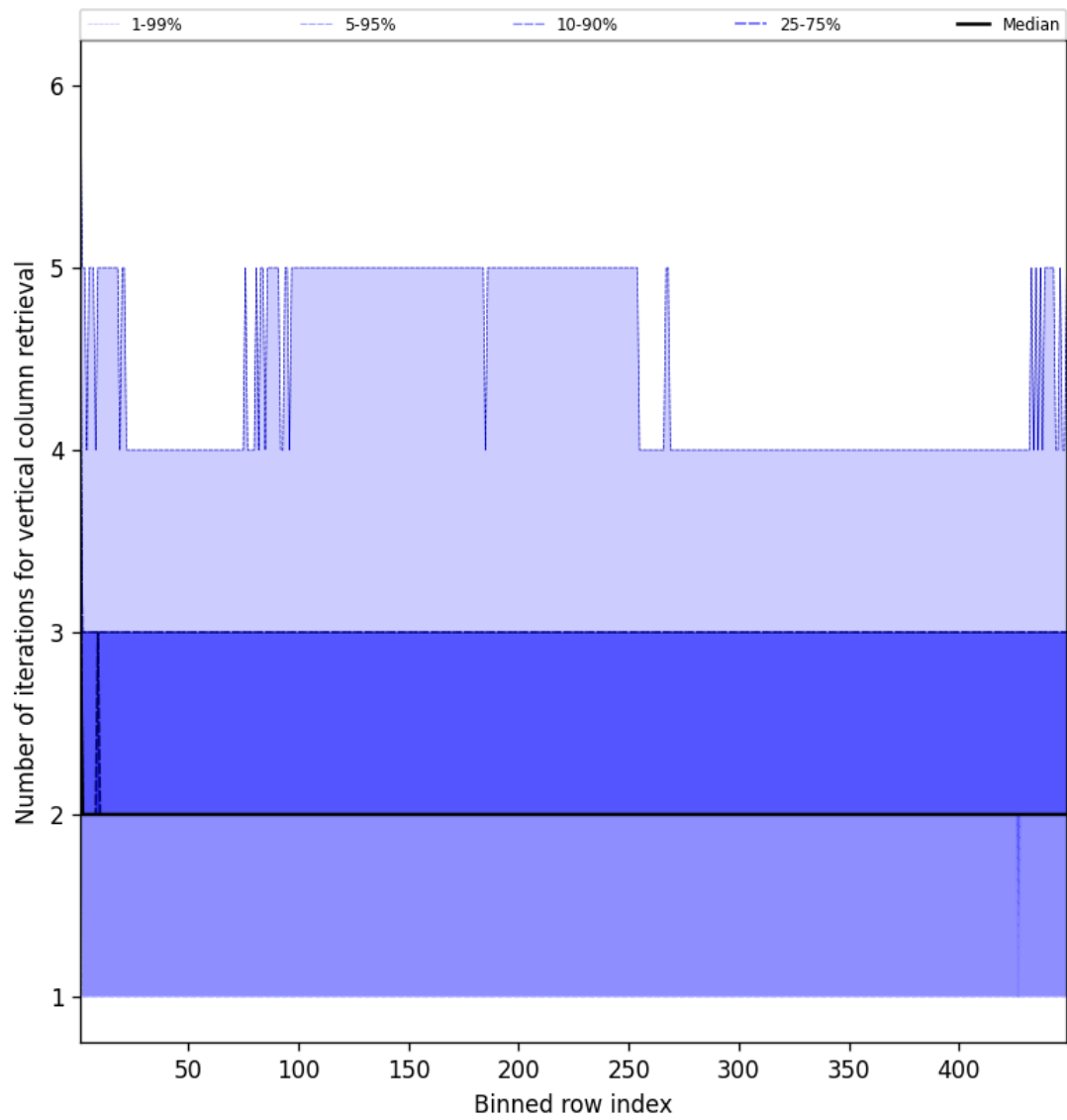
Figure 51: Along track statistics of “Number of iterations for vertical column retrieval” for 2025-07-01 to 2025-07-02
