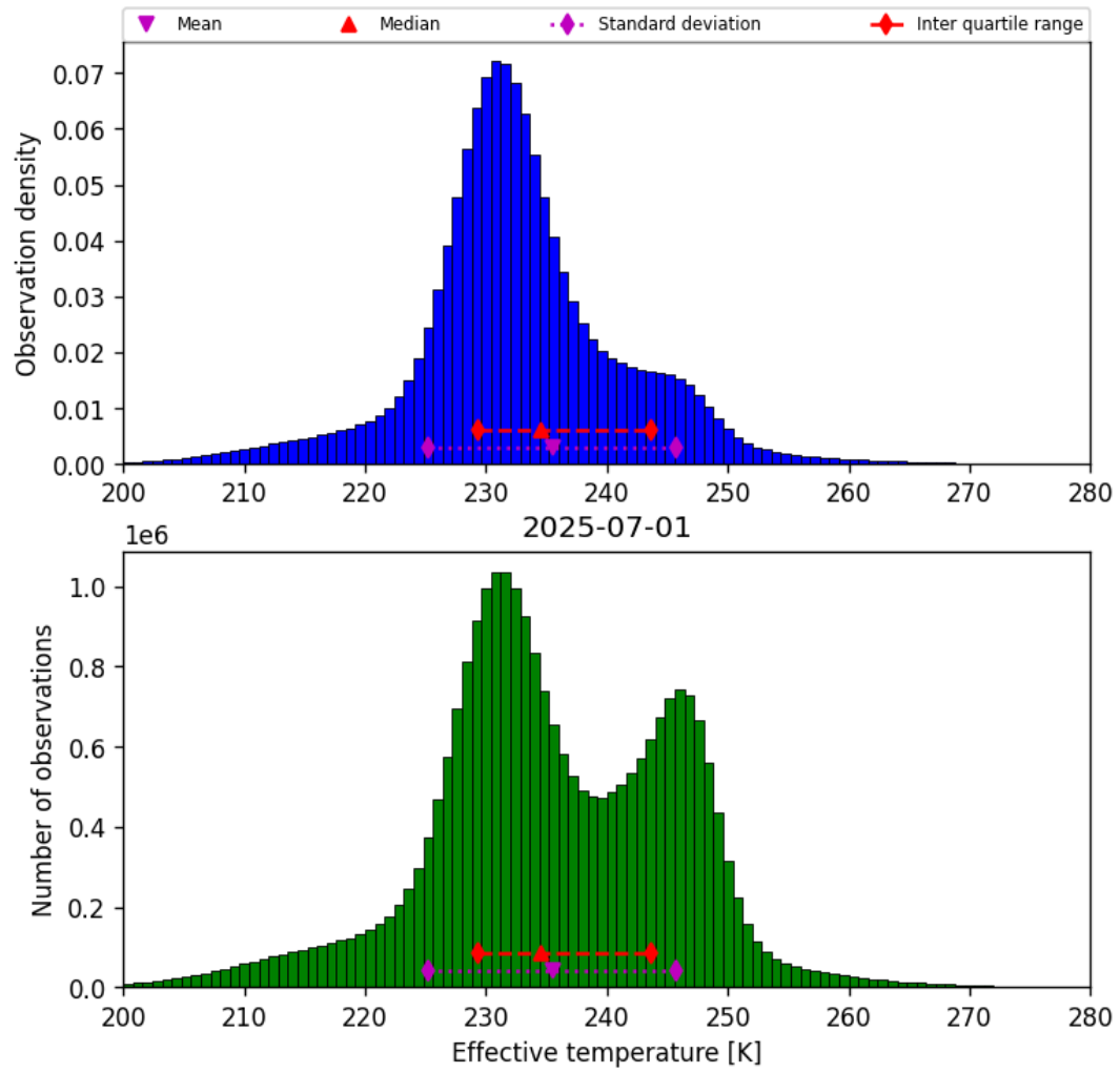
Figure 38: Histogram of “Effective temperature” for 2025-07-01 to 2025-07-02
