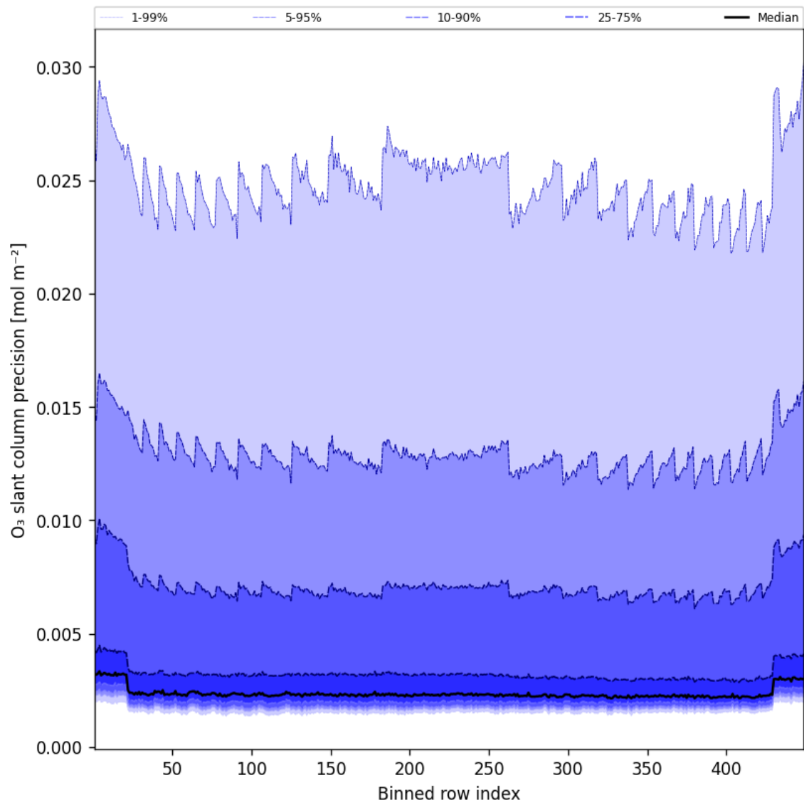
Figure 44: Along track statistics of “O 3 slant column precision” for 2025-07-01 to 2025-07-02
