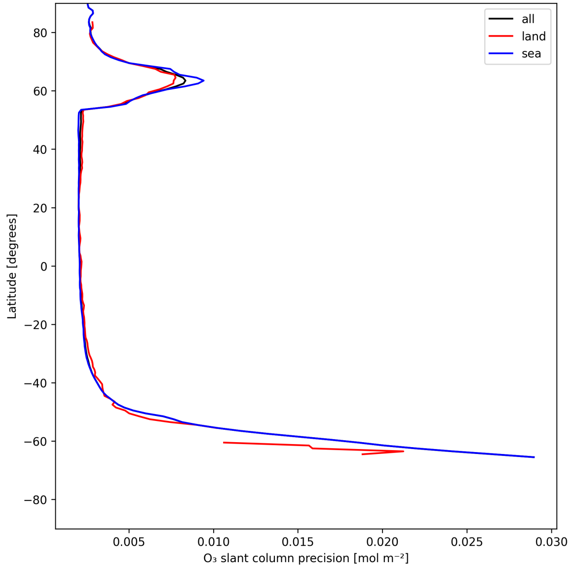
Figure 20: Zonal average of “O 3 slant column precision” for 2025-07-01 to 2025-07-02.
