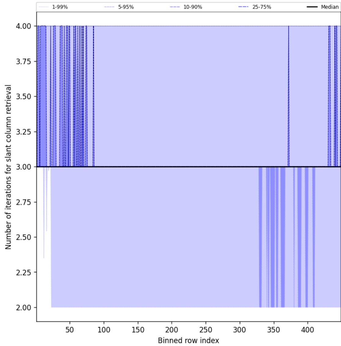
Figure 45: Along track statistics of “Number of iterations for slant column retrieval” for 2025-07-01 to 2025-07-02
