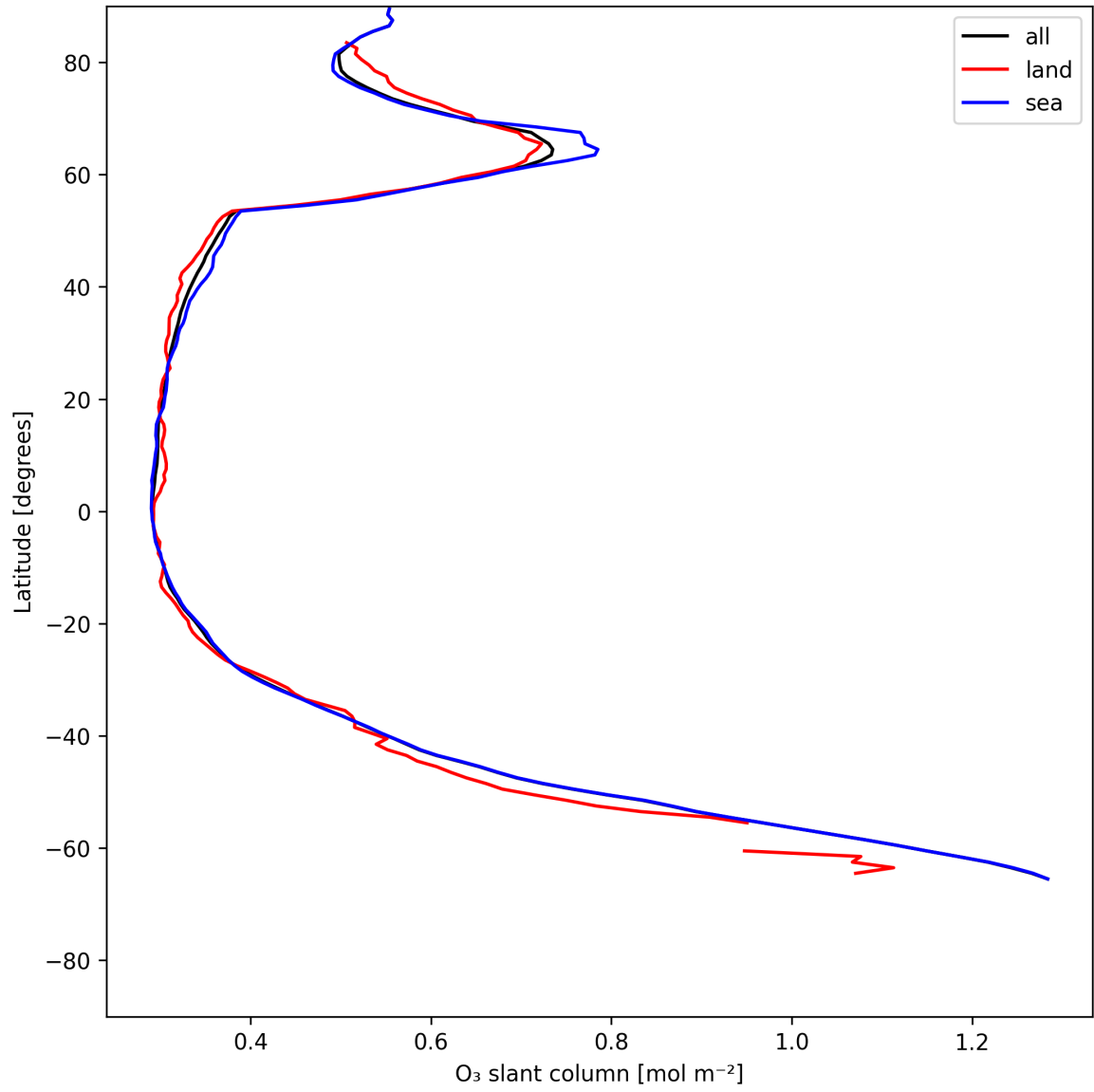
Figure 19: Zonal average of “O 3 slant column” for 2025-07-01 to 2025-07-02.
