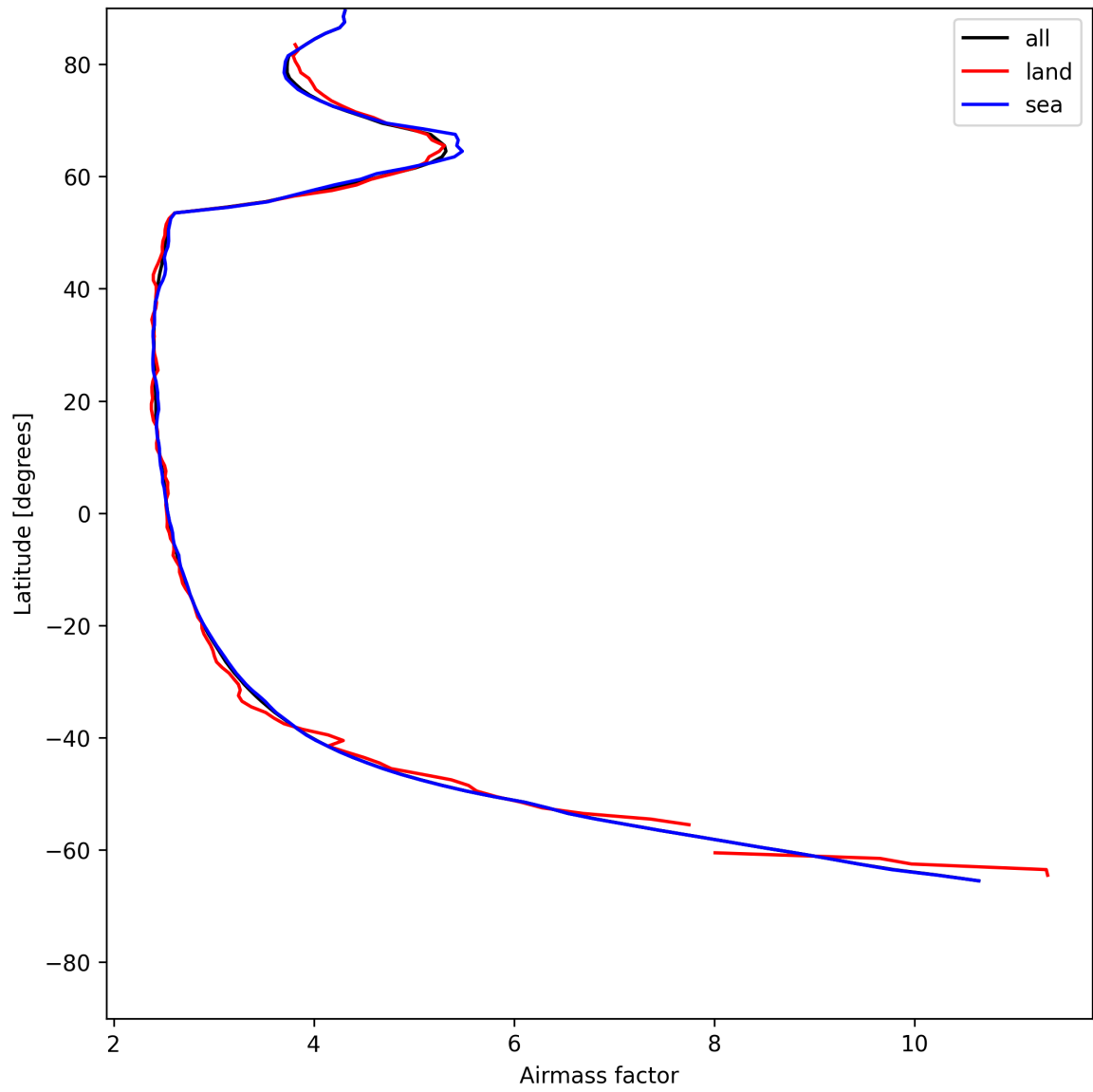
Figure 25: Zonal average of “Airmass factor” for 2025-07-01 to 2025-07-02.
