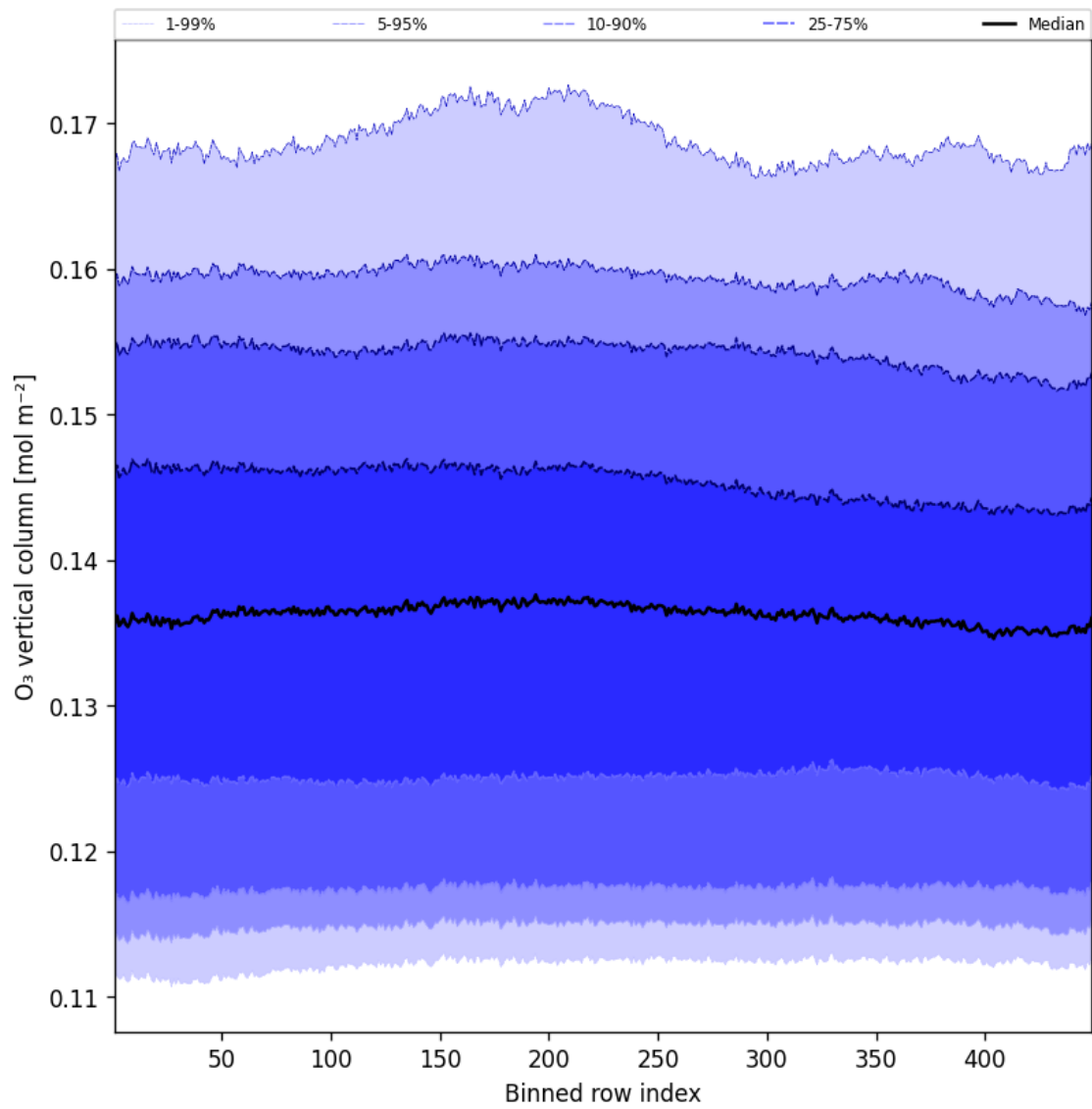
Figure 41: Along track statistics of “O 3 vertical column” for 2025-07-01 to 2025-07-02
