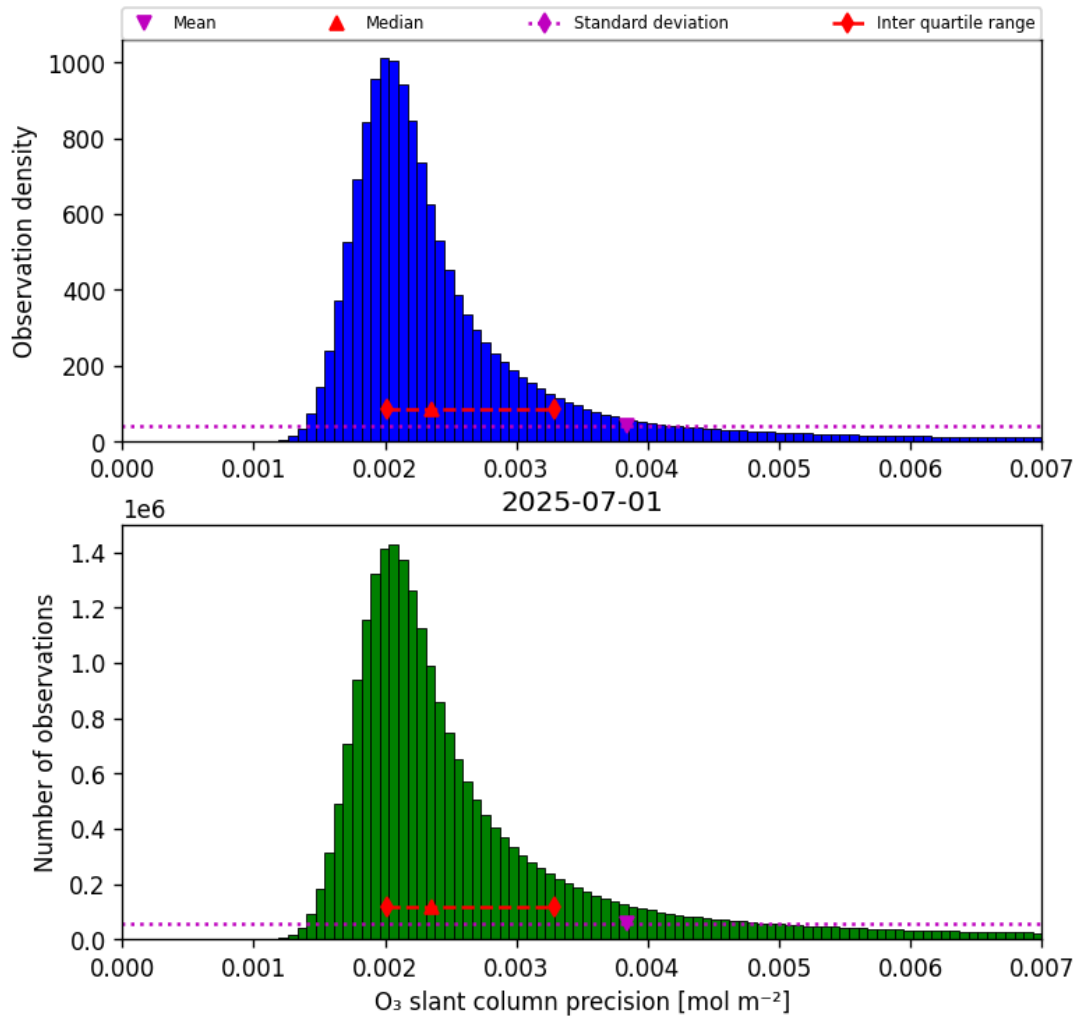
Figure 32: Histogram of “O 3 slant column precision” for 2025-07-01 to 2025-07-02
