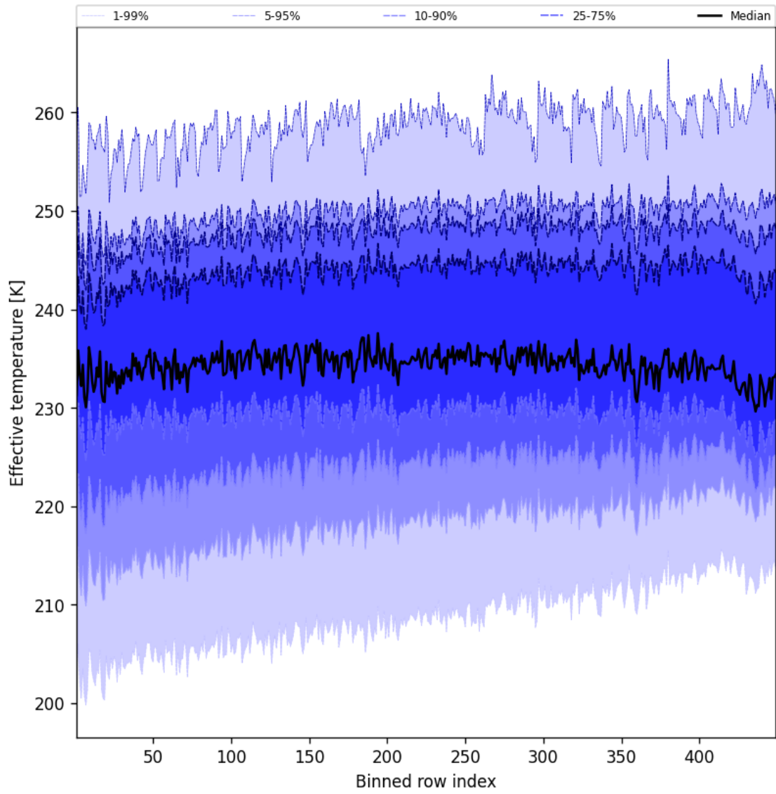
Figure 50: Along track statistics of “Effective temperature” for 2025-07-01 to 2025-07-02
