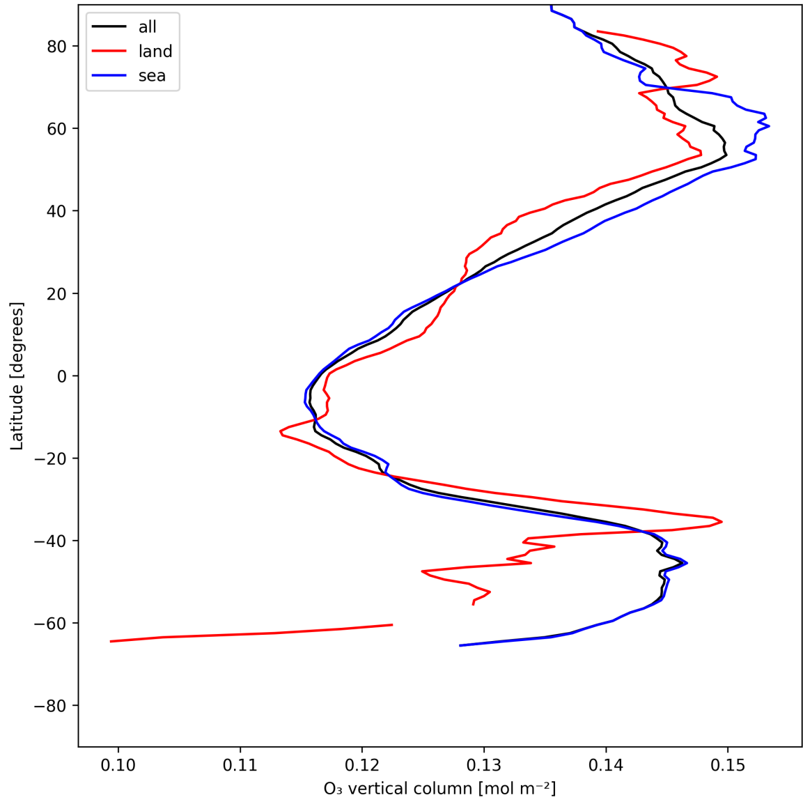
Figure 17: Zonal average of “O 3 vertical column” for 2025-07-01 to 2025-07-02.
