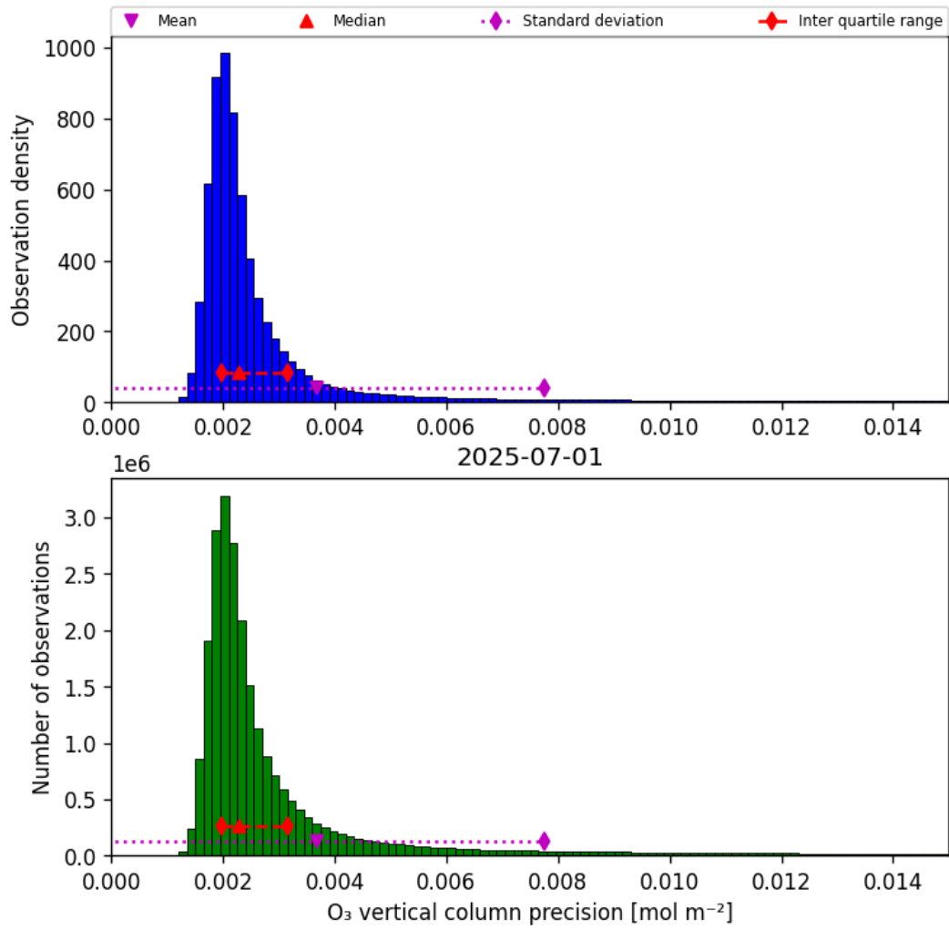
Figure 30: Histogram of “O 3 vertical column precision” for 2025-07-01 to 2025-07-02
