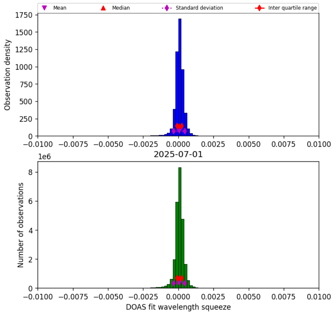
Figure 36: Histogram of “DOAS fit wavelength squeeze” for 2025-07-01 to 2025-07-02
