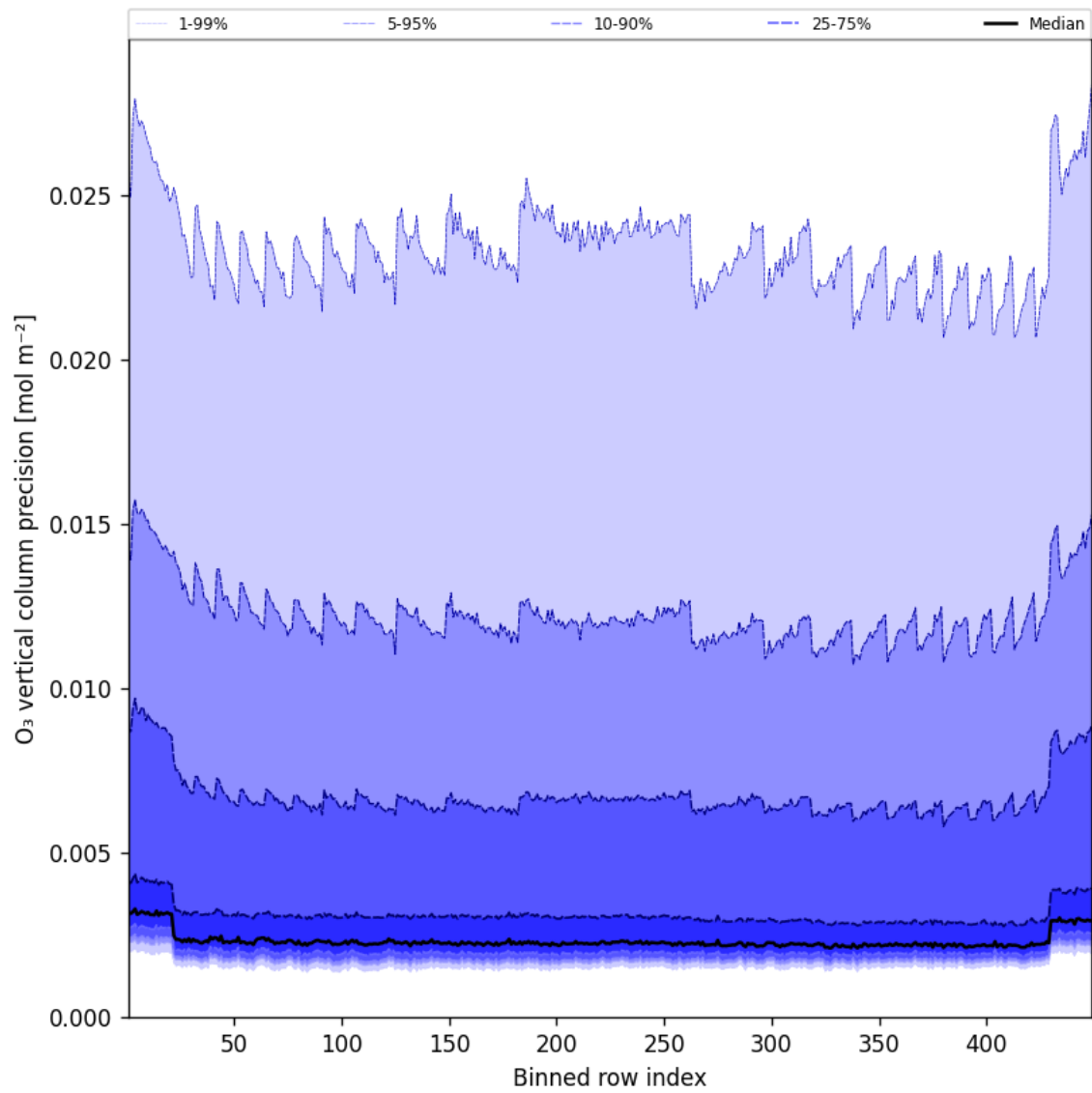
Figure 42: Along track statistics of “O 3 vertical column precision” for 2025-07-01 to 2025-07-02
