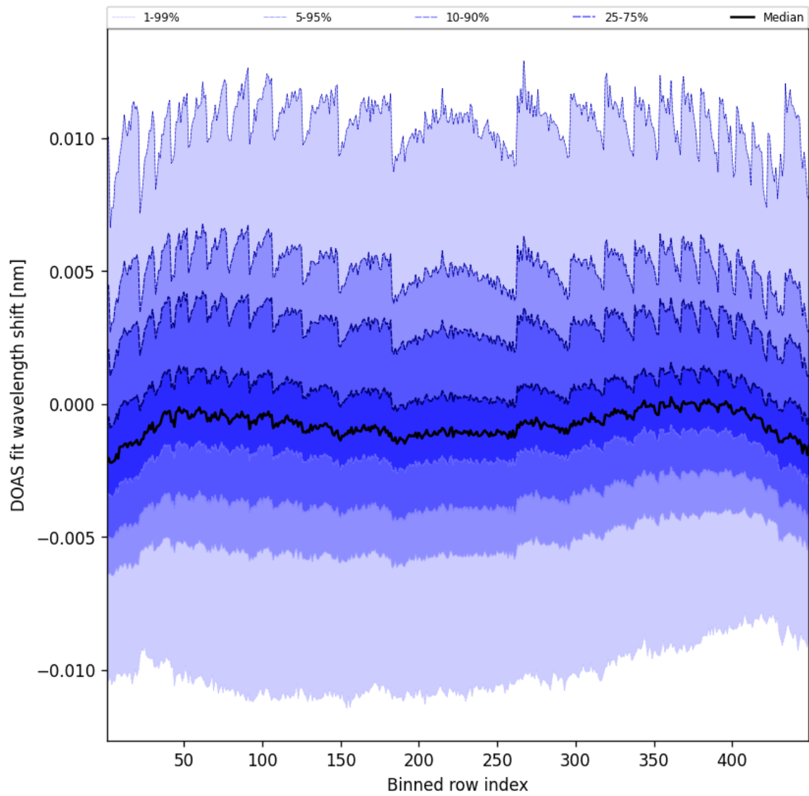
Figure 47: Along track statistics of “DOAS fit wavelength shift” for 2025-07-01 to 2025-07-02
