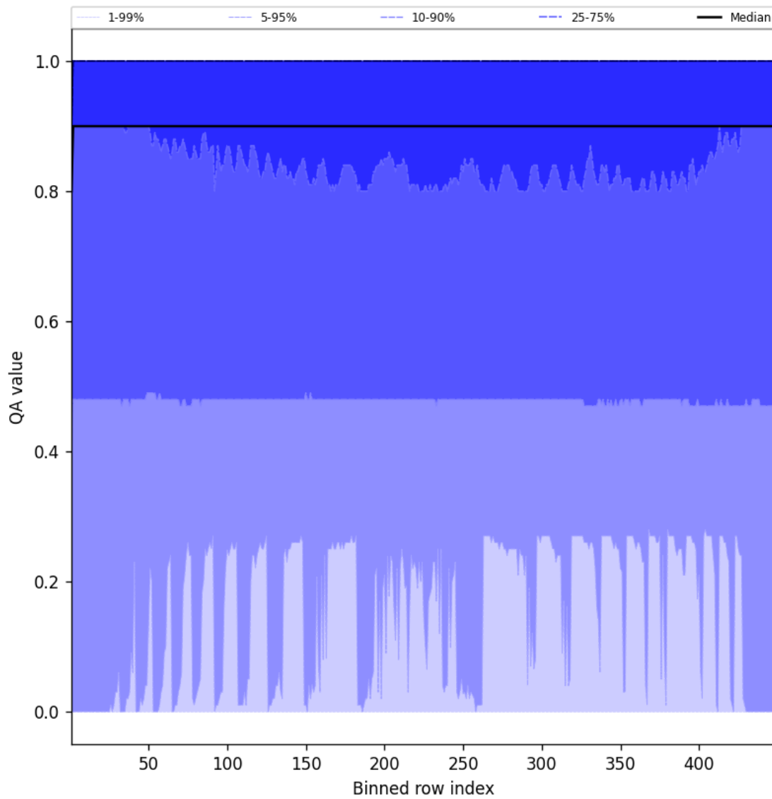
Figure 40: Along track statistics of “QA value” for 2025-07-01 to 2025-07-02
