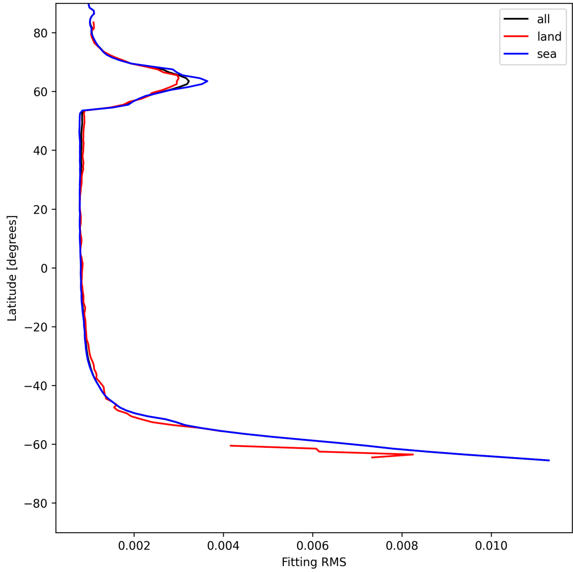
Figure 22: Zonal average of “Fitting RMS” for 2025-07-01 to 2025-07-02.
