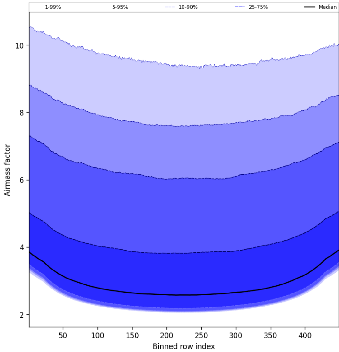
Figure 49: Along track statistics of “Airmass factor” for 2025-07-01 to 2025-07-02
