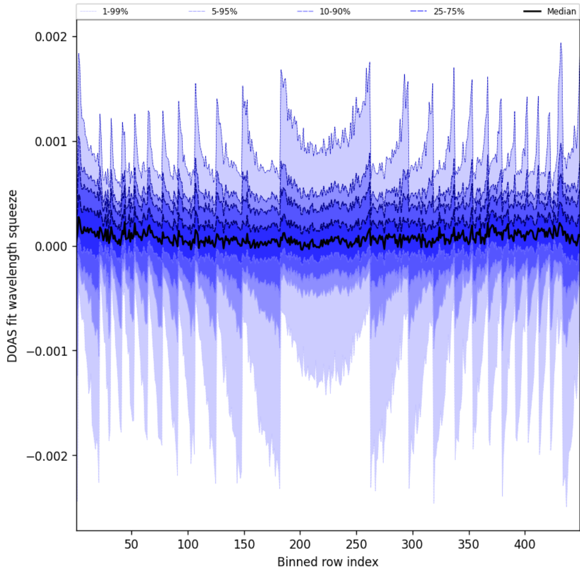
Figure 48: Along track statistics of “DOAS fit wavelength squeeze” for 2025-07-01 to 2025-07-02
