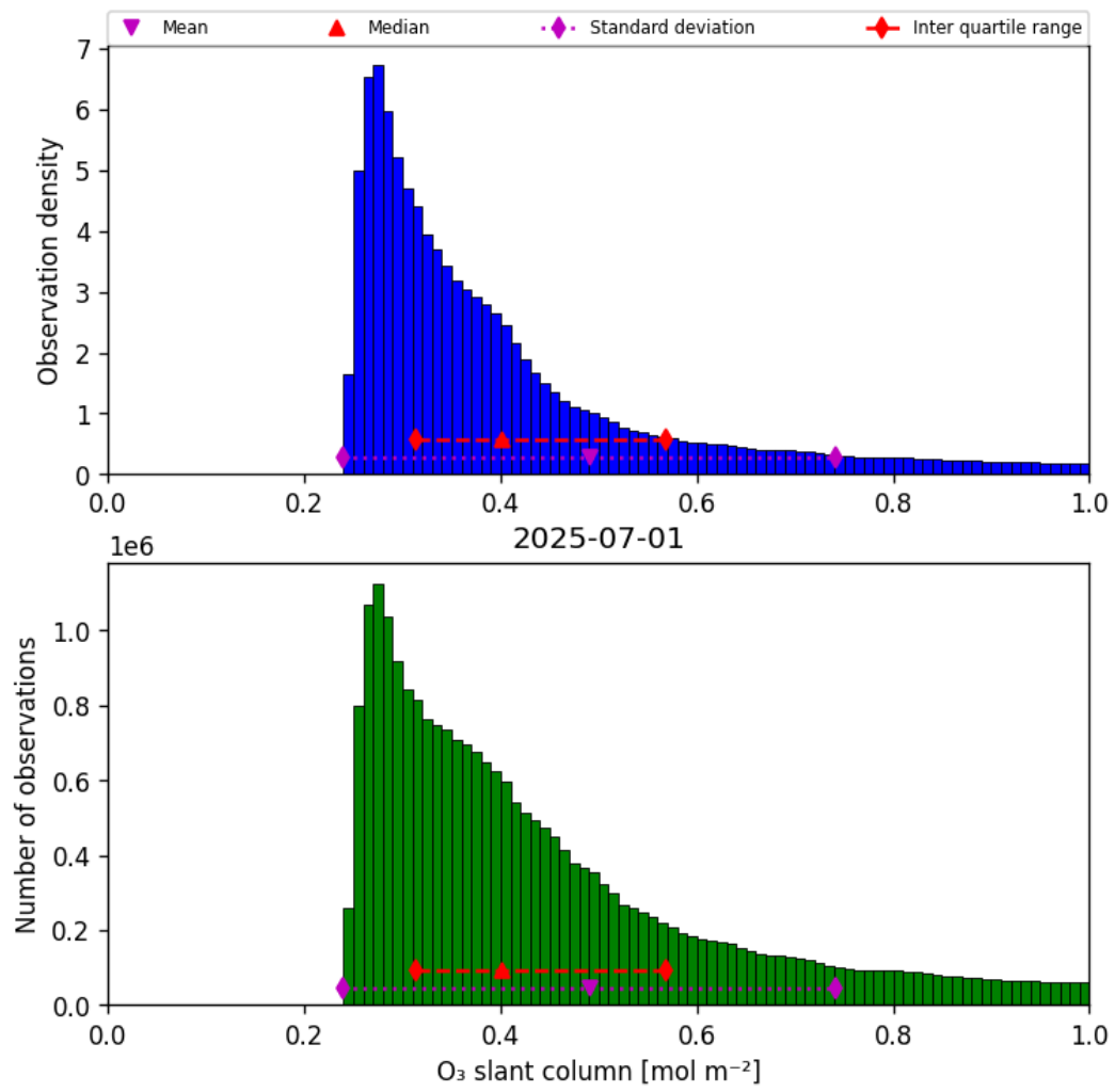
Figure 31: Histogram of “O 3 slant column” for 2025-07-01 to 2025-07-02
