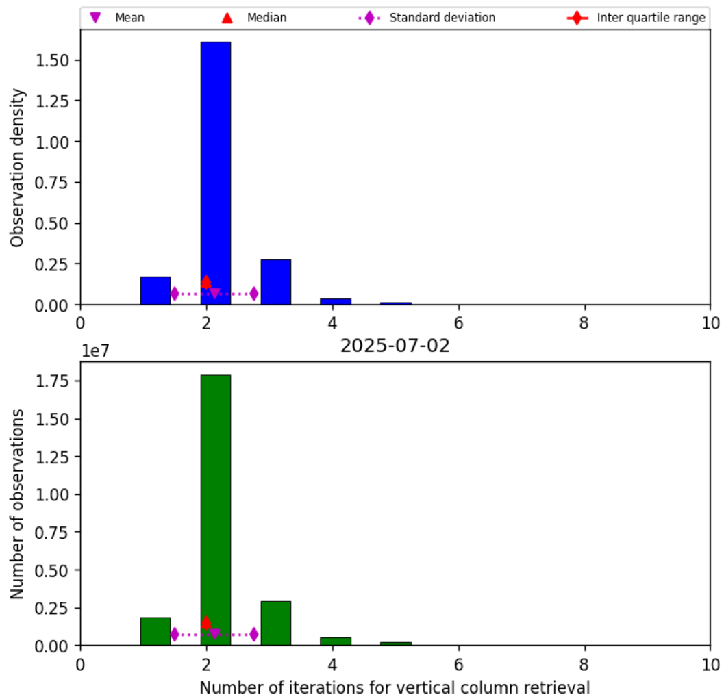
Figure 39: Histogram of “Number of iterations for vertical column retrieval” for 2025-07-02 to 2025-07-03
