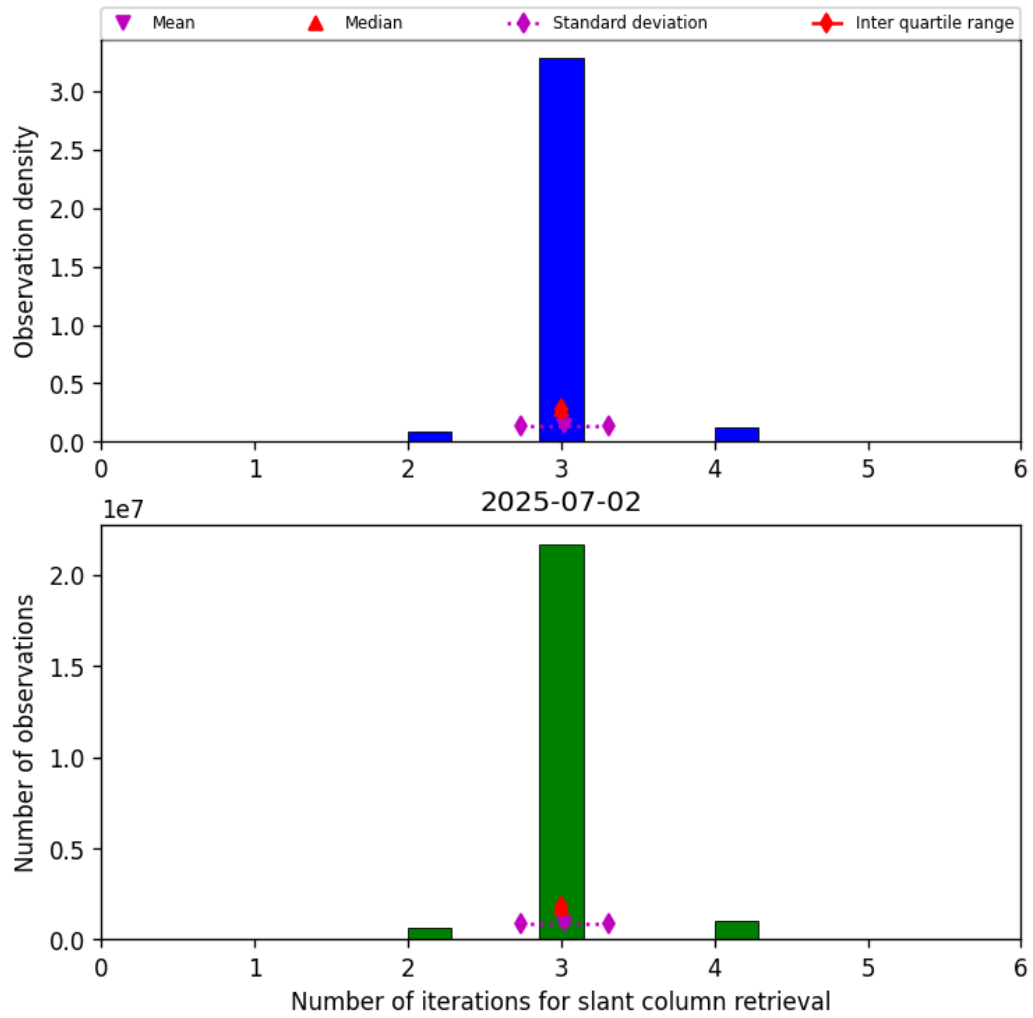
Figure 33: Histogram of “Number of iterations for slant column retrieval” for 2025-07-02 to 2025-07-03
