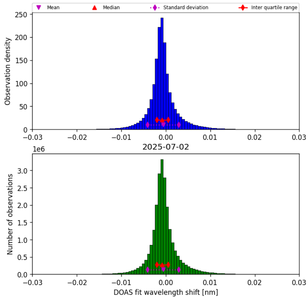
Figure 35: Histogram of “DOAS fit wavelength shift” for 2025-07-02 to 2025-07-03
