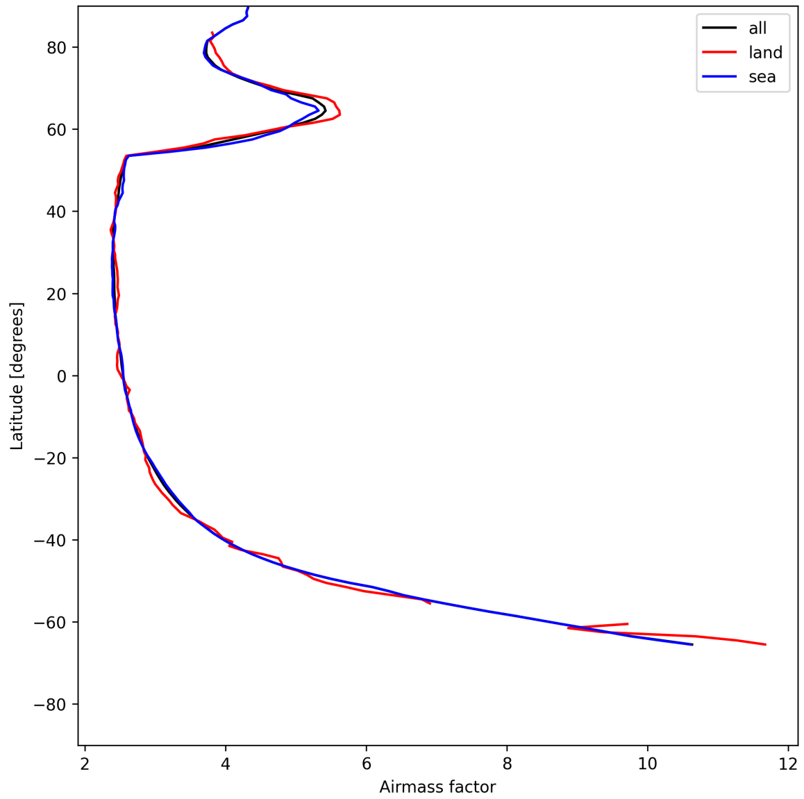
Figure 25: Zonal average of “Airmass factor” for 2025-07-02 to 2025-07-03.
