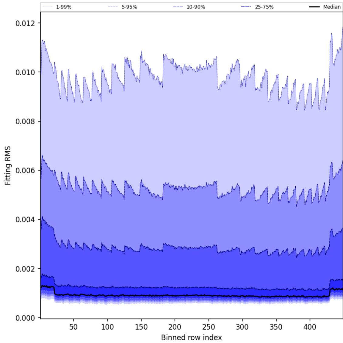
Figure 46: Along track statistics of “Fitting RMS” for 2025-07-02 to 2025-07-03
