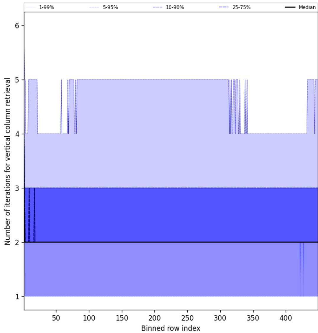
Figure 51: Along track statistics of “Number of iterations for vertical column retrieval” for 2025-07-02 to 2025-07-03
