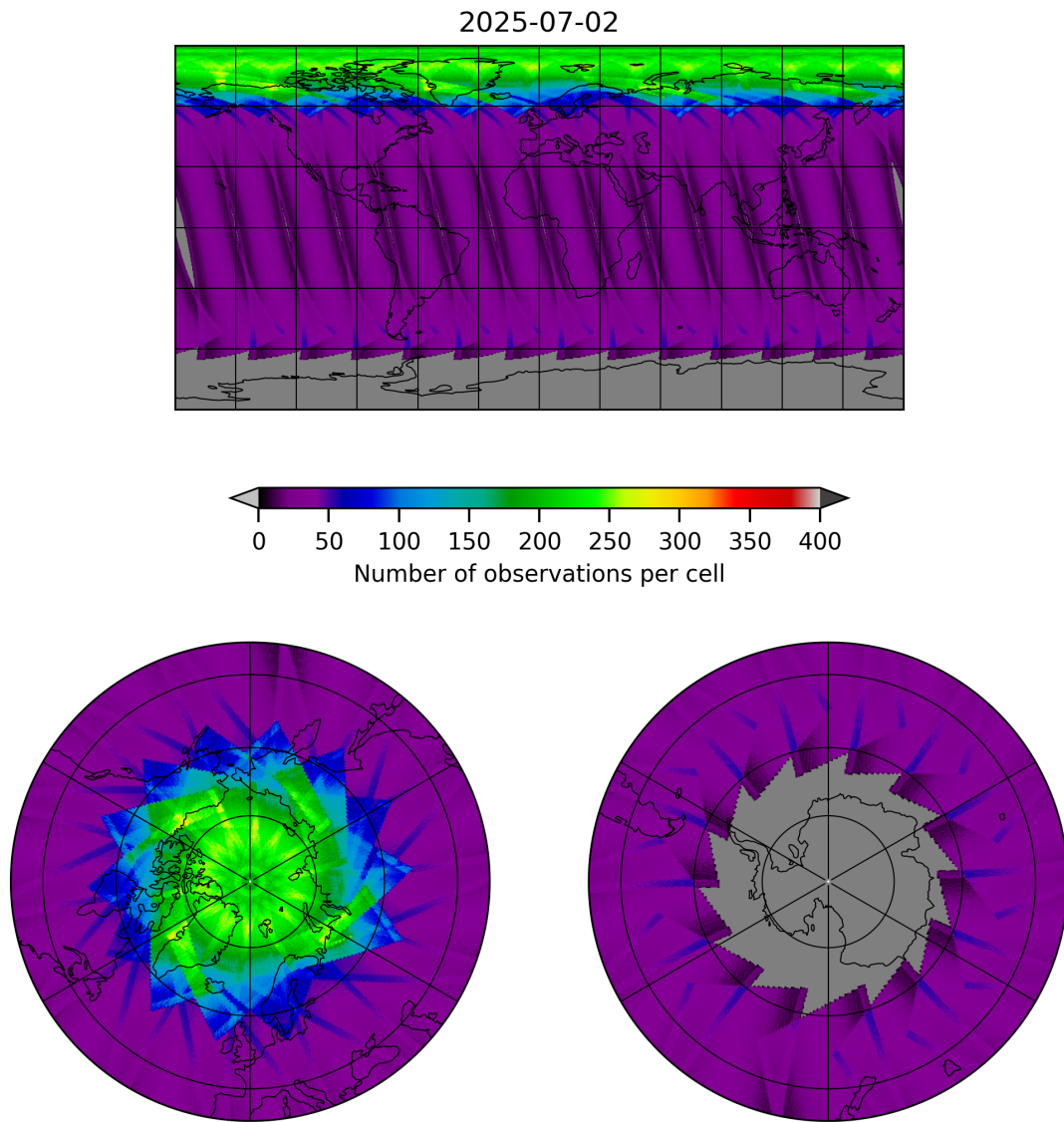
Figure 15: Map of the number of observations for 2025-07-02 to 2025-07-03
