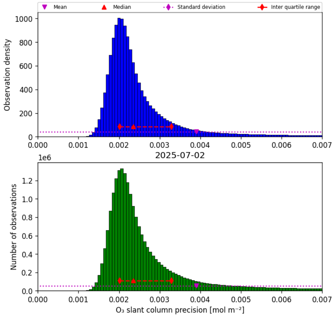
Figure 32: Histogram of “O 3 slant column precision” for 2025-07-02 to 2025-07-03
