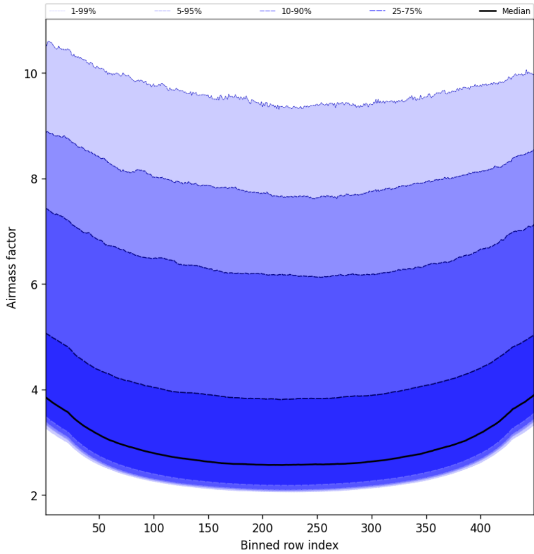
Figure 49: Along track statistics of “Airmass factor” for 2025-07-02 to 2025-07-03
