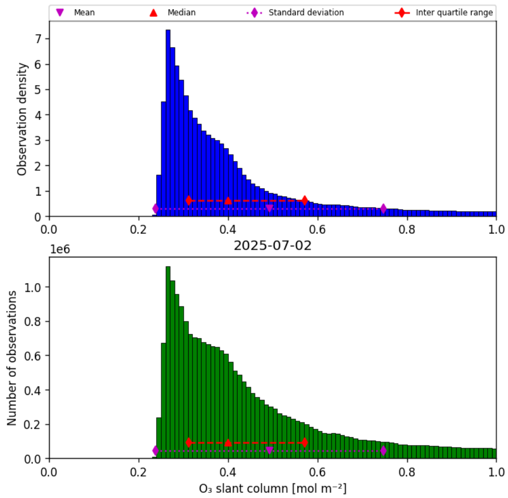
Figure 31: Histogram of “O 3 slant column” for 2025-07-02 to 2025-07-03
