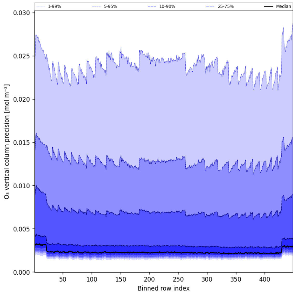
Figure 42: Along track statistics of “O 3 vertical column precision” for 2025-07-02 to 2025-07-03
