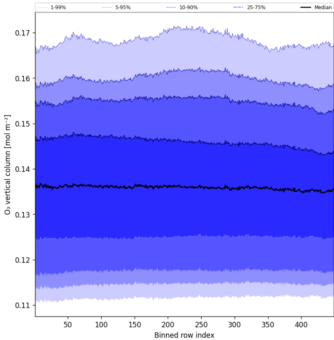
Figure 41: Along track statistics of “O 3 vertical column” for 2025-07-02 to 2025-07-03
