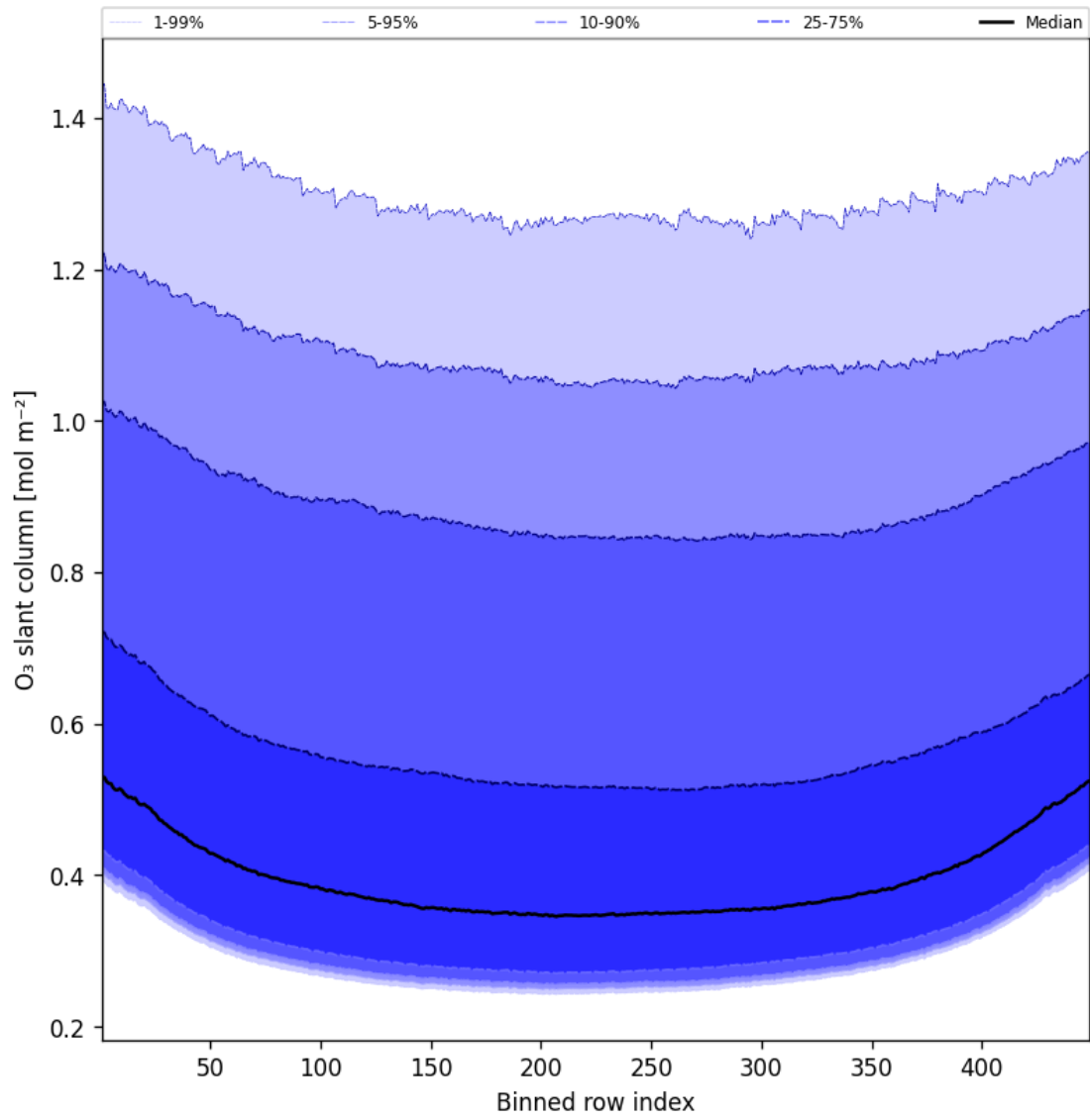
Figure 43: Along track statistics of “O 3 slant column” for 2025-07-02 to 2025-07-03
