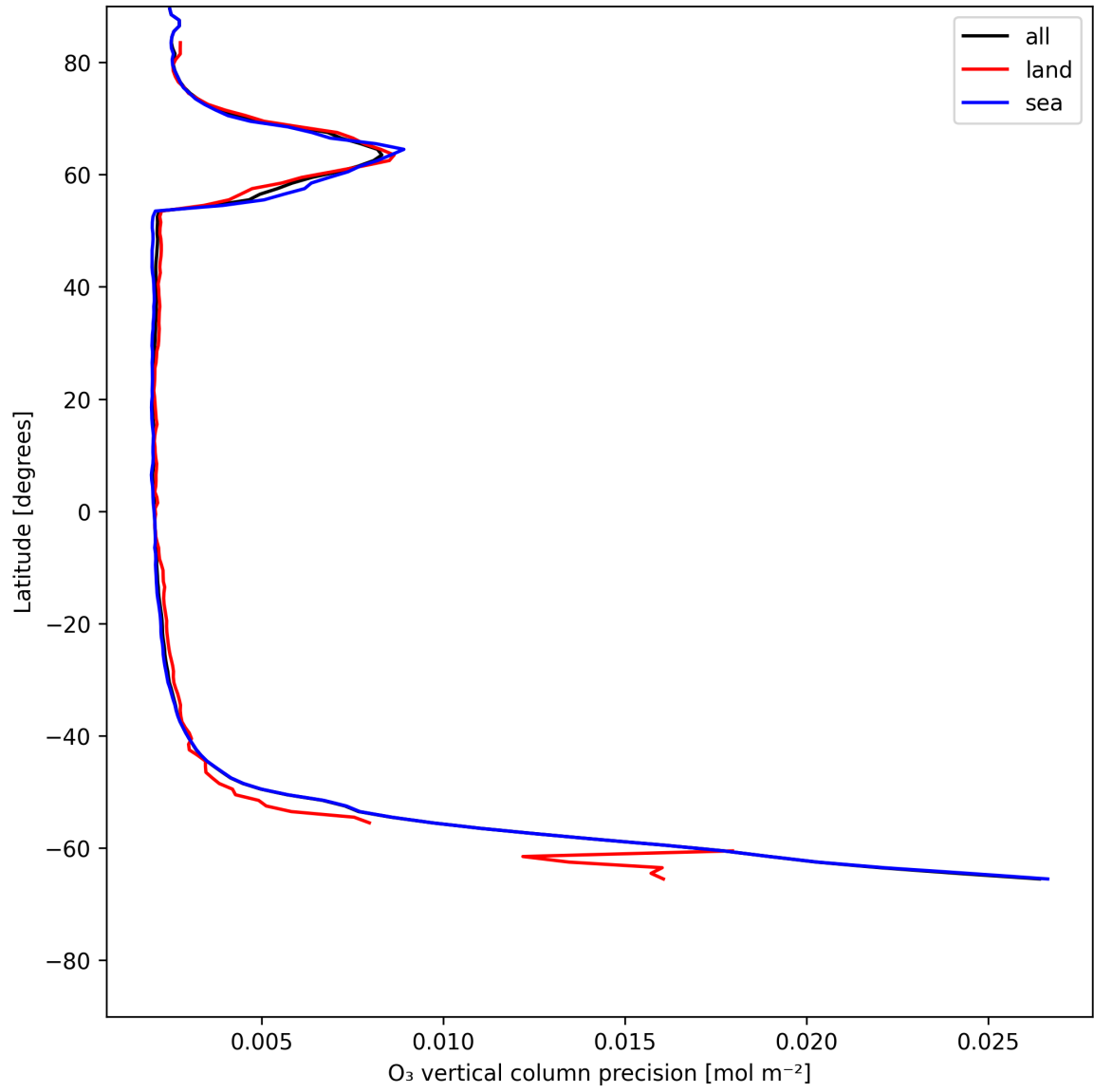
Figure 18: Zonal average of “O 3 vertical column precision” for 2025-07-02 to 2025-07-03.
