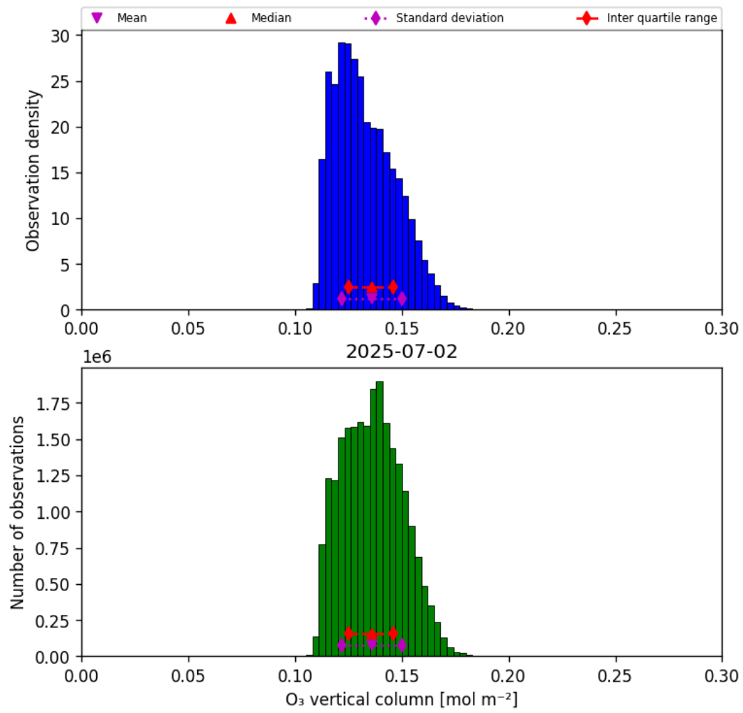
Figure 29: Histogram of “O 3 vertical column” for 2025-07-02 to 2025-07-03
