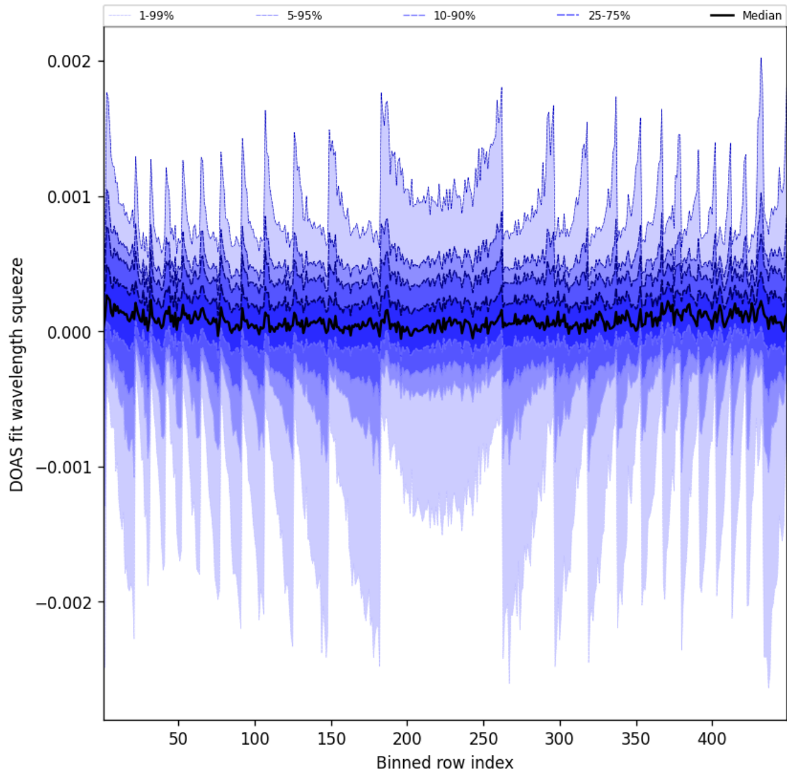
Figure 48: Along track statistics of “DOAS fit wavelength squeeze” for 2025-07-02 to 2025-07-03
