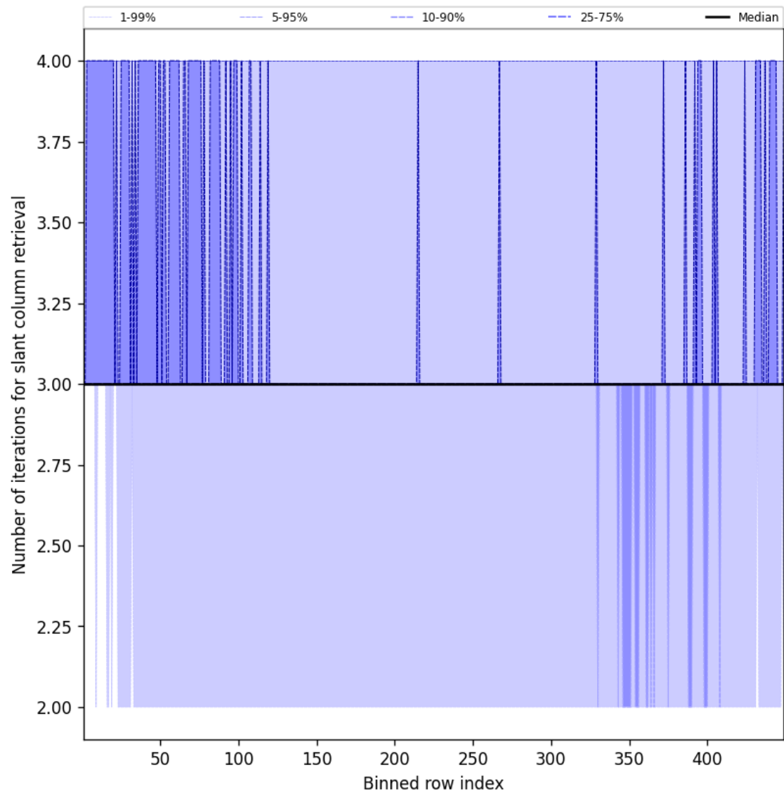
Figure 45: Along track statistics of “Number of iterations for slant column retrieval” for 2025-07-02 to 2025-07-03
