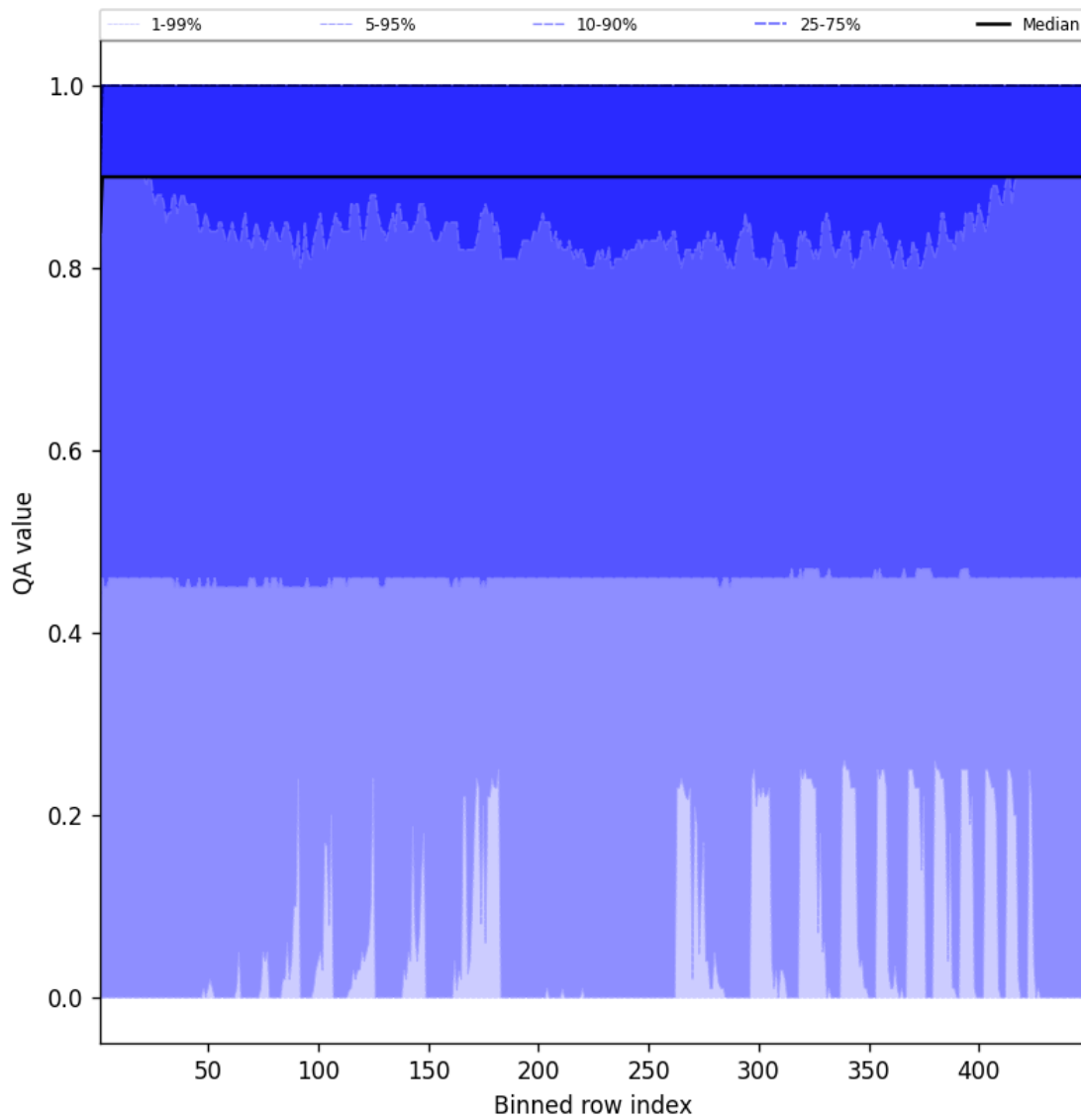
Figure 40: Along track statistics of “QA value” for 2025-07-02 to 2025-07-03
