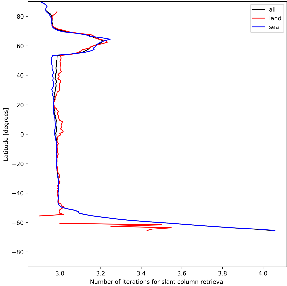
Figure 21: Zonal average of “Number of iterations for slant column retrieval” for 2025-07-02 to 2025-07-03.
