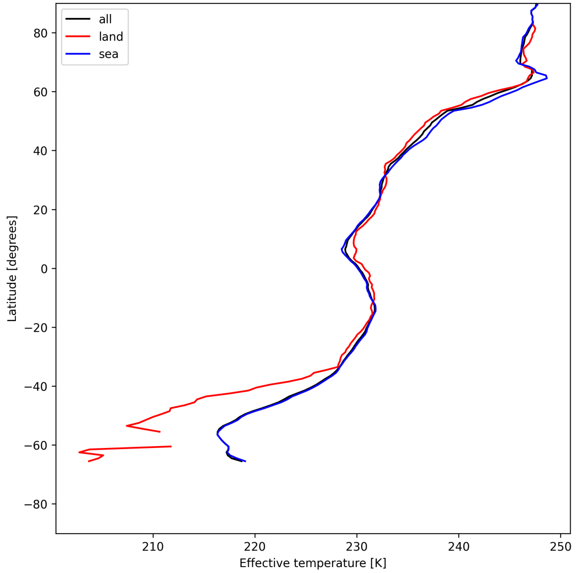
Figure 26: Zonal average of “Effective temperature” for 2025-07-02 to 2025-07-03.
