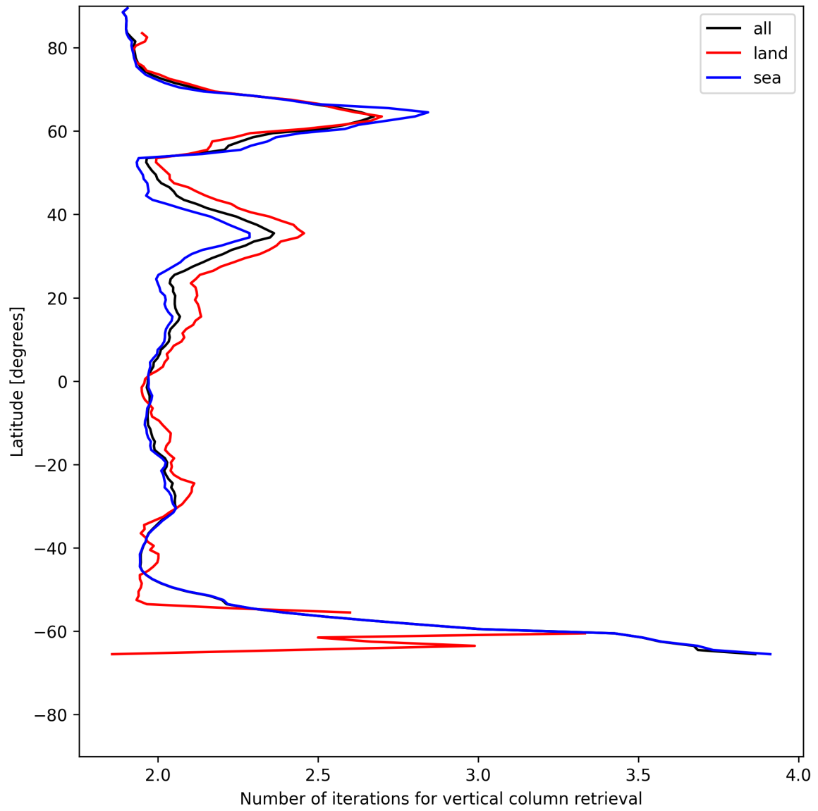
Figure 27: Zonal average of “Number of iterations for vertical column retrieval” for 2025-07-02 to 2025-07-03.
