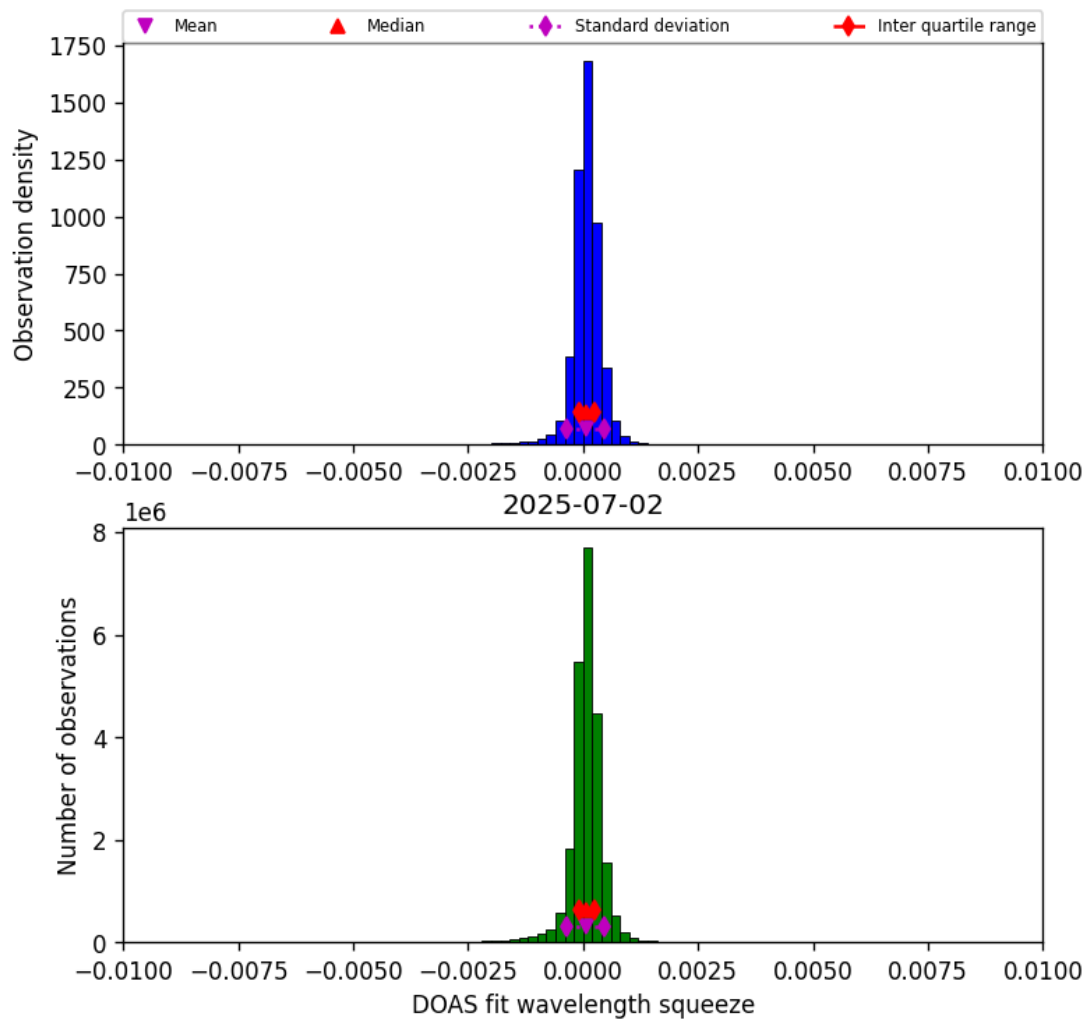
Figure 36: Histogram of “DOAS fit wavelength squeeze” for 2025-07-02 to 2025-07-03
