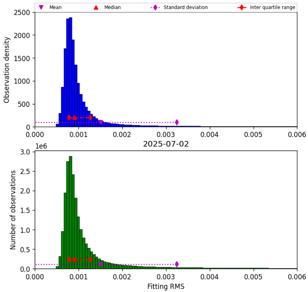
Figure 34: Histogram of “Fitting RMS” for 2025-07-02 to 2025-07-03
