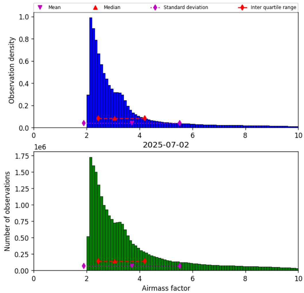
Figure 37: Histogram of “Airmass factor” for 2025-07-02 to 2025-07-03
