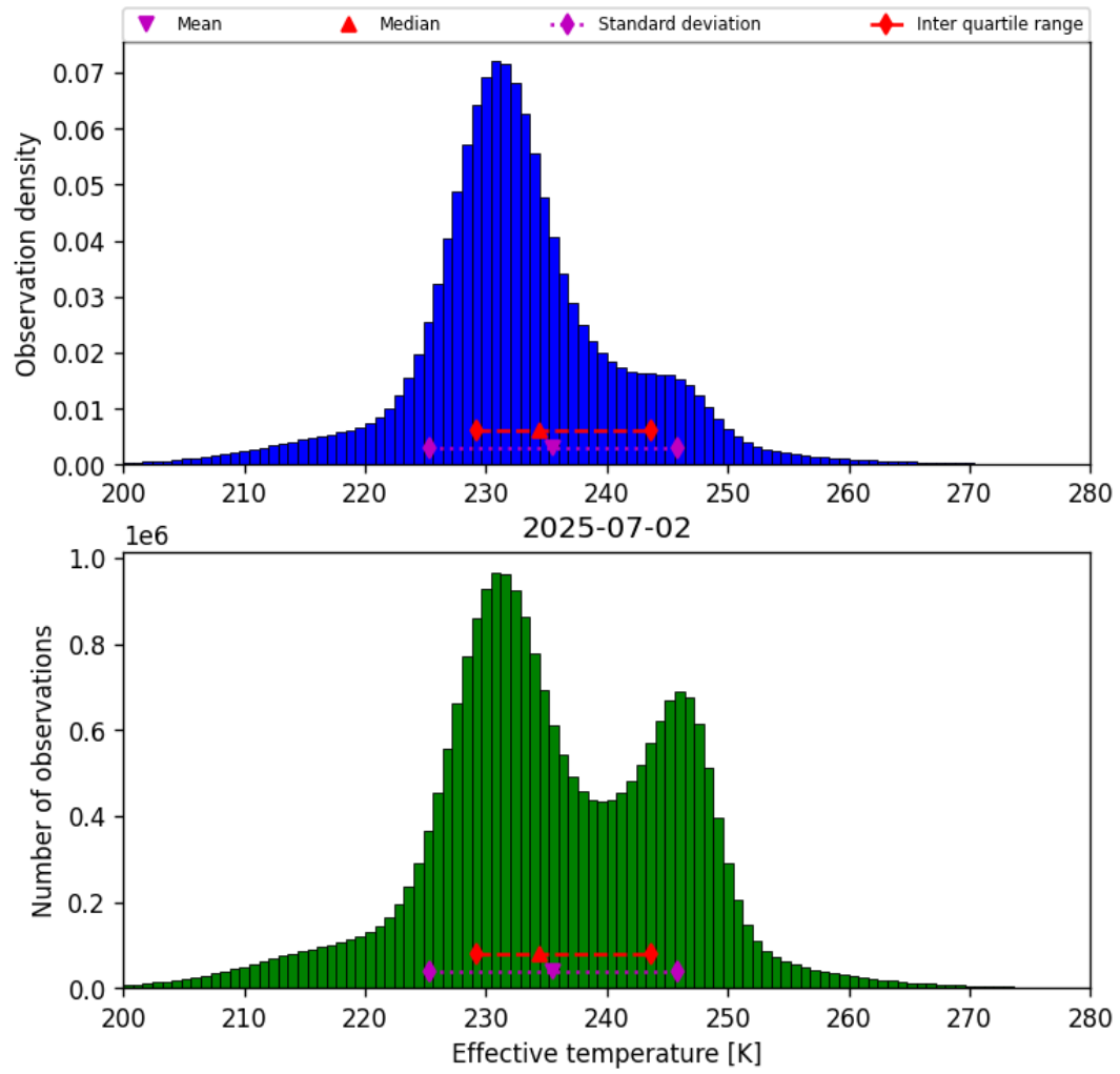
Figure 38: Histogram of “Effective temperature” for 2025-07-02 to 2025-07-03
