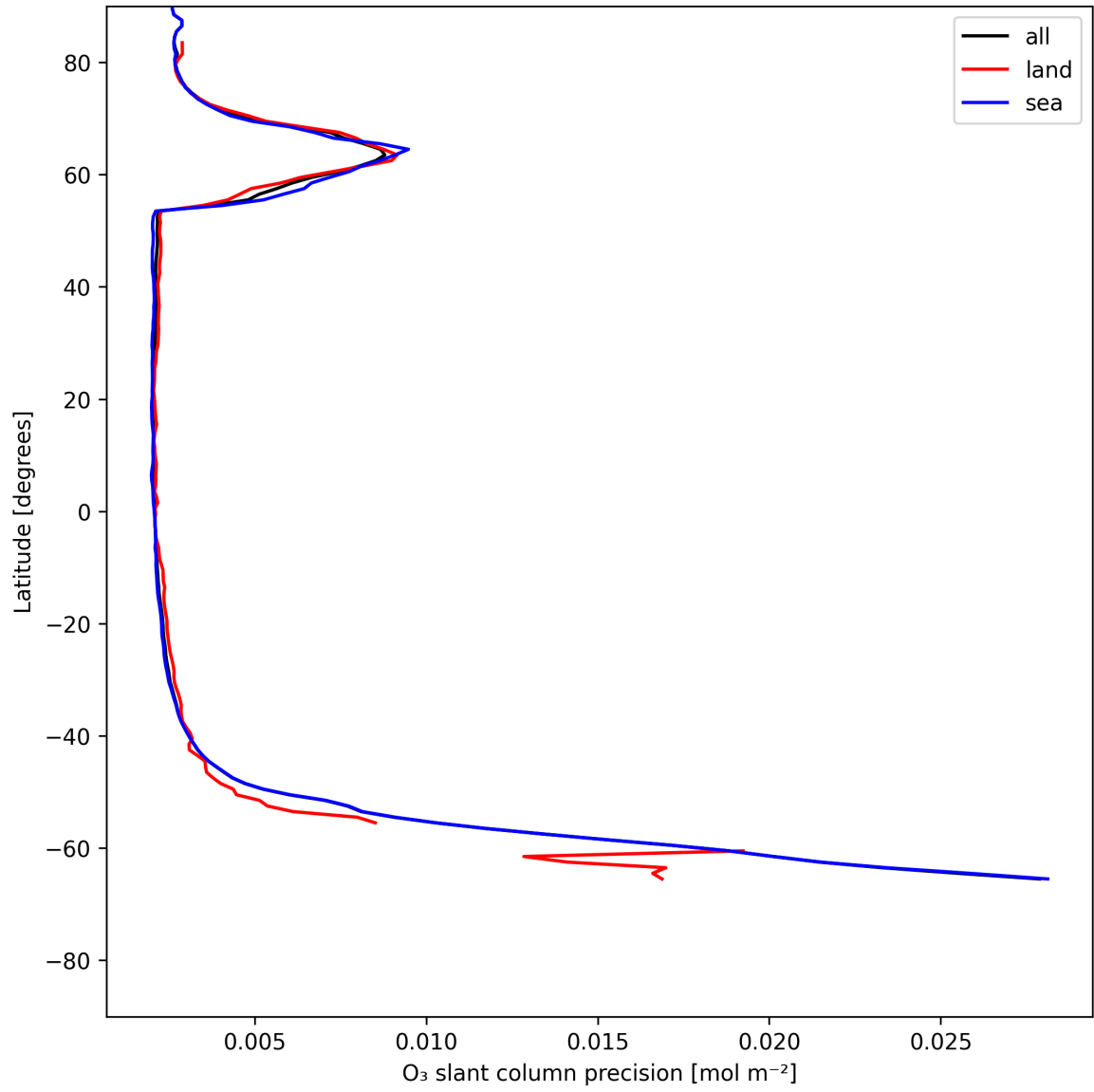
Figure 20: Zonal average of “O 3 slant column precision” for 2025-07-02 to 2025-07-03.
