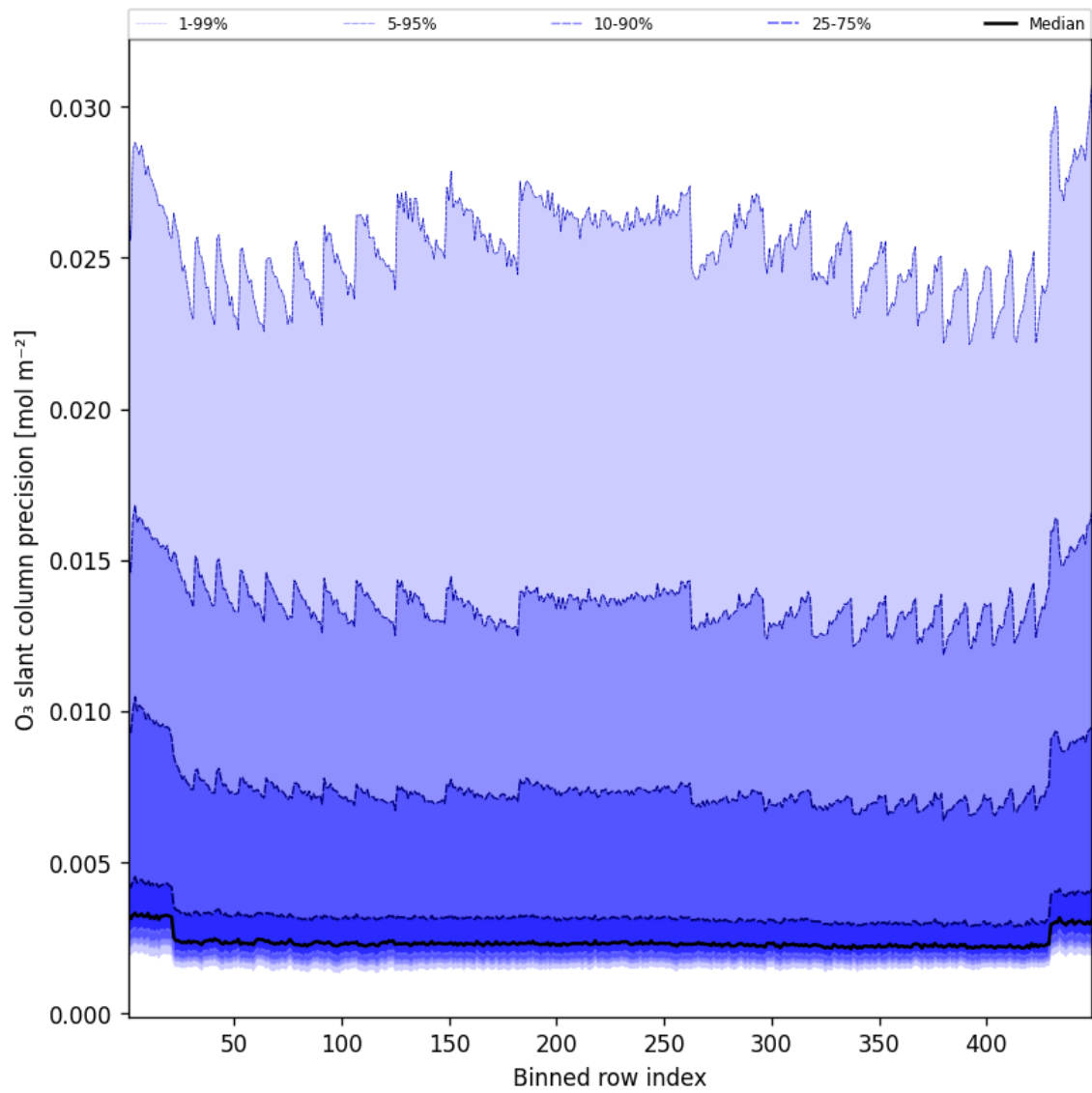
Figure 44: Along track statistics of “O 3 slant column precision” for 2025-07-02 to 2025-07-03
