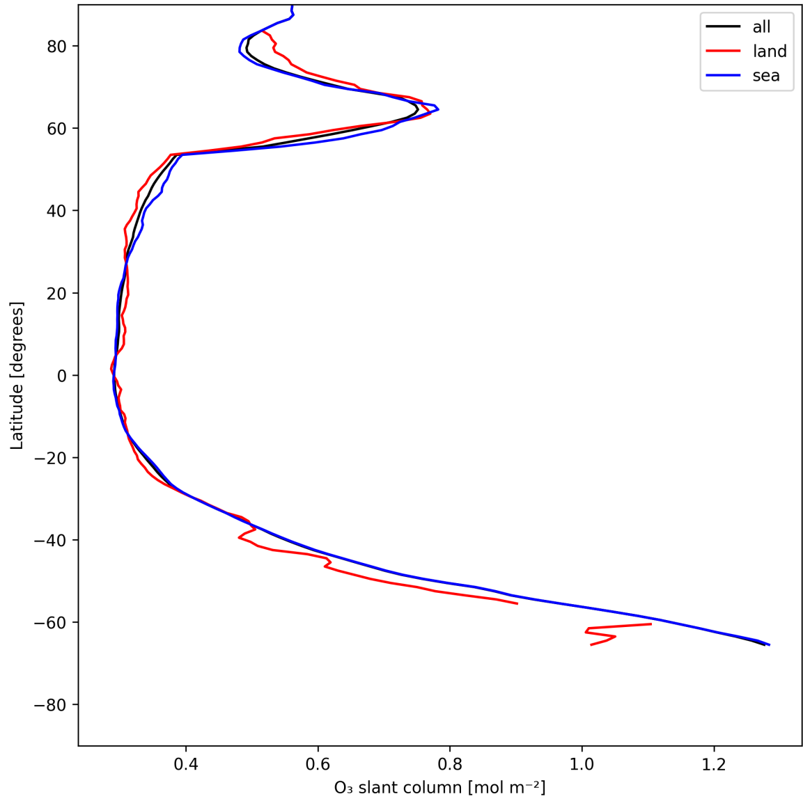
Figure 19: Zonal average of “O 3 slant column” for 2025-07-02 to 2025-07-03.
