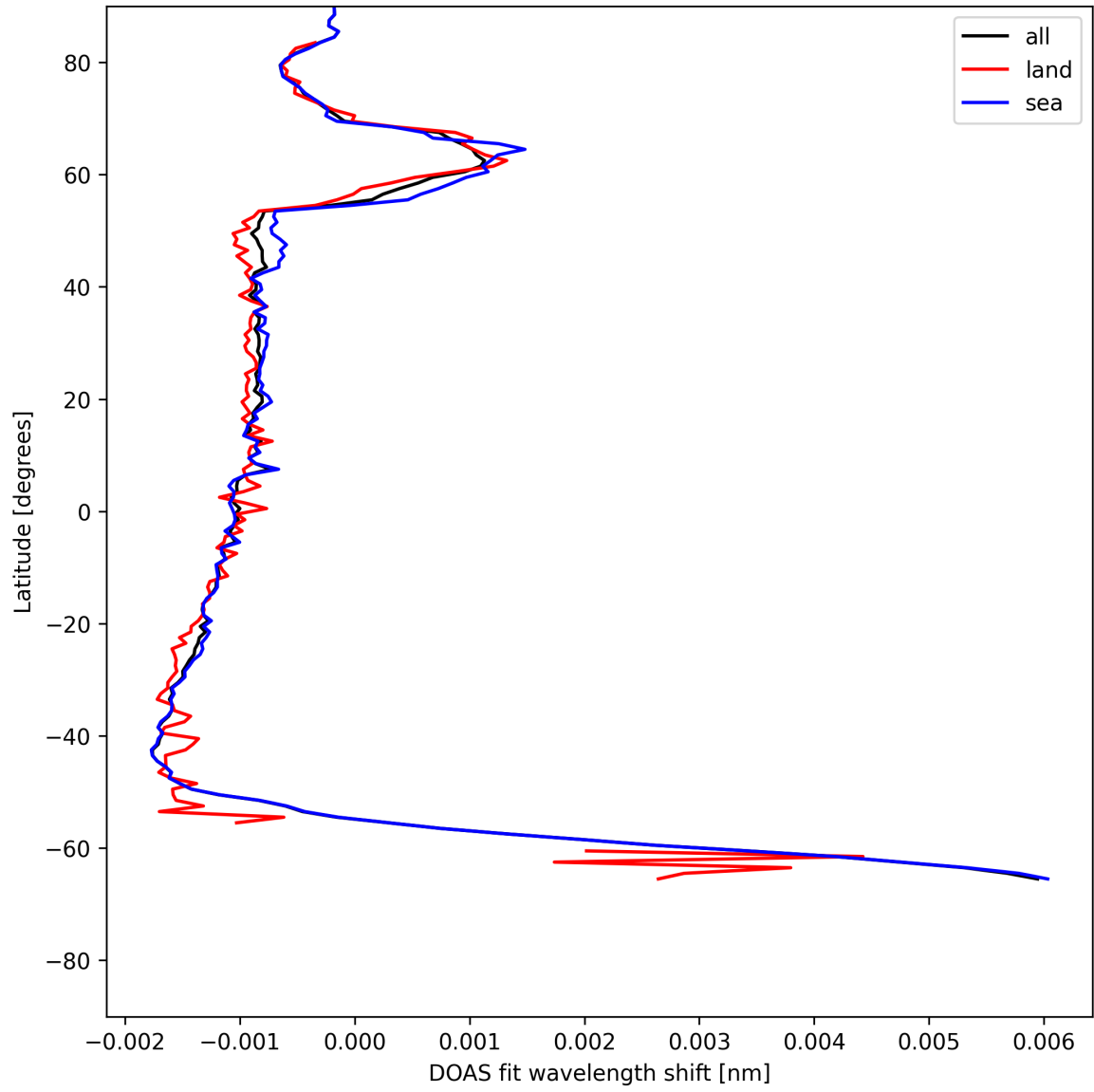
Figure 23: Zonal average of “DOAS fit wavelength shift” for 2025-07-02 to 2025-07-03.
