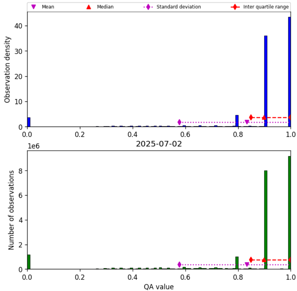
Figure 28: Histogram of “QA value” for 2025-07-02 to 2025-07-03
