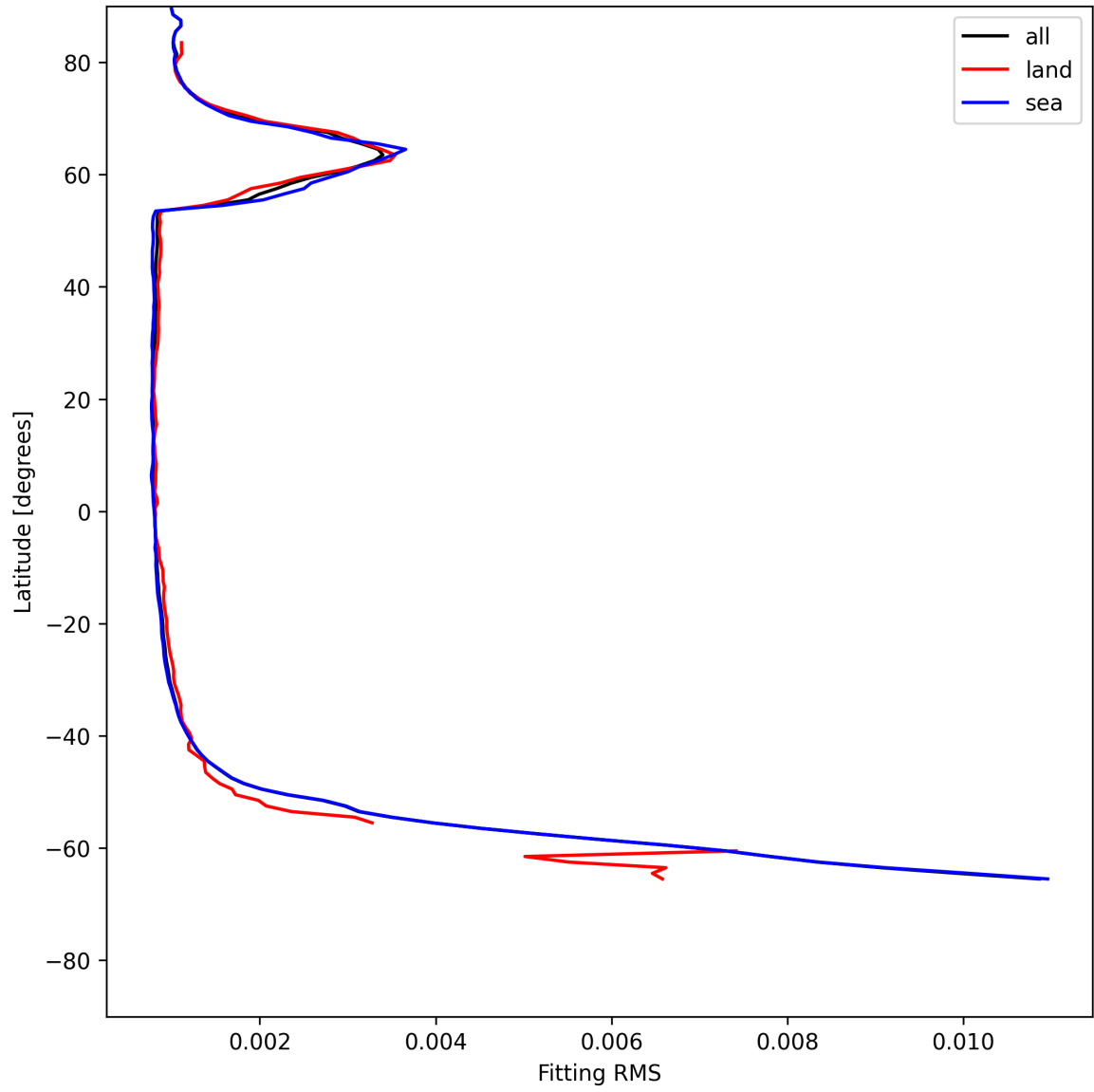
Figure 22: Zonal average of “Fitting RMS” for 2025-07-02 to 2025-07-03.
