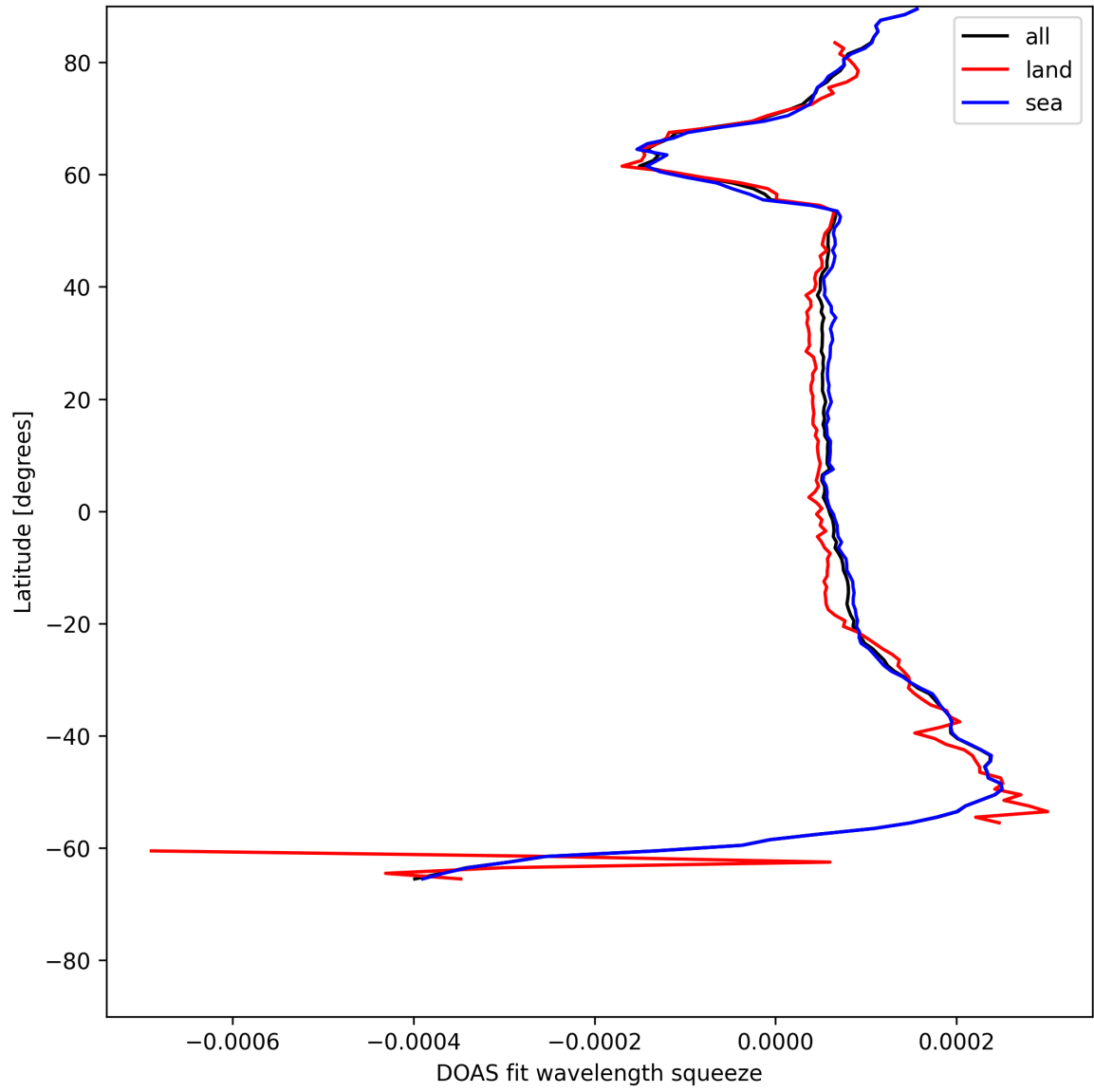
Figure 24: Zonal average of “DOAS fit wavelength squeeze” for 2025-07-02 to 2025-07-03.
