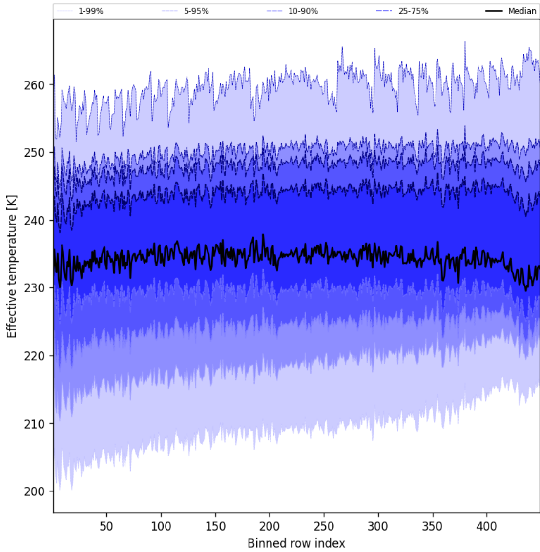
Figure 50: Along track statistics of “Effective temperature” for 2025-07-02 to 2025-07-03
