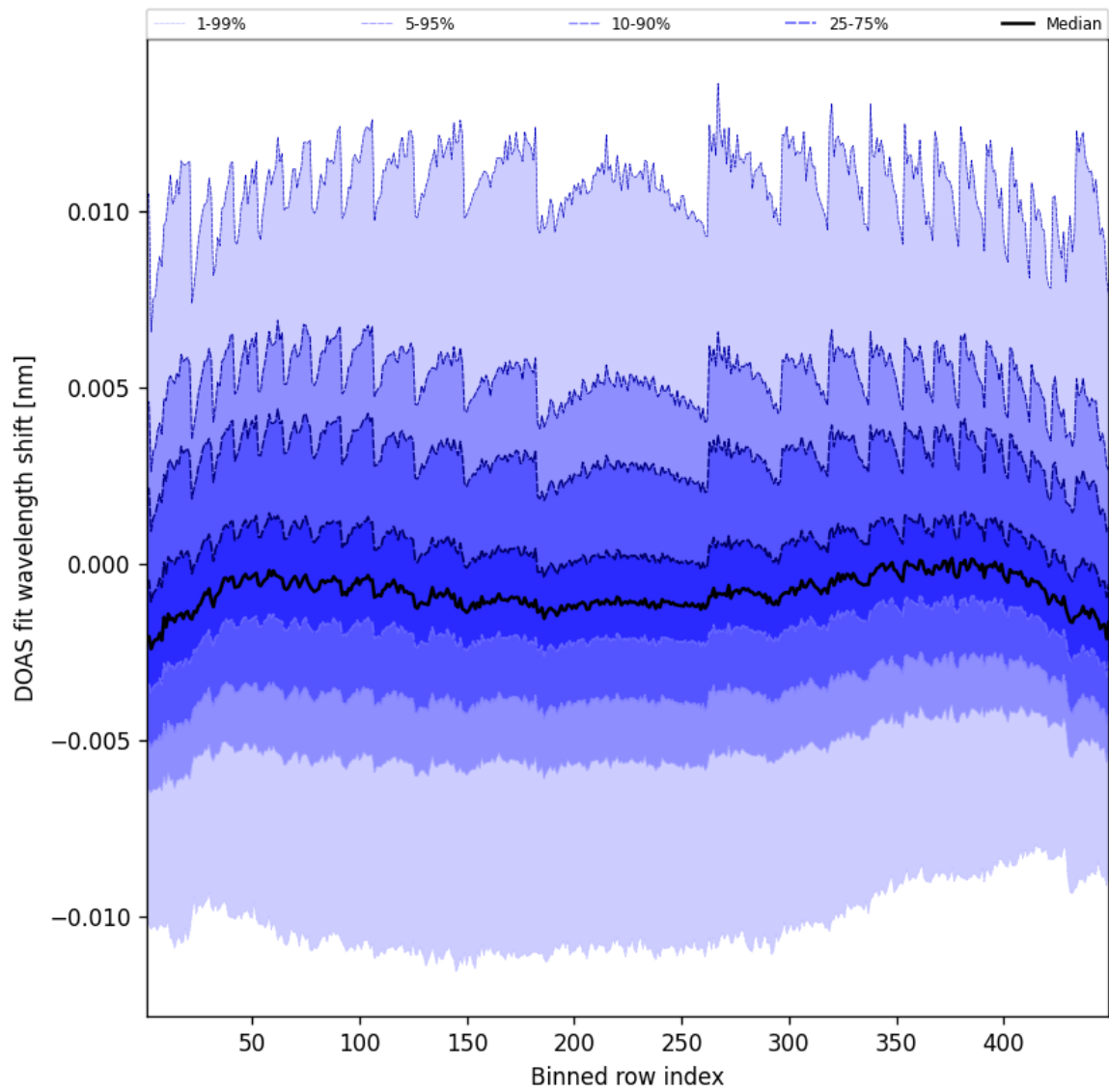
Figure 47: Along track statistics of “DOAS fit wavelength shift” for 2025-07-02 to 2025-07-03
