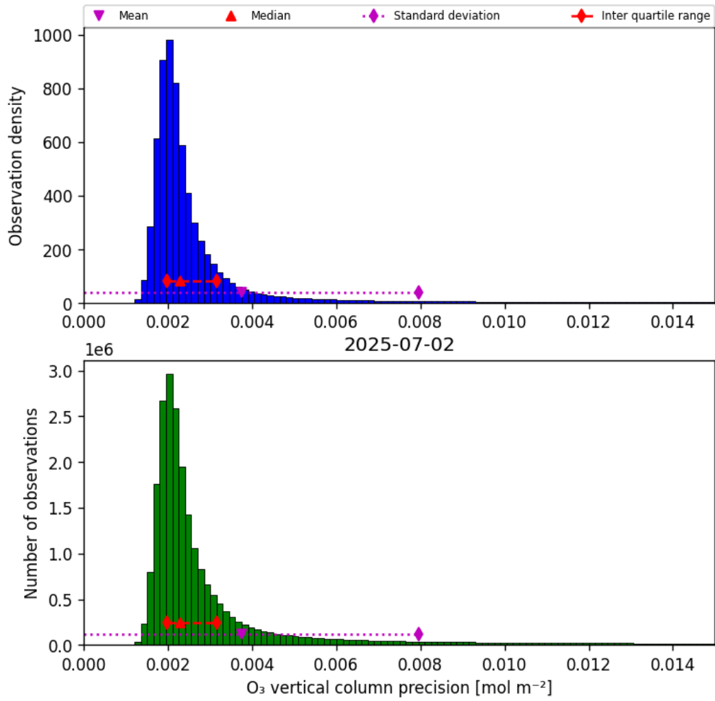
Figure 30: Histogram of “O 3 vertical column precision” for 2025-07-02 to 2025-07-03
