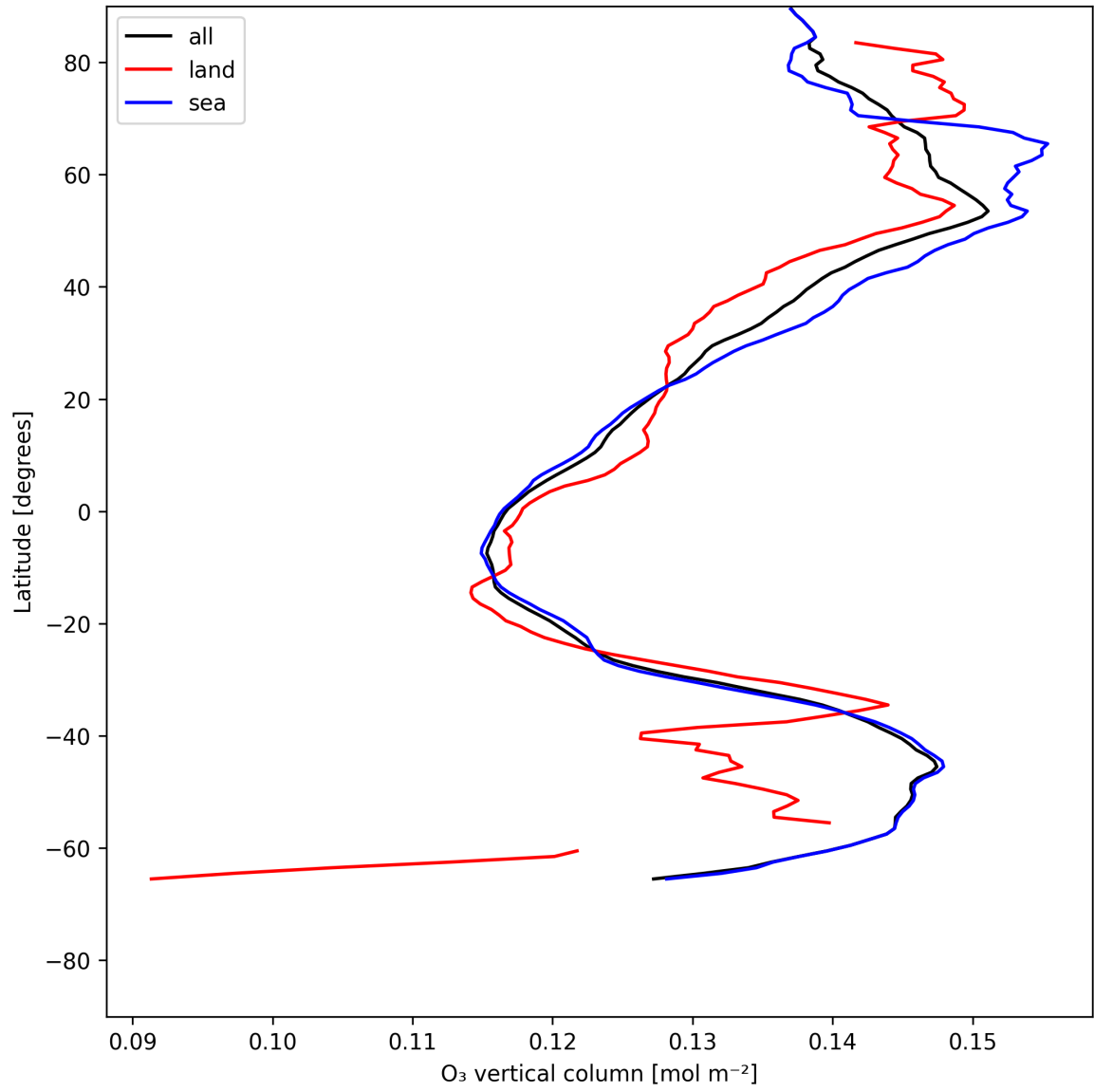
Figure 17: Zonal average of “O 3 vertical column” for 2025-07-02 to 2025-07-03.
