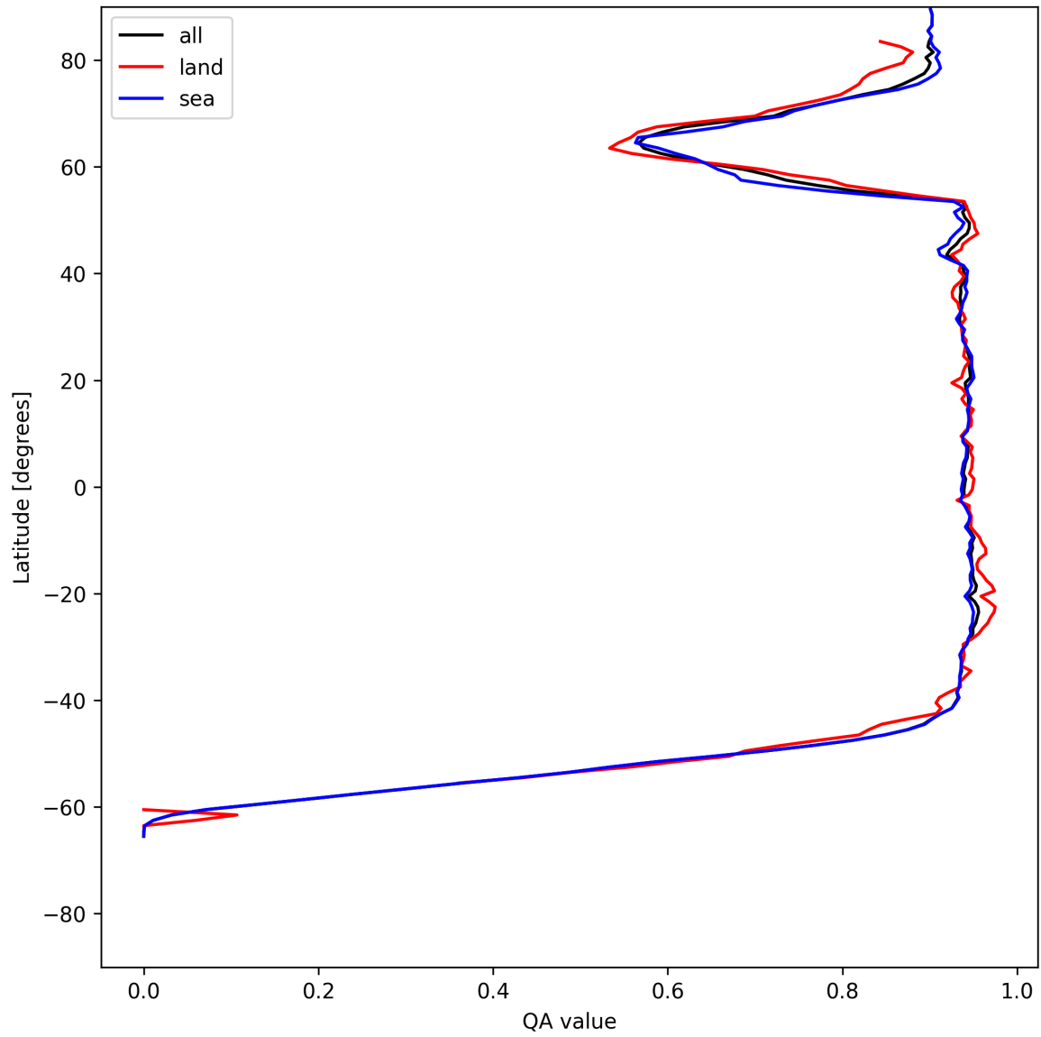
Figure 16: Zonal average of “QA value” for 2025-07-02 to 2025-07-03.
