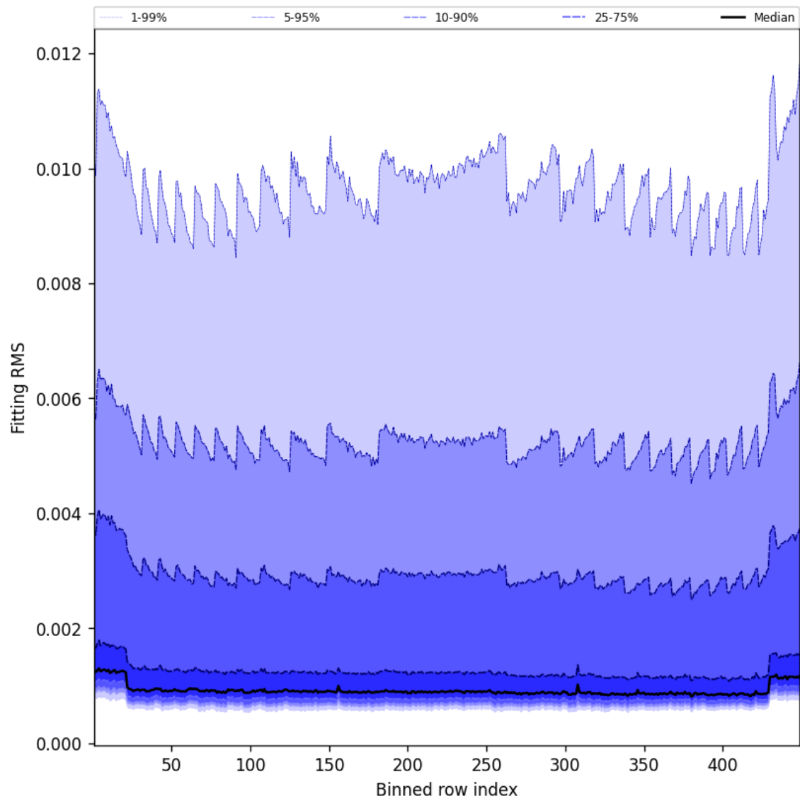
Figure 46: Along track statistics of “Fitting RMS” for 2025-07-03 to 2025-07-04
