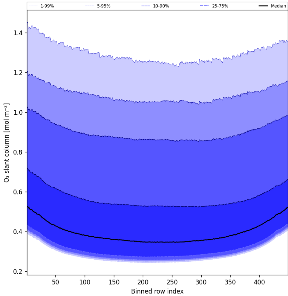
Figure 43: Along track statistics of “O 3 slant column” for 2025-07-03 to 2025-07-04
