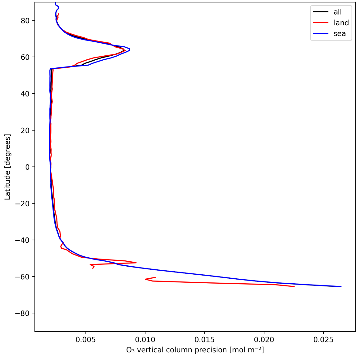
Figure 18: Zonal average of “O 3 vertical column precision” for 2025-07-03 to 2025-07-04.
