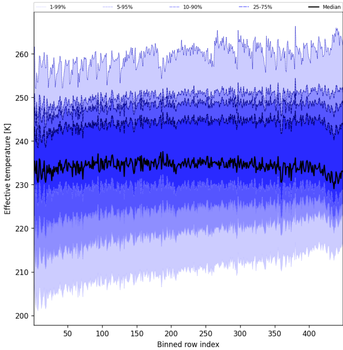
Figure 50: Along track statistics of “Effective temperature” for 2025-07-03 to 2025-07-04
