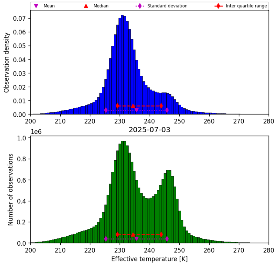
Figure 38: Histogram of “Effective temperature” for 2025-07-03 to 2025-07-04
