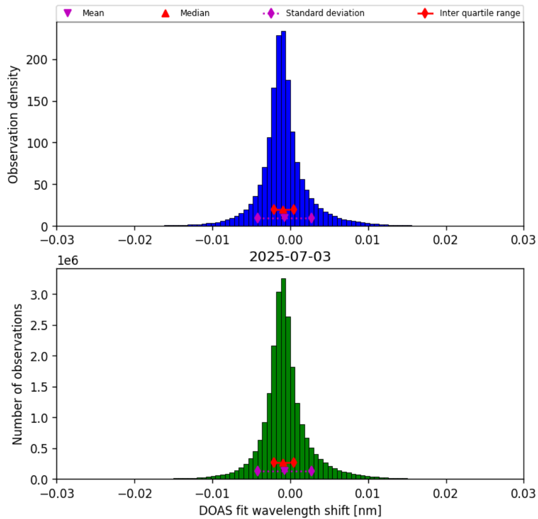
Figure 35: Histogram of “DOAS fit wavelength shift” for 2025-07-03 to 2025-07-04
