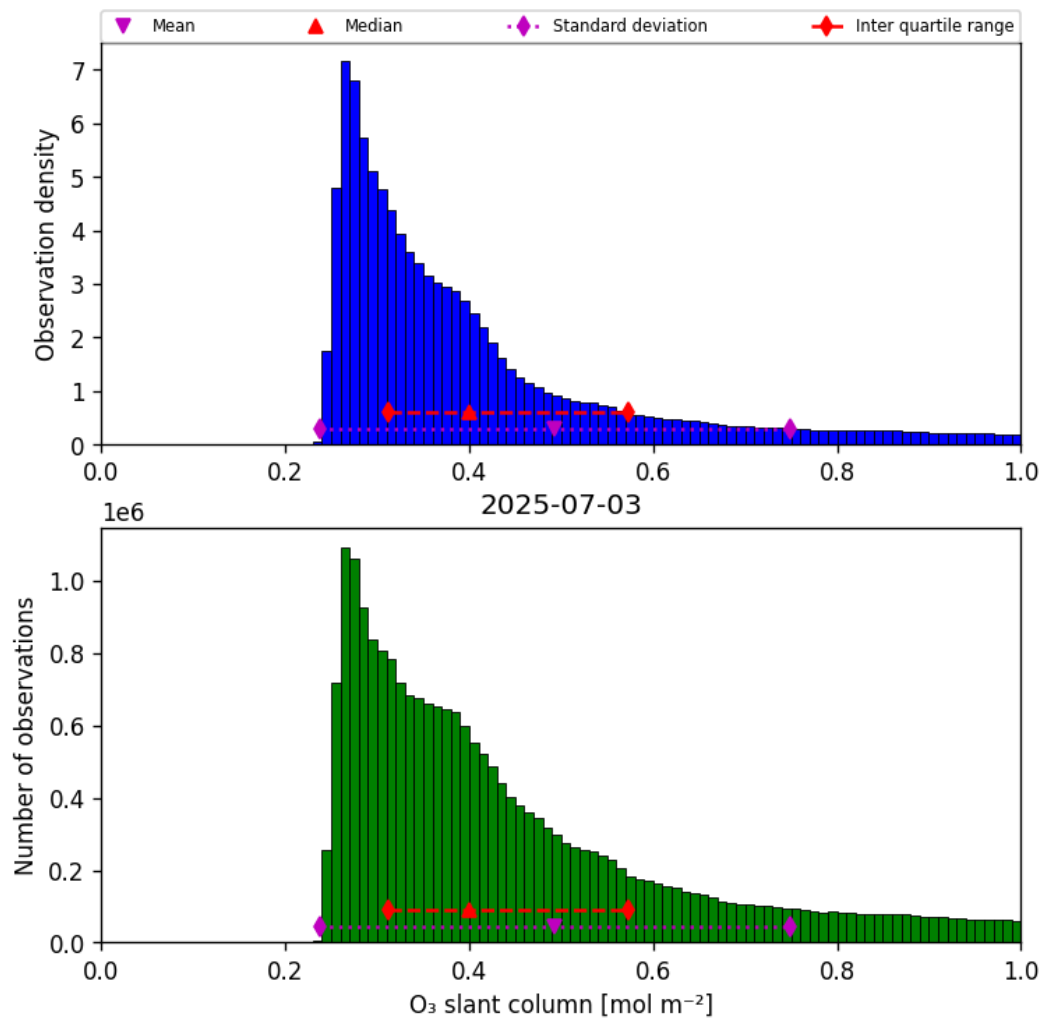
Figure 31: Histogram of “O 3 slant column” for 2025-07-03 to 2025-07-04
