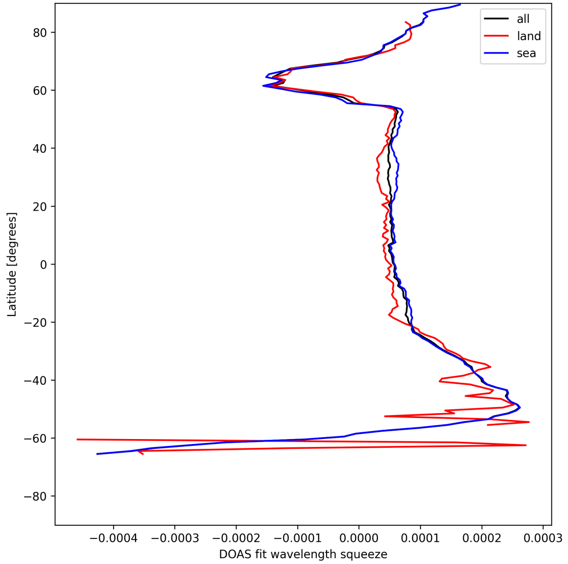
Figure 24: Zonal average of “DOAS fit wavelength squeeze” for 2025-07-03 to 2025-07-04.
