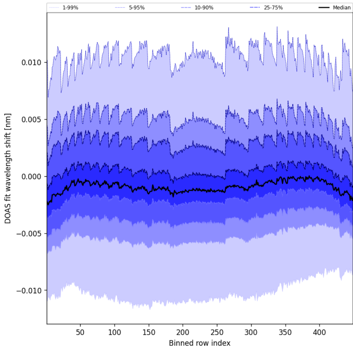
Figure 47: Along track statistics of “DOAS fit wavelength shift” for 2025-07-03 to 2025-07-04
