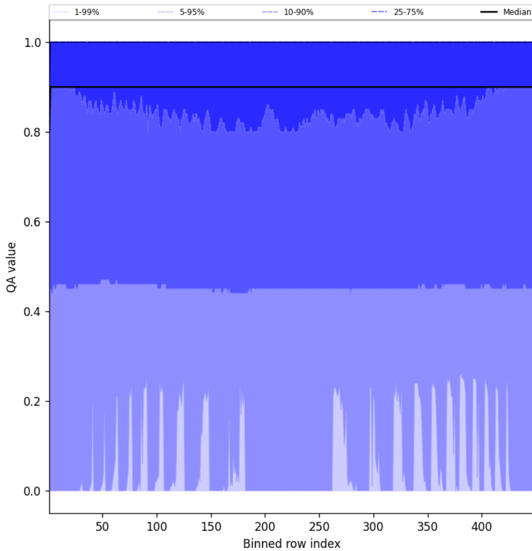
Figure 40: Along track statistics of “QA value” for 2025-07-03 to 2025-07-04
