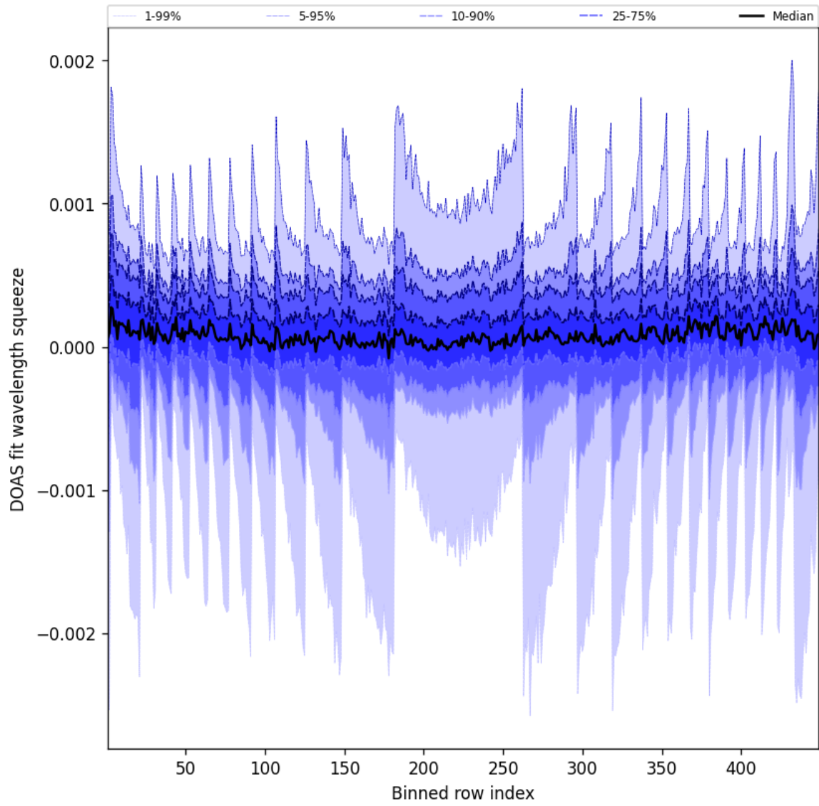
Figure 48: Along track statistics of “DOAS fit wavelength squeeze” for 2025-07-03 to 2025-07-04
