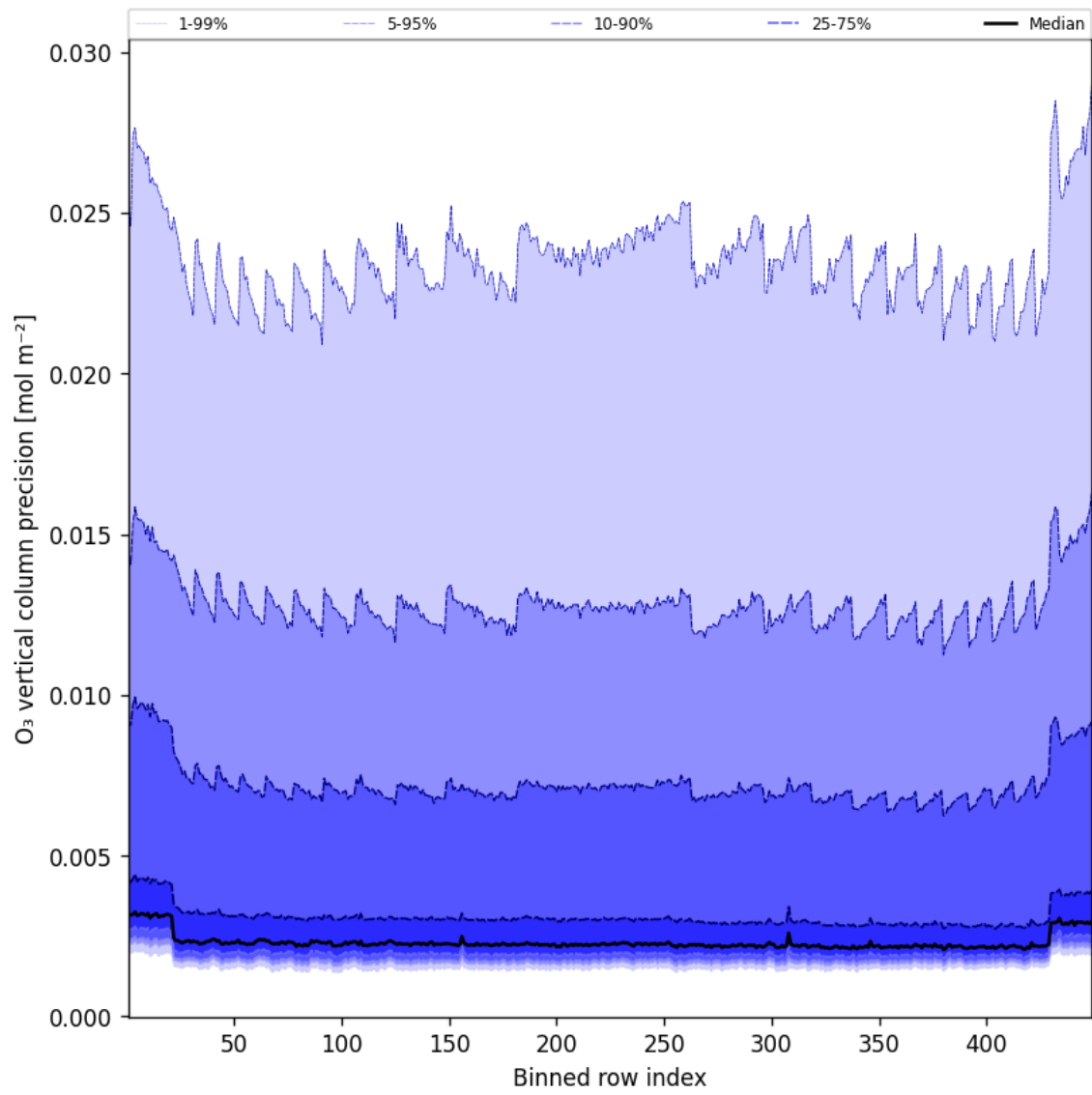
Figure 42: Along track statistics of “O 3 vertical column precision” for 2025-07-03 to 2025-07-04
