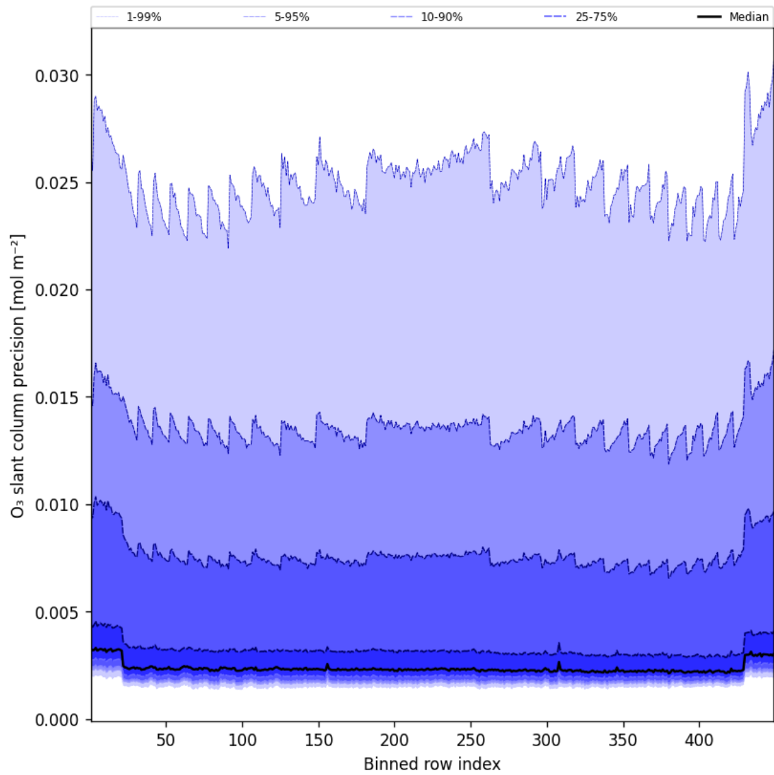
Figure 44: Along track statistics of “O 3 slant column precision” for 2025-07-03 to 2025-07-04
