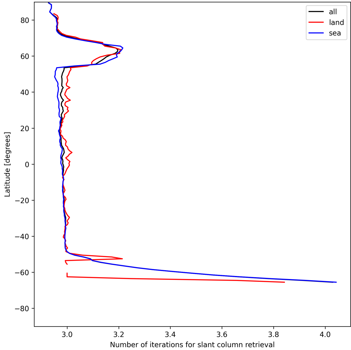
Figure 21: Zonal average of “Number of iterations for slant column retrieval” for 2025-07-03 to 2025-07-04.
