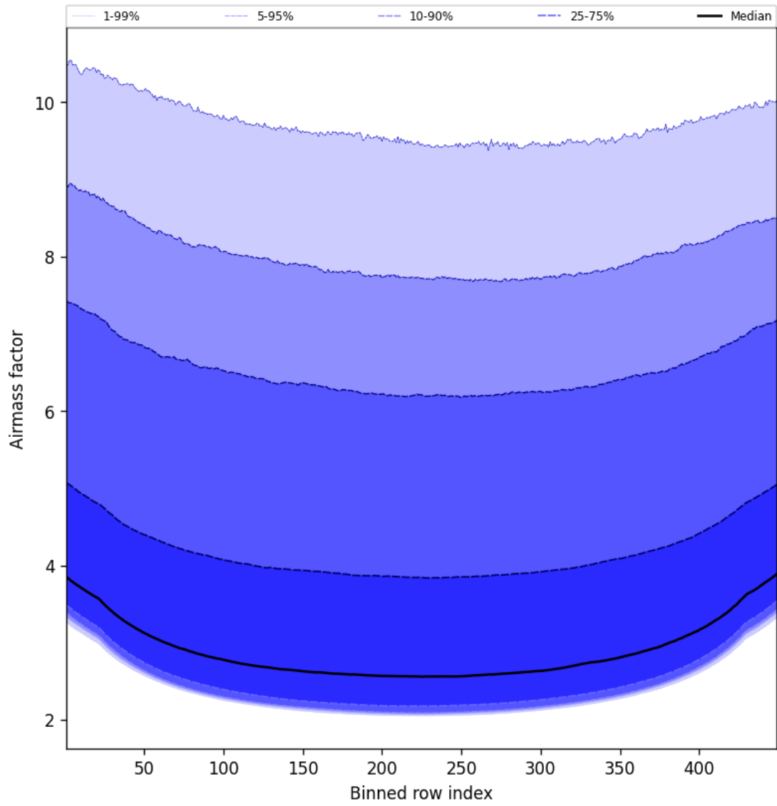
Figure 49: Along track statistics of “Airmass factor” for 2025-07-03 to 2025-07-04
