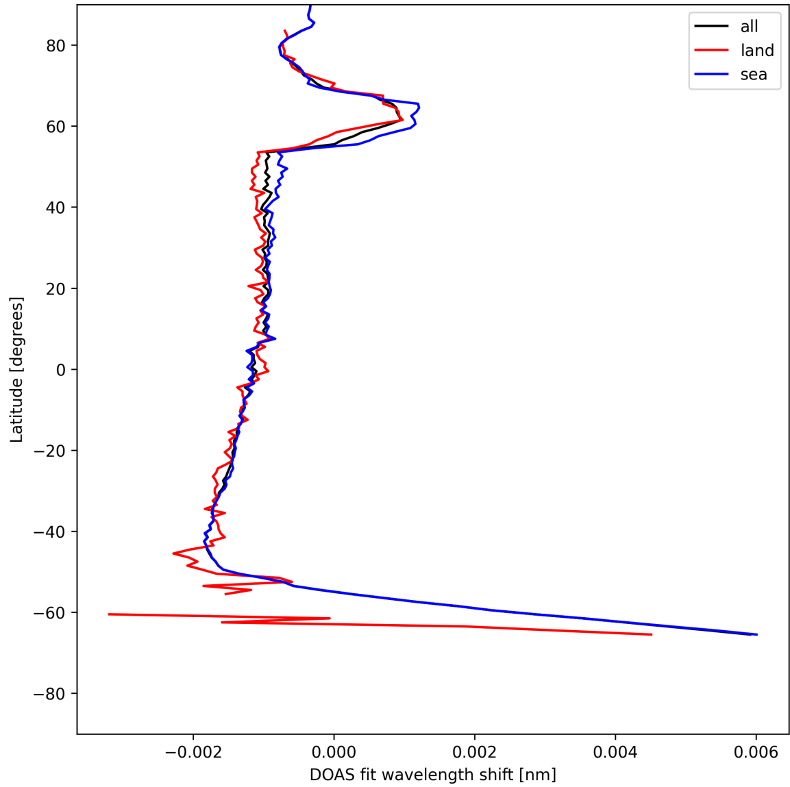
Figure 23: Zonal average of “DOAS fit wavelength shift” for 2025-07-03 to 2025-07-04.
