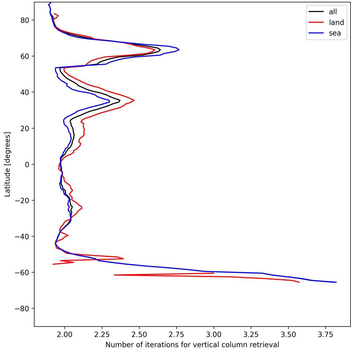
Figure 27: Zonal average of “Number of iterations for vertical column retrieval” for 2025-07-03 to 2025-07-04.
