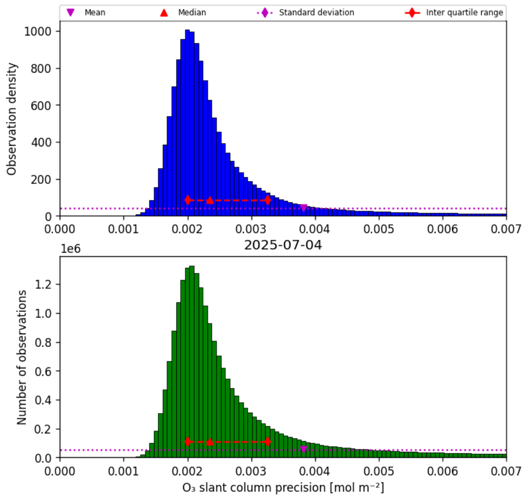
Figure 32: Histogram of “O 3 slant column precision” for 2025-07-04 to 2025-07-05
