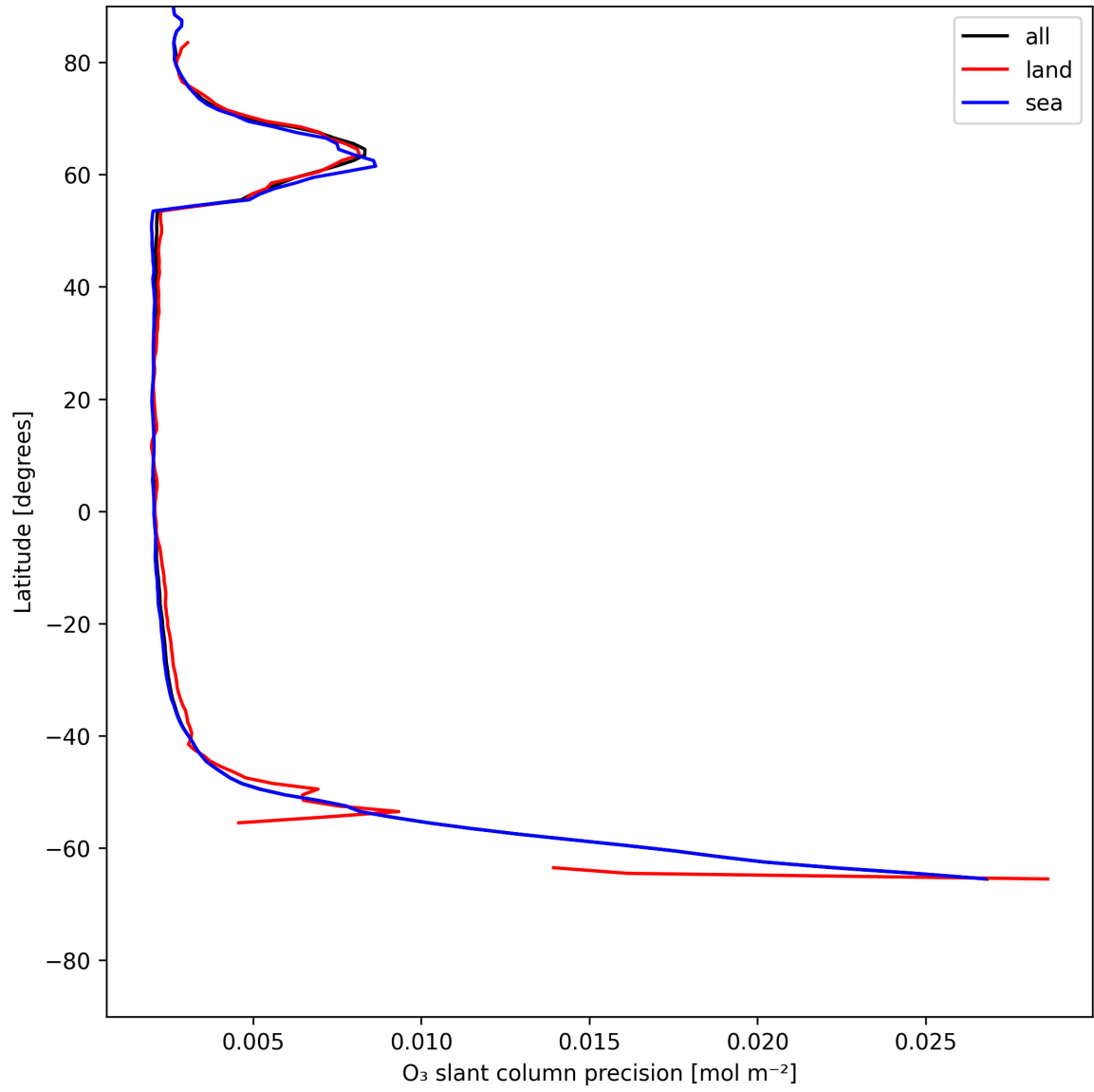
Figure 20: Zonal average of “O 3 slant column precision” for 2025-07-04 to 2025-07-05.
