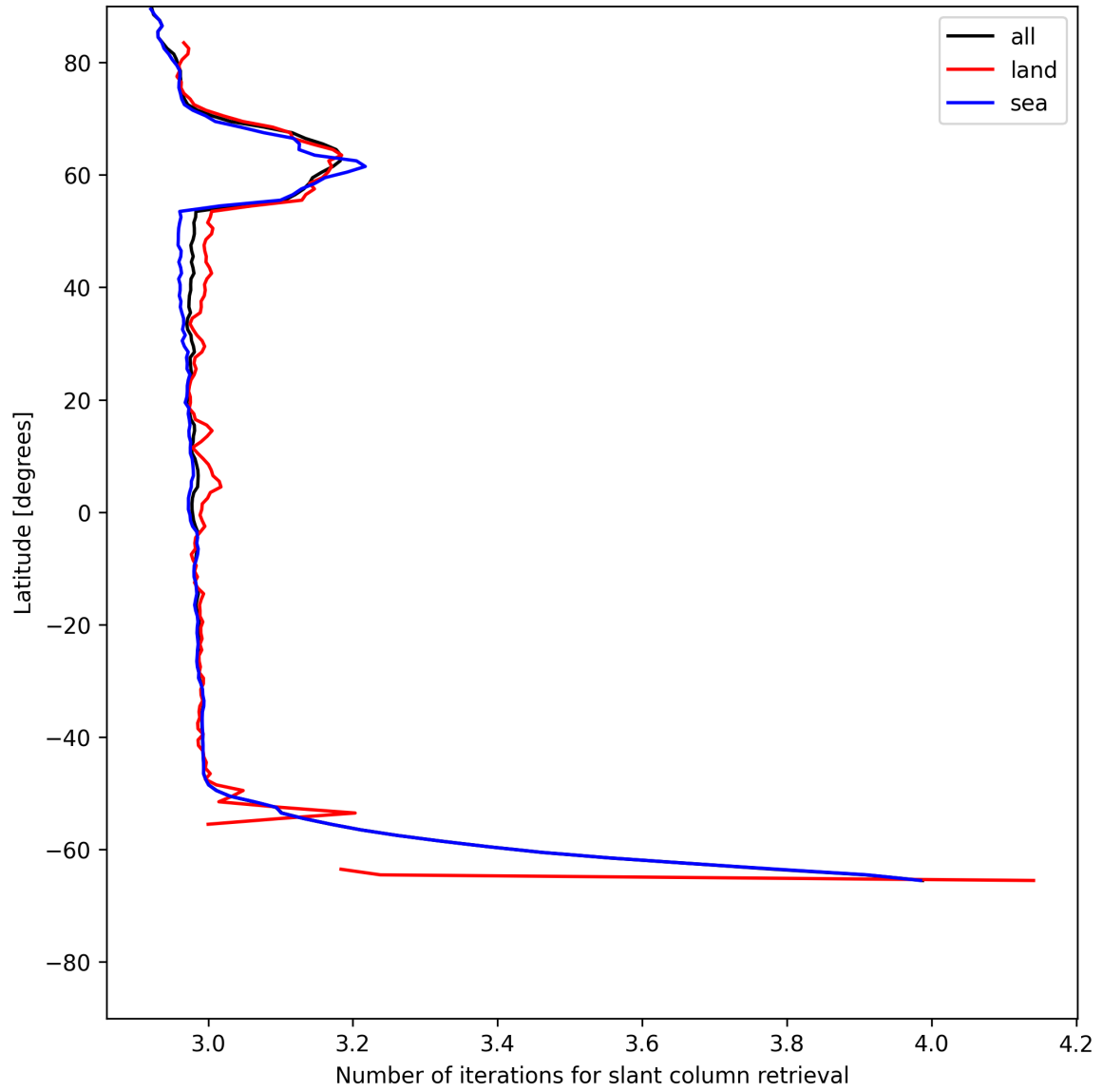
Figure 21: Zonal average of “Number of iterations for slant column retrieval” for 2025-07-04 to 2025-07-05.
