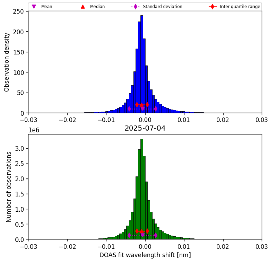
Figure 35: Histogram of “DOAS fit wavelength shift” for 2025-07-04 to 2025-07-05
