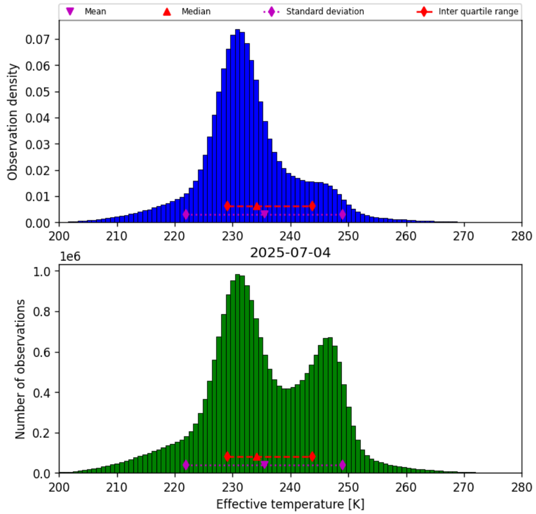
Figure 38: Histogram of “Effective temperature” for 2025-07-04 to 2025-07-05
