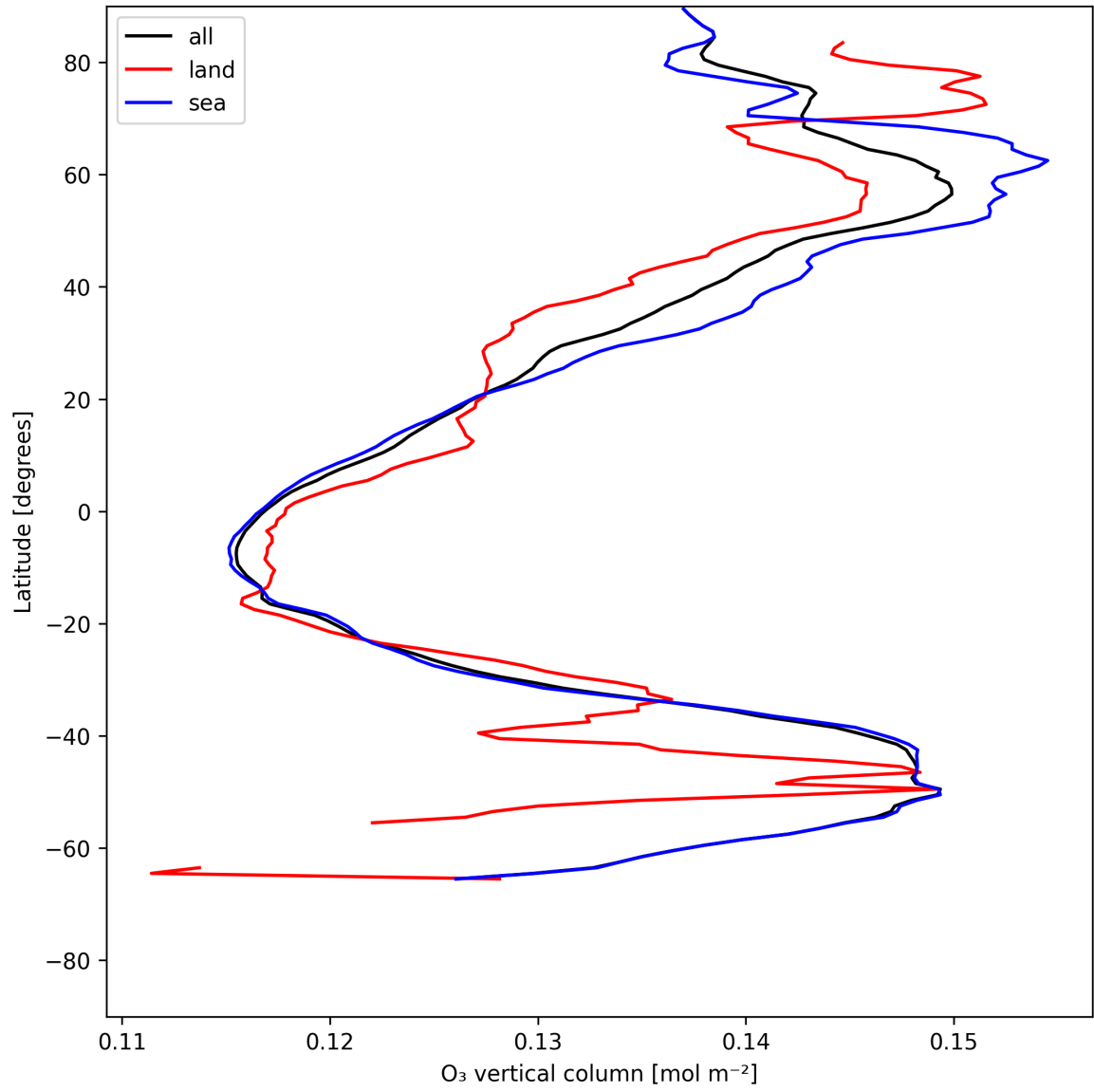
Figure 17: Zonal average of “O 3 vertical column” for 2025-07-04 to 2025-07-05.
