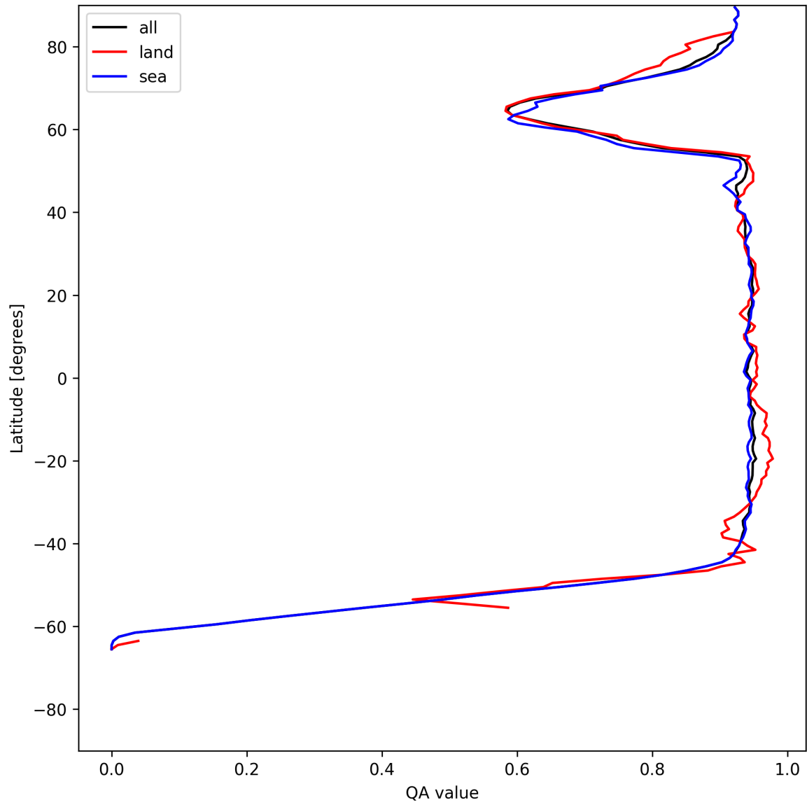
Figure 16: Zonal average of “QA value” for 2025-07-04 to 2025-07-05.
