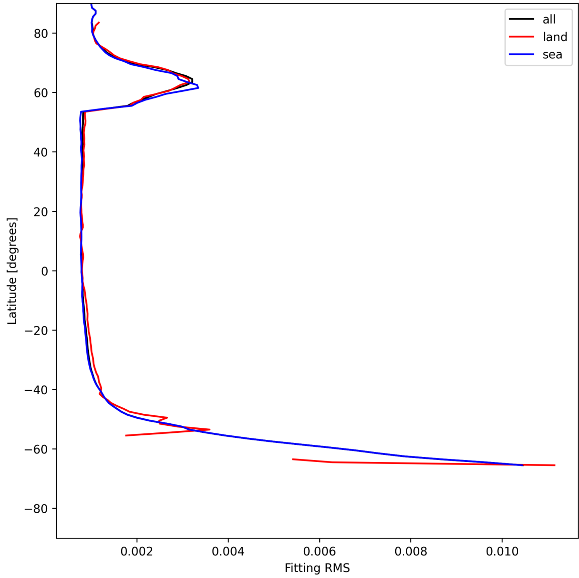
Figure 22: Zonal average of “Fitting RMS” for 2025-07-04 to 2025-07-05.
