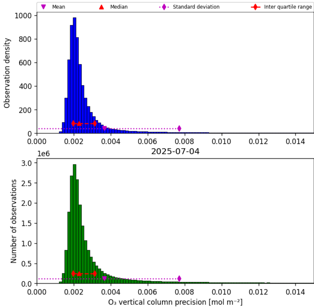
Figure 30: Histogram of “O 3 vertical column precision” for 2025-07-04 to 2025-07-05
