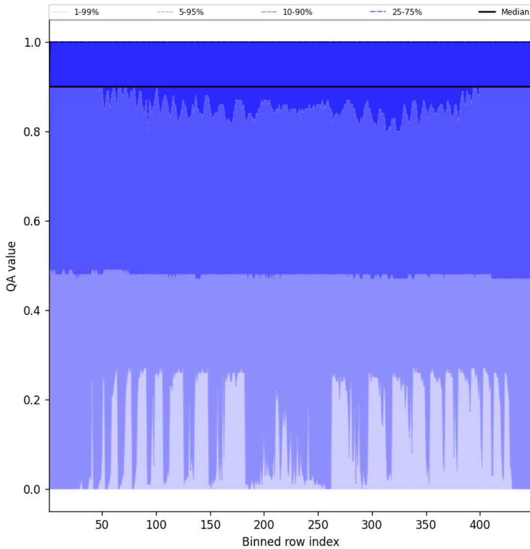
Figure 40: Along track statistics of “QA value” for 2025-07-04 to 2025-07-05
