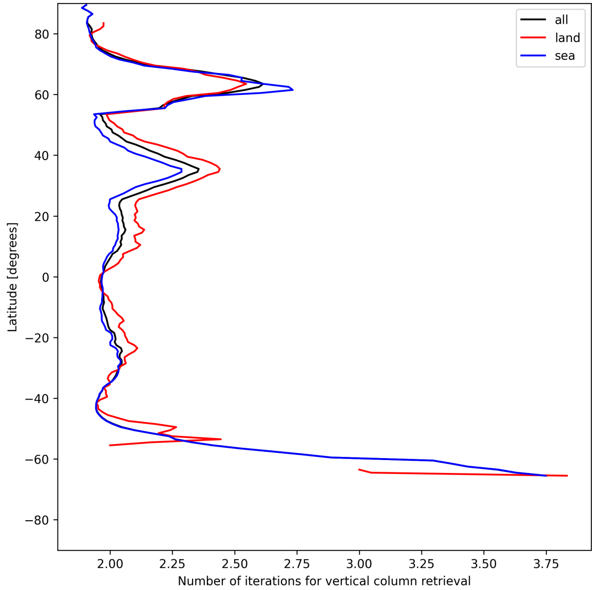
Figure 27: Zonal average of “Number of iterations for vertical column retrieval” for 2025-07-04 to 2025-07-05.
