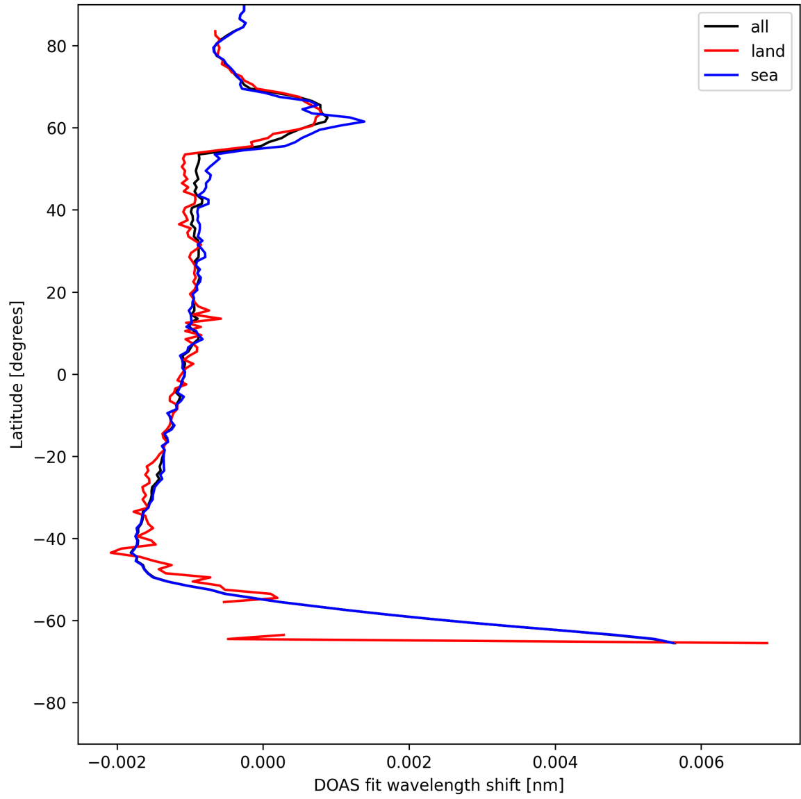
Figure 23: Zonal average of “DOAS fit wavelength shift” for 2025-07-04 to 2025-07-05.
