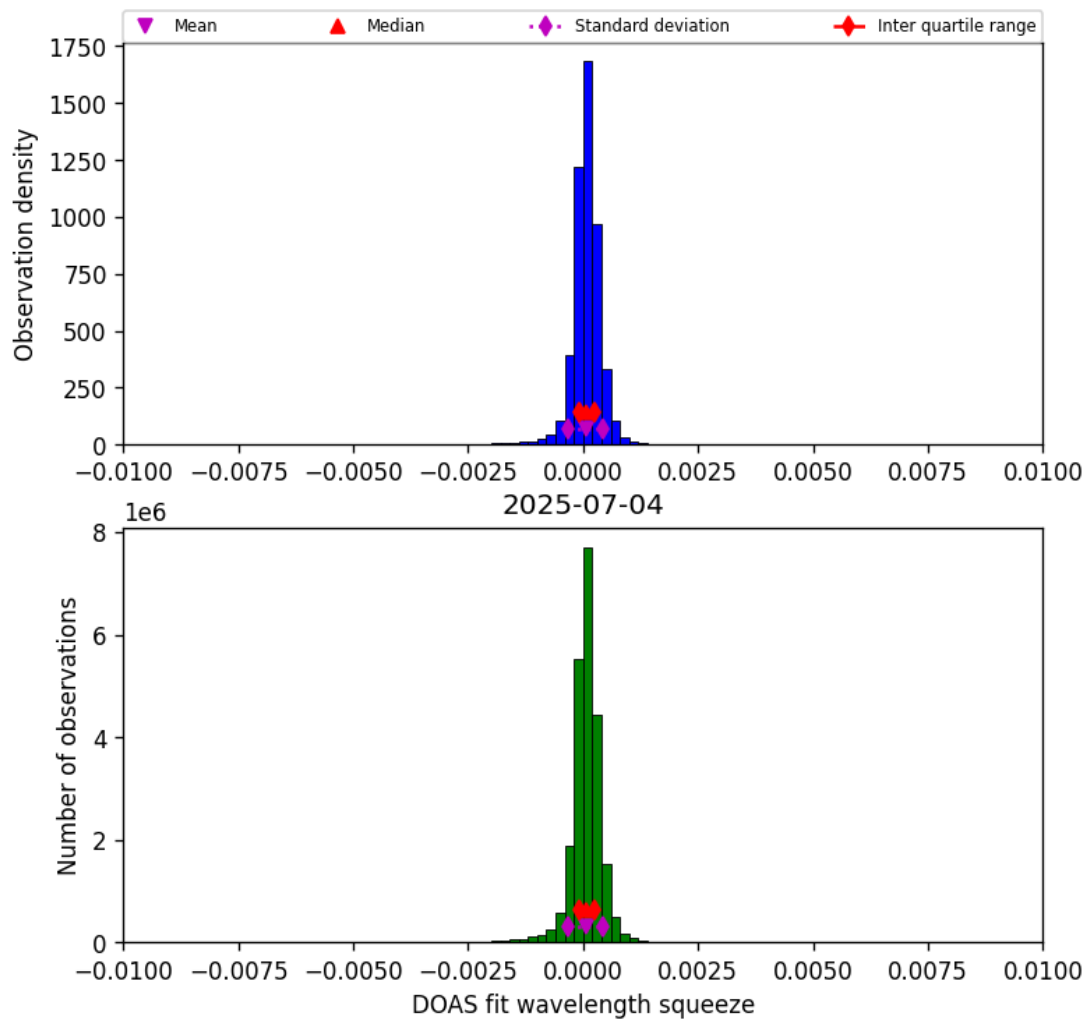
Figure 36: Histogram of “DOAS fit wavelength squeeze” for 2025-07-04 to 2025-07-05
