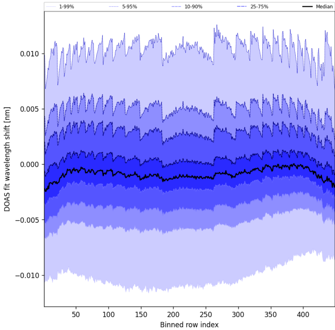
Figure 47: Along track statistics of “DOAS fit wavelength shift” for 2025-07-04 to 2025-07-05
