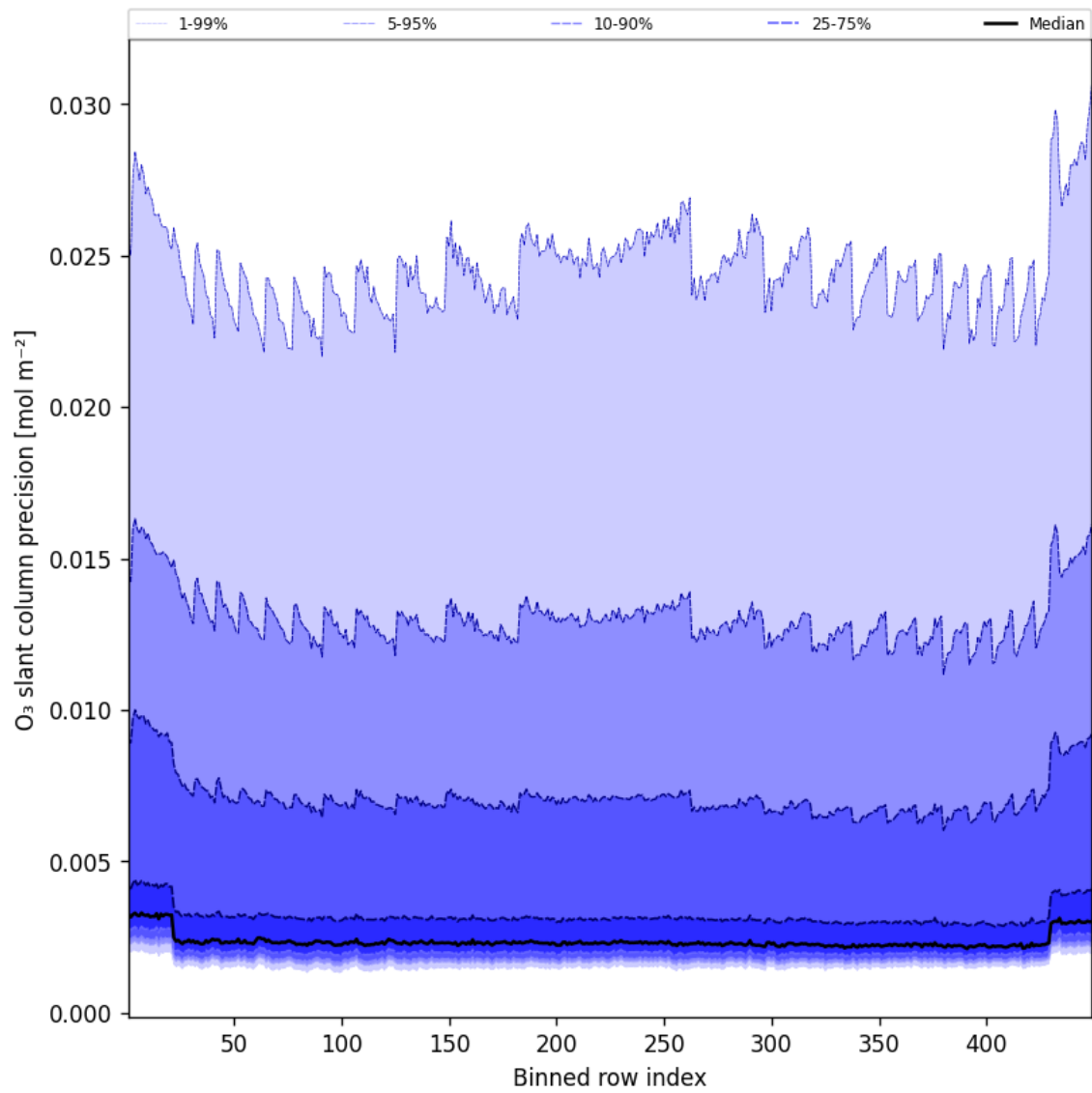
Figure 44: Along track statistics of “O 3 slant column precision” for 2025-07-04 to 2025-07-05
