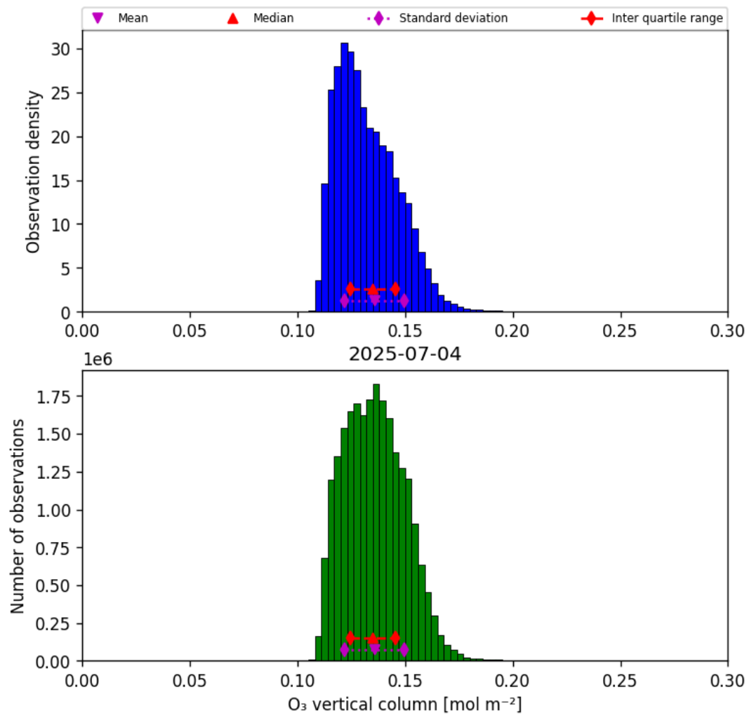
Figure 29: Histogram of “O 3 vertical column” for 2025-07-04 to 2025-07-05
