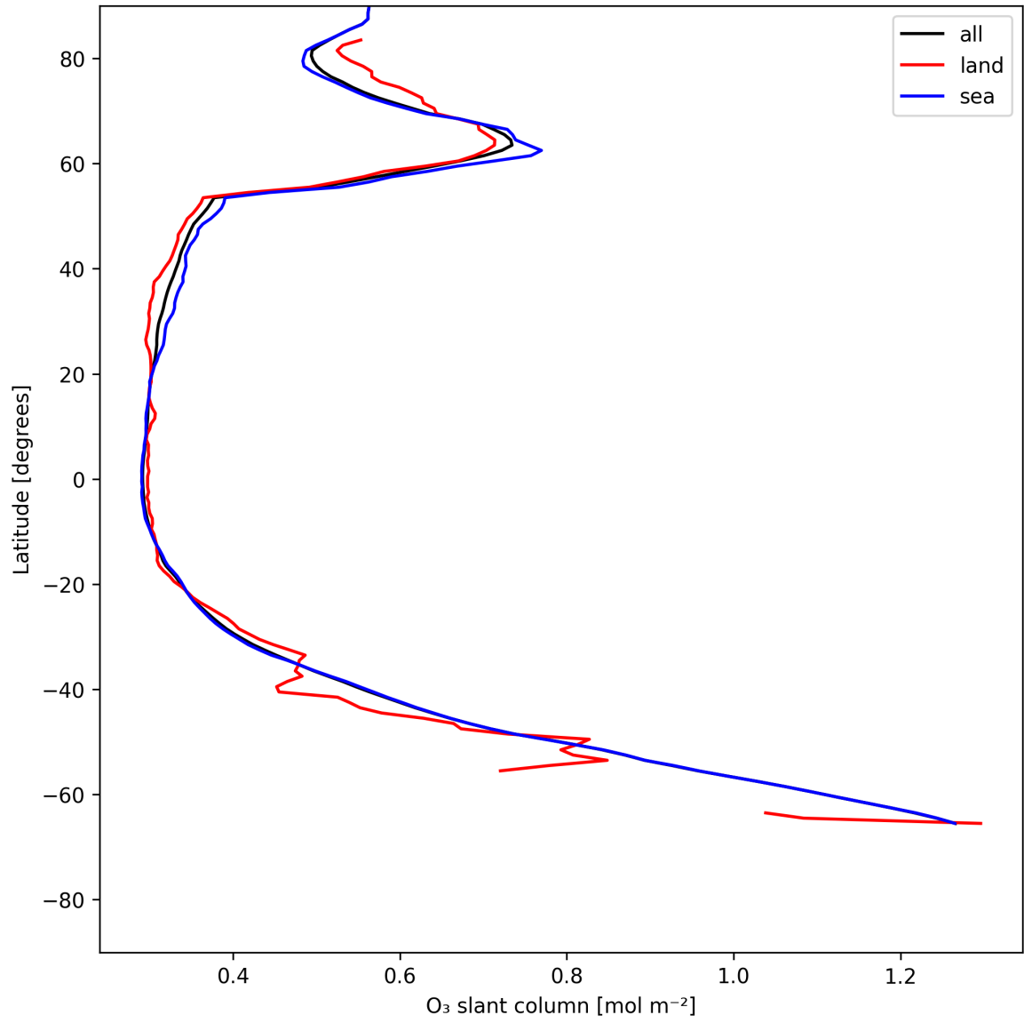
Figure 19: Zonal average of “O 3 slant column” for 2025-07-04 to 2025-07-05.
