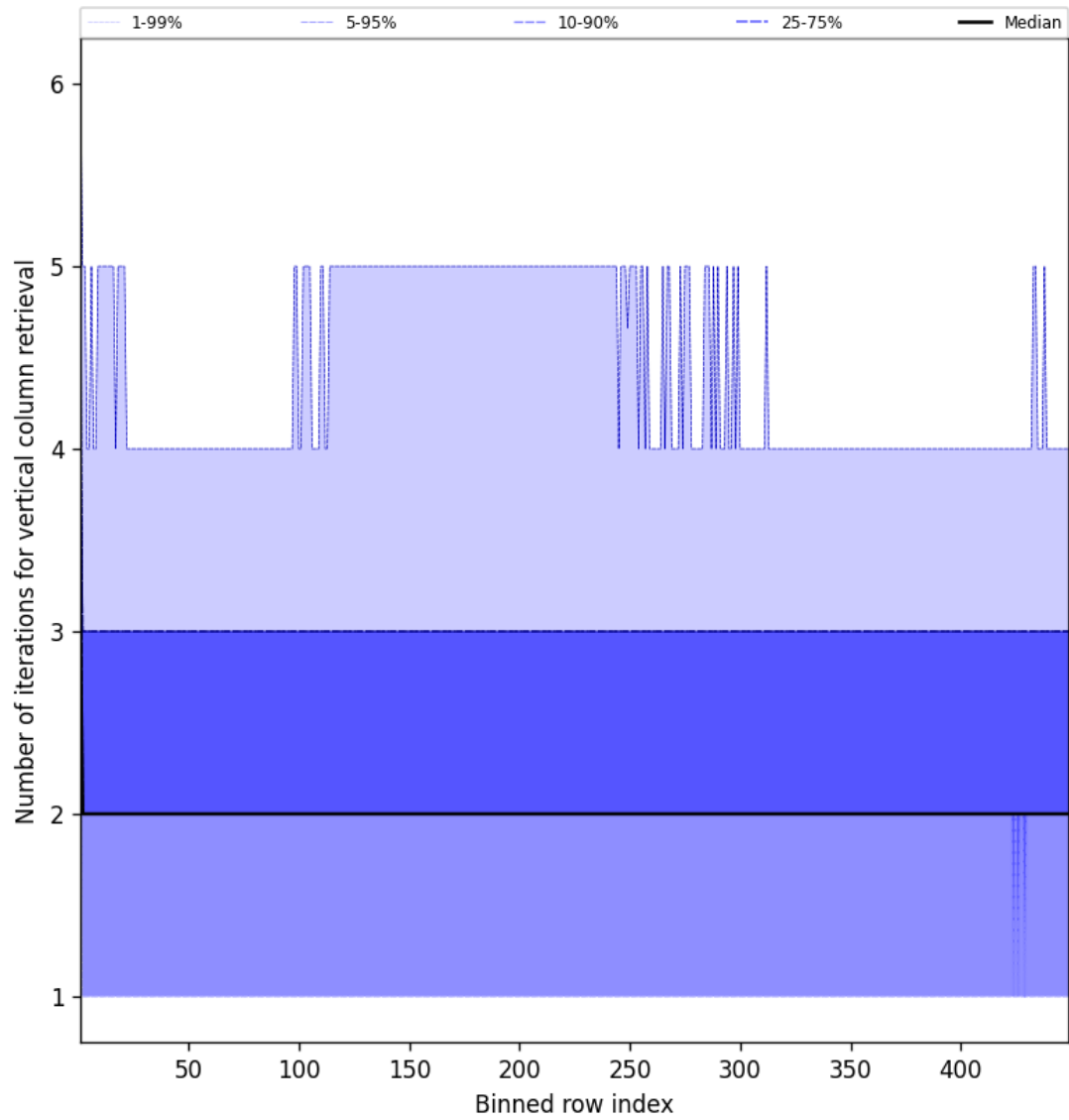
Figure 51: Along track statistics of “Number of iterations for vertical column retrieval” for 2025-07-04 to 2025-07-05
