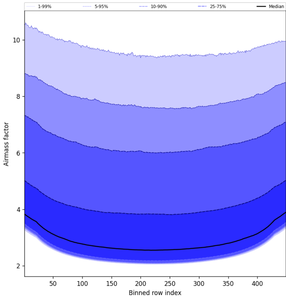
Figure 49: Along track statistics of “Airmass factor” for 2025-07-04 to 2025-07-05
