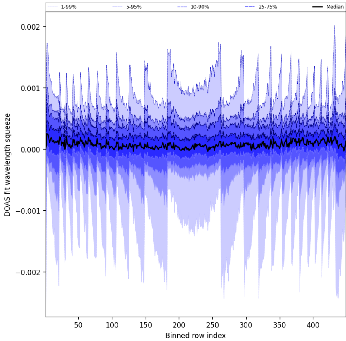
Figure 48: Along track statistics of “DOAS fit wavelength squeeze” for 2025-07-04 to 2025-07-05
