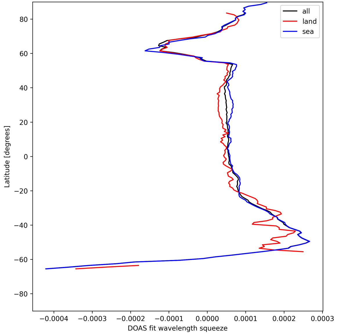
Figure 24: Zonal average of “DOAS fit wavelength squeeze” for 2025-07-04 to 2025-07-05.
