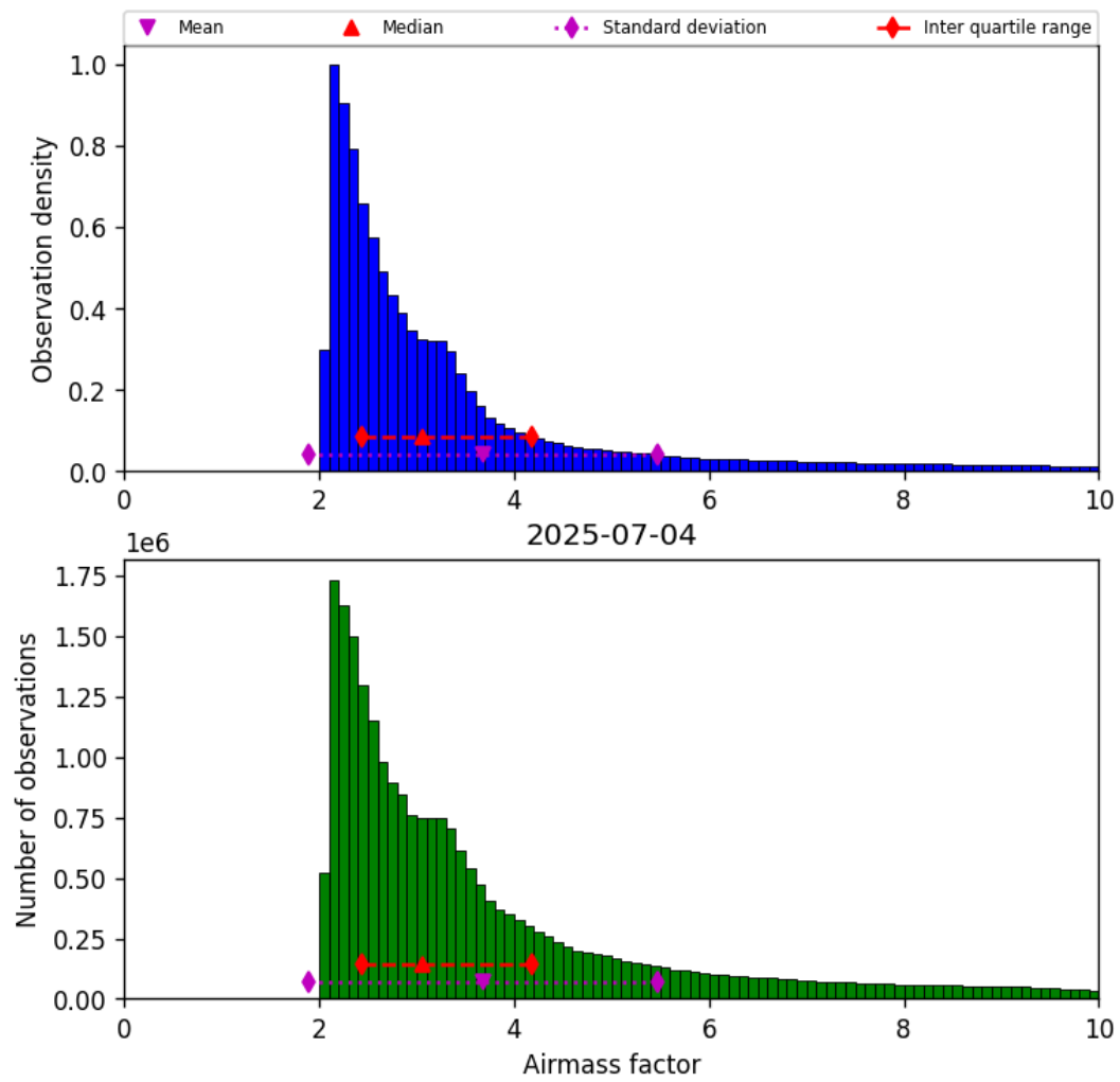
Figure 37: Histogram of “Airmass factor” for 2025-07-04 to 2025-07-05
