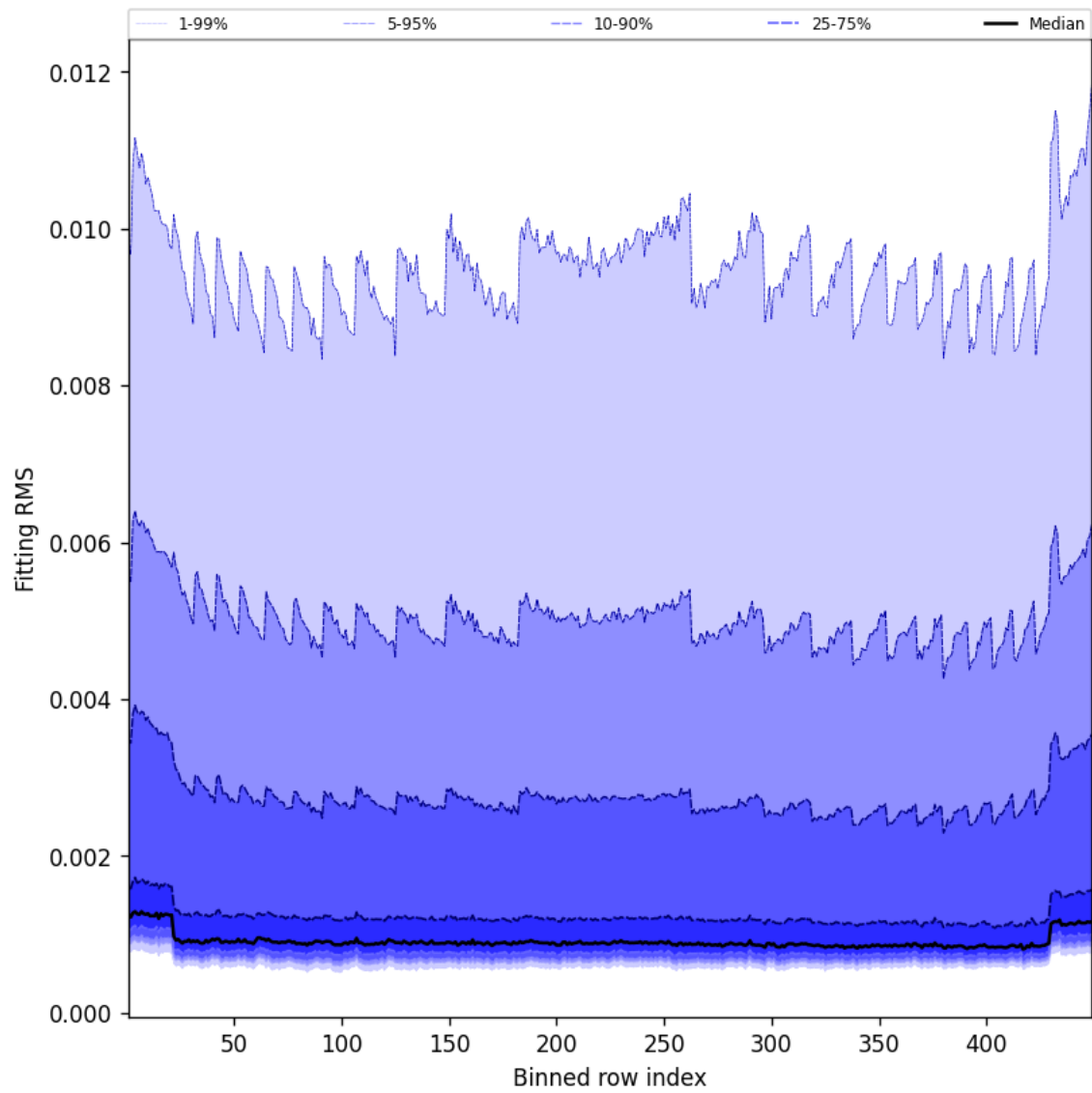
Figure 46: Along track statistics of “Fitting RMS” for 2025-07-04 to 2025-07-05
