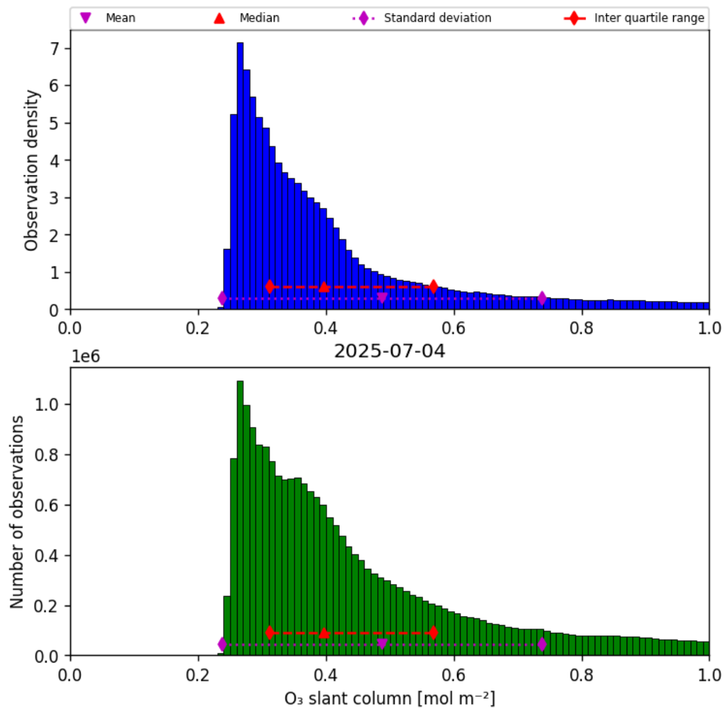
Figure 31: Histogram of “O 3 slant column” for 2025-07-04 to 2025-07-05
