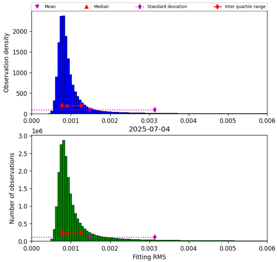
Figure 34: Histogram of “Fitting RMS” for 2025-07-04 to 2025-07-05
