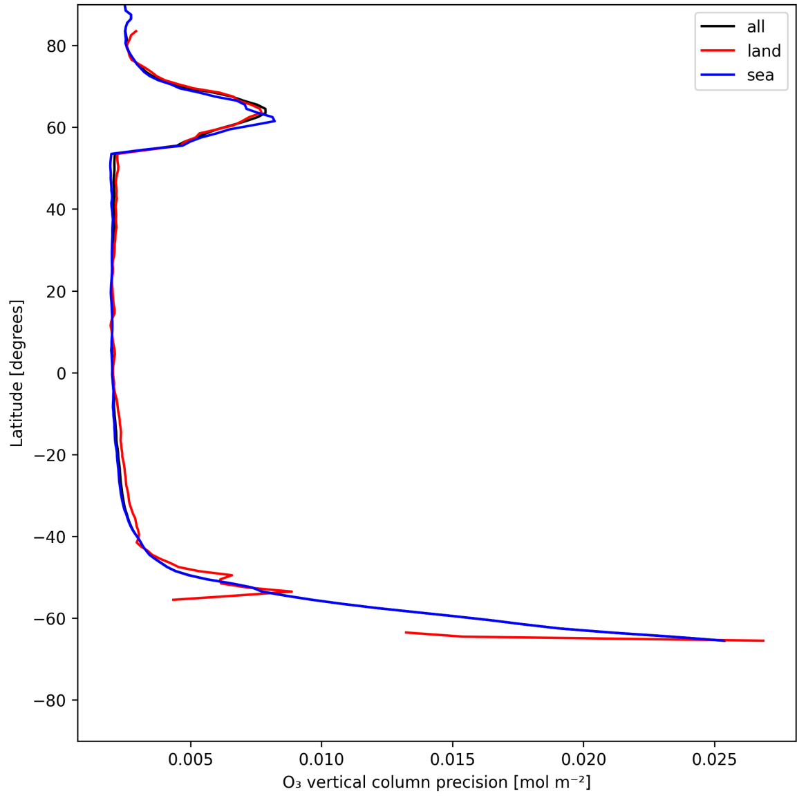
Figure 18: Zonal average of “O 3 vertical column precision” for 2025-07-04 to 2025-07-05.
