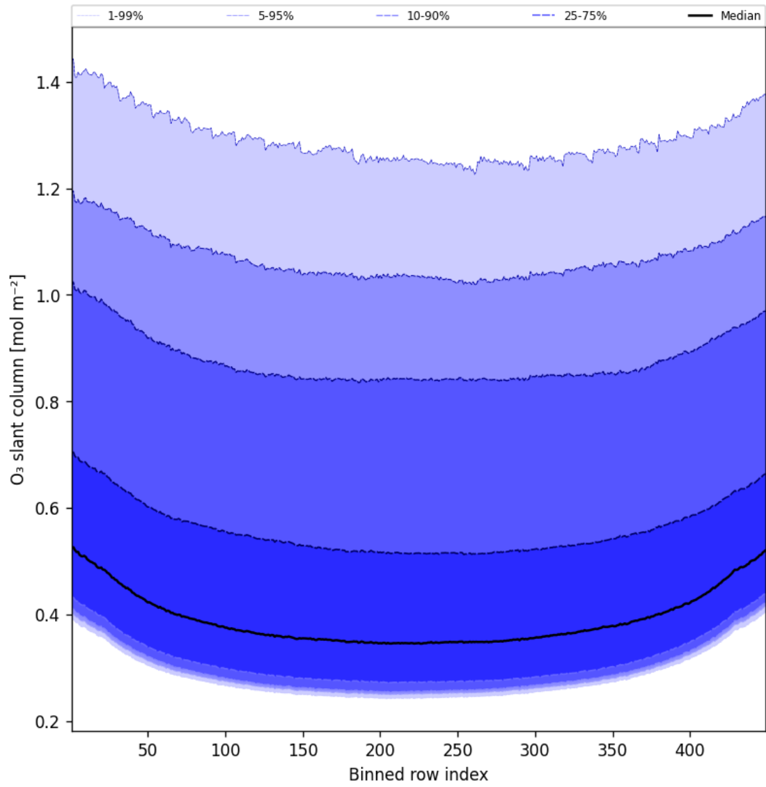
Figure 43: Along track statistics of “O 3 slant column” for 2025-07-04 to 2025-07-05
