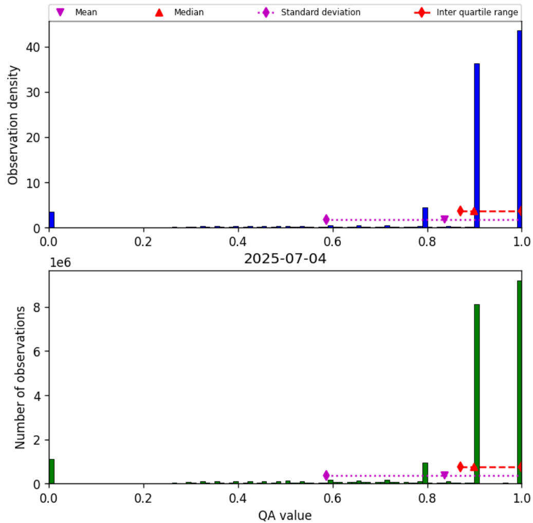
Figure 28: Histogram of “QA value” for 2025-07-04 to 2025-07-05
