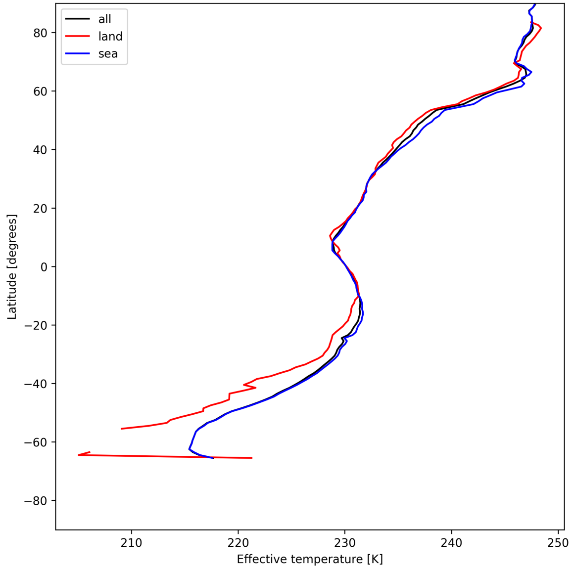
Figure 26: Zonal average of "Effective temperature" for 2025-07-04 to 2025-07-05.
