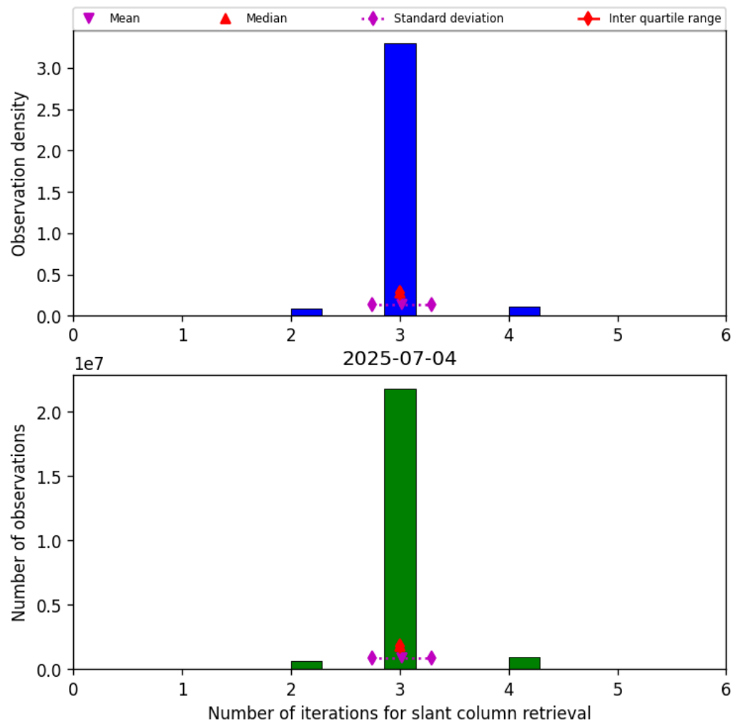
Figure 33: Histogram of “Number of iterations for slant column retrieval” for 2025-07-04 to 2025-07-05
