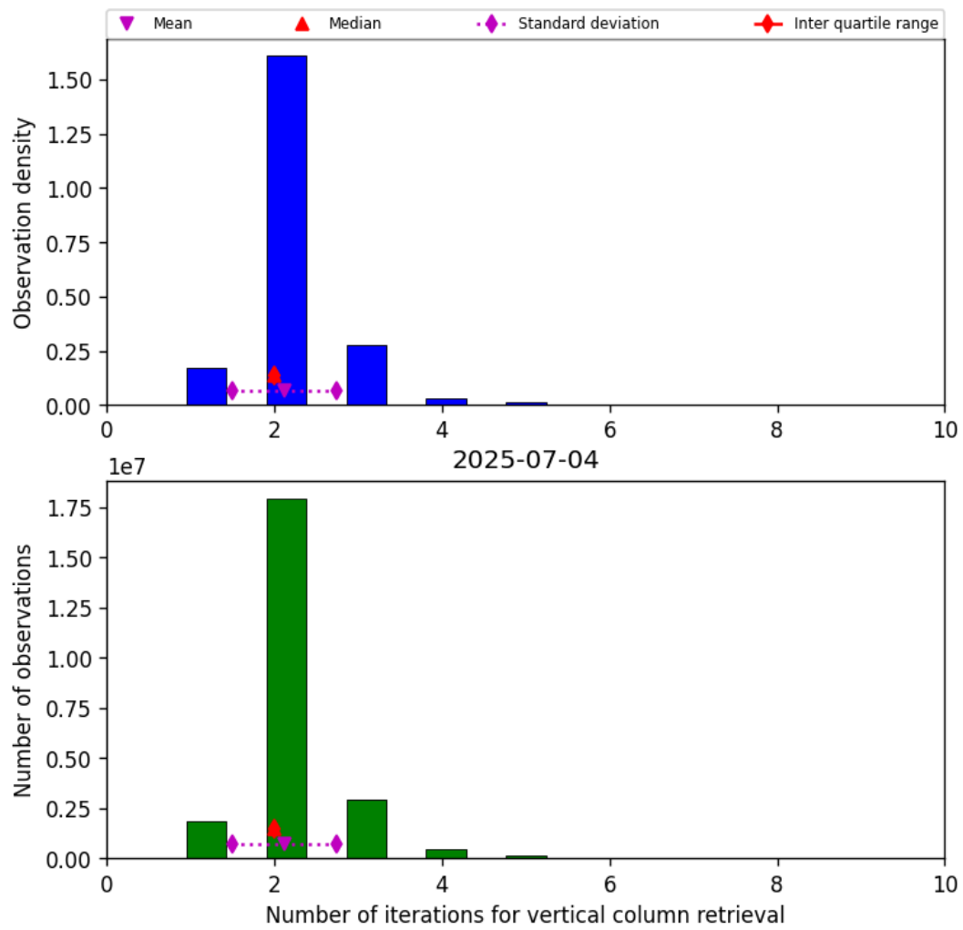
Figure 39: Histogram of “Number of iterations for vertical column retrieval” for 2025-07-04 to 2025-07-05
