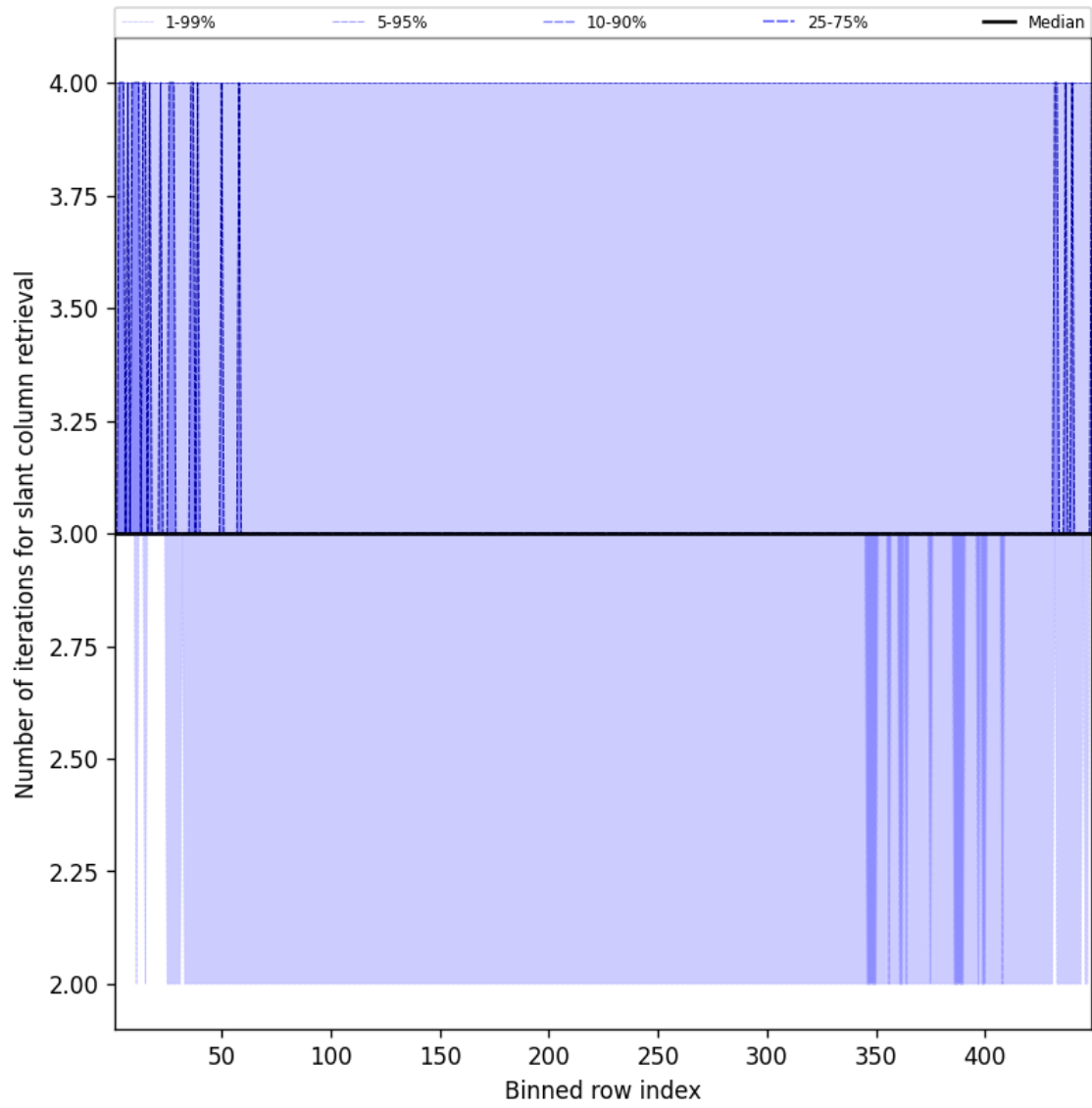
Figure 45: Along track statistics of “Number of iterations for slant column retrieval” for 2025-07-04 to 2025-07-05
