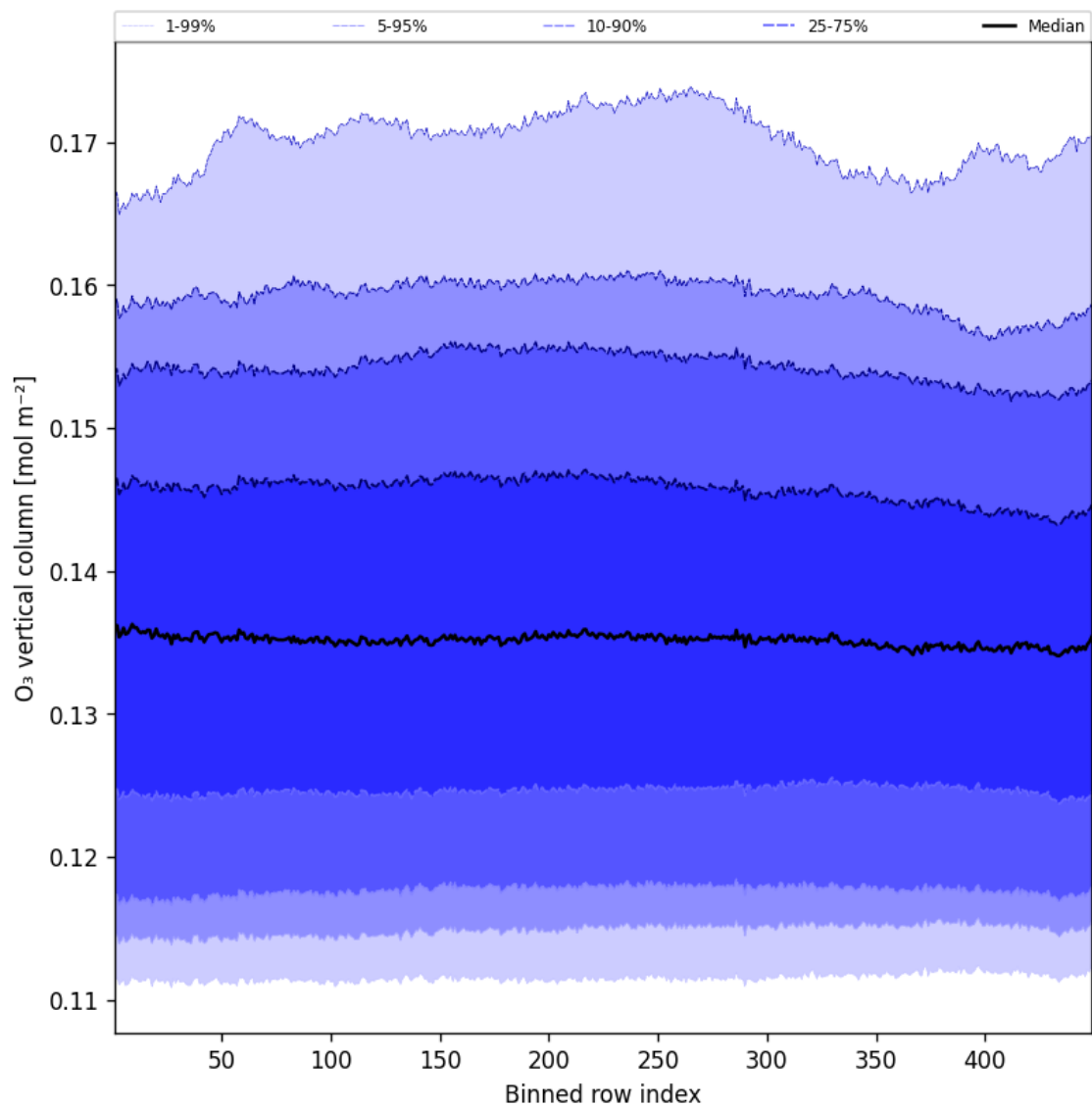
Figure 41: Along track statistics of “O 3 vertical column” for 2025-07-04 to 2025-07-05
