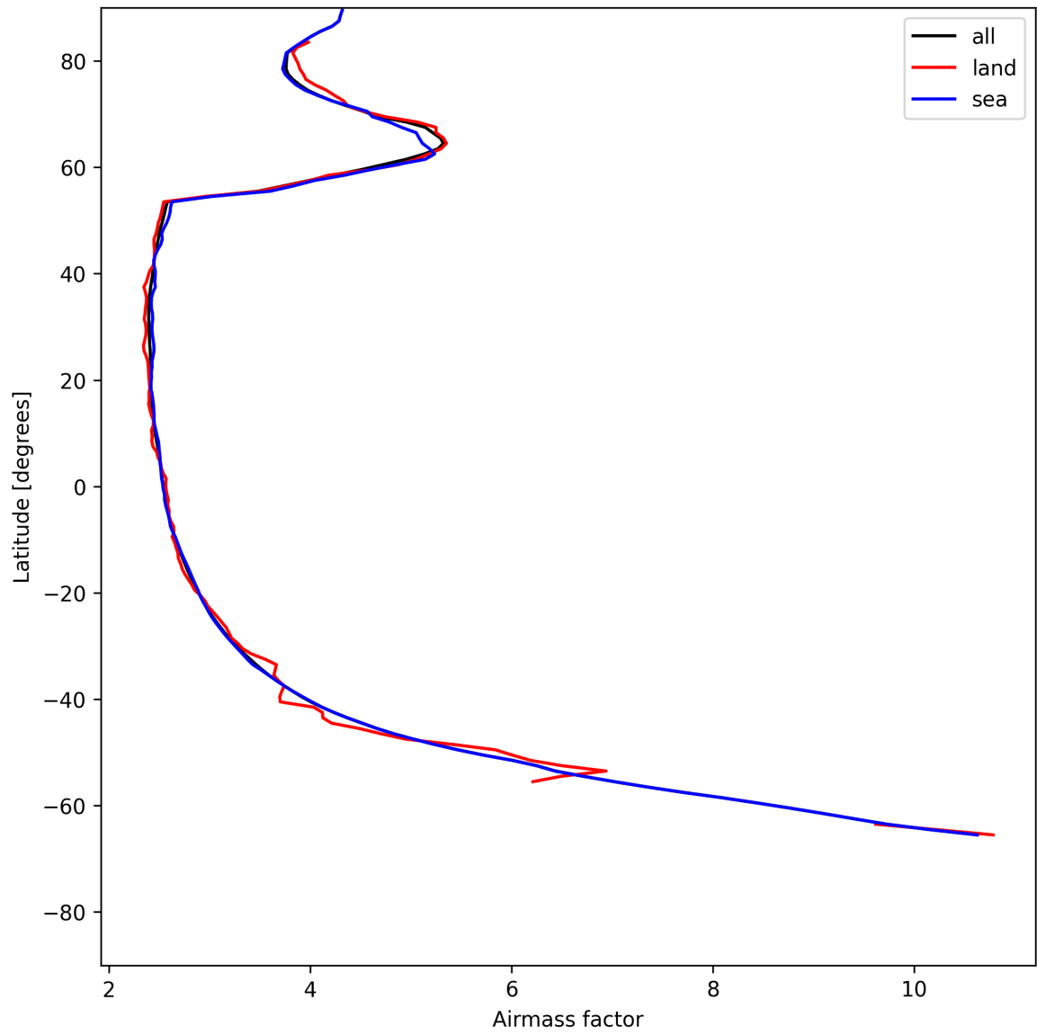
Figure 25: Zonal average of “Airmass factor” for 2025-07-04 to 2025-07-05.
