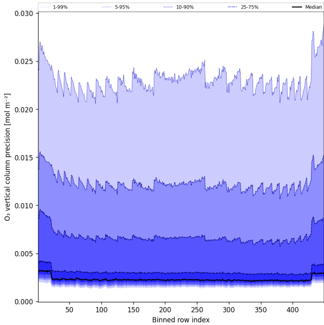
Figure 42: Along track statistics of “O 3 vertical column precision” for 2025-07-04 to 2025-07-05
