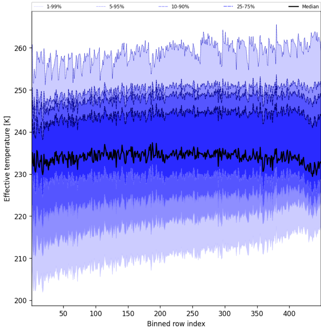
Figure 50: Along track statistics of “Effective temperature” for 2025-07-04 to 2025-07-05
