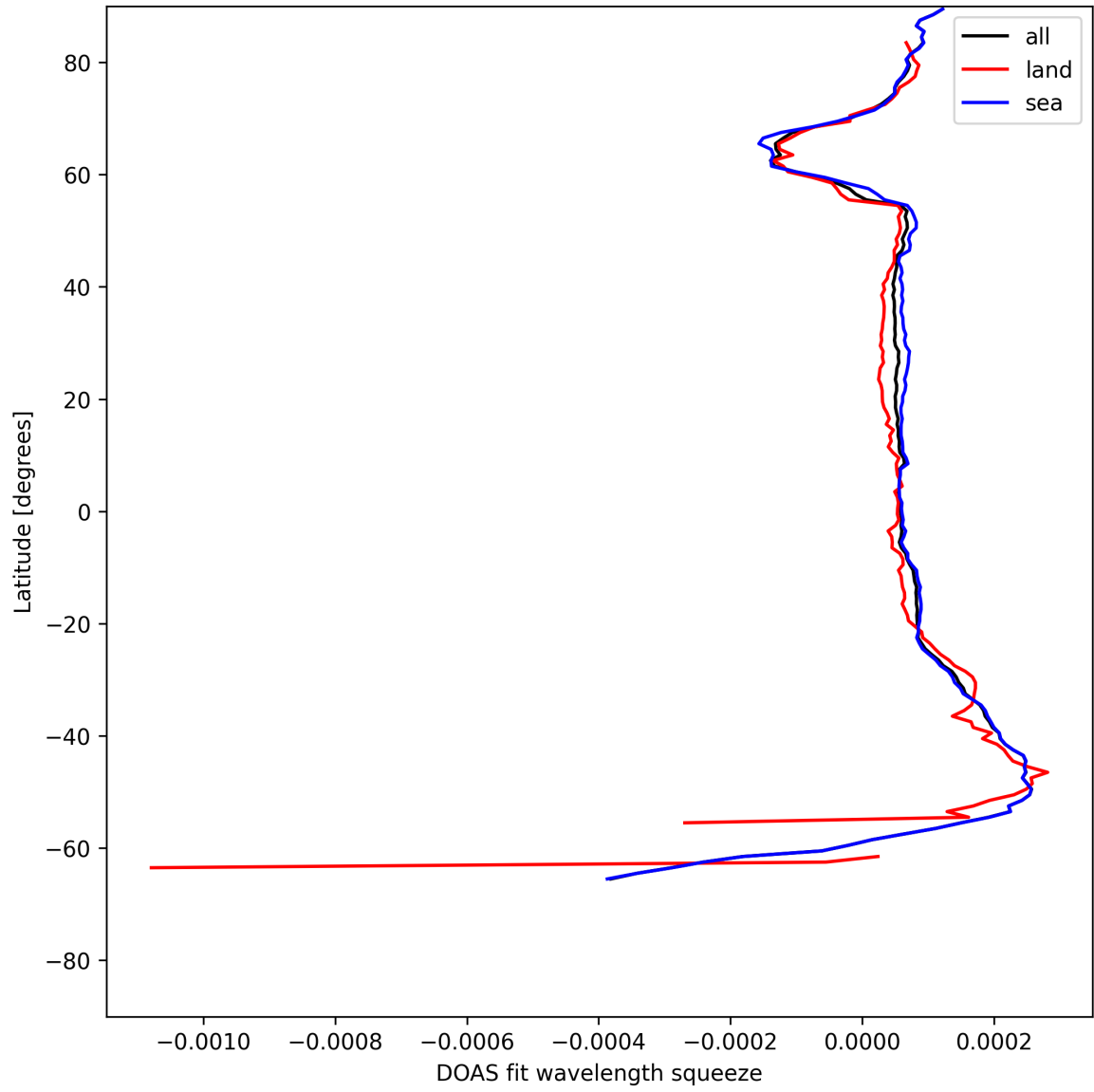
Figure 24: Zonal average of “DOAS fit wavelength squeeze” for 2025-07-05 to 2025-07-06.
