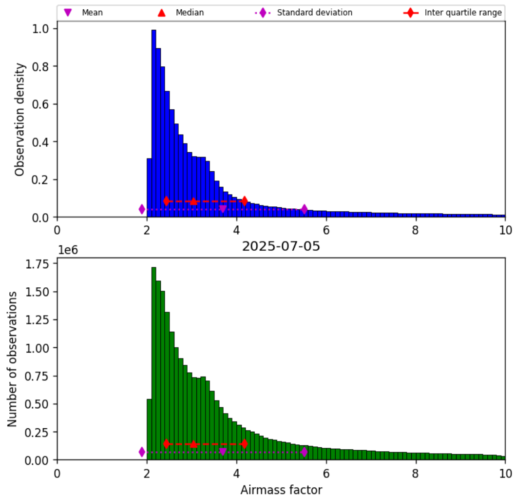
Figure 37: Histogram of “Airmass factor” for 2025-07-05 to 2025-07-06
