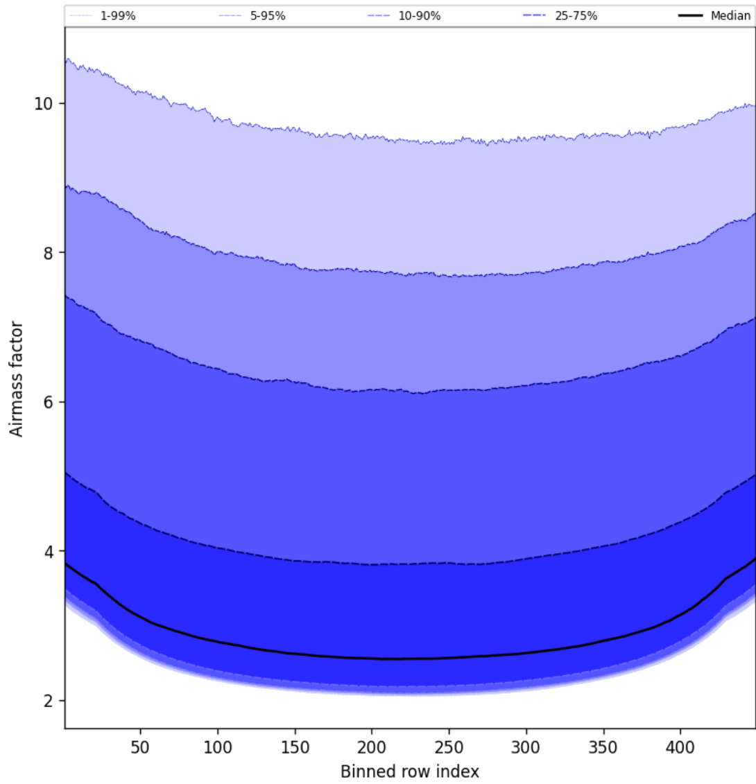
Figure 49: Along track statistics of “Airmass factor” for 2025-07-05 to 2025-07-06
