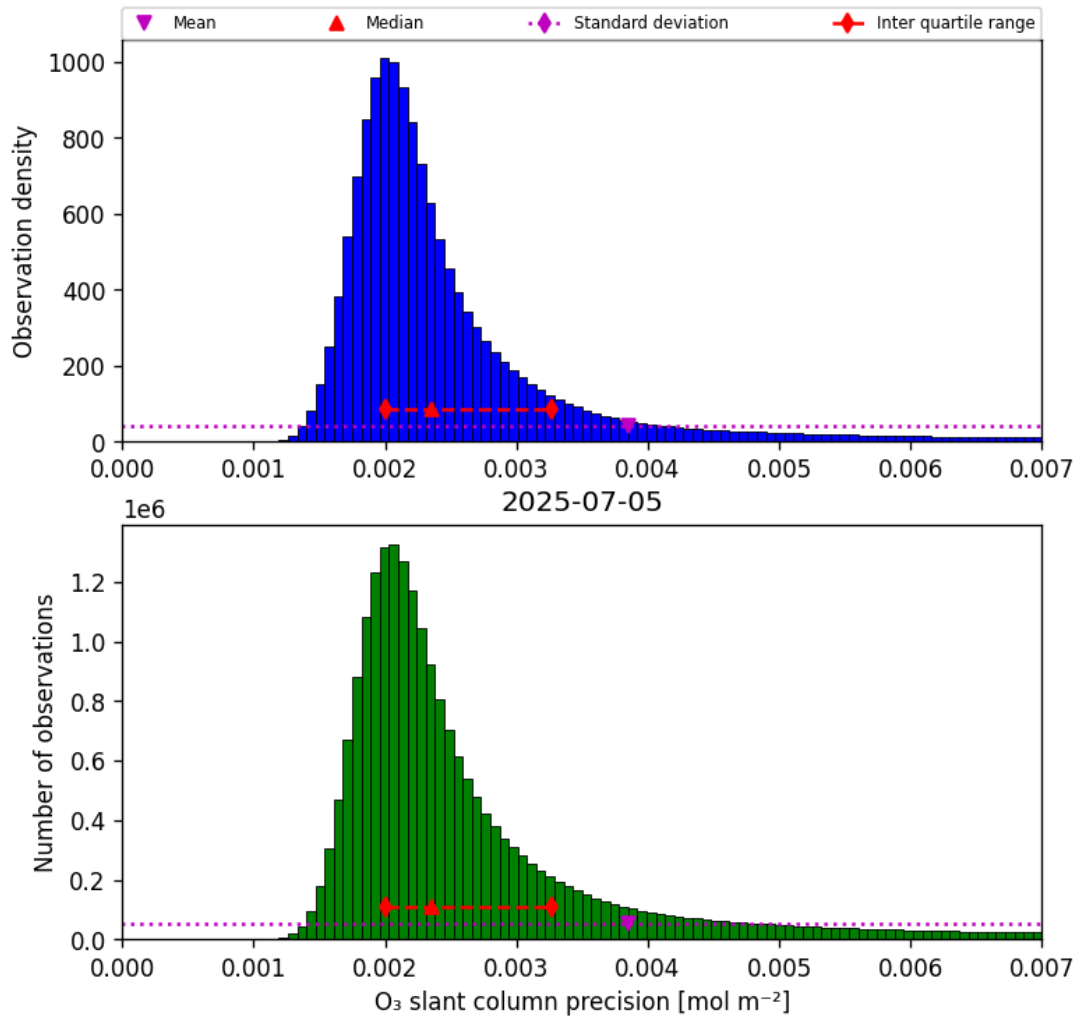
Figure 32: Histogram of “O 3 slant column precision” for 2025-07-05 to 2025-07-06
