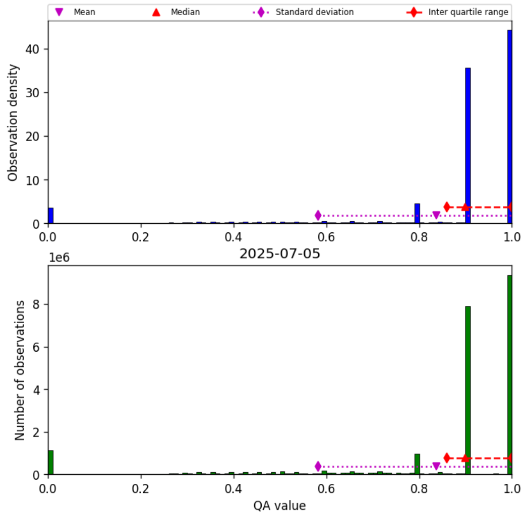
Figure 28: Histogram of “QA value” for 2025-07-05 to 2025-07-06
