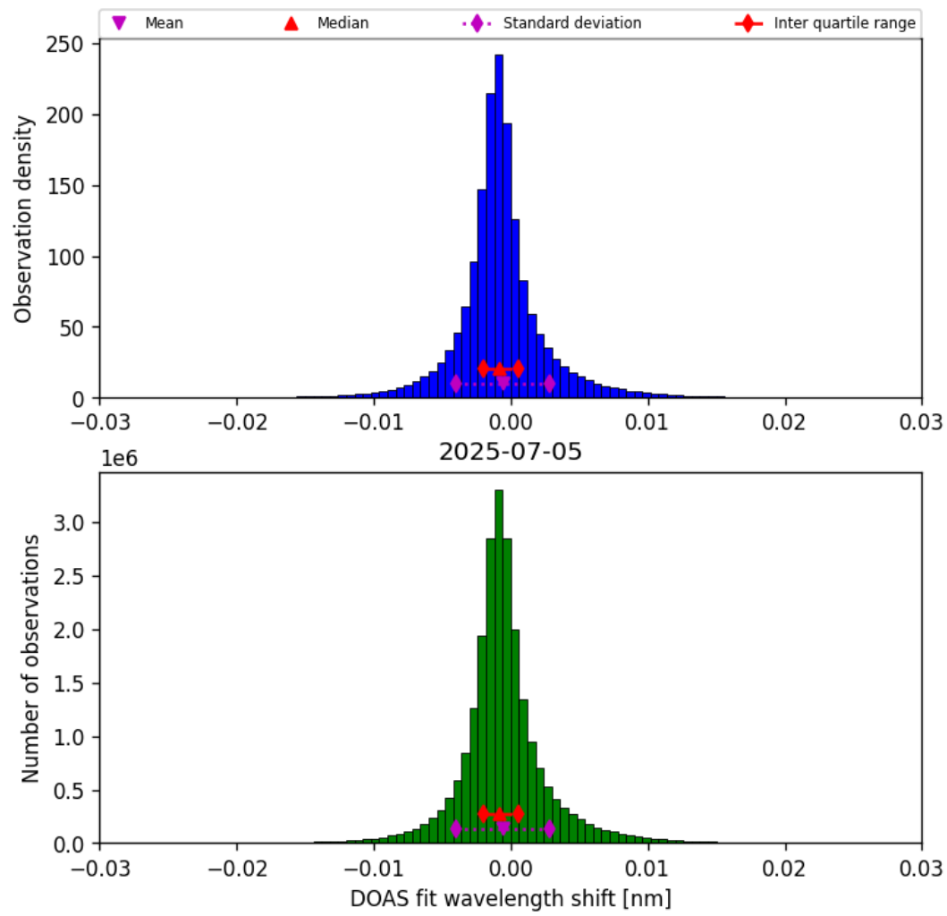
Figure 35: Histogram of “DOAS fit wavelength shift” for 2025-07-05 to 2025-07-06
