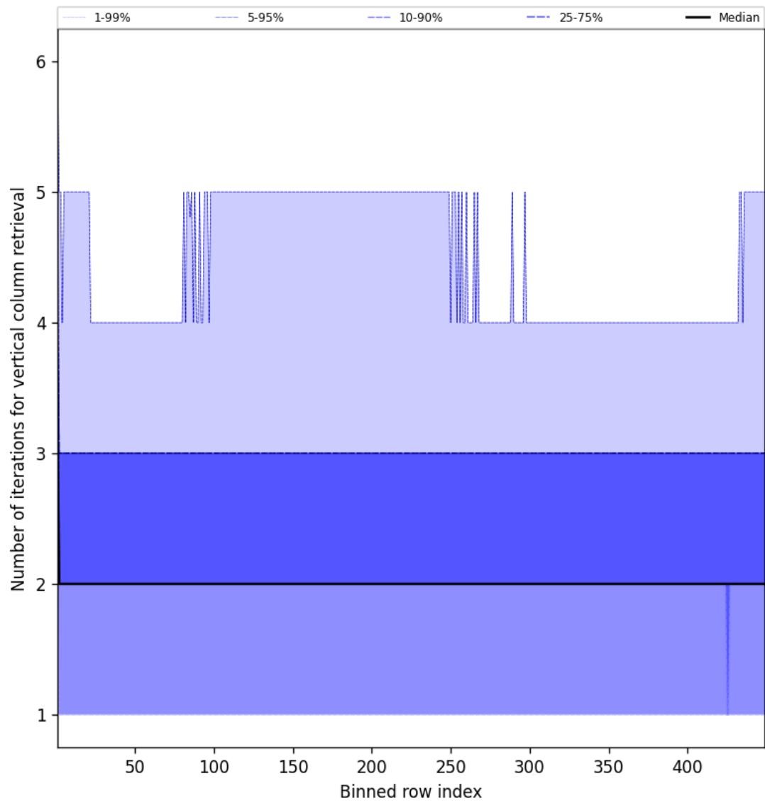
Figure 51: Along track statistics of “Number of iterations for vertical column retrieval” for 2025-07-05 to 2025-07-06
