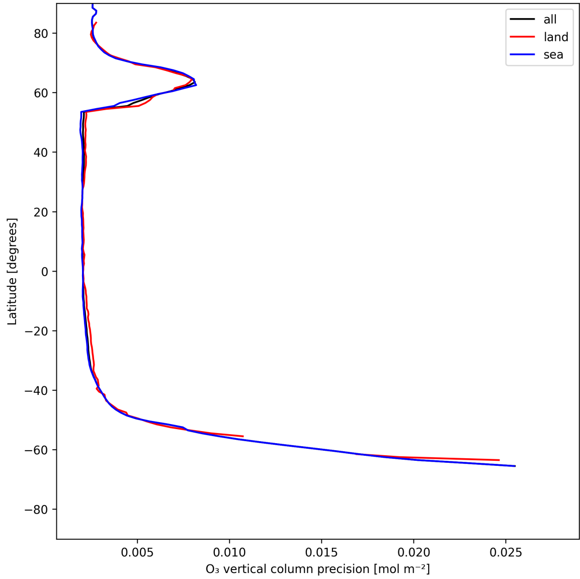
Figure 18: Zonal average of “O 3 vertical column precision” for 2025-07-05 to 2025-07-06.
