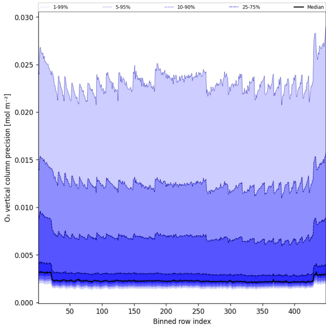
Figure 42: Along track statistics of “O 3 vertical column precision” for 2025-07-05 to 2025-07-06
