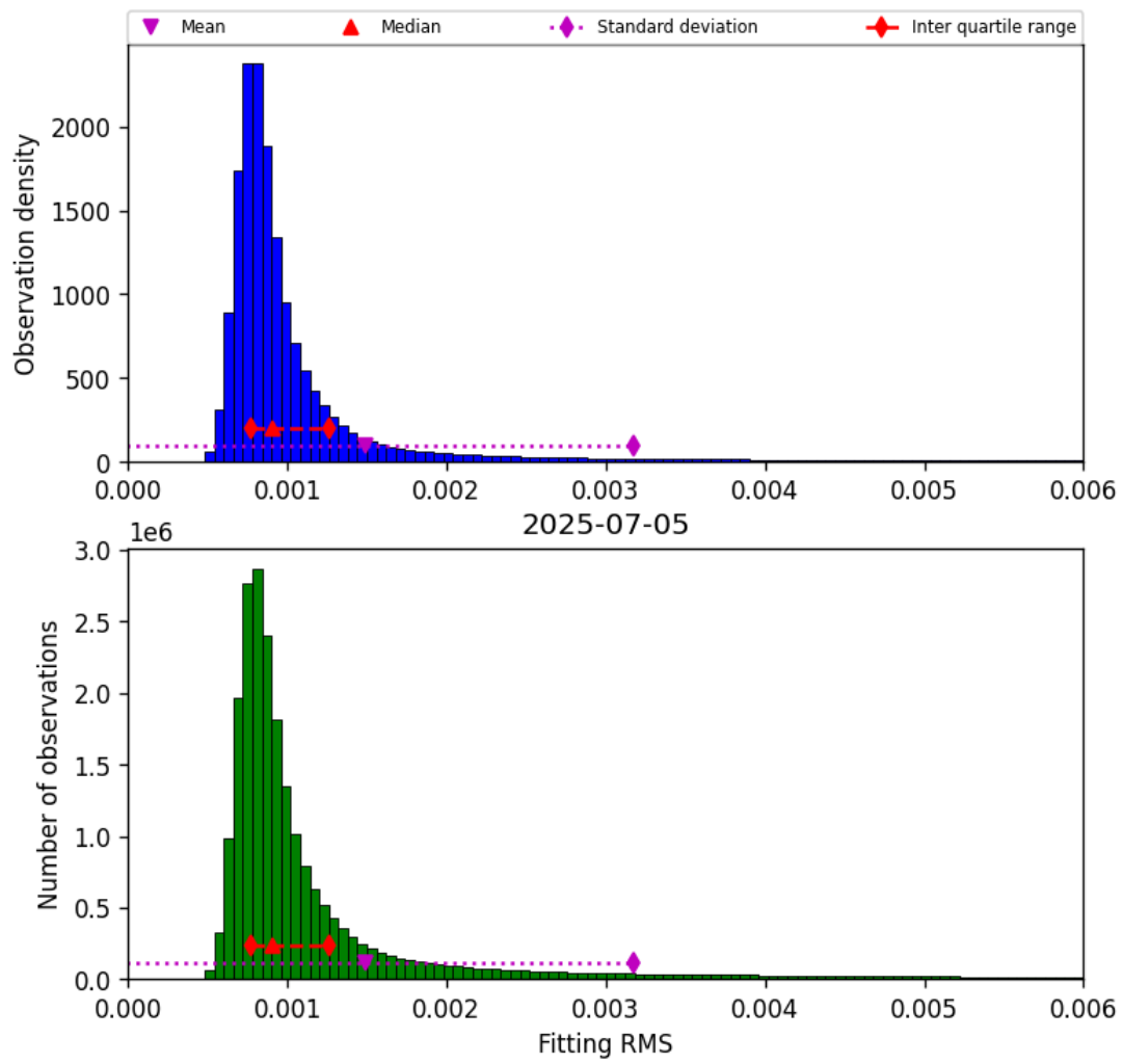
Figure 34: Histogram of “Fitting RMS” for 2025-07-05 to 2025-07-06
