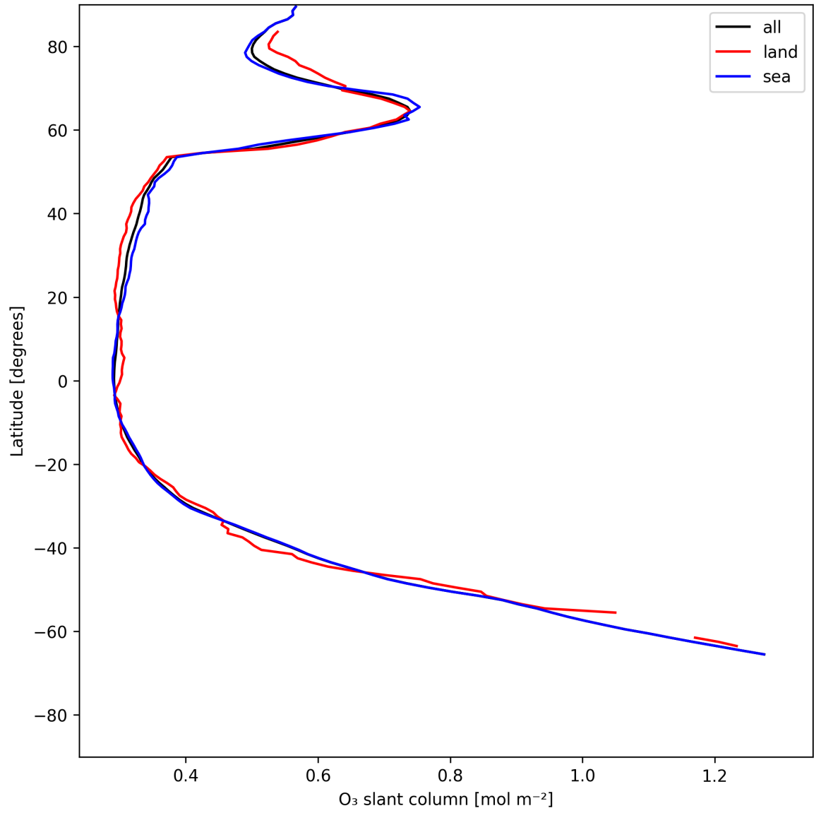
Figure 19: Zonal average of “O 3 slant column” for 2025-07-05 to 2025-07-06.
