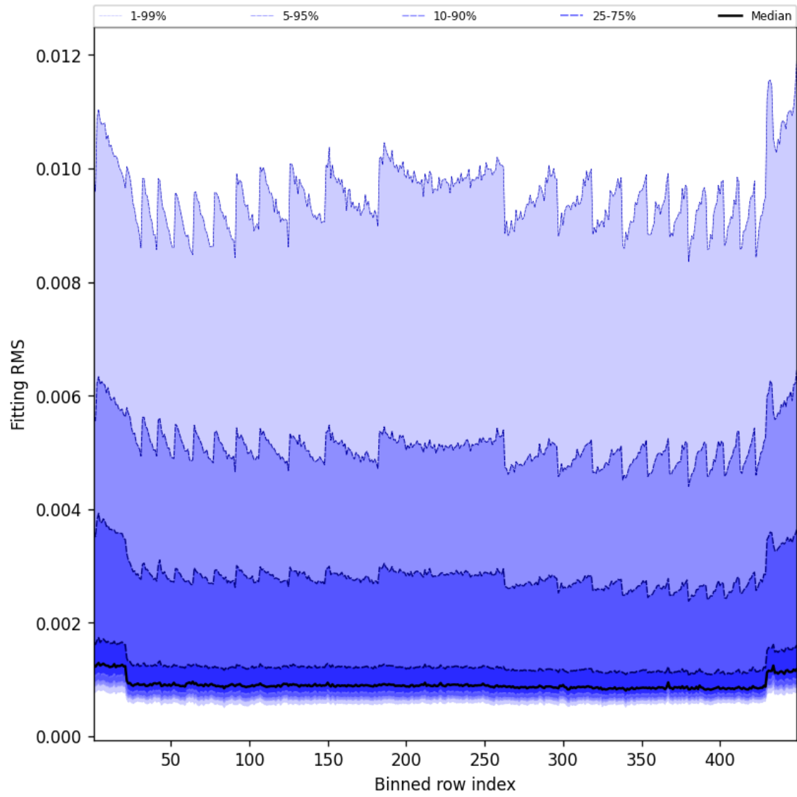
Figure 46: Along track statistics of “Fitting RMS” for 2025-07-05 to 2025-07-06
