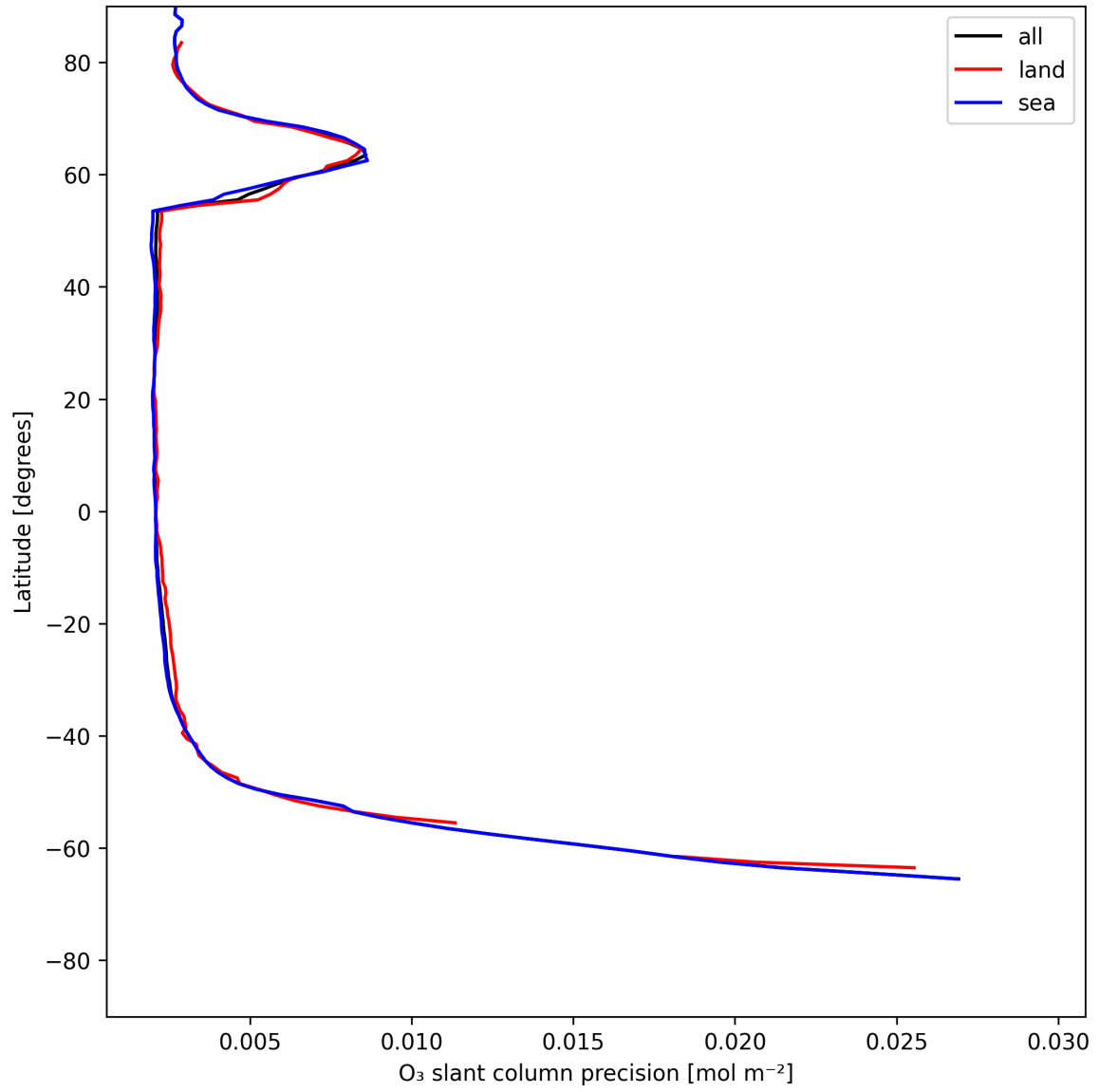
Figure 20: Zonal average of “O 3 slant column precision” for 2025-07-05 to 2025-07-06.
