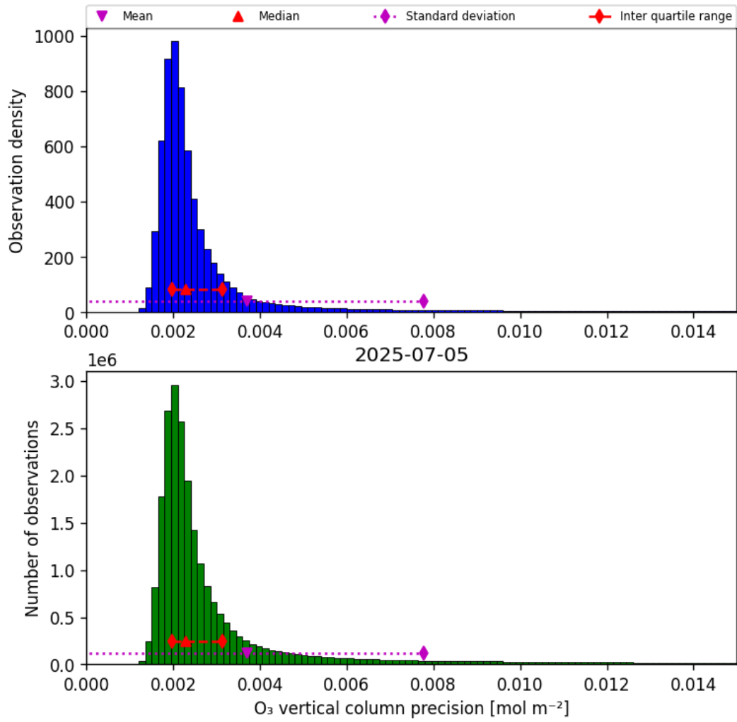
Figure 30: Histogram of “O 3 vertical column precision” for 2025-07-05 to 2025-07-06
