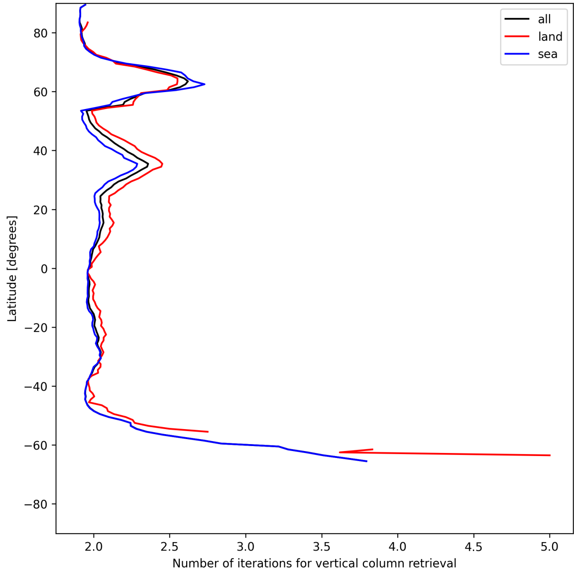
Figure 27: Zonal average of “Number of iterations for vertical column retrieval” for 2025-07-05 to 2025-07-06.
