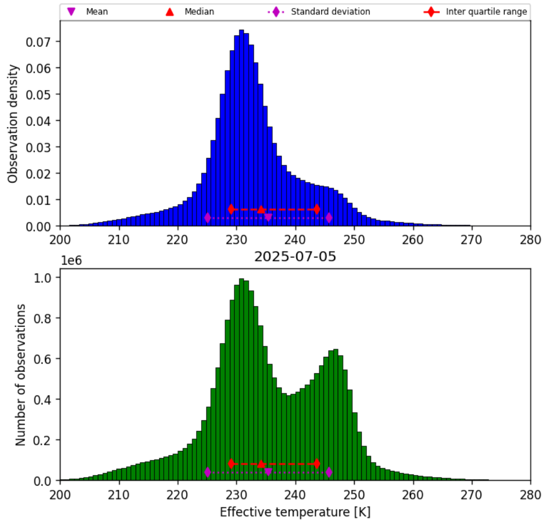
Figure 38: Histogram of “Effective temperature” for 2025-07-05 to 2025-07-06
