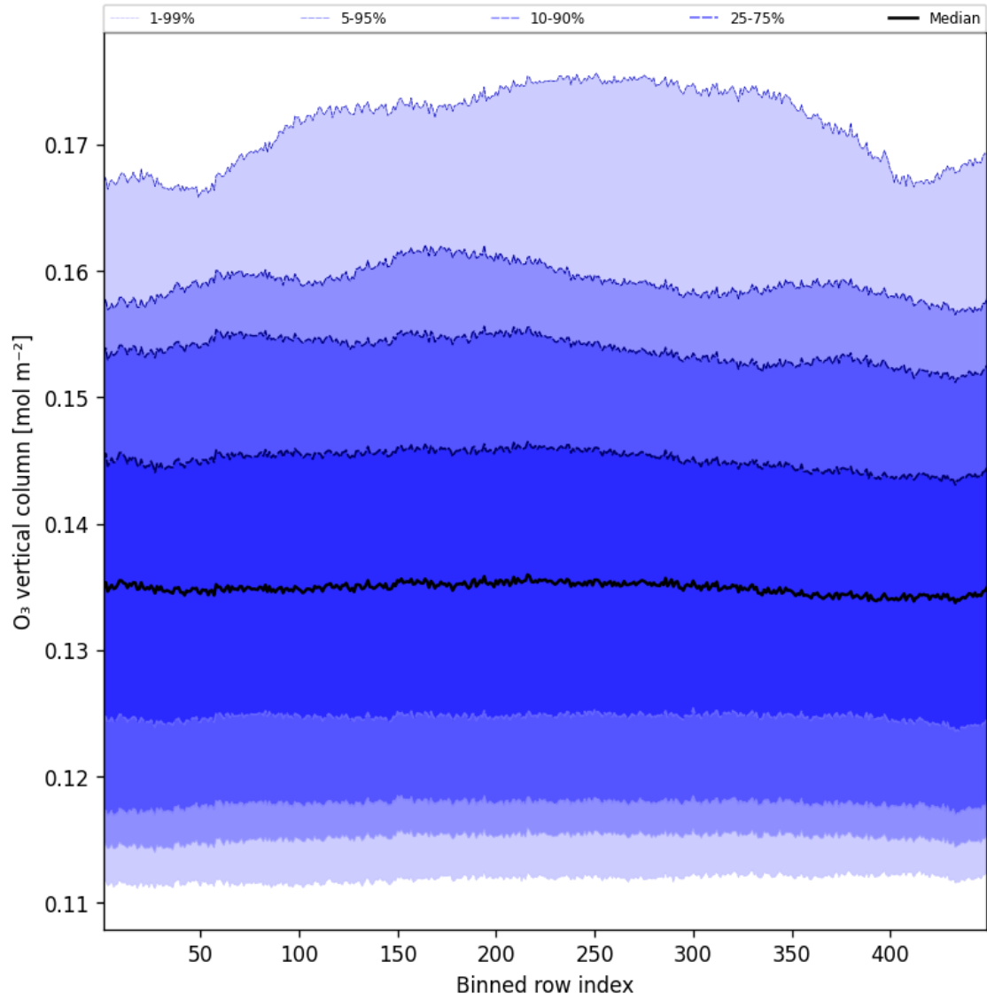
Figure 41: Along track statistics of “O 3 vertical column” for 2025-07-05 to 2025-07-06
