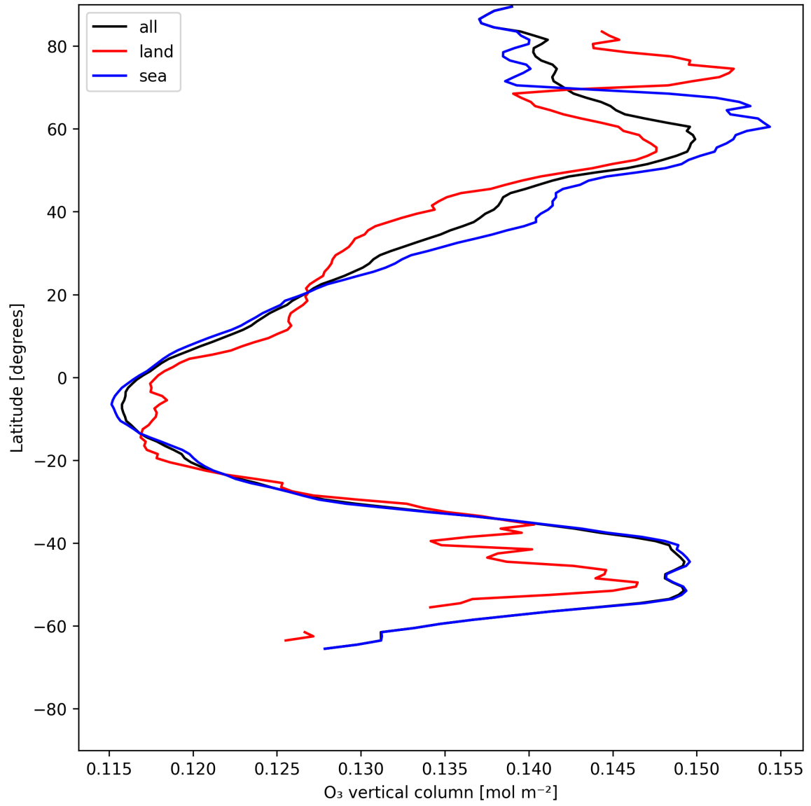
Figure 17: Zonal average of “O 3 vertical column” for 2025-07-05 to 2025-07-06.
