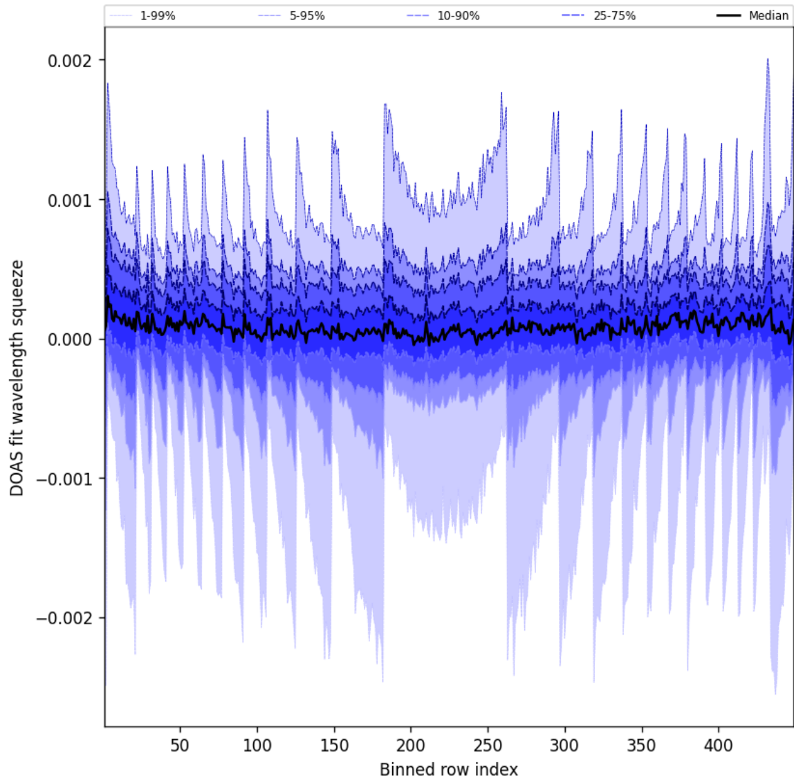
Figure 48: Along track statistics of “DOAS fit wavelength squeeze” for 2025-07-05 to 2025-07-06
