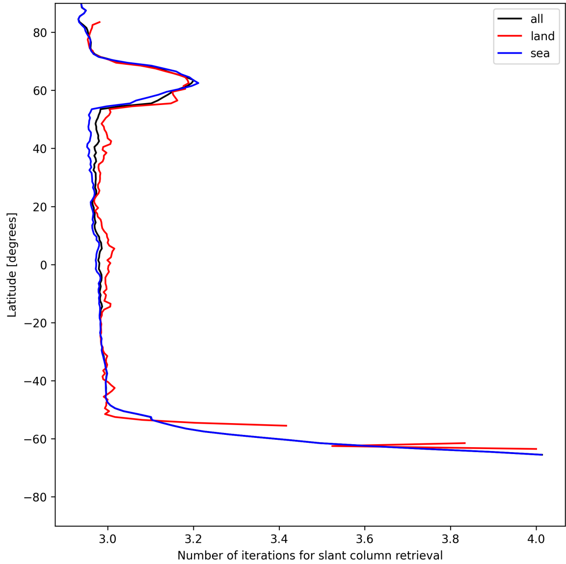
Figure 21: Zonal average of “Number of iterations for slant column retrieval” for 2025-07-05 to 2025-07-06.
