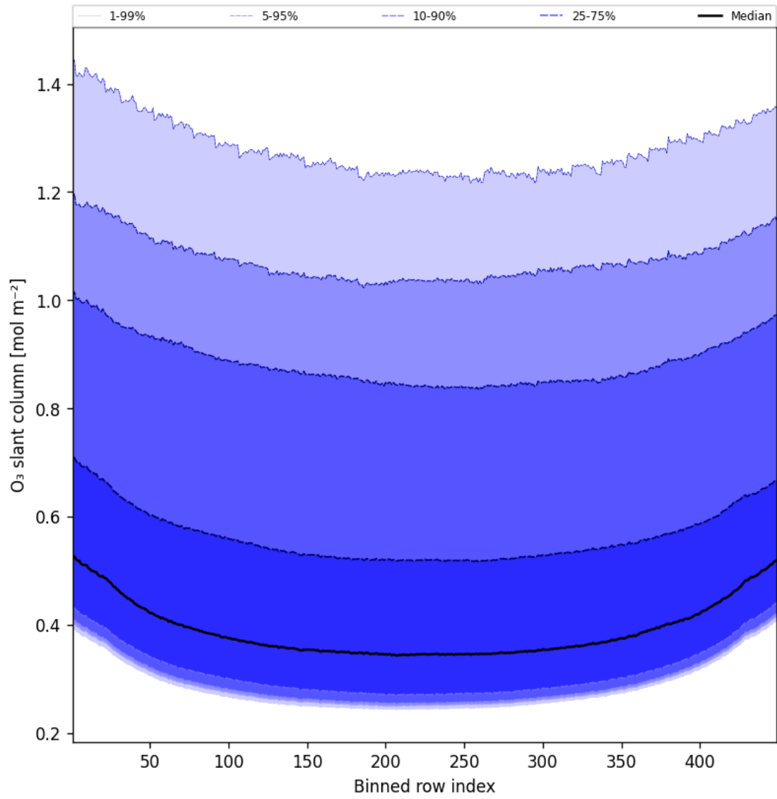
Figure 43: Along track statistics of “O 3 slant column” for 2025-07-05 to 2025-07-06
