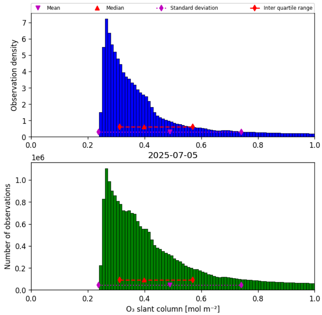
Figure 31: Histogram of “O 3 slant column” for 2025-07-05 to 2025-07-06
