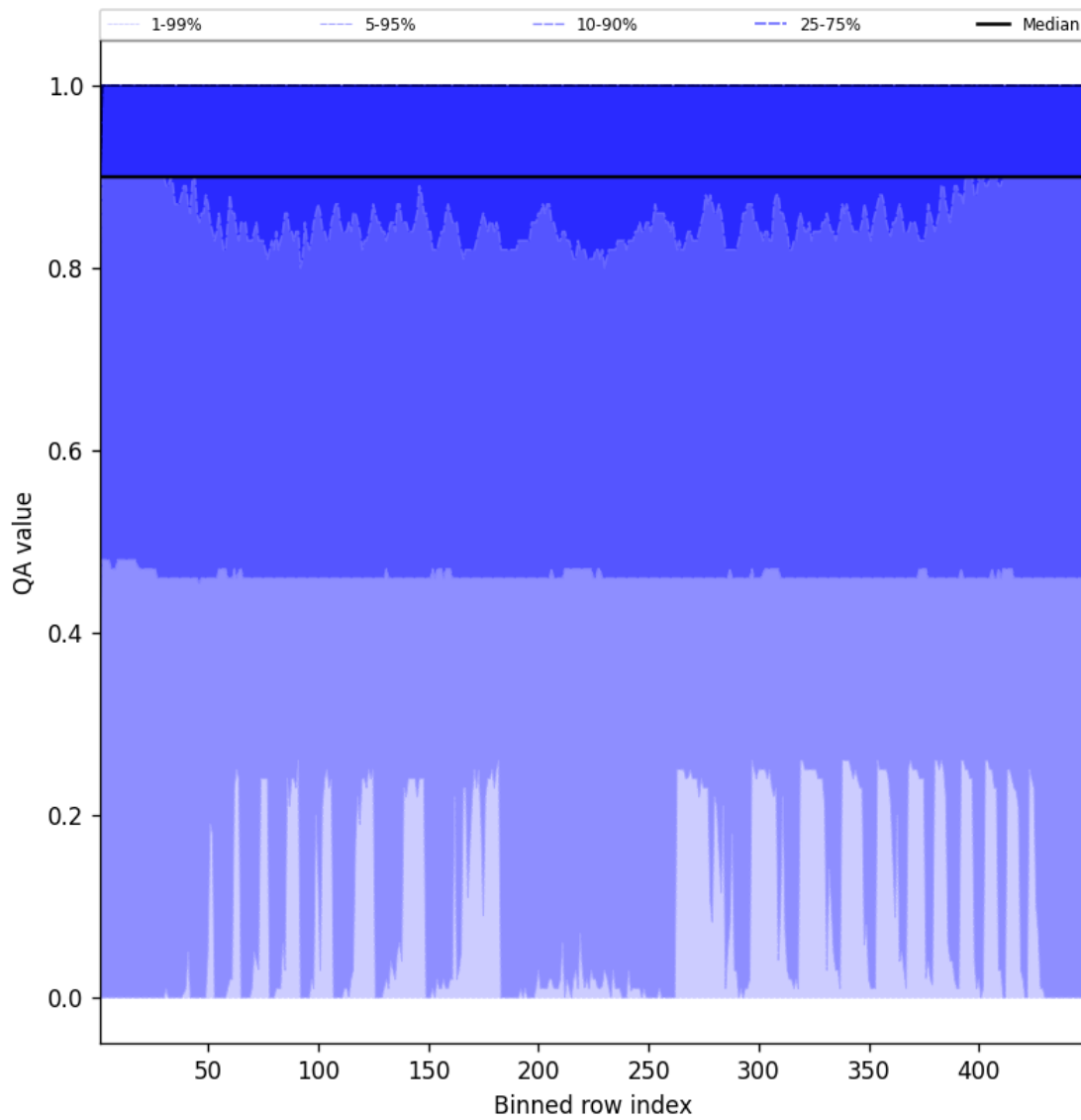
Figure 40: Along track statistics of “QA value” for 2025-07-05 to 2025-07-06
