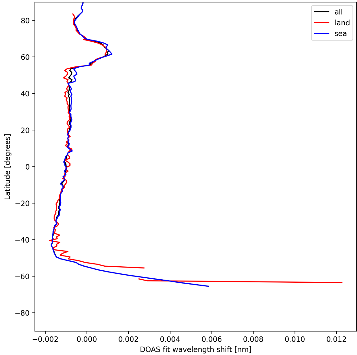
Figure 23: Zonal average of “DOAS fit wavelength shift” for 2025-07-05 to 2025-07-06.
