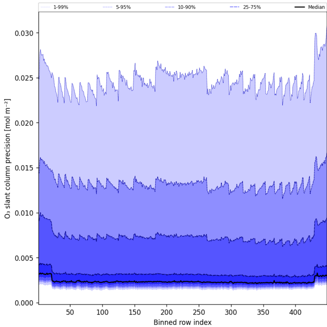
Figure 44: Along track statistics of “O 3 slant column precision” for 2025-07-05 to 2025-07-06
