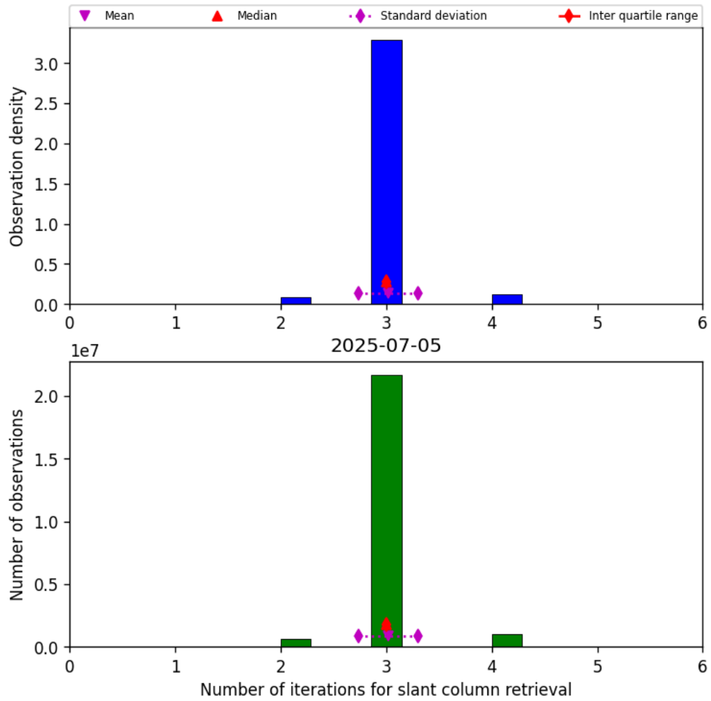
Figure 33: Histogram of “Number of iterations for slant column retrieval” for 2025-07-05 to 2025-07-06
