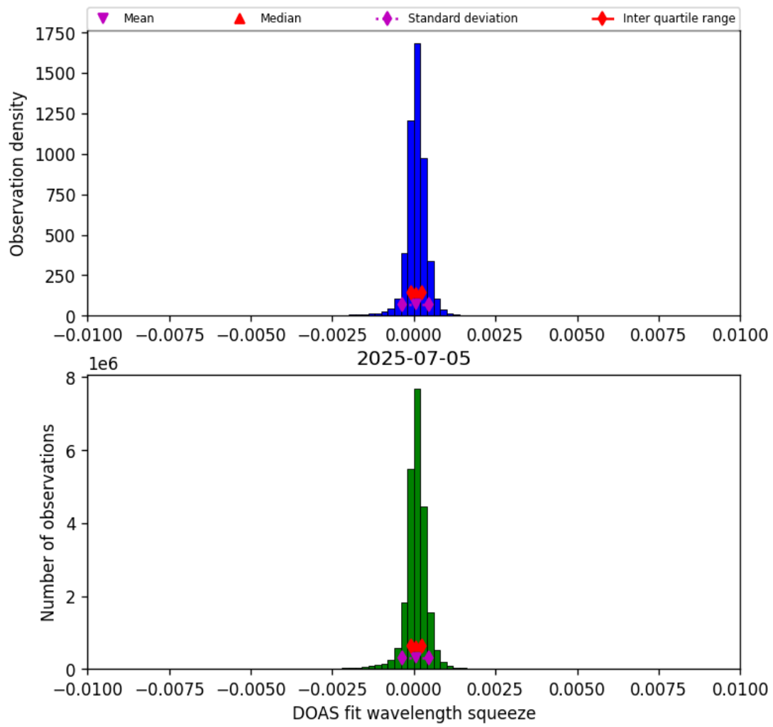
Figure 36: Histogram of “DOAS fit wavelength squeeze” for 2025-07-05 to 2025-07-06
