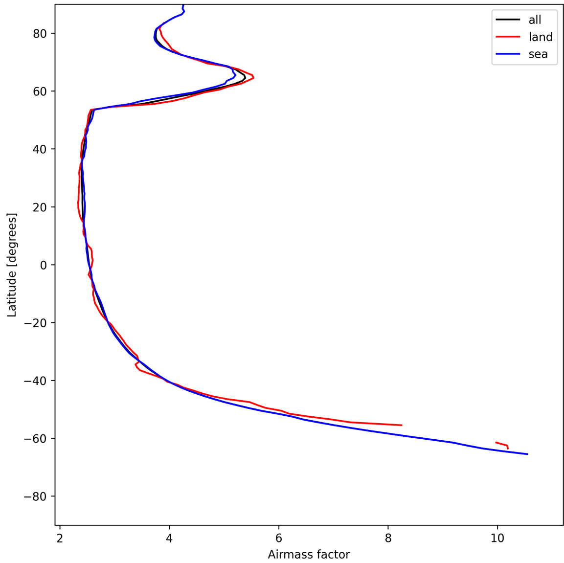
Figure 25: Zonal average of “Airmass factor” for 2025-07-05 to 2025-07-06.
