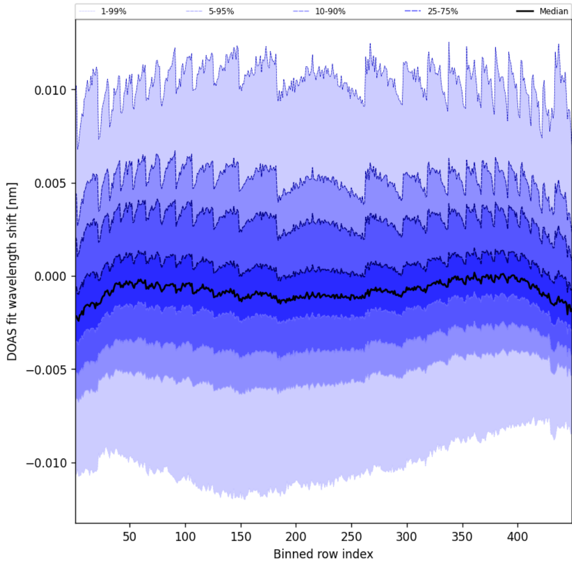
Figure 47: Along track statistics of “DOAS fit wavelength shift” for 2025-07-05 to 2025-07-06
