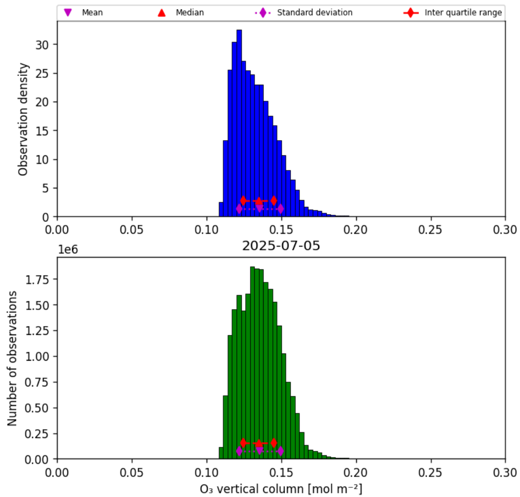
Figure 29: Histogram of “O 3 vertical column” for 2025-07-05 to 2025-07-06
