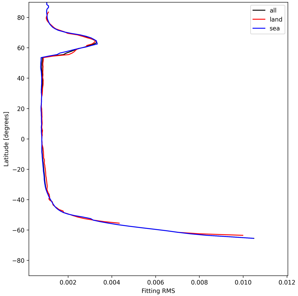
Figure 22: Zonal average of “Fitting RMS” for 2025-07-05 to 2025-07-06.
