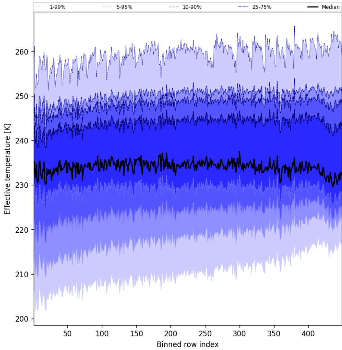
Figure 50: Along track statistics of “Effective temperature” for 2025-07-05 to 2025-07-06
