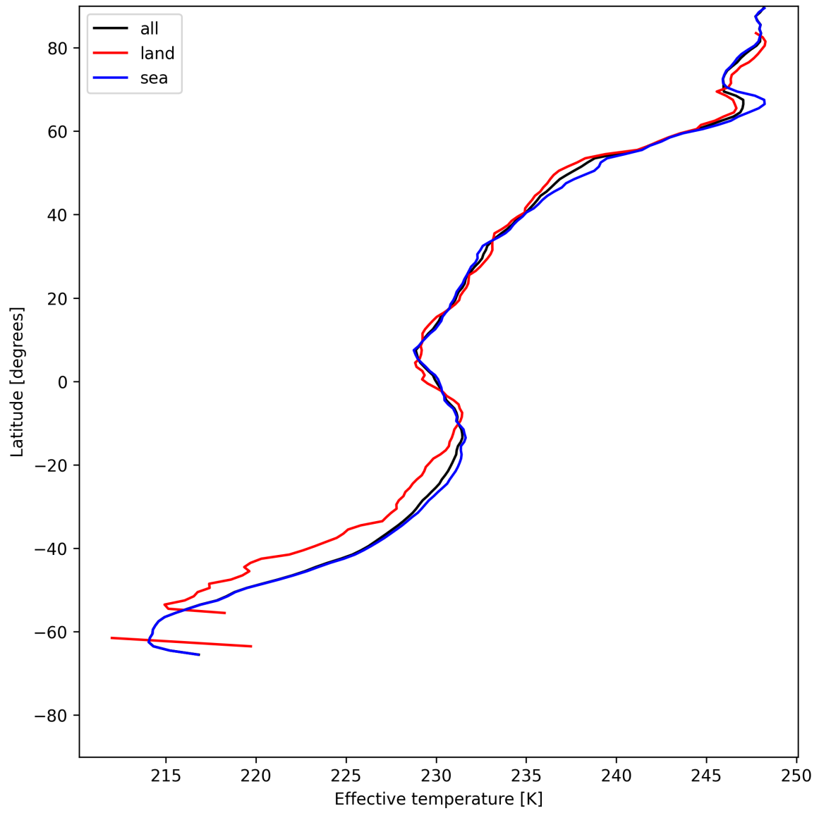
Figure 26: Zonal average of "Effective temperature" for 2025-07-05 to 2025-07-06.
