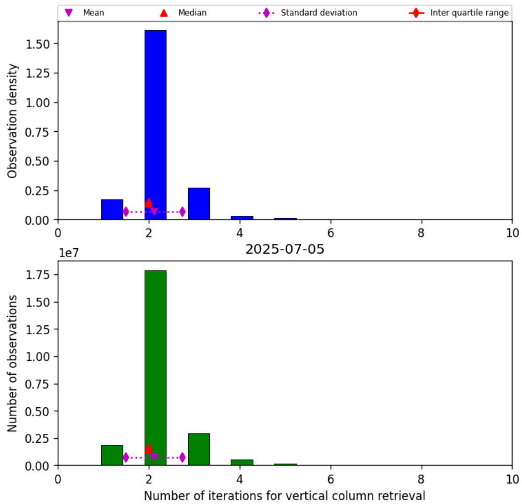
Figure 39: Histogram of “Number of iterations for vertical column retrieval” for 2025-07-05 to 2025-07-06
