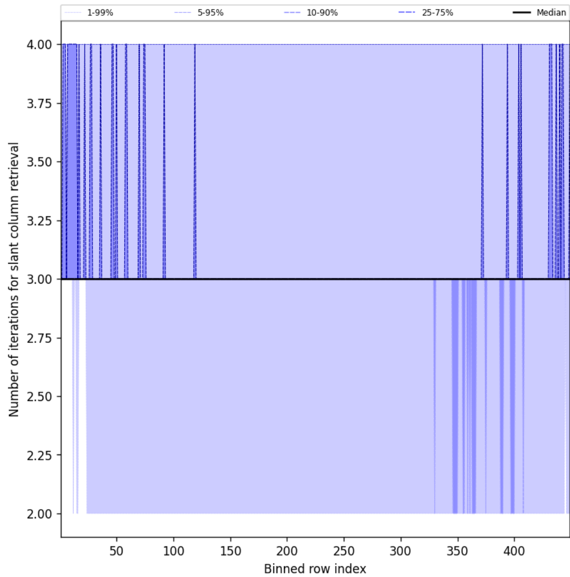
Figure 45: Along track statistics of “Number of iterations for slant column retrieval” for 2025-07-05 to 2025-07-06
