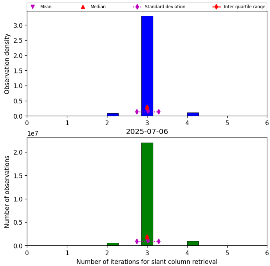
Figure 33: Histogram of “Number of iterations for slant column retrieval” for 2025-07-06 to 2025-07-06
