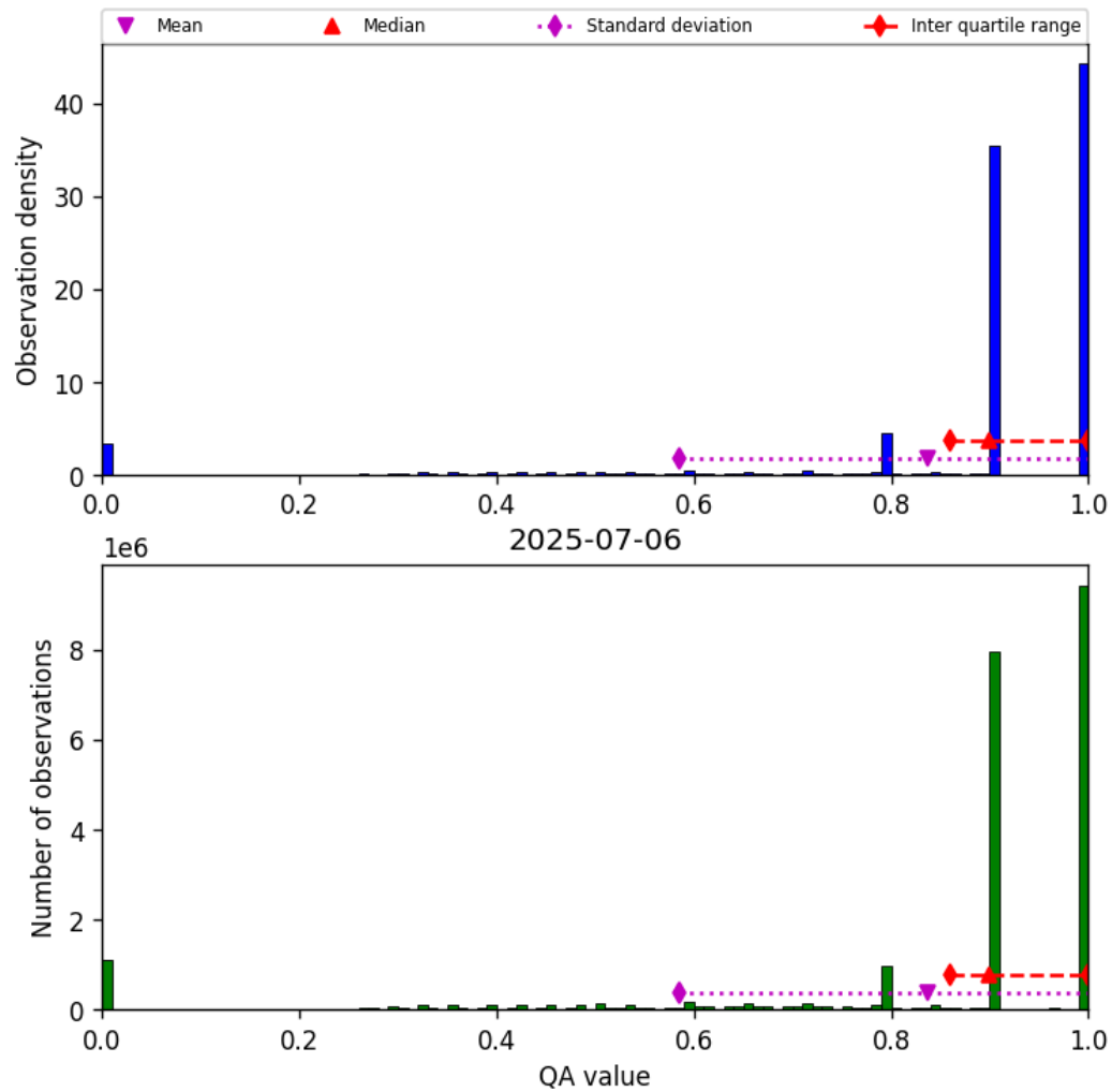
Figure 28: Histogram of “QA value” for 2025-07-06 to 2025-07-06
