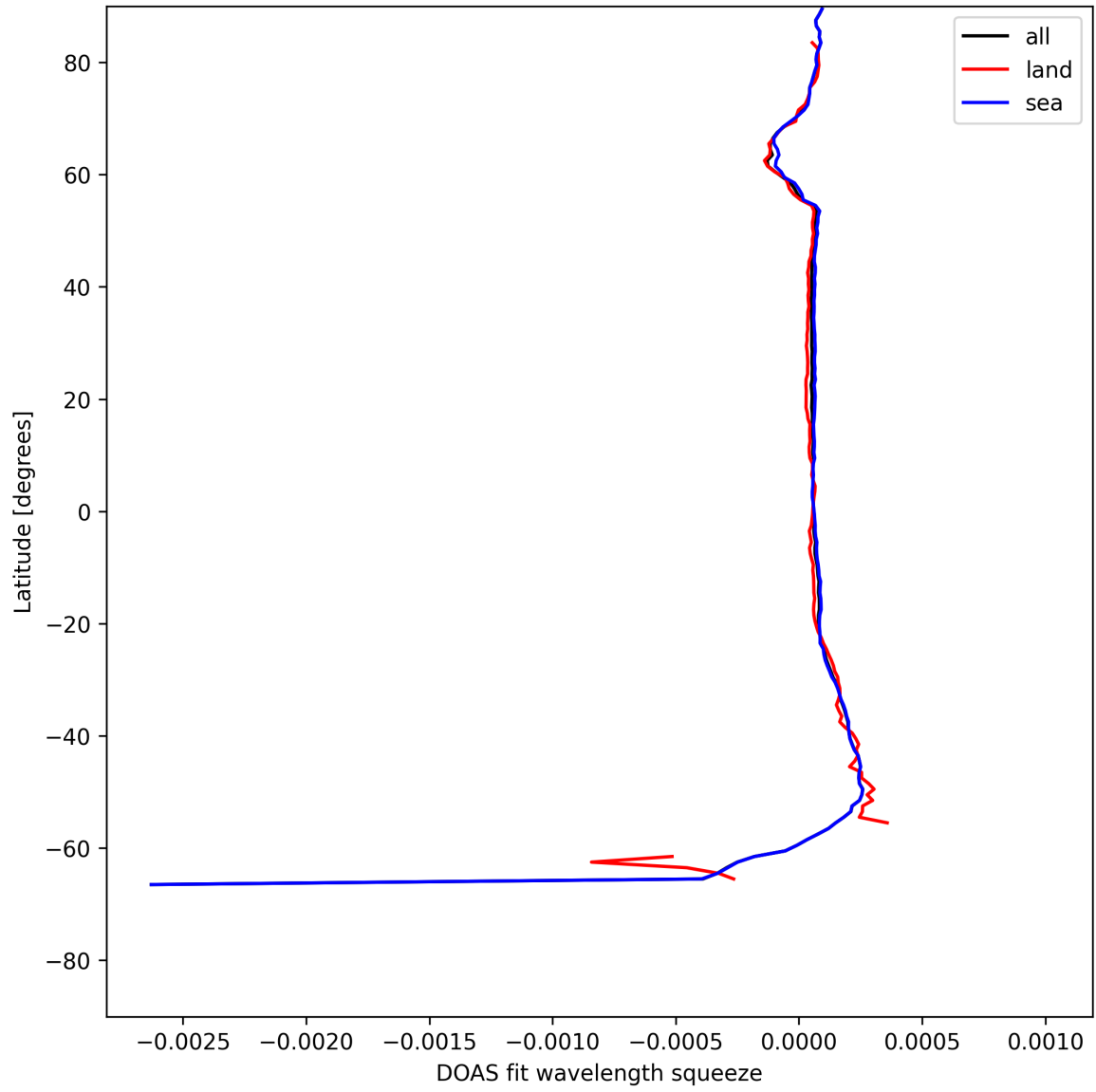
Figure 24: Zonal average of “DOAS fit wavelength squeeze” for 2025-07-06 to 2025-07-06.
