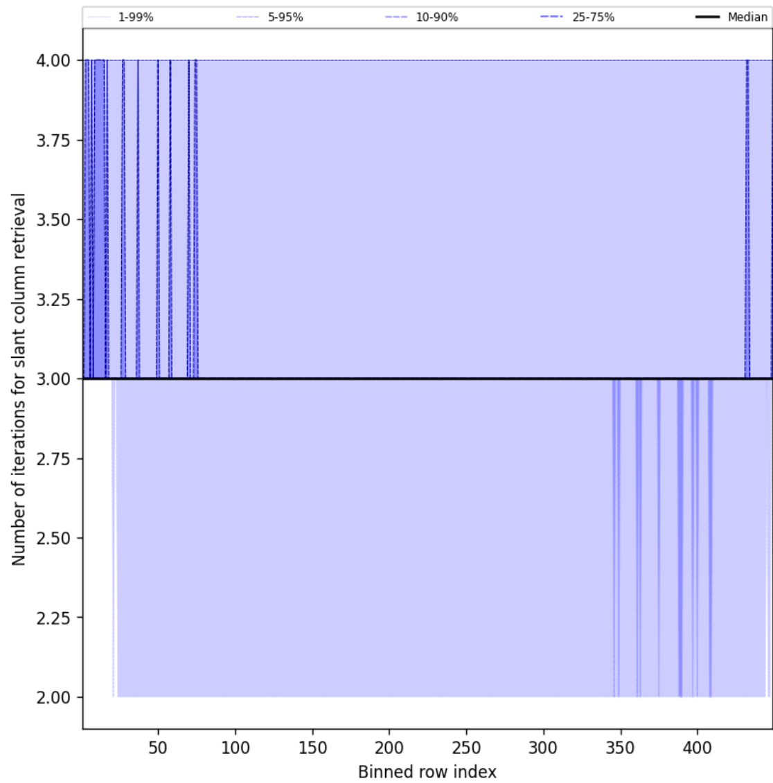
Figure 45: Along track statistics of “Number of iterations for slant column retrieval” for 2025-07-06 to 2025-07-06
