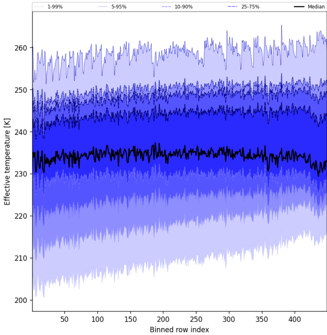
Figure 50: Along track statistics of “Effective temperature” for 2025-07-06 to 2025-07-06
