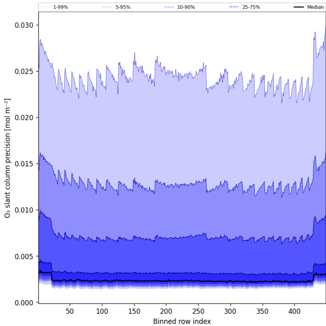
Figure 44: Along track statistics of “O 3 slant column precision” for 2025-07-06 to 2025-07-06
