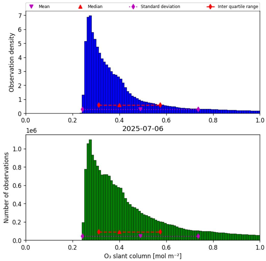
Figure 31: Histogram of “O 3 slant column” for 2025-07-06 to 2025-07-06
