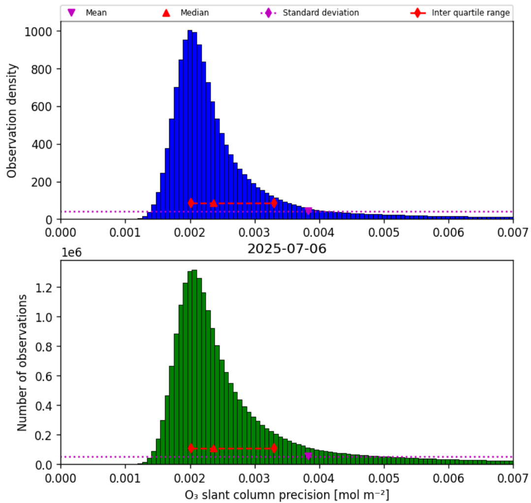
Figure 32: Histogram of “O 3 slant column precision” for 2025-07-06 to 2025-07-06
