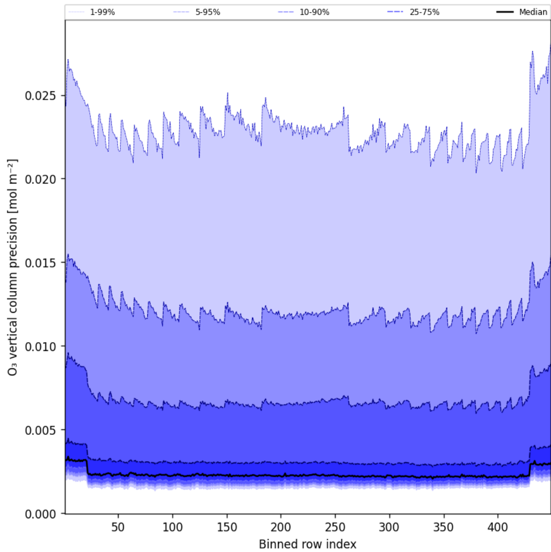
Figure 42: Along track statistics of “O 3 vertical column precision” for 2025-07-06 to 2025-07-06
