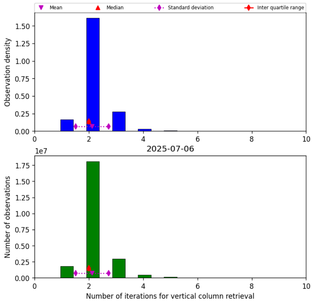
Figure 39: Histogram of “Number of iterations for vertical column retrieval” for 2025-07-06 to 2025-07-06
