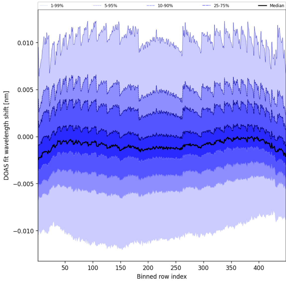
Figure 47: Along track statistics of “DOAS fit wavelength shift” for 2025-07-06 to 2025-07-06
