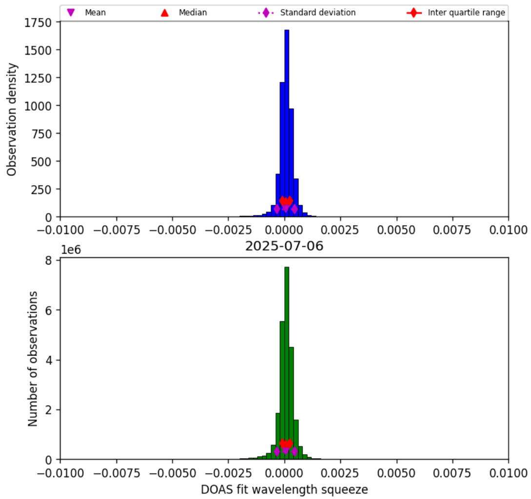
Figure 36: Histogram of “DOAS fit wavelength squeeze” for 2025-07-06 to 2025-07-06
