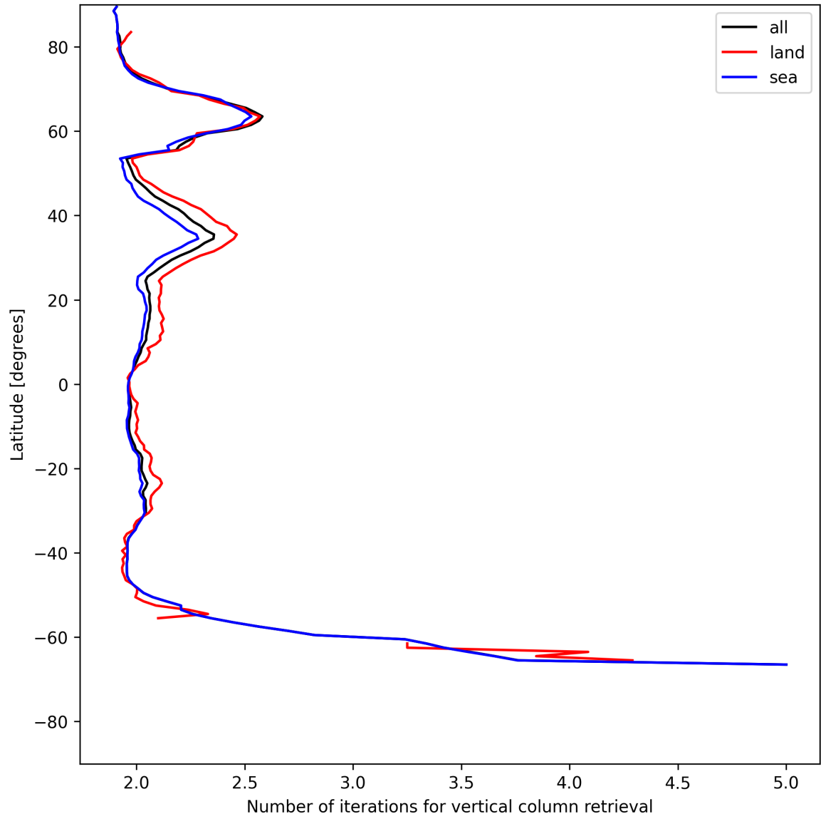
Figure 27: Zonal average of “Number of iterations for vertical column retrieval” for 2025-07-06 to 2025-07-06.
