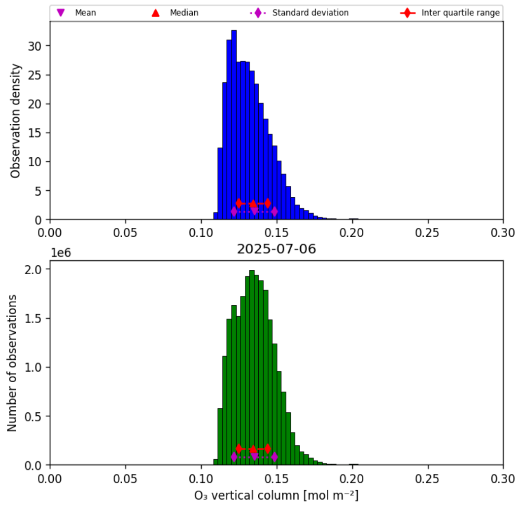
Figure 29: Histogram of “O 3 vertical column” for 2025-07-06 to 2025-07-06
