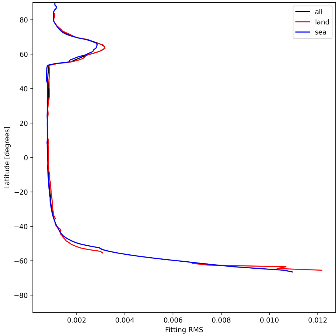
Figure 22: Zonal average of “Fitting RMS” for 2025-07-06 to 2025-07-06.
