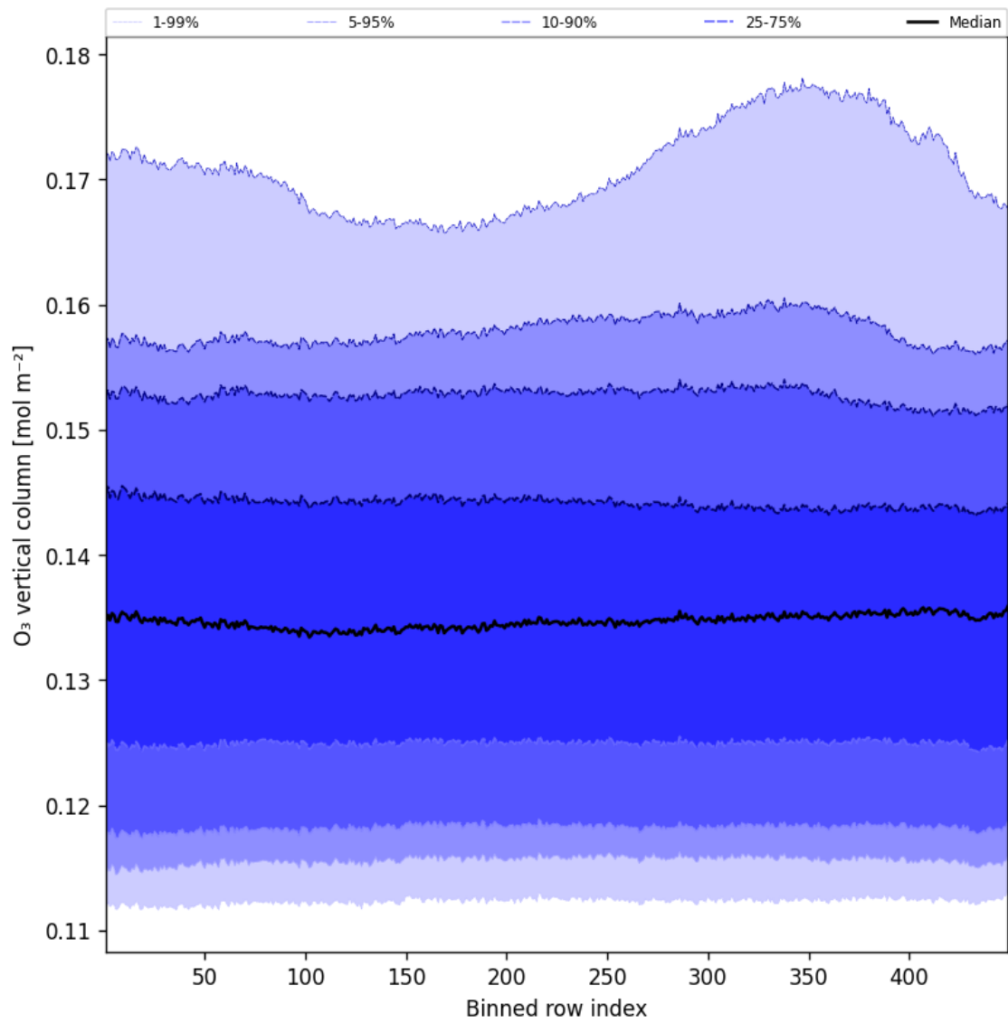
Figure 41: Along track statistics of “O 3 vertical column” for 2025-07-06 to 2025-07-06
