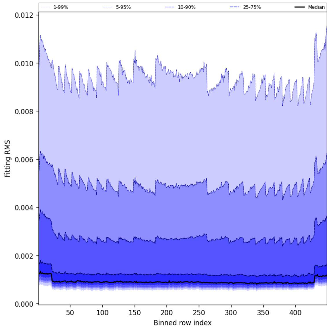
Figure 46: Along track statistics of “Fitting RMS” for 2025-07-06 to 2025-07-06
