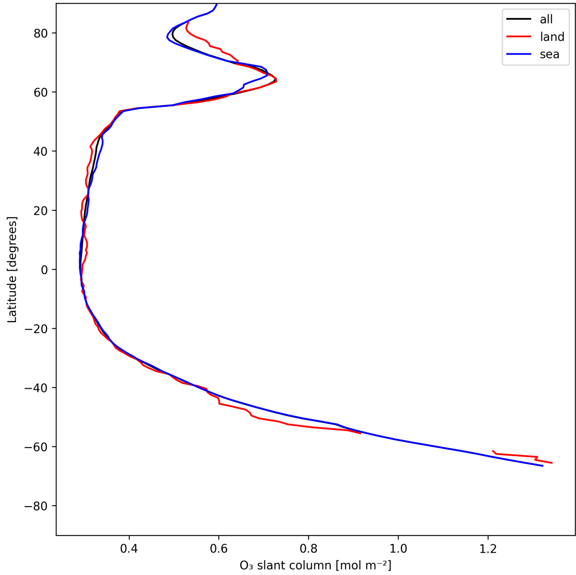
Figure 19: Zonal average of “O 3 slant column” for 2025-07-06 to 2025-07-06.
