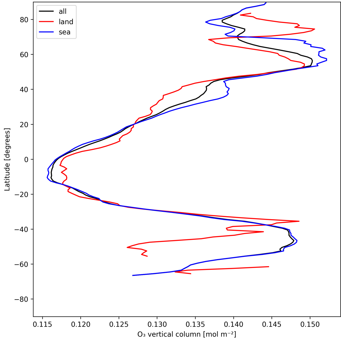
Figure 17: Zonal average of “O 3 vertical column” for 2025-07-06 to 2025-07-06.
