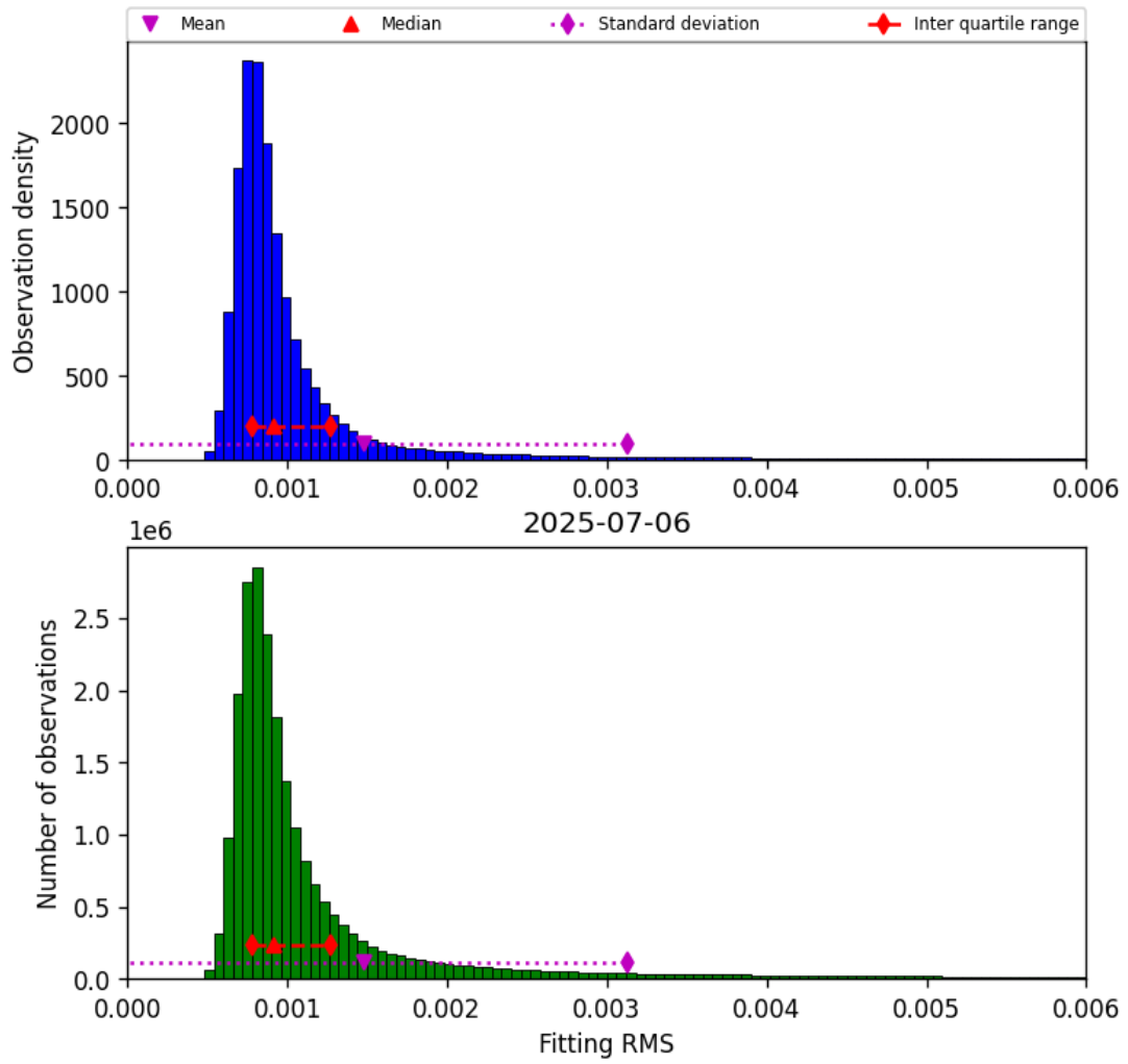
Figure 34: Histogram of “Fitting RMS” for 2025-07-06 to 2025-07-06
