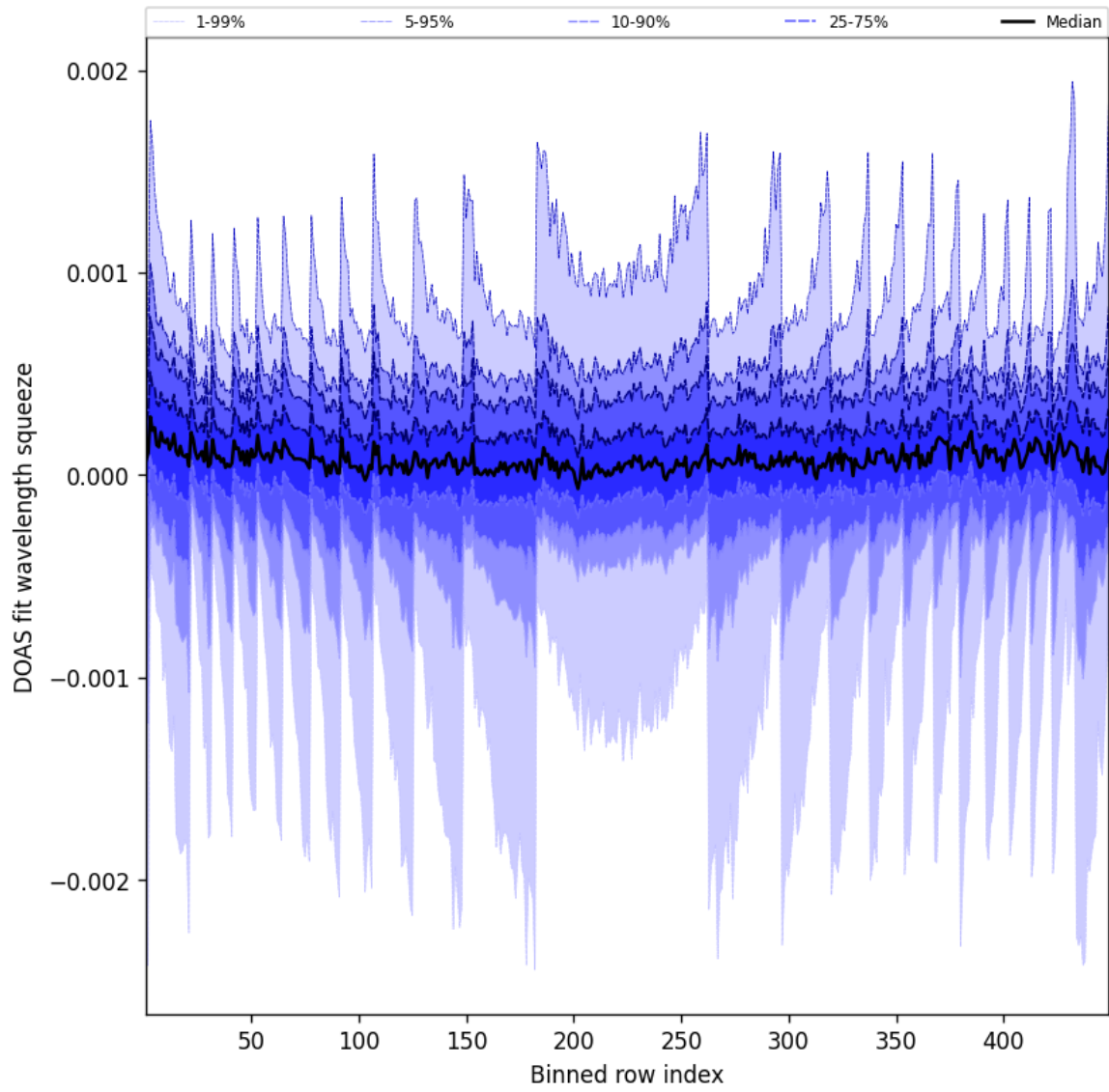
Figure 48: Along track statistics of “DOAS fit wavelength squeeze” for 2025-07-06 to 2025-07-06
