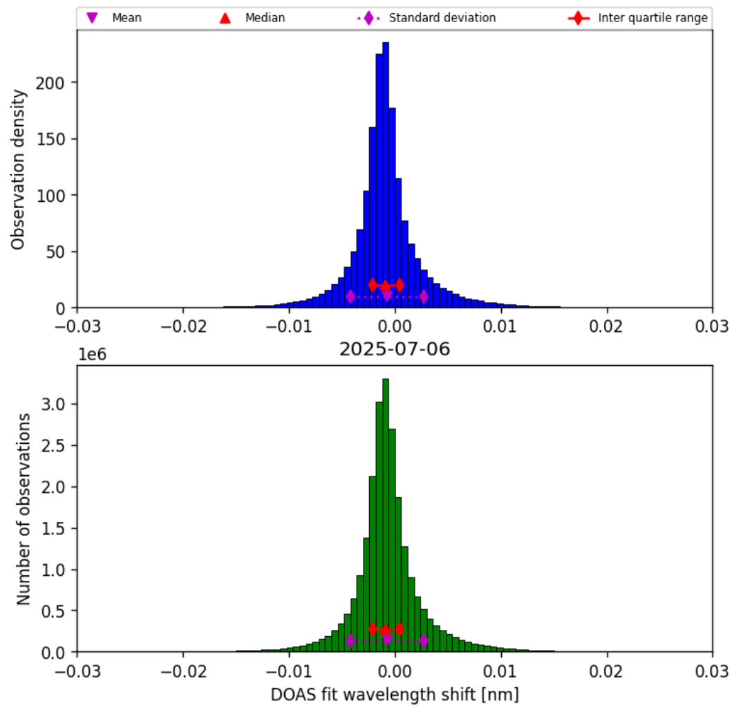
Figure 35: Histogram of “DOAS fit wavelength shift” for 2025-07-06 to 2025-07-06
