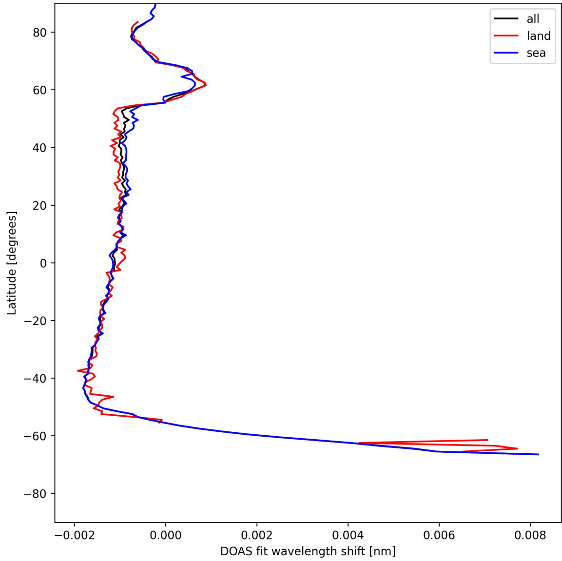
Figure 23: Zonal average of “DOAS fit wavelength shift” for 2025-07-06 to 2025-07-06.
