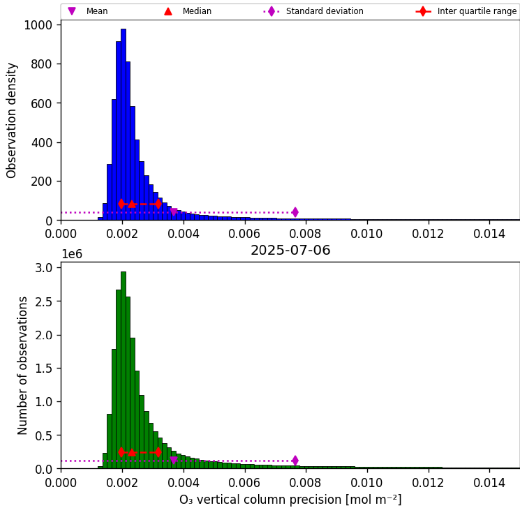
Figure 30: Histogram of “O 3 vertical column precision” for 2025-07-06 to 2025-07-06
