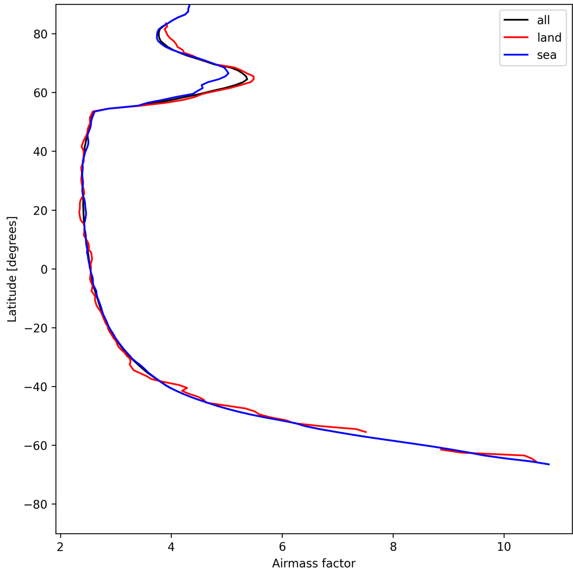
Figure 25: Zonal average of “Airmass factor” for 2025-07-06 to 2025-07-06.
