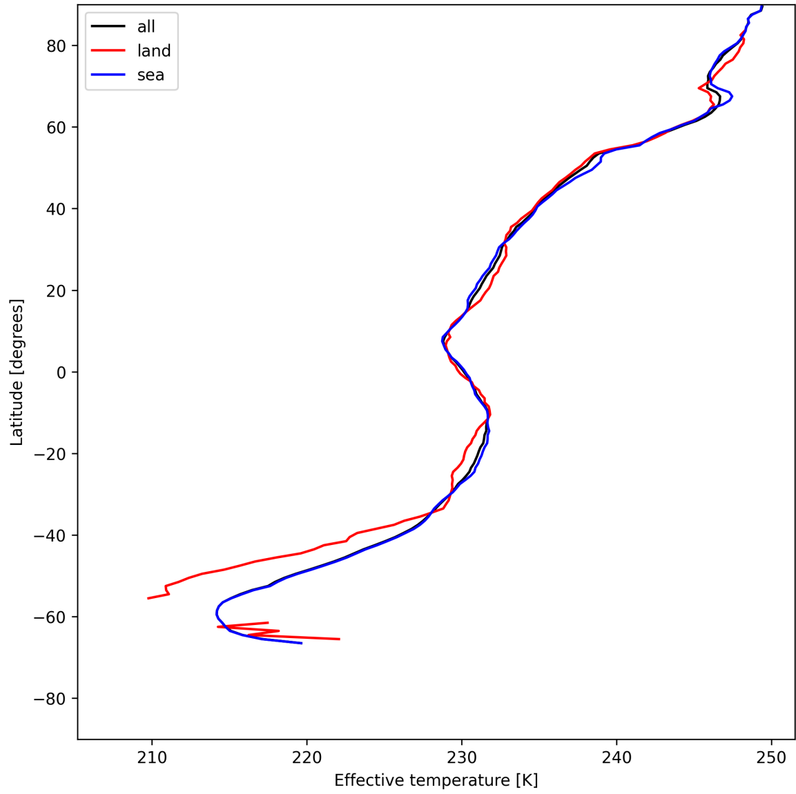
Figure 26: Zonal average of "Effective temperature" for 2025-07-06 to 2025-07-06.
