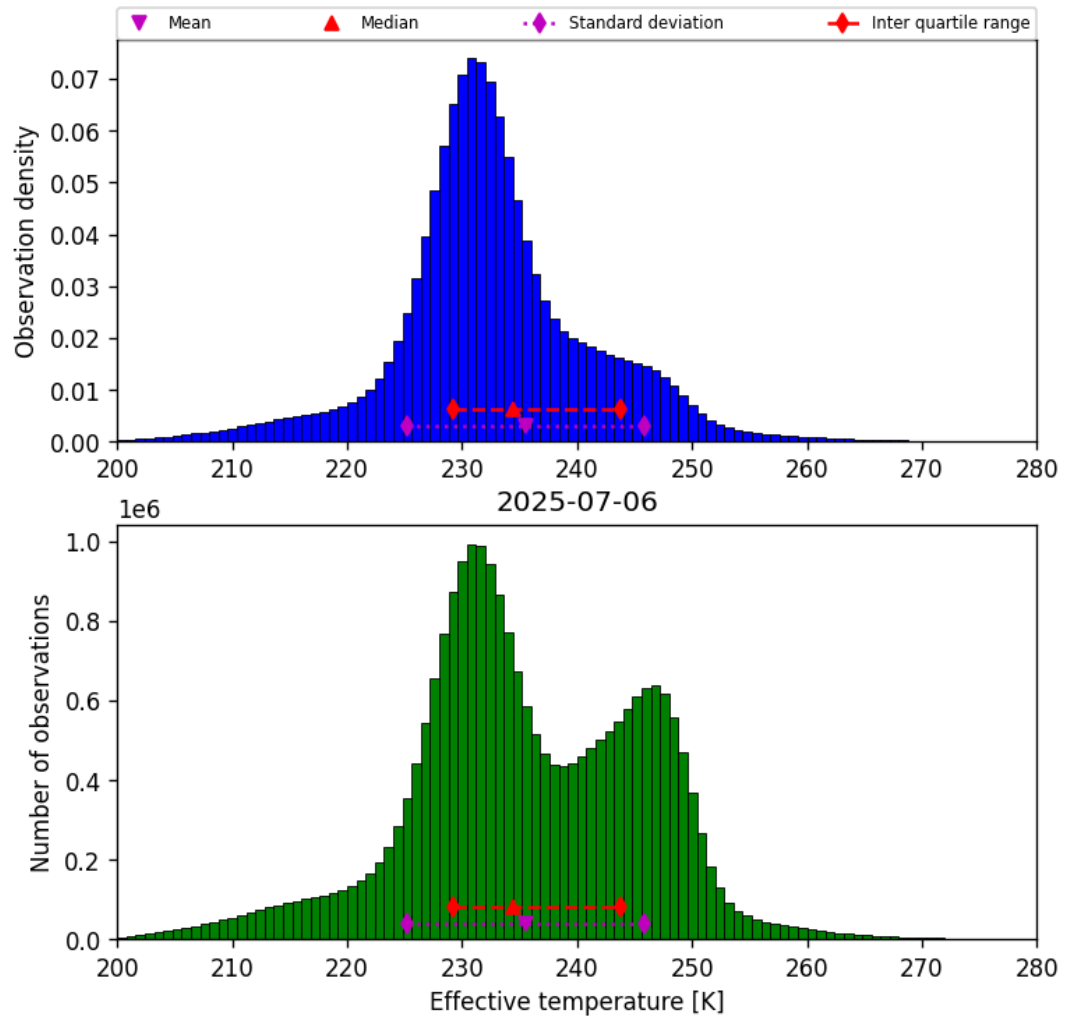
Figure 38: Histogram of “Effective temperature” for 2025-07-06 to 2025-07-06
