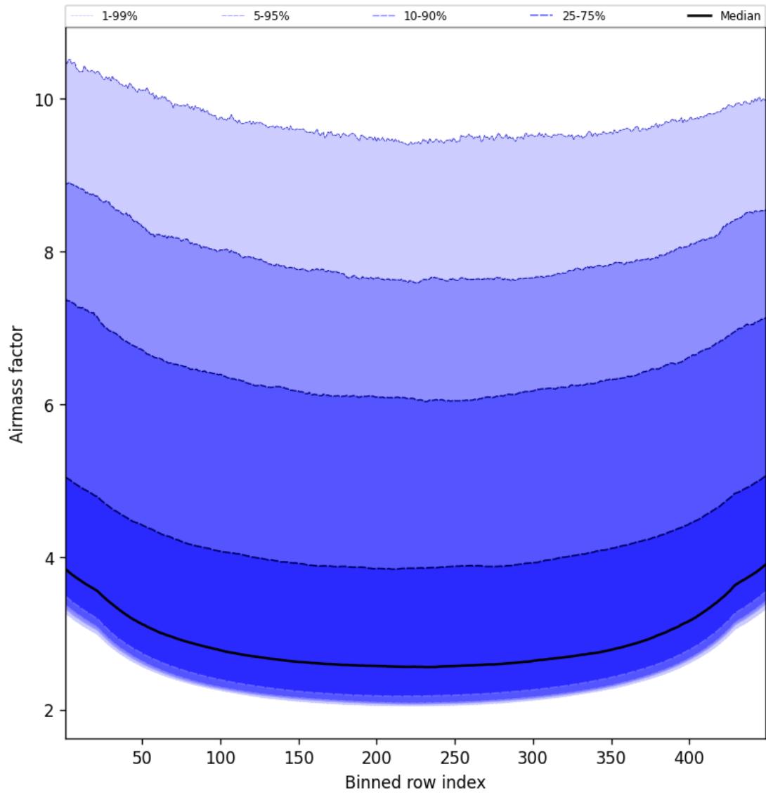
Figure 49: Along track statistics of “Airmass factor” for 2025-07-06 to 2025-07-06
