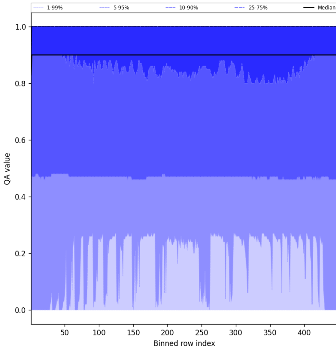
Figure 40: Along track statistics of “QA value” for 2025-07-06 to 2025-07-06
