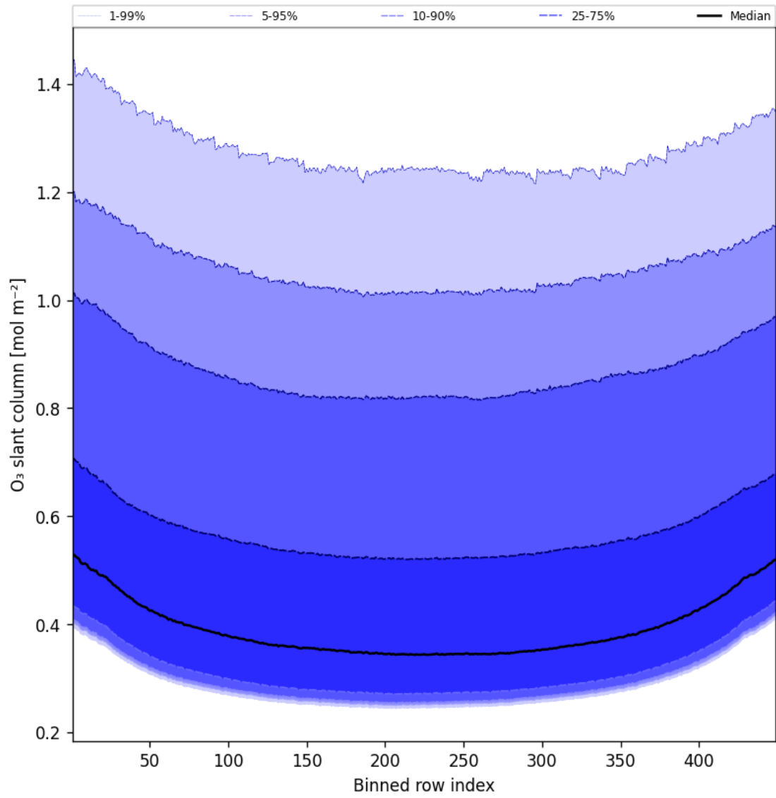
Figure 43: Along track statistics of “O 3 slant column” for 2025-07-06 to 2025-07-06
