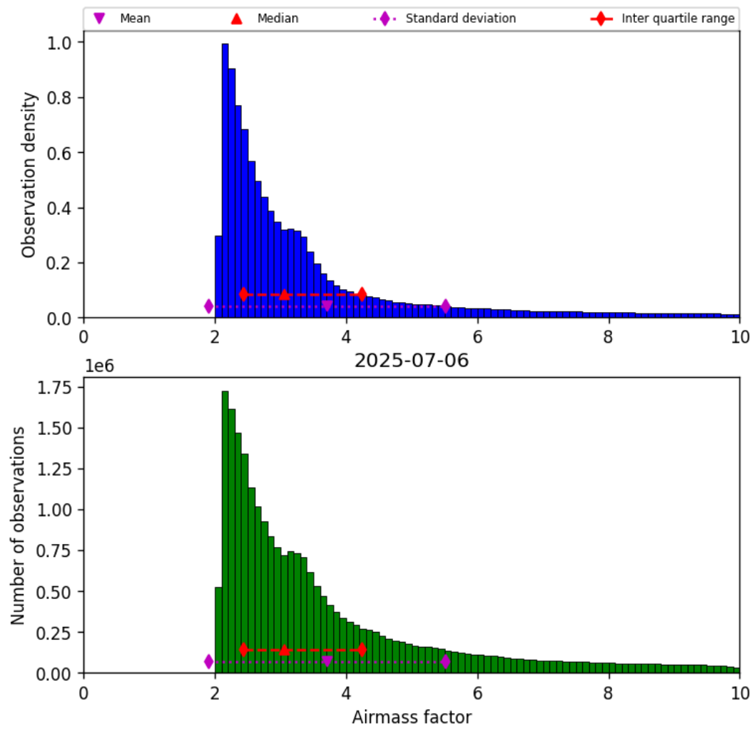
Figure 37: Histogram of “Airmass factor” for 2025-07-06 to 2025-07-06
