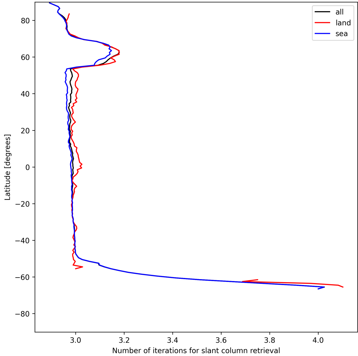
Figure 21: Zonal average of “Number of iterations for slant column retrieval” for 2025-07-06 to 2025-07-06.
