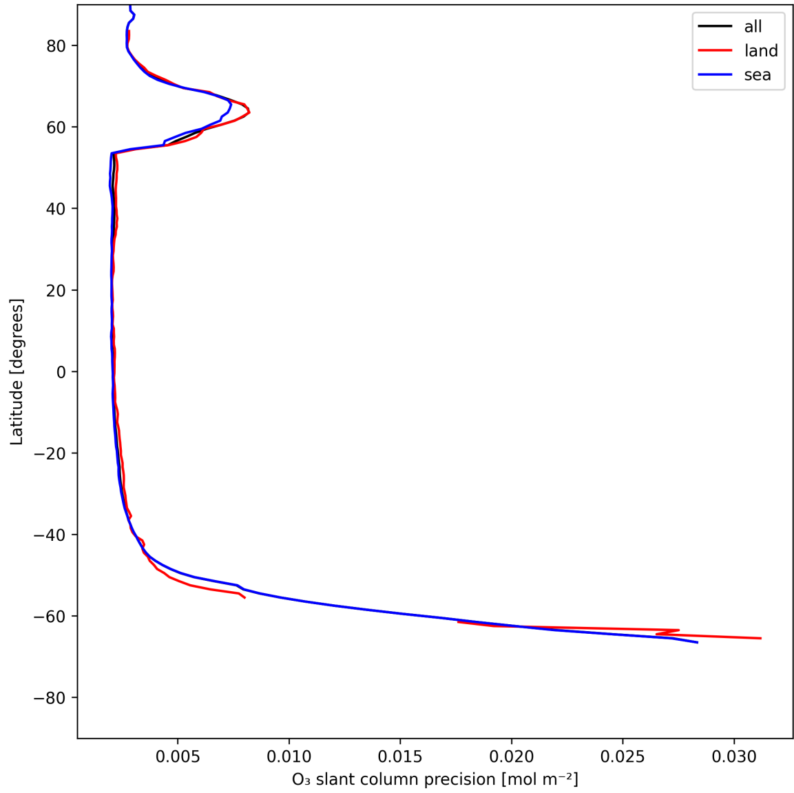
Figure 20: Zonal average of “O 3 slant column precision” for 2025-07-06 to 2025-07-06.
