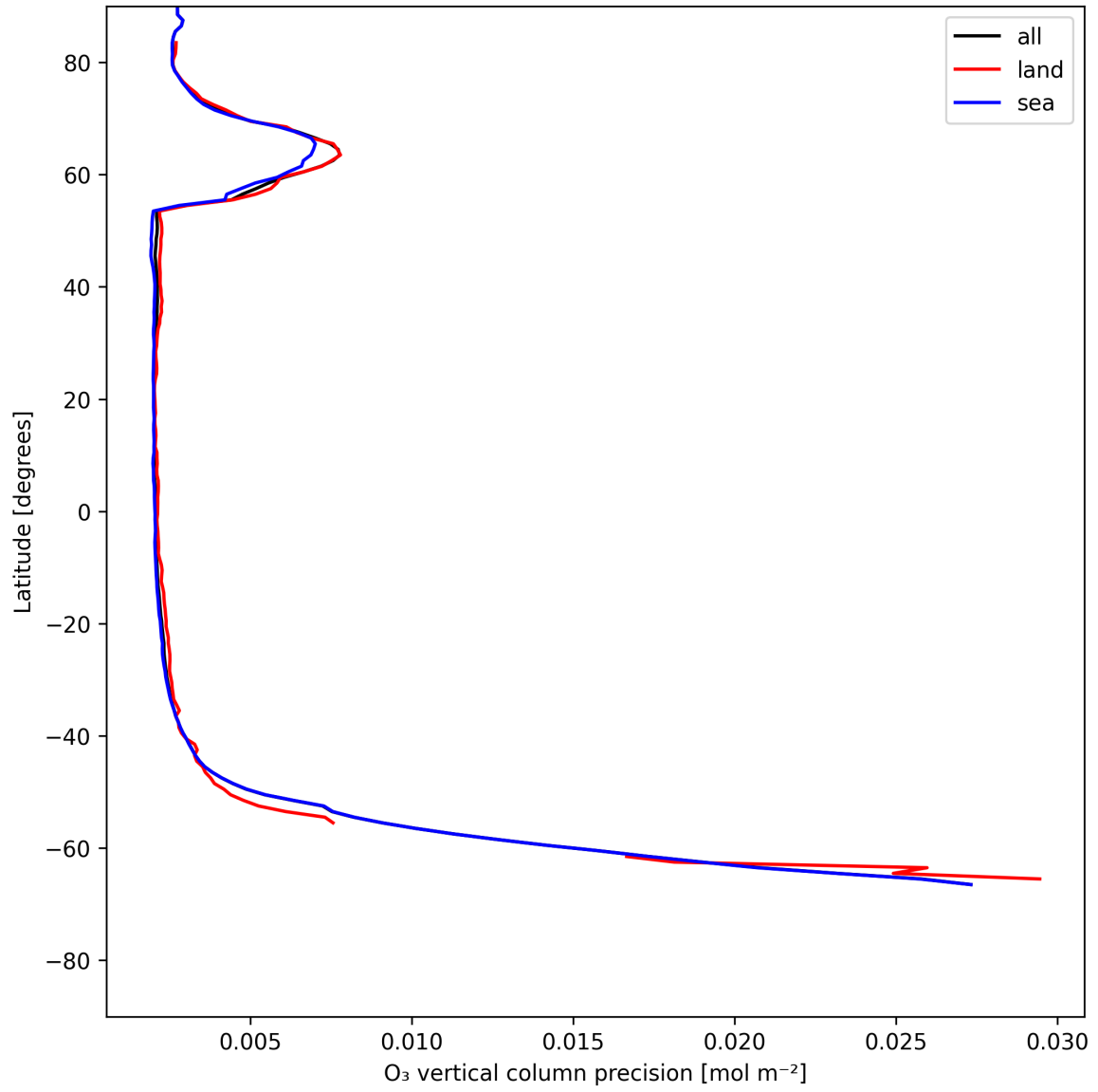
Figure 18: Zonal average of “O 3 vertical column precision” for 2025-07-06 to 2025-07-06.
