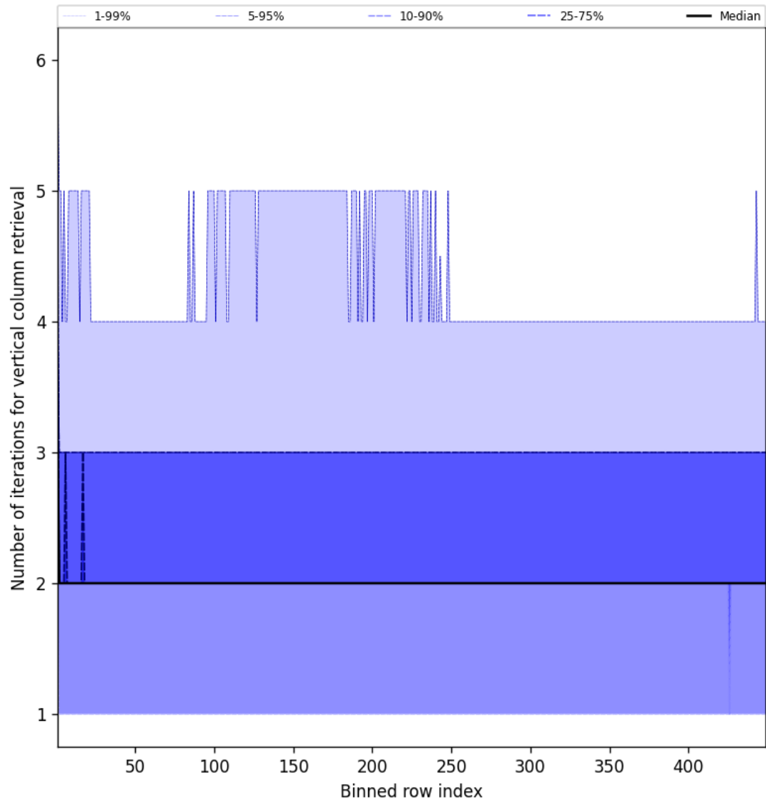
Figure 51: Along track statistics of “Number of iterations for vertical column retrieval” for 2025-07-06 to 2025-07-06
