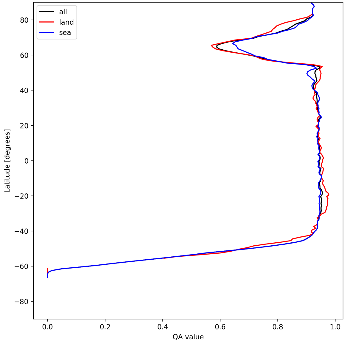
Figure 16: Zonal average of “QA value” for 2025-07-06 to 2025-07-06.
