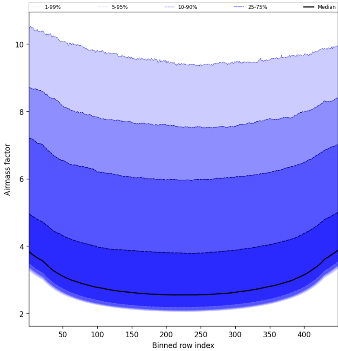
Figure 49: Along track statistics of “Airmass factor” for 2025-07-08 to 2025-07-09
