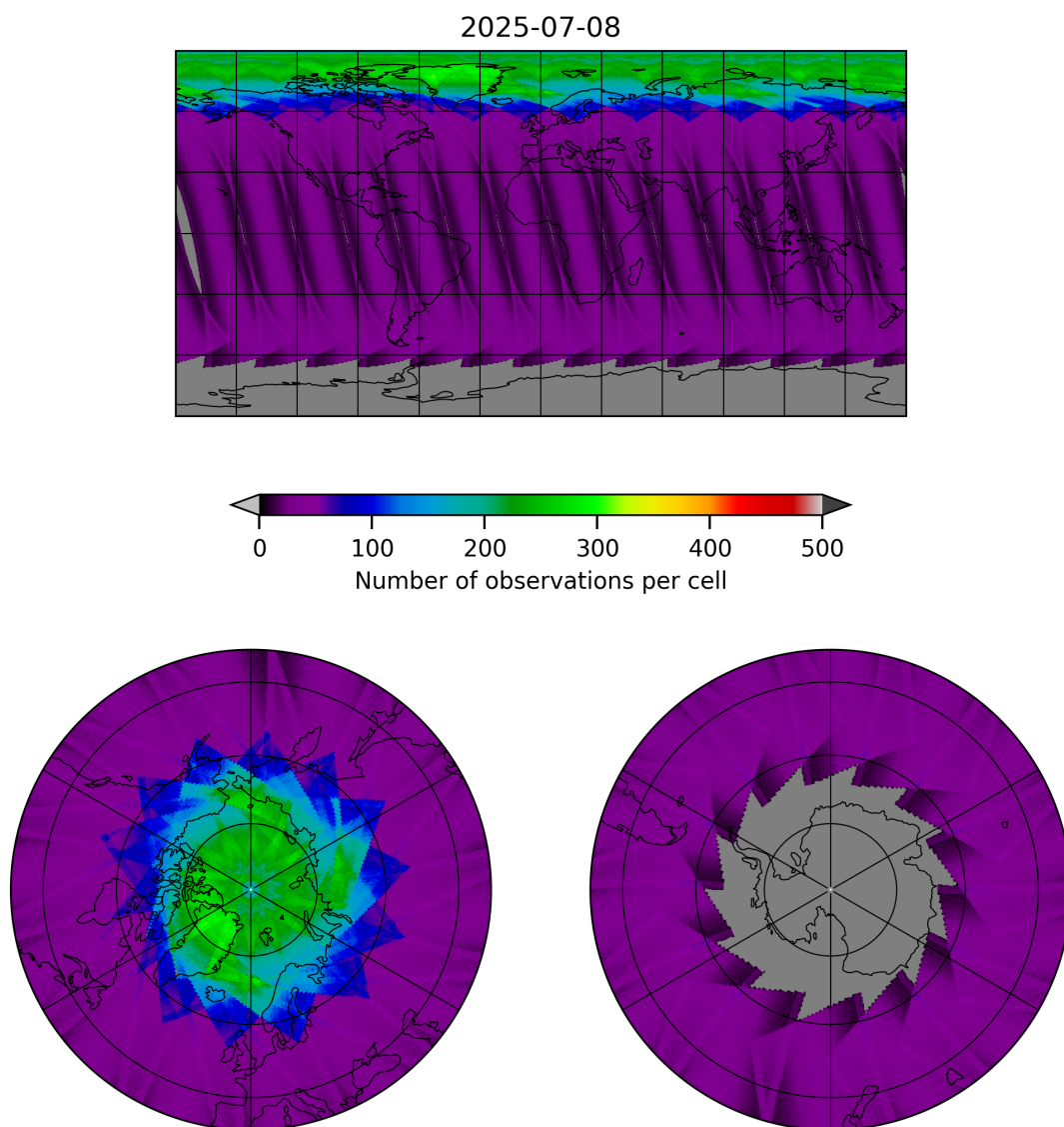
Figure 15: Map of the number of observations for 2025-07-08 to 2025-07-09
