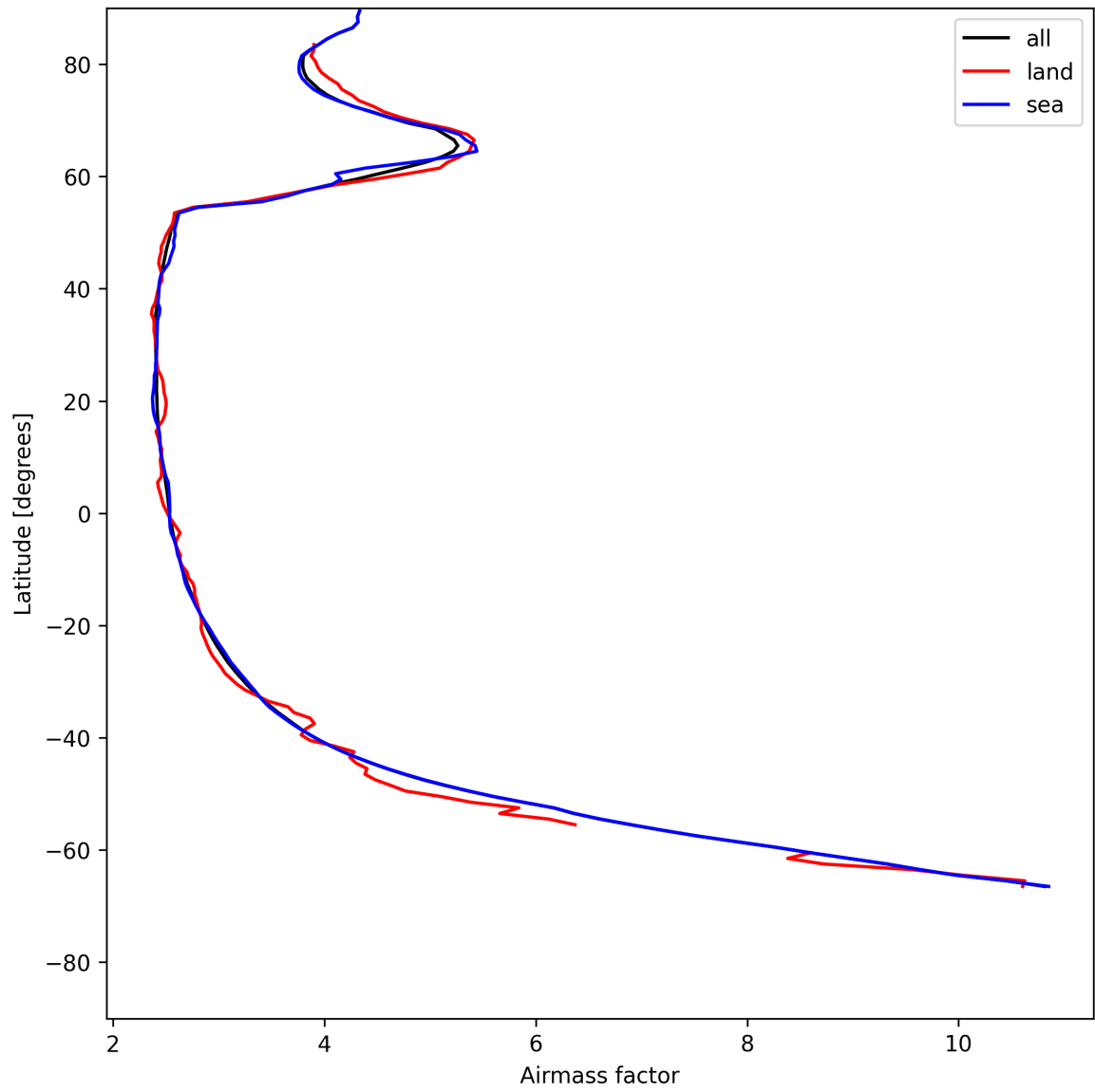
Figure 25: Zonal average of “Airmass factor” for 2025-07-08 to 2025-07-09.
