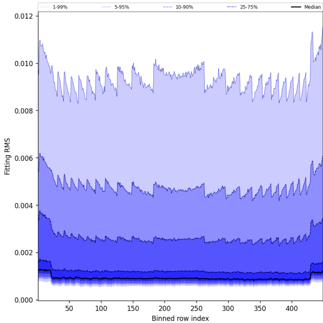
Figure 46: Along track statistics of “Fitting RMS” for 2025-07-08 to 2025-07-09
