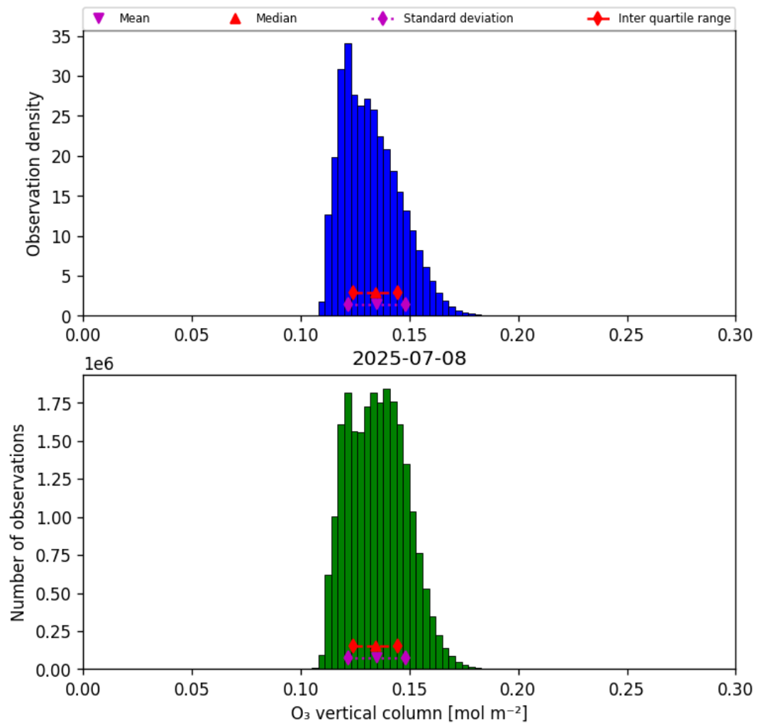
Figure 29: Histogram of “O 3 vertical column” for 2025-07-08 to 2025-07-09
