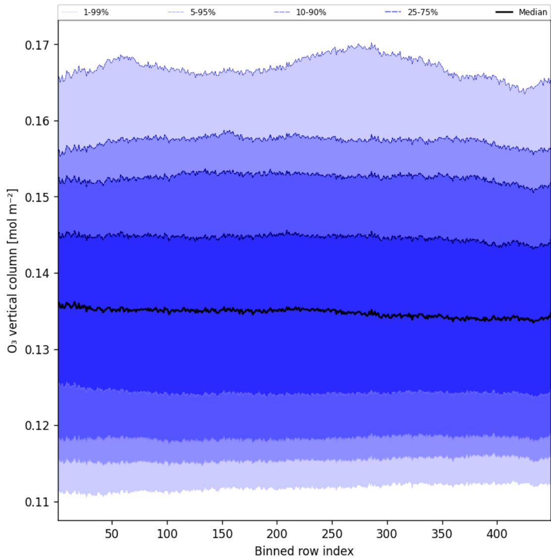
Figure 41: Along track statistics of “O 3 vertical column” for 2025-07-08 to 2025-07-09
