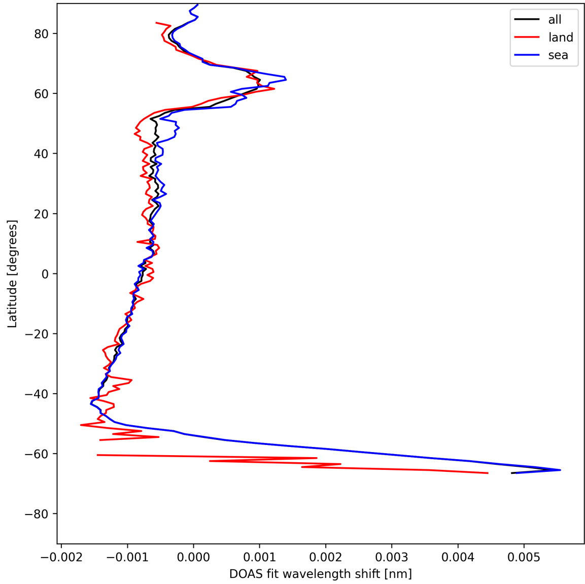
Figure 23: Zonal average of “DOAS fit wavelength shift” for 2025-07-08 to 2025-07-09.
