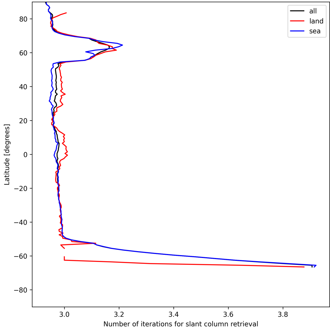
Figure 21: Zonal average of “Number of iterations for slant column retrieval” for 2025-07-08 to 2025-07-09.
