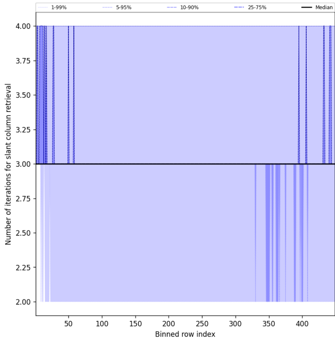
Figure 45: Along track statistics of “Number of iterations for slant column retrieval” for 2025-07-08 to 2025-07-09
