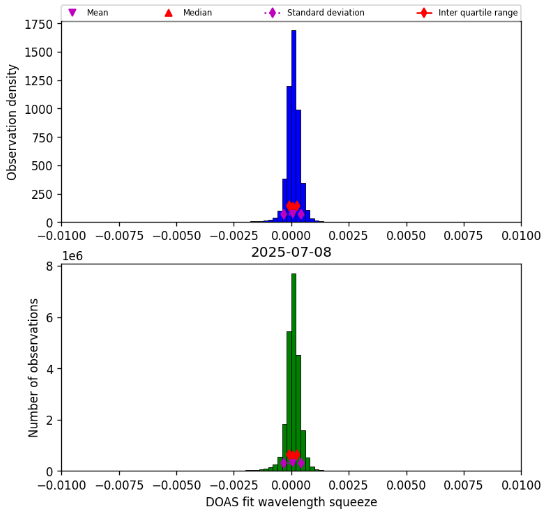
Figure 36: Histogram of “DOAS fit wavelength squeeze” for 2025-07-08 to 2025-07-09
