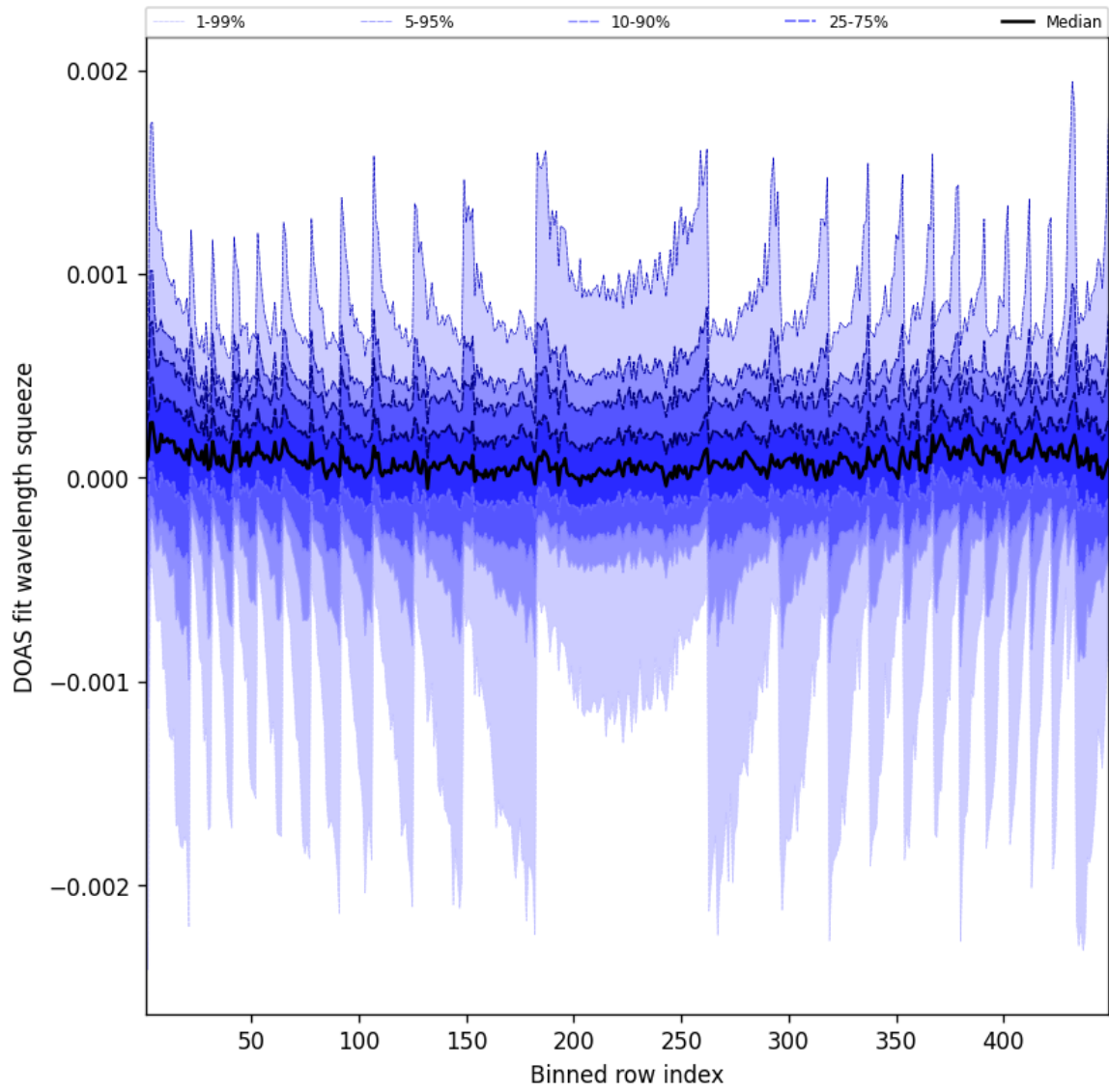
Figure 48: Along track statistics of “DOAS fit wavelength squeeze” for 2025-07-08 to 2025-07-09
