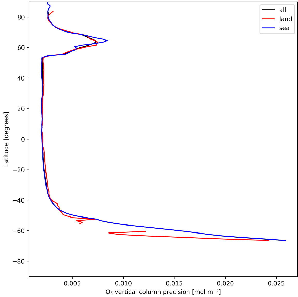
Figure 18: Zonal average of “O 3 vertical column precision” for 2025-07-08 to 2025-07-09.
