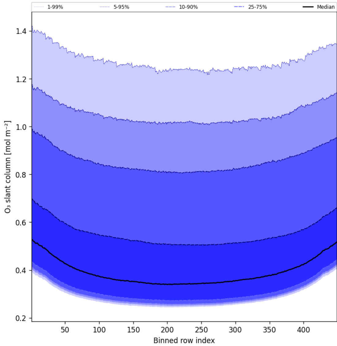
Figure 43: Along track statistics of “O 3 slant column” for 2025-07-08 to 2025-07-09
