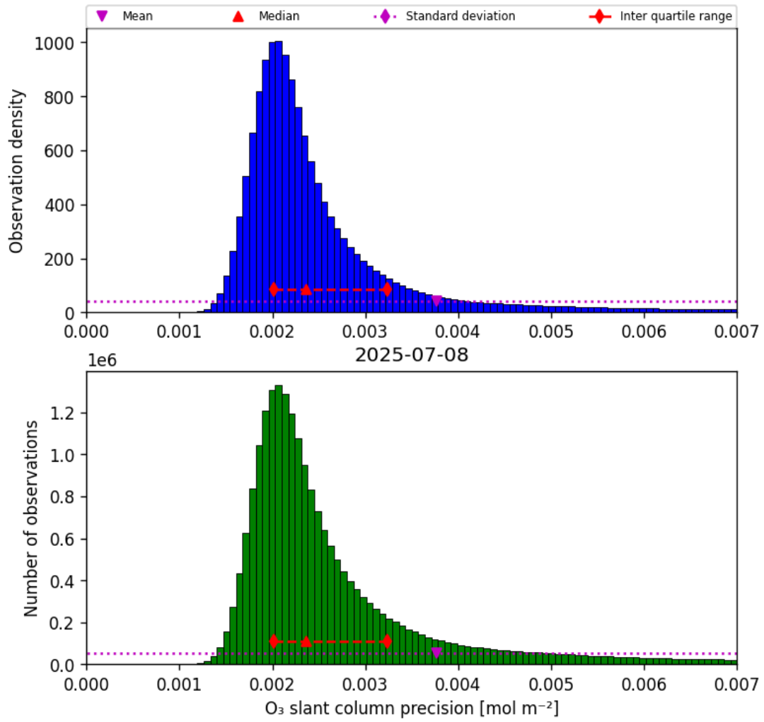
Figure 32: Histogram of “O 3 slant column precision” for 2025-07-08 to 2025-07-09
