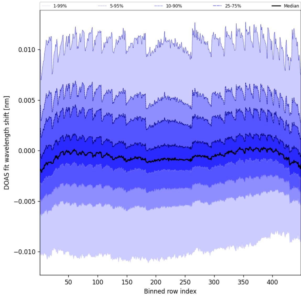
Figure 47: Along track statistics of “DOAS fit wavelength shift” for 2025-07-08 to 2025-07-09
