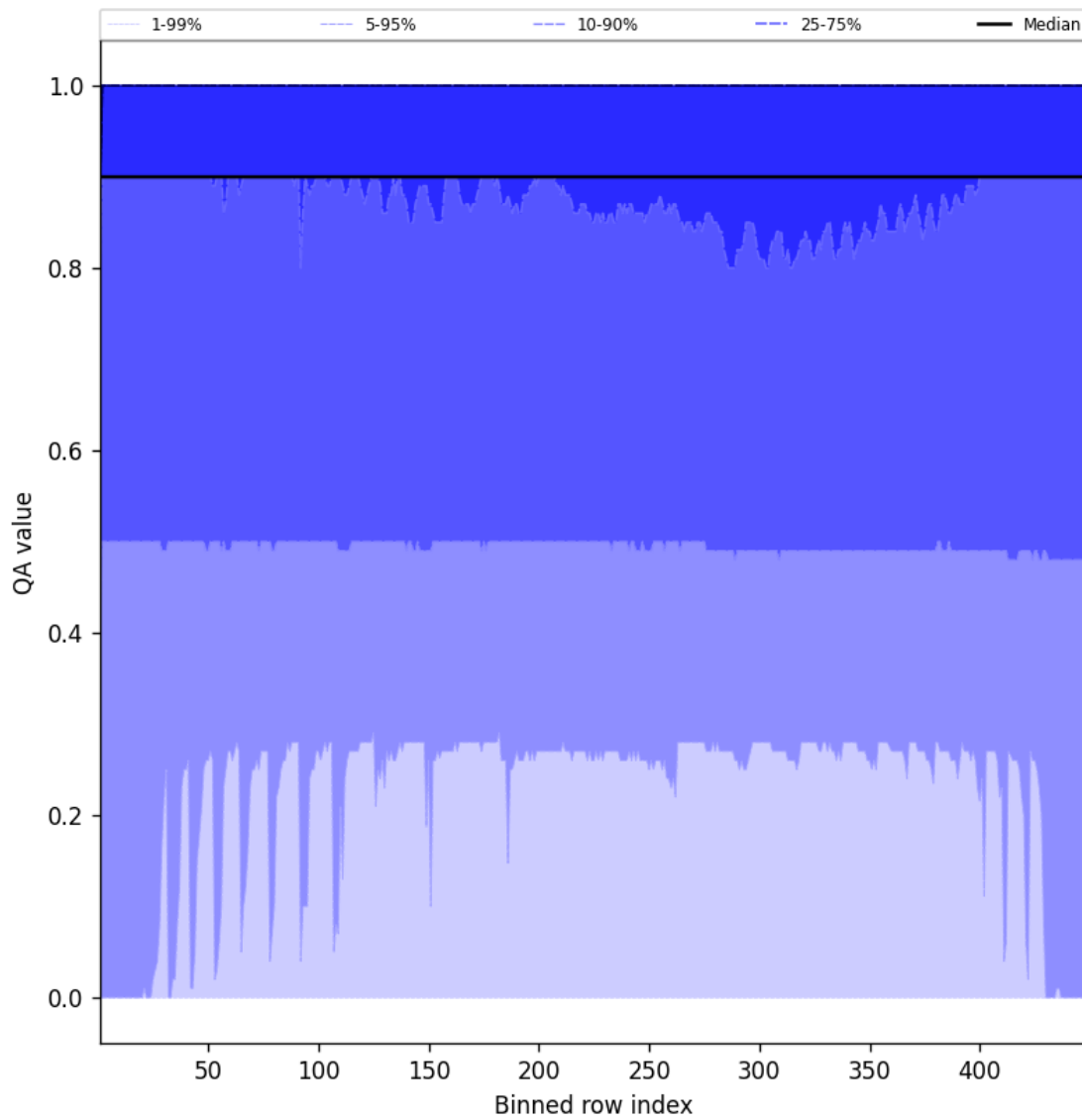
Figure 40: Along track statistics of “QA value” for 2025-07-08 to 2025-07-09
