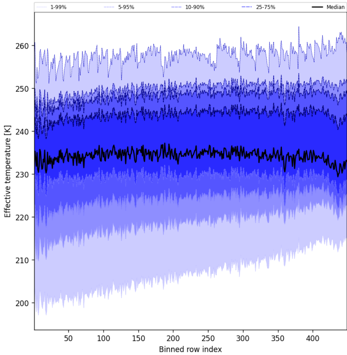
Figure 50: Along track statistics of “Effective temperature” for 2025-07-08 to 2025-07-09
