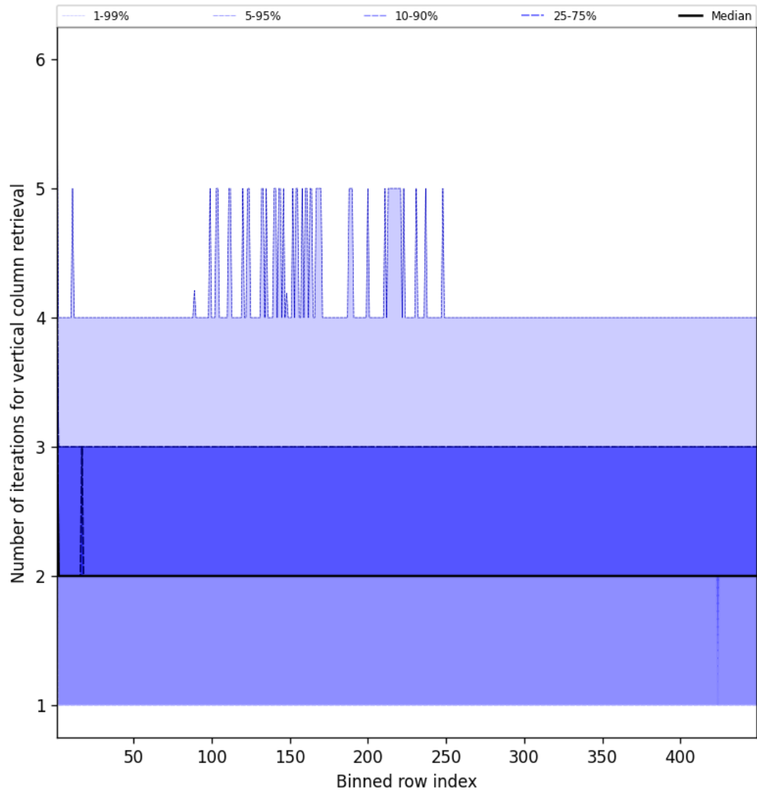
Figure 51: Along track statistics of “Number of iterations for vertical column retrieval” for 2025-07-08 to 2025-07-09
