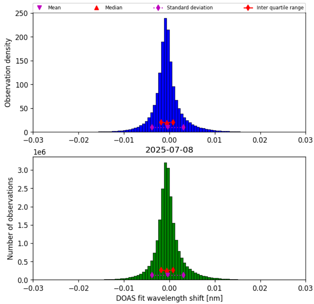
Figure 35: Histogram of “DOAS fit wavelength shift” for 2025-07-08 to 2025-07-09
