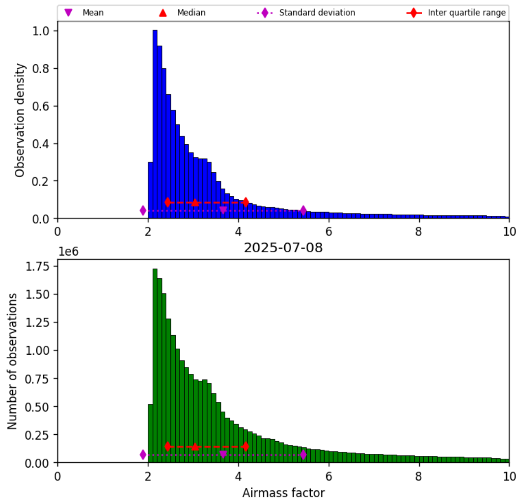
Figure 37: Histogram of “Airmass factor” for 2025-07-08 to 2025-07-09
