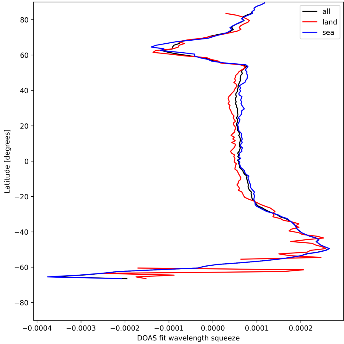
Figure 24: Zonal average of “DOAS fit wavelength squeeze” for 2025-07-08 to 2025-07-09.
