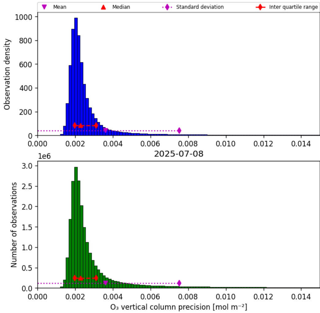
Figure 30: Histogram of "O 3 vertical column precision" for 2025-07-08 to 2025-07-09
