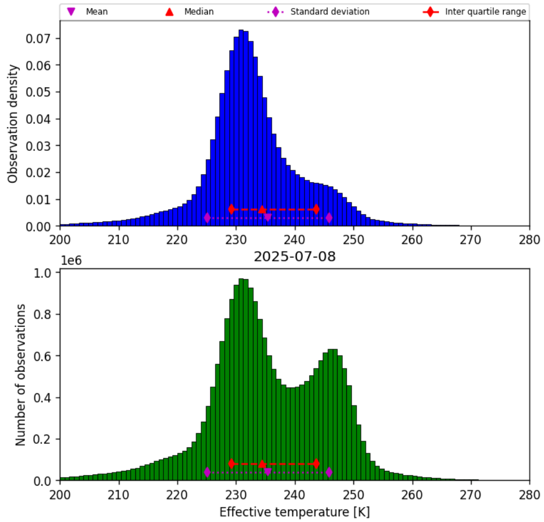
Figure 38: Histogram of “Effective temperature” for 2025-07-08 to 2025-07-09
