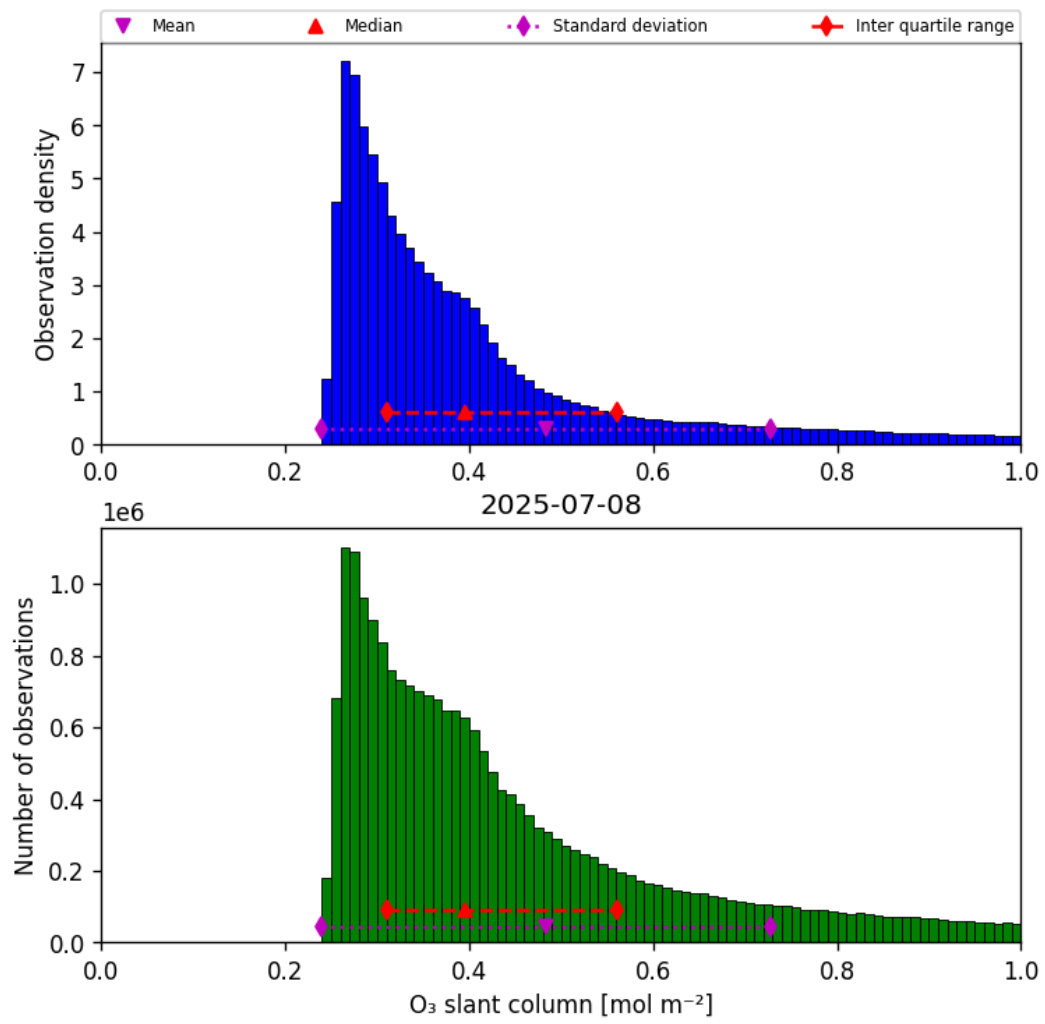
Figure 31: Histogram of “O 3 slant column” for 2025-07-08 to 2025-07-09
