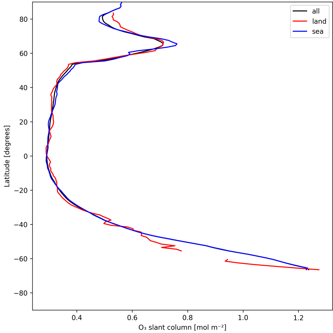
Figure 19: Zonal average of “O 3 slant column” for 2025-07-08 to 2025-07-09.
