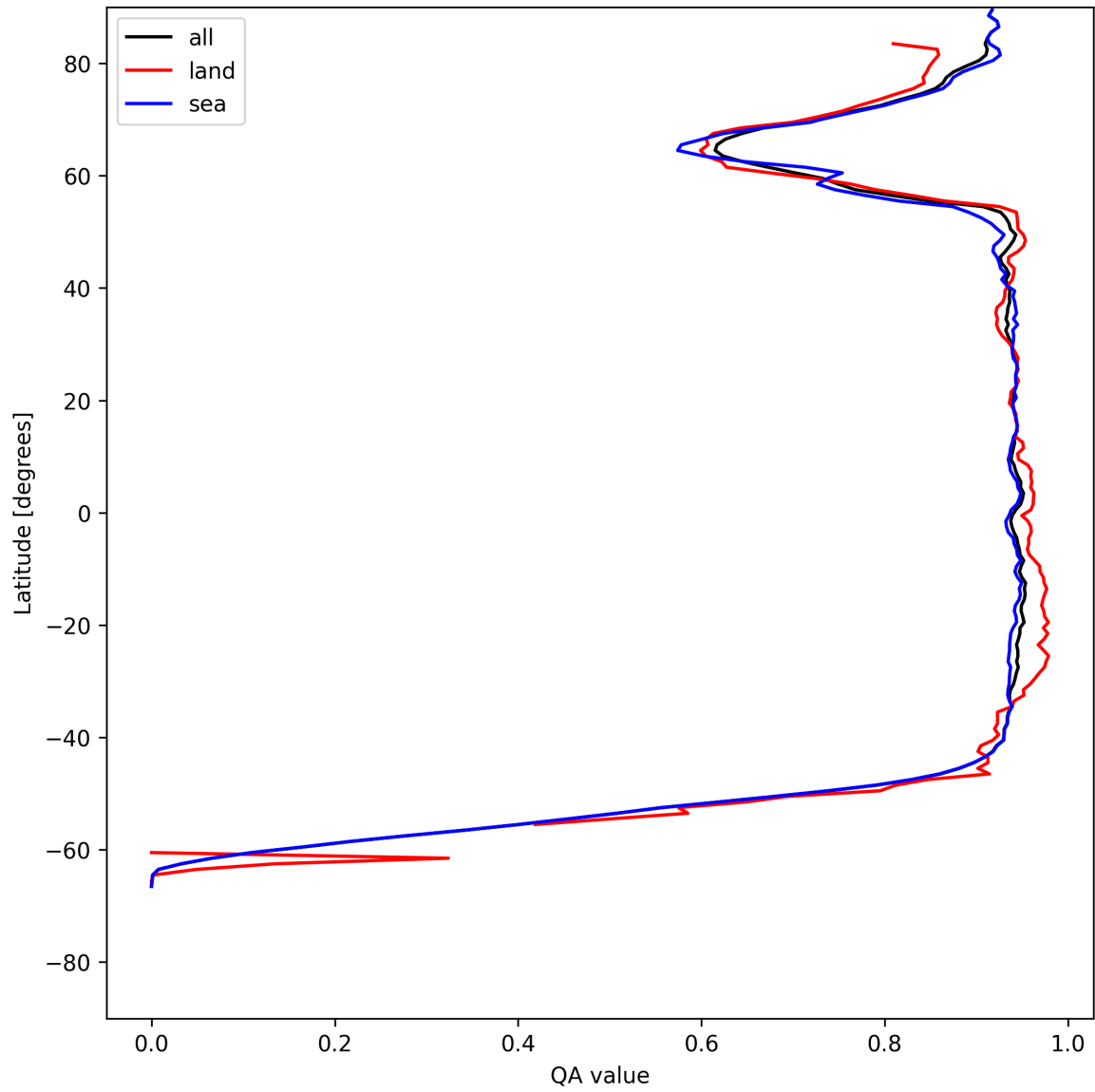
Figure 16: Zonal average of “QA value” for 2025-07-08 to 2025-07-09.
