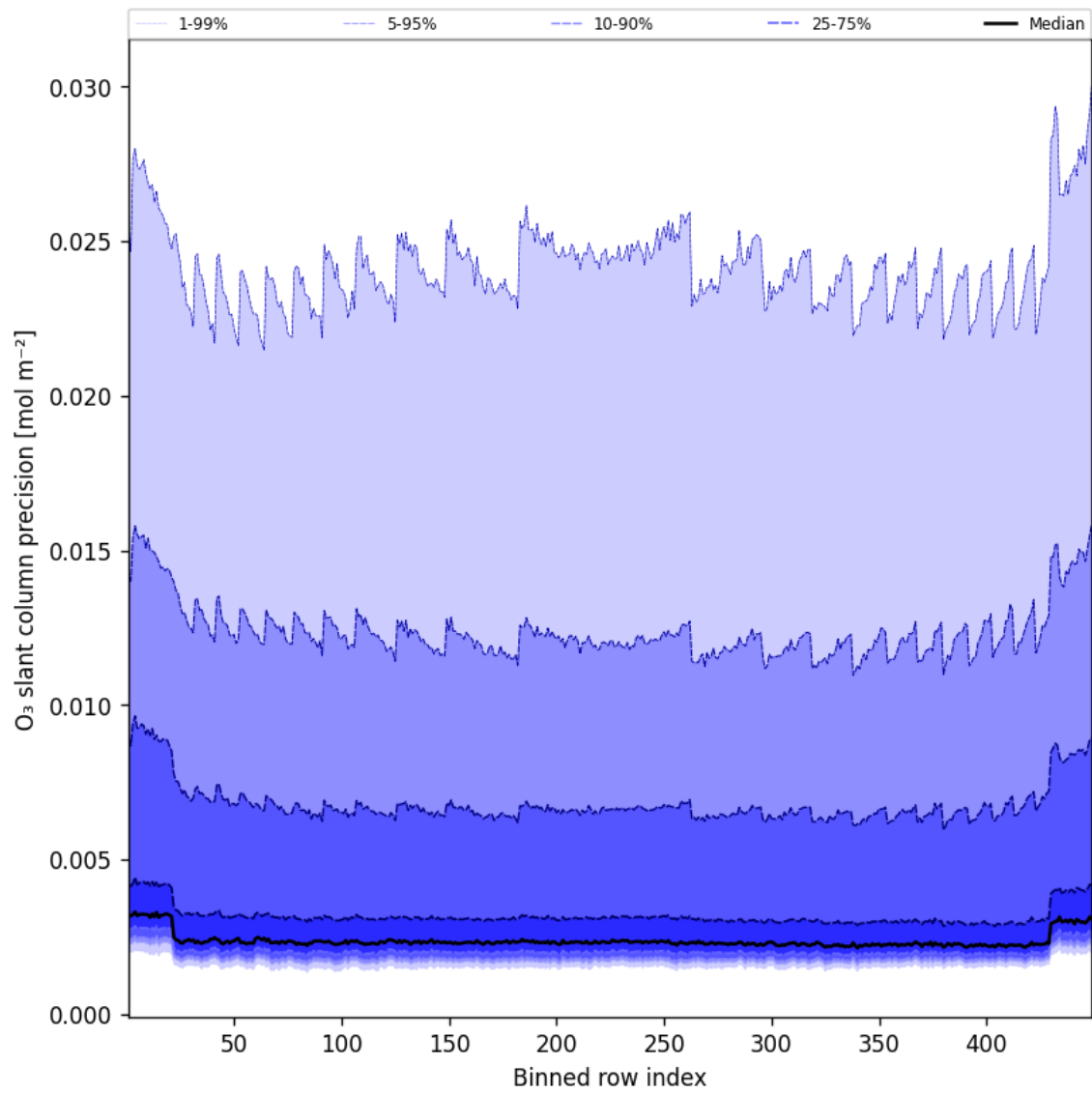
Figure 44: Along track statistics of “O 3 slant column precision” for 2025-07-08 to 2025-07-09
