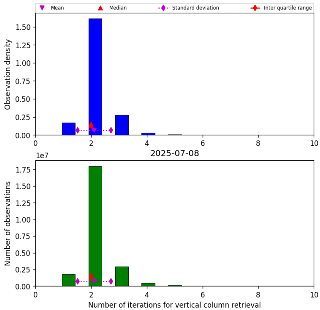
Figure 39: Histogram of “Number of iterations for vertical column retrieval” for 2025-07-08 to 2025-07-09
