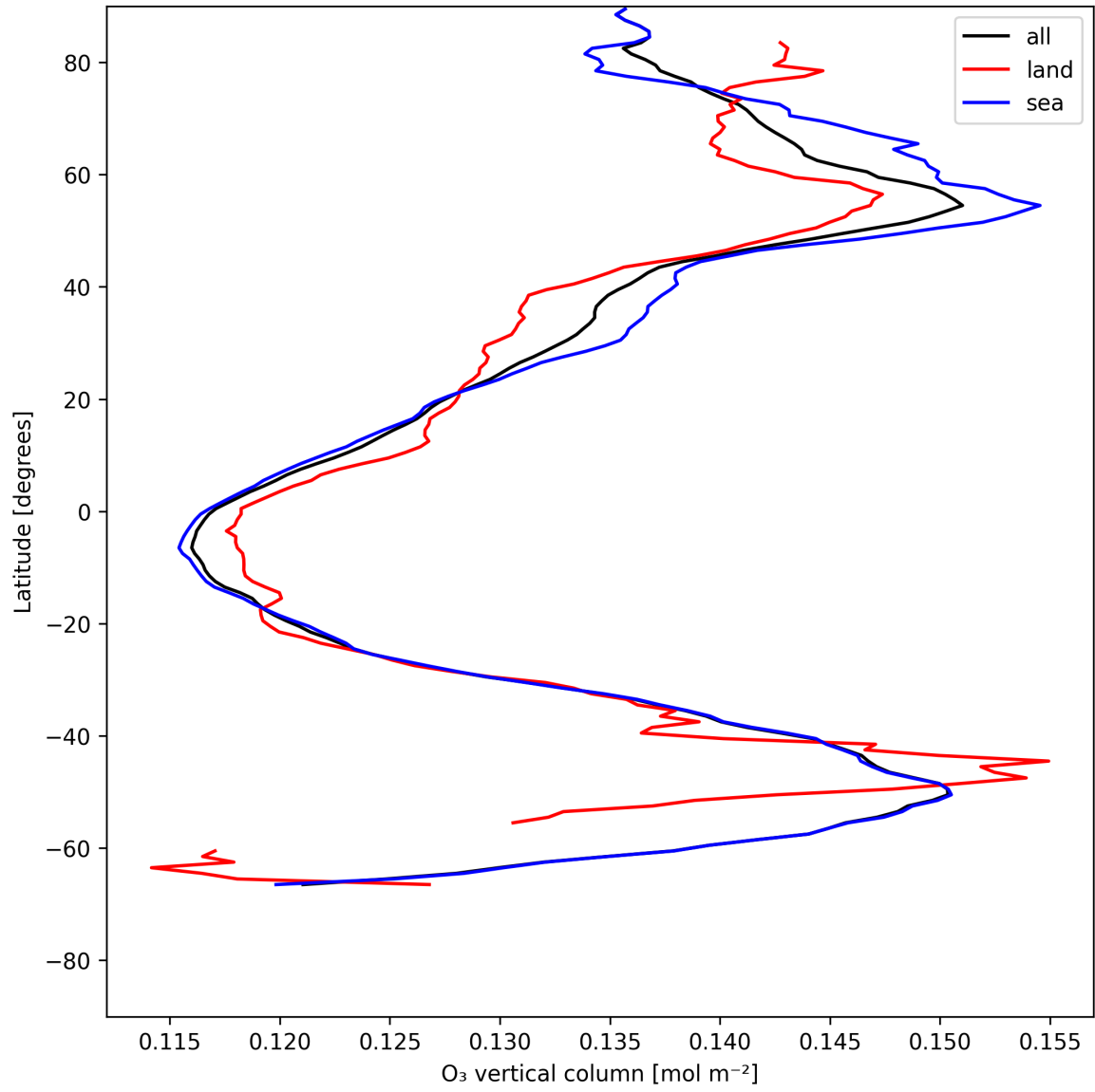
Figure 17: Zonal average of “O 3 vertical column” for 2025-07-08 to 2025-07-09.
