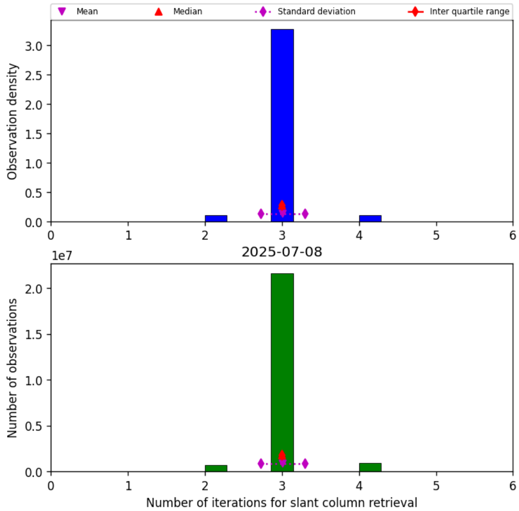
Figure 33: Histogram of “Number of iterations for slant column retrieval” for 2025-07-08 to 2025-07-09
