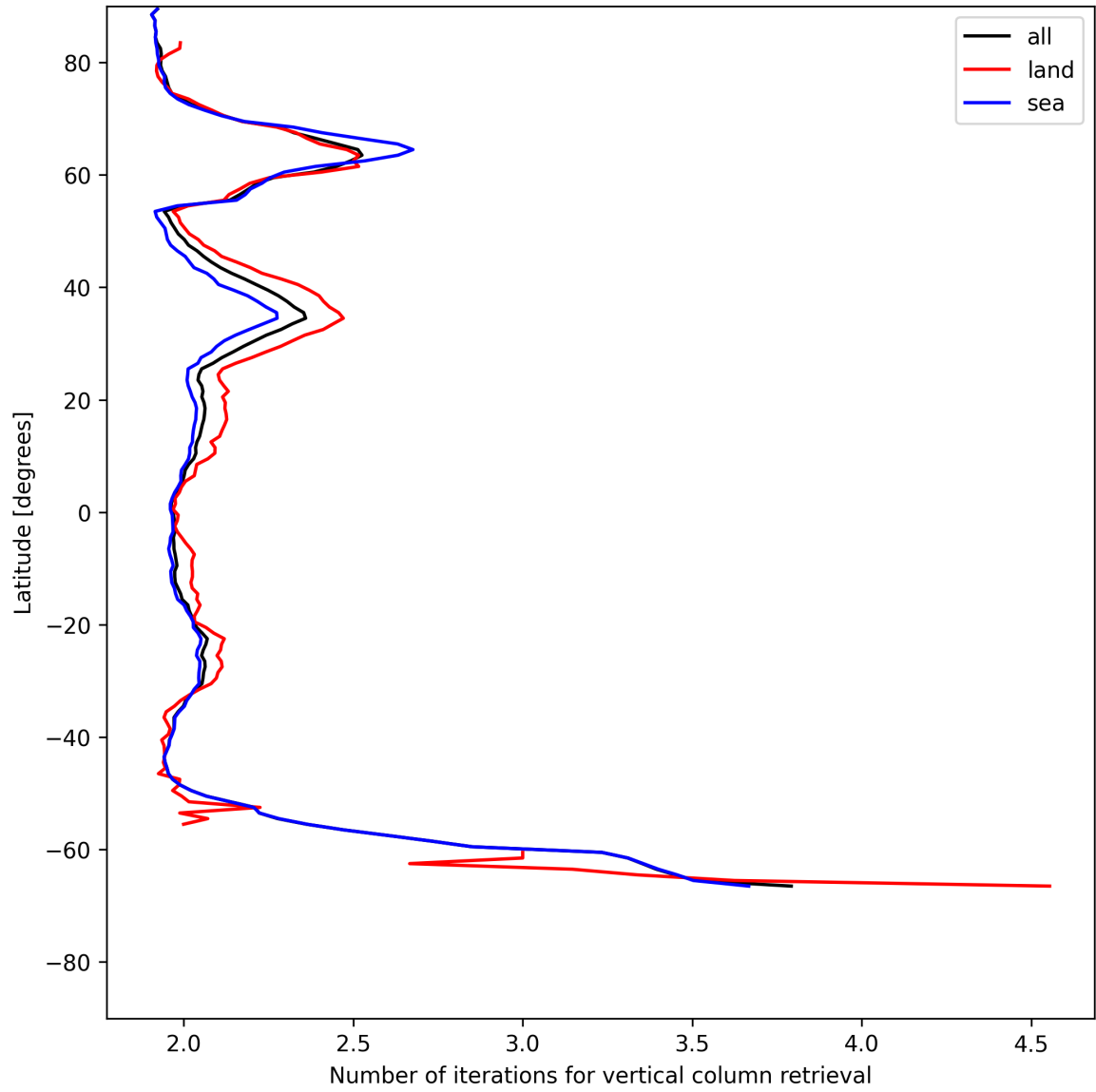
Figure 27: Zonal average of “Number of iterations for vertical column retrieval” for 2025-07-08 to 2025-07-09.
