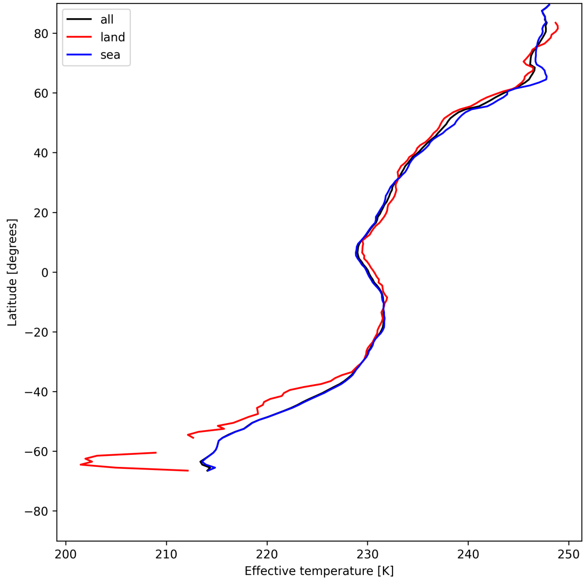
Figure 26: Zonal average of “Effective temperature” for 2025-07-08 to 2025-07-09.
