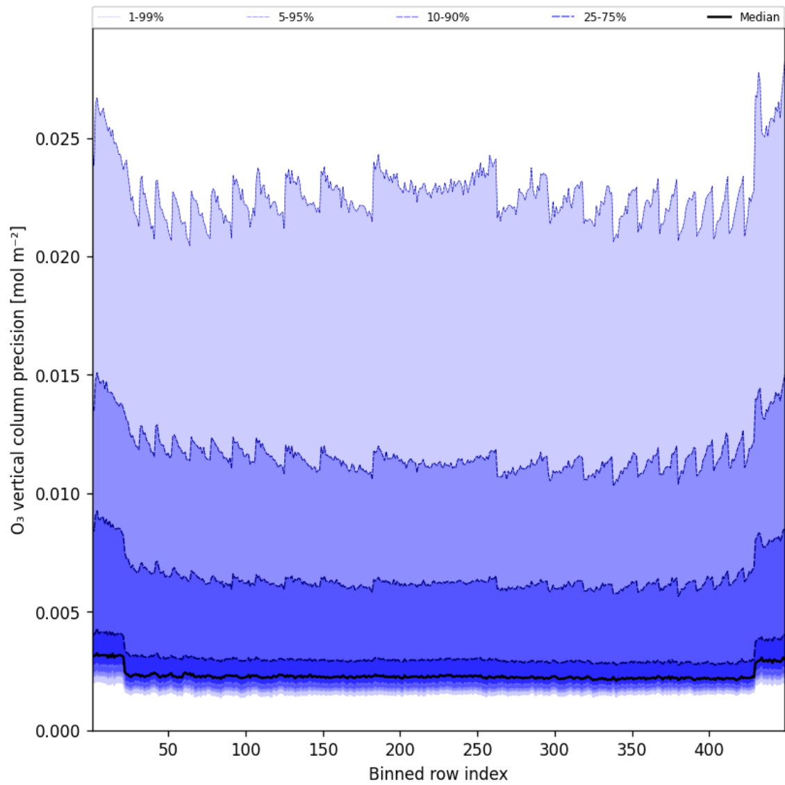
Figure 42: Along track statistics of “O 3 vertical column precision” for 2025-07-08 to 2025-07-09
