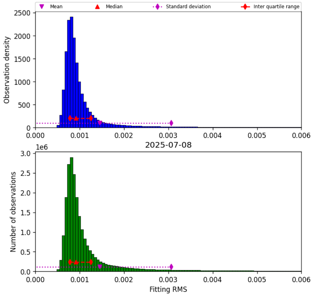
Figure 34: Histogram of “Fitting RMS” for 2025-07-08 to 2025-07-09
