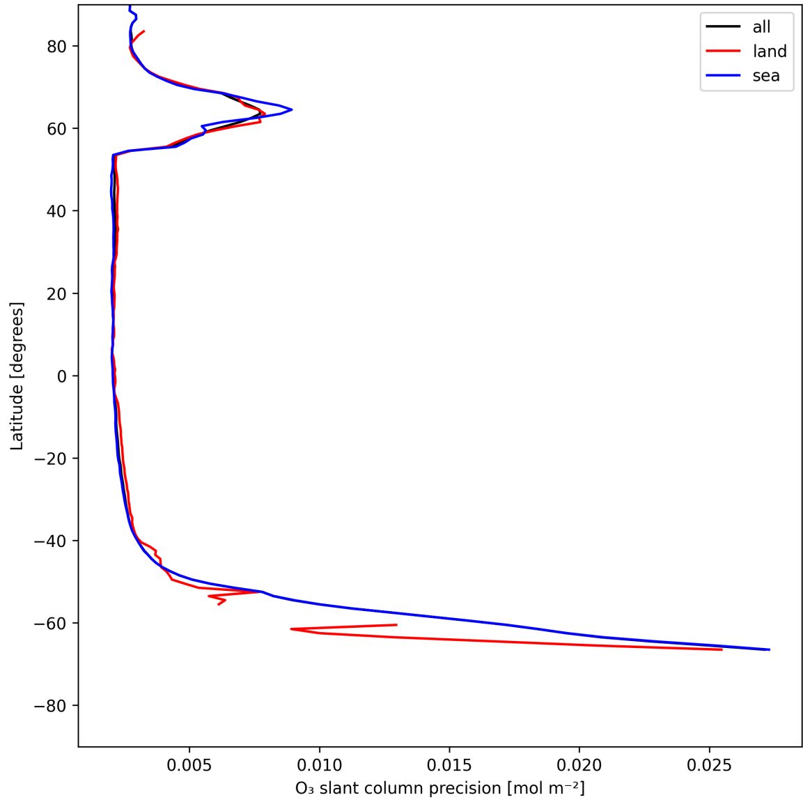
Figure 20: Zonal average of “O 3 slant column precision” for 2025-07-08 to 2025-07-09.
