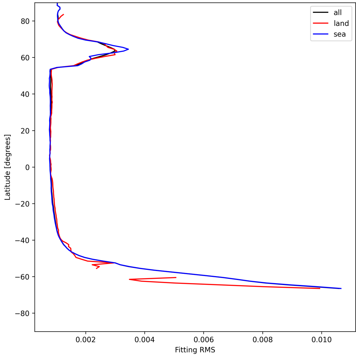
Figure 22: Zonal average of “Fitting RMS” for 2025-07-08 to 2025-07-09.
