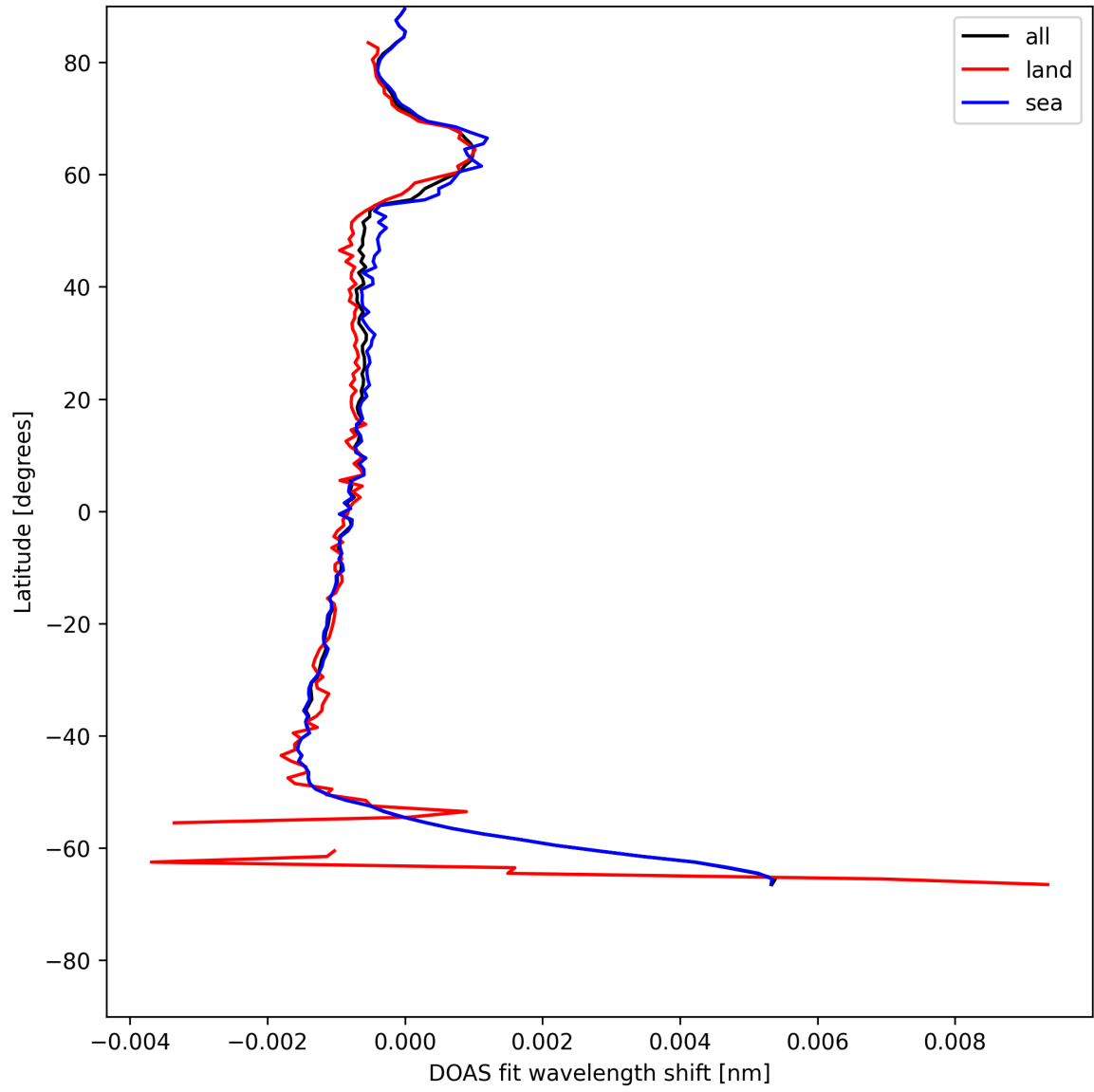
Figure 23: Zonal average of “DOAS fit wavelength shift” for 2025-07-09 to 2025-07-10.
