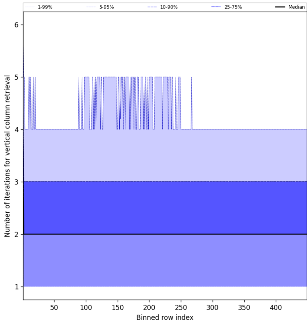
Figure 51: Along track statistics of “Number of iterations for vertical column retrieval” for 2025-07-09 to 2025-07-10
