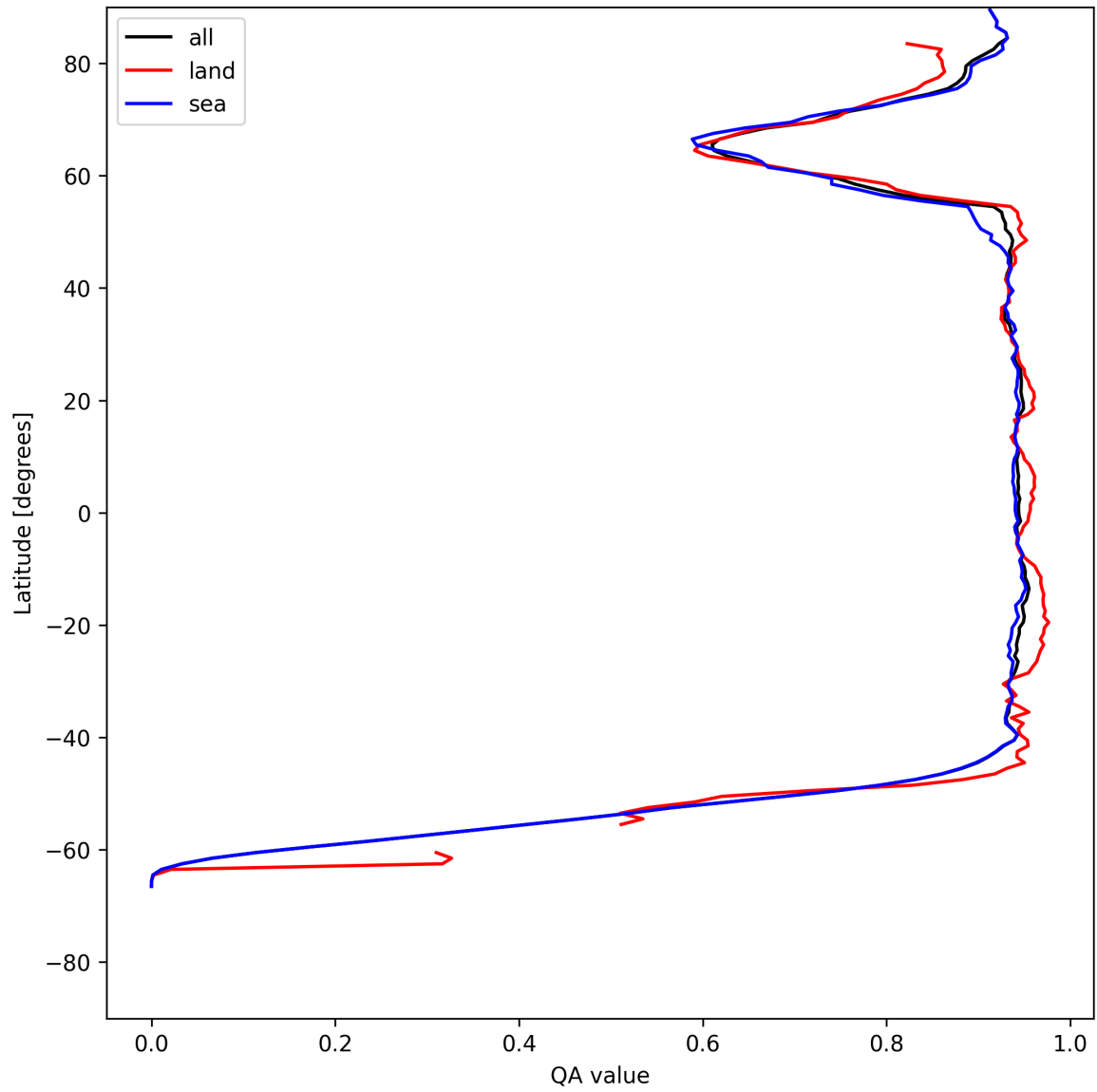
Figure 16: Zonal average of “QA value” for 2025-07-09 to 2025-07-10.
