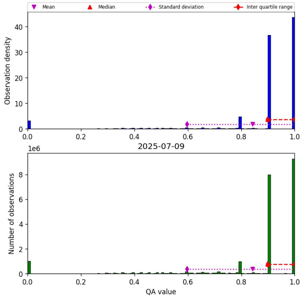
Figure 28: Histogram of “QA value” for 2025-07-09 to 2025-07-10
