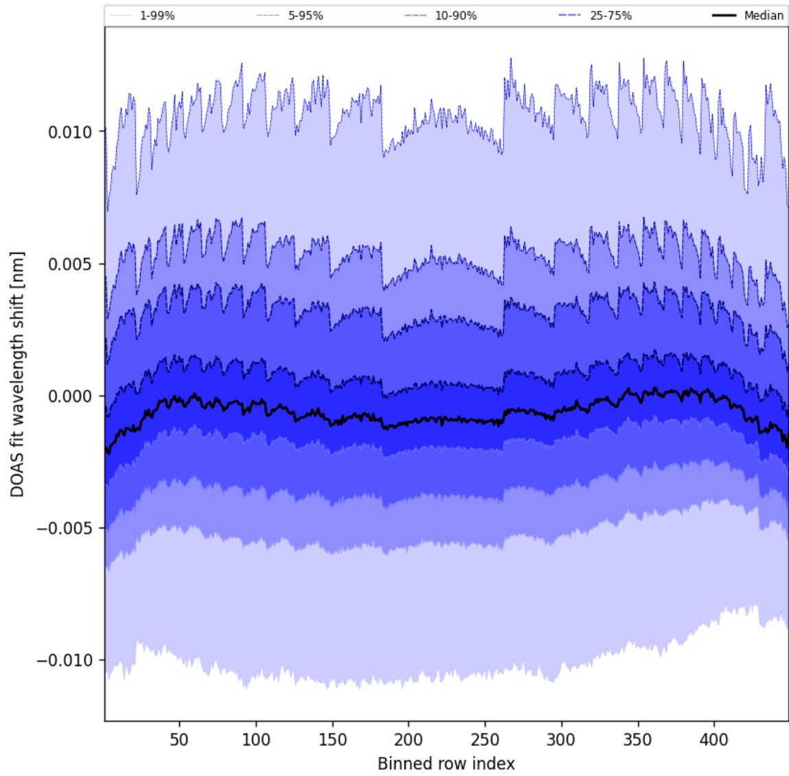
Figure 47: Along track statistics of "DOAS fit wavelength shift" for 2025-07-09 to 2025-07-10
