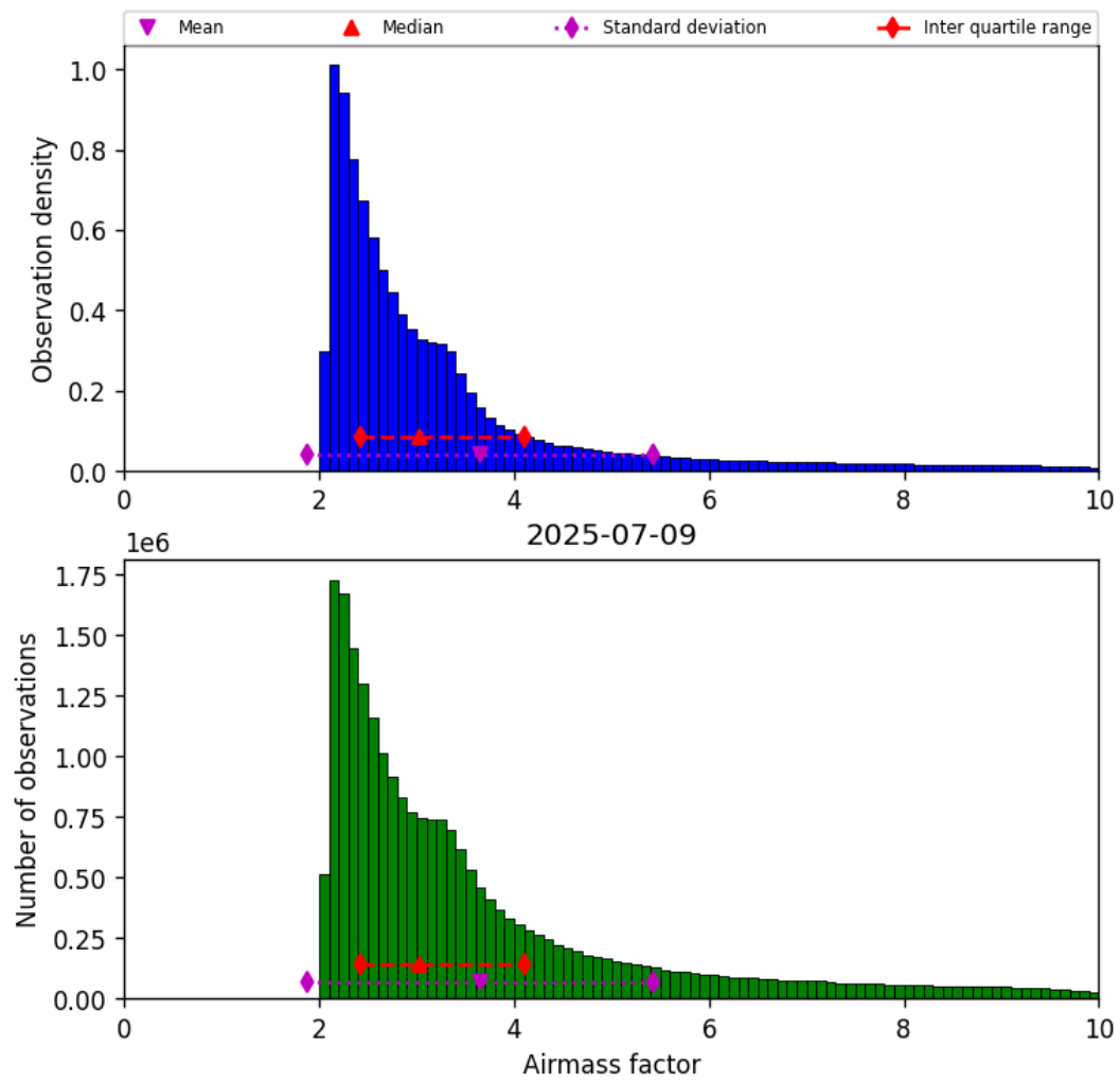
Figure 37: Histogram of “Airmass factor” for 2025-07-09 to 2025-07-10
