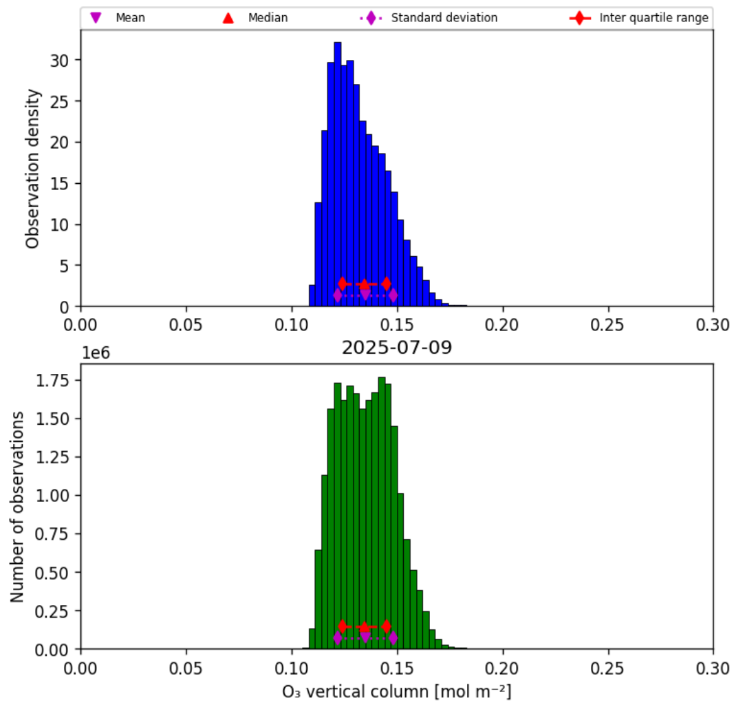
Figure 29: Histogram of “O 3 vertical column” for 2025-07-09 to 2025-07-10
