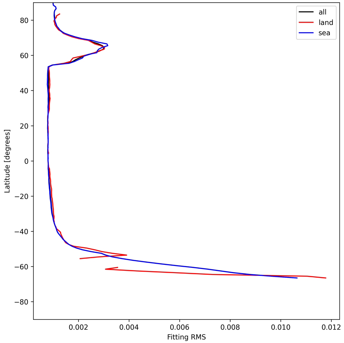
Figure 22: Zonal average of “Fitting RMS” for 2025-07-09 to 2025-07-10.
