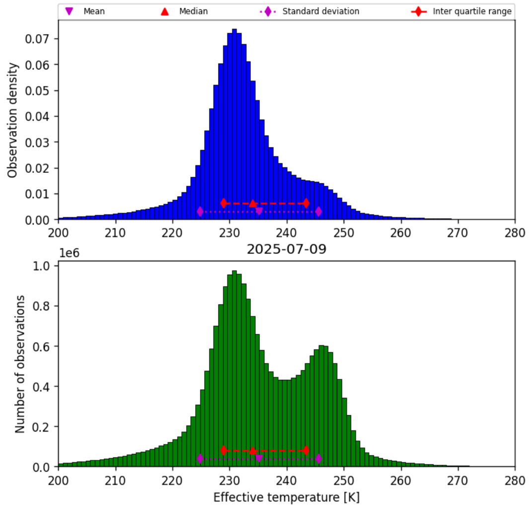
Figure 38: Histogram of “Effective temperature” for 2025-07-09 to 2025-07-10
