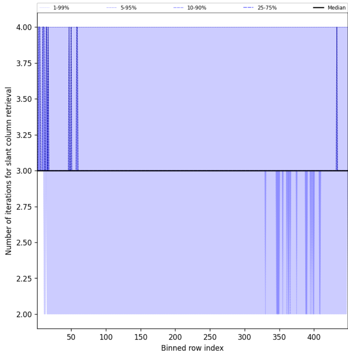
Figure 45: Along track statistics of “Number of iterations for slant column retrieval” for 2025-07-09 to 2025-07-10
