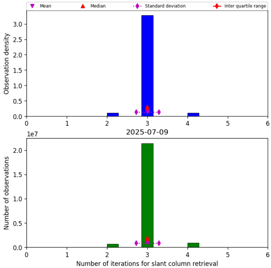
Figure 33: Histogram of “Number of iterations for slant column retrieval” for 2025-07-09 to 2025-07-10
