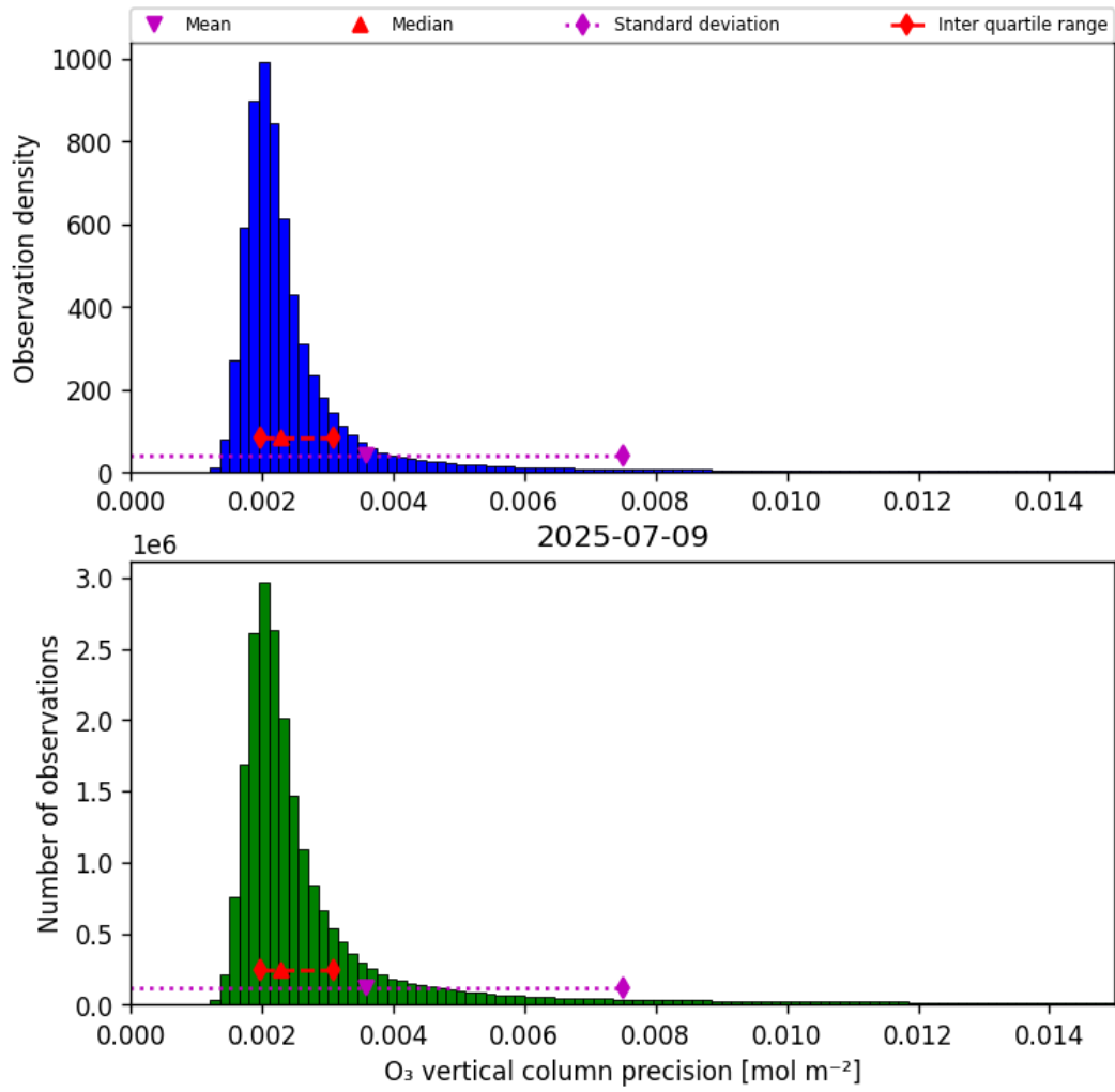
Figure 30: Histogram of “O 3 vertical column precision” for 2025-07-09 to 2025-07-10
