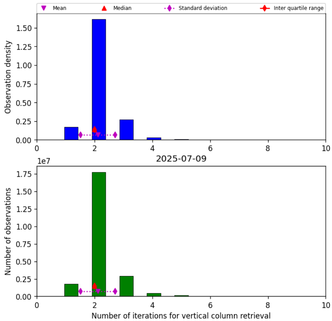
Figure 39: Histogram of “Number of iterations for vertical column retrieval” for 2025-07-09 to 2025-07-10
