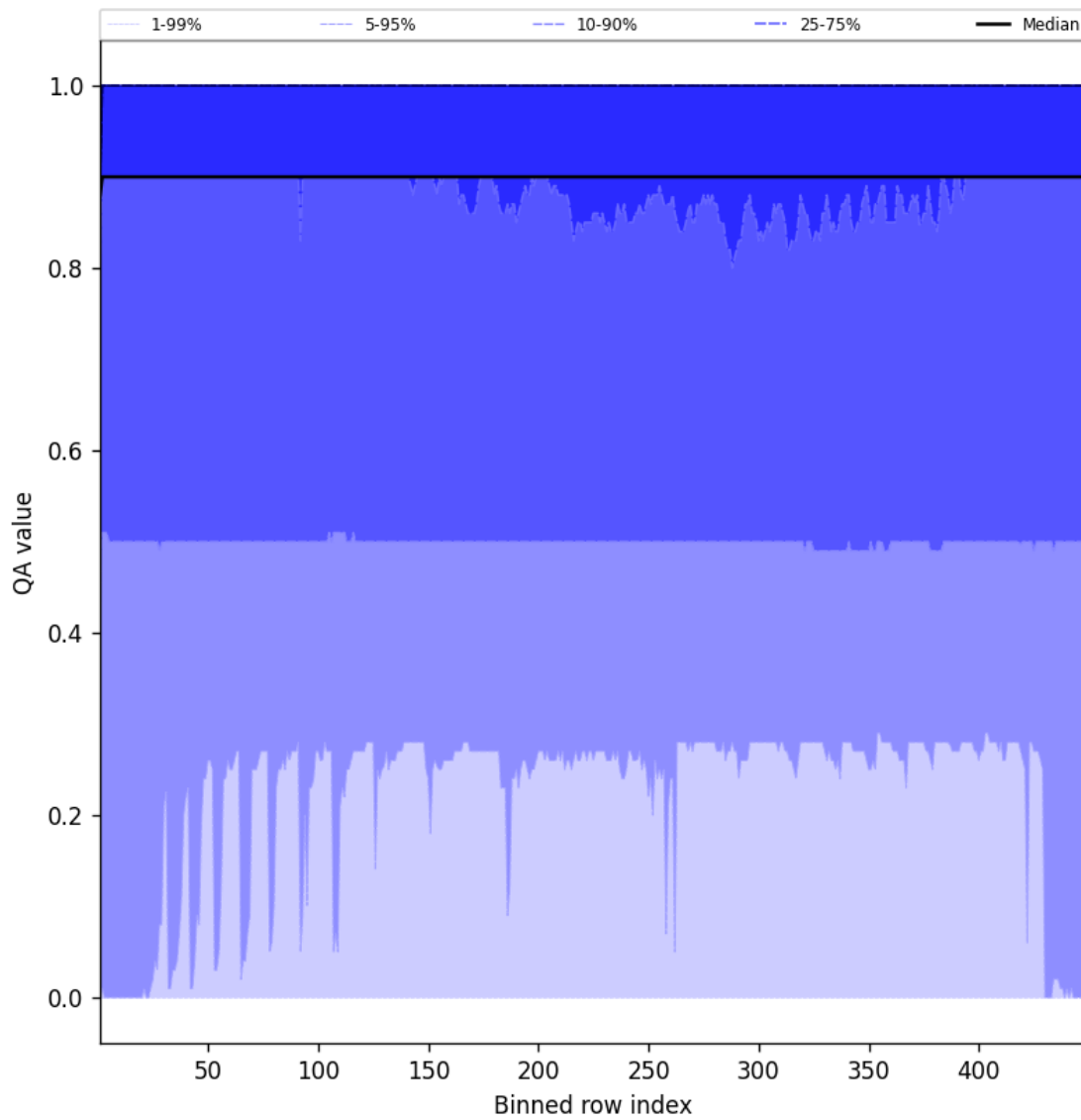
Figure 40: Along track statistics of “QA value” for 2025-07-09 to 2025-07-10
