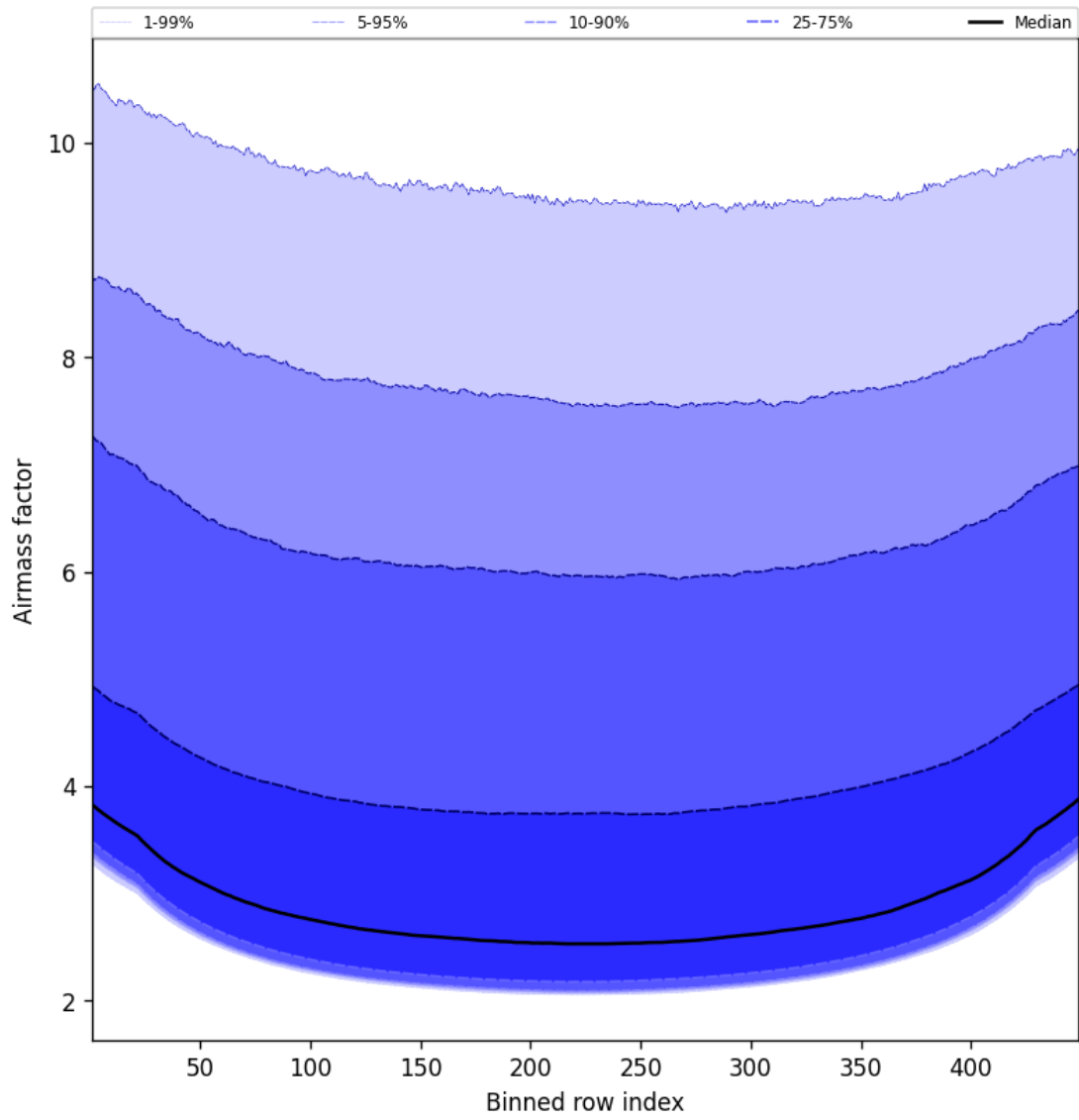
Figure 49: Along track statistics of “Airmass factor” for 2025-07-09 to 2025-07-10
