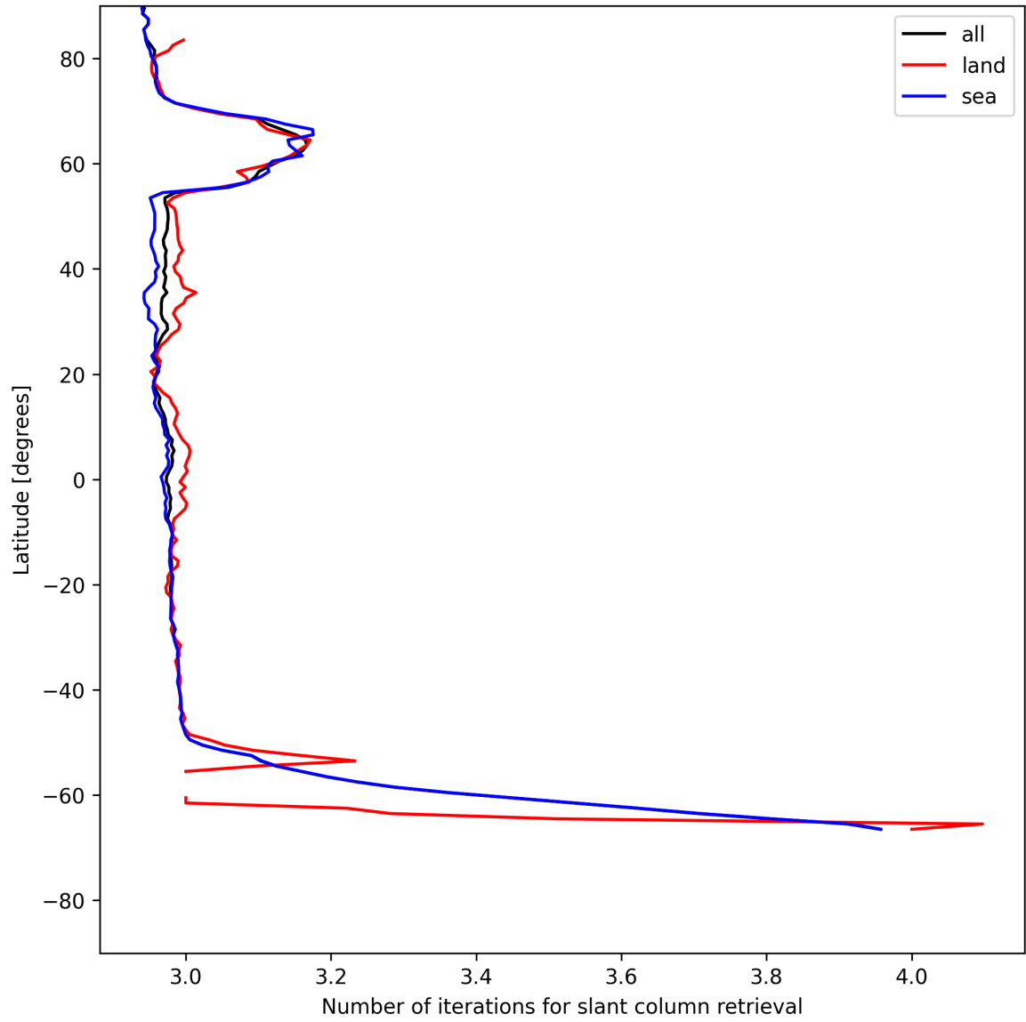
Figure 21: Zonal average of “Number of iterations for slant column retrieval” for 2025-07-09 to 2025-07-10.
