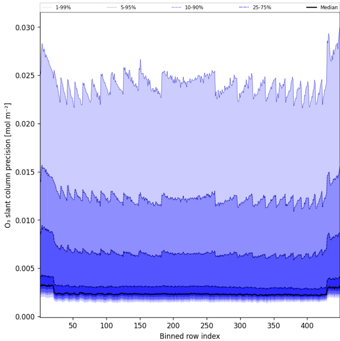
Figure 44: Along track statistics of “O 3 slant column precision” for 2025-07-09 to 2025-07-10
