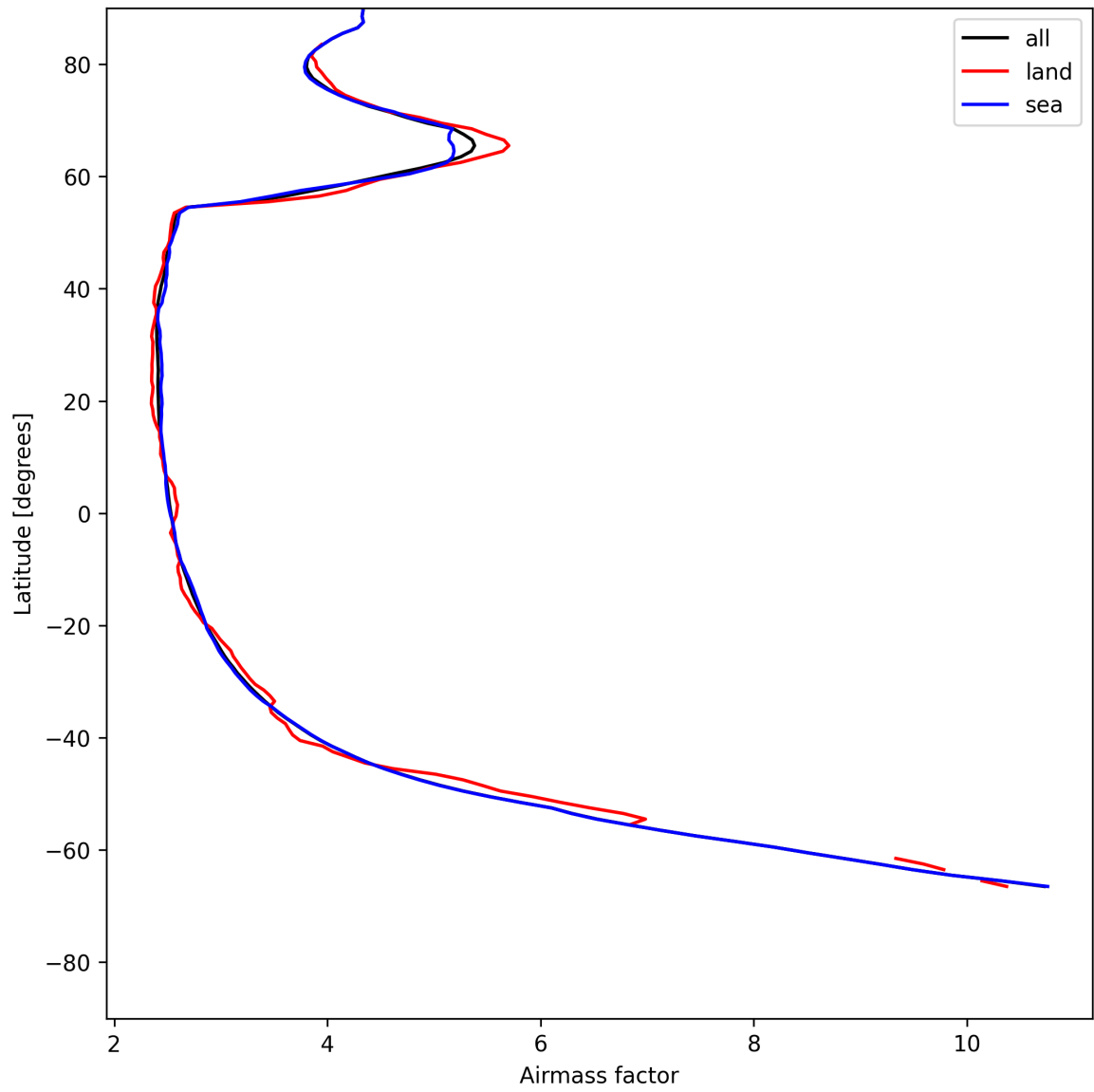
Figure 25: Zonal average of “Airmass factor” for 2025-07-10 to 2025-07-11.
