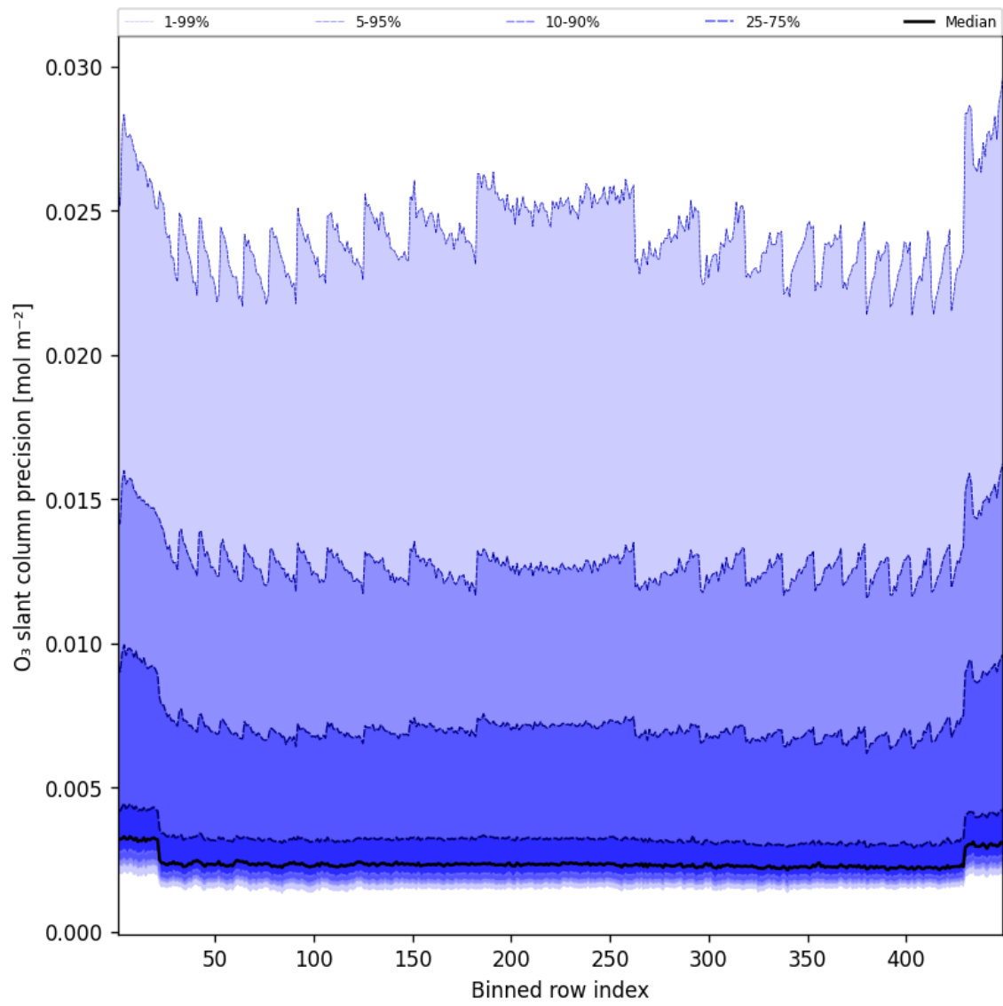
Figure 44: Along track statistics of “O 3 slant column precision” for 2025-07-10 to 2025-07-11
