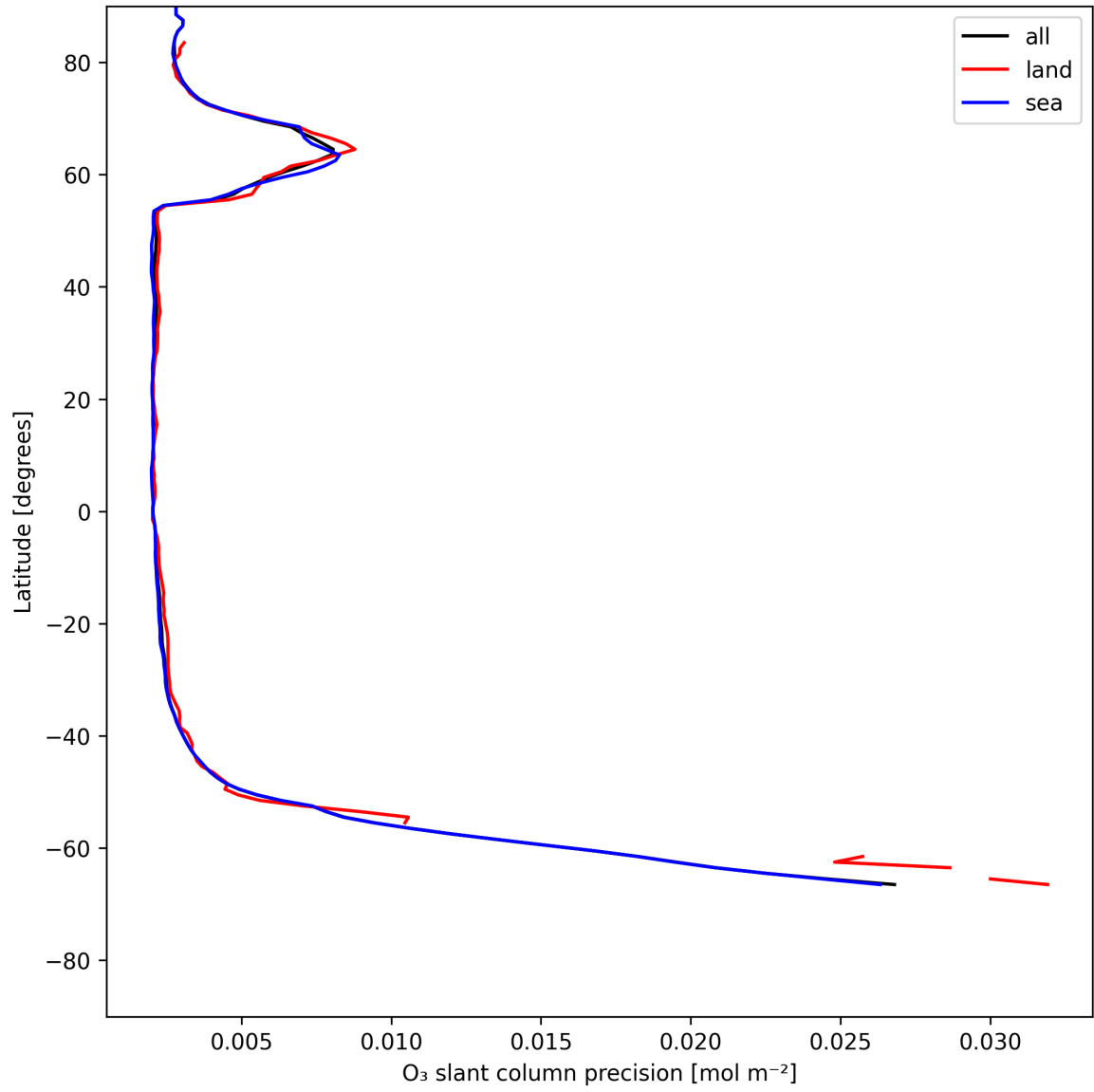
Figure 20: Zonal average of "O 3 slant column precision" for 2025-07-10 to 2025-07-11.
