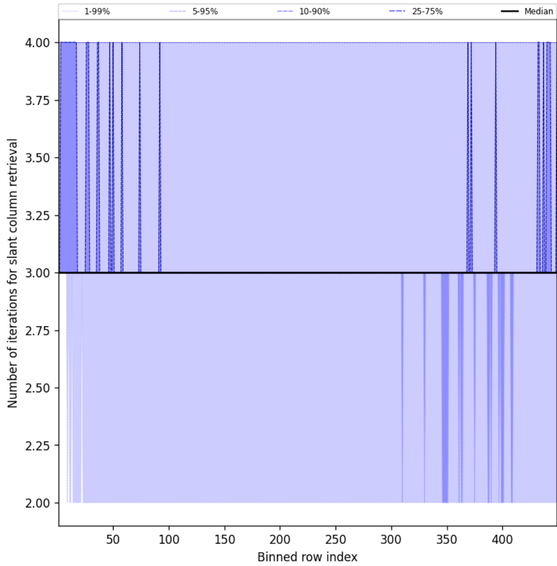
Figure 45: Along track statistics of “Number of iterations for slant column retrieval” for 2025-07-10 to 2025-07-11
