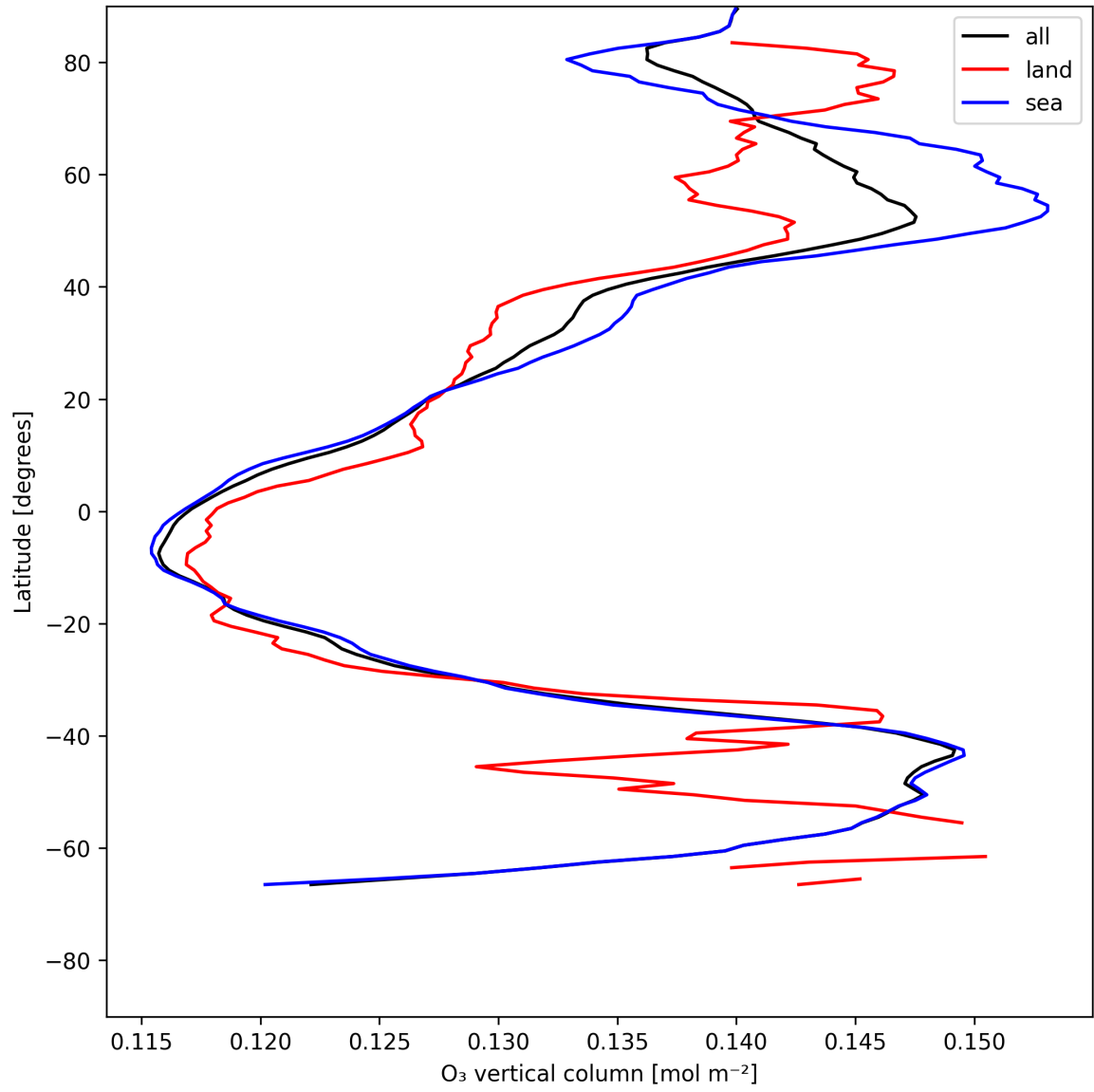
Figure 17: Zonal average of “O 3 vertical column” for 2025-07-10 to 2025-07-11.
