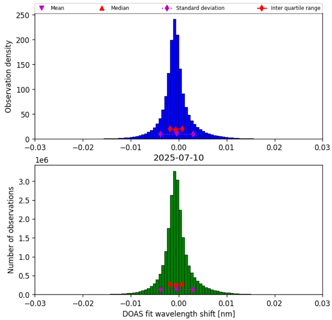
Figure 35: Histogram of “DOAS fit wavelength shift” for 2025-07-10 to 2025-07-11
