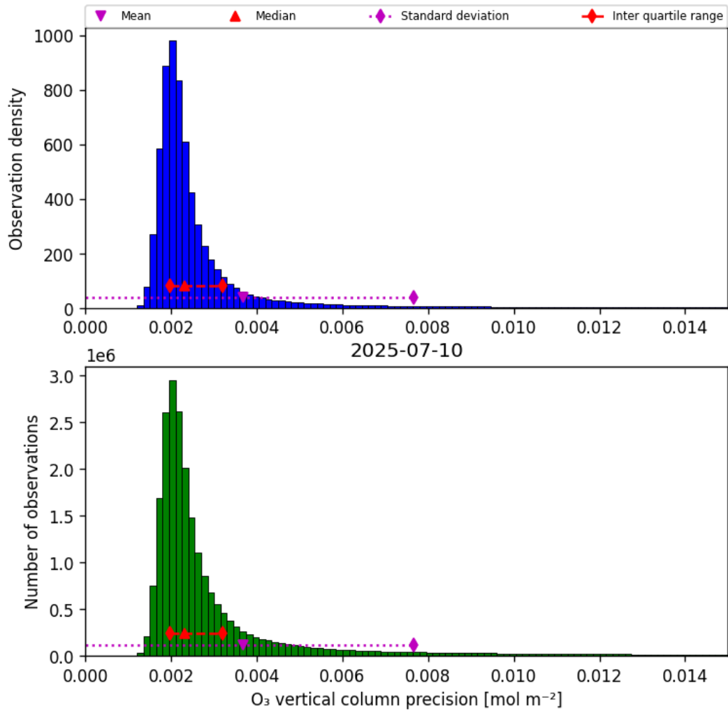
Figure 30: Histogram of “O 3 vertical column precision” for 2025-07-10 to 2025-07-11
