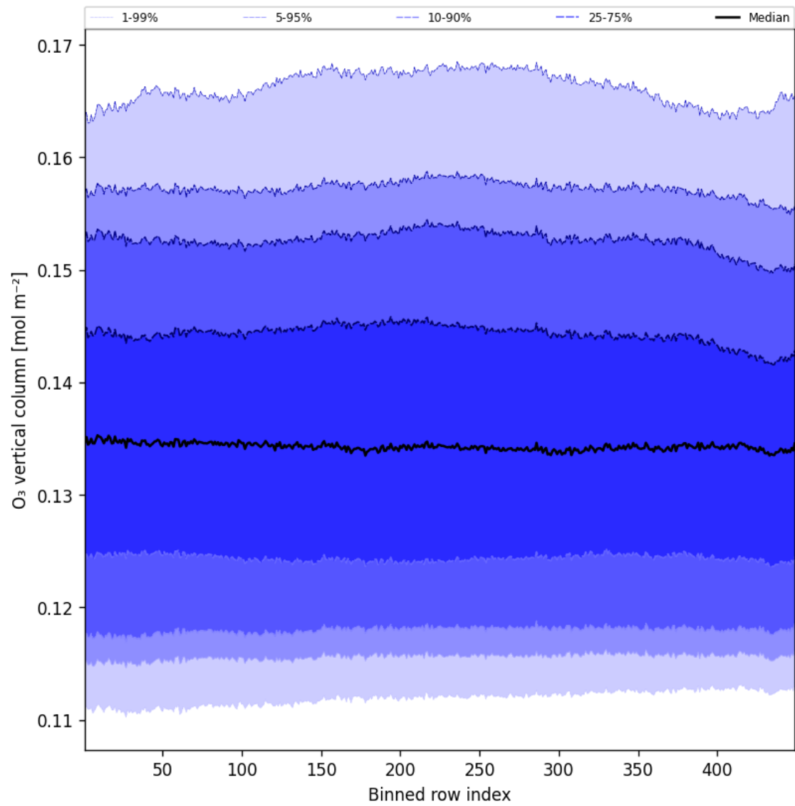
Figure 41: Along track statistics of “O 3 vertical column” for 2025-07-10 to 2025-07-11
