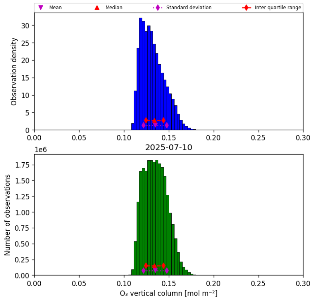
Figure 29: Histogram of “O 3 vertical column” for 2025-07-10 to 2025-07-11
