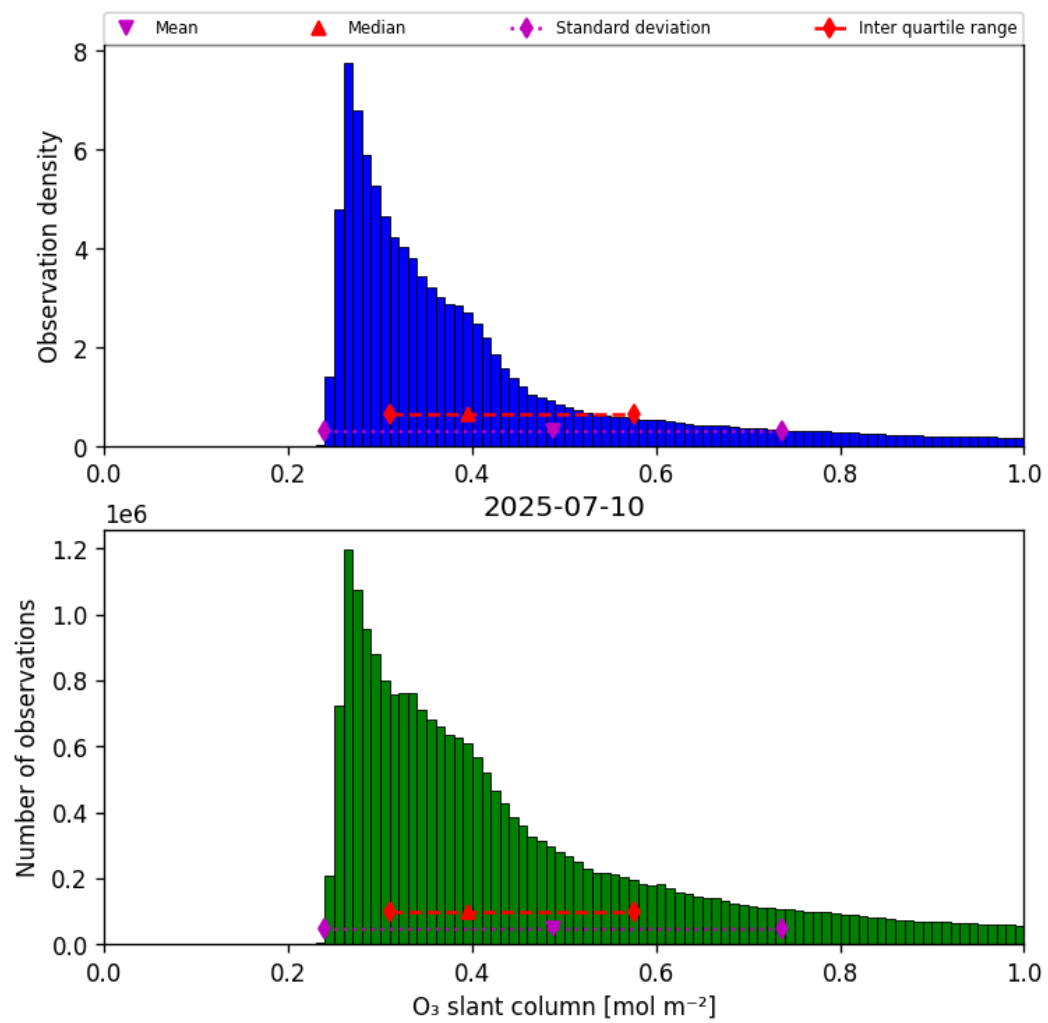
Figure 31: Histogram of “O 3 slant column” for 2025-07-10 to 2025-07-11
