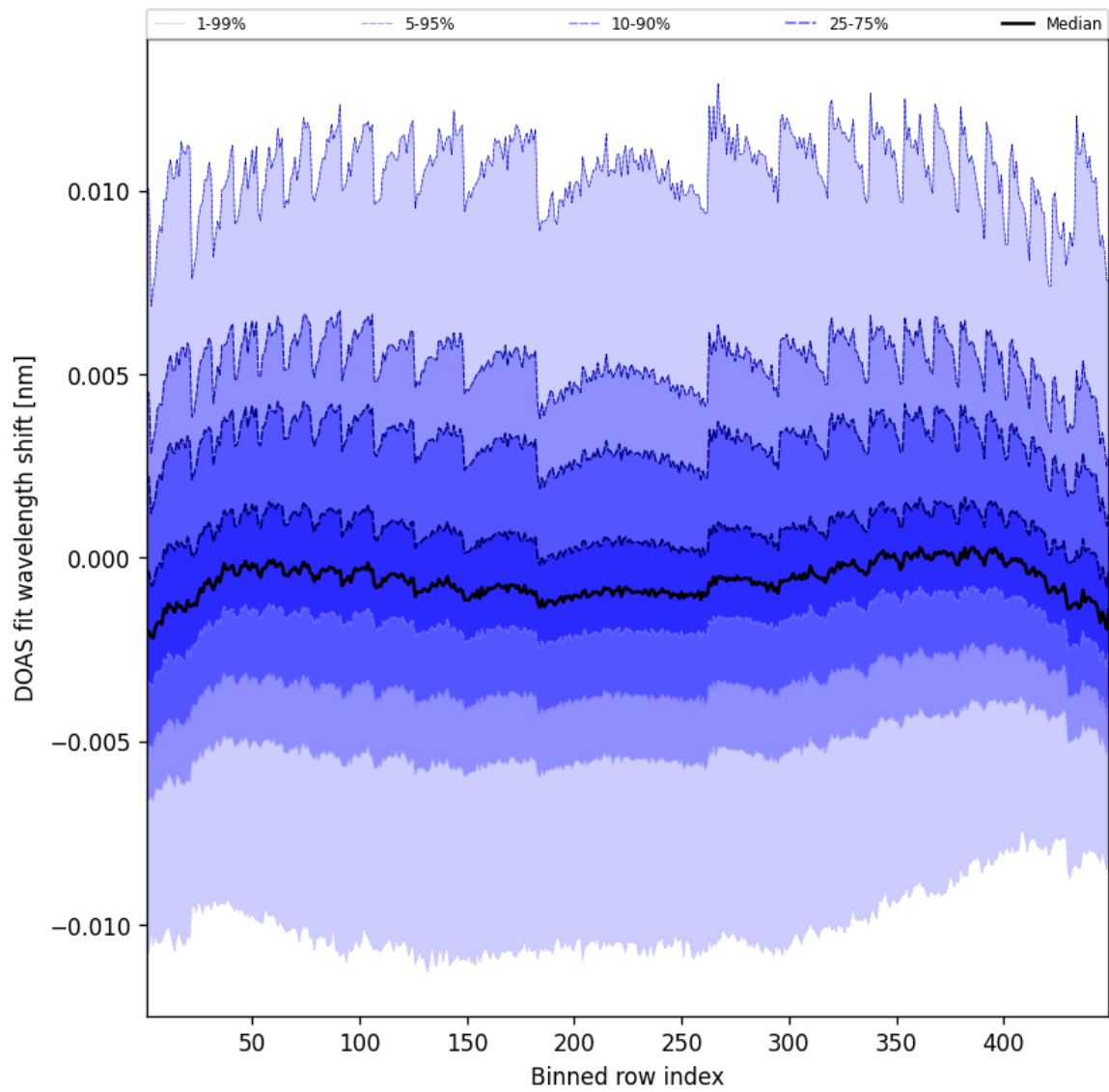
Figure 47: Along track statistics of “DOAS fit wavelength shift” for 2025-07-10 to 2025-07-11
