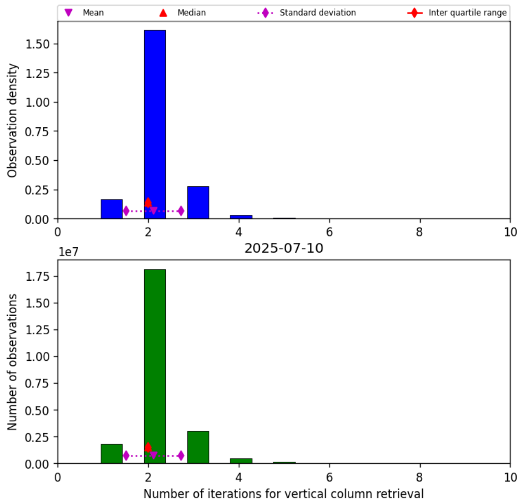
Figure 39: Histogram of “Number of iterations for vertical column retrieval” for 2025-07-10 to 2025-07-11
