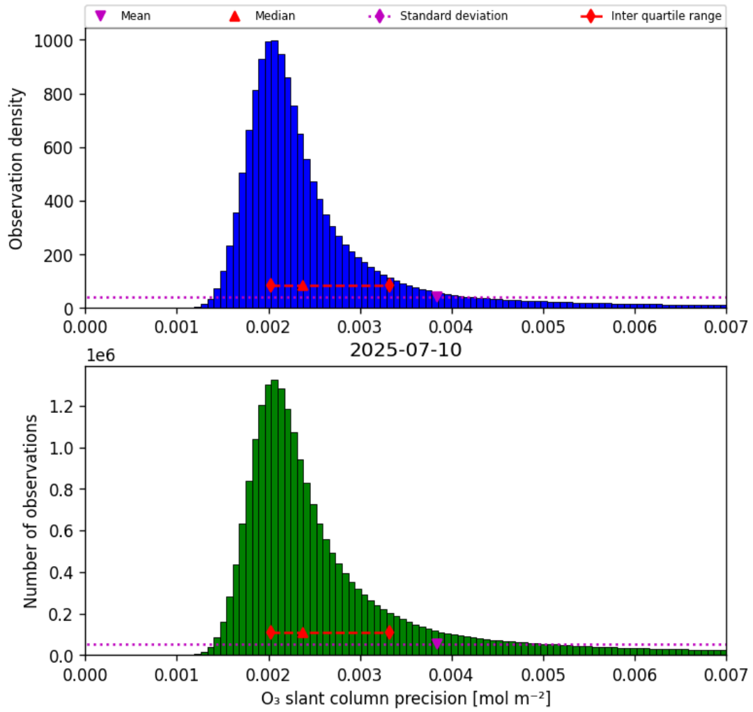
Figure 32: Histogram of “O 3 slant column precision” for 2025-07-10 to 2025-07-11
