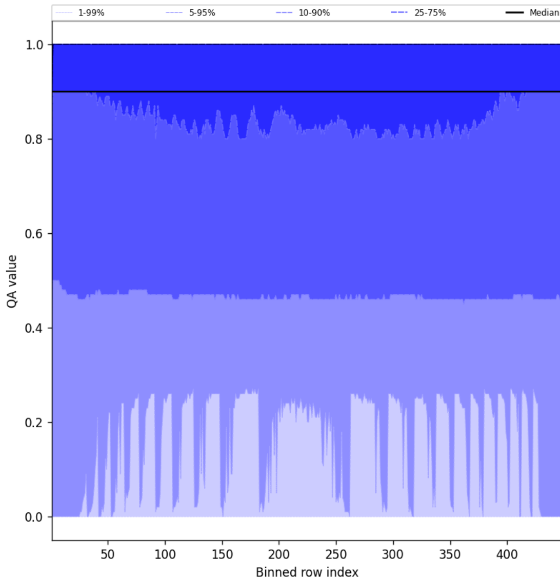
Figure 40: Along track statistics of “QA value” for 2025-07-10 to 2025-07-11
