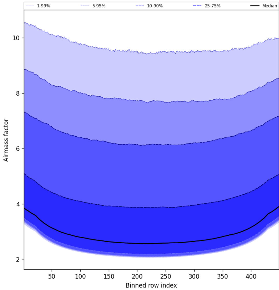
Figure 49: Along track statistics of “Airmass factor” for 2025-07-10 to 2025-07-11
