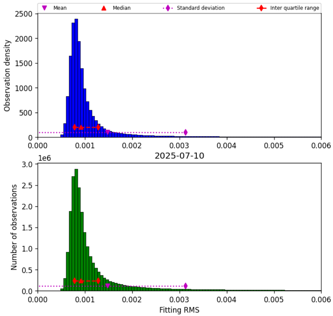
Figure 34: Histogram of “Fitting RMS” for 2025-07-10 to 2025-07-11
