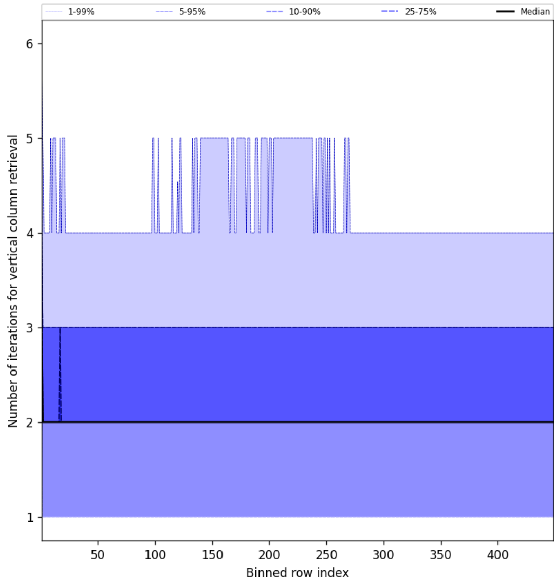
Figure 51: Along track statistics of “Number of iterations for vertical column retrieval” for 2025-07-10 to 2025-07-11
