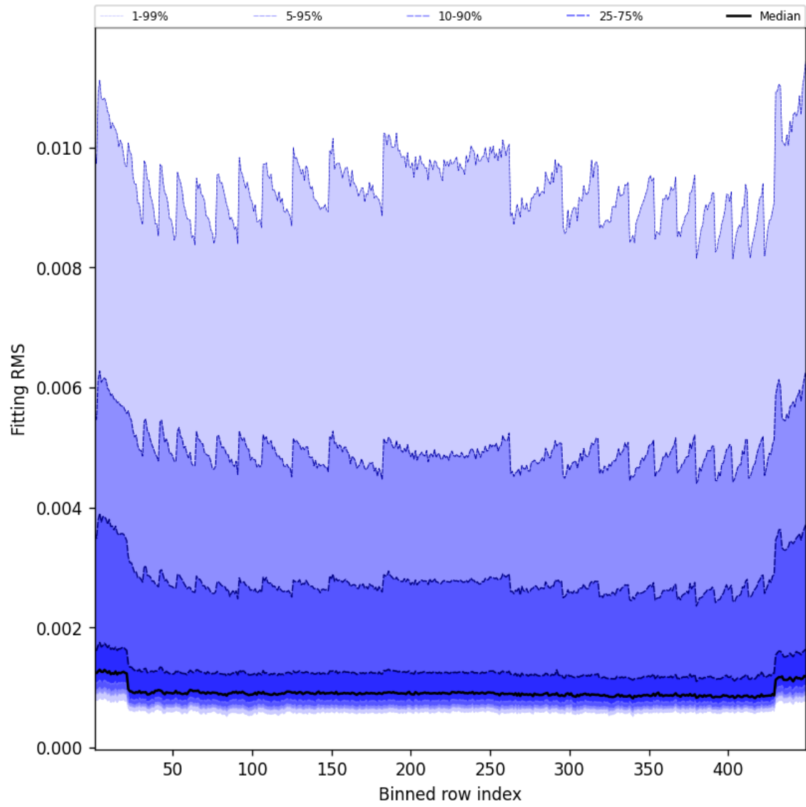
Figure 46: Along track statistics of “Fitting RMS” for 2025-07-10 to 2025-07-11
