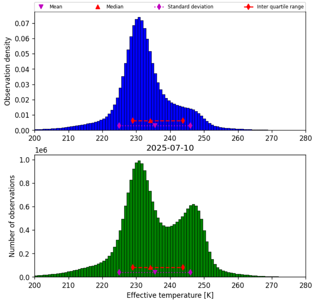
Figure 38: Histogram of “Effective temperature” for 2025-07-10 to 2025-07-11
