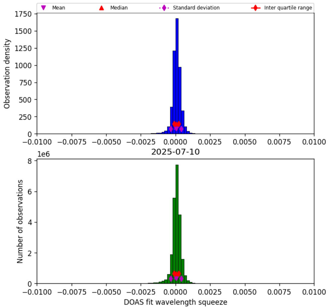
Figure 36: Histogram of “DOAS fit wavelength squeeze” for 2025-07-10 to 2025-07-11
