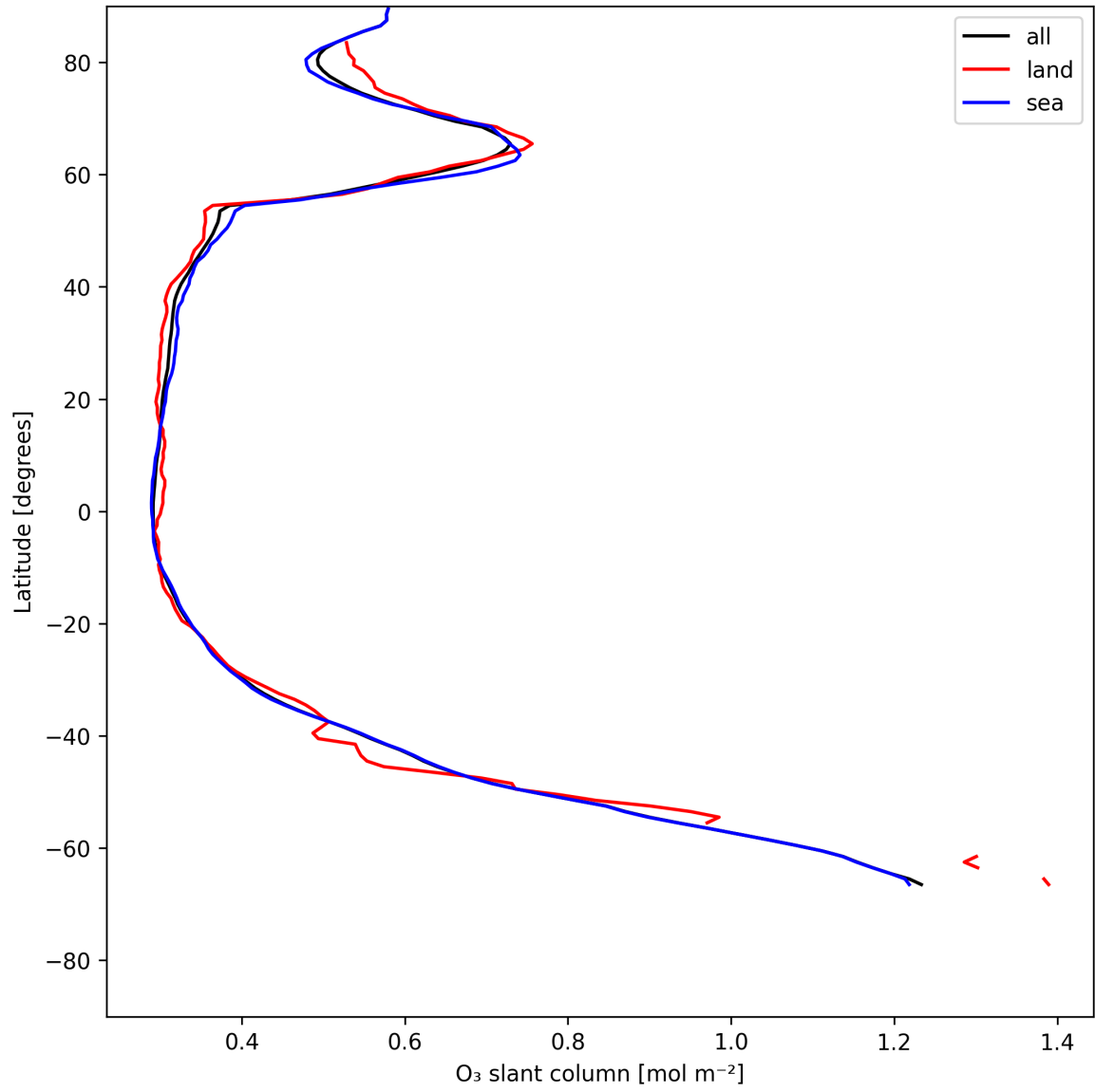
Figure 19: Zonal average of “O 3 slant column” for 2025-07-10 to 2025-07-11.
