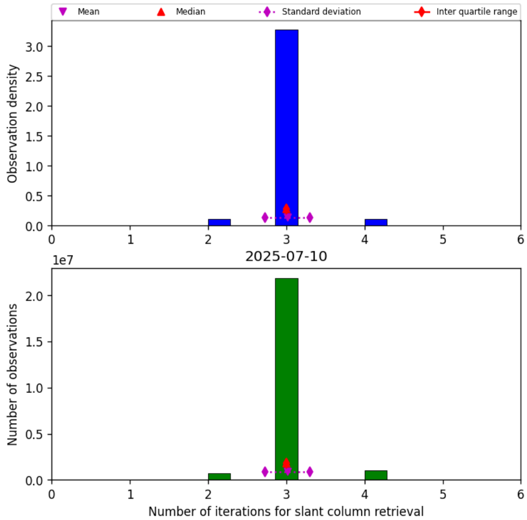
Figure 33: Histogram of “Number of iterations for slant column retrieval” for 2025-07-10 to 2025-07-11
