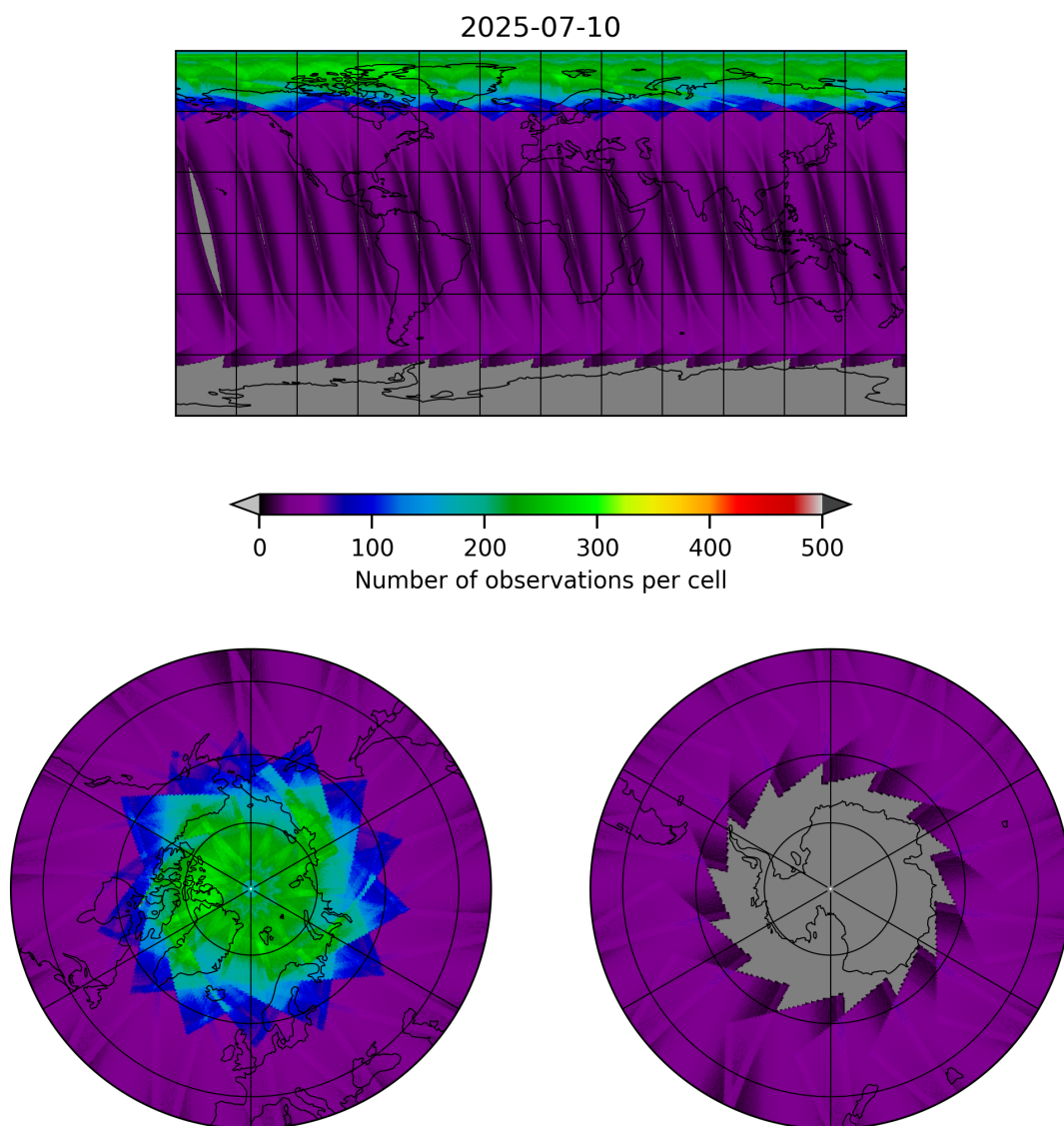
Figure 15: Map of the number of observations for 2025-07-10 to 2025-07-11
