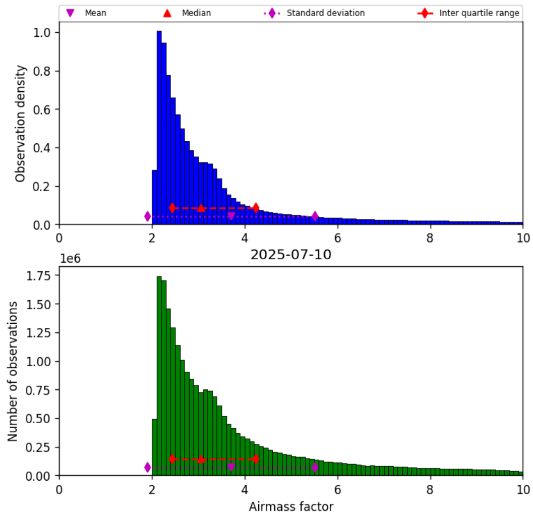
Figure 37: Histogram of “Airmass factor” for 2025-07-10 to 2025-07-11
