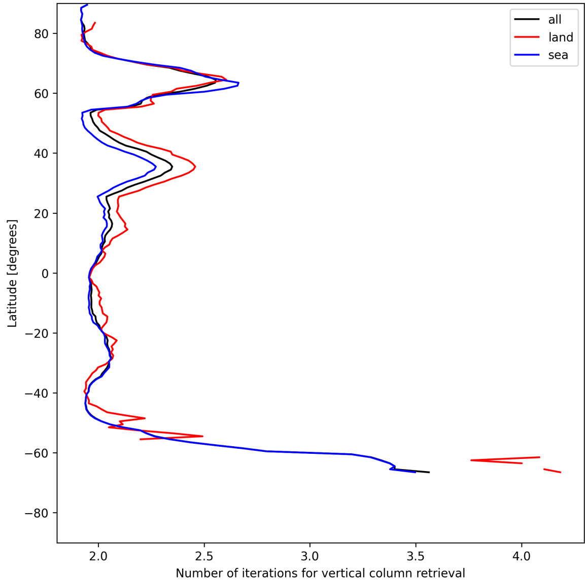
Figure 27: Zonal average of “Number of iterations for vertical column retrieval” for 2025-07-10 to 2025-07-11.
