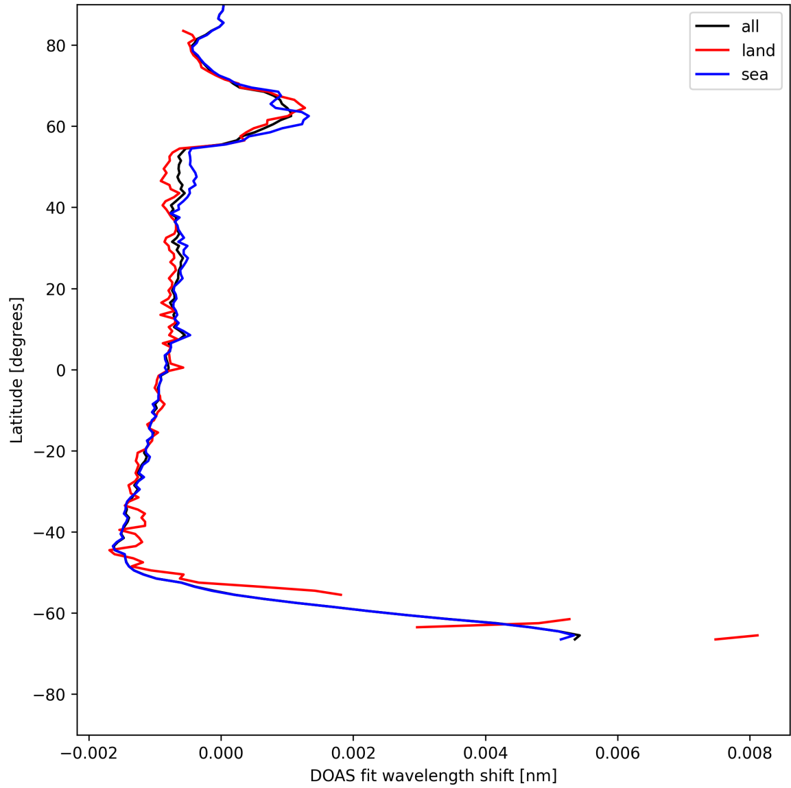
Figure 23: Zonal average of "DOAS fit wavelength shift" for 2025-07-10 to 2025-07-11.
