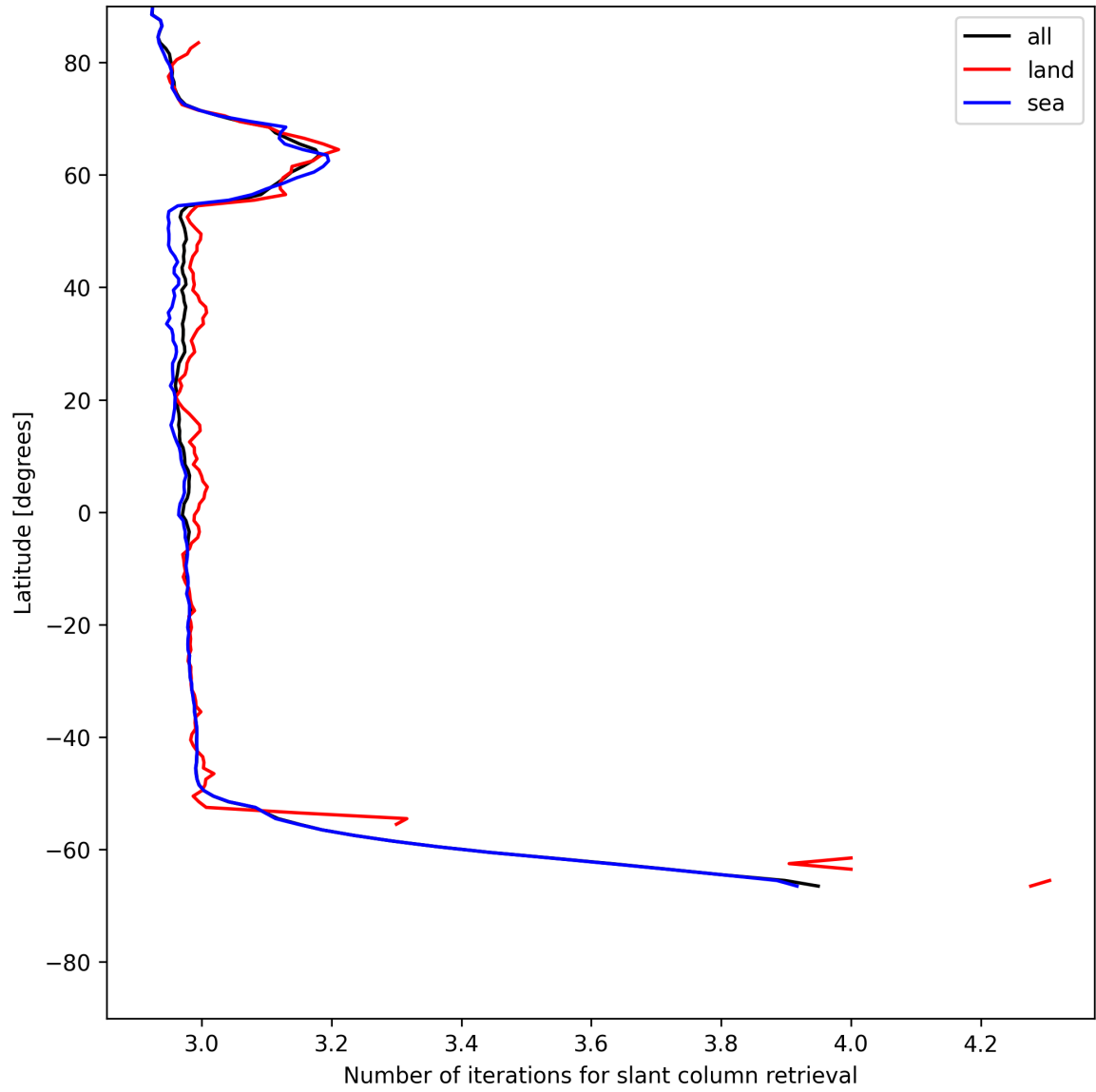
Figure 21: Zonal average of “Number of iterations for slant column retrieval” for 2025-07-10 to 2025-07-11.
