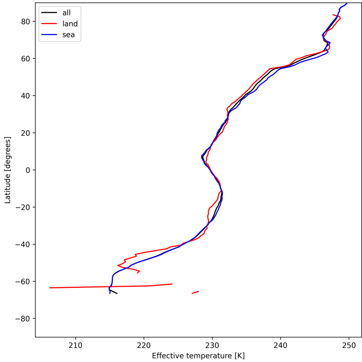
Figure 26: Zonal average of "Effective temperature" for 2025-07-10 to 2025-07-11.
