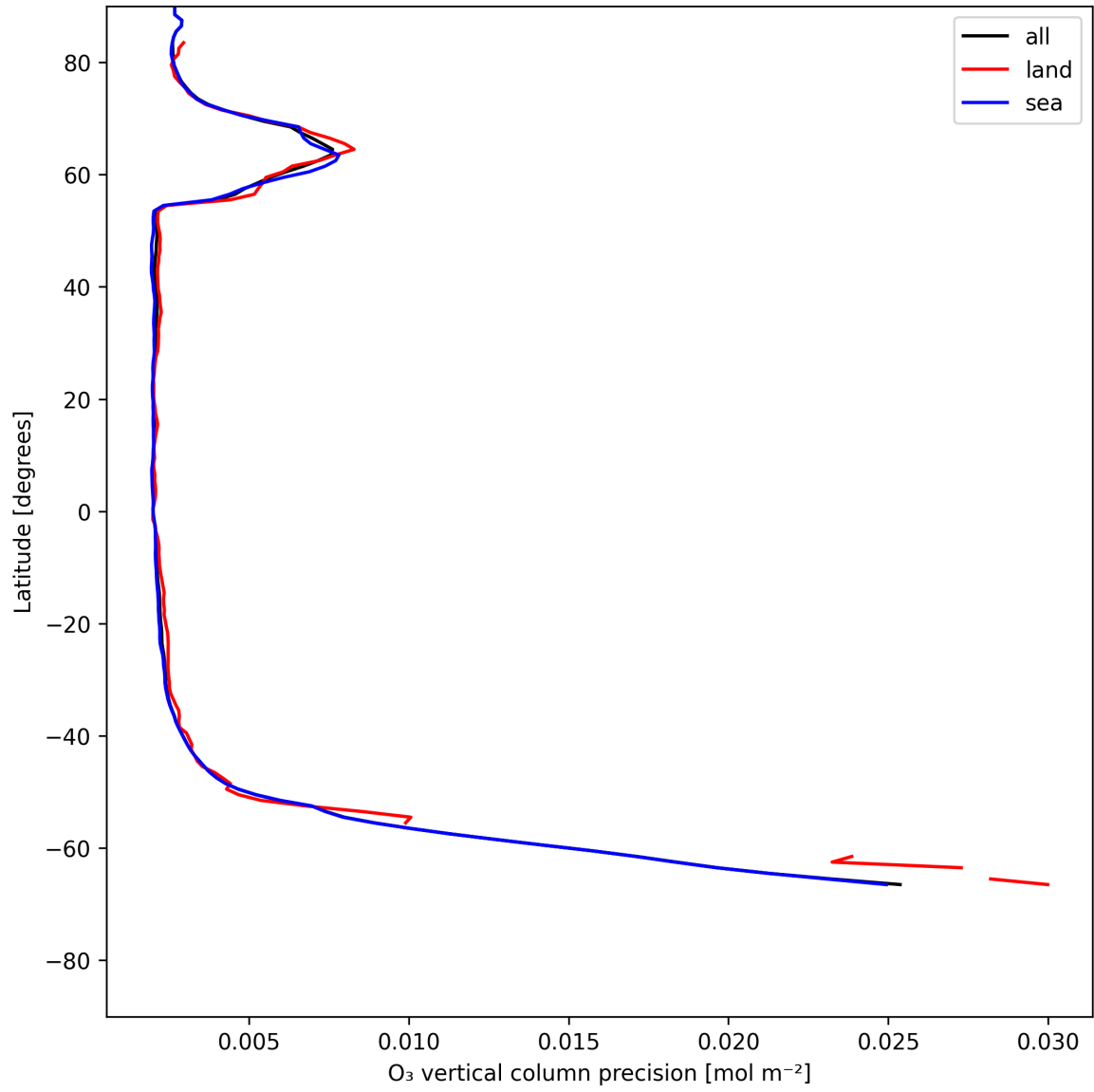
Figure 18: Zonal average of "O 3 vertical column precision" for 2025-07-10 to 2025-07-11.
