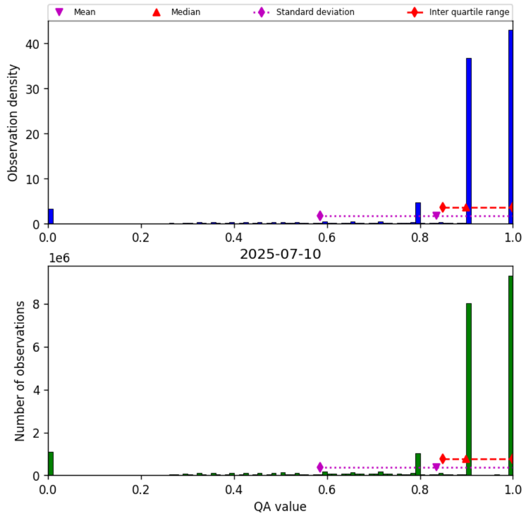
Figure 28: Histogram of “QA value” for 2025-07-10 to 2025-07-11
