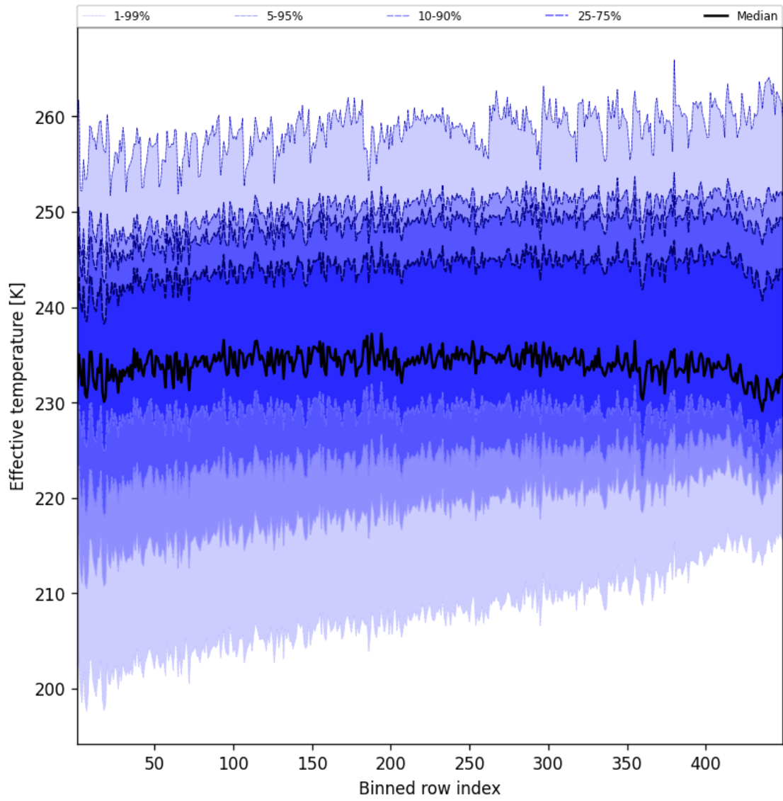
Figure 50: Along track statistics of “Effective temperature” for 2025-07-10 to 2025-07-11
