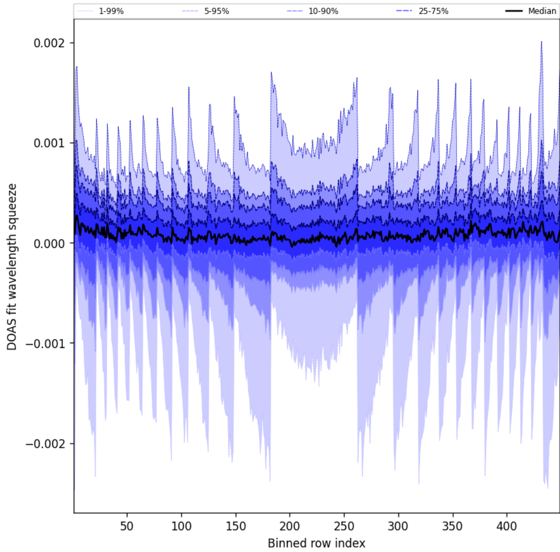
Figure 48: Along track statistics of “DOAS fit wavelength squeeze” for 2025-07-10 to 2025-07-11
