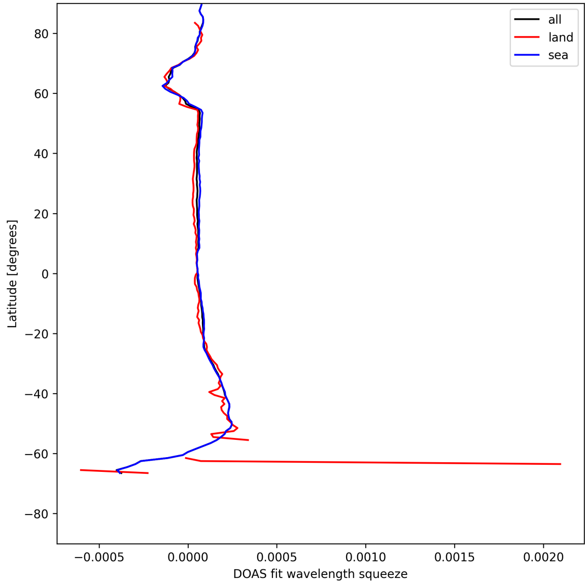
Figure 24: Zonal average of “DOAS fit wavelength squeeze” for 2025-07-10 to 2025-07-11.
