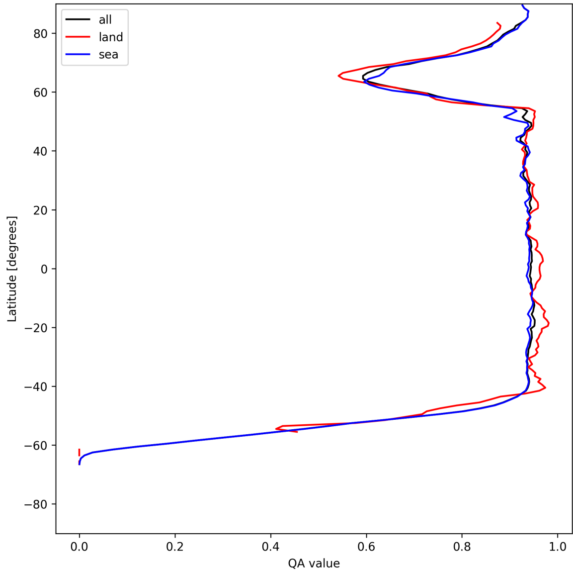
Figure 16: Zonal average of “QA value” for 2025-07-10 to 2025-07-11.
