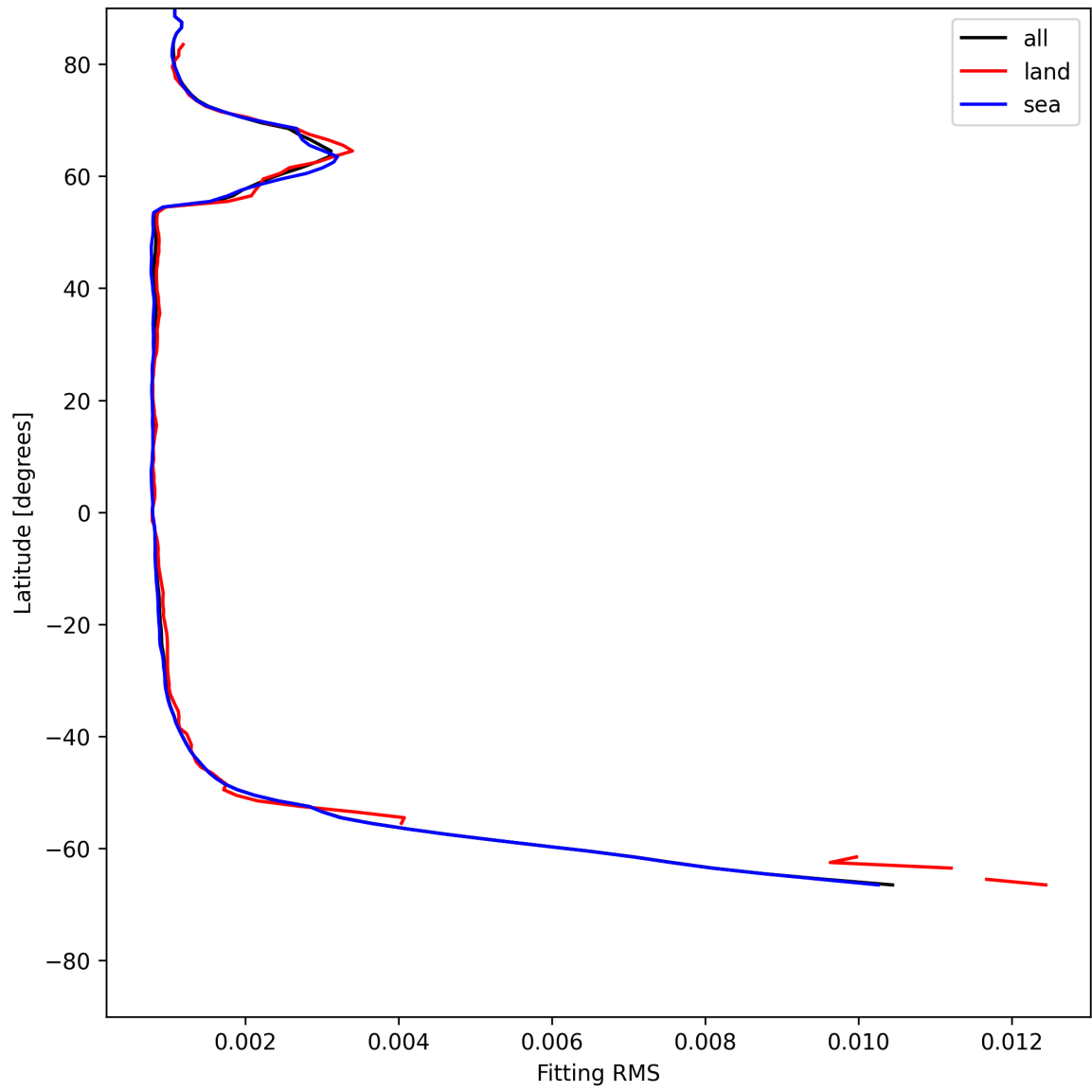
Figure 22: Zonal average of “Fitting RMS” for 2025-07-10 to 2025-07-11.
