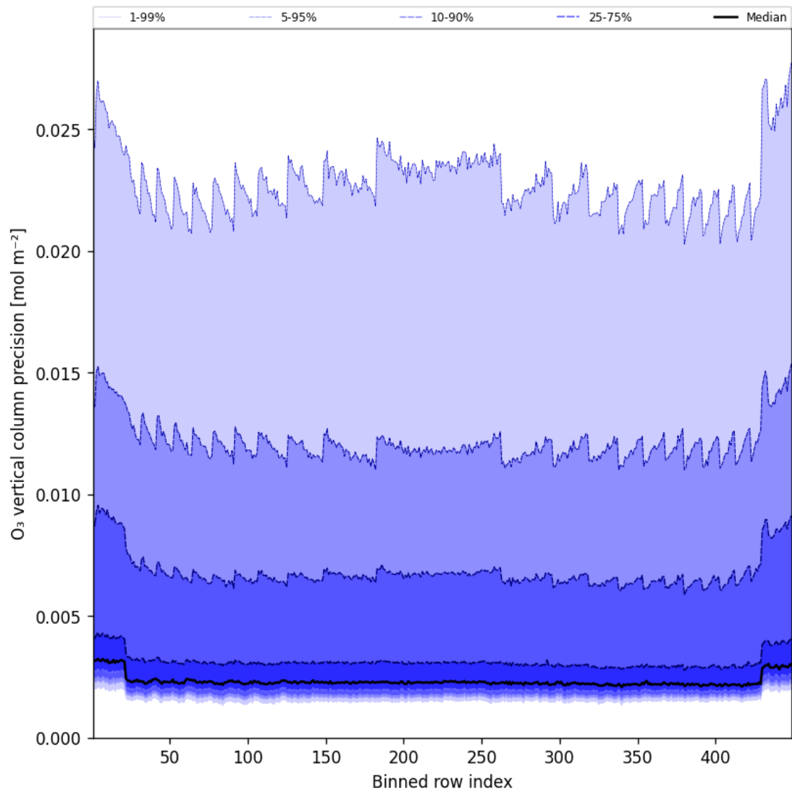
Figure 42: Along track statistics of “O 3 vertical column precision” for 2025-07-10 to 2025-07-11
