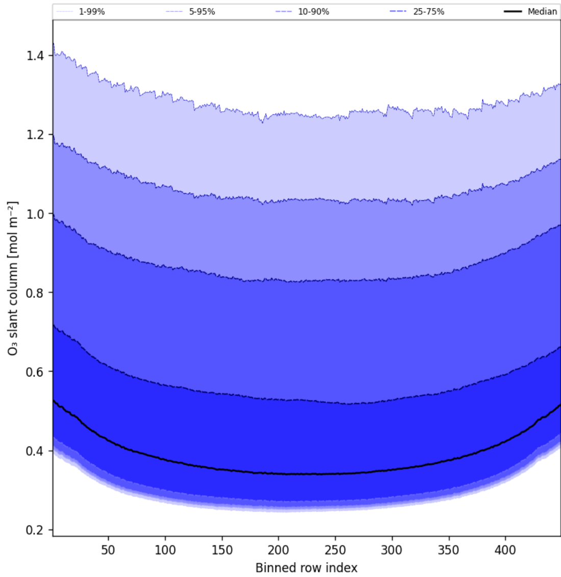
Figure 43: Along track statistics of “O 3 slant column” for 2025-07-10 to 2025-07-11
