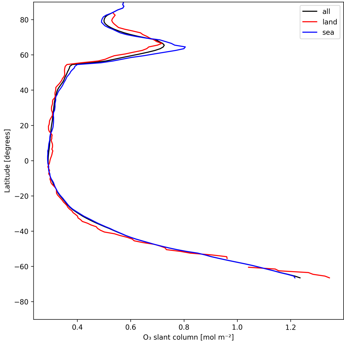
Figure 19: Zonal average of “O 3 slant column” for 2025-07-11 to 2025-07-11.
