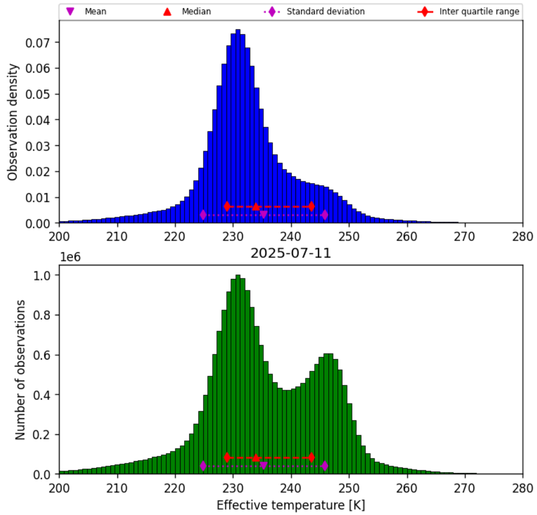
Figure 38: Histogram of “Effective temperature” for 2025-07-11 to 2025-07-11
