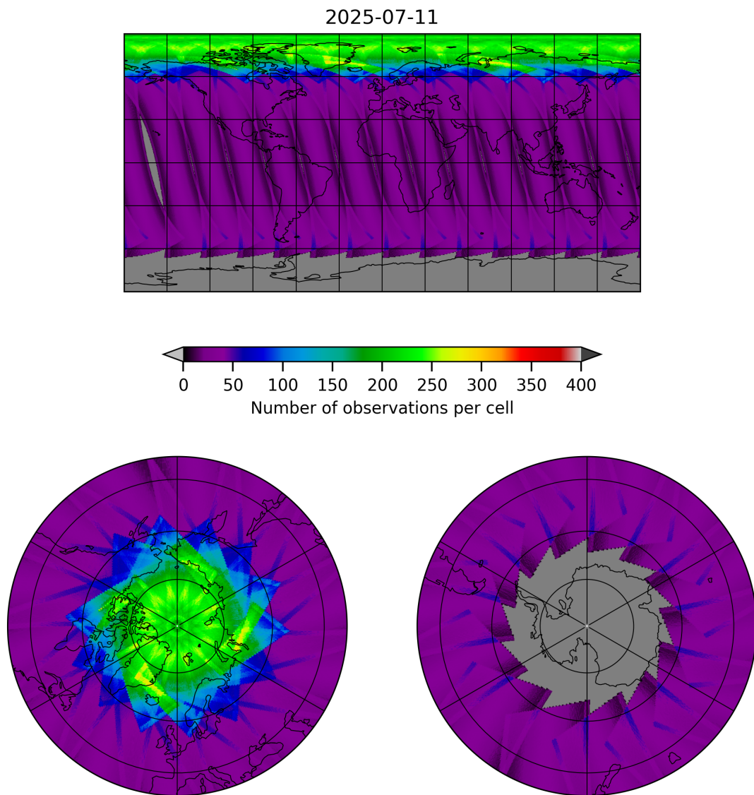
Figure 15: Map of the number of observations for 2025-07-11 to 2025-07-11
