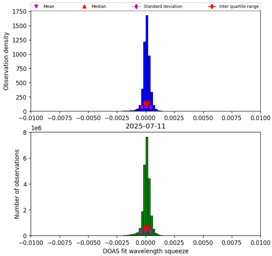
Figure 36: Histogram of “DOAS fit wavelength squeeze” for 2025-07-11 to 2025-07-11
