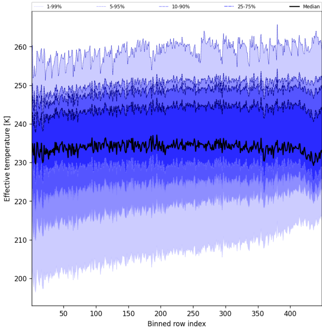
Figure 50: Along track statistics of “Effective temperature” for 2025-07-11 to 2025-07-11
