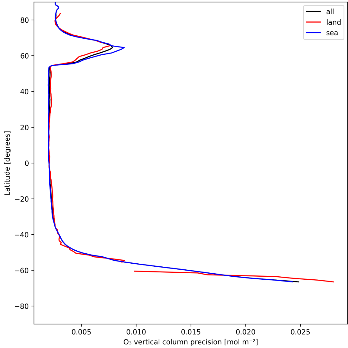
Figure 18: Zonal average of “O 3 vertical column precision” for 2025-07-11 to 2025-07-11.
