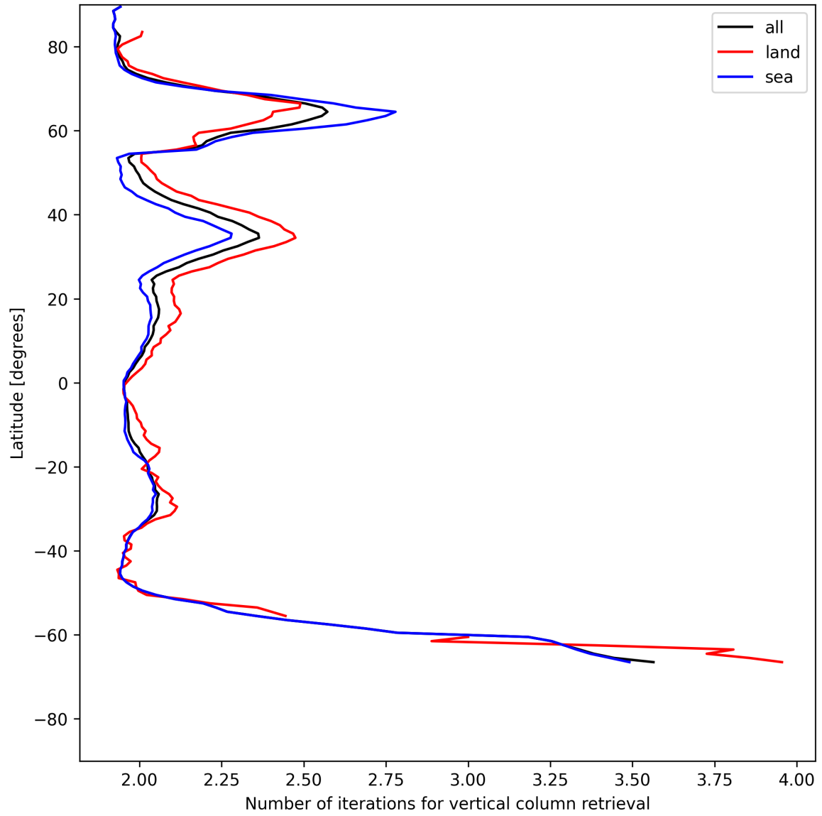
Figure 27: Zonal average of “Number of iterations for vertical column retrieval” for 2025-07-11 to 2025-07-11.
