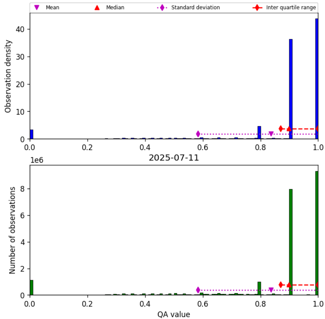
Figure 28: Histogram of “QA value” for 2025-07-11 to 2025-07-11
