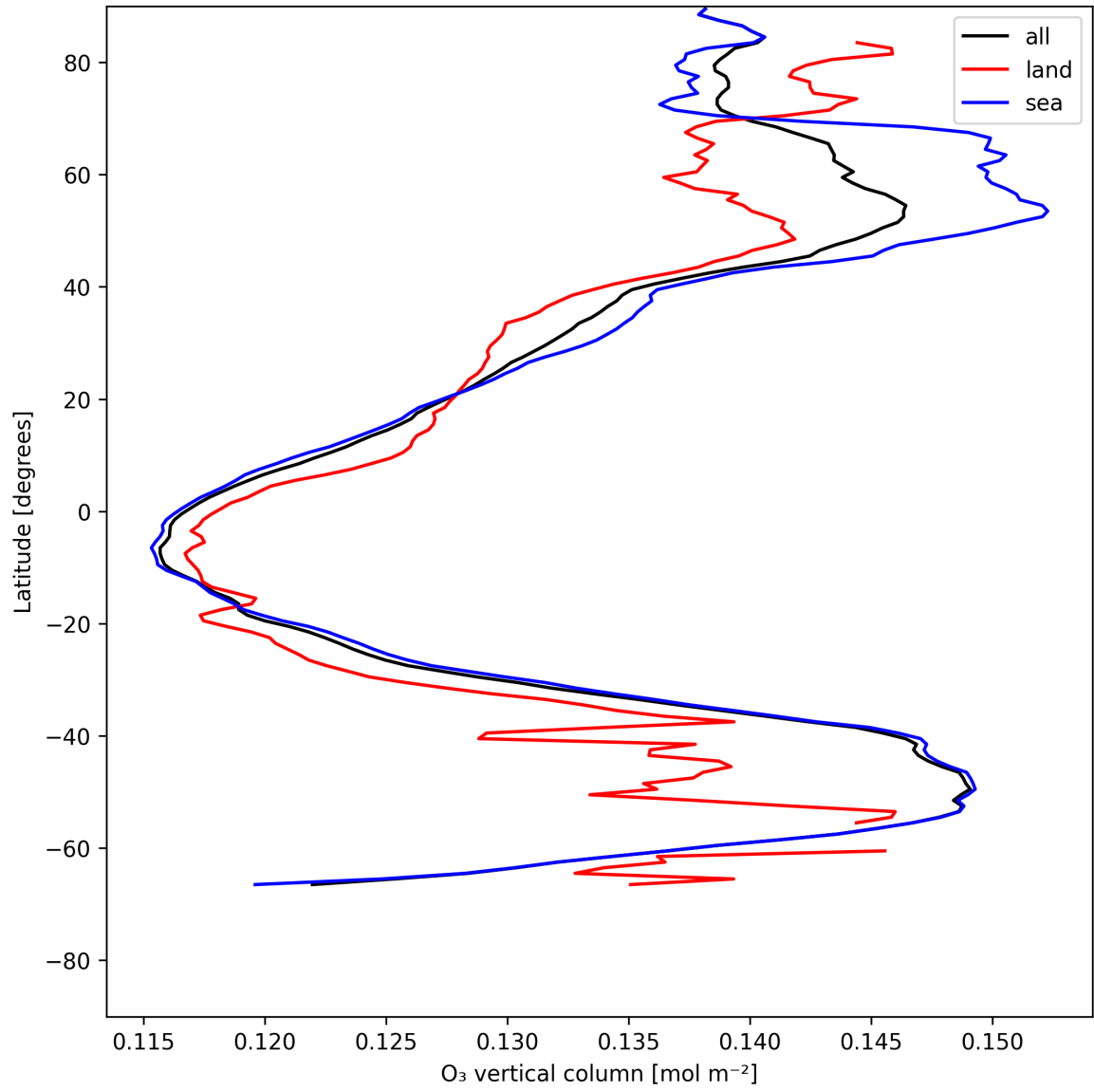
Figure 17: Zonal average of “O 3 vertical column” for 2025-07-11 to 2025-07-11.
