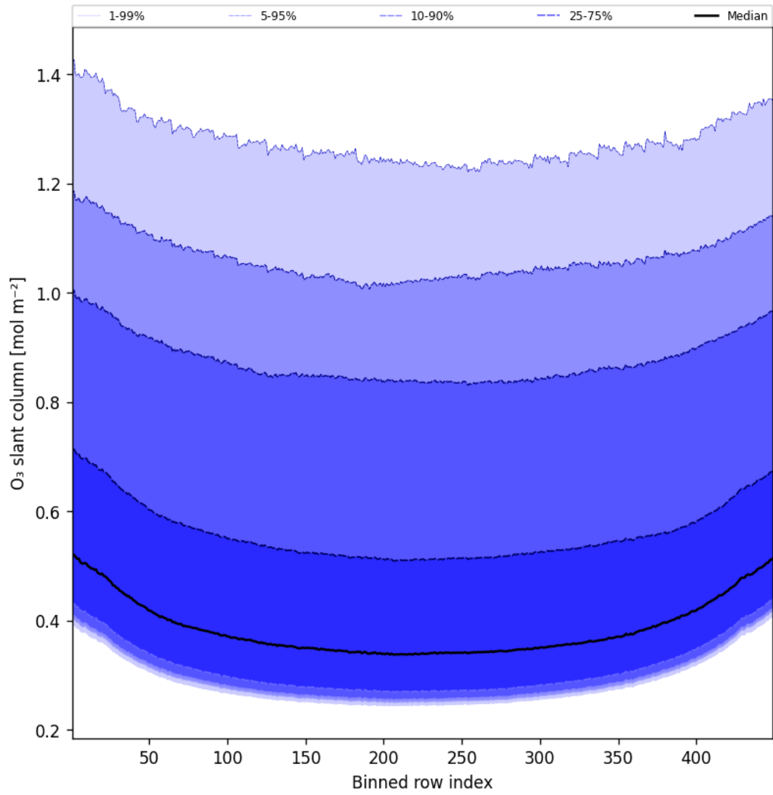
Figure 43: Along track statistics of “O 3 slant column” for 2025-07-11 to 2025-07-11
