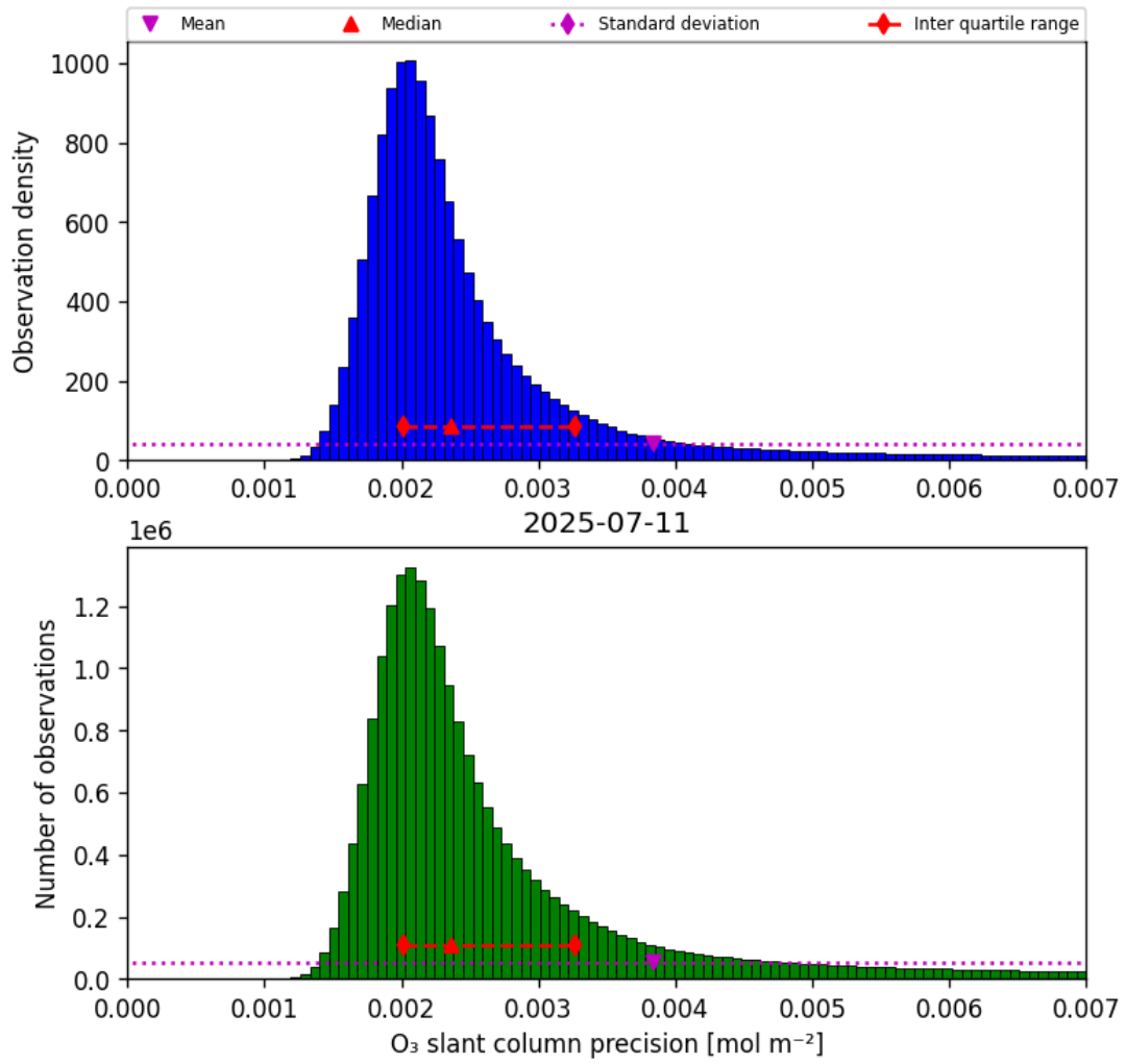
Figure 32: Histogram of “O 3 slant column precision” for 2025-07-11 to 2025-07-11
