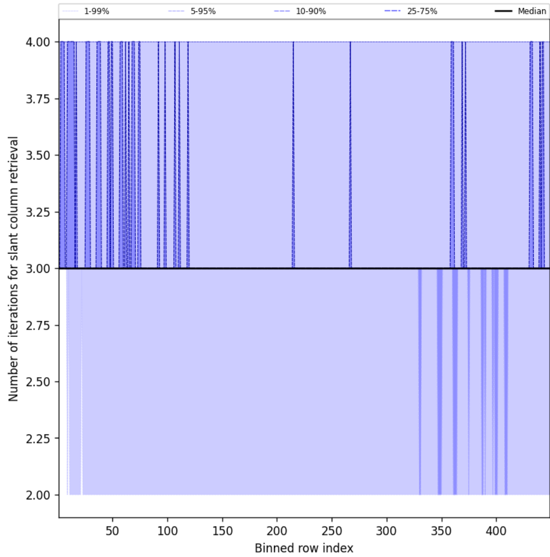
Figure 45: Along track statistics of “Number of iterations for slant column retrieval” for 2025-07-11 to 2025-07-11
