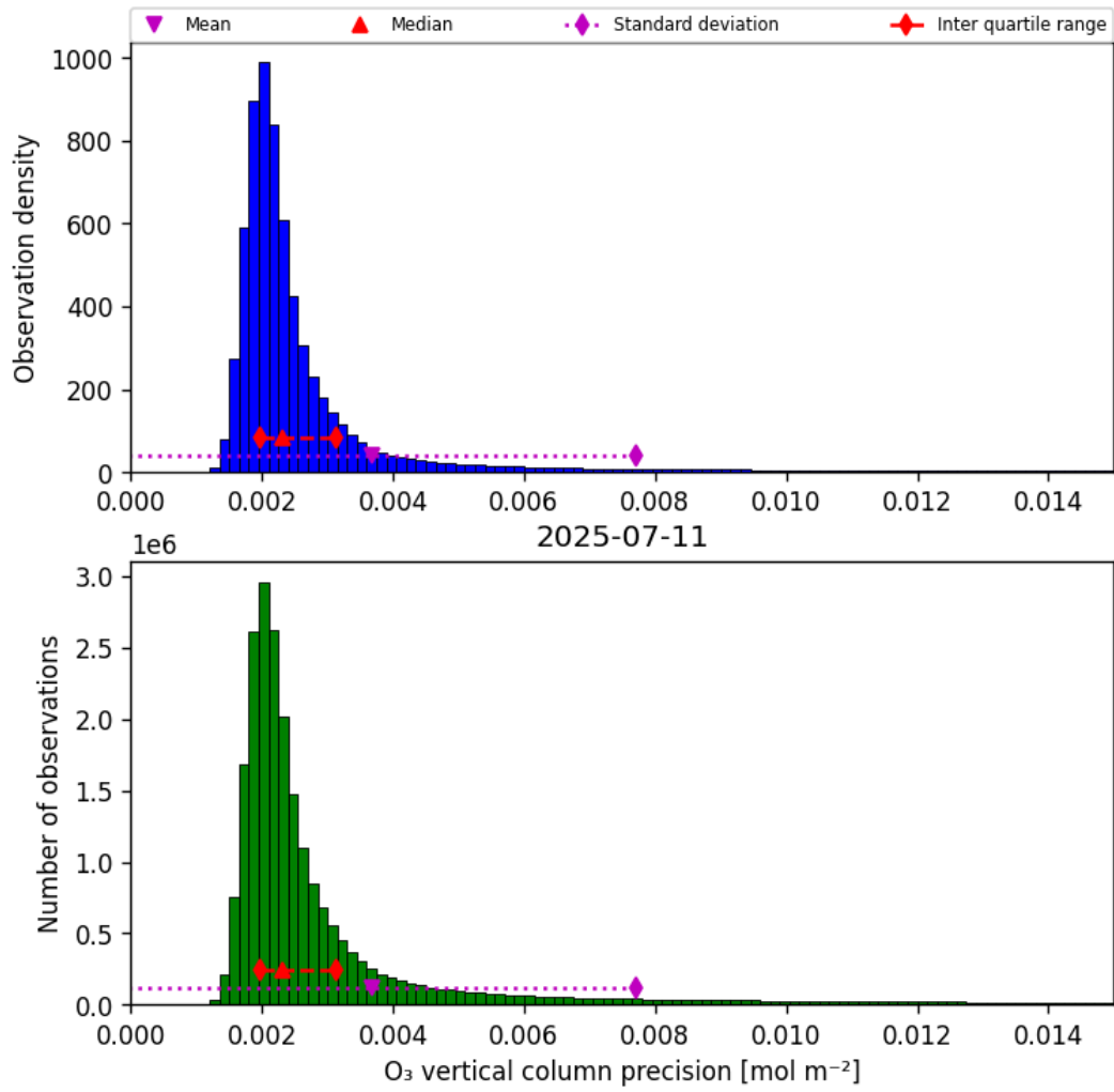
Figure 30: Histogram of “O 3 vertical column precision” for 2025-07-11 to 2025-07-11
