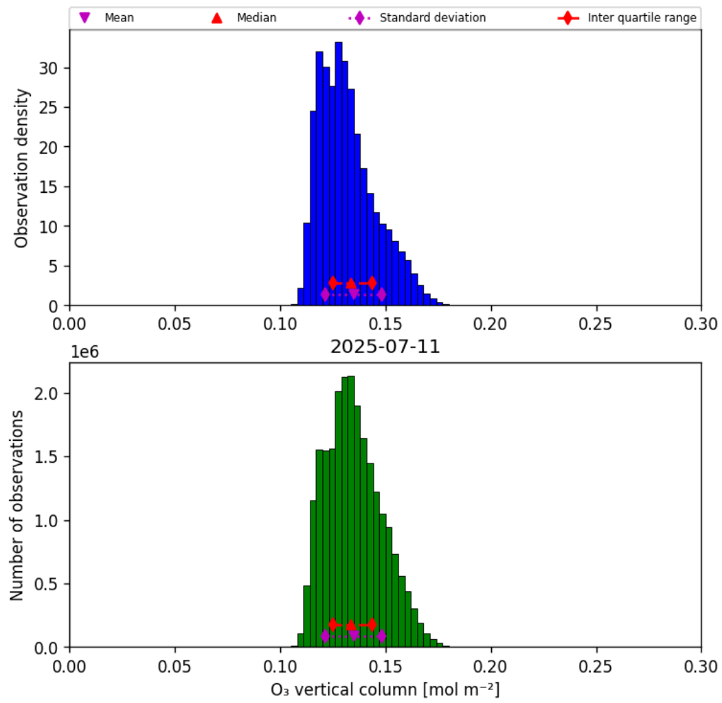
Figure 29: Histogram of “O 3 vertical column” for 2025-07-11 to 2025-07-11
