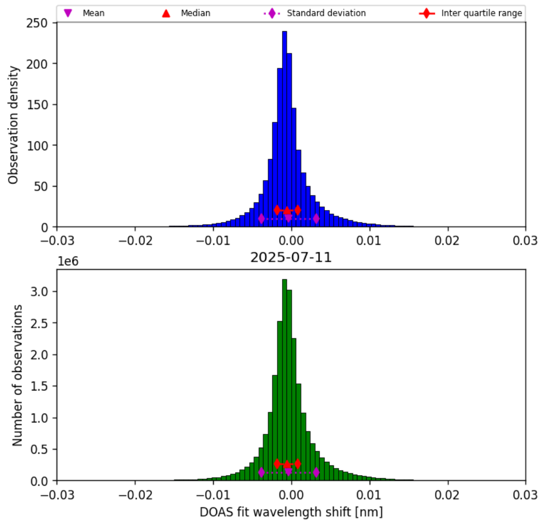
Figure 35: Histogram of “DOAS fit wavelength shift” for 2025-07-11 to 2025-07-11
