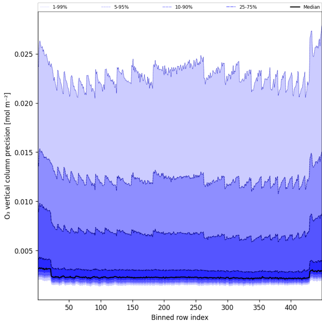
Figure 42: Along track statistics of “O 3 vertical column precision” for 2025-07-11 to 2025-07-11
