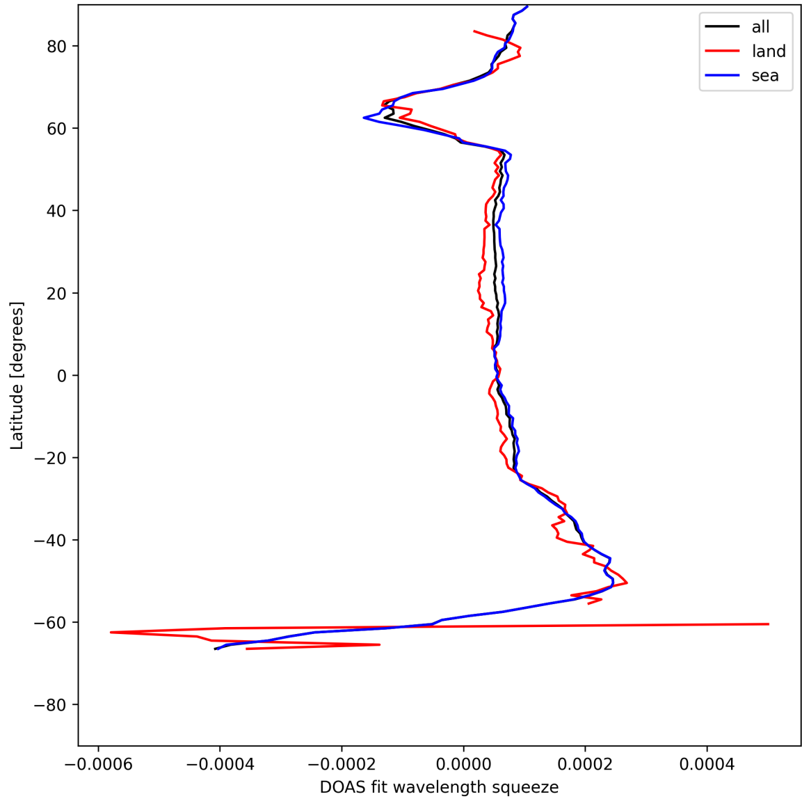
Figure 24: Zonal average of “DOAS fit wavelength squeeze” for 2025-07-11 to 2025-07-11.
