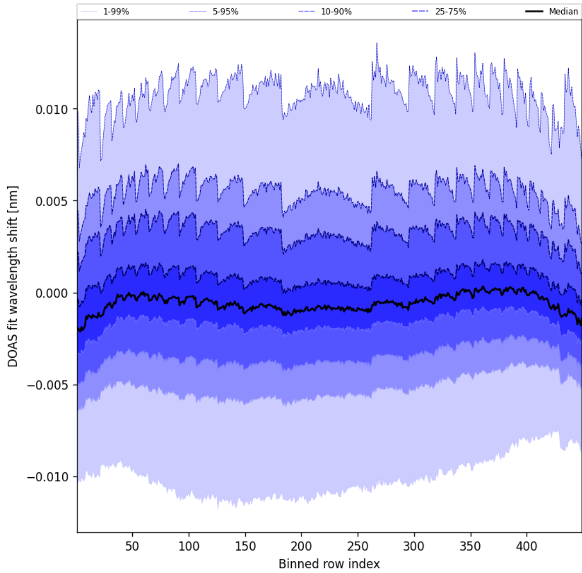
Figure 47: Along track statistics of "DOAS fit wavelength shift" for 2025-07-11 to 2025-07-11
