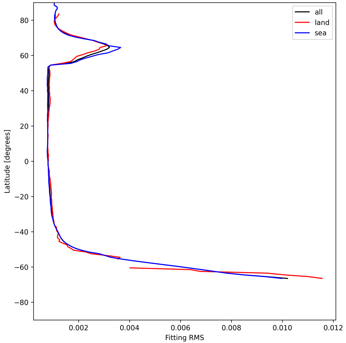
Figure 22: Zonal average of “Fitting RMS” for 2025-07-11 to 2025-07-11.
