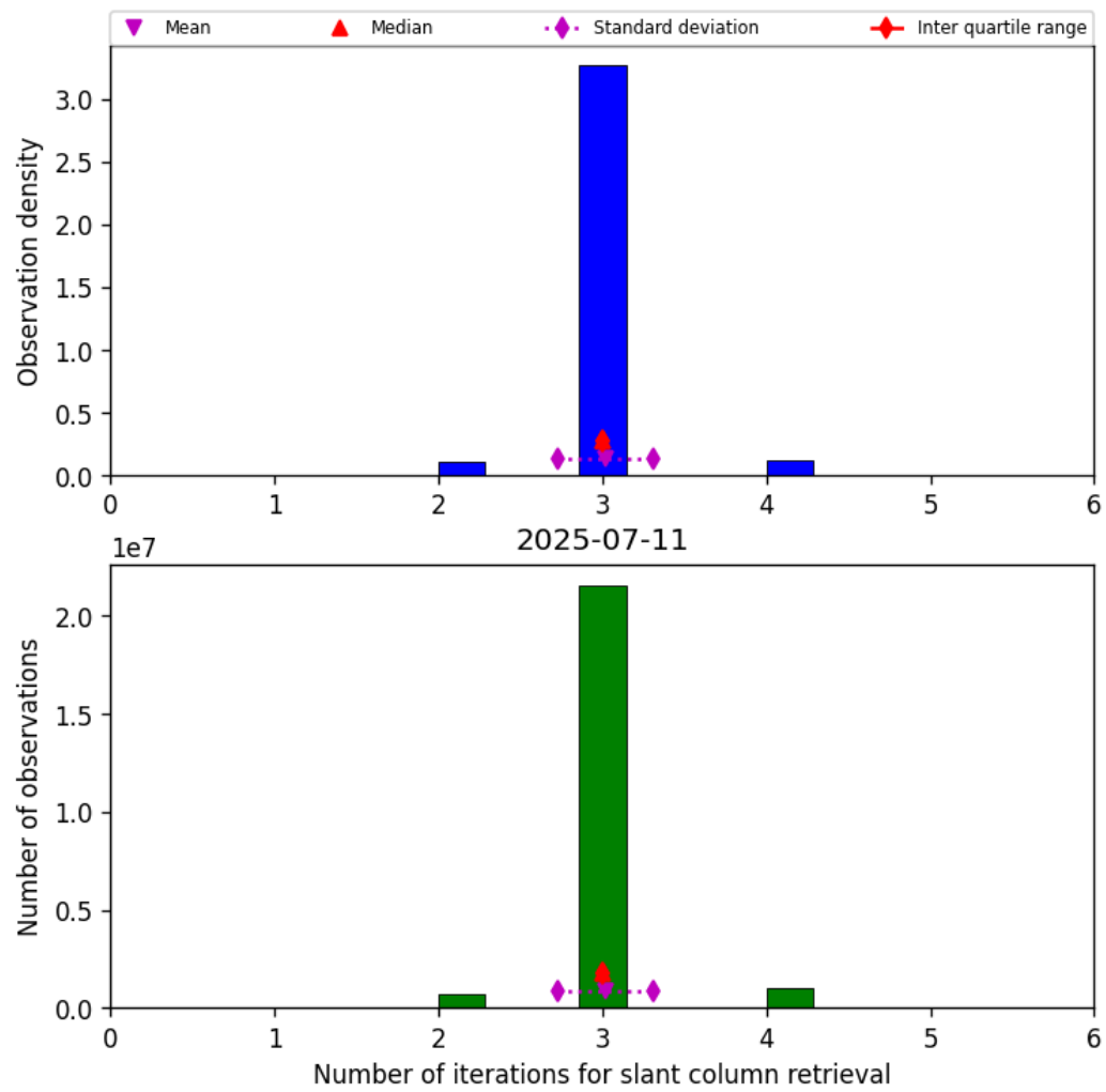
Figure 33: Histogram of “Number of iterations for slant column retrieval” for 2025-07-11 to 2025-07-11
