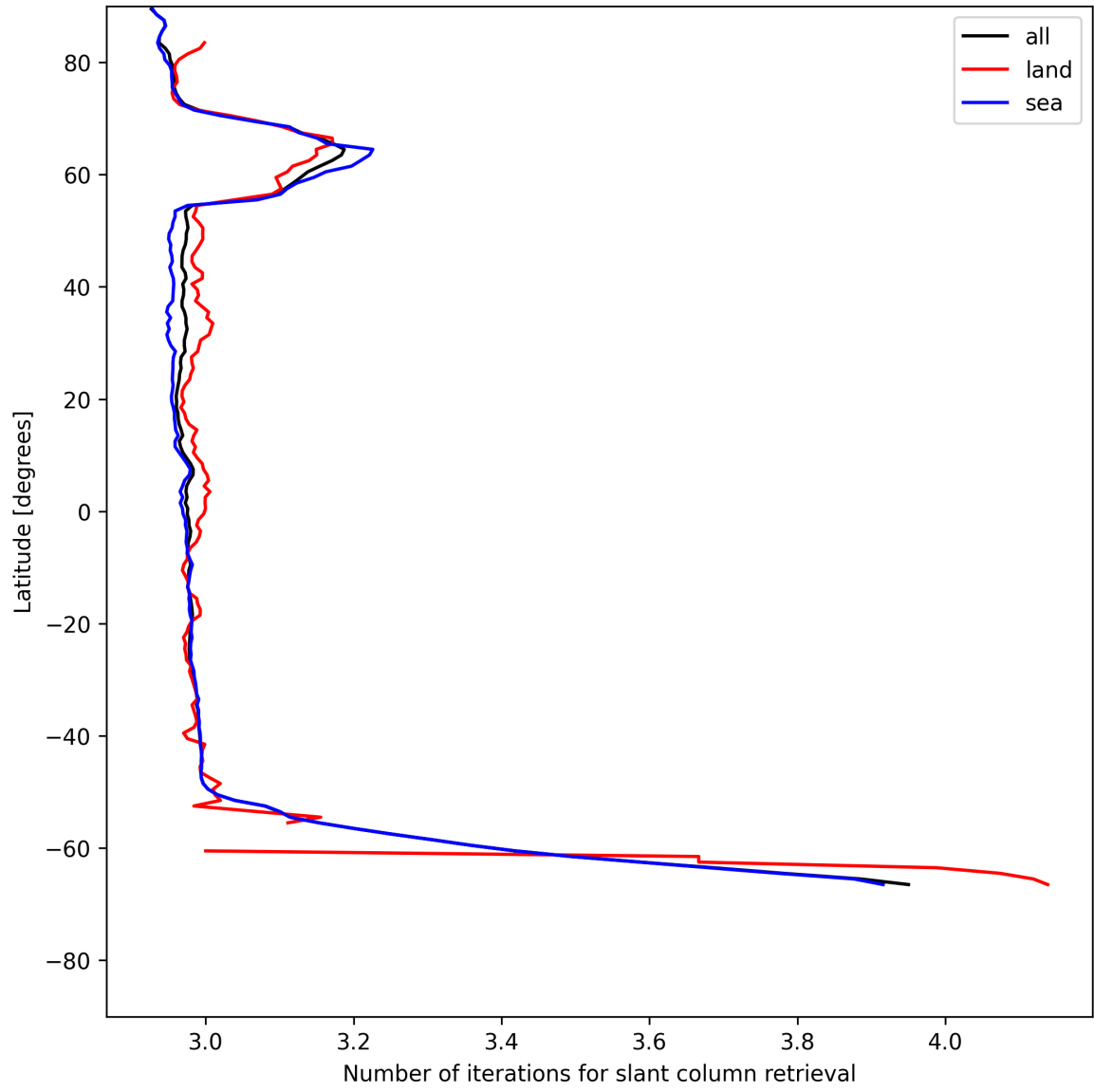
Figure 21: Zonal average of “Number of iterations for slant column retrieval” for 2025-07-11 to 2025-07-11.
