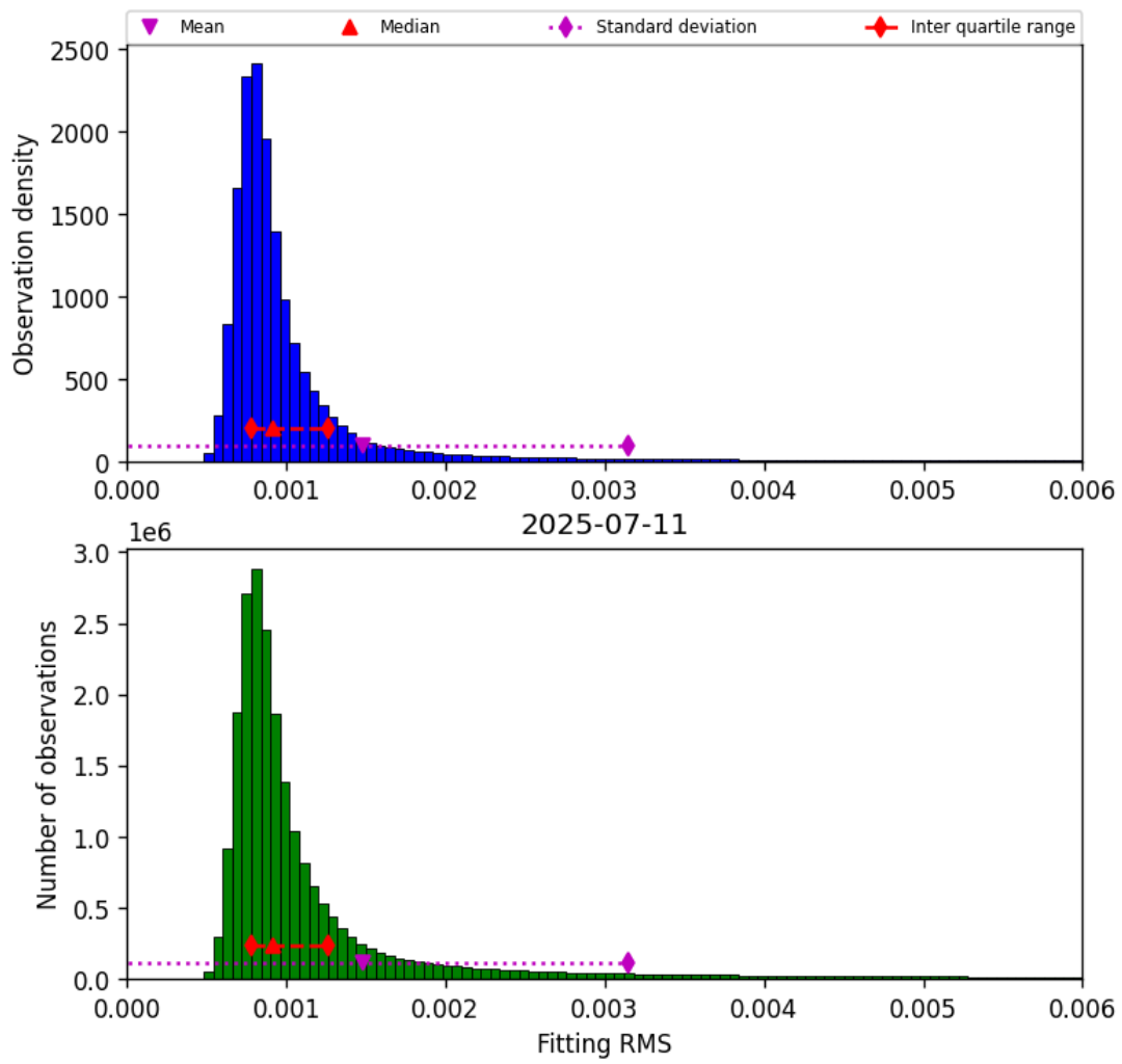
Figure 34: Histogram of “Fitting RMS” for 2025-07-11 to 2025-07-11
