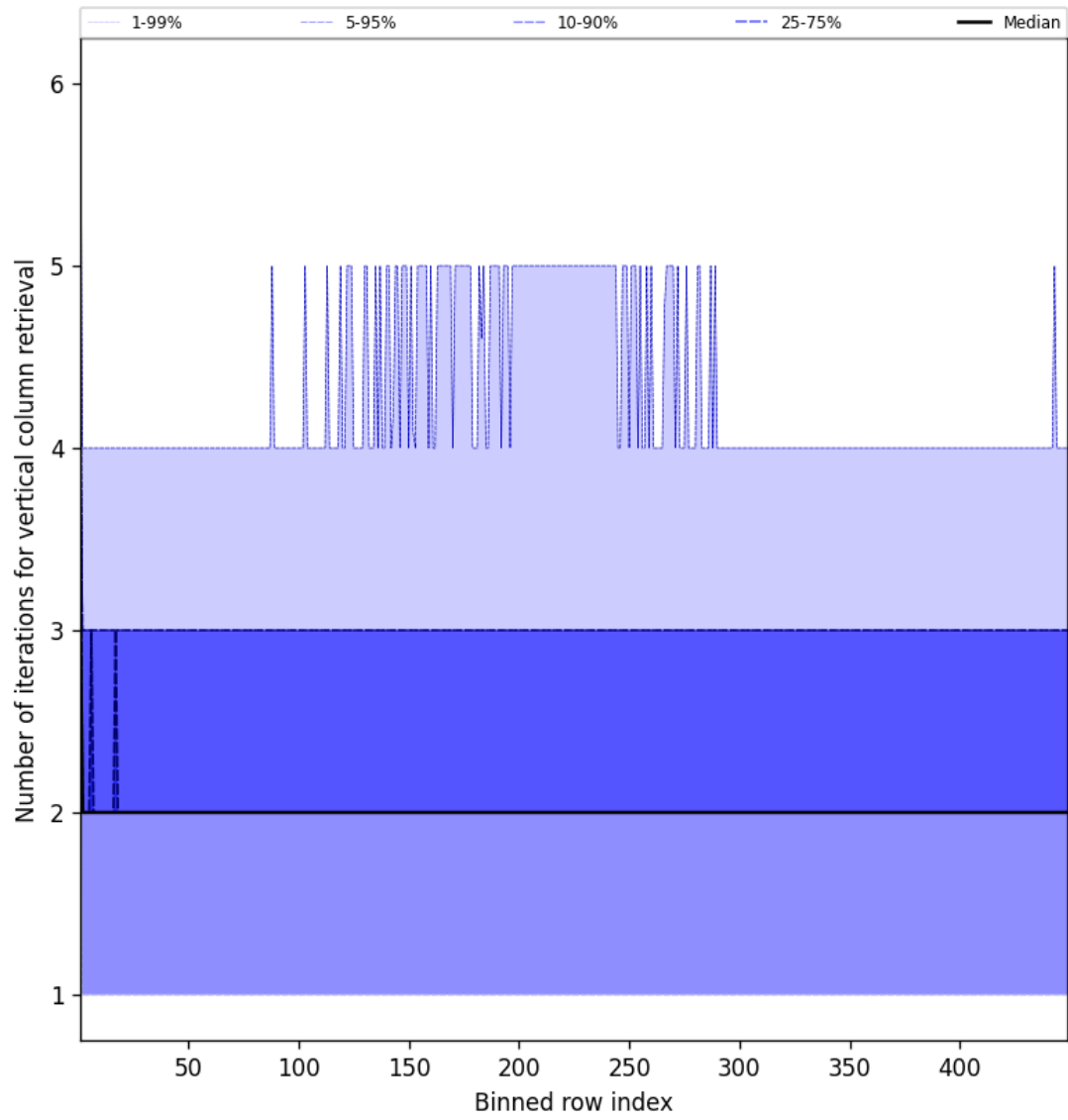
Figure 51: Along track statistics of “Number of iterations for vertical column retrieval” for 2025-07-11 to 2025-07-11
