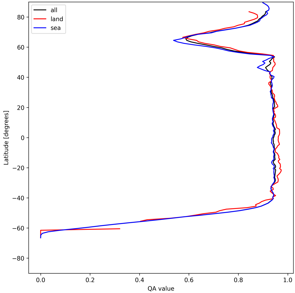
Figure 16: Zonal average of “QA value” for 2025-07-11 to 2025-07-11.
