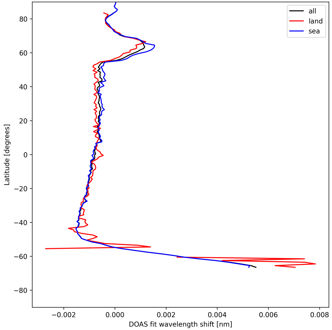
Figure 23: Zonal average of “DOAS fit wavelength shift” for 2025-07-11 to 2025-07-11.
