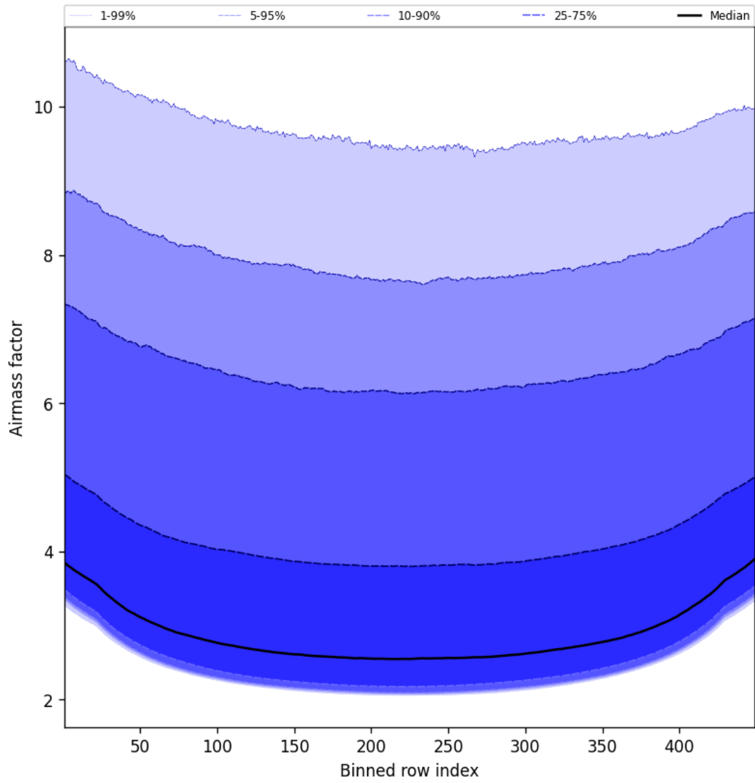
Figure 49: Along track statistics of “Airmass factor” for 2025-07-11 to 2025-07-11
