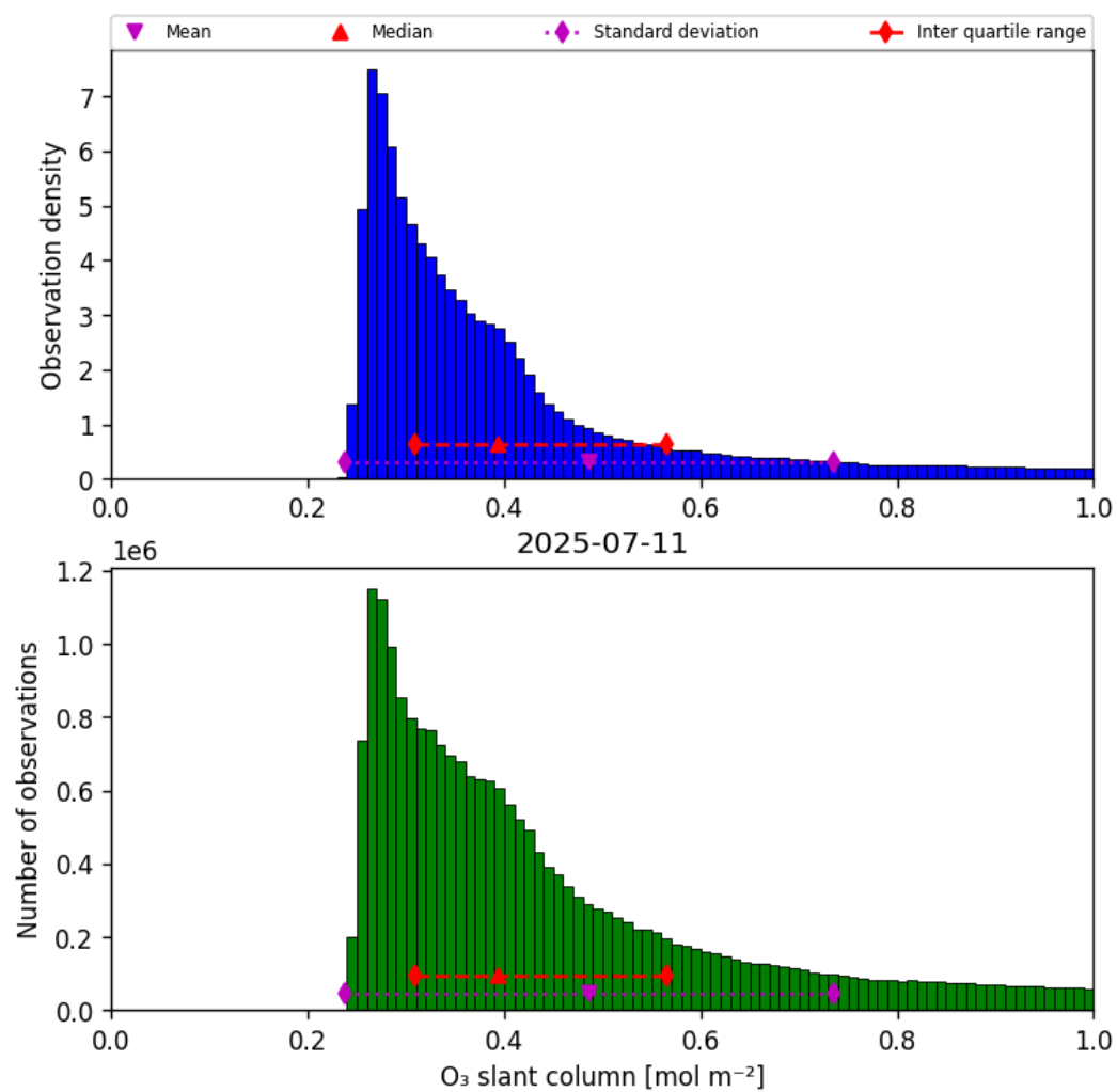
Figure 31: Histogram of “O 3 slant column” for 2025-07-11 to 2025-07-11
