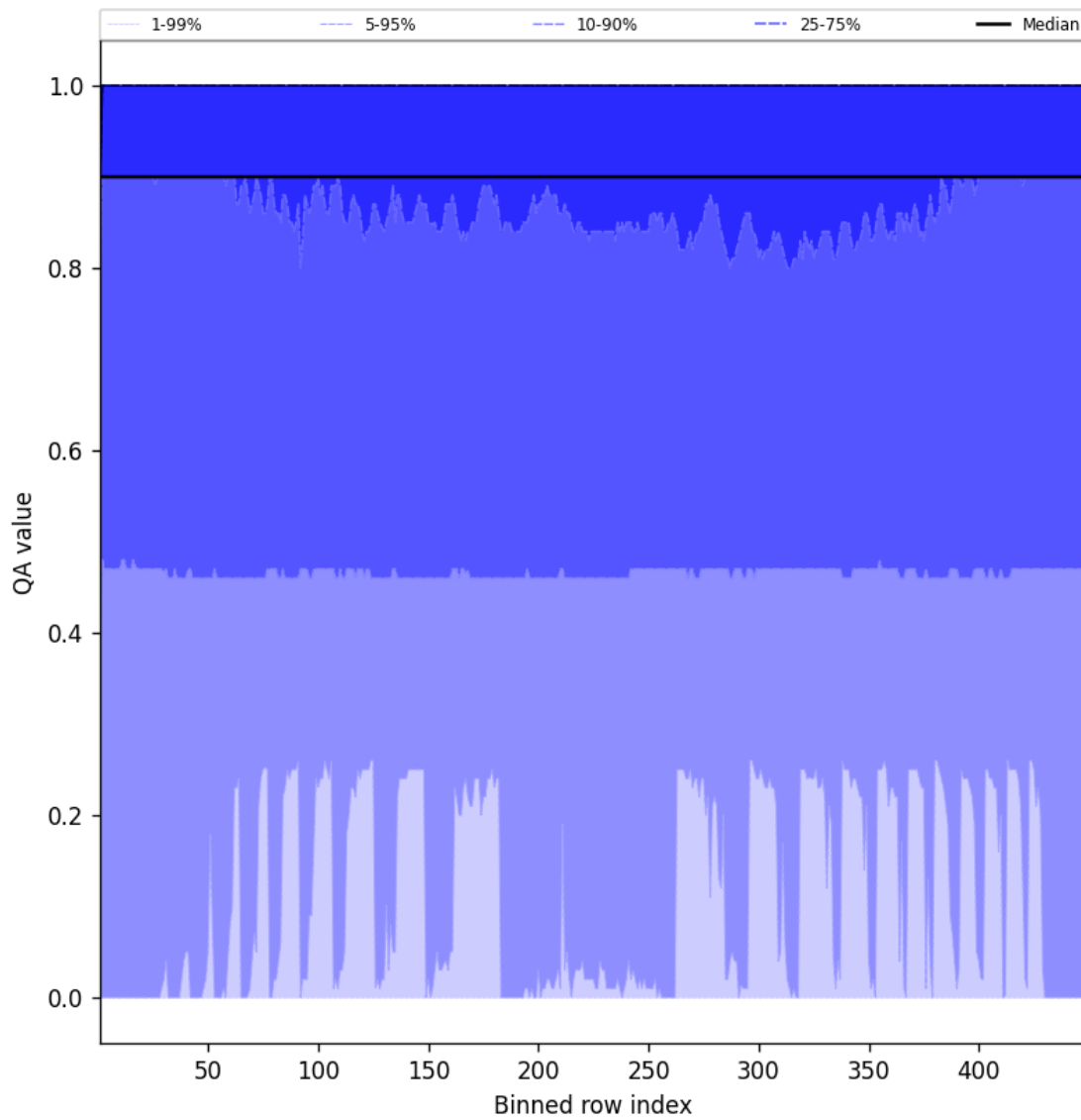
Figure 40: Along track statistics of “QA value” for 2025-07-11 to 2025-07-11
