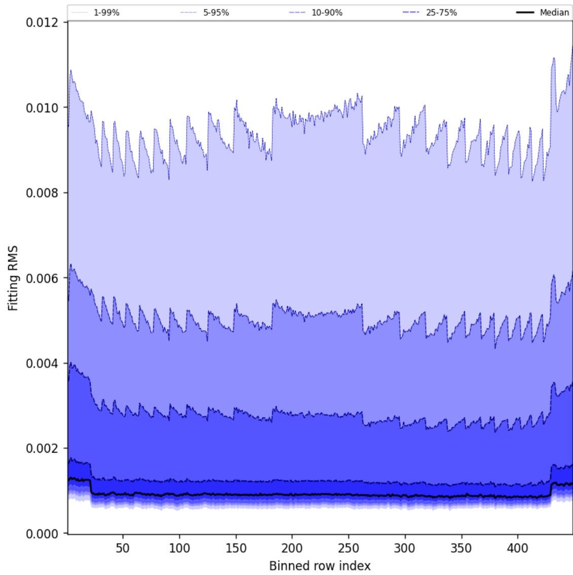
Figure 46: Along track statistics of “Fitting RMS” for 2025-07-11 to 2025-07-11
