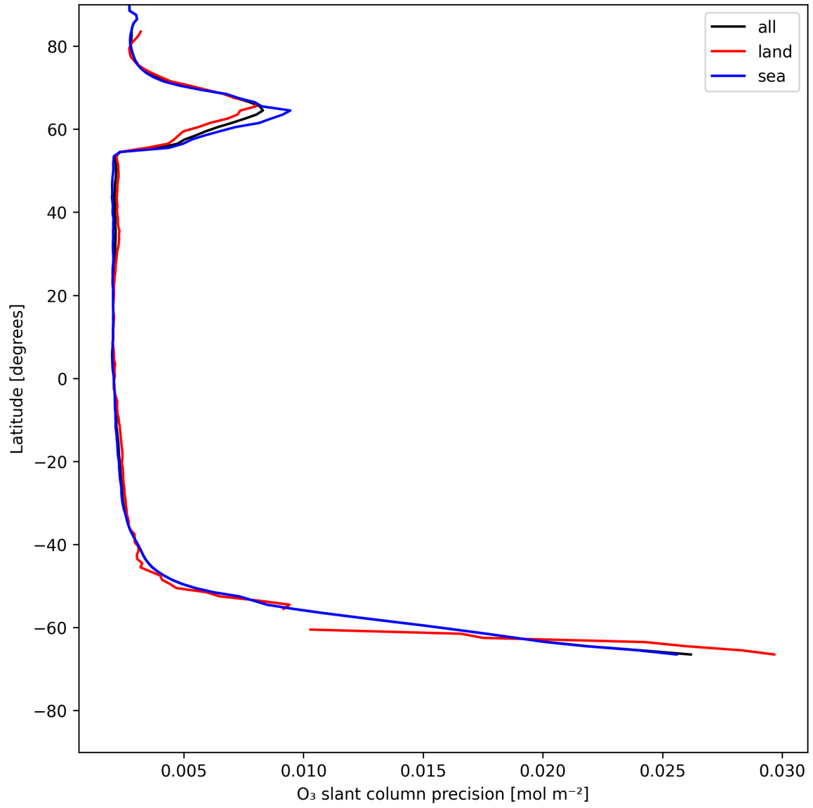
Figure 20: Zonal average of “O 3 slant column precision” for 2025-07-11 to 2025-07-11.
