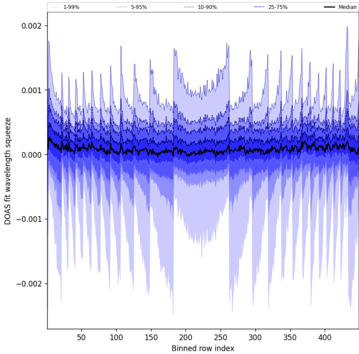
Figure 48: Along track statistics of “DOAS fit wavelength squeeze” for 2025-07-11 to 2025-07-11
