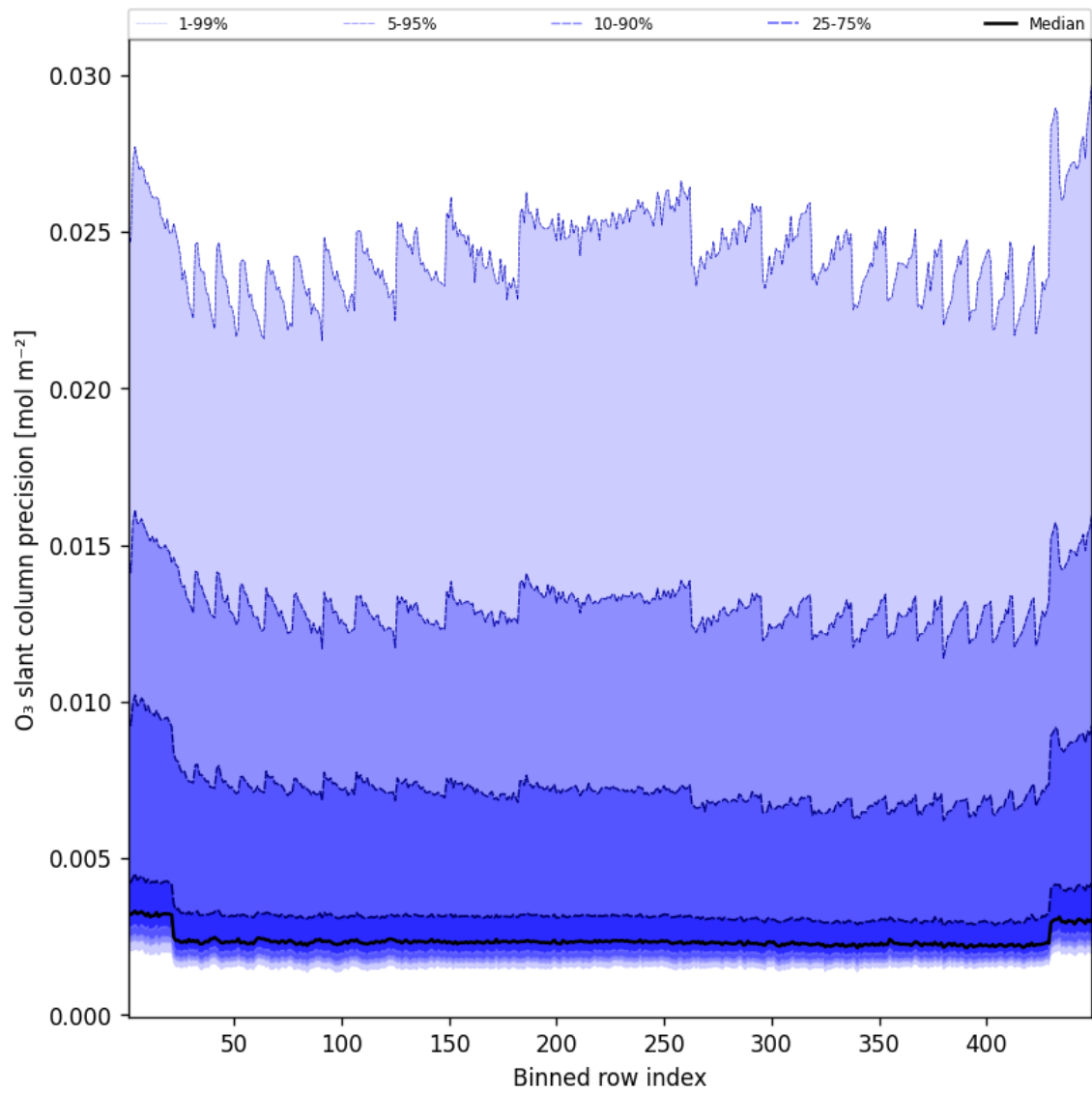
Figure 44: Along track statistics of “O 3 slant column precision” for 2025-07-11 to 2025-07-11
