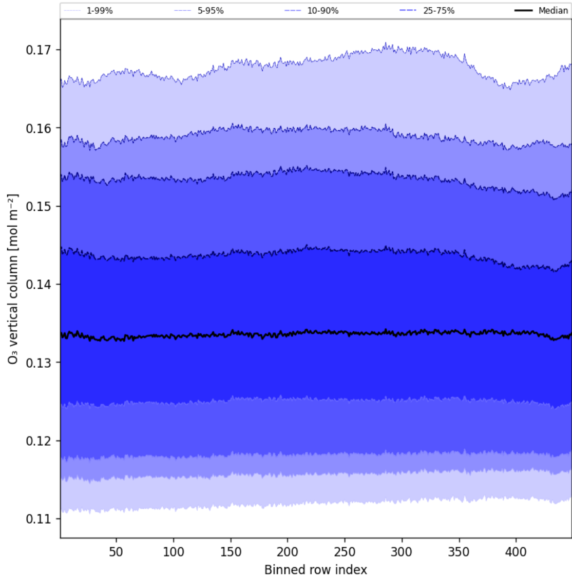
Figure 41: Along track statistics of “O 3 vertical column” for 2025-07-11 to 2025-07-11
