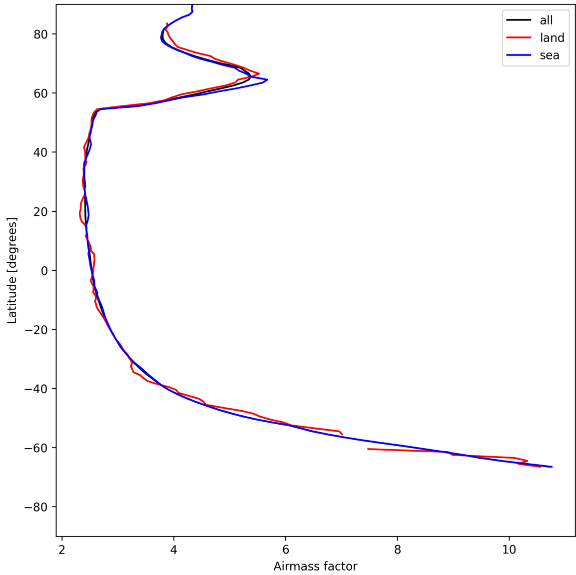
Figure 25: Zonal average of “Airmass factor” for 2025-07-11 to 2025-07-11.
