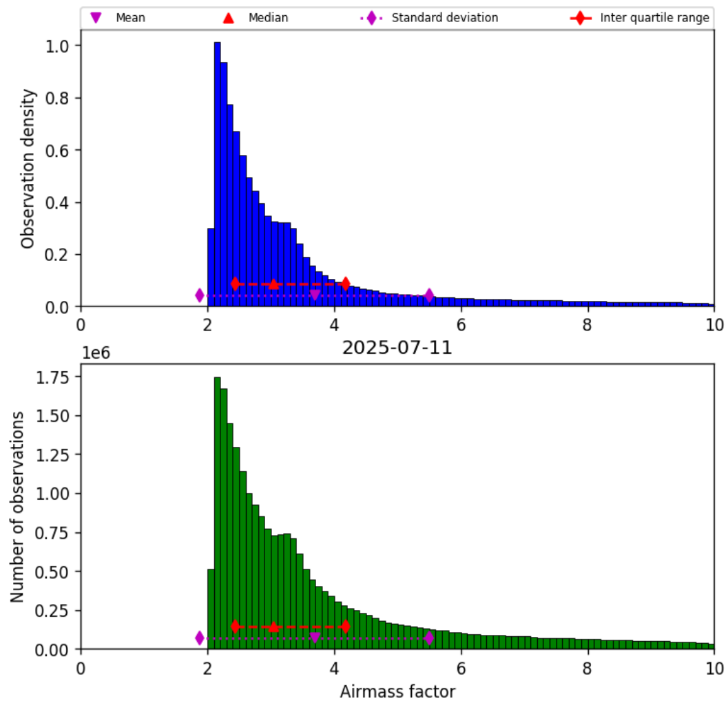
Figure 37: Histogram of “Airmass factor” for 2025-07-11 to 2025-07-11
