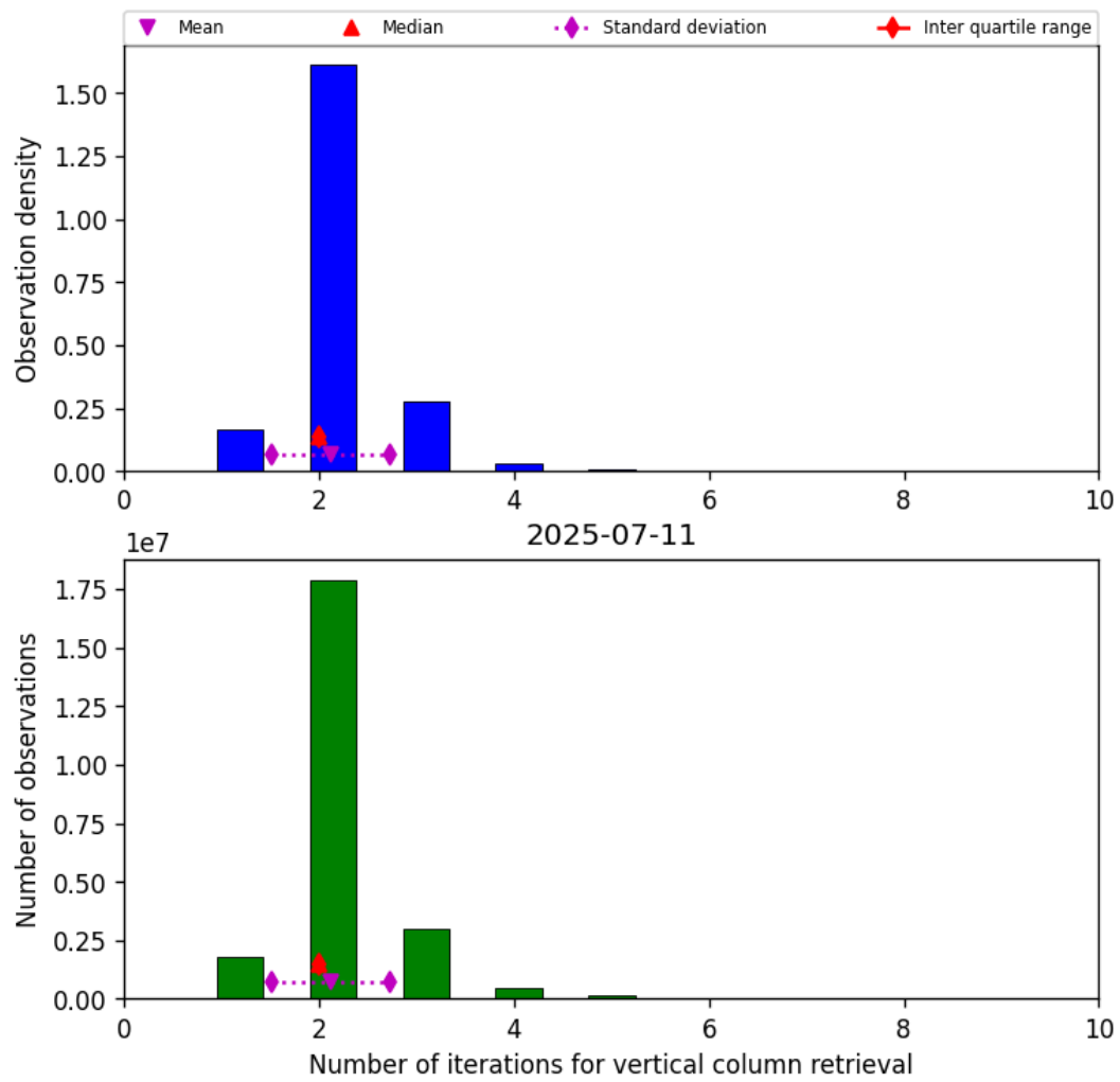
Figure 39: Histogram of “Number of iterations for vertical column retrieval” for 2025-07-11 to 2025-07-11
