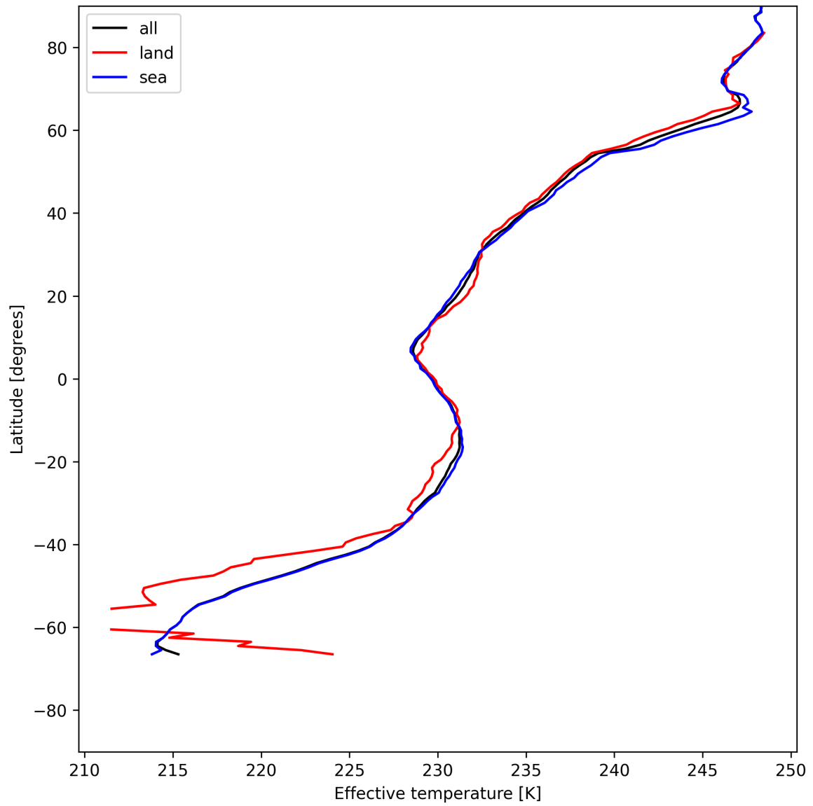
Figure 26: Zonal average of "Effective temperature" for 2025-07-11 to 2025-07-11.
