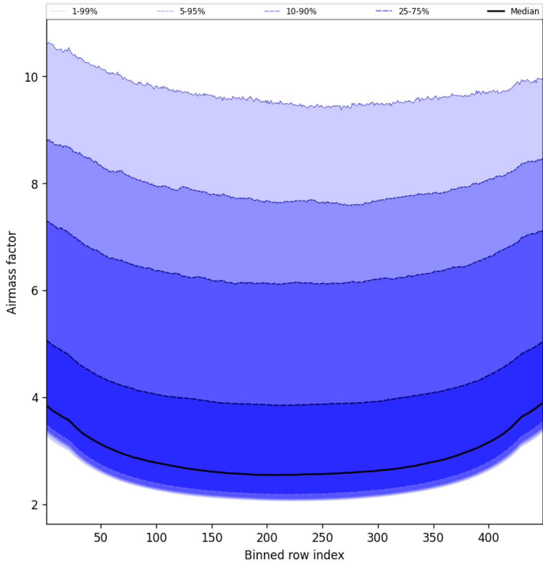
Figure 49: Along track statistics of “Airmass factor” for 2025-07-12 to 2025-07-13
