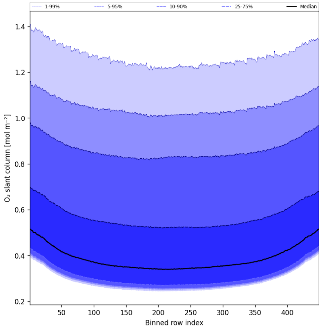
Figure 43: Along track statistics of “O 3 slant column” for 2025-07-12 to 2025-07-13
