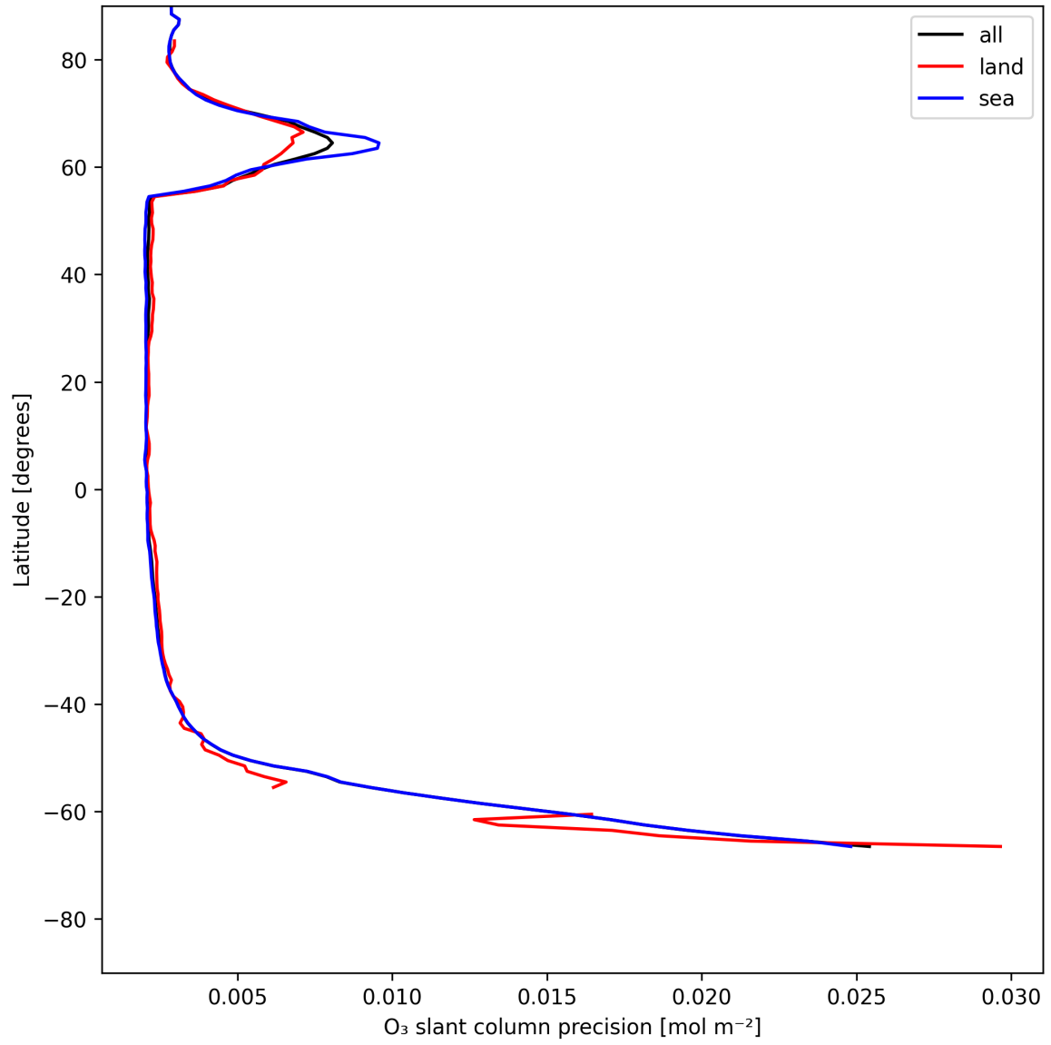
Figure 20: Zonal average of "O 3 slant column precision" for 2025-07-12 to 2025-07-13.
