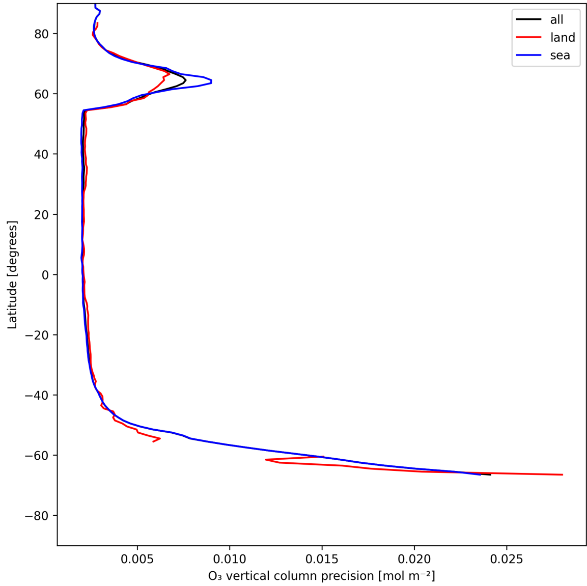
Figure 18: Zonal average of “O 3 vertical column precision” for 2025-07-12 to 2025-07-13.
