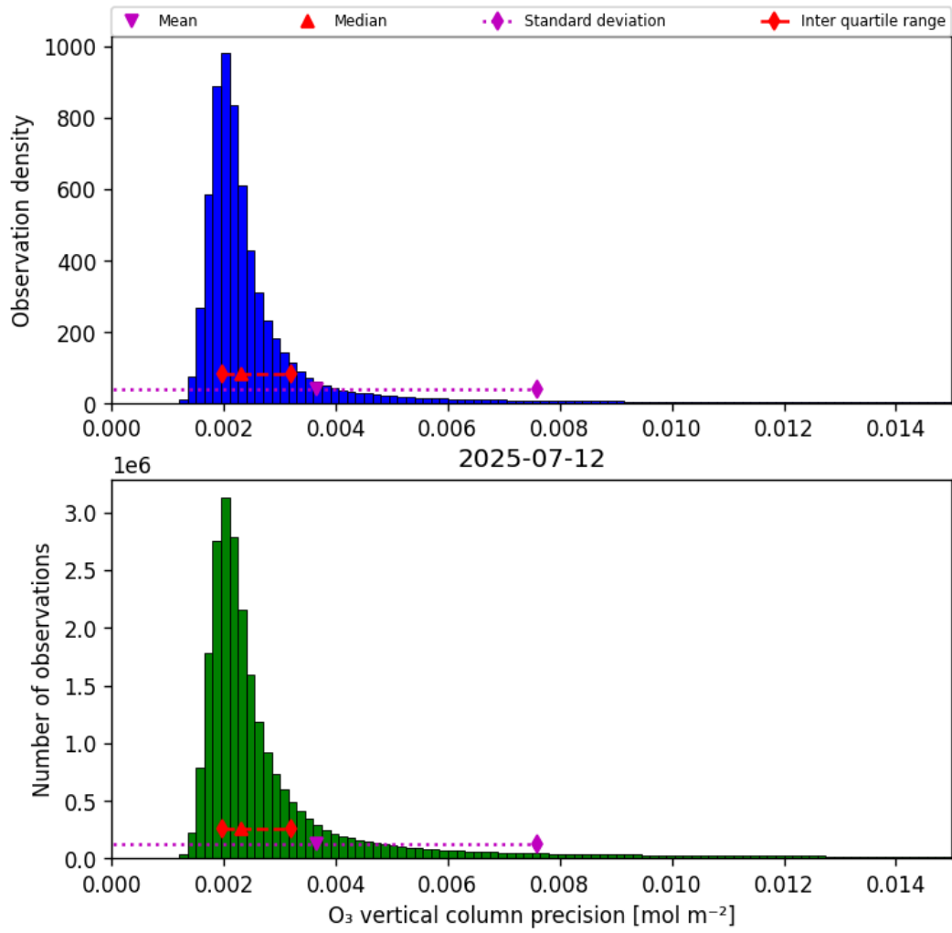
Figure 30: Histogram of "O 3 vertical column precision" for 2025-07-12 to 2025-07-13
