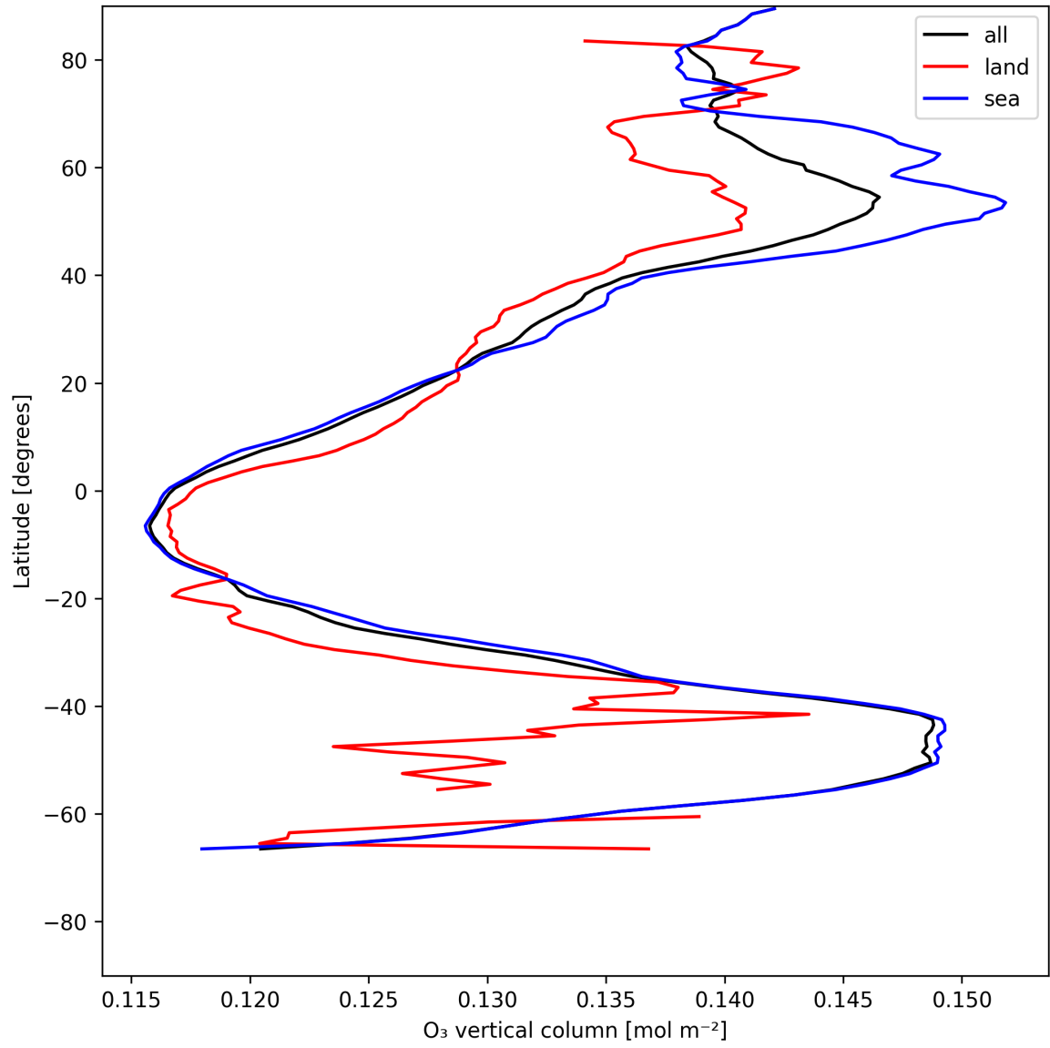
Figure 17: Zonal average of “O 3 vertical column” for 2025-07-12 to 2025-07-13.
