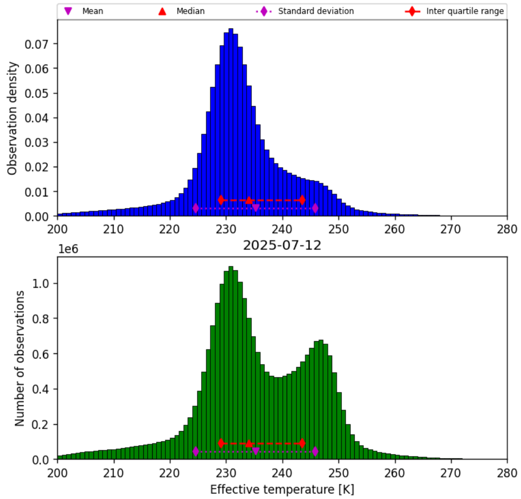
Figure 38: Histogram of “Effective temperature” for 2025-07-12 to 2025-07-13
