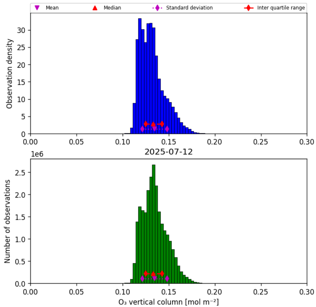
Figure 29: Histogram of “O 3 vertical column” for 2025-07-12 to 2025-07-13
