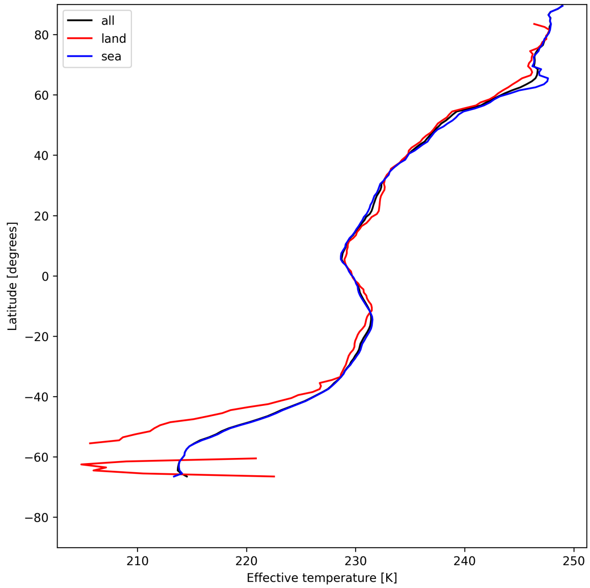
Figure 26: Zonal average of "Effective temperature" for 2025-07-12 to 2025-07-13.
