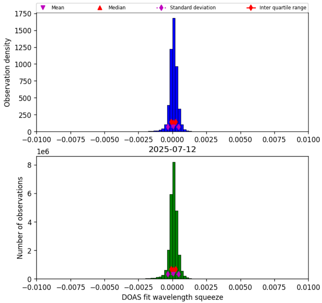
Figure 36: Histogram of “DOAS fit wavelength squeeze” for 2025-07-12 to 2025-07-13
