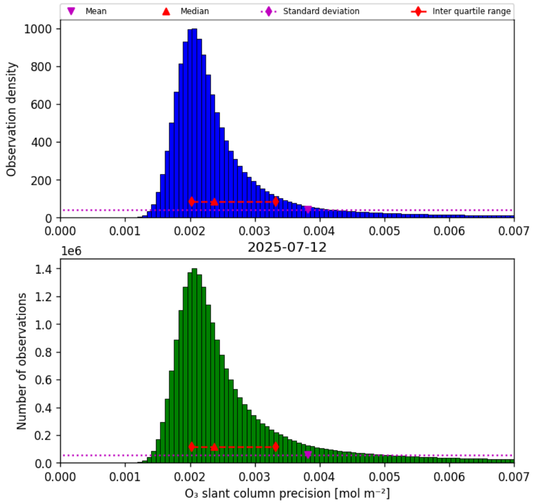
Figure 32: Histogram of “O 3 slant column precision” for 2025-07-12 to 2025-07-13
