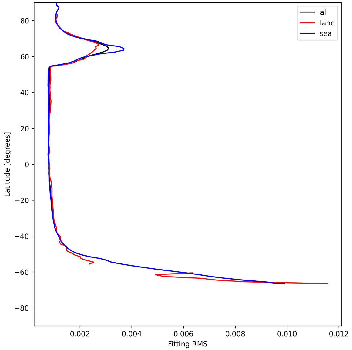
Figure 22: Zonal average of “Fitting RMS” for 2025-07-12 to 2025-07-13.
