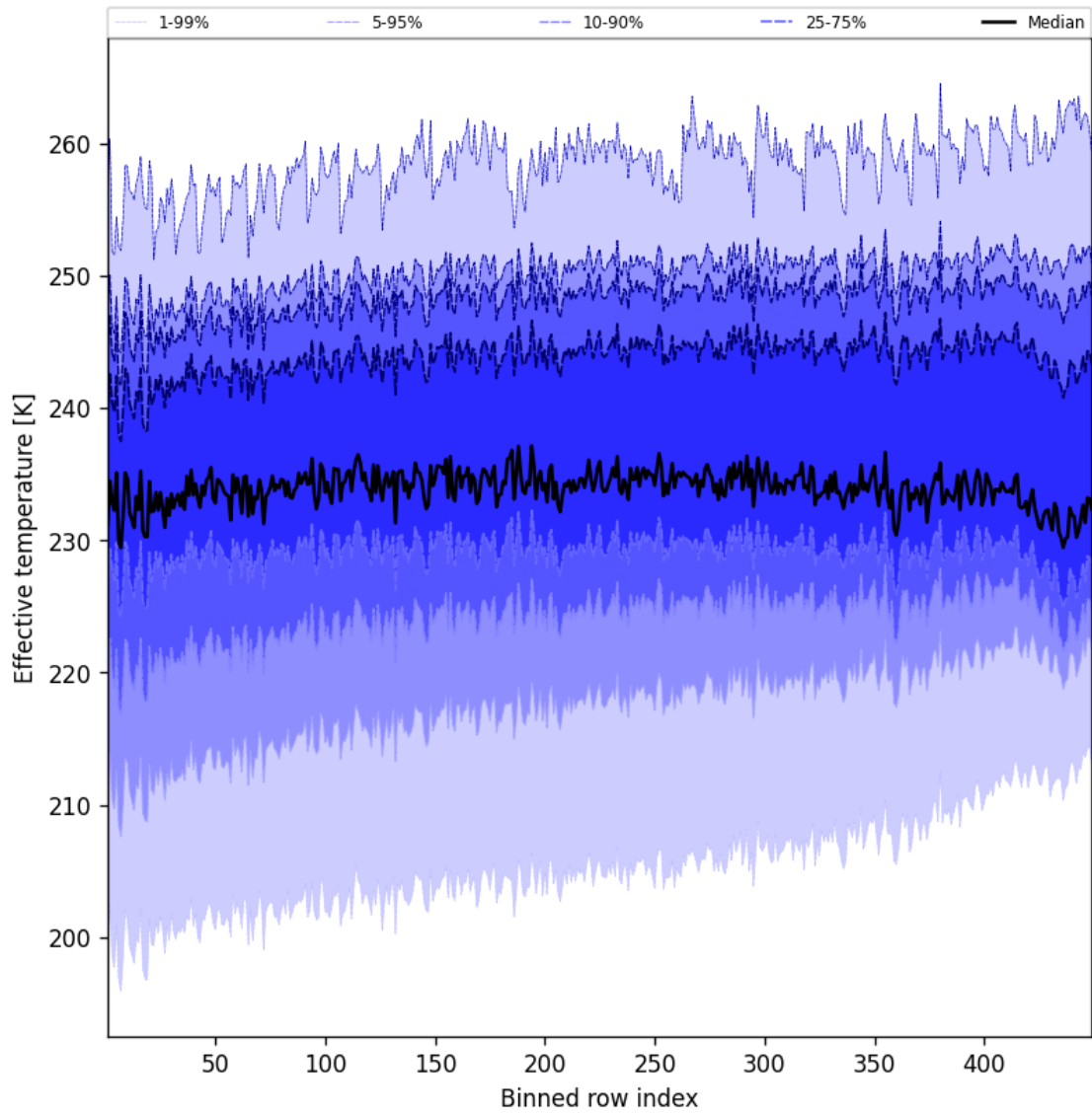
Figure 50: Along track statistics of “Effective temperature” for 2025-07-12 to 2025-07-13
