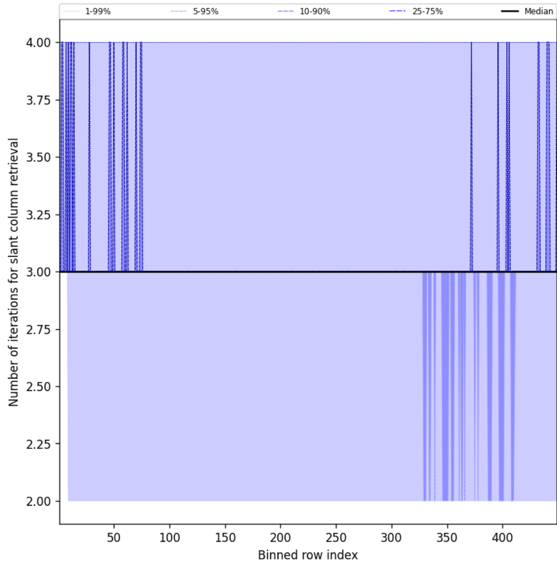
Figure 45: Along track statistics of “Number of iterations for slant column retrieval” for 2025-07-12 to 2025-07-13
