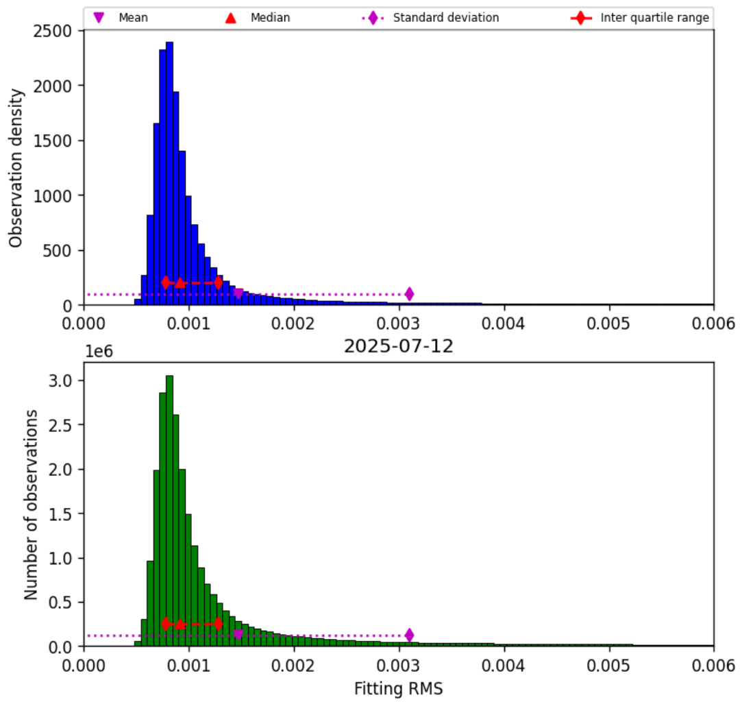
Figure 34: Histogram of “Fitting RMS” for 2025-07-12 to 2025-07-13
