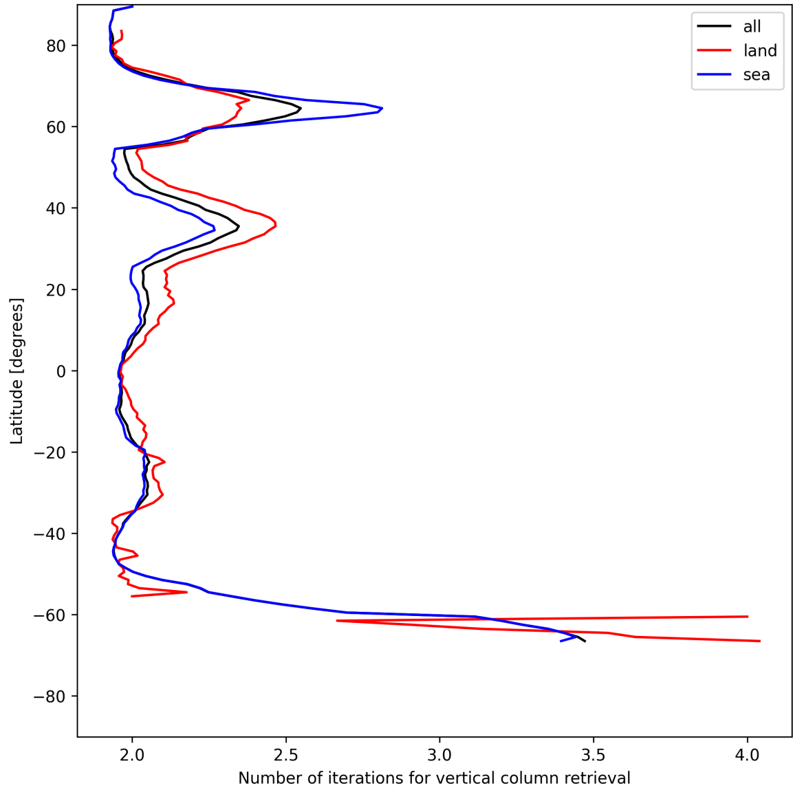
Figure 27: Zonal average of “Number of iterations for vertical column retrieval” for 2025-07-12 to 2025-07-13.
