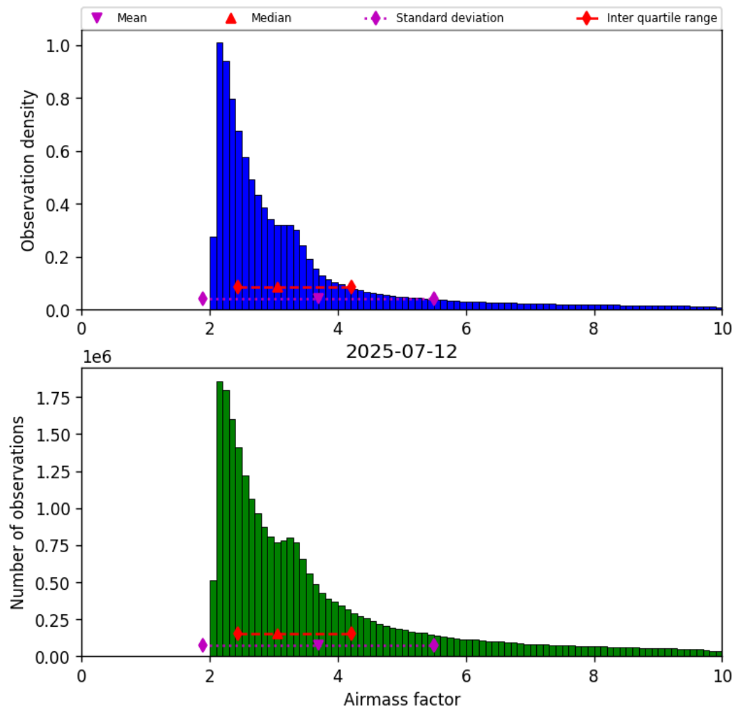
Figure 37: Histogram of “Airmass factor” for 2025-07-12 to 2025-07-13
