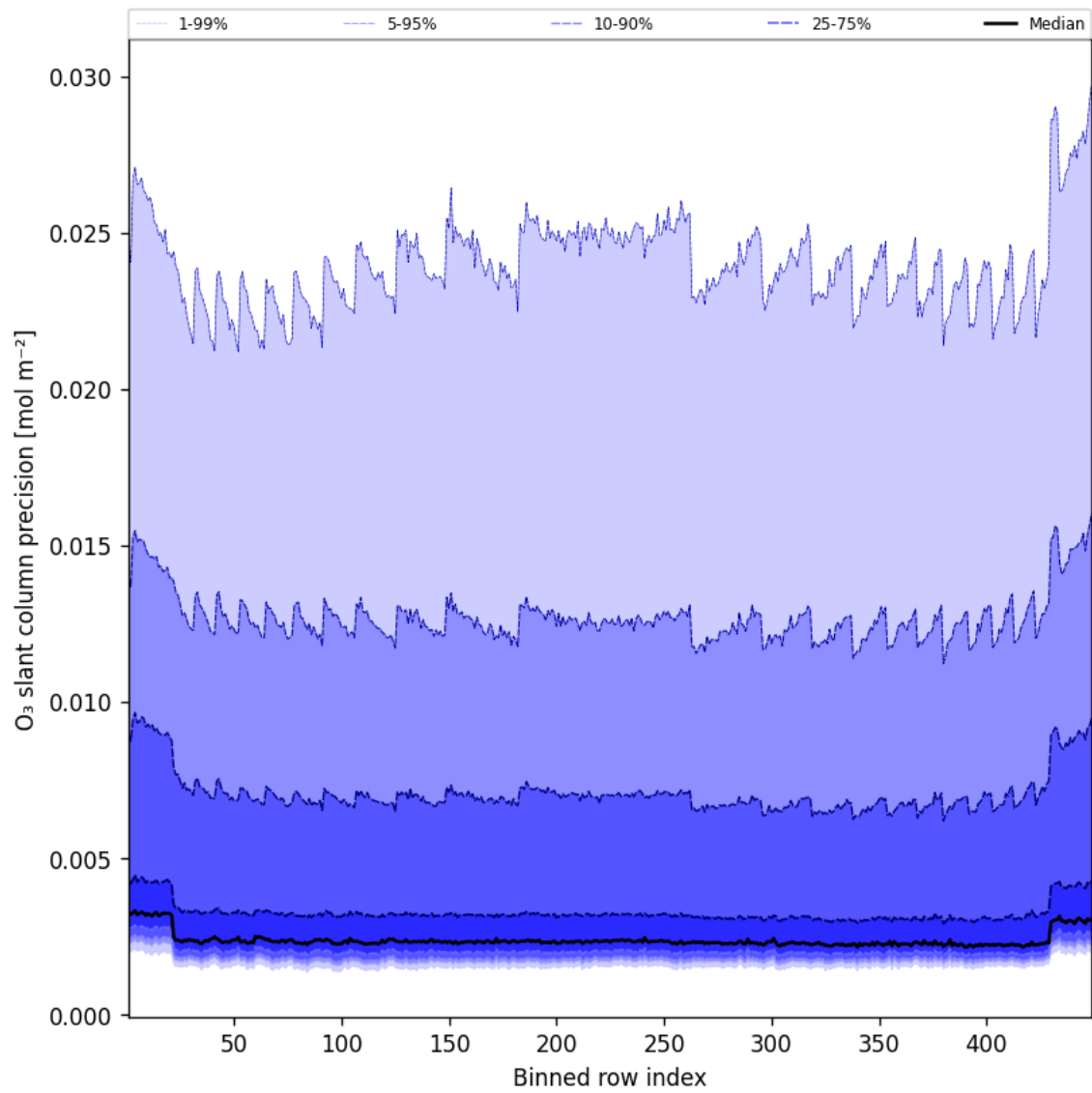
Figure 44: Along track statistics of “O 3 slant column precision” for 2025-07-12 to 2025-07-13
