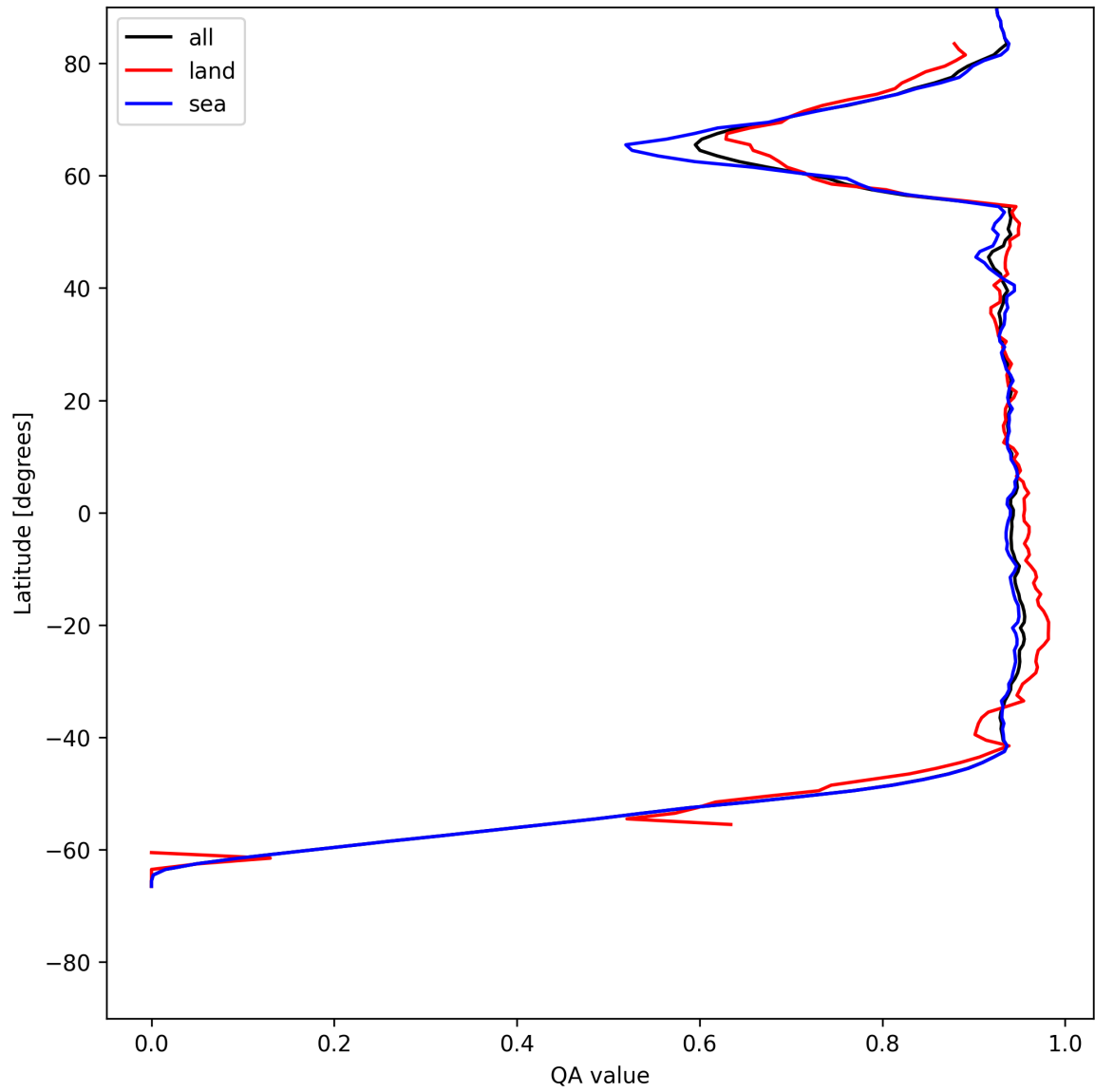
Figure 16: Zonal average of “QA value” for 2025-07-12 to 2025-07-13.
