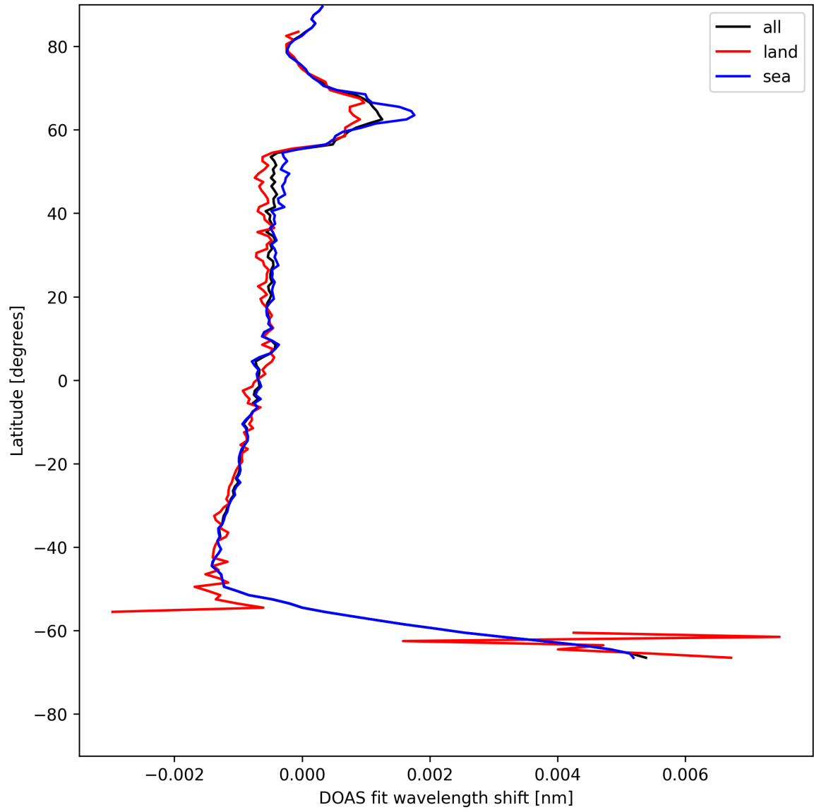
Figure 23: Zonal average of “DOAS fit wavelength shift” for 2025-07-12 to 2025-07-13.
