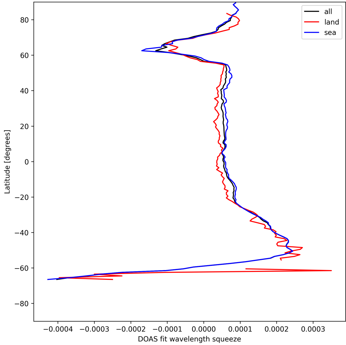
Figure 24: Zonal average of “DOAS fit wavelength squeeze” for 2025-07-12 to 2025-07-13.
