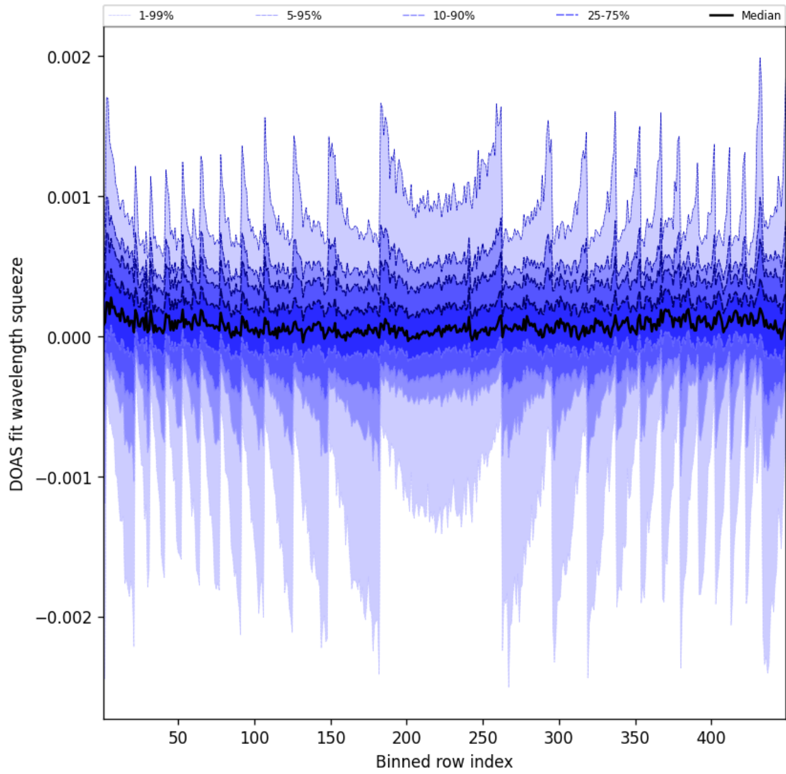
Figure 48: Along track statistics of “DOAS fit wavelength squeeze” for 2025-07-12 to 2025-07-13
