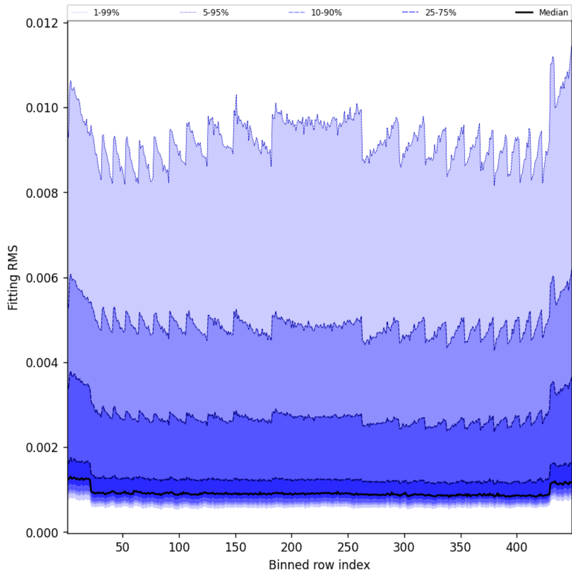
Figure 46: Along track statistics of “Fitting RMS” for 2025-07-12 to 2025-07-13
