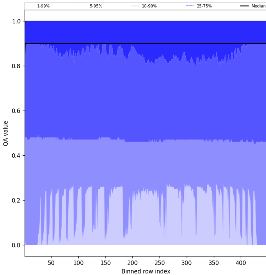
Figure 40: Along track statistics of “QA value” for 2025-07-12 to 2025-07-13
