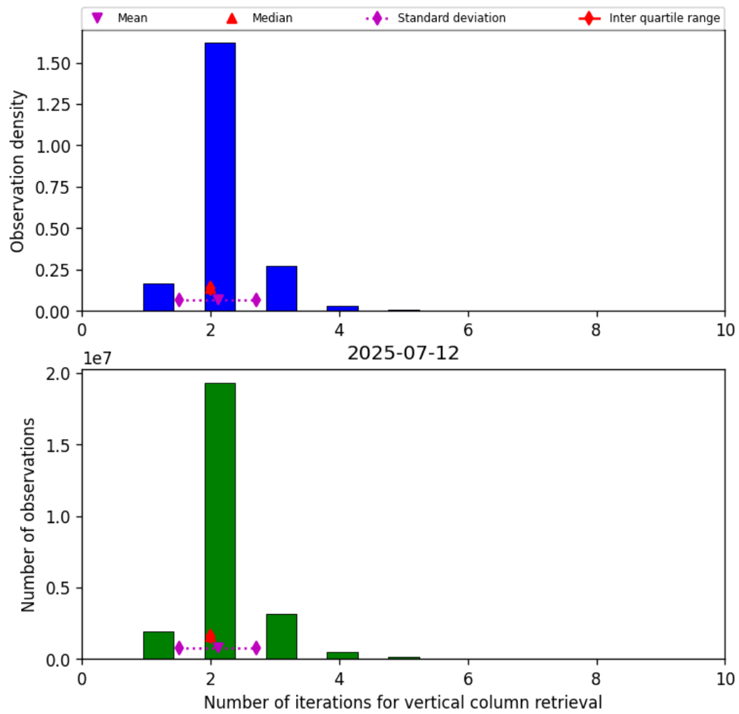
Figure 39: Histogram of “Number of iterations for vertical column retrieval” for 2025-07-12 to 2025-07-13
