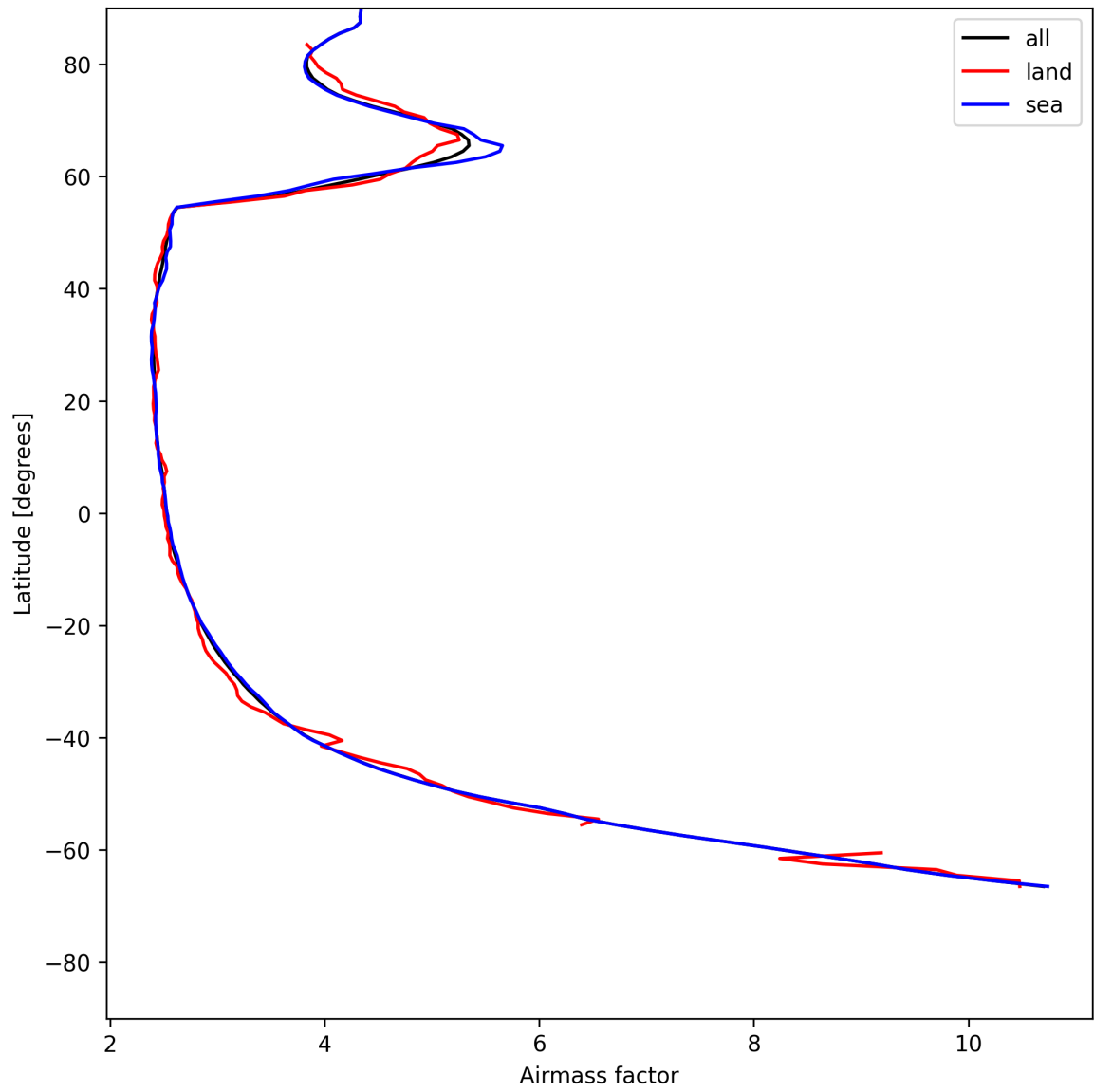
Figure 25: Zonal average of “Airmass factor” for 2025-07-12 to 2025-07-13.
