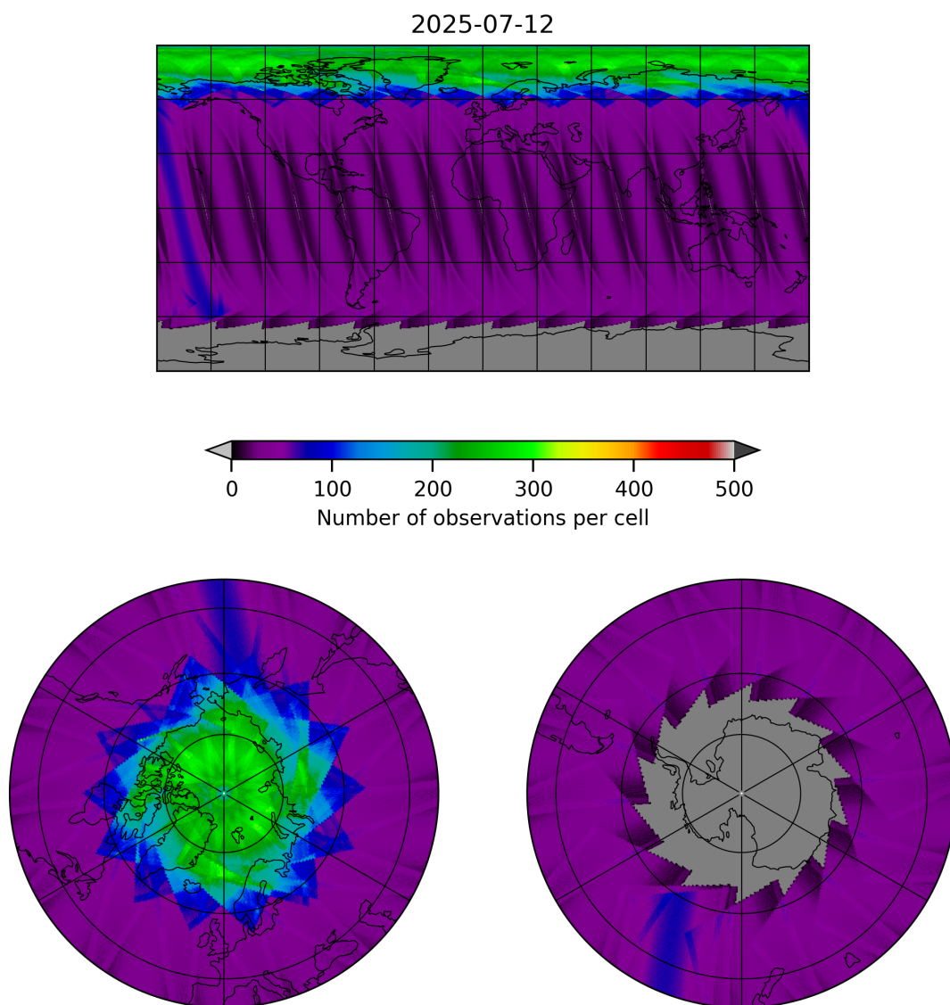
Figure 15: Map of the number of observations for 2025-07-12 to 2025-07-13
