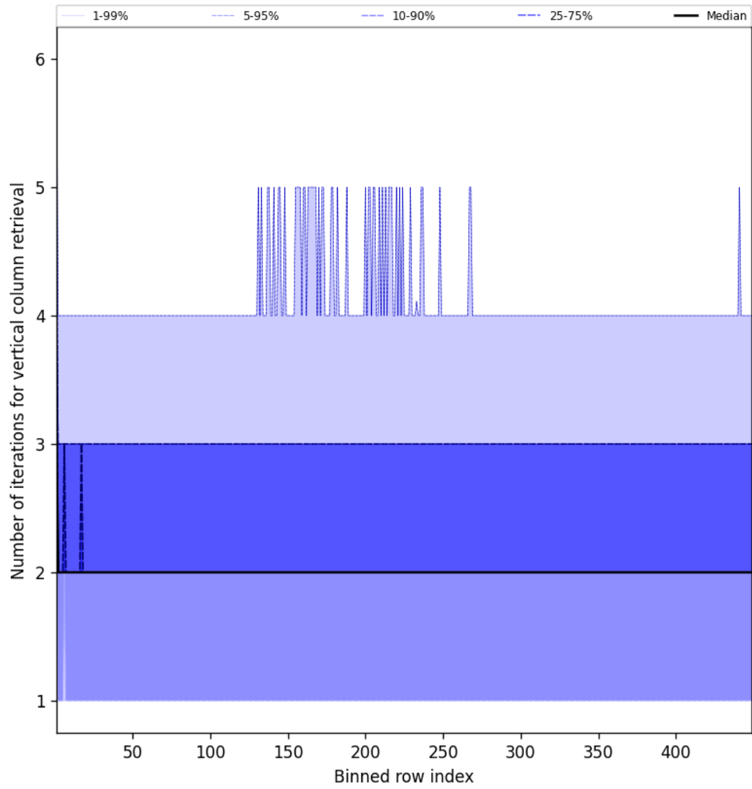
Figure 51: Along track statistics of “Number of iterations for vertical column retrieval” for 2025-07-12 to 2025-07-13
