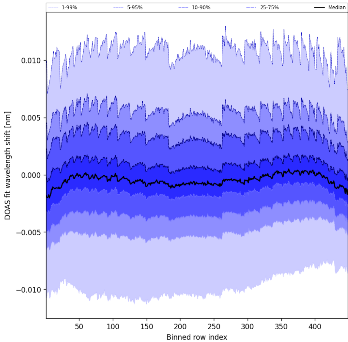
Figure 47: Along track statistics of “DOAS fit wavelength shift” for 2025-07-12 to 2025-07-13
