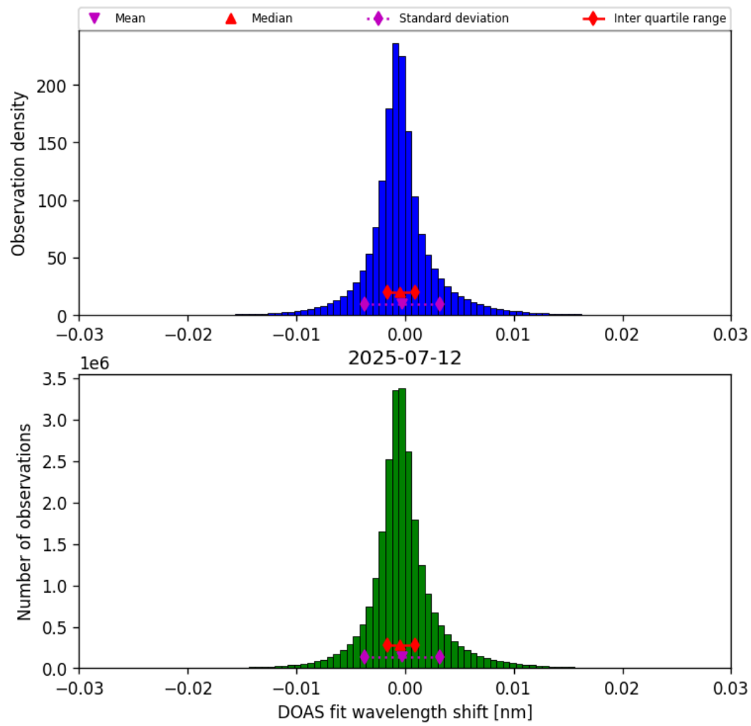
Figure 35: Histogram of “DOAS fit wavelength shift” for 2025-07-12 to 2025-07-13
