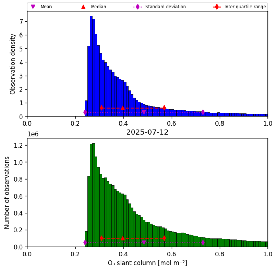
Figure 31: Histogram of “O 3 slant column” for 2025-07-12 to 2025-07-13
