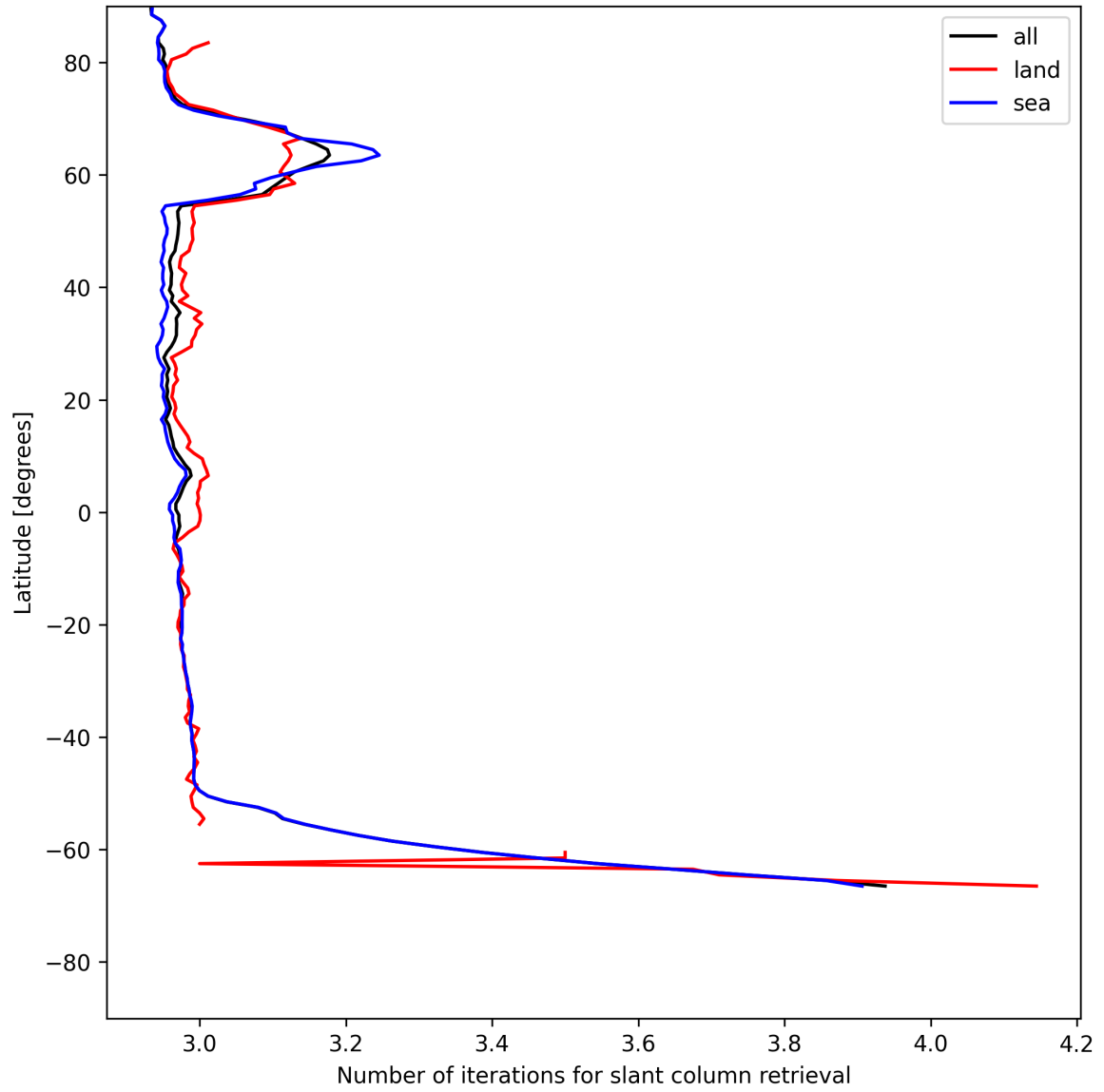
Figure 21: Zonal average of “Number of iterations for slant column retrieval” for 2025-07-12 to 2025-07-13.
