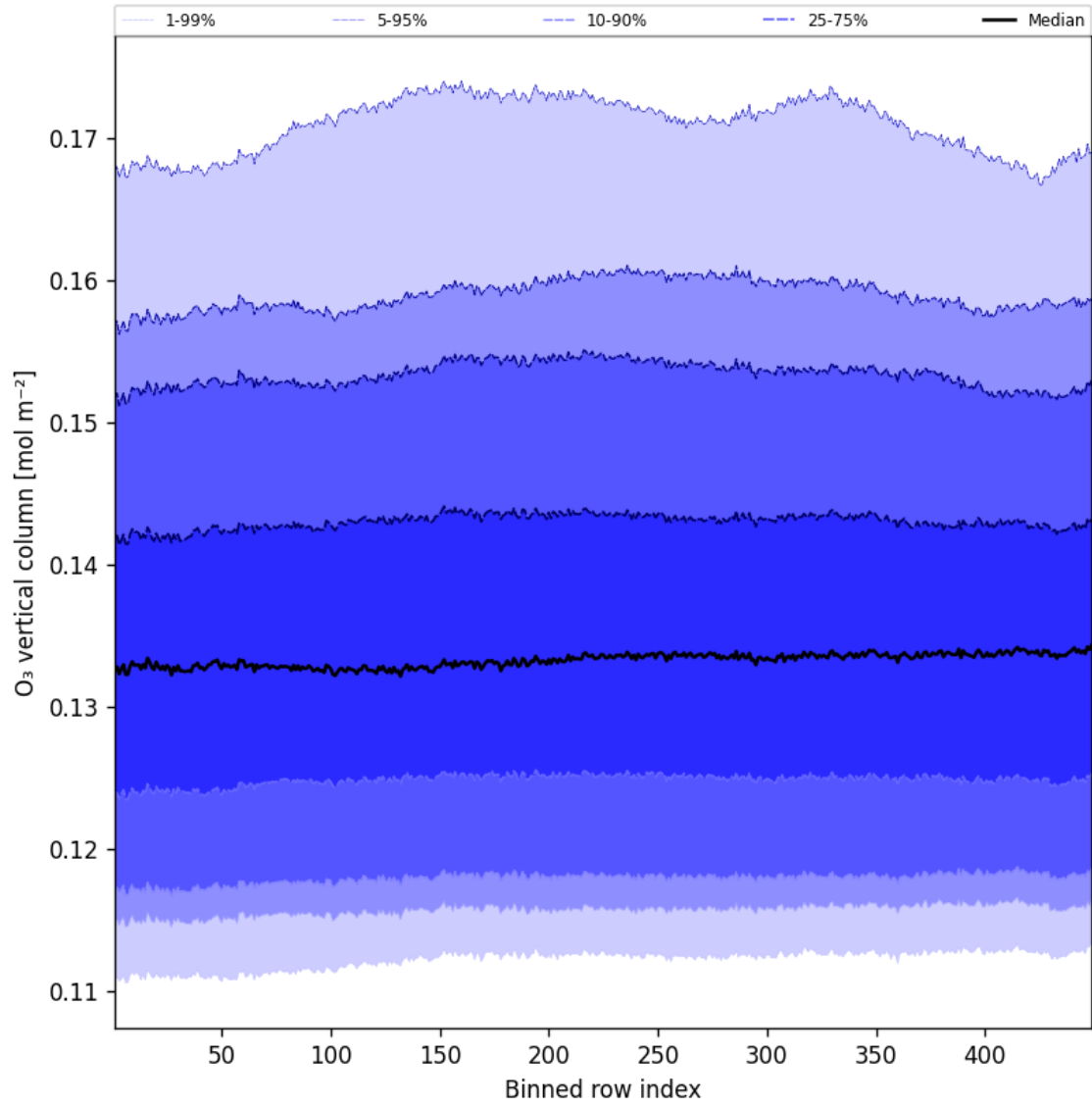
Figure 41: Along track statistics of “O 3 vertical column” for 2025-07-12 to 2025-07-13
