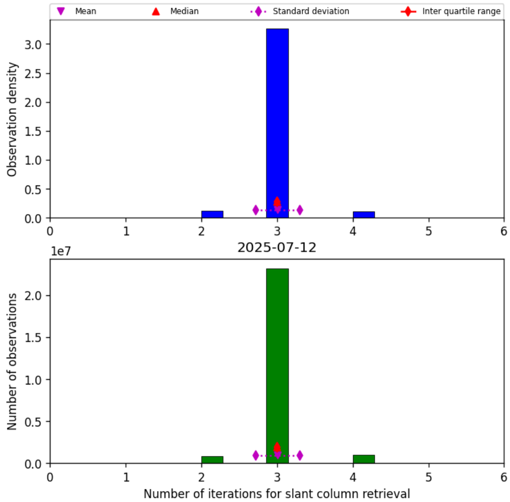
Figure 33: Histogram of “Number of iterations for slant column retrieval” for 2025-07-12 to 2025-07-13
