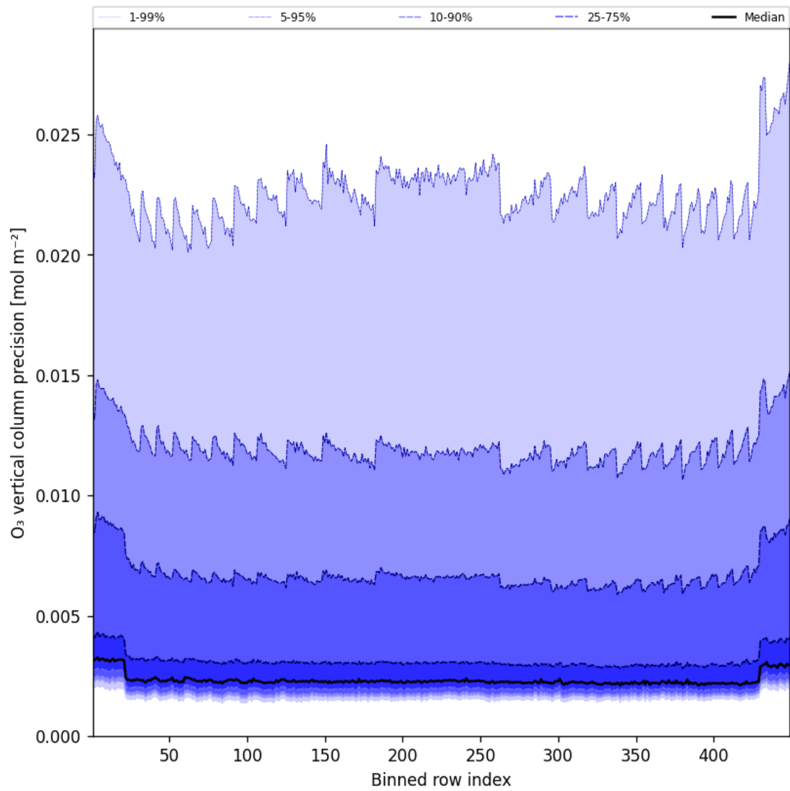
Figure 42: Along track statistics of “O 3 vertical column precision” for 2025-07-12 to 2025-07-13
