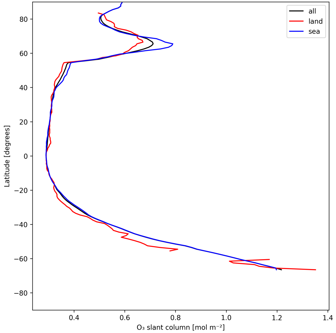
Figure 19: Zonal average of “O 3 slant column” for 2025-07-12 to 2025-07-13.
