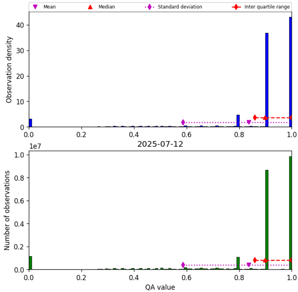
Figure 28: Histogram of “QA value” for 2025-07-12 to 2025-07-13
