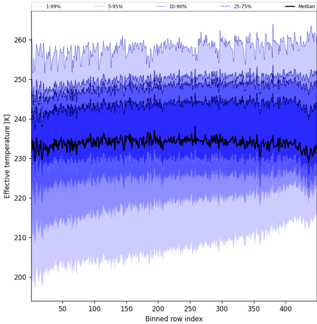
Figure 50: Along track statistics of “Effective temperature” for 2025-07-14 to 2025-07-15
