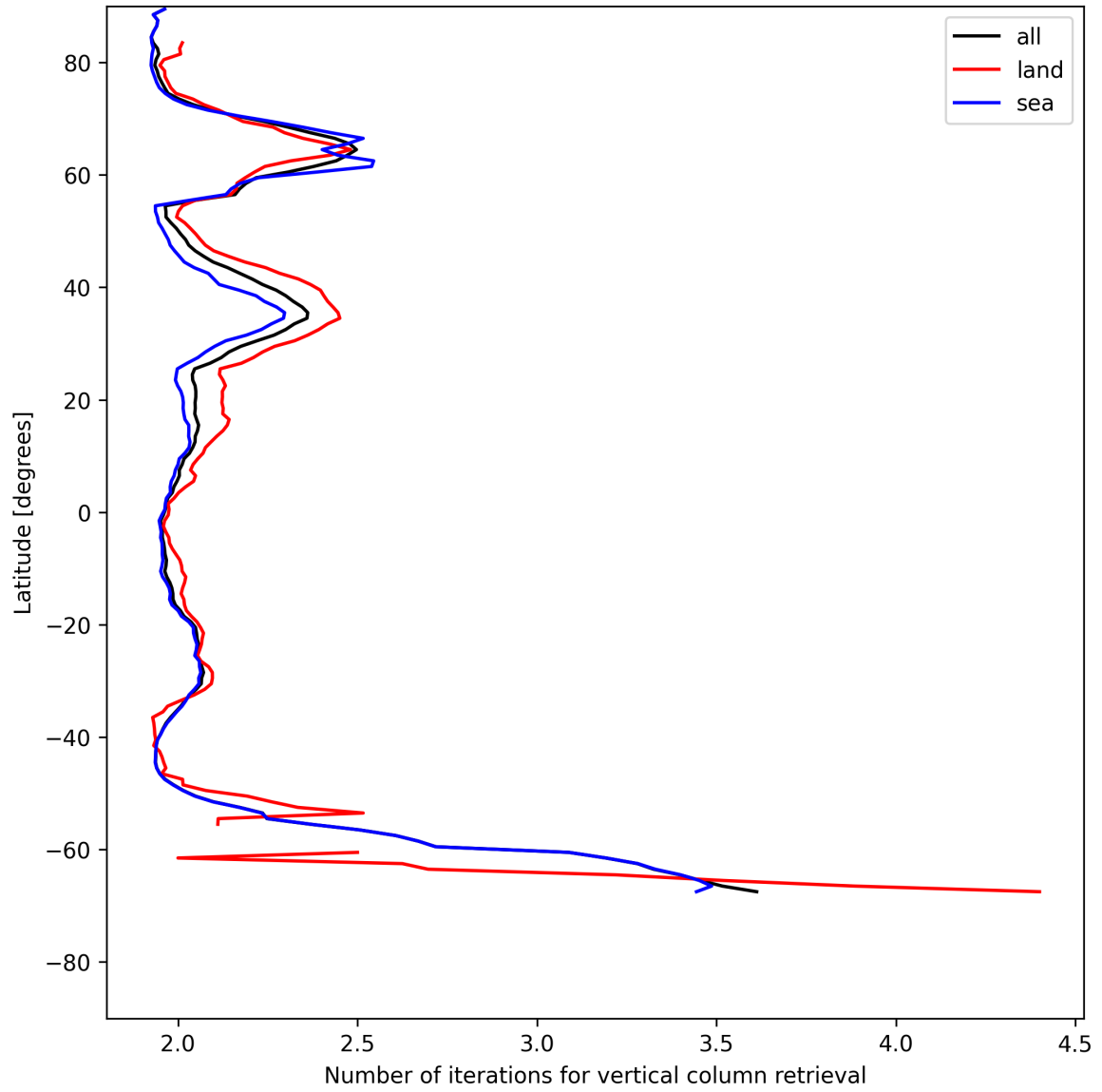
Figure 27: Zonal average of “Number of iterations for vertical column retrieval” for 2025-07-14 to 2025-07-15.
