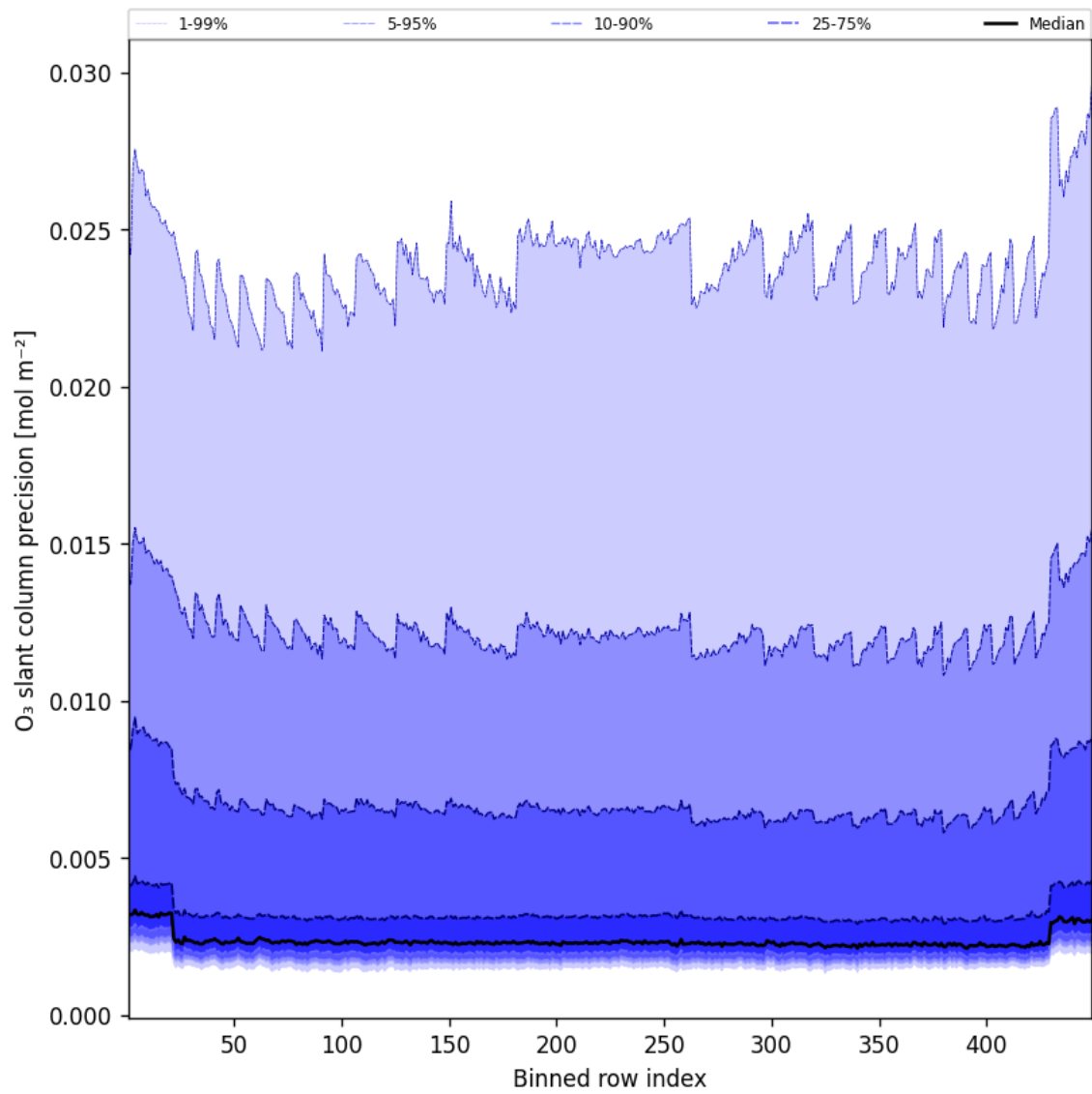
Figure 44: Along track statistics of “O 3 slant column precision” for 2025-07-14 to 2025-07-15
