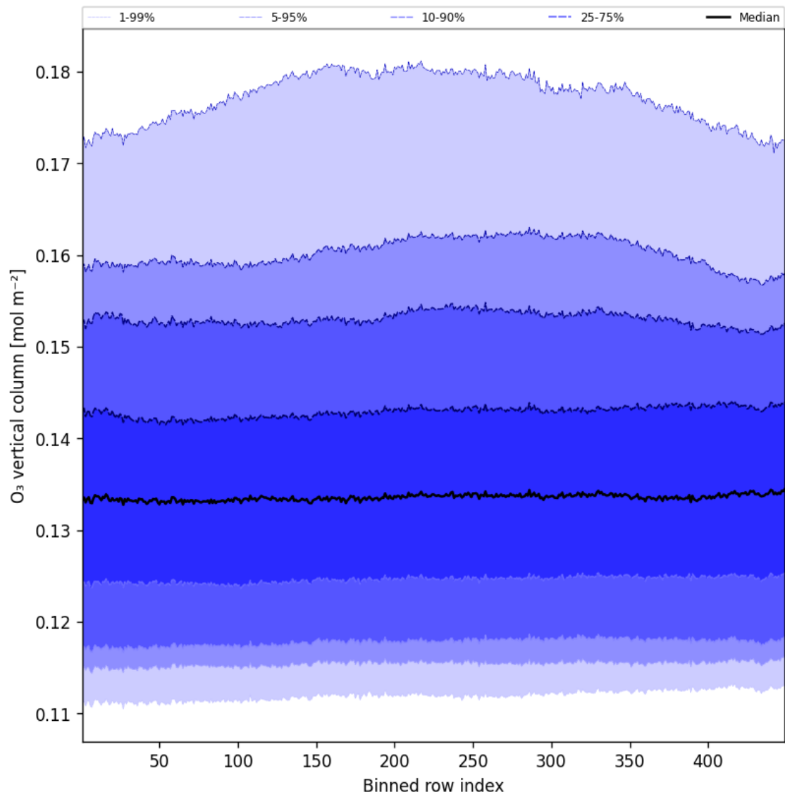
Figure 41: Along track statistics of “O 3 vertical column” for 2025-07-14 to 2025-07-15
