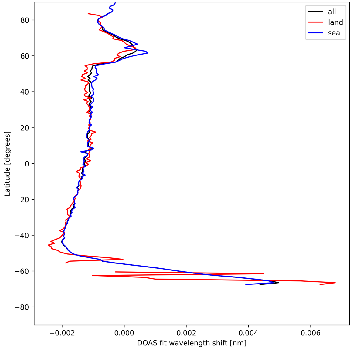
Figure 23: Zonal average of “DOAS fit wavelength shift” for 2025-07-14 to 2025-07-15.
