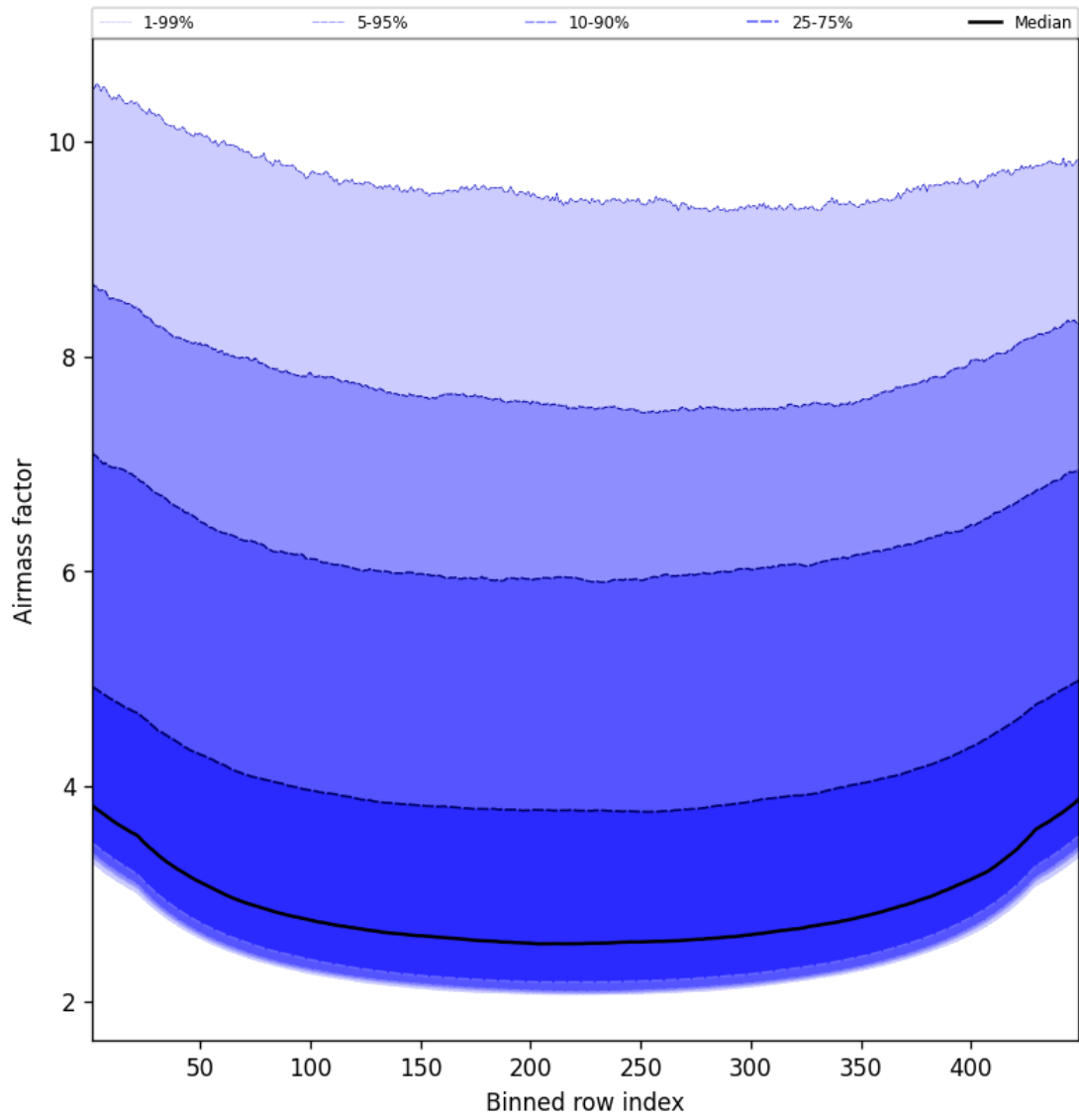
Figure 49: Along track statistics of “Airmass factor” for 2025-07-14 to 2025-07-15
