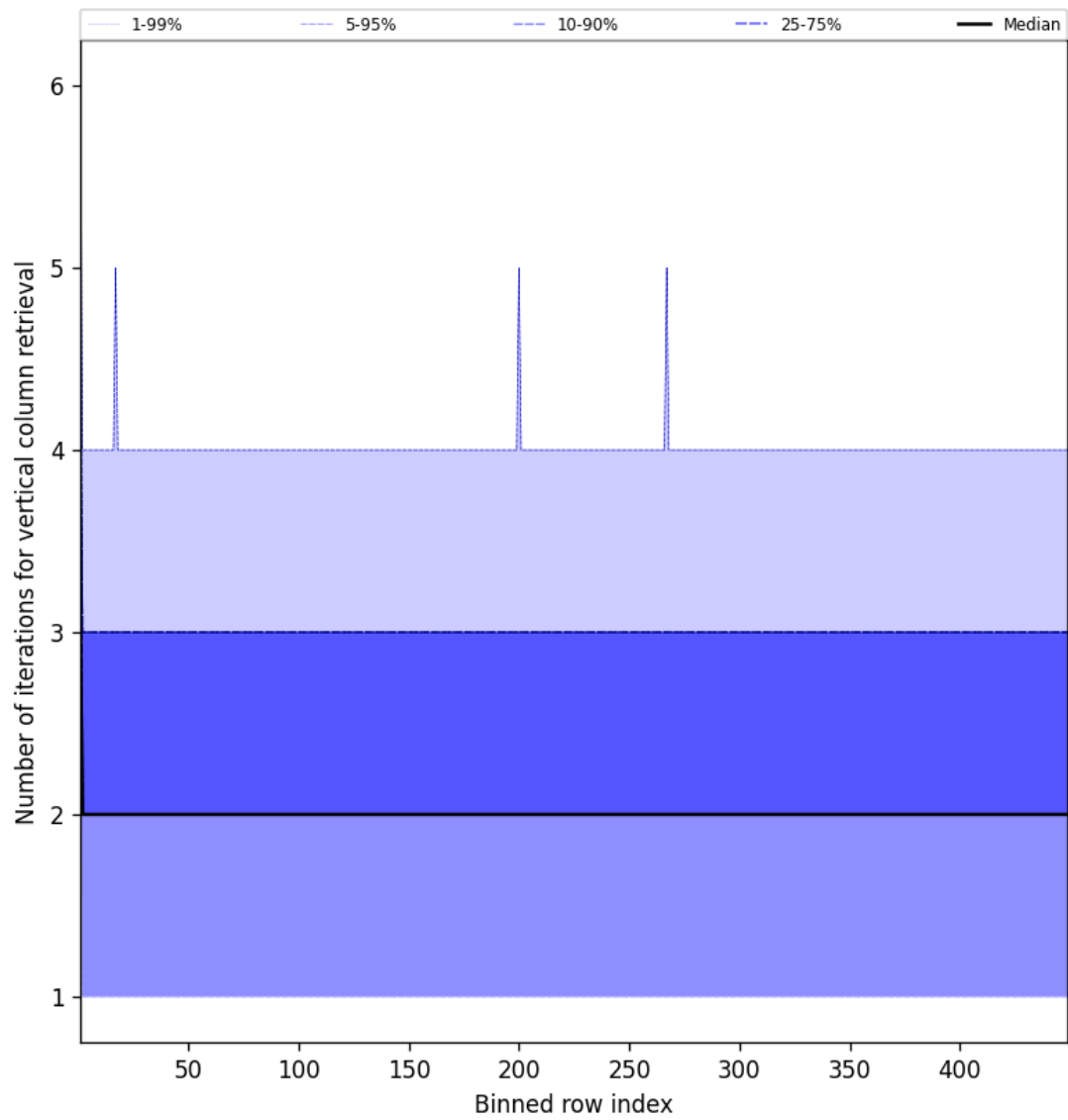
Figure 51: Along track statistics of “Number of iterations for vertical column retrieval” for 2025-07-14 to 2025-07-15
