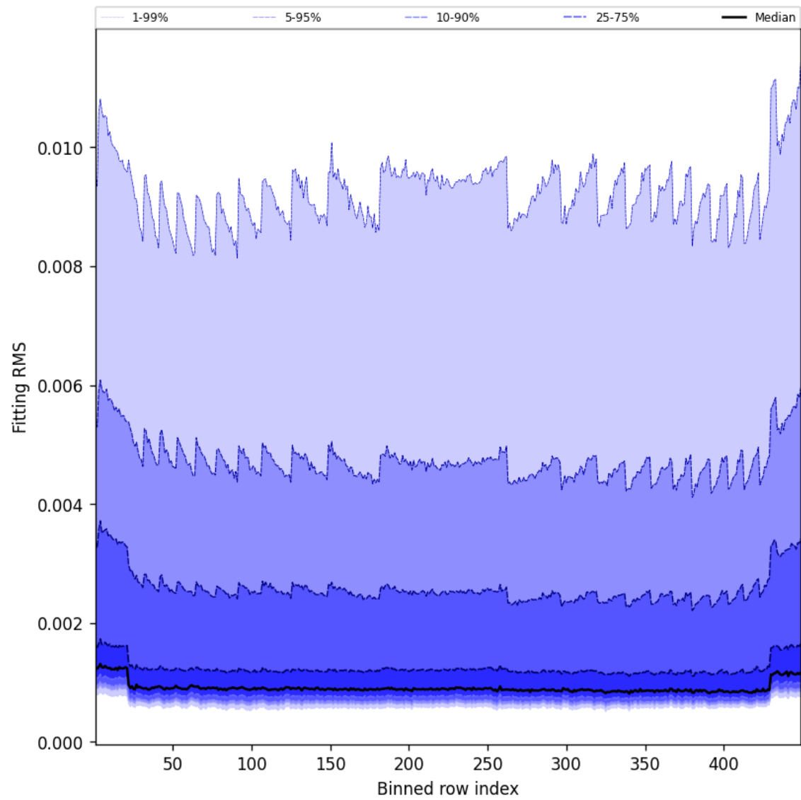
Figure 46: Along track statistics of “Fitting RMS” for 2025-07-14 to 2025-07-15
