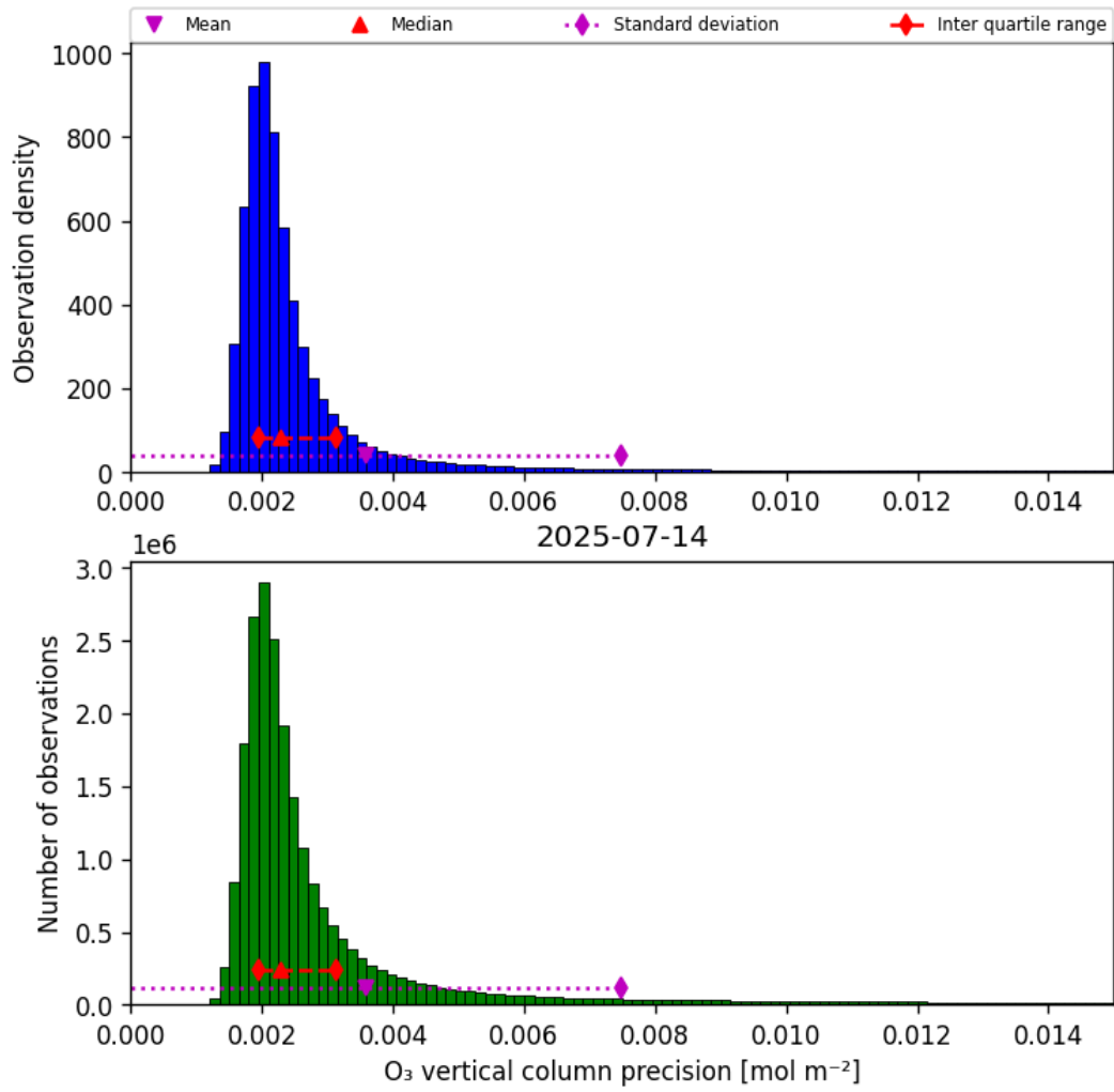
Figure 30: Histogram of “O 3 vertical column precision” for 2025-07-14 to 2025-07-15
