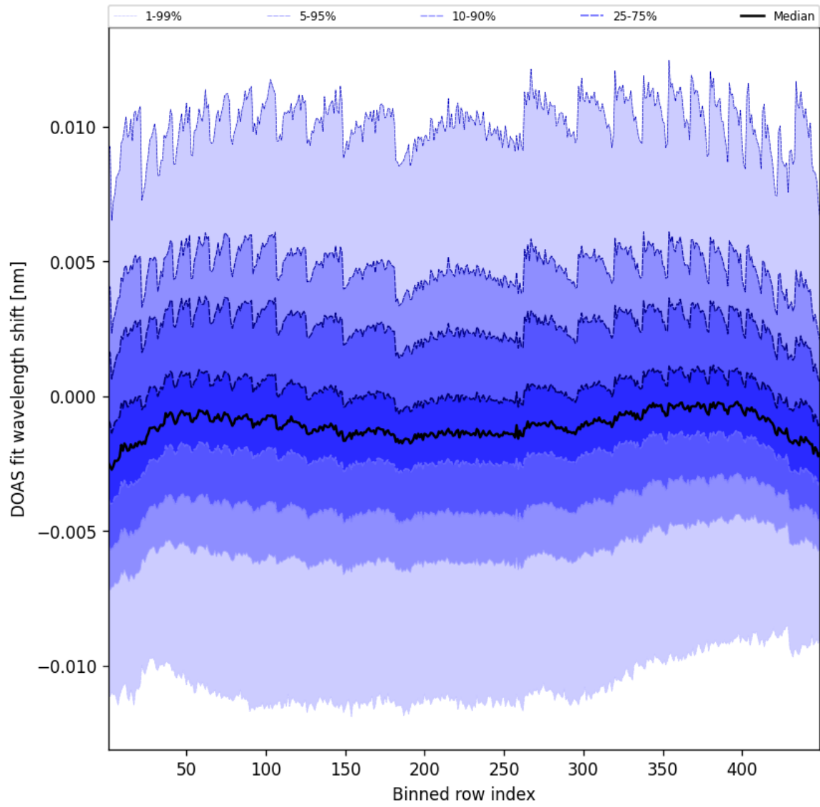
Figure 47: Along track statistics of “DOAS fit wavelength shift” for 2025-07-14 to 2025-07-15
