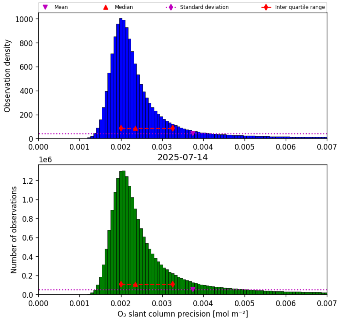
Figure 32: Histogram of “O 3 slant column precision” for 2025-07-14 to 2025-07-15
