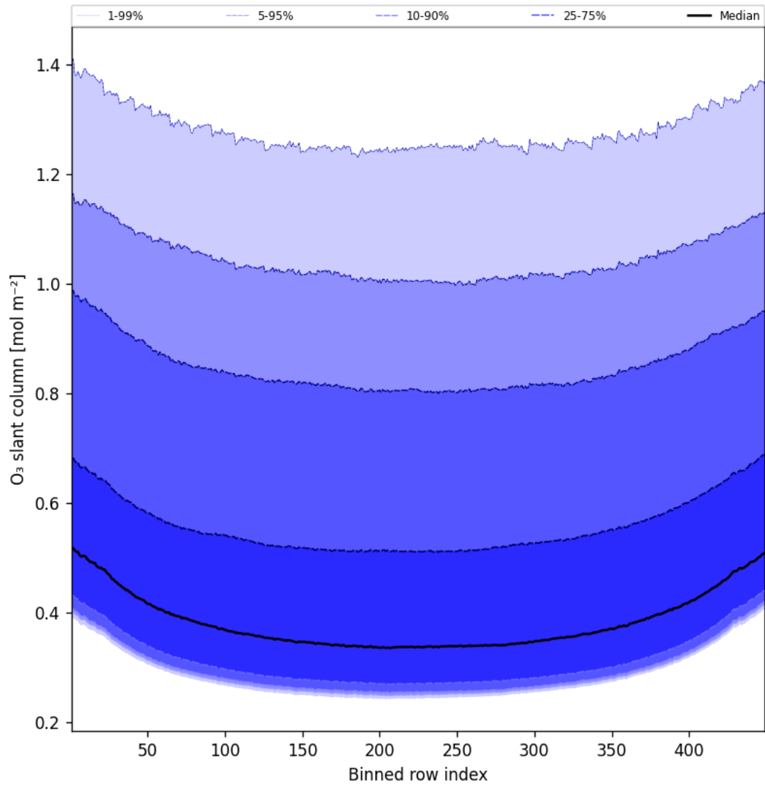
Figure 43: Along track statistics of “O 3 slant column” for 2025-07-14 to 2025-07-15
