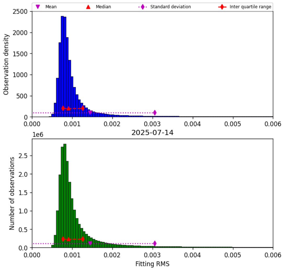
Figure 34: Histogram of “Fitting RMS” for 2025-07-14 to 2025-07-15
