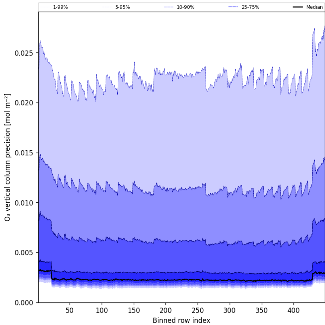
Figure 42: Along track statistics of “O 3 vertical column precision” for 2025-07-14 to 2025-07-15
