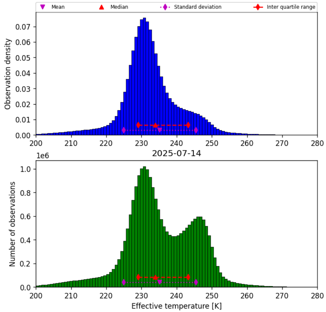
Figure 38: Histogram of “Effective temperature” for 2025-07-14 to 2025-07-15
