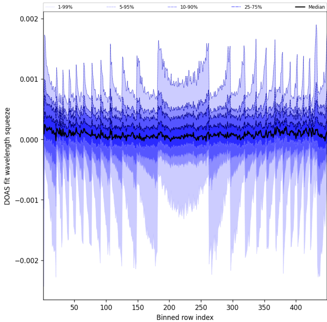
Figure 48: Along track statistics of “DOAS fit wavelength squeeze” for 2025-07-14 to 2025-07-15
