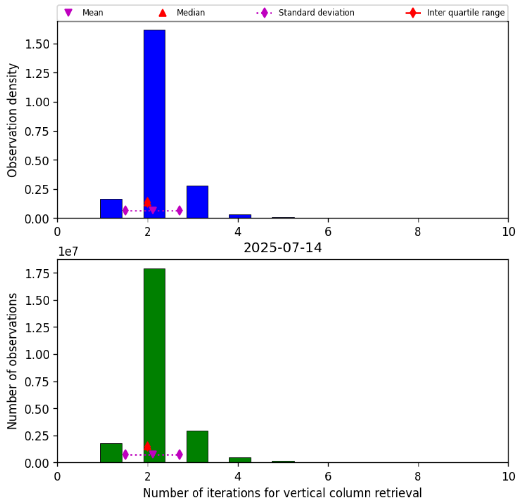
Figure 39: Histogram of “Number of iterations for vertical column retrieval” for 2025-07-14 to 2025-07-15
