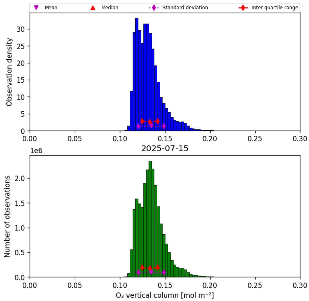
Figure 29: Histogram of “O 3 vertical column” for 2025-07-15 to 2025-07-16
