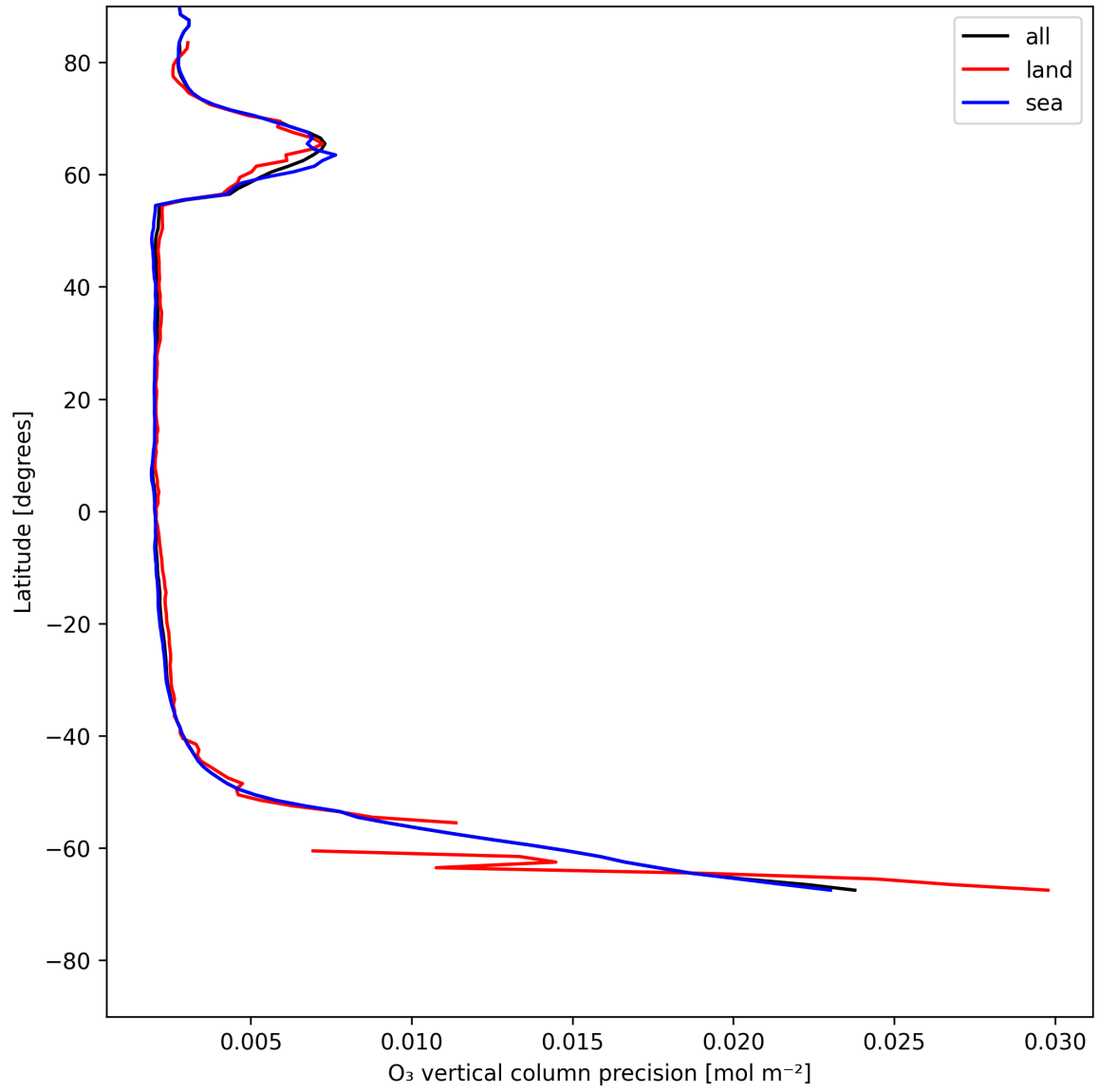
Figure 18: Zonal average of “O 3 vertical column precision” for 2025-07-15 to 2025-07-16.
