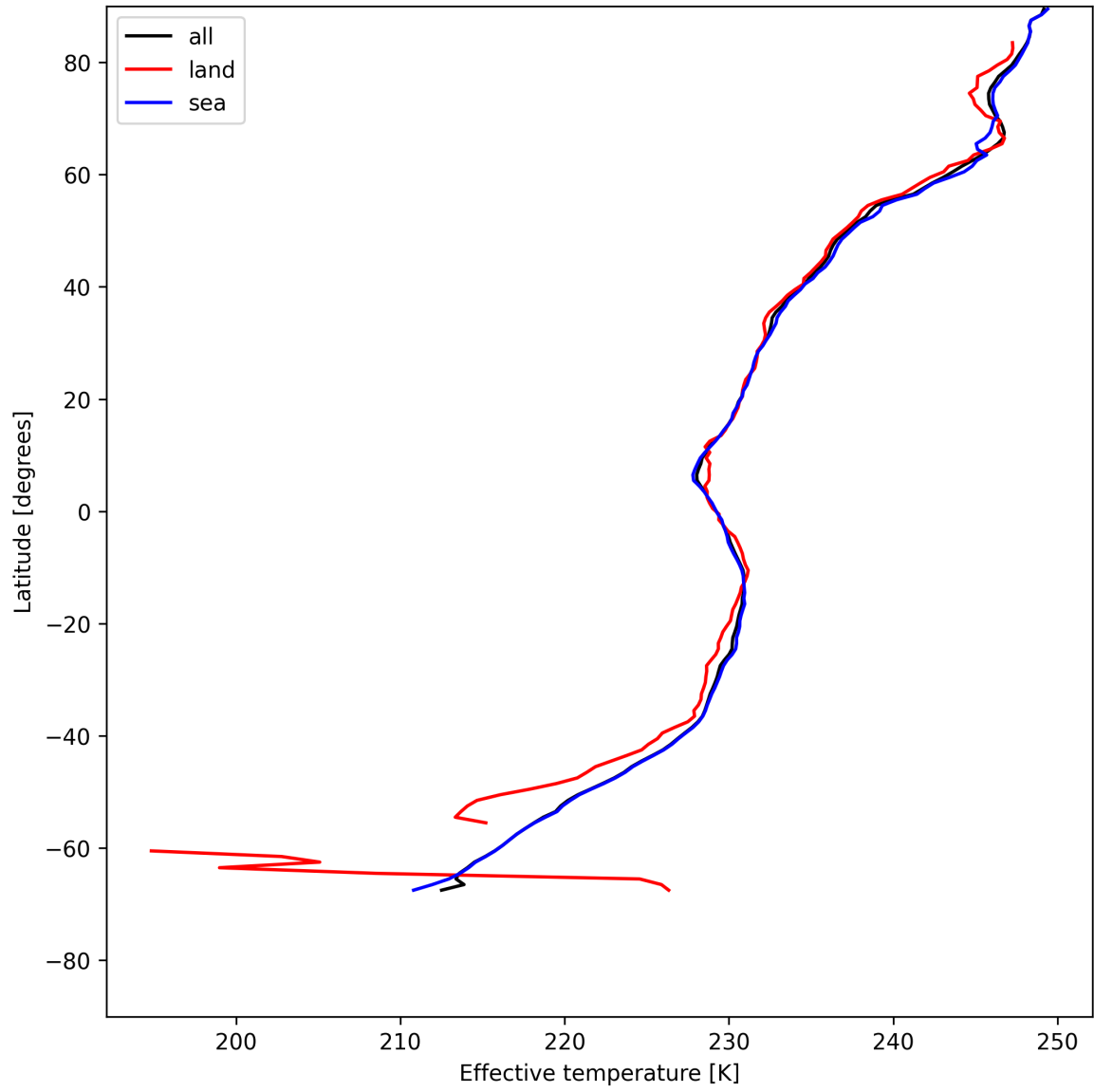
Figure 26: Zonal average of "Effective temperature" for 2025-07-15 to 2025-07-16.
