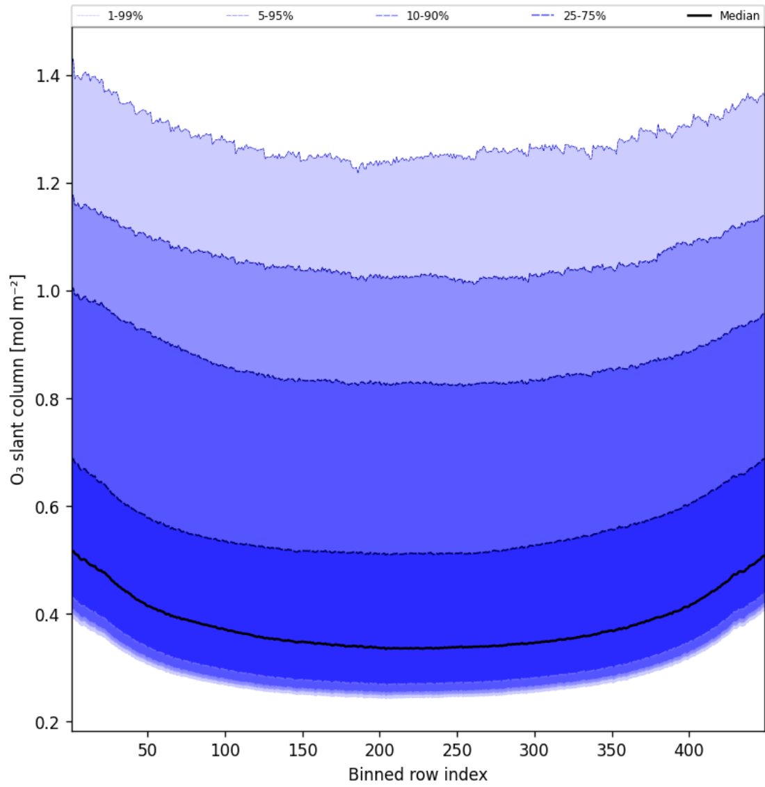
Figure 43: Along track statistics of “O 3 slant column” for 2025-07-15 to 2025-07-16
