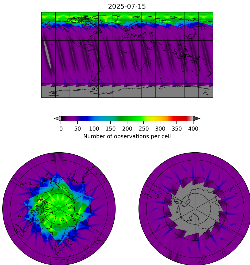
Figure 15: Map of the number of observations for 2025-07-15 to 2025-07-16
