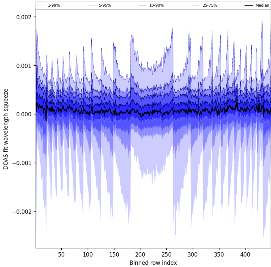
Figure 48: Along track statistics of “DOAS fit wavelength squeeze” for 2025-07-15 to 2025-07-16
