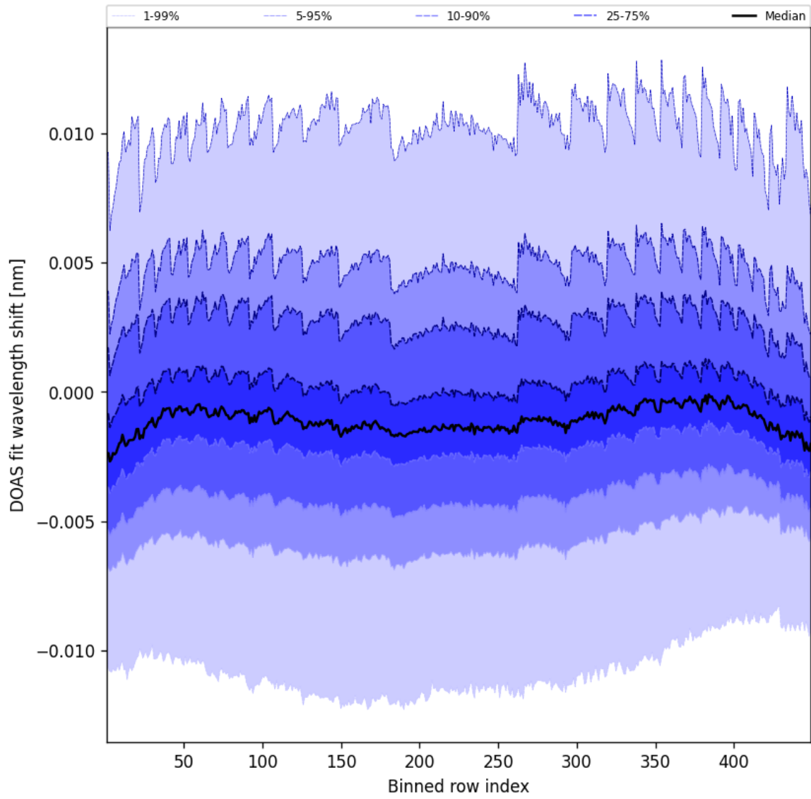
Figure 47: Along track statistics of “DOAS fit wavelength shift” for 2025-07-15 to 2025-07-16
