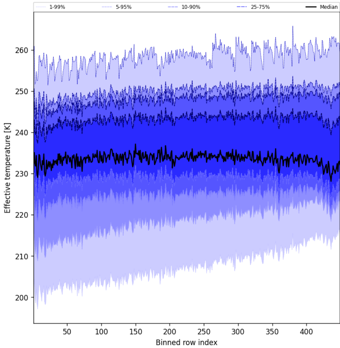
Figure 50: Along track statistics of “Effective temperature” for 2025-07-15 to 2025-07-16
