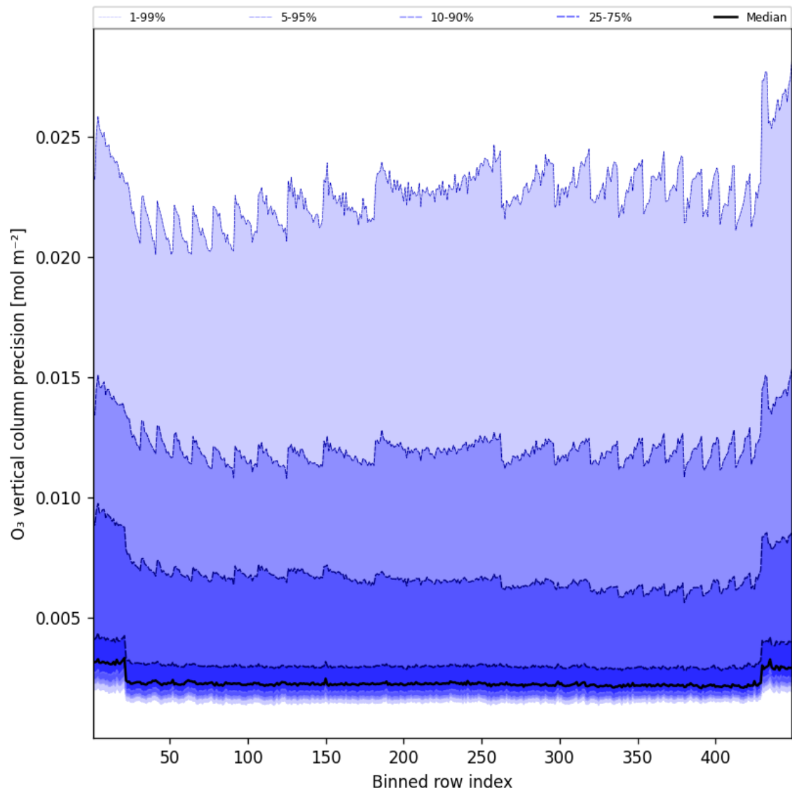
Figure 42: Along track statistics of “O 3 vertical column precision” for 2025-07-15 to 2025-07-16
