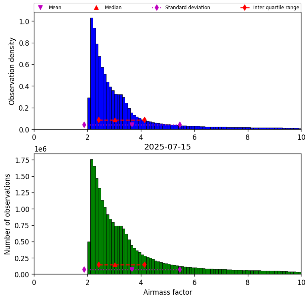
Figure 37: Histogram of “Airmass factor” for 2025-07-15 to 2025-07-16
