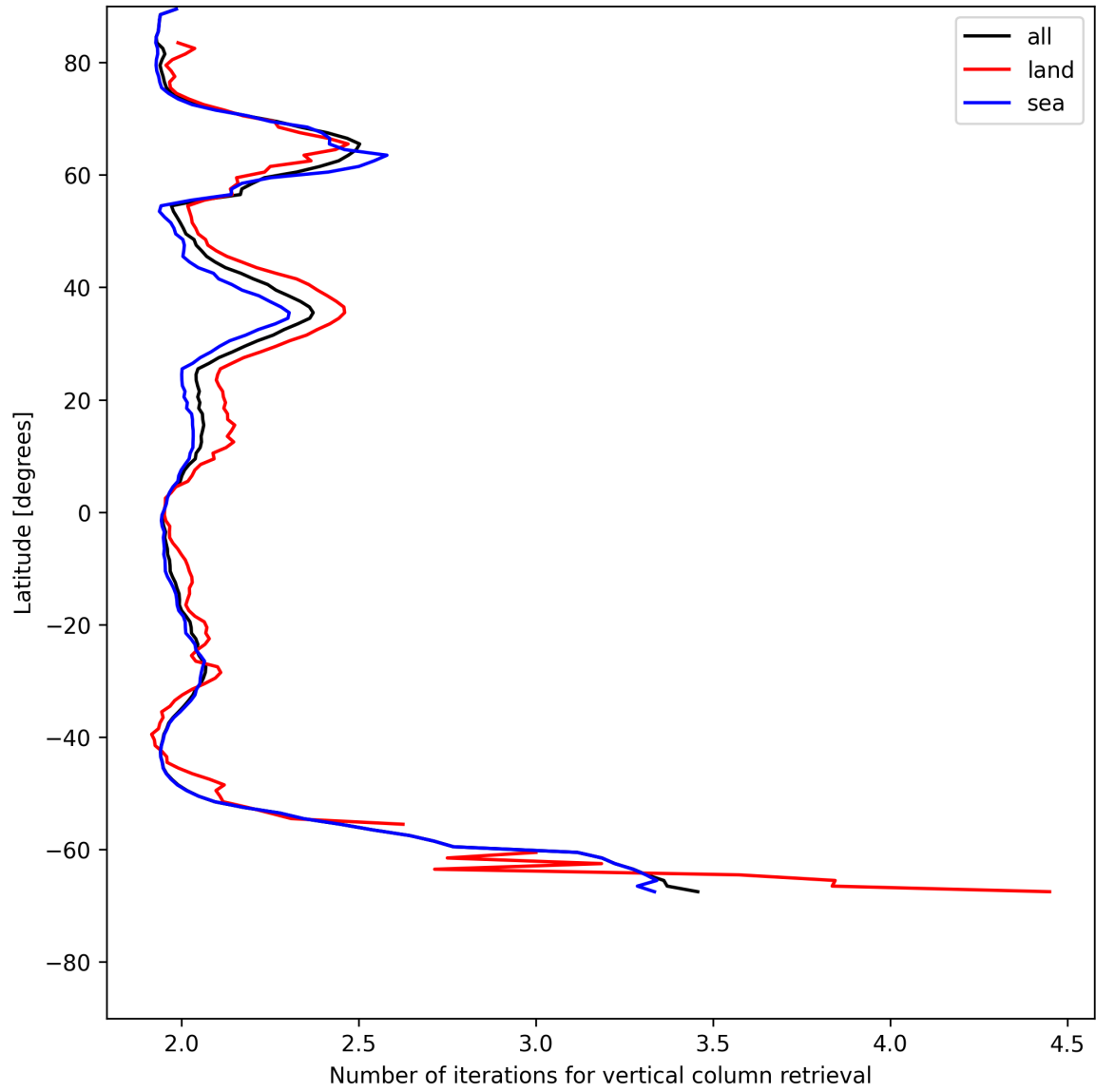
Figure 27: Zonal average of “Number of iterations for vertical column retrieval” for 2025-07-15 to 2025-07-16.
