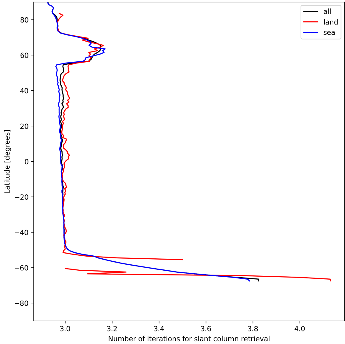
Figure 21: Zonal average of “Number of iterations for slant column retrieval” for 2025-07-15 to 2025-07-16.
