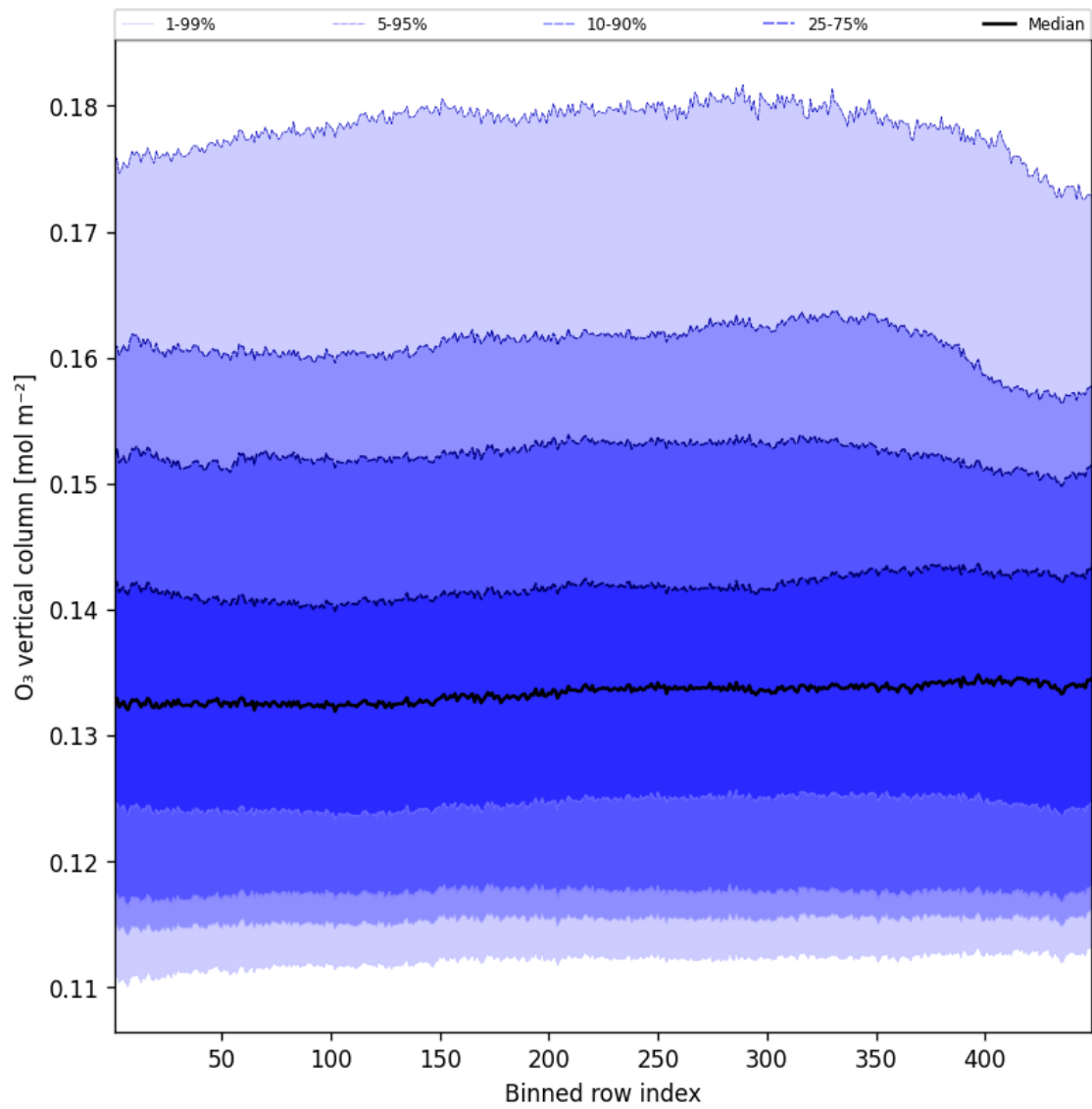
Figure 41: Along track statistics of “O 3 vertical column” for 2025-07-15 to 2025-07-16
