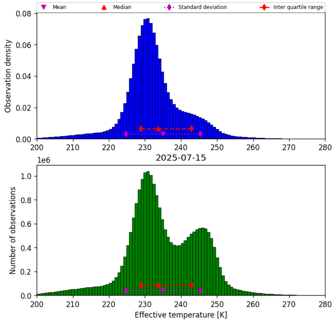
Figure 38: Histogram of “Effective temperature” for 2025-07-15 to 2025-07-16
