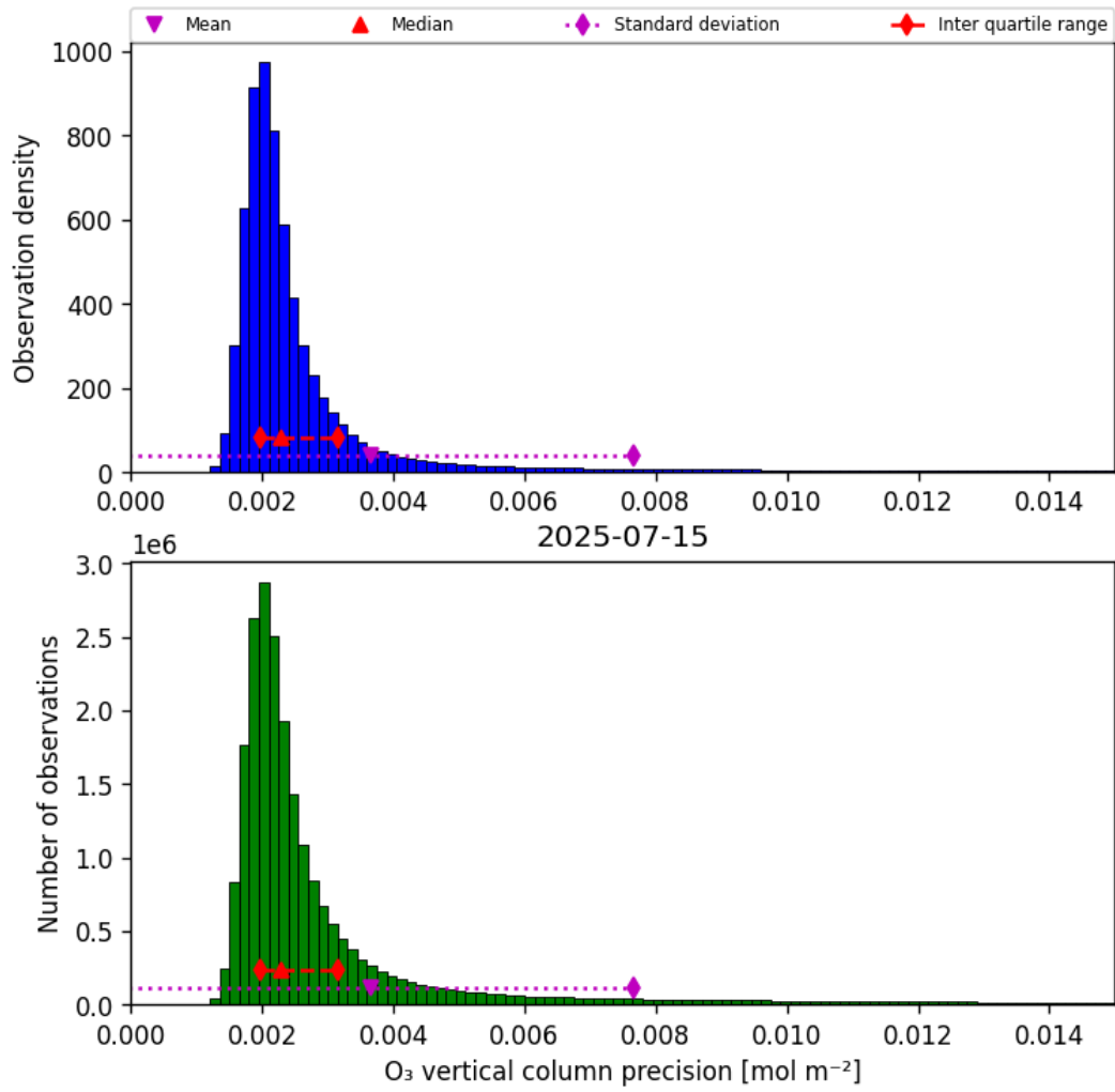
Figure 30: Histogram of “O 3 vertical column precision” for 2025-07-15 to 2025-07-16
