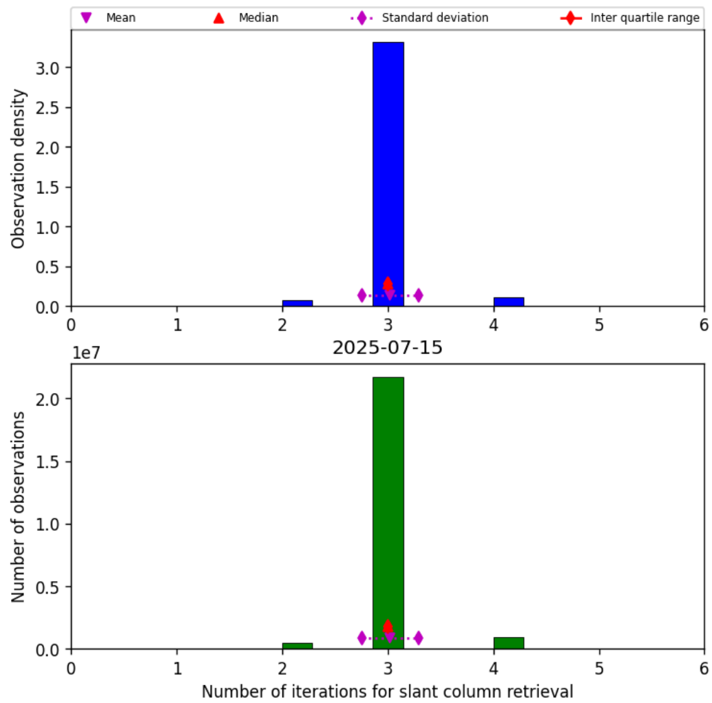
Figure 33: Histogram of “Number of iterations for slant column retrieval” for 2025-07-15 to 2025-07-16
