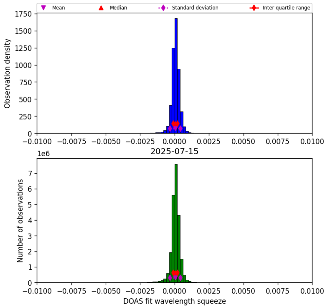
Figure 36: Histogram of “DOAS fit wavelength squeeze” for 2025-07-15 to 2025-07-16
