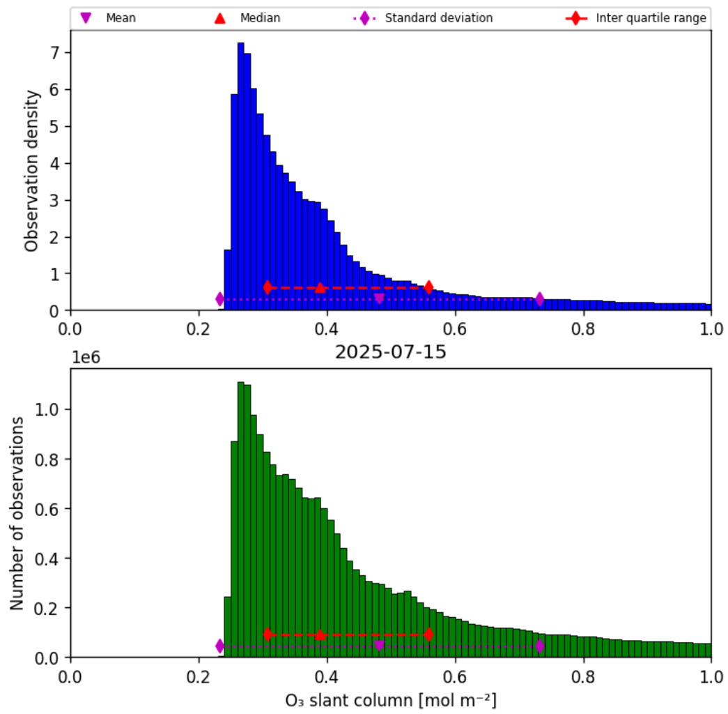
Figure 31: Histogram of “O 3 slant column” for 2025-07-15 to 2025-07-16
