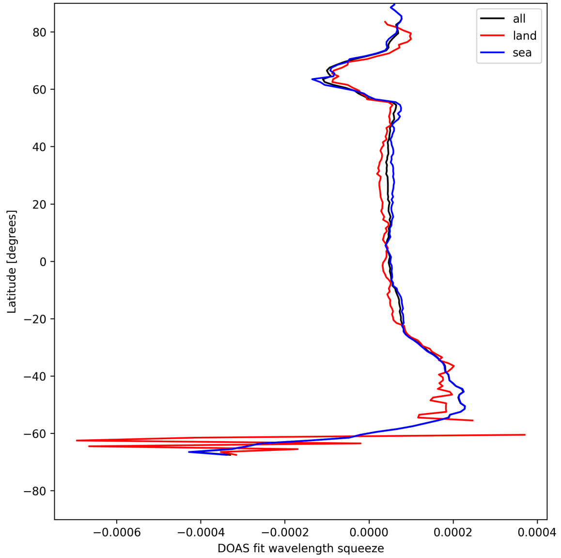
Figure 24: Zonal average of “DOAS fit wavelength squeeze” for 2025-07-15 to 2025-07-16.
