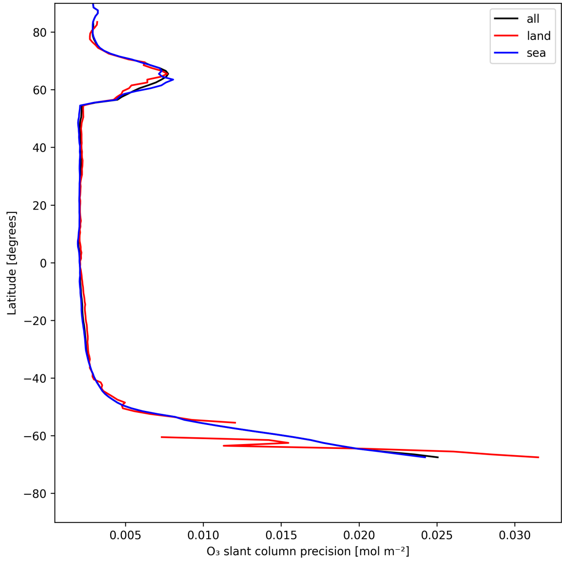
Figure 20: Zonal average of "O 3 slant column precision" for 2025-07-15 to 2025-07-16.
