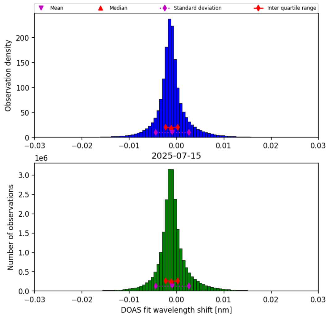
Figure 35: Histogram of “DOAS fit wavelength shift” for 2025-07-15 to 2025-07-16
