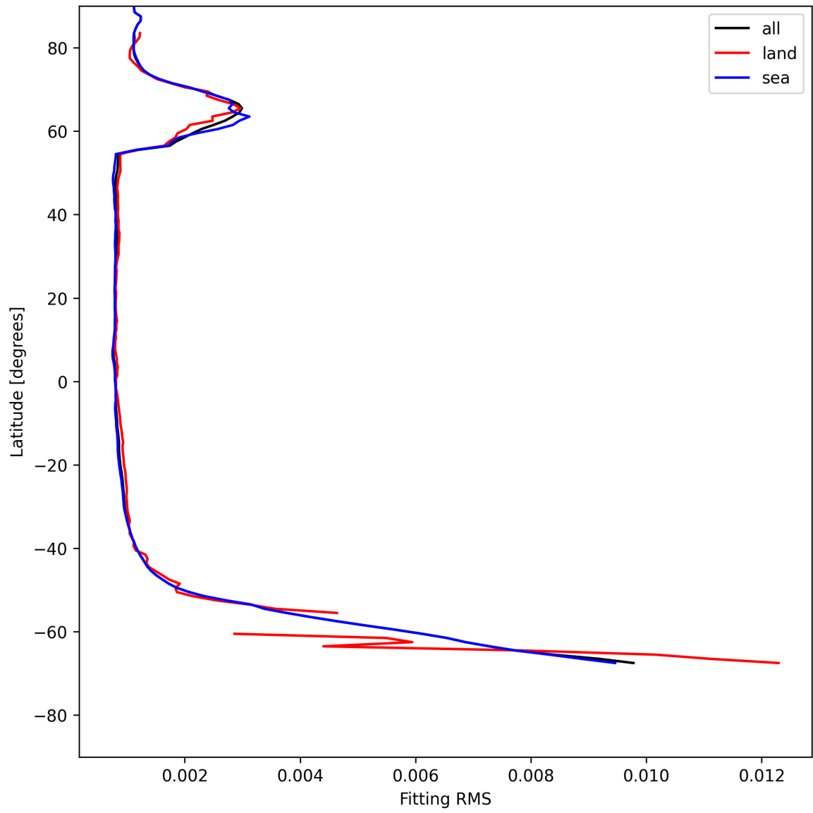
Figure 22: Zonal average of “Fitting RMS” for 2025-07-15 to 2025-07-16.
