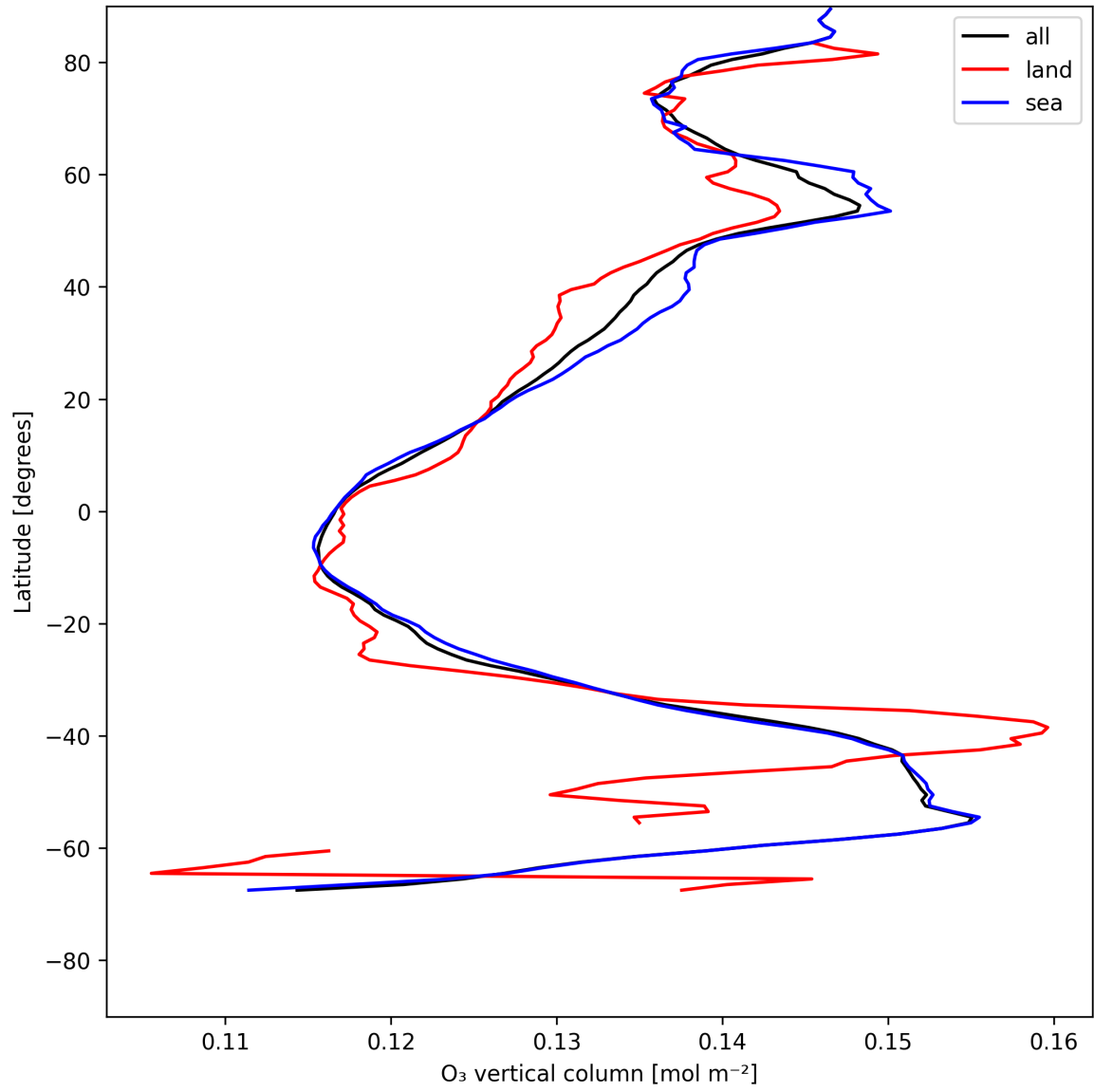
Figure 17: Zonal average of “O 3 vertical column” for 2025-07-15 to 2025-07-16.
