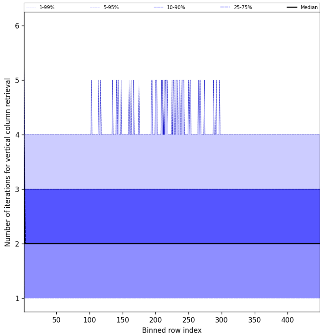
Figure 51: Along track statistics of “Number of iterations for vertical column retrieval” for 2025-07-15 to 2025-07-16
