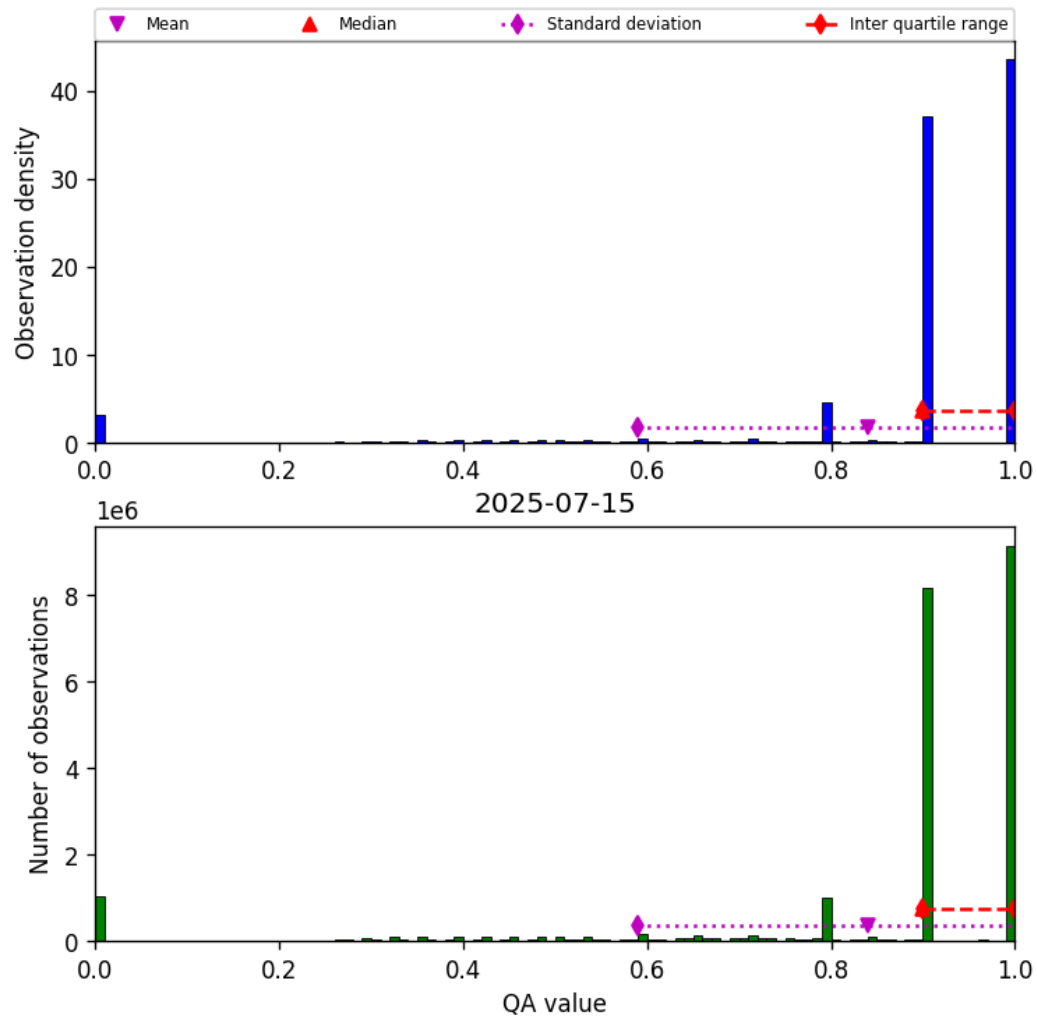
Figure 28: Histogram of “QA value” for 2025-07-15 to 2025-07-16
