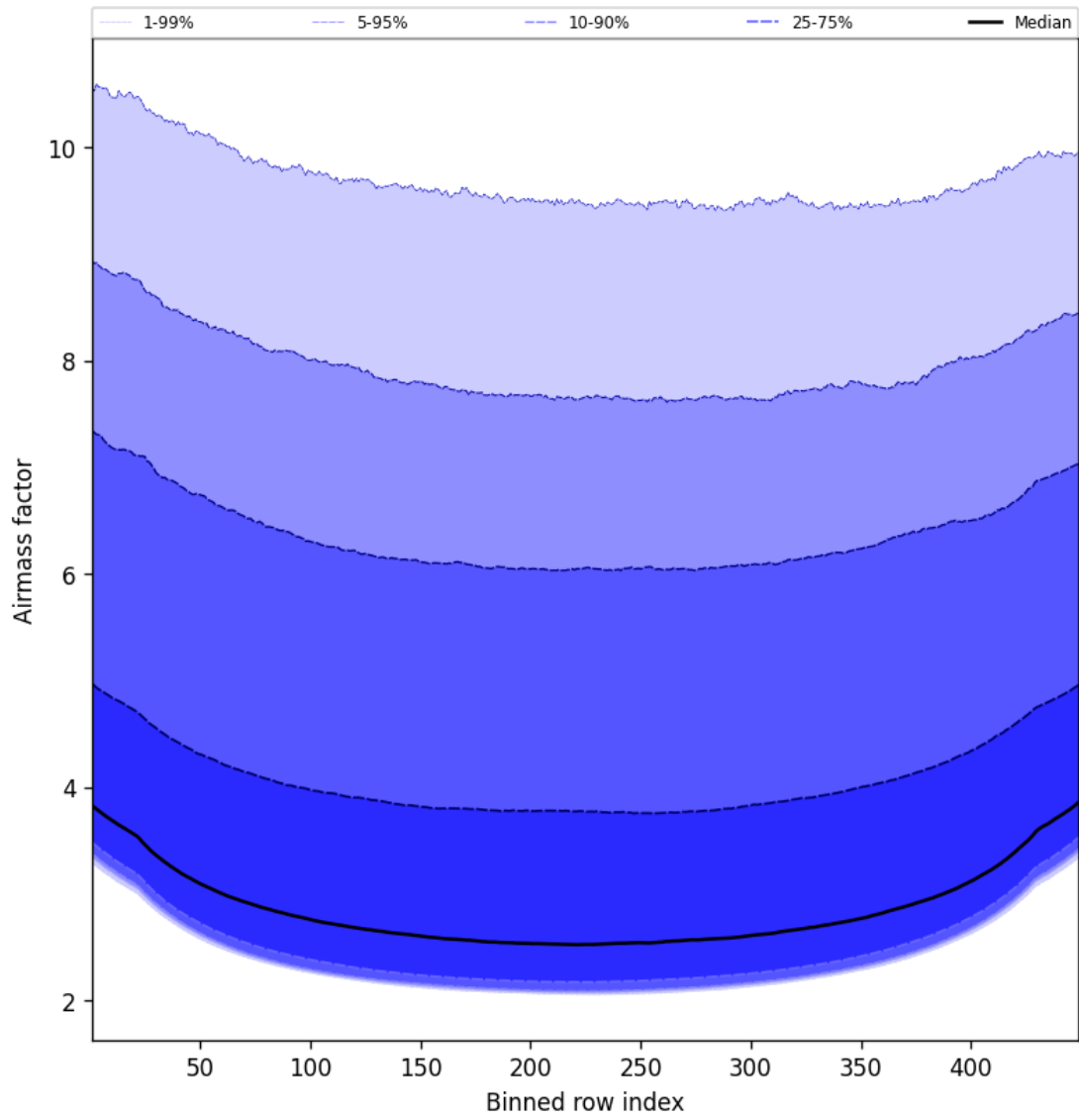
Figure 49: Along track statistics of “Airmass factor” for 2025-07-15 to 2025-07-16
