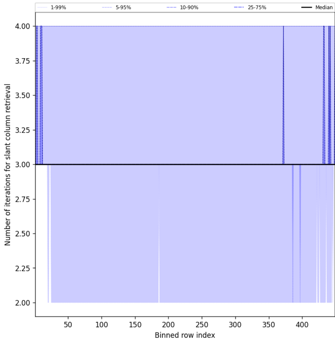
Figure 45: Along track statistics of “Number of iterations for slant column retrieval” for 2025-07-15 to 2025-07-16
