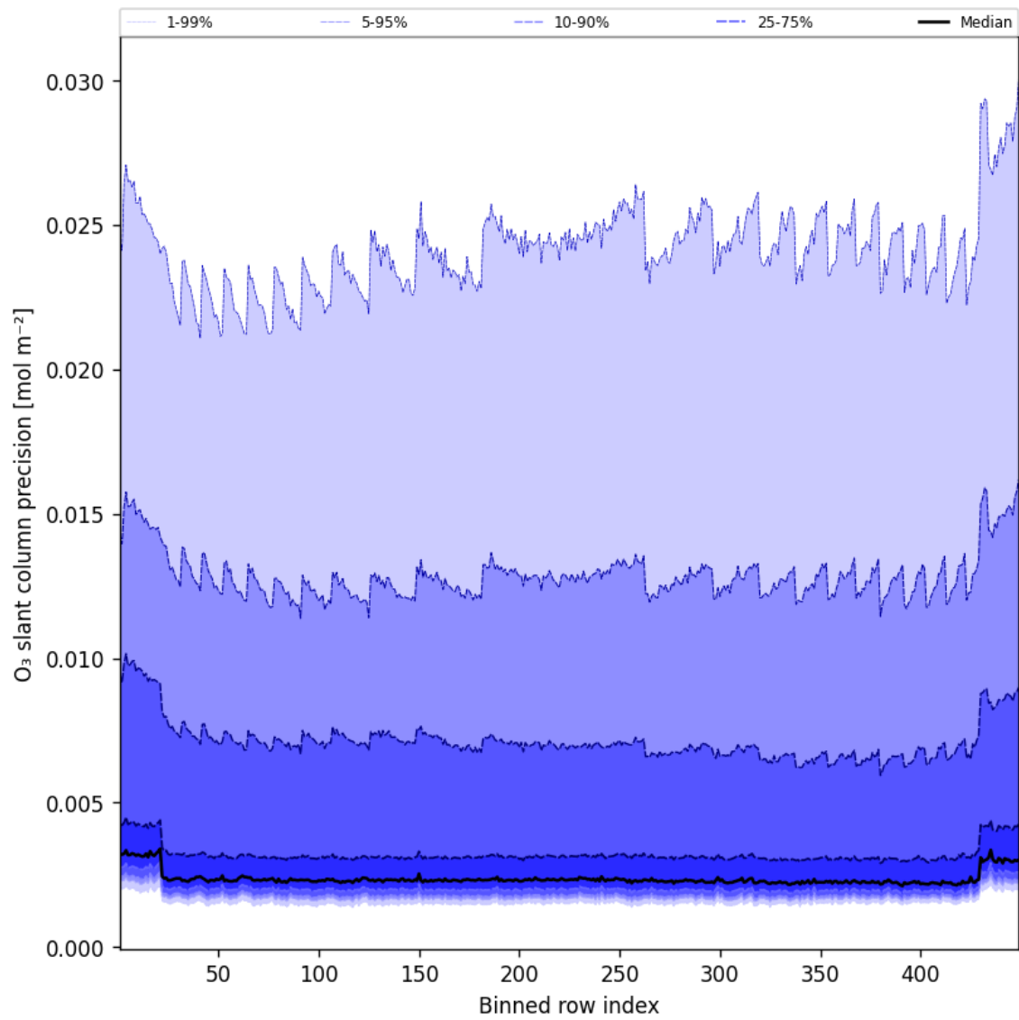
Figure 44: Along track statistics of “O 3 slant column precision” for 2025-07-15 to 2025-07-16
