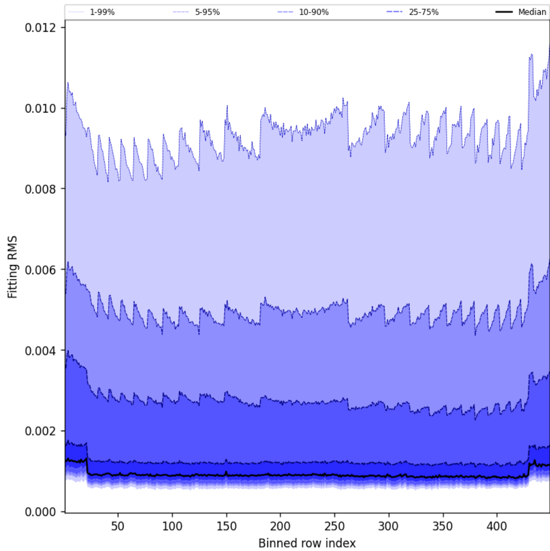
Figure 46: Along track statistics of “Fitting RMS” for 2025-07-15 to 2025-07-16
