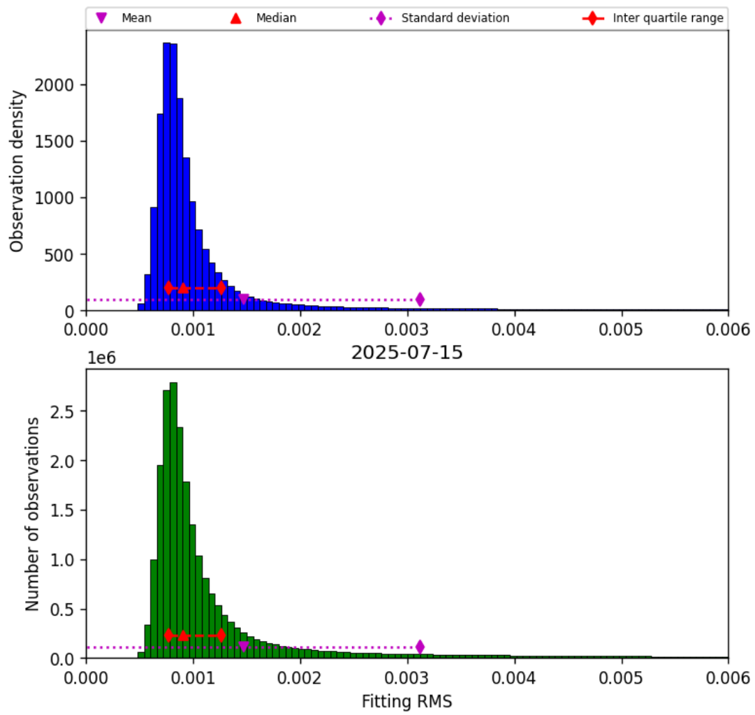
Figure 34: Histogram of “Fitting RMS” for 2025-07-15 to 2025-07-16
