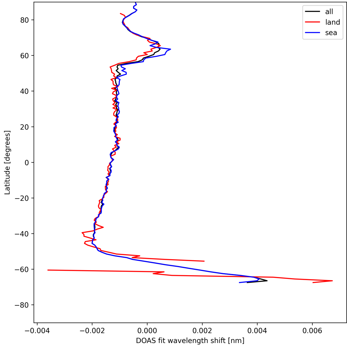
Figure 23: Zonal average of “DOAS fit wavelength shift” for 2025-07-15 to 2025-07-16.
