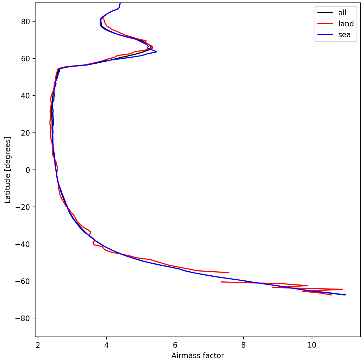
Figure 25: Zonal average of “Airmass factor” for 2025-07-15 to 2025-07-16.
