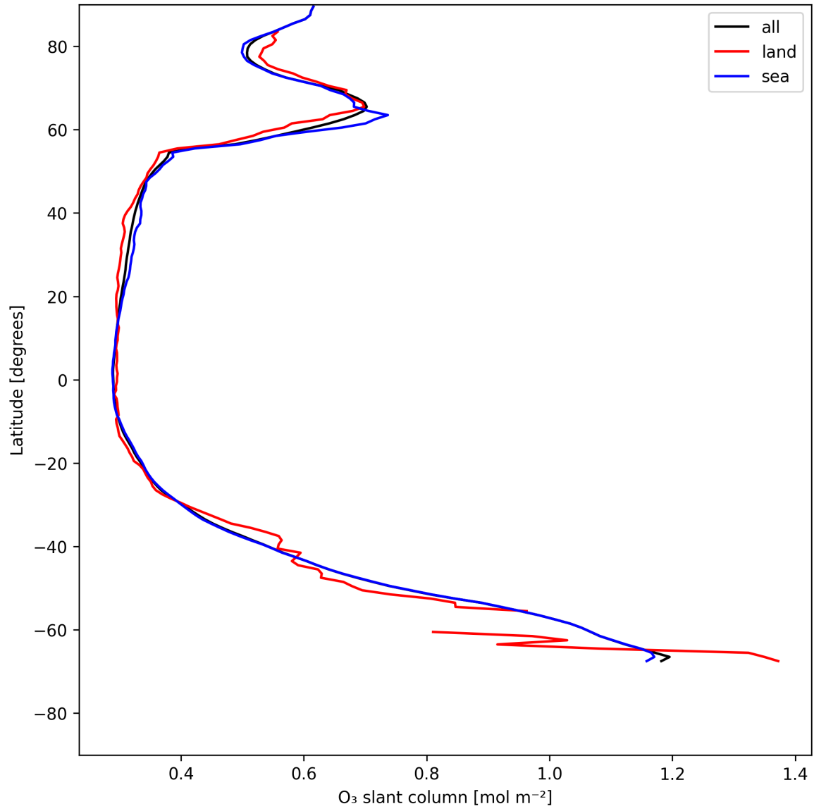
Figure 19: Zonal average of “O 3 slant column” for 2025-07-15 to 2025-07-16.
