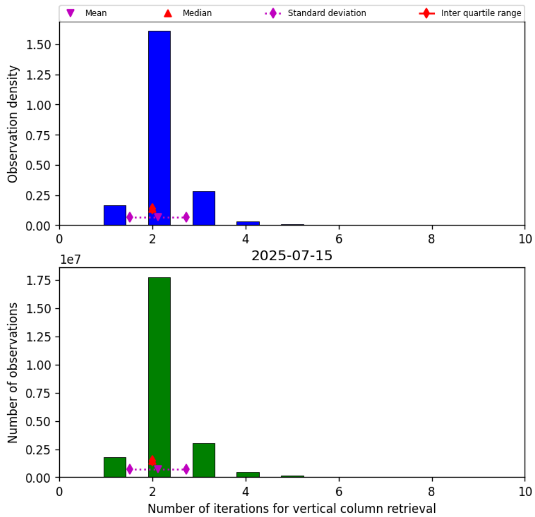
Figure 39: Histogram of “Number of iterations for vertical column retrieval” for 2025-07-15 to 2025-07-16
