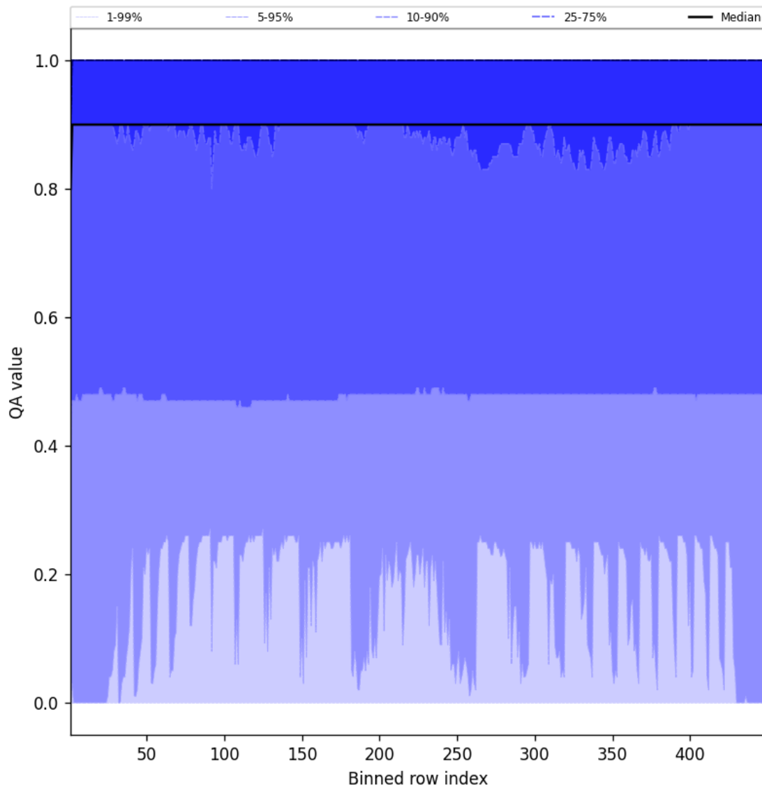
Figure 40: Along track statistics of “QA value” for 2025-07-15 to 2025-07-16
