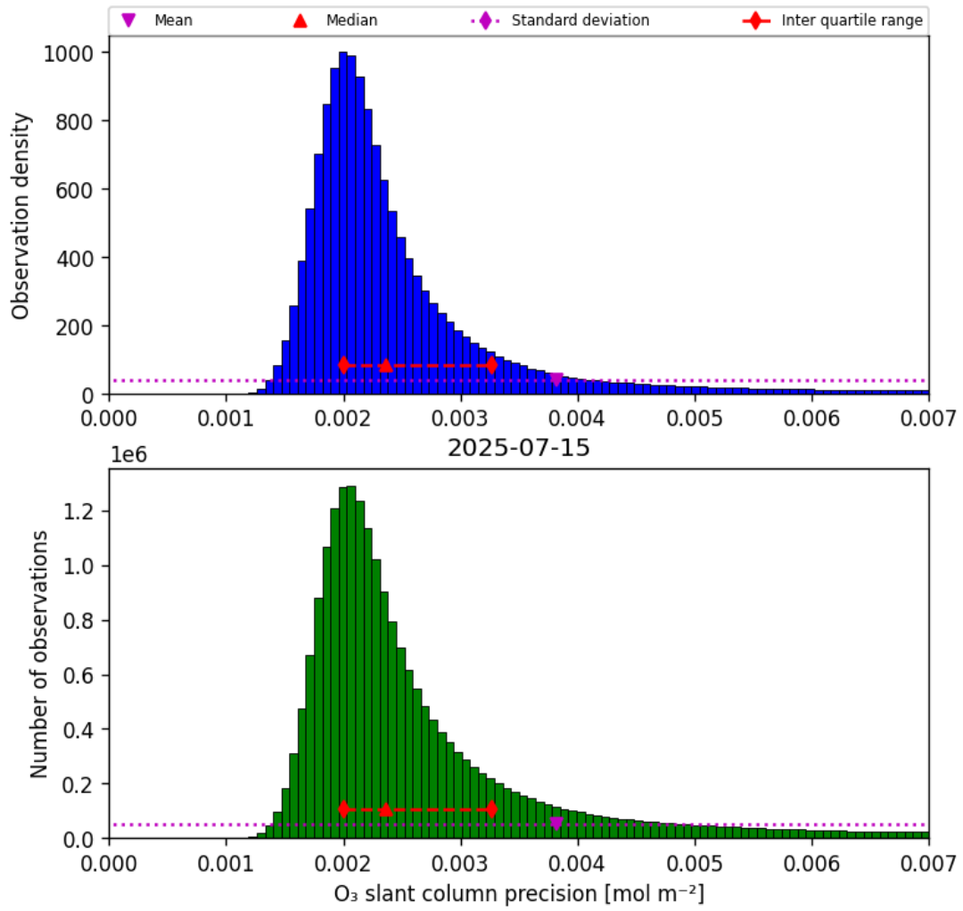
Figure 32: Histogram of “O 3 slant column precision” for 2025-07-15 to 2025-07-16
