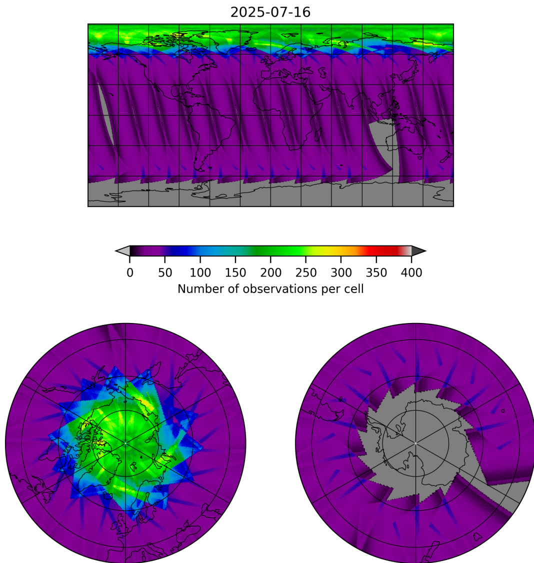
Figure 15: Map of the number of observations for 2025-07-16 to 2025-07-16
