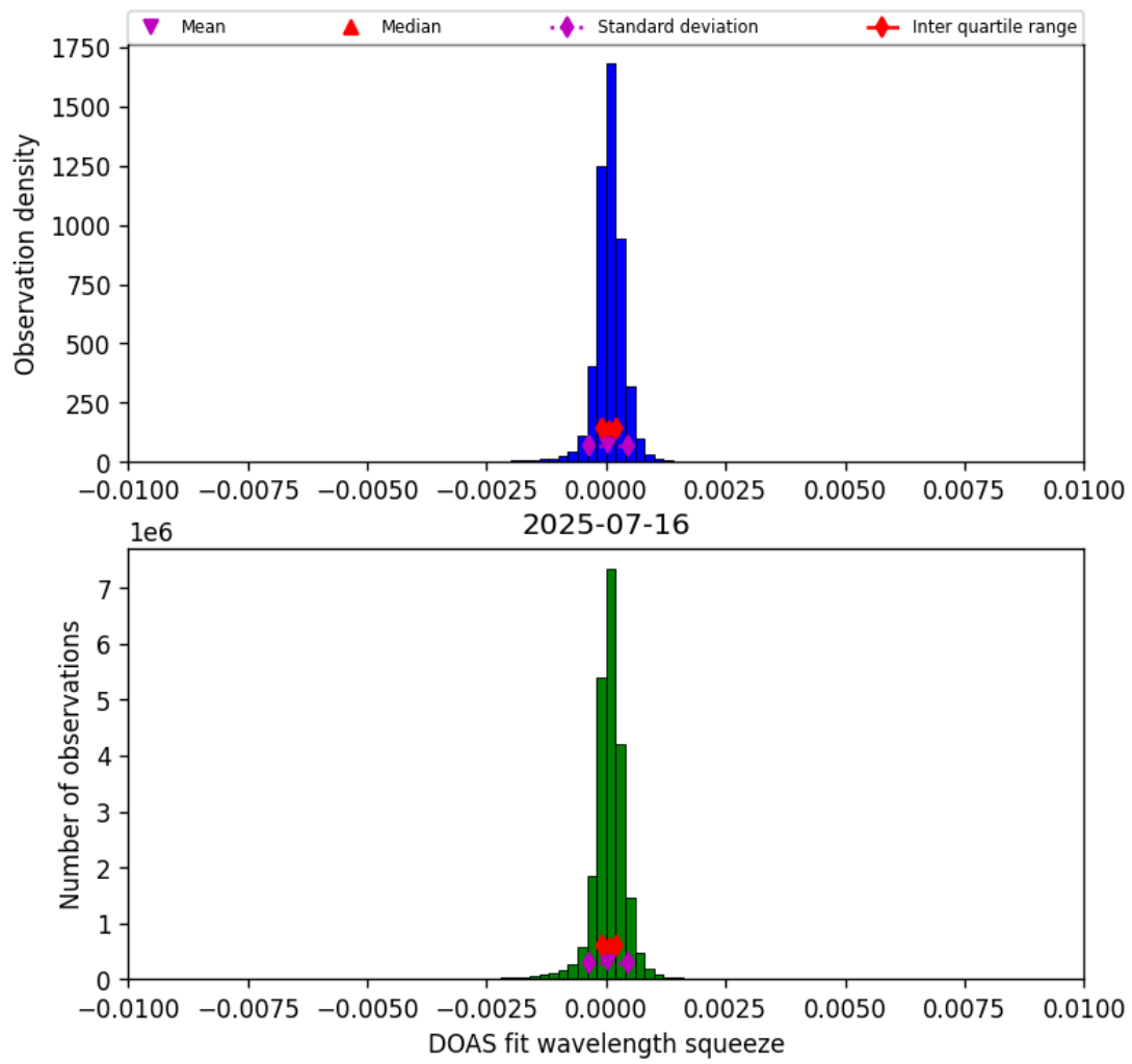
Figure 36: Histogram of “DOAS fit wavelength squeeze” for 2025-07-16 to 2025-07-16
