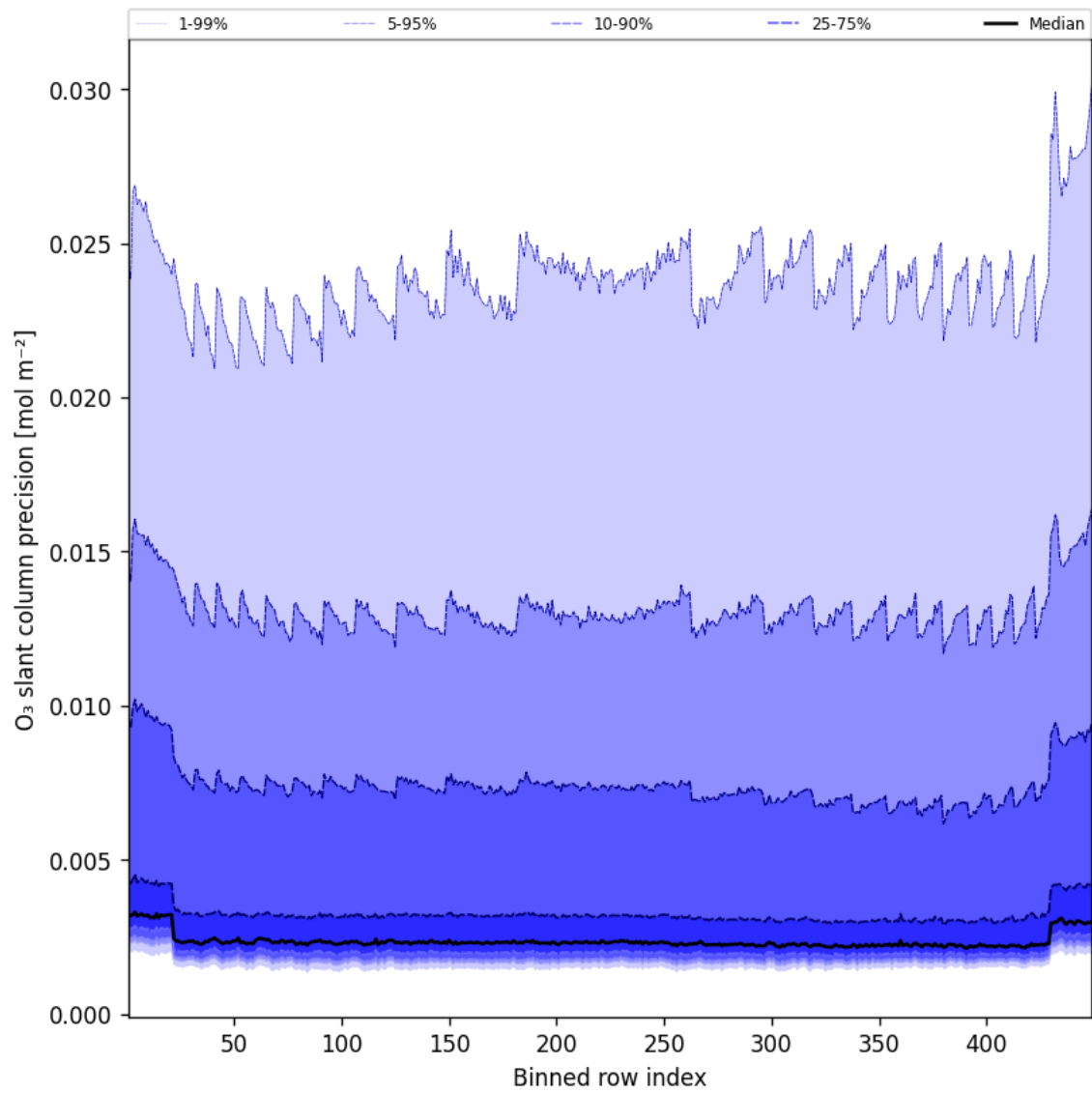
Figure 44: Along track statistics of “O 3 slant column precision” for 2025-07-16 to 2025-07-16
