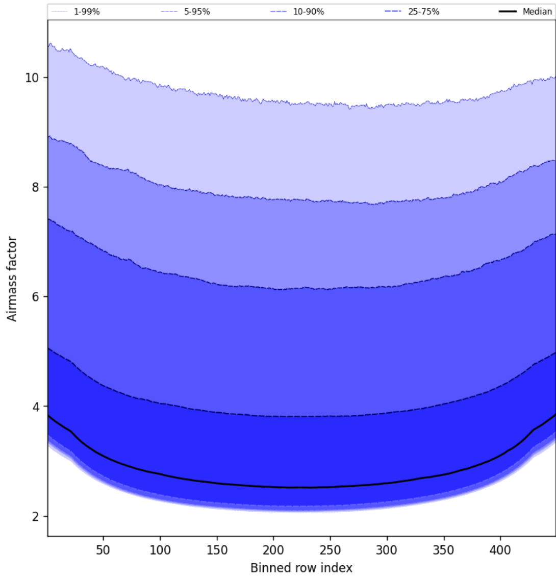
Figure 49: Along track statistics of “Airmass factor” for 2025-07-16 to 2025-07-16
