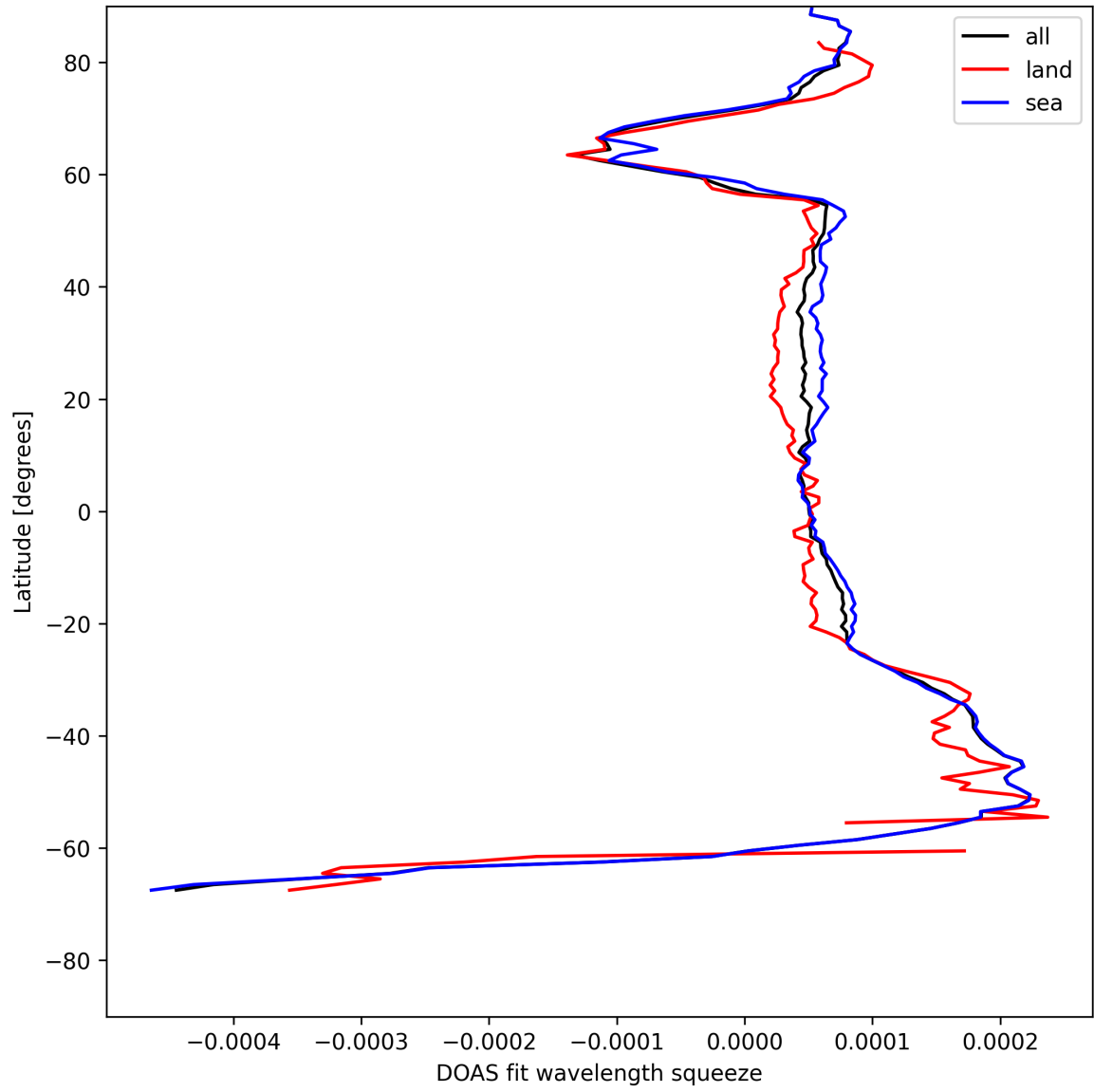
Figure 24: Zonal average of “DOAS fit wavelength squeeze” for 2025-07-16 to 2025-07-16.
