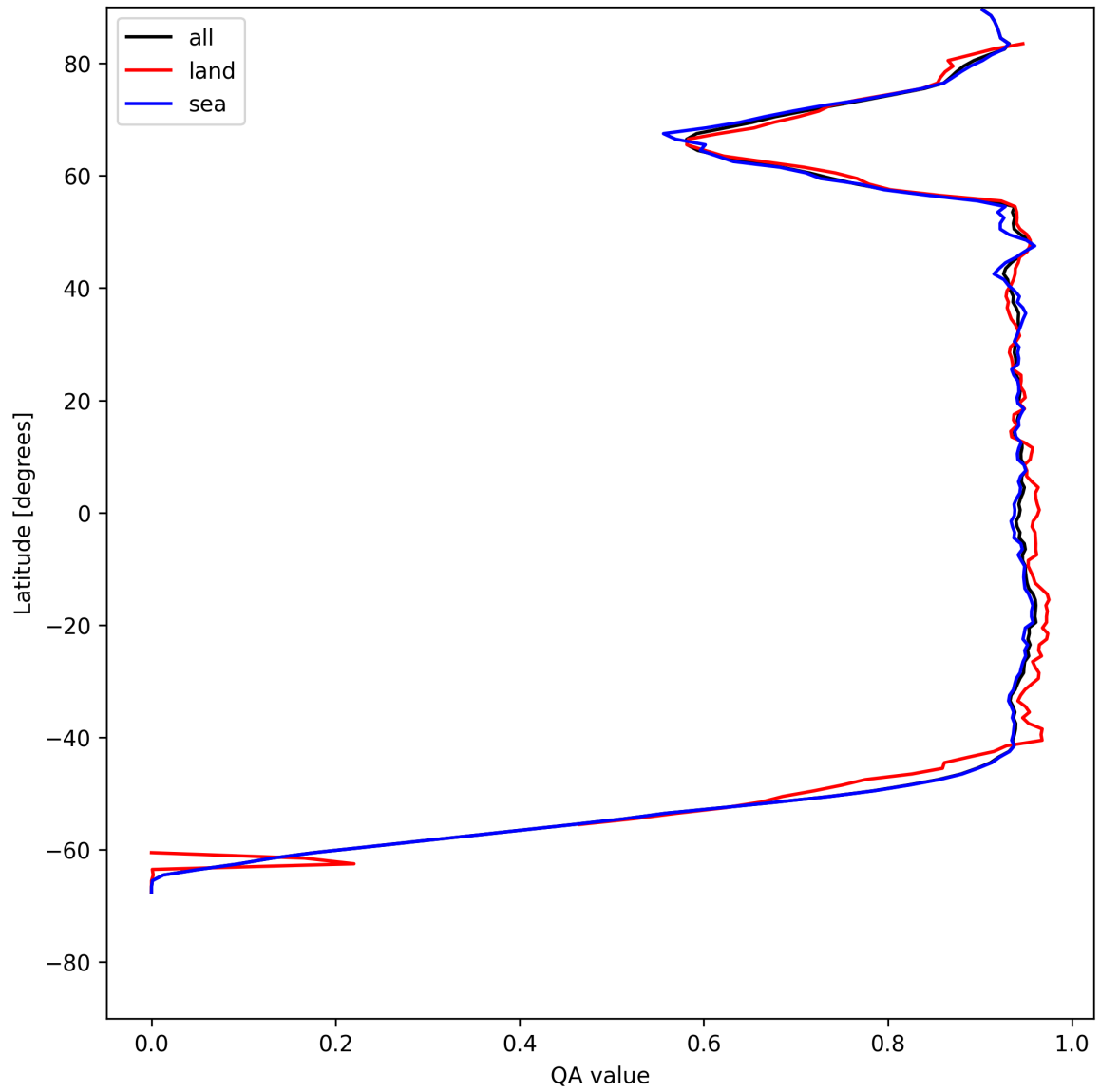
Figure 16: Zonal average of “QA value” for 2025-07-16 to 2025-07-16.
