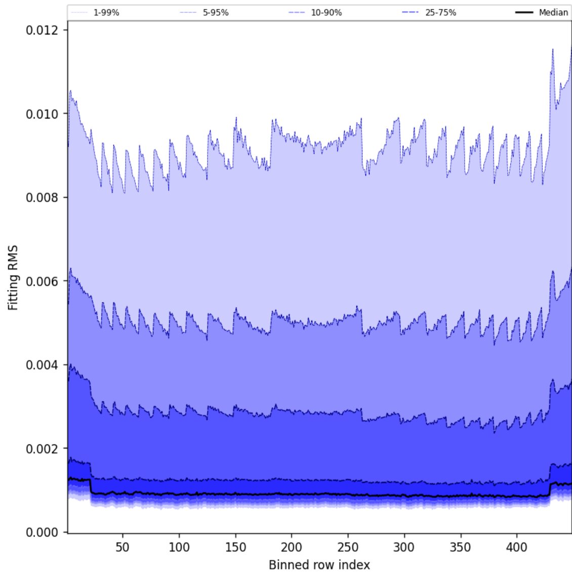
Figure 46: Along track statistics of “Fitting RMS” for 2025-07-16 to 2025-07-16
