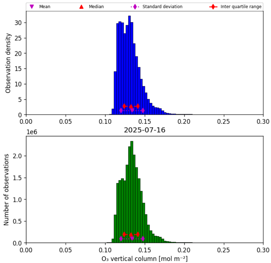
Figure 29: Histogram of “O 3 vertical column” for 2025-07-16 to 2025-07-16
