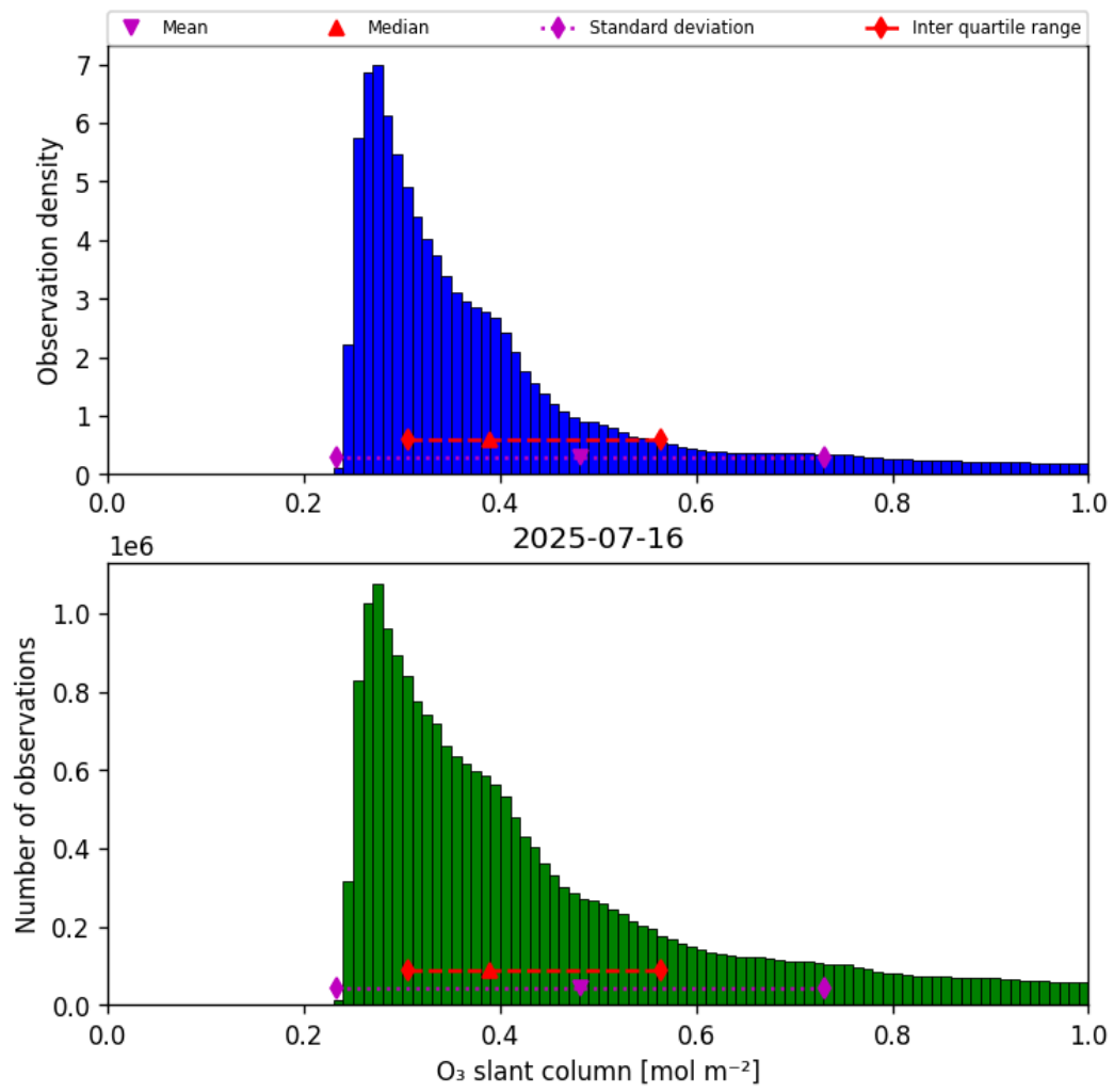
Figure 31: Histogram of “O 3 slant column” for 2025-07-16 to 2025-07-16
