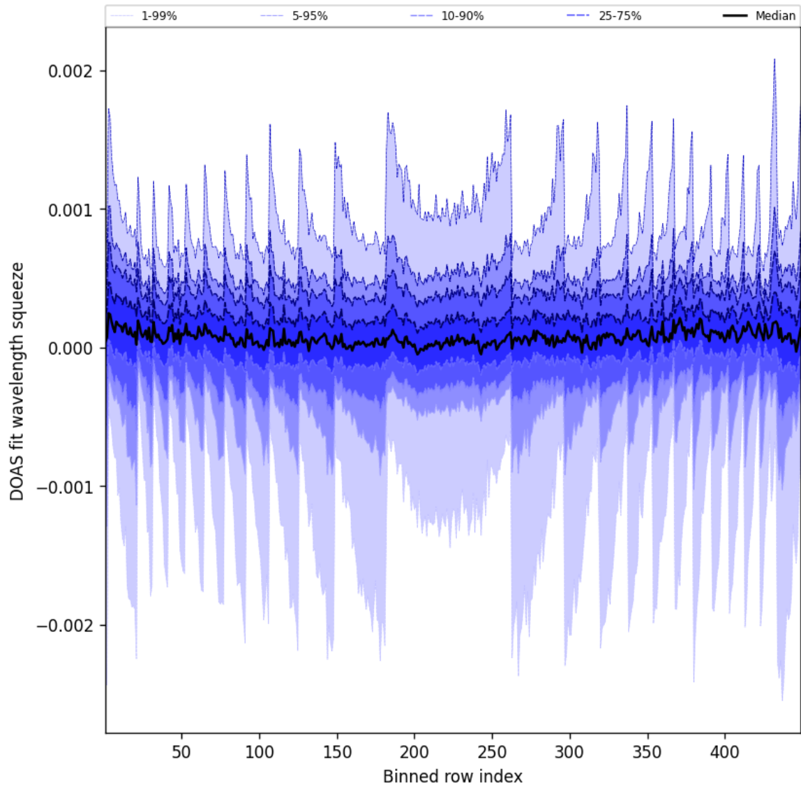
Figure 48: Along track statistics of “DOAS fit wavelength squeeze” for 2025-07-16 to 2025-07-16
