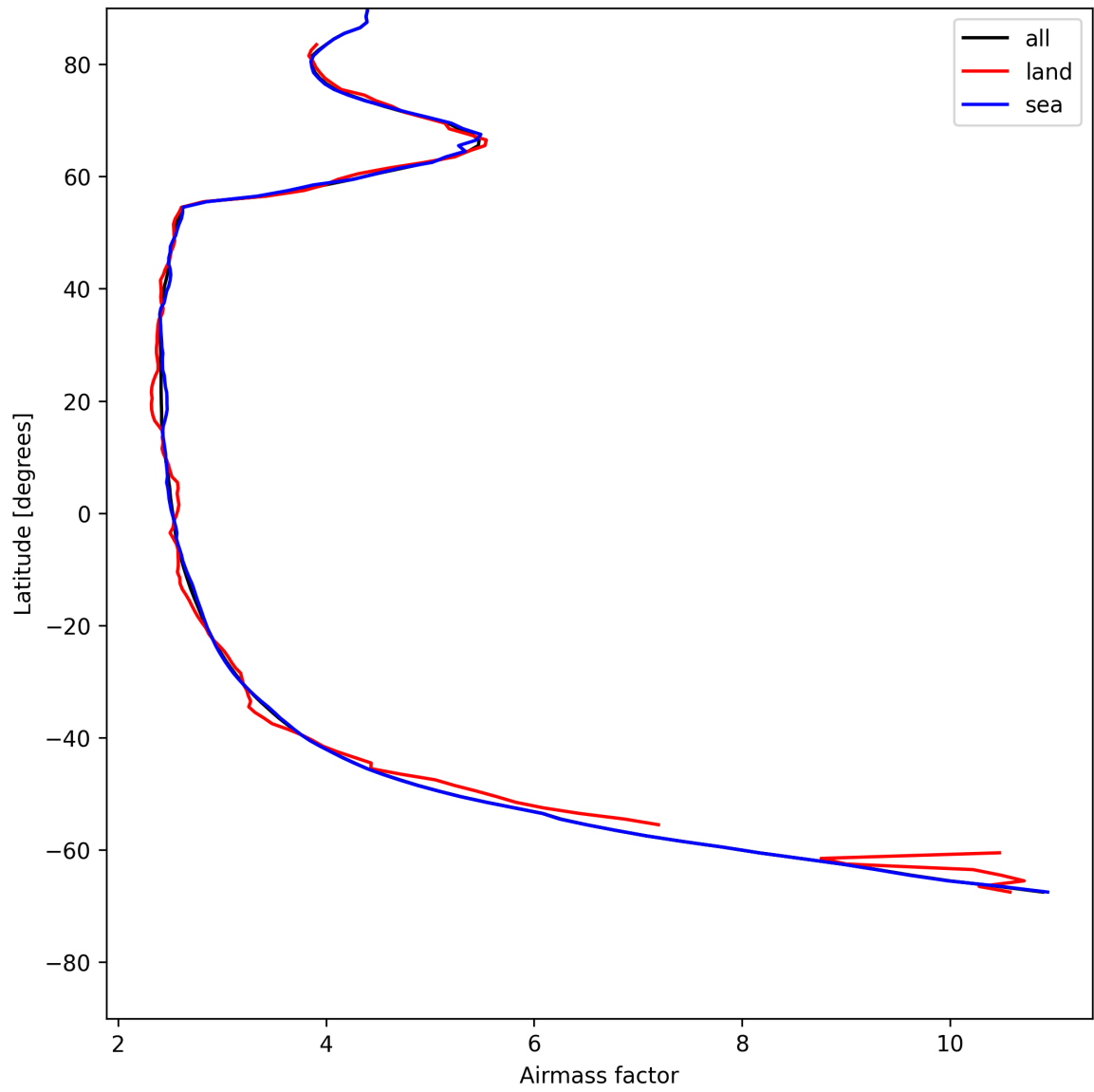
Figure 25: Zonal average of “Airmass factor” for 2025-07-16 to 2025-07-16.
