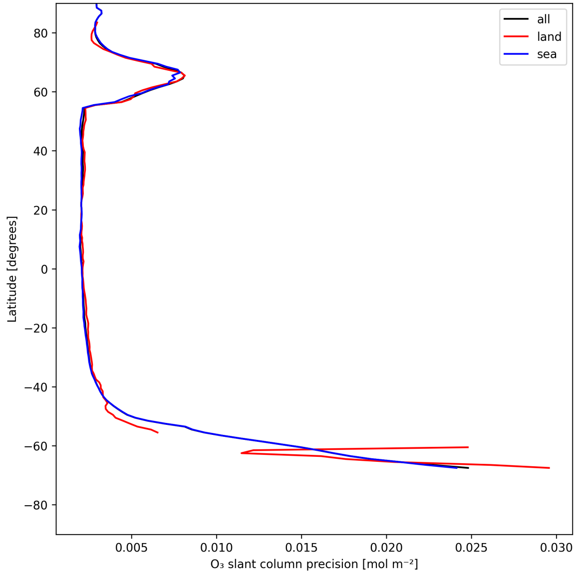
Figure 20: Zonal average of “O 3 slant column precision” for 2025-07-16 to 2025-07-16.
