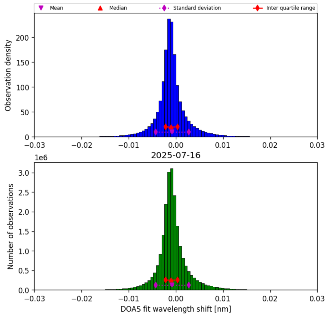
Figure 35: Histogram of “DOAS fit wavelength shift” for 2025-07-16 to 2025-07-16
