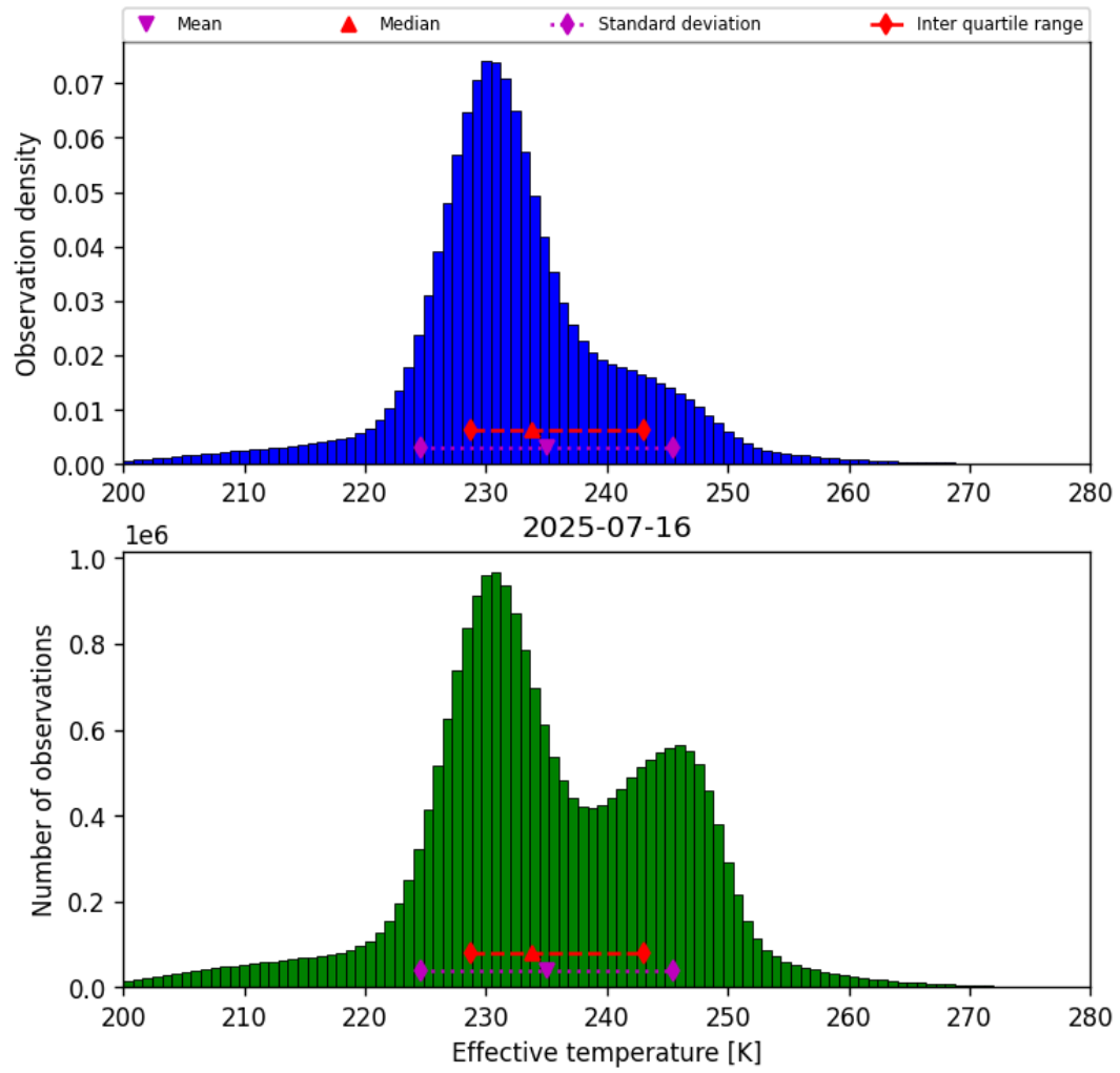
Figure 38: Histogram of “Effective temperature” for 2025-07-16 to 2025-07-16
