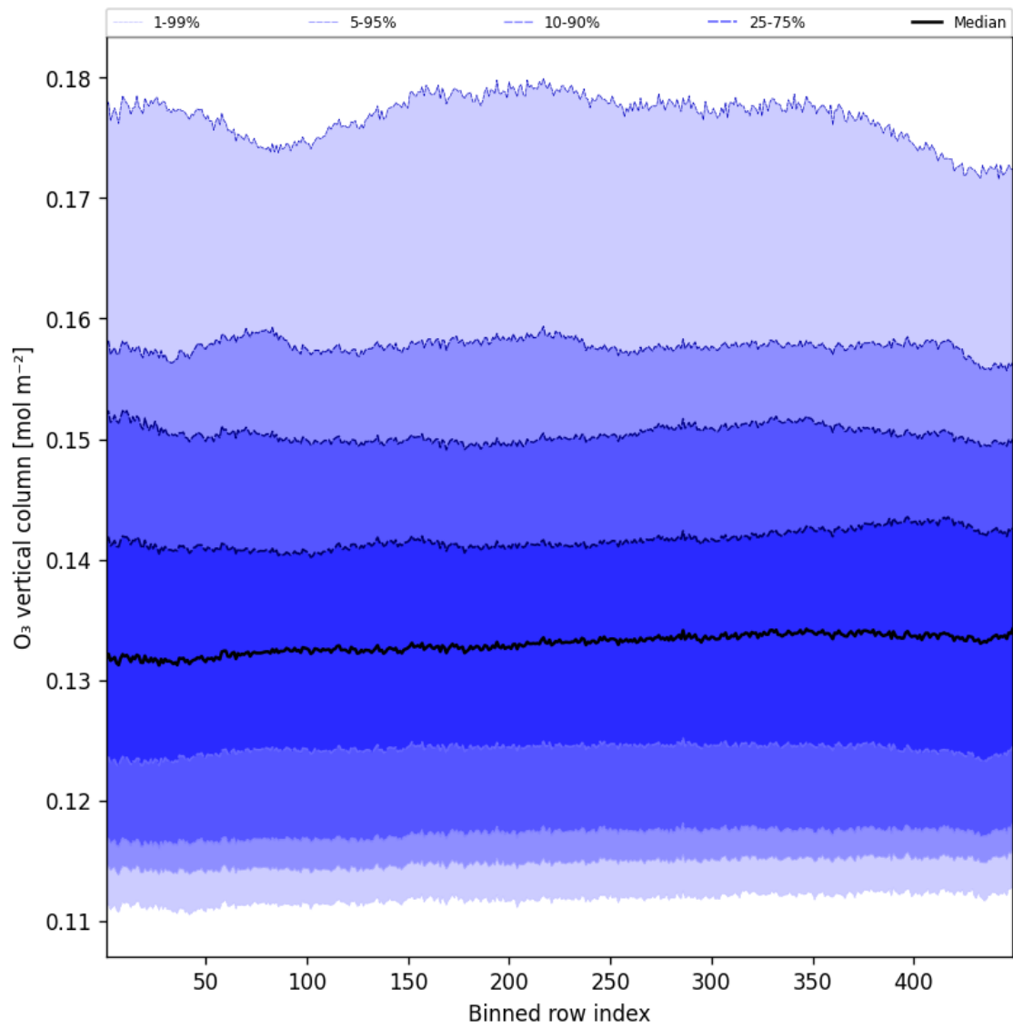
Figure 41: Along track statistics of “O 3 vertical column” for 2025-07-16 to 2025-07-16
