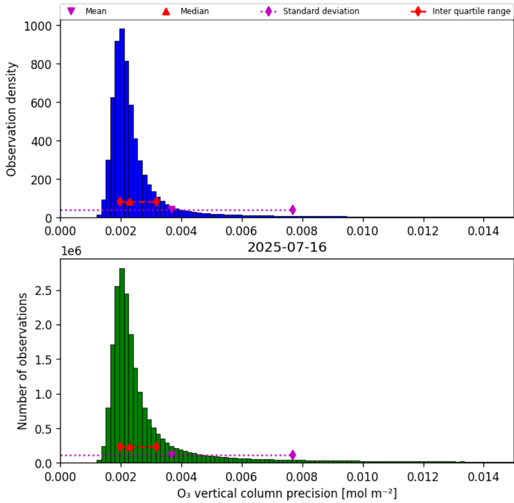
Figure 30: Histogram of "O 3 vertical column precision" for 2025-07-16 to 2025-07-16
