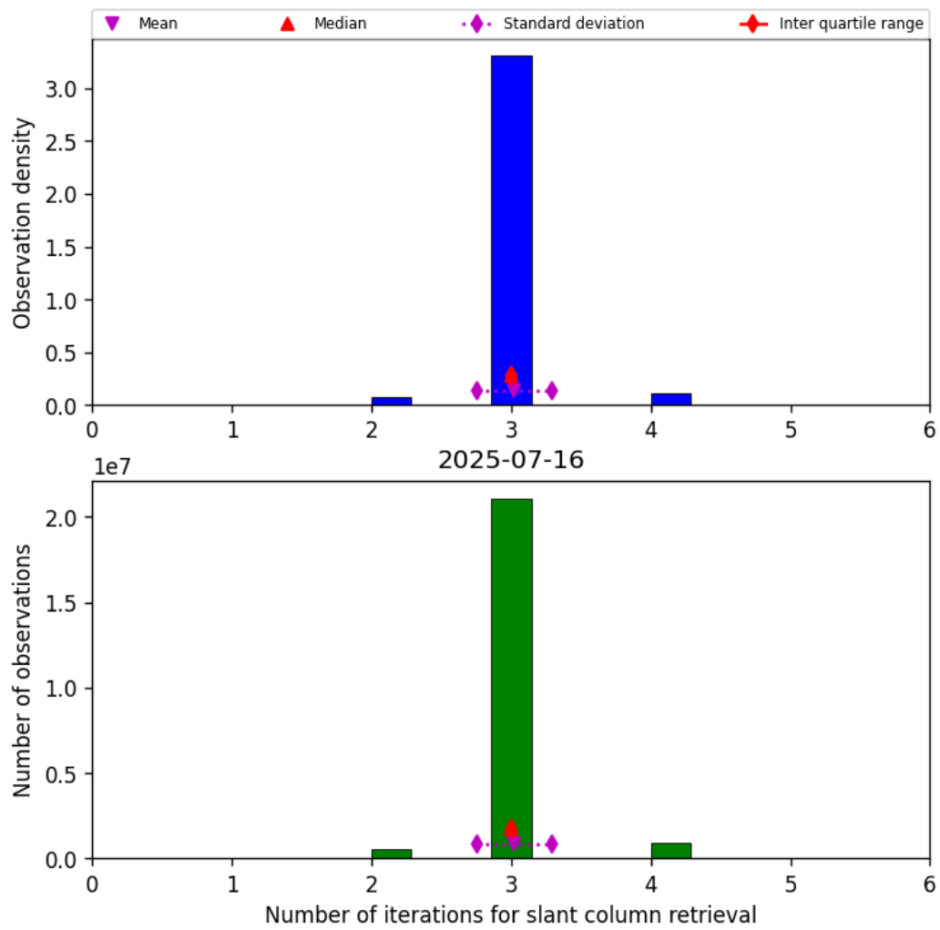
Figure 33: Histogram of "Number of iterations for slant column retrieval" for 2025-07-16 to 2025-07-16
