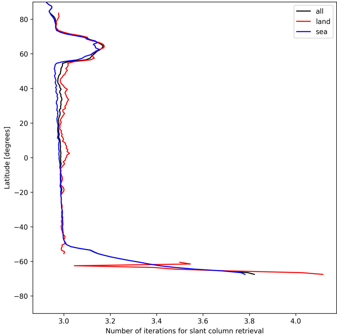
Figure 21: Zonal average of “Number of iterations for slant column retrieval” for 2025-07-16 to 2025-07-16.
