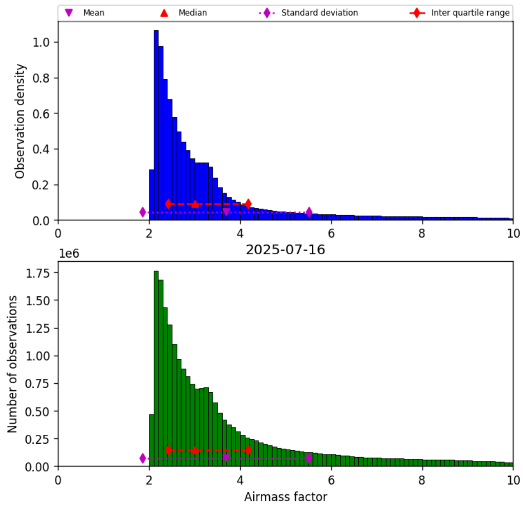
Figure 37: Histogram of “Airmass factor” for 2025-07-16 to 2025-07-16
