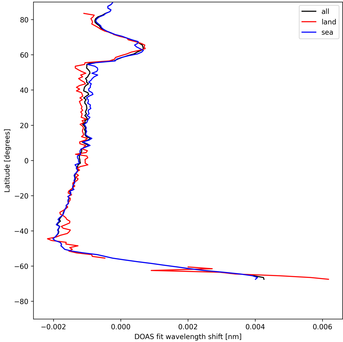
Figure 23: Zonal average of “DOAS fit wavelength shift” for 2025-07-16 to 2025-07-16.
