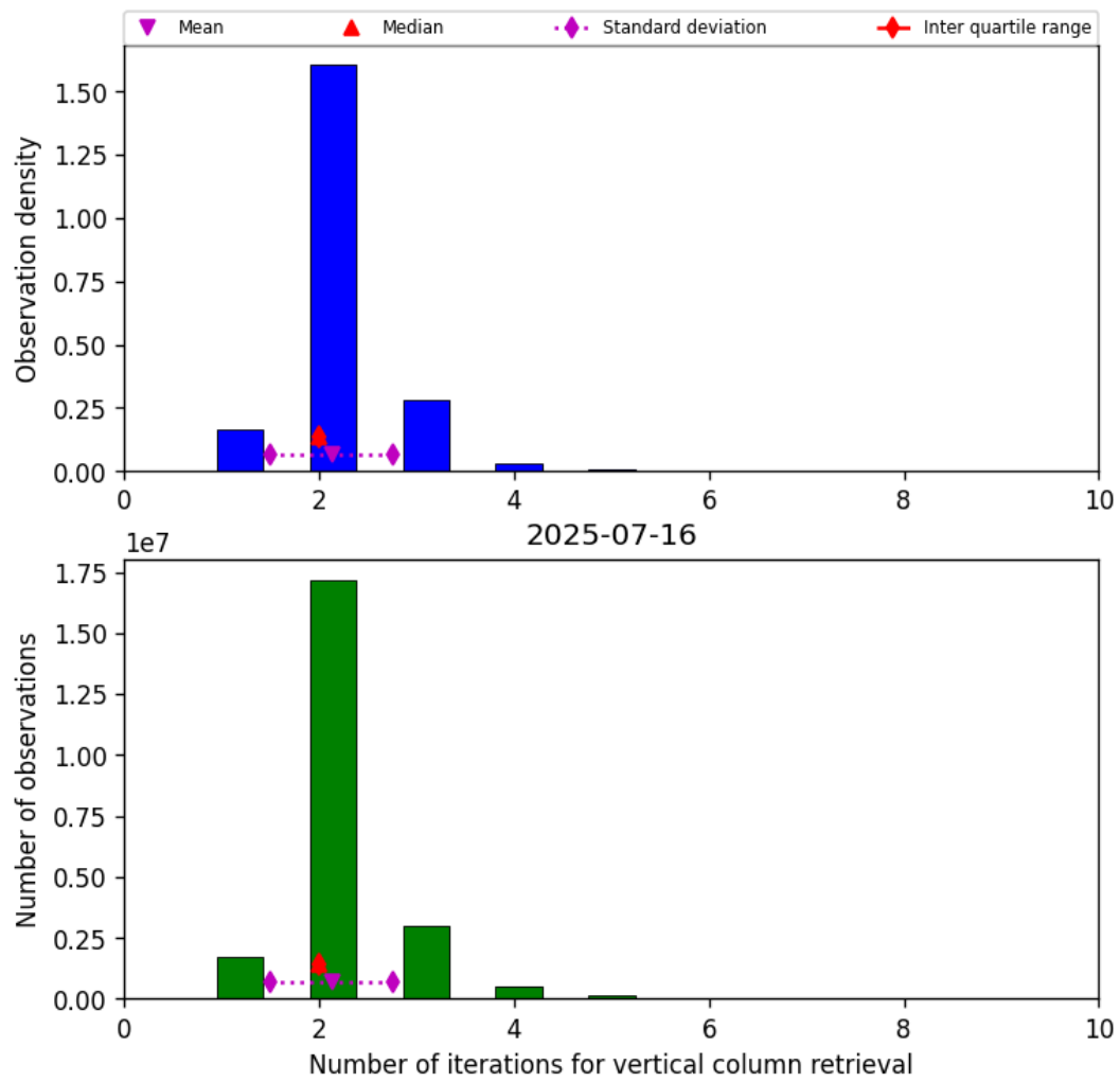
Figure 39: Histogram of “Number of iterations for vertical column retrieval” for 2025-07-16 to 2025-07-16
