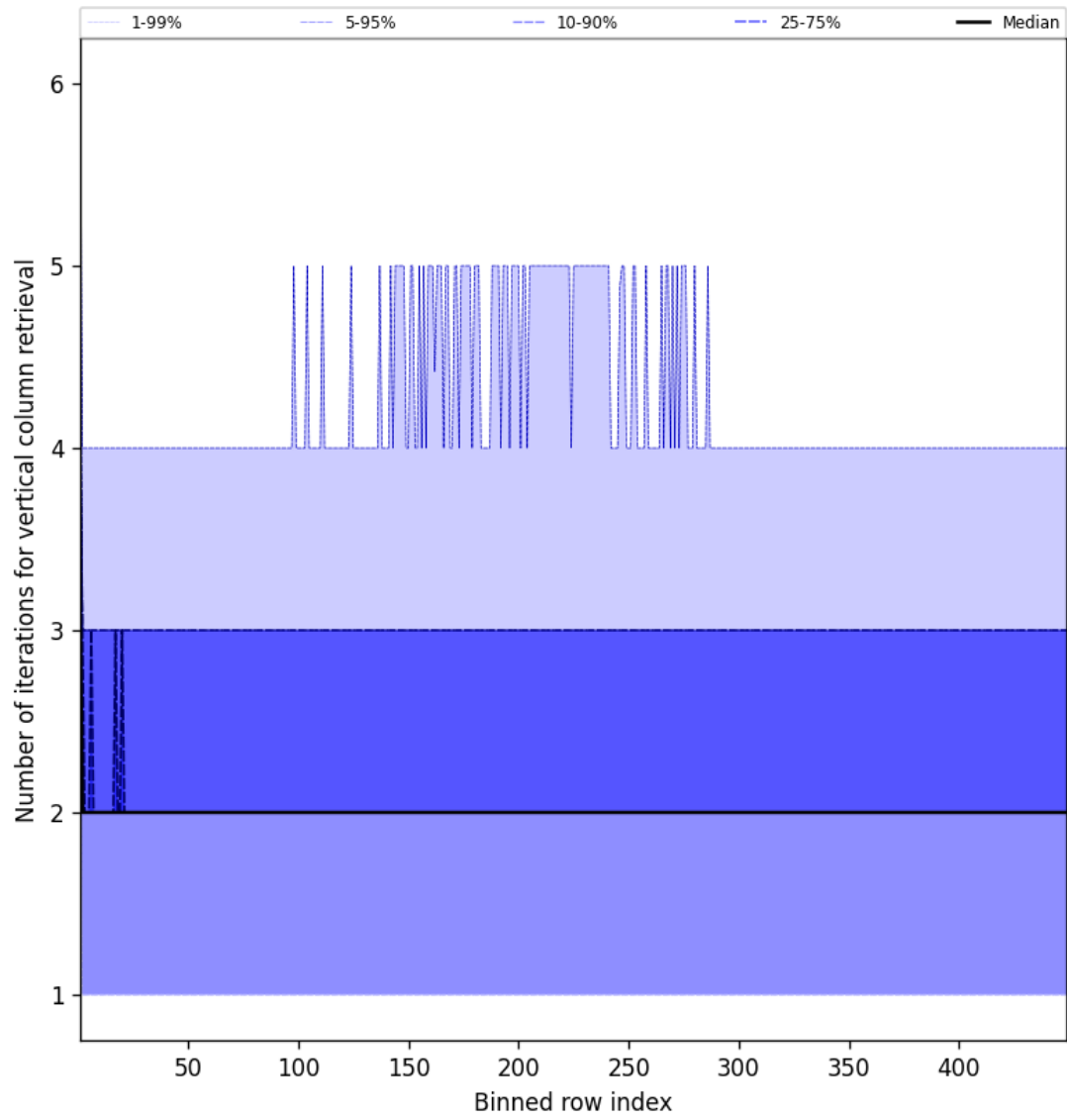
Figure 51: Along track statistics of “Number of iterations for vertical column retrieval” for 2025-07-16 to 2025-07-16
