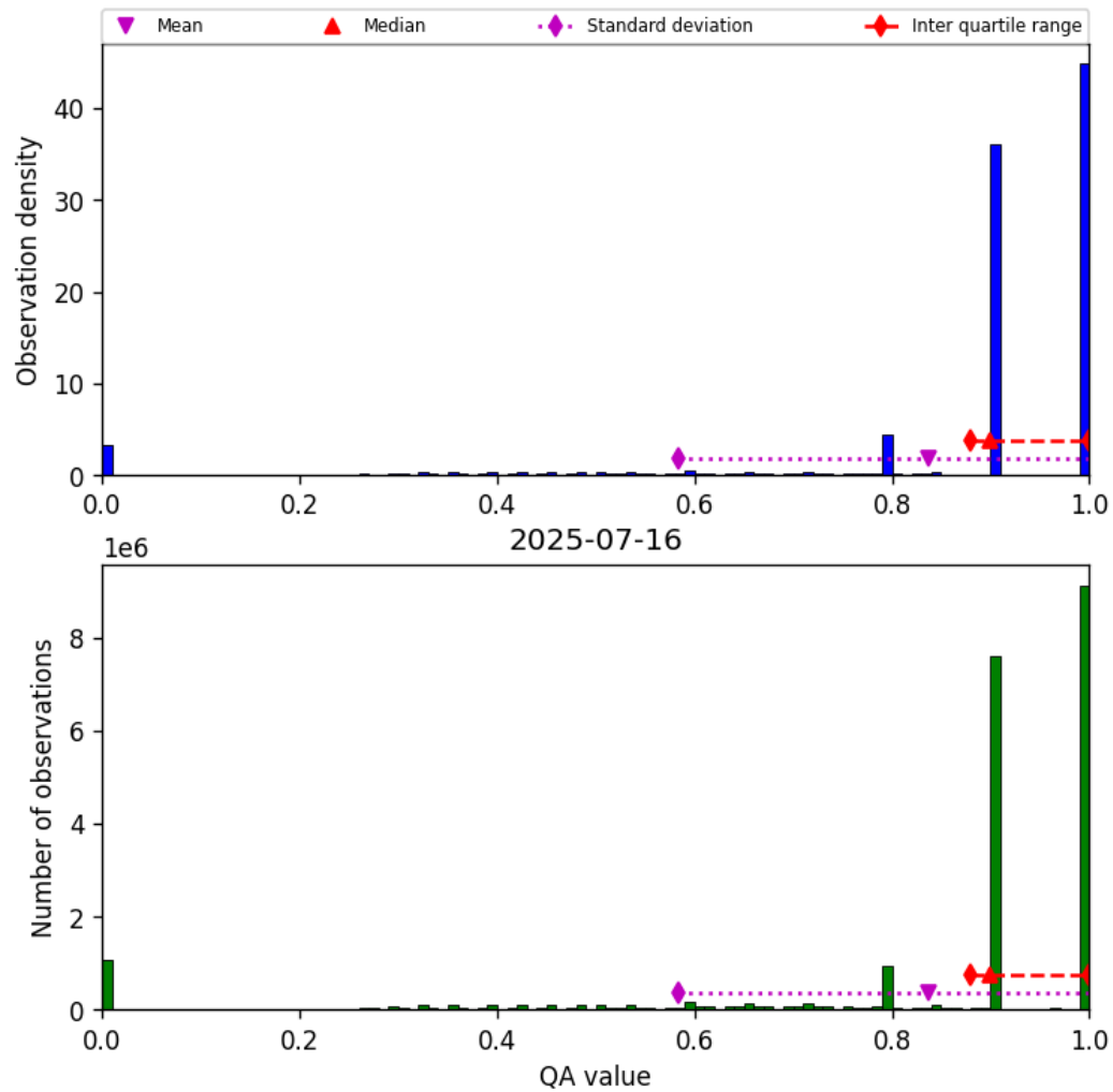
Figure 28: Histogram of “QA value” for 2025-07-16 to 2025-07-16
