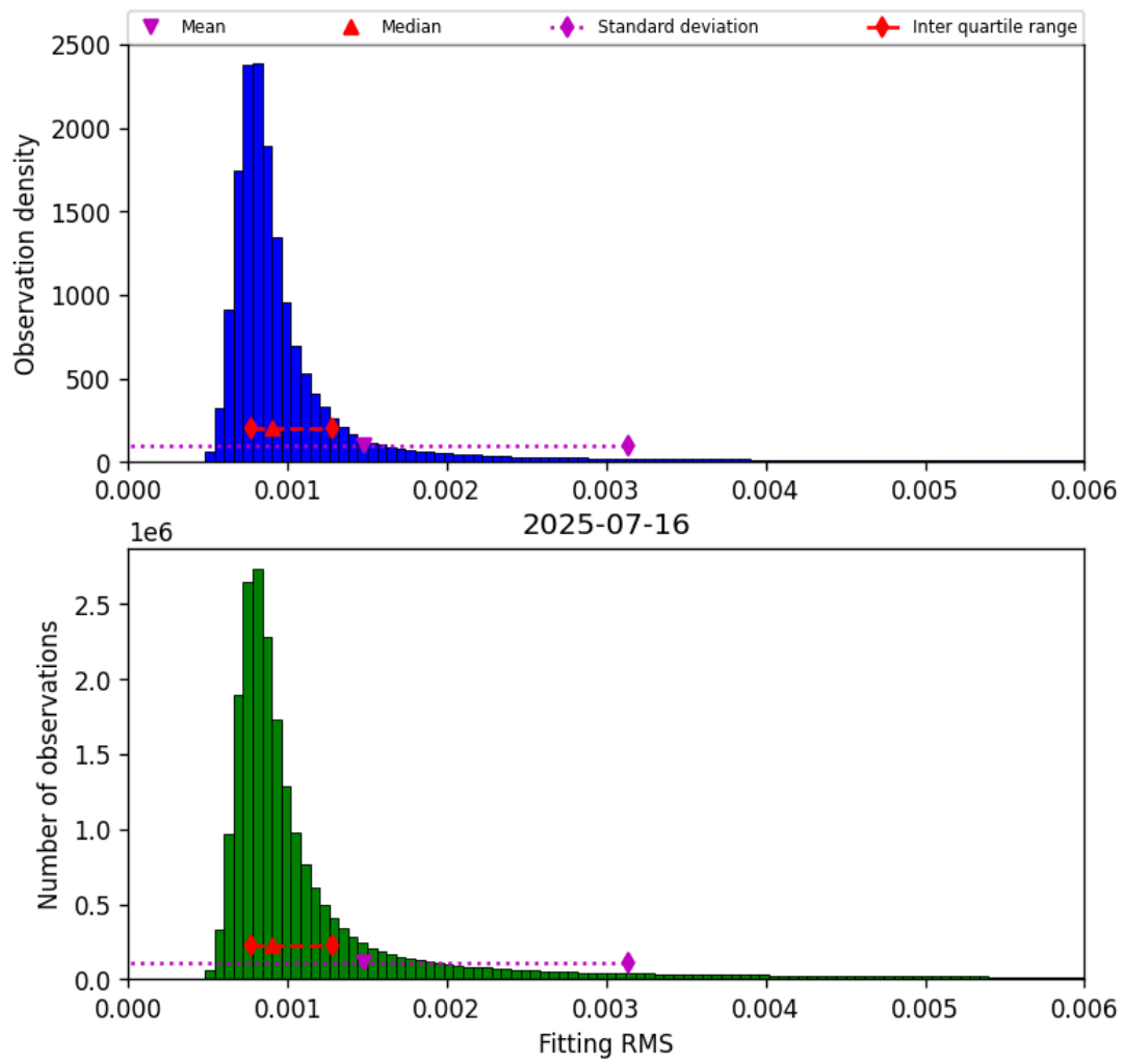
Figure 34: Histogram of “Fitting RMS” for 2025-07-16 to 2025-07-16
