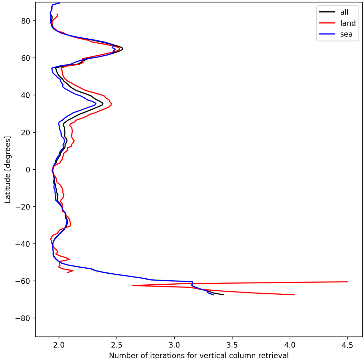
Figure 27: Zonal average of “Number of iterations for vertical column retrieval” for 2025-07-16 to 2025-07-16.
