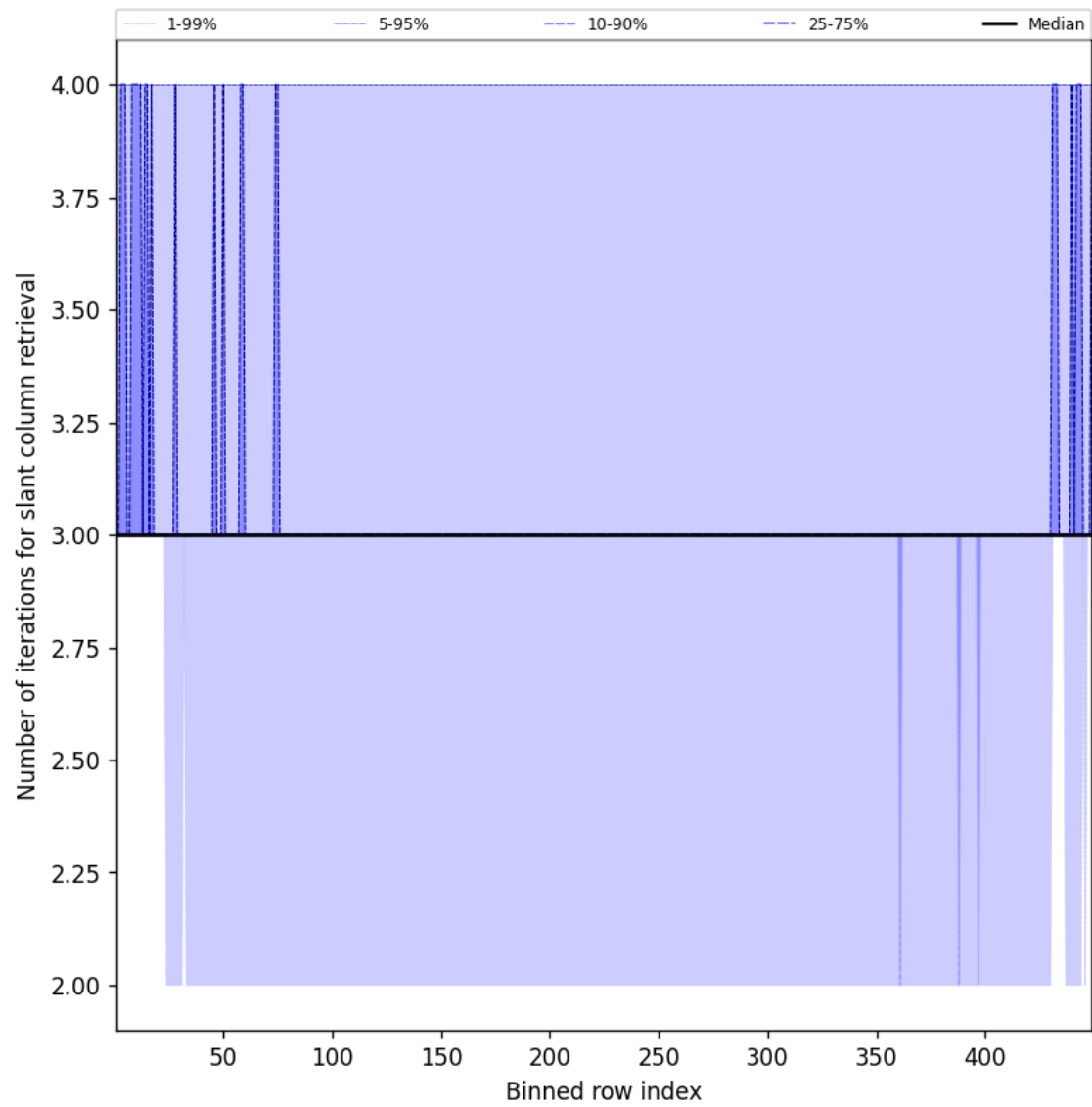
Figure 45: Along track statistics of “Number of iterations for slant column retrieval” for 2025-07-16 to 2025-07-16
