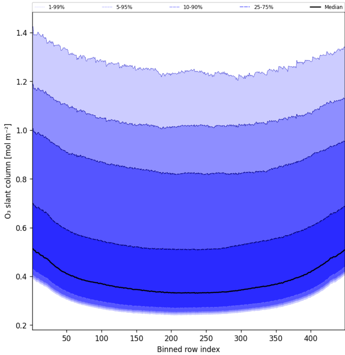
Figure 43: Along track statistics of “O 3 slant column” for 2025-07-16 to 2025-07-16
