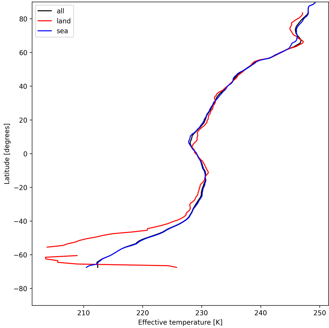
Figure 26: Zonal average of “Effective temperature” for 2025-07-16 to 2025-07-16.
