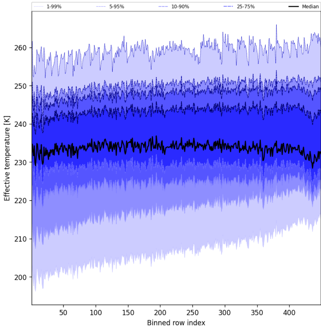
Figure 50: Along track statistics of “Effective temperature” for 2025-07-16 to 2025-07-16
