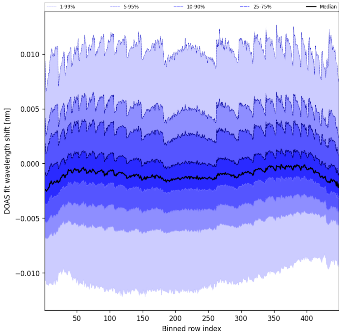
Figure 47: Along track statistics of “DOAS fit wavelength shift” for 2025-07-16 to 2025-07-16
