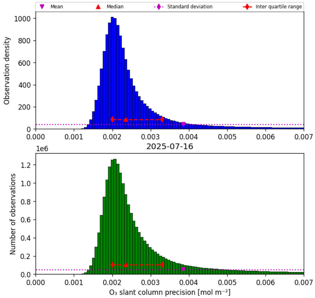
Figure 32: Histogram of “O 3 slant column precision” for 2025-07-16 to 2025-07-16
