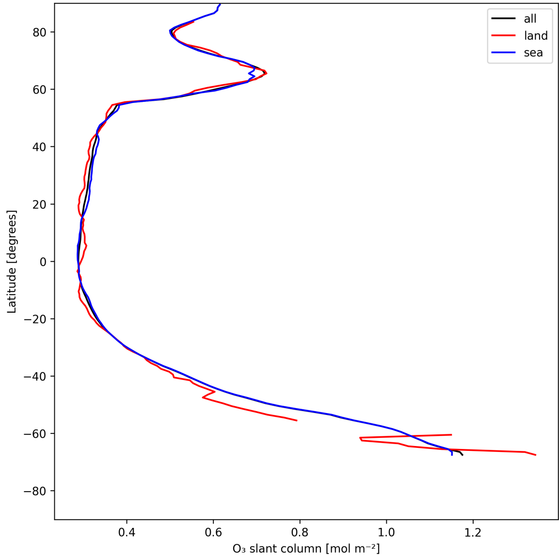
Figure 19: Zonal average of “O 3 slant column” for 2025-07-16 to 2025-07-16.
