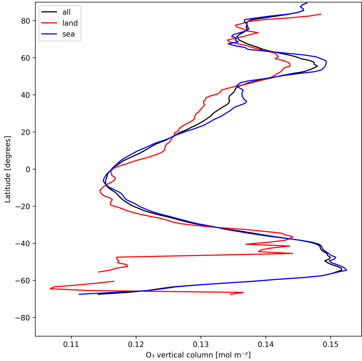
Figure 17: Zonal average of “O 3 vertical column” for 2025-07-16 to 2025-07-16.
