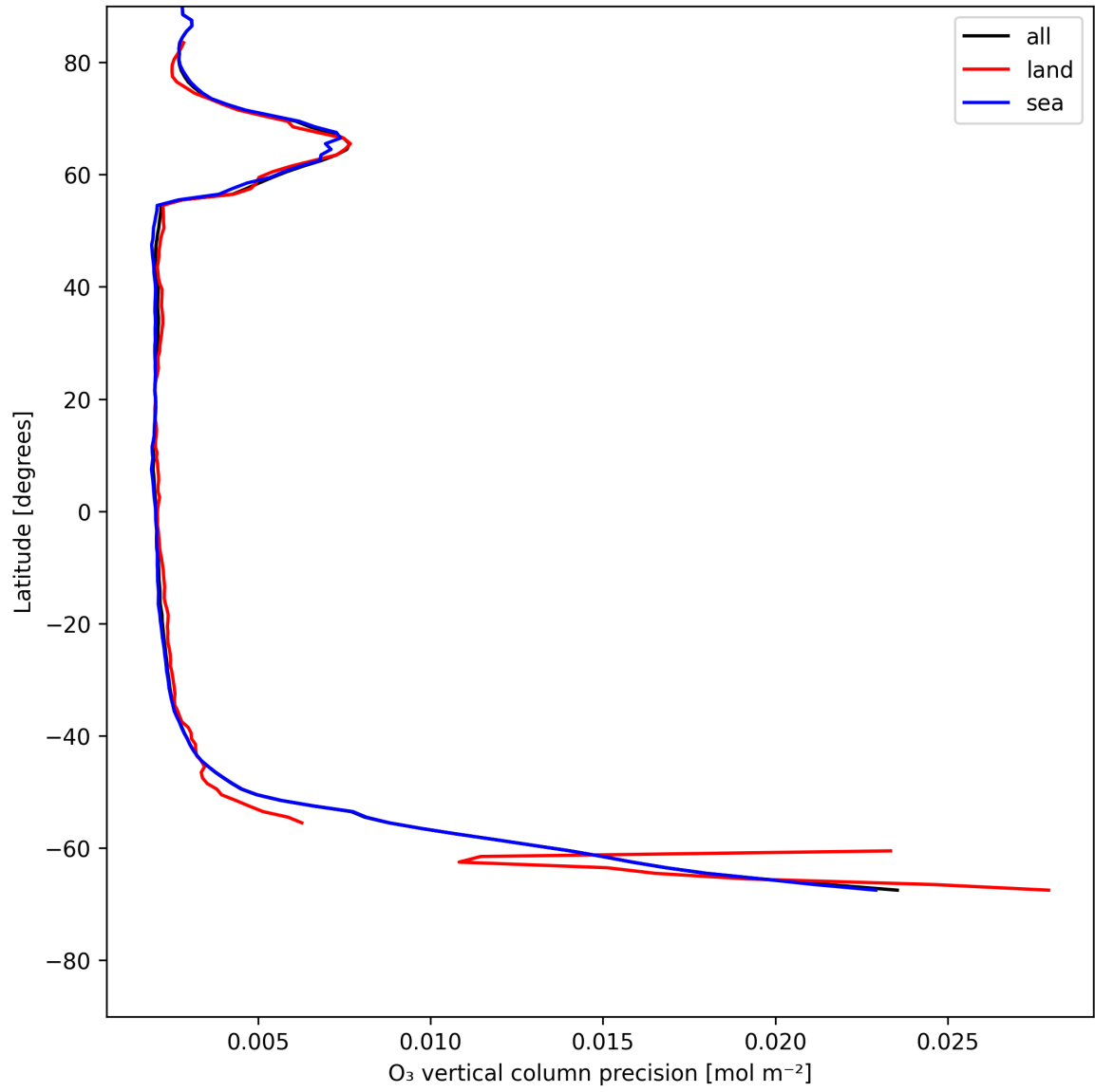
Figure 18: Zonal average of “O 3 vertical column precision” for 2025-07-16 to 2025-07-16.
