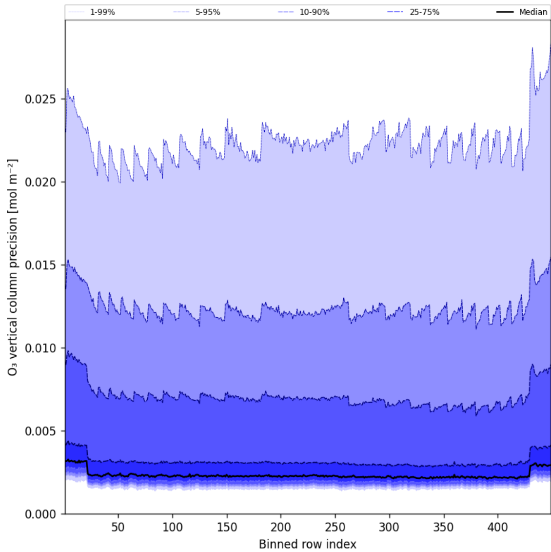
Figure 42: Along track statistics of “O 3 vertical column precision” for 2025-07-16 to 2025-07-16
