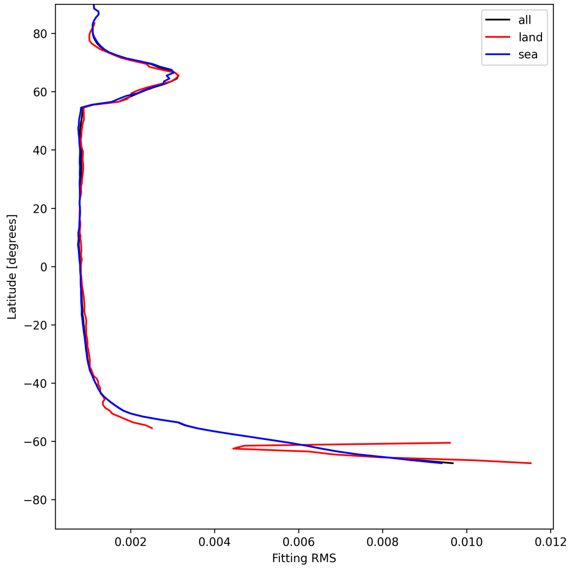
Figure 22: Zonal average of “Fitting RMS” for 2025-07-16 to 2025-07-16.
