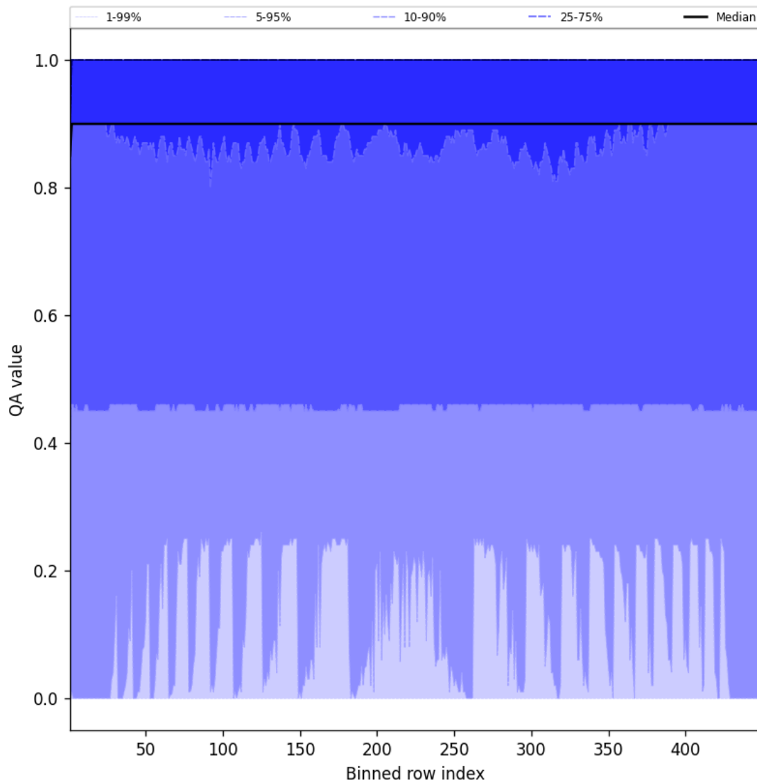
Figure 40: Along track statistics of “QA value” for 2025-07-16 to 2025-07-16
