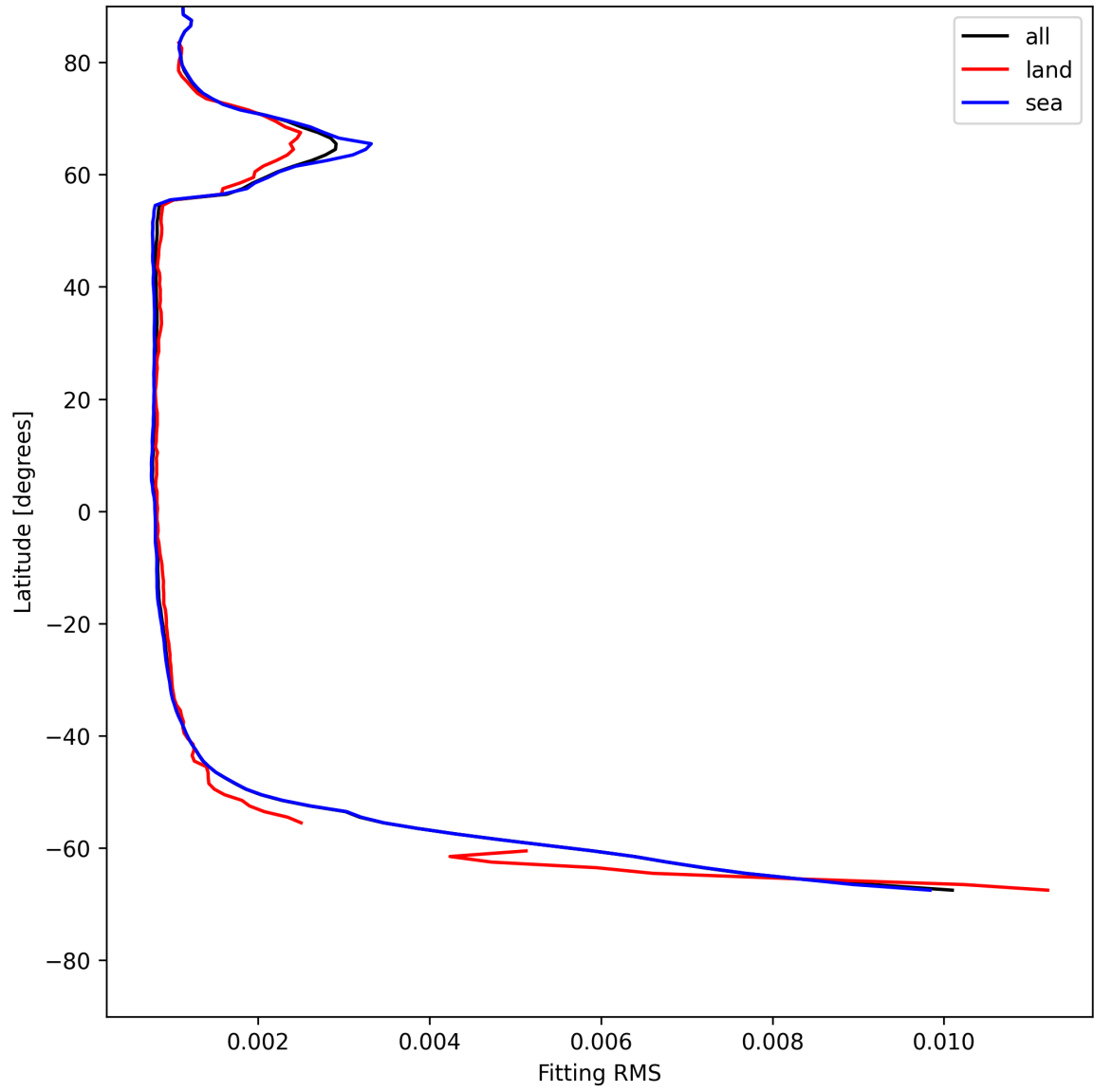
Figure 22: Zonal average of “Fitting RMS” for 2025-07-17 to 2025-07-18.
