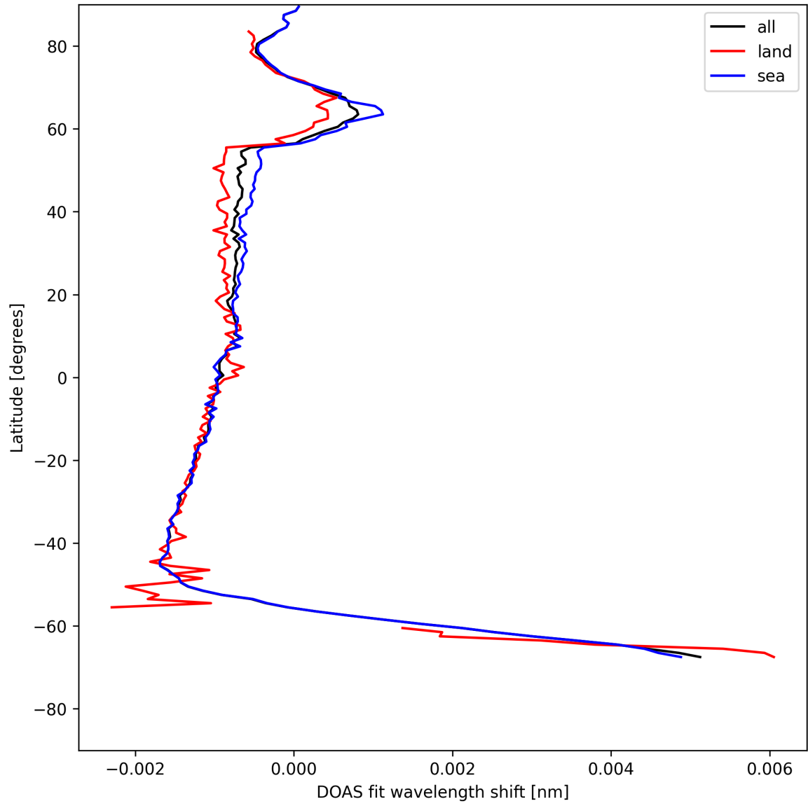
Figure 23: Zonal average of “DOAS fit wavelength shift” for 2025-07-17 to 2025-07-18.
