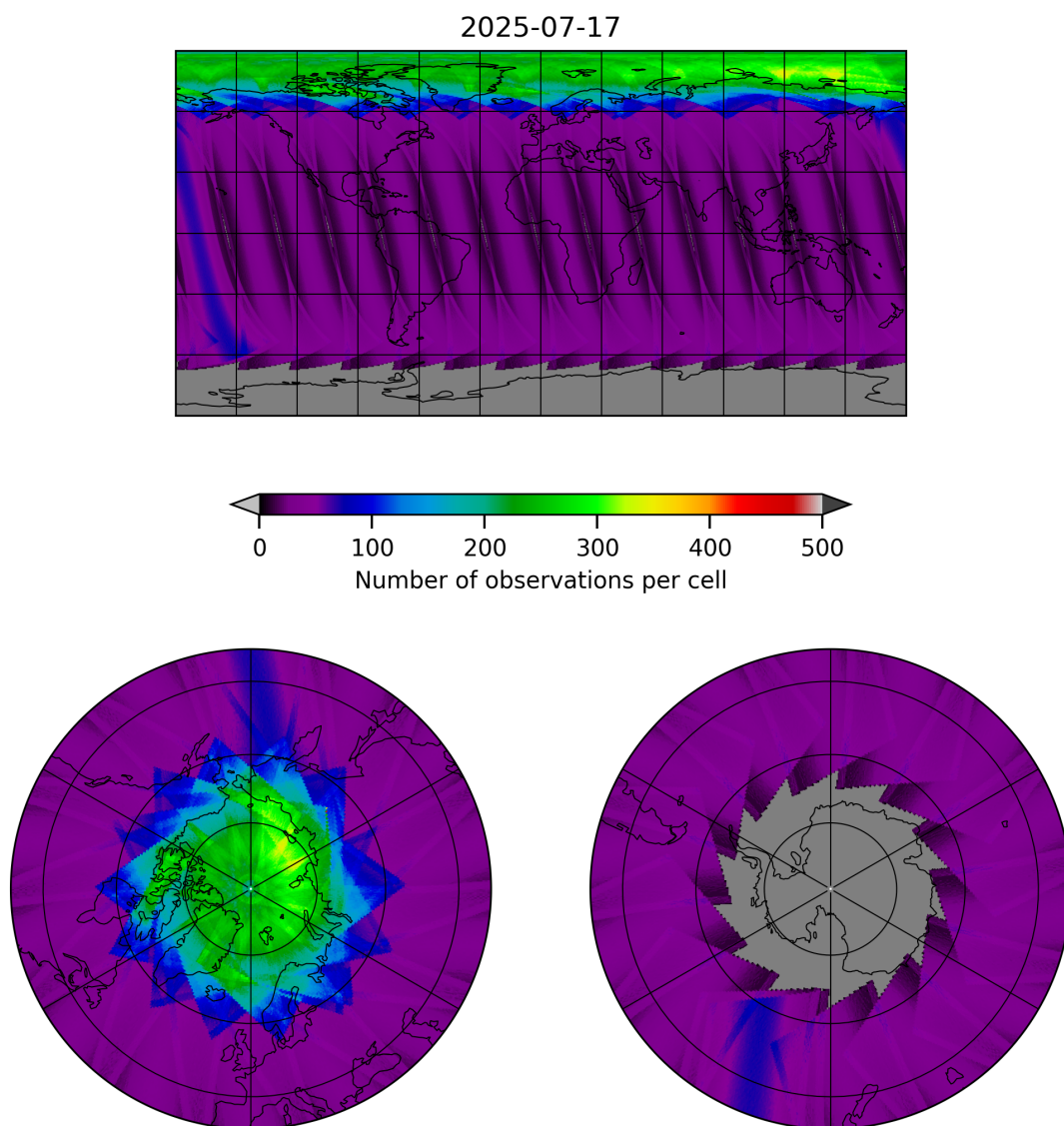
Figure 15: Map of the number of observations for 2025-07-17 to 2025-07-18
