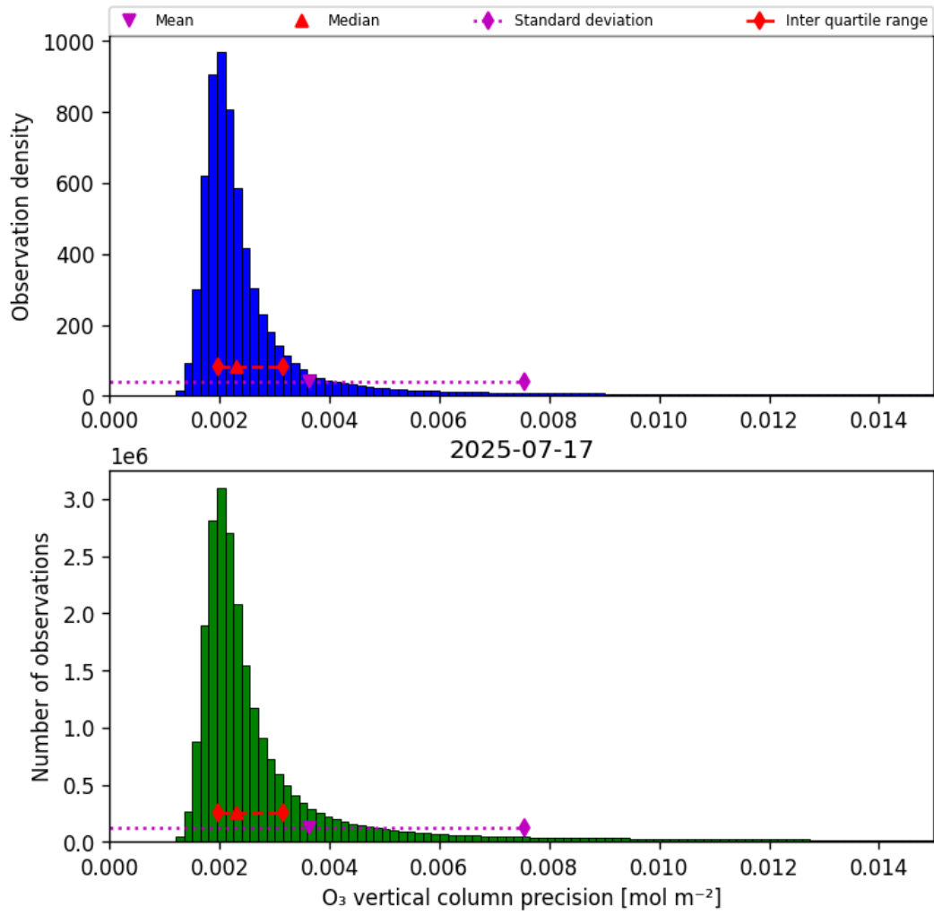
Figure 30: Histogram of “O 3 vertical column precision” for 2025-07-17 to 2025-07-18
