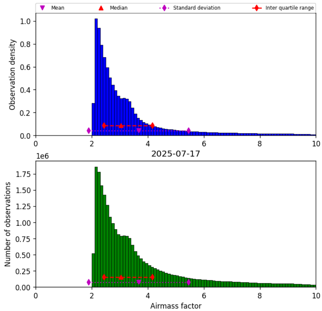
Figure 37: Histogram of “Airmass factor” for 2025-07-17 to 2025-07-18
