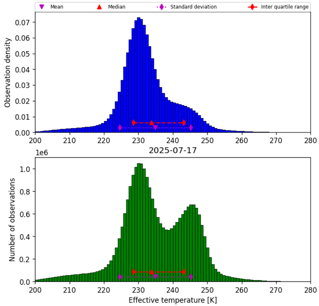
Figure 38: Histogram of “Effective temperature” for 2025-07-17 to 2025-07-18
