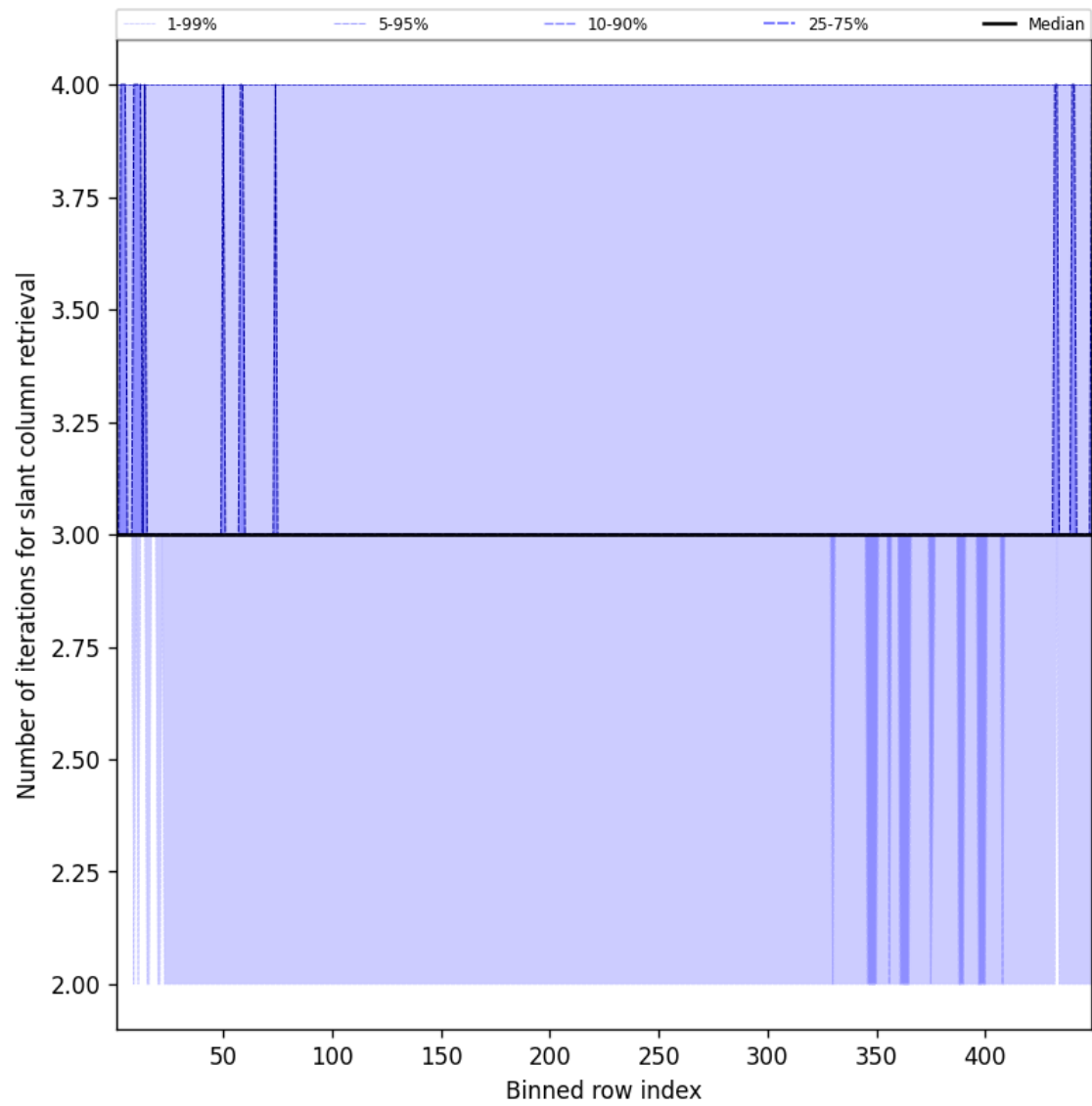
Figure 45: Along track statistics of “Number of iterations for slant column retrieval” for 2025-07-17 to 2025-07-18
