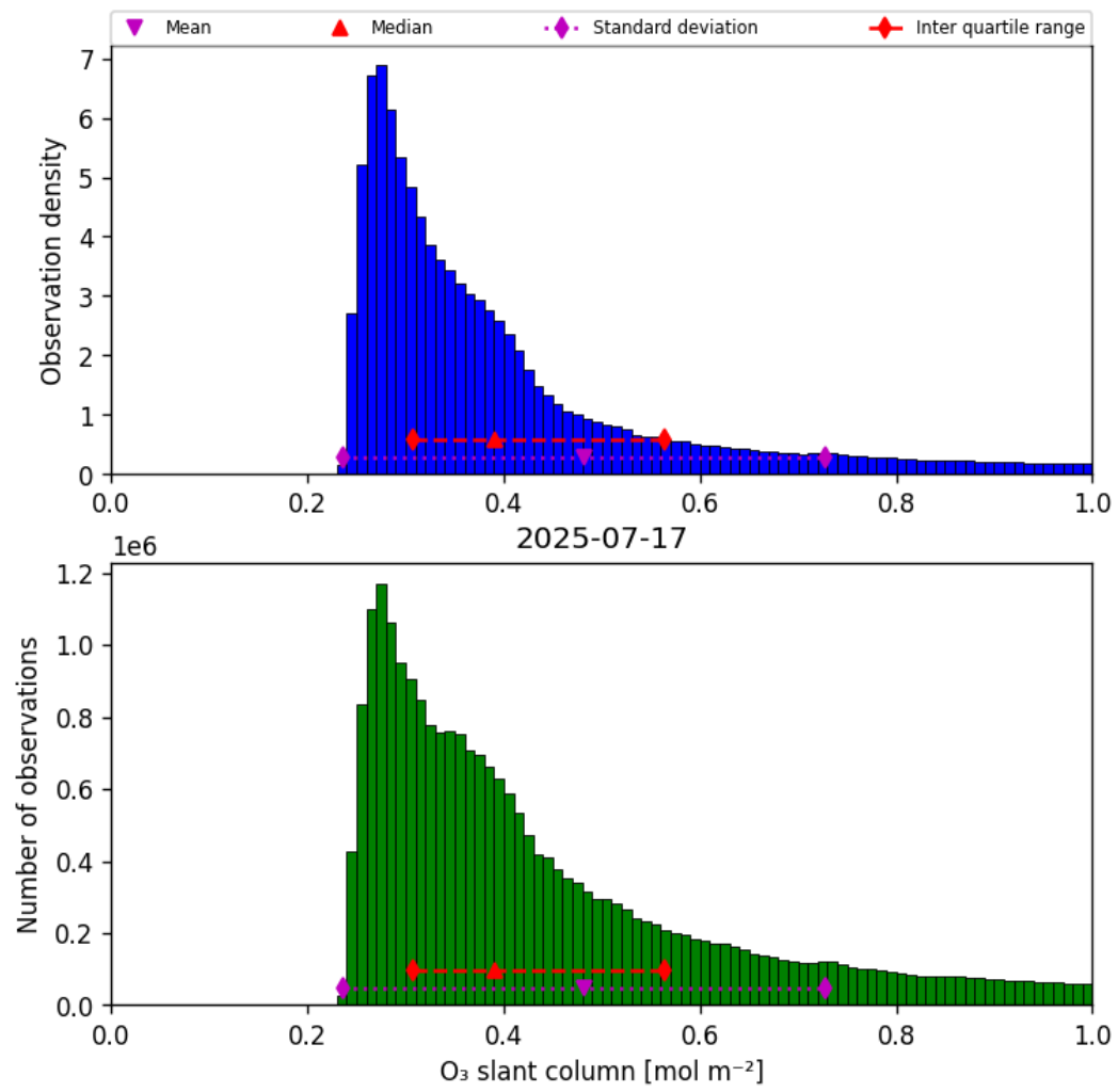
Figure 31: Histogram of “O 3 slant column” for 2025-07-17 to 2025-07-18
