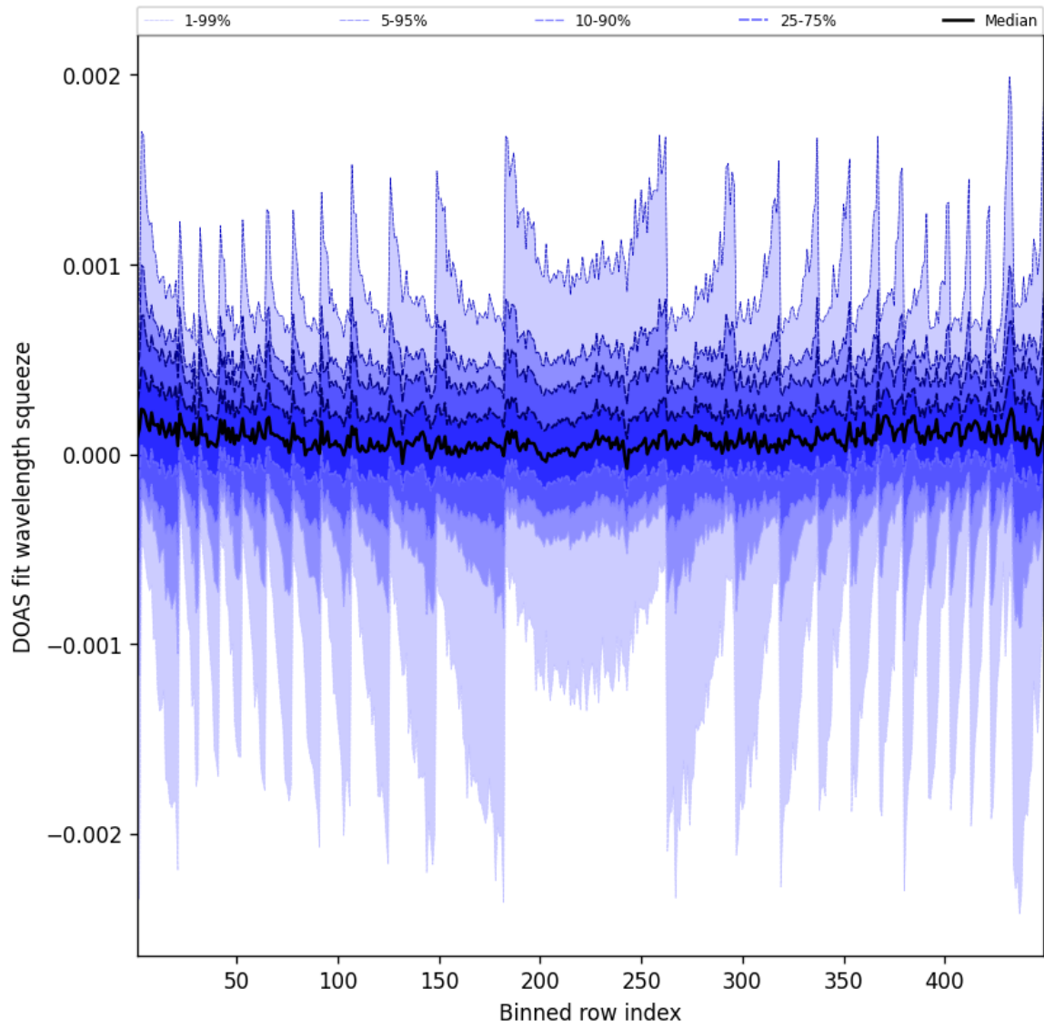
Figure 48: Along track statistics of “DOAS fit wavelength squeeze” for 2025-07-17 to 2025-07-18
