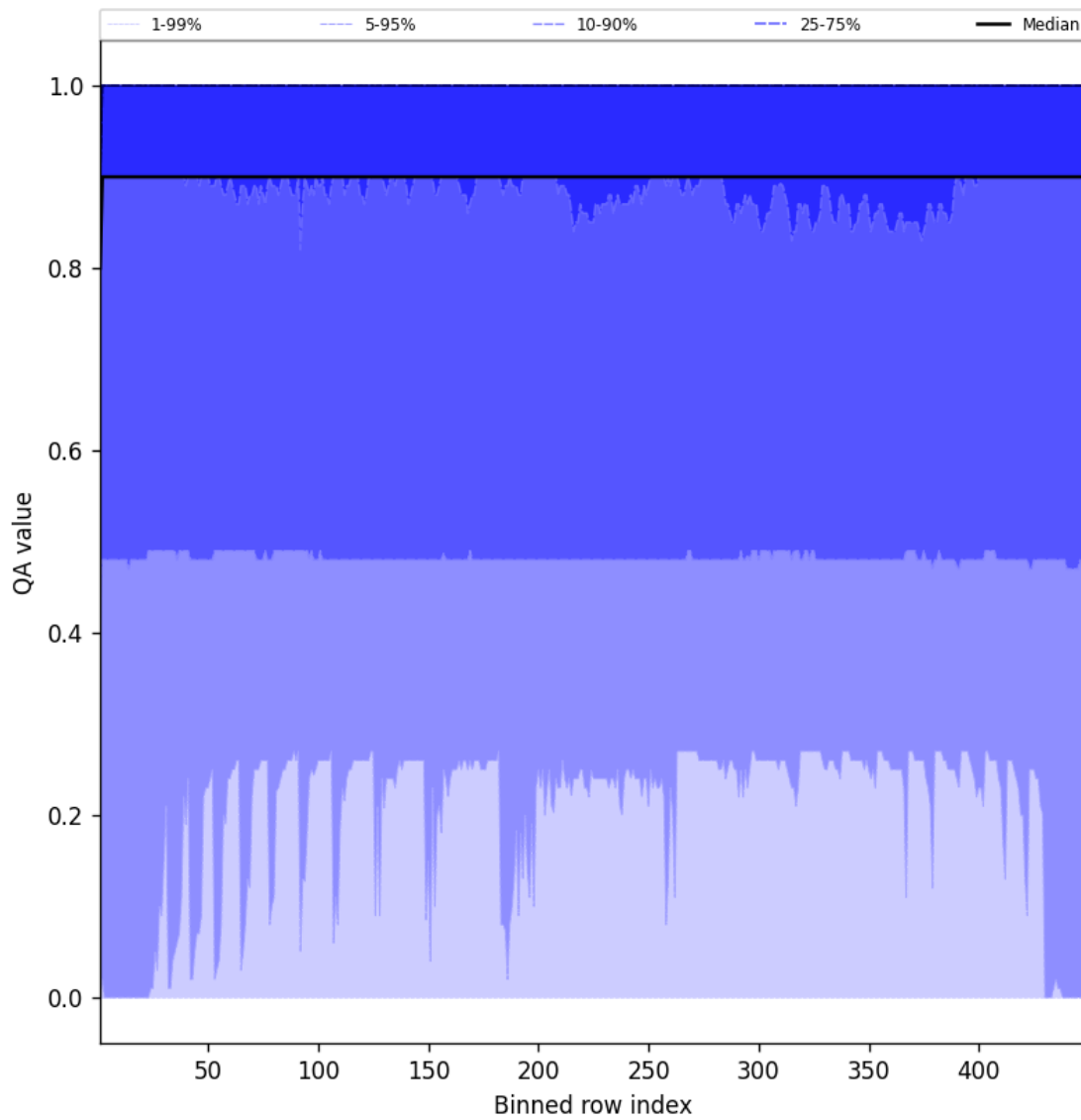
Figure 40: Along track statistics of “QA value” for 2025-07-17 to 2025-07-18
