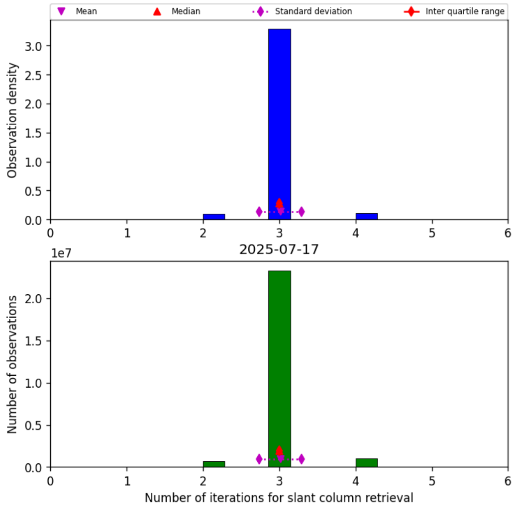
Figure 33: Histogram of “Number of iterations for slant column retrieval” for 2025-07-17 to 2025-07-18
