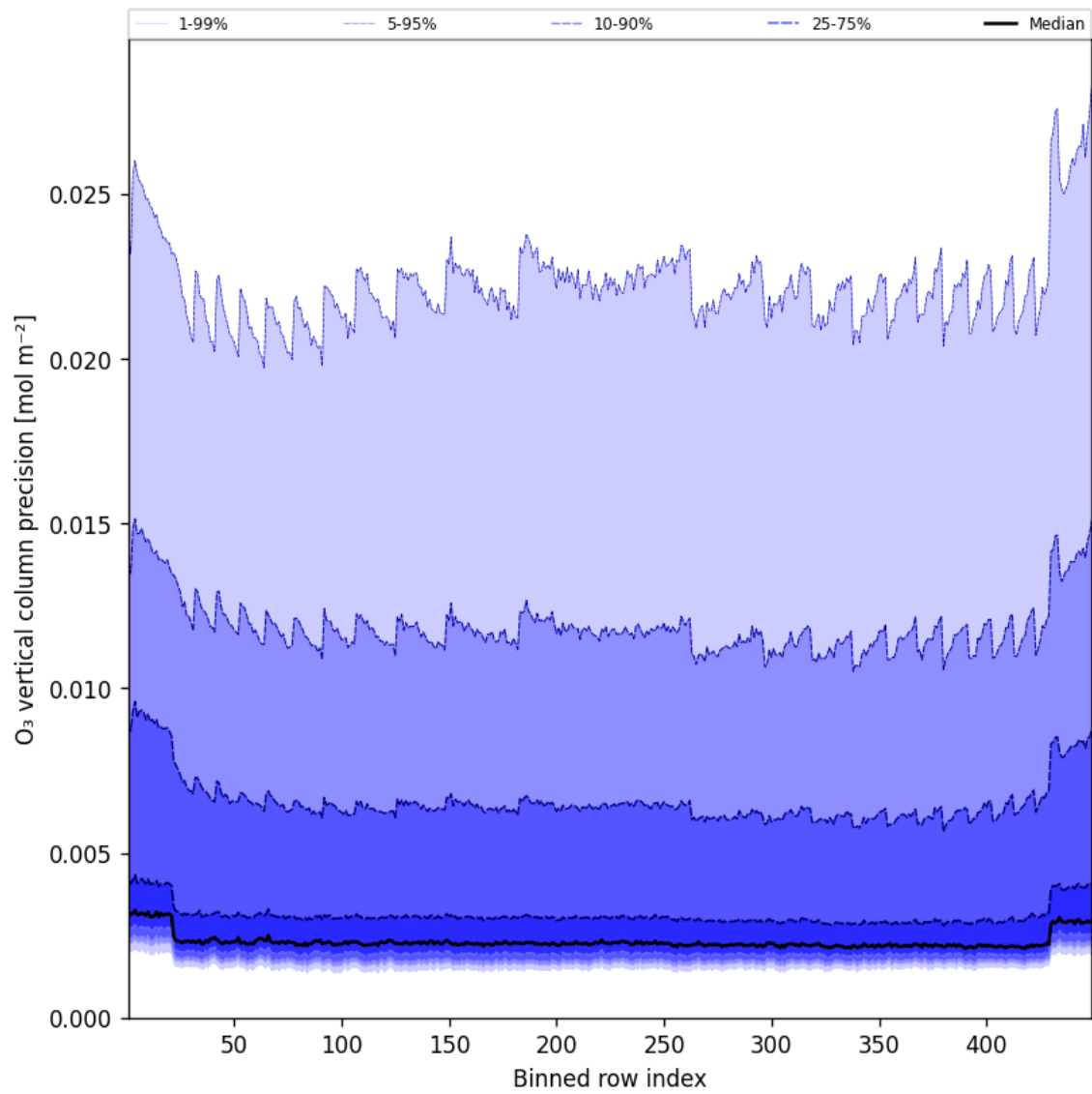
Figure 42: Along track statistics of “O 3 vertical column precision” for 2025-07-17 to 2025-07-18
