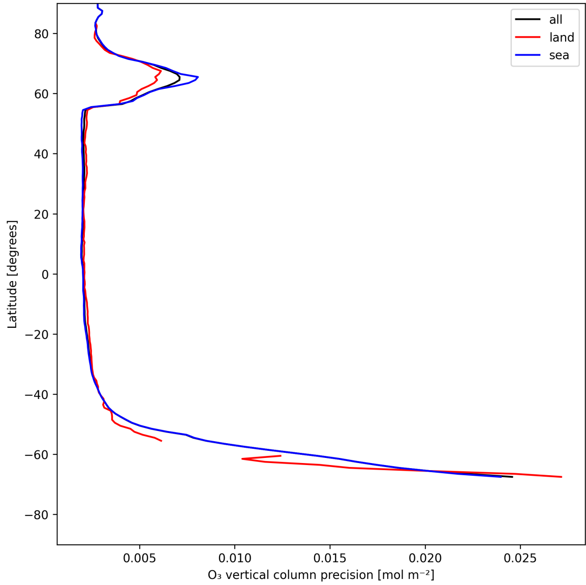
Figure 18: Zonal average of “O 3 vertical column precision” for 2025-07-17 to 2025-07-18.
