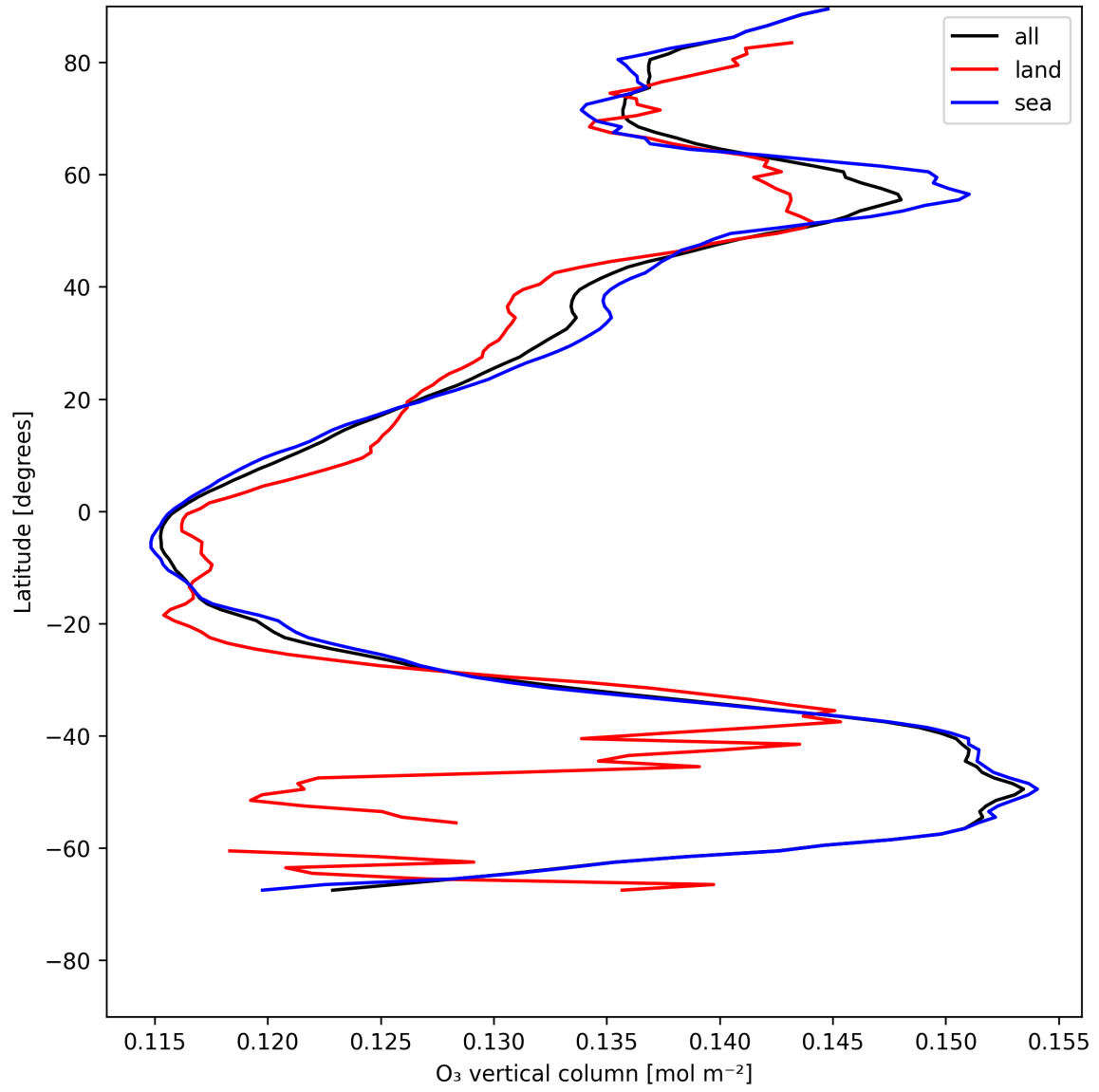
Figure 17: Zonal average of “O 3 vertical column” for 2025-07-17 to 2025-07-18.
