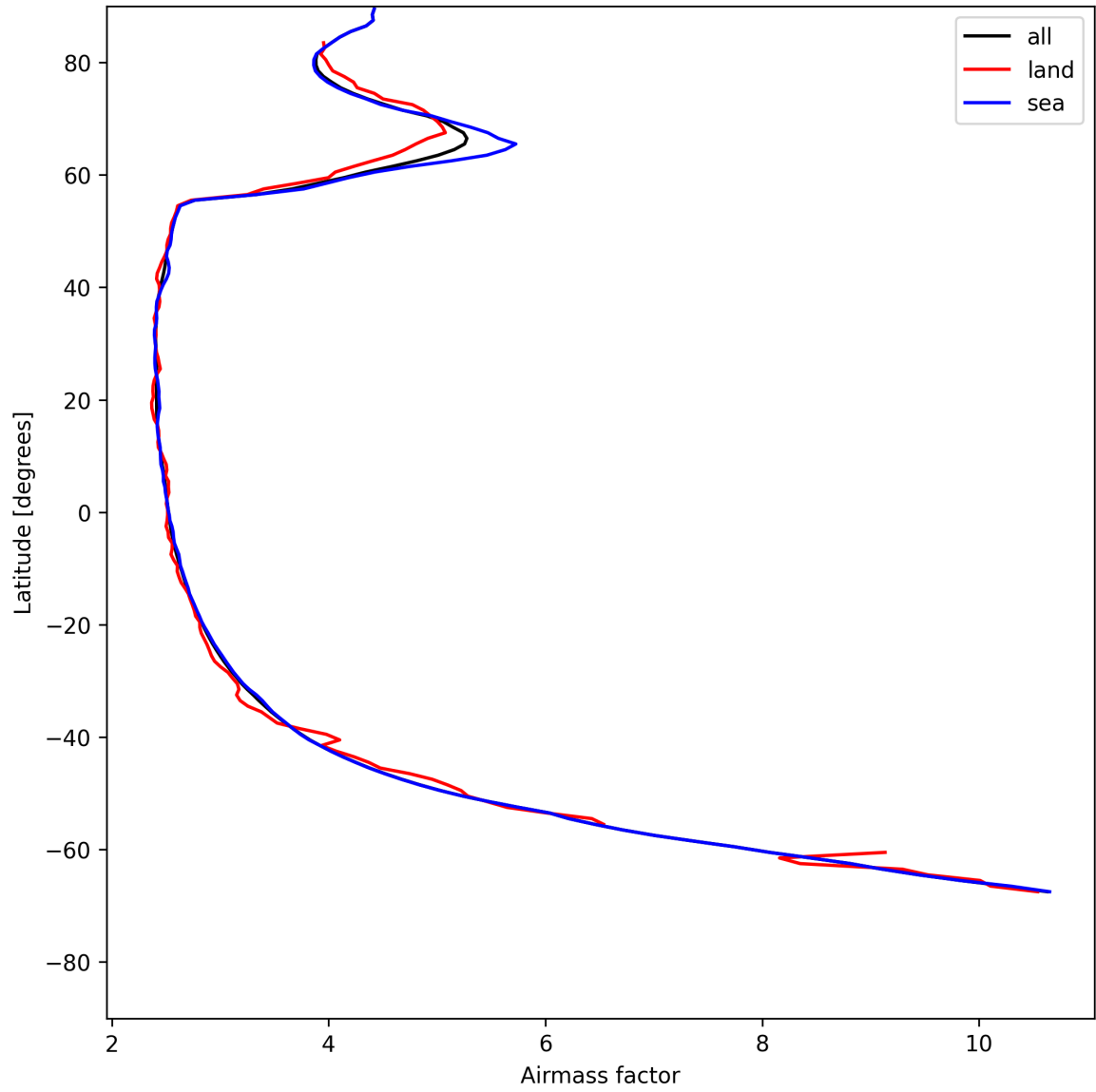
Figure 25: Zonal average of “Airmass factor” for 2025-07-17 to 2025-07-18.
