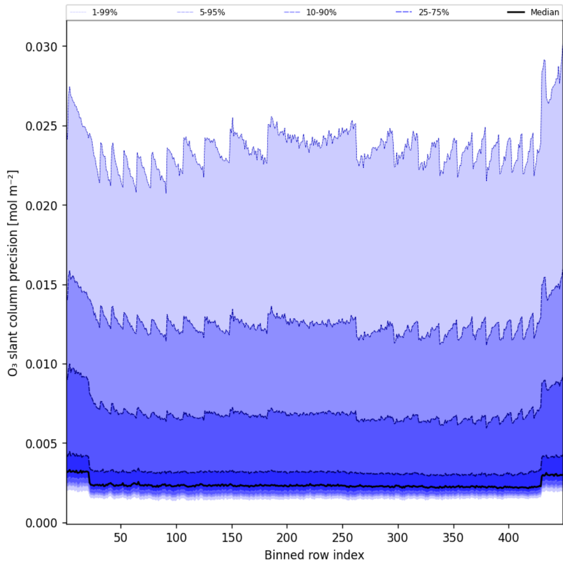
Figure 44: Along track statistics of “O 3 slant column precision” for 2025-07-17 to 2025-07-18
