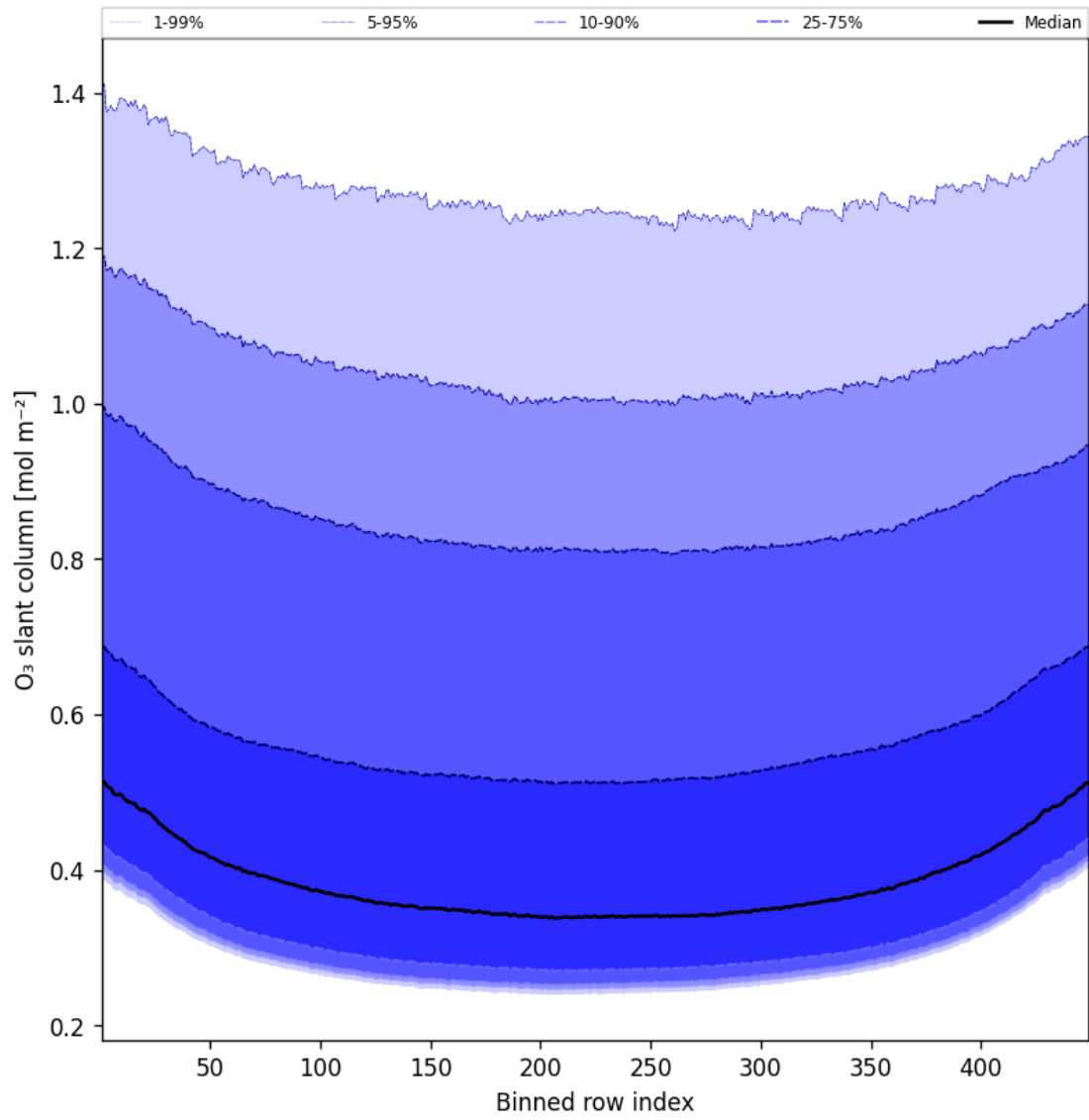
Figure 43: Along track statistics of “O 3 slant column” for 2025-07-17 to 2025-07-18
