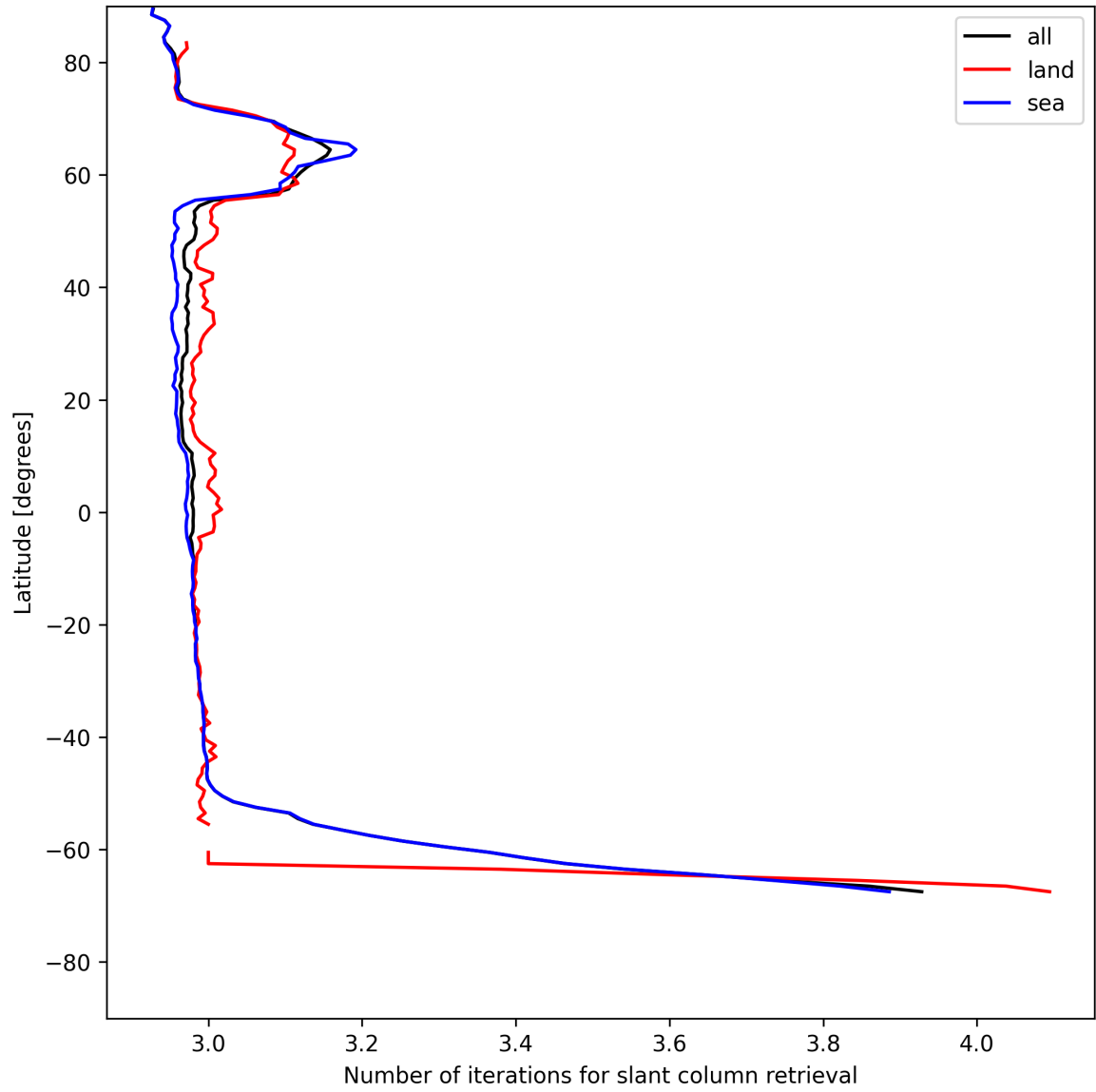
Figure 21: Zonal average of “Number of iterations for slant column retrieval” for 2025-07-17 to 2025-07-18.
