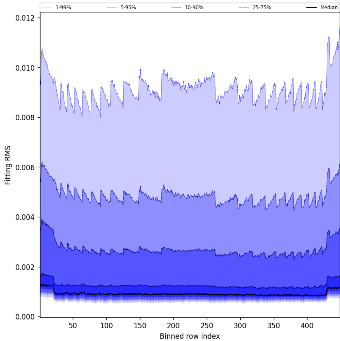
Figure 46: Along track statistics of “Fitting RMS” for 2025-07-17 to 2025-07-18
