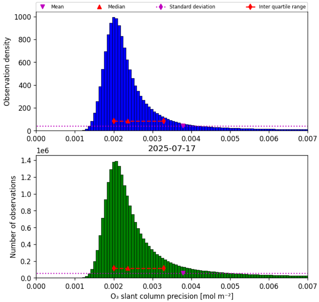
Figure 32: Histogram of “O 3 slant column precision” for 2025-07-17 to 2025-07-18
