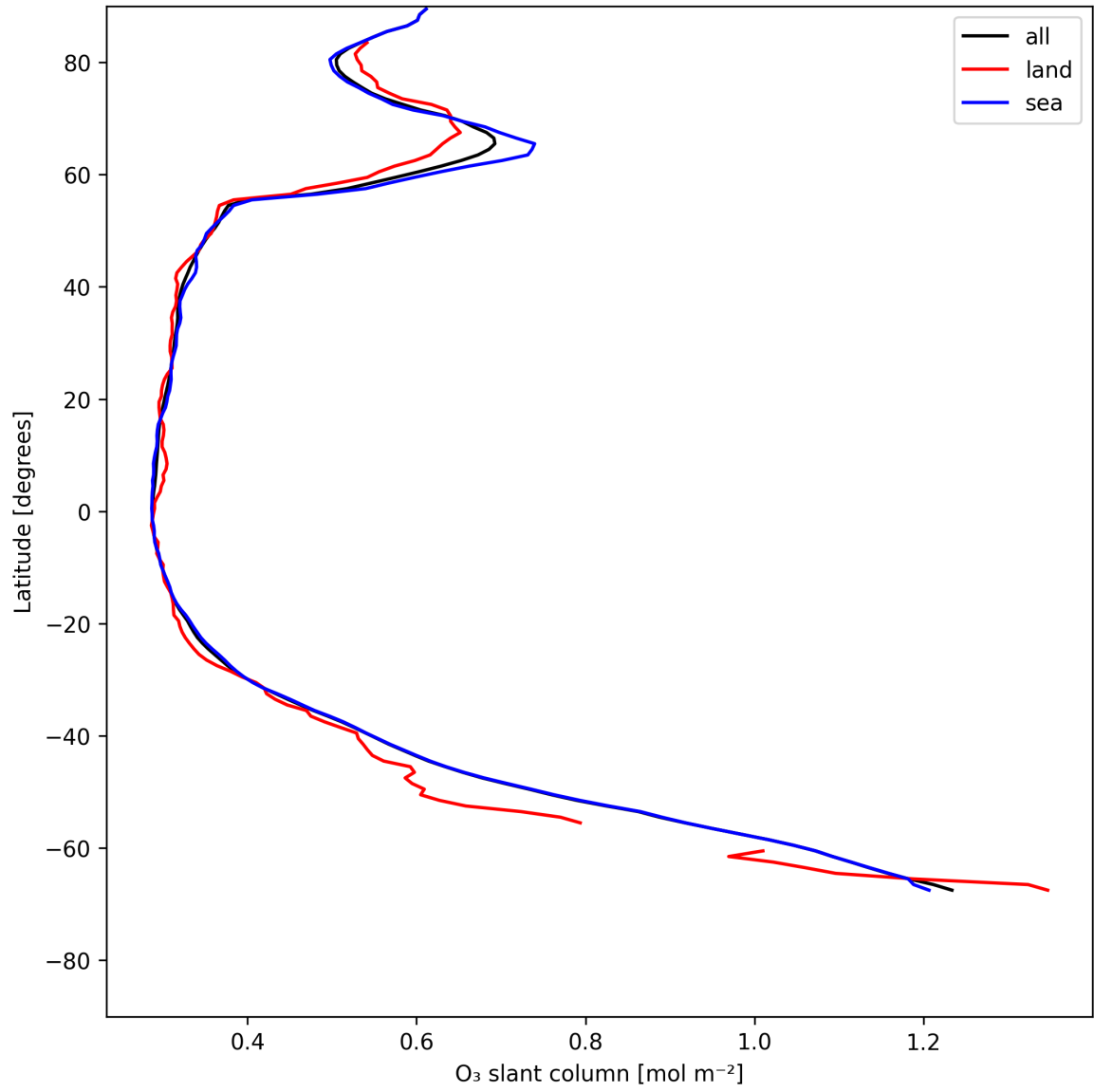
Figure 19: Zonal average of “O 3 slant column” for 2025-07-17 to 2025-07-18.
