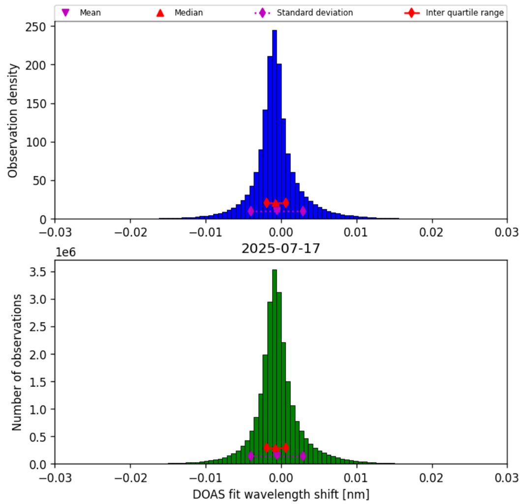
Figure 35: Histogram of “DOAS fit wavelength shift” for 2025-07-17 to 2025-07-18
