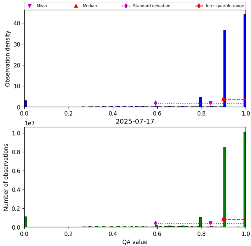
Figure 28: Histogram of “QA value” for 2025-07-17 to 2025-07-18
