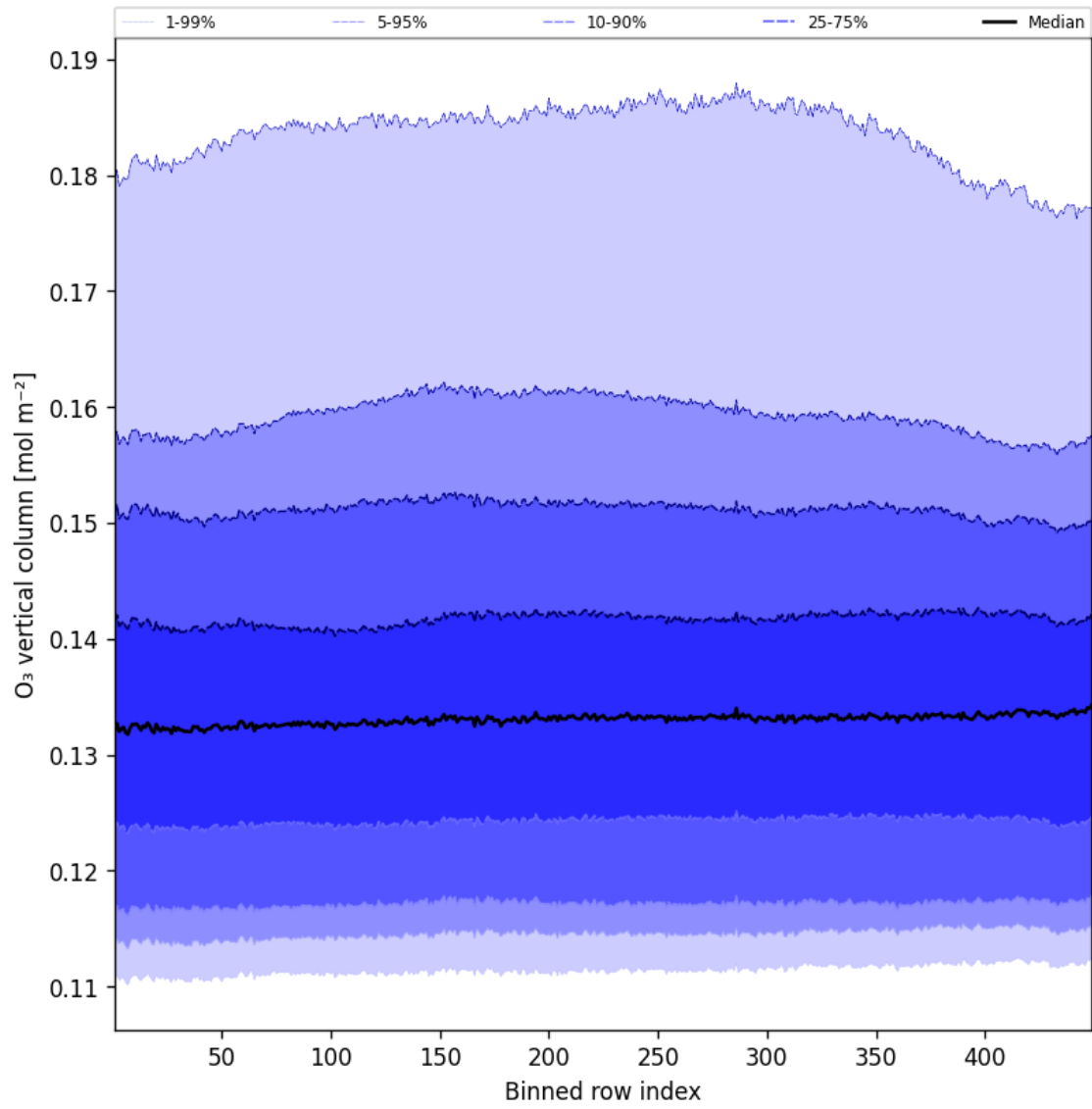
Figure 41: Along track statistics of “O 3 vertical column” for 2025-07-17 to 2025-07-18
