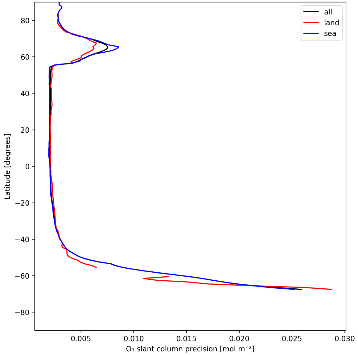
Figure 20: Zonal average of “O 3 slant column precision” for 2025-07-17 to 2025-07-18.
