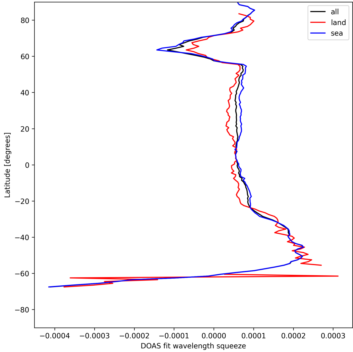
Figure 24: Zonal average of “DOAS fit wavelength squeeze” for 2025-07-17 to 2025-07-18.
