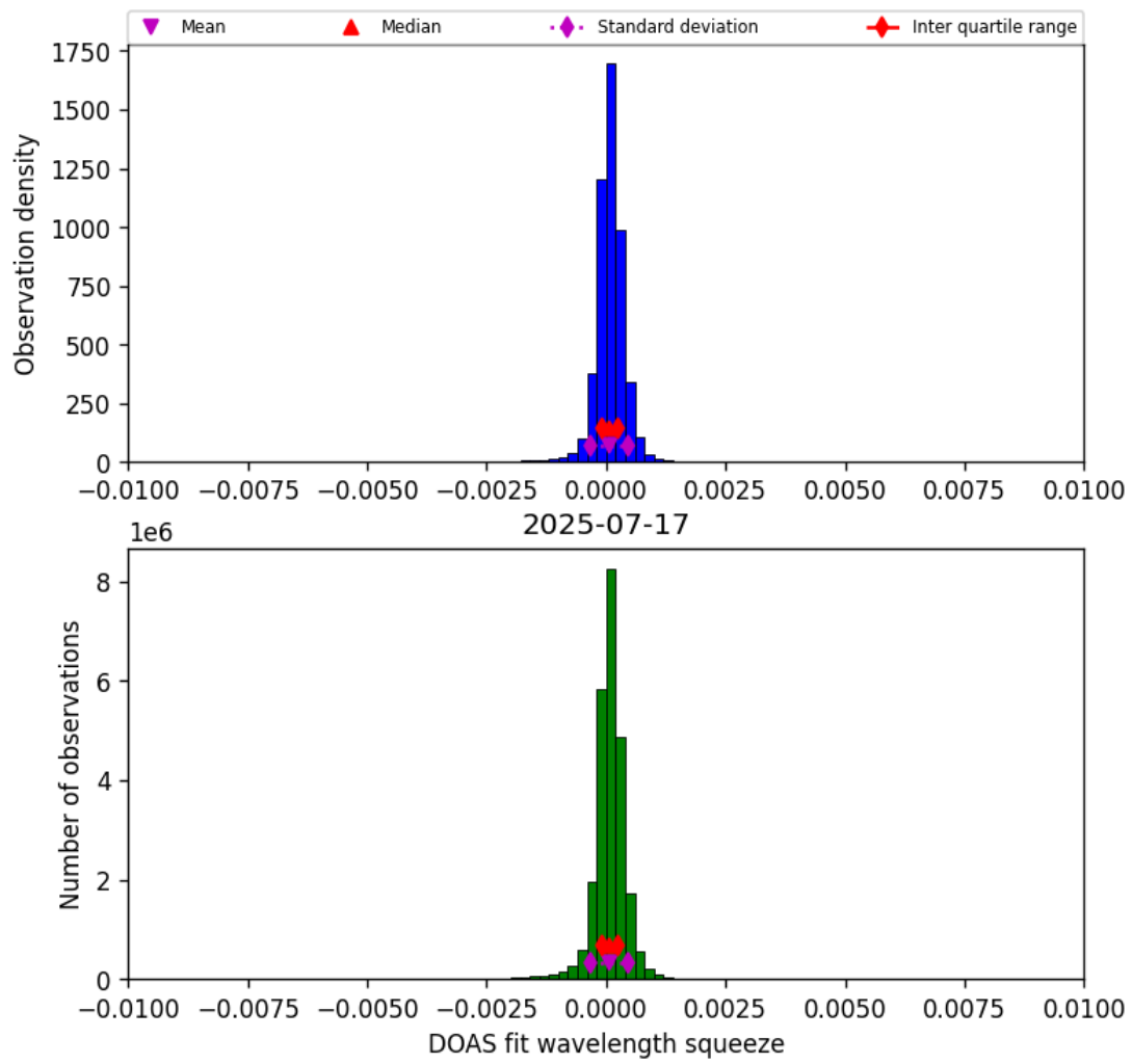
Figure 36: Histogram of “DOAS fit wavelength squeeze” for 2025-07-17 to 2025-07-18
