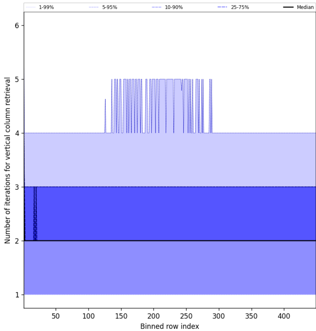
Figure 51: Along track statistics of “Number of iterations for vertical column retrieval” for 2025-07-17 to 2025-07-18
