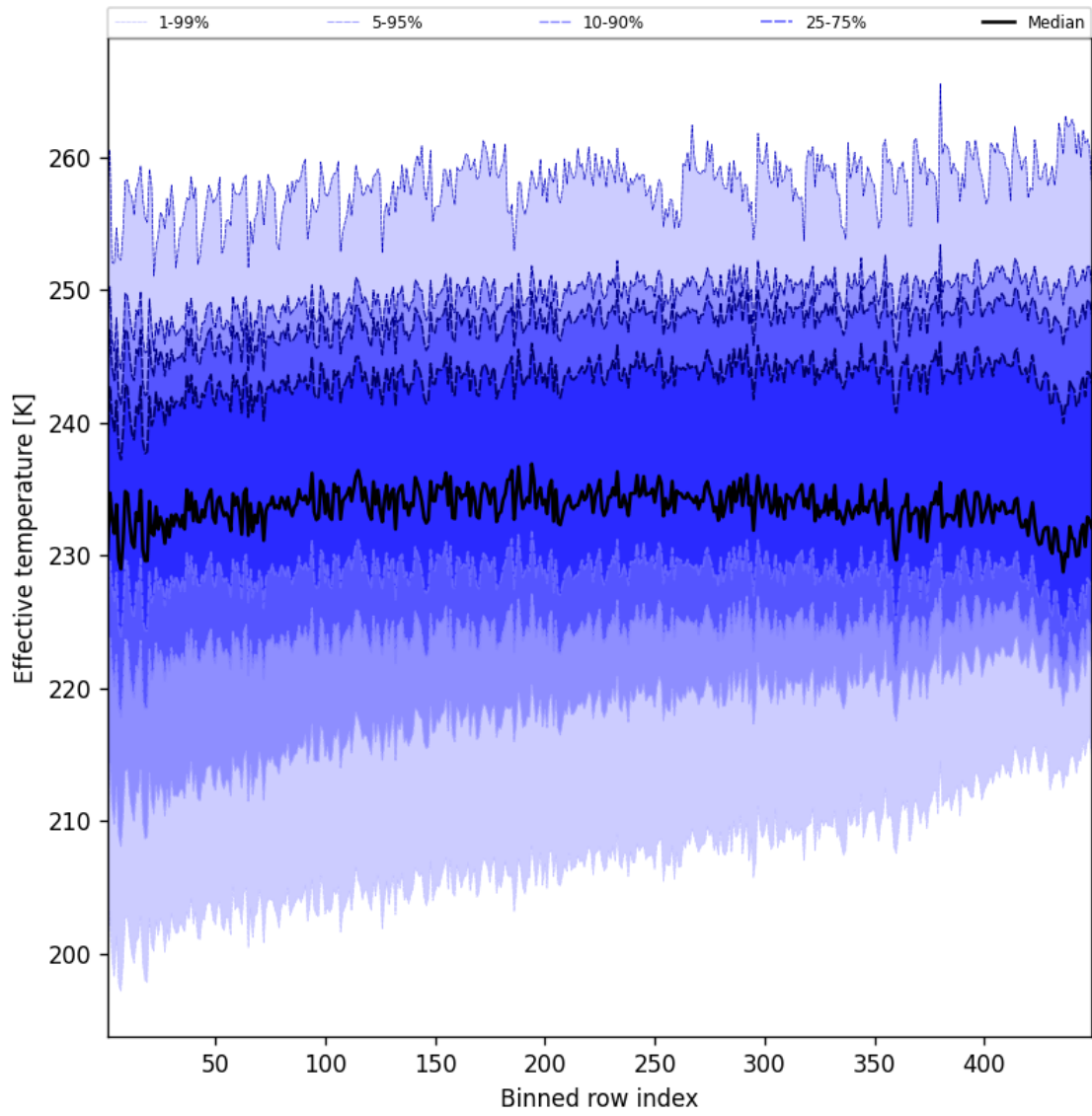
Figure 50: Along track statistics of “Effective temperature” for 2025-07-17 to 2025-07-18
