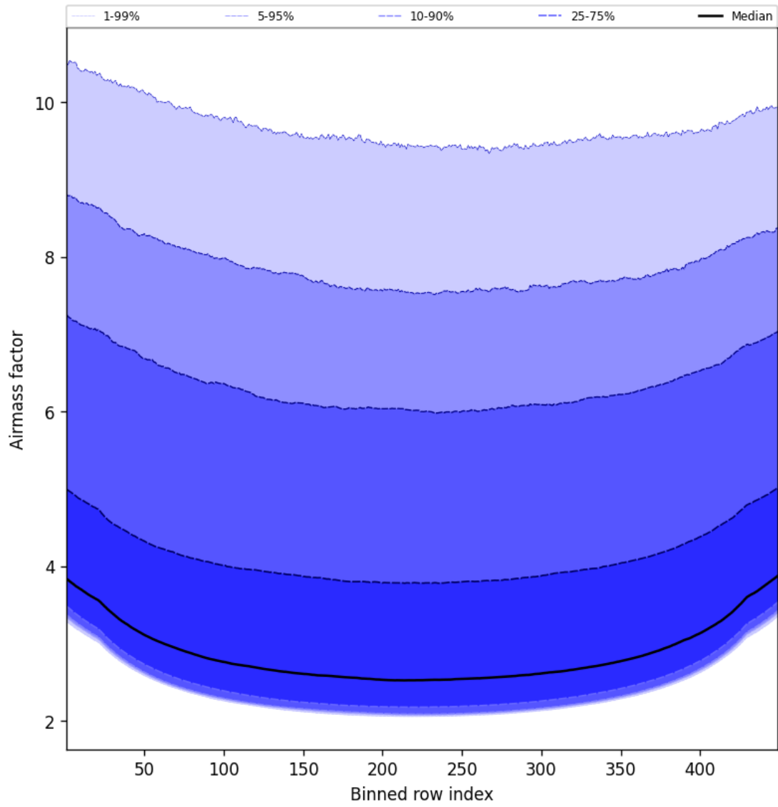
Figure 49: Along track statistics of “Airmass factor” for 2025-07-17 to 2025-07-18
