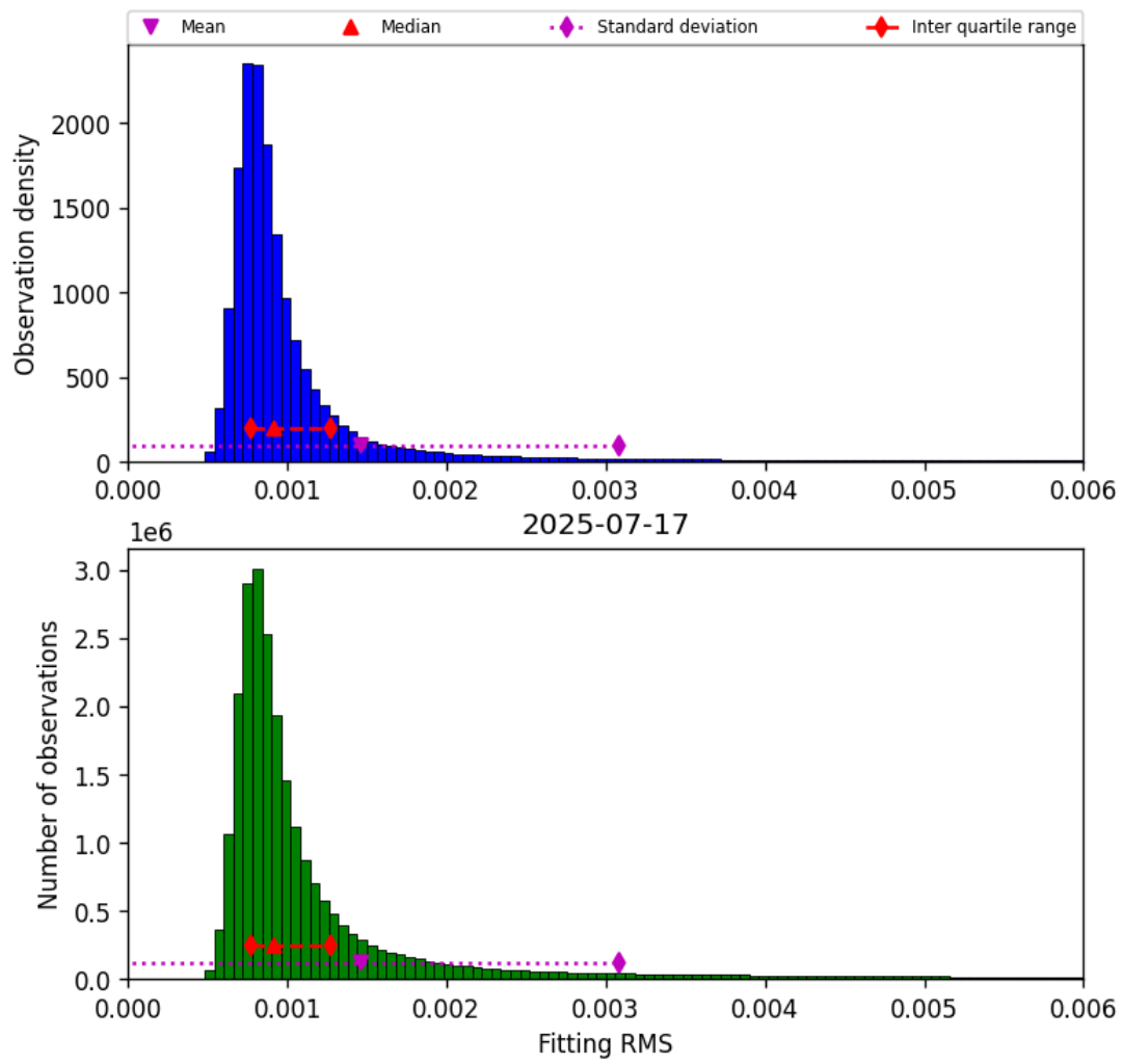
Figure 34: Histogram of “Fitting RMS” for 2025-07-17 to 2025-07-18
