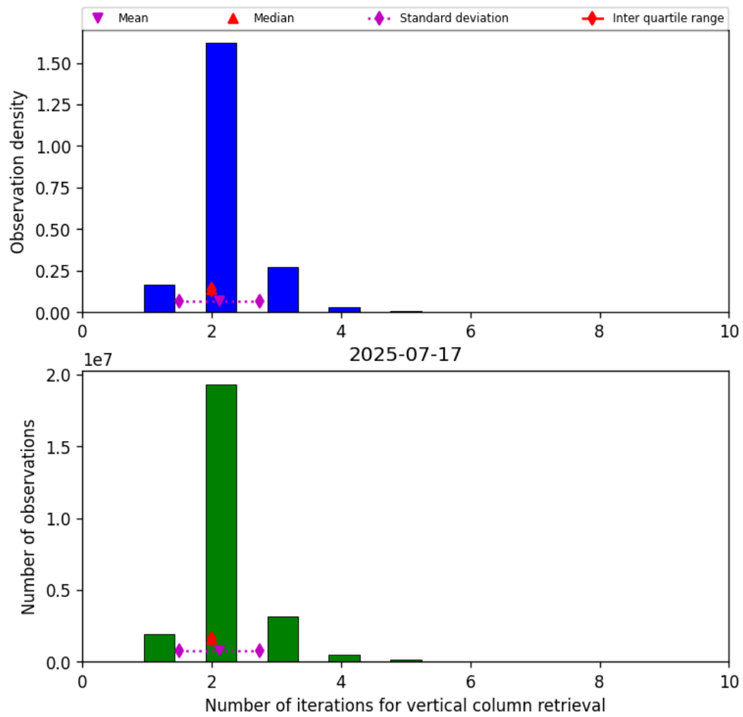
Figure 39: Histogram of “Number of iterations for vertical column retrieval” for 2025-07-17 to 2025-07-18
