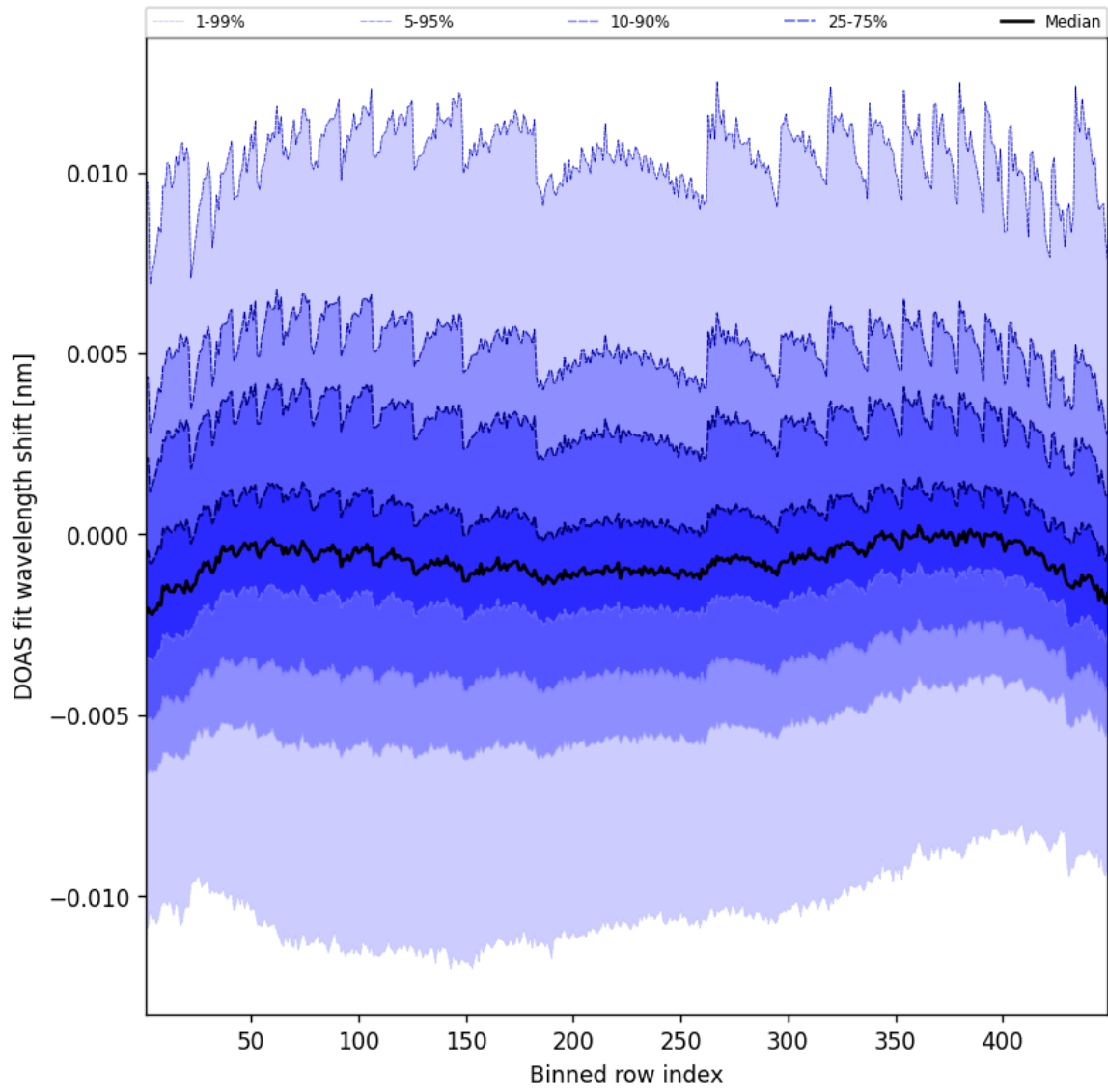
Figure 47: Along track statistics of “DOAS fit wavelength shift” for 2025-07-17 to 2025-07-18
