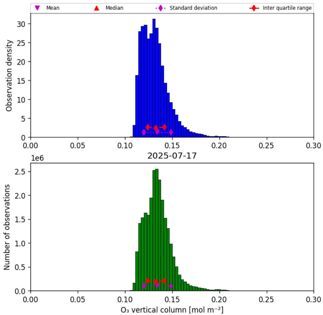
Figure 29: Histogram of “O 3 vertical column” for 2025-07-17 to 2025-07-18
