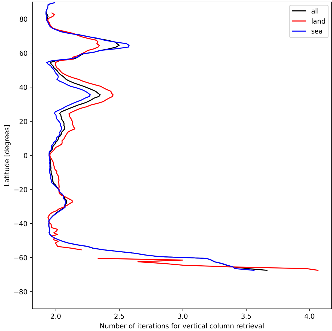
Figure 27: Zonal average of “Number of iterations for vertical column retrieval” for 2025-07-17 to 2025-07-18.
