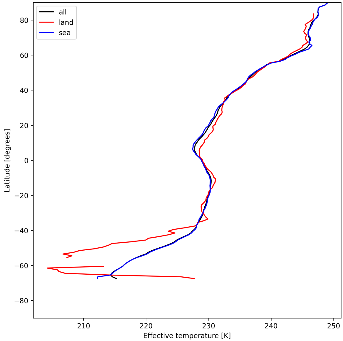
Figure 26: Zonal average of “Effective temperature” for 2025-07-17 to 2025-07-18.
