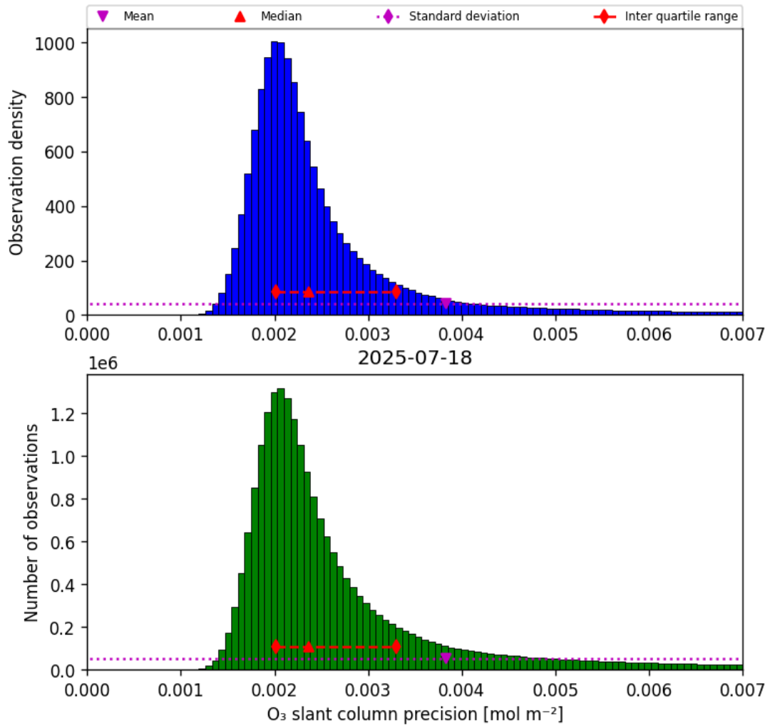
Figure 32: Histogram of “O 3 slant column precision” for 2025-07-18 to 2025-07-19
