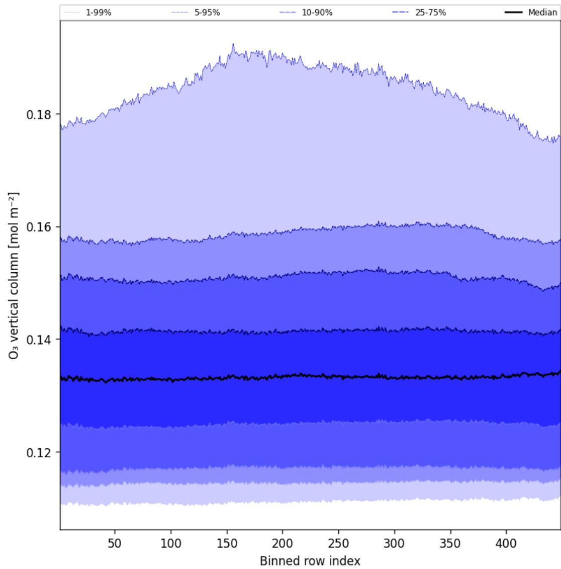
Figure 41: Along track statistics of “O 3 vertical column” for 2025-07-18 to 2025-07-19
