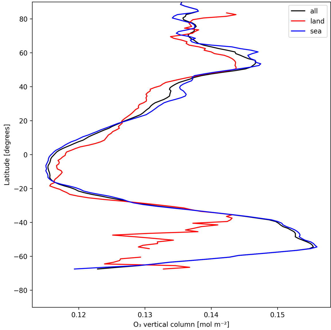
Figure 17: Zonal average of “O 3 vertical column” for 2025-07-18 to 2025-07-19.
