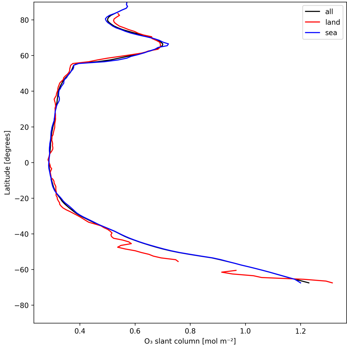
Figure 19: Zonal average of “O 3 slant column” for 2025-07-18 to 2025-07-19.
