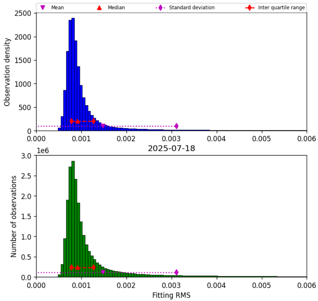
Figure 34: Histogram of “Fitting RMS” for 2025-07-18 to 2025-07-19
