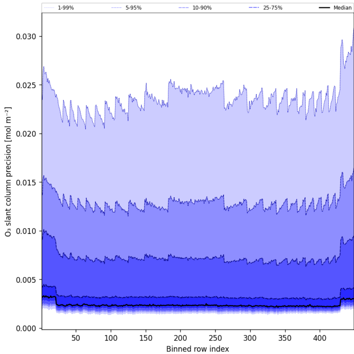
Figure 44: Along track statistics of “O 3 slant column precision” for 2025-07-18 to 2025-07-19
