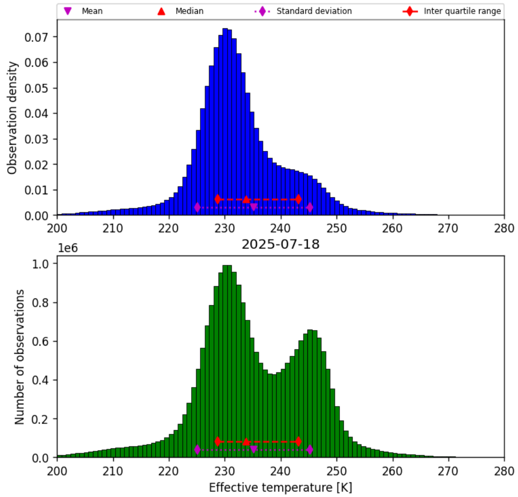
Figure 38: Histogram of “Effective temperature” for 2025-07-18 to 2025-07-19
