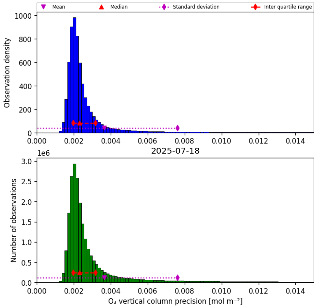
Figure 30: Histogram of “O 3 vertical column precision” for 2025-07-18 to 2025-07-19
