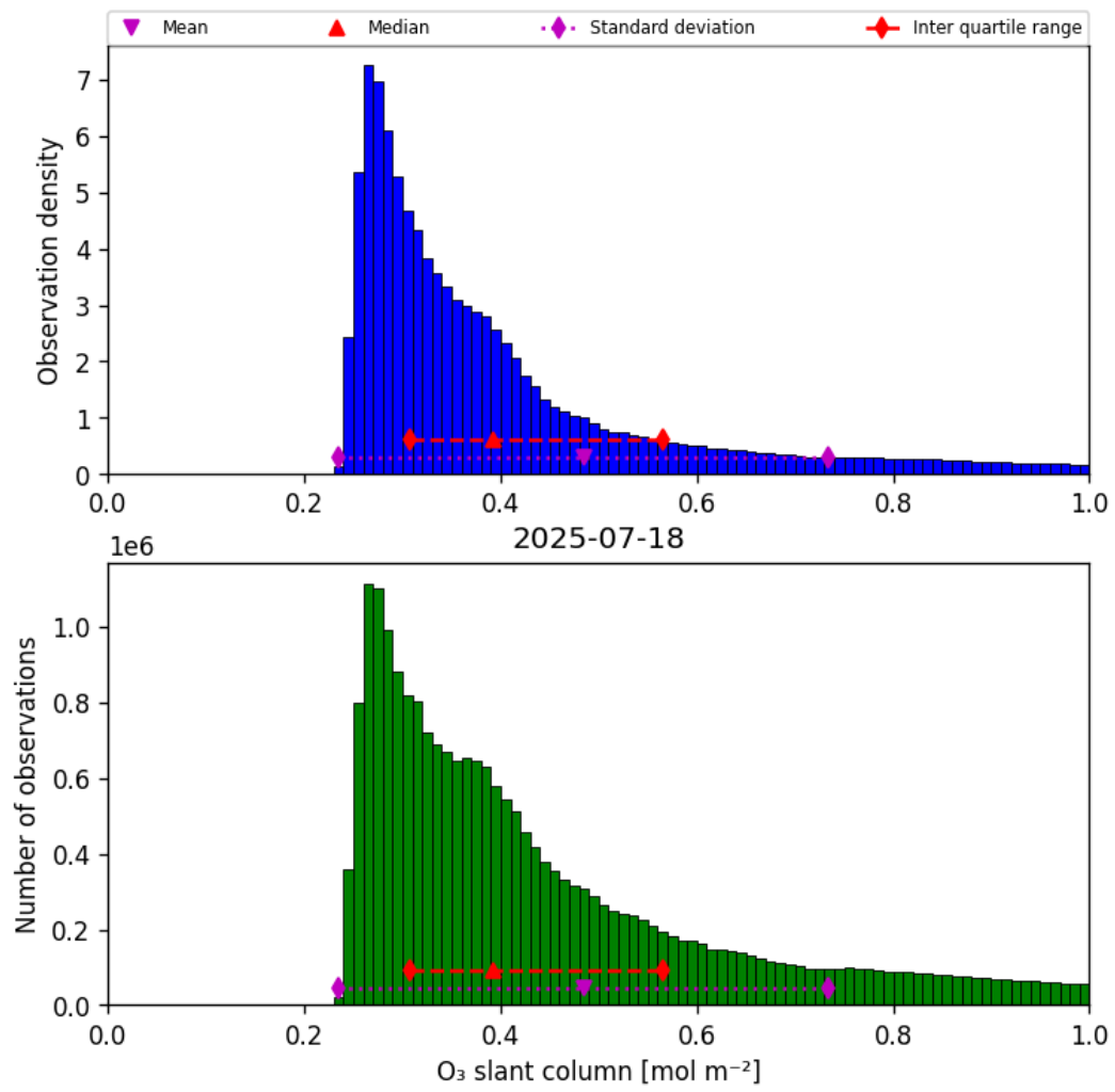
Figure 31: Histogram of “O 3 slant column” for 2025-07-18 to 2025-07-19
