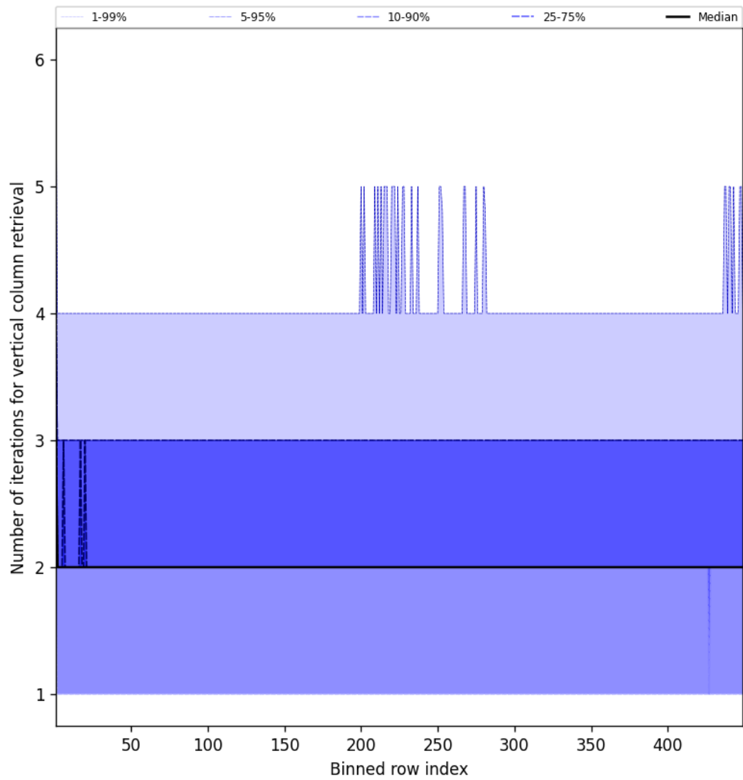
Figure 51: Along track statistics of “Number of iterations for vertical column retrieval” for 2025-07-18 to 2025-07-19
