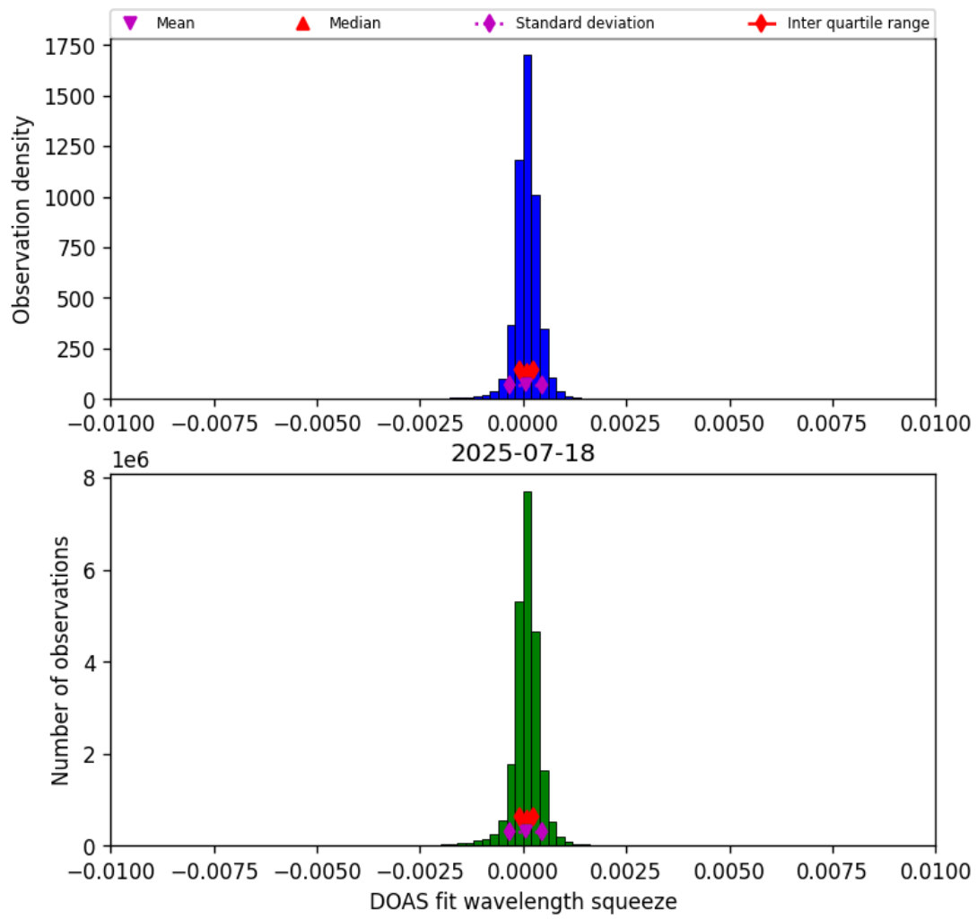
Figure 36: Histogram of “DOAS fit wavelength squeeze” for 2025-07-18 to 2025-07-19
