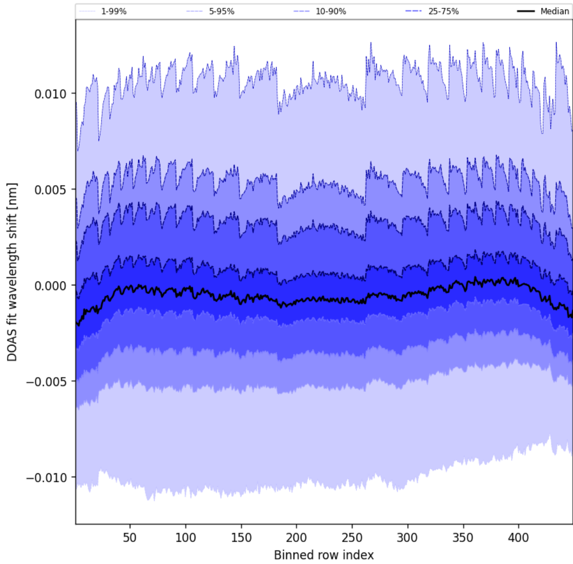
Figure 47: Along track statistics of “DOAS fit wavelength shift” for 2025-07-18 to 2025-07-19
