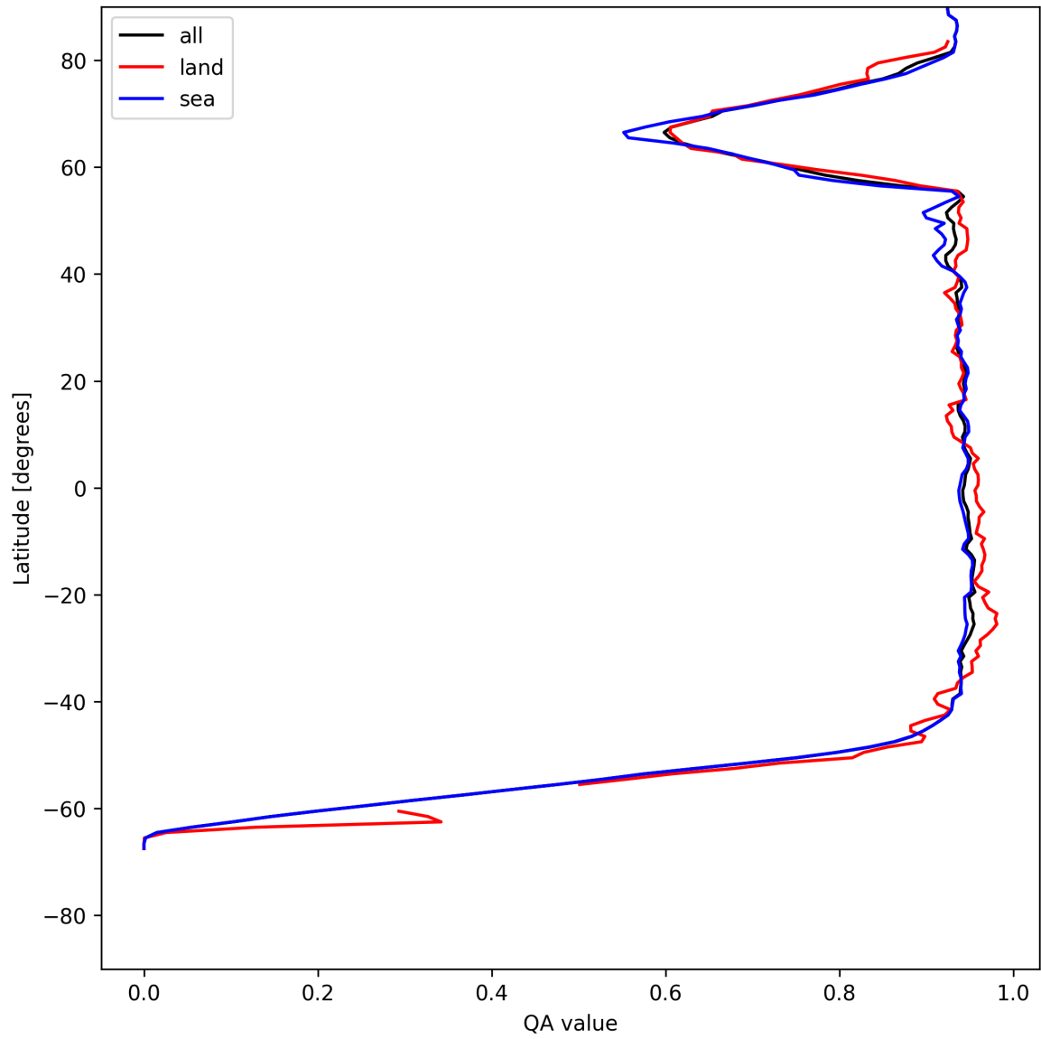
Figure 16: Zonal average of “QA value” for 2025-07-18 to 2025-07-19.
