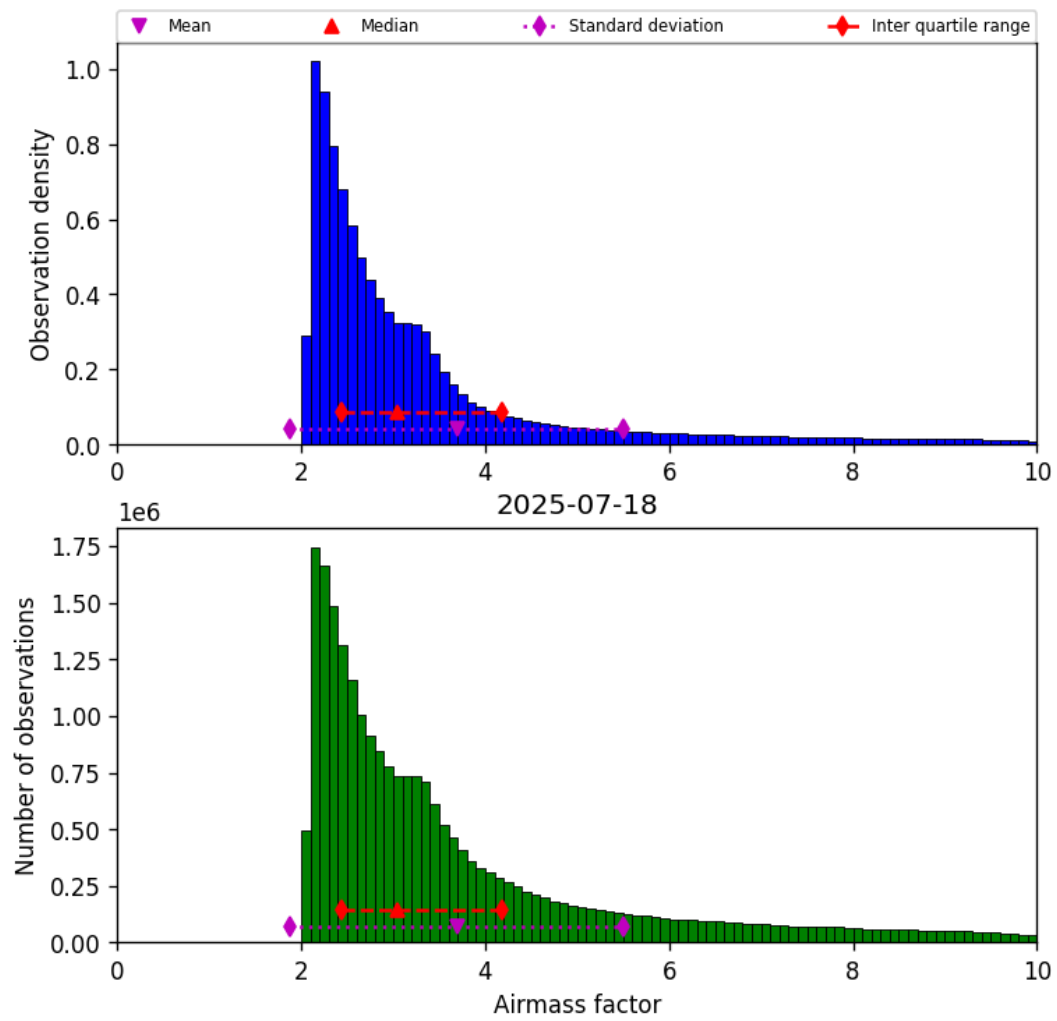
Figure 37: Histogram of “Airmass factor” for 2025-07-18 to 2025-07-19
