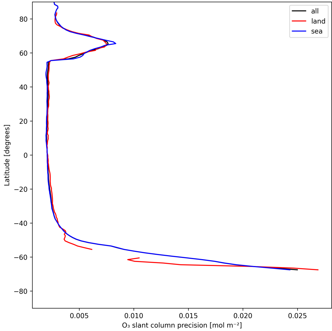
Figure 20: Zonal average of “O 3 slant column precision” for 2025-07-18 to 2025-07-19.
