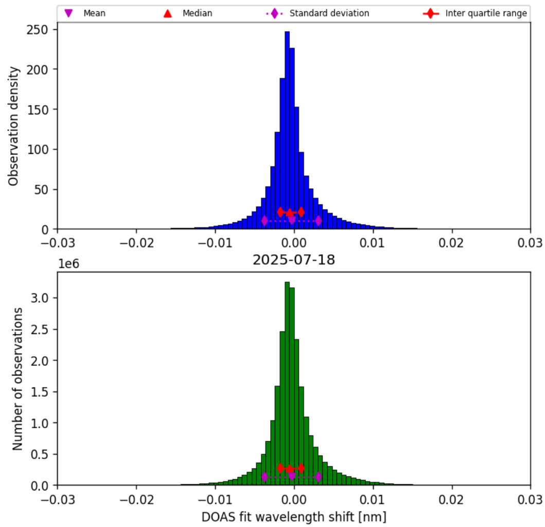
Figure 35: Histogram of “DOAS fit wavelength shift” for 2025-07-18 to 2025-07-19
