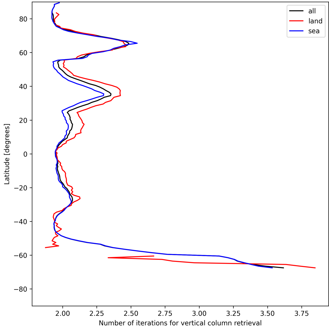
Figure 27: Zonal average of “Number of iterations for vertical column retrieval” for 2025-07-18 to 2025-07-19.
