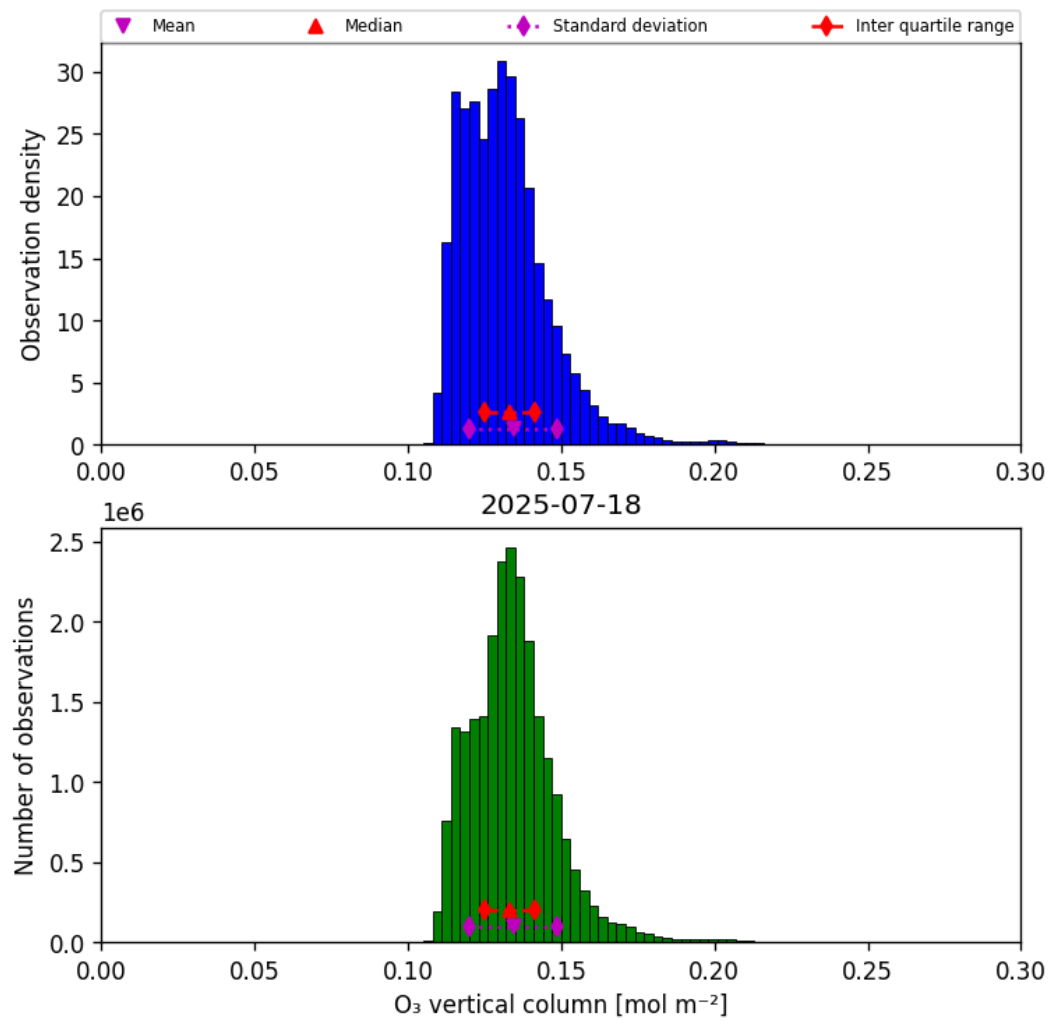
Figure 29: Histogram of “O 3 vertical column” for 2025-07-18 to 2025-07-19
