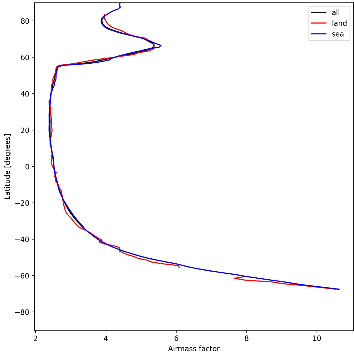
Figure 25: Zonal average of “Airmass factor” for 2025-07-18 to 2025-07-19.
