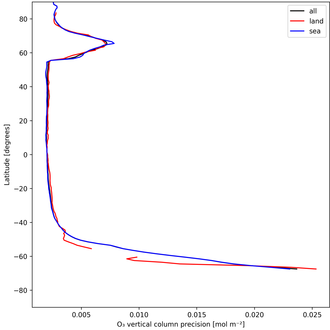
Figure 18: Zonal average of "O 3 vertical column precision" for 2025-07-18 to 2025-07-19.
