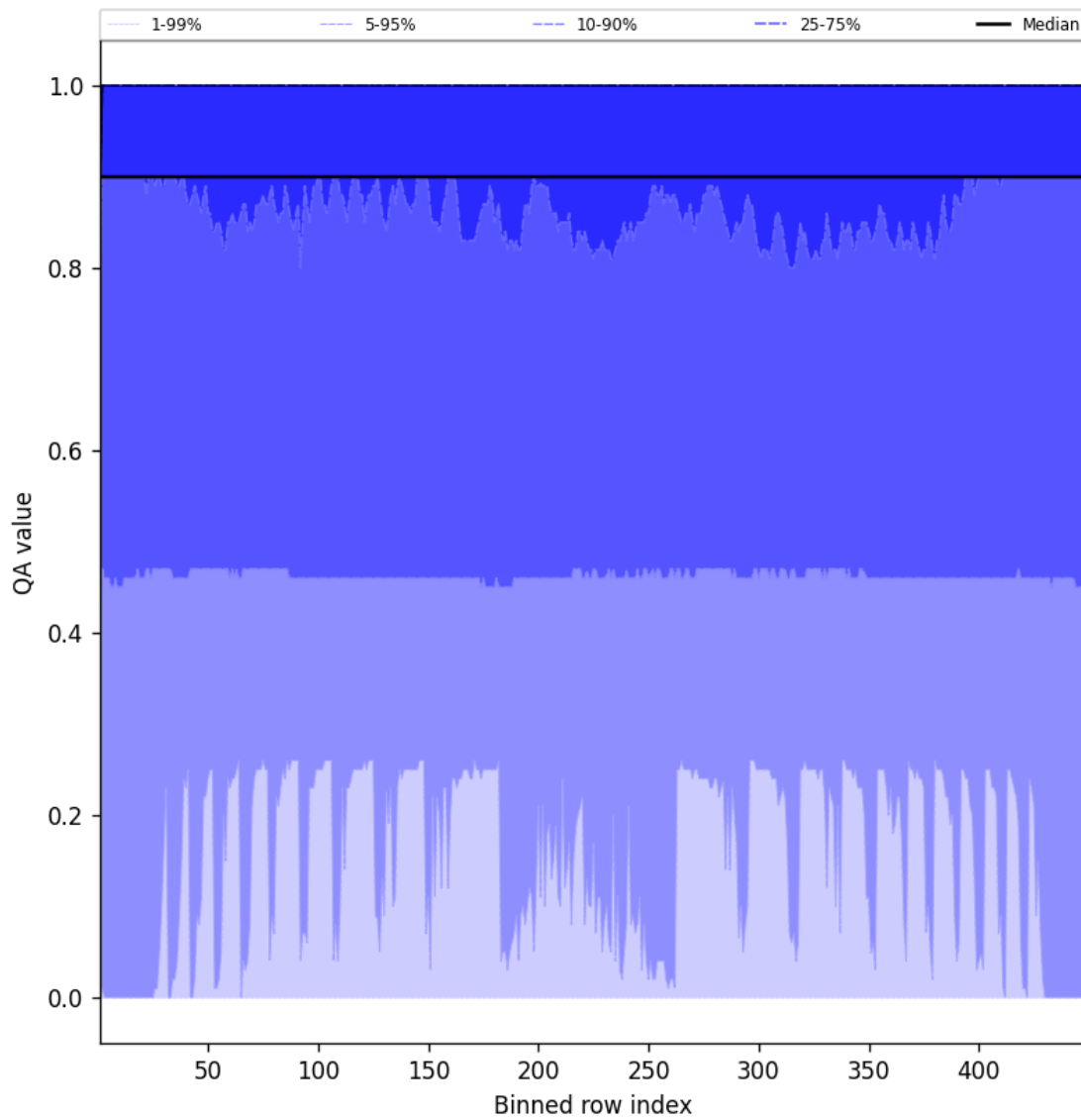
Figure 40: Along track statistics of “QA value” for 2025-07-18 to 2025-07-19
