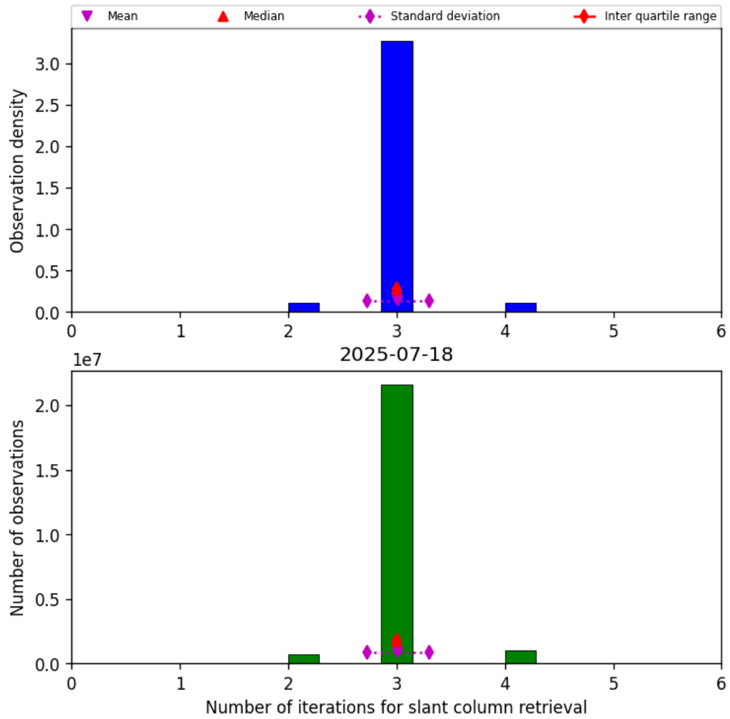
Figure 33: Histogram of “Number of iterations for slant column retrieval” for 2025-07-18 to 2025-07-19
