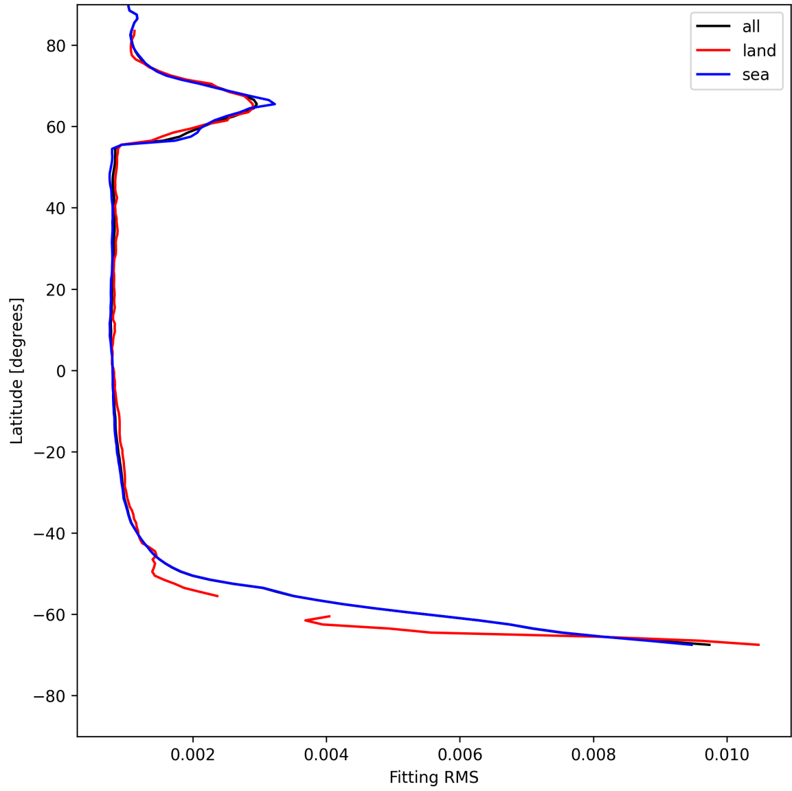
Figure 22: Zonal average of “Fitting RMS” for 2025-07-18 to 2025-07-19.
