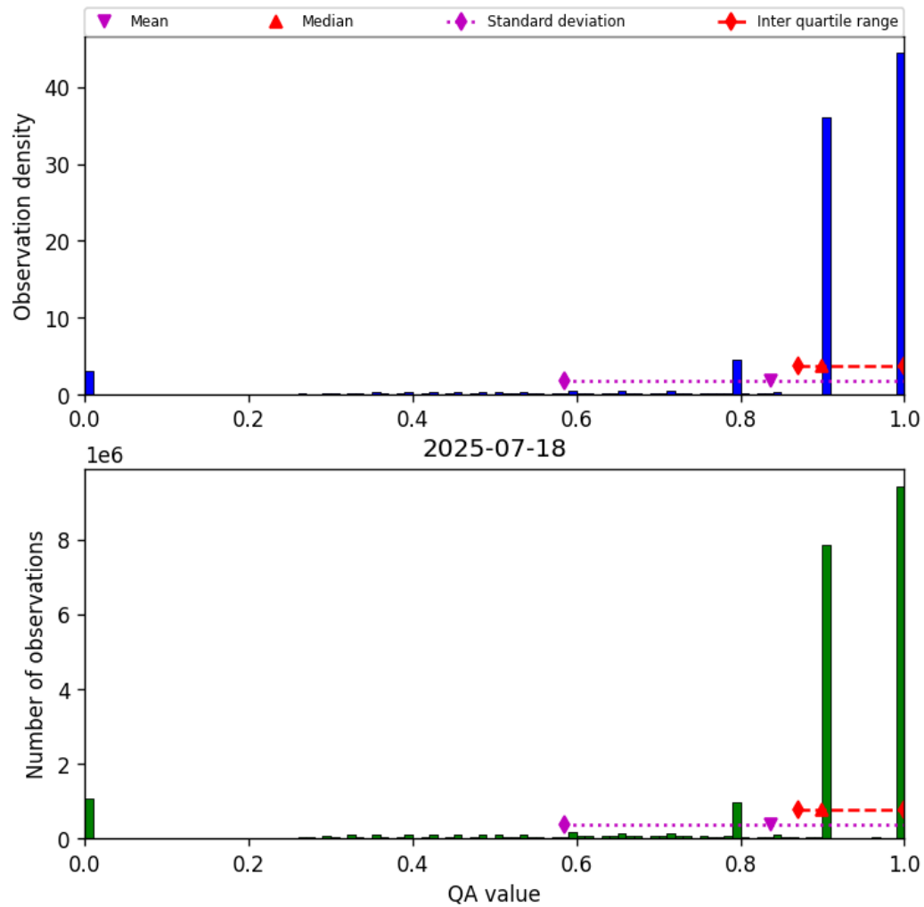
Figure 28: Histogram of “QA value” for 2025-07-18 to 2025-07-19
