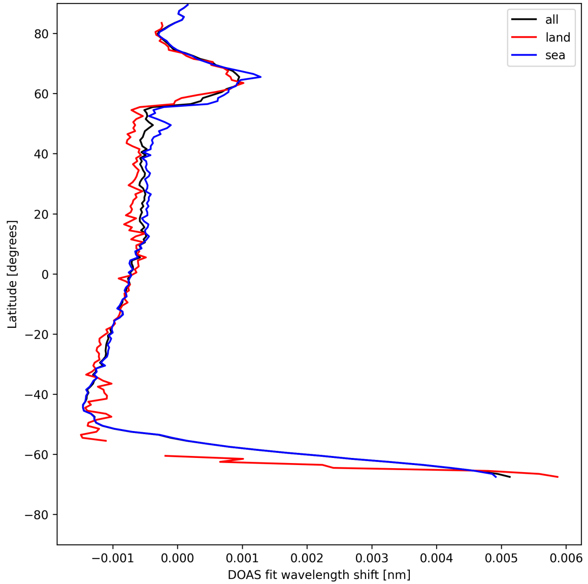
Figure 23: Zonal average of "DOAS fit wavelength shift" for 2025-07-18 to 2025-07-19.
