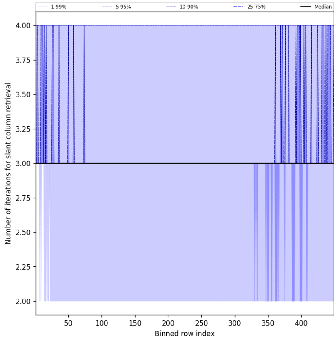
Figure 45: Along track statistics of “Number of iterations for slant column retrieval” for 2025-07-18 to 2025-07-19
