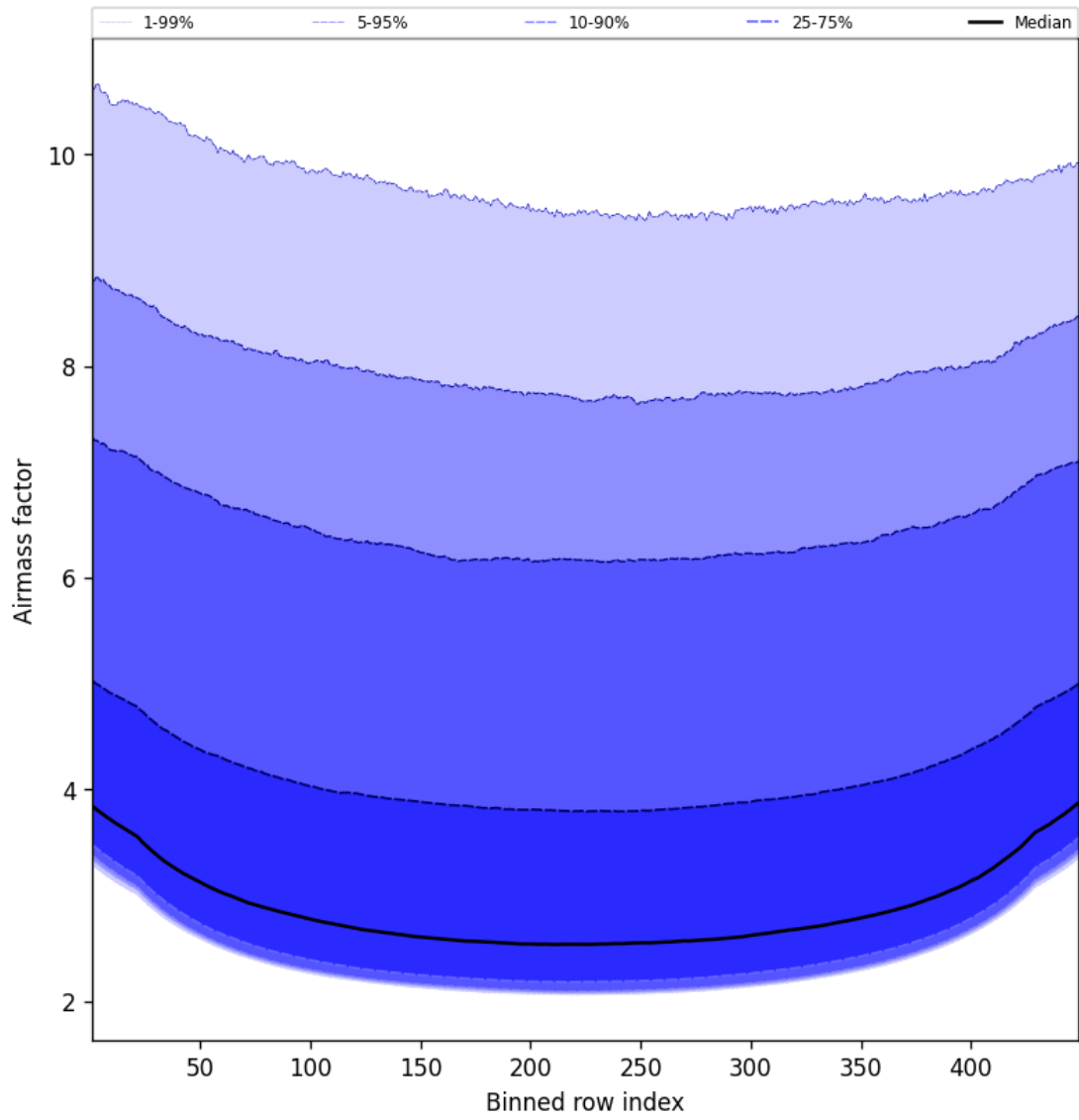
Figure 49: Along track statistics of “Airmass factor” for 2025-07-18 to 2025-07-19
