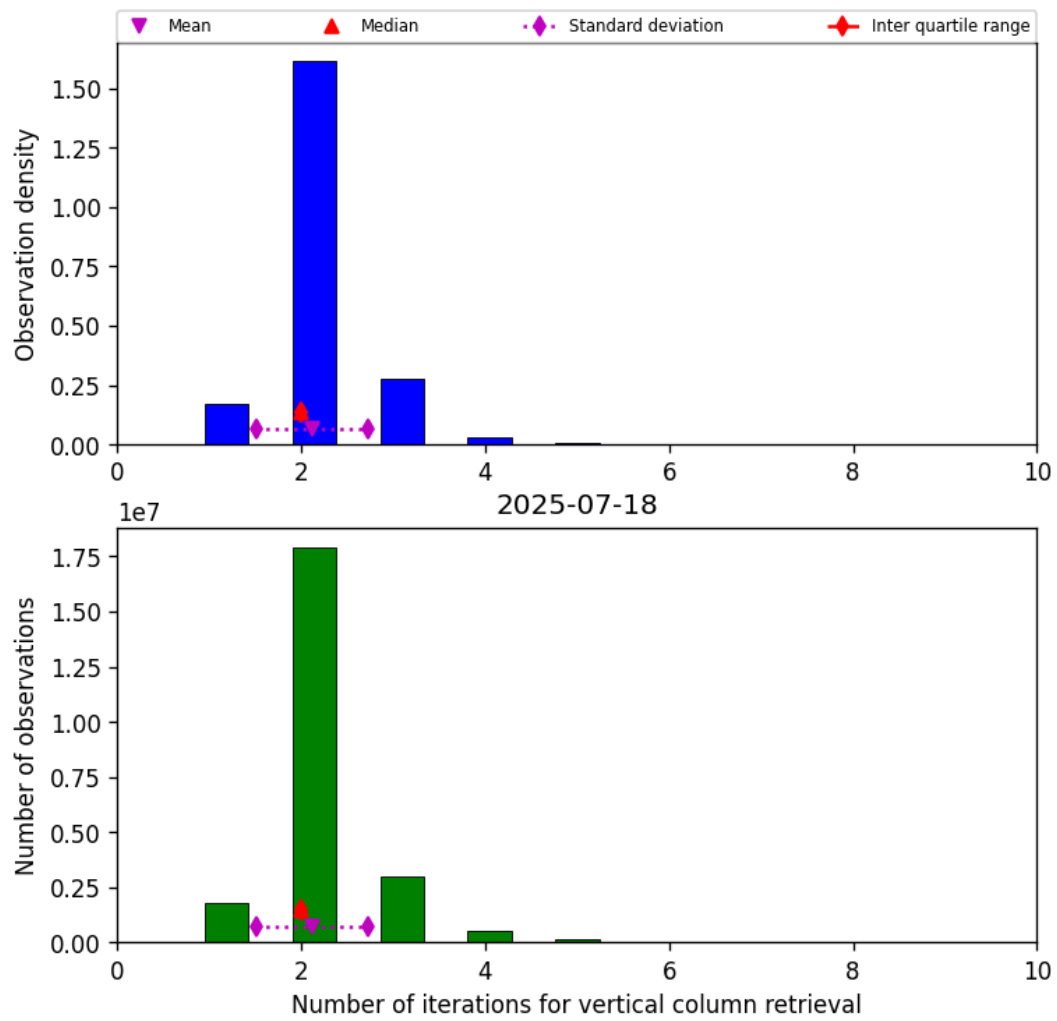
Figure 39: Histogram of “Number of iterations for vertical column retrieval” for 2025-07-18 to 2025-07-19
