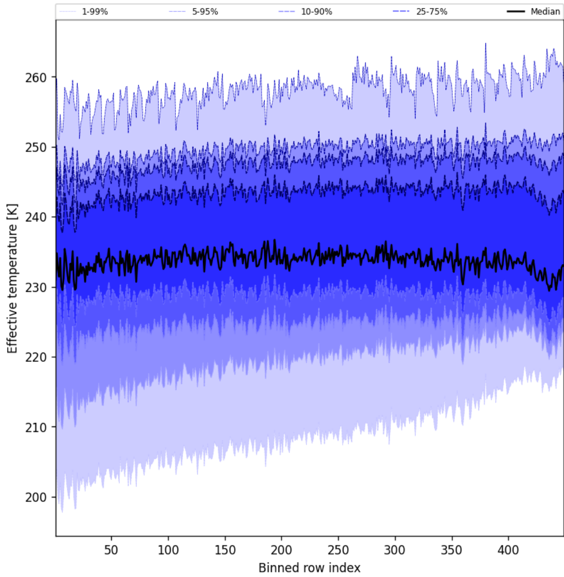
Figure 50: Along track statistics of “Effective temperature” for 2025-07-18 to 2025-07-19
