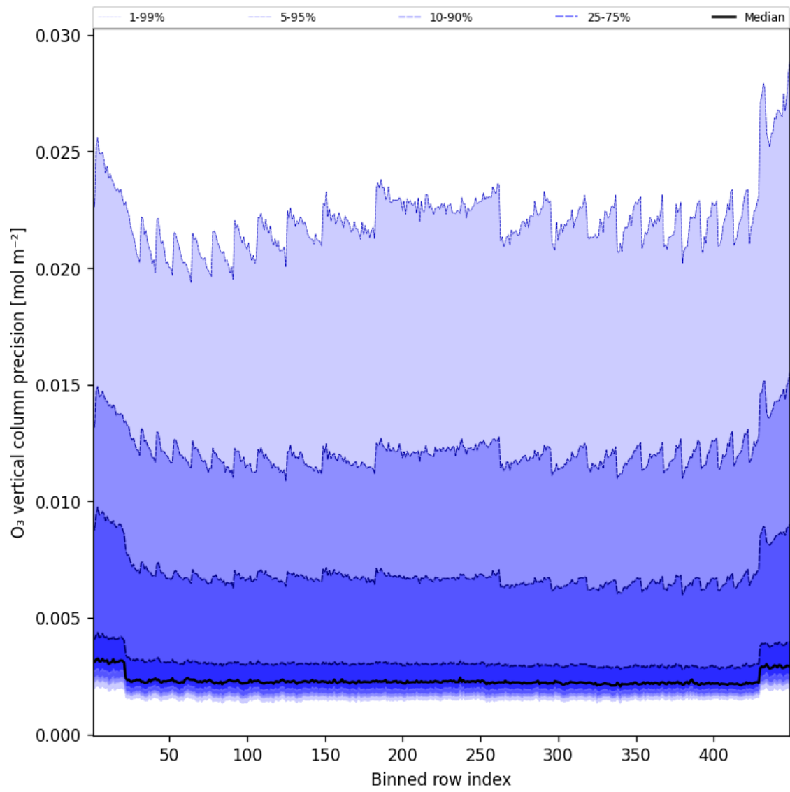
Figure 42: Along track statistics of “O 3 vertical column precision” for 2025-07-18 to 2025-07-19
