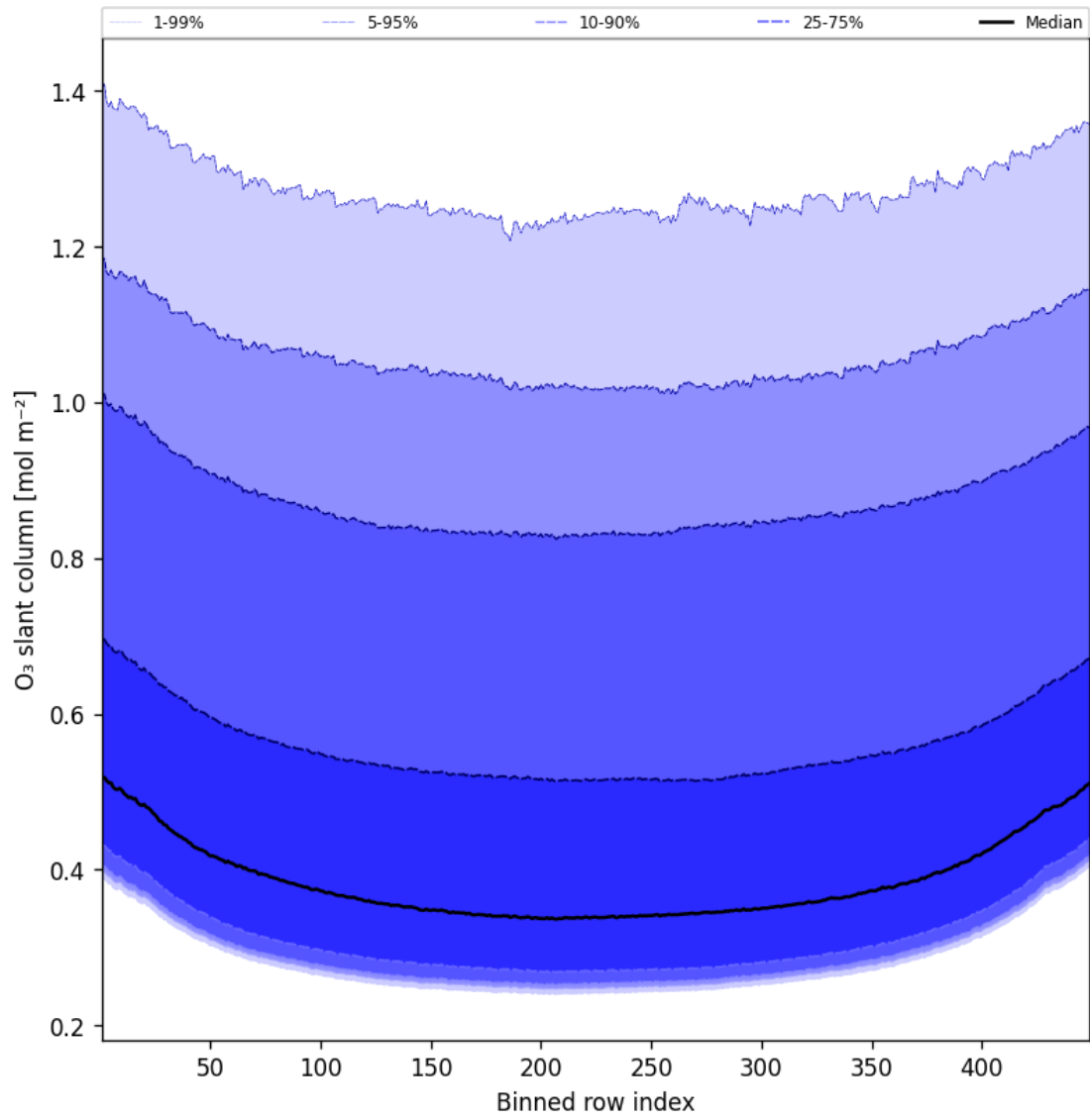
Figure 43: Along track statistics of “O 3 slant column” for 2025-07-18 to 2025-07-19
