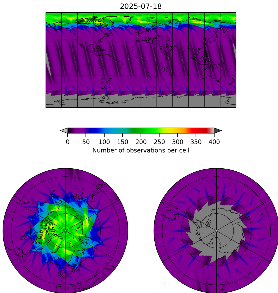
Figure 15: Map of the number of observations for 2025-07-18 to 2025-07-19
