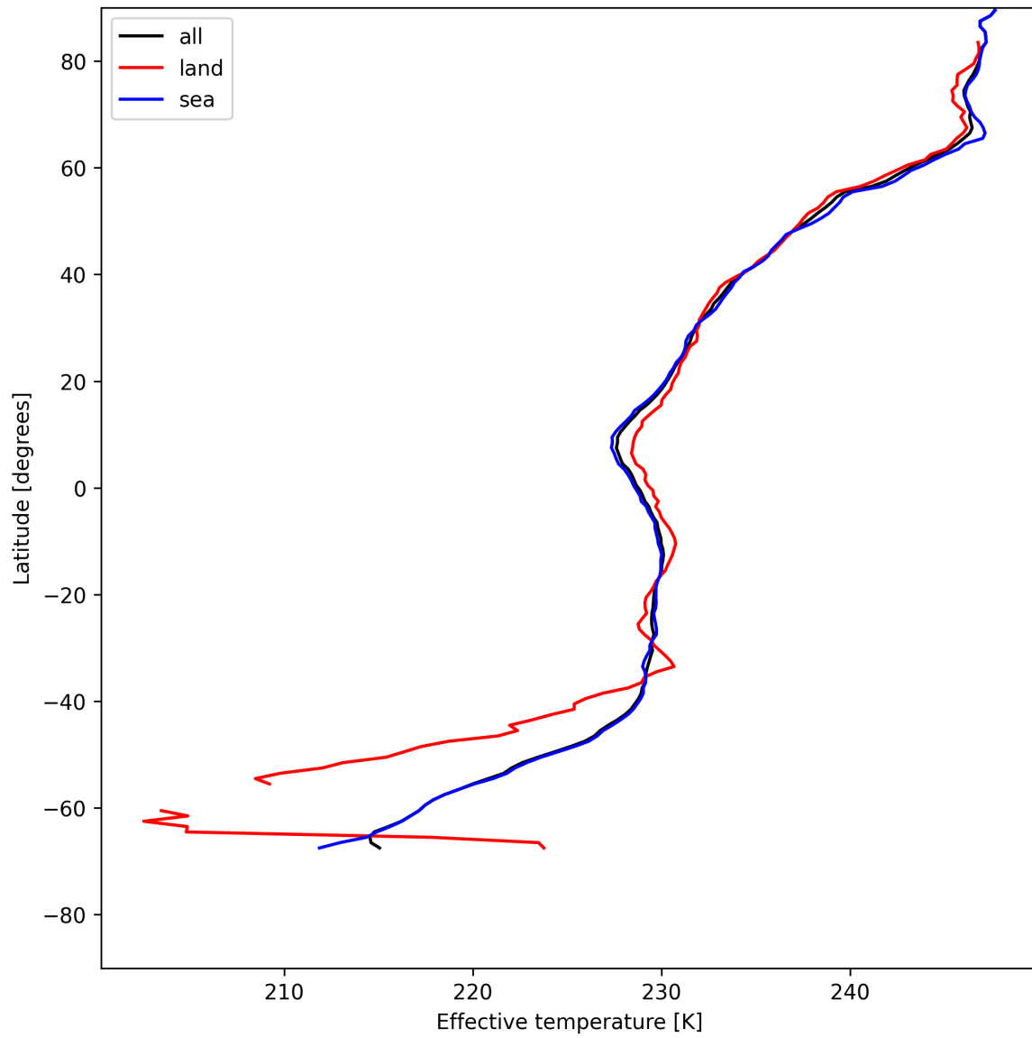
Figure 26: Zonal average of "Effective temperature" for 2025-07-18 to 2025-07-19.
