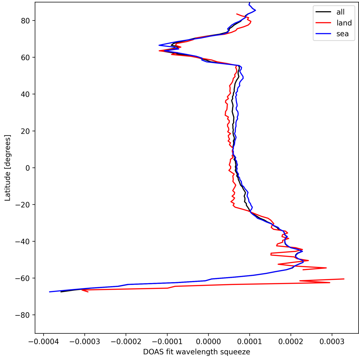
Figure 24: Zonal average of “DOAS fit wavelength squeeze” for 2025-07-18 to 2025-07-19.
