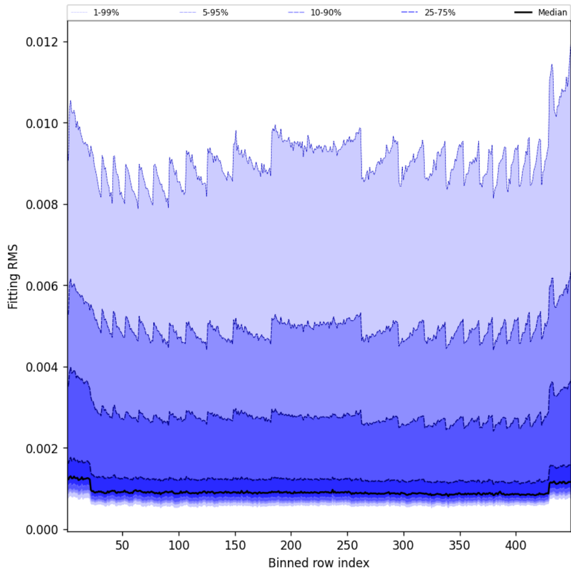
Figure 46: Along track statistics of “Fitting RMS” for 2025-07-18 to 2025-07-19
