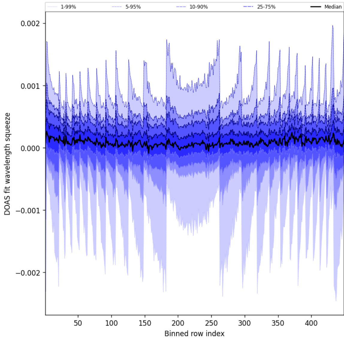
Figure 48: Along track statistics of “DOAS fit wavelength squeeze” for 2025-07-18 to 2025-07-19
