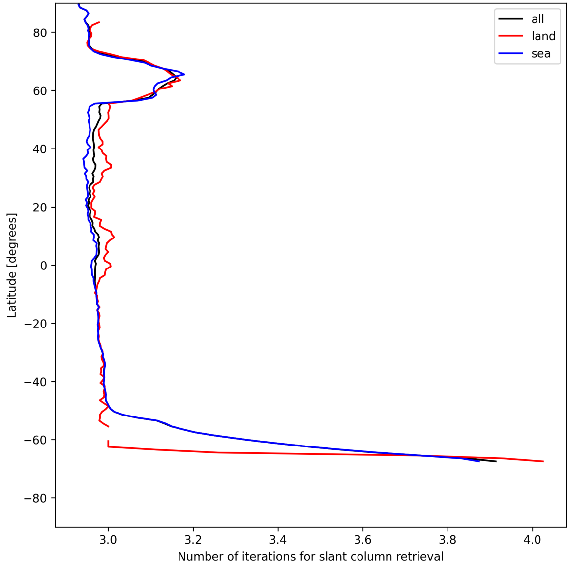
Figure 21: Zonal average of “Number of iterations for slant column retrieval” for 2025-07-18 to 2025-07-19.
