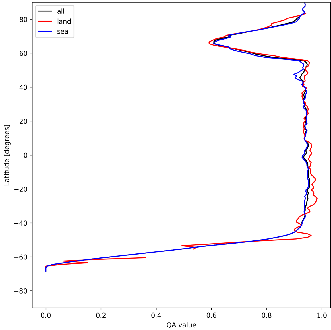
Figure 16: Zonal average of “QA value” for 2025-07-19 to 2025-07-20.
