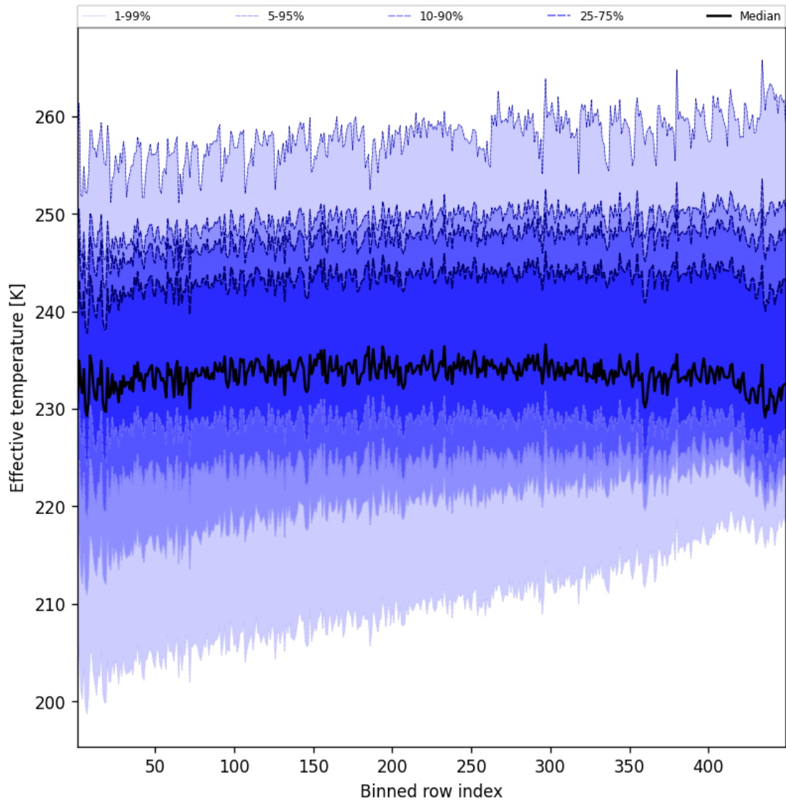
Figure 50: Along track statistics of “Effective temperature” for 2025-07-19 to 2025-07-20
