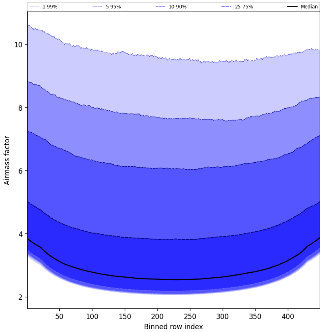
Figure 49: Along track statistics of “Airmass factor” for 2025-07-19 to 2025-07-20
