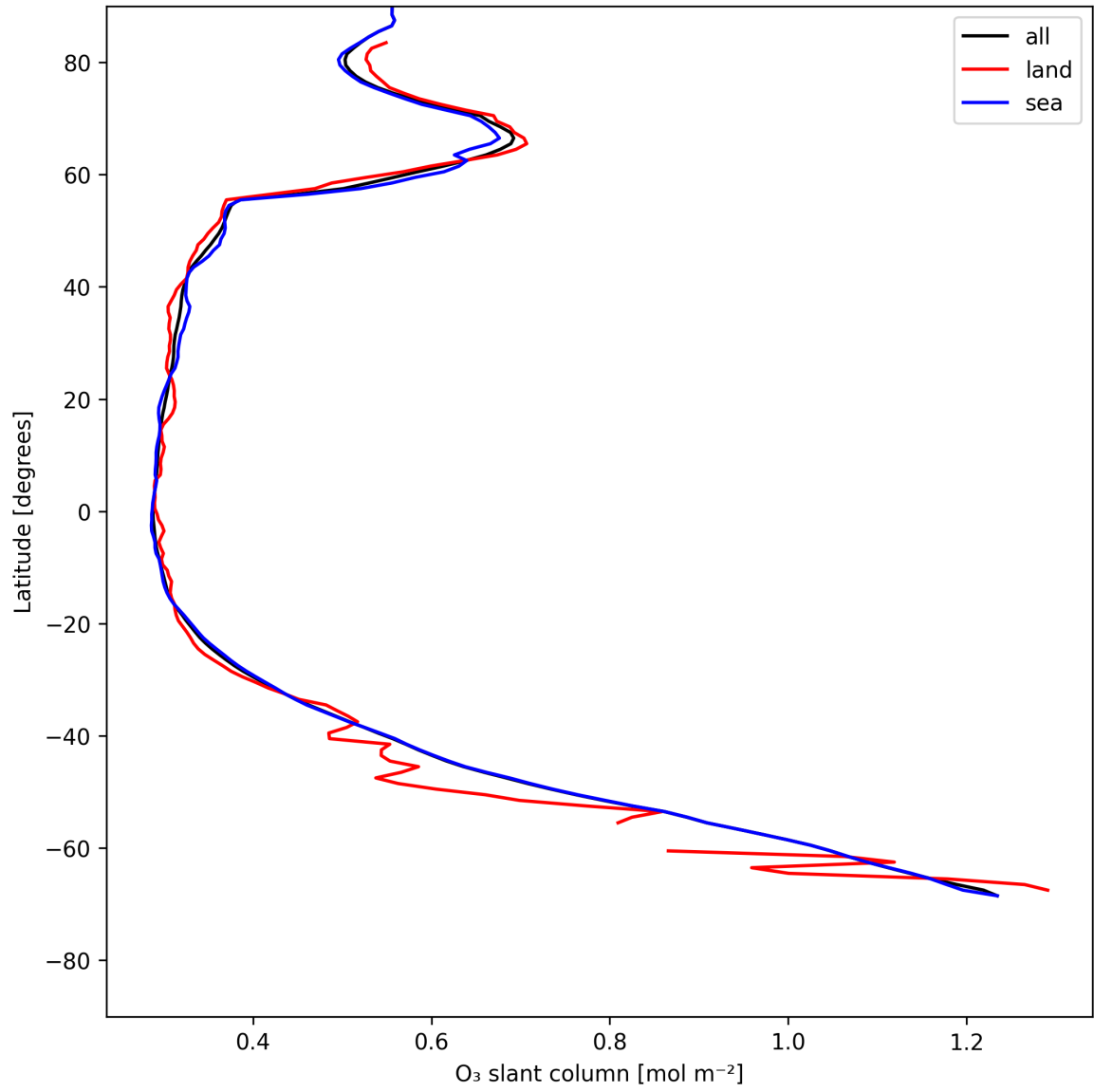
Figure 19: Zonal average of “O 3 slant column” for 2025-07-19 to 2025-07-20.
