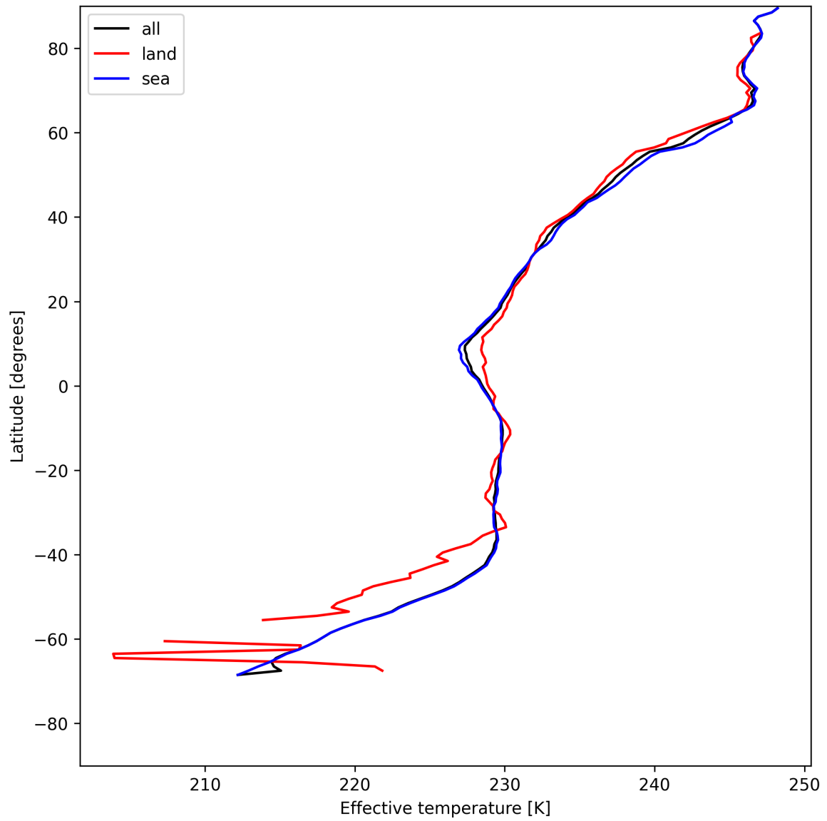
Figure 26: Zonal average of “Effective temperature” for 2025-07-19 to 2025-07-20.
