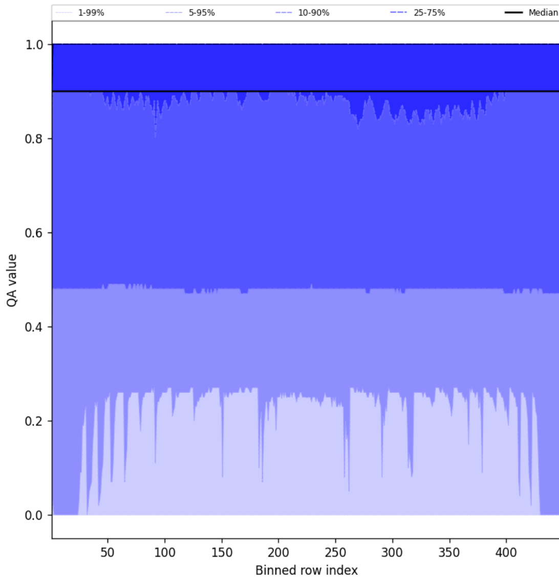
Figure 40: Along track statistics of “QA value” for 2025-07-19 to 2025-07-20
