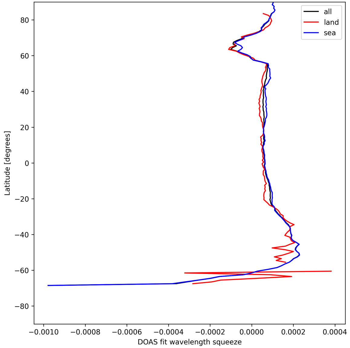
Figure 24: Zonal average of “DOAS fit wavelength squeeze” for 2025-07-19 to 2025-07-20.
