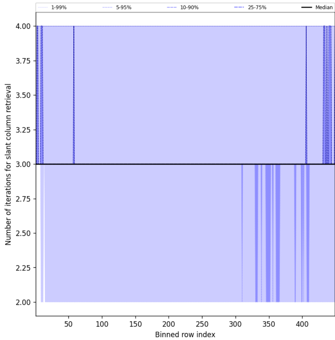
Figure 45: Along track statistics of “Number of iterations for slant column retrieval” for 2025-07-19 to 2025-07-20
