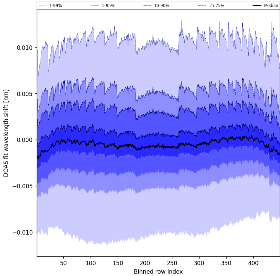
Figure 47: Along track statistics of “DOAS fit wavelength shift” for 2025-07-19 to 2025-07-20
