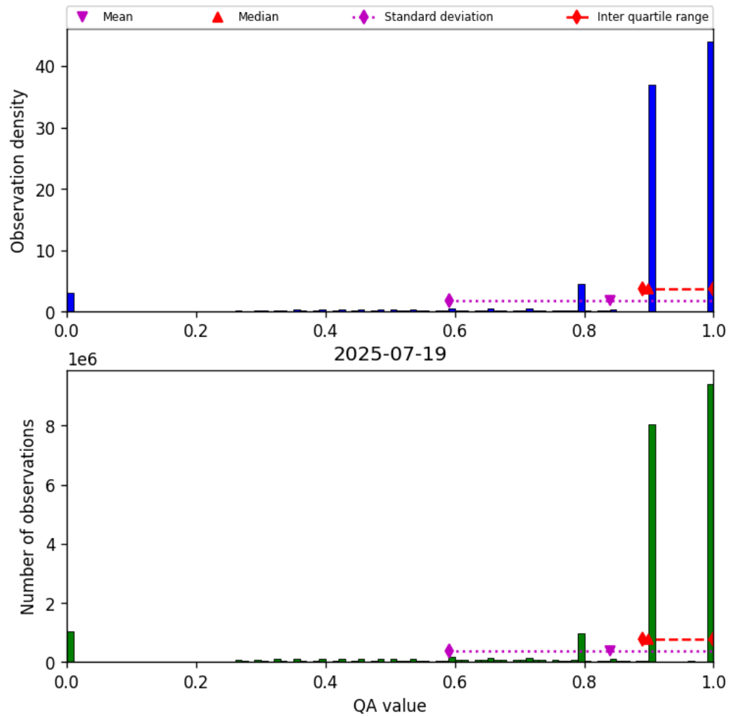
Figure 28: Histogram of “QA value” for 2025-07-19 to 2025-07-20
