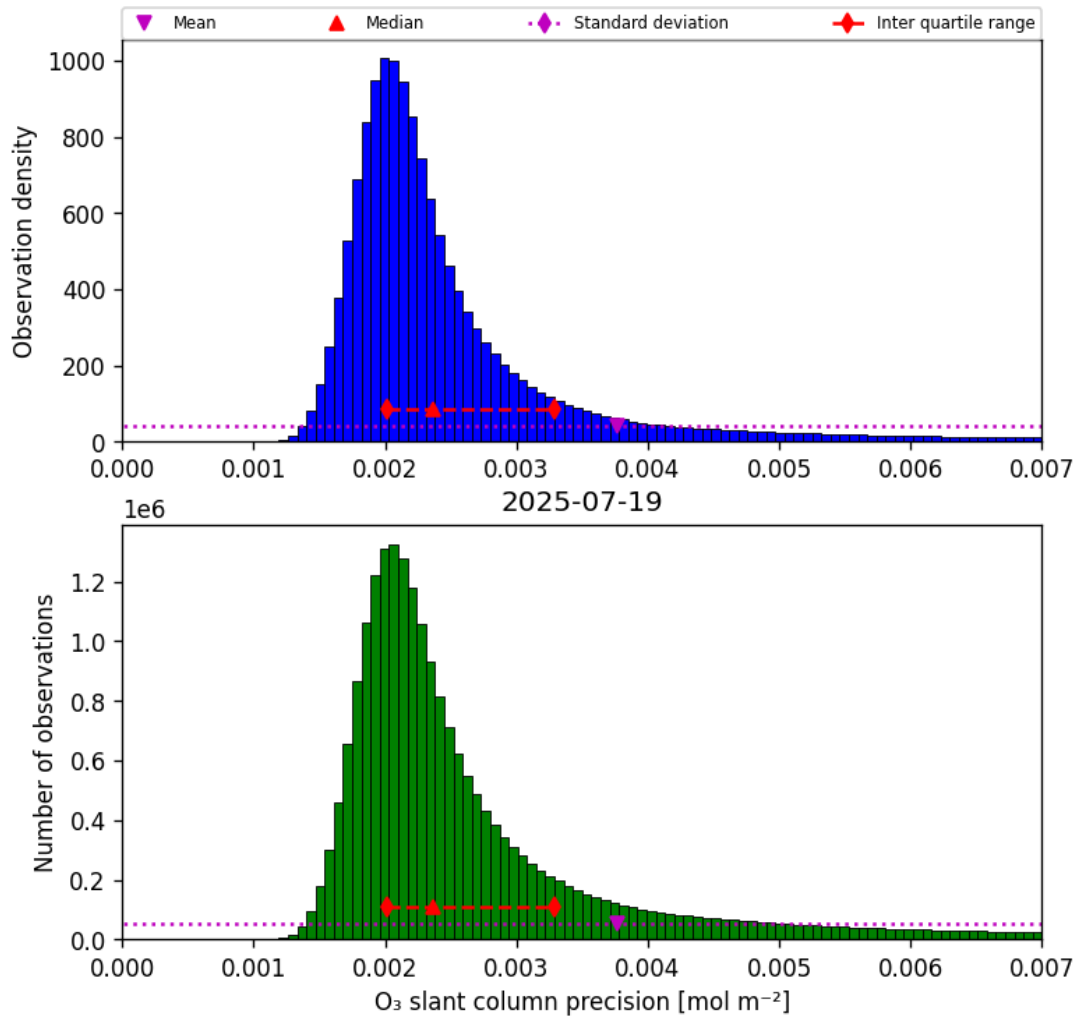
Figure 32: Histogram of “O 3 slant column precision” for 2025-07-19 to 2025-07-20
