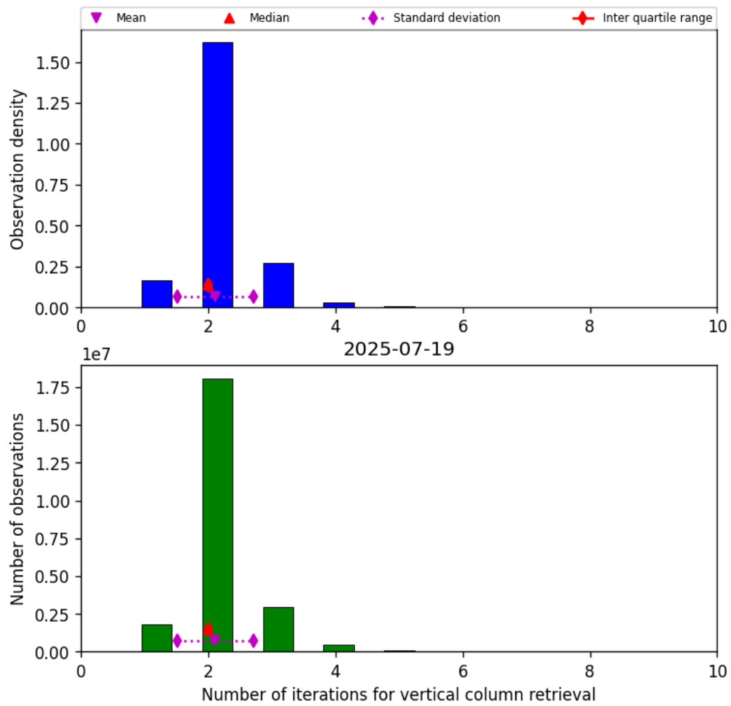
Figure 39: Histogram of “Number of iterations for vertical column retrieval” for 2025-07-19 to 2025-07-20
