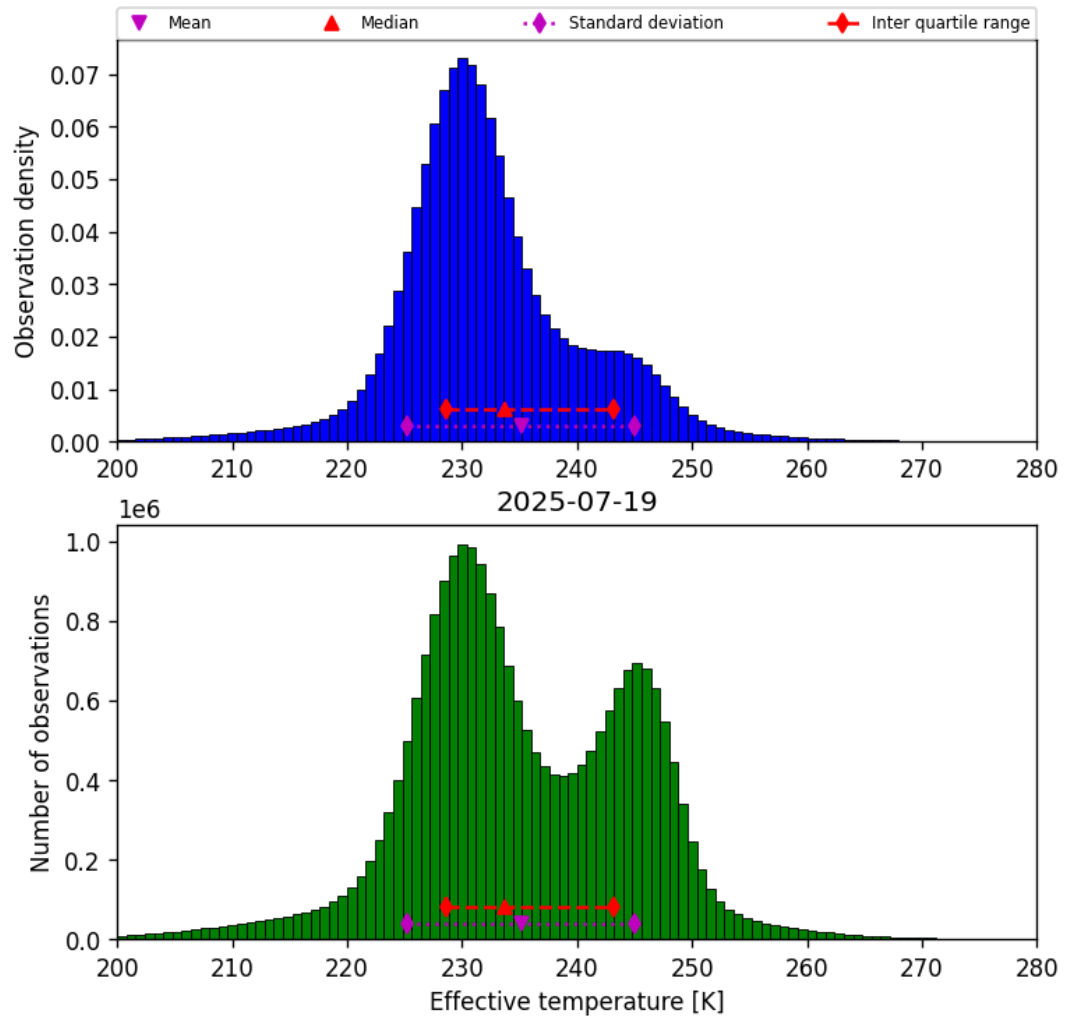
Figure 38: Histogram of “Effective temperature” for 2025-07-19 to 2025-07-20
