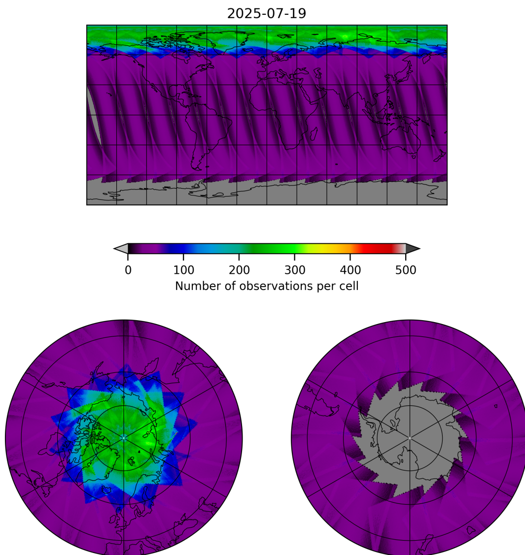
Figure 15: Map of the number of observations for 2025-07-19 to 2025-07-20
