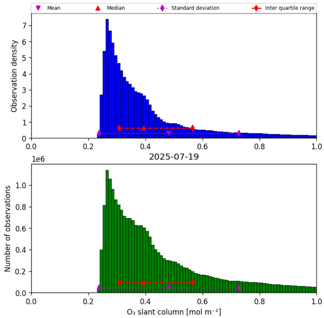
Figure 31: Histogram of “O 3 slant column” for 2025-07-19 to 2025-07-20
