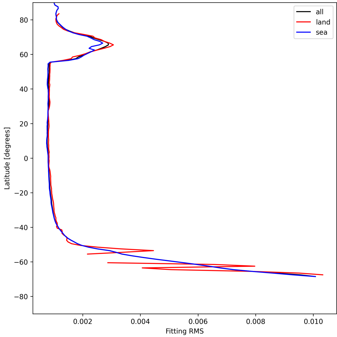
Figure 22: Zonal average of “Fitting RMS” for 2025-07-19 to 2025-07-20.
