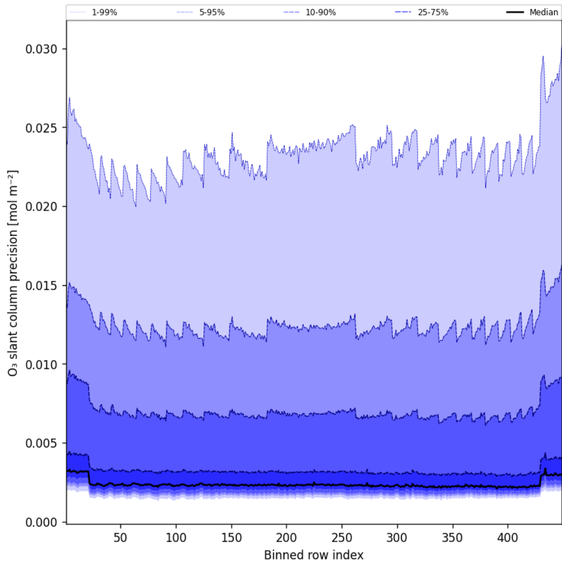
Figure 44: Along track statistics of “O 3 slant column precision” for 2025-07-19 to 2025-07-20
