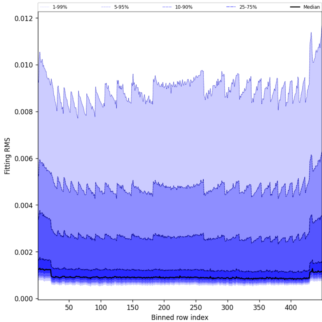
Figure 46: Along track statistics of “Fitting RMS” for 2025-07-19 to 2025-07-20
