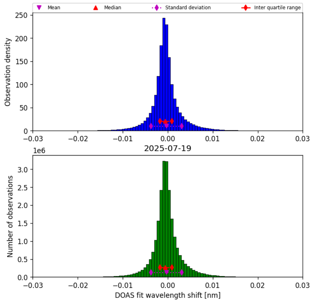
Figure 35: Histogram of “DOAS fit wavelength shift” for 2025-07-19 to 2025-07-20
