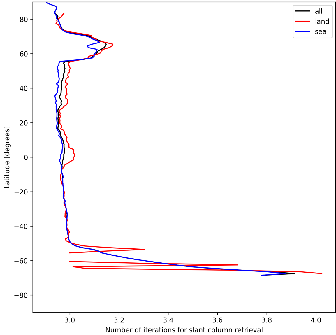
Figure 21: Zonal average of “Number of iterations for slant column retrieval” for 2025-07-19 to 2025-07-20.
