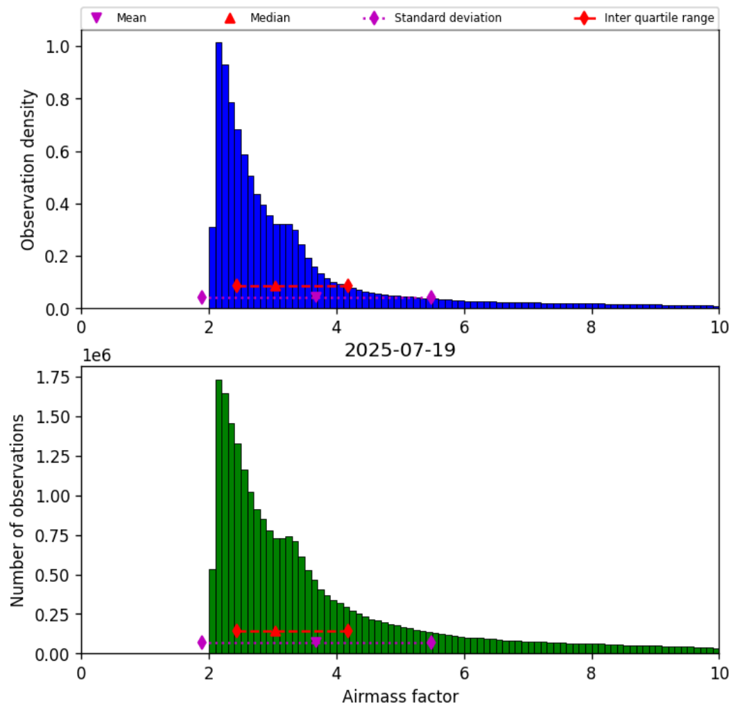
Figure 37: Histogram of “Airmass factor” for 2025-07-19 to 2025-07-20
