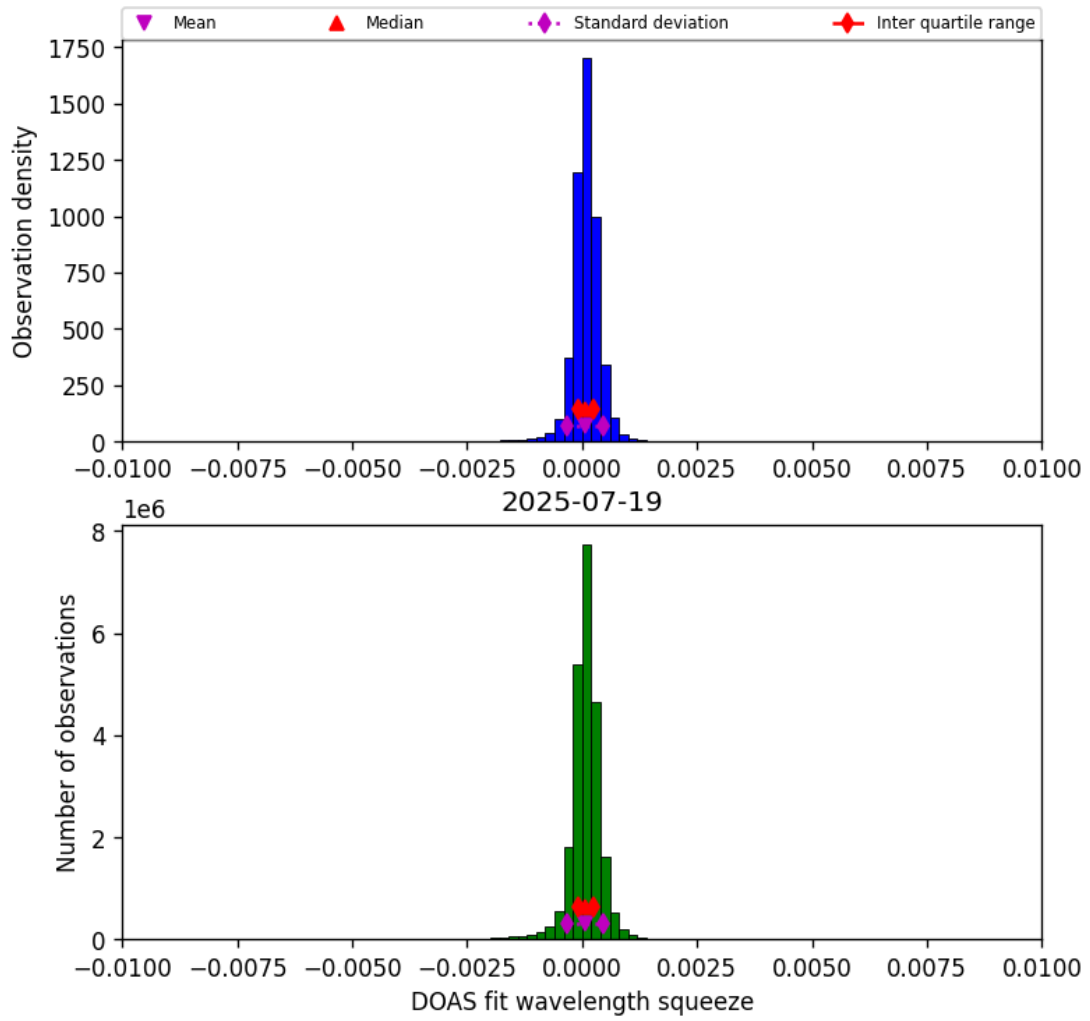
Figure 36: Histogram of “DOAS fit wavelength squeeze” for 2025-07-19 to 2025-07-20
