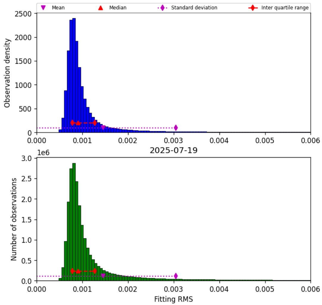
Figure 34: Histogram of “Fitting RMS” for 2025-07-19 to 2025-07-20
