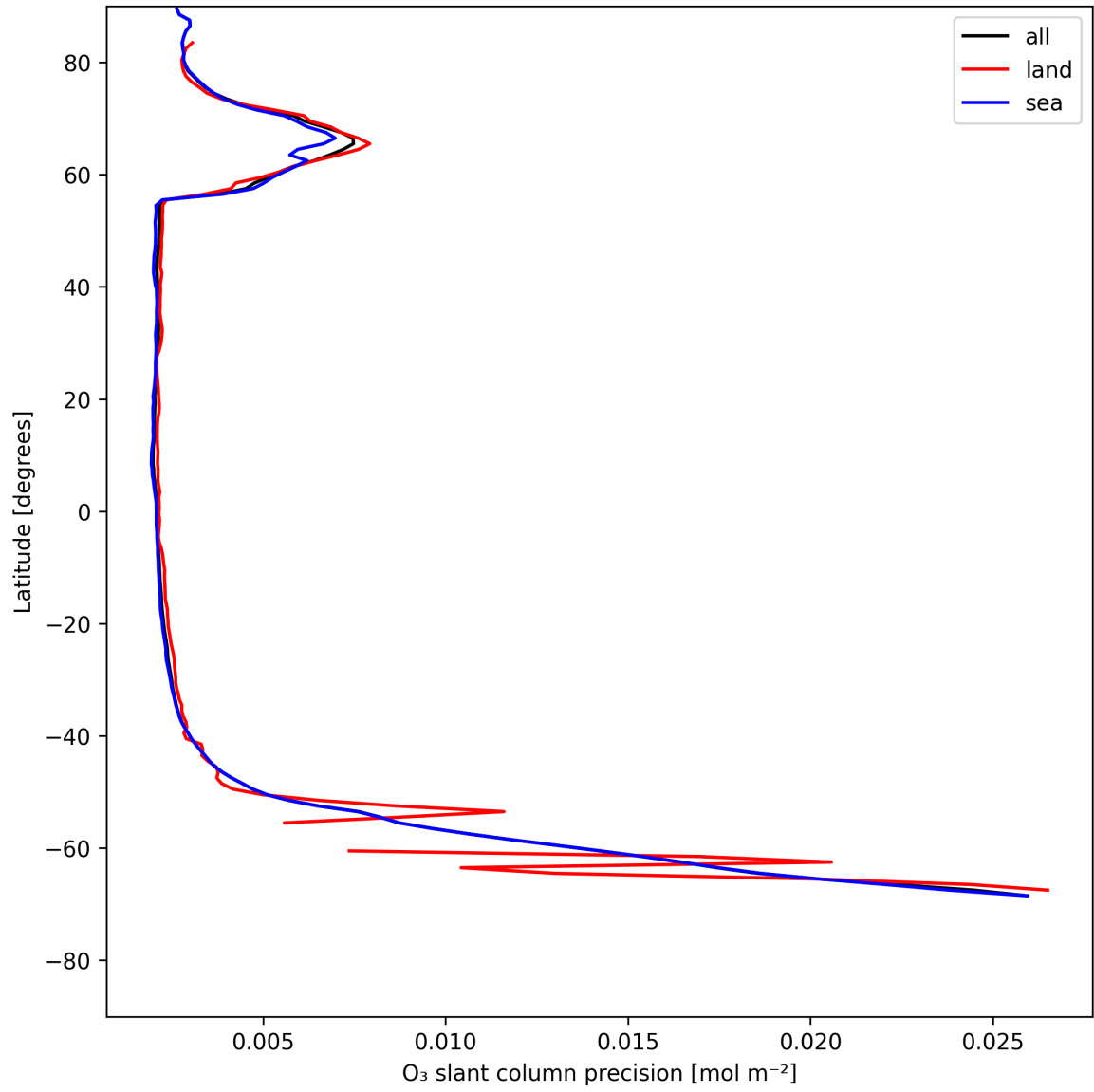
Figure 20: Zonal average of "O 3 slant column precision" for 2025-07-19 to 2025-07-20.
