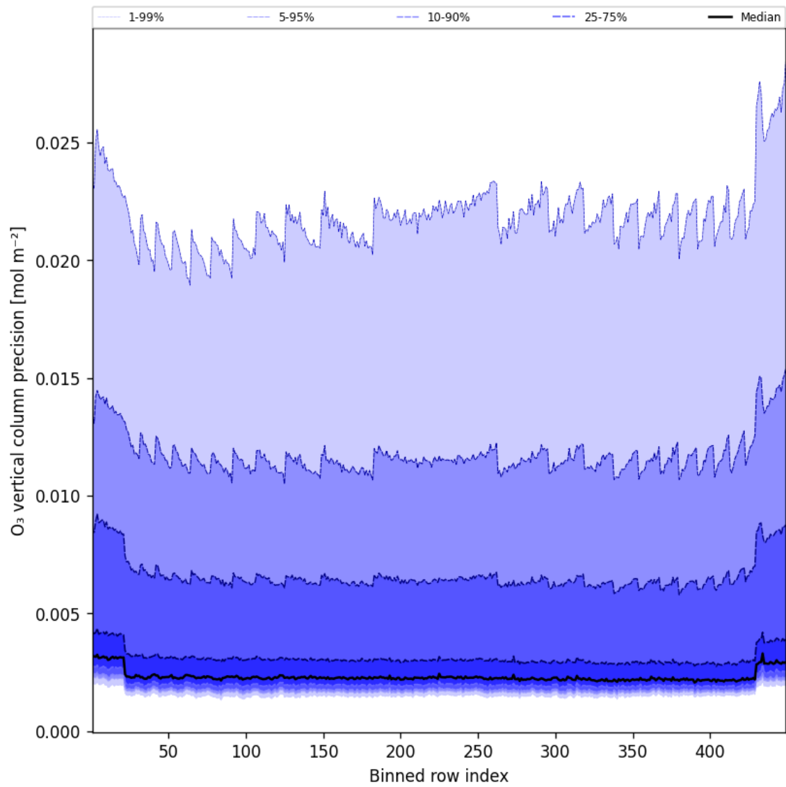
Figure 42: Along track statistics of “O 3 vertical column precision” for 2025-07-19 to 2025-07-20
