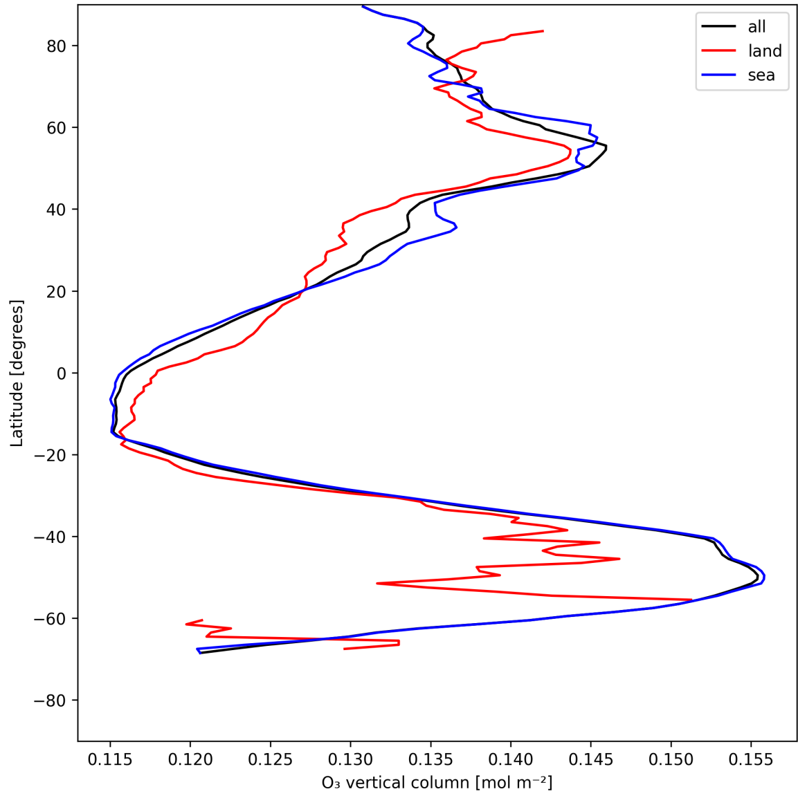
Figure 17: Zonal average of “O 3 vertical column” for 2025-07-19 to 2025-07-20.
