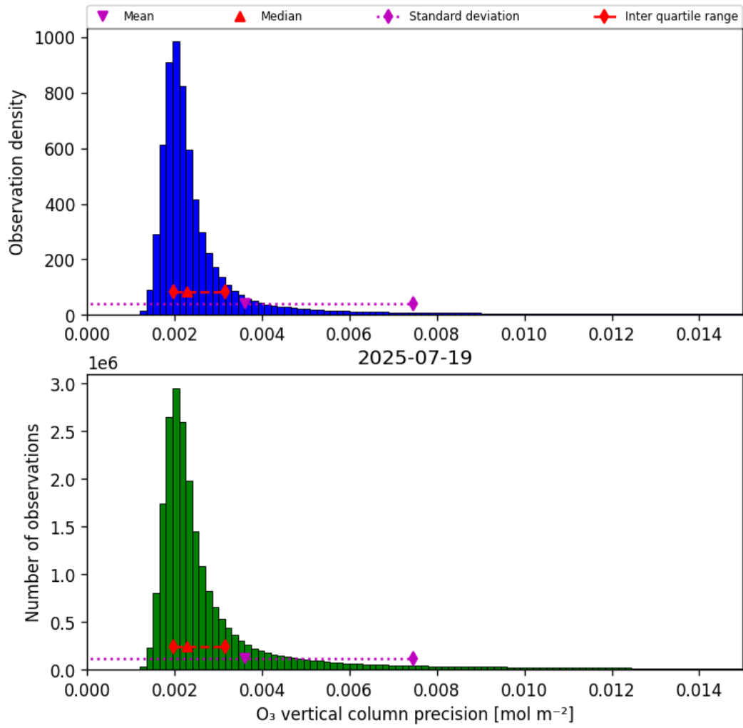
Figure 30: Histogram of “O 3 vertical column precision” for 2025-07-19 to 2025-07-20
