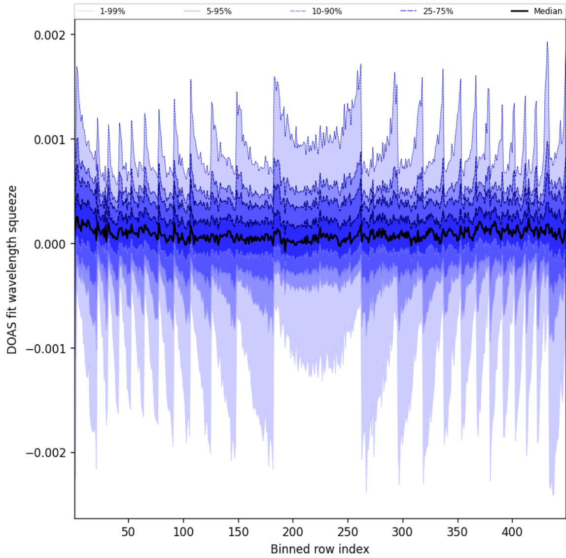
Figure 48: Along track statistics of “DOAS fit wavelength squeeze” for 2025-07-19 to 2025-07-20
