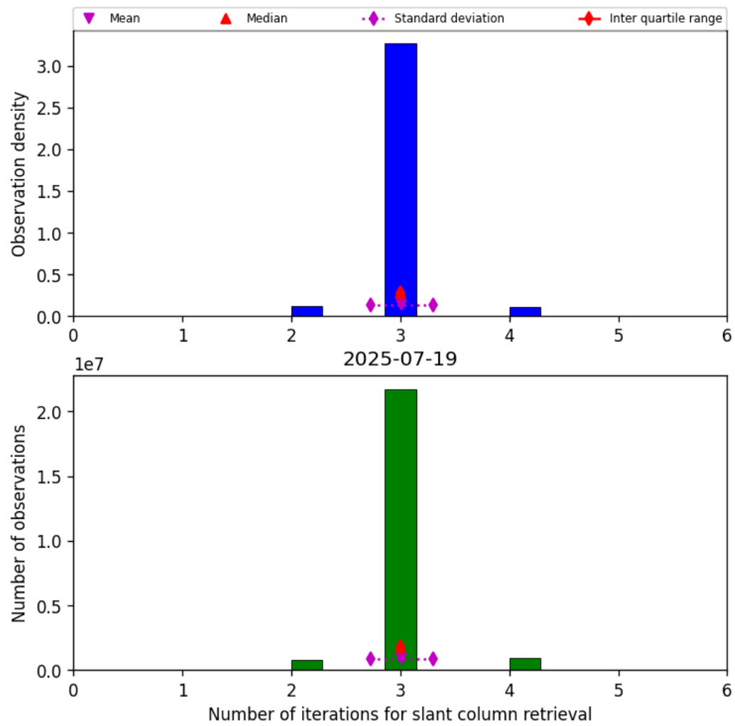
Figure 33: Histogram of “Number of iterations for slant column retrieval” for 2025-07-19 to 2025-07-20
