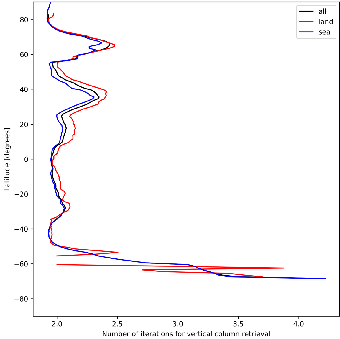
Figure 27: Zonal average of “Number of iterations for vertical column retrieval” for 2025-07-19 to 2025-07-20.
