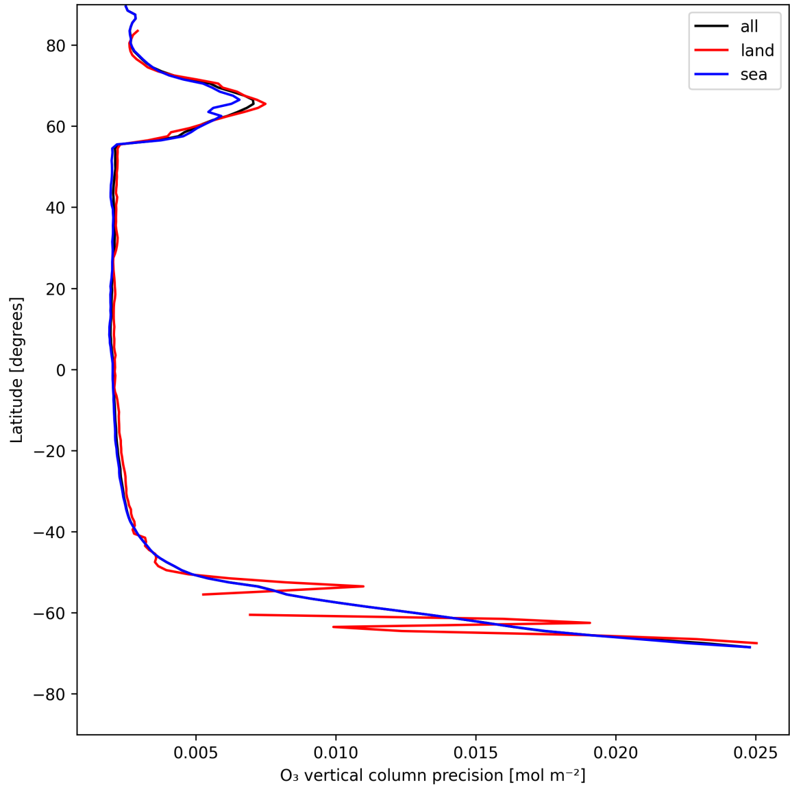
Figure 18: Zonal average of “O 3 vertical column precision” for 2025-07-19 to 2025-07-20.
