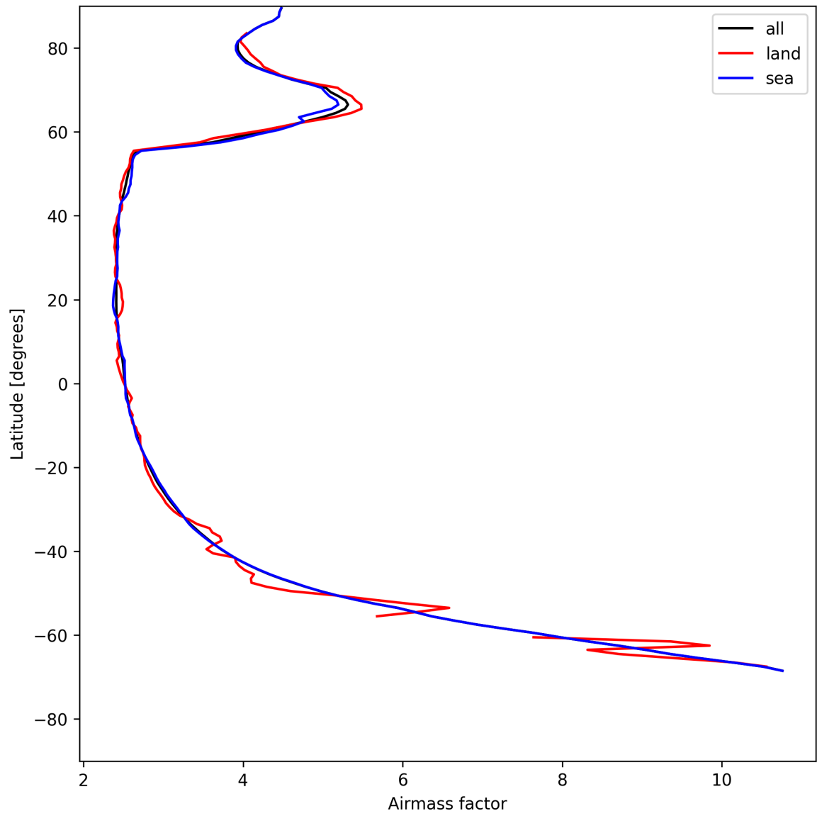
Figure 25: Zonal average of “Airmass factor” for 2025-07-19 to 2025-07-20.
