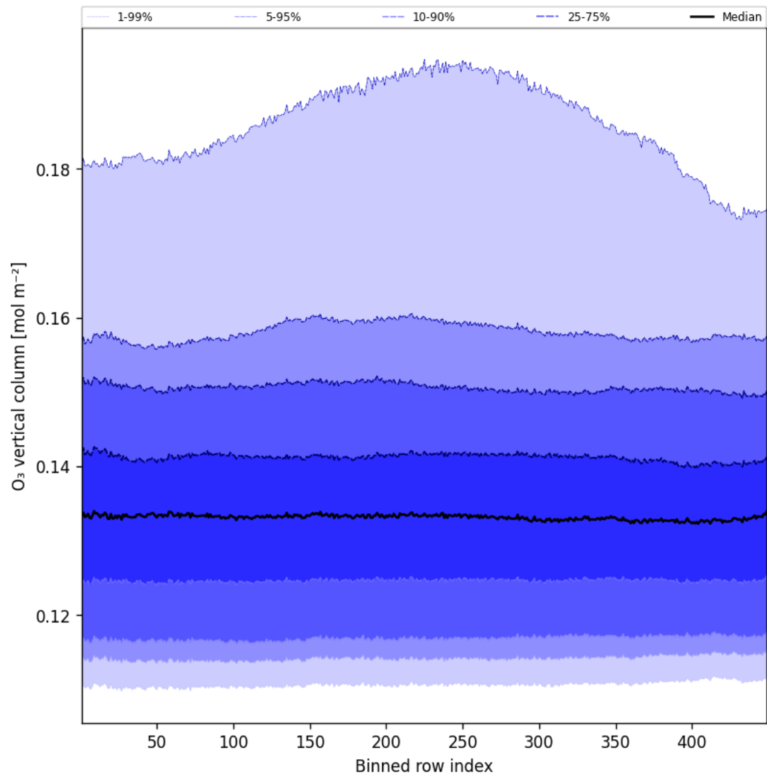
Figure 41: Along track statistics of “O 3 vertical column” for 2025-07-19 to 2025-07-20
