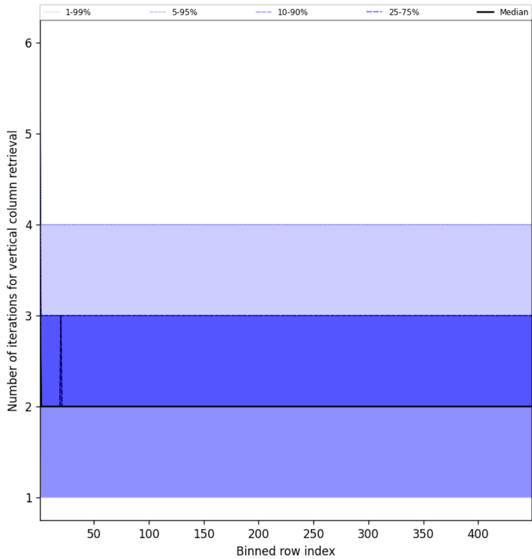
Figure 51: Along track statistics of “Number of iterations for vertical column retrieval” for 2025-07-19 to 2025-07-20
