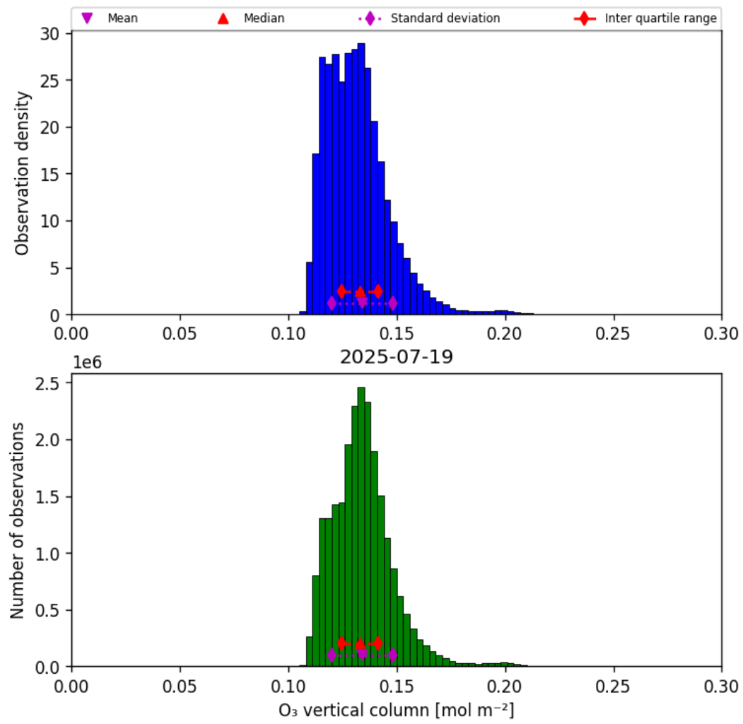
Figure 29: Histogram of “O 3 vertical column” for 2025-07-19 to 2025-07-20
