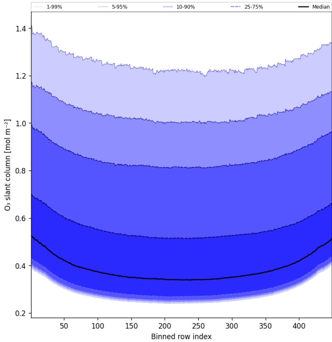
Figure 43: Along track statistics of “O 3 slant column” for 2025-07-19 to 2025-07-20
