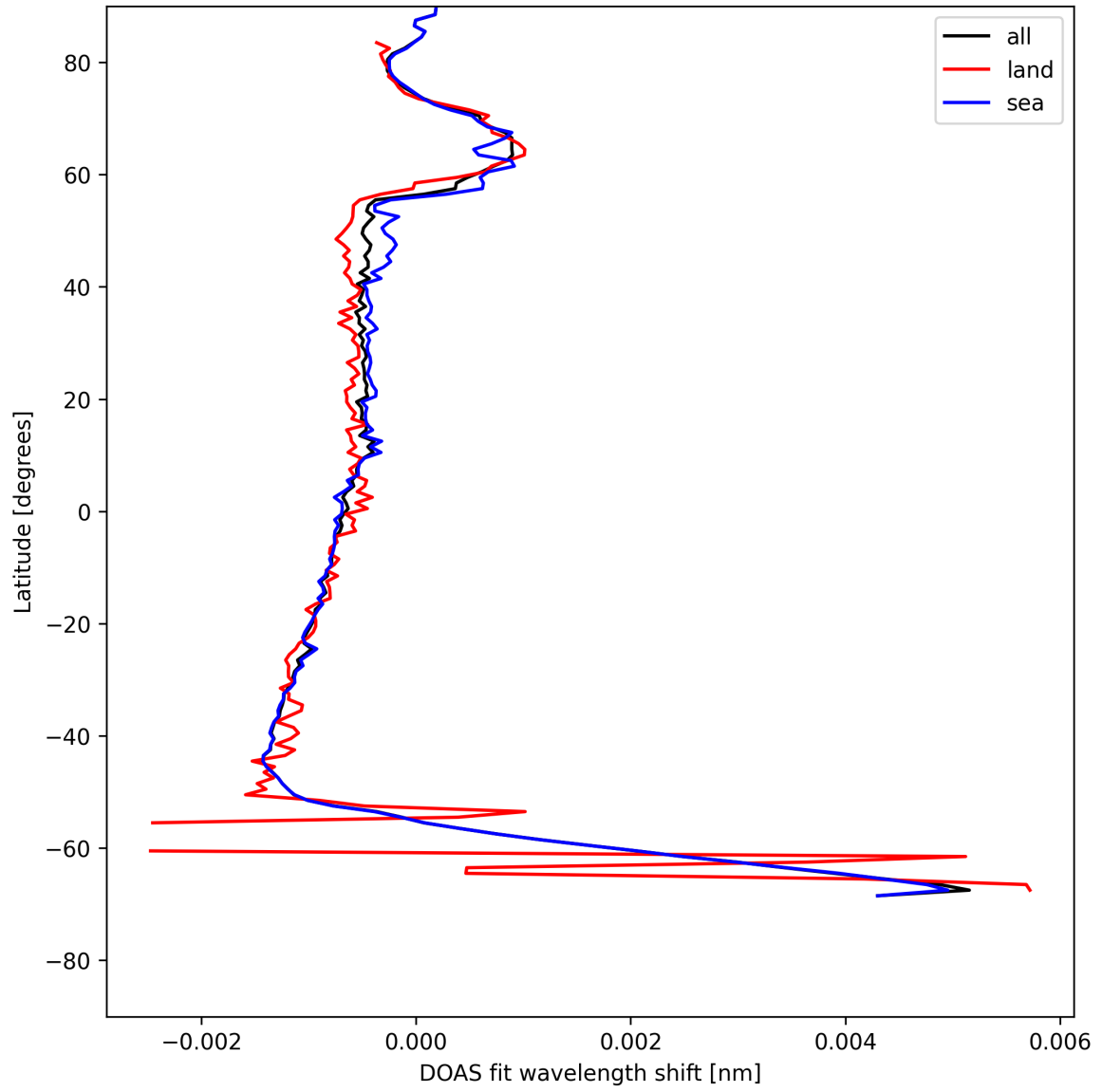
Figure 23: Zonal average of "DOAS fit wavelength shift" for 2025-07-19 to 2025-07-20.
