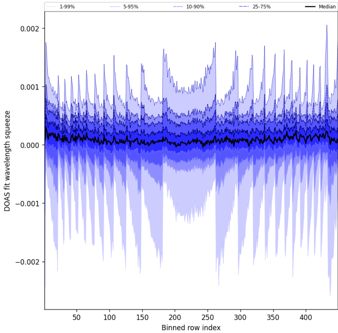
Figure 48: Along track statistics of “DOAS fit wavelength squeeze” for 2025-07-20 to 2025-07-21
