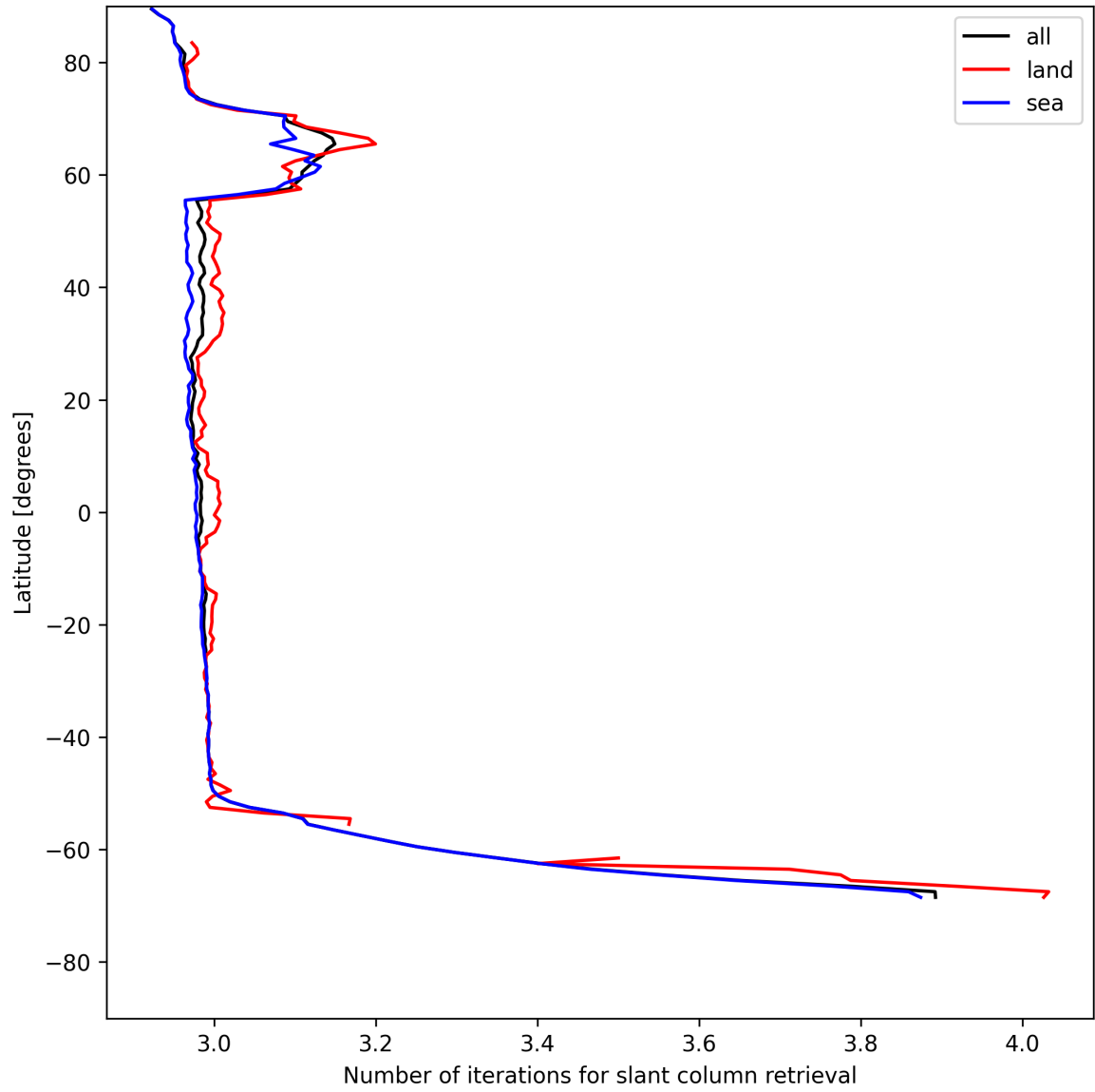
Figure 21: Zonal average of “Number of iterations for slant column retrieval” for 2025-07-20 to 2025-07-21.
