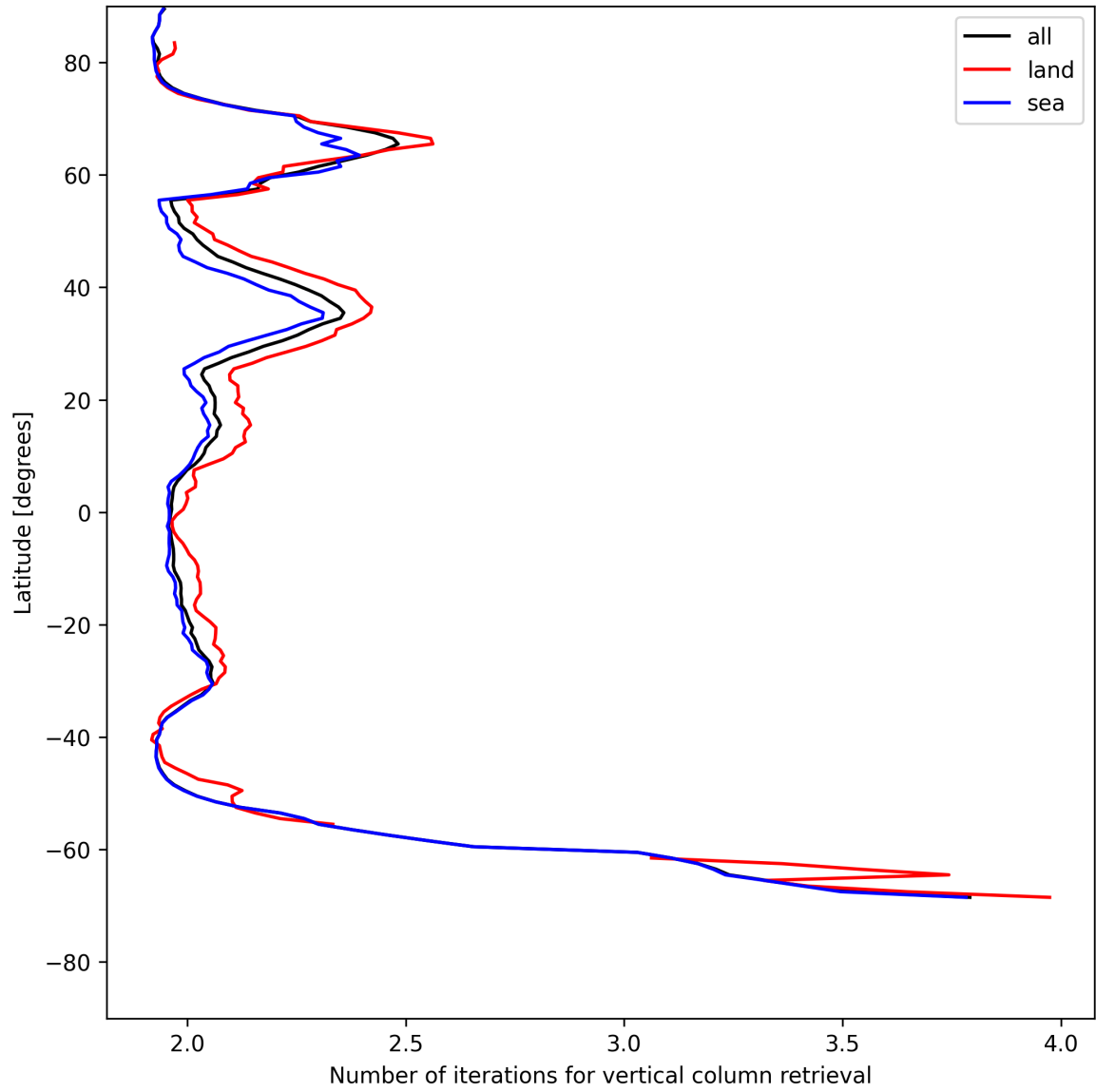
Figure 27: Zonal average of “Number of iterations for vertical column retrieval” for 2025-07-20 to 2025-07-21.
