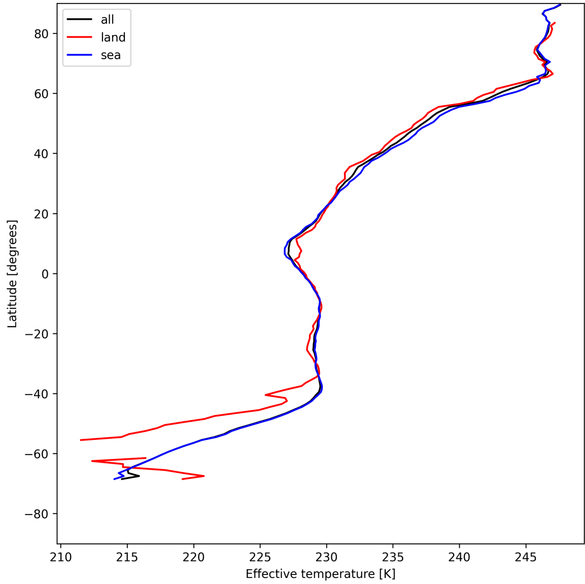
Figure 26: Zonal average of "Effective temperature" for 2025-07-20 to 2025-07-21.
