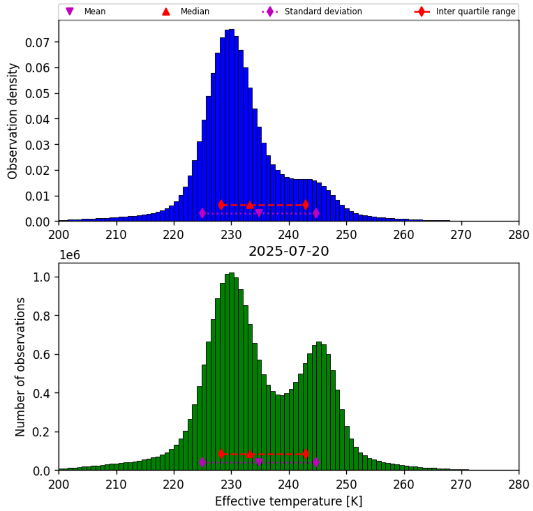
Figure 38: Histogram of “Effective temperature” for 2025-07-20 to 2025-07-21
