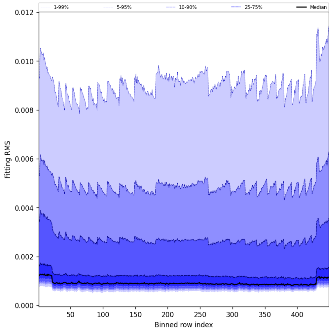
Figure 46: Along track statistics of “Fitting RMS” for 2025-07-20 to 2025-07-21
