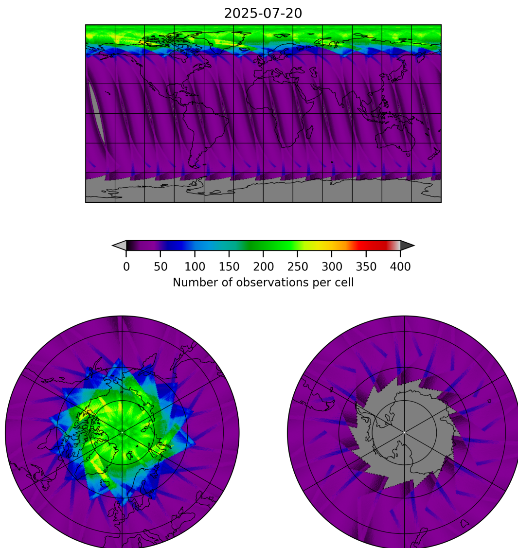
Figure 15: Map of the number of observations for 2025-07-20 to 2025-07-21
