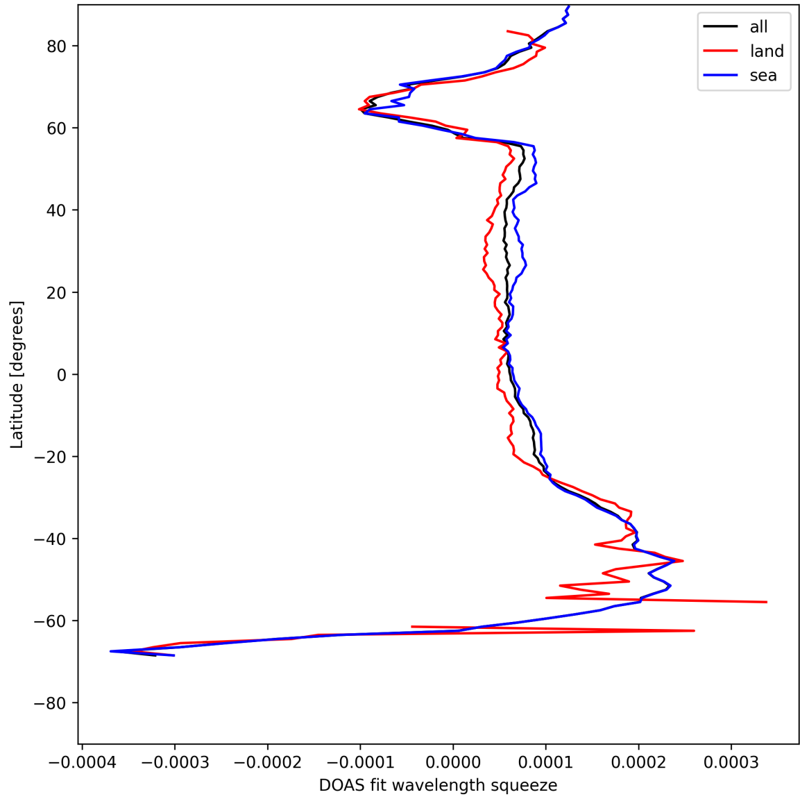
Figure 24: Zonal average of “DOAS fit wavelength squeeze” for 2025-07-20 to 2025-07-21.
