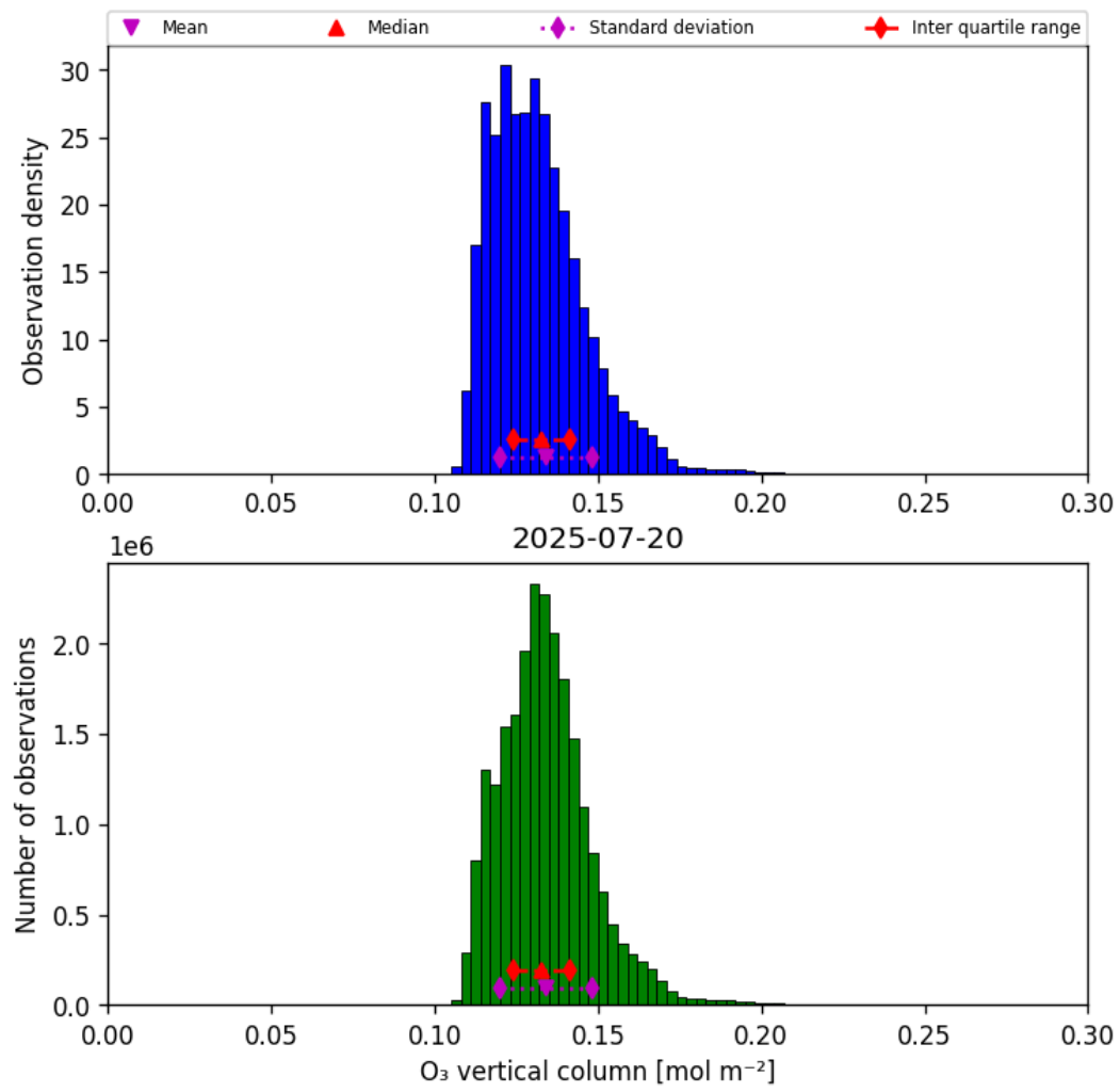
Figure 29: Histogram of “O 3 vertical column” for 2025-07-20 to 2025-07-21
