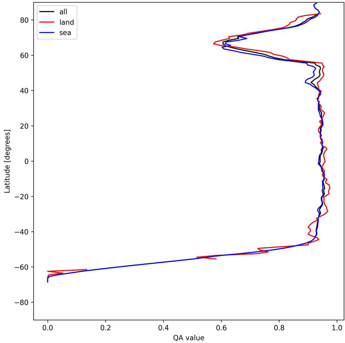
Figure 16: Zonal average of “QA value” for 2025-07-20 to 2025-07-21.
