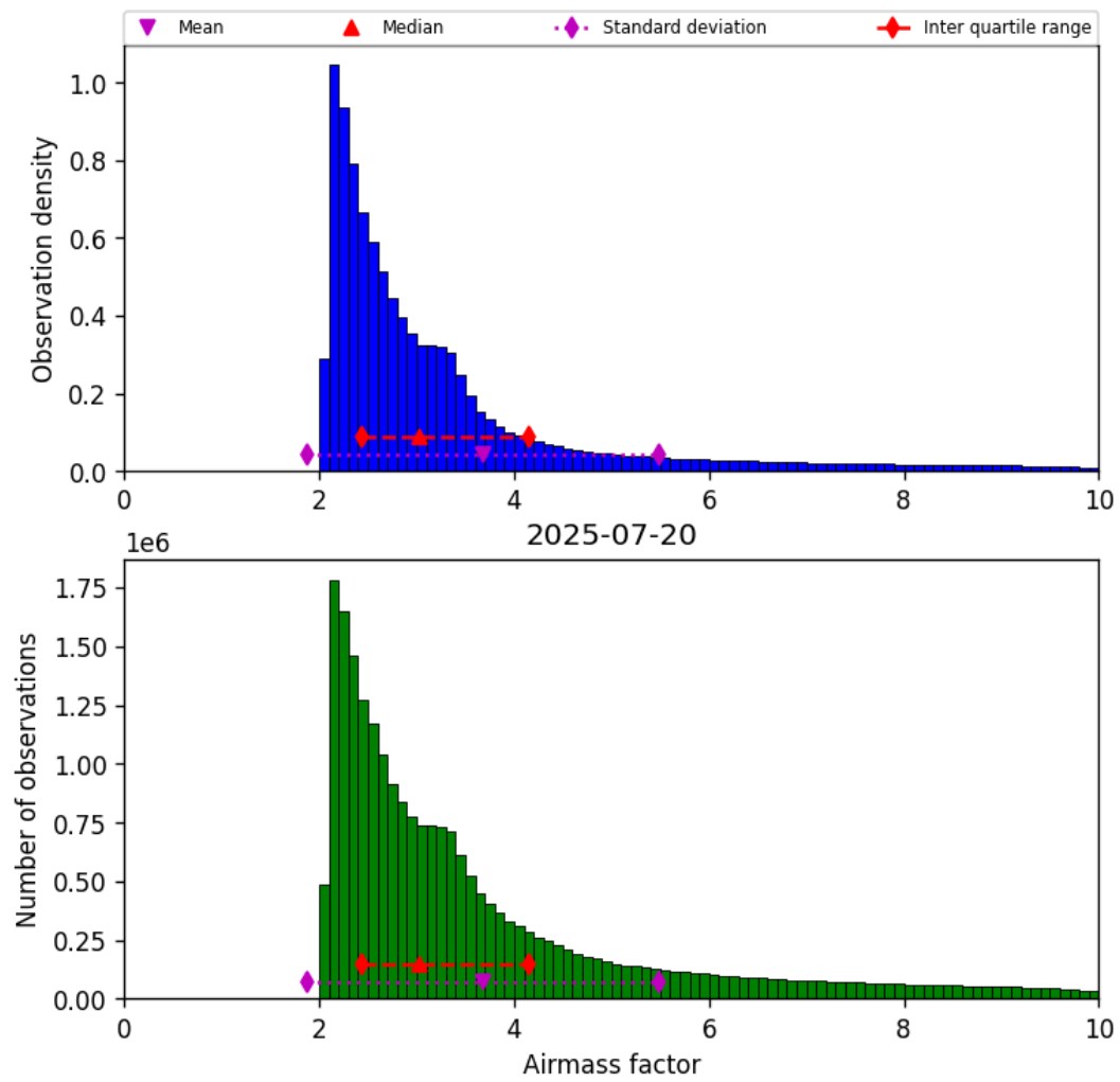
Figure 37: Histogram of “Airmass factor” for 2025-07-20 to 2025-07-21
