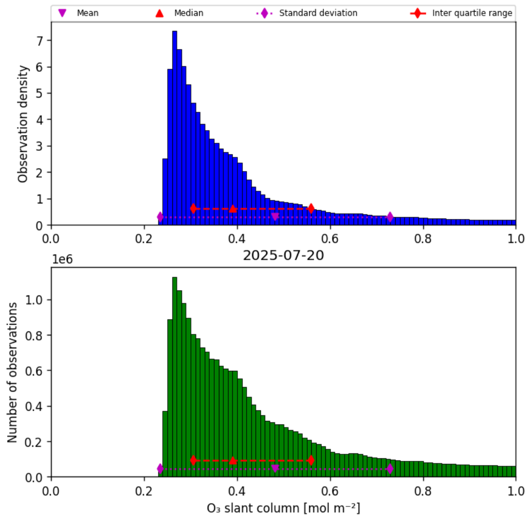
Figure 31: Histogram of “O 3 slant column” for 2025-07-20 to 2025-07-21
