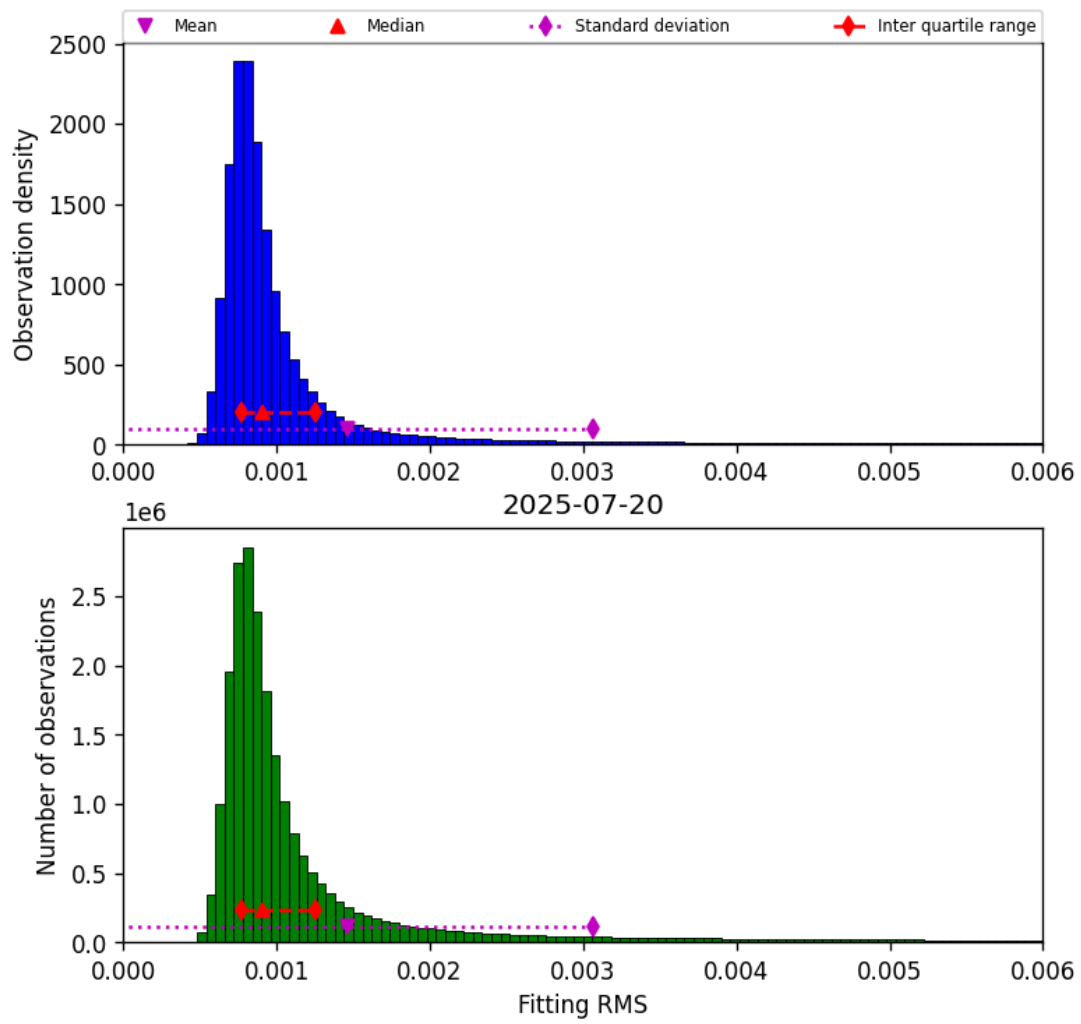
Figure 34: Histogram of “Fitting RMS” for 2025-07-20 to 2025-07-21
