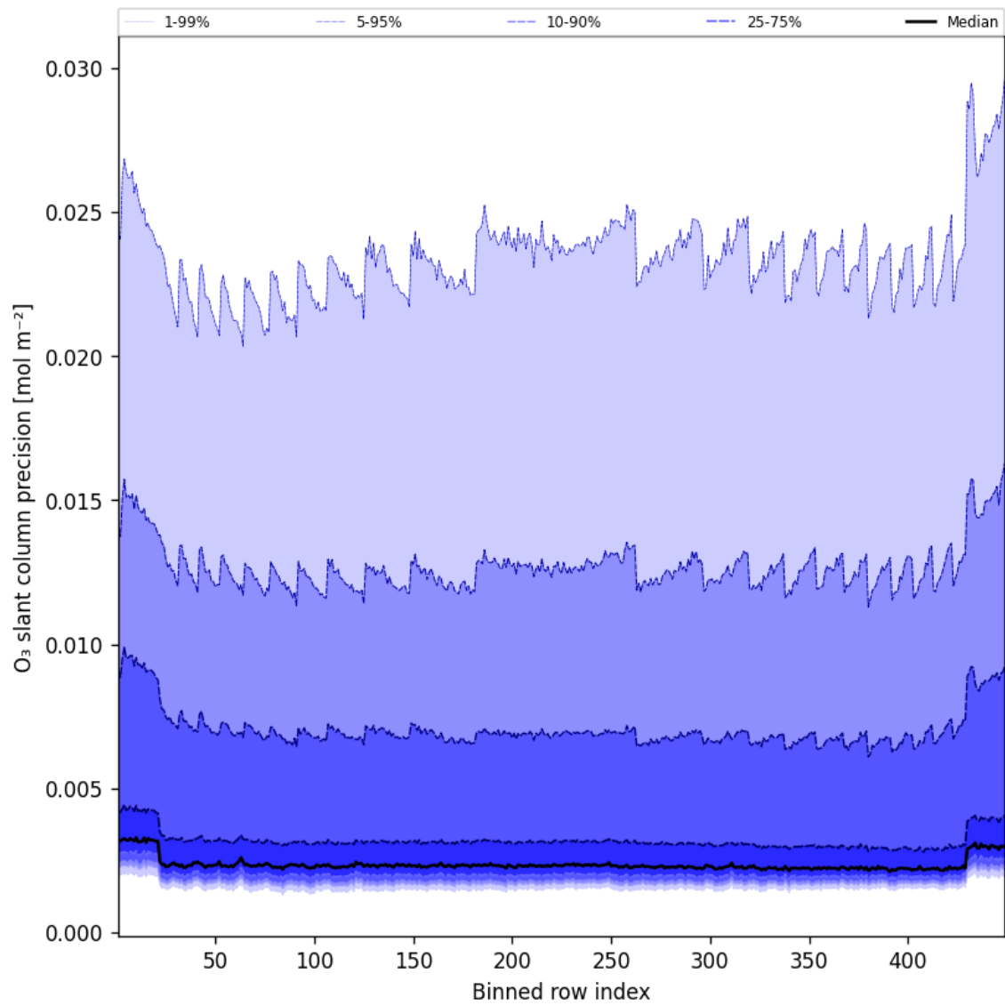
Figure 44: Along track statistics of “O 3 slant column precision” for 2025-07-20 to 2025-07-21
