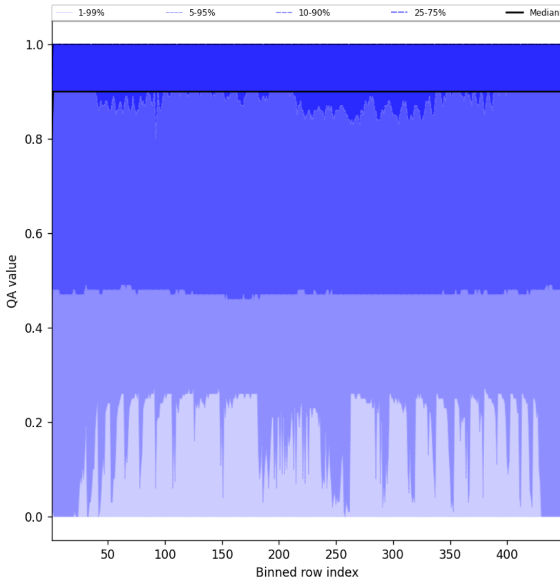
Figure 40: Along track statistics of “QA value” for 2025-07-20 to 2025-07-21
