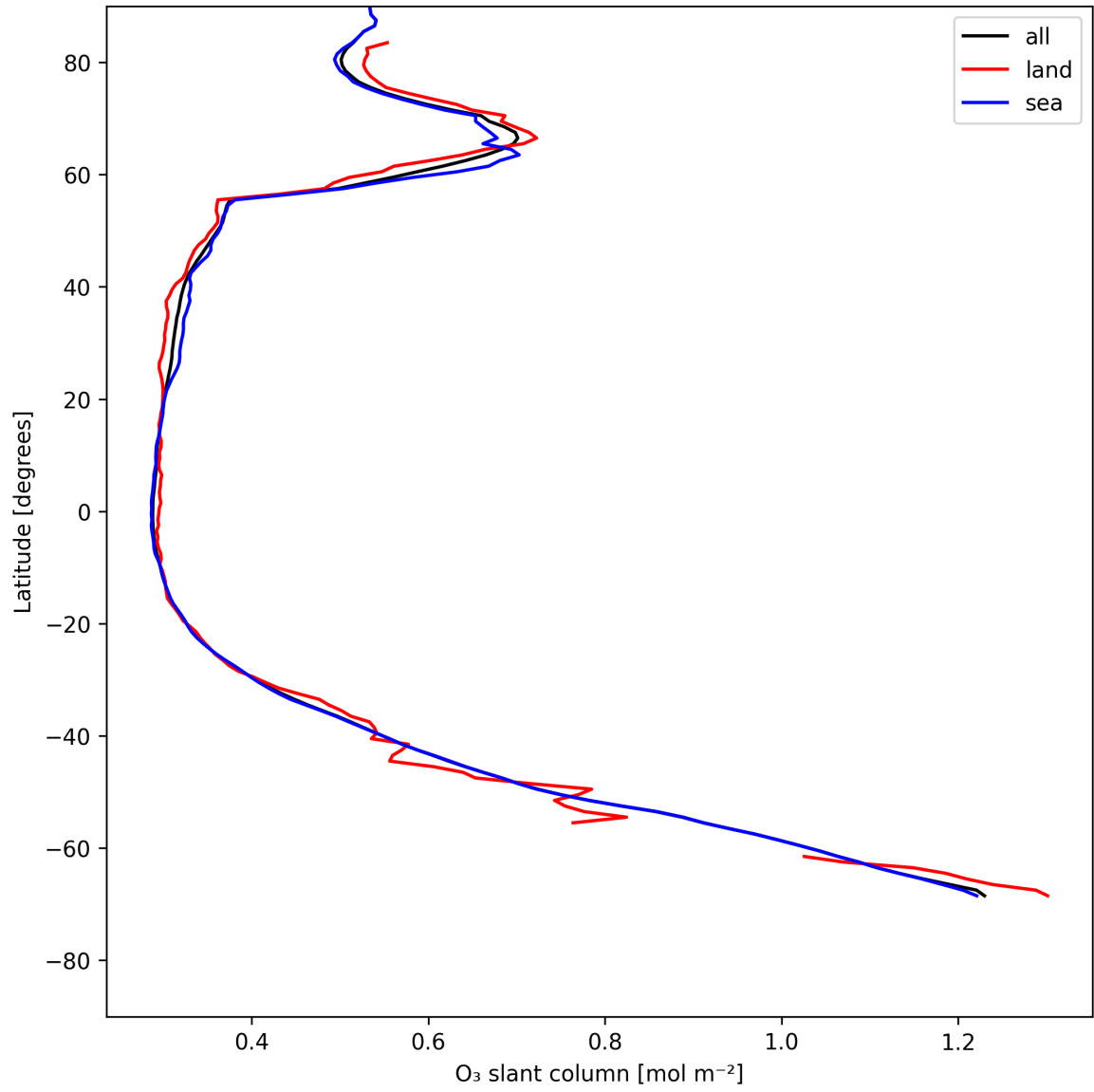
Figure 19: Zonal average of “O 3 slant column” for 2025-07-20 to 2025-07-21.
