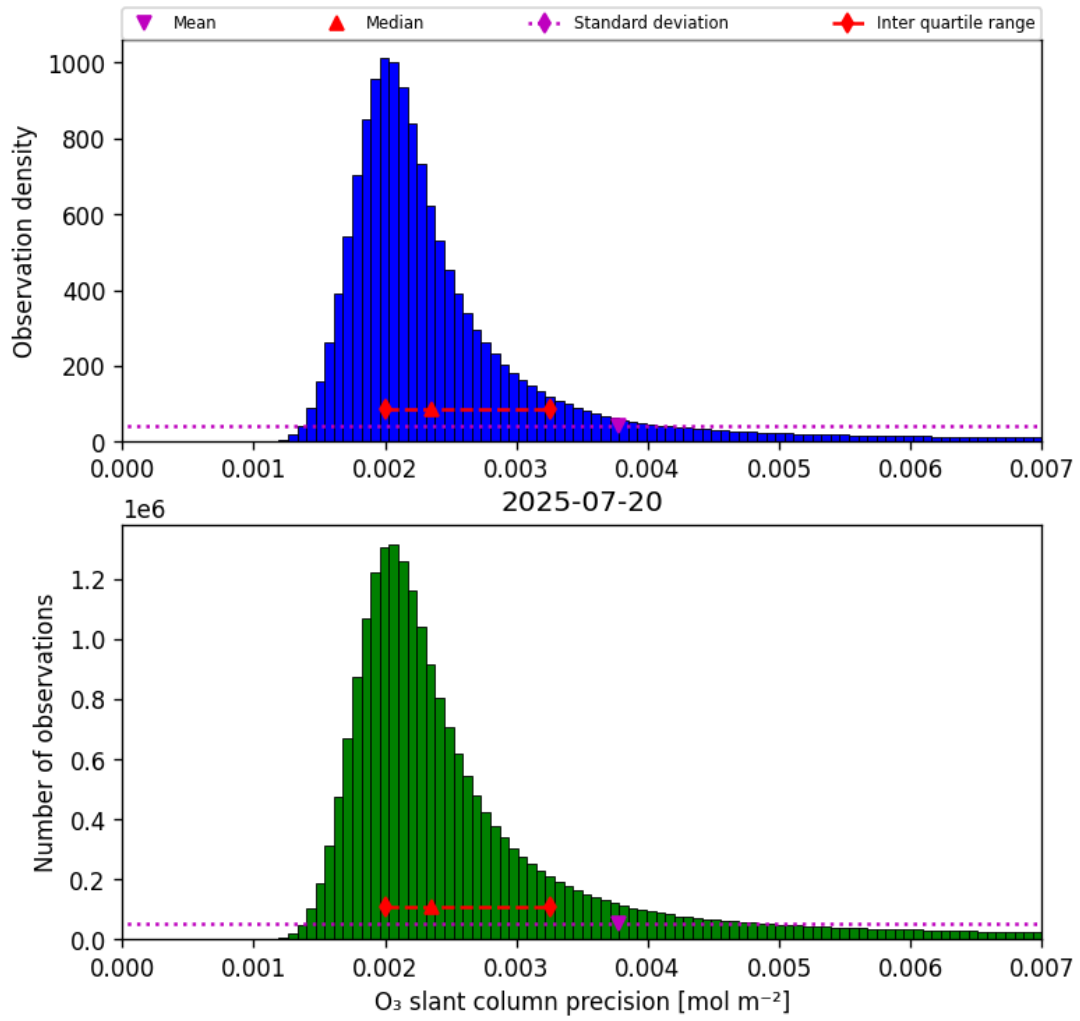
Figure 32: Histogram of “O 3 slant column precision” for 2025-07-20 to 2025-07-21
