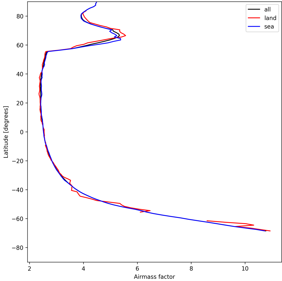
Figure 25: Zonal average of “Airmass factor” for 2025-07-20 to 2025-07-21.
