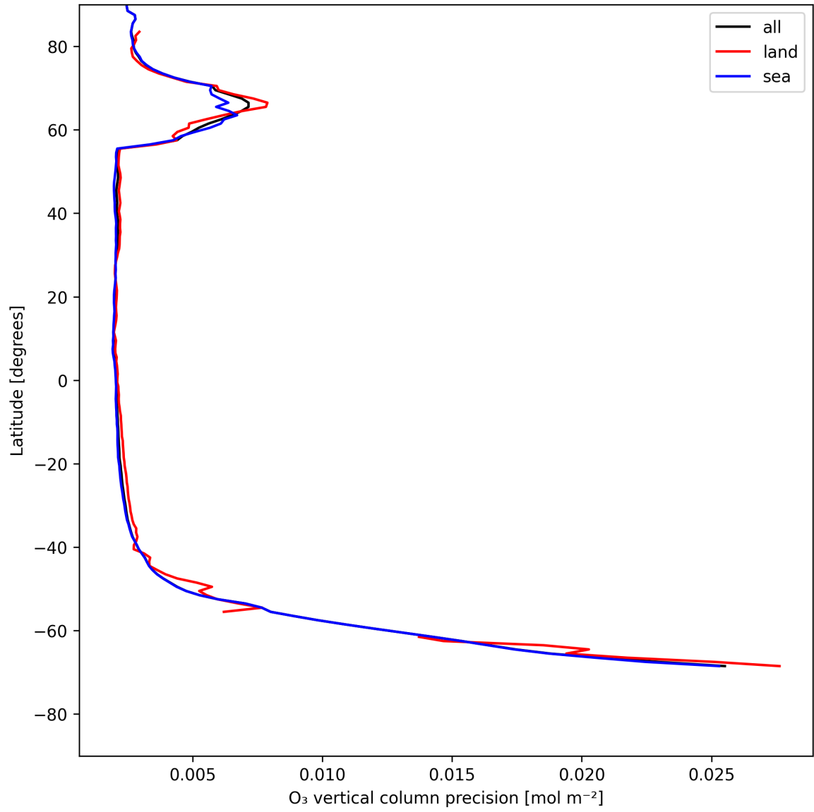
Figure 18: Zonal average of "O 3 vertical column precision" for 2025-07-20 to 2025-07-21.
