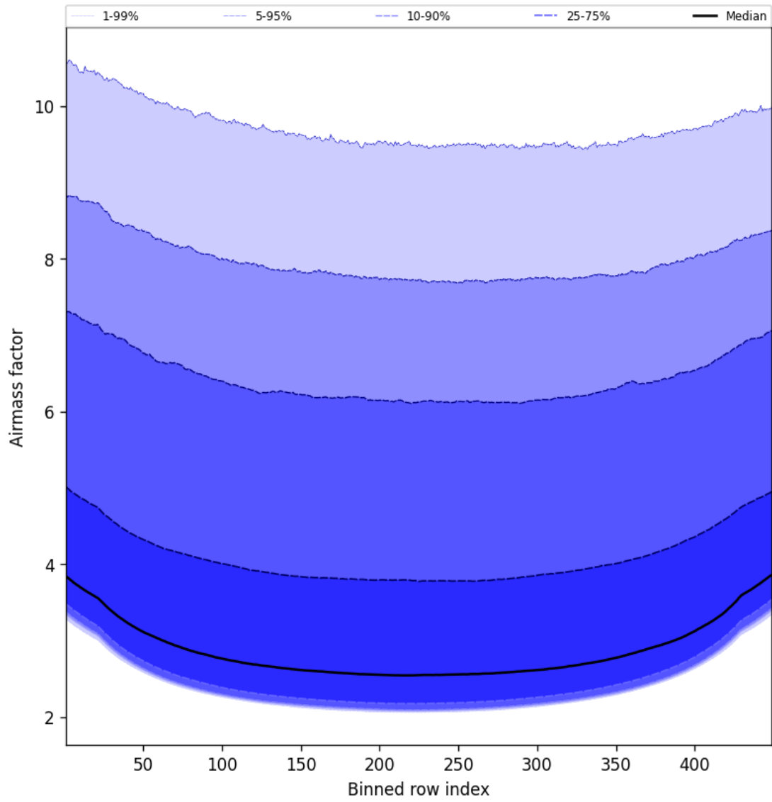
Figure 49: Along track statistics of “Airmass factor” for 2025-07-20 to 2025-07-21
