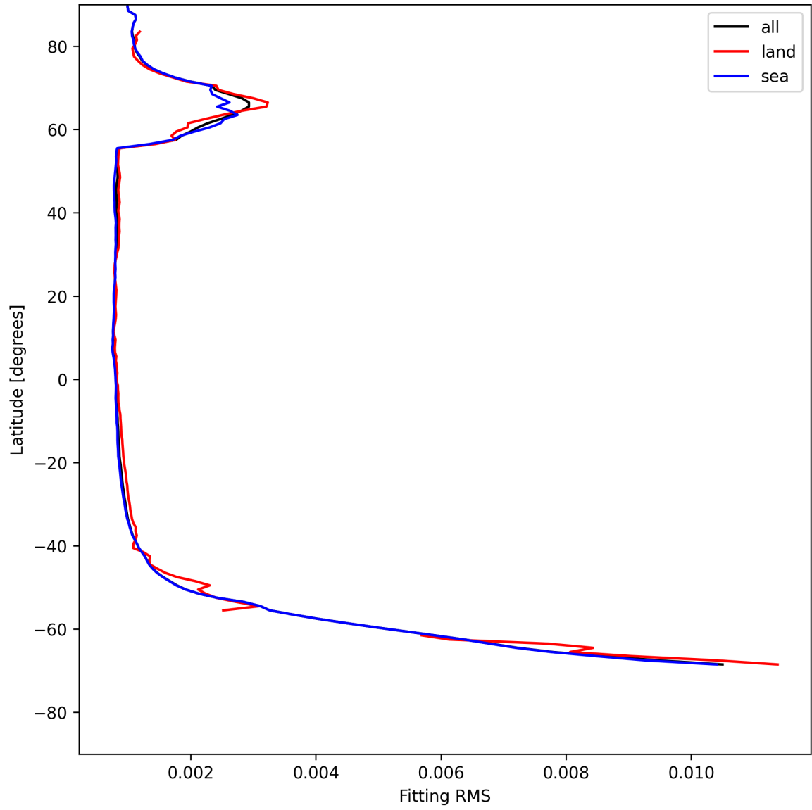
Figure 22: Zonal average of “Fitting RMS” for 2025-07-20 to 2025-07-21.
