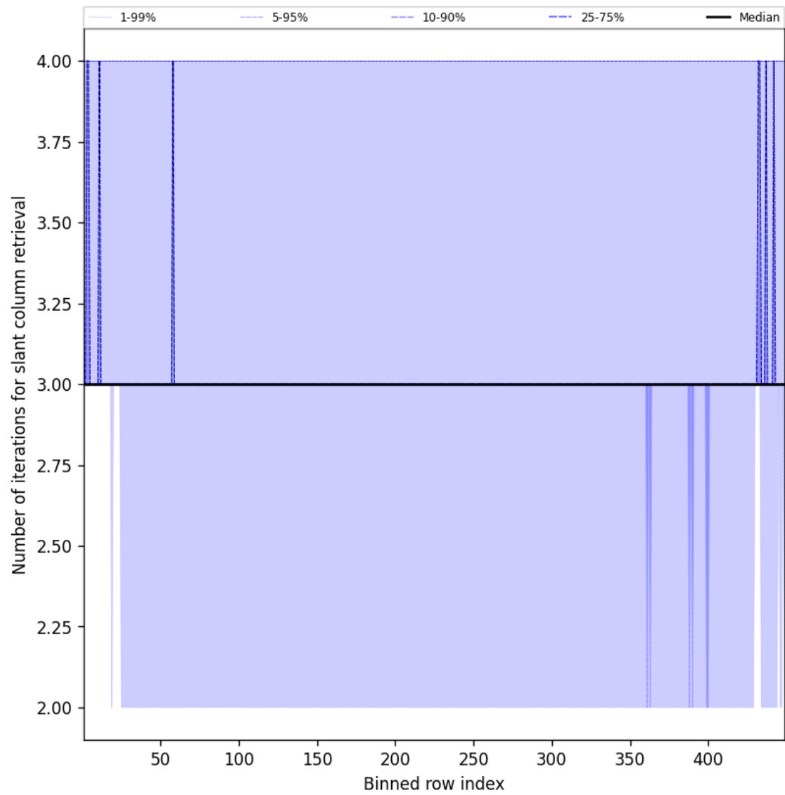
Figure 45: Along track statistics of “Number of iterations for slant column retrieval” for 2025-07-20 to 2025-07-21
