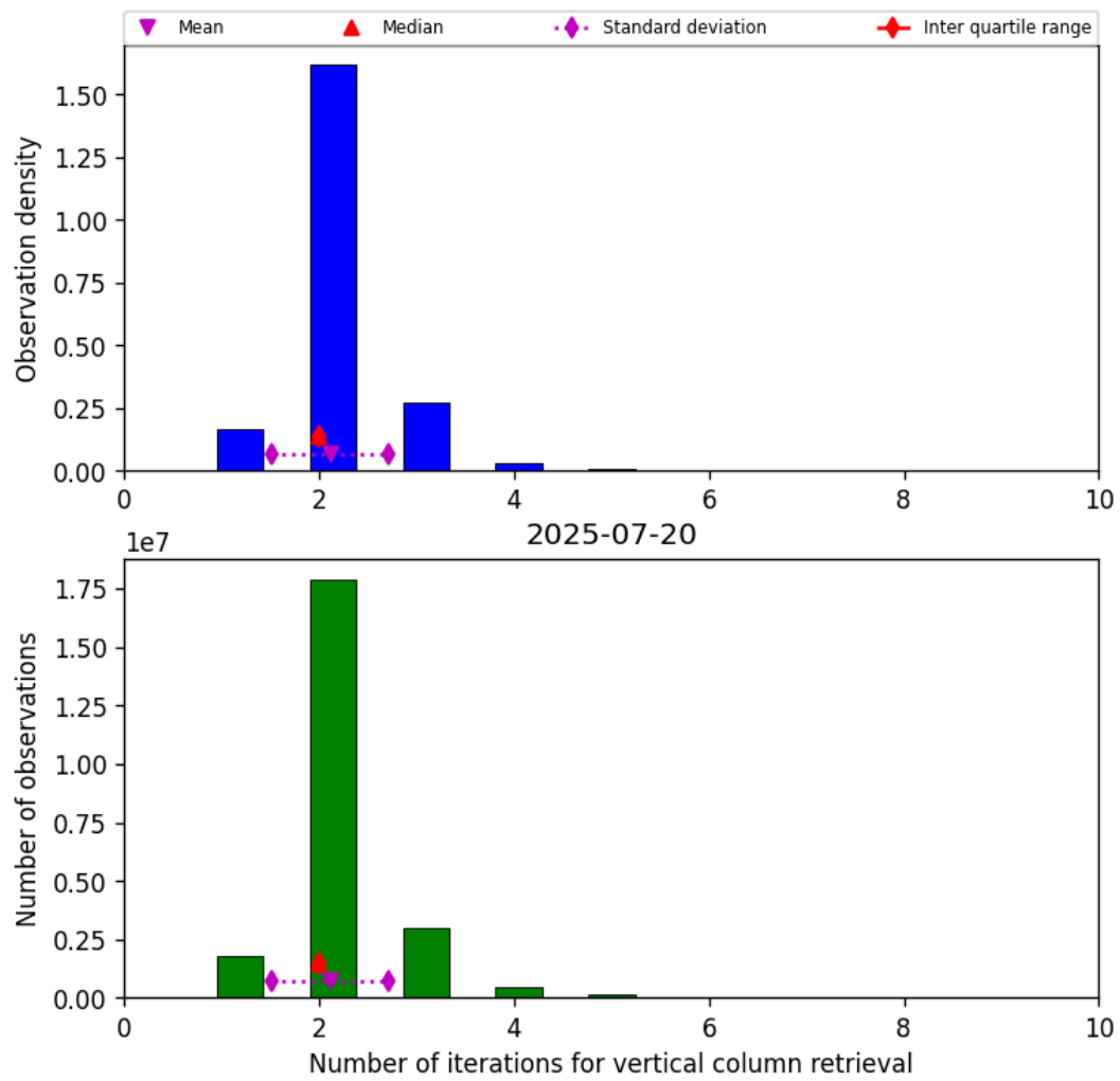
Figure 39: Histogram of “Number of iterations for vertical column retrieval” for 2025-07-20 to 2025-07-21
