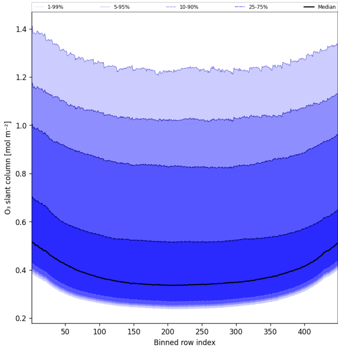
Figure 43: Along track statistics of “O 3 slant column” for 2025-07-20 to 2025-07-21
