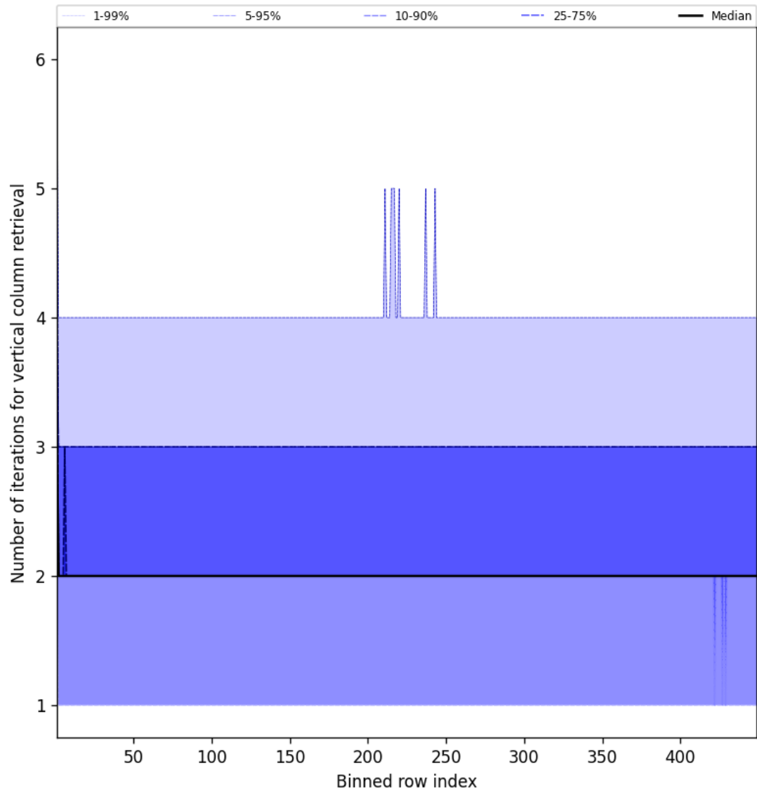
Figure 51: Along track statistics of “Number of iterations for vertical column retrieval” for 2025-07-20 to 2025-07-21
