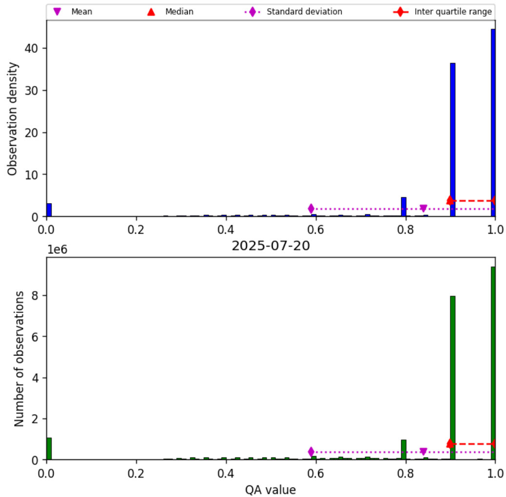
Figure 28: Histogram of “QA value” for 2025-07-20 to 2025-07-21
