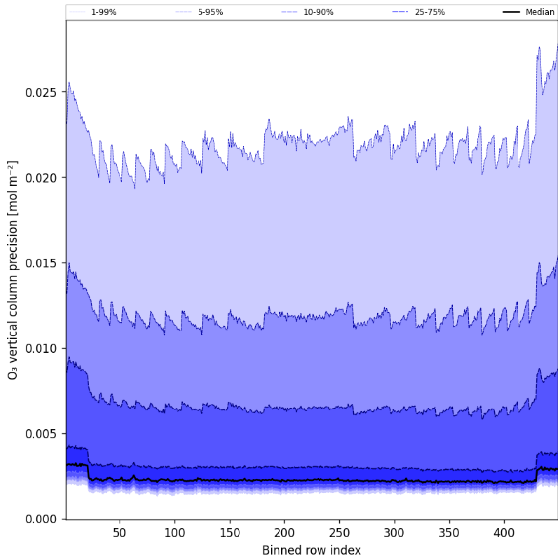
Figure 42: Along track statistics of “O 3 vertical column precision” for 2025-07-20 to 2025-07-21
