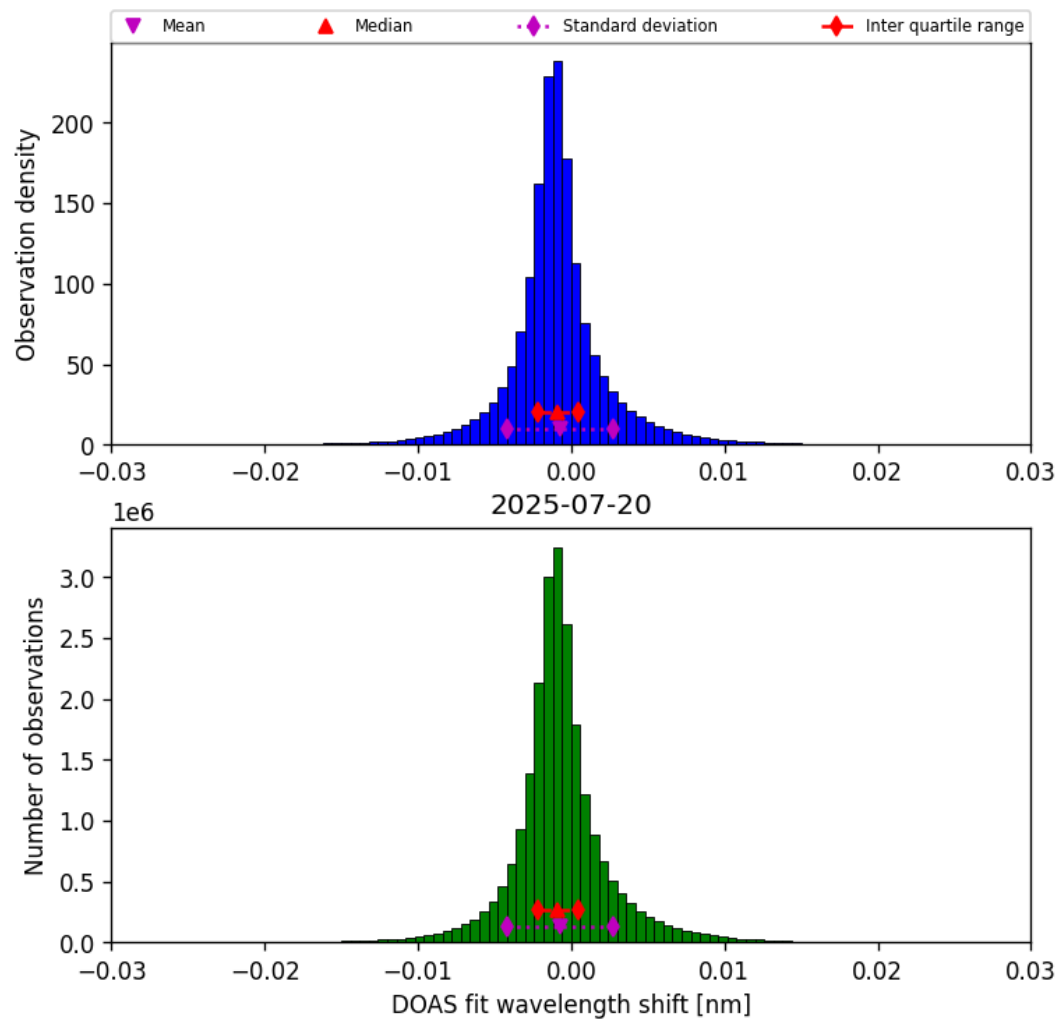
Figure 35: Histogram of “DOAS fit wavelength shift” for 2025-07-20 to 2025-07-21
