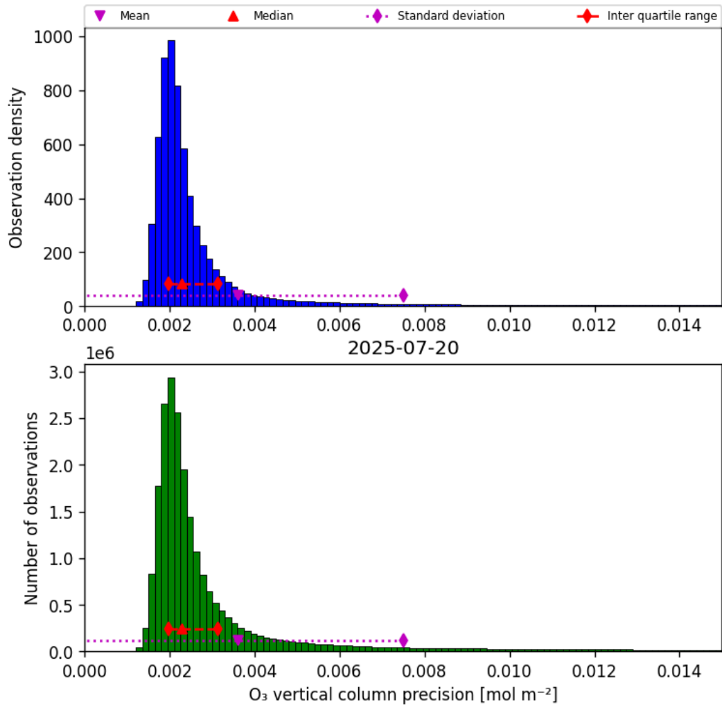
Figure 30: Histogram of “O 3 vertical column precision” for 2025-07-20 to 2025-07-21
