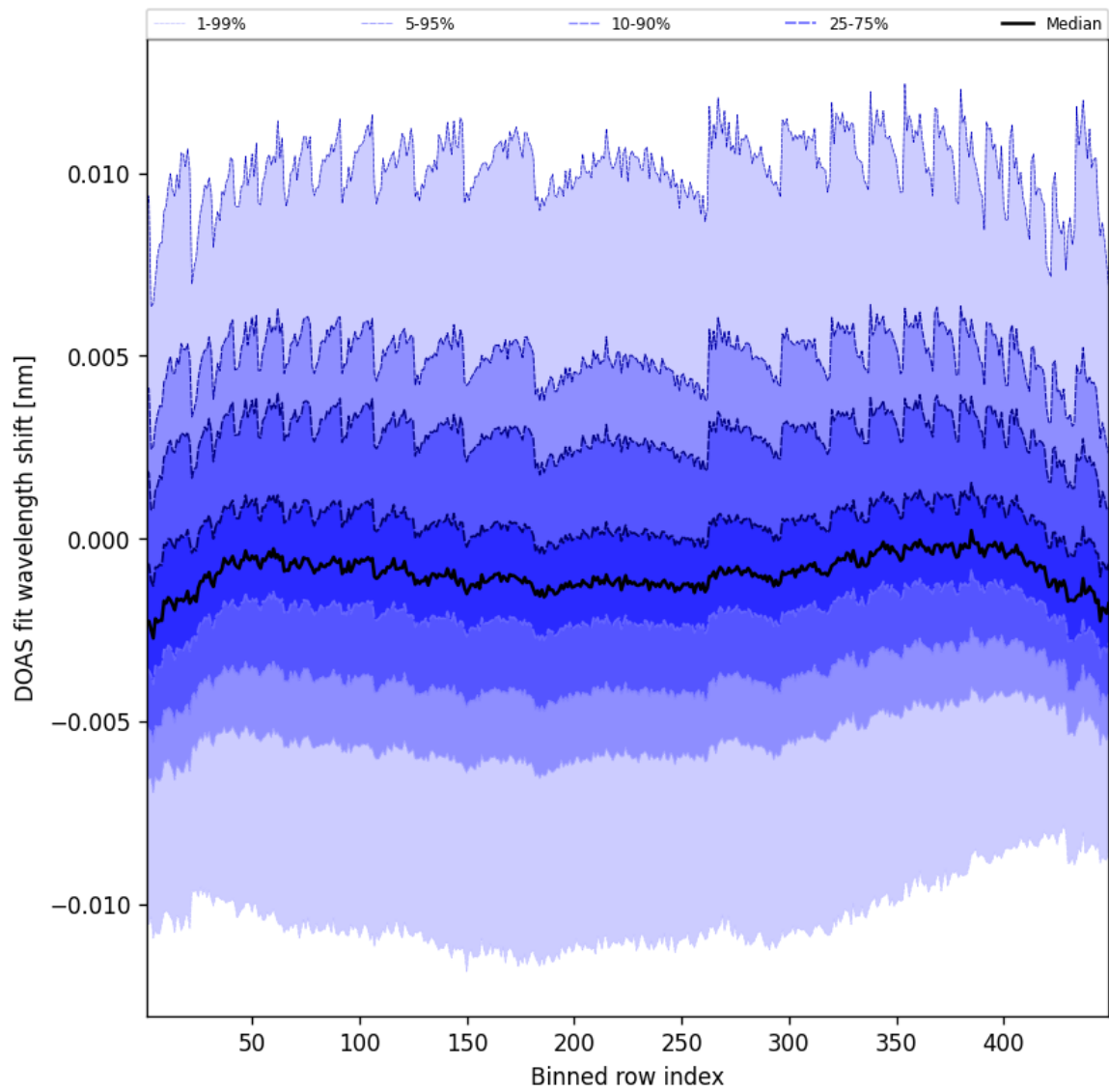
Figure 47: Along track statistics of “DOAS fit wavelength shift” for 2025-07-20 to 2025-07-21
