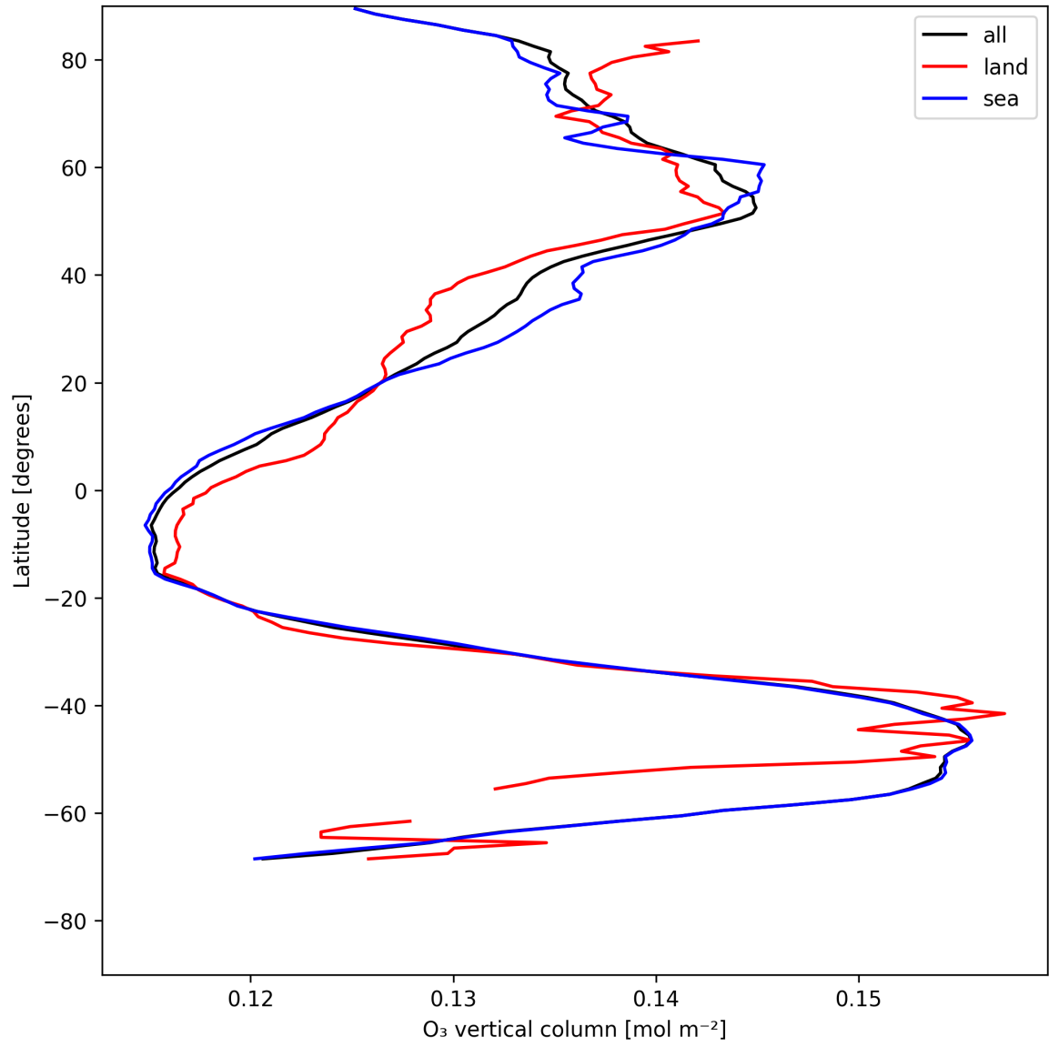
Figure 17: Zonal average of “O 3 vertical column” for 2025-07-20 to 2025-07-21.
