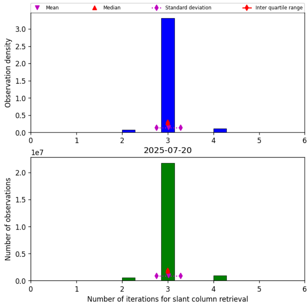
Figure 33: Histogram of “Number of iterations for slant column retrieval” for 2025-07-20 to 2025-07-21
