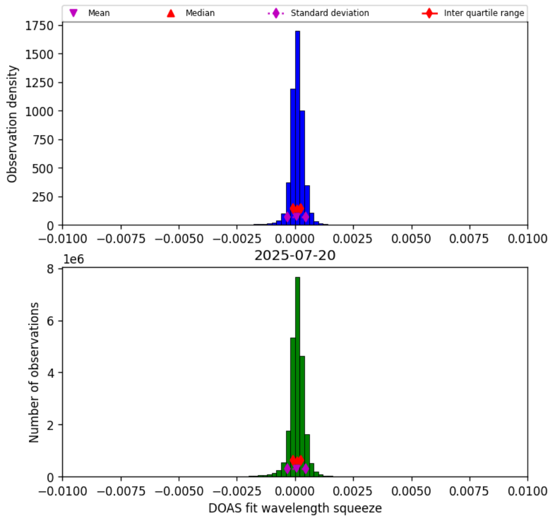
Figure 36: Histogram of “DOAS fit wavelength squeeze” for 2025-07-20 to 2025-07-21
