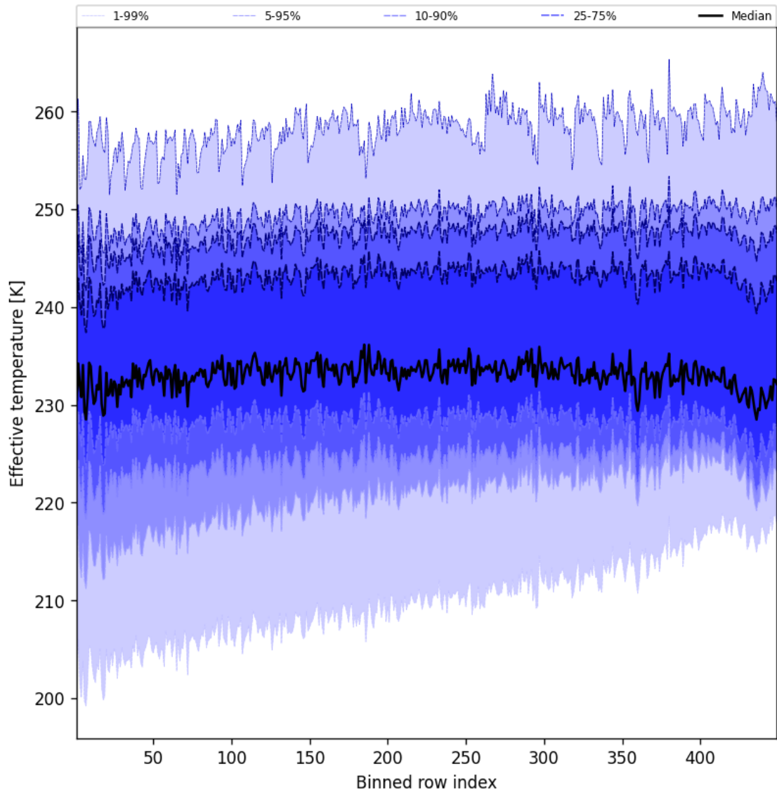
Figure 50: Along track statistics of “Effective temperature” for 2025-07-20 to 2025-07-21
