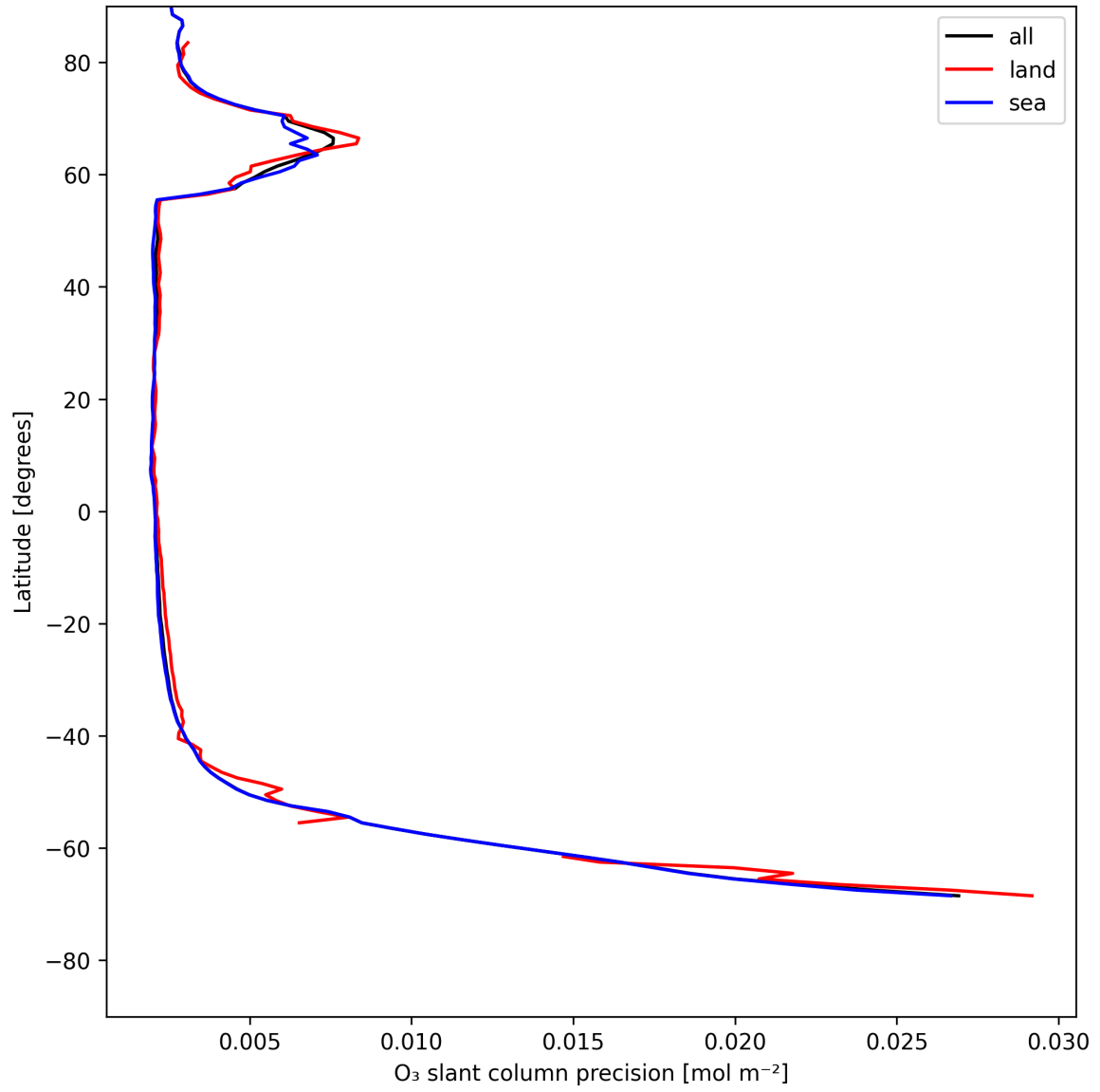
Figure 20: Zonal average of “O 3 slant column precision” for 2025-07-20 to 2025-07-21.
