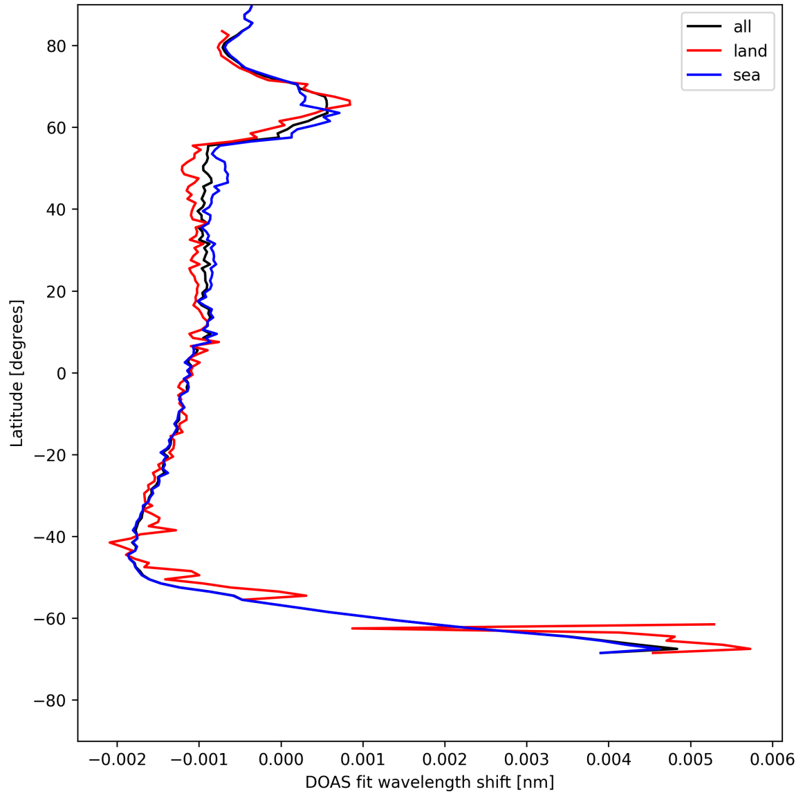
Figure 23: Zonal average of “DOAS fit wavelength shift” for 2025-07-20 to 2025-07-21.
