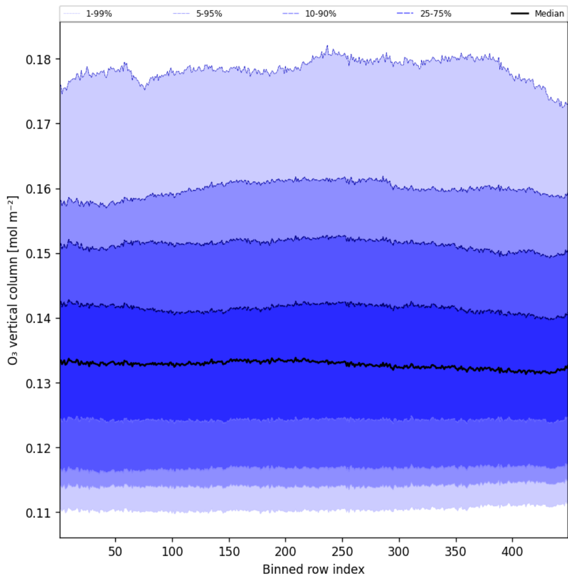
Figure 41: Along track statistics of “O 3 vertical column” for 2025-07-20 to 2025-07-21
