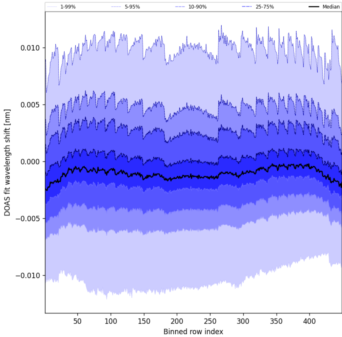
Figure 47: Along track statistics of “DOAS fit wavelength shift” for 2025-07-21 to 2025-07-22
