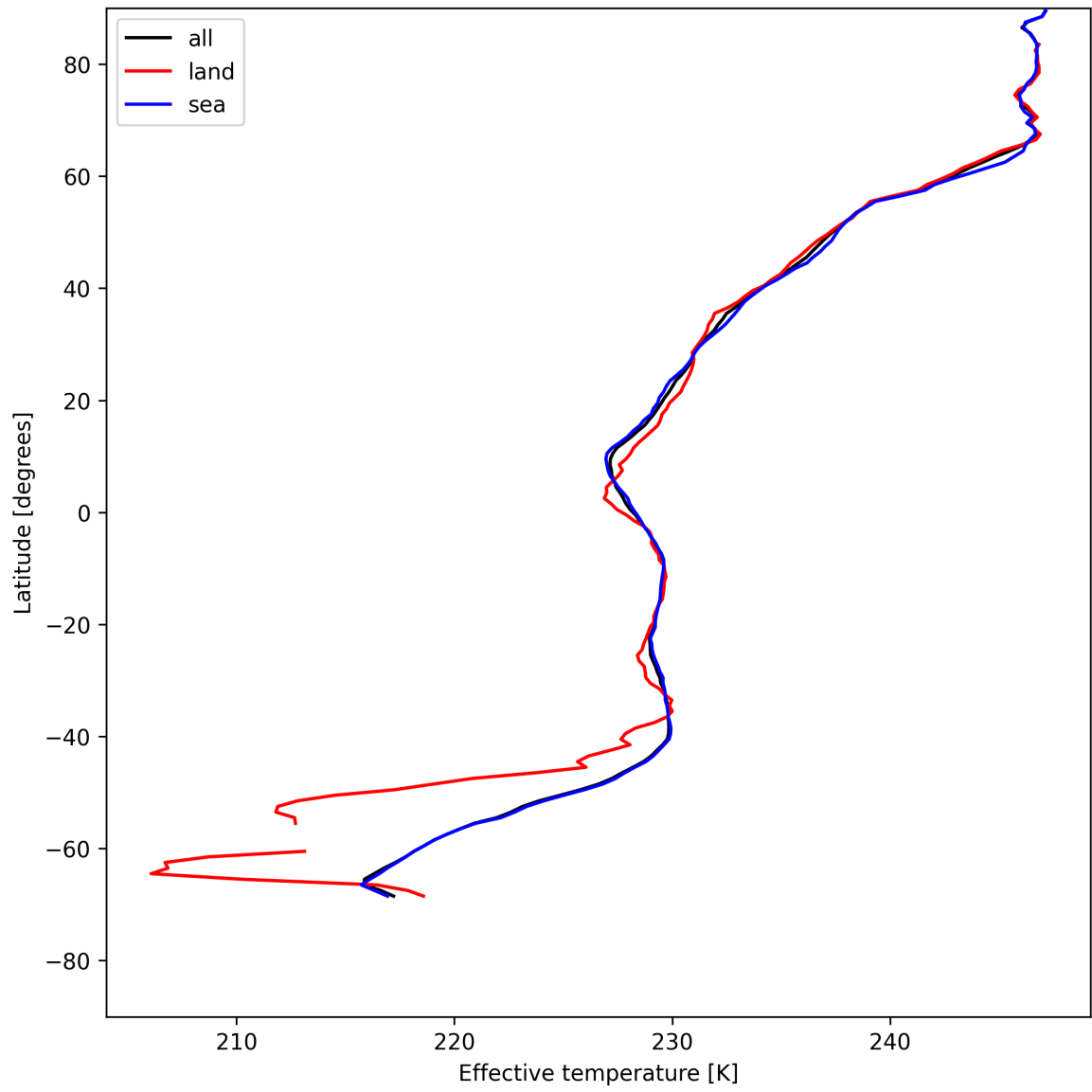
Figure 26: Zonal average of “Effective temperature” for 2025-07-21 to 2025-07-22.
