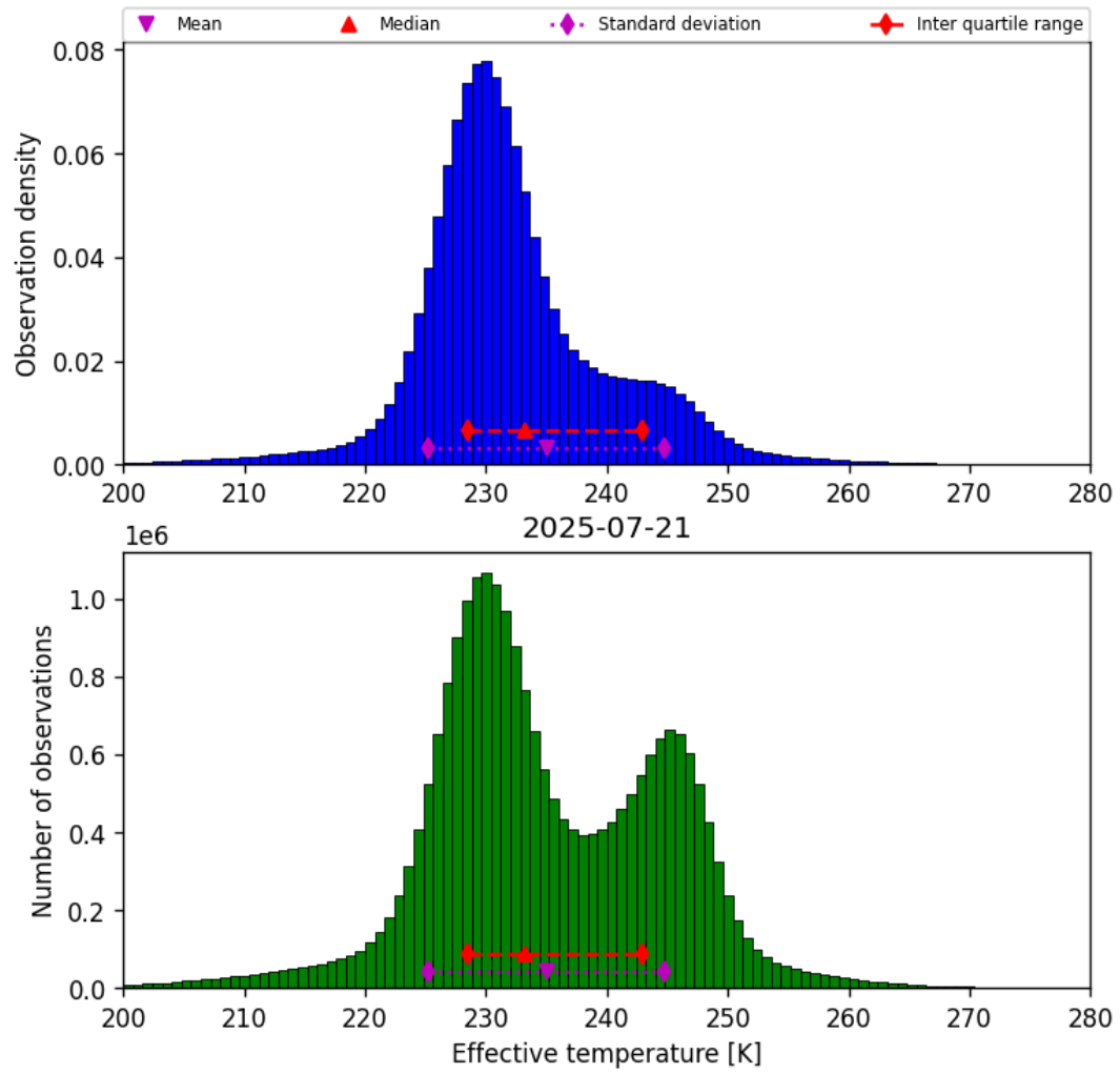
Figure 38: Histogram of “Effective temperature” for 2025-07-21 to 2025-07-22
