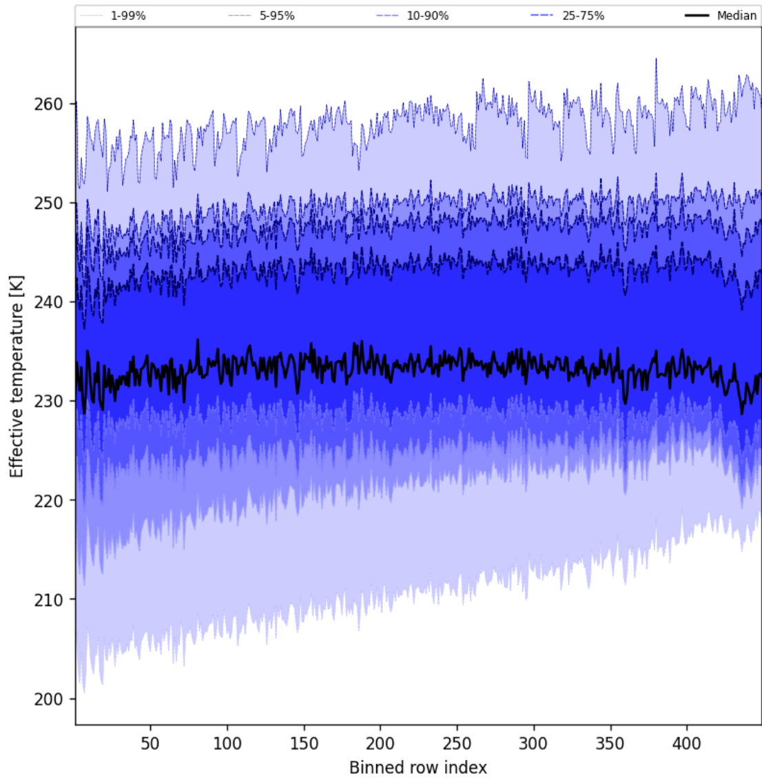
Figure 50: Along track statistics of “Effective temperature” for 2025-07-21 to 2025-07-22
