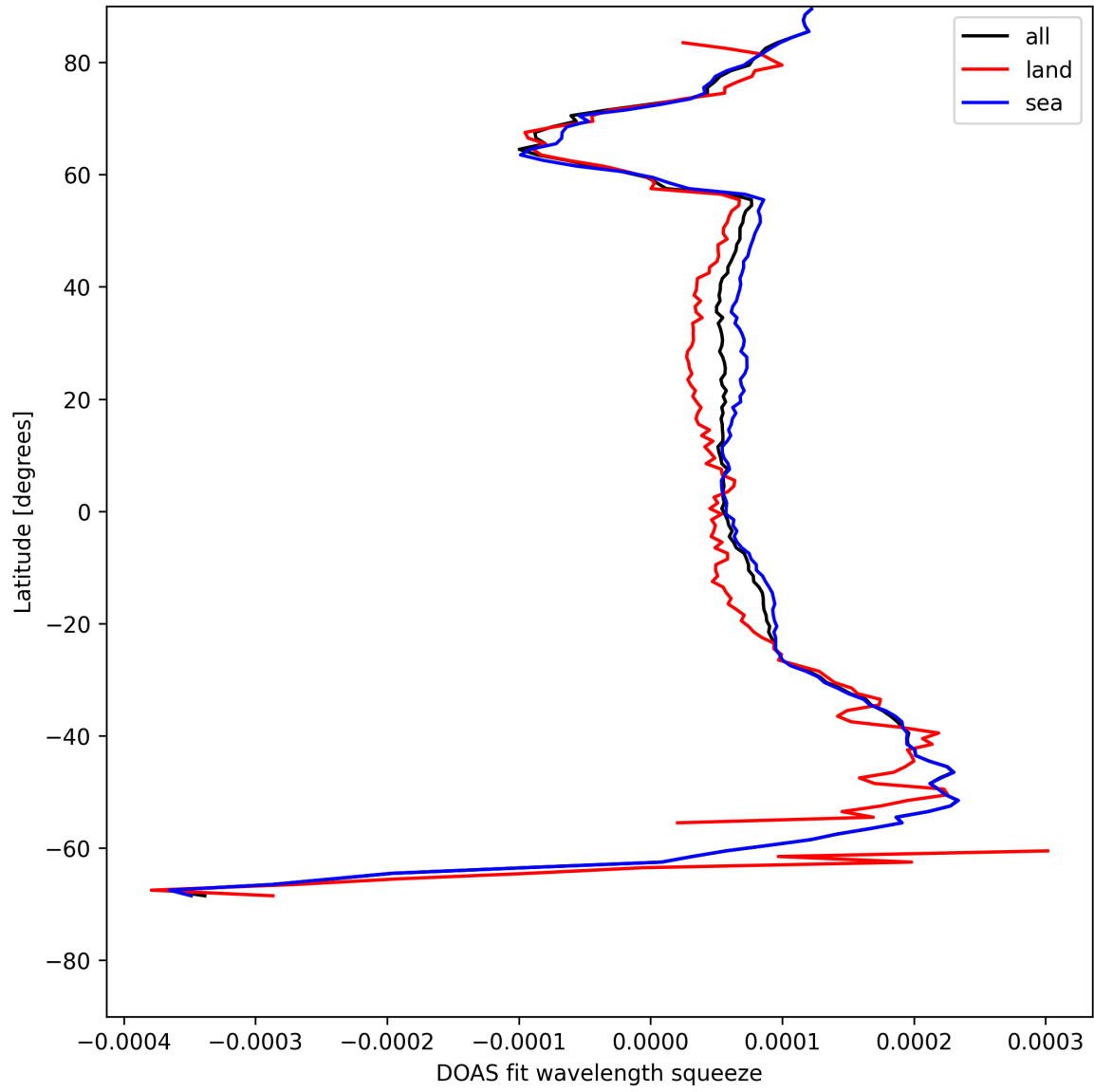
Figure 24: Zonal average of “DOAS fit wavelength squeeze” for 2025-07-21 to 2025-07-22.
