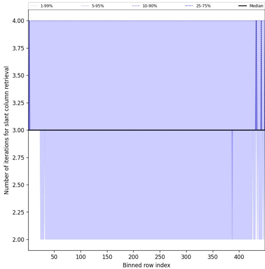
Figure 45: Along track statistics of “Number of iterations for slant column retrieval” for 2025-07-21 to 2025-07-22
