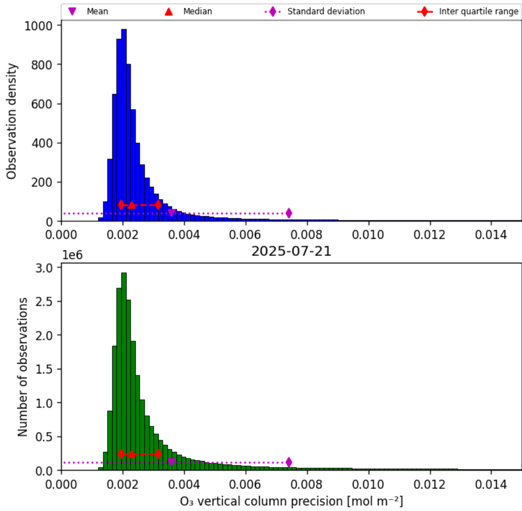
Figure 30: Histogram of “O 3 vertical column precision” for 2025-07-21 to 2025-07-22
