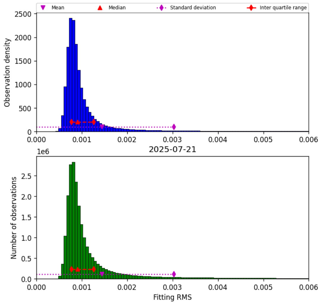
Figure 34: Histogram of “Fitting RMS” for 2025-07-21 to 2025-07-22
