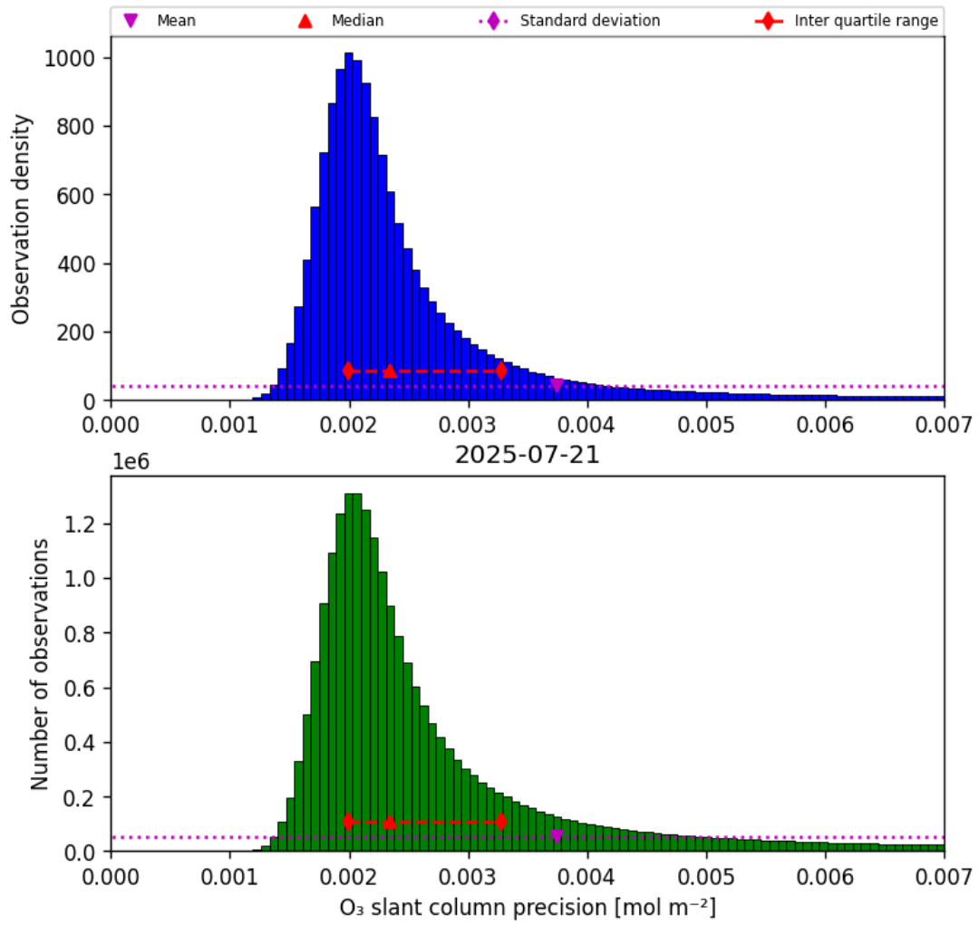
Figure 32: Histogram of “O 3 slant column precision” for 2025-07-21 to 2025-07-22
