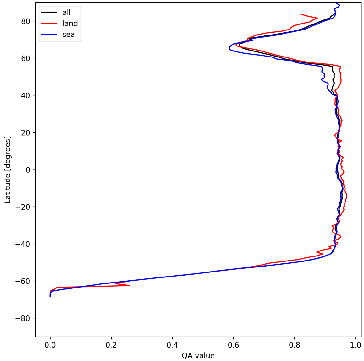
Figure 16: Zonal average of “QA value” for 2025-07-21 to 2025-07-22.
