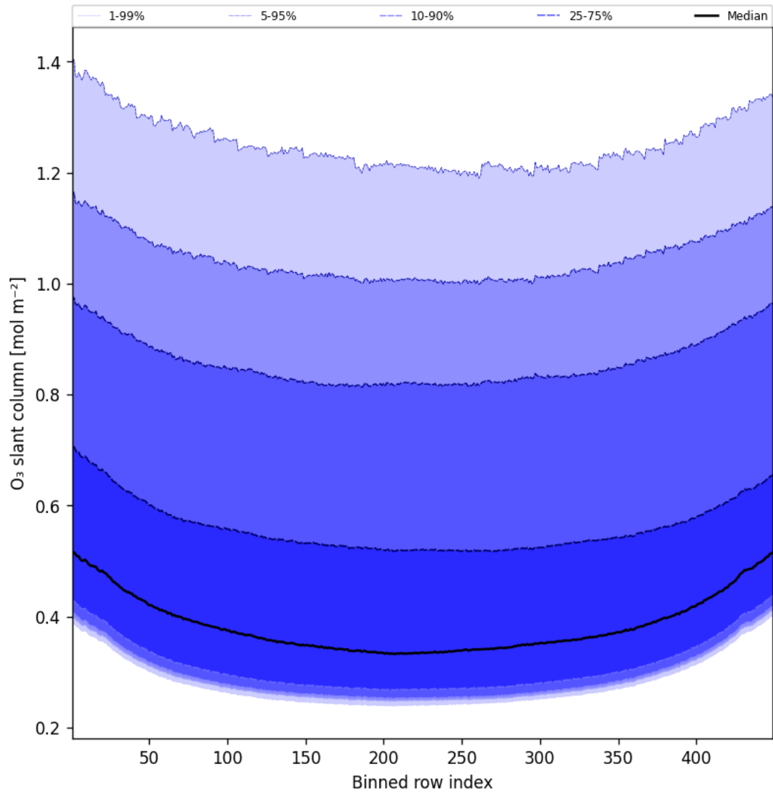
Figure 43: Along track statistics of “O 3 slant column” for 2025-07-21 to 2025-07-22
