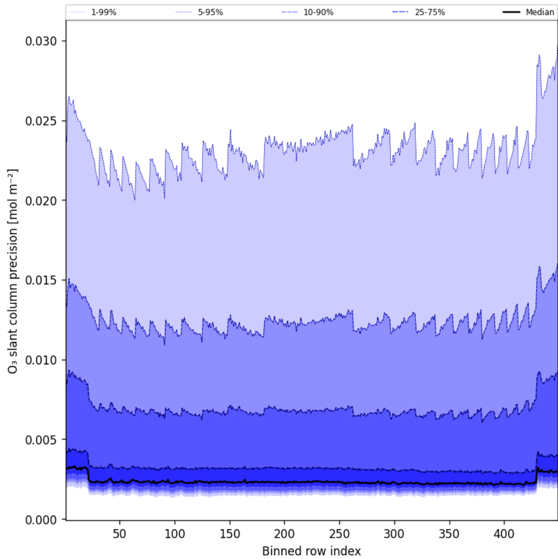
Figure 44: Along track statistics of “O 3 slant column precision” for 2025-07-21 to 2025-07-22
