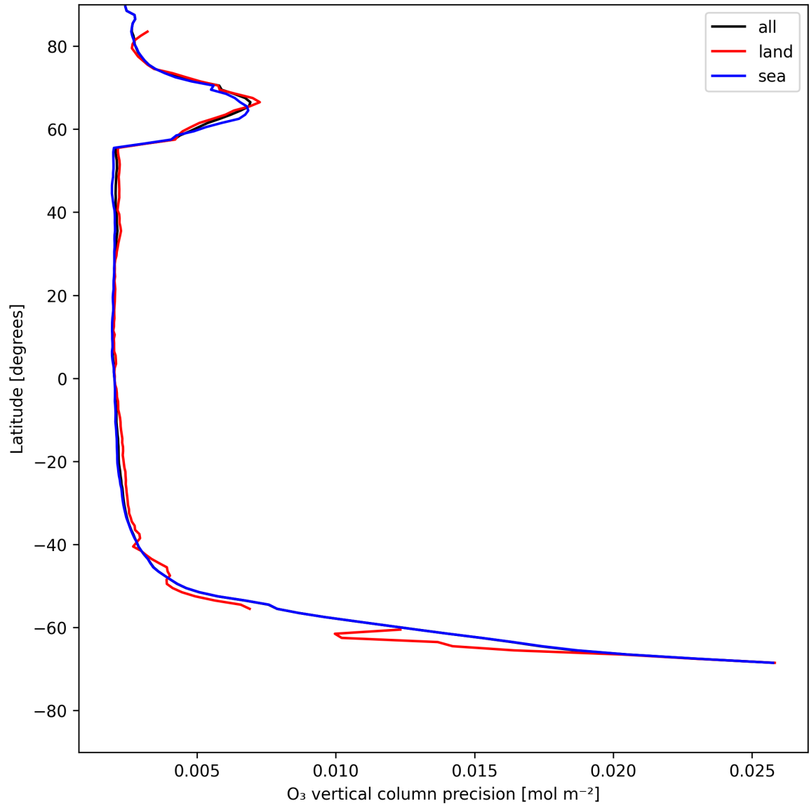
Figure 18: Zonal average of “O 3 vertical column precision” for 2025-07-21 to 2025-07-22.
