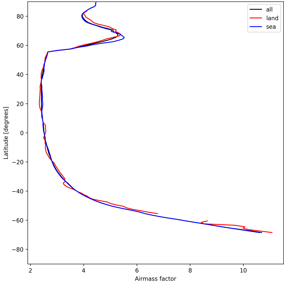
Figure 25: Zonal average of “Airmass factor” for 2025-07-21 to 2025-07-22.
