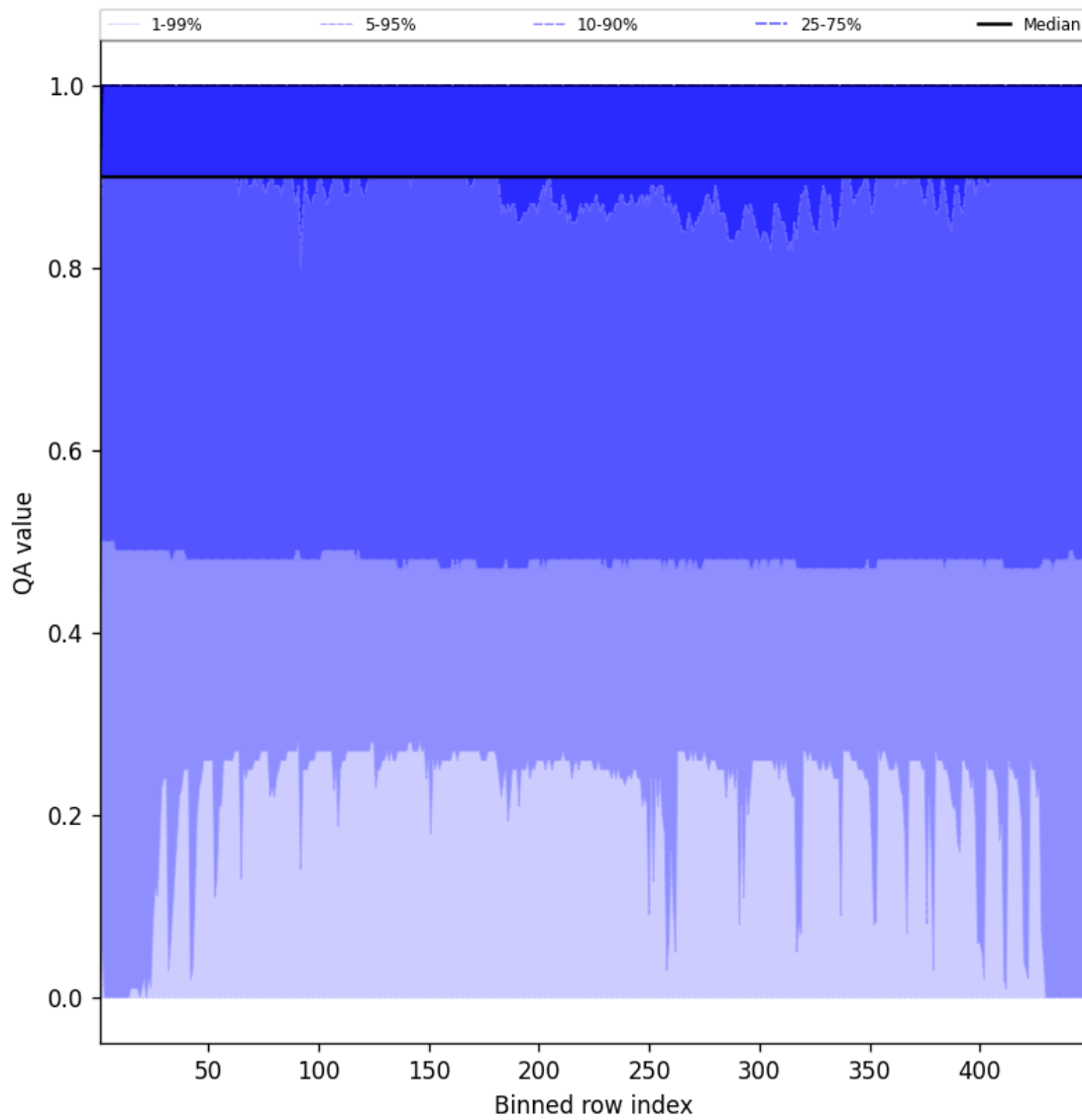
Figure 40: Along track statistics of “QA value” for 2025-07-21 to 2025-07-22
