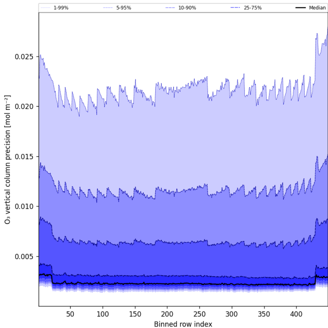
Figure 42: Along track statistics of “O 3 vertical column precision” for 2025-07-21 to 2025-07-22
