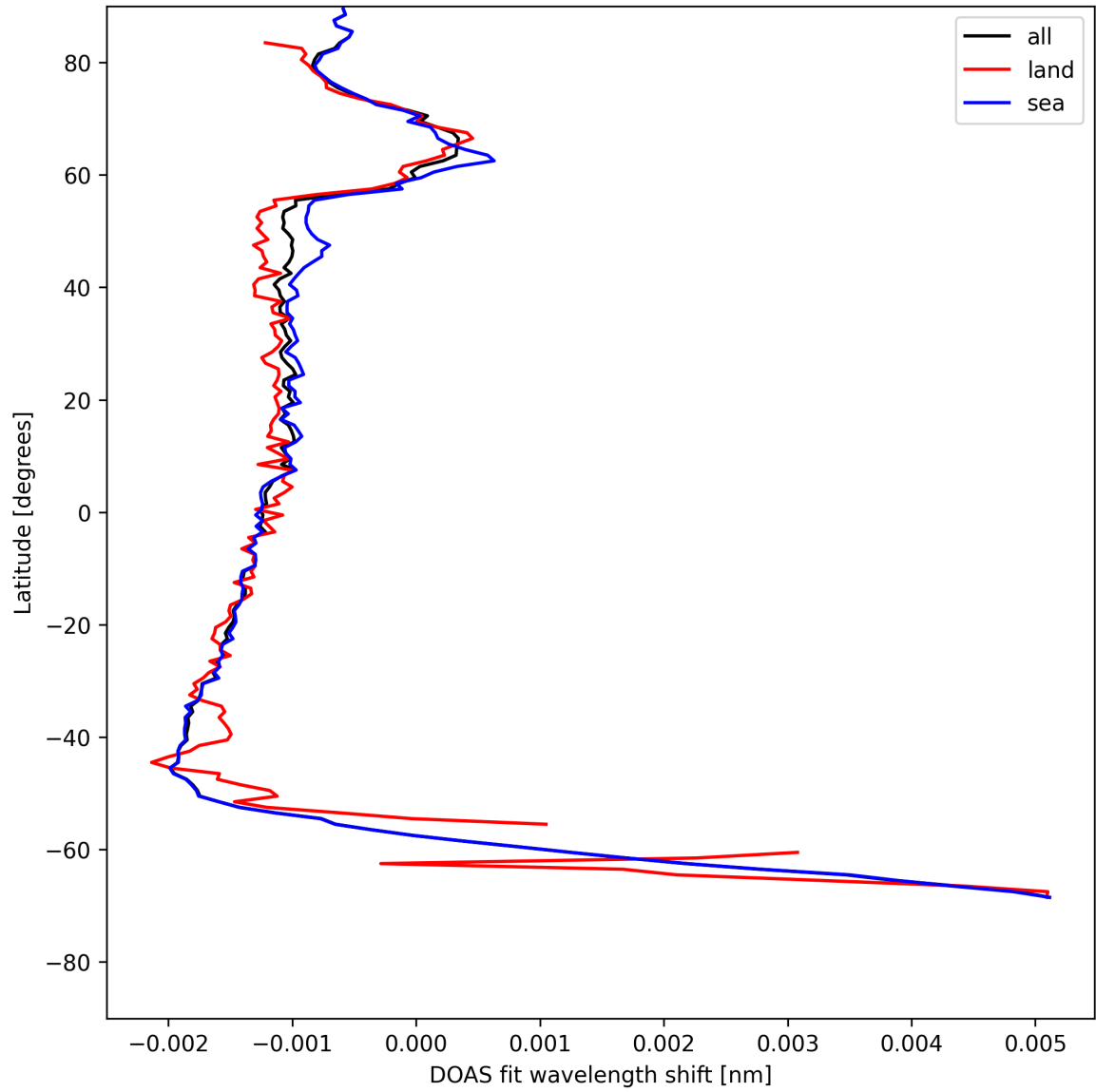
Figure 23: Zonal average of “DOAS fit wavelength shift” for 2025-07-21 to 2025-07-22.
