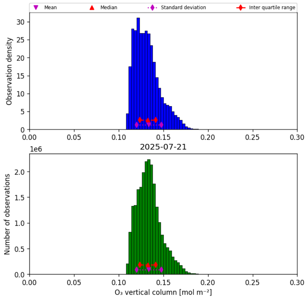
Figure 29: Histogram of “O 3 vertical column” for 2025-07-21 to 2025-07-22
