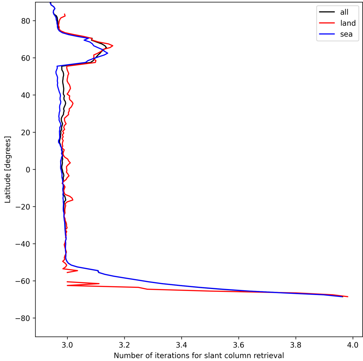
Figure 21: Zonal average of “Number of iterations for slant column retrieval” for 2025-07-21 to 2025-07-22.
