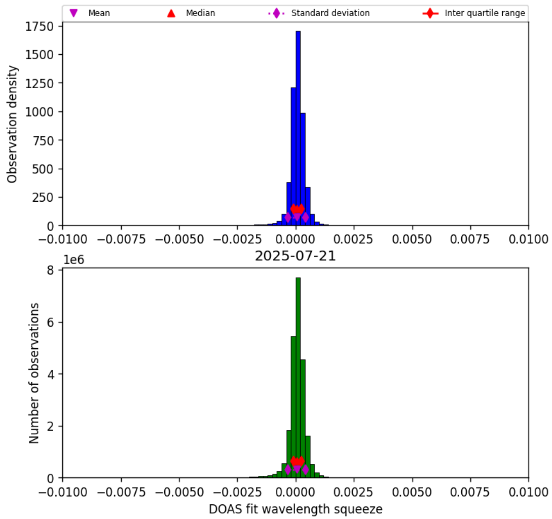
Figure 36: Histogram of “DOAS fit wavelength squeeze” for 2025-07-21 to 2025-07-22
