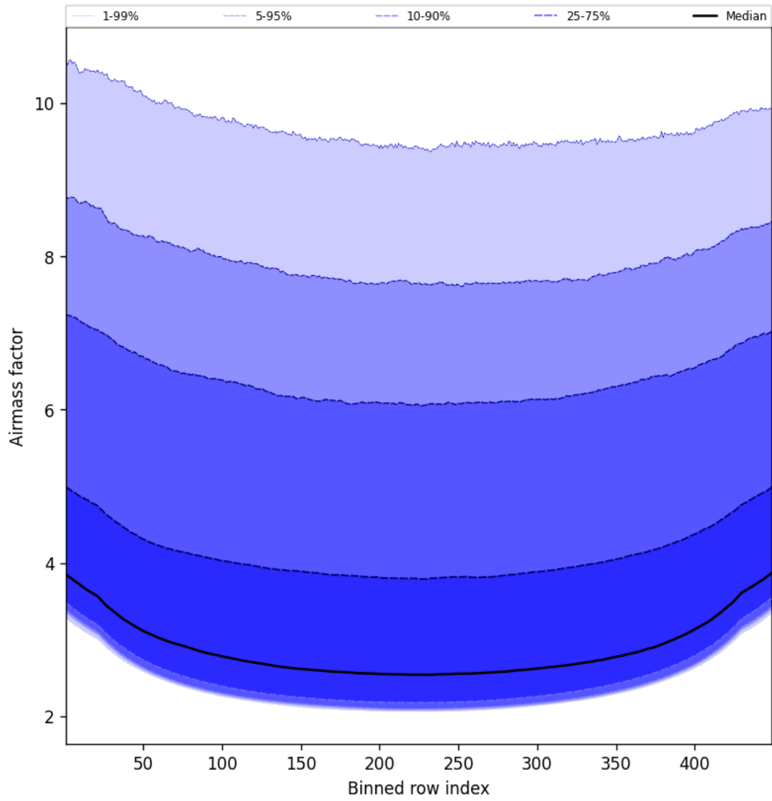
Figure 49: Along track statistics of “Airmass factor” for 2025-07-21 to 2025-07-22
