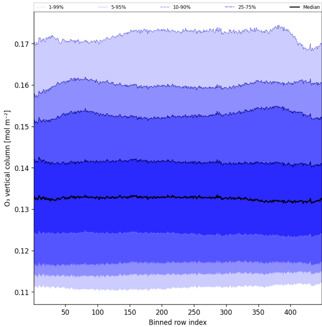
Figure 41: Along track statistics of “ O_3 vertical column” for 2025-07-21 to 2025-07-22
