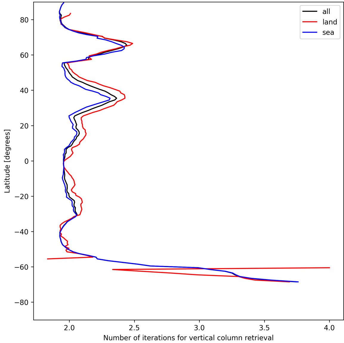
Figure 27: Zonal average of “Number of iterations for vertical column retrieval” for 2025-07-21 to 2025-07-22.
