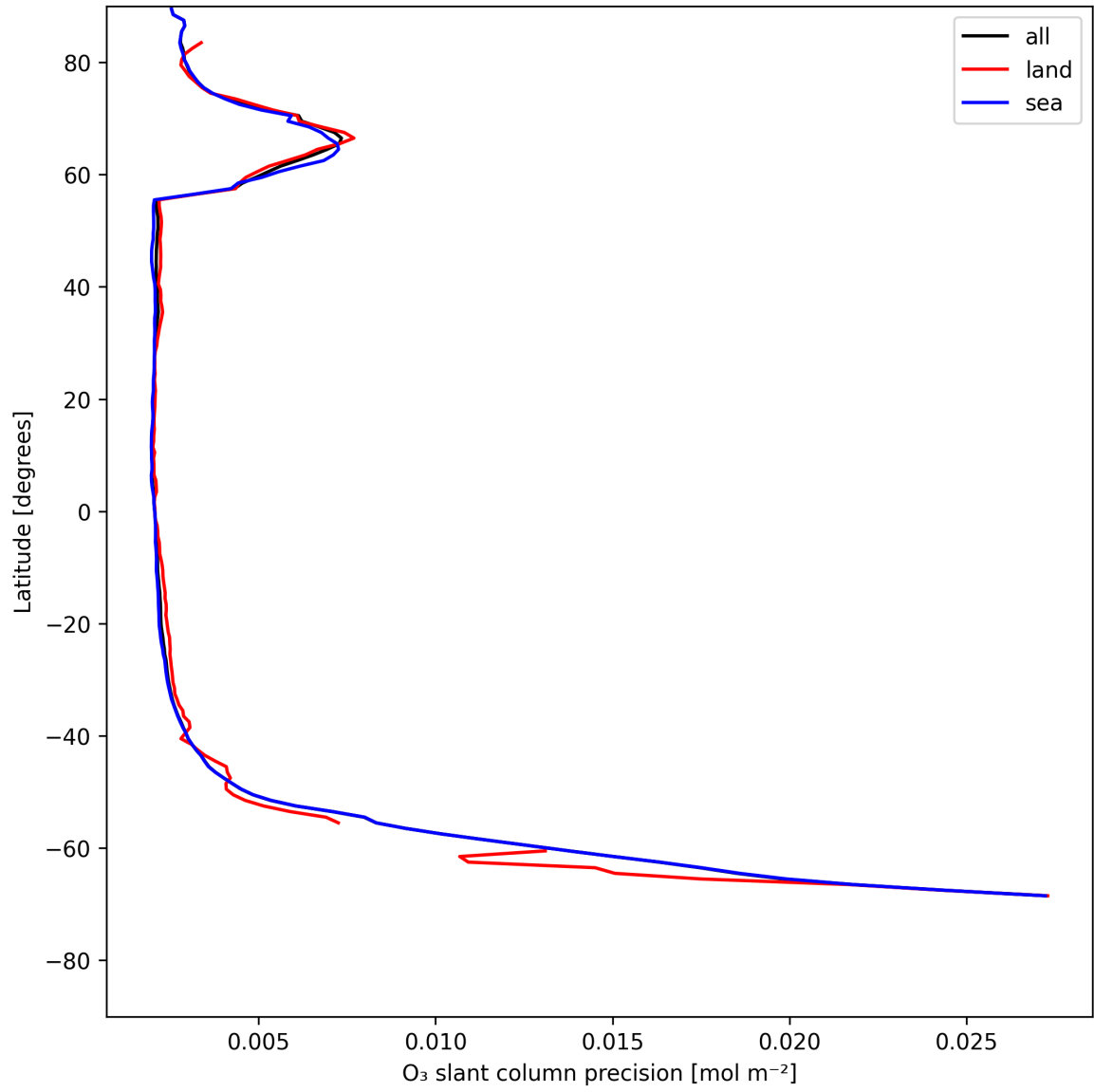
Figure 20: Zonal average of “O 3 slant column precision” for 2025-07-21 to 2025-07-22.
