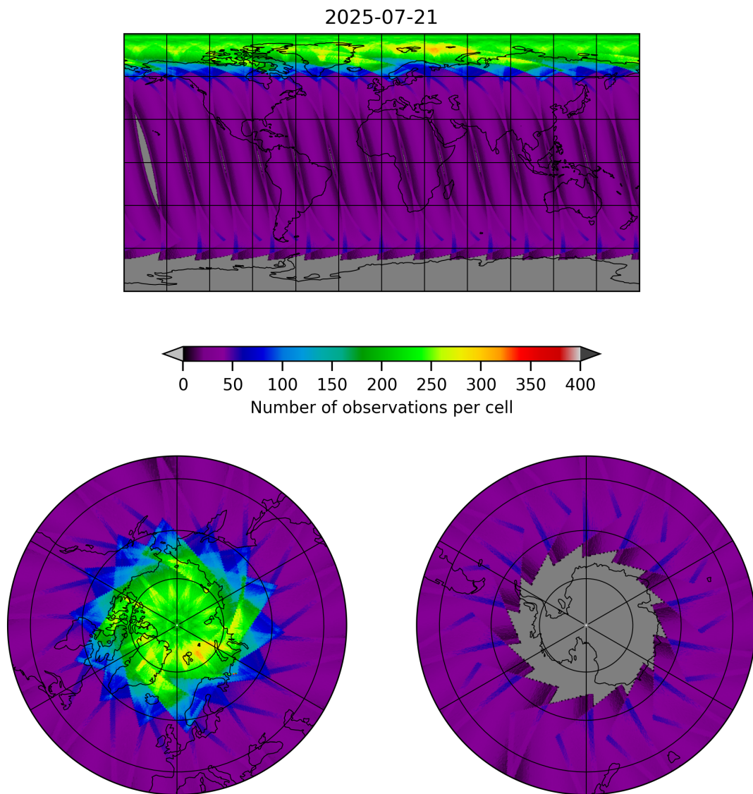
Figure 15: Map of the number of observations for 2025-07-21 to 2025-07-22
