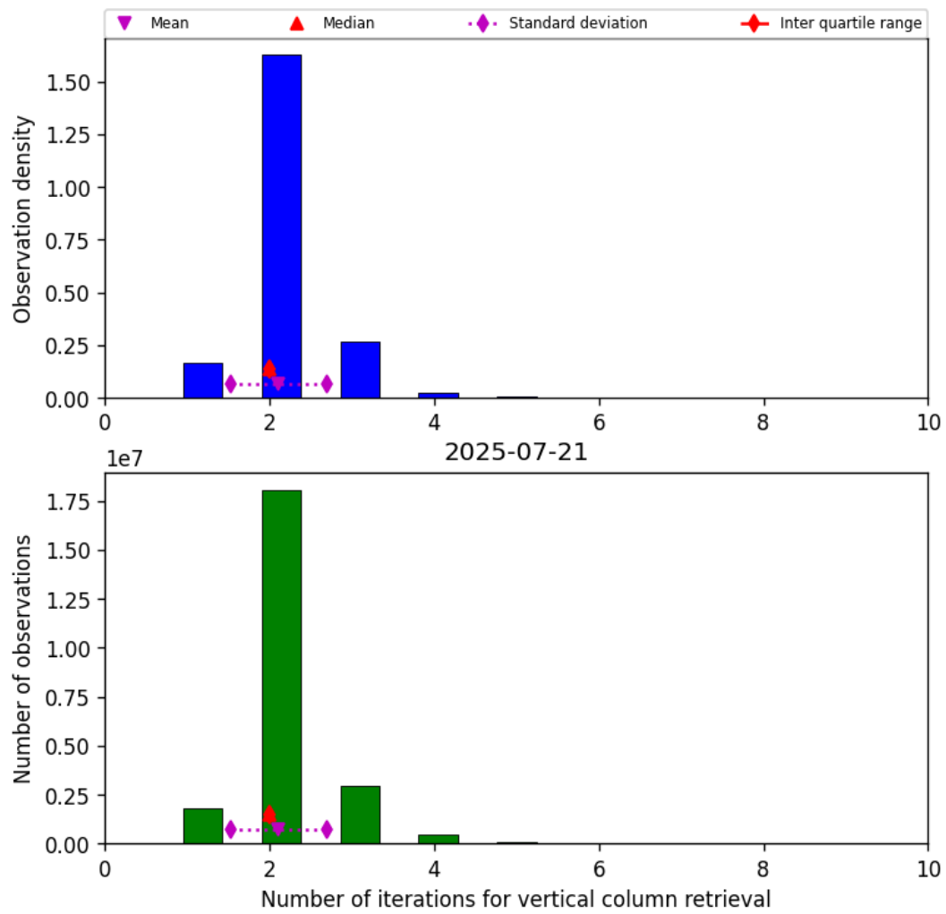
Figure 39: Histogram of “Number of iterations for vertical column retrieval” for 2025-07-21 to 2025-07-22
