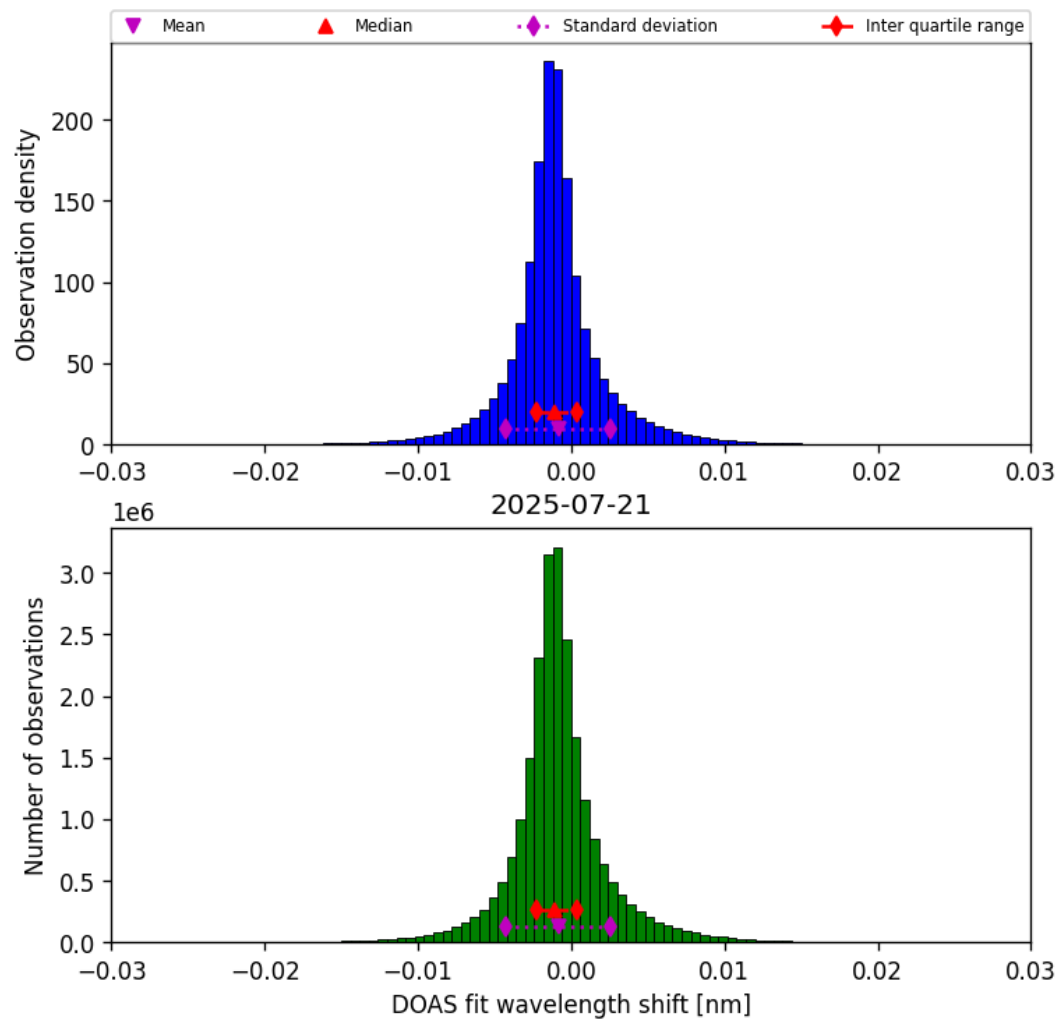
Figure 35: Histogram of “DOAS fit wavelength shift” for 2025-07-21 to 2025-07-22
