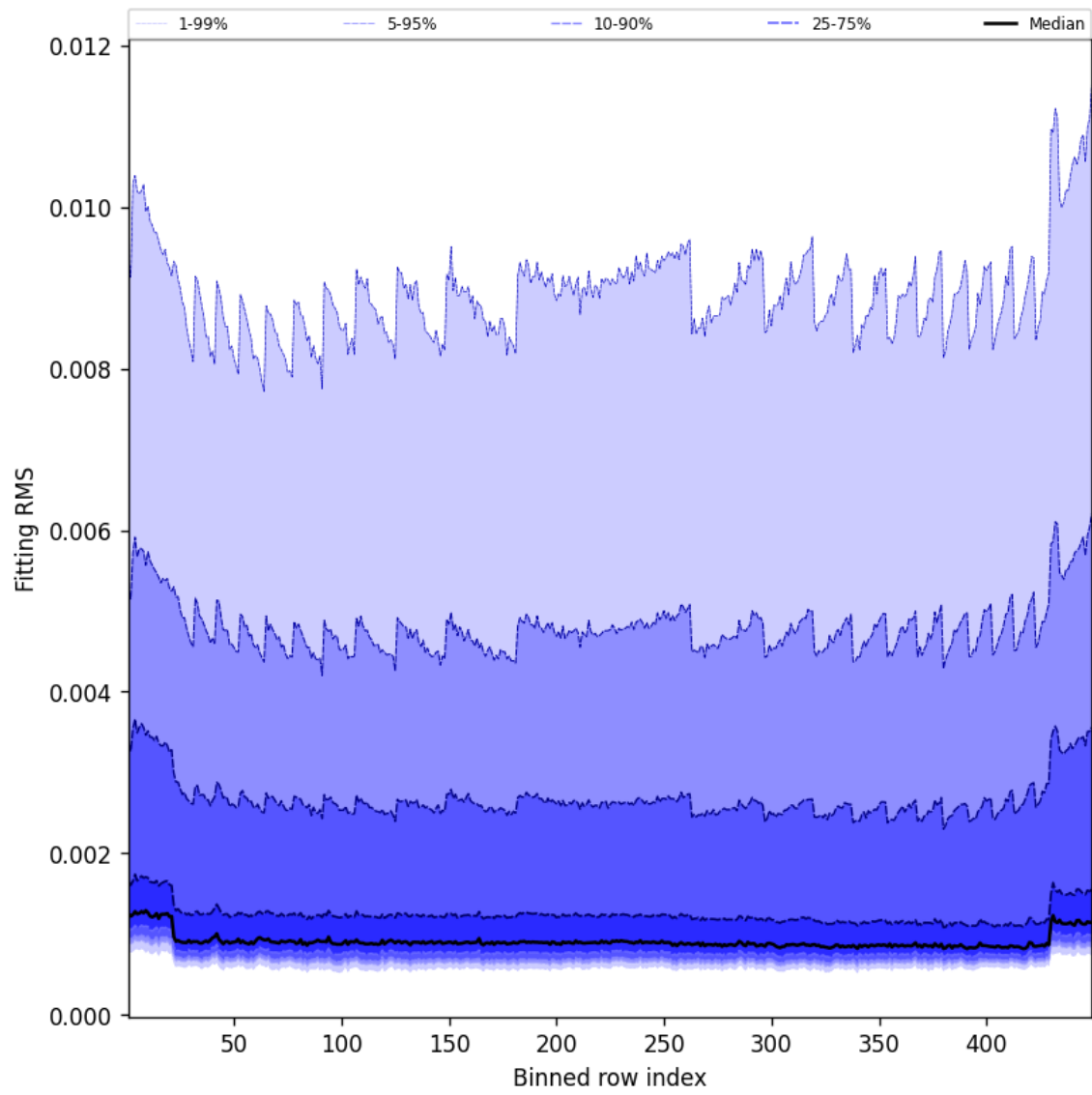
Figure 46: Along track statistics of “Fitting RMS” for 2025-07-21 to 2025-07-22
