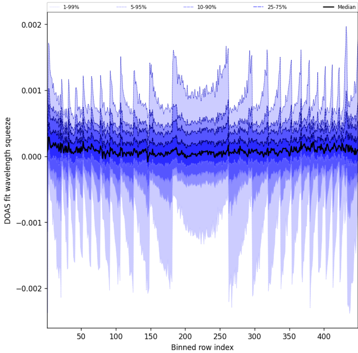
Figure 48: Along track statistics of “DOAS fit wavelength squeeze” for 2025-07-21 to 2025-07-22
