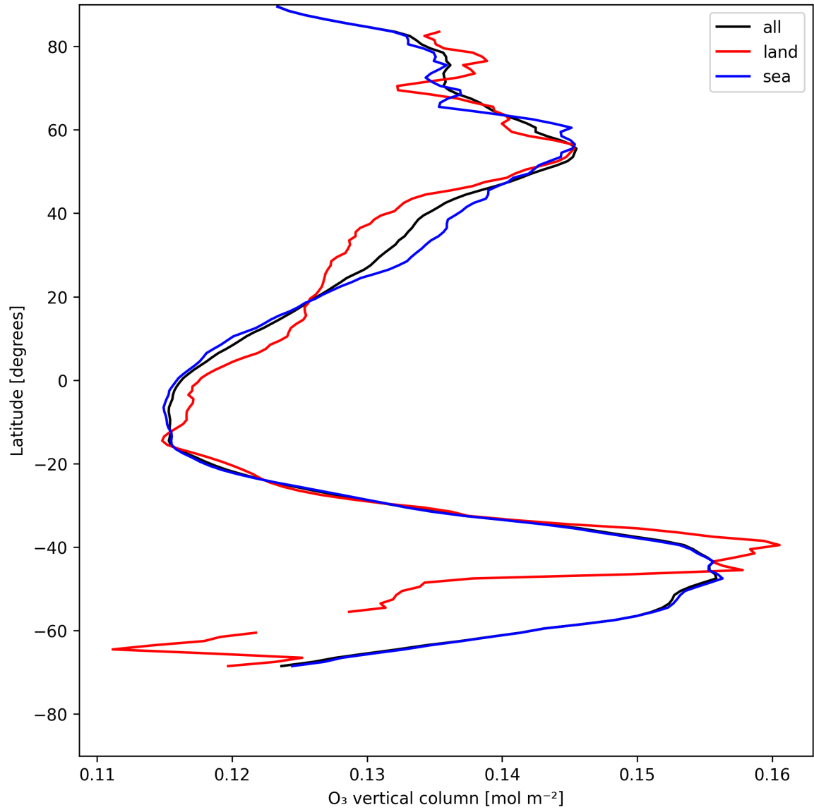
Figure 17: Zonal average of “O 3 vertical column” for 2025-07-21 to 2025-07-22.
