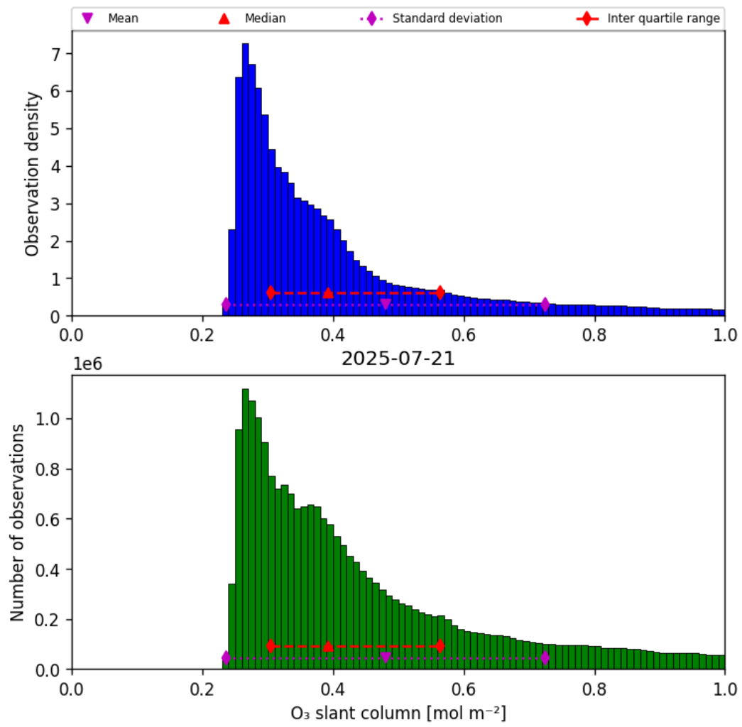
Figure 31: Histogram of “O 3 slant column” for 2025-07-21 to 2025-07-22
