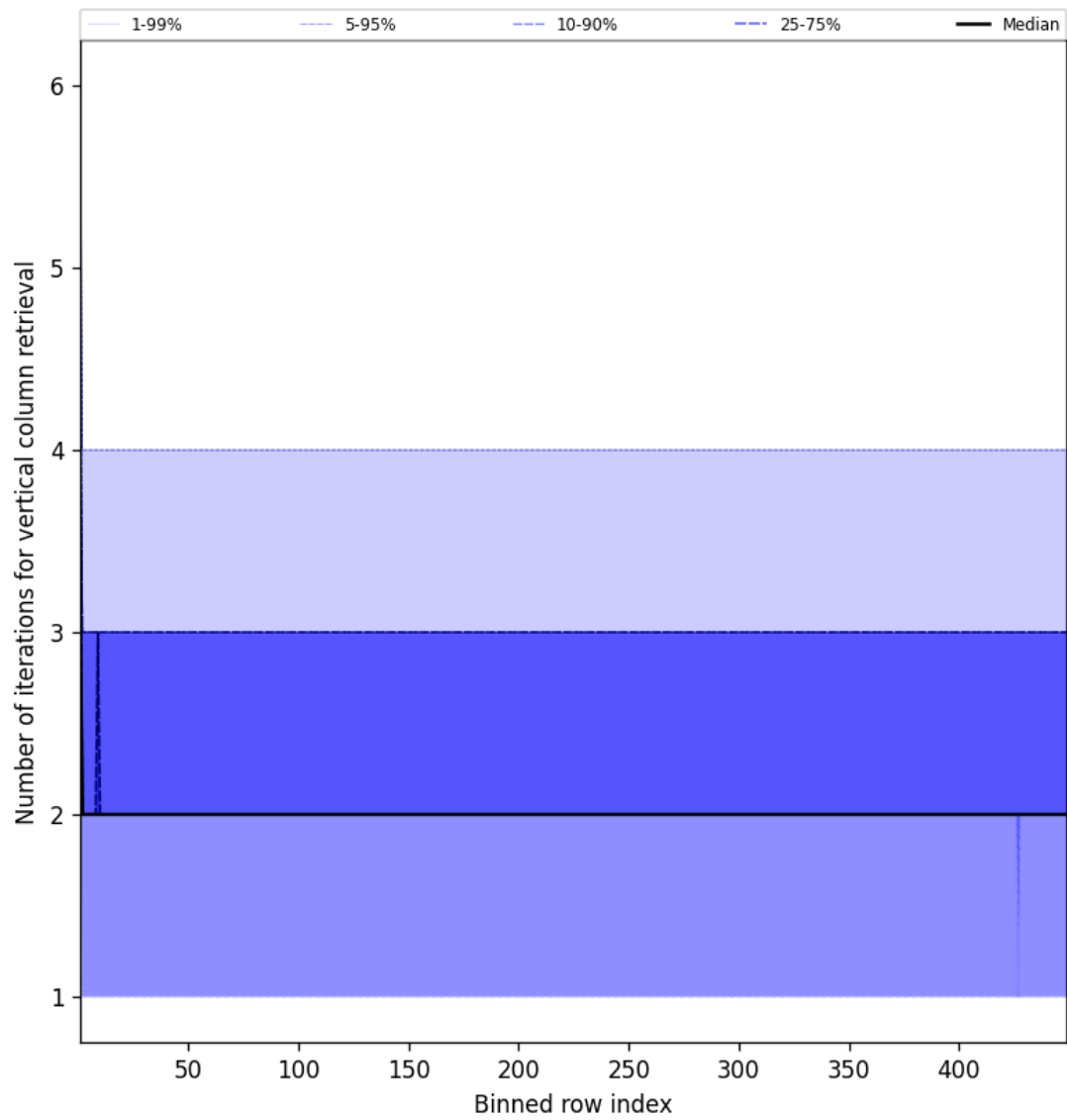
Figure 51: Along track statistics of “Number of iterations for vertical column retrieval” for 2025-07-21 to 2025-07-22
