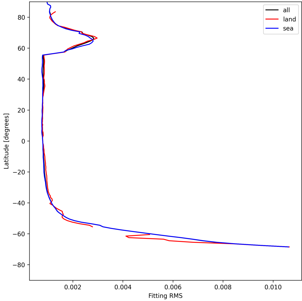
Figure 22: Zonal average of “Fitting RMS” for 2025-07-21 to 2025-07-22.
