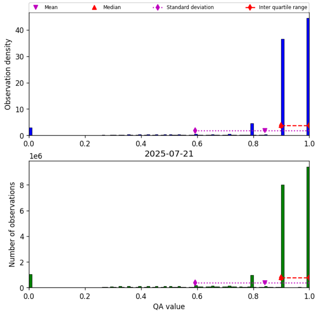
Figure 28: Histogram of “QA value” for 2025-07-21 to 2025-07-22
