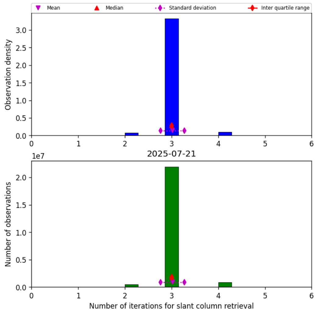
Figure 33: Histogram of “Number of iterations for slant column retrieval” for 2025-07-21 to 2025-07-22
