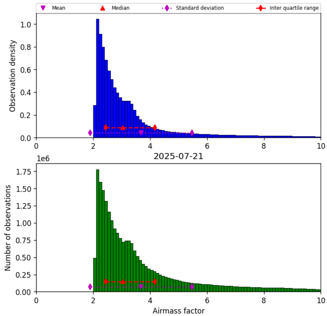
Figure 37: Histogram of “Airmass factor” for 2025-07-21 to 2025-07-22
