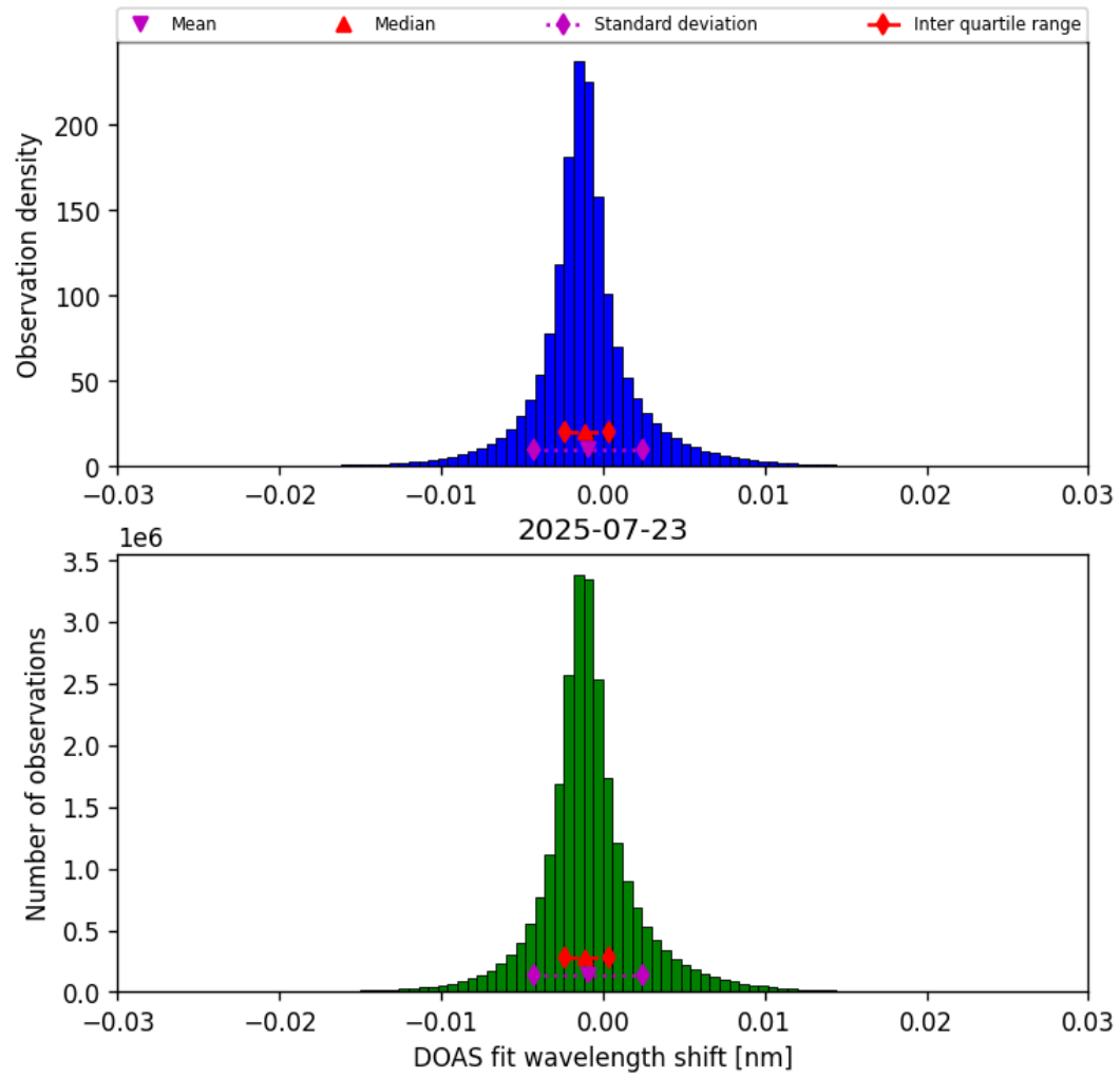
Figure 35: Histogram of “DOAS fit wavelength shift” for 2025-07-23 to 2025-07-24
