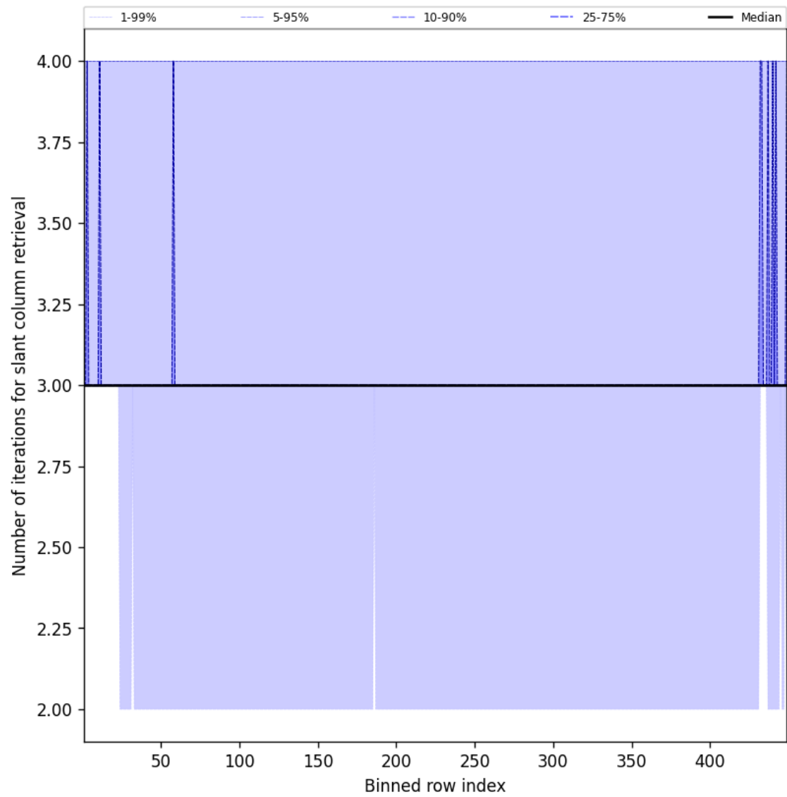
Figure 45: Along track statistics of “Number of iterations for slant column retrieval” for 2025-07-23 to 2025-07-24
