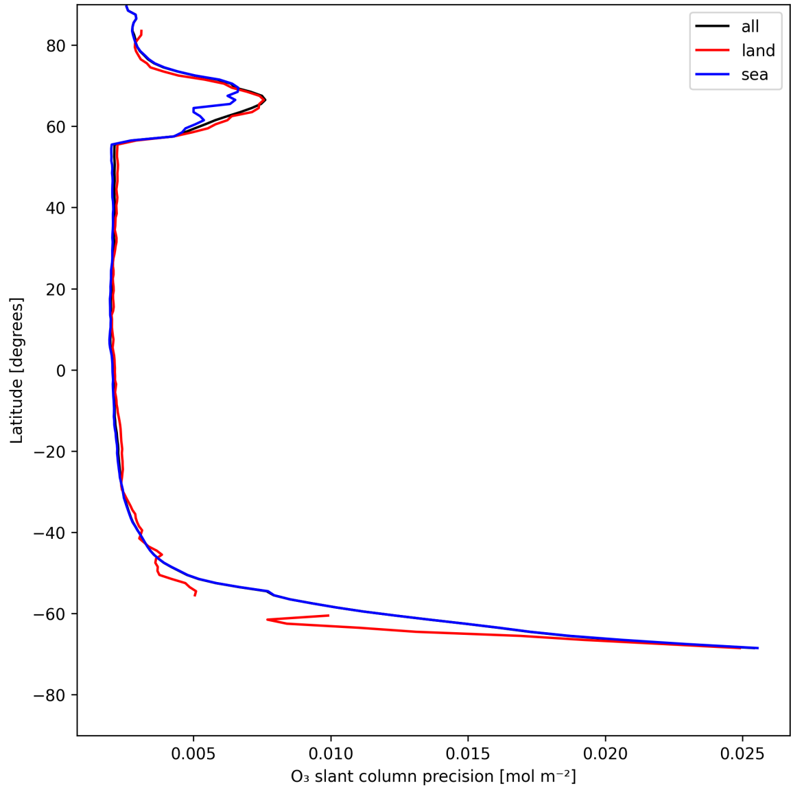
Figure 20: Zonal average of "O 3 slant column precision" for 2025-07-23 to 2025-07-24.
