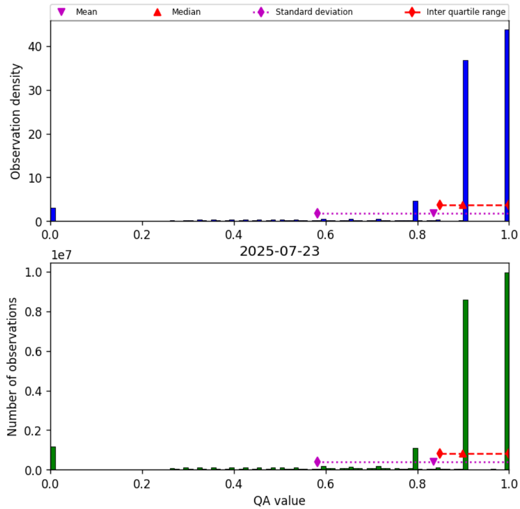
Figure 28: Histogram of “QA value” for 2025-07-23 to 2025-07-24
