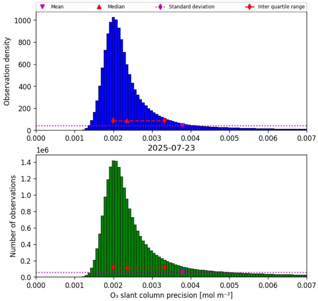
Figure 32: Histogram of “O 3 slant column precision” for 2025-07-23 to 2025-07-24
