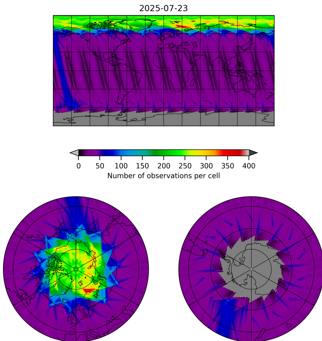
Figure 15: Map of the number of observations for 2025-07-23 to 2025-07-24
