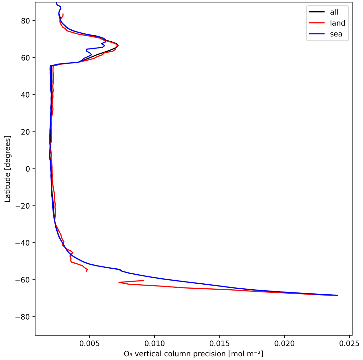
Figure 18: Zonal average of "O 3 vertical column precision" for 2025-07-23 to 2025-07-24.
