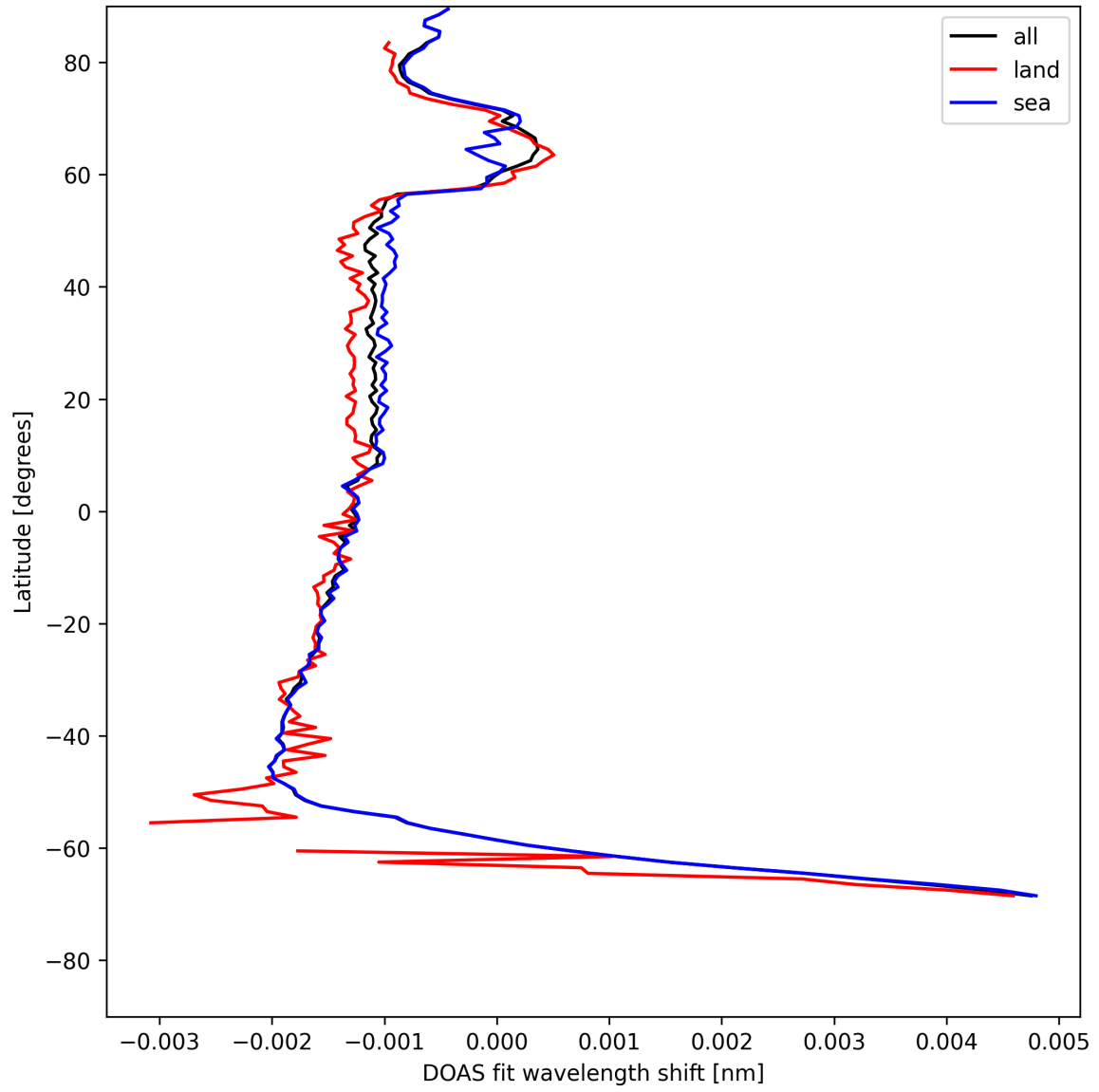
Figure 23: Zonal average of “DOAS fit wavelength shift” for 2025-07-23 to 2025-07-24.
