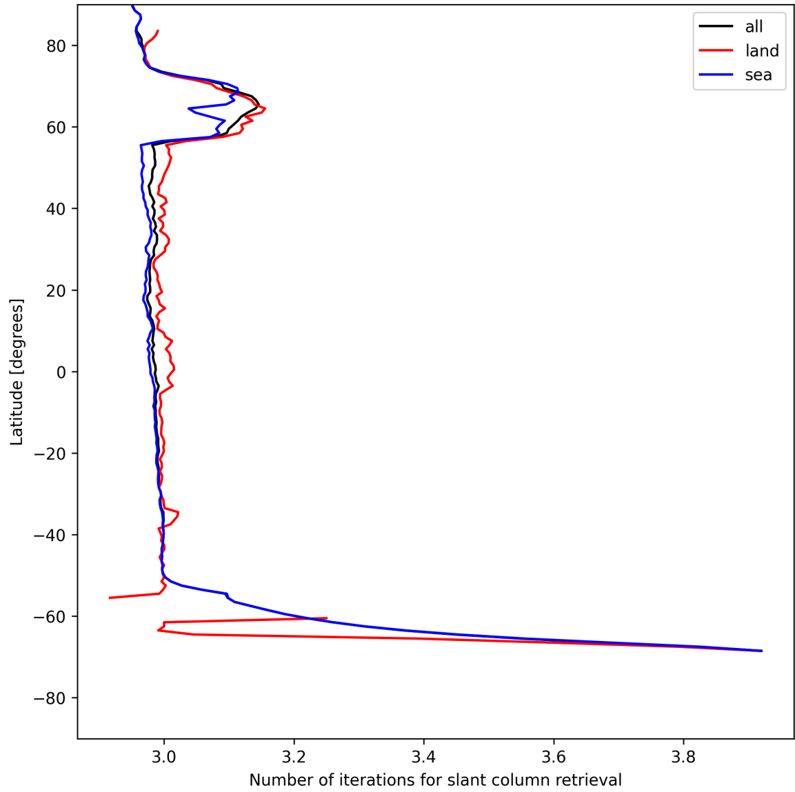
Figure 21: Zonal average of “Number of iterations for slant column retrieval” for 2025-07-23 to 2025-07-24.
