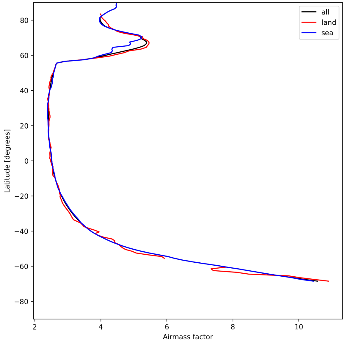
Figure 25: Zonal average of “Airmass factor” for 2025-07-23 to 2025-07-24.
