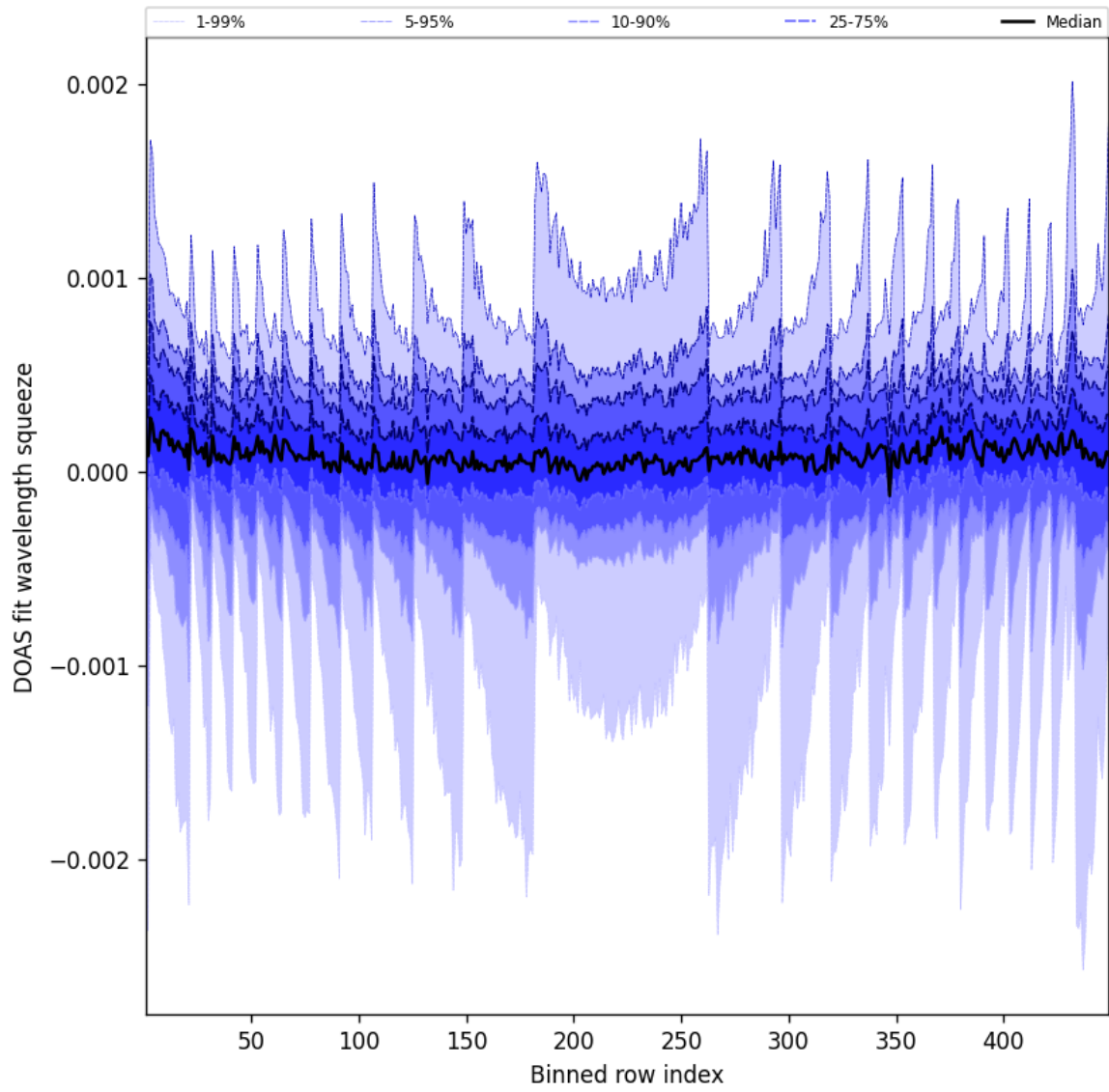
Figure 48: Along track statistics of “DOAS fit wavelength squeeze” for 2025-07-23 to 2025-07-24
