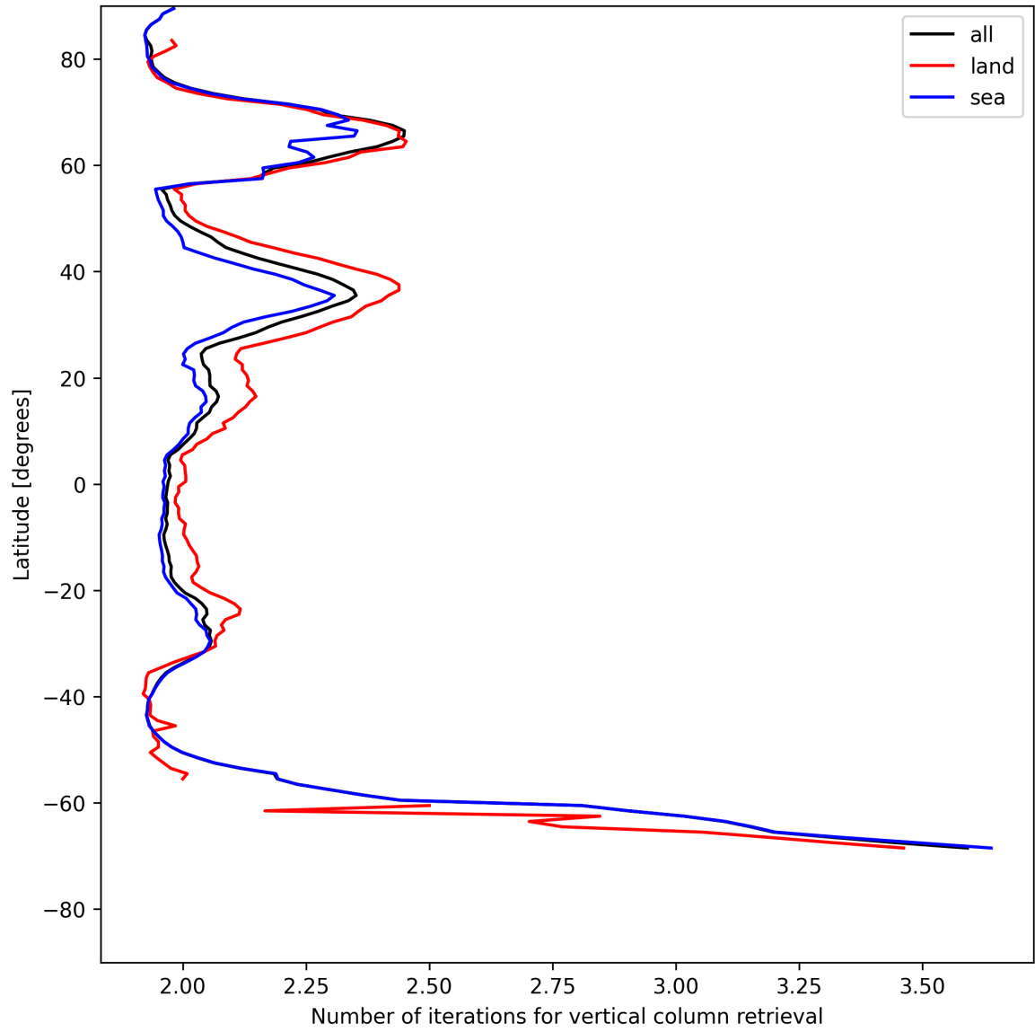
Figure 27: Zonal average of “Number of iterations for vertical column retrieval” for 2025-07-23 to 2025-07-24.
