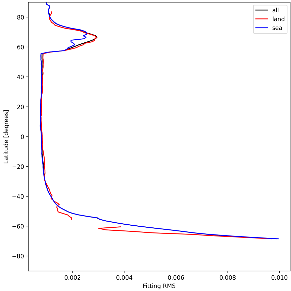
Figure 22: Zonal average of “Fitting RMS” for 2025-07-23 to 2025-07-24.
