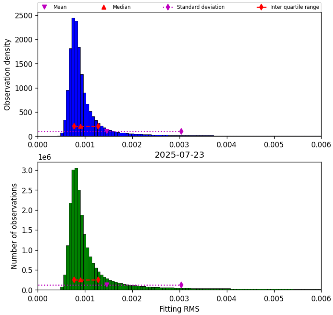
Figure 34: Histogram of “Fitting RMS” for 2025-07-23 to 2025-07-24
