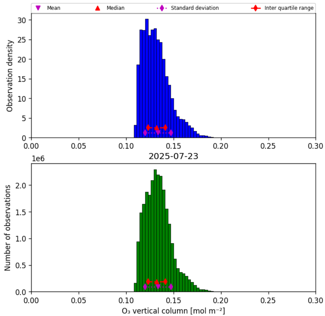
Figure 29: Histogram of “O 3 vertical column” for 2025-07-23 to 2025-07-24
