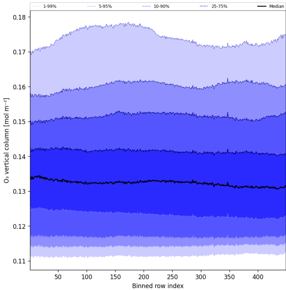
Figure 41: Along track statistics of “O 3 vertical column” for 2025-07-23 to 2025-07-24
