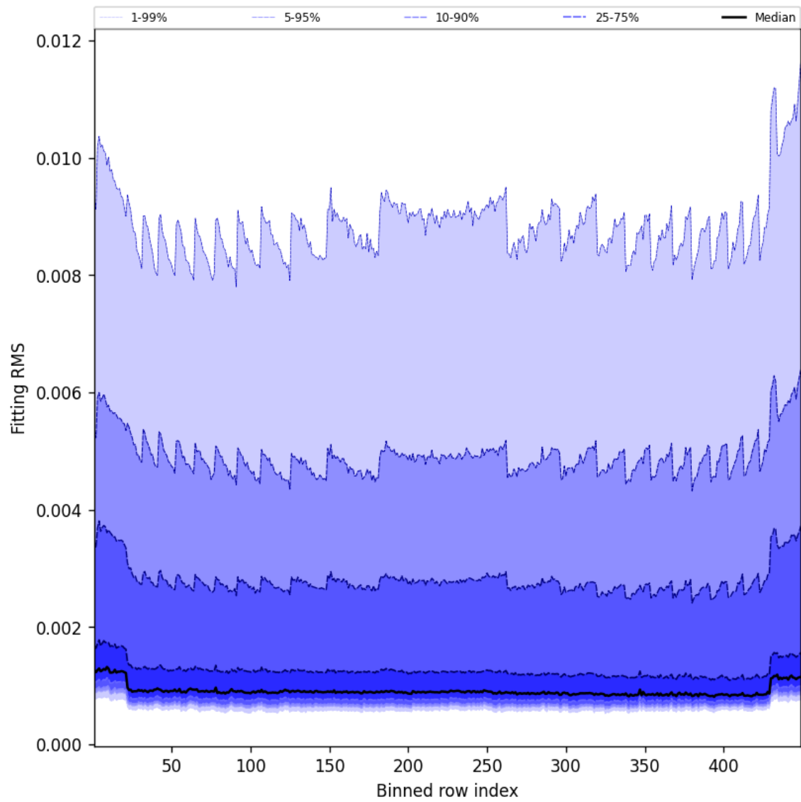
Figure 46: Along track statistics of “Fitting RMS” for 2025-07-23 to 2025-07-24
