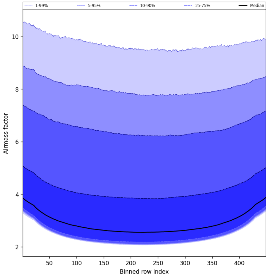
Figure 49: Along track statistics of “Airmass factor” for 2025-07-23 to 2025-07-24
