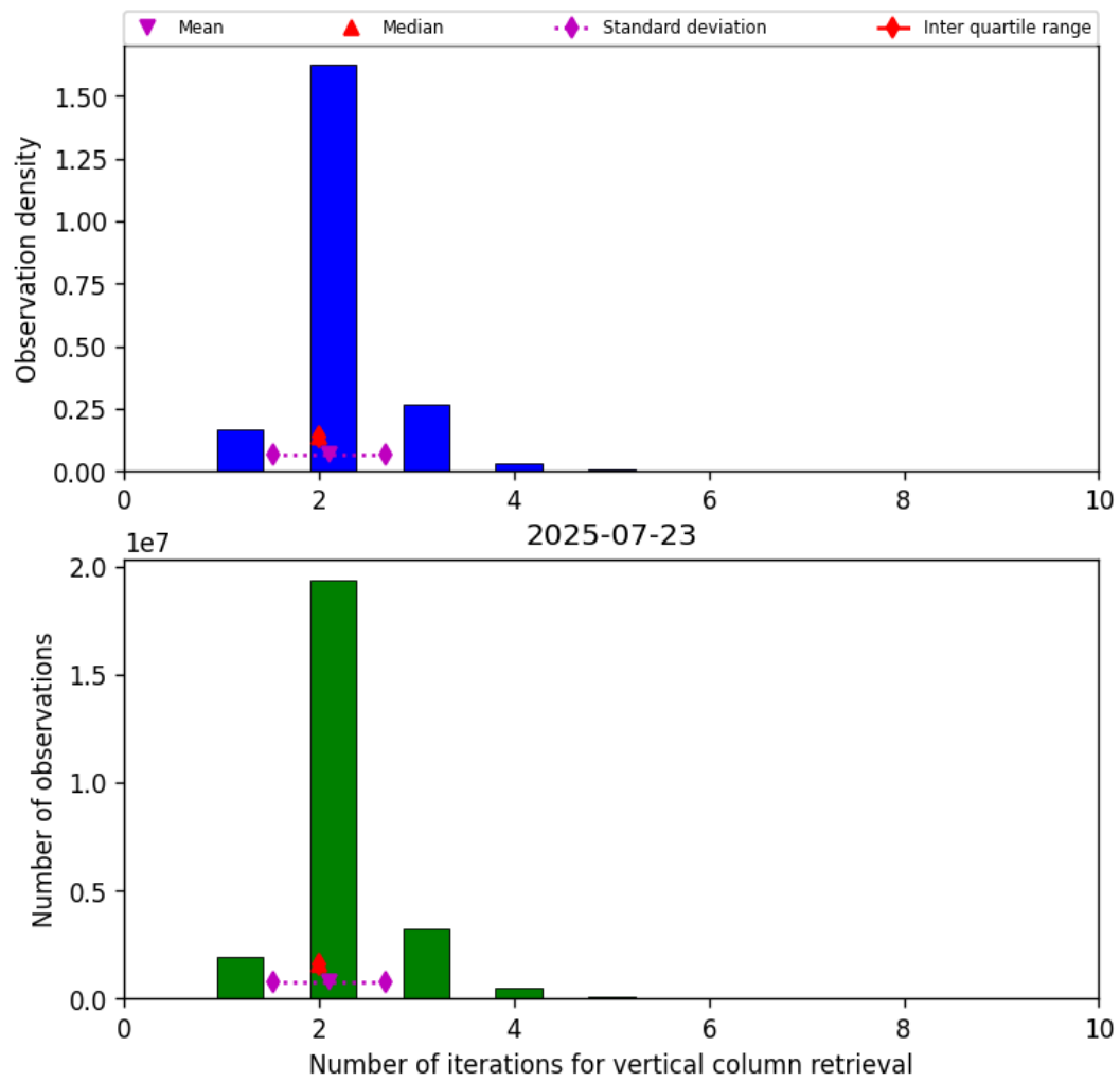
Figure 39: Histogram of “Number of iterations for vertical column retrieval” for 2025-07-23 to 2025-07-24
