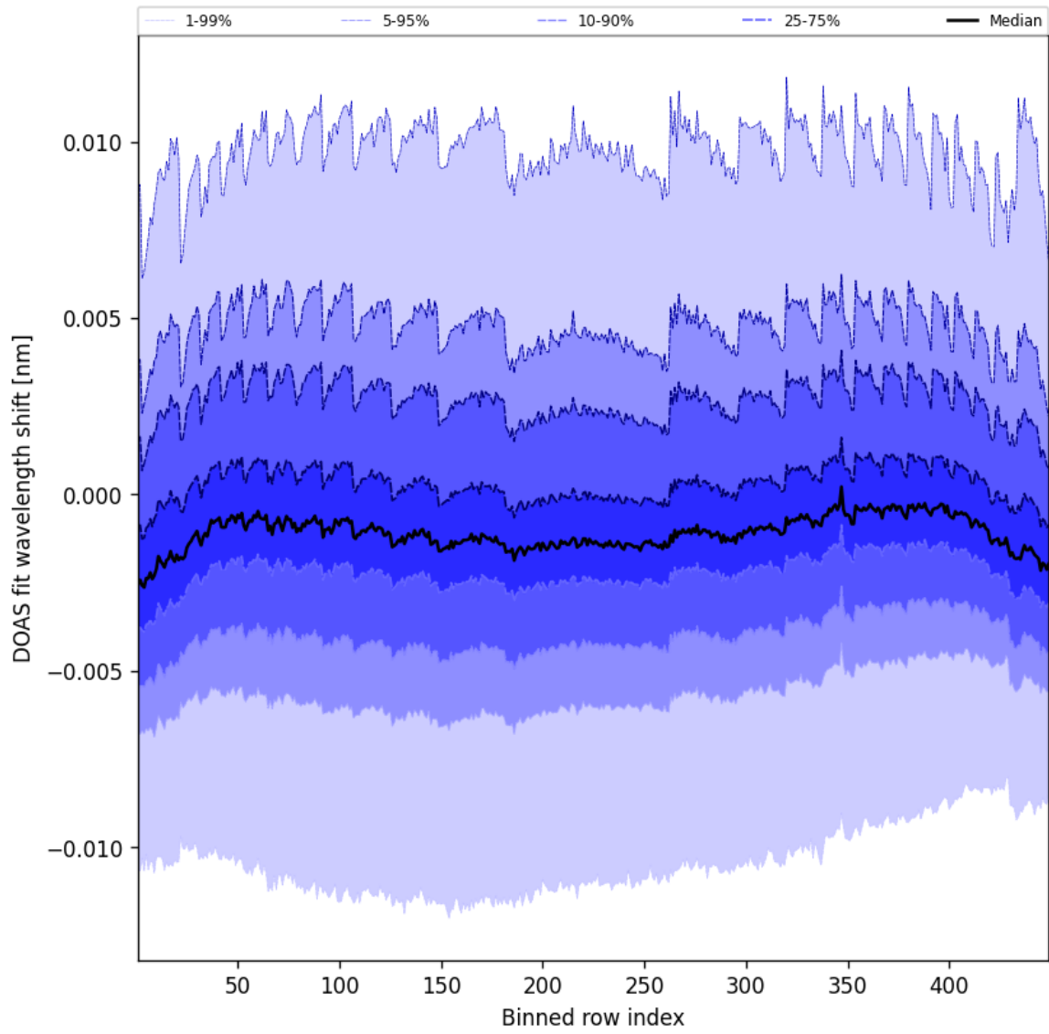
Figure 47: Along track statistics of “DOAS fit wavelength shift” for 2025-07-23 to 2025-07-24
