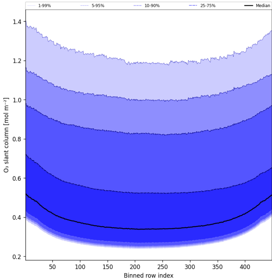
Figure 43: Along track statistics of “O 3 slant column” for 2025-07-23 to 2025-07-24
