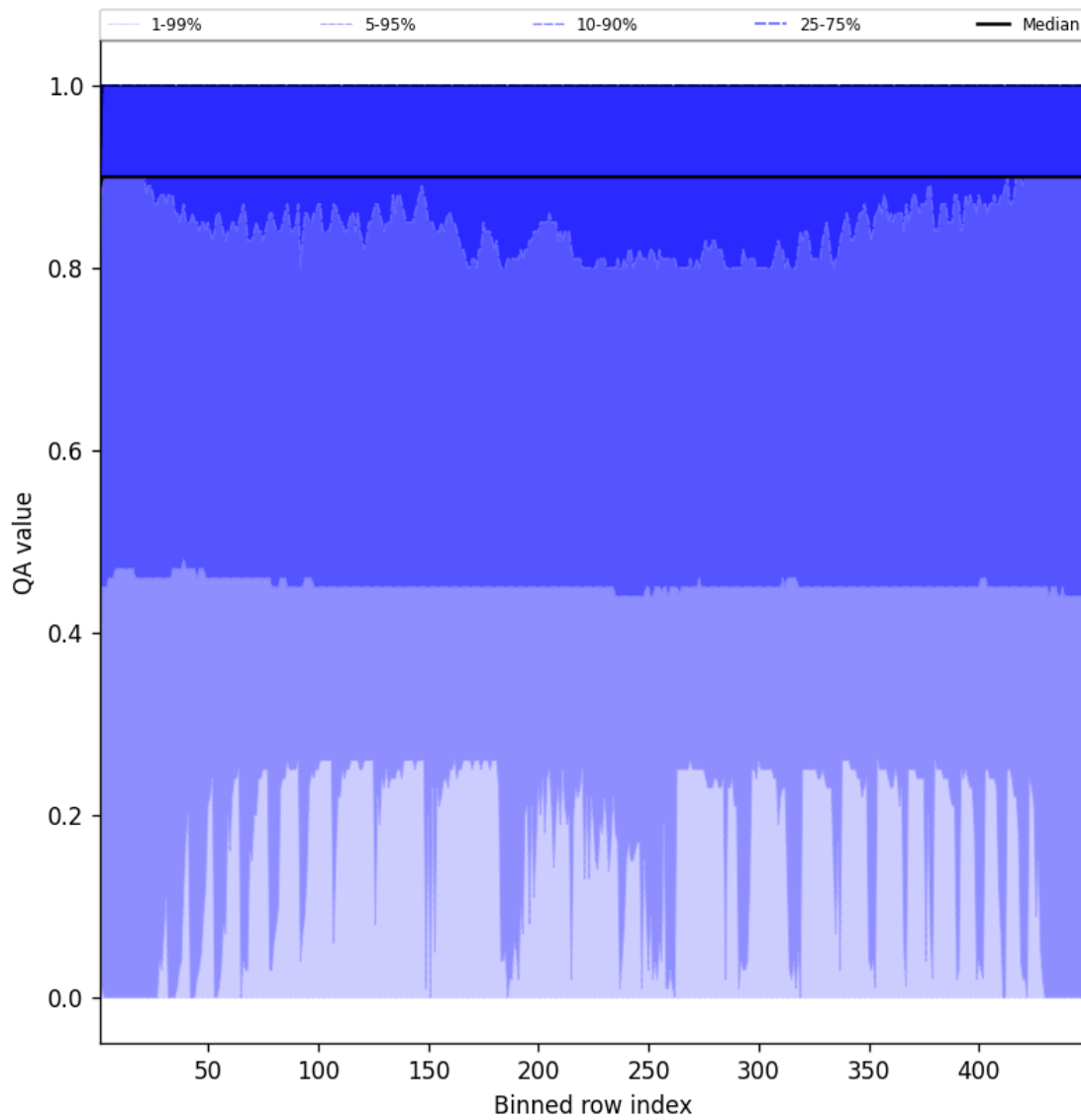
Figure 40: Along track statistics of “QA value” for 2025-07-23 to 2025-07-24
