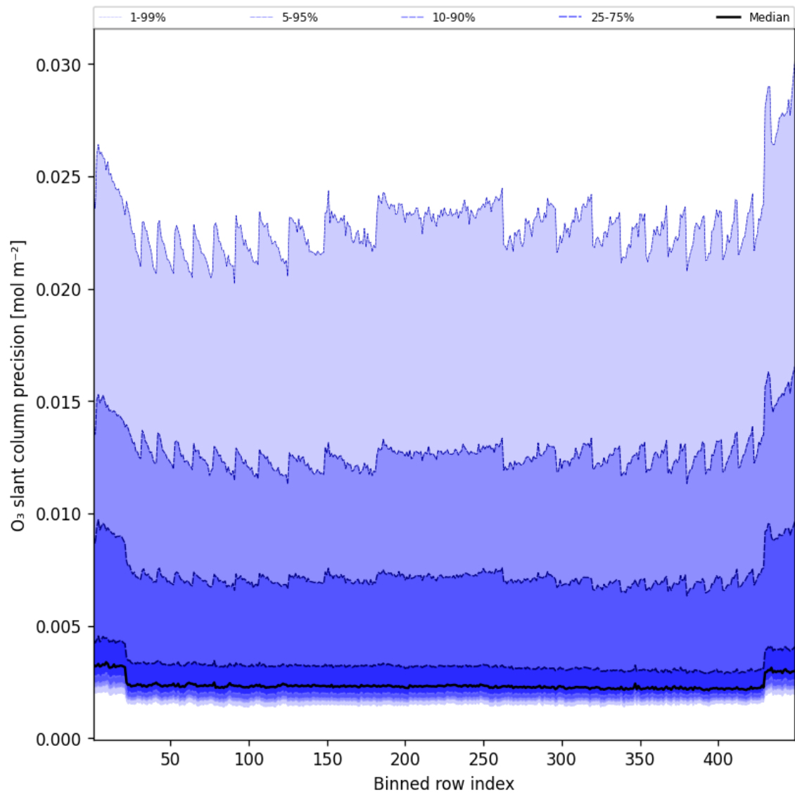
Figure 44: Along track statistics of “O 3 slant column precision” for 2025-07-23 to 2025-07-24
