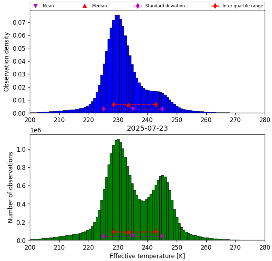
Figure 38: Histogram of “Effective temperature” for 2025-07-23 to 2025-07-24
