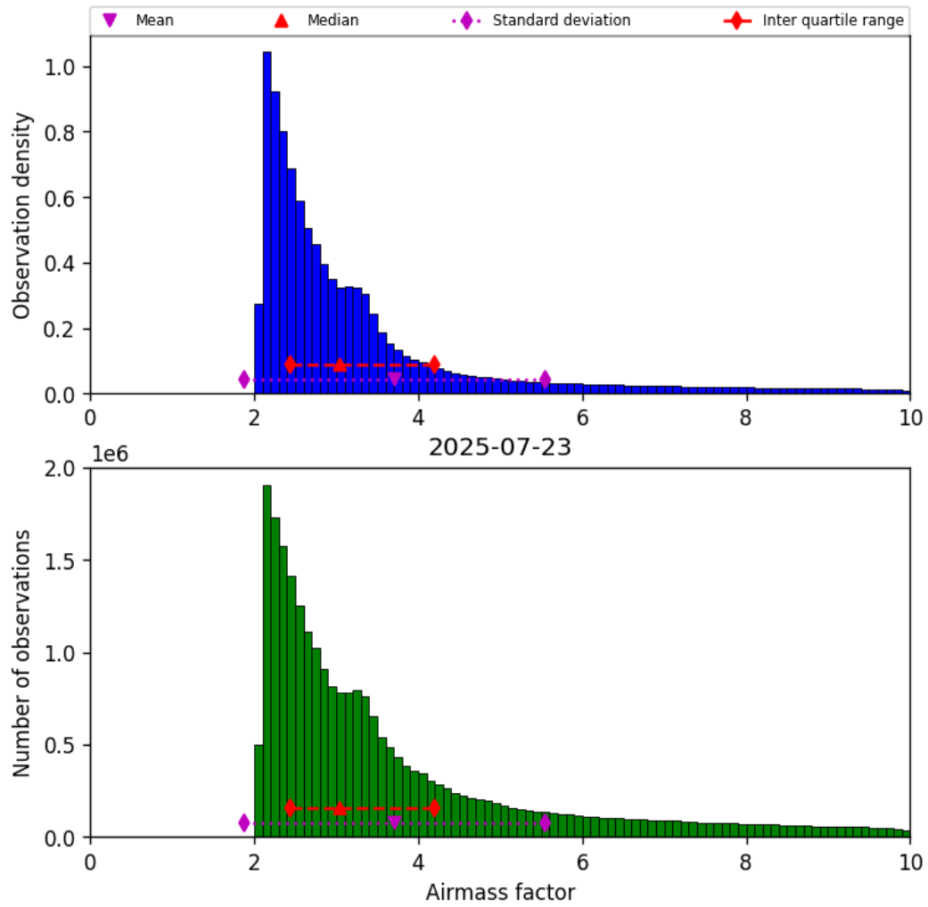
Figure 37: Histogram of “Airmass factor” for 2025-07-23 to 2025-07-24
