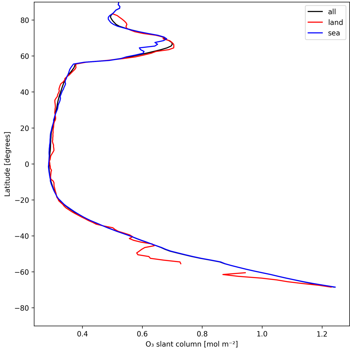
Figure 19: Zonal average of “O 3 slant column” for 2025-07-23 to 2025-07-24.
