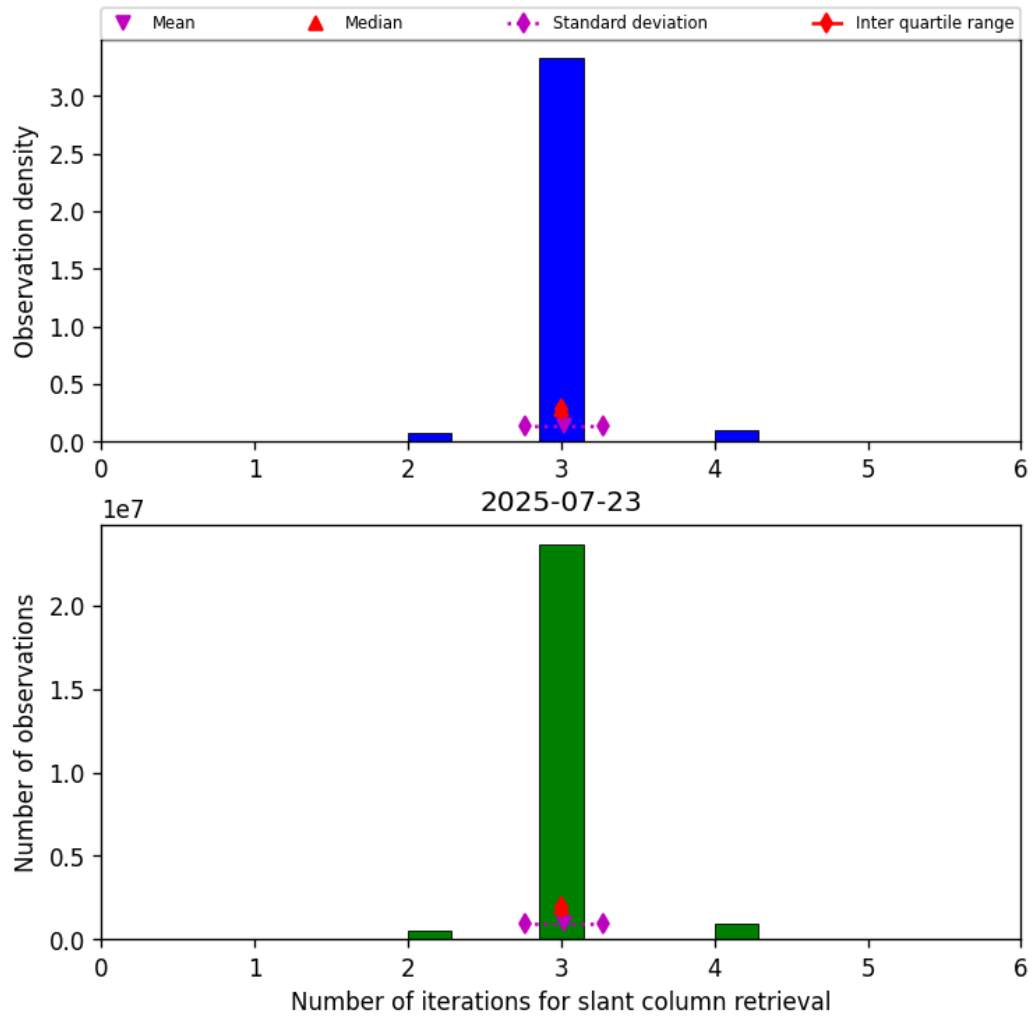
Figure 33: Histogram of “Number of iterations for slant column retrieval” for 2025-07-23 to 2025-07-24
