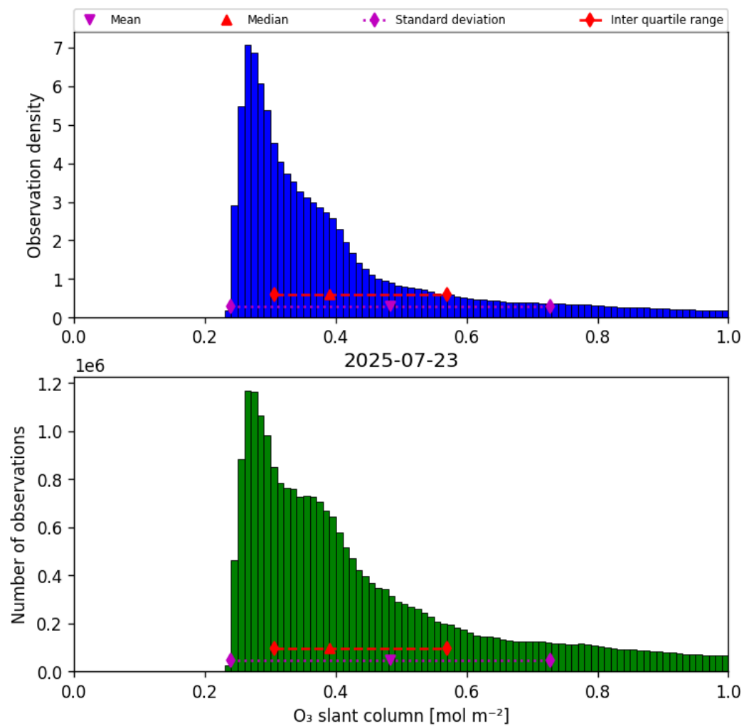
Figure 31: Histogram of “O 3 slant column” for 2025-07-23 to 2025-07-24
