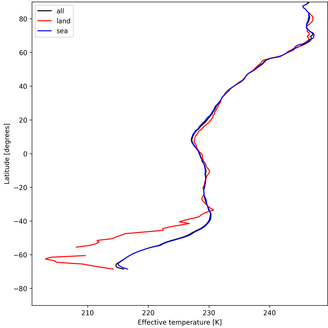
Figure 26: Zonal average of “Effective temperature” for 2025-07-23 to 2025-07-24.
