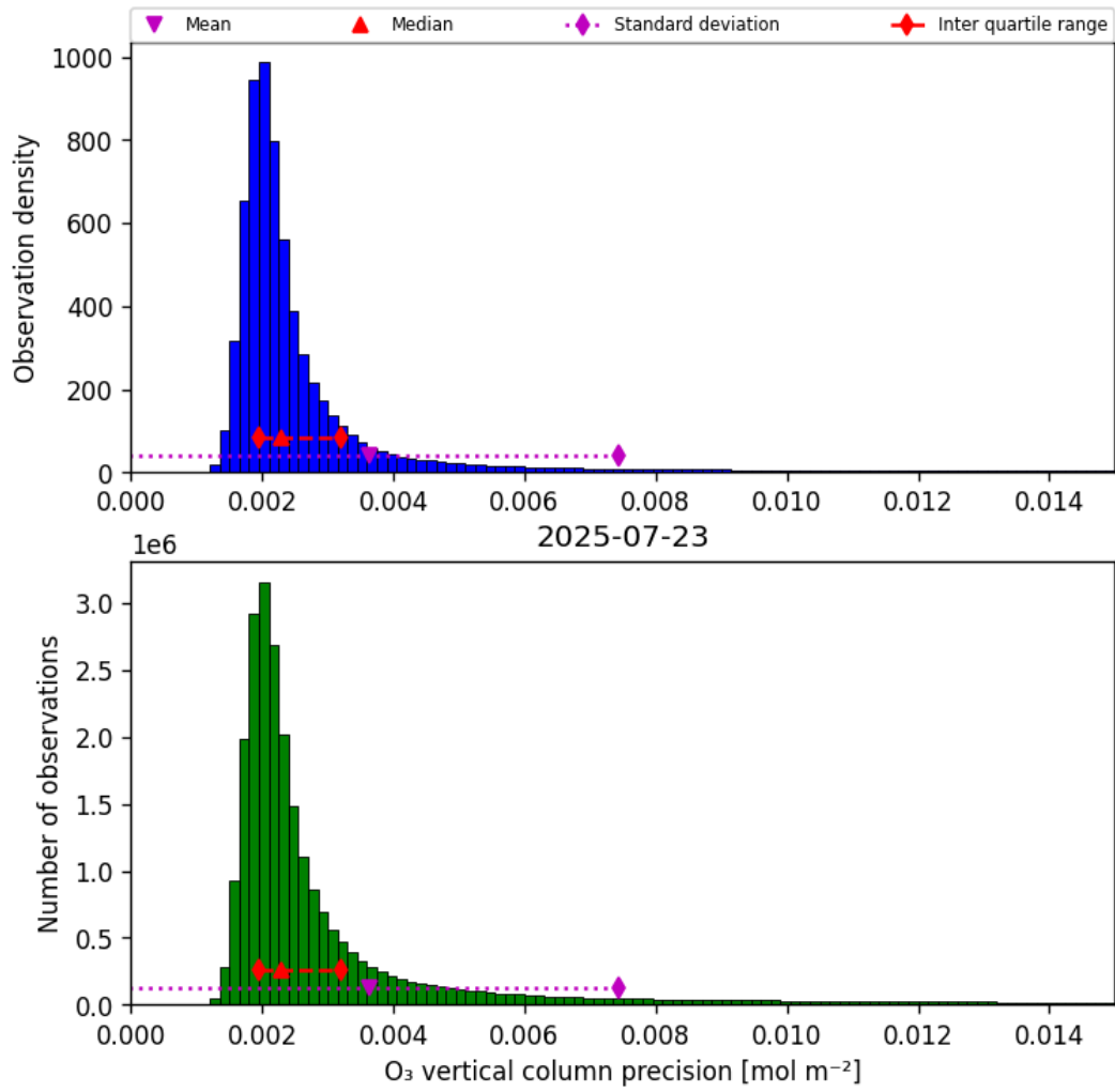
Figure 30: Histogram of “O 3 vertical column precision” for 2025-07-23 to 2025-07-24
