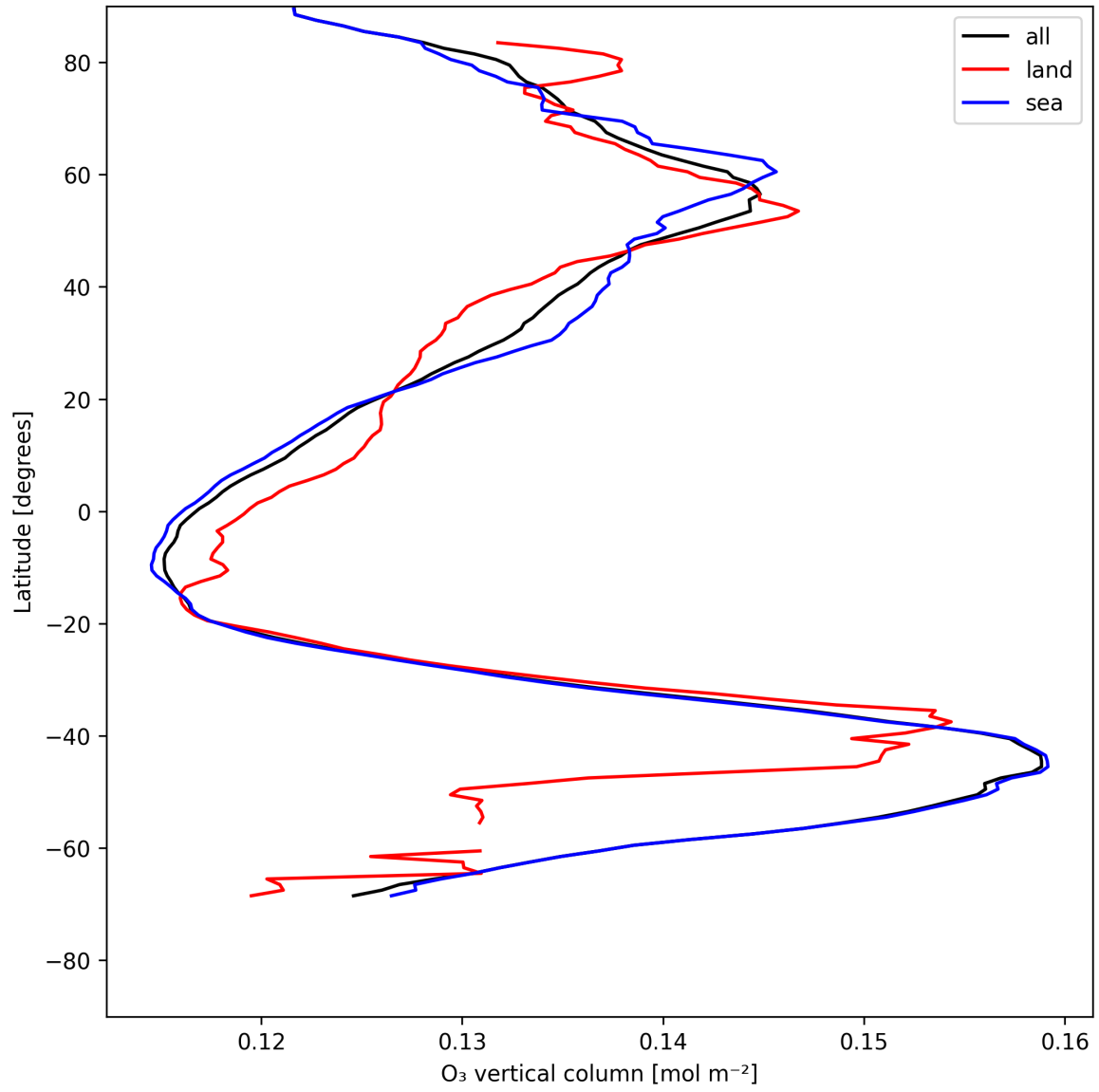
Figure 17: Zonal average of “O 3 vertical column” for 2025-07-23 to 2025-07-24.
