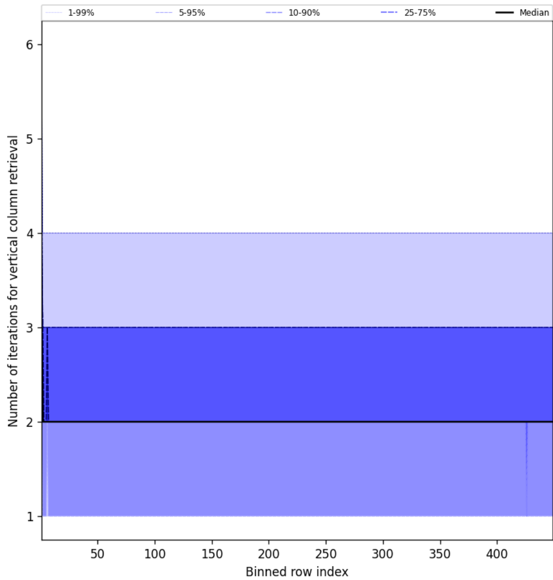
Figure 51: Along track statistics of “Number of iterations for vertical column retrieval” for 2025-07-23 to 2025-07-24
