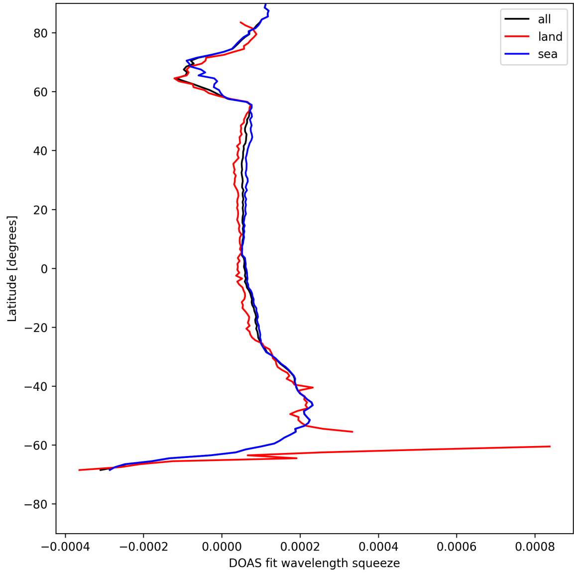
Figure 24: Zonal average of "DOAS fit wavelength squeeze" for 2025-07-23 to 2025-07-24.
