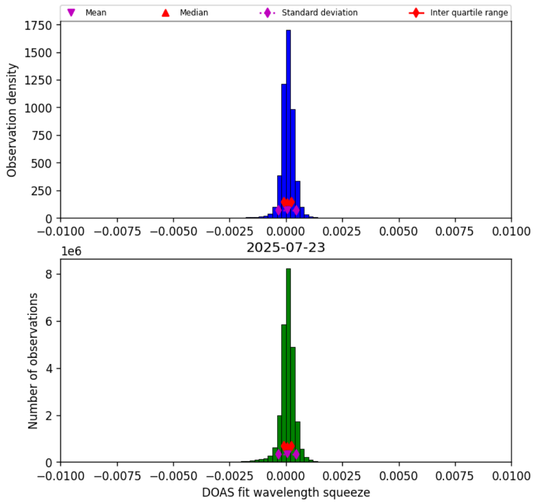
Figure 36: Histogram of “DOAS fit wavelength squeeze” for 2025-07-23 to 2025-07-24
