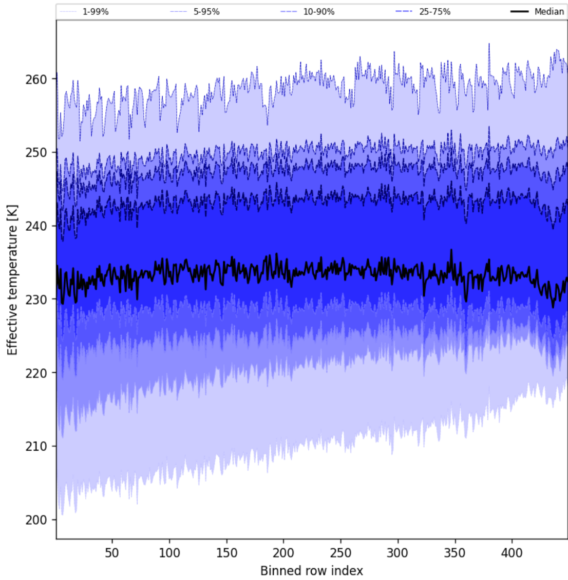
Figure 50: Along track statistics of “Effective temperature” for 2025-07-23 to 2025-07-24
