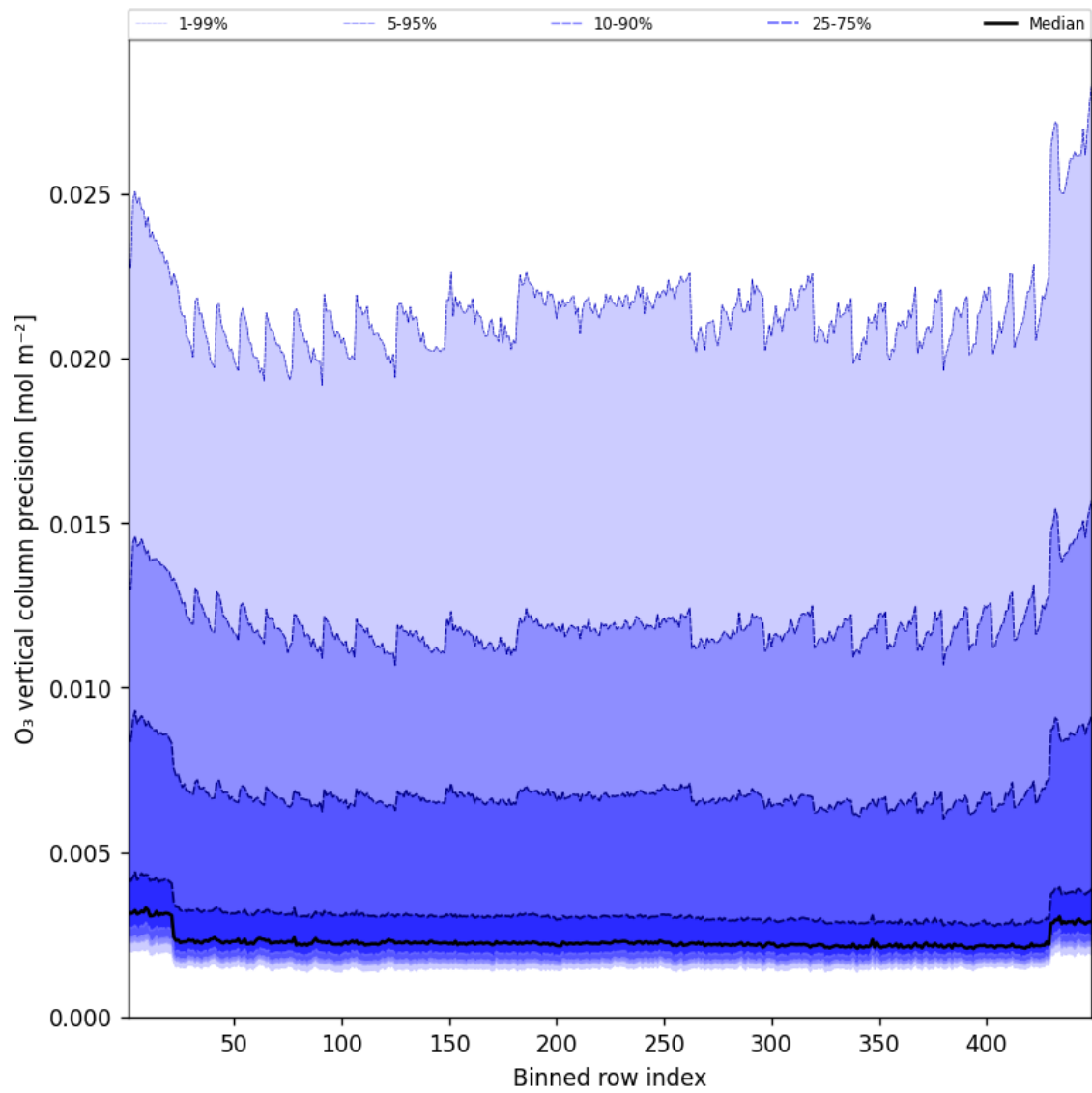
Figure 42: Along track statistics of “O 3 vertical column precision” for 2025-07-23 to 2025-07-24
