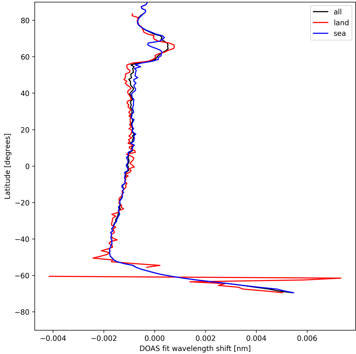
Figure 23: Zonal average of "DOAS fit wavelength shift" for 2025-07-24 to 2025-07-25.
