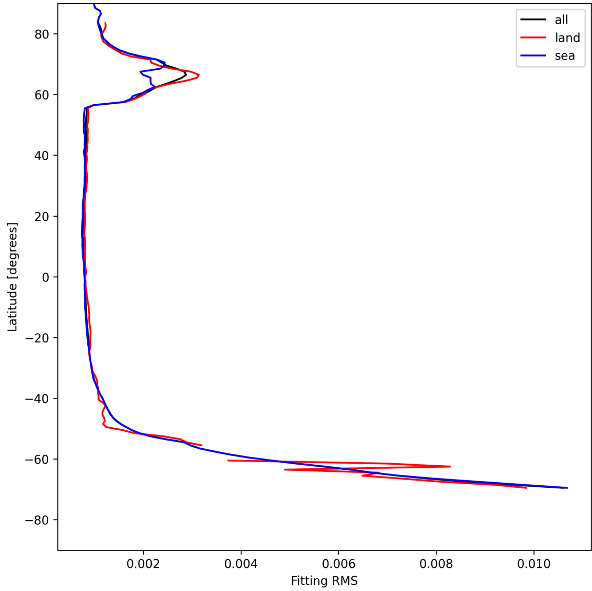
Figure 22: Zonal average of “Fitting RMS” for 2025-07-24 to 2025-07-25.
