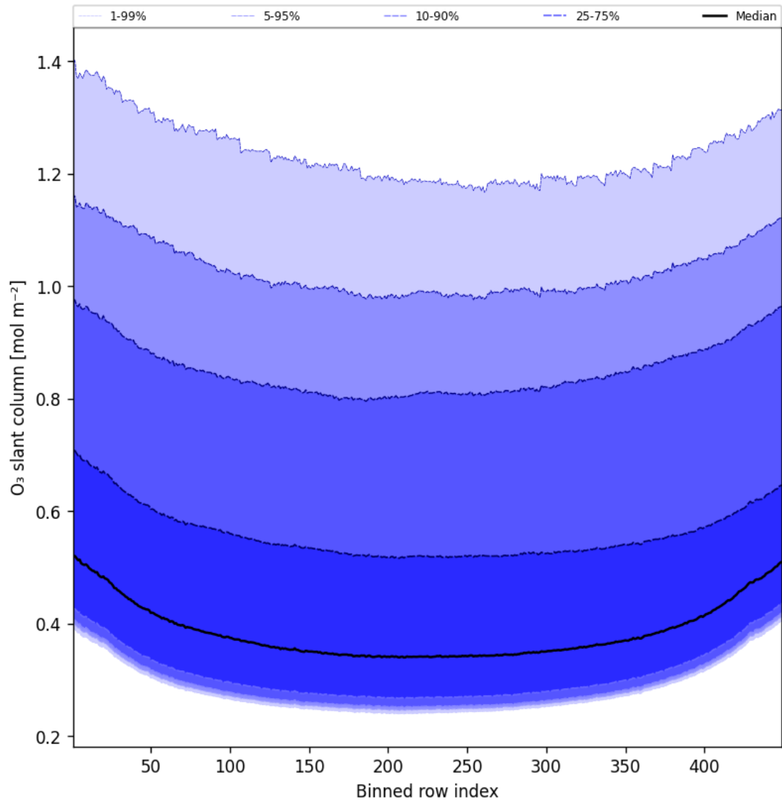
Figure 43: Along track statistics of “O 3 slant column” for 2025-07-24 to 2025-07-25
