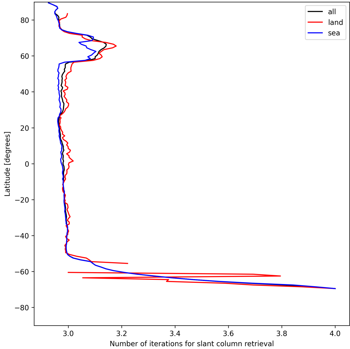
Figure 21: Zonal average of “Number of iterations for slant column retrieval” for 2025-07-24 to 2025-07-25.
