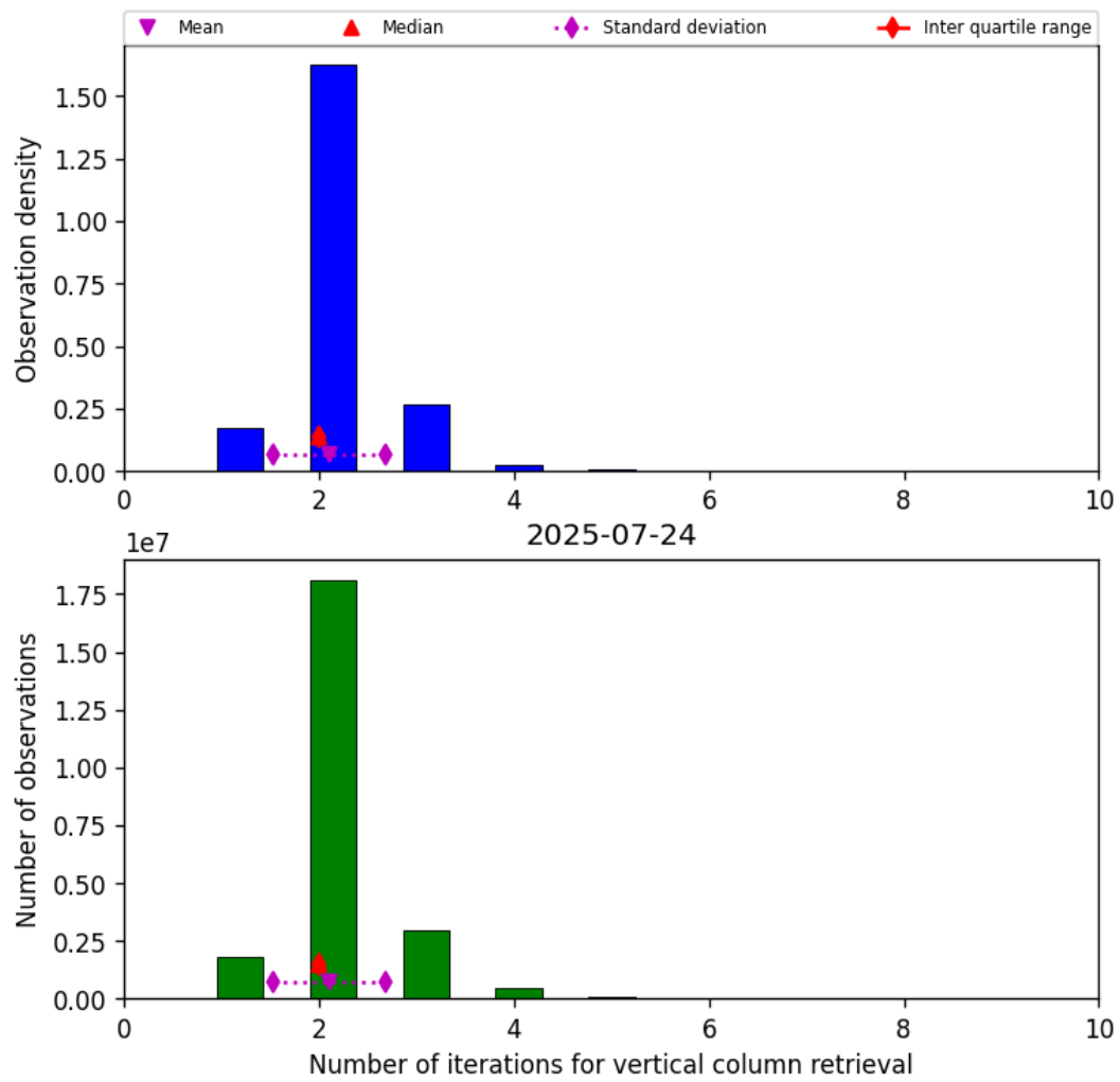
Figure 39: Histogram of “Number of iterations for vertical column retrieval” for 2025-07-24 to 2025-07-25
