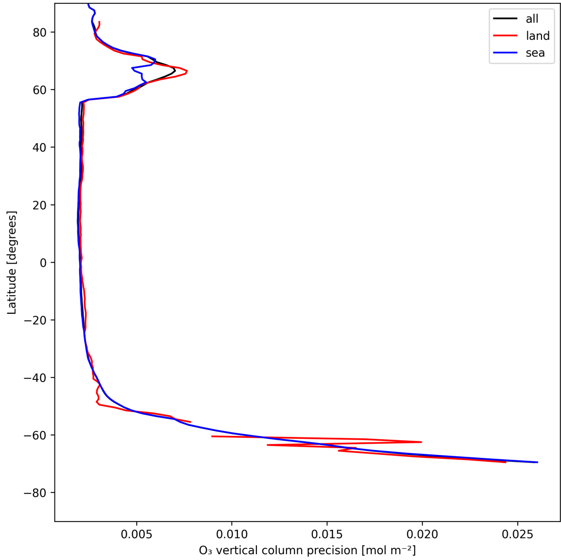
Figure 18: Zonal average of “O 3 vertical column precision” for 2025-07-24 to 2025-07-25.
