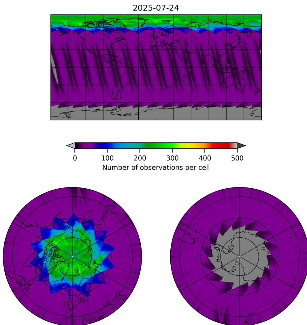
Figure 15: Map of the number of observations for 2025-07-24 to 2025-07-25
