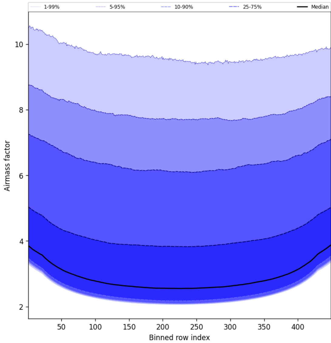
Figure 49: Along track statistics of “Airmass factor” for 2025-07-24 to 2025-07-25
