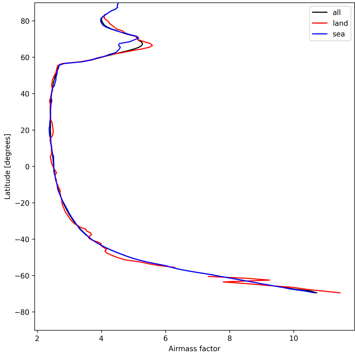
Figure 25: Zonal average of “Airmass factor” for 2025-07-24 to 2025-07-25.
