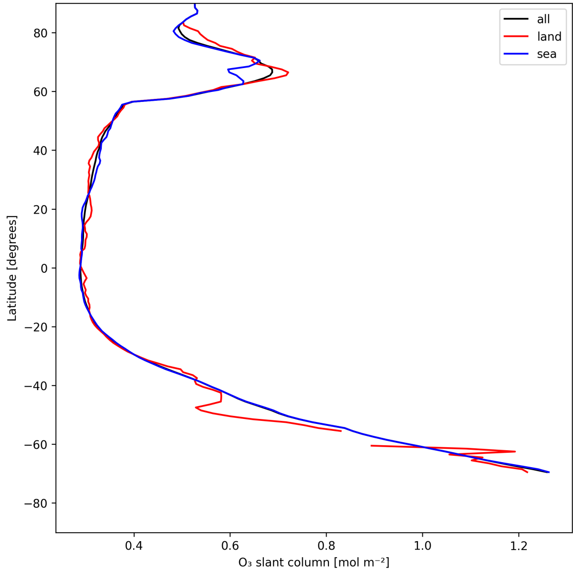
Figure 19: Zonal average of “O 3 slant column” for 2025-07-24 to 2025-07-25.
