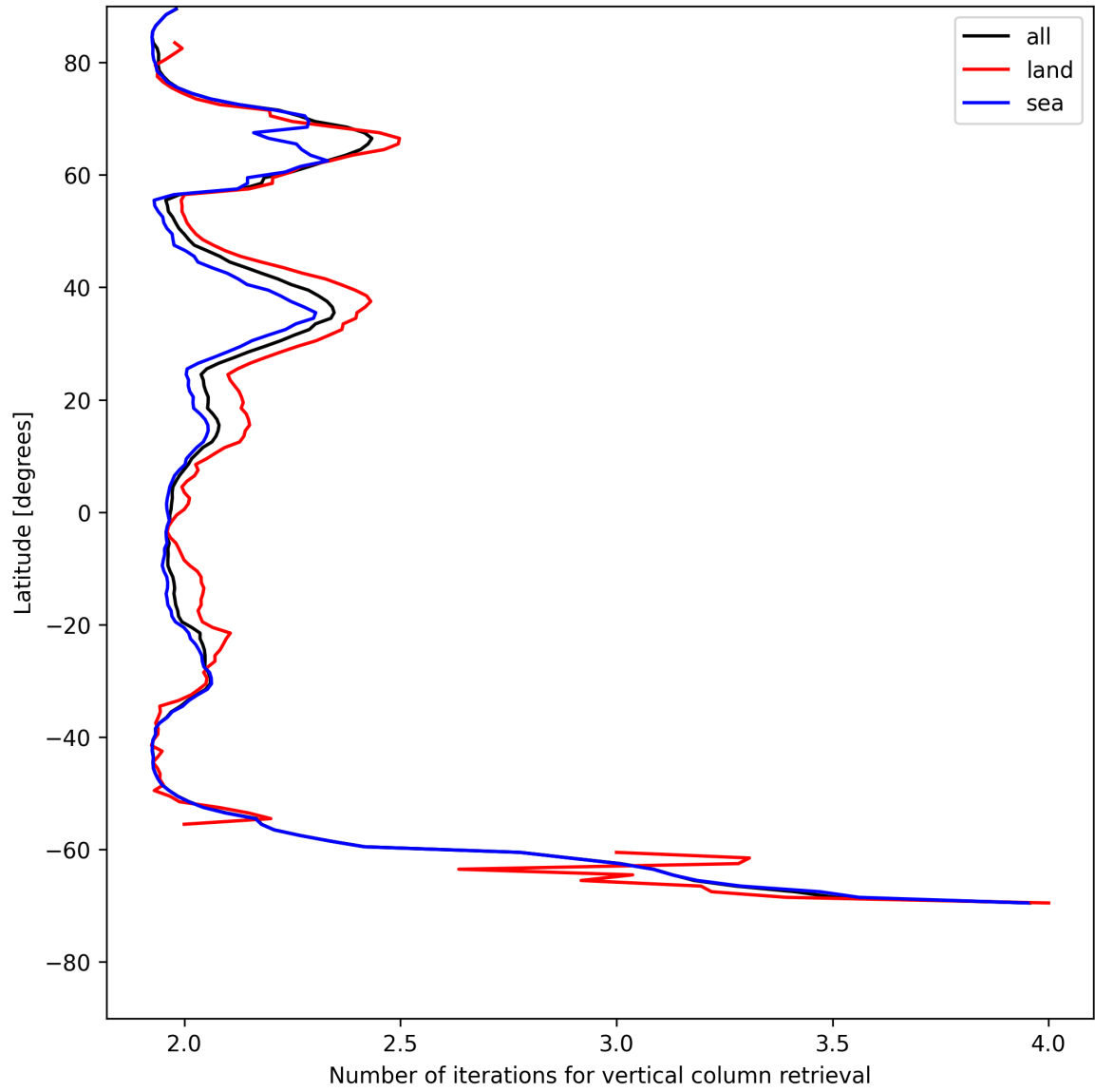
Figure 27: Zonal average of “Number of iterations for vertical column retrieval” for 2025-07-24 to 2025-07-25.
