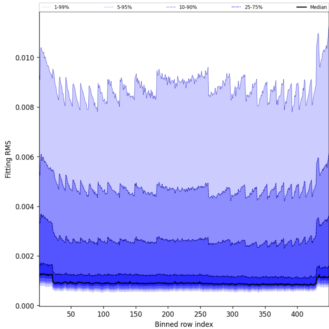
Figure 46: Along track statistics of “Fitting RMS” for 2025-07-24 to 2025-07-25
