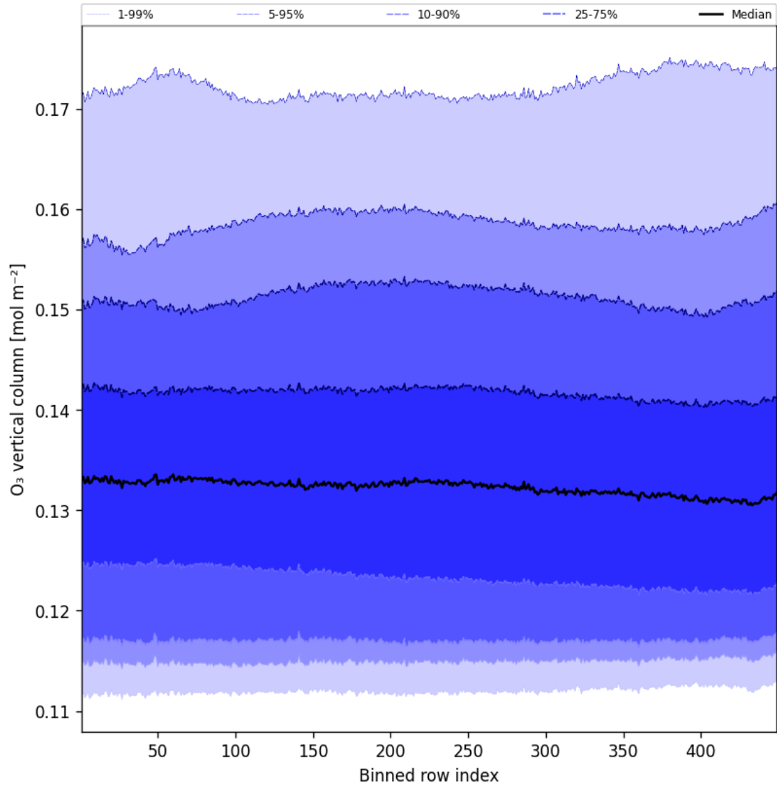
Figure 41: Along track statistics of “O 3 vertical column” for 2025-07-24 to 2025-07-25
