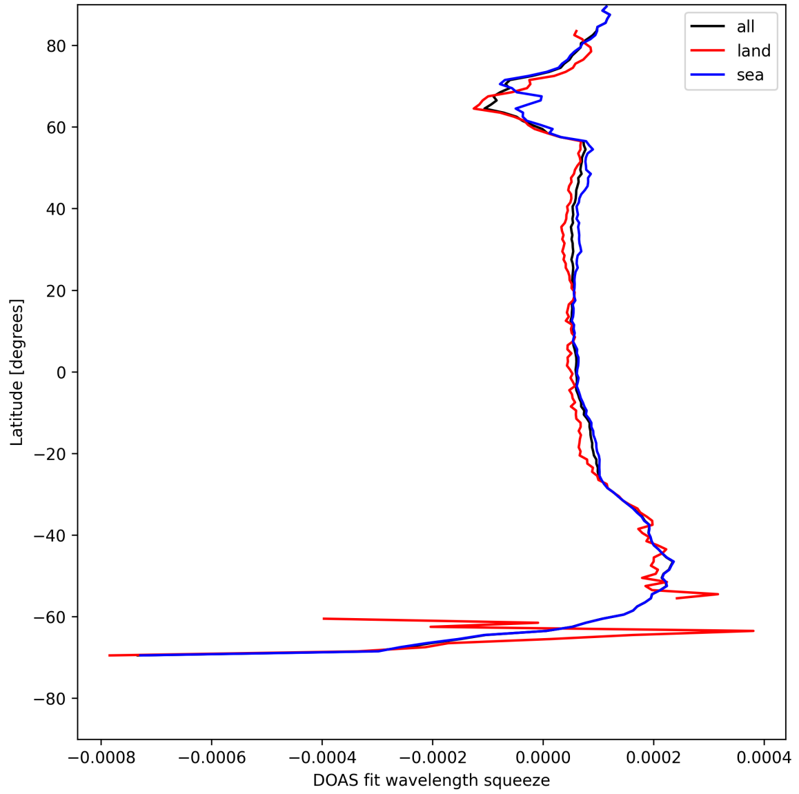
Figure 24: Zonal average of “DOAS fit wavelength squeeze” for 2025-07-24 to 2025-07-25.
