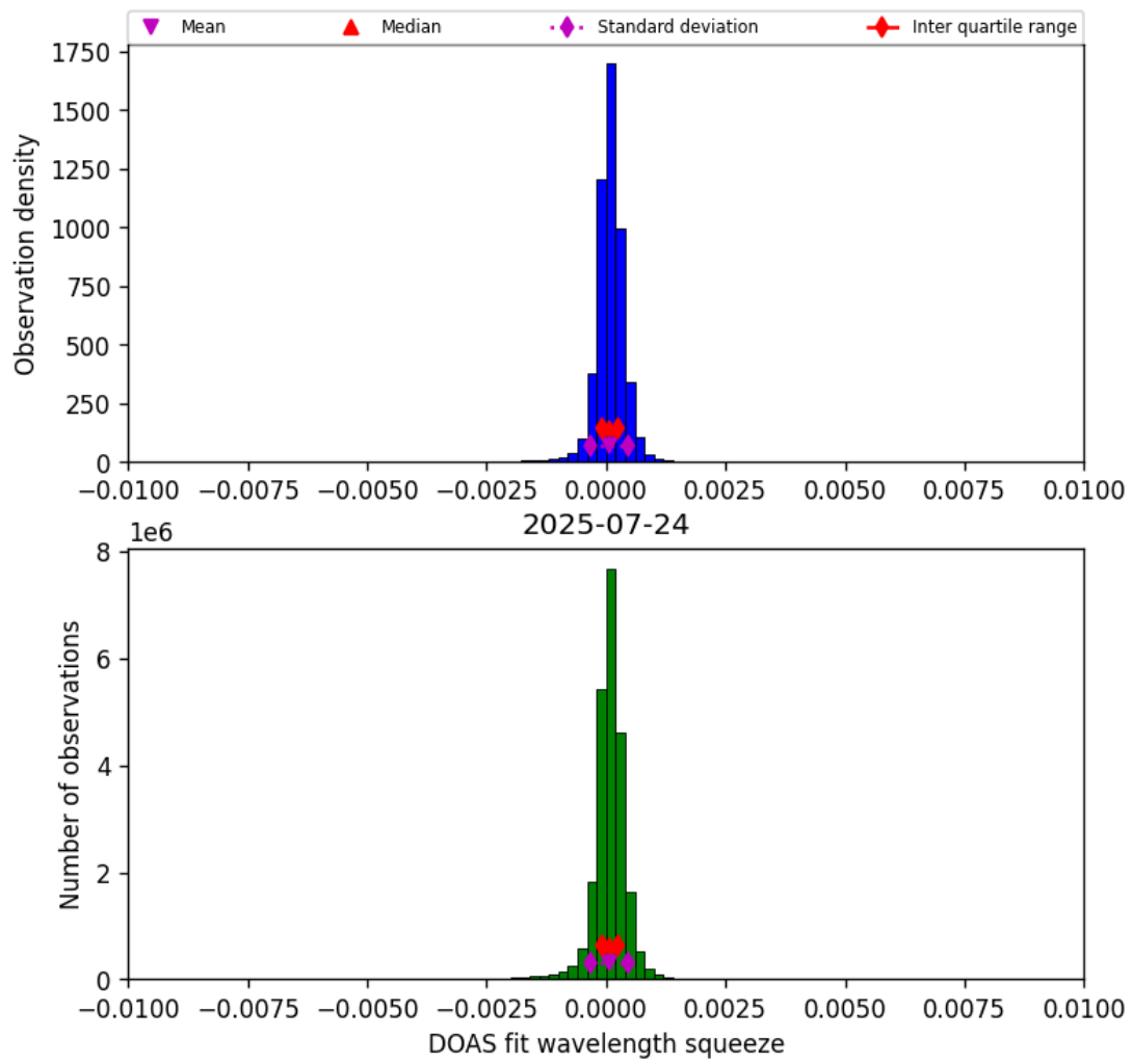
Figure 36: Histogram of “DOAS fit wavelength squeeze” for 2025-07-24 to 2025-07-25
