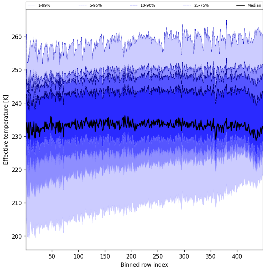
Figure 50: Along track statistics of “Effective temperature” for 2025-07-24 to 2025-07-25
