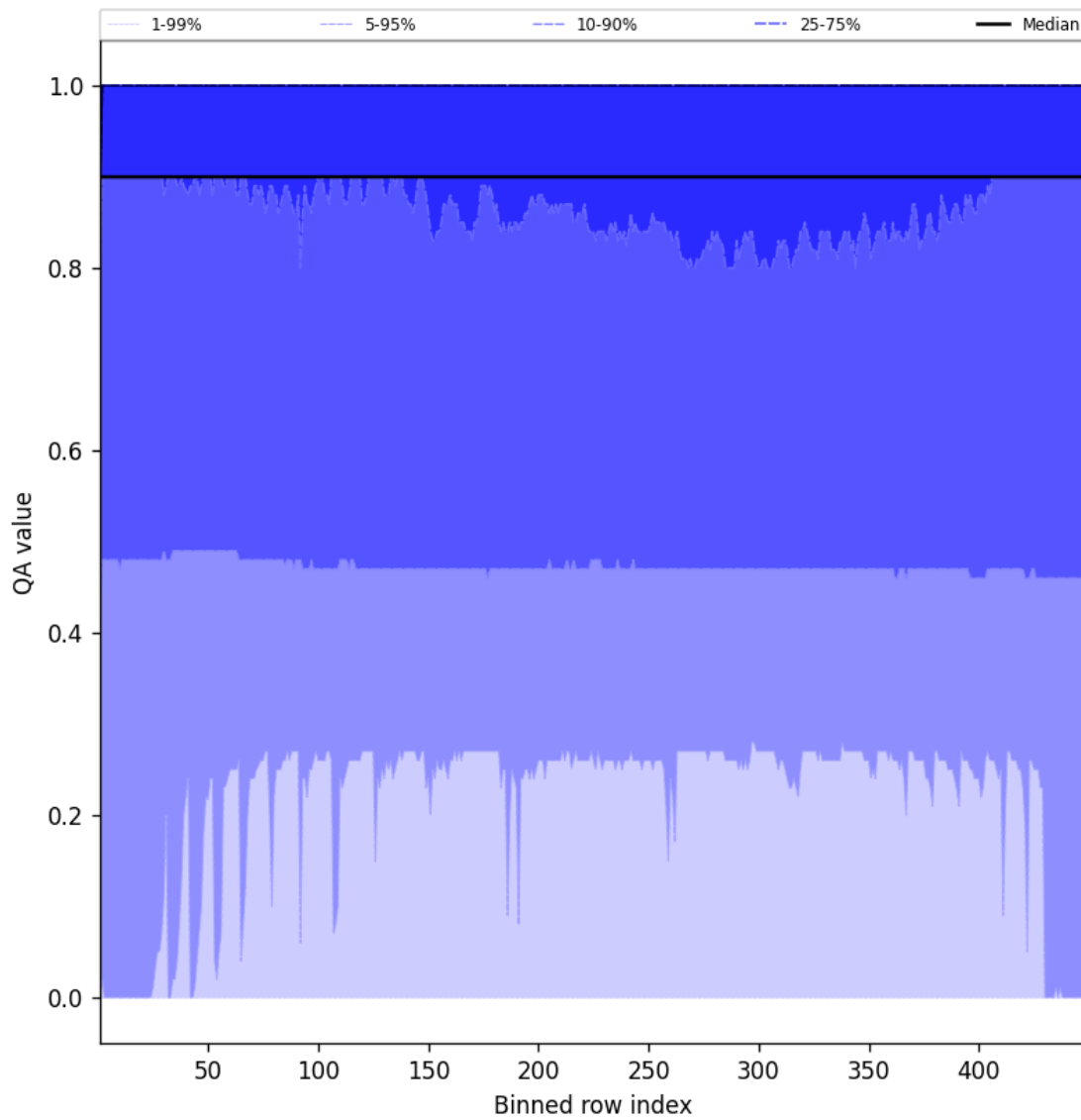
Figure 40: Along track statistics of “QA value” for 2025-07-24 to 2025-07-25
