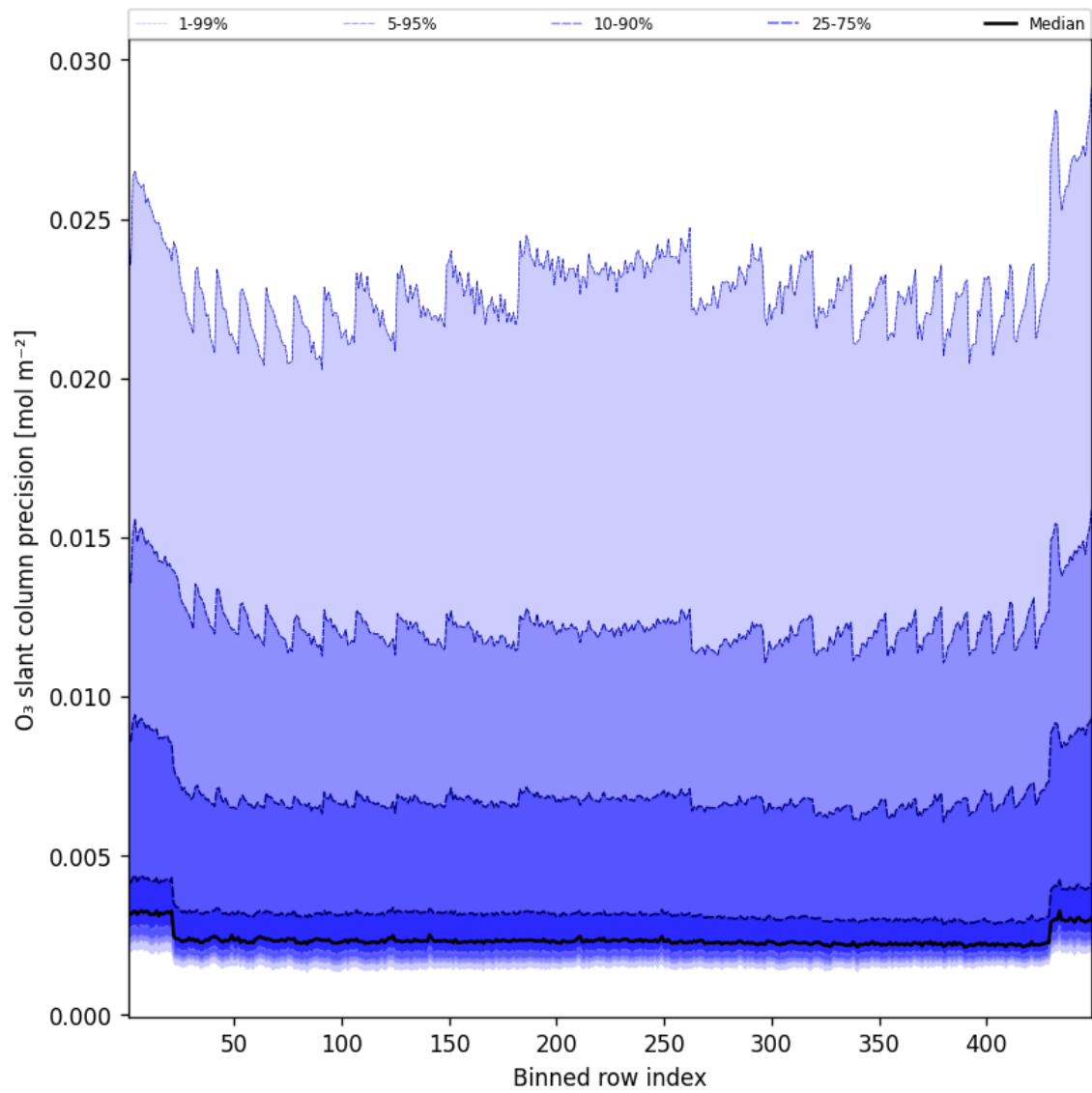
Figure 44: Along track statistics of “O 3 slant column precision” for 2025-07-24 to 2025-07-25
