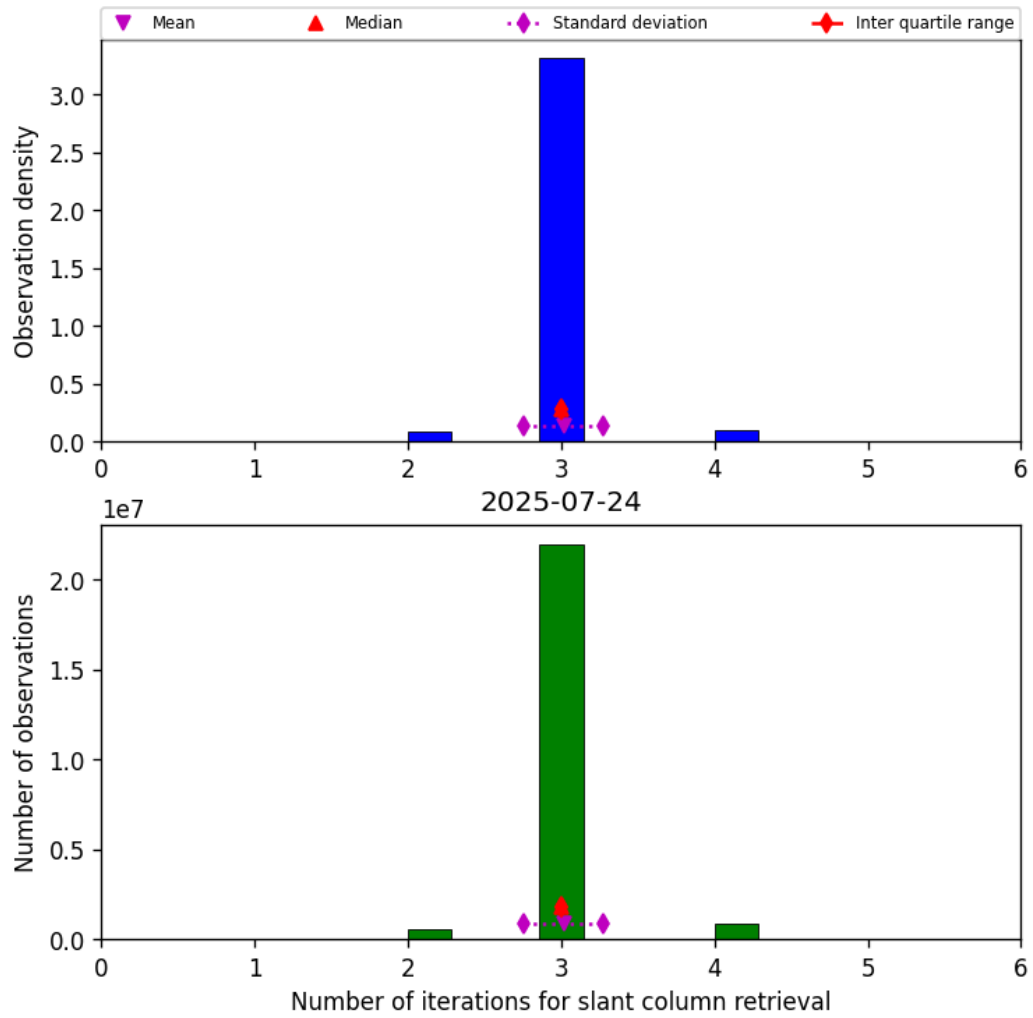
Figure 33: Histogram of “Number of iterations for slant column retrieval” for 2025-07-24 to 2025-07-25
