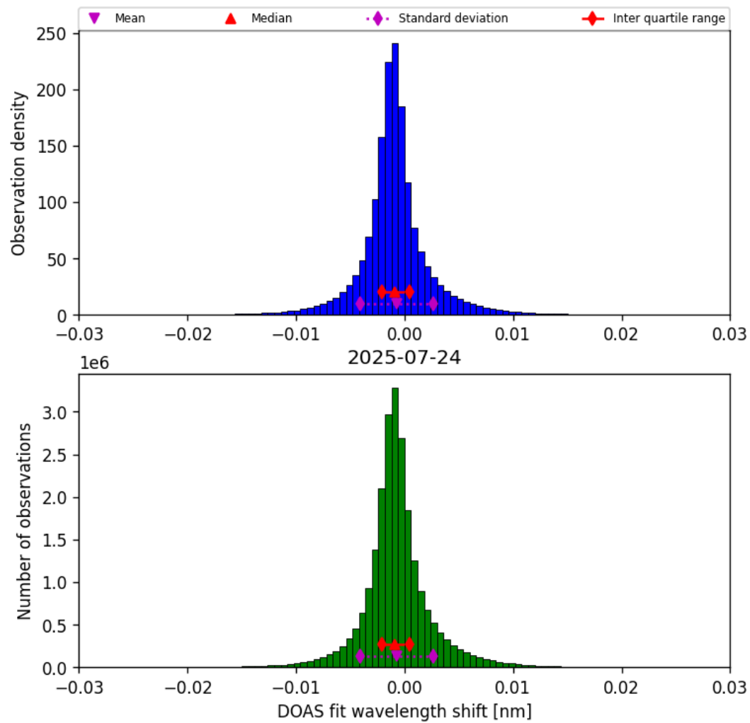
Figure 35: Histogram of “DOAS fit wavelength shift” for 2025-07-24 to 2025-07-25
