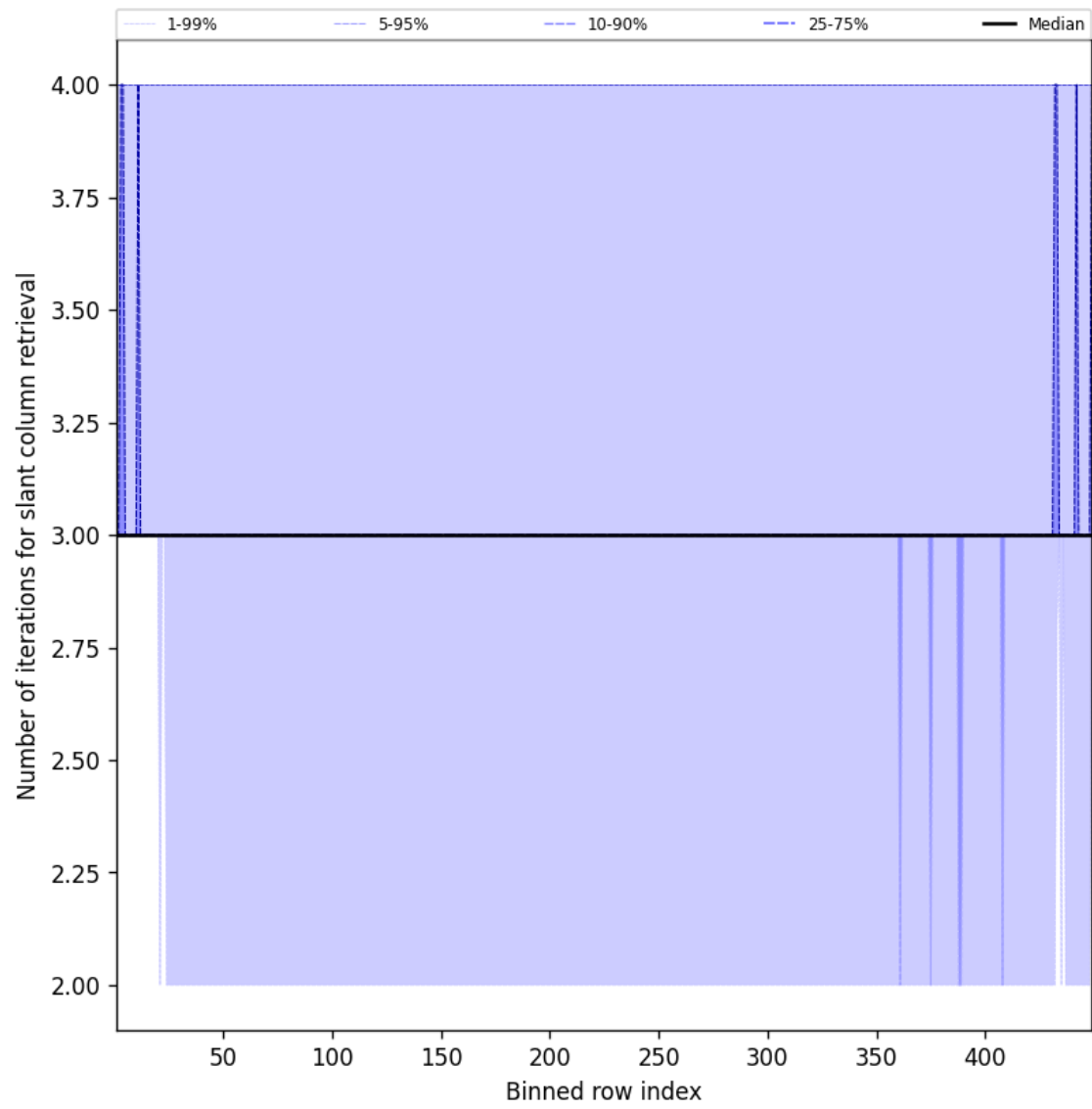
Figure 45: Along track statistics of “Number of iterations for slant column retrieval” for 2025-07-24 to 2025-07-25
