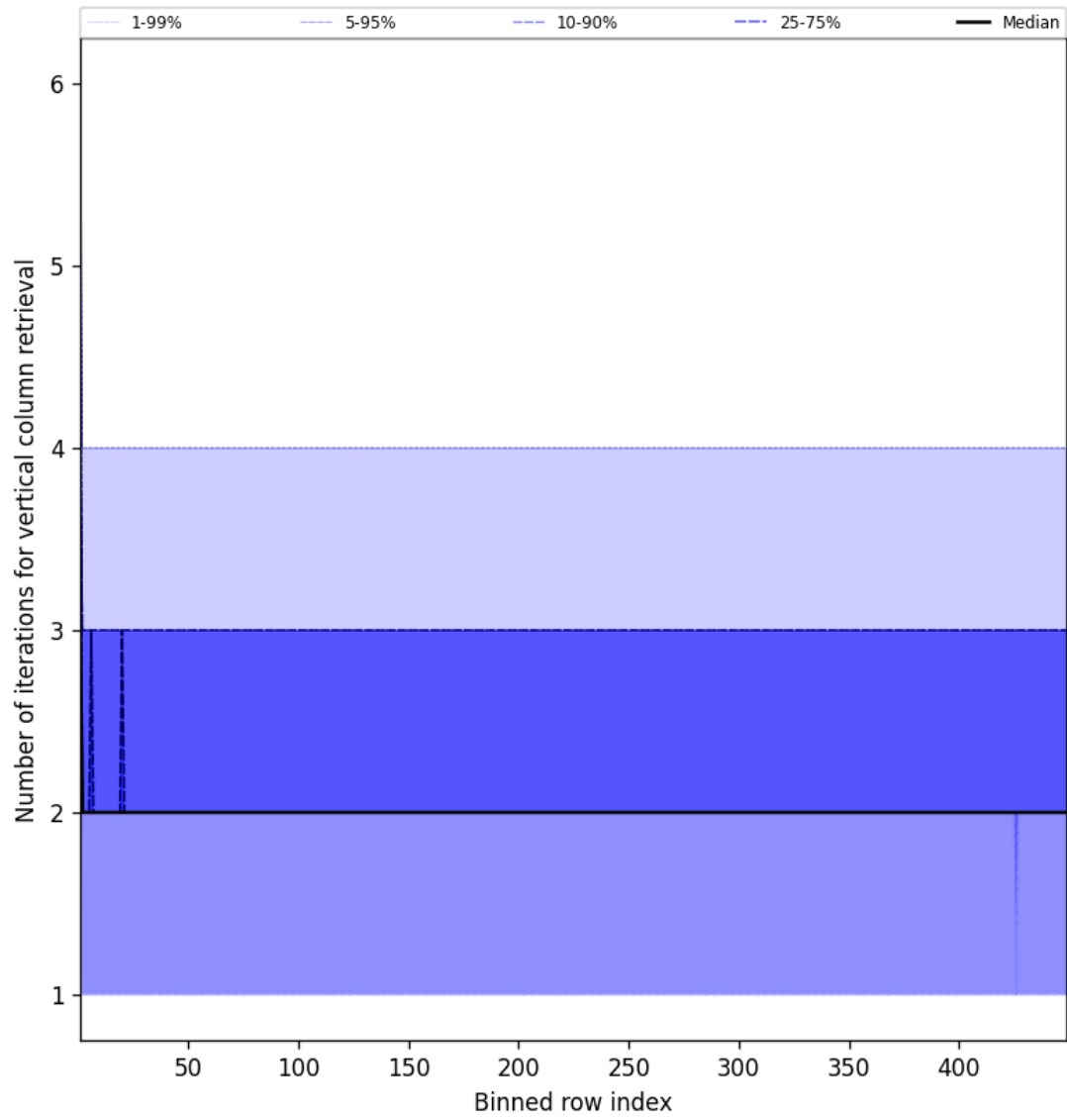
Figure 51: Along track statistics of “Number of iterations for vertical column retrieval” for 2025-07-24 to 2025-07-25
