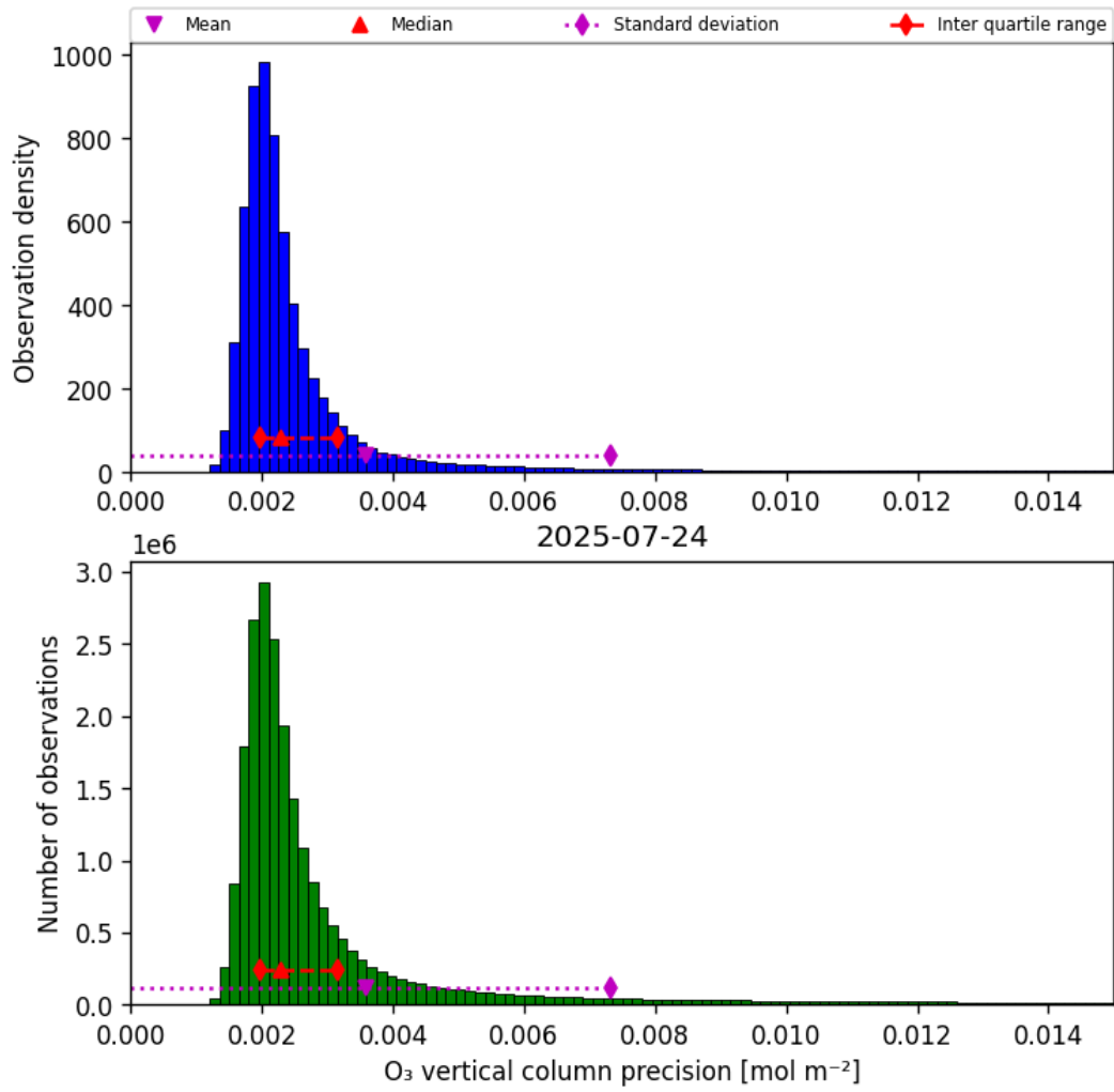
Figure 30: Histogram of “O 3 vertical column precision” for 2025-07-24 to 2025-07-25
