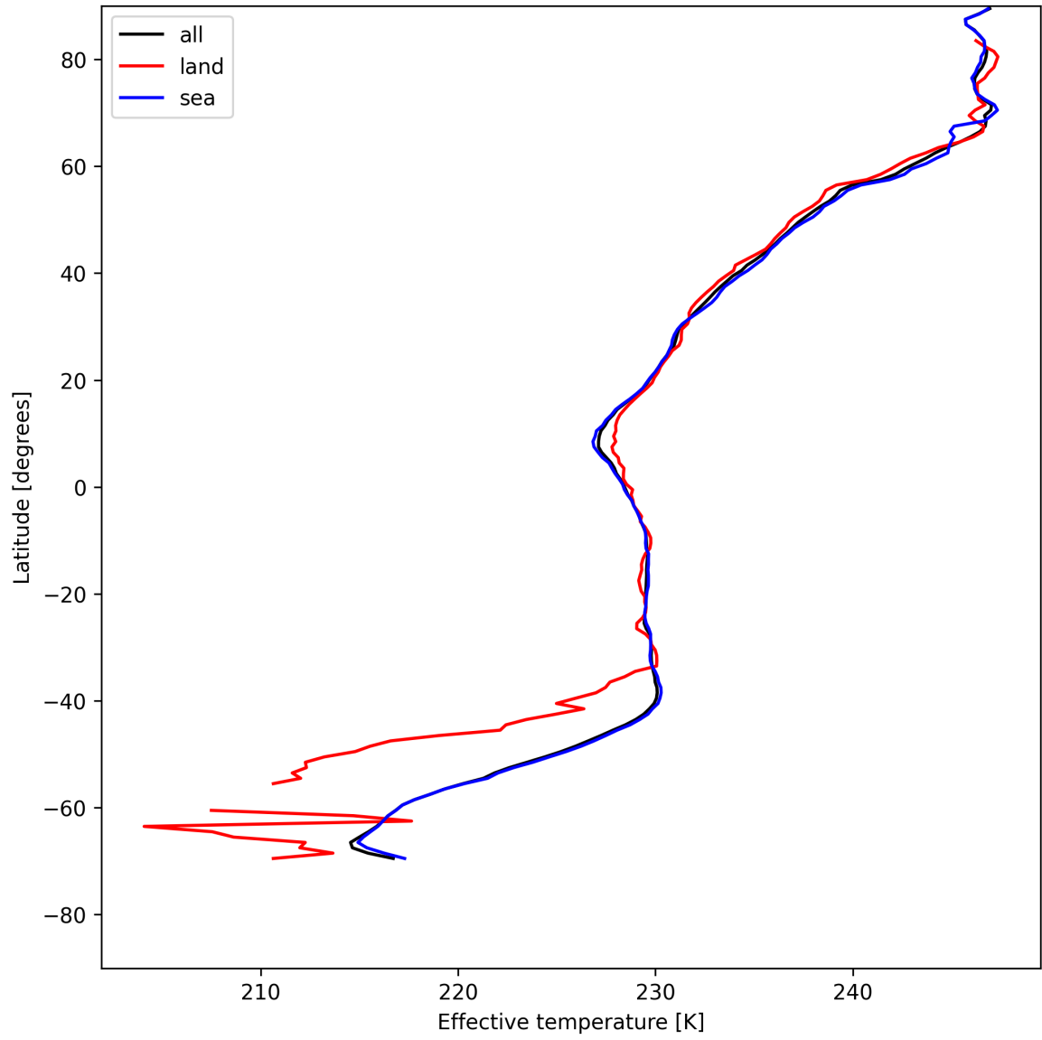
Figure 26: Zonal average of “Effective temperature” for 2025-07-24 to 2025-07-25.
