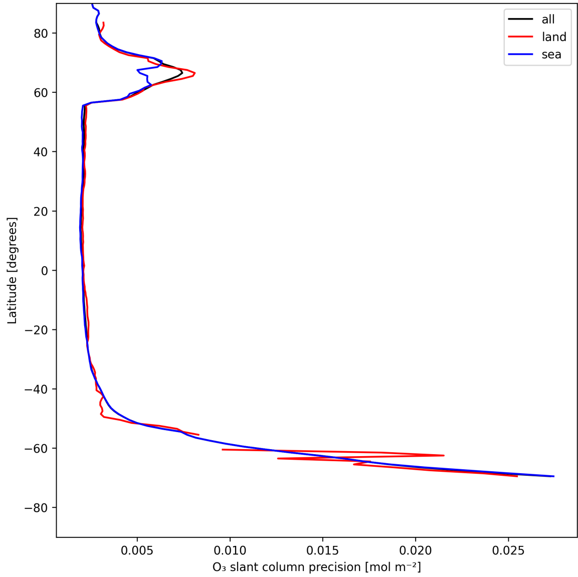
Figure 20: Zonal average of "O 3 slant column precision" for 2025-07-24 to 2025-07-25.
