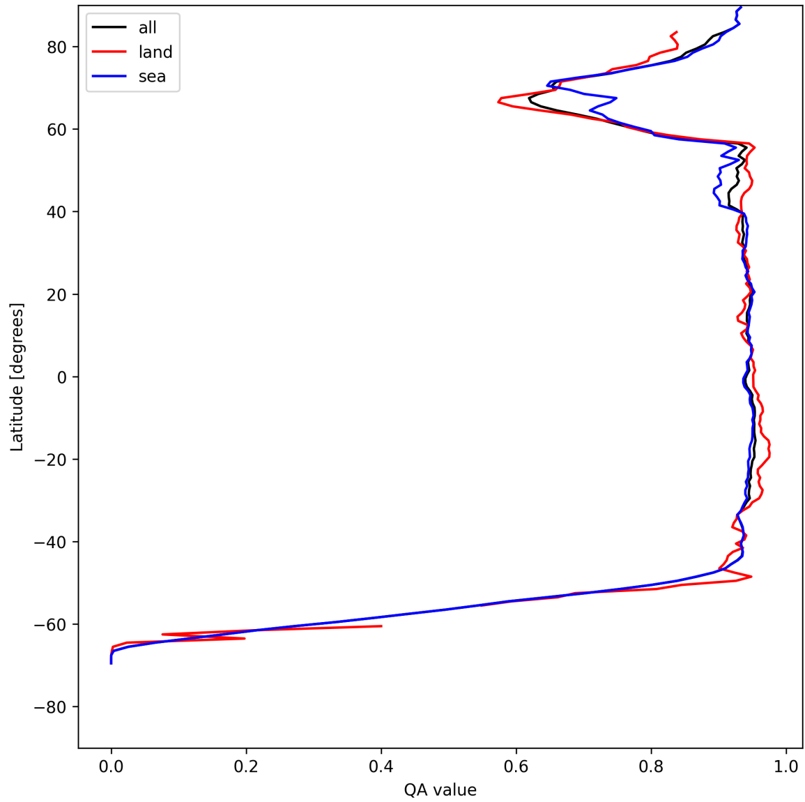
Figure 16: Zonal average of “QA value” for 2025-07-24 to 2025-07-25.
