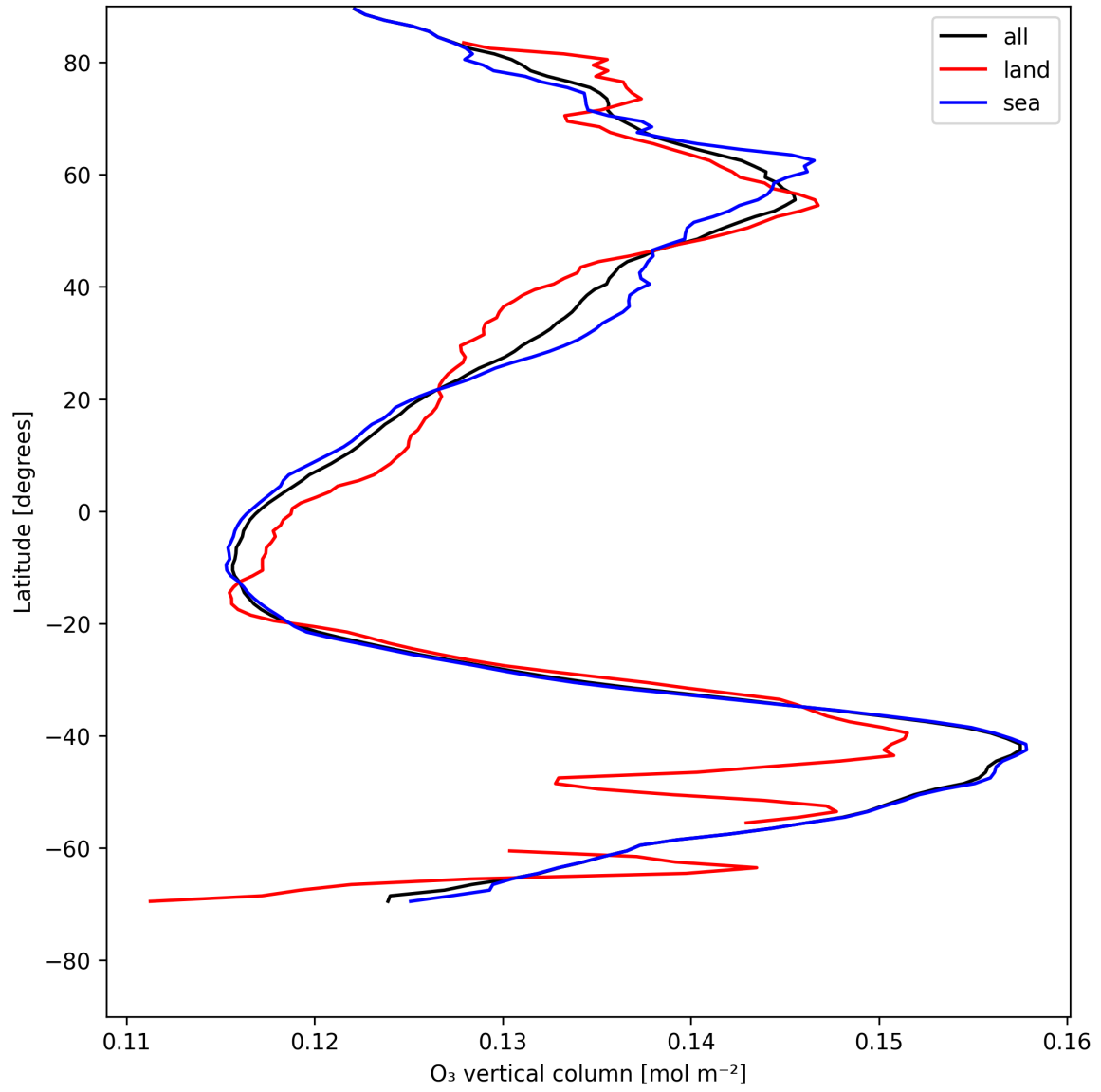
Figure 17: Zonal average of “O 3 vertical column” for 2025-07-24 to 2025-07-25.
