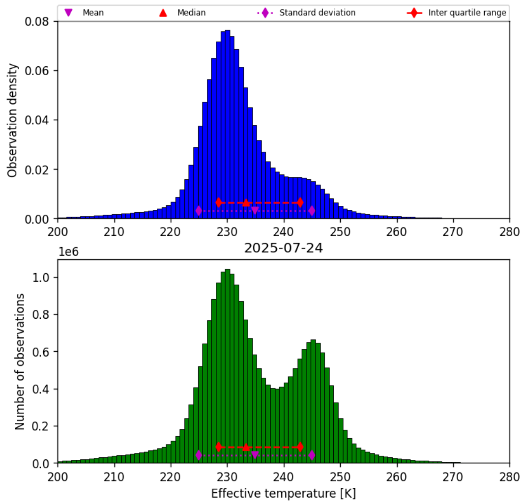
Figure 38: Histogram of “Effective temperature” for 2025-07-24 to 2025-07-25
