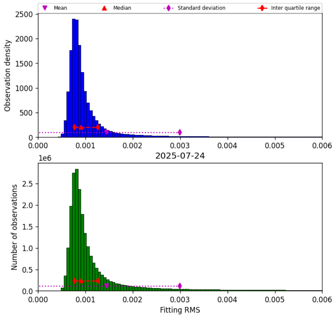
Figure 34: Histogram of “Fitting RMS” for 2025-07-24 to 2025-07-25
