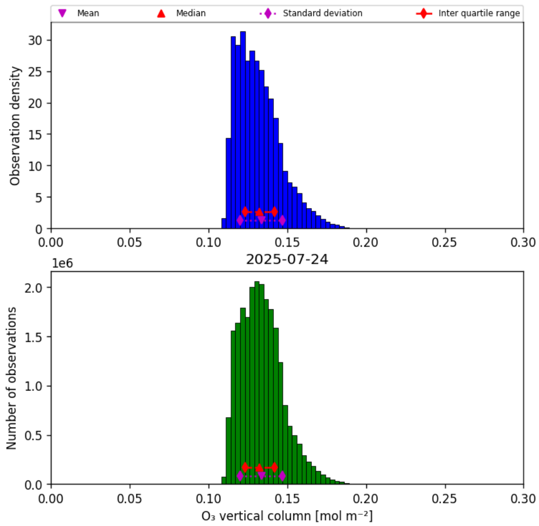
Figure 29: Histogram of “O 3 vertical column” for 2025-07-24 to 2025-07-25
