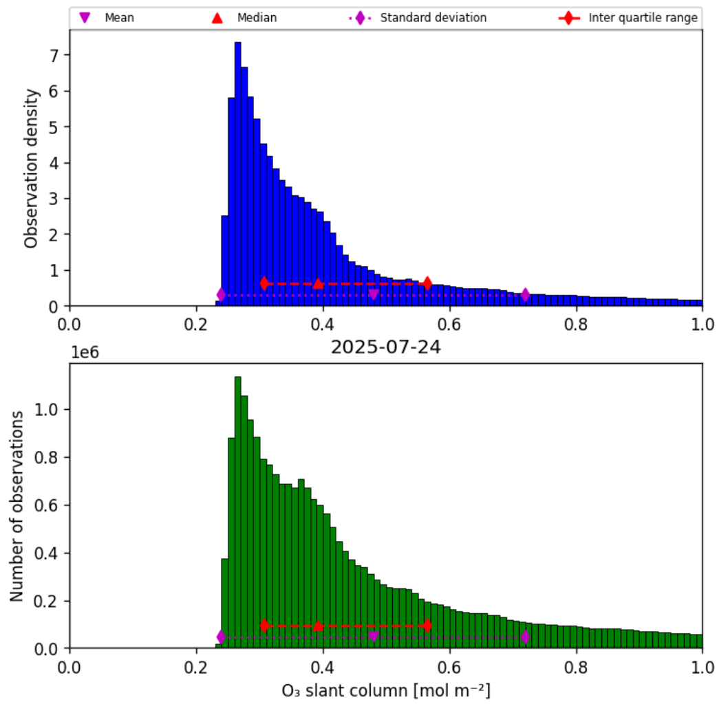
Figure 31: Histogram of “O 3 slant column” for 2025-07-24 to 2025-07-25
