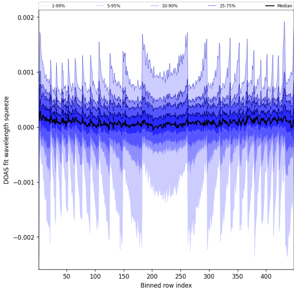
Figure 48: Along track statistics of “DOAS fit wavelength squeeze” for 2025-07-24 to 2025-07-25
