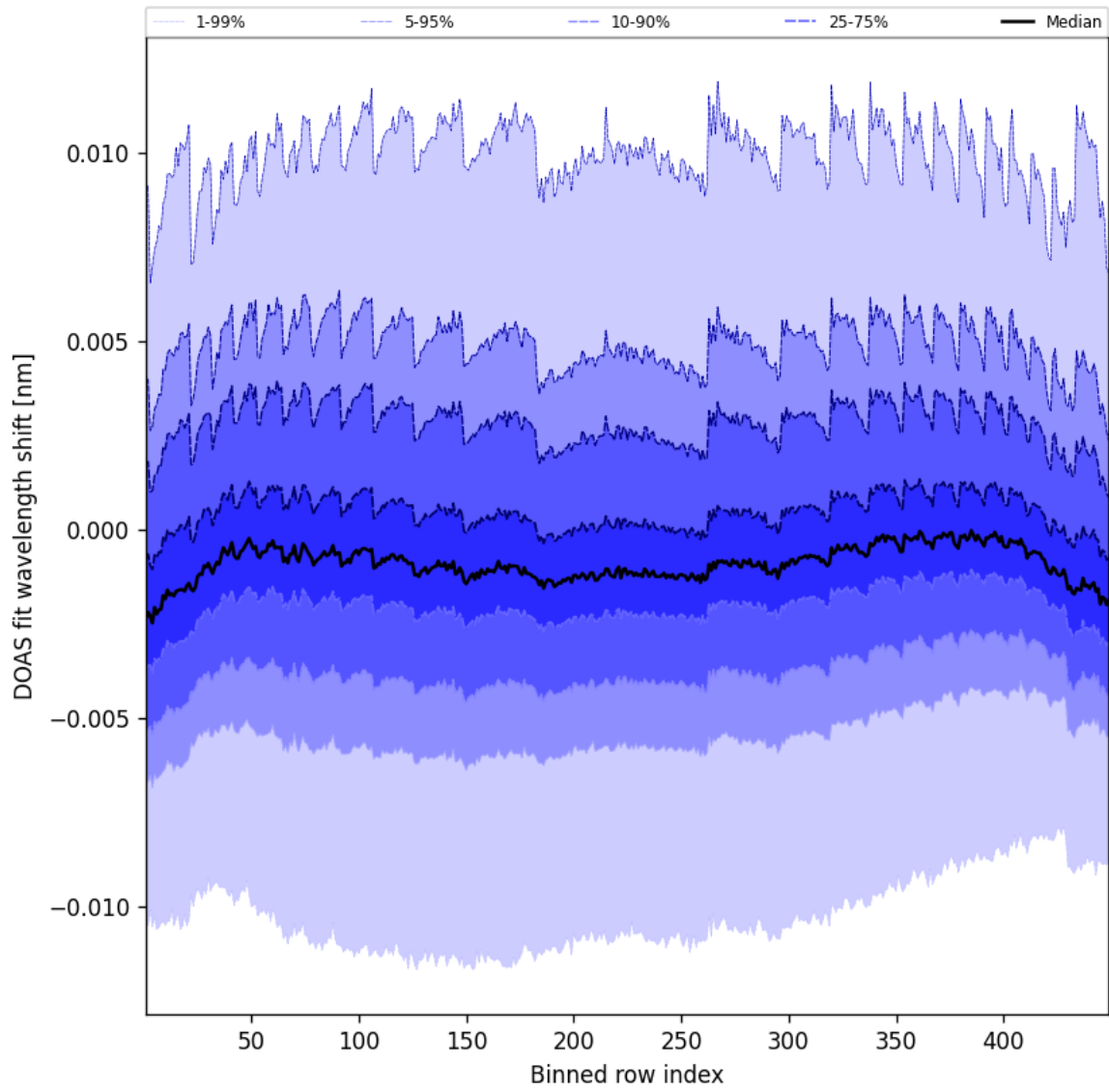
Figure 47: Along track statistics of “DOAS fit wavelength shift” for 2025-07-24 to 2025-07-25
