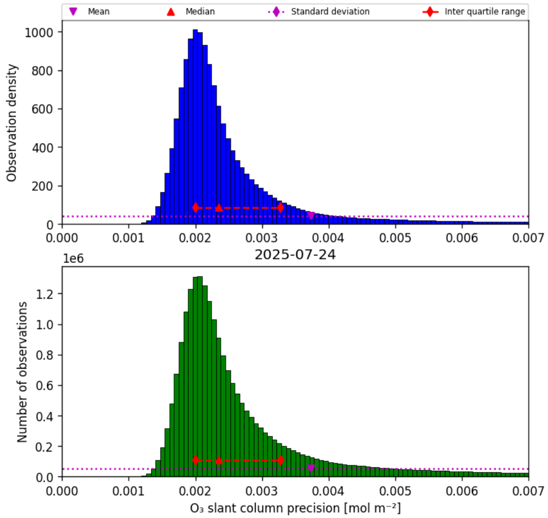
Figure 32: Histogram of “O 3 slant column precision” for 2025-07-24 to 2025-07-25
