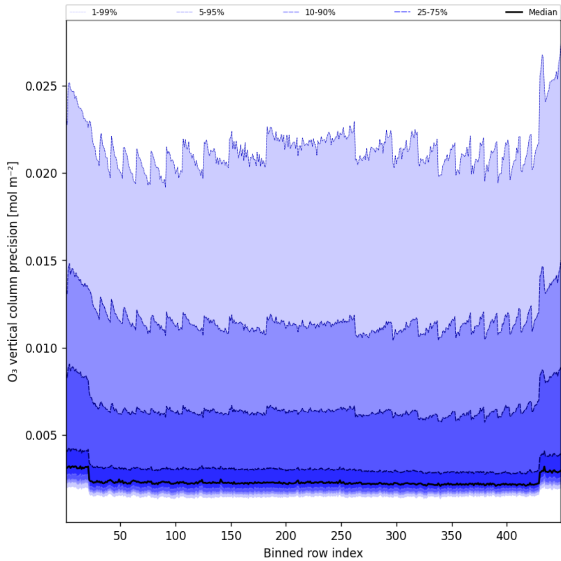
Figure 42: Along track statistics of “O 3 vertical column precision” for 2025-07-24 to 2025-07-25
