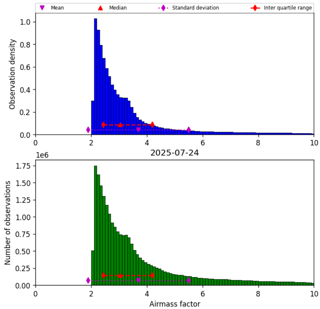
Figure 37: Histogram of “Airmass factor” for 2025-07-24 to 2025-07-25
