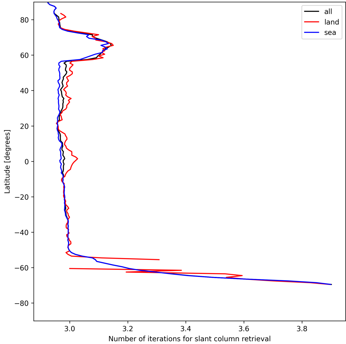
Figure 21: Zonal average of “Number of iterations for slant column retrieval” for 2025-07-25 to 2025-07-26.
