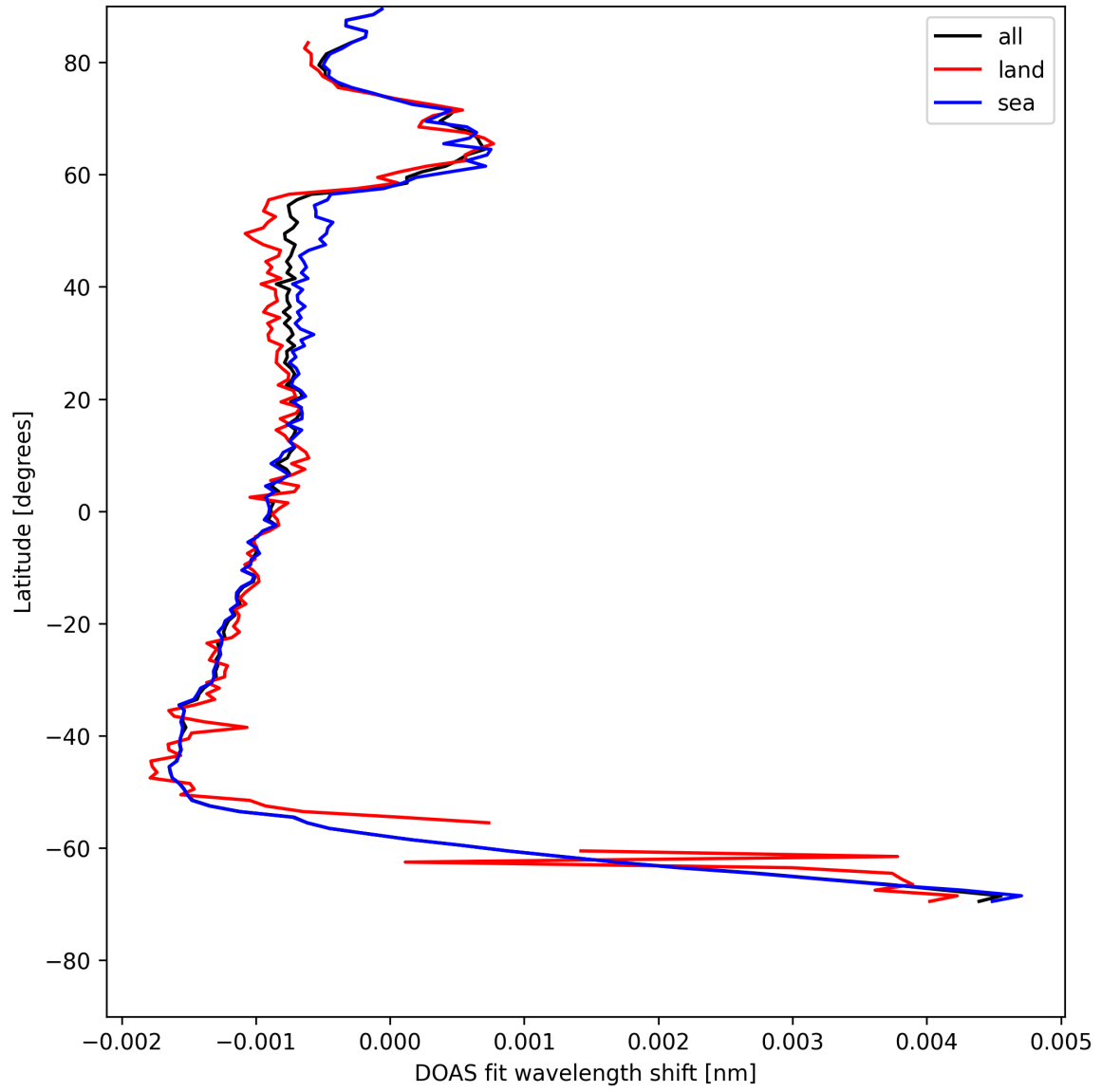
Figure 23: Zonal average of “DOAS fit wavelength shift” for 2025-07-25 to 2025-07-26.
