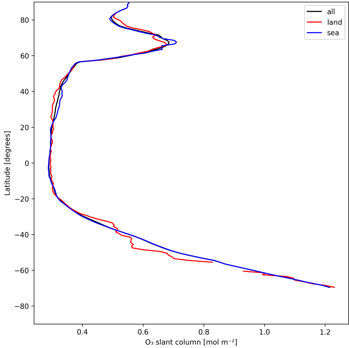
Figure 19: Zonal average of “O 3 slant column” for 2025-07-25 to 2025-07-26.
