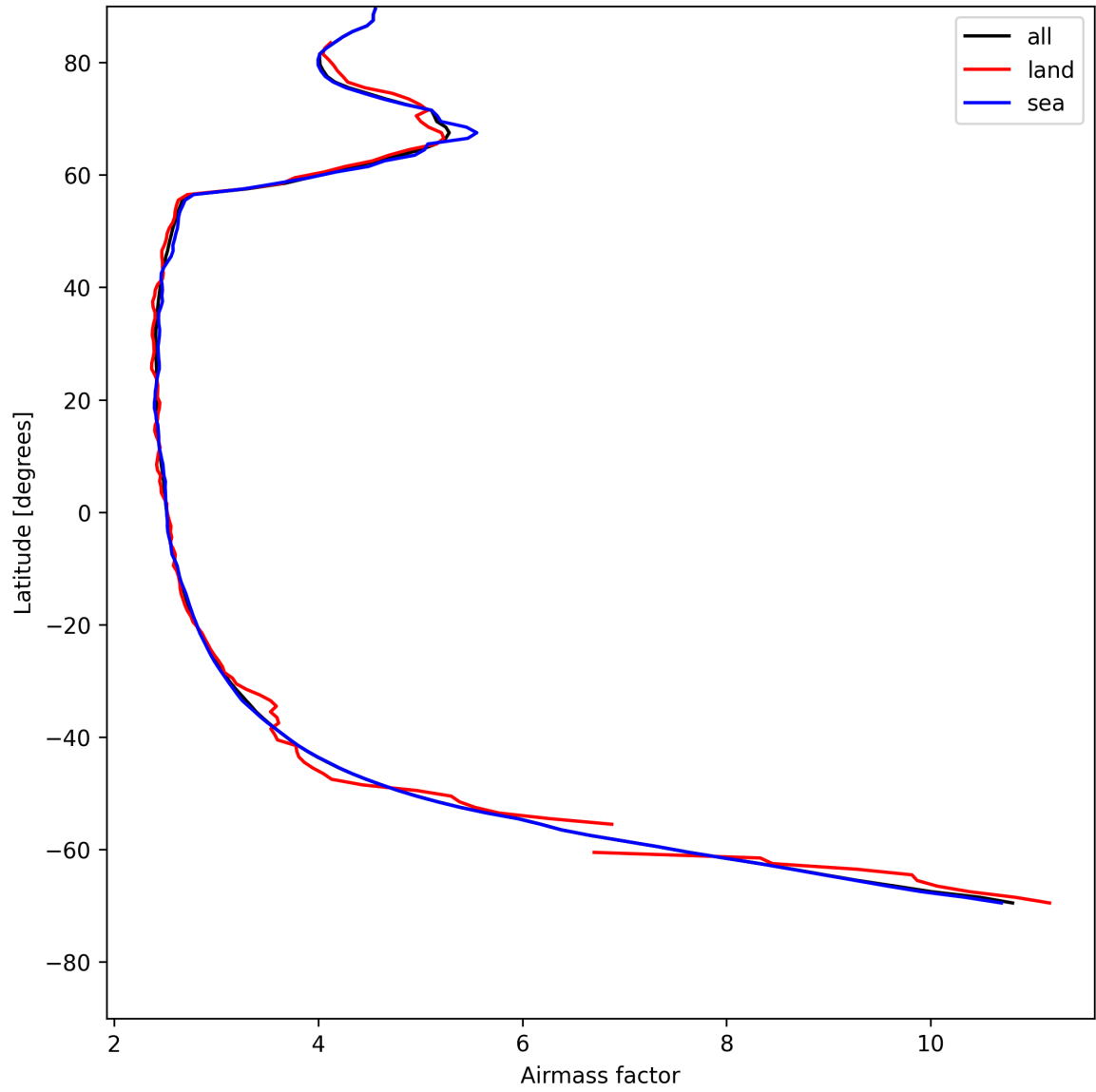
Figure 25: Zonal average of “Airmass factor” for 2025-07-25 to 2025-07-26.
