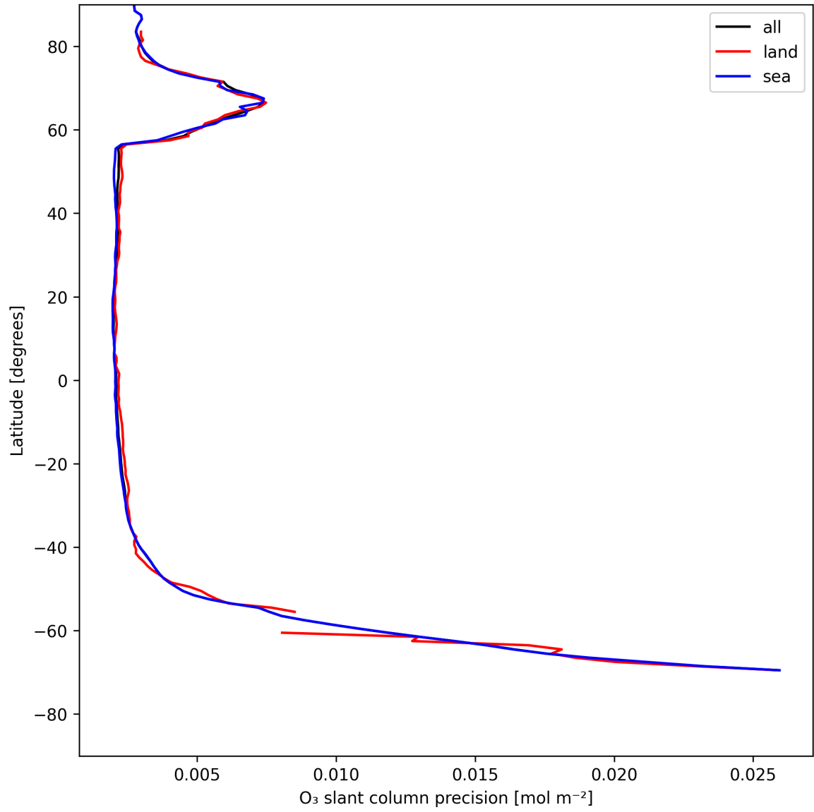
Figure 20: Zonal average of “O 3 slant column precision” for 2025-07-25 to 2025-07-26.
