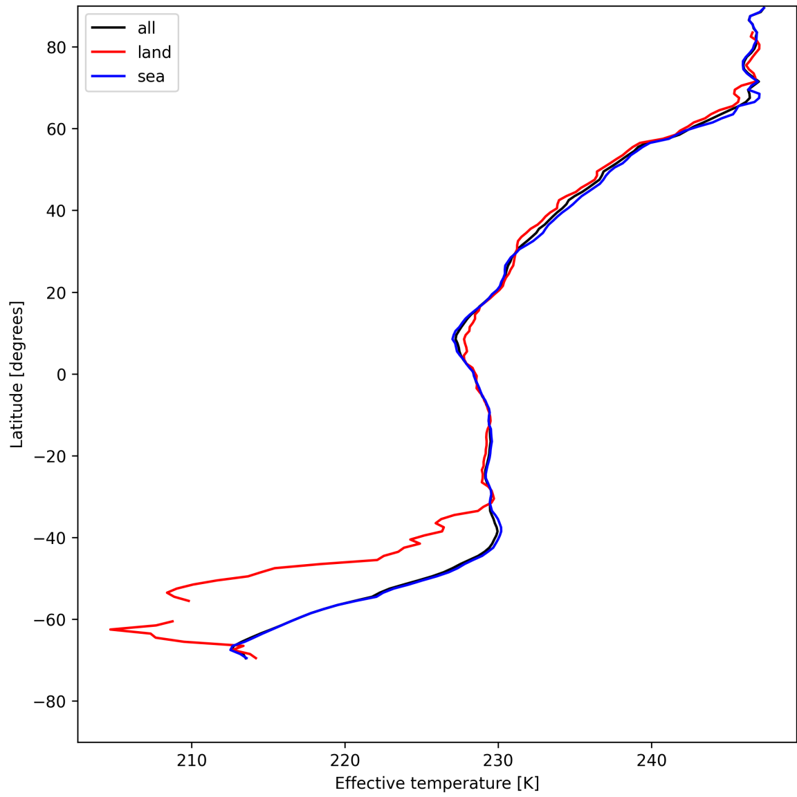
Figure 26: Zonal average of “Effective temperature” for 2025-07-25 to 2025-07-26.
