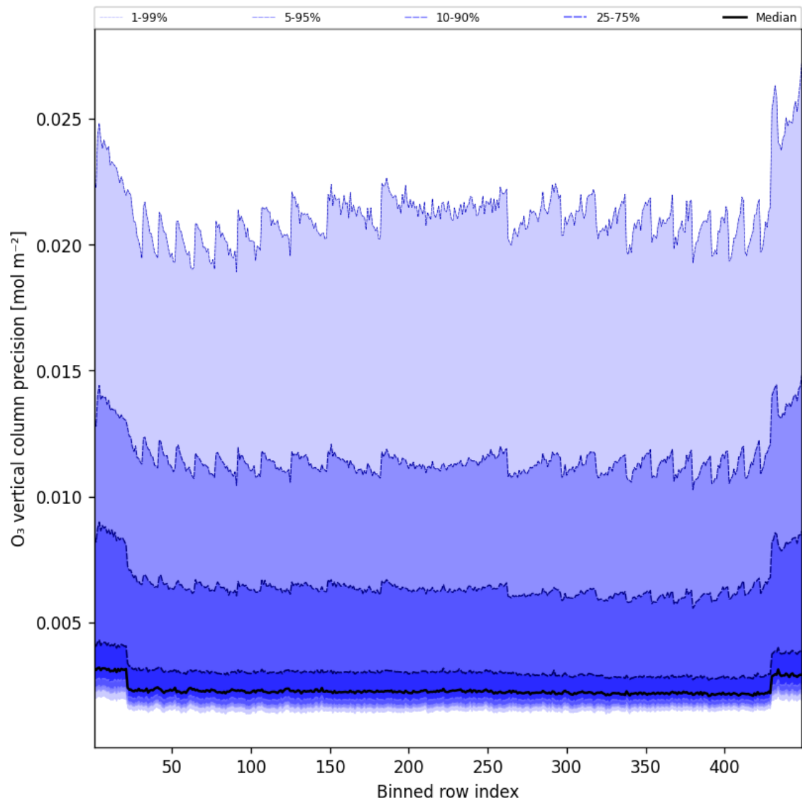
Figure 42: Along track statistics of “O 3 vertical column precision” for 2025-07-25 to 2025-07-26
