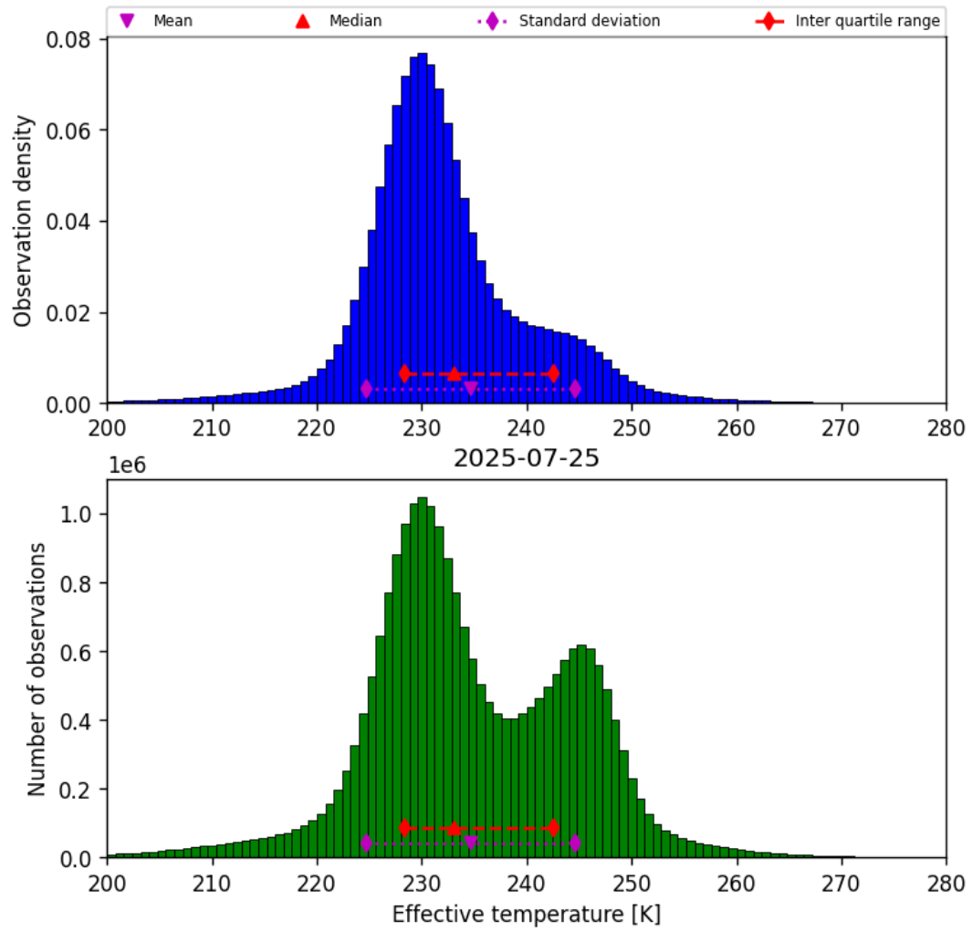
Figure 38: Histogram of “Effective temperature” for 2025-07-25 to 2025-07-26
