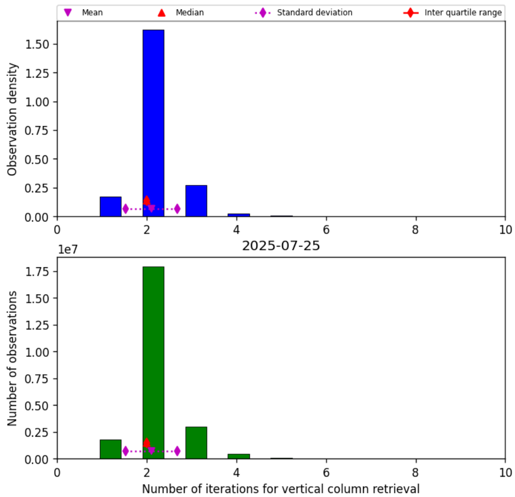
Figure 39: Histogram of “Number of iterations for vertical column retrieval” for 2025-07-25 to 2025-07-26
