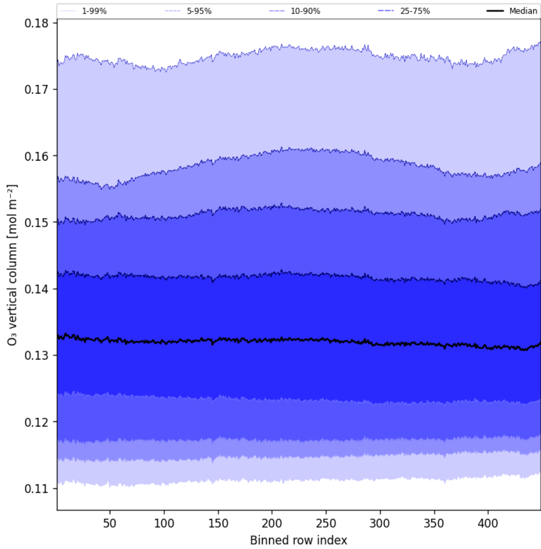
Figure 41: Along track statistics of “O 3 vertical column” for 2025-07-25 to 2025-07-26
