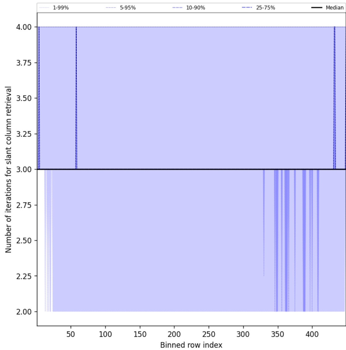
Figure 45: Along track statistics of “Number of iterations for slant column retrieval” for 2025-07-25 to 2025-07-26
