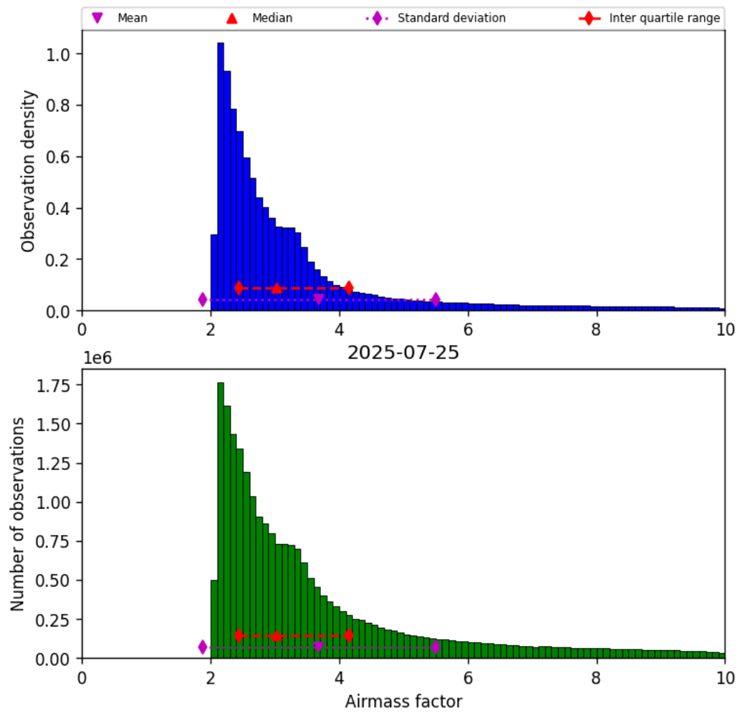
Figure 37: Histogram of “Airmass factor” for 2025-07-25 to 2025-07-26
