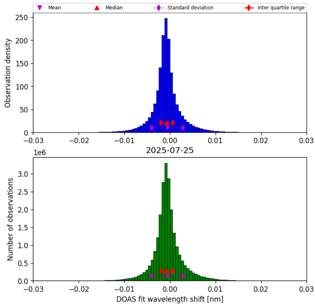
Figure 35: Histogram of “DOAS fit wavelength shift” for 2025-07-25 to 2025-07-26
