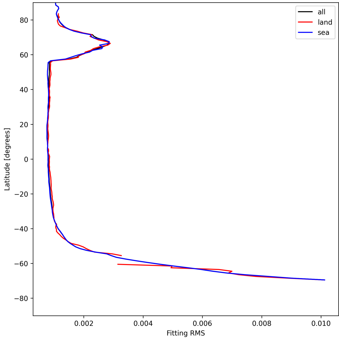
Figure 22: Zonal average of “Fitting RMS” for 2025-07-25 to 2025-07-26.
