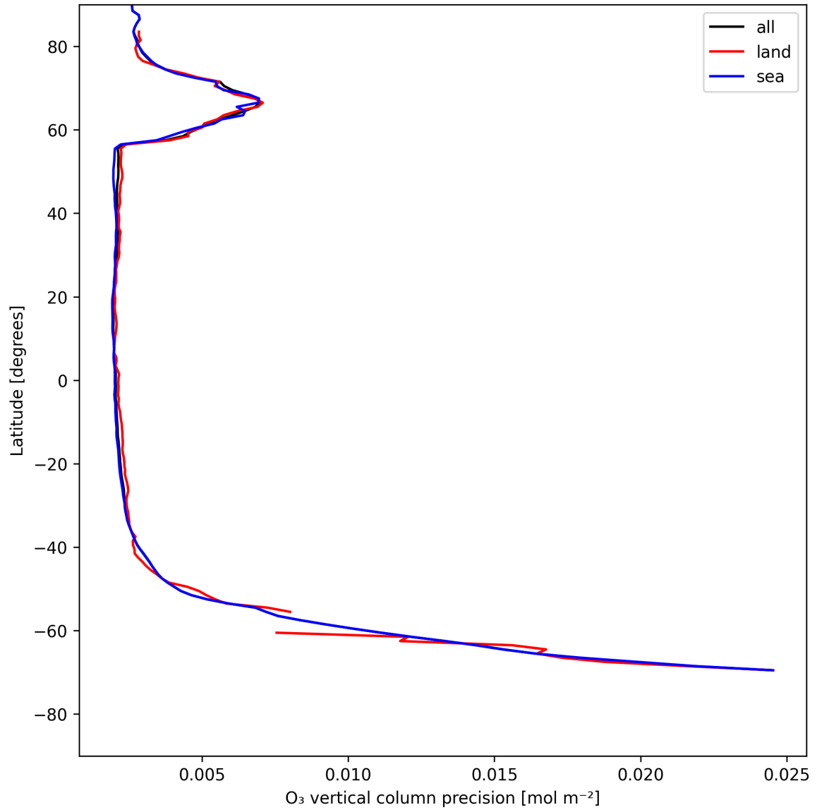
Figure 18: Zonal average of “O 3 vertical column precision” for 2025-07-25 to 2025-07-26.
