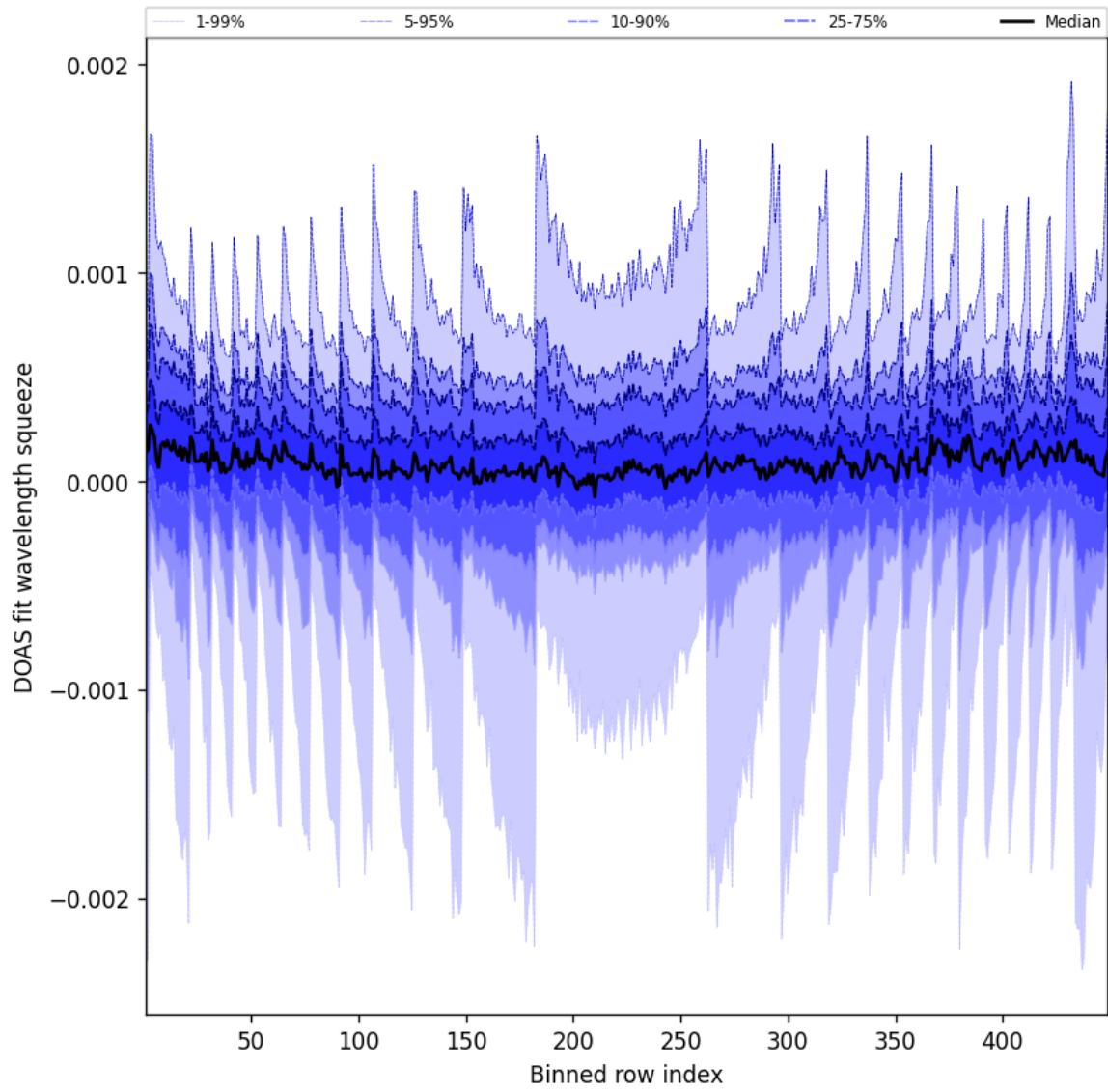
Figure 48: Along track statistics of “DOAS fit wavelength squeeze” for 2025-07-25 to 2025-07-26
