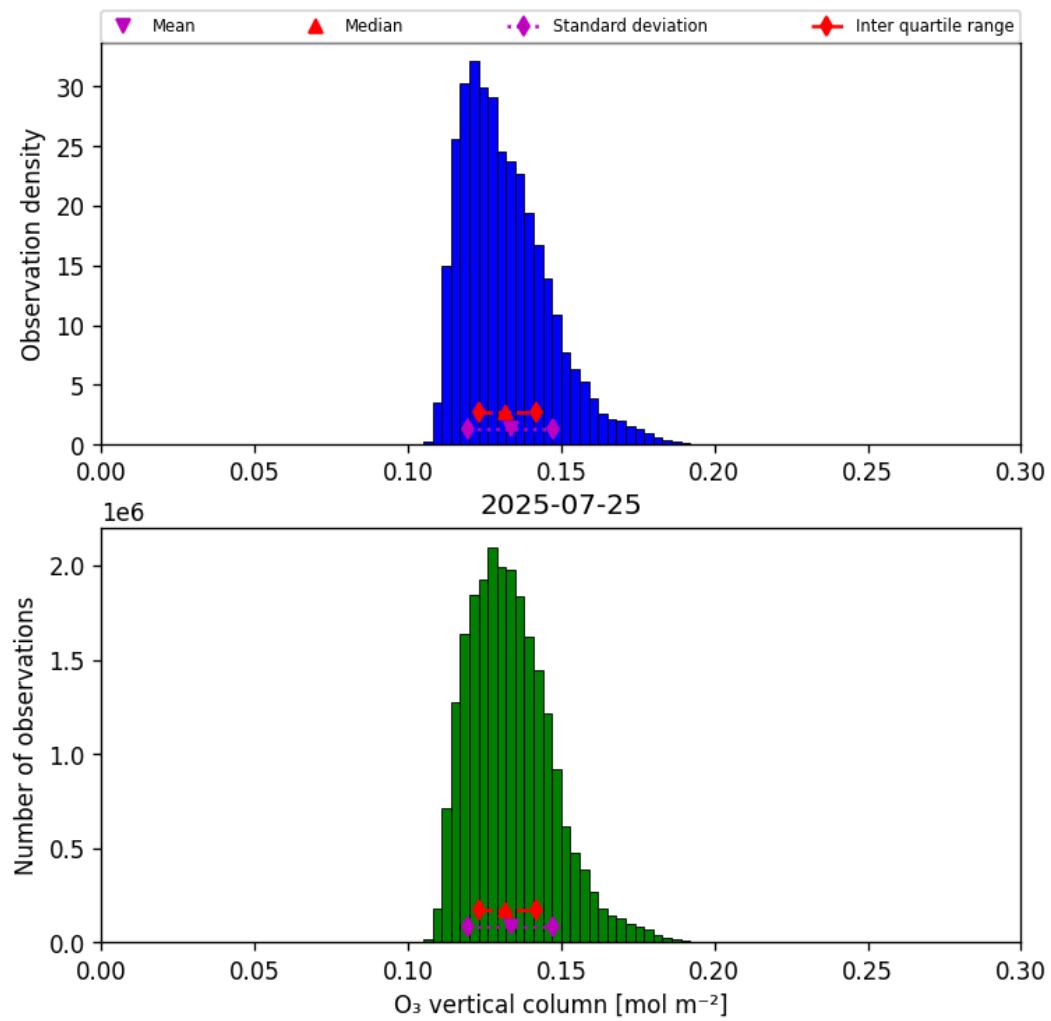
Figure 29: Histogram of “O 3 vertical column” for 2025-07-25 to 2025-07-26
