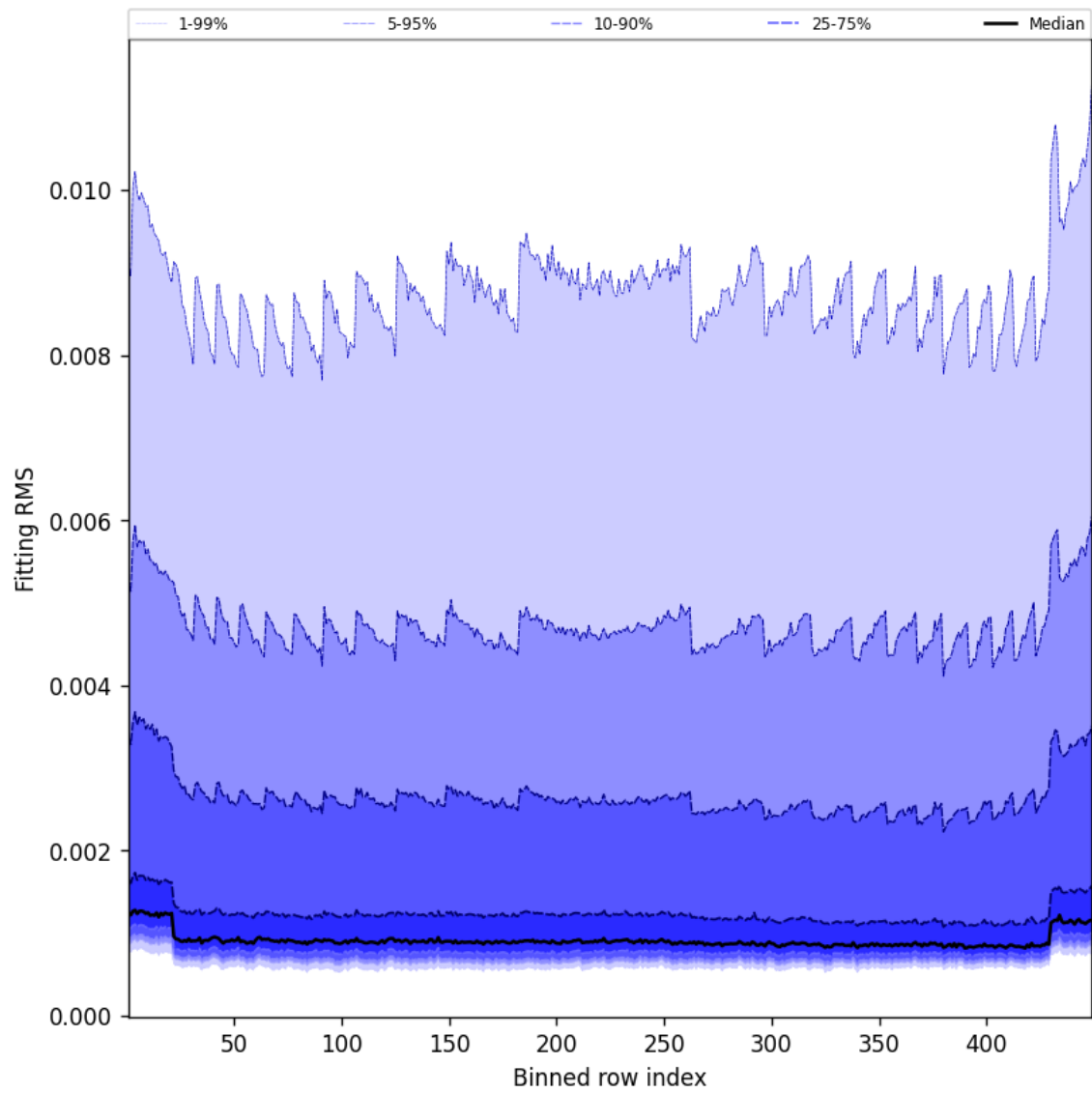
Figure 46: Along track statistics of “Fitting RMS” for 2025-07-25 to 2025-07-26
