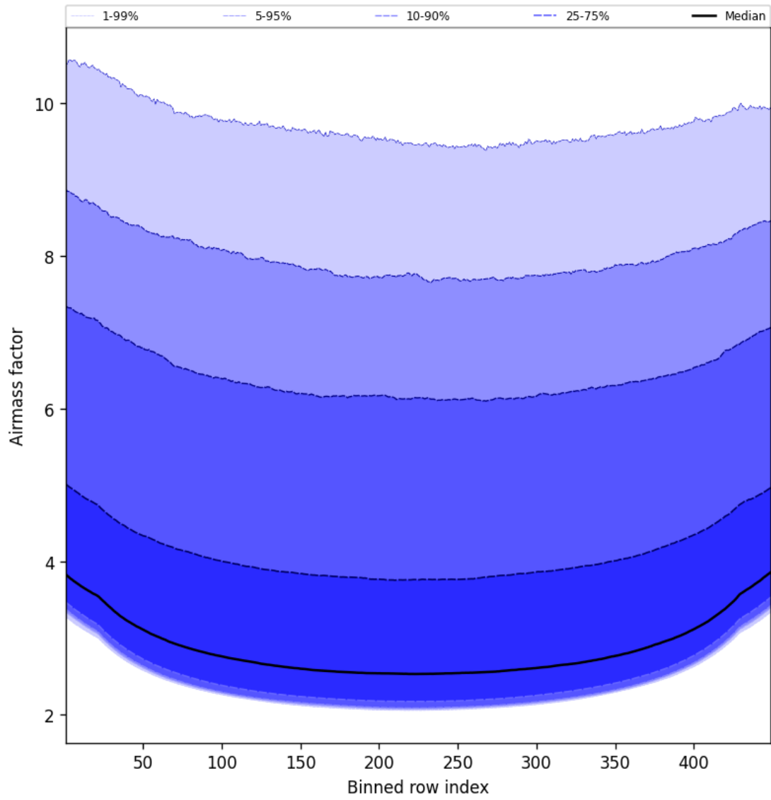
Figure 49: Along track statistics of “Airmass factor” for 2025-07-25 to 2025-07-26
