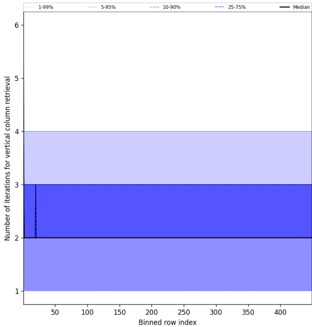
Figure 51: Along track statistics of “Number of iterations for vertical column retrieval” for 2025-07-25 to 2025-07-26
