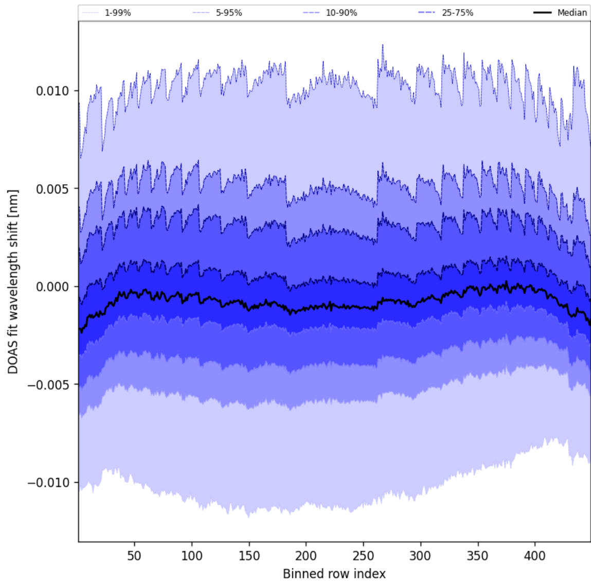
Figure 47: Along track statistics of “DOAS fit wavelength shift” for 2025-07-25 to 2025-07-26
