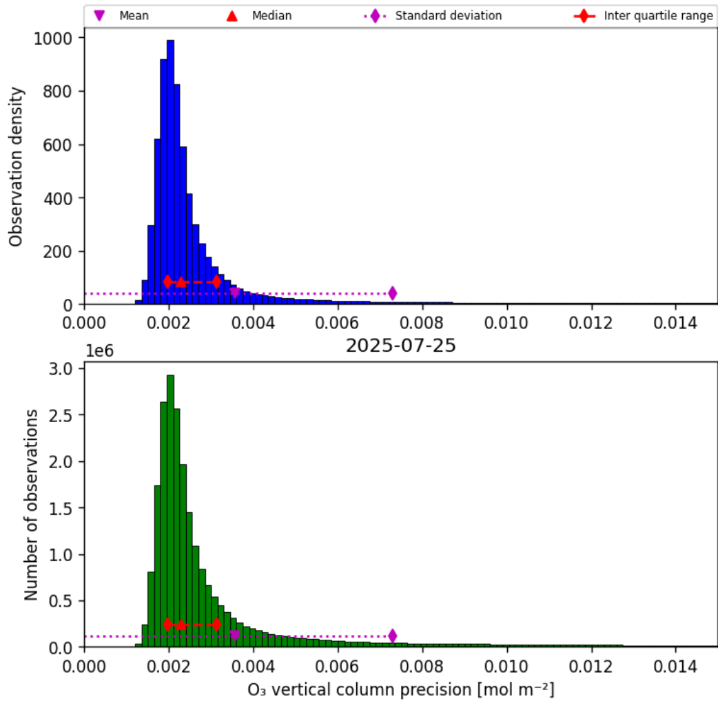
Figure 30: Histogram of “O 3 vertical column precision” for 2025-07-25 to 2025-07-26
