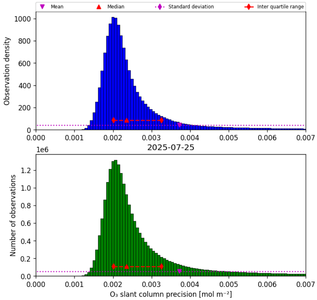
Figure 32: Histogram of “O 3 slant column precision” for 2025-07-25 to 2025-07-26
