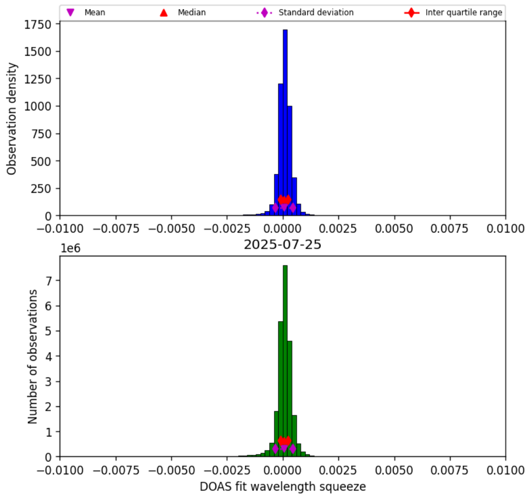
Figure 36: Histogram of “DOAS fit wavelength squeeze” for 2025-07-25 to 2025-07-26
