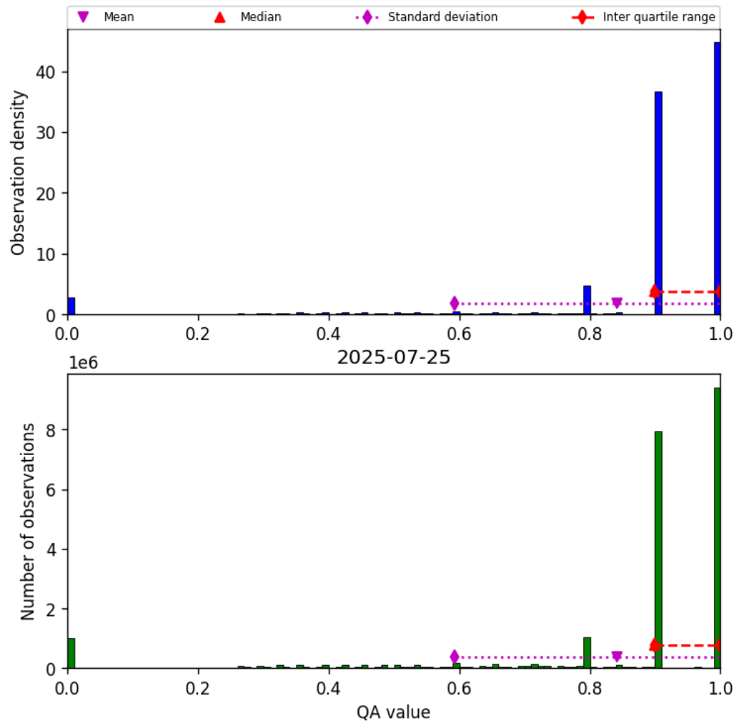
Figure 28: Histogram of “QA value” for 2025-07-25 to 2025-07-26
