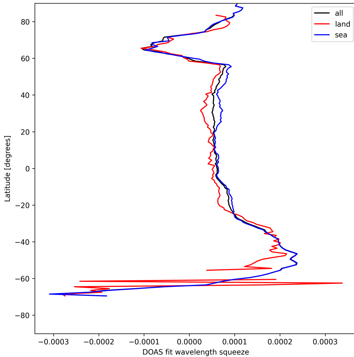
Figure 24: Zonal average of “DOAS fit wavelength squeeze” for 2025-07-25 to 2025-07-26.
