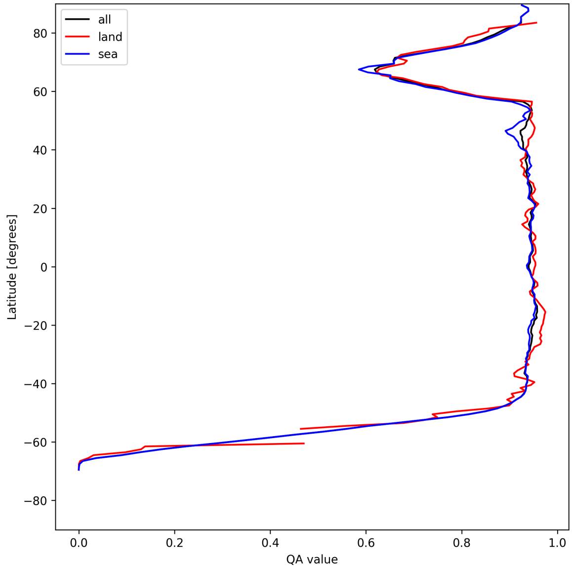
Figure 16: Zonal average of “QA value” for 2025-07-25 to 2025-07-26.
