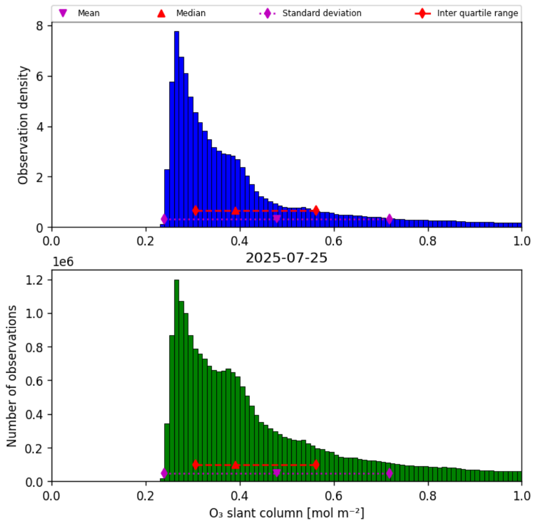
Figure 31: Histogram of “O 3 slant column” for 2025-07-25 to 2025-07-26
