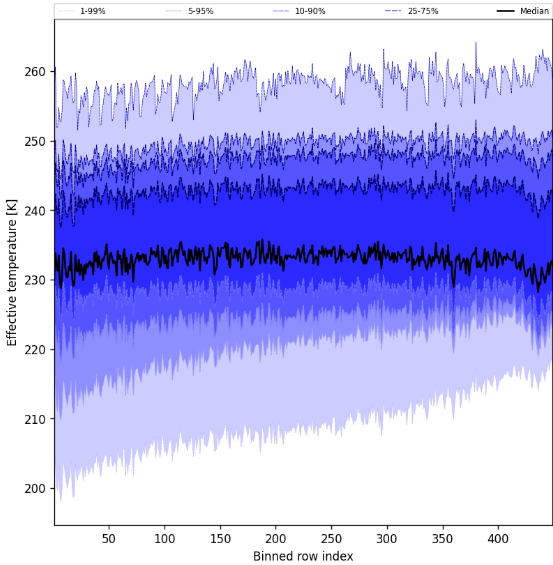
Figure 50: Along track statistics of “Effective temperature” for 2025-07-25 to 2025-07-26
