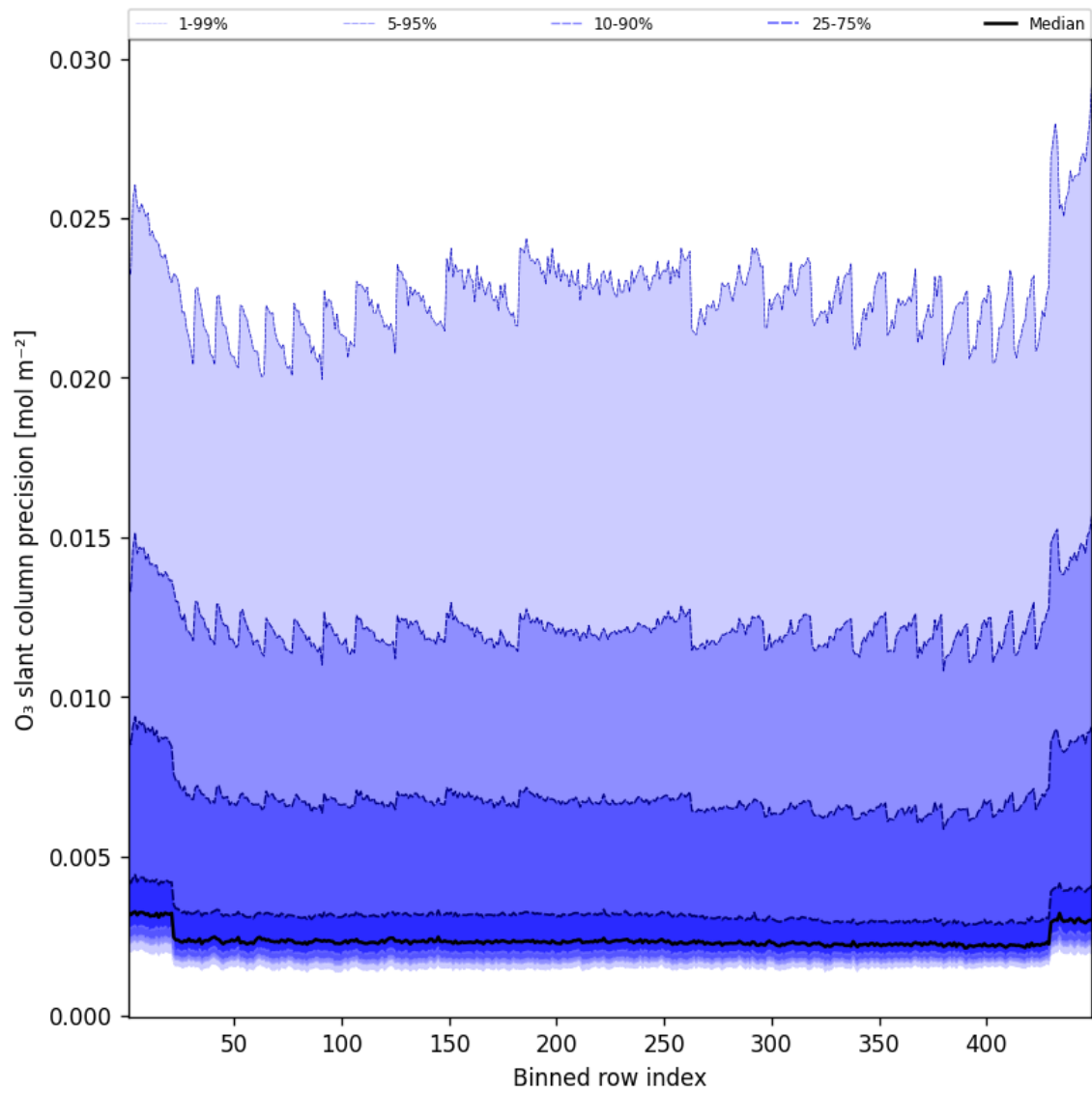
Figure 44: Along track statistics of “O 3 slant column precision” for 2025-07-25 to 2025-07-26
