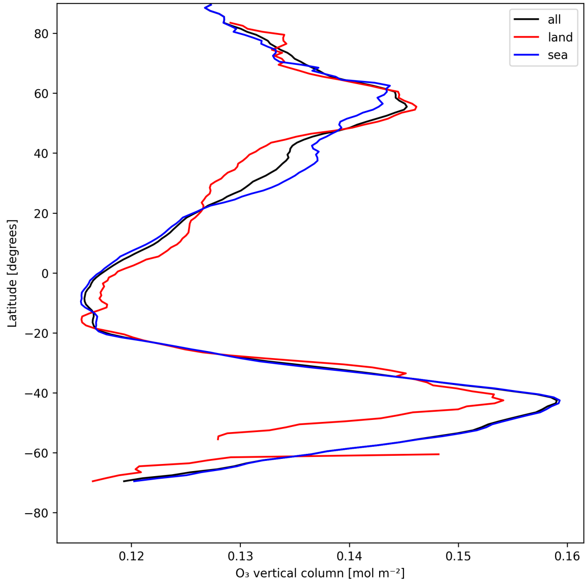
Figure 17: Zonal average of “O 3 vertical column” for 2025-07-25 to 2025-07-26.
