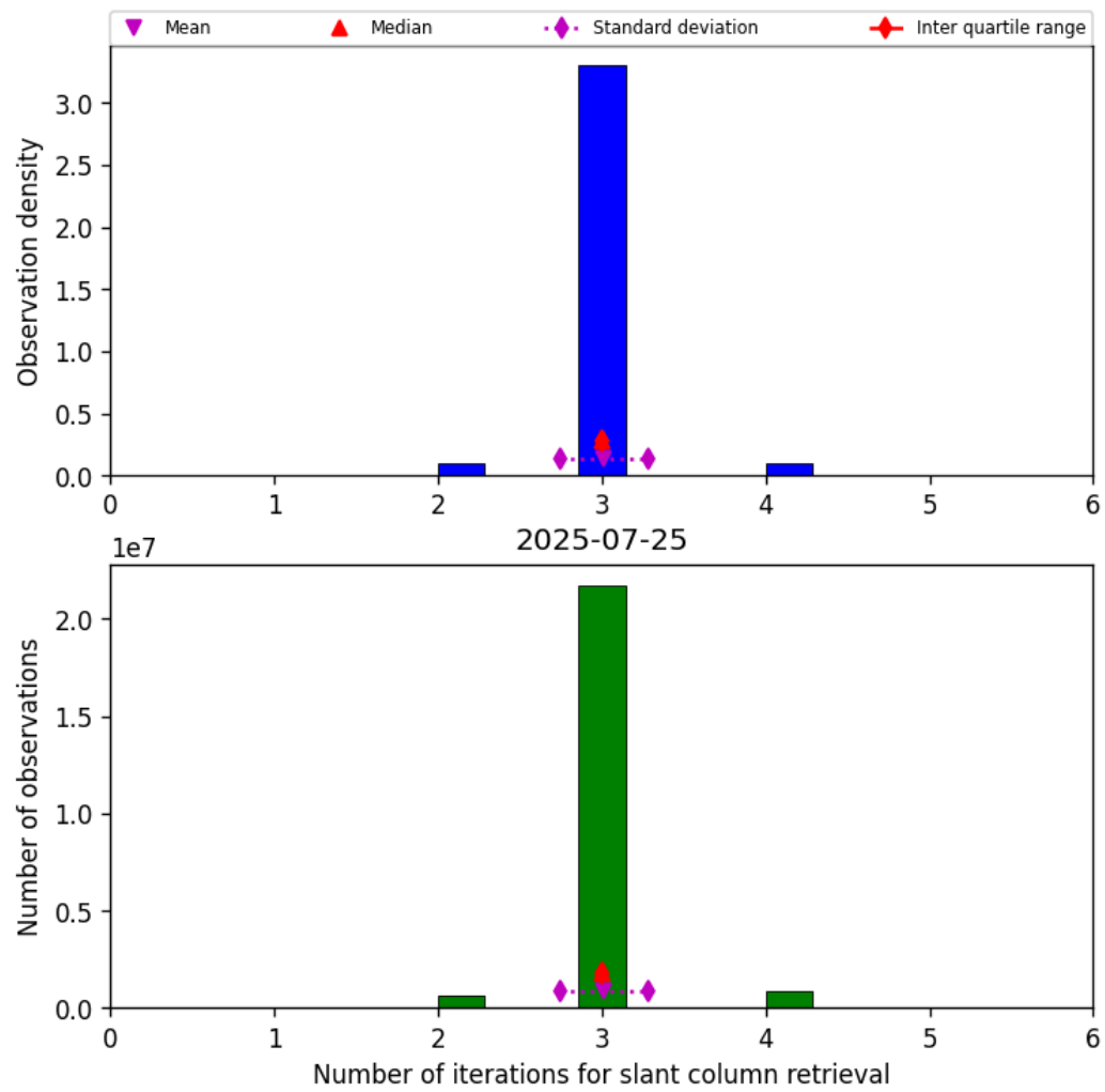
Figure 33: Histogram of "Number of iterations for slant column retrieval" for 2025-07-25 to 2025-07-26
