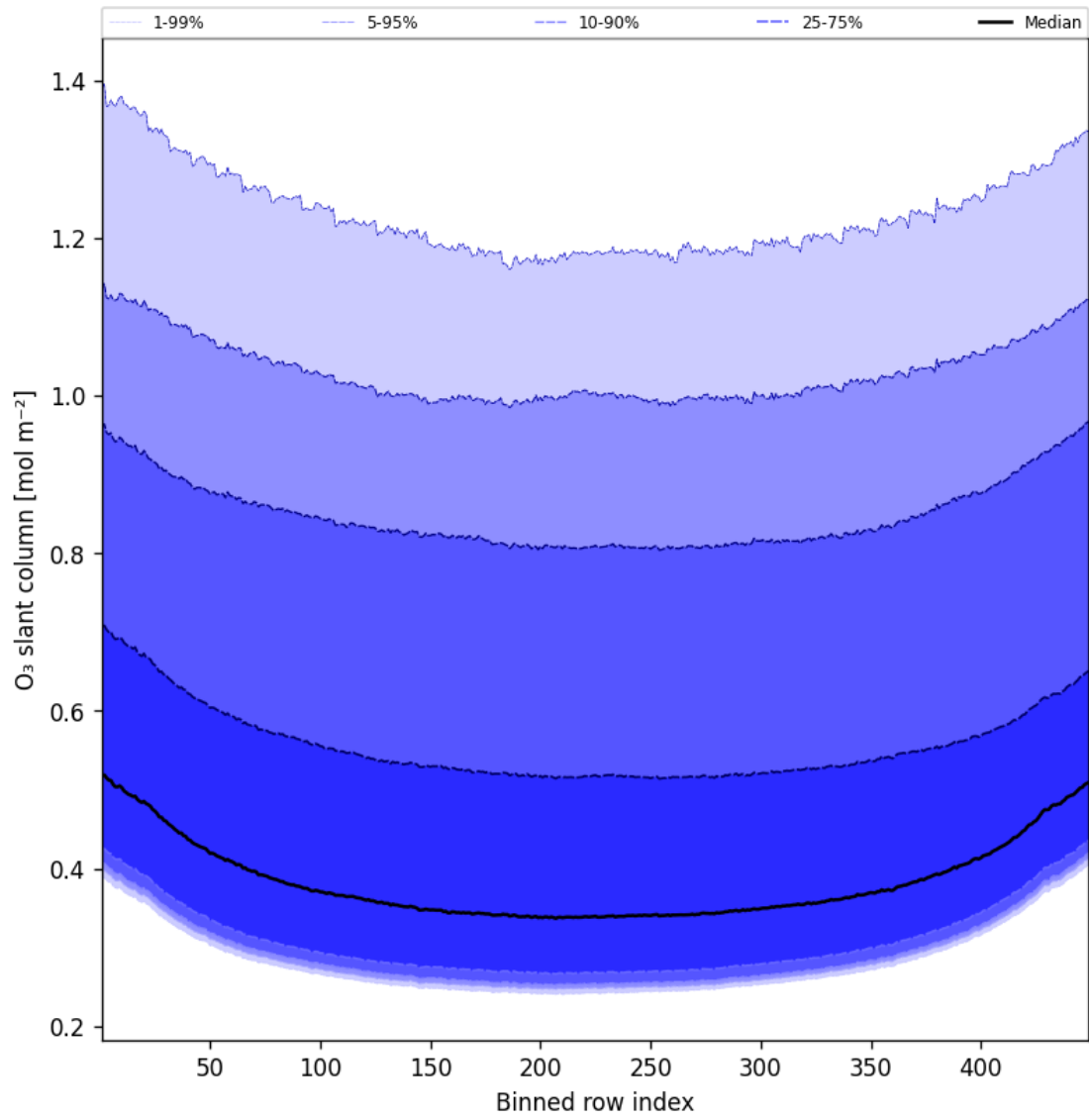
Figure 43: Along track statistics of “O 3 slant column” for 2025-07-25 to 2025-07-26
