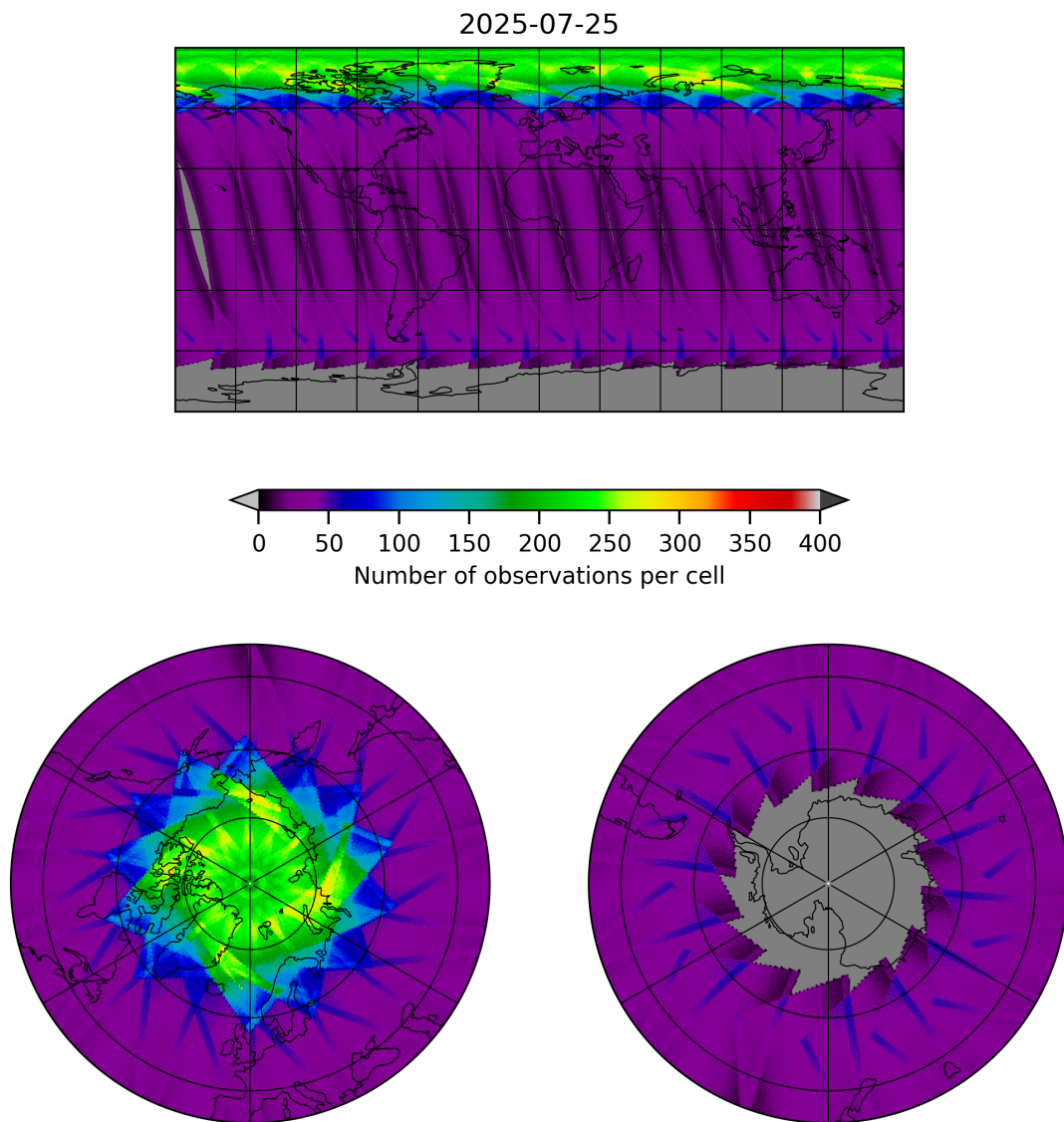
Figure 15: Map of the number of observations for 2025-07-25 to 2025-07-26
