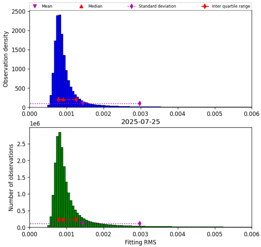
Figure 34: Histogram of “Fitting RMS” for 2025-07-25 to 2025-07-26
