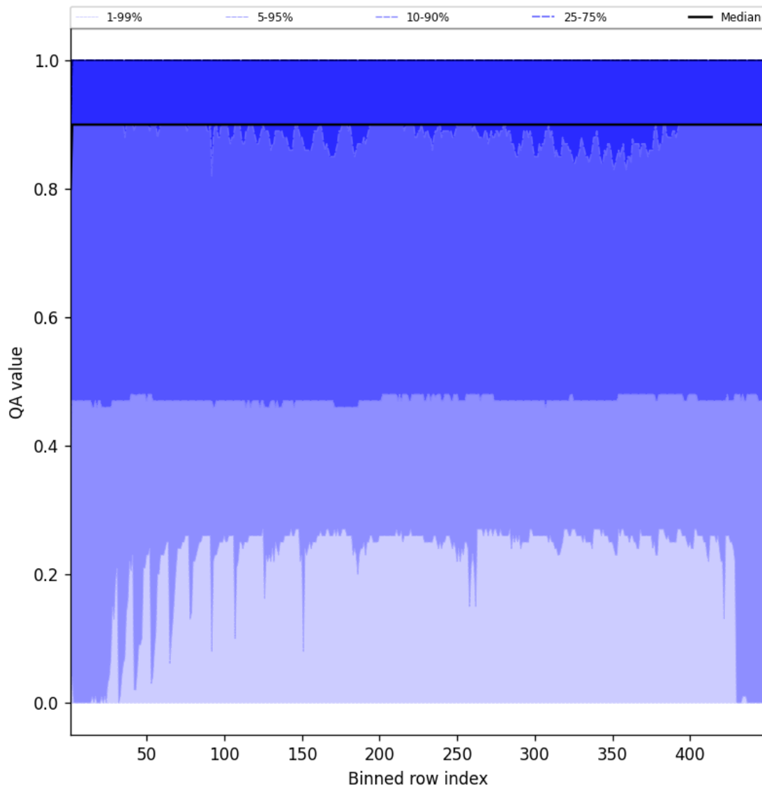
Figure 40: Along track statistics of “QA value” for 2025-07-25 to 2025-07-26
