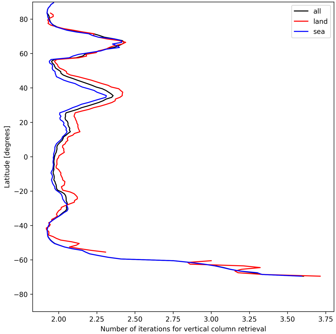
Figure 27: Zonal average of “Number of iterations for vertical column retrieval” for 2025-07-25 to 2025-07-26.
