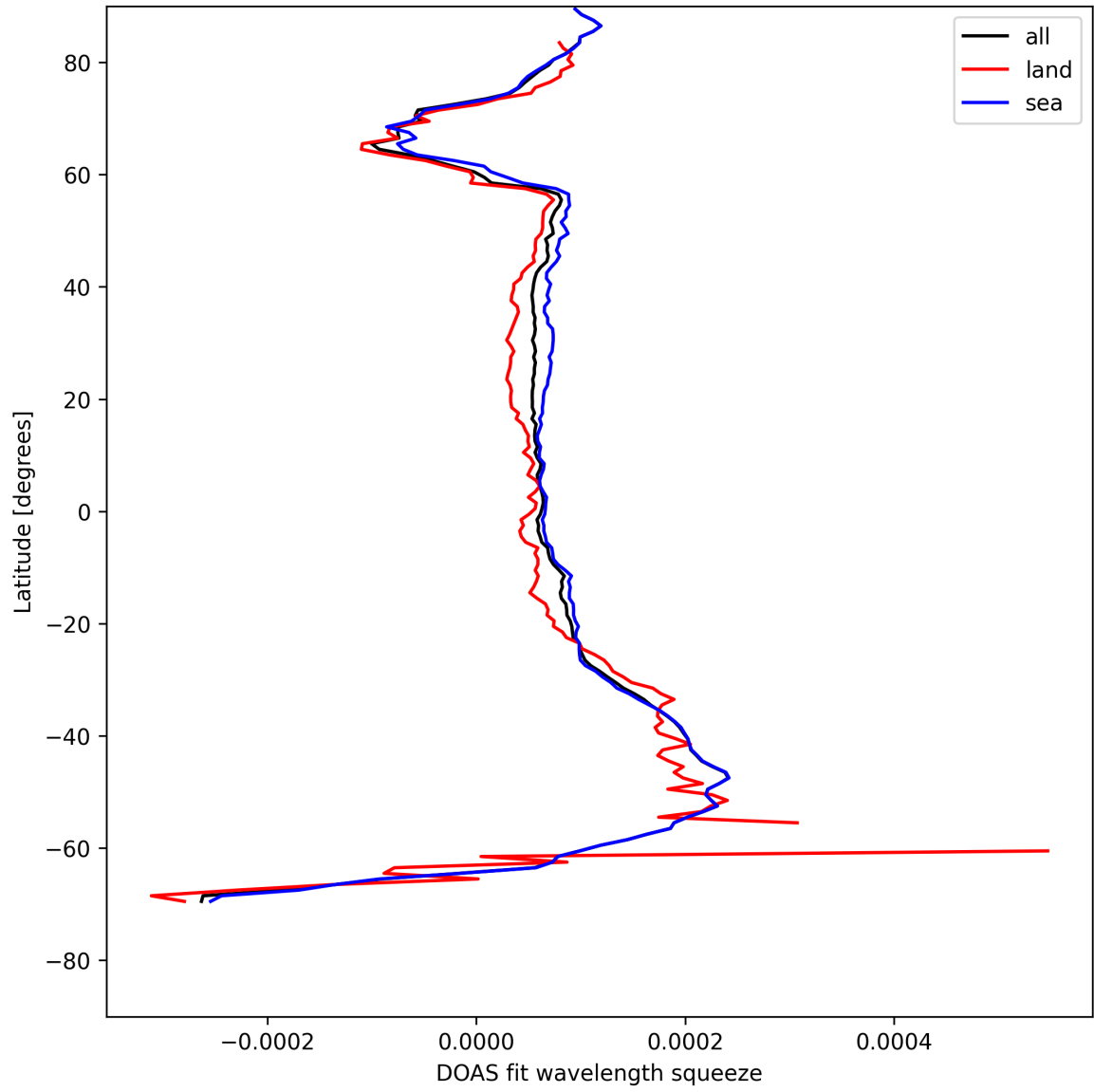
Figure 24: Zonal average of “DOAS fit wavelength squeeze” for 2025-07-26 to 2025-07-27.
