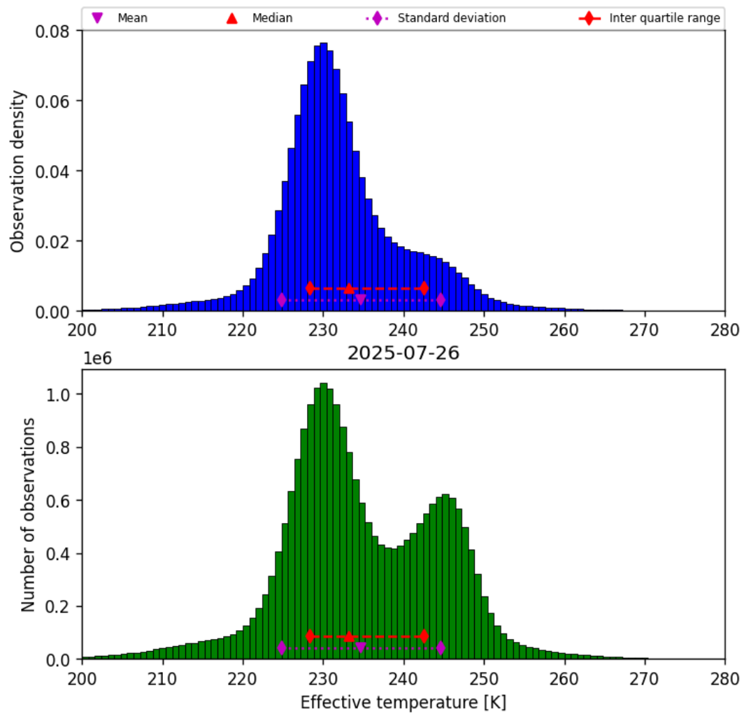
Figure 38: Histogram of “Effective temperature” for 2025-07-26 to 2025-07-27
