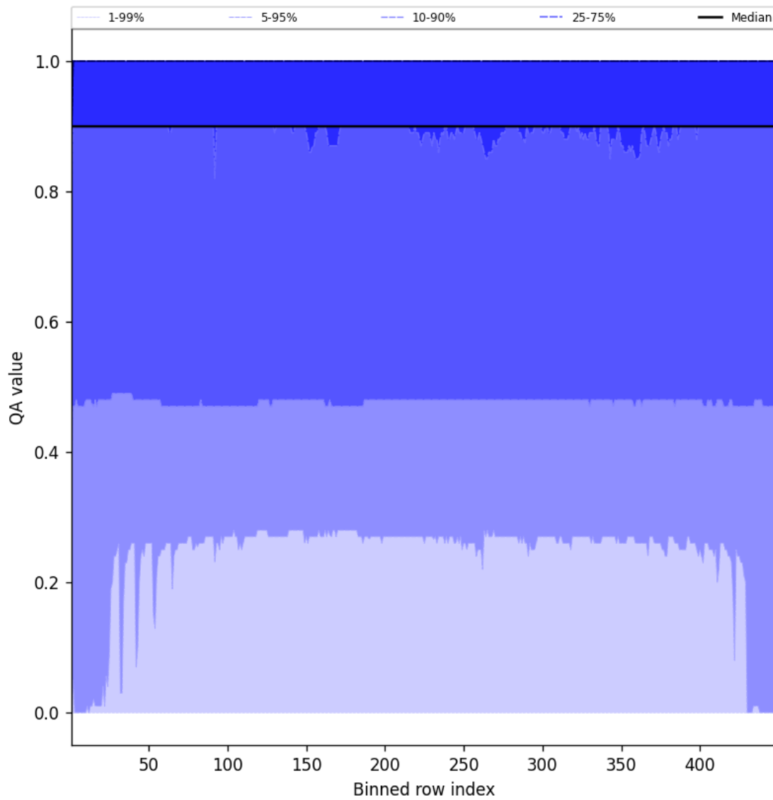
Figure 40: Along track statistics of “QA value” for 2025-07-26 to 2025-07-27
