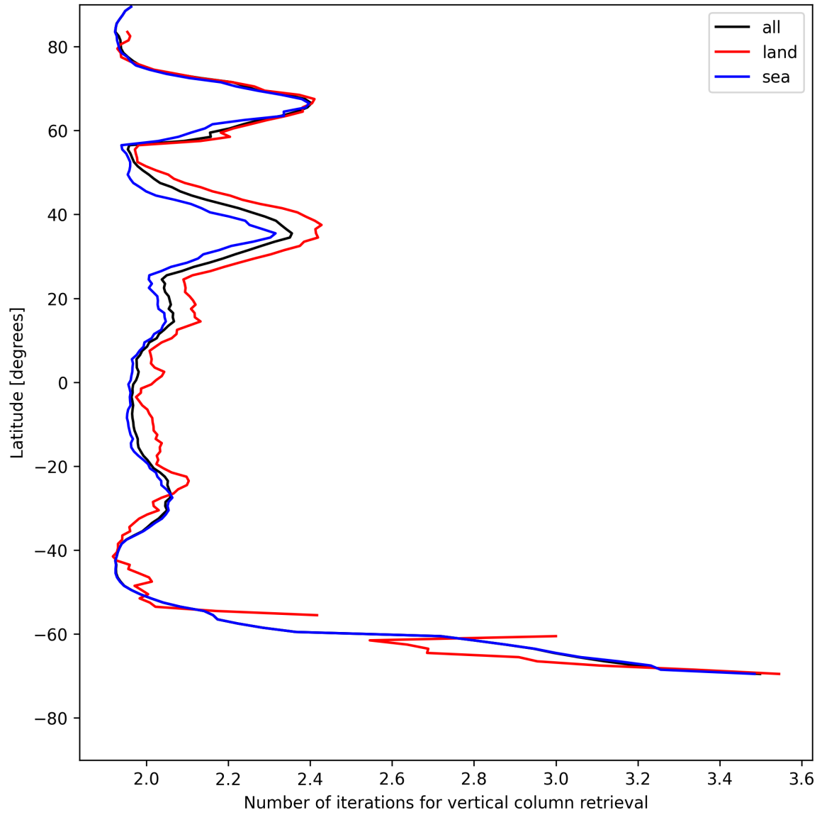
Figure 27: Zonal average of “Number of iterations for vertical column retrieval” for 2025-07-26 to 2025-07-27.
