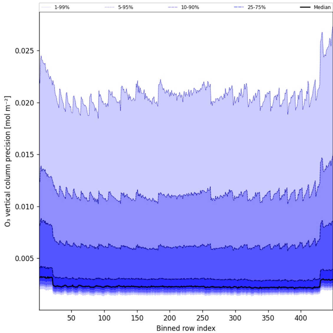
Figure 42: Along track statistics of “O 3 vertical column precision” for 2025-07-26 to 2025-07-27
