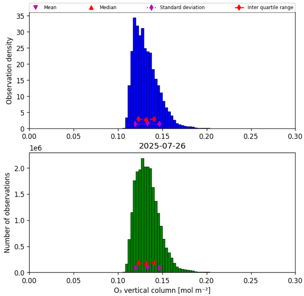
Figure 29: Histogram of “O 3 vertical column” for 2025-07-26 to 2025-07-27
