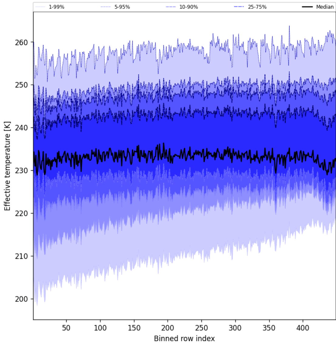
Figure 50: Along track statistics of “Effective temperature” for 2025-07-26 to 2025-07-27
