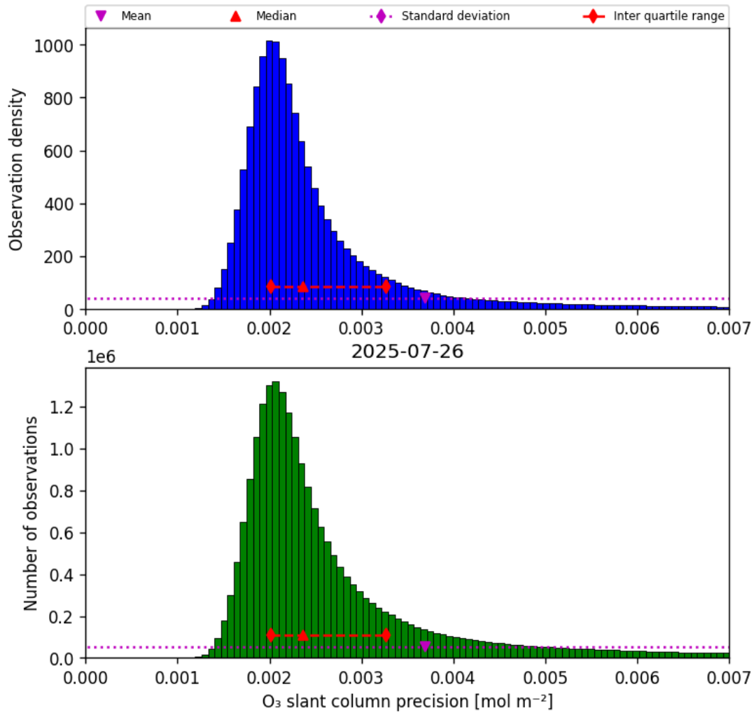
Figure 32: Histogram of “O 3 slant column precision” for 2025-07-26 to 2025-07-27
