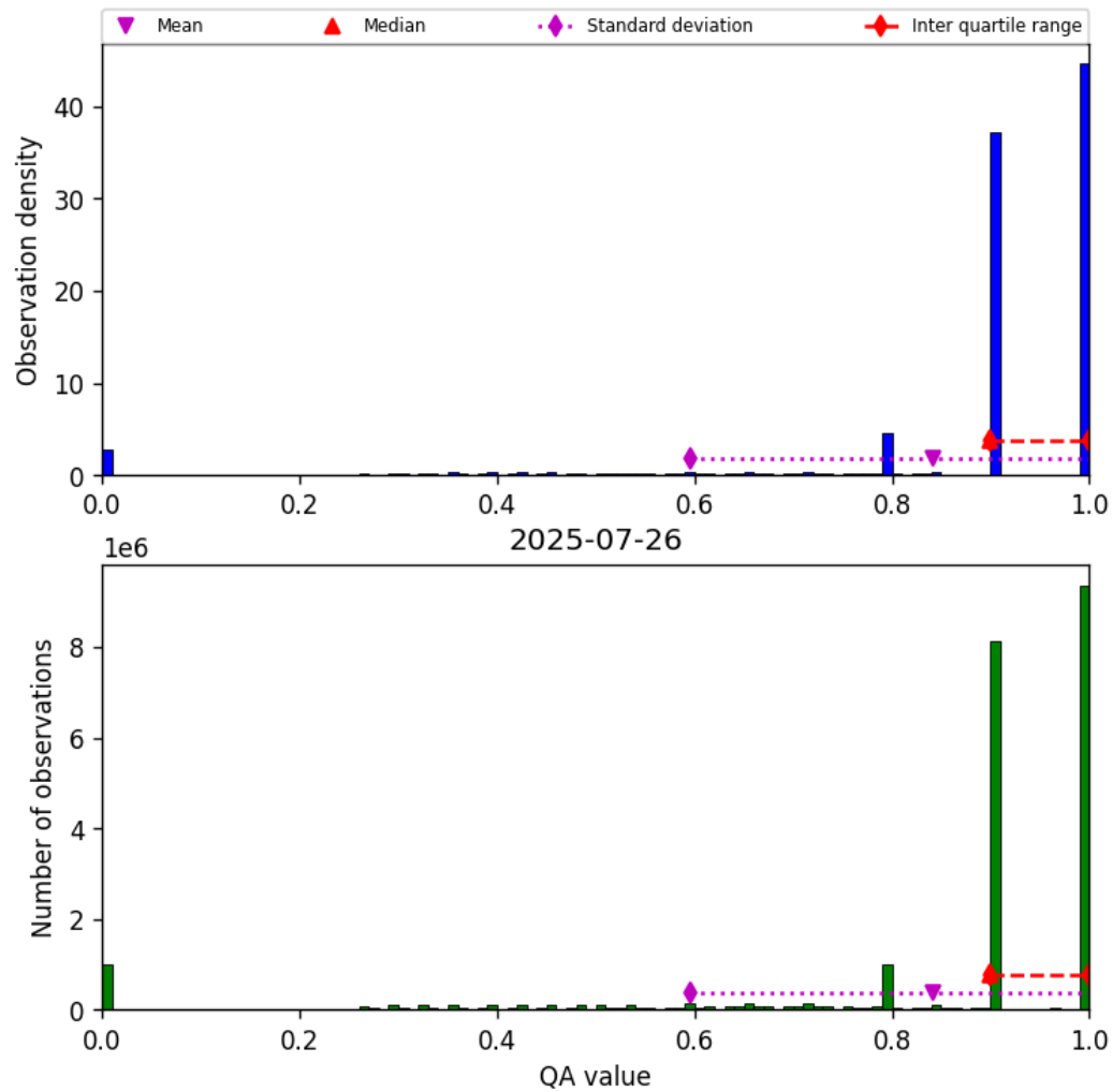
Figure 28: Histogram of “QA value” for 2025-07-26 to 2025-07-27
