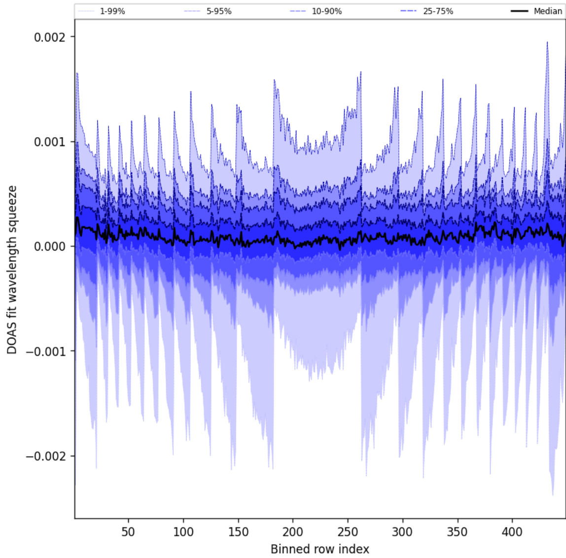
Figure 48: Along track statistics of “DOAS fit wavelength squeeze” for 2025-07-26 to 2025-07-27
