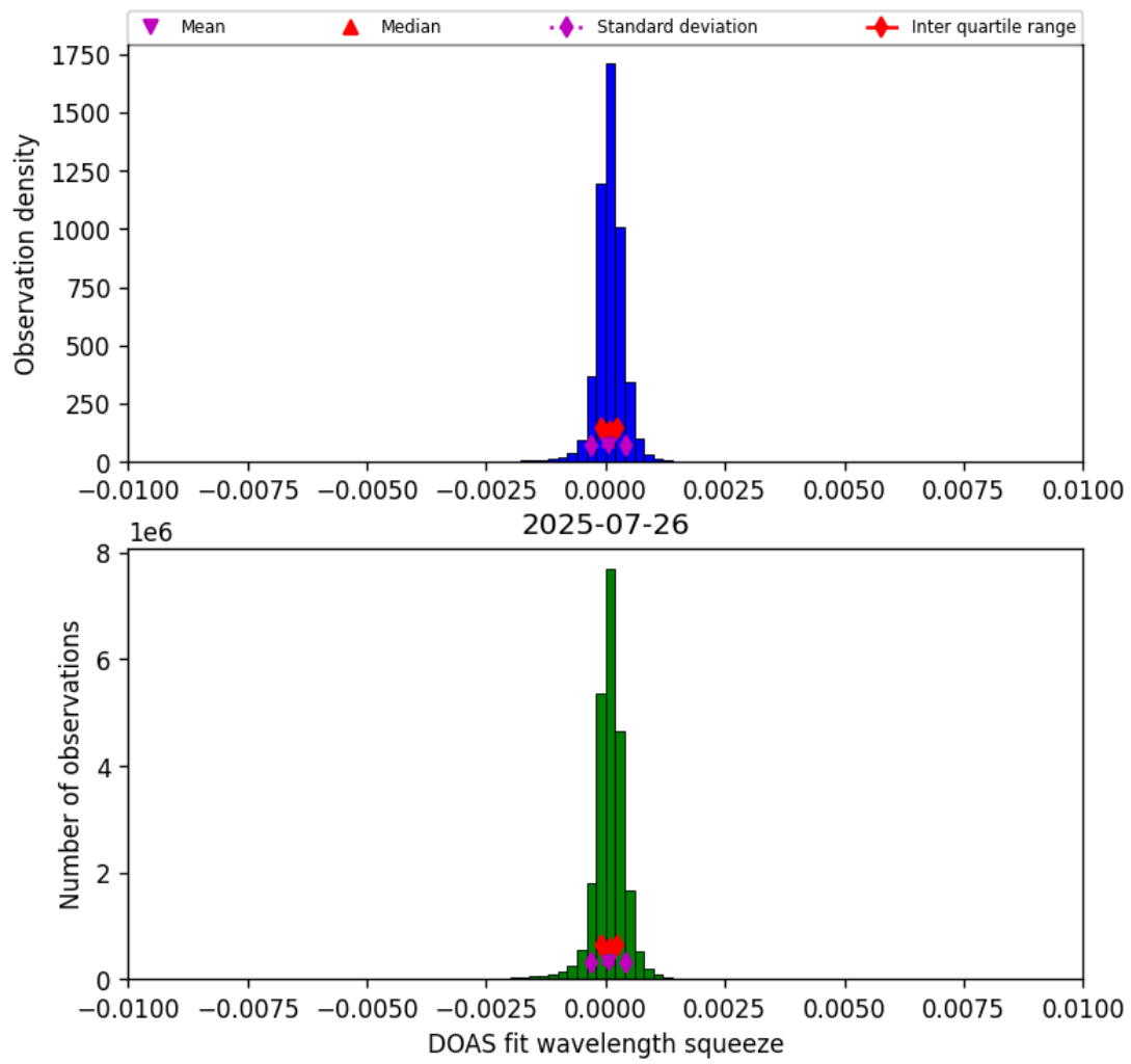
Figure 36: Histogram of “DOAS fit wavelength squeeze” for 2025-07-26 to 2025-07-27
