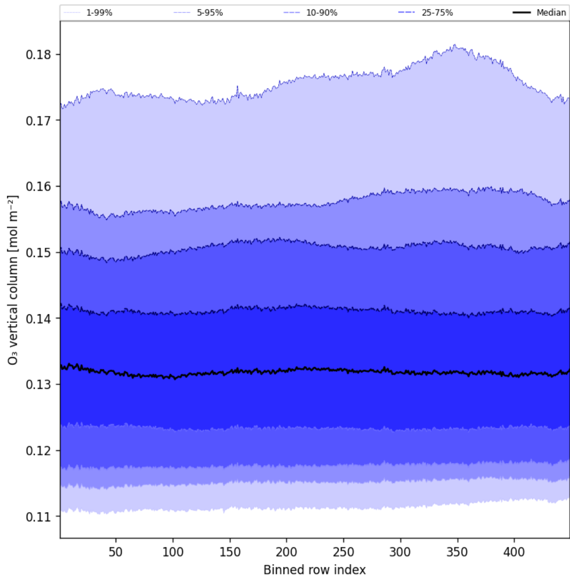
Figure 41: Along track statistics of “O 3 vertical column” for 2025-07-26 to 2025-07-27
