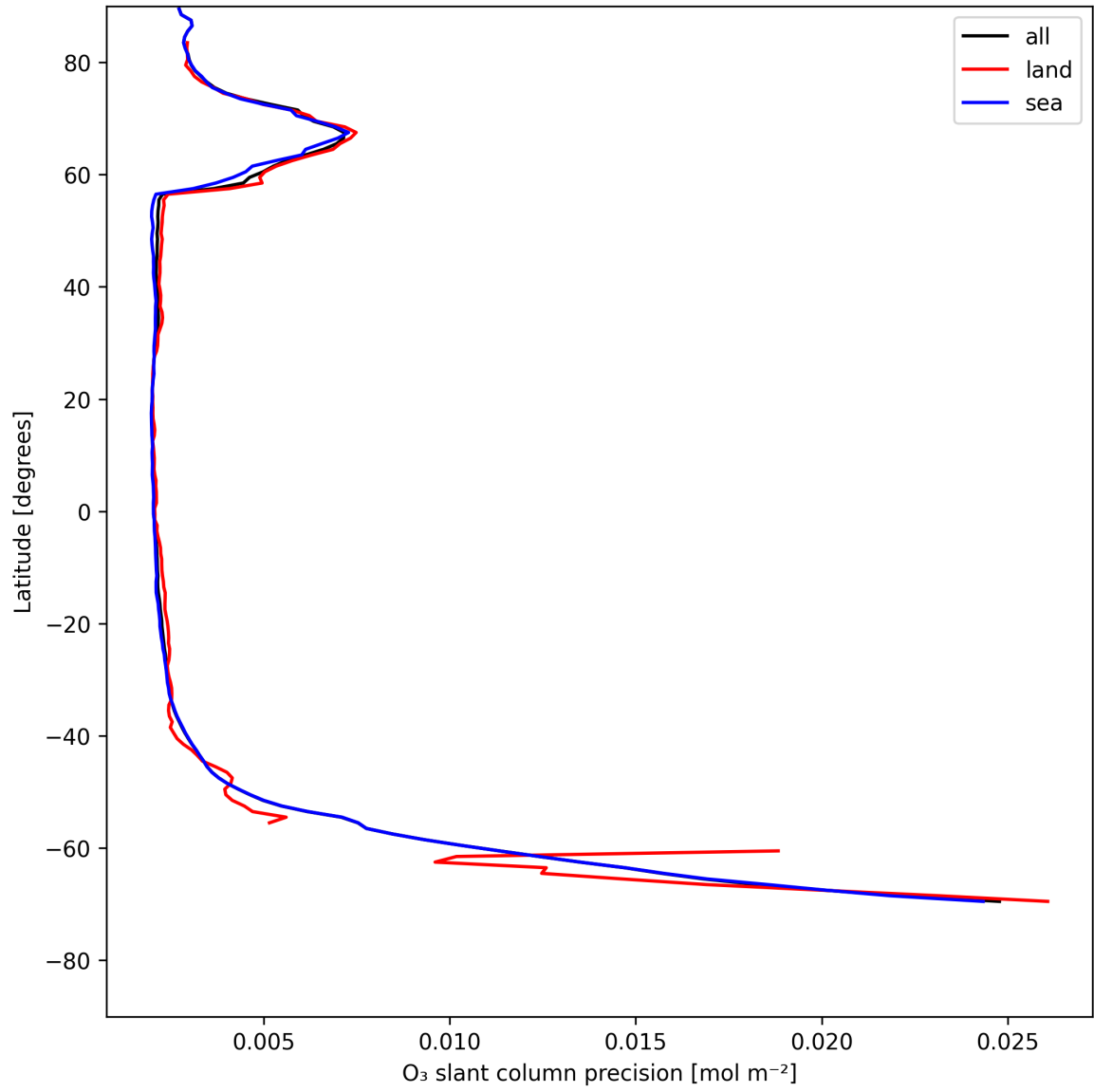
Figure 20: Zonal average of “O 3 slant column precision” for 2025-07-26 to 2025-07-27.
