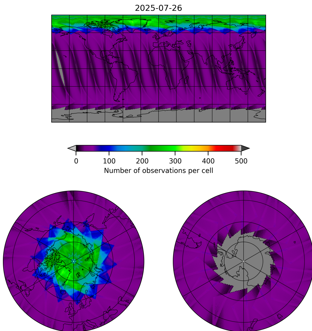
Figure 15: Map of the number of observations for 2025-07-26 to 2025-07-27
