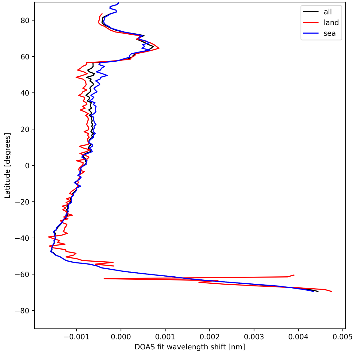
Figure 23: Zonal average of “DOAS fit wavelength shift” for 2025-07-26 to 2025-07-27.
