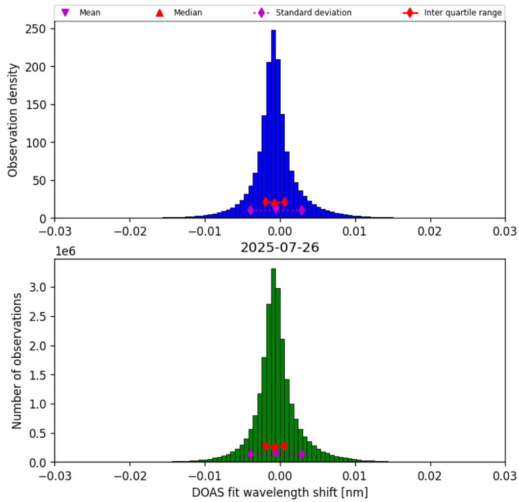
Figure 35: Histogram of “DOAS fit wavelength shift” for 2025-07-26 to 2025-07-27
