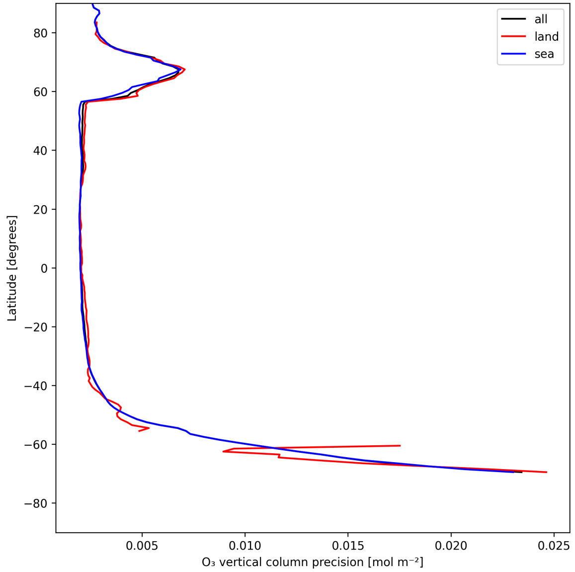
Figure 18: Zonal average of “O 3 vertical column precision” for 2025-07-26 to 2025-07-27.
