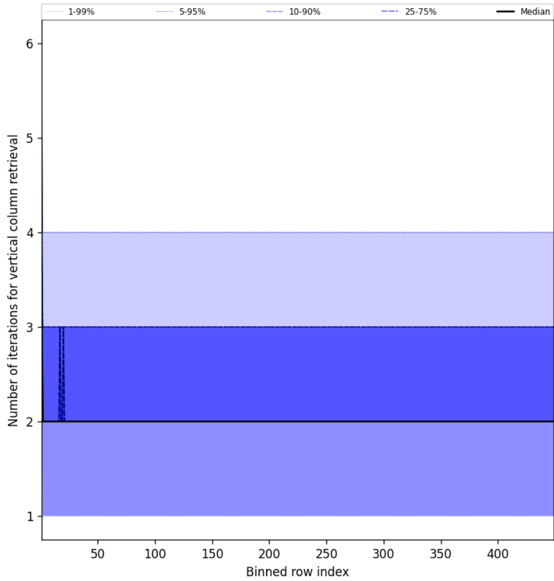
Figure 51: Along track statistics of “Number of iterations for vertical column retrieval” for 2025-07-26 to 2025-07-27
