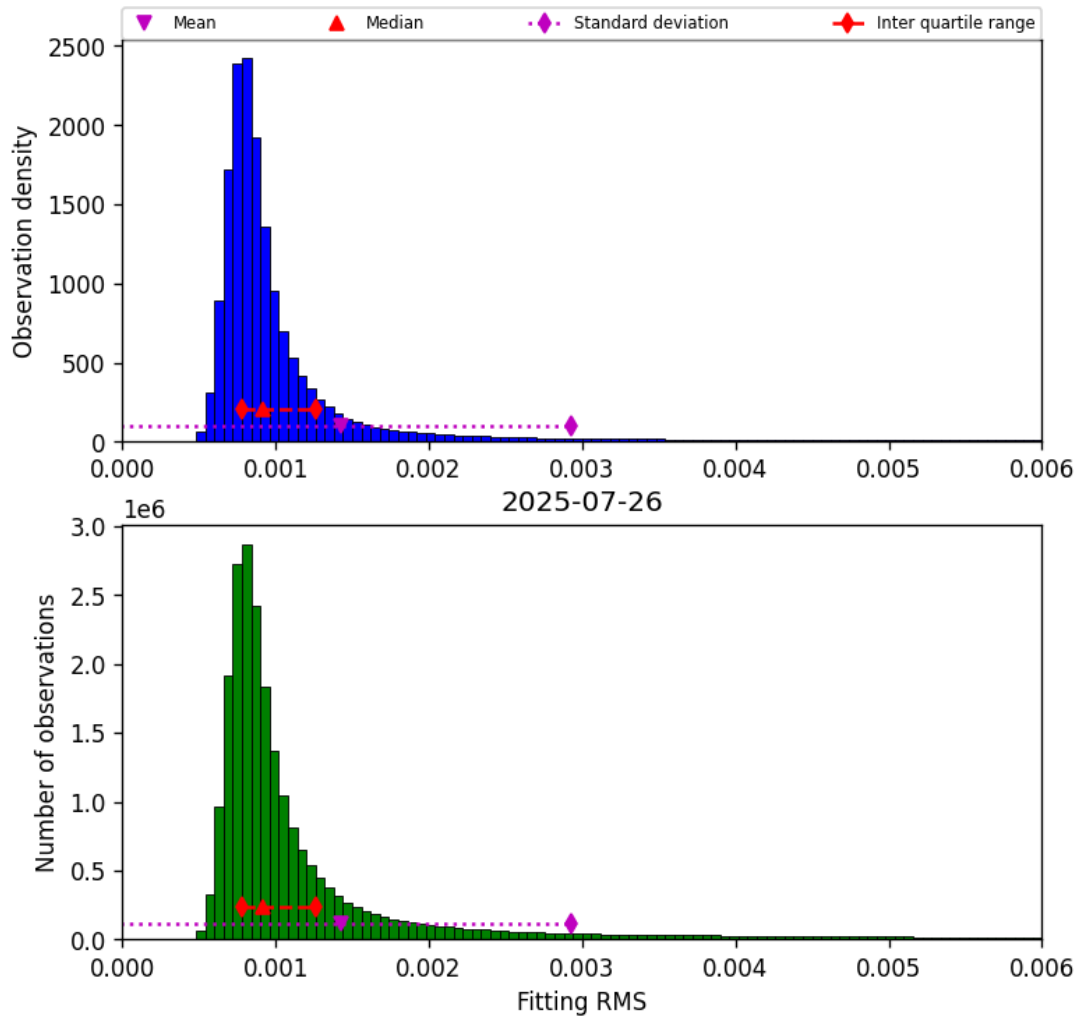
Figure 34: Histogram of “Fitting RMS” for 2025-07-26 to 2025-07-27
