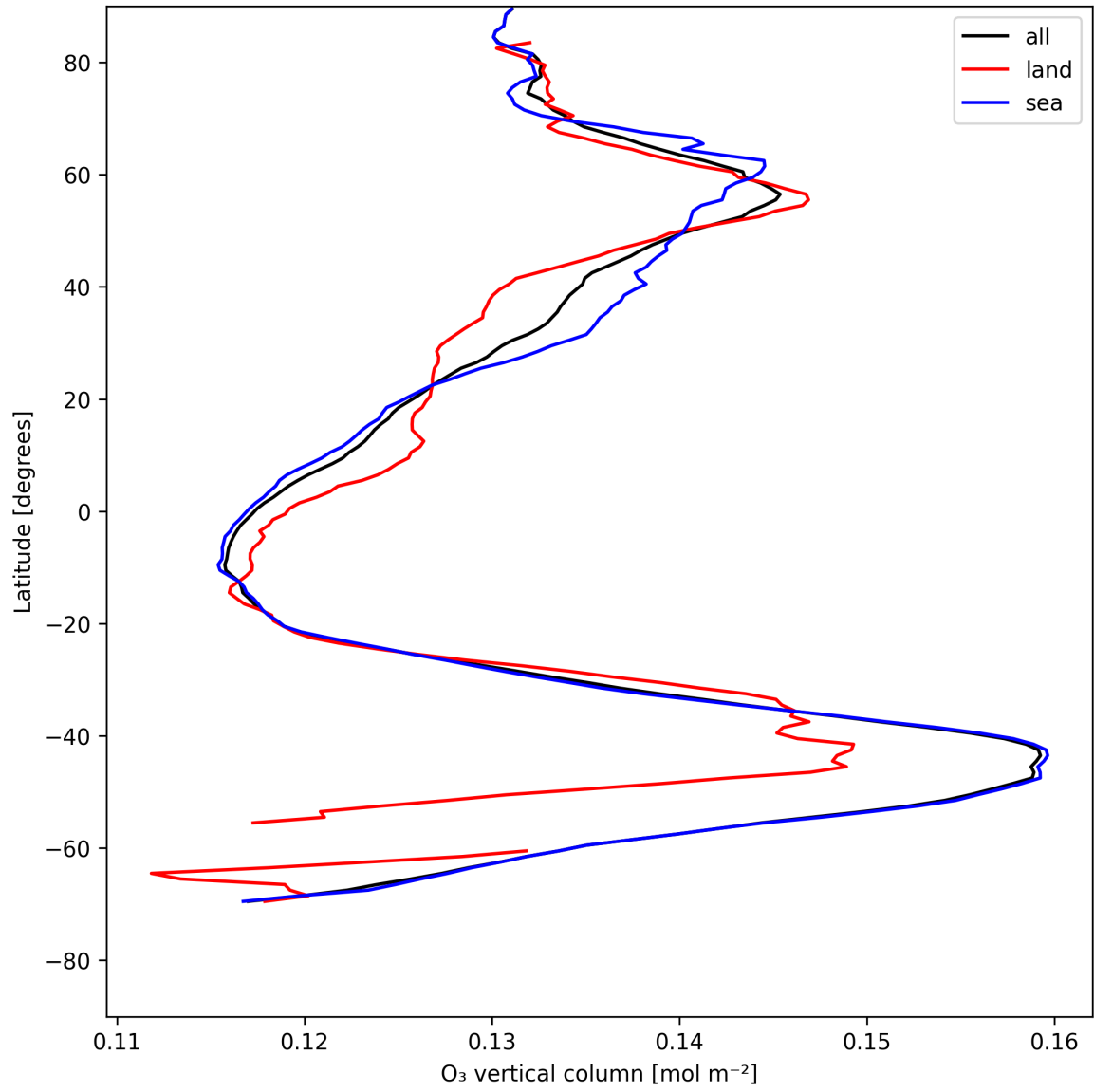
Figure 17: Zonal average of “O 3 vertical column” for 2025-07-26 to 2025-07-27.
