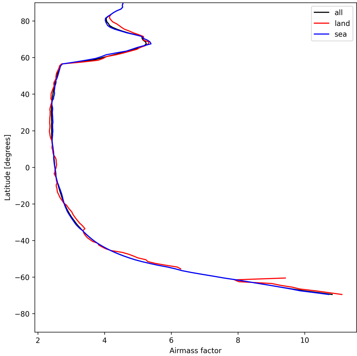
Figure 25: Zonal average of “Airmass factor” for 2025-07-26 to 2025-07-27.
