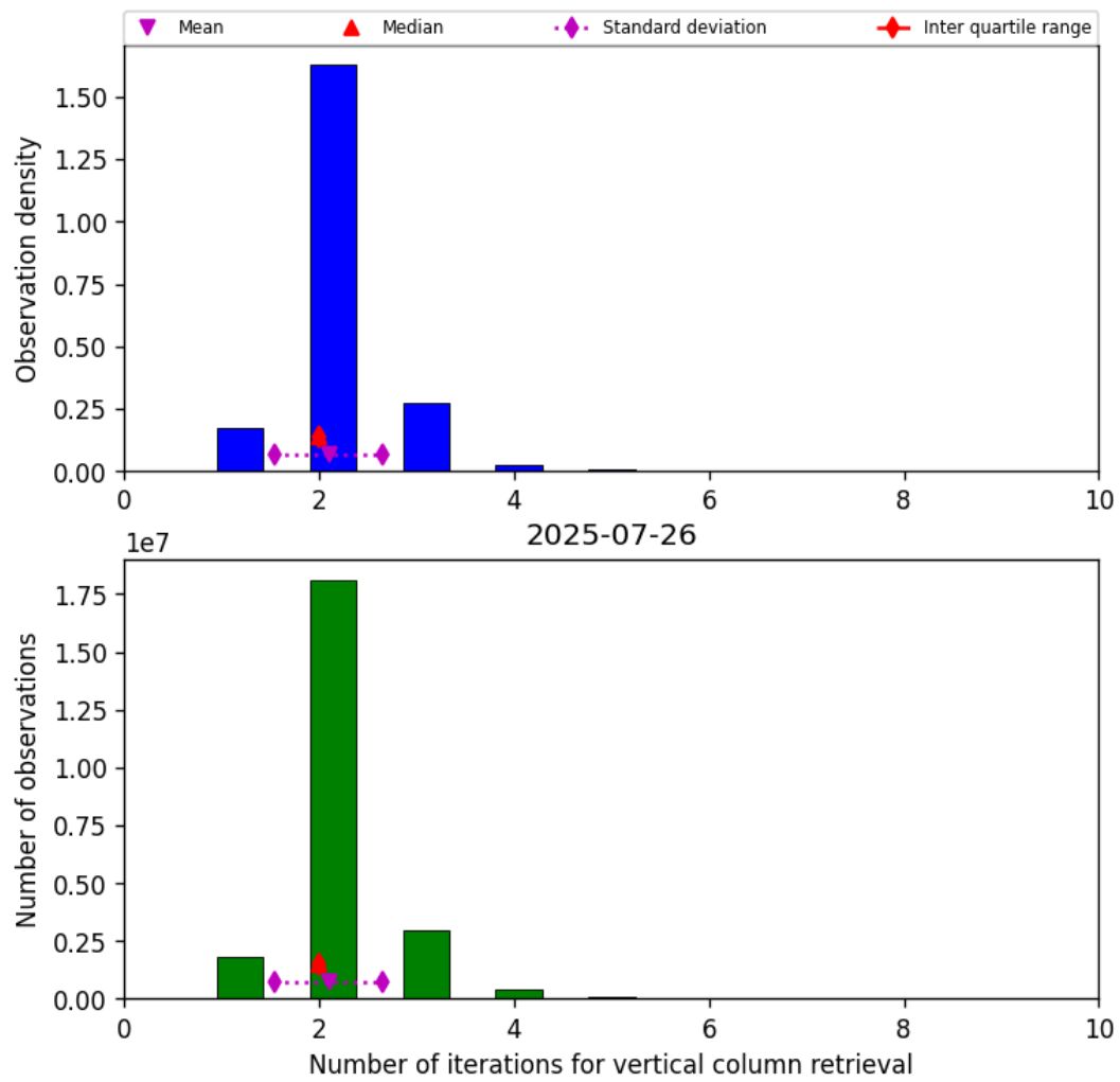
Figure 39: Histogram of “Number of iterations for vertical column retrieval” for 2025-07-26 to 2025-07-27
