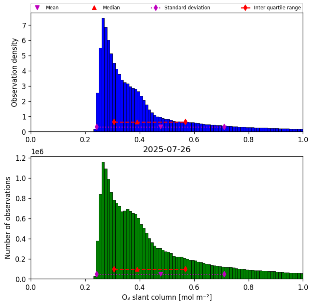
Figure 31: Histogram of “O 3 slant column” for 2025-07-26 to 2025-07-27
