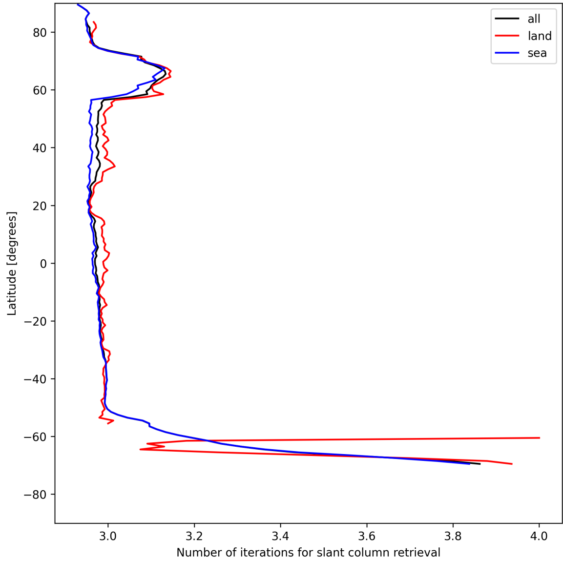
Figure 21: Zonal average of “Number of iterations for slant column retrieval” for 2025-07-26 to 2025-07-27.
