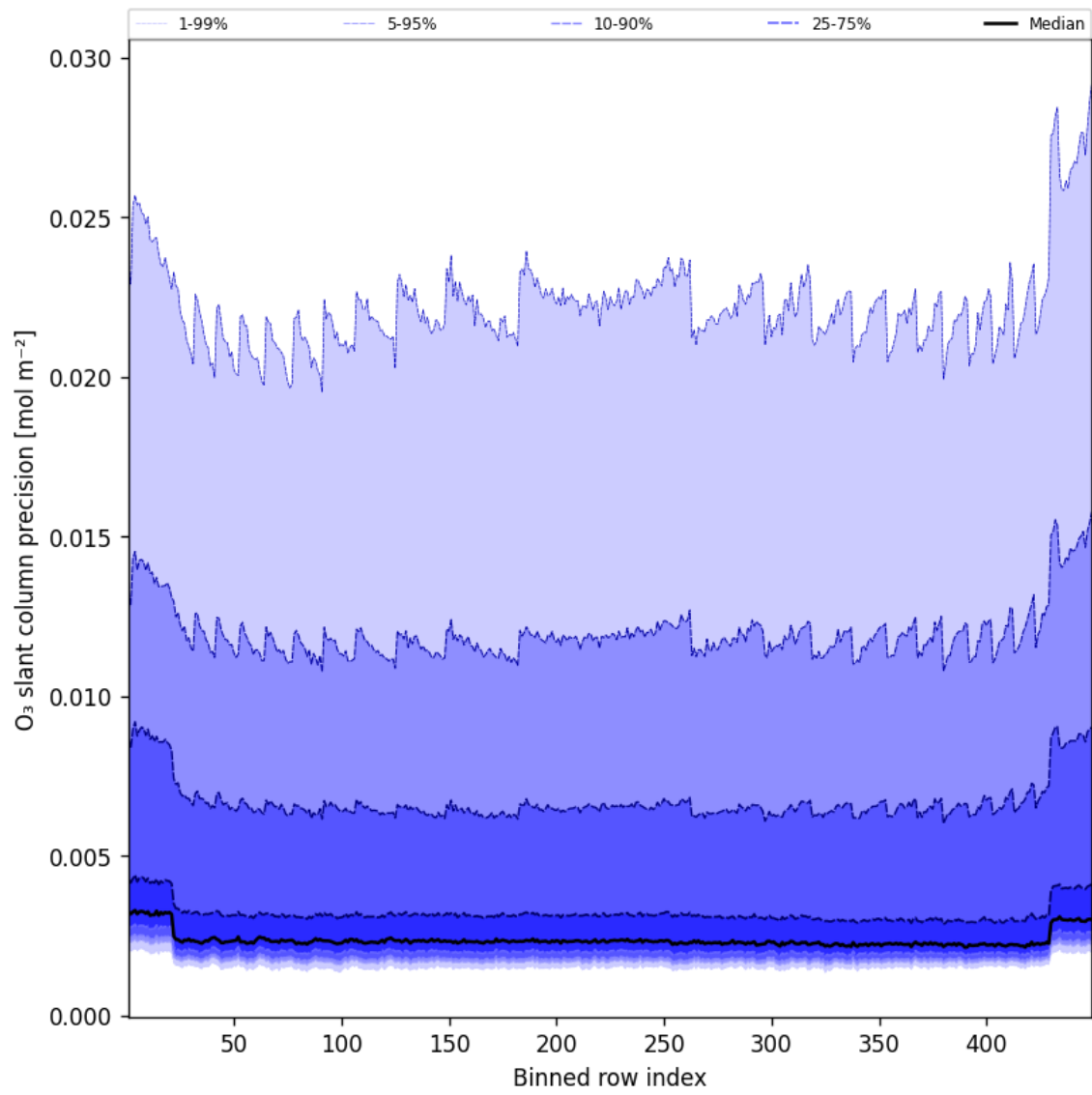
Figure 44: Along track statistics of “O 3 slant column precision” for 2025-07-26 to 2025-07-27
