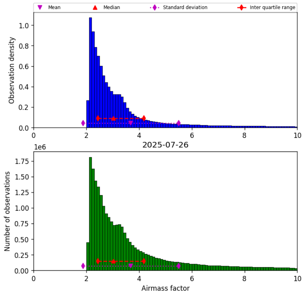
Figure 37: Histogram of “Airmass factor” for 2025-07-26 to 2025-07-27
