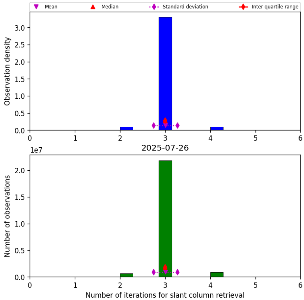
Figure 33: Histogram of “Number of iterations for slant column retrieval” for 2025-07-26 to 2025-07-27
