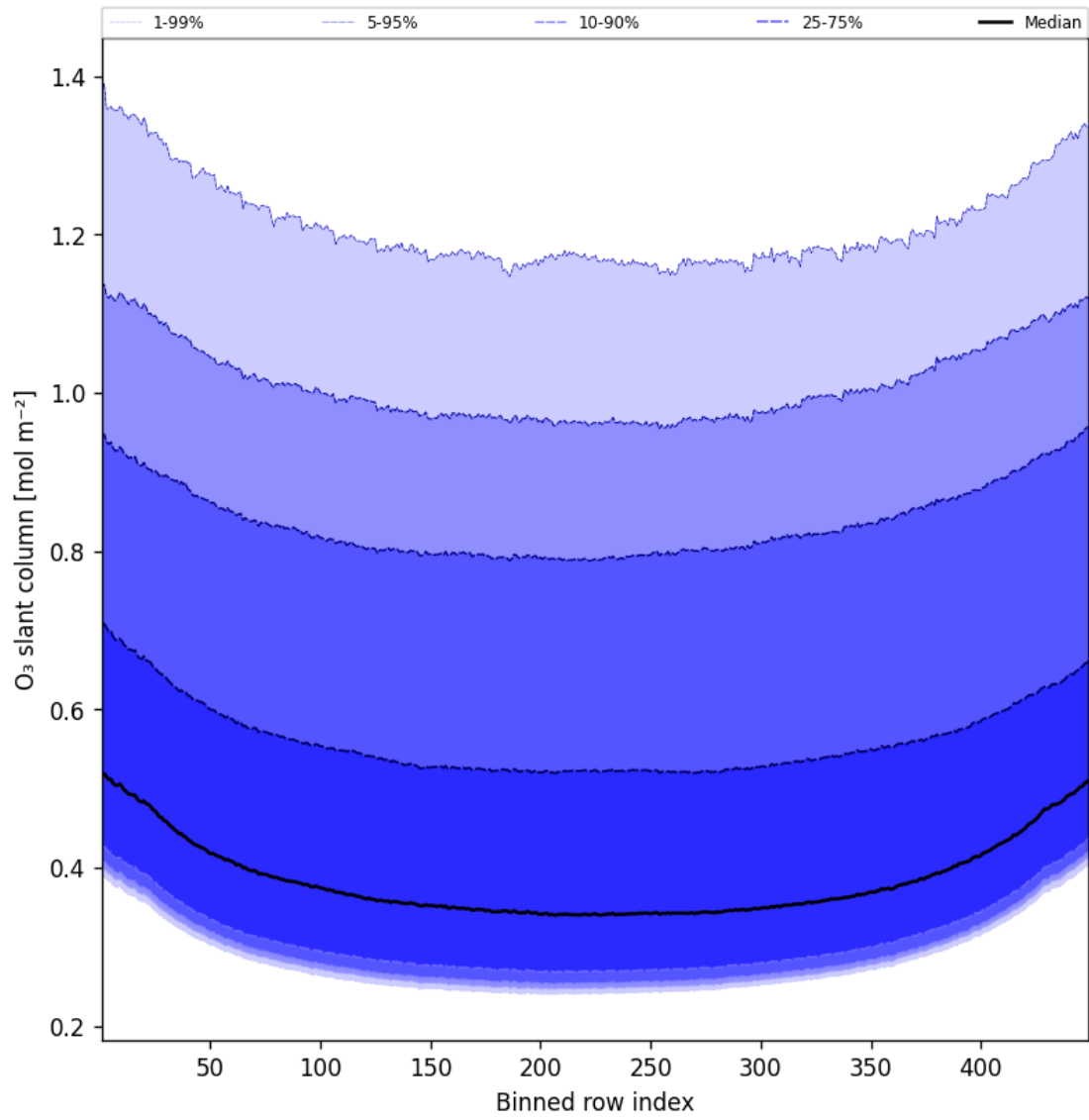
Figure 43: Along track statistics of “O 3 slant column” for 2025-07-26 to 2025-07-27
