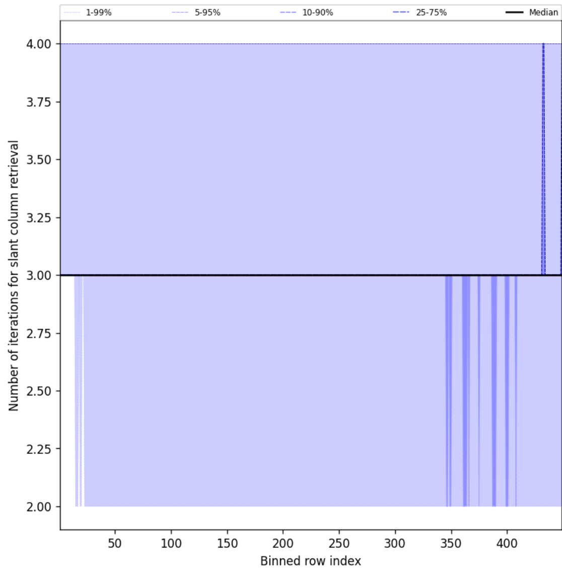
Figure 45: Along track statistics of “Number of iterations for slant column retrieval” for 2025-07-26 to 2025-07-27
