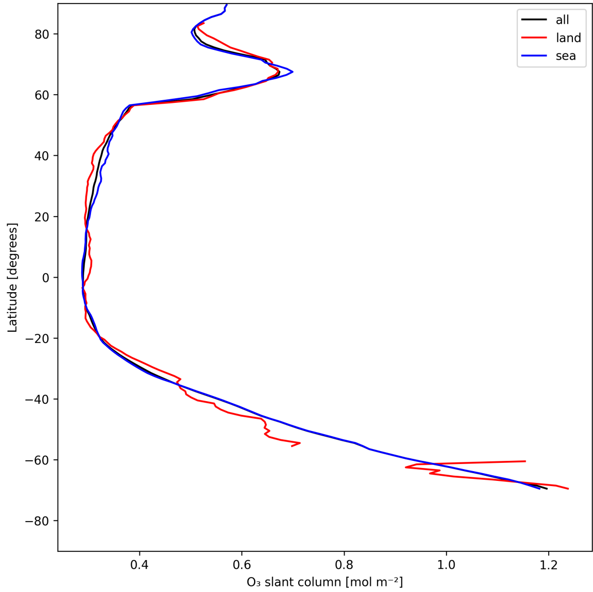
Figure 19: Zonal average of “O 3 slant column” for 2025-07-26 to 2025-07-27.
