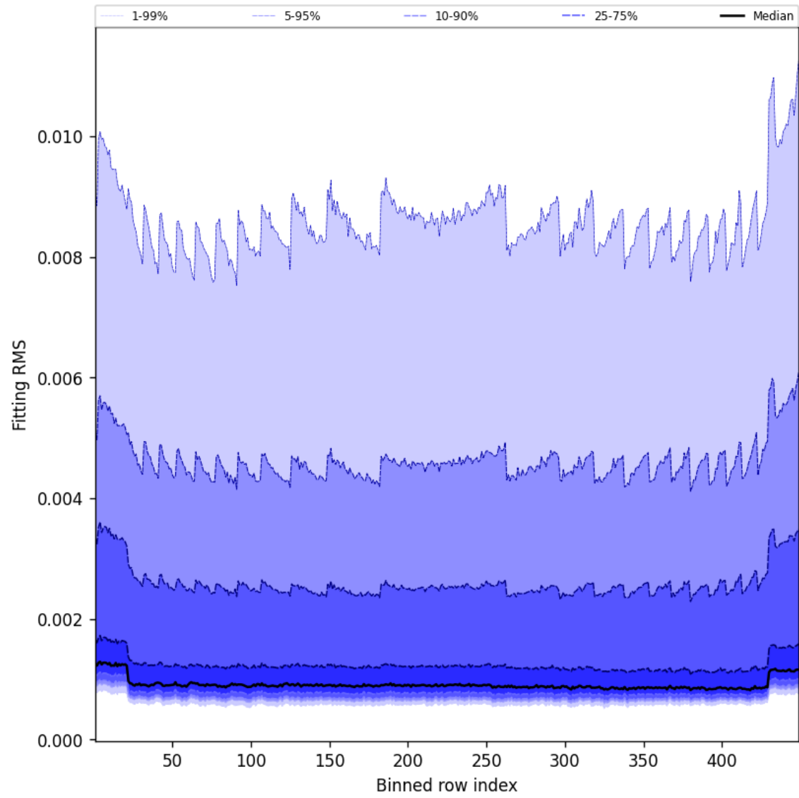
Figure 46: Along track statistics of “Fitting RMS” for 2025-07-26 to 2025-07-27
