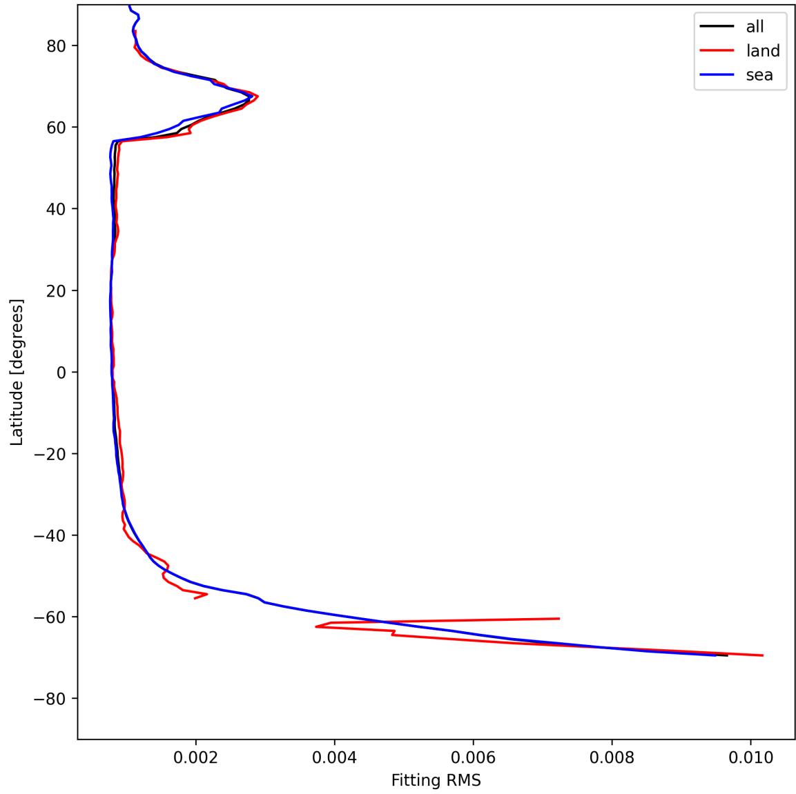
Figure 22: Zonal average of “Fitting RMS” for 2025-07-26 to 2025-07-27.
