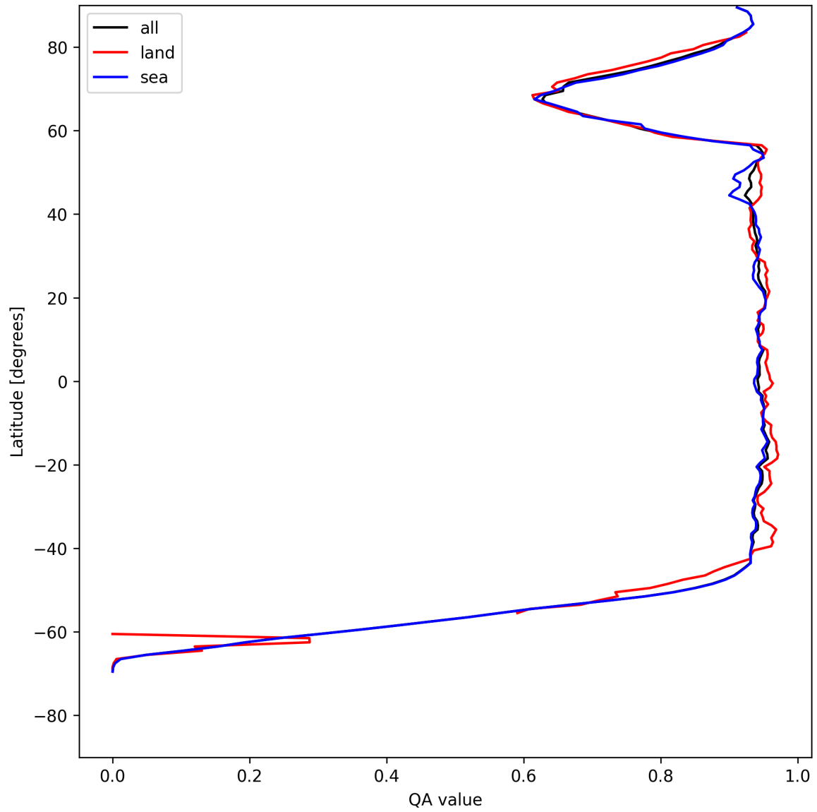
Figure 16: Zonal average of “QA value” for 2025-07-26 to 2025-07-27.
