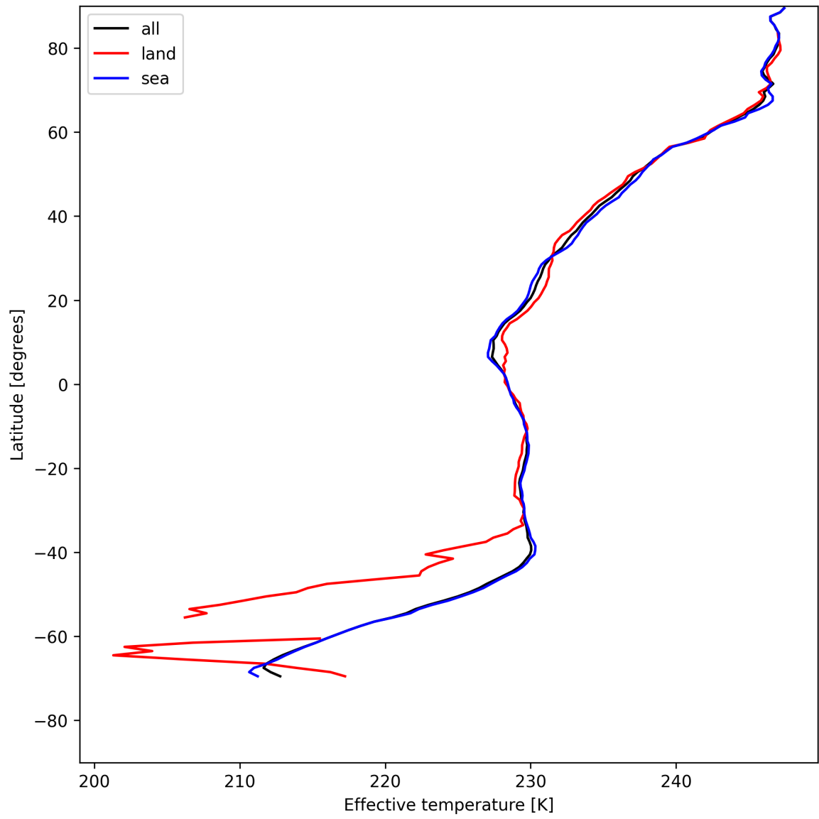
Figure 26: Zonal average of “Effective temperature” for 2025-07-26 to 2025-07-27.
