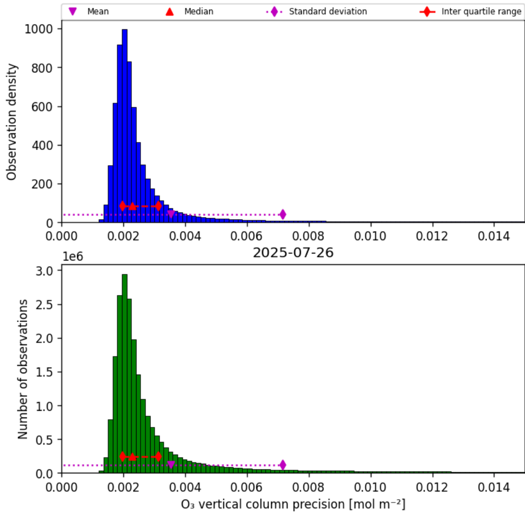
Figure 30: Histogram of “O 3 vertical column precision” for 2025-07-26 to 2025-07-27
