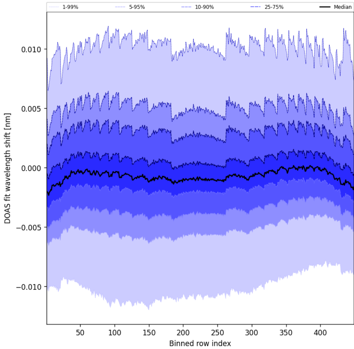
Figure 47: Along track statistics of “DOAS fit wavelength shift” for 2025-07-26 to 2025-07-27
