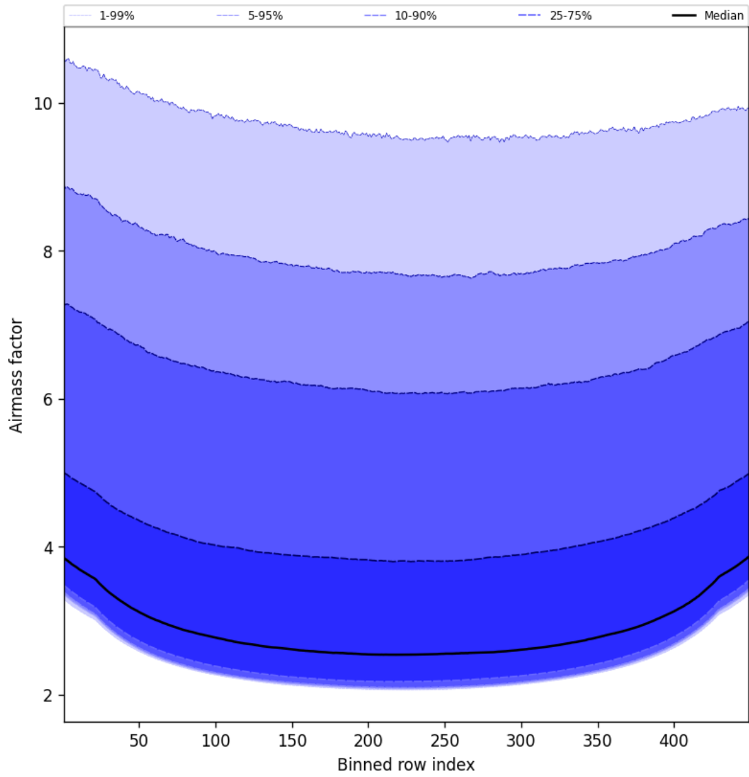
Figure 49: Along track statistics of “Airmass factor” for 2025-07-26 to 2025-07-27
