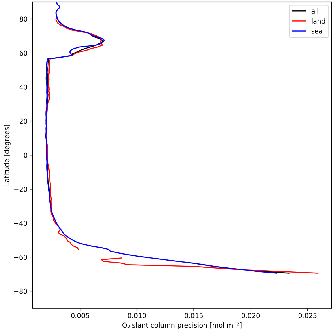
Figure 20: Zonal average of “O 3 slant column precision” for 2025-07-27 to 2025-07-27.
