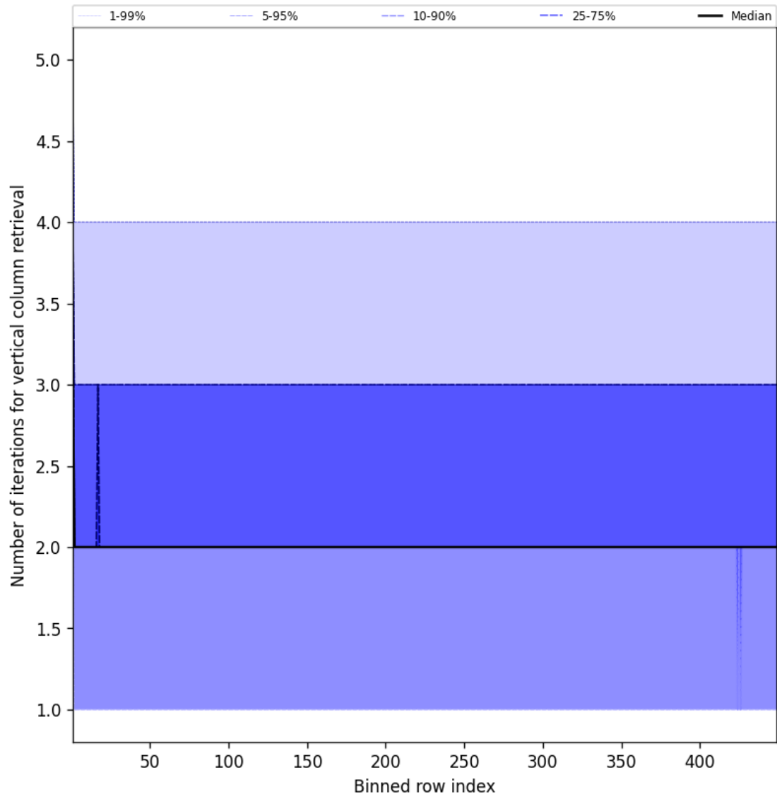
Figure 51: Along track statistics of “Number of iterations for vertical column retrieval” for 2025-07-27 to 2025-07-27
