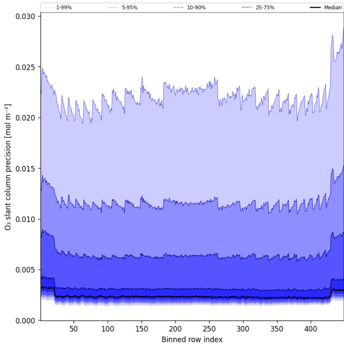
Figure 44: Along track statistics of “O 3 slant column precision” for 2025-07-27 to 2025-07-27
