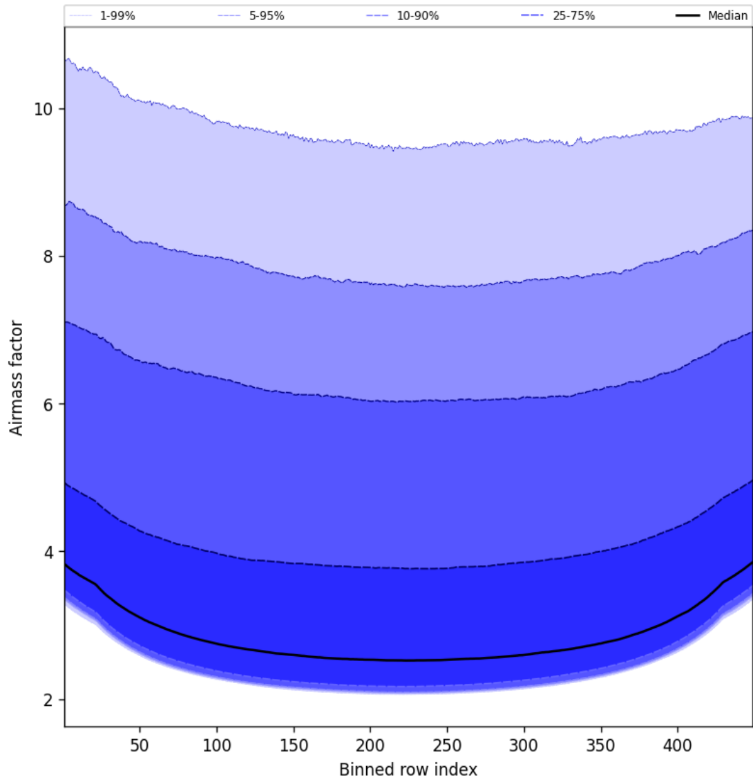
Figure 49: Along track statistics of “Airmass factor” for 2025-07-27 to 2025-07-27
