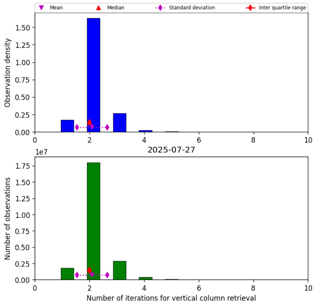
Figure 39: Histogram of “Number of iterations for vertical column retrieval” for 2025-07-27 to 2025-07-27
