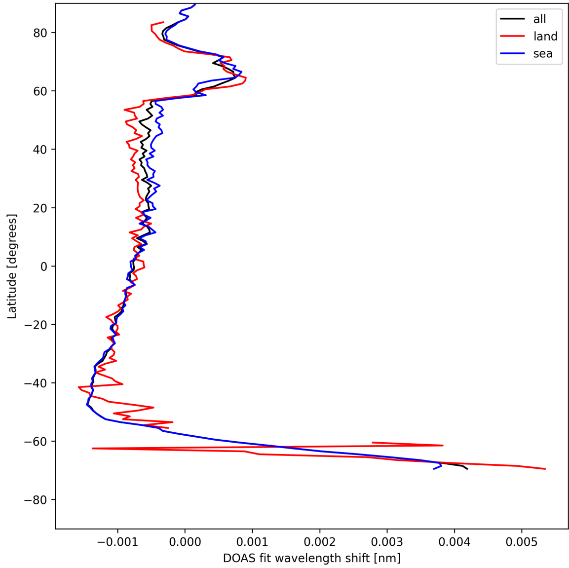
Figure 23: Zonal average of “DOAS fit wavelength shift” for 2025-07-27 to 2025-07-27.
