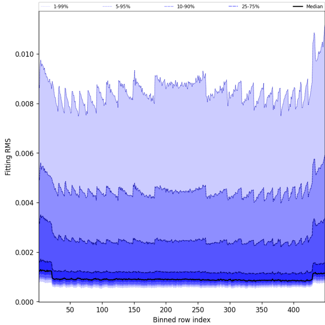
Figure 46: Along track statistics of “Fitting RMS” for 2025-07-27 to 2025-07-27
