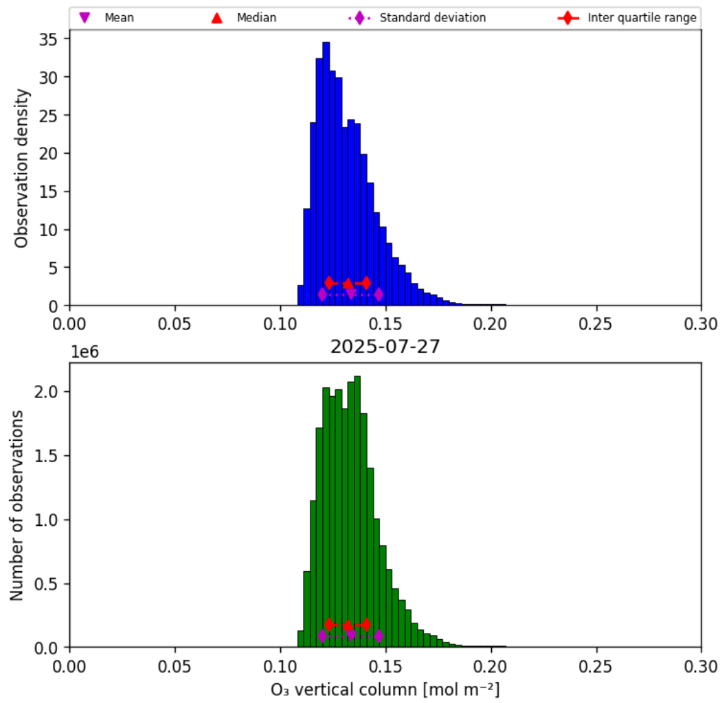
Figure 29: Histogram of “O 3 vertical column” for 2025-07-27 to 2025-07-27
