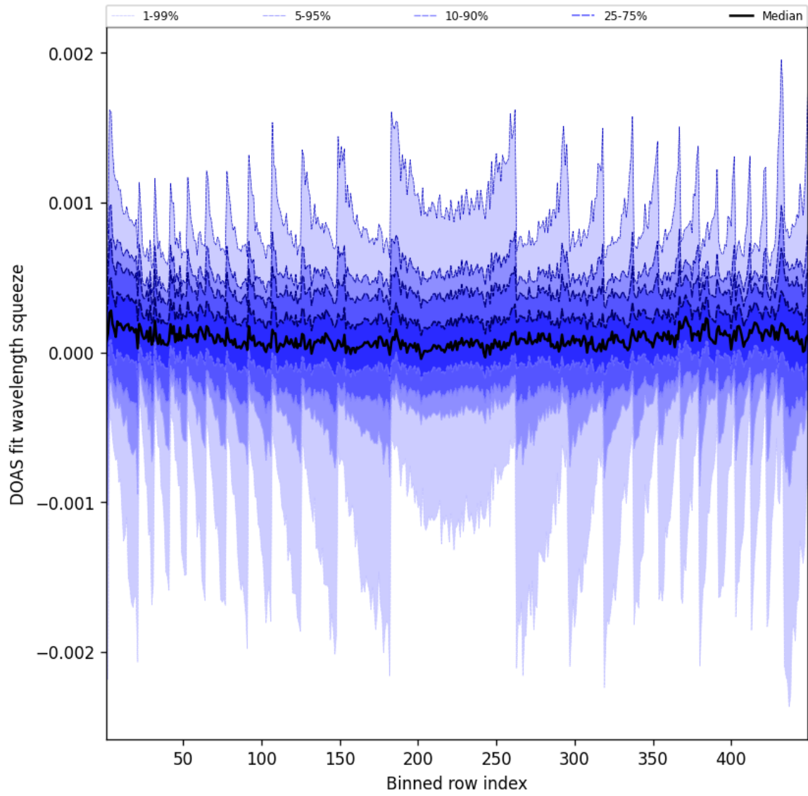
Figure 48: Along track statistics of “DOAS fit wavelength squeeze” for 2025-07-27 to 2025-07-27
