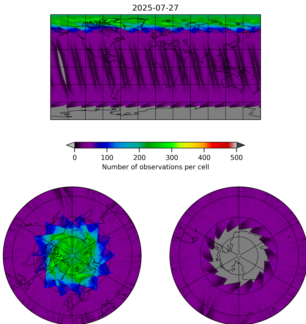
Figure 15: Map of the number of observations for 2025-07-27 to 2025-07-27
