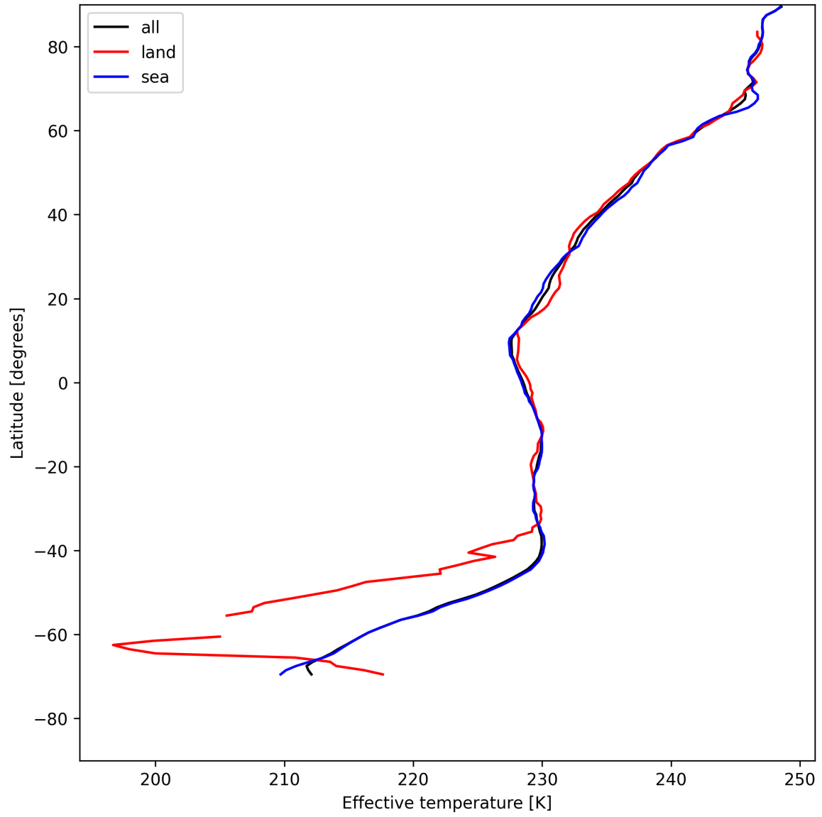
Figure 26: Zonal average of “Effective temperature” for 2025-07-27 to 2025-07-27.
