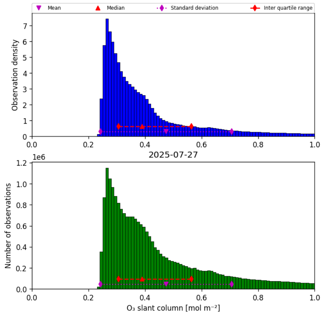
Figure 31: Histogram of “O 3 slant column” for 2025-07-27 to 2025-07-27
