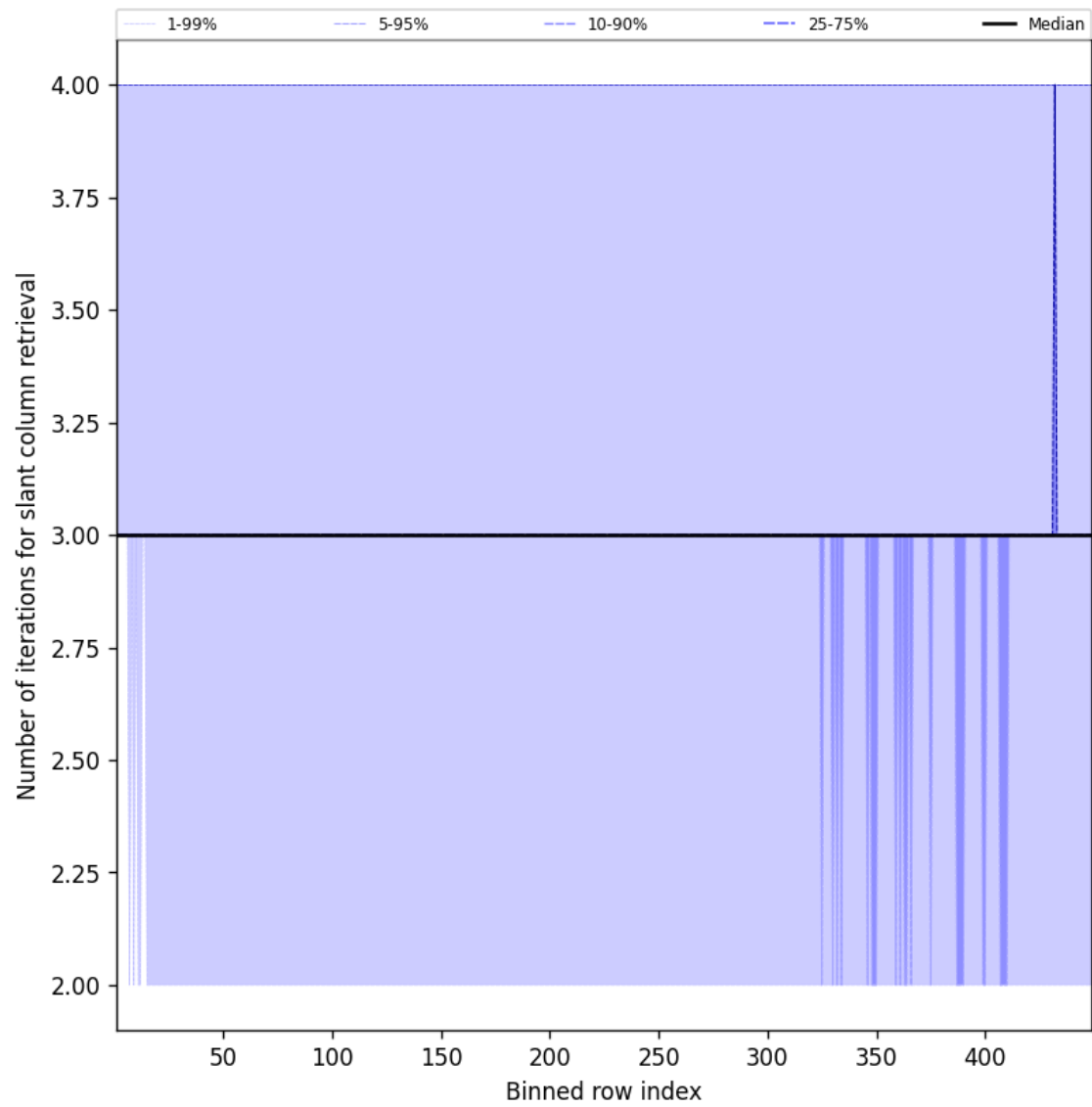
Figure 45: Along track statistics of “Number of iterations for slant column retrieval” for 2025-07-27 to 2025-07-27
