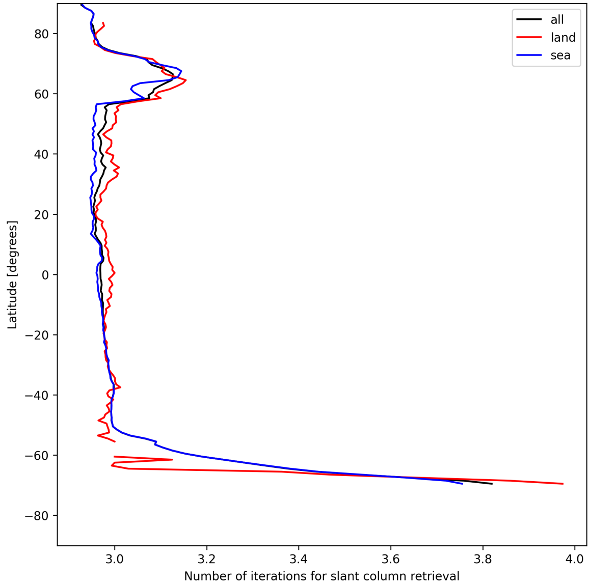
Figure 21: Zonal average of “Number of iterations for slant column retrieval” for 2025-07-27 to 2025-07-27.
