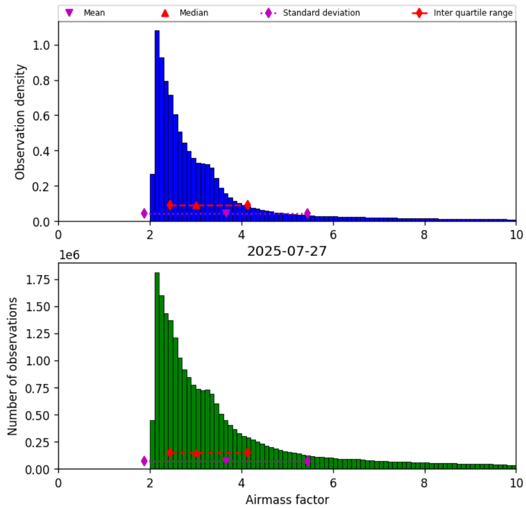
Figure 37: Histogram of “Airmass factor” for 2025-07-27 to 2025-07-27
