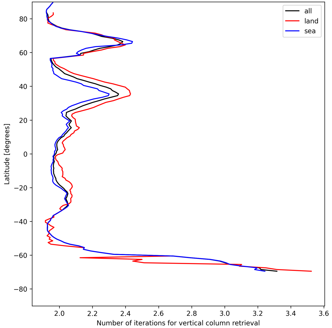
Figure 27: Zonal average of “Number of iterations for vertical column retrieval” for 2025-07-27 to 2025-07-27.
