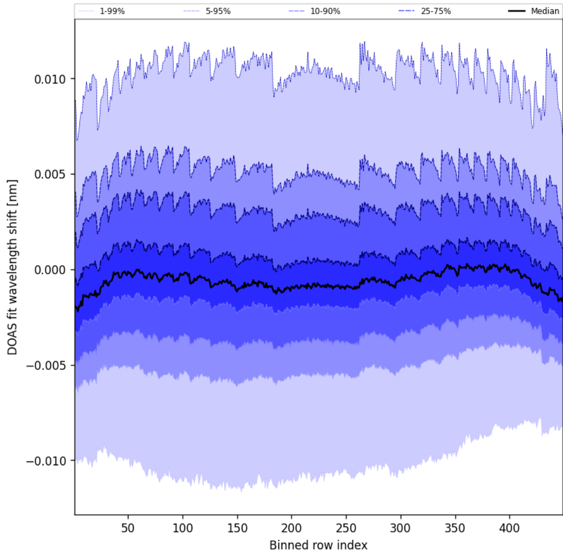
Figure 47: Along track statistics of “DOAS fit wavelength shift” for 2025-07-27 to 2025-07-27
