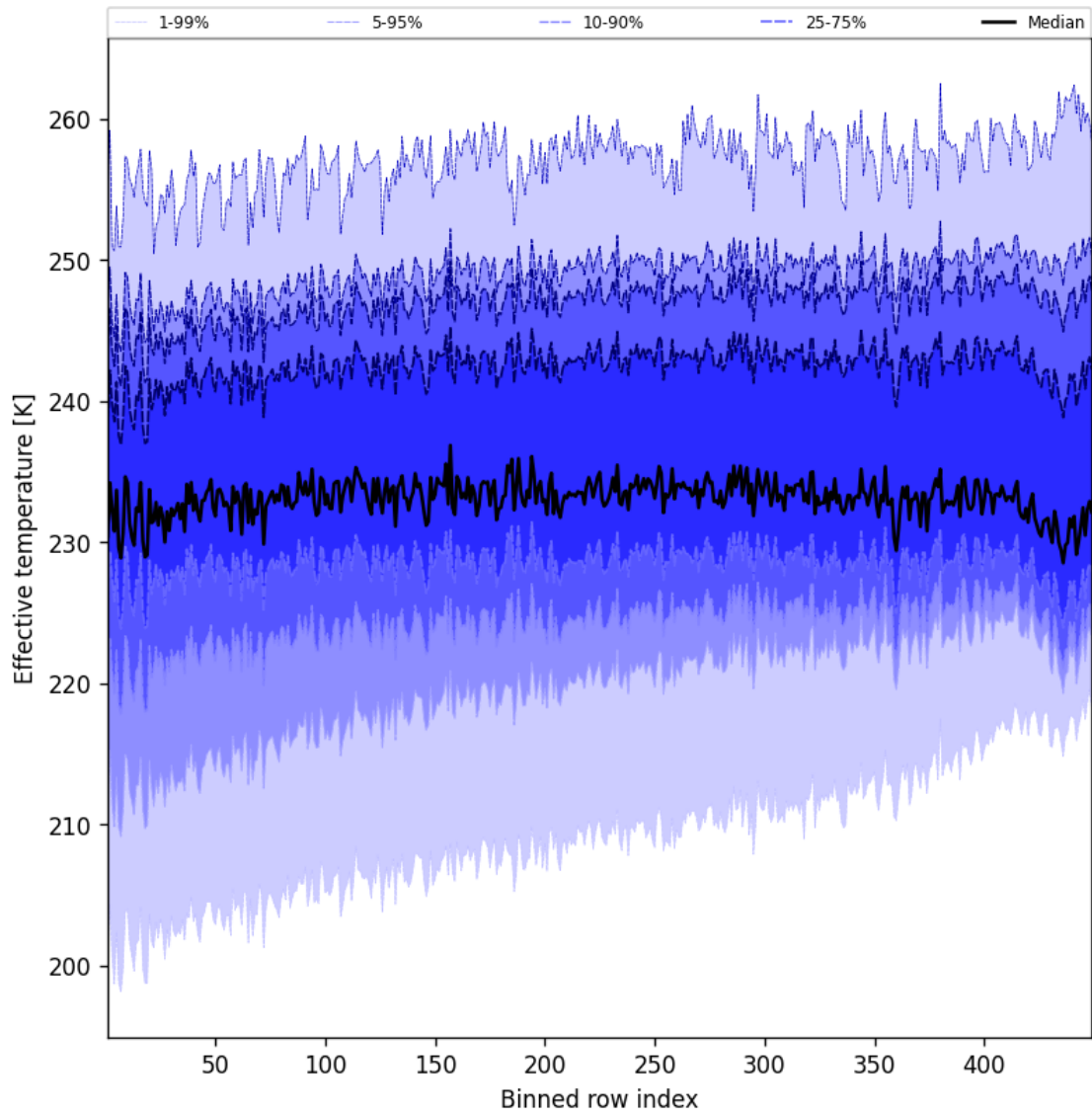
Figure 50: Along track statistics of “Effective temperature” for 2025-07-27 to 2025-07-27
