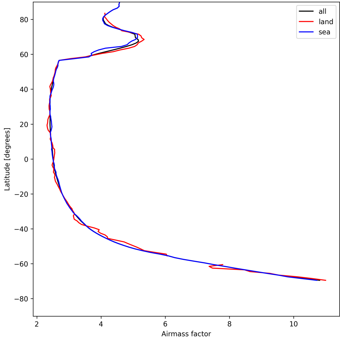
Figure 25: Zonal average of “Airmass factor” for 2025-07-27 to 2025-07-27.
