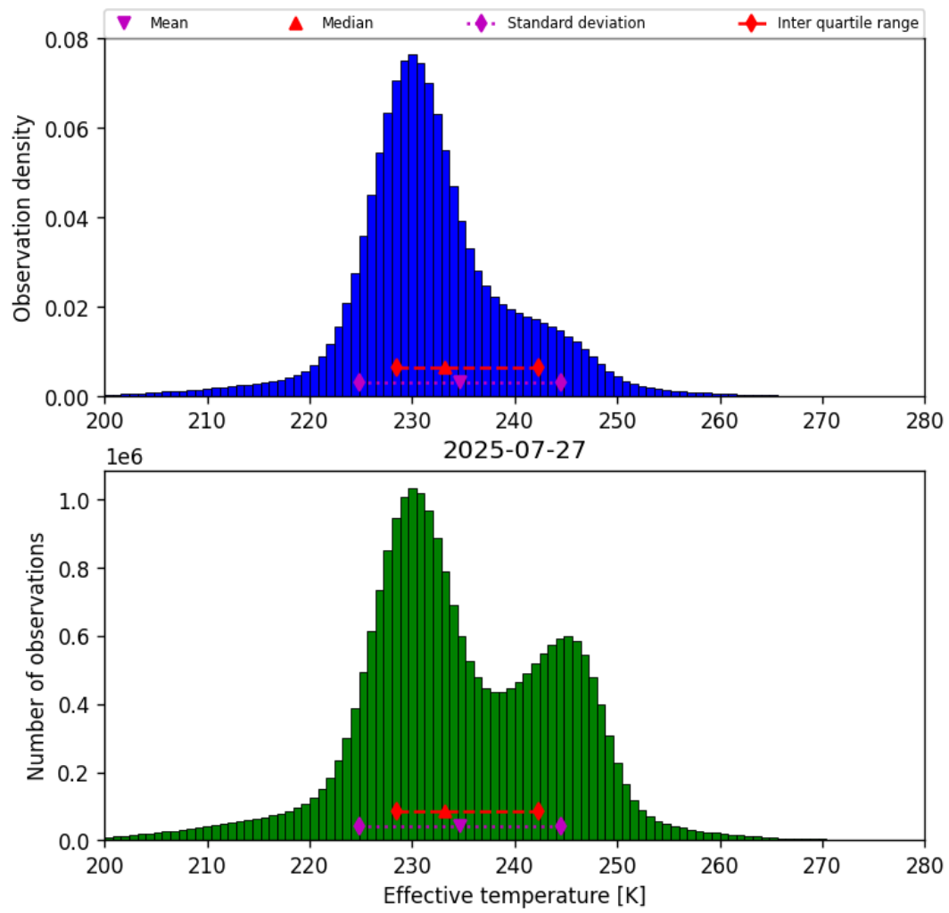
Figure 38: Histogram of “Effective temperature” for 2025-07-27 to 2025-07-27
