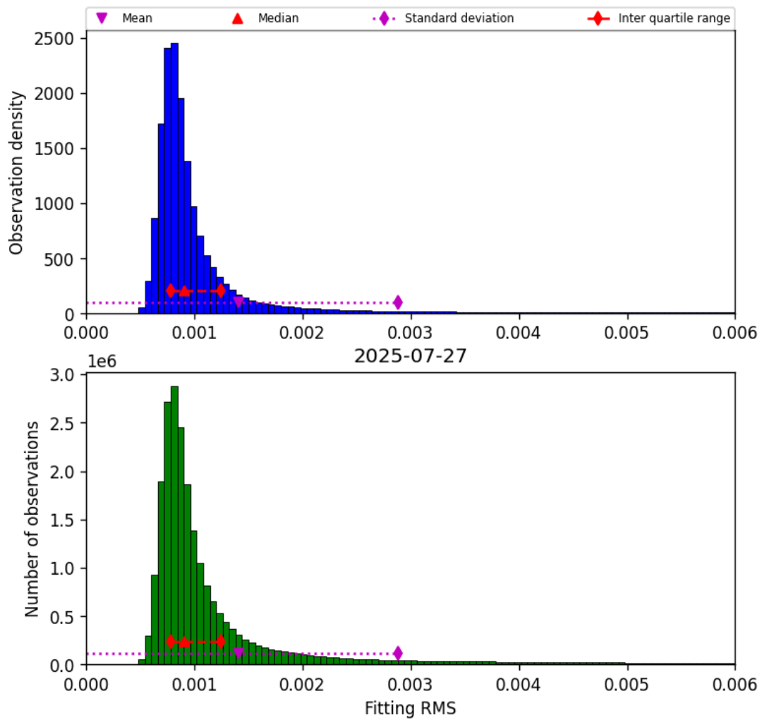
Figure 34: Histogram of “Fitting RMS” for 2025-07-27 to 2025-07-27
