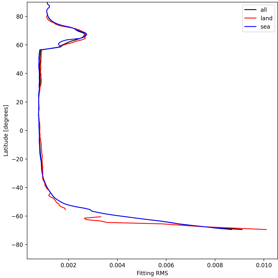
Figure 22: Zonal average of “Fitting RMS” for 2025-07-27 to 2025-07-27.
