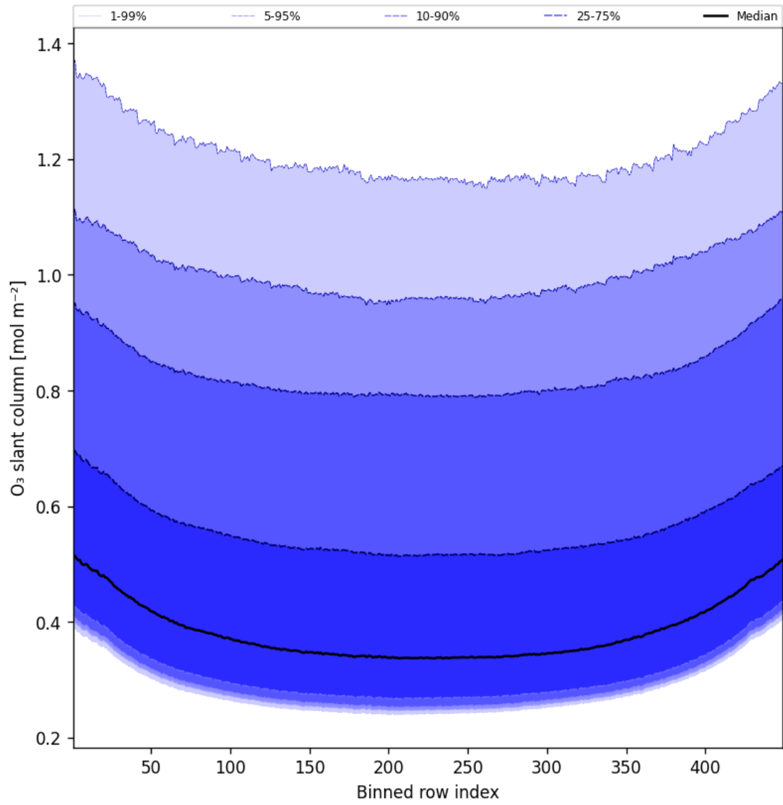
Figure 43: Along track statistics of “O 3 slant column” for 2025-07-27 to 2025-07-27
