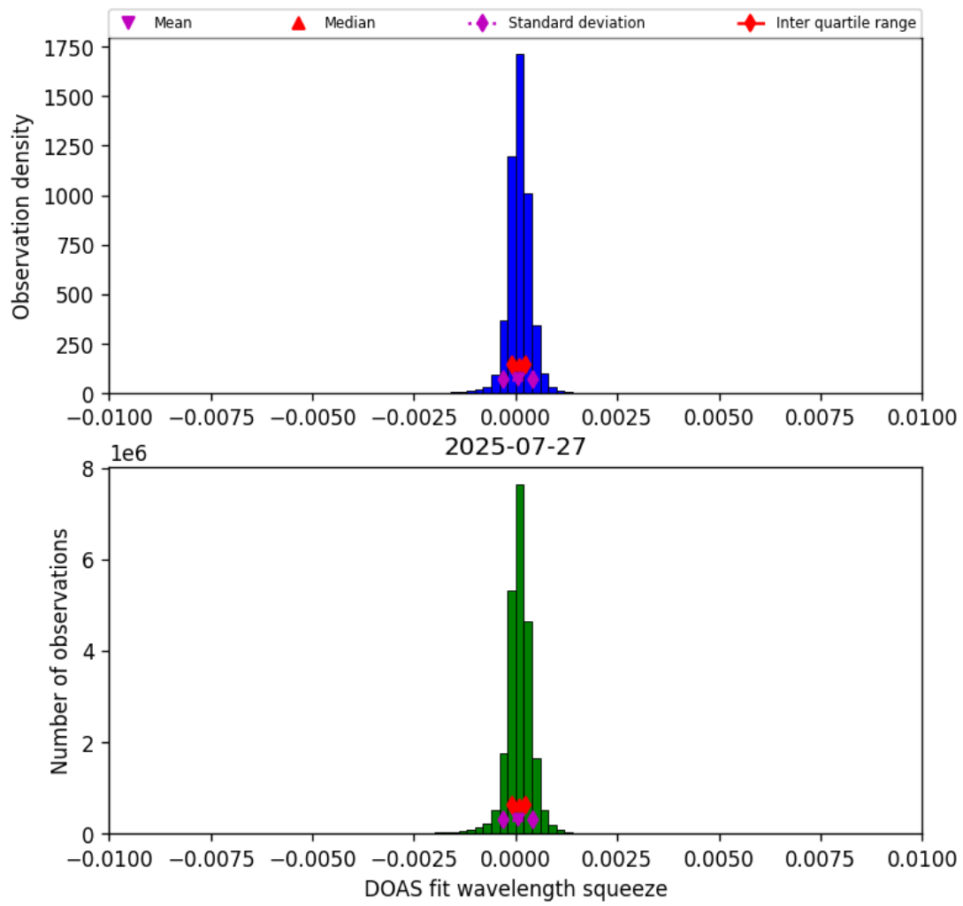
Figure 36: Histogram of “DOAS fit wavelength squeeze” for 2025-07-27 to 2025-07-27
