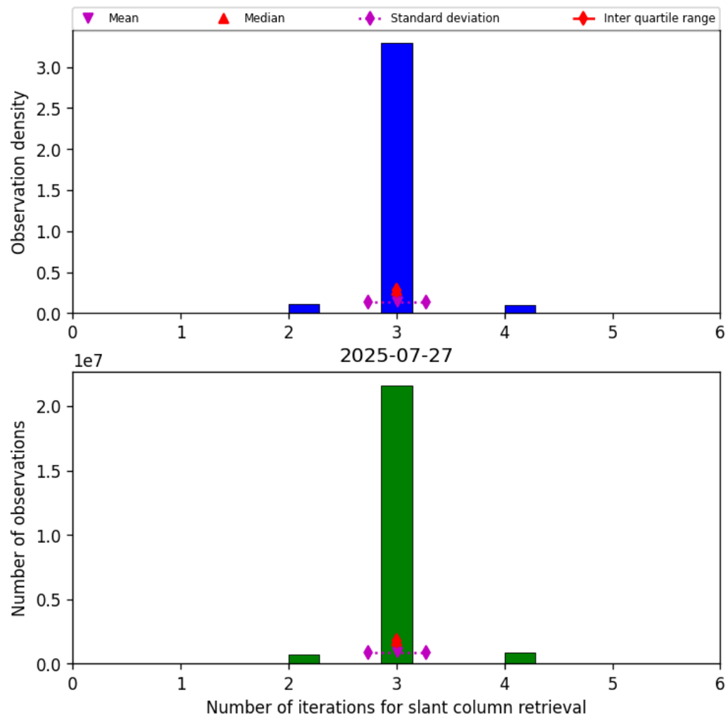
Figure 33: Histogram of “Number of iterations for slant column retrieval” for 2025-07-27 to 2025-07-27
