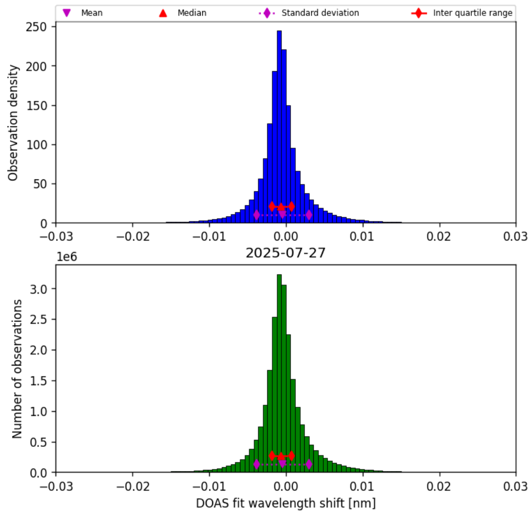
Figure 35: Histogram of “DOAS fit wavelength shift” for 2025-07-27 to 2025-07-27
