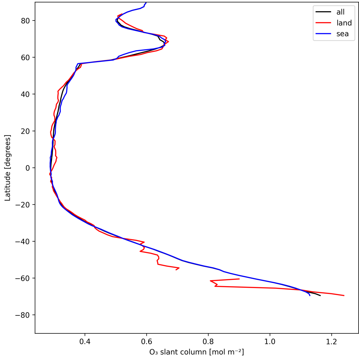
Figure 19: Zonal average of “O 3 slant column” for 2025-07-27 to 2025-07-27.
