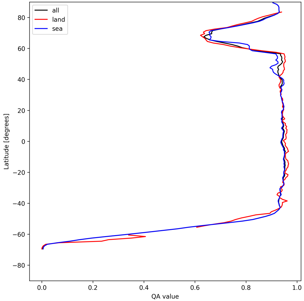
Figure 16: Zonal average of “QA value” for 2025-07-27 to 2025-07-27.
