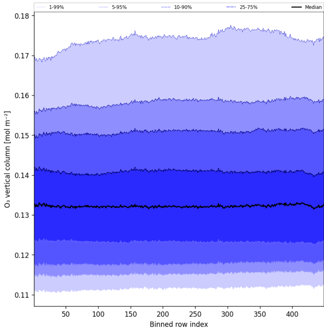
Figure 41: Along track statistics of “O 3 vertical column” for 2025-07-27 to 2025-07-27
