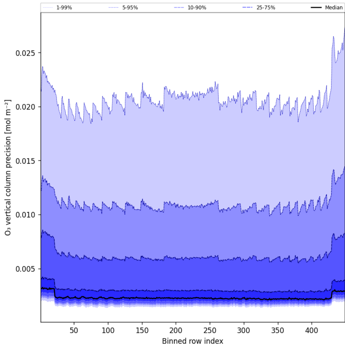
Figure 42: Along track statistics of “O 3 vertical column precision” for 2025-07-27 to 2025-07-27
