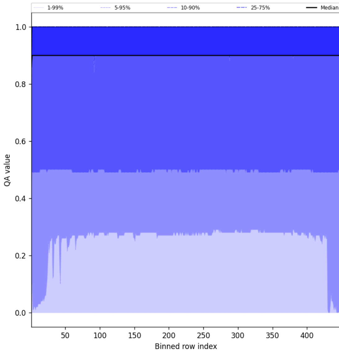
Figure 40: Along track statistics of “QA value” for 2025-07-27 to 2025-07-27
