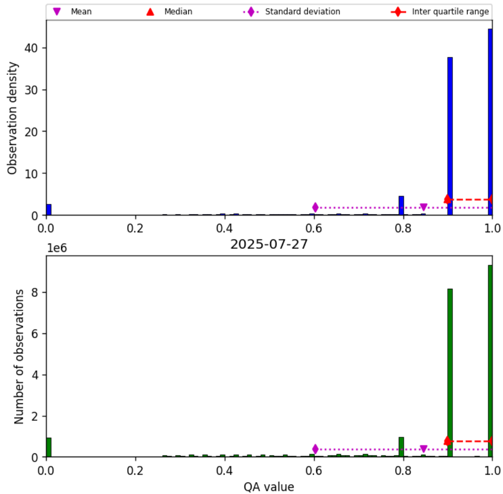
Figure 28: Histogram of “QA value” for 2025-07-27 to 2025-07-27
