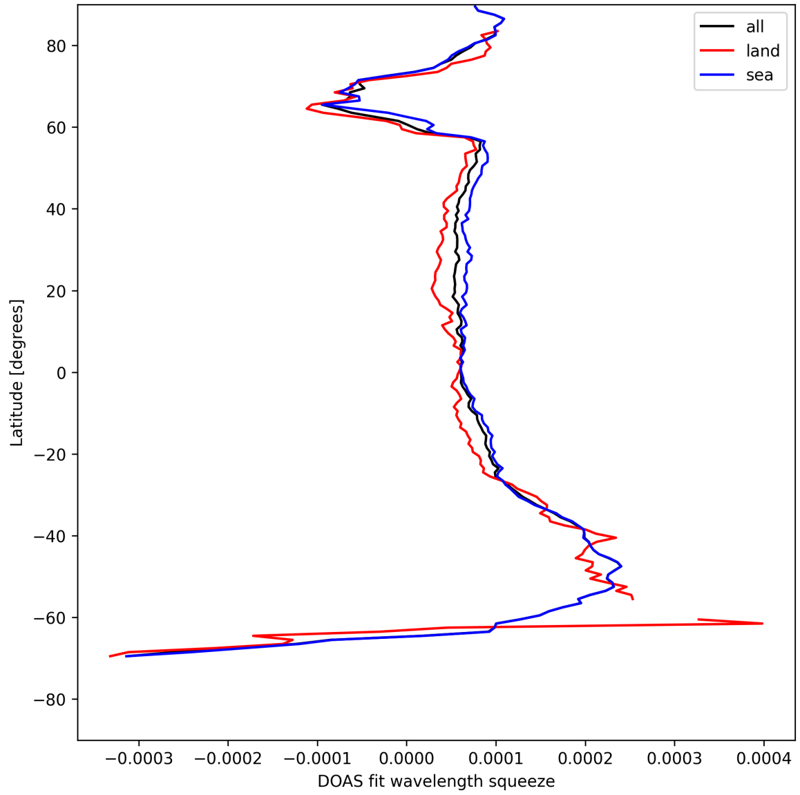
Figure 24: Zonal average of “DOAS fit wavelength squeeze” for 2025-07-27 to 2025-07-27.
