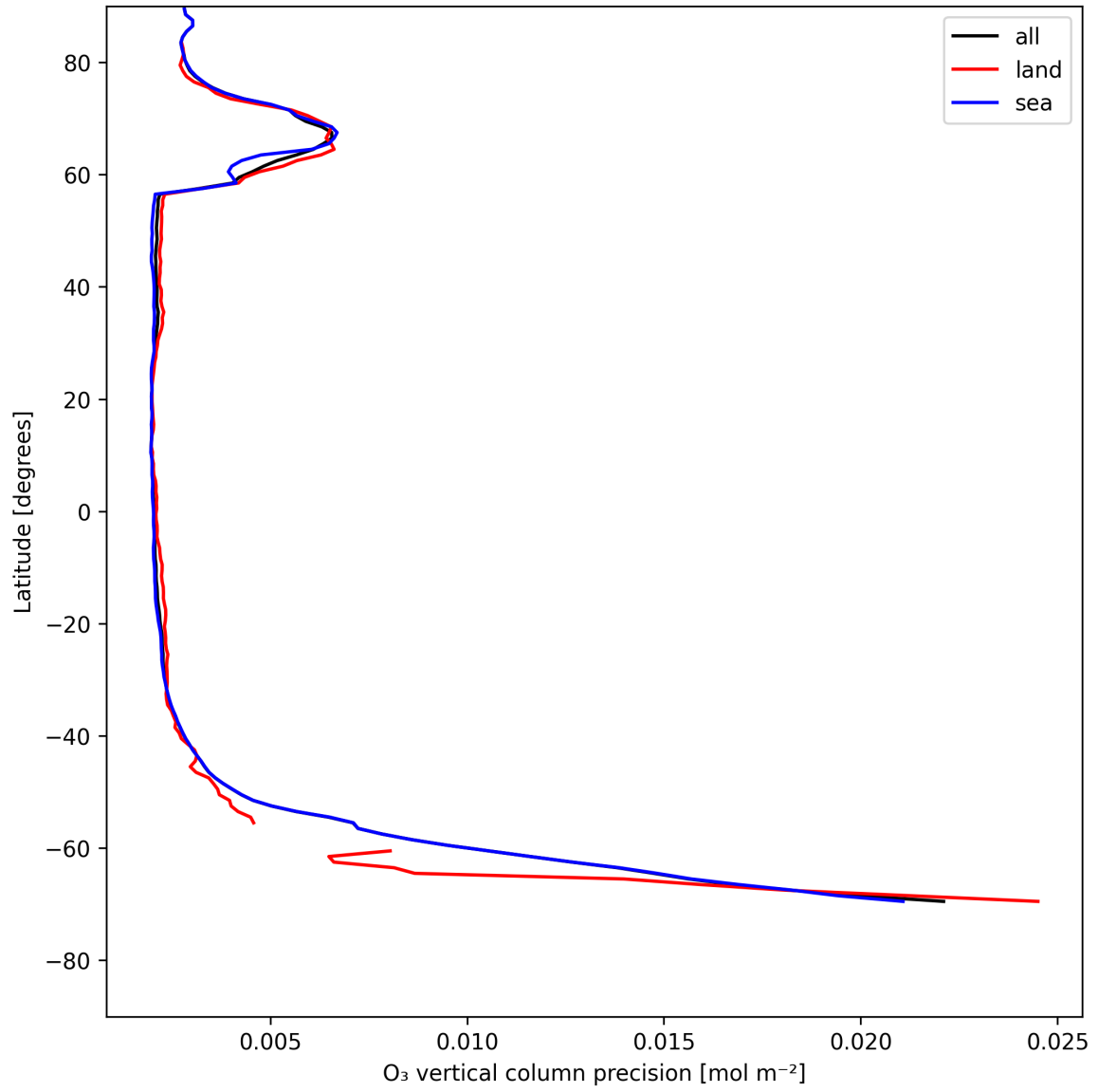
Figure 18: Zonal average of “O 3 vertical column precision” for 2025-07-27 to 2025-07-27.
