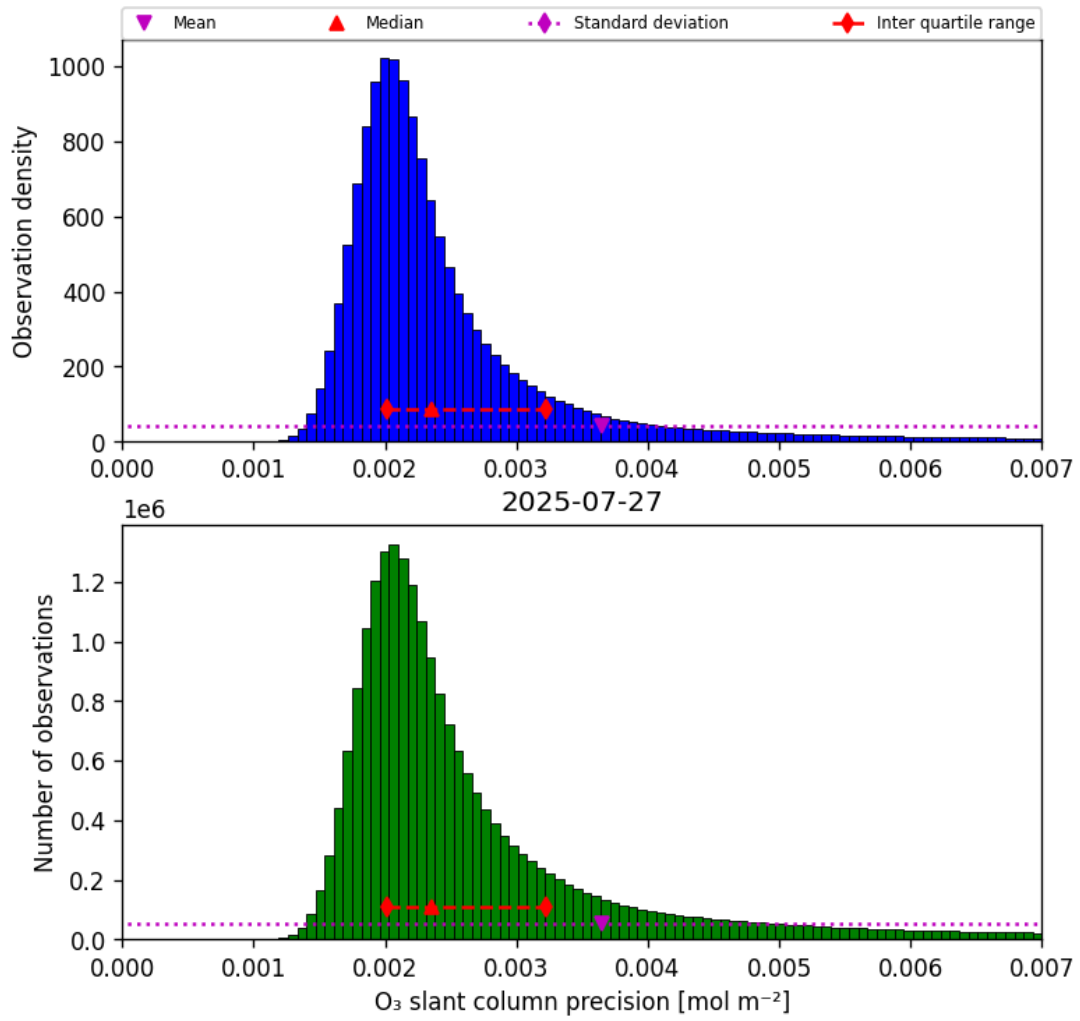
Figure 32: Histogram of “O 3 slant column precision” for 2025-07-27 to 2025-07-27
