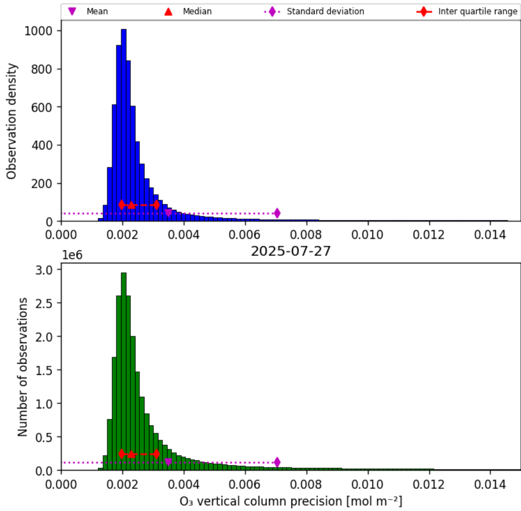
Figure 30: Histogram of “O 3 vertical column precision” for 2025-07-27 to 2025-07-27
