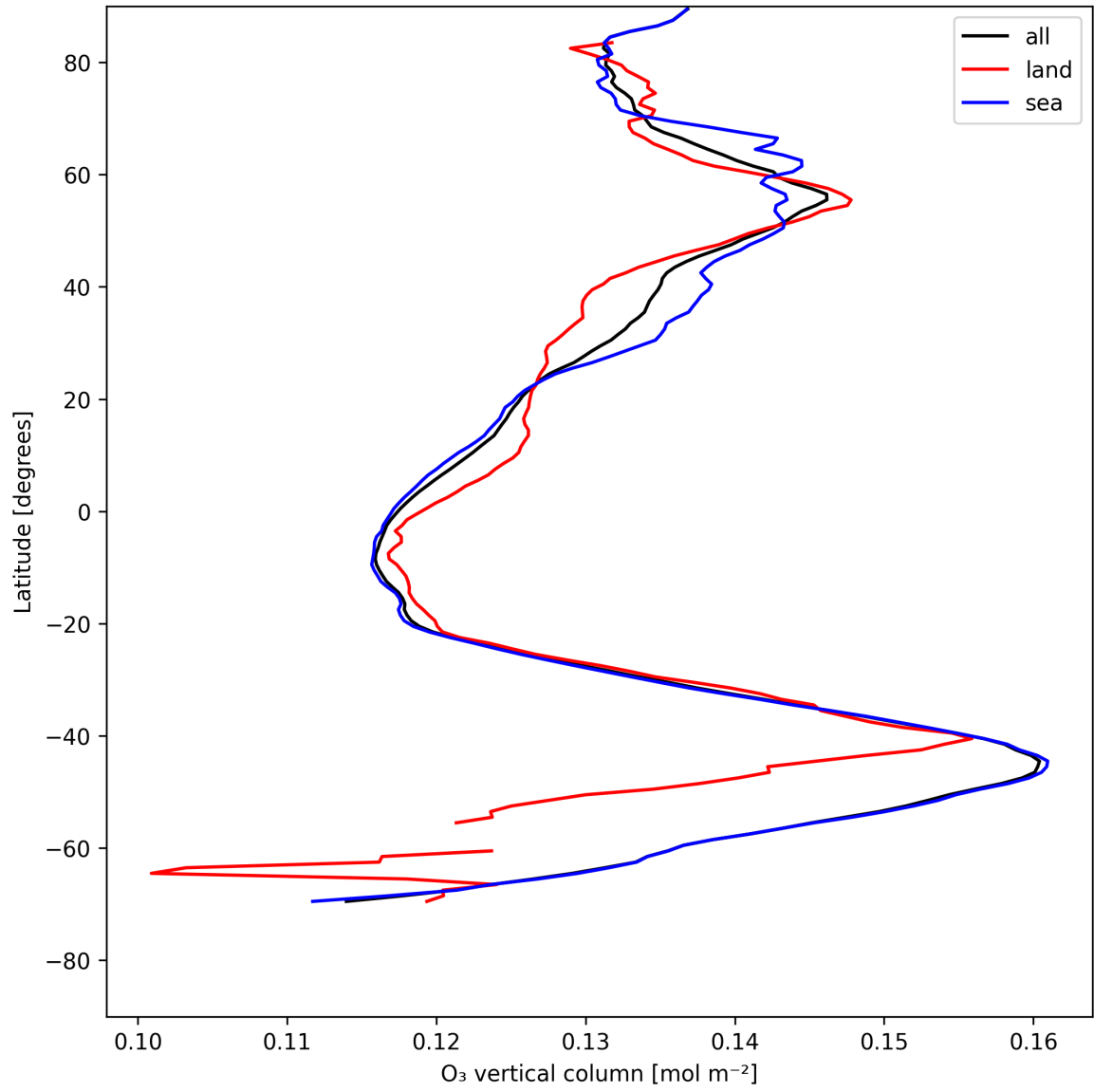
Figure 17: Zonal average of “O 3 vertical column” for 2025-07-27 to 2025-07-27.
